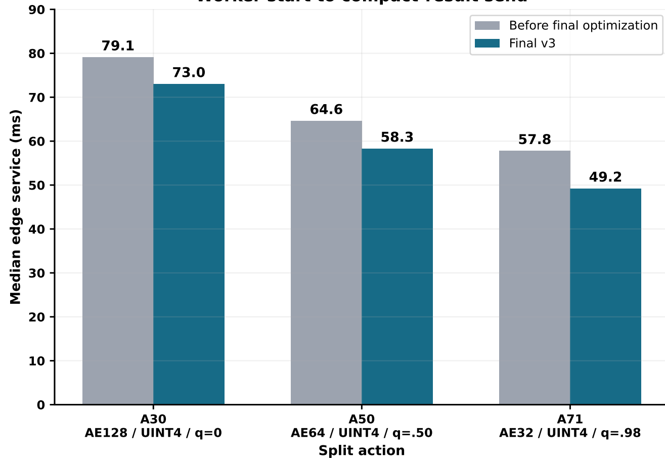
Worker start to compact-result send
