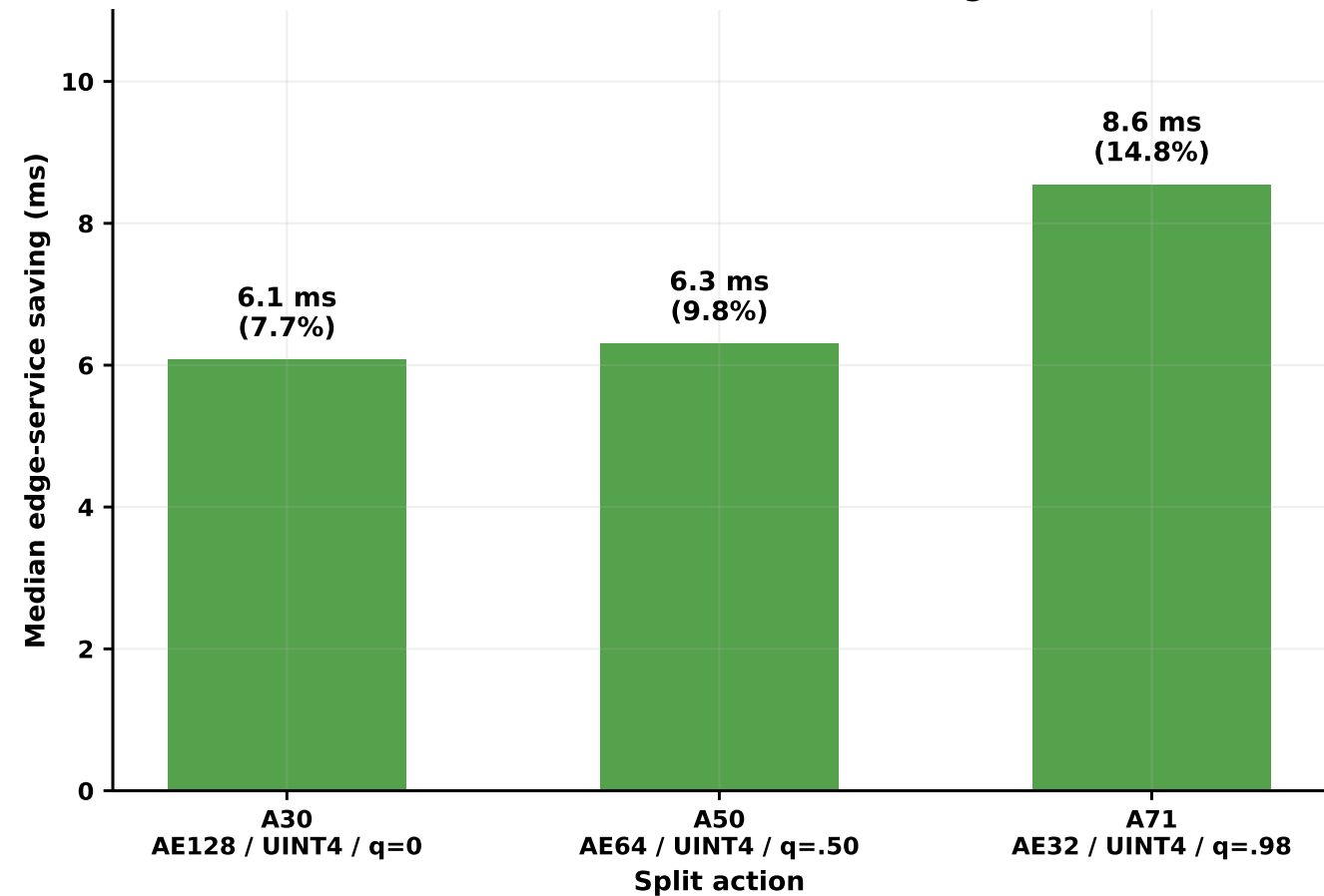
Measured incremental saving
