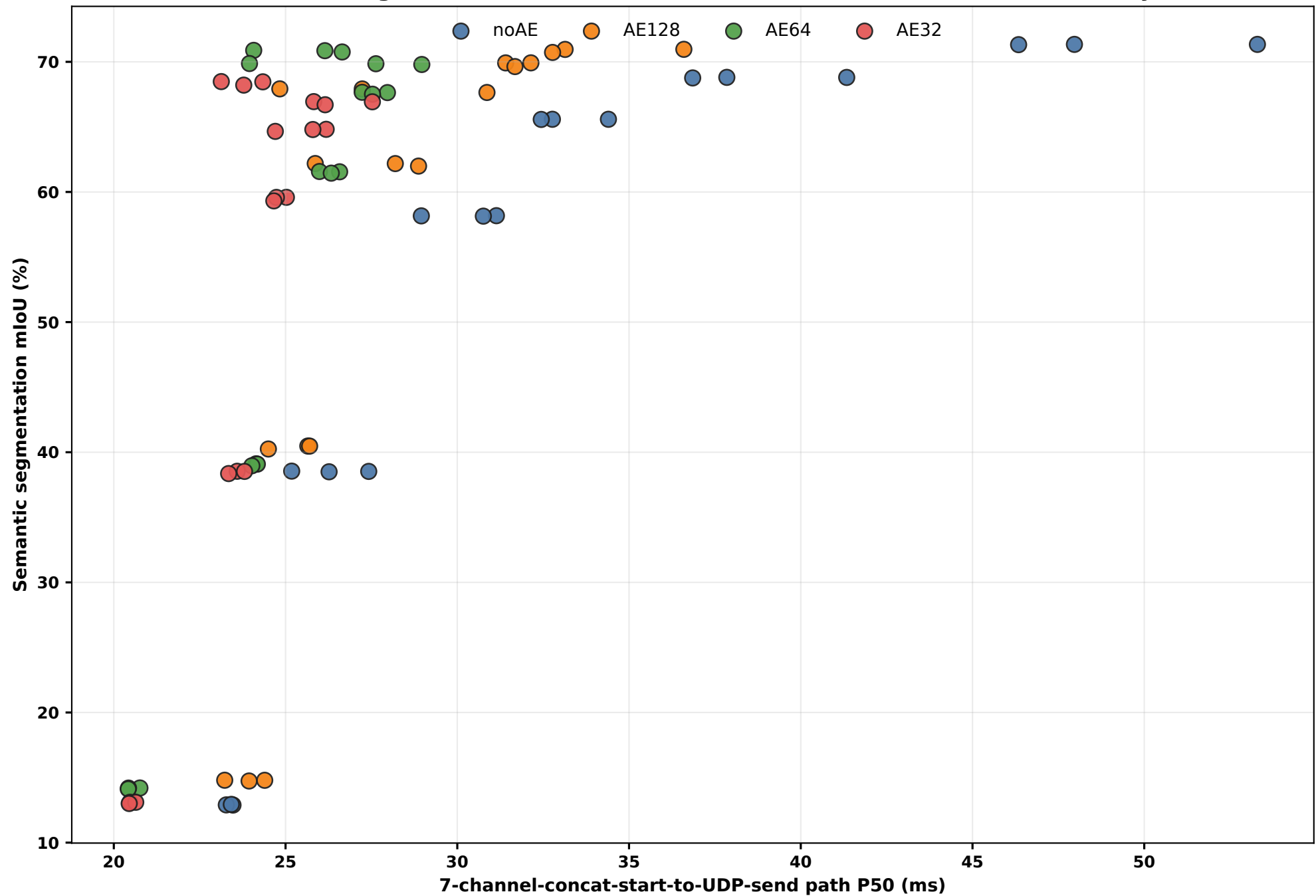
Semantic segmentation mIoU vs 7-channel-concat-start-to-UDP-send latency
