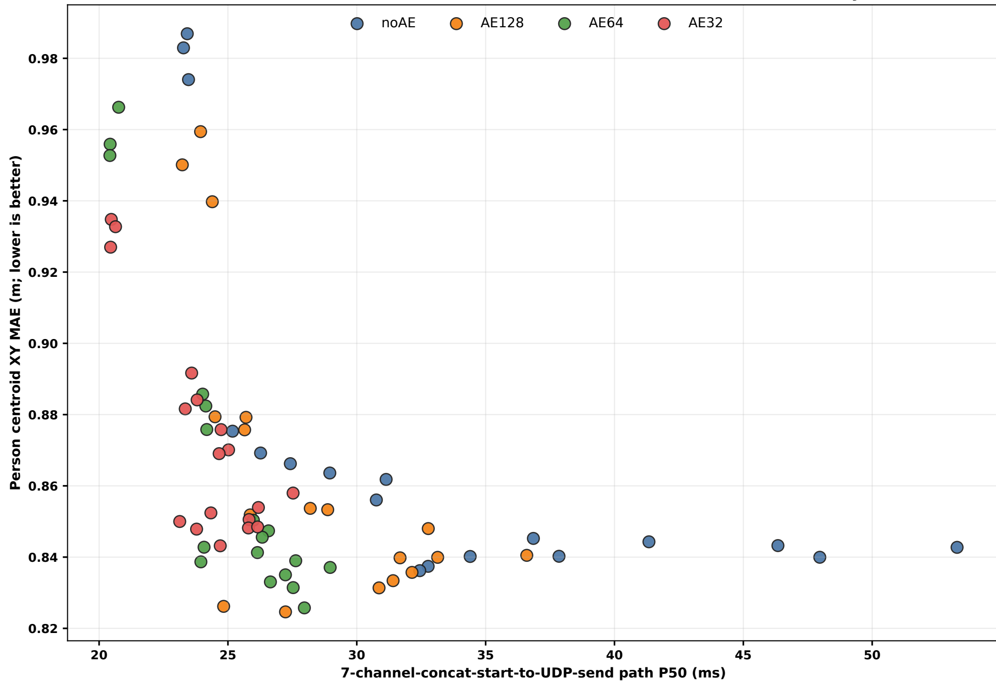
Person localization error vs 7-channel-concat-start-to-UDP-send latency
