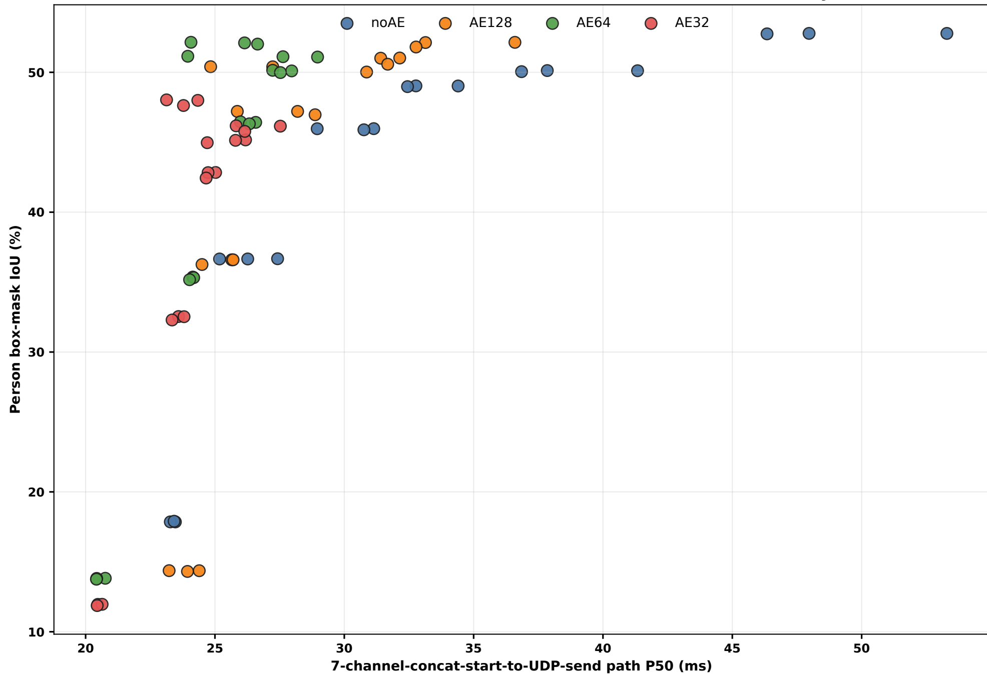
Person box-mask IoU vs 7-channel-concat-start-to-UDP-send latency
