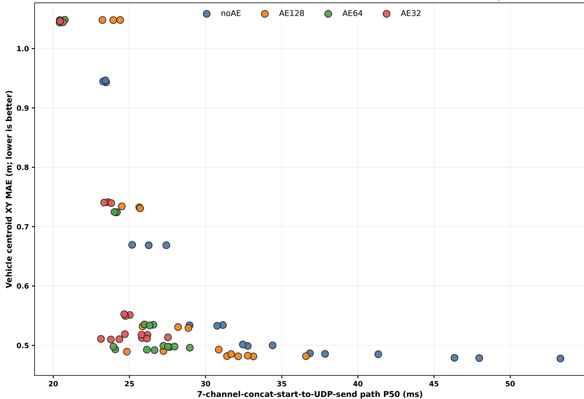
Vehicle localization error vs 7-channel-concat-start-to-UDP-send latency
