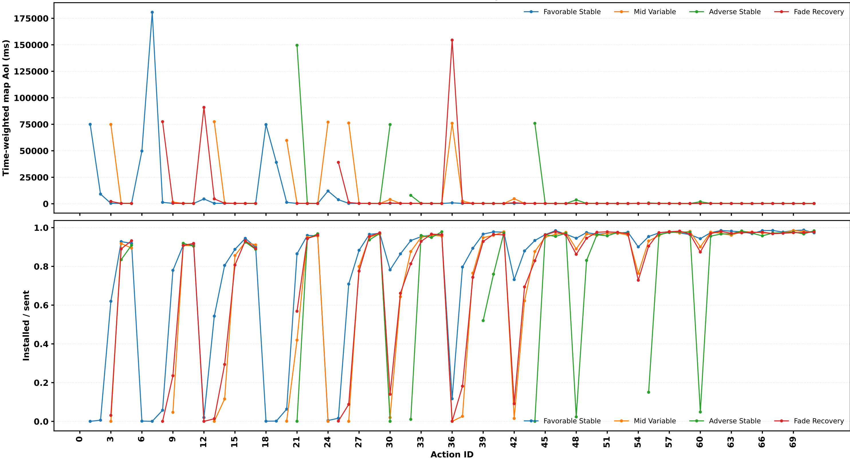
Matched action across all four network profiles (counterfactual)
