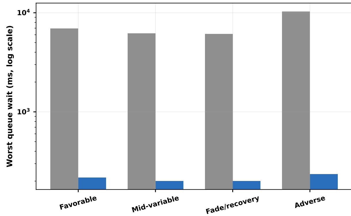
Final edge service: FIFO backlog versus strict latest-only
