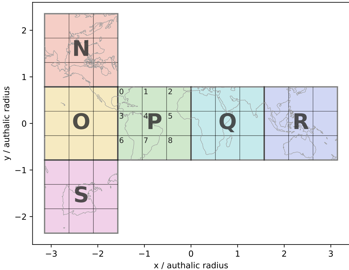
(0, 0)-rHEALPix planar grid: resolution 0 cells, resolution 1 sub-grid
