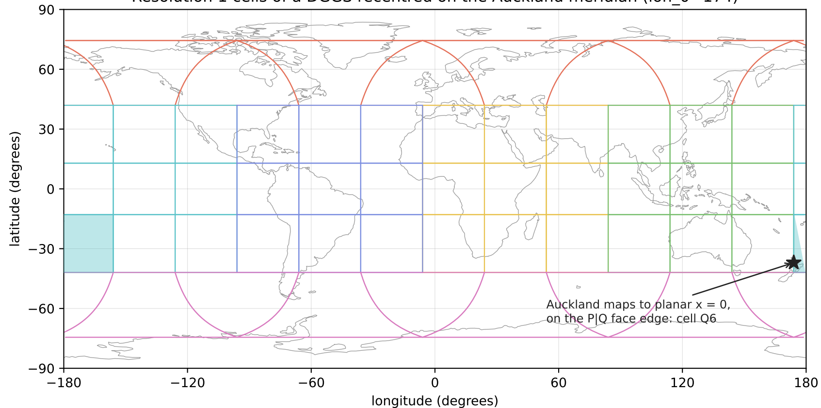
Resolution 1 cells of a DGGs recentred on the Auckland meridian (lon_0=174)
