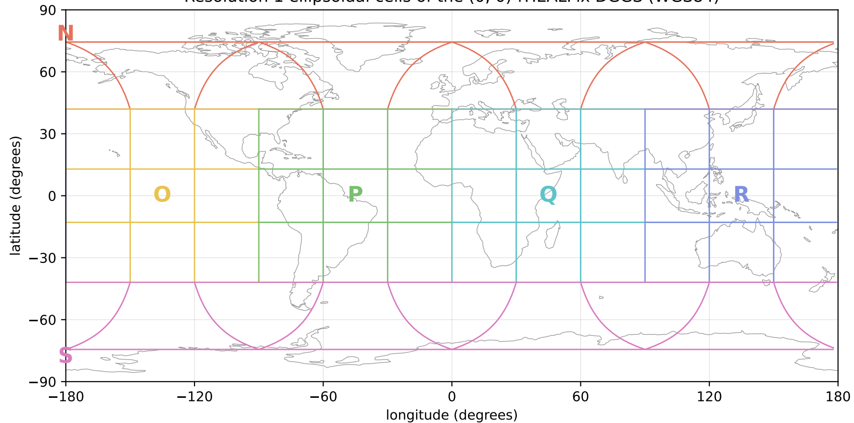
Resolution 1 ellipsoidal cells of the (0, 0)-rHEALPix DGGs (WGS84)
