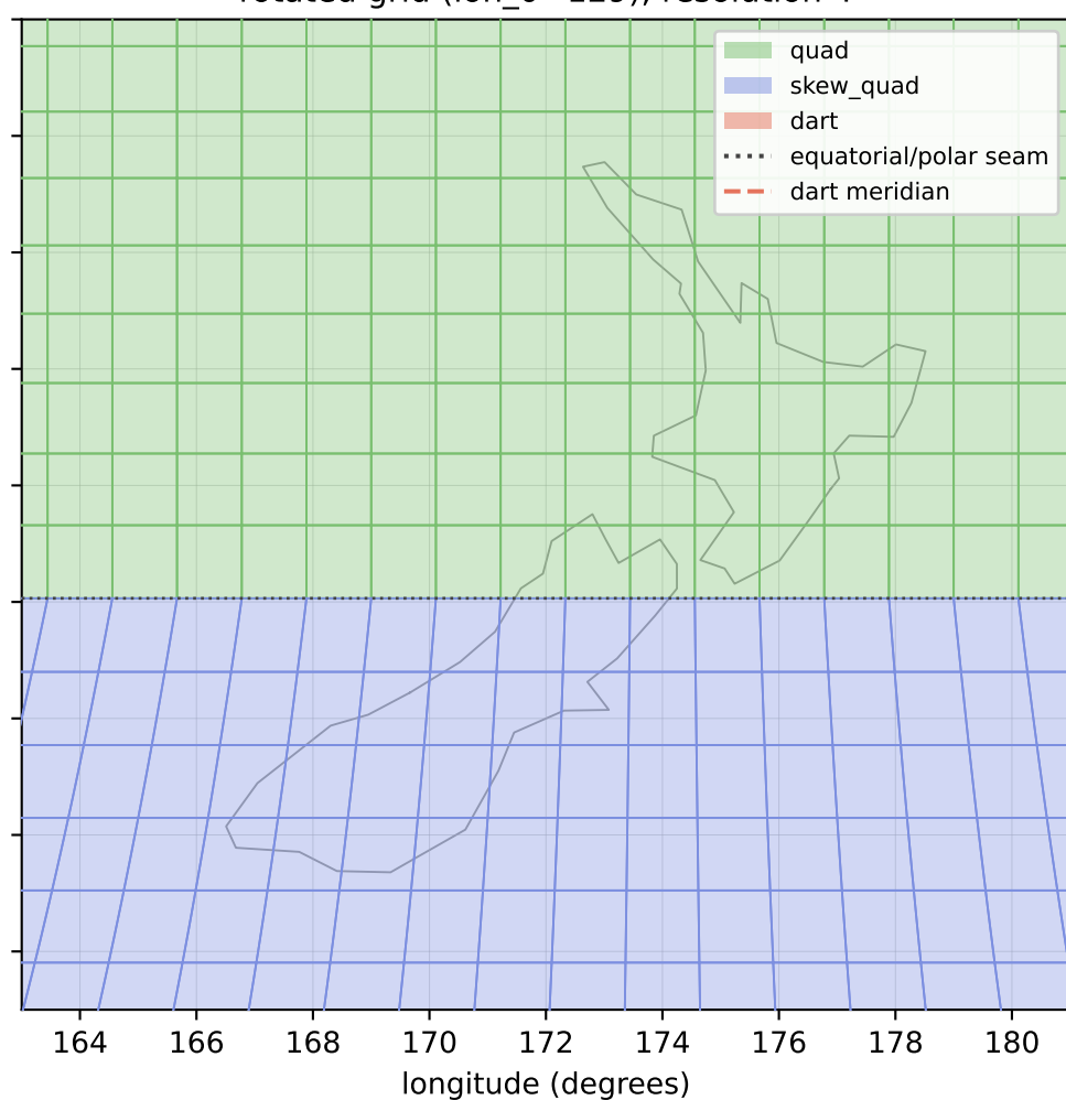
rotated grid (lon_0=129), resolution 4
