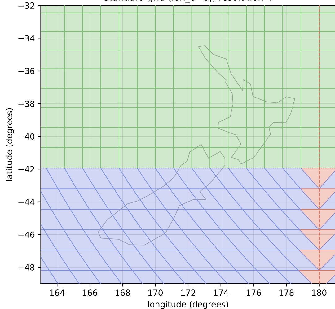
standard grid (lon_0=0), resolution 4
