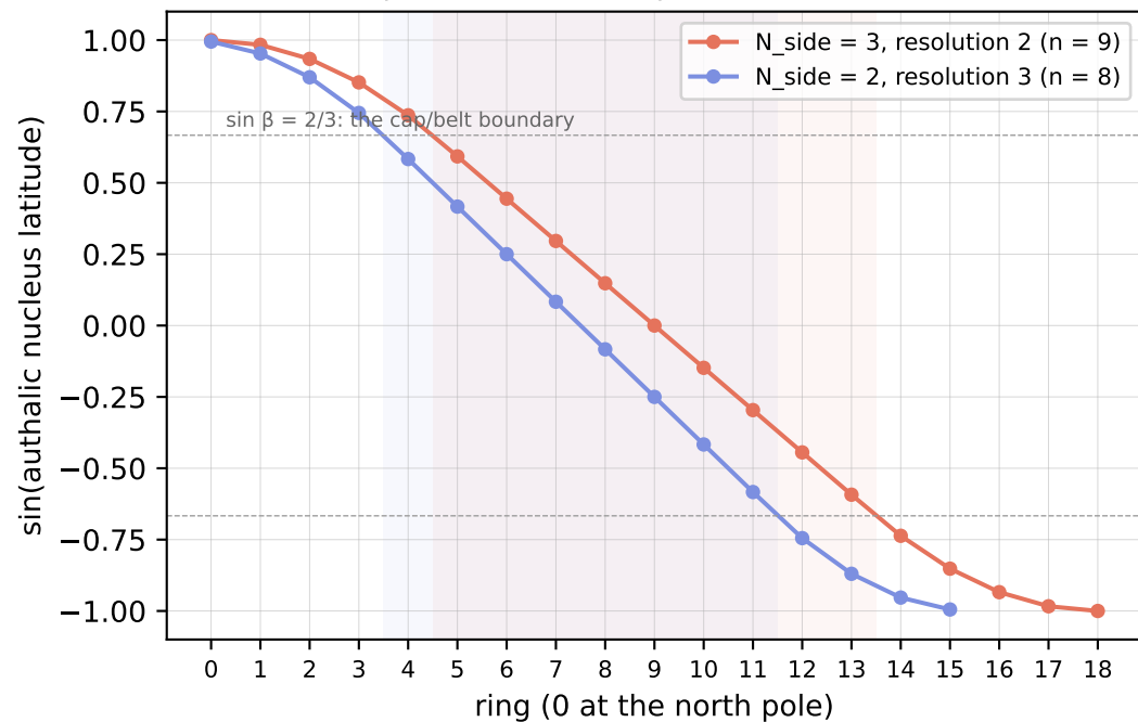
Equal-area rows: \sin \beta is linear in the belt
