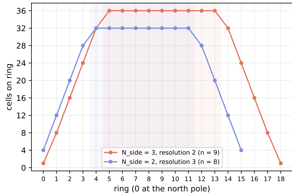
Population: 8m (odd n ) or 8m + 4 (even n ) in the caps, 4n in the belt
