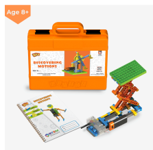
Discovering Motions
