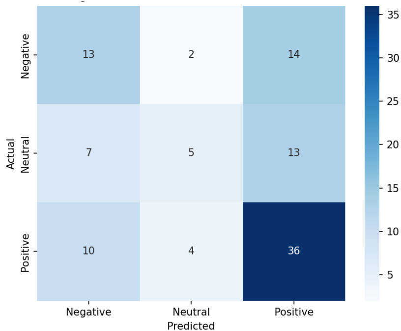
Figure 9: Random Forest (Default) Classification Report and Confusion Matrix.
