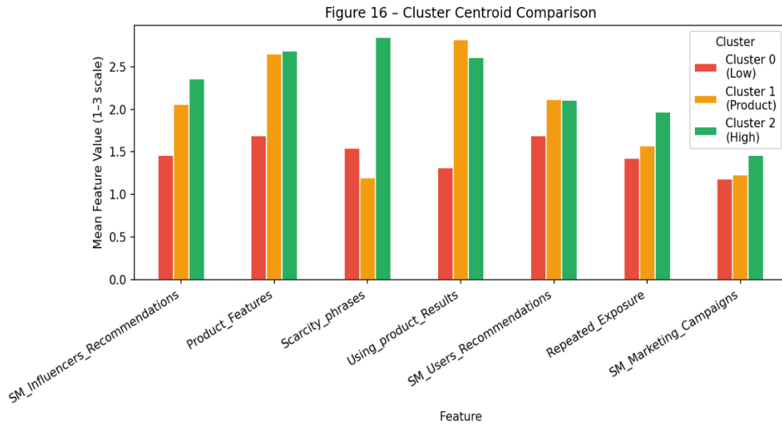
Figure 16 – K-Means Cluster Centroid Comparison Bar Chart
