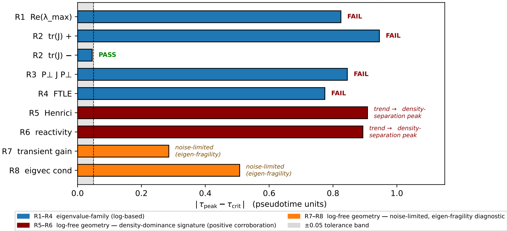
Eight independent readouts of the same drift field vs analytic \tau_{\text{crit}} \approx 0.004
