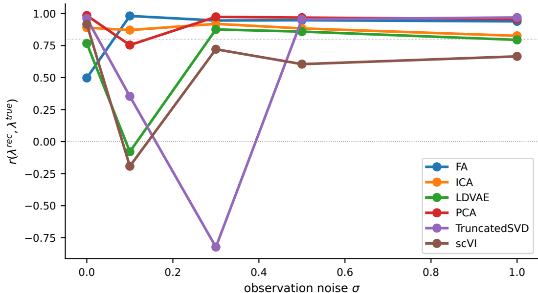
Sweep B — commitment system: \lambda -curve correlation vs noise (oracle pseudotime)
