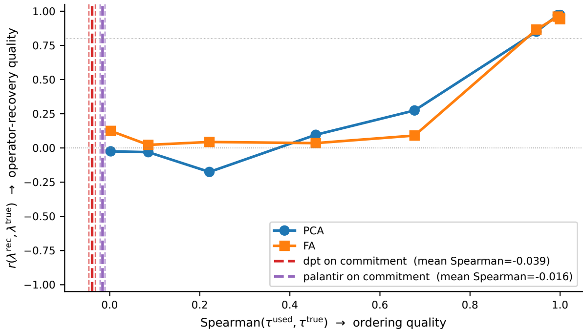
Cause A vs B diagnostic on commitment ( \sigma=0.3 )
