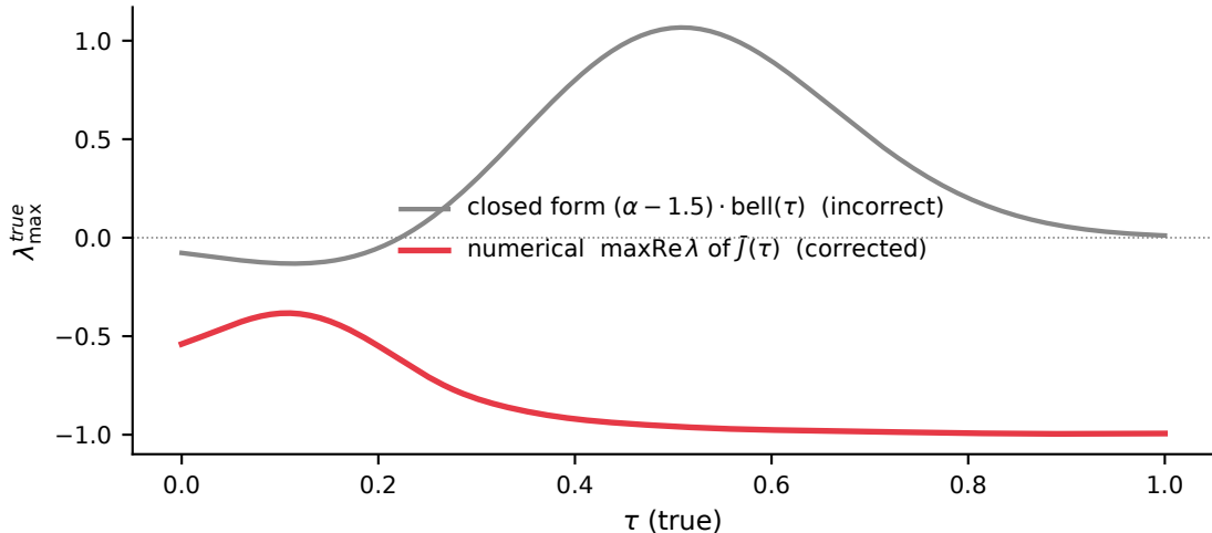
Bifurcation — closed-form vs numerical ground truth
