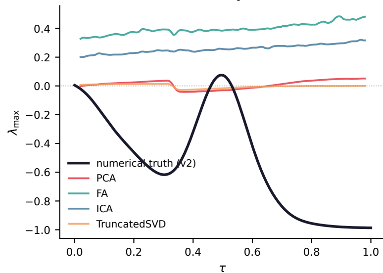
b recovered \lambda (oracle pt, linear embeddings)
