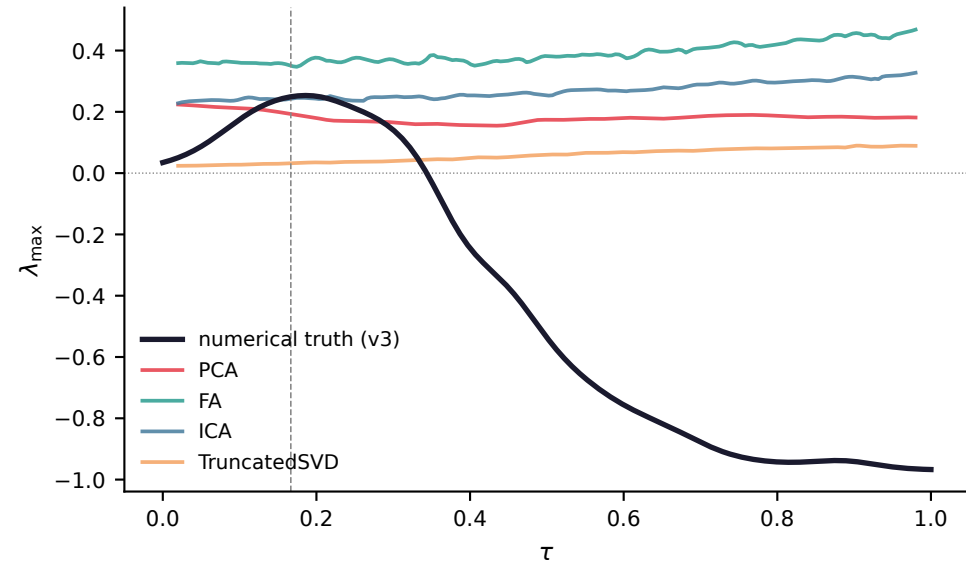
a recovered \lambda vs v3 truth (oracle \times linear)
