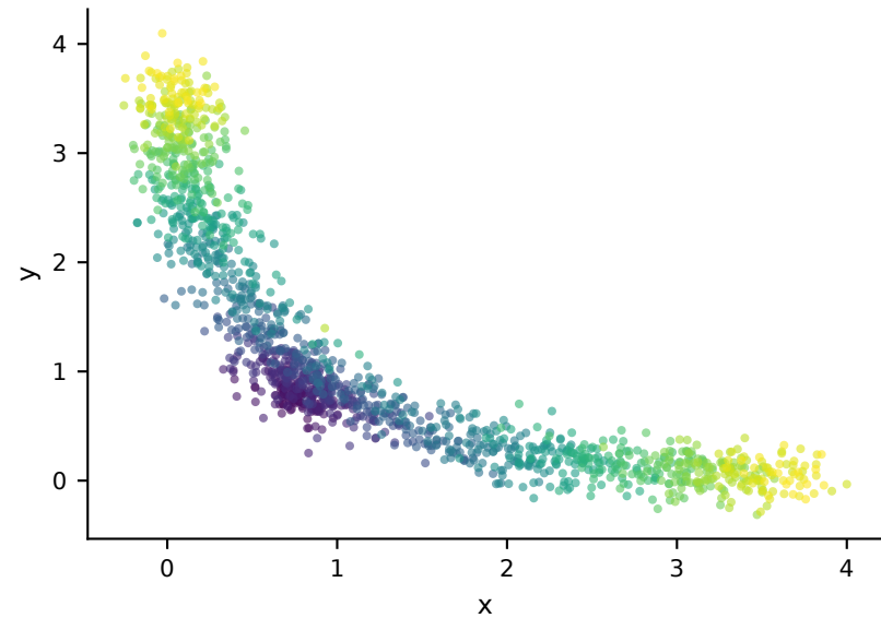
c v3 SDE-integrated transit
