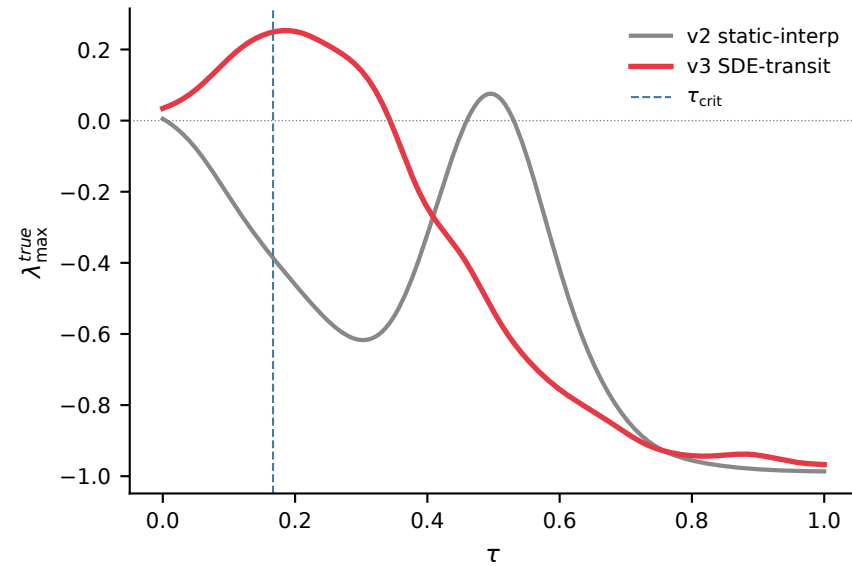
a ground-truth \lambda(\tau) — v2 vs v3
