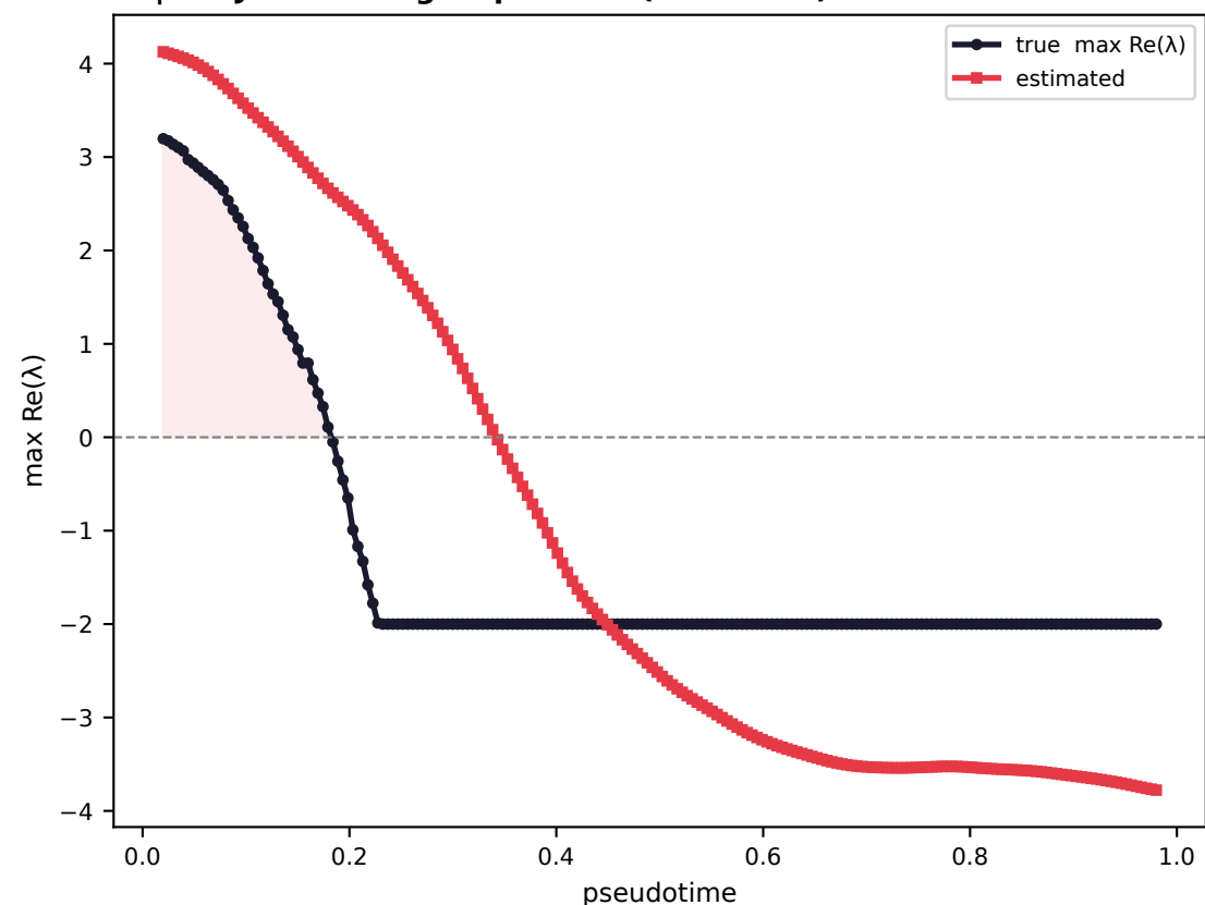
d | S4 bridge transport ( W_2=0.07 vs baseline 4.01)
