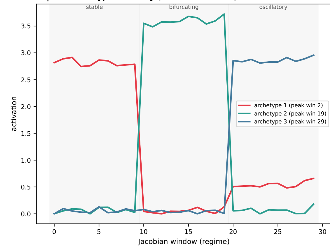
c | S3 archetype recovery (3 distinct = True)
