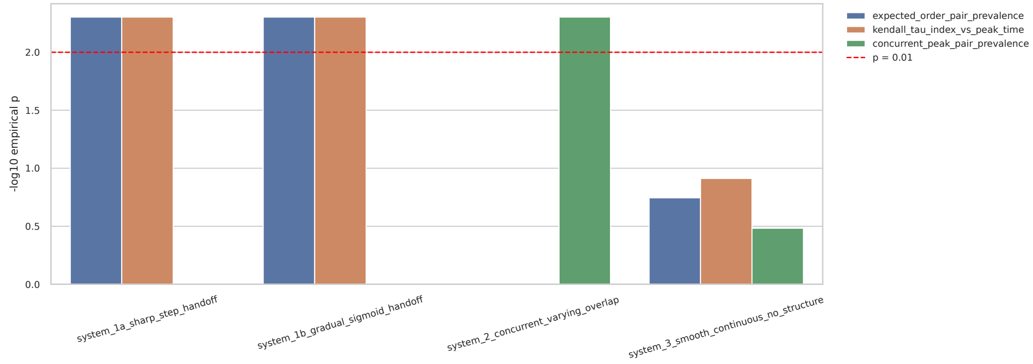
Synthetic peak-timing null-model p-values for target metrics
