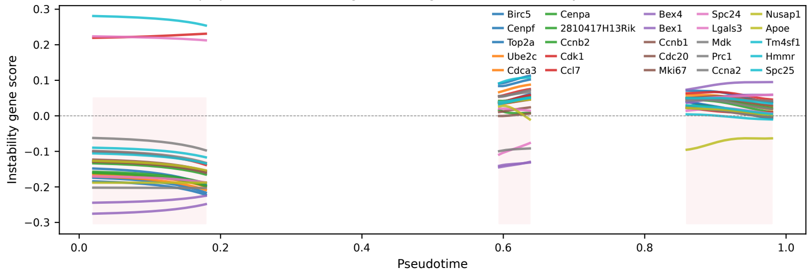
Top 25 instability-driving genes across pseudotime (score = projection onto max-eigenvalue eigenvector; shown only in sensitive windows)
