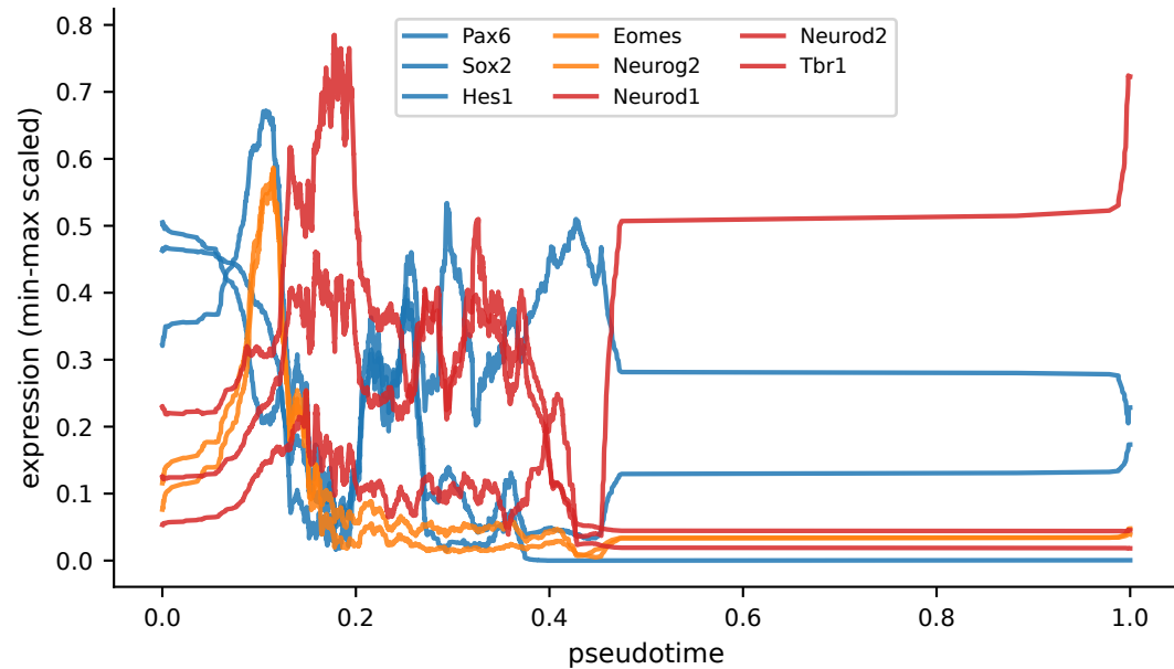
Uncorrected pseudotime
