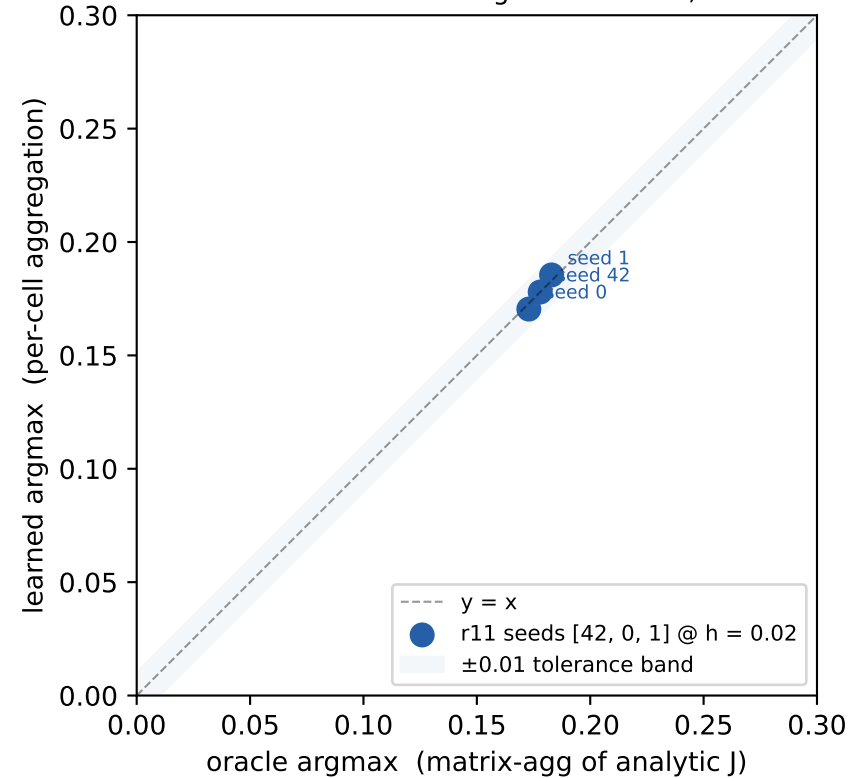
C. r11 learned-vs-oracle argmax: 3 seeds, max dev 0.003
