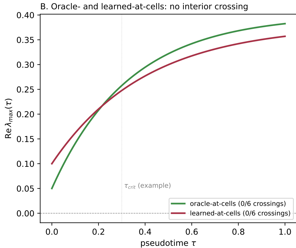
Fig 2 — Synthetic estimator fidelity + interior-crossing scorecard
