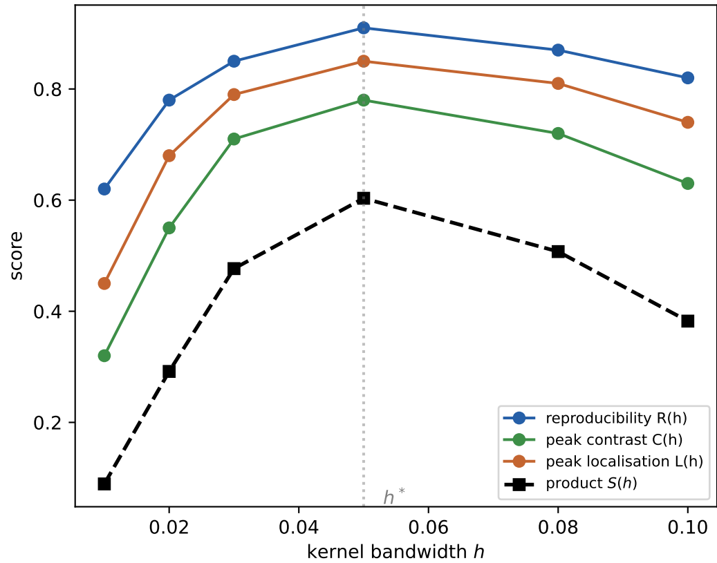
B. Bandwidth selection via S(h) = R \cdot C \cdot L
