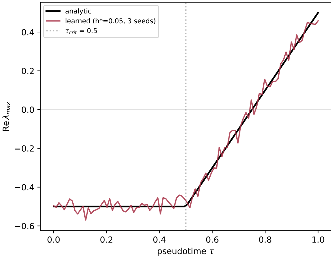
A. Eigenvalue crossing localises \tau_{crit} within one bandwidth
