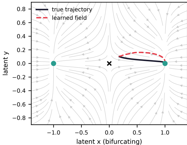
a S1 drift-field recovery (endpoint MSE = 0.0005) S2 Jacobian eigenspectrum (corr = 0.79)
