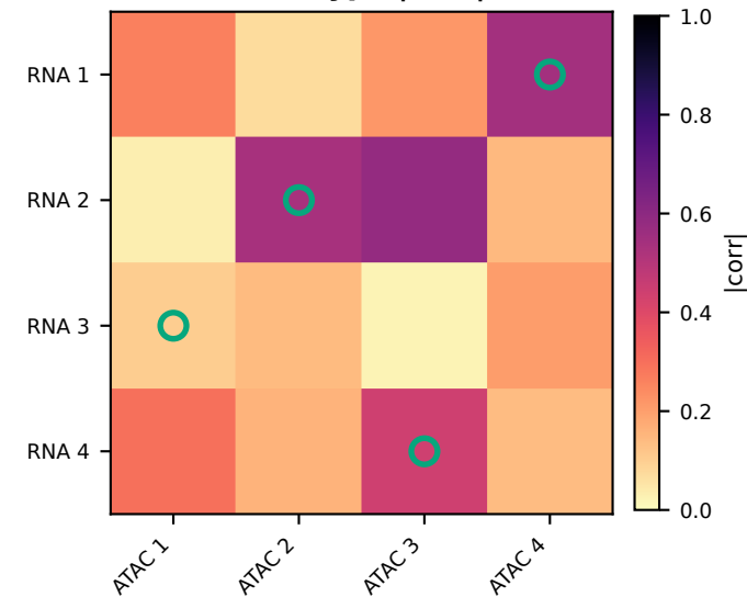
d M2 archetype |corr| (matched mean=0.41)
