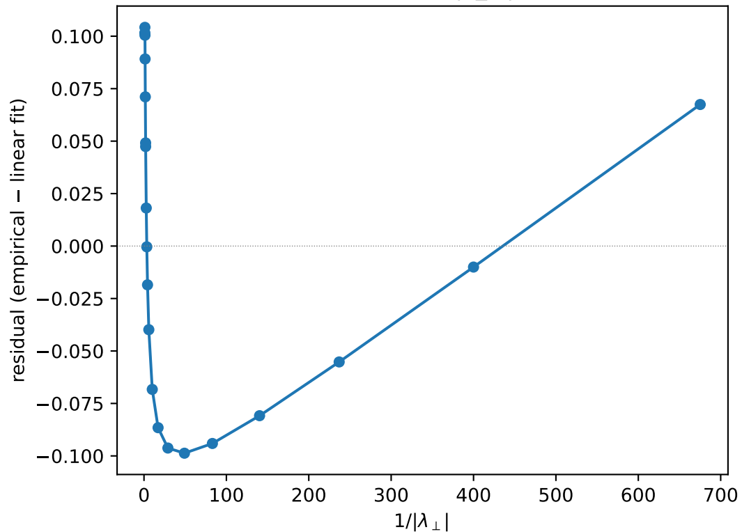
Residuals show where the 1/|\lambda_{\perp}| law breaks down
