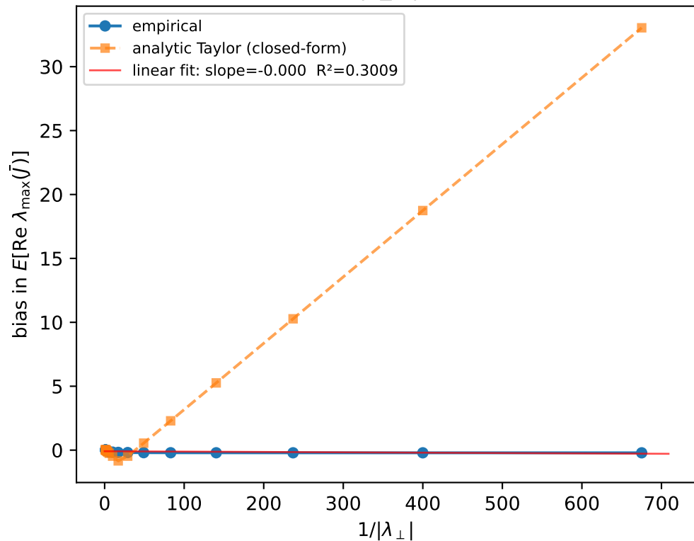
E (empirical): bias-vs- 1/|\lambda_{\perp}| from actual cell clouds
