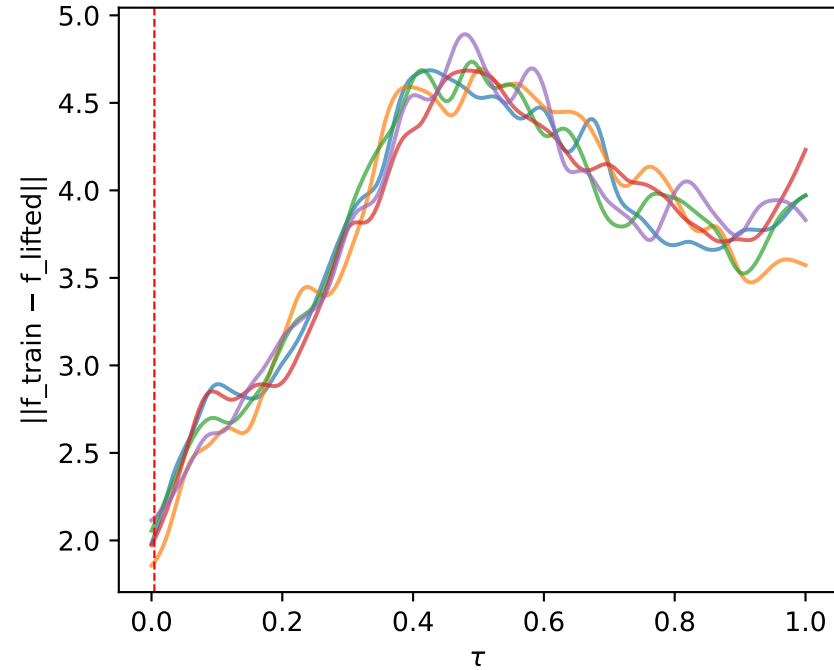
raw disagreement
