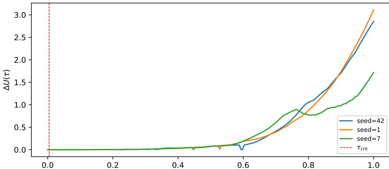
T6: Boltzmann-inverted barrier from KDE of w
