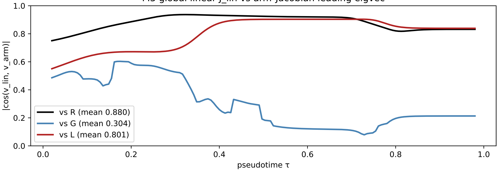
M3 global linear J_lin vs arm-Jacobian leading eigvec
