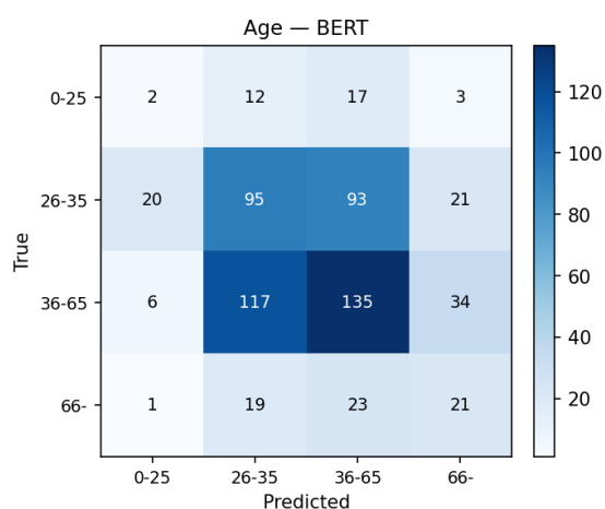
(a) BERT
