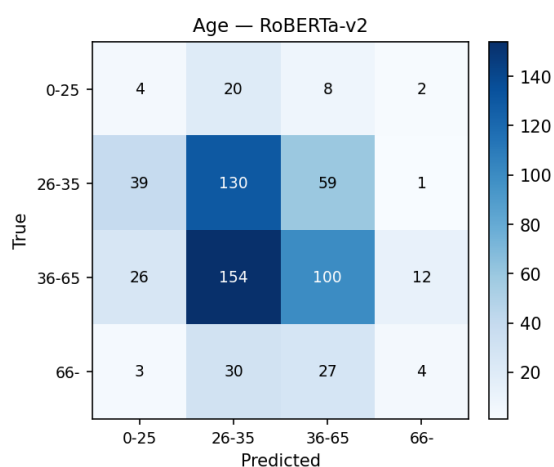
(c) RoBERTa
