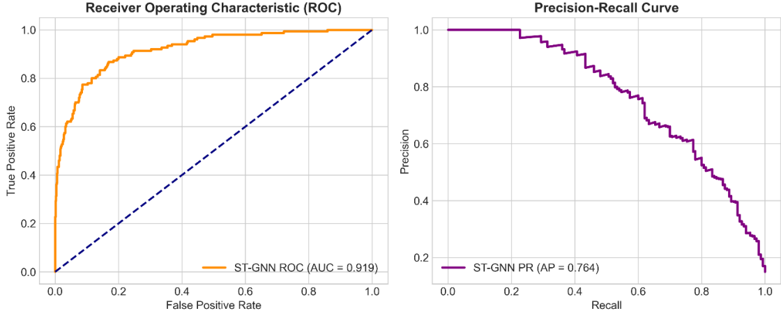
Figure 8: ROC and Precision-Recall curves for the threshold-based discrimination task. Left: Receiver Operating Characteristic curve. Right: Precision-Recall curve. Note: the curve-derived AUC/AP values plotted here should be regenerated from the exact same evaluation run used to produce Table 8 before final submission, to ensure a single, internally consistent set of reported numbers.
