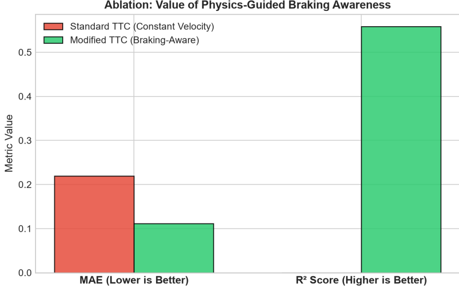
Figure 10: Ablation: value of physics-guided braking awareness. Comparison of Standard TTC (constant-velocity) versus Modified TTC (braking-aware) as the basis for the continuous risk target, evaluated by MAE and R^2 .
