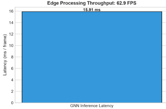
Figure 6: ST-GNN inference latency benchmark. Measured per-frame inference latency of the isolated ST-GNN forward pass, averaged over 100 consecutive iterations on the held-out test split.
