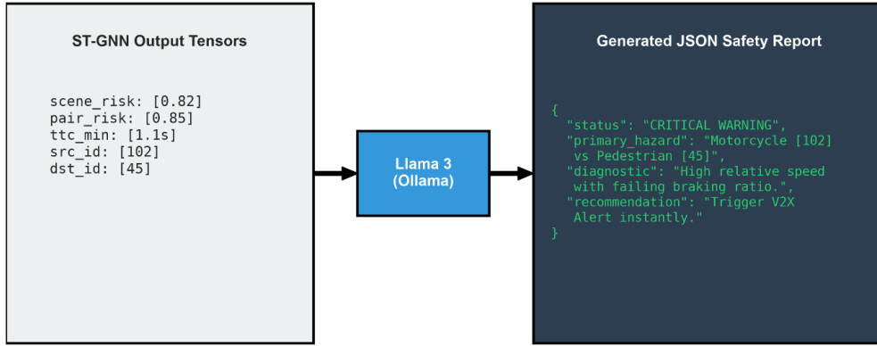
Figure 7: LLM grounding and reporting flow. ST-GNN output tensors (scene risk, pairwise risk, TTC_{min} , source/target agent IDs) feeding a structured telemetry payload into the locally deployed Llama-3 model (via Ollama), which produces a structured JSON safety report.
