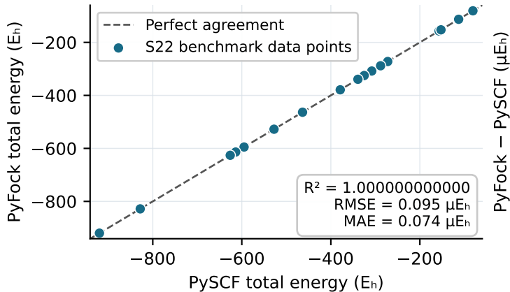
S22 energy parity (def2-SVP)
