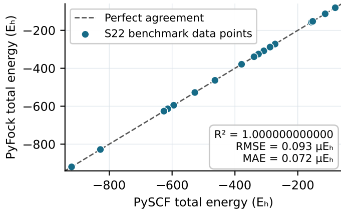
S22 energy parity (def2-SVP, SAO/spherical)
