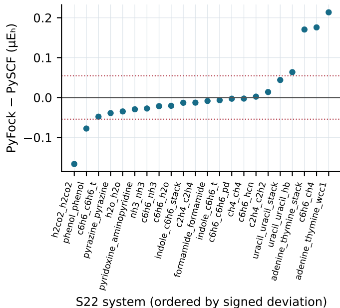
Signed numerical deviations
