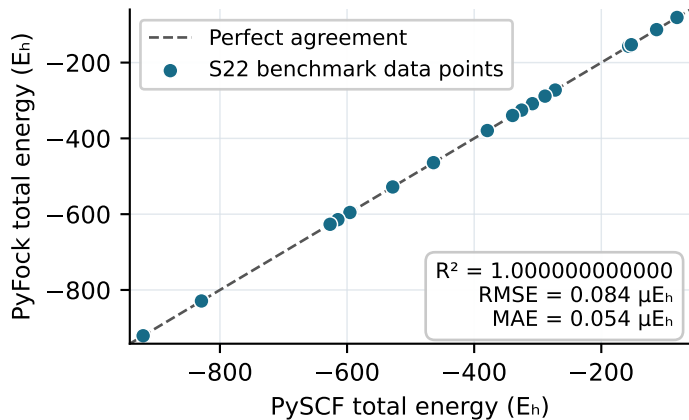
S22 energy parity (def2-TZVP)
