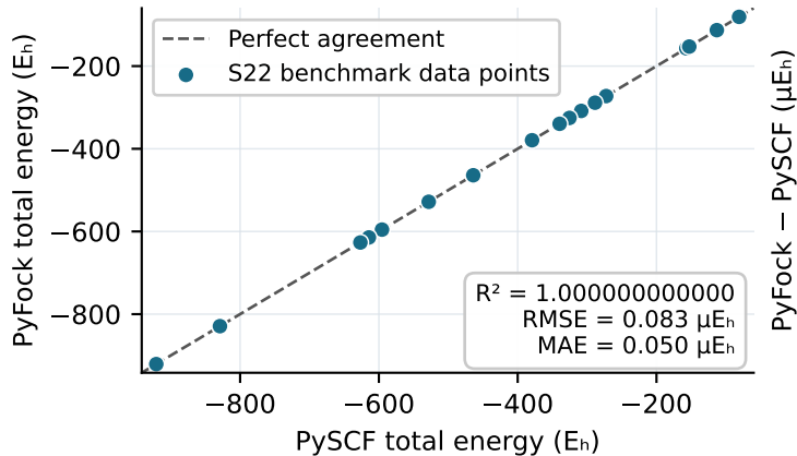
S22 energy parity (def2-TZVP, SAO/spherical)
