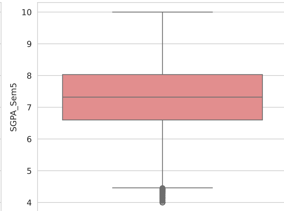
Boxplot of SGPA_Sem5
