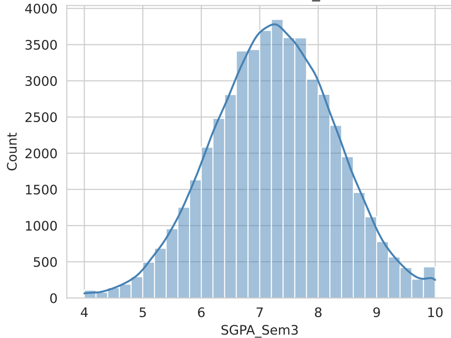
Distribution of SGPA_Sem3
