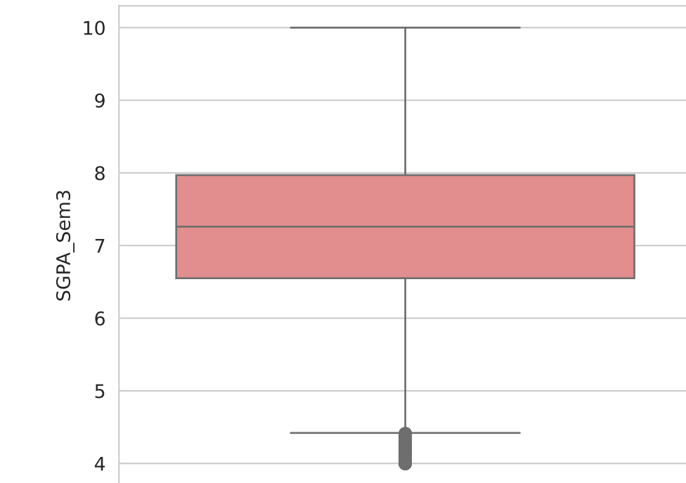
Boxplot of SGPA_Sem3
