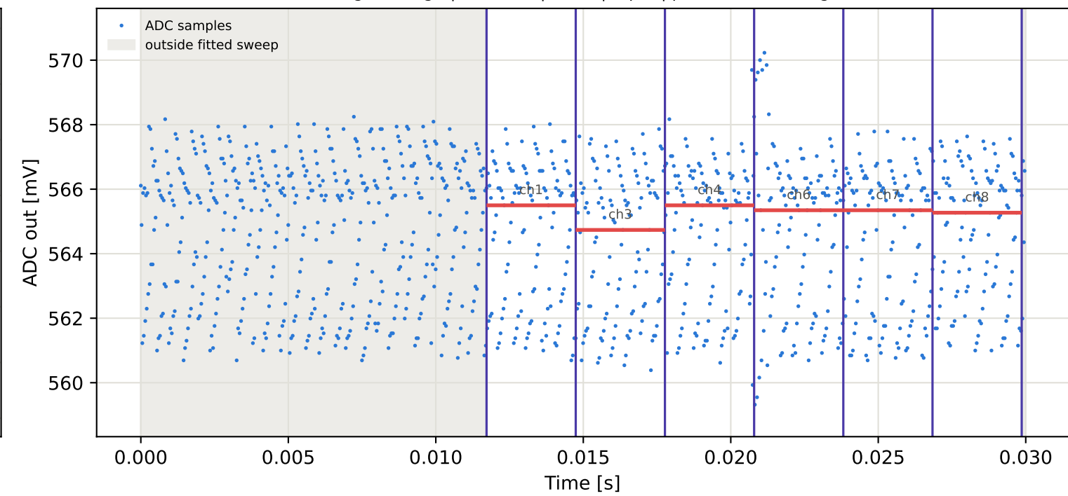
Tag7 &lt;- Tag4 | 965 MHz | run 0 | rep 1 | phase -62.49 deg
