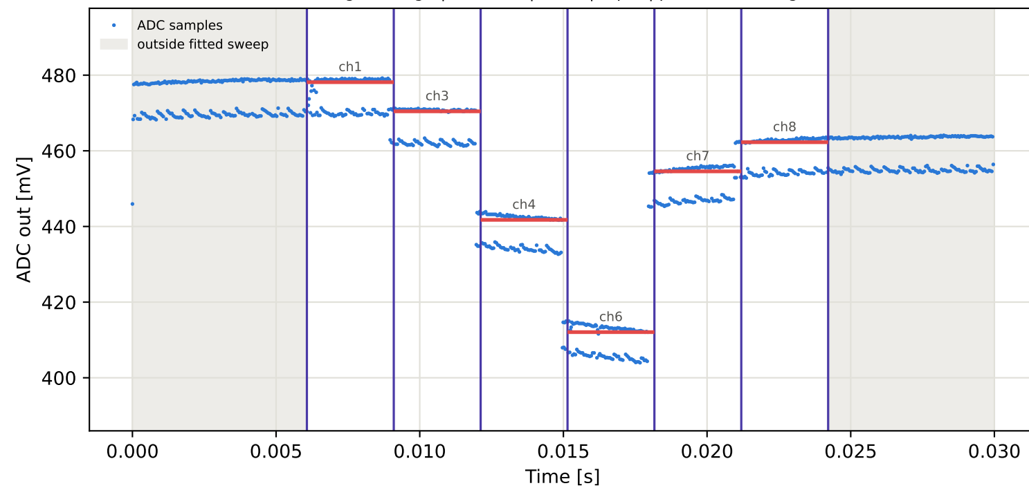
Tag8 &lt;- Tag1 | 925 MHz | run 0 | rep 1 | phase 131.35 deg
