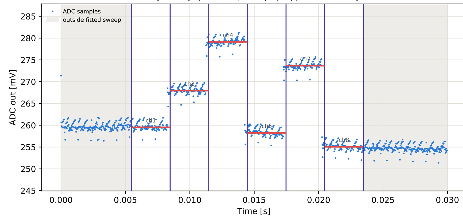
Tag6 &lt;- Tag1 | 985 MHz | run 0 | rep 1 | phase -75.89 deg
