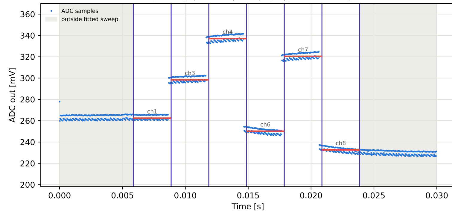
Tag3 &lt;- Tag6 | 935 MHz | run 0 | rep 1 | phase -71.77 deg
