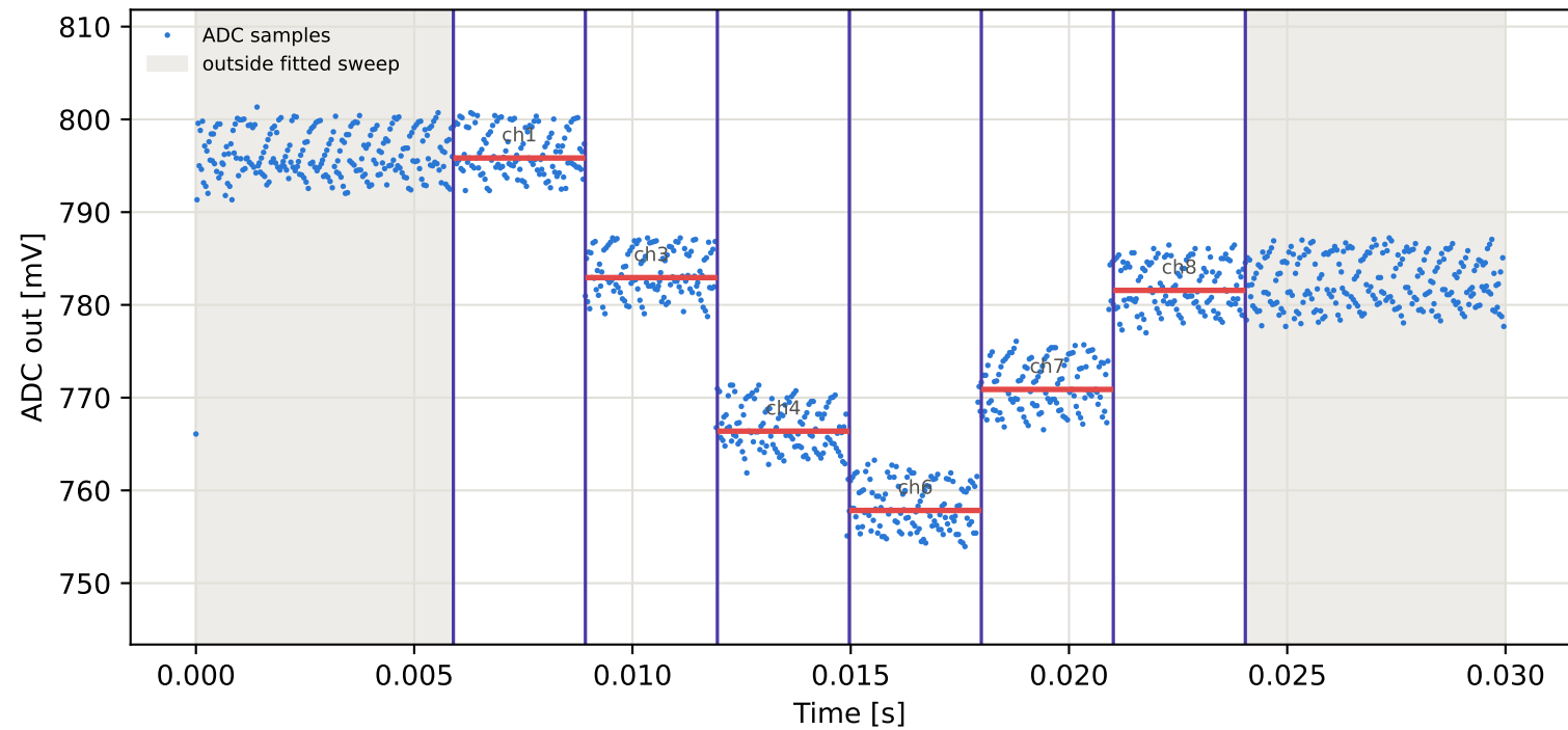
Tag7 &lt;- Tag6 | 885 MHz | run 0 | rep 1 | phase -151.50 deg
