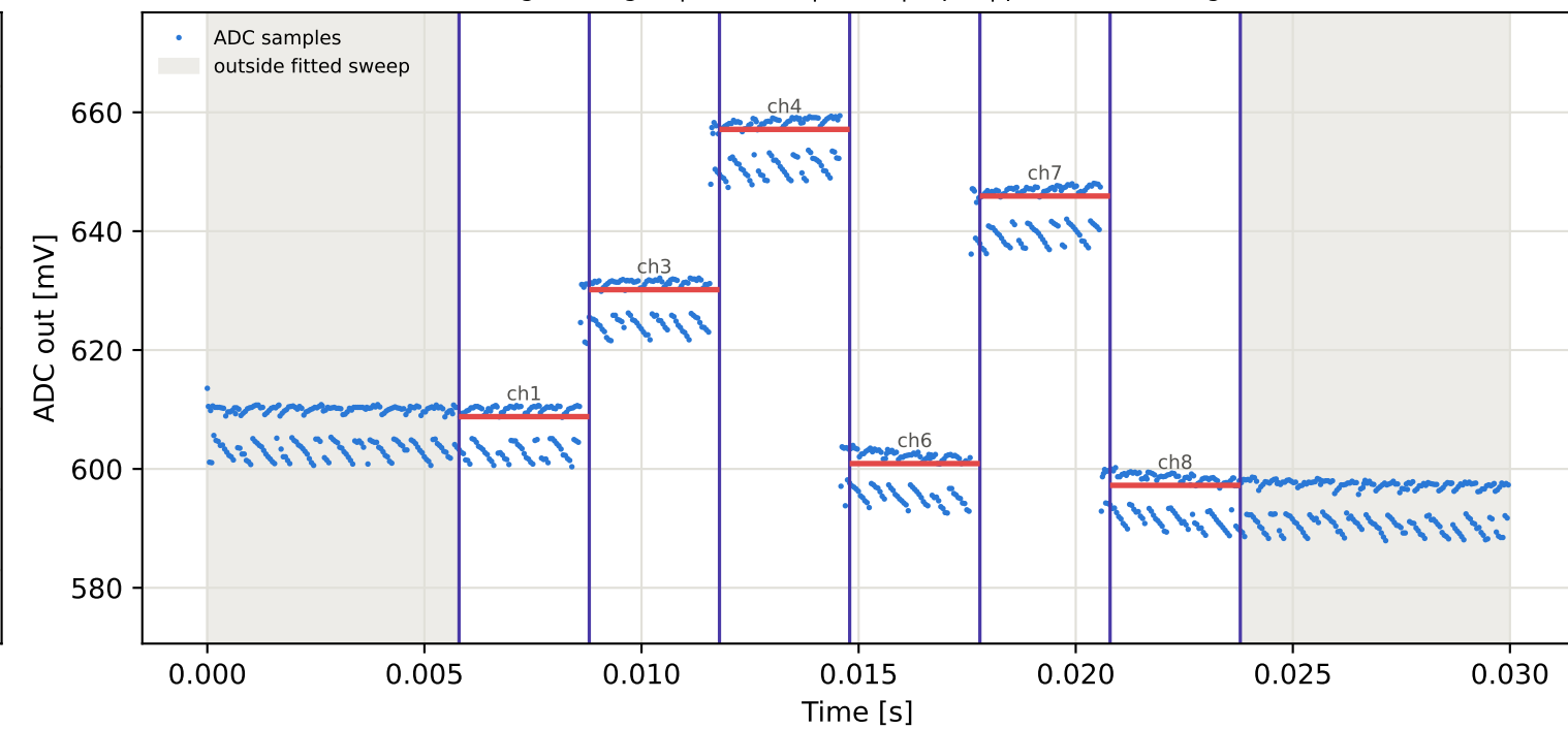
Tag6 &lt;- Tag3 | 965 MHz | run 0 | rep 1 | phase 79.23 deg
