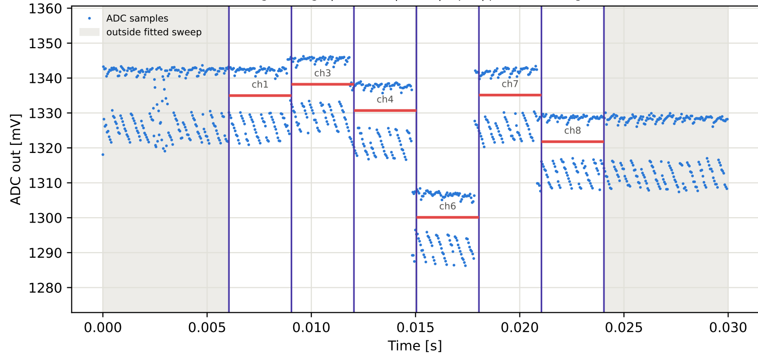
Tag8 &lt;- Tag5 | 935 MHz | run 0 | rep 1 | phase 155.92 deg
