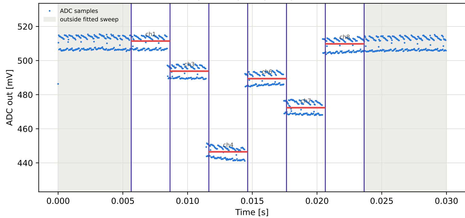
Tag9 &lt;- Tag8 | 975 MHz | run 0 | rep 1 | phase 73.55 deg
