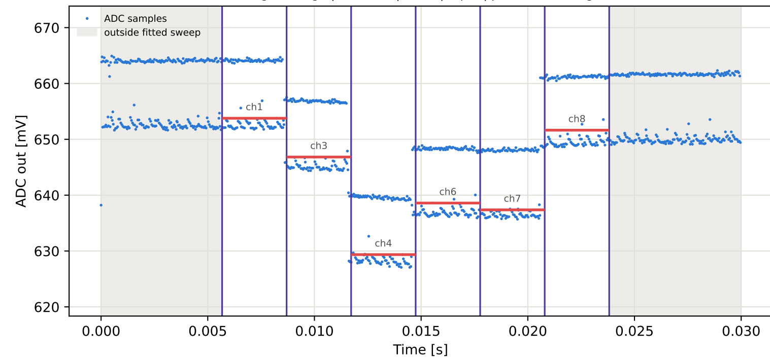
Tag4 &lt;- Tag15 | 965 MHz | run 0 | rep 1 | phase 155.22 deg
