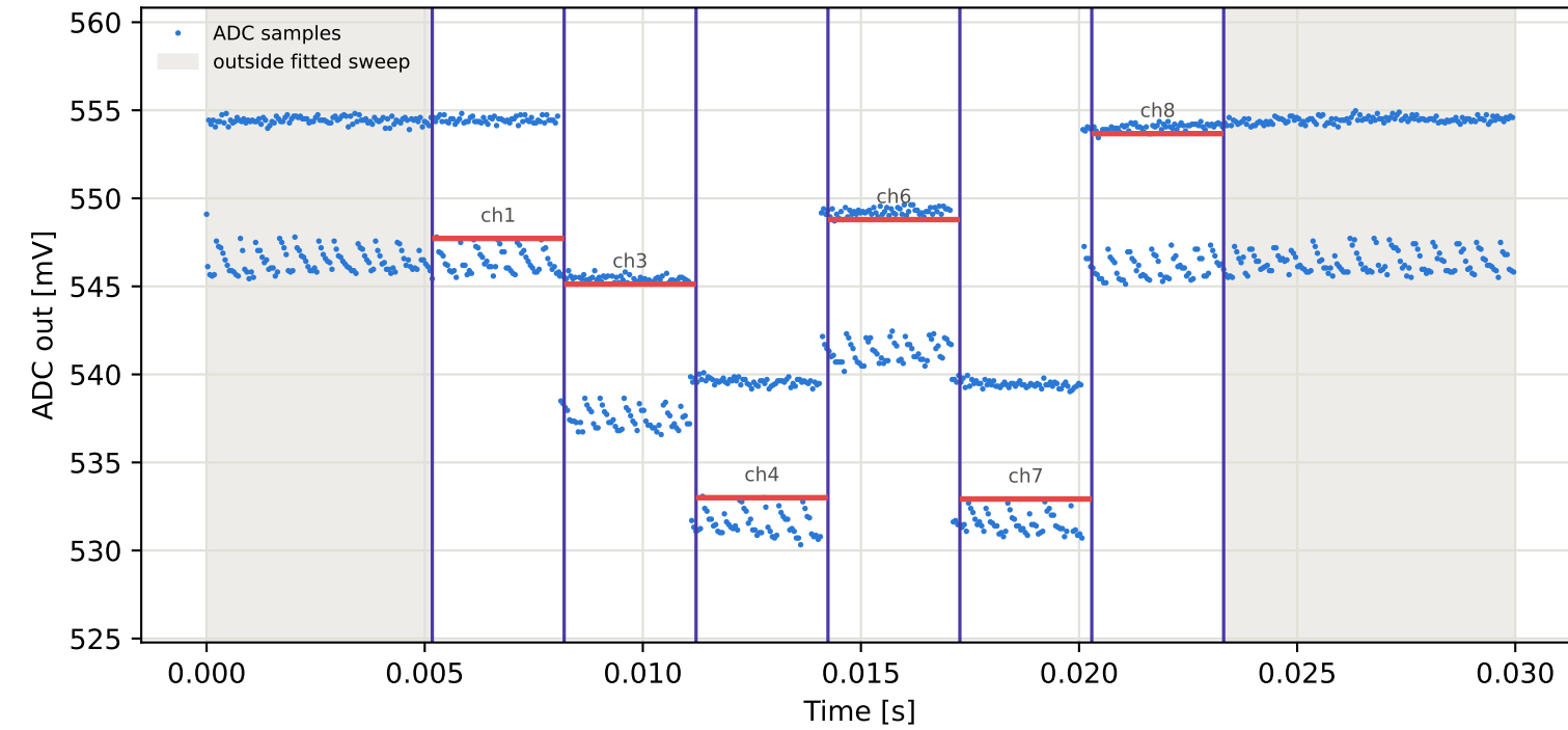
Tag4 &lt;- Tag9 | 845 MHz | run 0 | rep 1 | phase 102.37 deg
