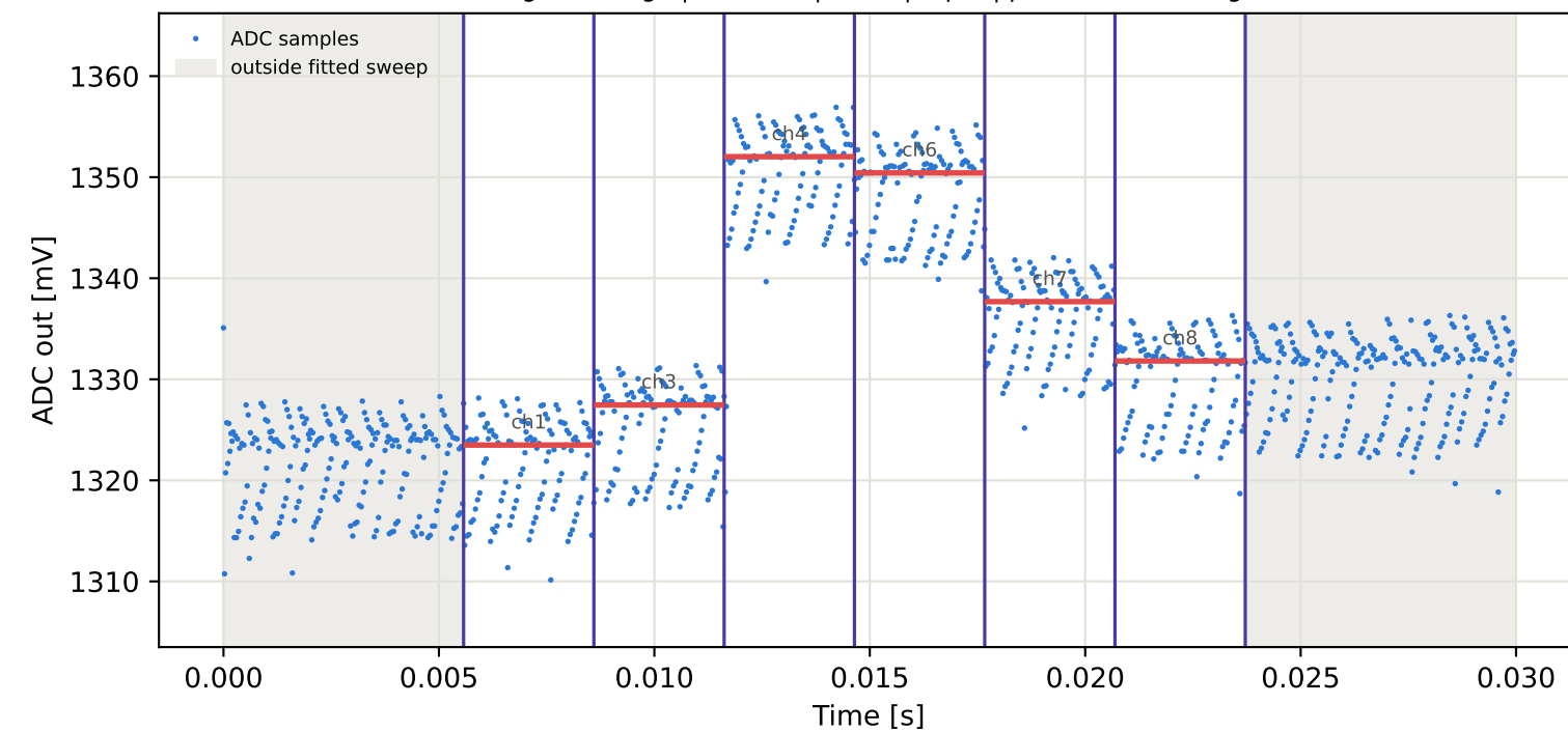
Tag16 &lt;- Tag6 | 965 MHz | run 0 | rep 1 | phase -134.18 deg
