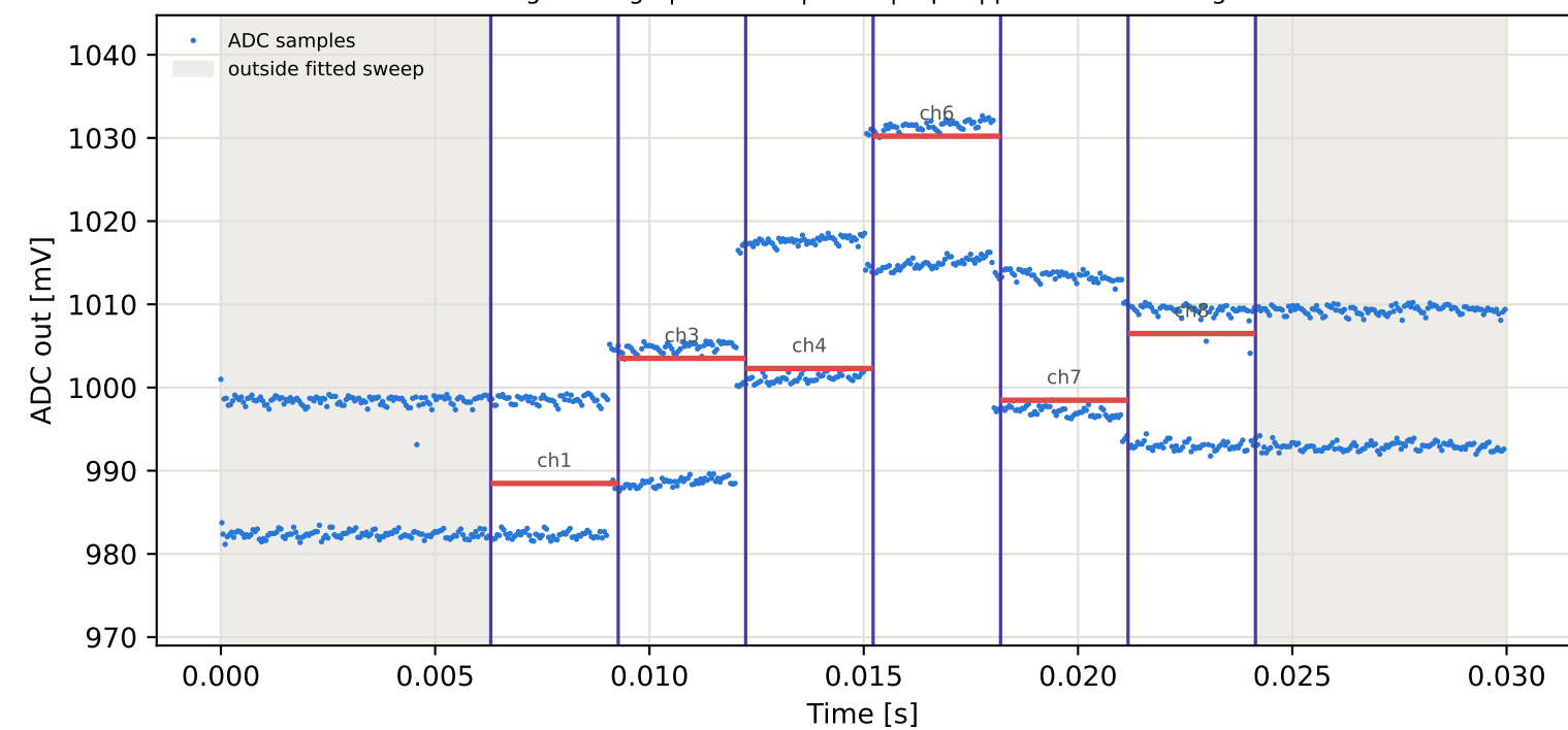
Tag5 &lt;- Tag1 | 905 MHz | run 0 | rep 1 | phase -158.32 deg
