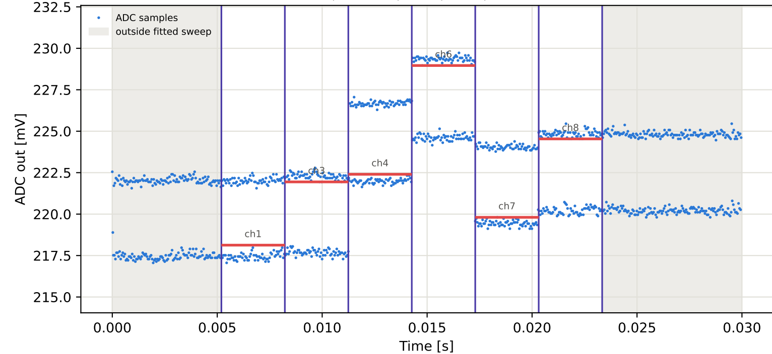
Tag5 &lt;- Tag1 | 975 MHz | run 0 | rep 1 | phase -167.26 deg
