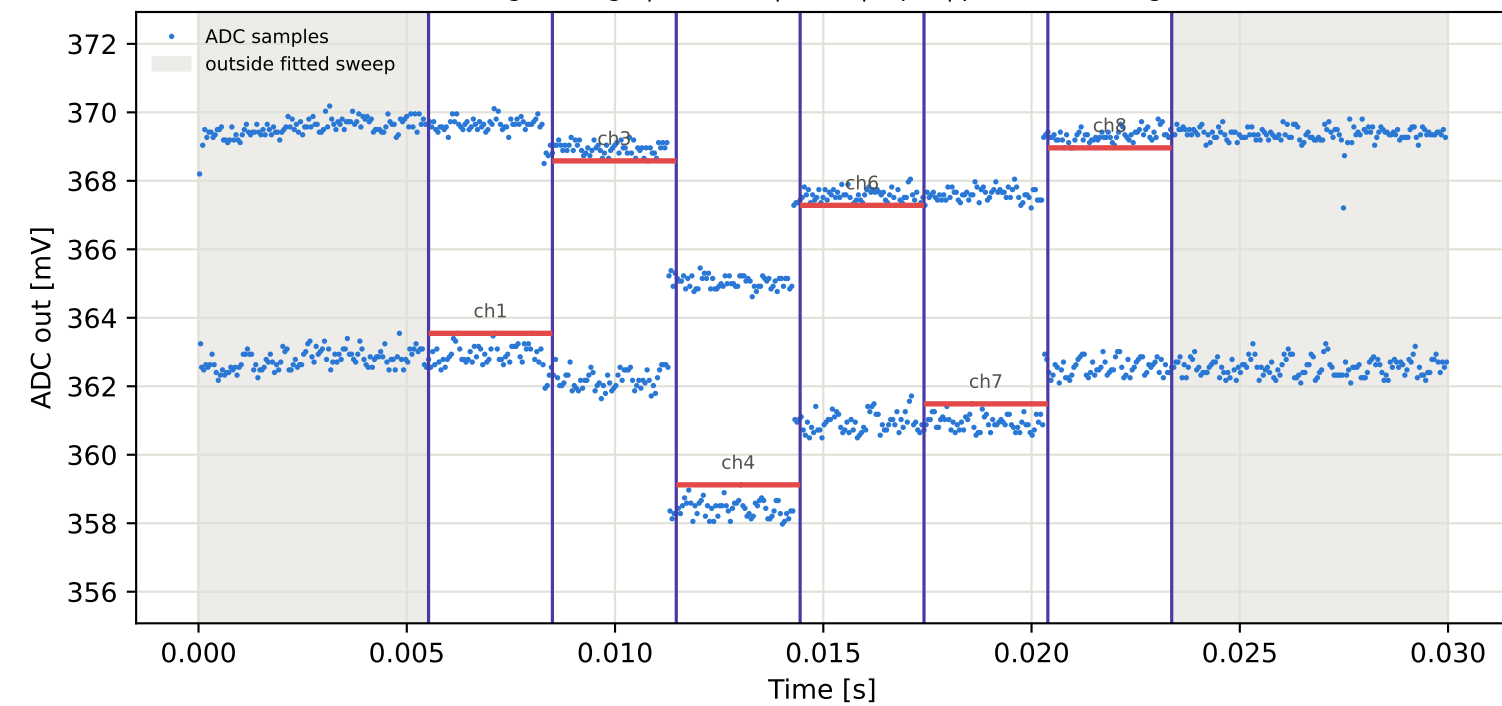
Tag4 &lt;- Tag7 | 995 MHz | run 0 | rep 1 | phase 23.77 deg
