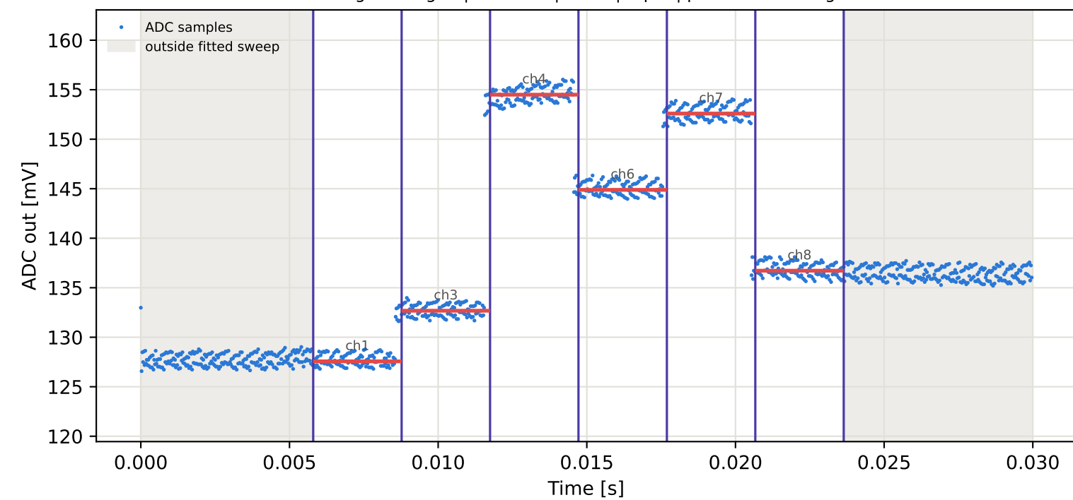
Tag7 &lt;- Tag3 | 805 MHz | run 0 | rep 1 | phase -69.40 deg
