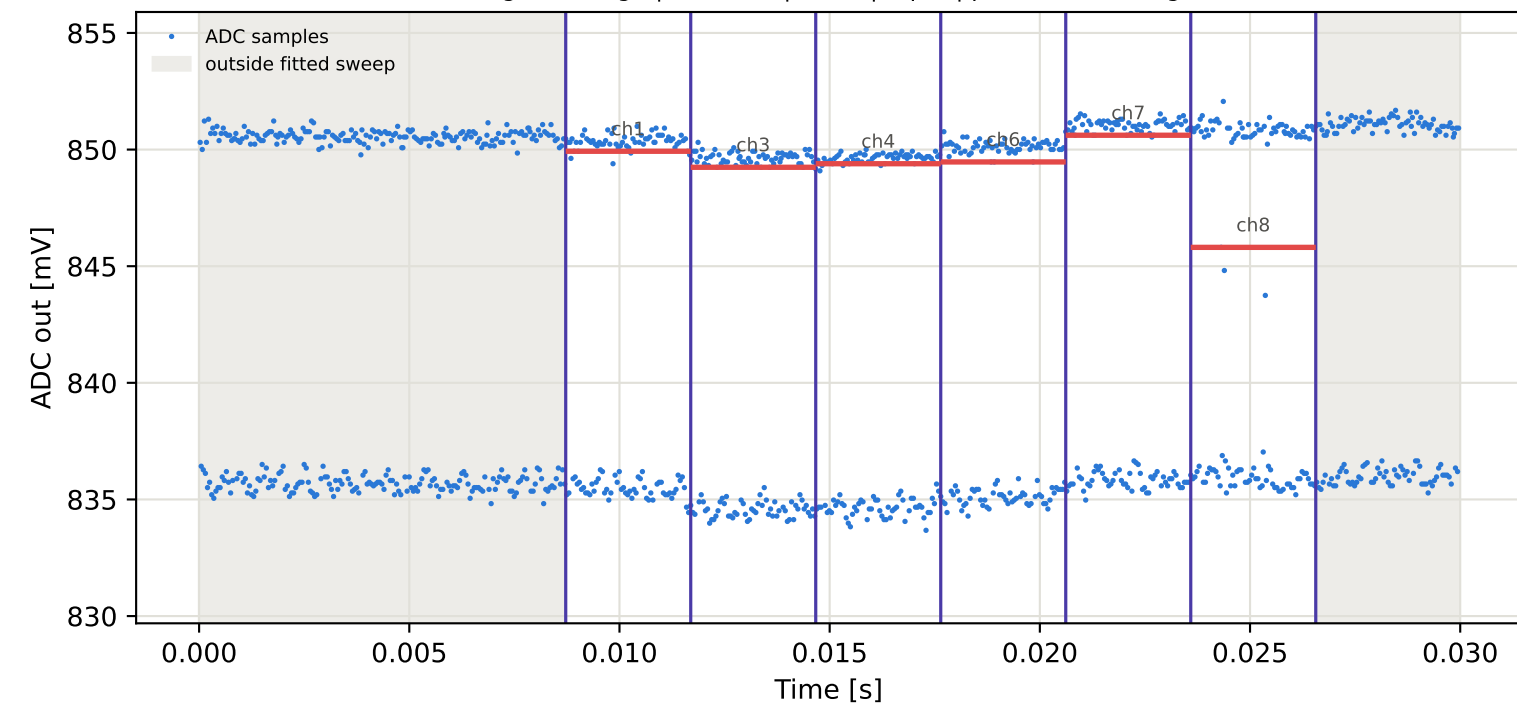
Tag16 &lt;- Tag4 | 995 MHz | run 0 | rep 1 | phase 70.78 deg
