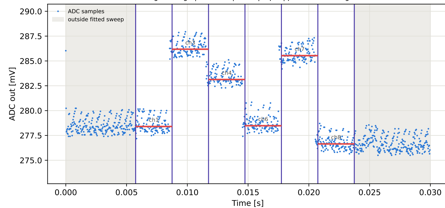
Tag2 &lt;- Tag5 | 825 MHz | run 0 | rep 1 | phase 147.34 deg
