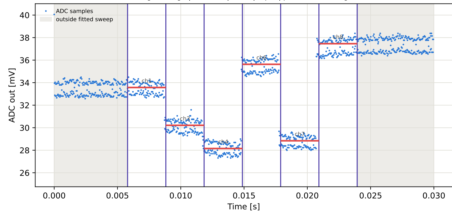
Tag3 &lt;- Tag9 | 915 MHz | run 0 | rep 1 | phase 9.25 deg
