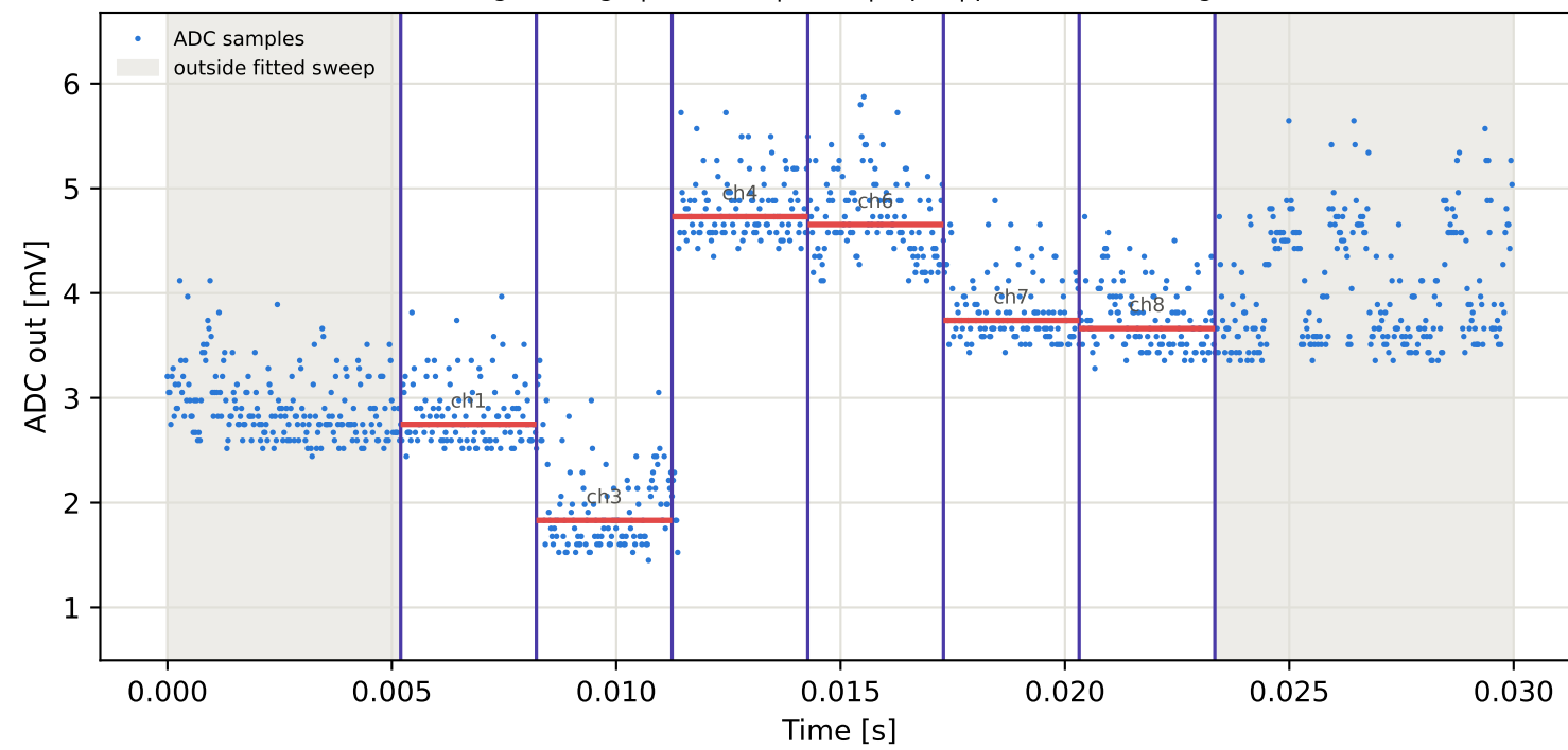
Tag2 &lt;- Tag5 | 785 MHz | run 0 | rep 1 | phase 76.10 deg
