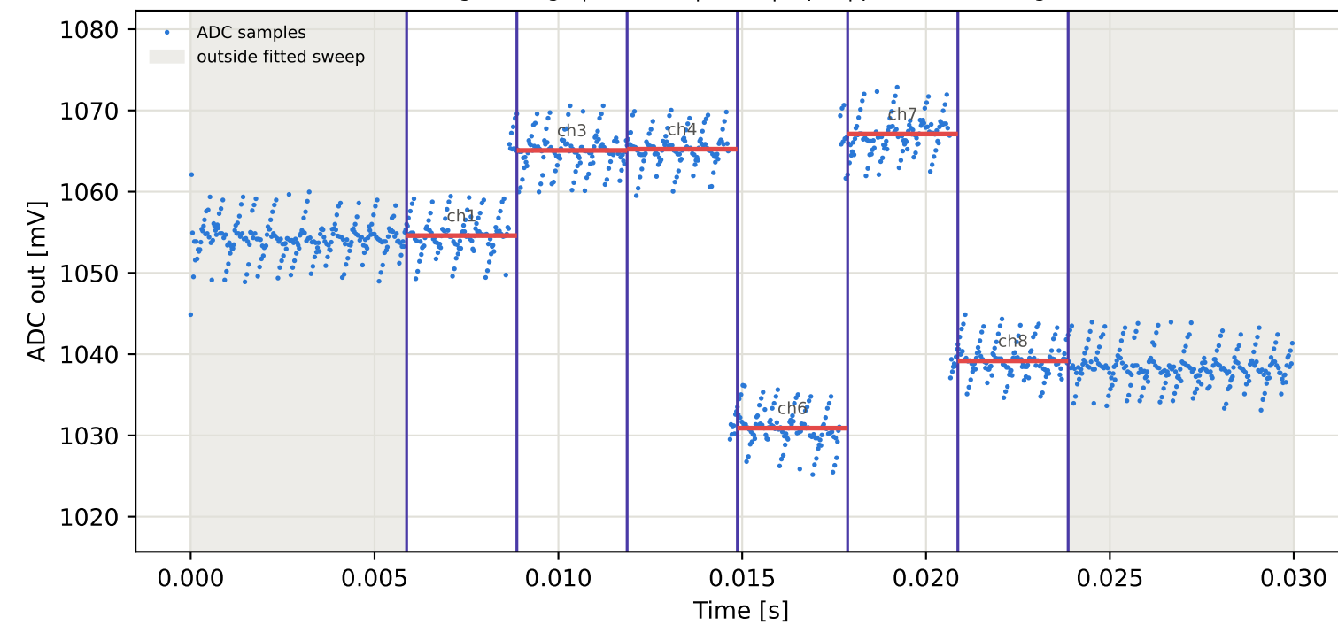
Tag4 &lt;- Tag15 | 945 MHz | run 0 | rep 1 | phase 113.08 deg
