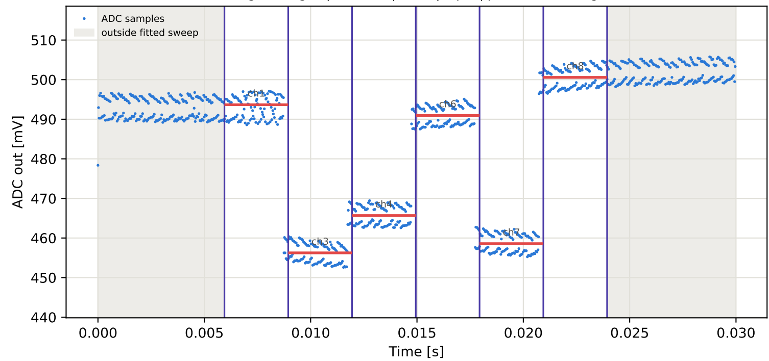
Tag5 &lt;- Tag2 | 855 MHz | run 0 | rep 1 | phase 85.63 deg
