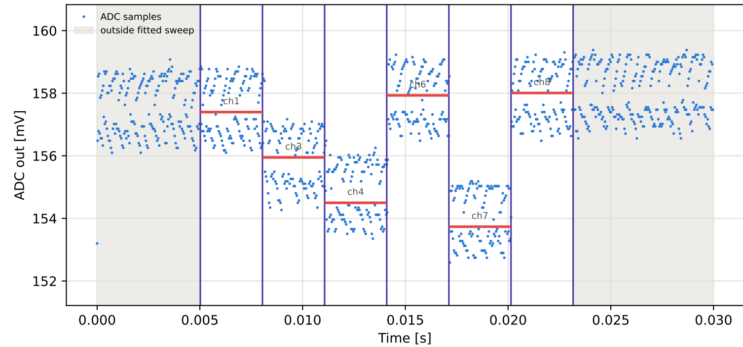
Tag16 &lt;- Tag15 | 795 MHz | run 0 | rep 1 | phase 63.20 deg
