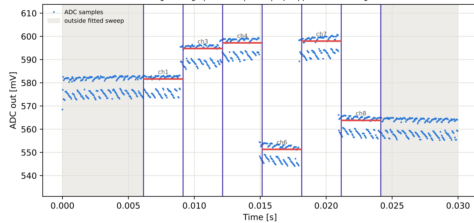
Tag6 &lt;- Tag9 | 945 MHz | run 0 | rep 1 | phase 32.18 deg
