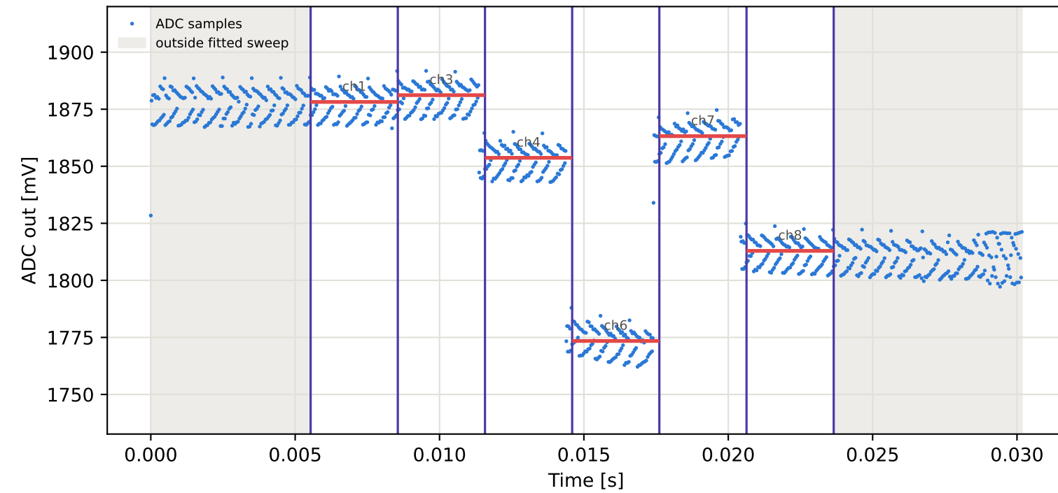
Tag8 &lt;- Tag6 | 895 MHz | run 0 | rep 1 | phase -38.14 deg
