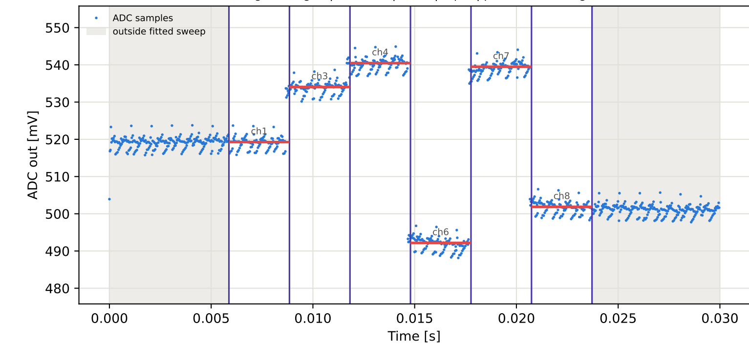
Tag5 &lt;- Tag3 | 945 MHz | run 0 | rep 1 | phase 2.40 deg
