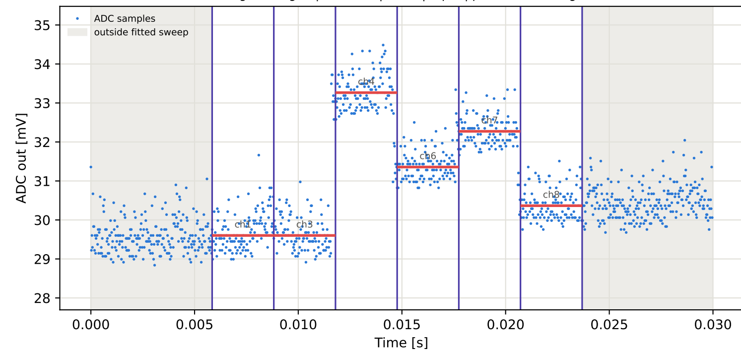
Tag2 &lt;- Tag15 | 775 MHz | run 0 | rep 1 | phase -95.58 deg
