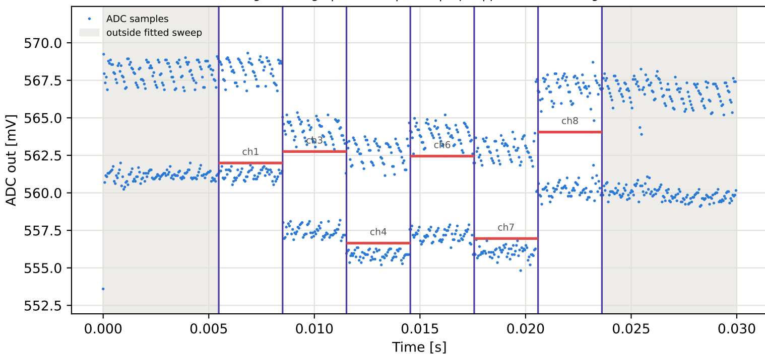
Tag10 &lt;- Tag1 | 875 MHz | run 0 | rep 1 | phase 100.69 deg
