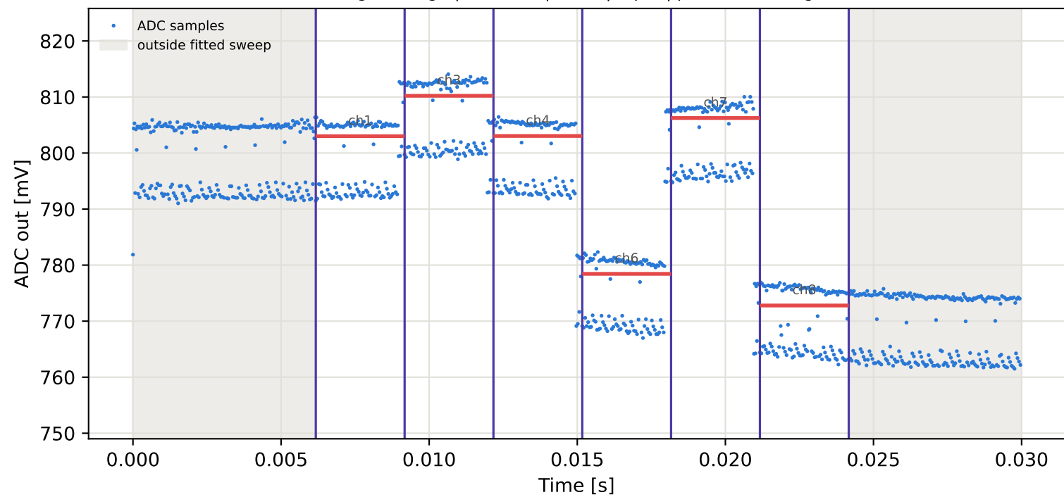
Tag3 &lt;- Tag15 | 885 MHz | run 0 | rep 1 | phase 8.55 deg
