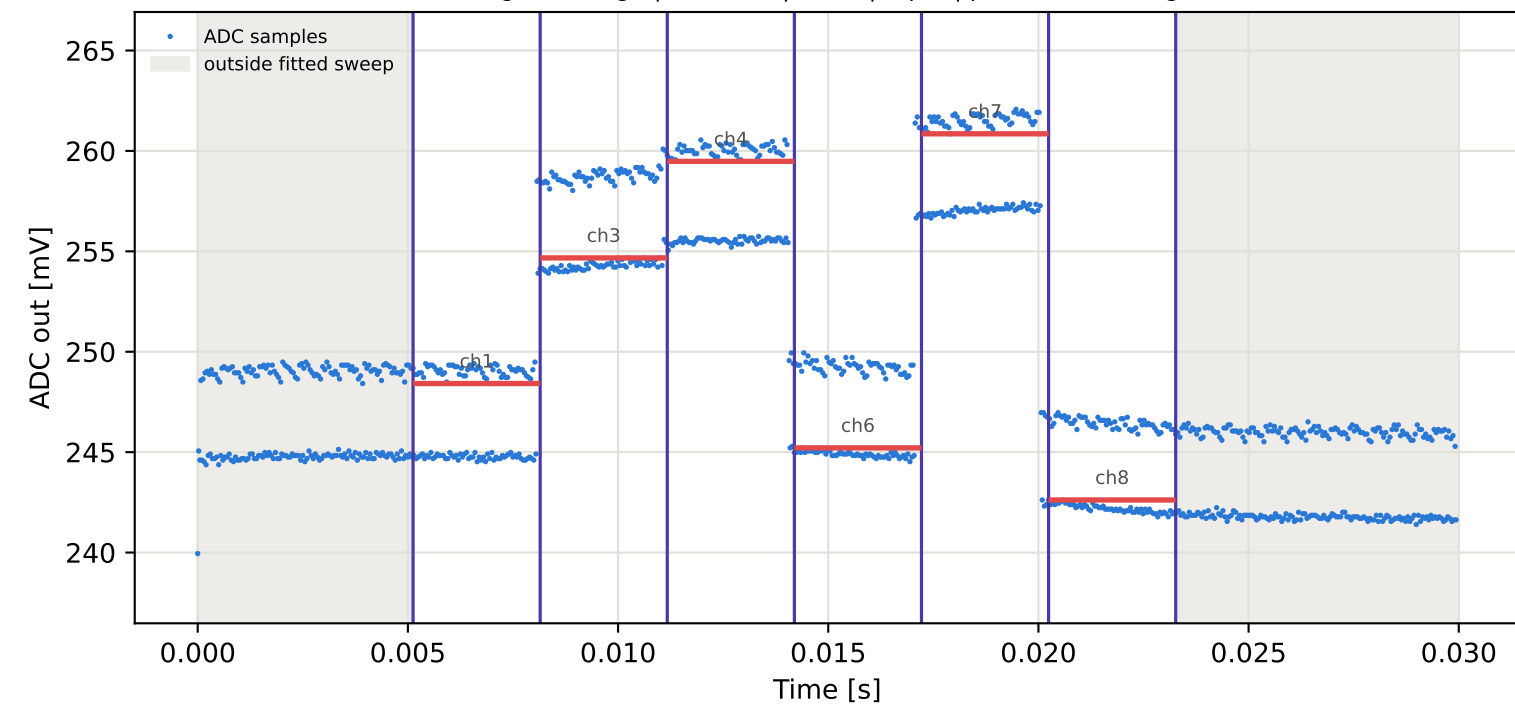
Tag10 &lt;- Tag9 | 845 MHz | run 0 | rep 1 | phase -114.85 deg
