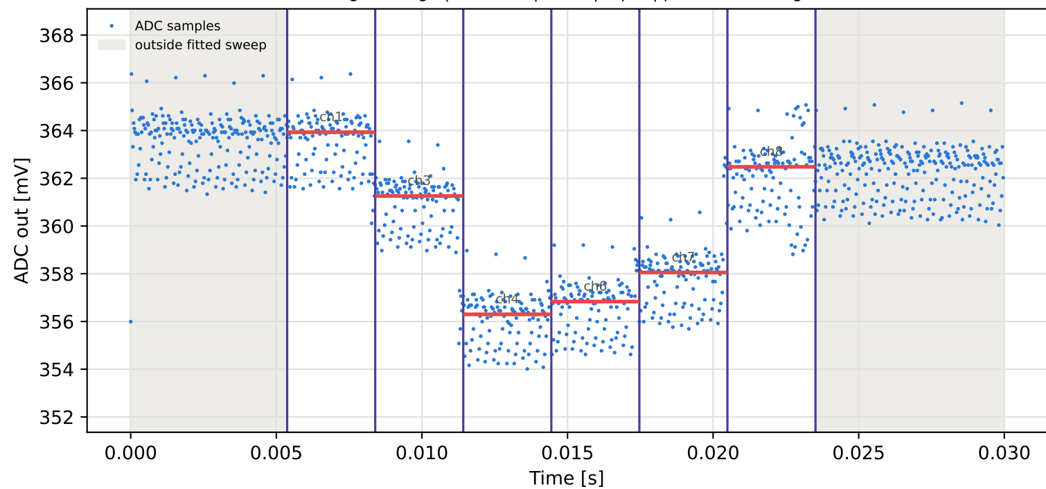
Tag3 &lt;- Tag2 | 825 MHz | run 0 | rep 1 | phase 69.00 deg
