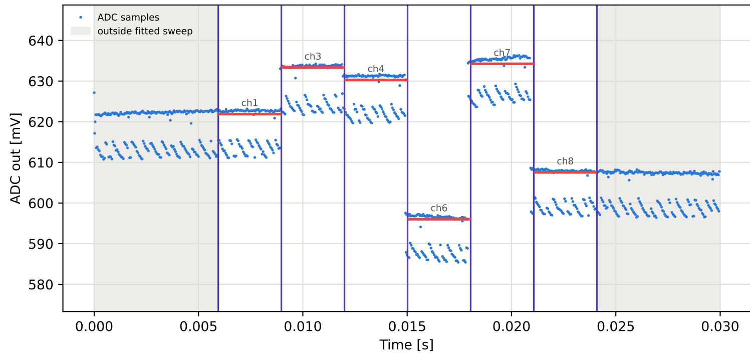
Tag6 &lt;- Tag9 | 965 MHz | run 0 | rep 1 | phase 23.32 deg
