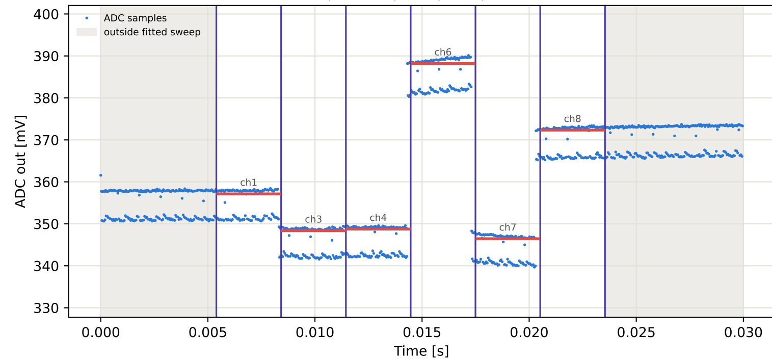
Tag5 &lt;- Tag4 | 955 MHz | run 0 | rep 1 | phase 167.10 deg
