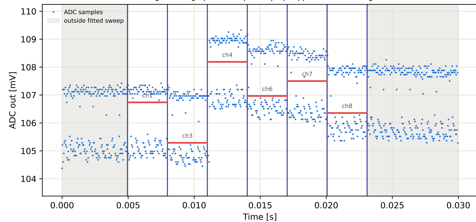
Tag10 &lt;- Tag9 | 785 MHz | run 0 | rep 1 | phase 136.36 deg
