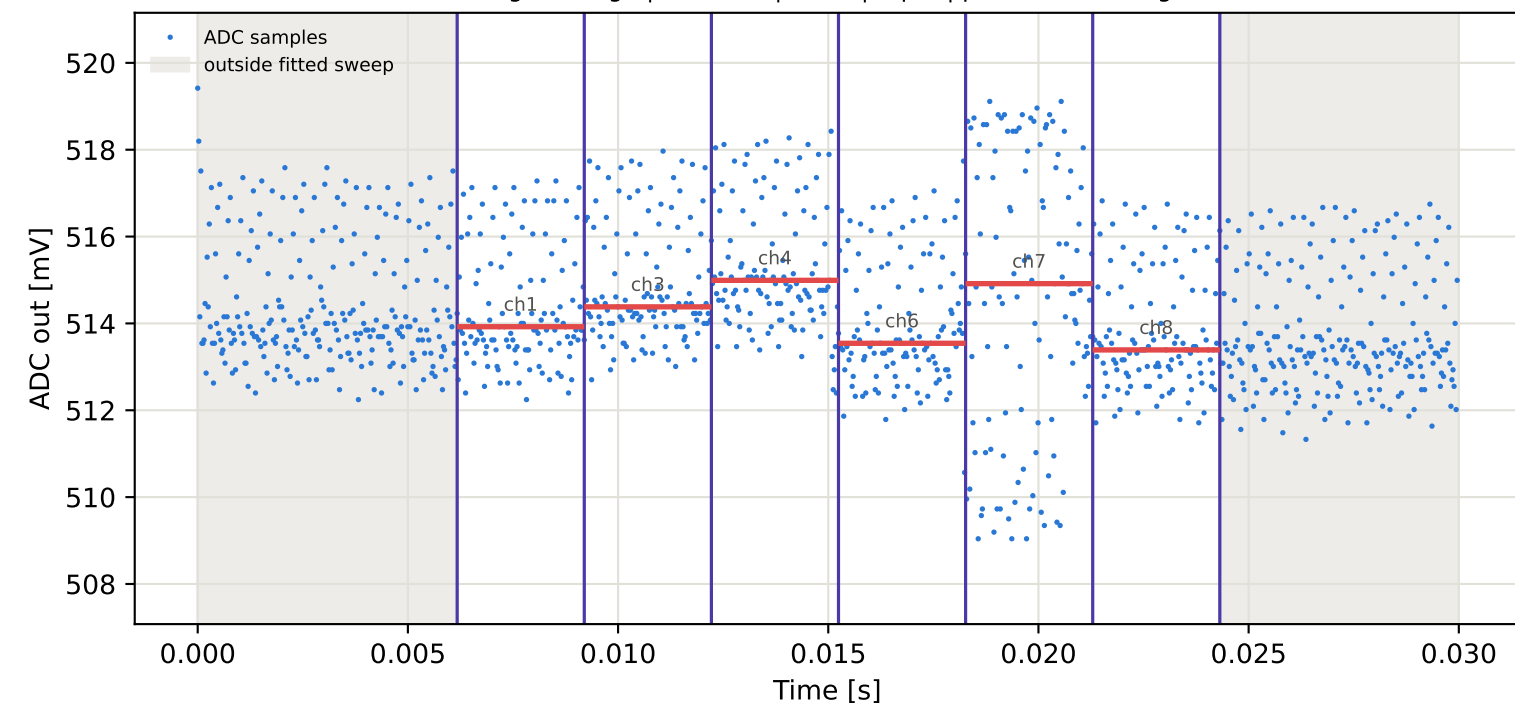
Tag3 &lt;- Tag2 | 955 MHz | run 0 | rep 1 | phase -59.92 deg
