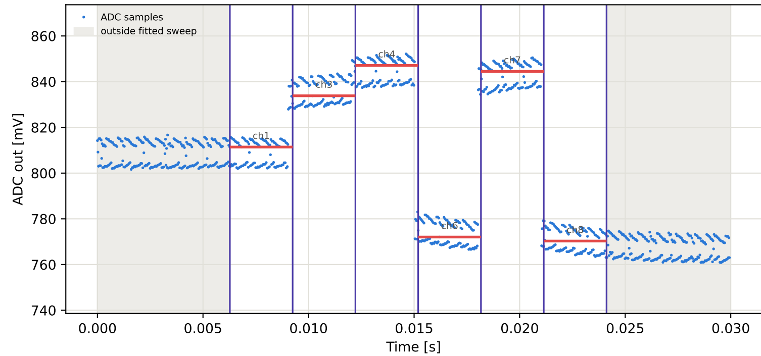
Tag9 &lt;- Tag2 | 925 MHz | run 0 | rep 1 | phase 38.70 deg
