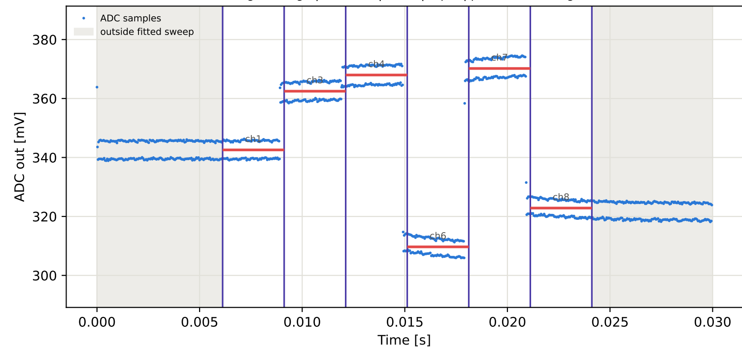
Tag5 &lt;- Tag1 | 995 MHz | run 0 | rep 1 | phase 36.93 deg
