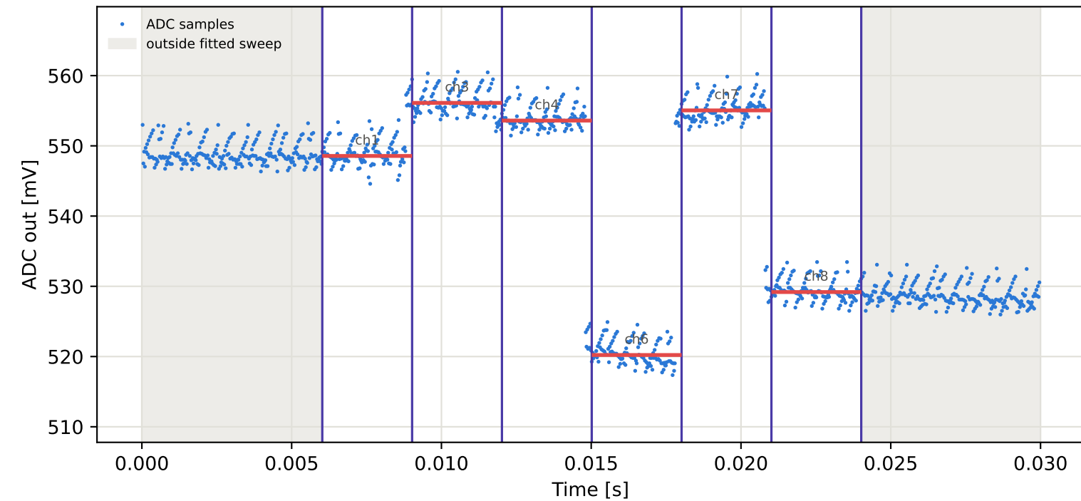
Tag7 &lt;- Tag10 | 915 MHz | run 0 | rep 1 | phase 62.94 deg
