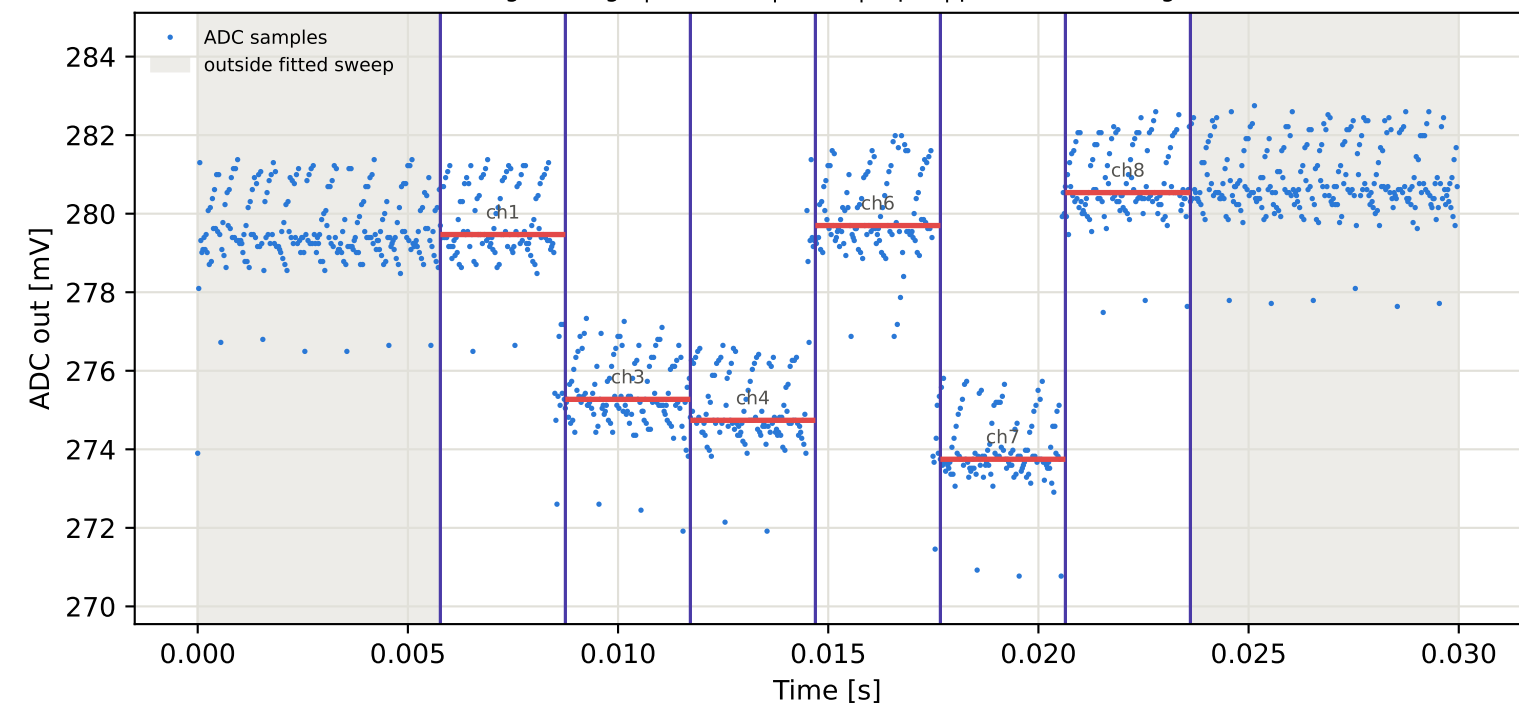
Tag8 &lt;- Tag7 | 805 MHz | run 0 | rep 1 | phase 138.59 deg
