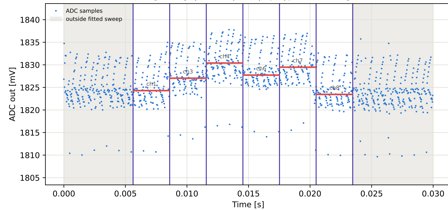
Tag8 &lt;- Tag4 | 895 MHz | run 0 | rep 1 | phase 15.03 deg
