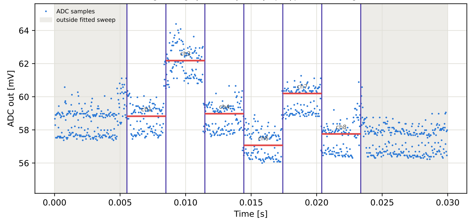
Tag2 &lt;- Tag6 | 805 MHz | run 0 | rep 1 | phase -74.58 deg
