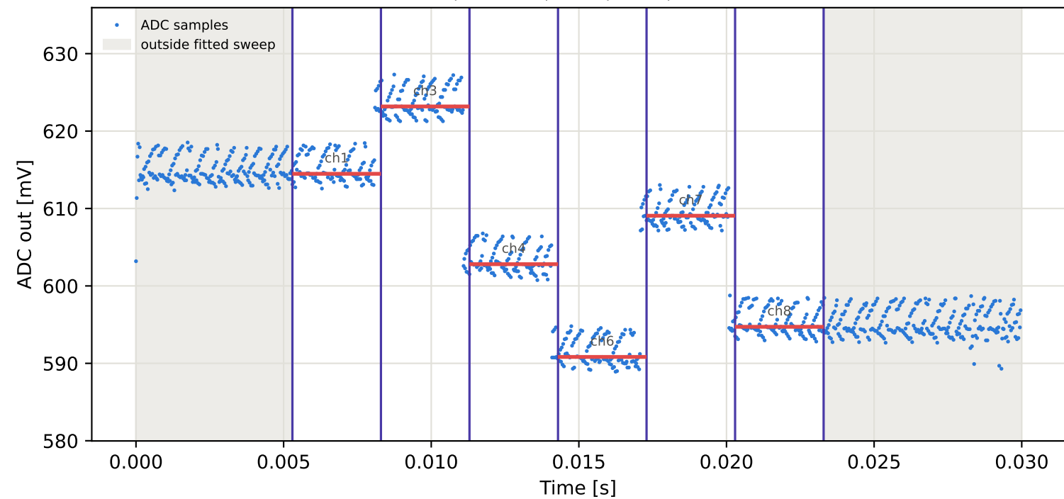
Tag4 &lt;- Tag3 | 835 MHz | run 0 | rep 1 | phase 27.99 deg
