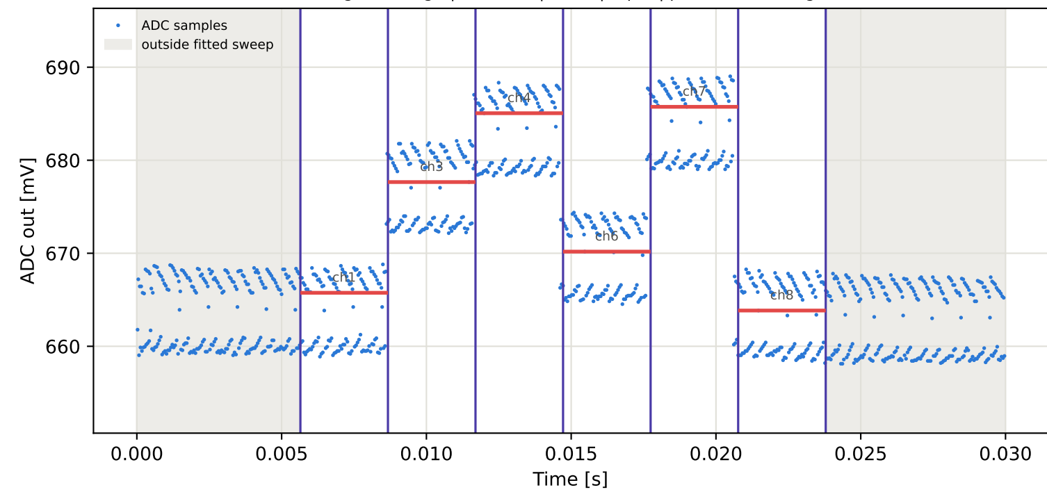
Tag2 &lt;- Tag10 | 825 MHz | run 0 | rep 1 | phase -94.71 deg
