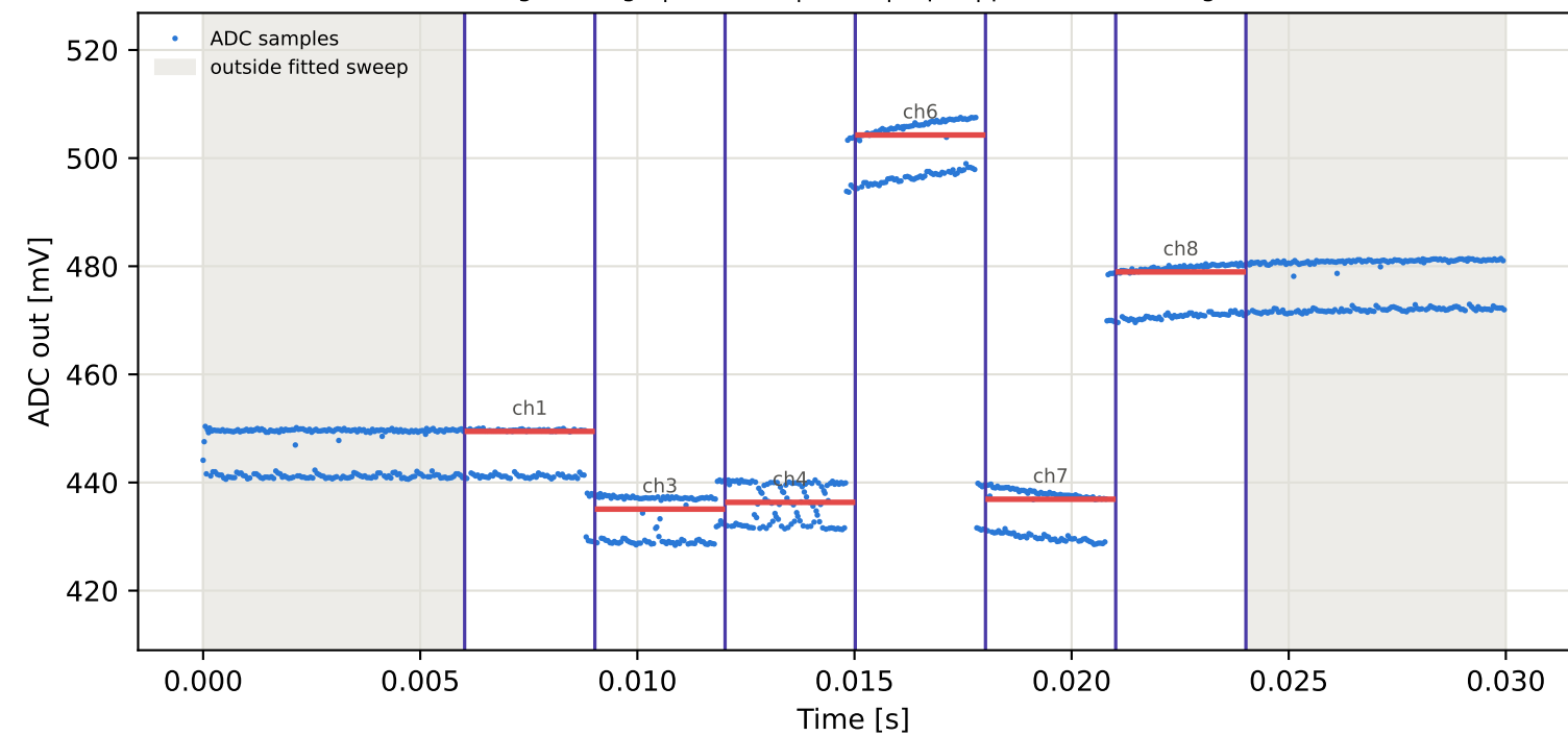
Tag7 &lt;- Tag6 | 925 MHz | run 0 | rep 1 | phase 19.41 deg
