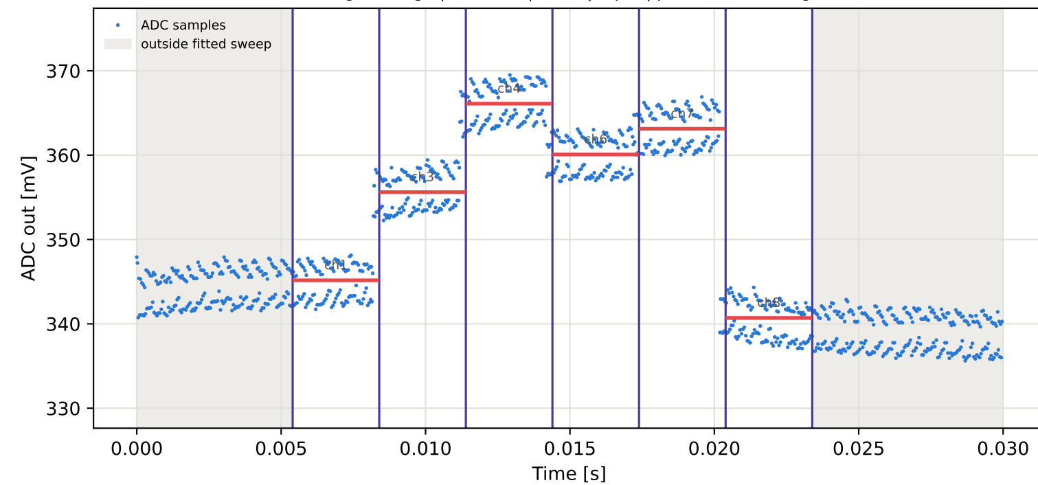
Tag2 &lt;- Tag5 | 905 MHz | run 0 | rep 1 | phase 144.93 deg
