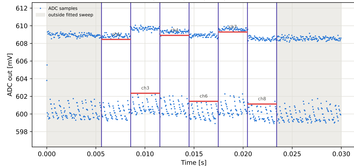
Tag15 &lt;- Tag1 | 855 MHz | run 0 | rep 1 | phase -40.78 deg
