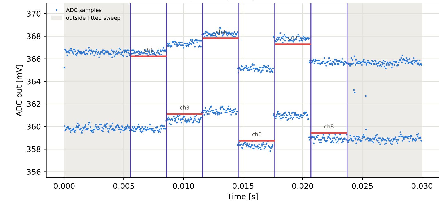
Tag4 &lt;- Tag2 | 995 MHz | run 0 | rep 1 | phase -52.66 deg
