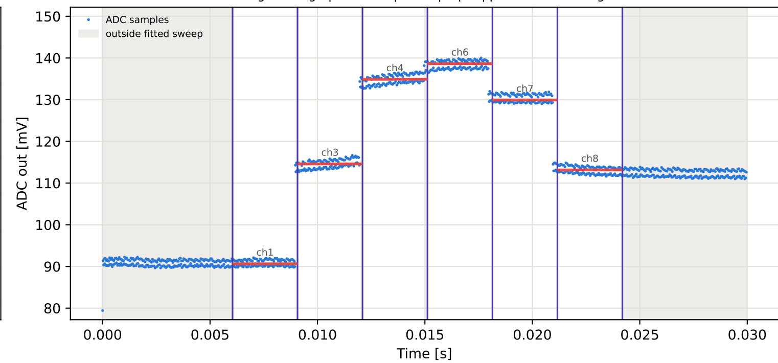
Tag1 &lt;- Tag8 | 865 MHz | run 0 | rep 1 | phase -158.43 deg
