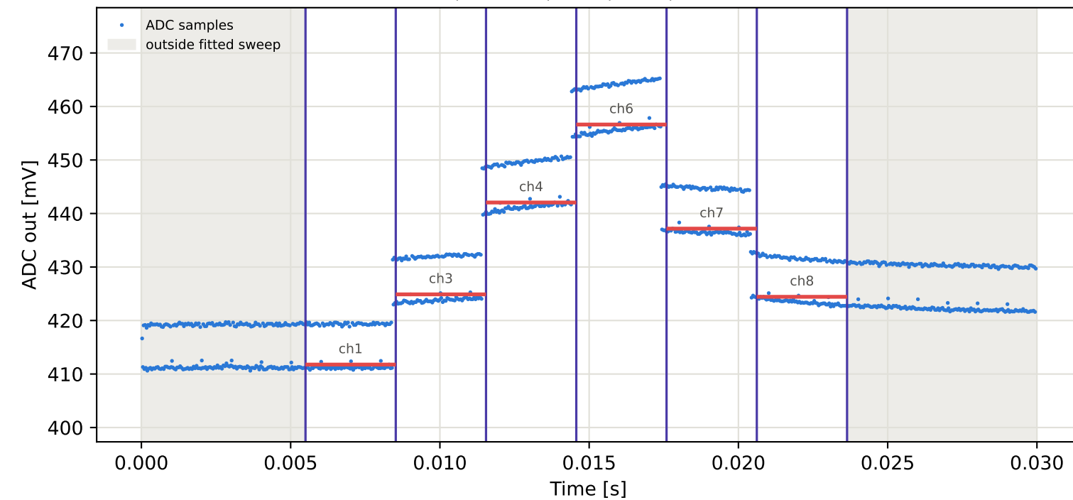
Tag1 &lt;- Tag9 | 905 MHz | run 0 | rep 1 | phase -131.86 deg
