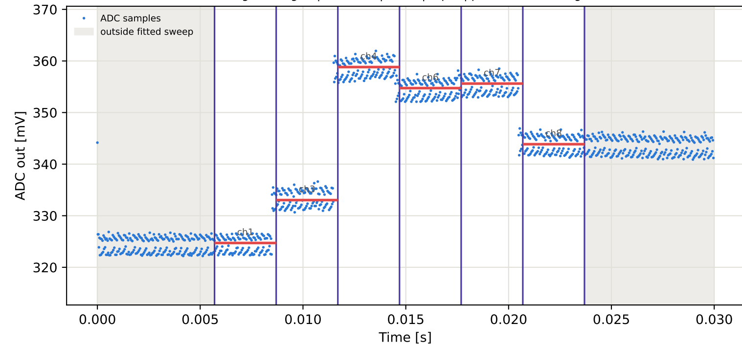
Tag3 &lt;- Tag16 | 825 MHz | run 0 | rep 1 | phase -113.25 deg
