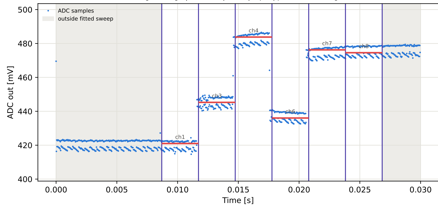
Tag5 &lt;- Tag1 | 875 MHz | run 0 | rep 1 | phase -63.94 deg
