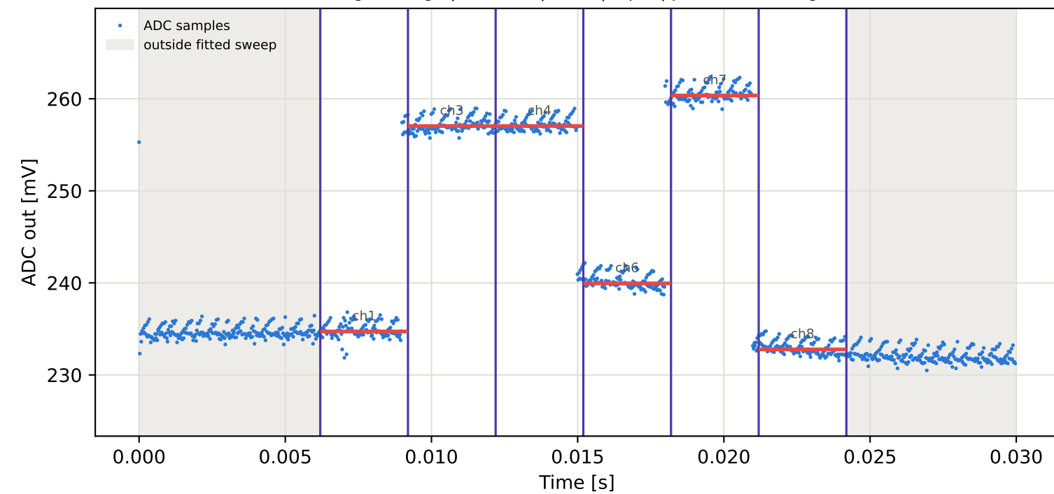
Tag8 &lt;- Tag1 | 835 MHz | run 0 | rep 1 | phase 134.98 deg
