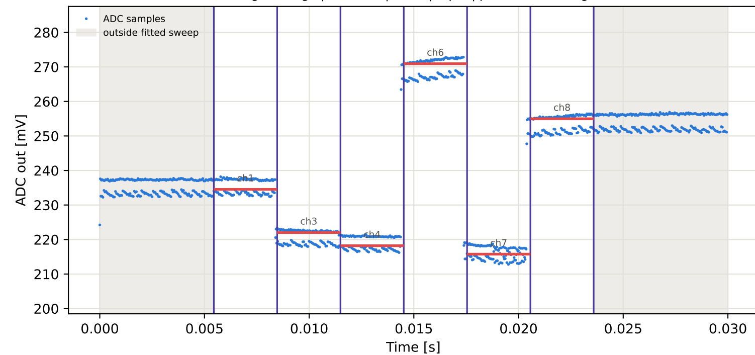
Tag5 &lt;- Tag3 | 975 MHz | run 0 | rep 1 | phase 155.75 deg
