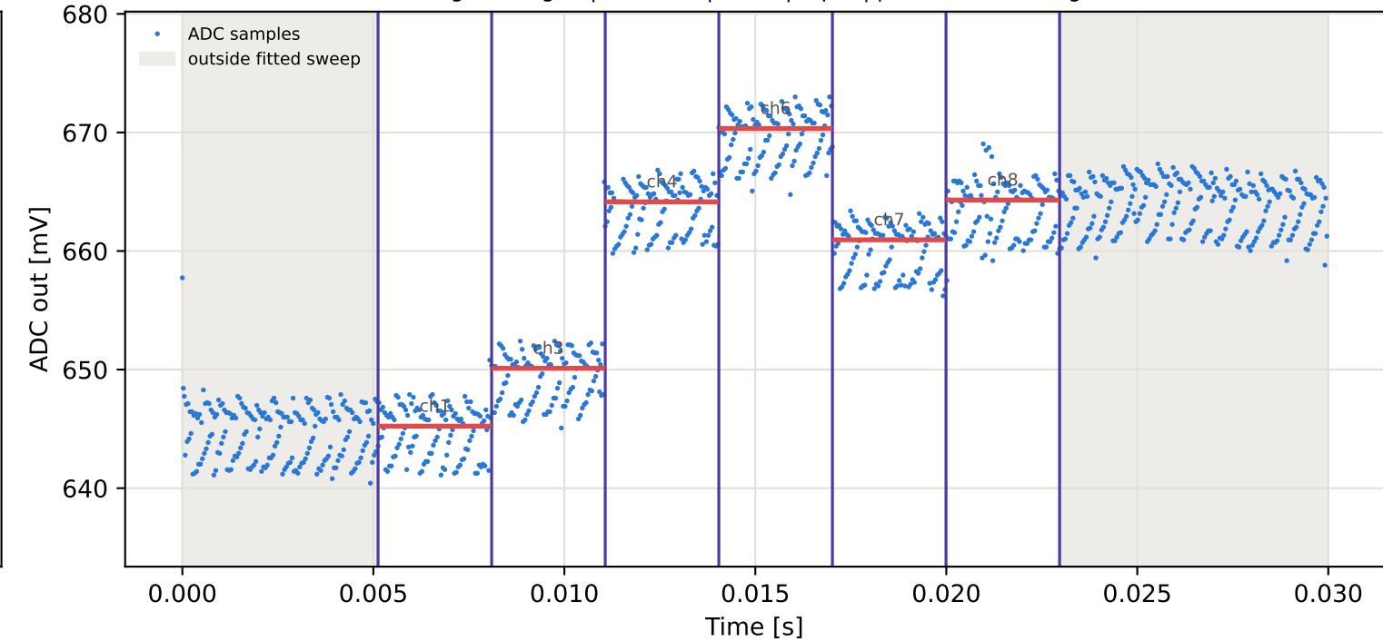
Tag7 &lt;- Tag15 | 865 MHz | run 0 | rep 1 | phase -134.85 deg
