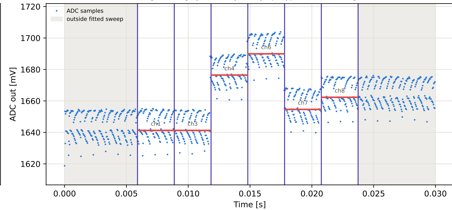
Tag2 &lt;- Tag10 | 975 MHz | run 0 | rep 1 | phase -93.60 deg
