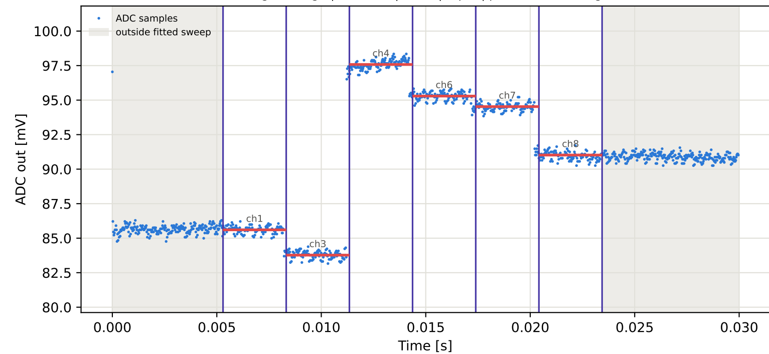
Tag8 &lt;- Tag1 | 795 MHz | run 0 | rep 1 | phase 112.67 deg
