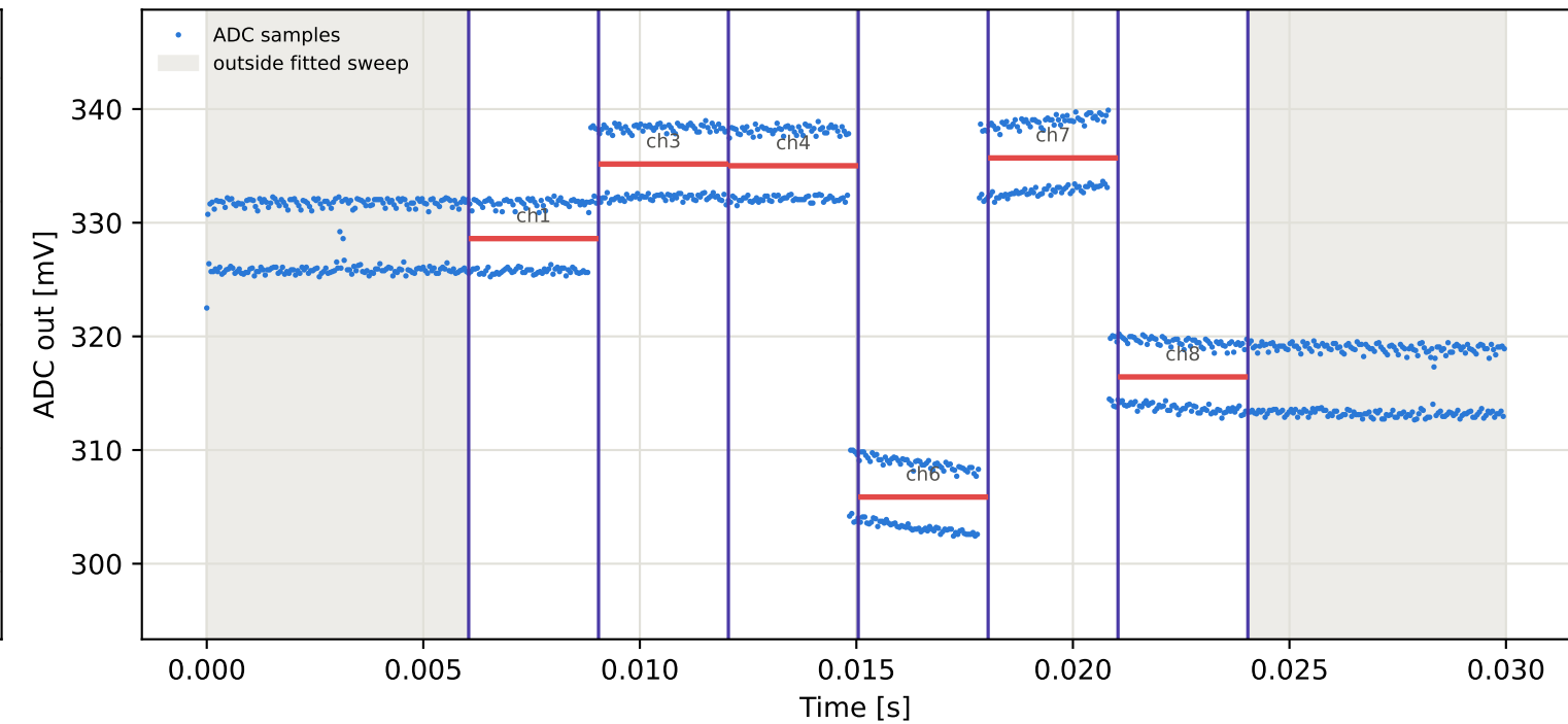
Tag10 &lt;- Tag1 | 935 MHz | run 0 | rep 1 | phase 40.36 deg
