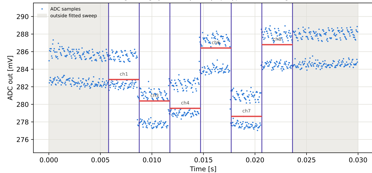
Tag3 &lt;- Tag10 | 825 MHz | run 0 | rep 1 | phase 161.21 deg
