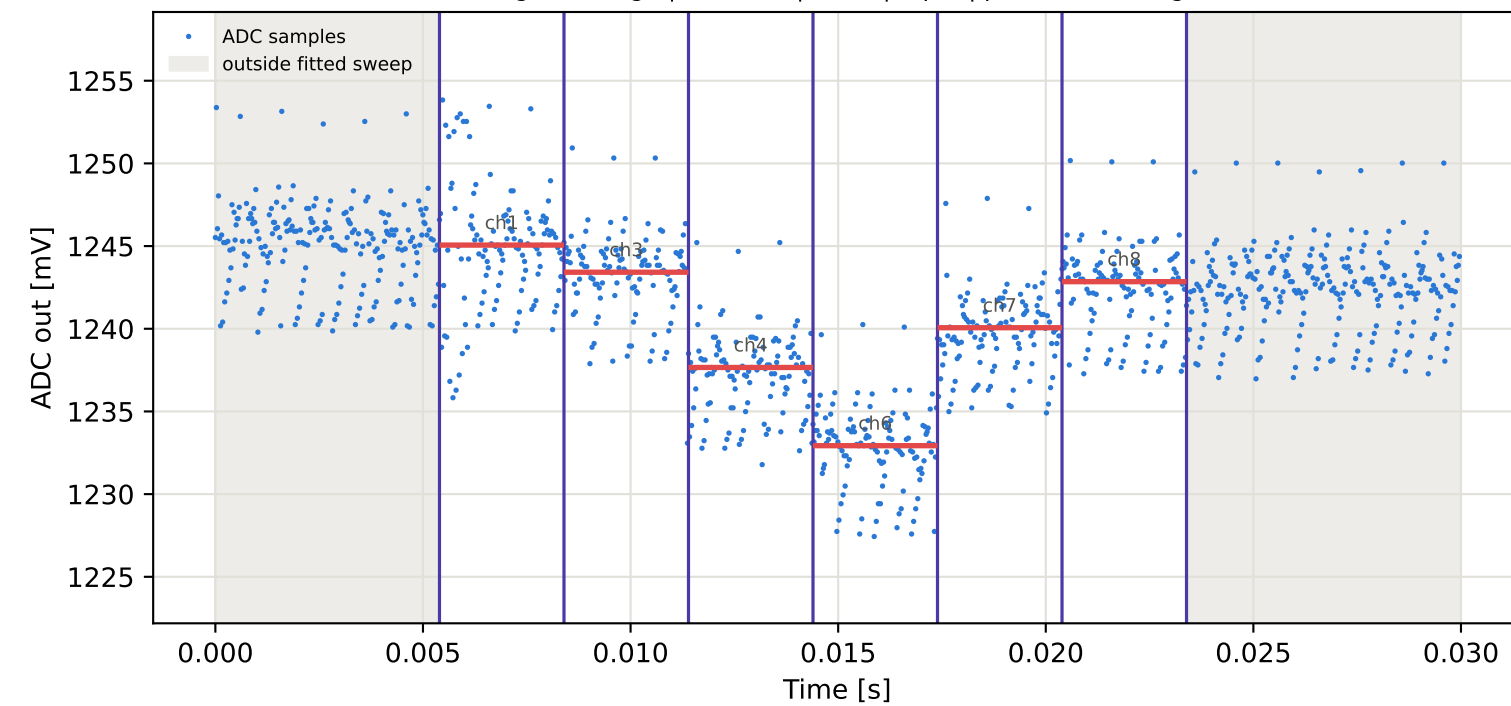
Tag16 &lt;- Tag4 | 875 MHz | run 0 | rep 1 | phase -139.28 deg
