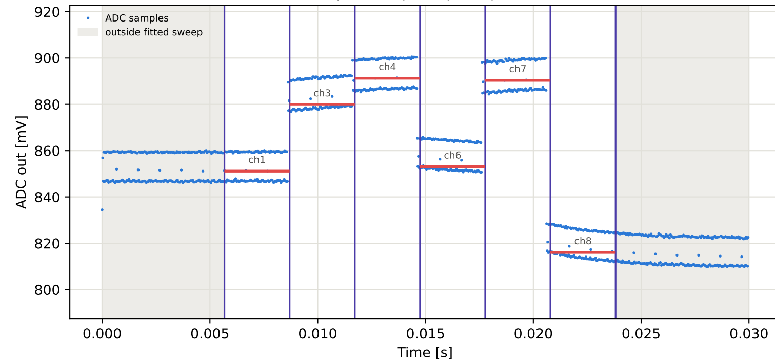
Tag3 &lt;- Tag16 | 875 MHz | run 0 | rep 1 | phase -58.40 deg
