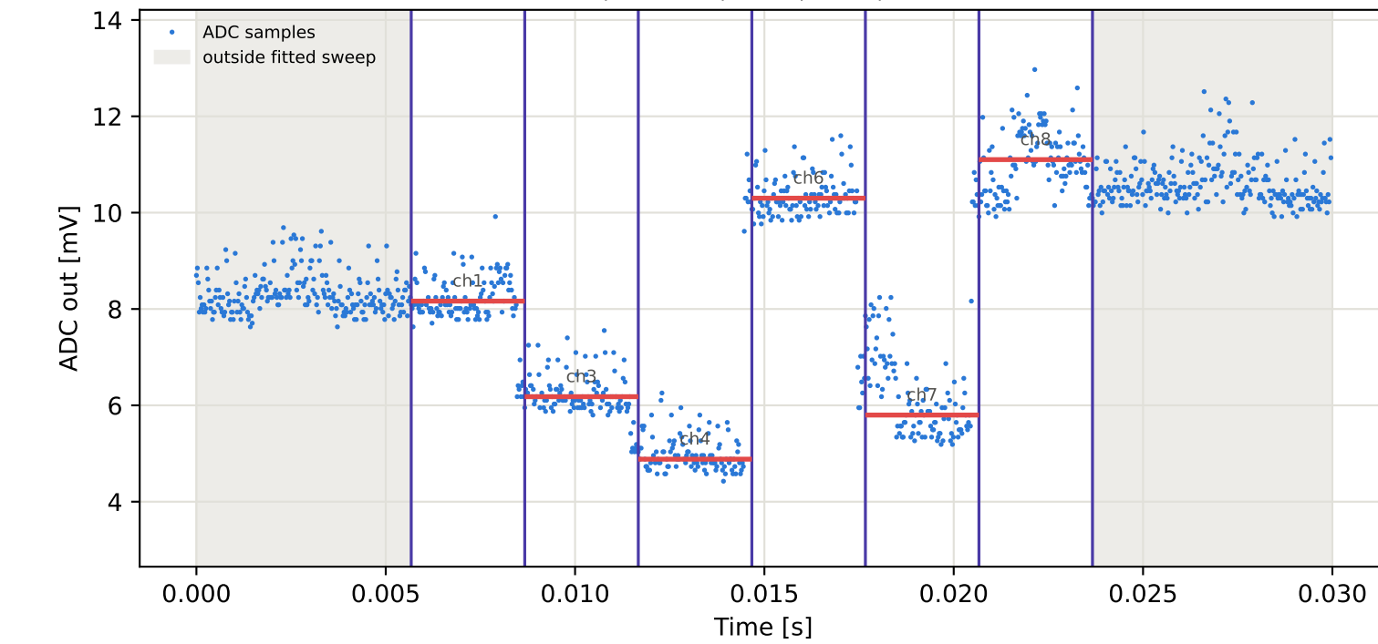
Tag2 &lt;- Tag15 | 955 MHz | run 0 | rep 1 | phase 133.00 deg
