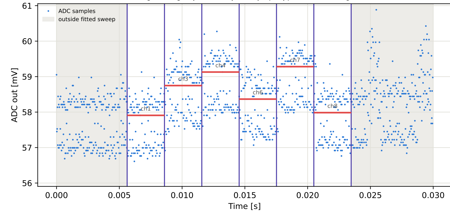
Tag2 &lt;- Tag16 | 805 MHz | run 0 | rep 1 | phase 128.11 deg
