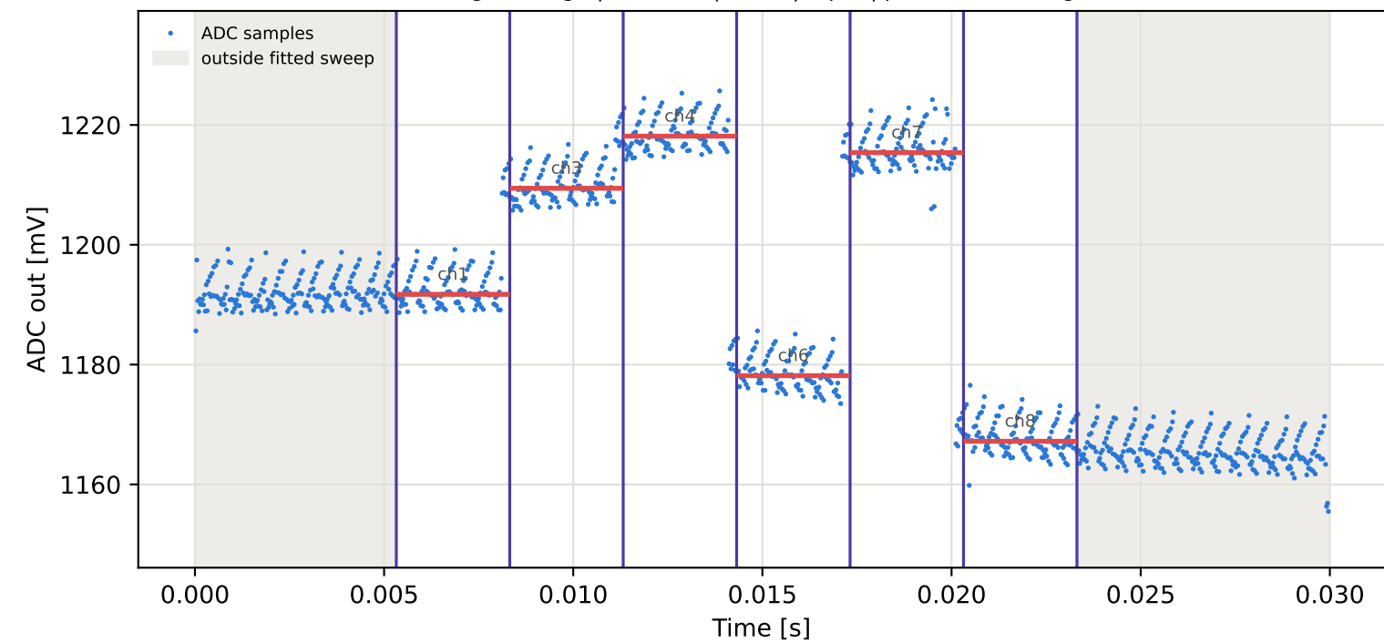
Tag4 &lt;- Tag8 | 905 MHz | run 0 | rep 1 | phase -109.92 deg
