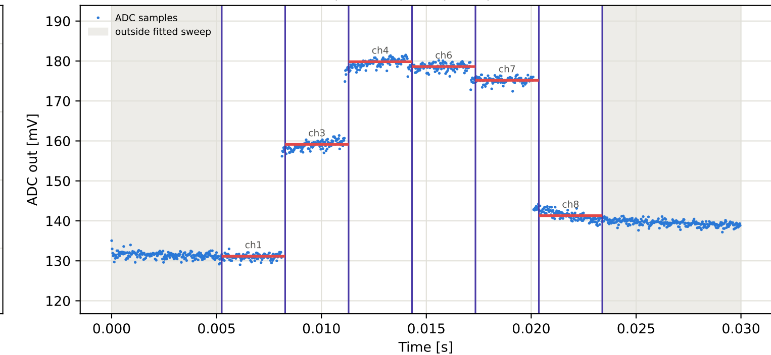
Tag6 &lt;- Tag10 | 885 MHz | run 0 | rep 1 | phase -109.70 deg
