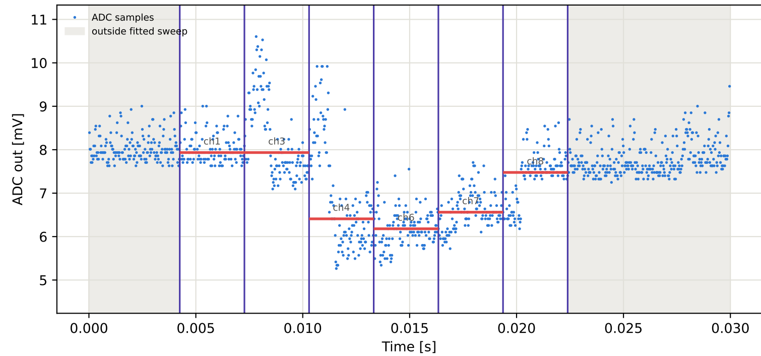
Tag2 &lt;- Tag6 | 955 MHz | run 0 | rep 1 | phase 178.28 deg
