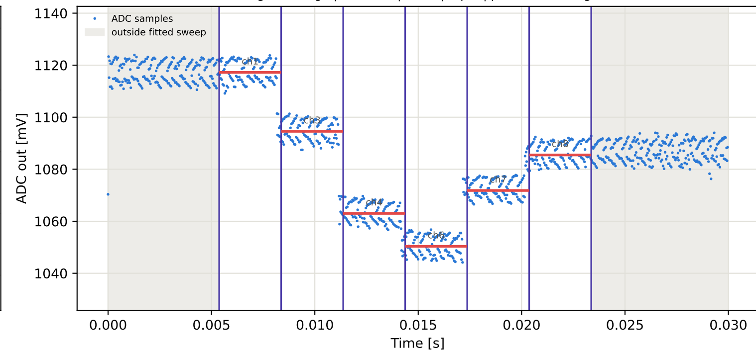
Tag16 &lt;- Tag7 | 885 MHz | run 0 | rep 1 | phase 50.30 deg
