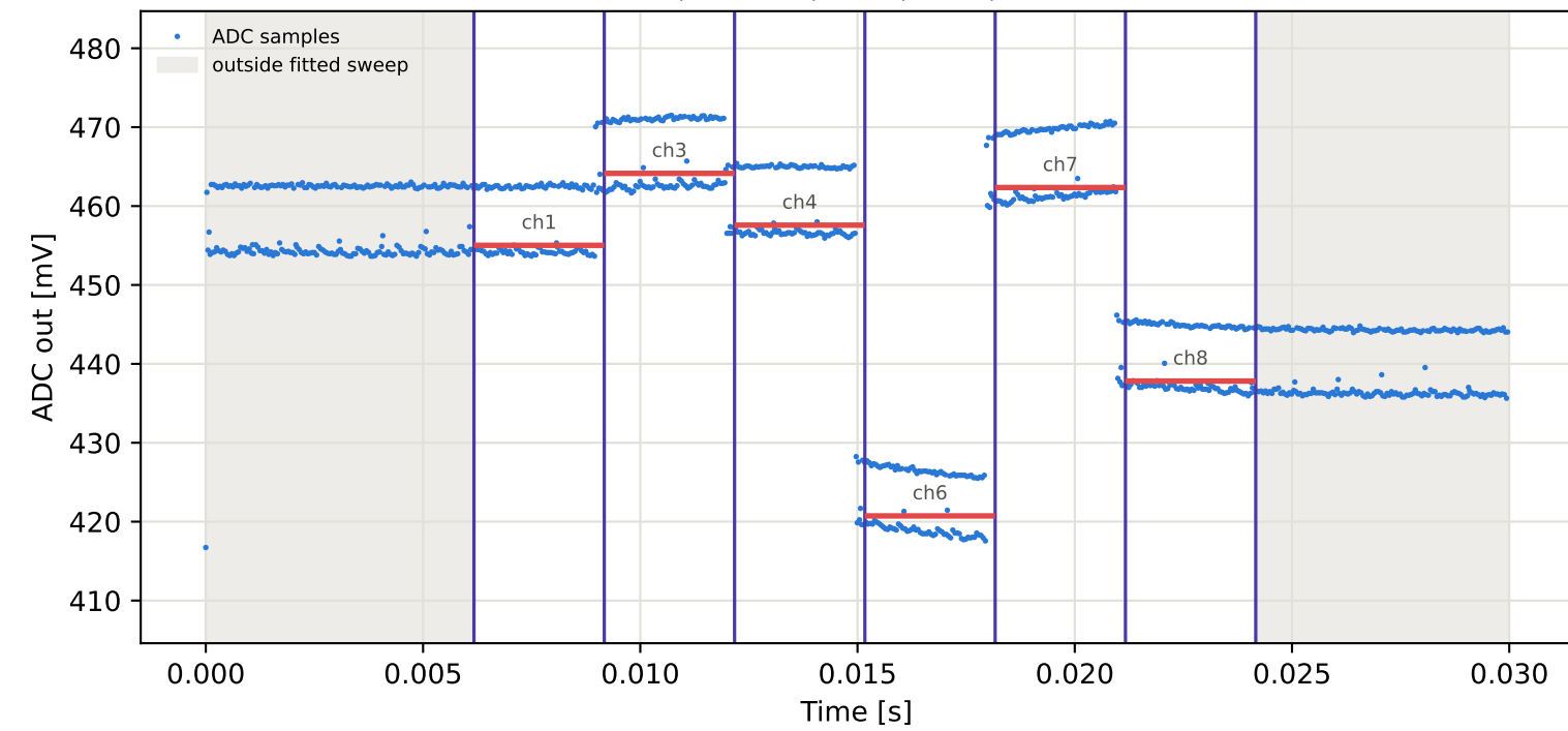
Tag9 &lt;- Tag7 | 945 MHz | run 0 | rep 1 | phase -2.87 deg
