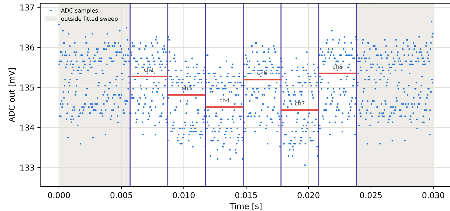
Tag6 &lt;- Tag5 | 805 MHz | run 0 | rep 1 | phase 123.21 deg
