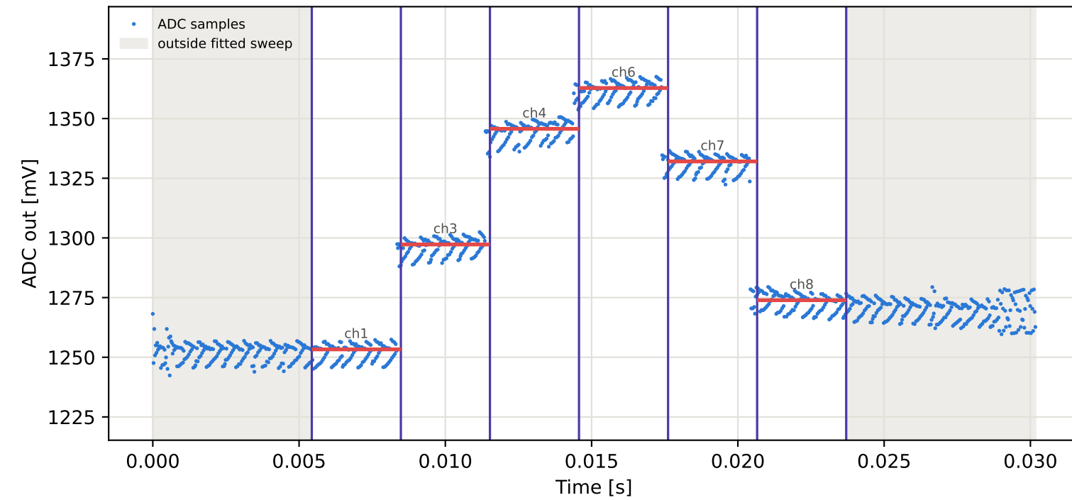
Tag16 &lt;- Tag6 | 895 MHz | run 0 | rep 1 | phase -128.01 deg
