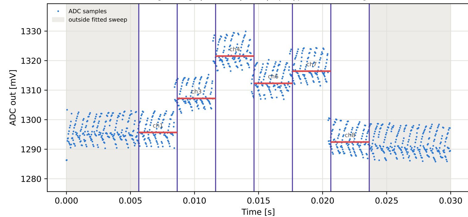
Tag4 &lt;- Tag15 | 915 MHz | run 0 | rep 1 | phase 77.26 deg
