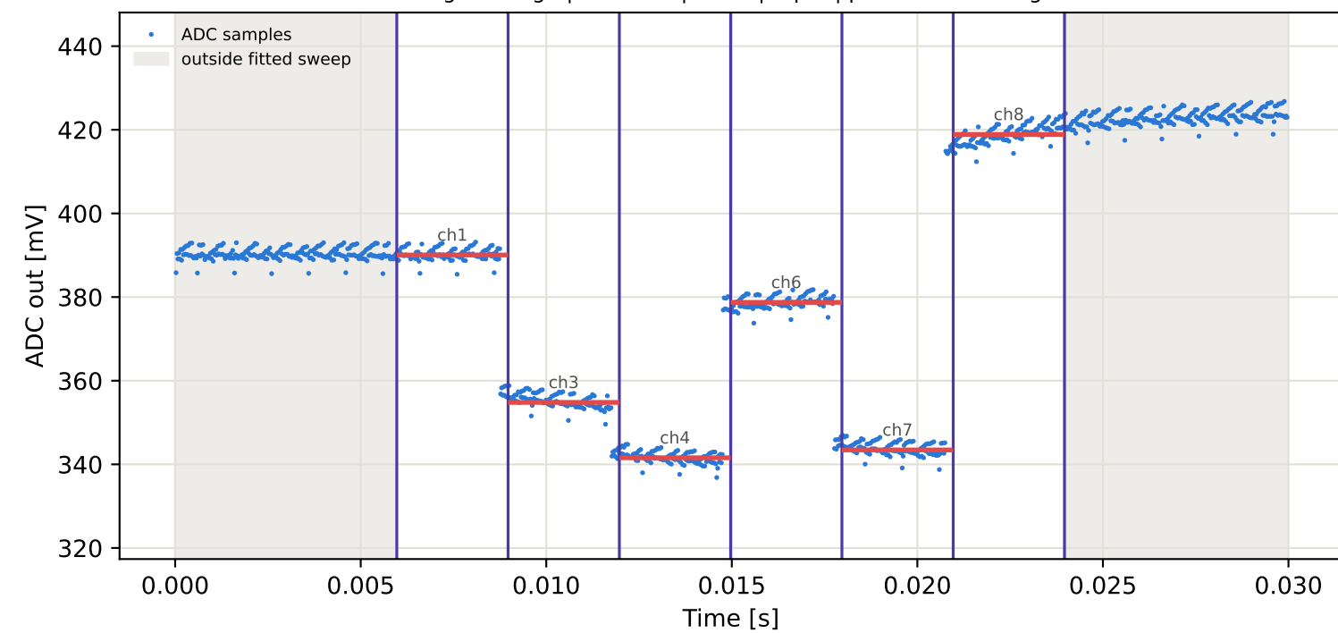
Tag8 &lt;- Tag10 | 895 MHz | run 0 | rep 1 | phase -85.24 deg
