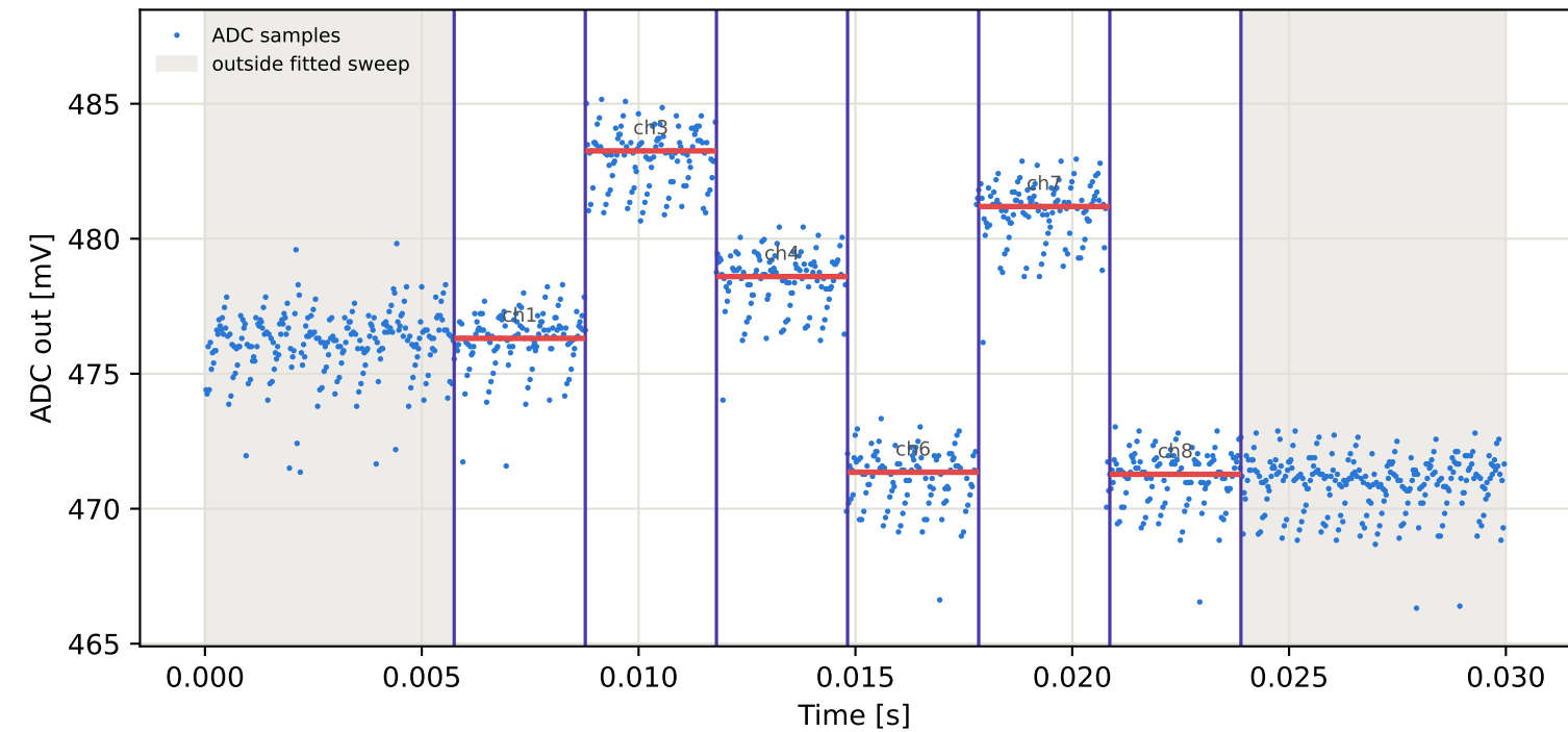
Tag6 &lt;- Tag10 | 855 MHz | run 0 | rep 1 | phase -179.22 deg
