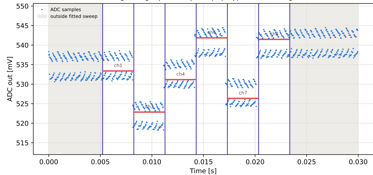
Tag5 &lt;- Tag2 | 835 MHz | run 0 | rep 1 | phase 127.62 deg
