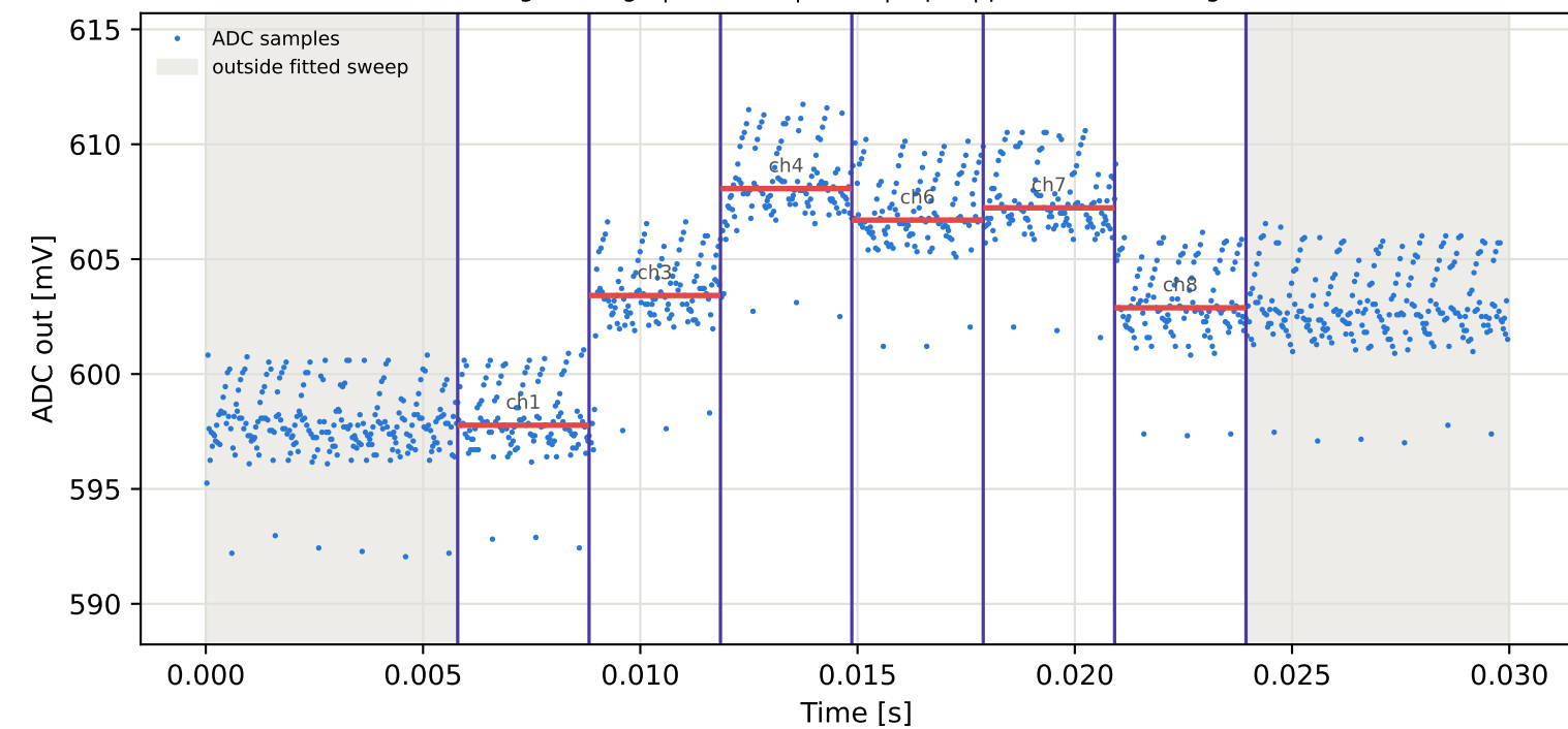
Tag7 &lt;- Tag5 | 855 MHz | run 0 | rep 1 | phase -109.71 deg
