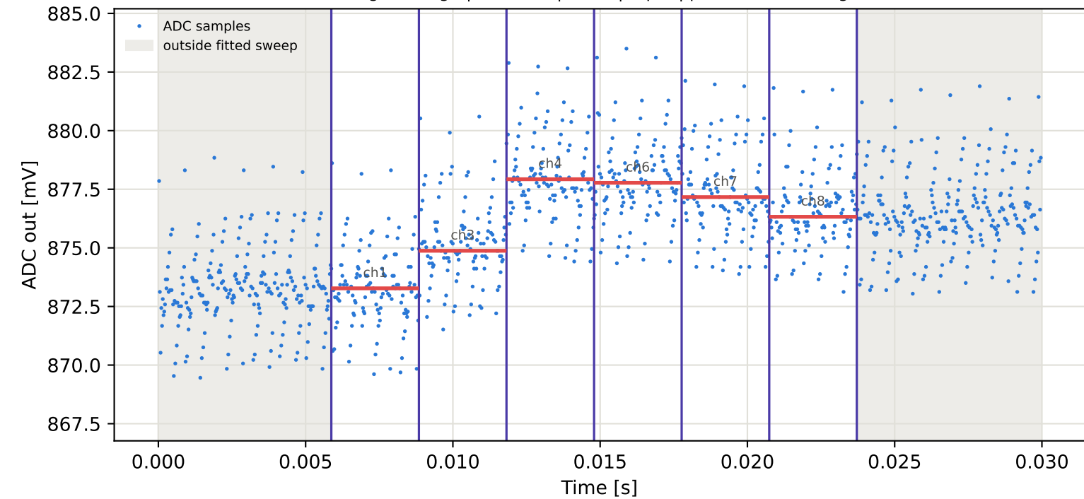
Tag8 &lt;- Tag15 | 865 MHz | run 0 | rep 1 | phase 93.94 deg
