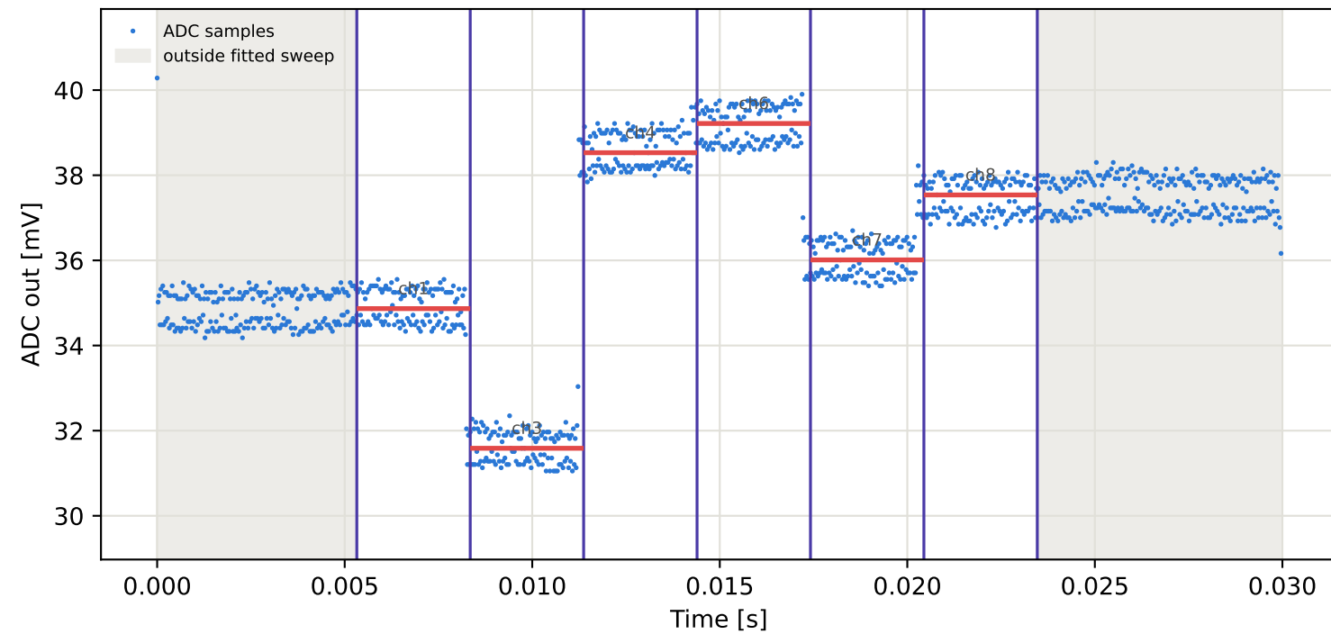
Tag8 &lt;- Tag1 | 785 MHz | run 0 | rep 1 | phase 54.38 deg
