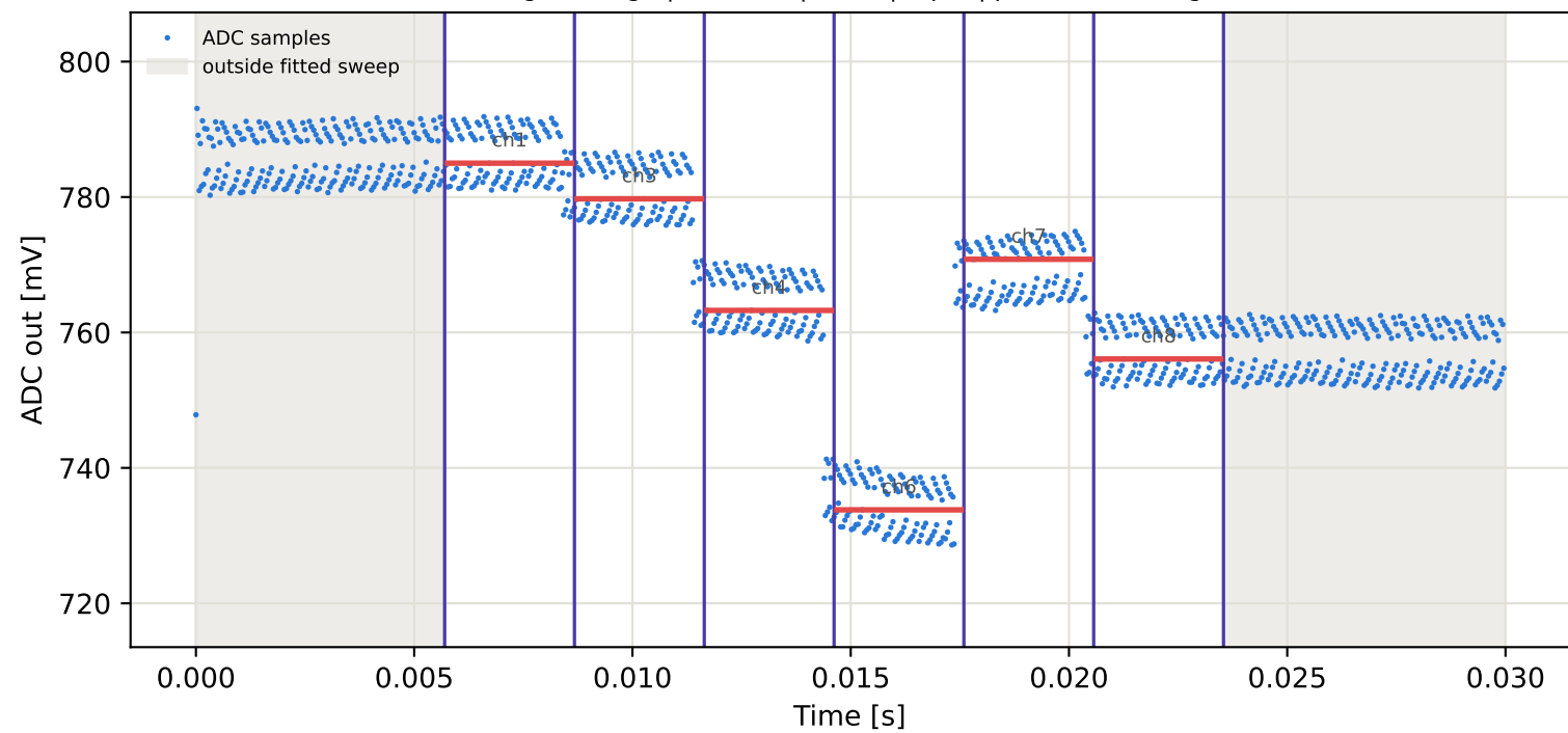
Tag3 &lt;- Tag15 | 895 MHz | run 0 | rep 1 | phase -10.80 deg
