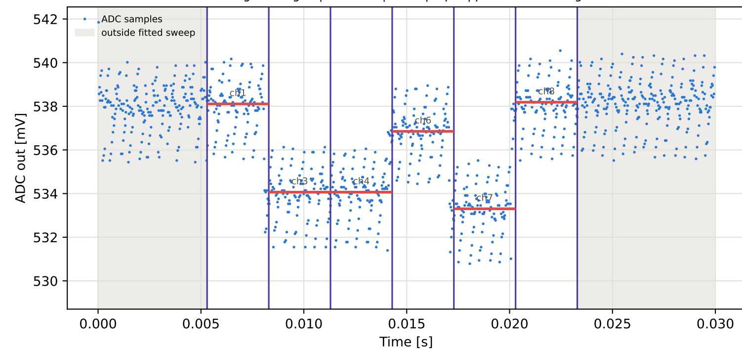
Tag5 &lt;- Tag16 | 835 MHz | run 0 | rep 1 | phase -147.65 deg
