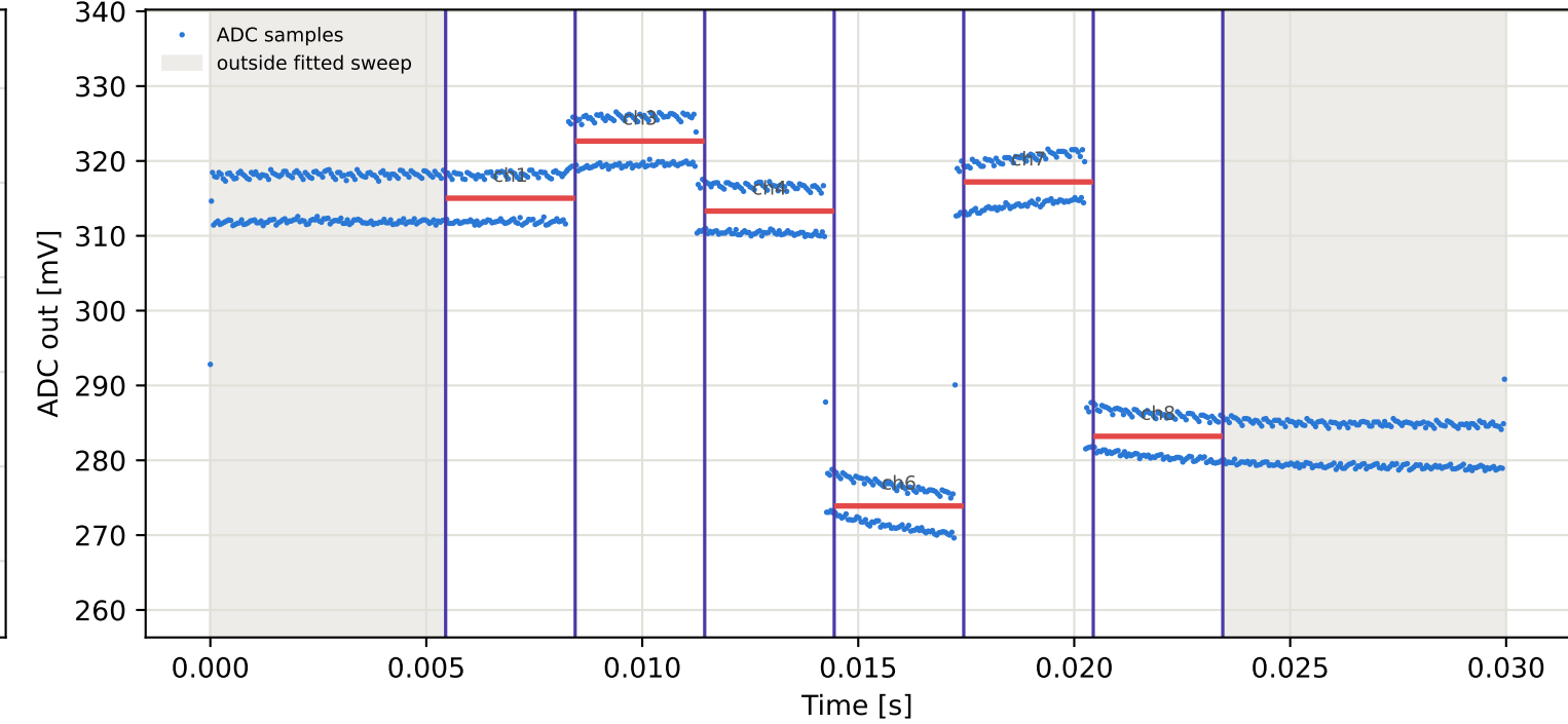
Tag3 &lt;- Tag2 | 905 MHz | run 0 | rep 1 | phase 126.09 deg
