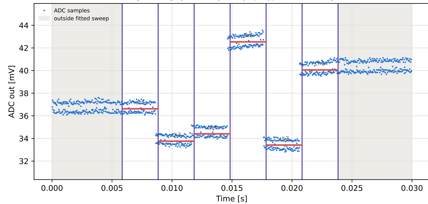
Tag10 &lt;- Tag9 | 975 MHz | run 0 | rep 1 | phase -27.34 deg
