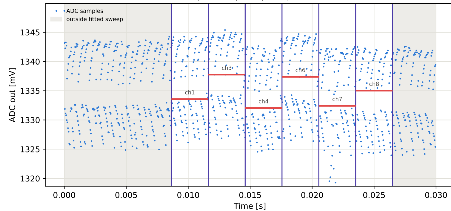
Tag16 &lt;- Tag4 | 965 MHz | run 0 | rep 1 | phase 81.57 deg
