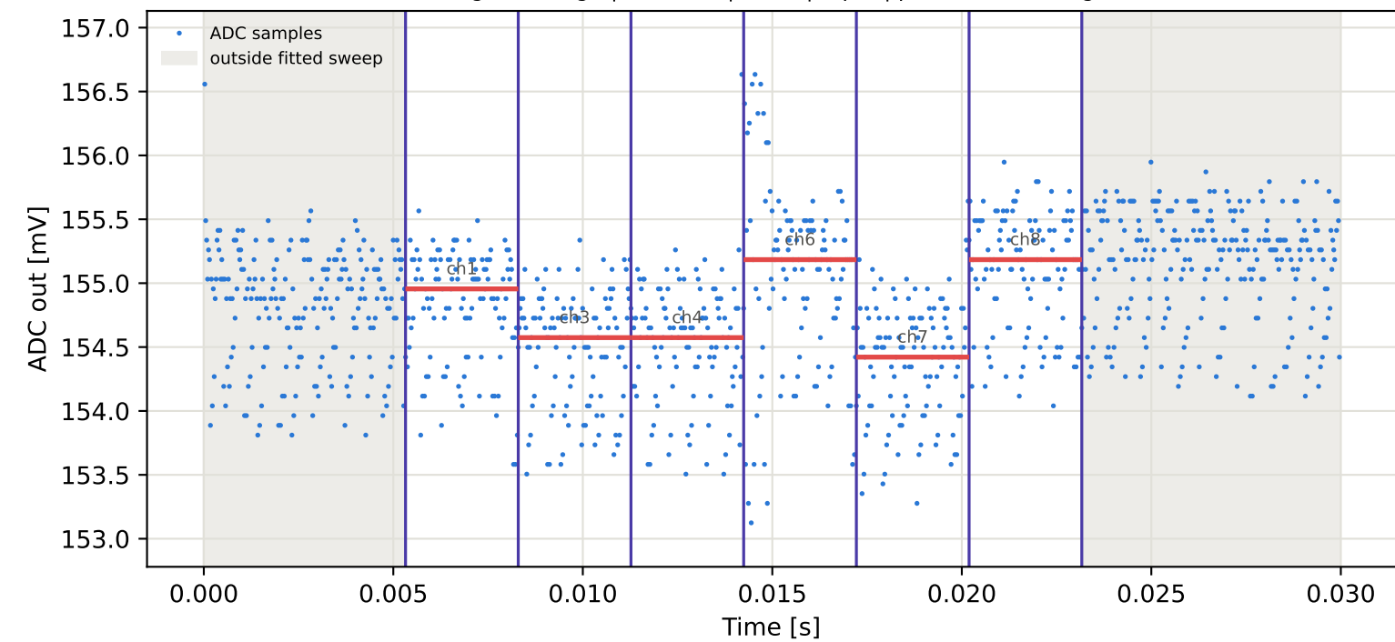
Tag16 &lt;- Tag4 | 795 MHz | run 0 | rep 1 | phase 82.30 deg
