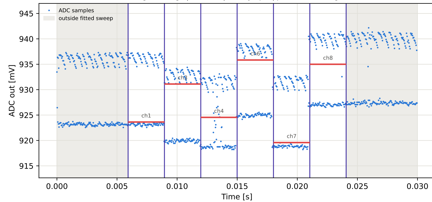
Tag16 &lt;- Tag4 | 845 MHz | run 0 | rep 1 | phase 142.38 deg
