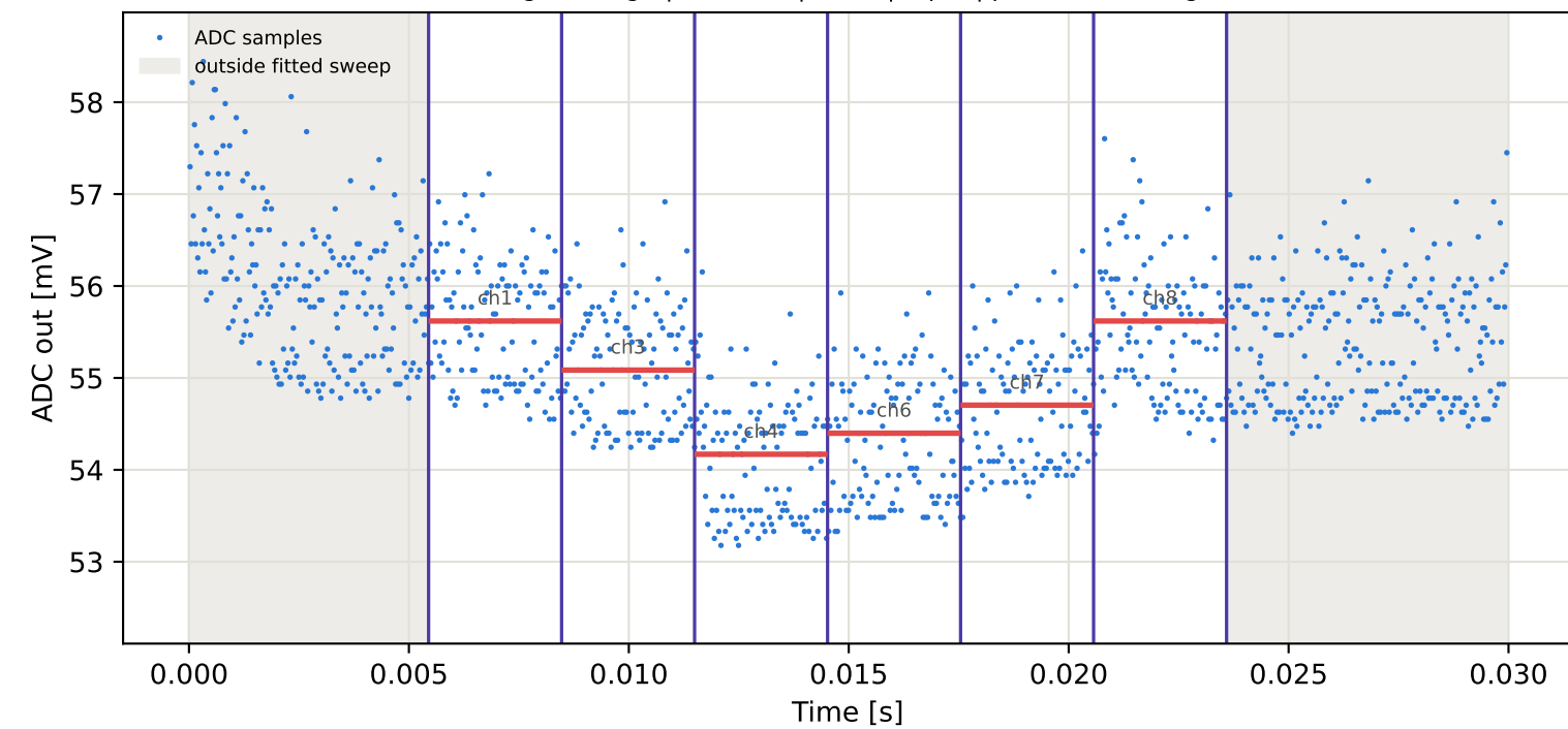
Tag2 &lt;- Tag5 | 945 MHz | run 0 | rep 1 | phase 29.51 deg
