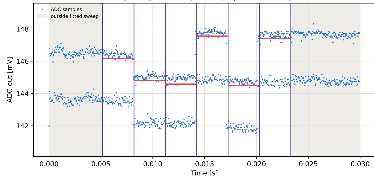
Tag3 &lt;- Tag2 | 785 MHz | run 0 | rep 1 | phase 158.38 deg
