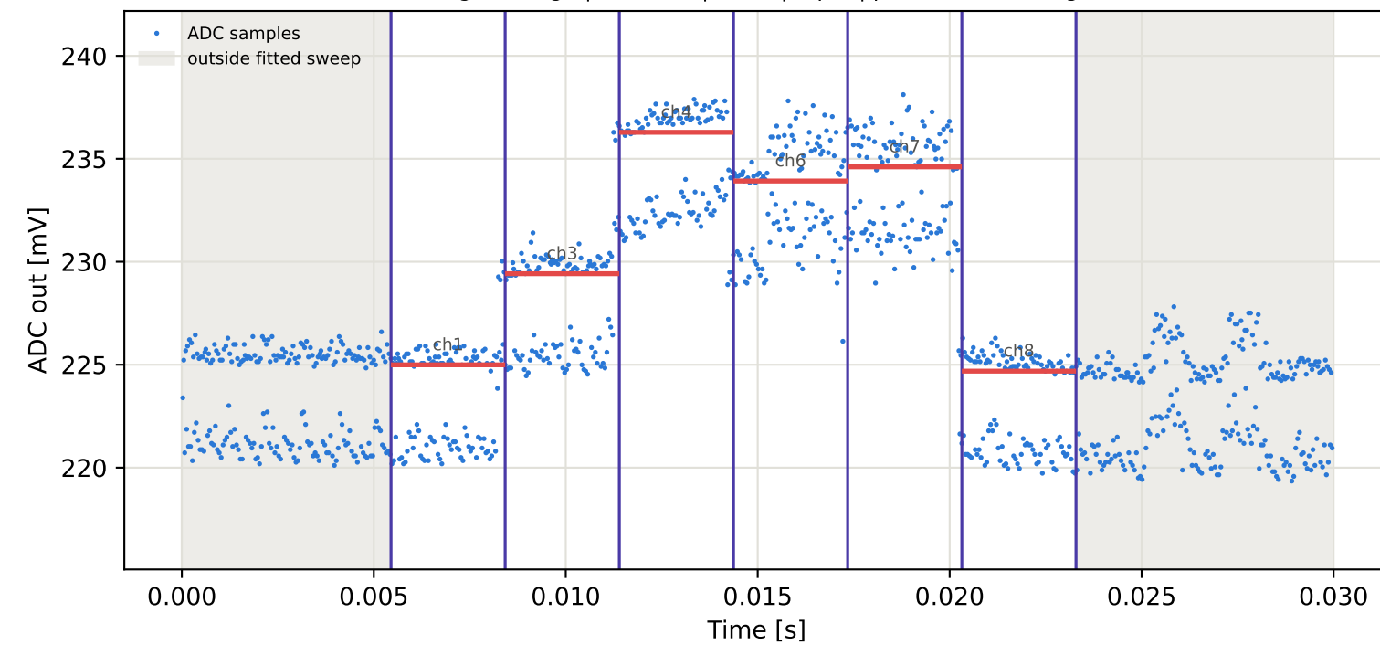
Tag3 &lt;- Tag10 | 925 MHz | run 0 | rep 1 | phase 90.25 deg
