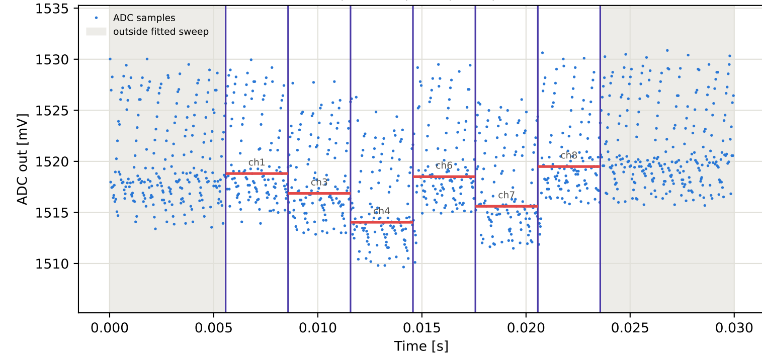
Tag15 &lt;- Tag10 | 965 MHz | run 0 | rep 1 | phase 98.58 deg
