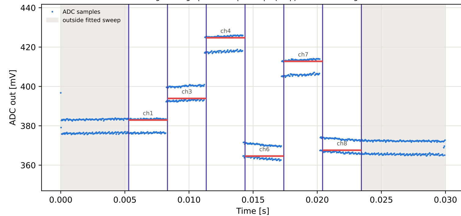
Tag3 &lt;- Tag6 | 985 MHz | run 0 | rep 1 | phase 84.74 deg
