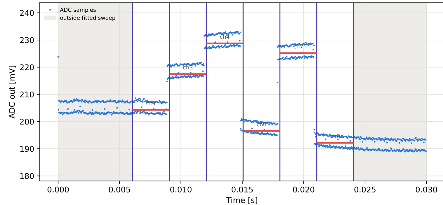
Tag1 &lt;- Tag3 | 925 MHz | run 0 | rep 1 | phase 32.51 deg
