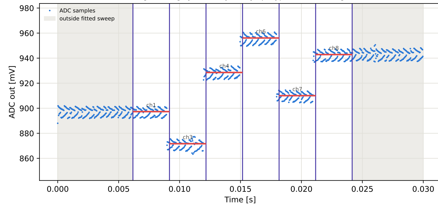
Tag2 &lt;- Tag1 | 835 MHz | run 0 | rep 1 | phase 111.85 deg
