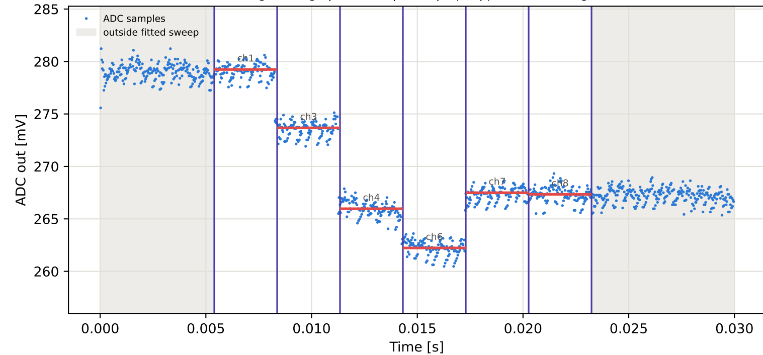
Tag2 &lt;- Tag7 | 865 MHz | run 0 | rep 1 | phase 90.30 deg
