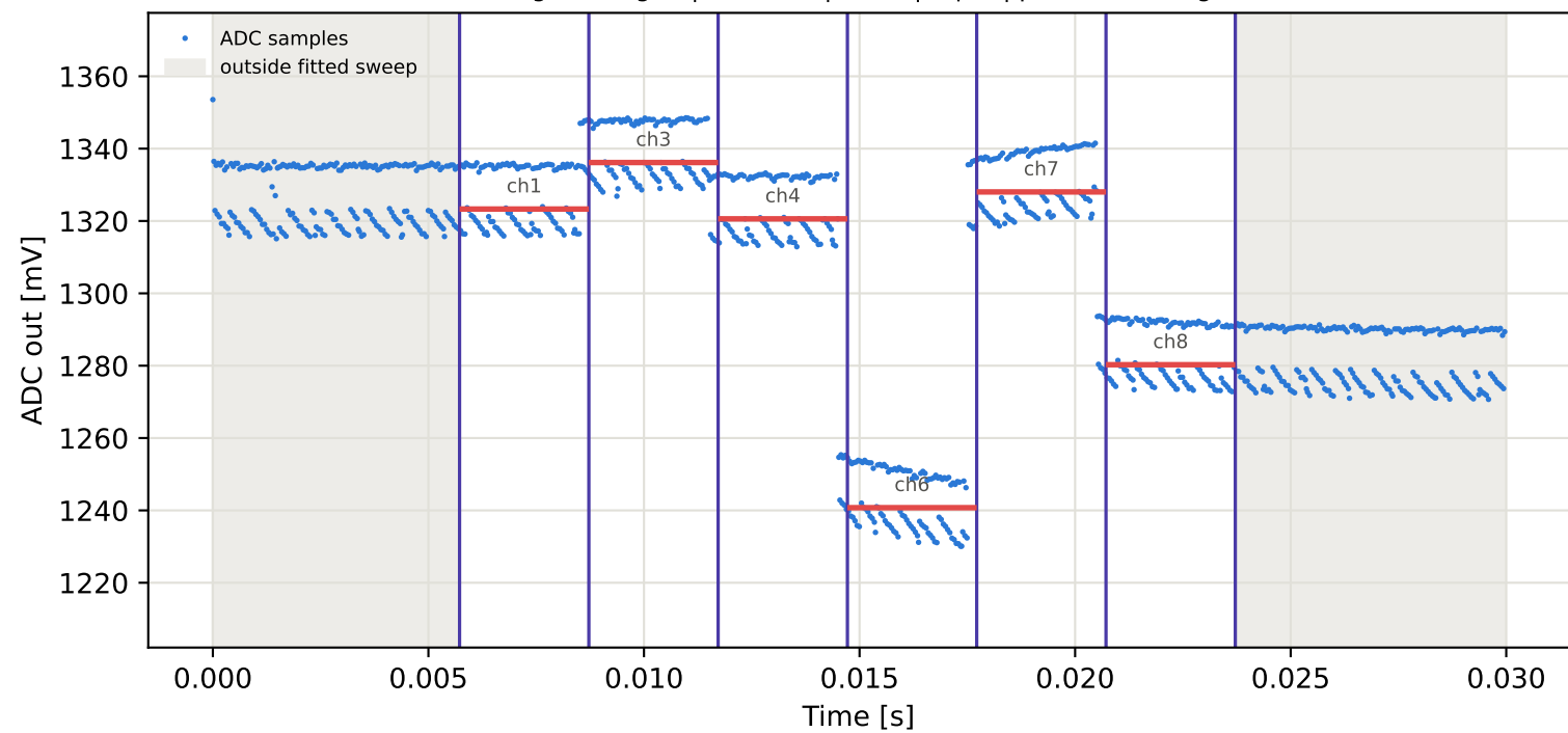
Tag4 &lt;- Tag3 | 915 MHz | run 0 | rep 1 | phase -142.47 deg
