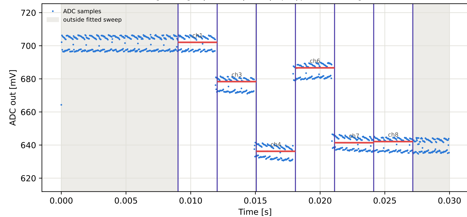
Tag7 &lt;- Tag3 | 865 MHz | run 0 | rep 1 | phase 178.41 deg
