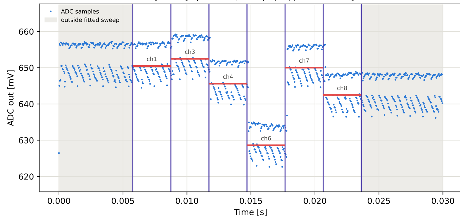
Tag6 &lt;- Tag5 | 955 MHz | run 0 | rep 1 | phase 12.35 deg
