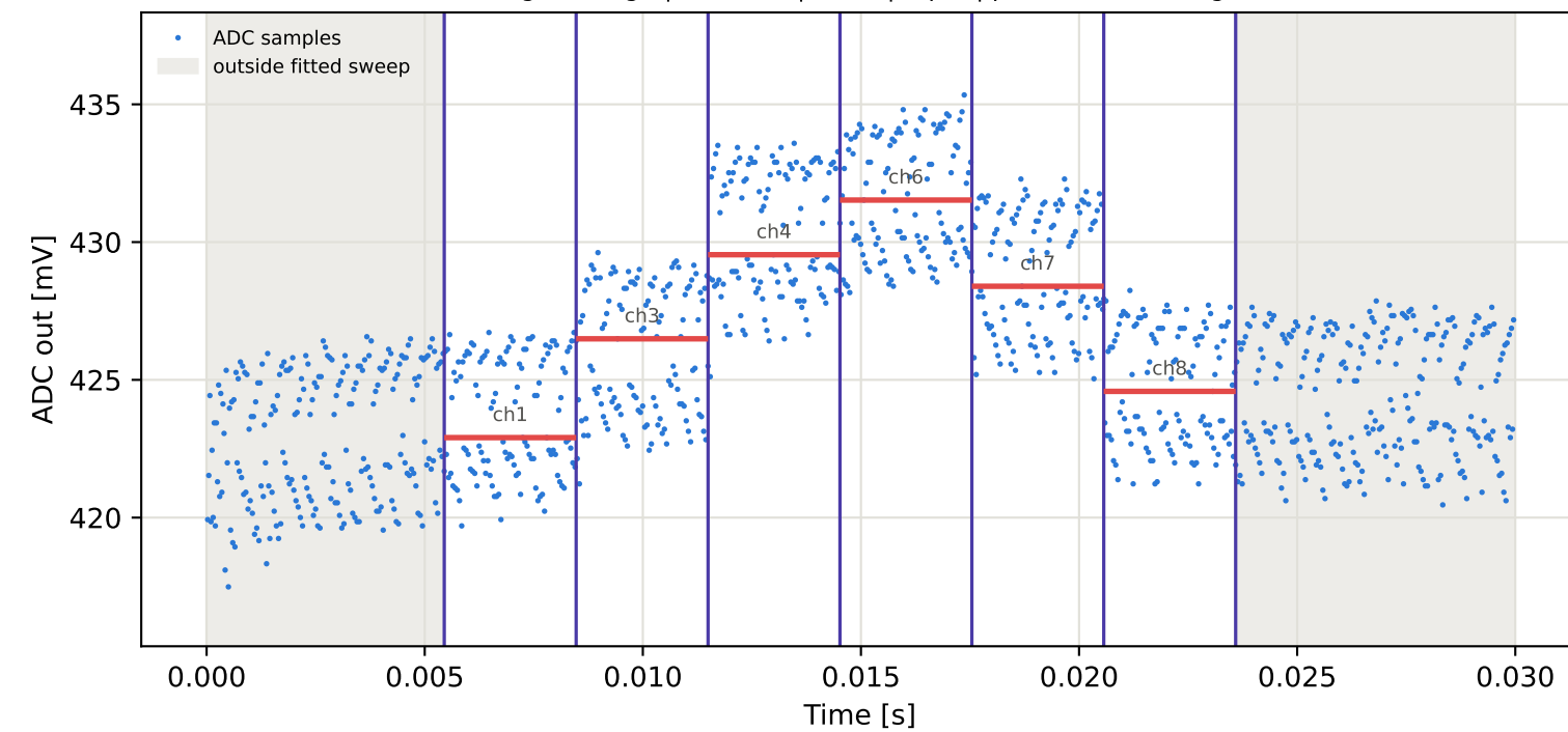
Tag2 &lt;- Tag5 | 915 MHz | run 0 | rep 1 | phase 178.85 deg
