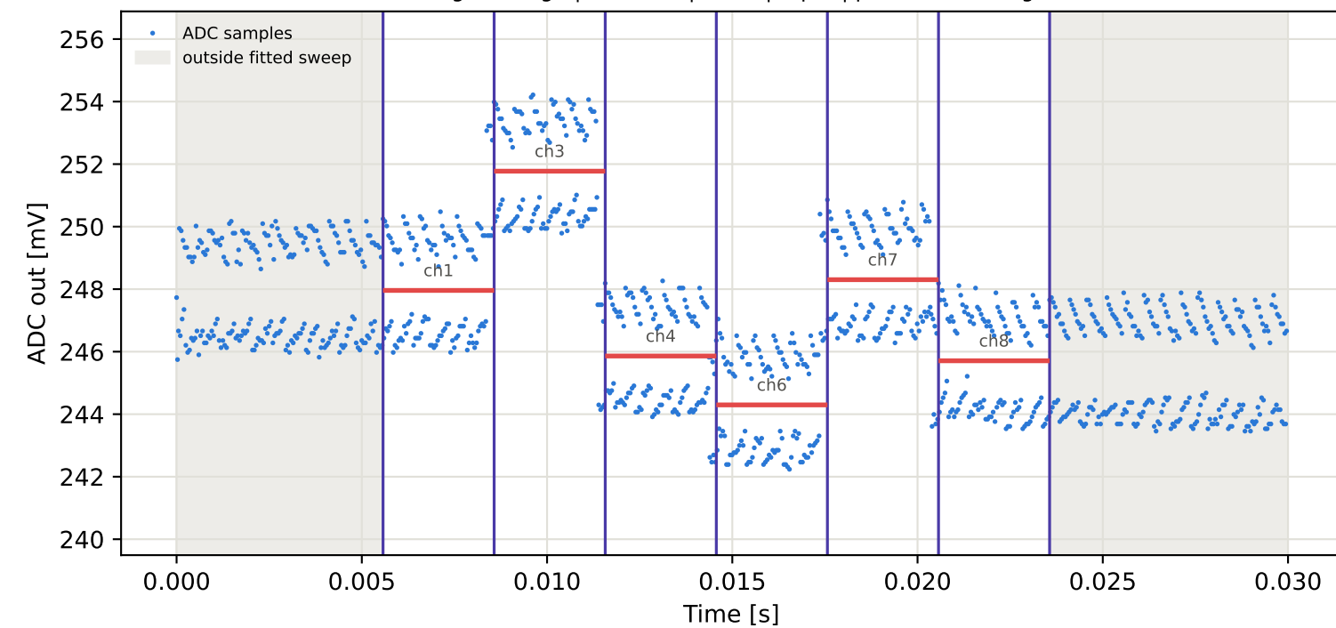
Tag6 &lt;- Tag1 | 825 MHz | run 0 | rep 1 | phase 30.96 deg
