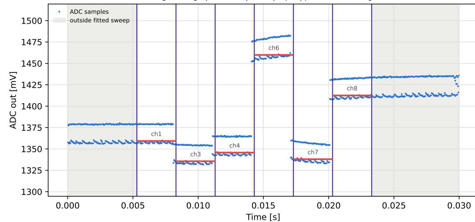
Tag4 &lt;- Tag9 | 935 MHz | run 0 | rep 1 | phase 174.27 deg
