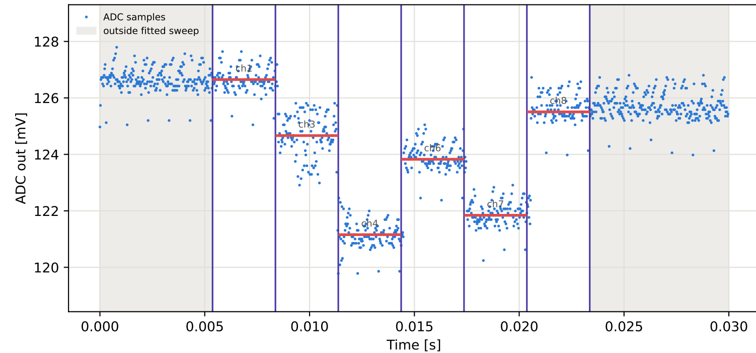
Tag4 &lt;- Tag9 | 805 MHz | run 0 | rep 1 | phase 50.05 deg
