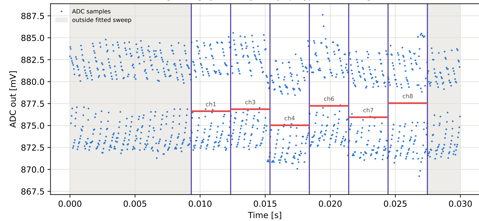
Tag8 &lt;- Tag4 | 955 MHz | run 0 | rep 1 | phase 157.38 deg
