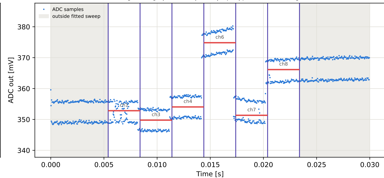
Tag2 &lt;- Tag8 | 905 MHz | run 0 | rep 1 | phase 6.86 deg
