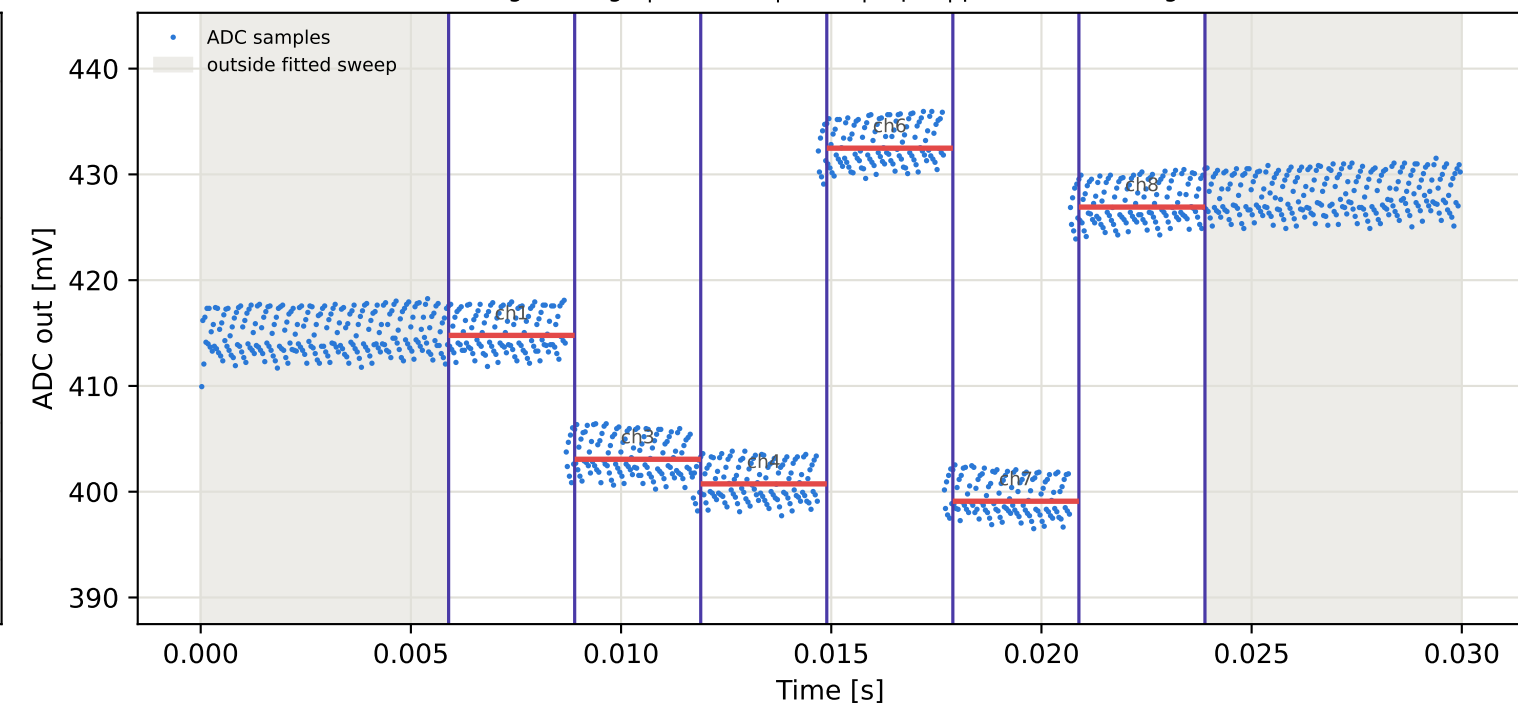
Tag3 &lt;- Tag9 | 985 MHz | run 0 | rep 1 | phase 148.06 deg
