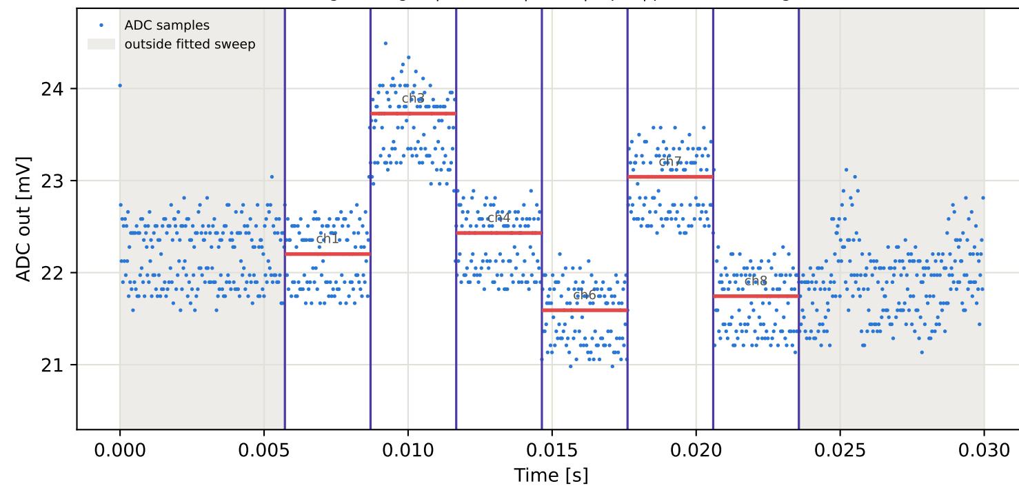
Tag5 &lt;- Tag16 | 805 MHz | run 0 | rep 1 | phase -173.08 deg
