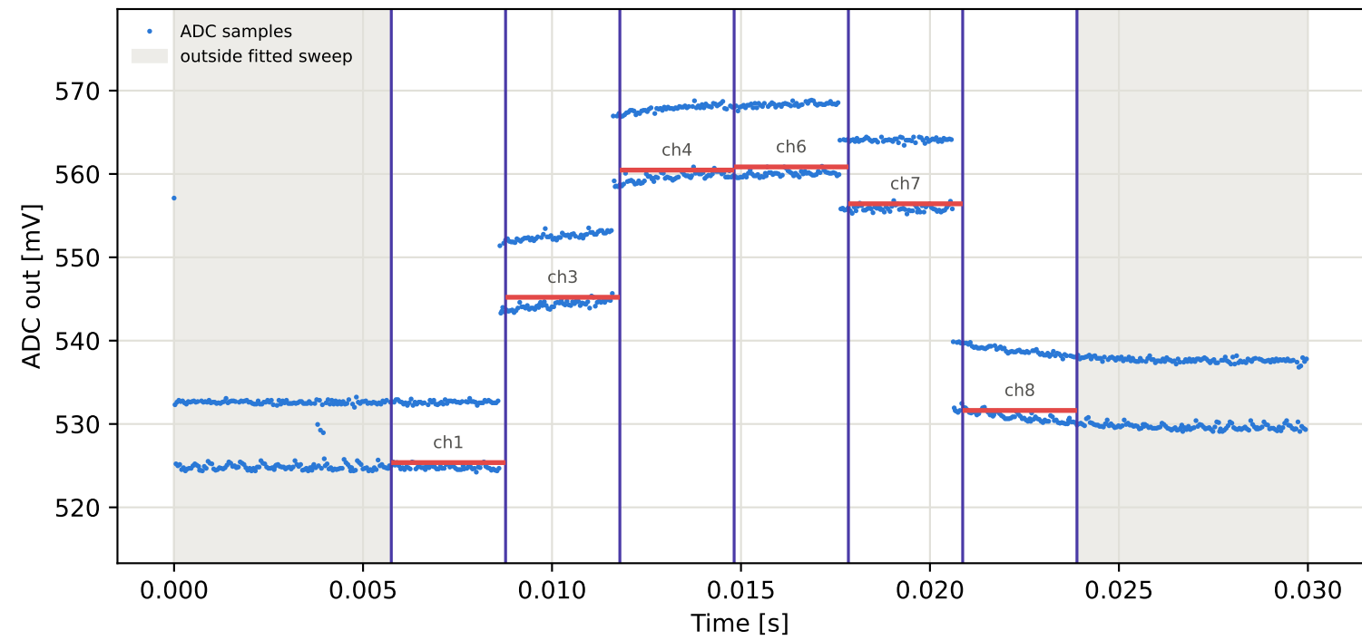
Tag10 &lt;- Tag3 | 875 MHz | run 0 | rep 1 | phase 178.32 deg
