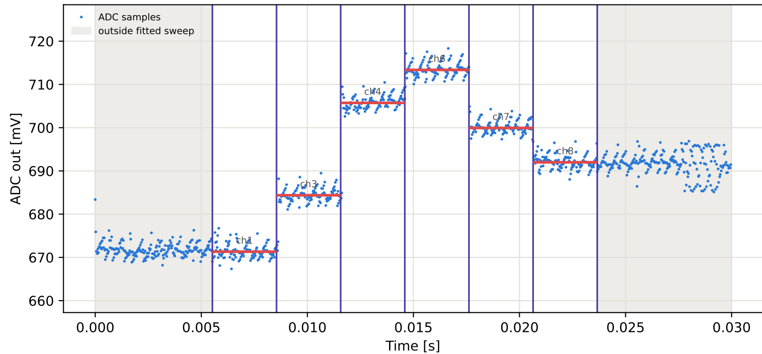
Tag6 &lt;- Tag5 | 875 MHz | run 0 | rep 1 | phase 59.63 deg
