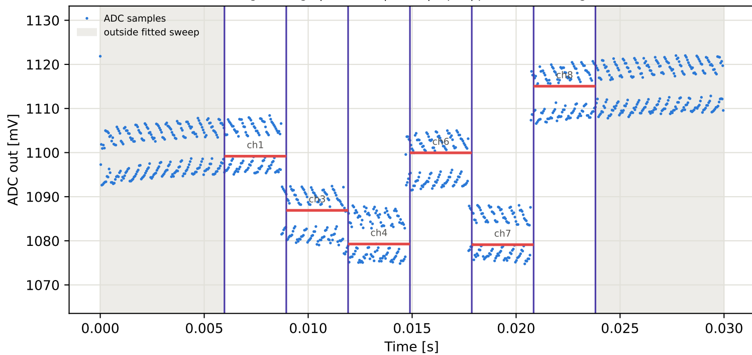
Tag5 &lt;- Tag8 | 875 MHz | run 0 | rep 1 | phase 52.27 deg
