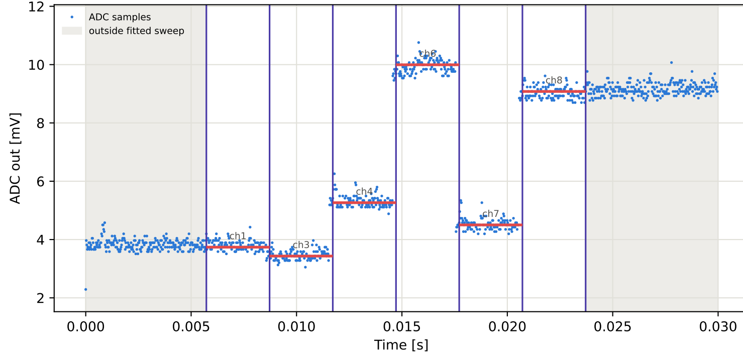
Tag1 &lt;- Tag3 | 875 MHz | run 0 | rep 1 | phase -50.39 deg
