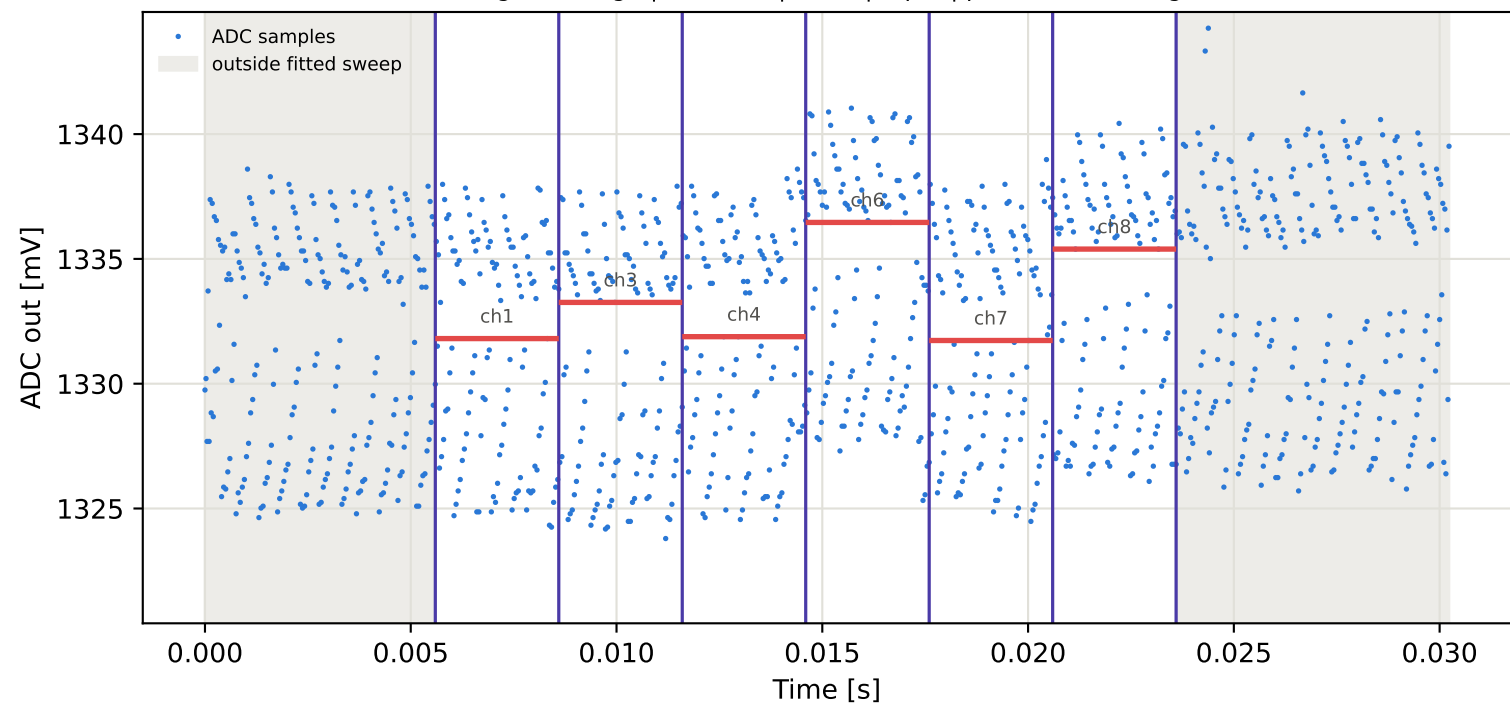
Tag15 &lt;- Tag4 | 895 MHz | run 0 | rep 1 | phase -135.54 deg
