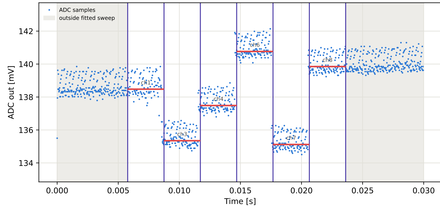
Tag3 &lt;- Tag2 | 775 MHz | run 0 | rep 1 | phase 115.77 deg
