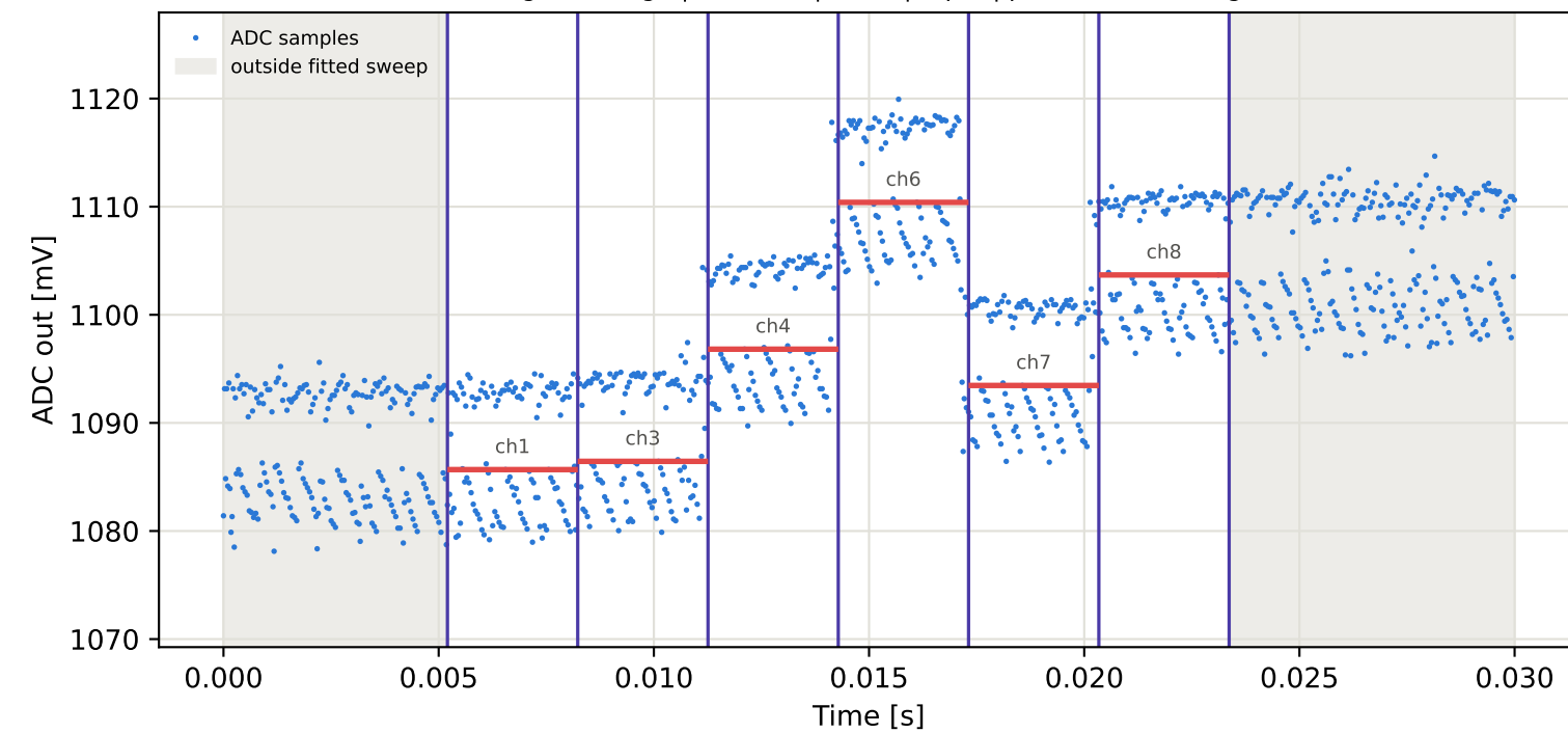
Tag15 &lt;- Tag9 | 885 MHz | run 0 | rep 1 | phase 62.80 deg
