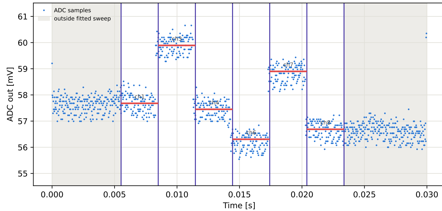
Tag5 &lt;- Tag16 | 795 MHz | run 0 | rep 1 | phase 131.48 deg
