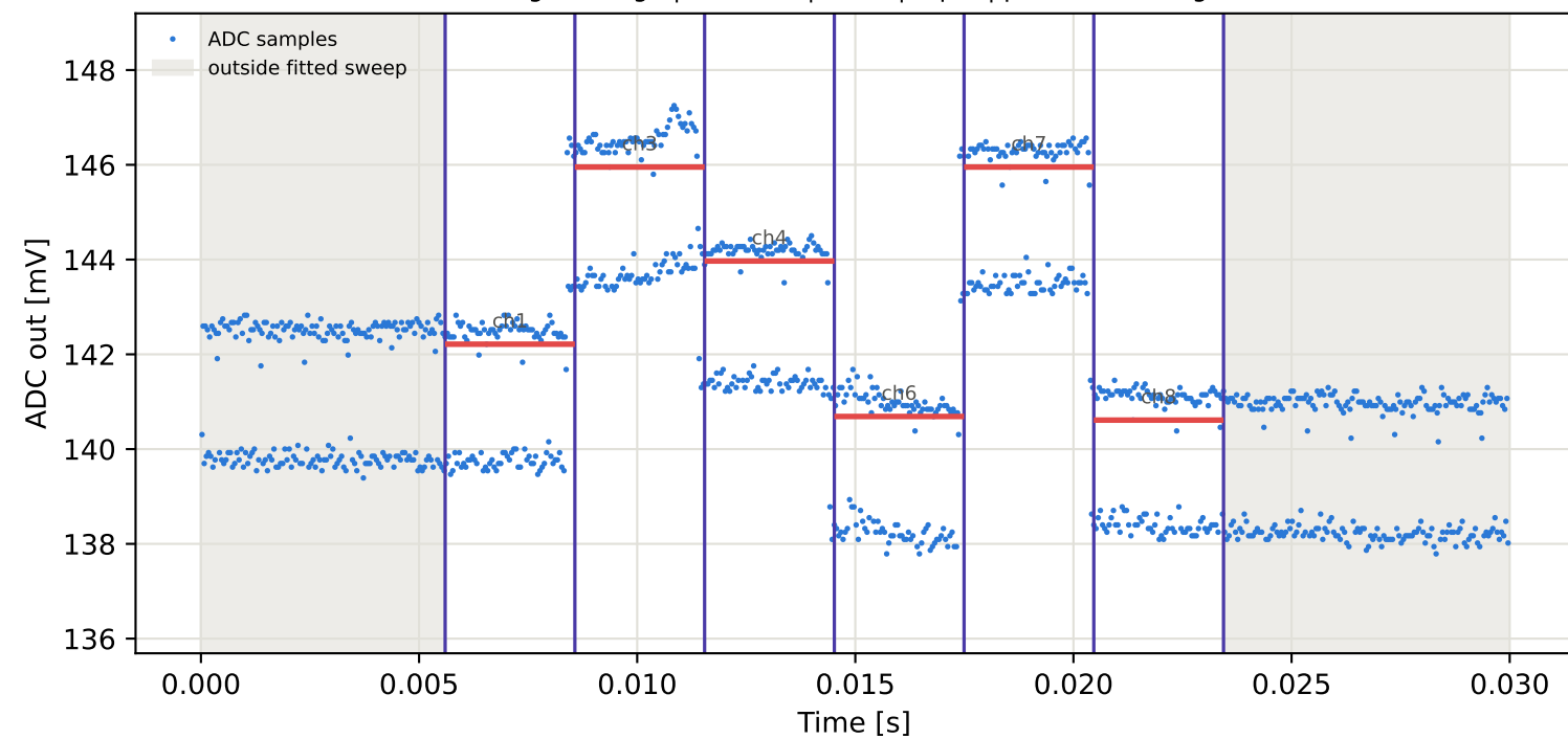
Tag3 &lt;- Tag9 | 785 MHz | run 0 | rep 1 | phase -8.40 deg
