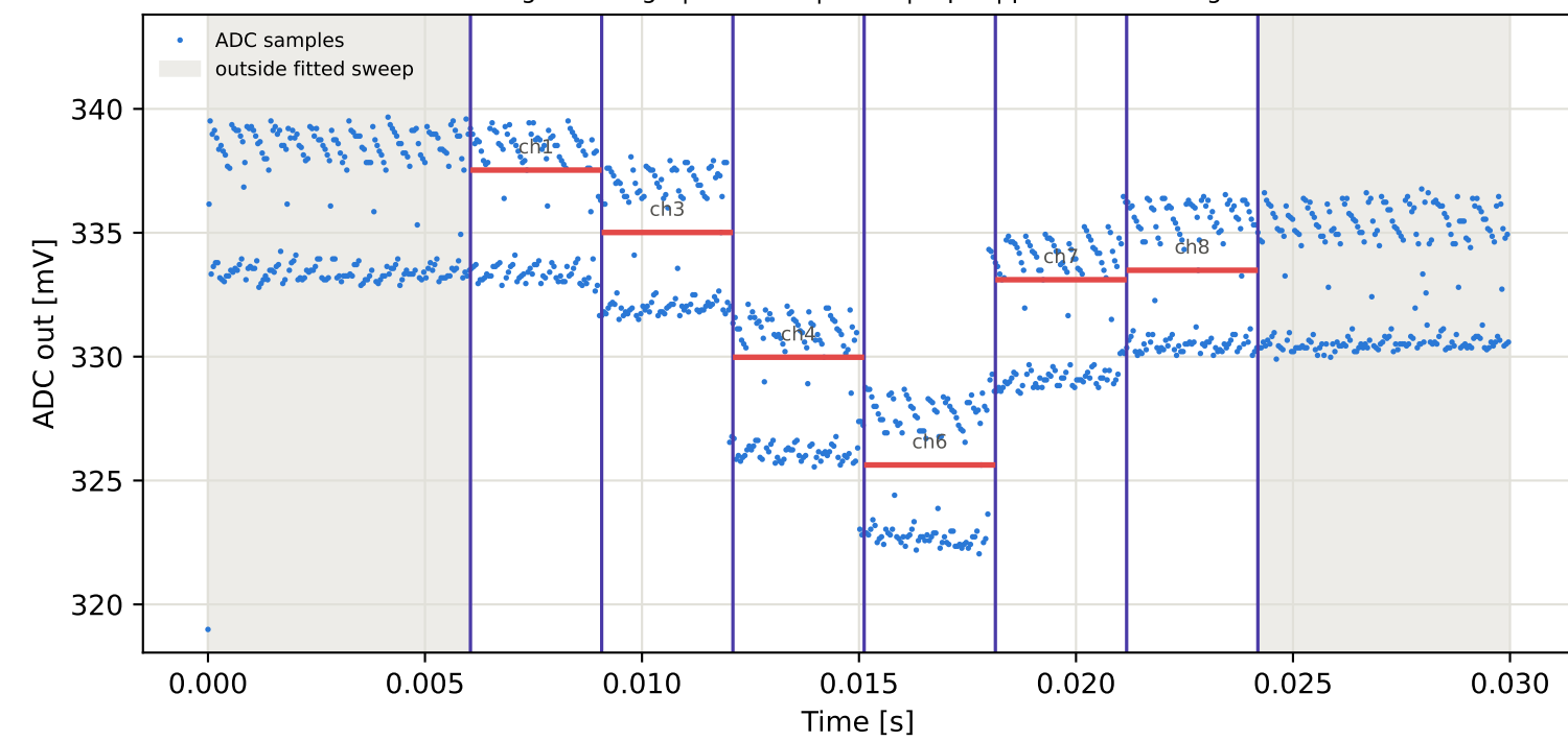
Tag10 &lt;- Tag9 | 935 MHz | run 0 | rep 1 | phase -125.32 deg
