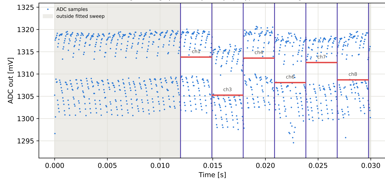
Tag16 &lt;- Tag4 | 985 MHz | run 0 | rep 1 | phase 57.35 deg
