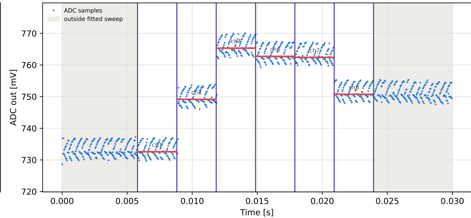
Tag8 &lt;- Tag7 | 855 MHz | run 0 | rep 1 | phase -171.69 deg
