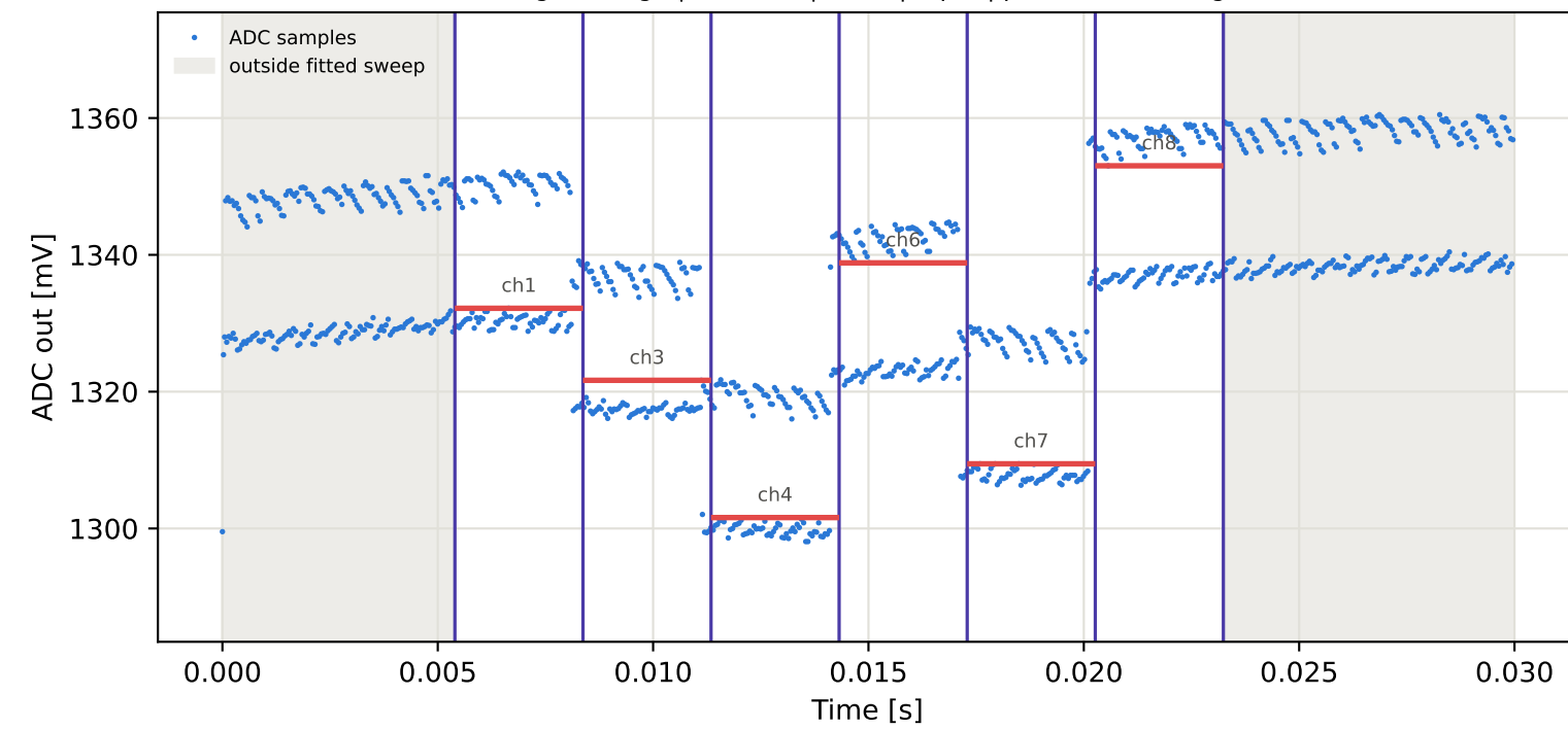
Tag9 &lt;- Tag10 | 935 MHz | run 0 | rep 1 | phase 175.23 deg
