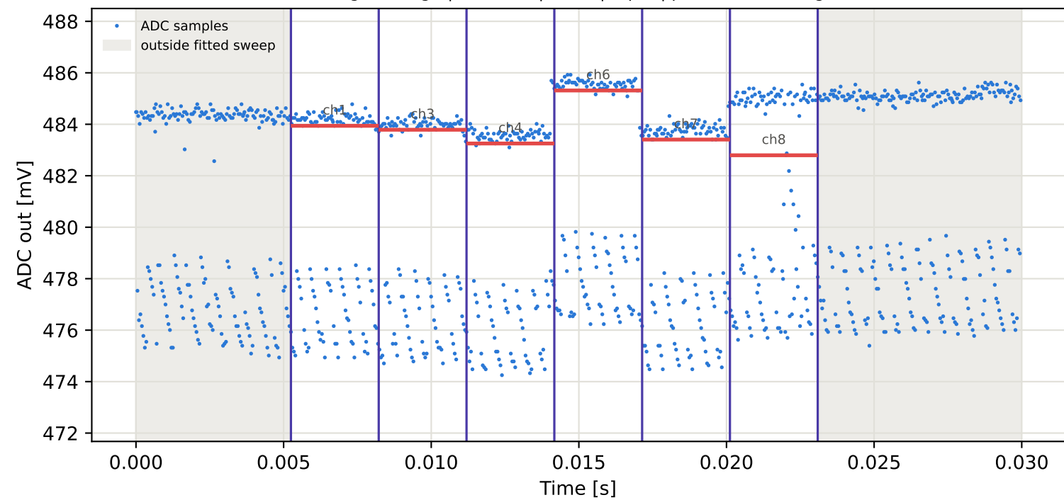
Tag7 &lt;- Tag4 | 975 MHz | run 0 | rep 1 | phase -39.81 deg
