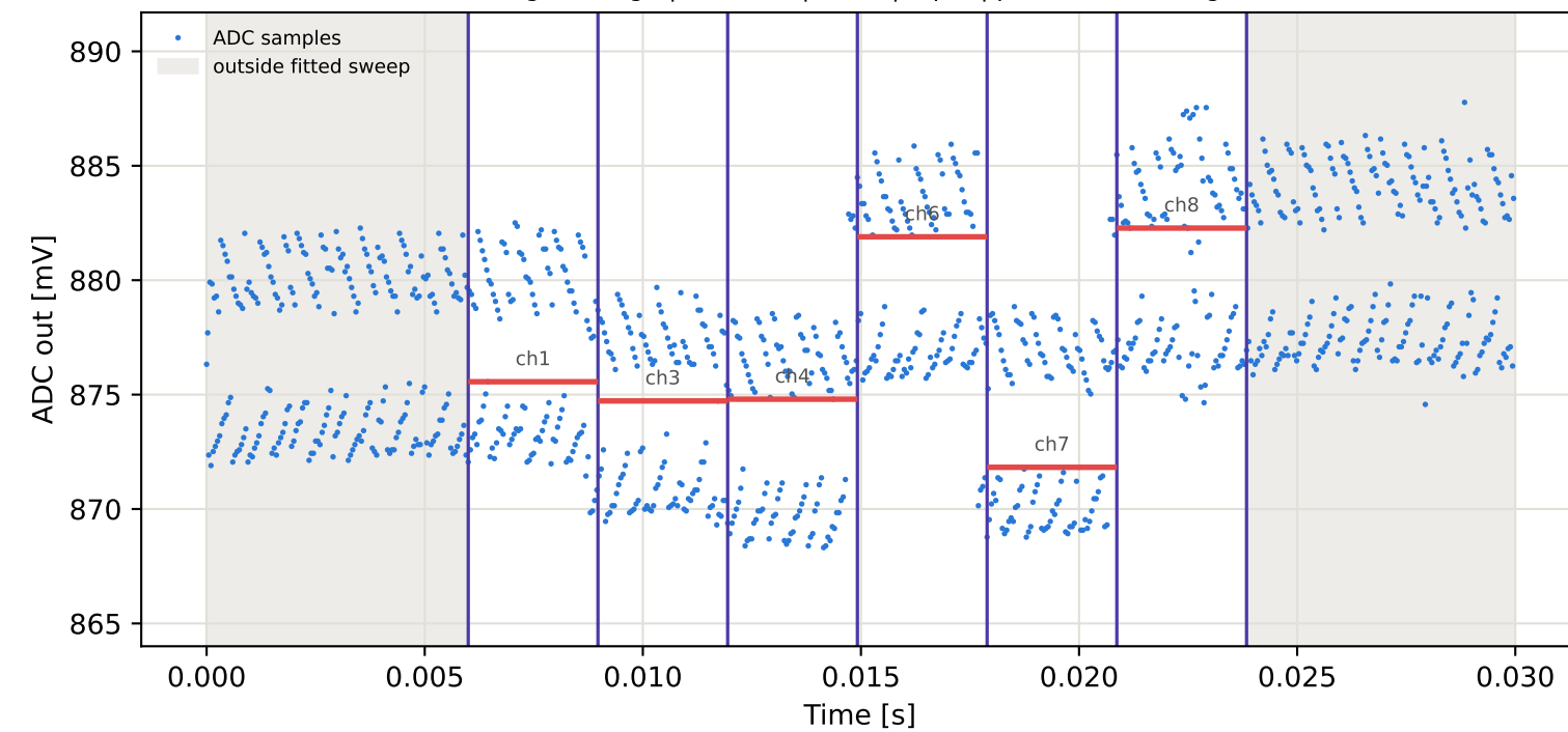
Tag8 &lt;- Tag4 | 865 MHz | run 0 | rep 1 | phase 24.58 deg
