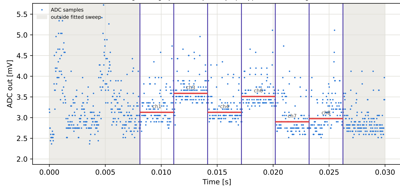
Tag2 &lt;- Tag8 | 795 MHz | run 0 | rep 1 | phase 143.06 deg
