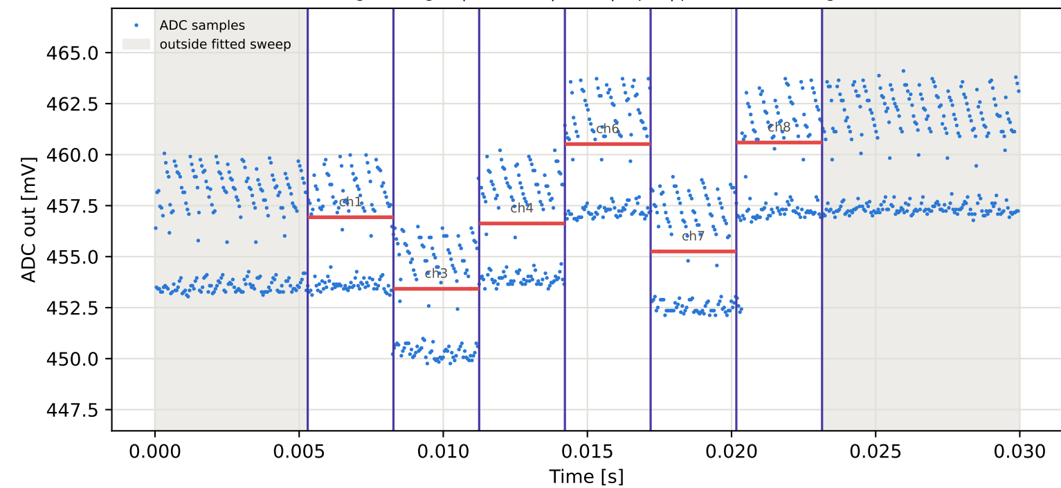
Tag5 &lt;- Tag16 | 845 MHz | run 0 | rep 1 | phase -99.22 deg
