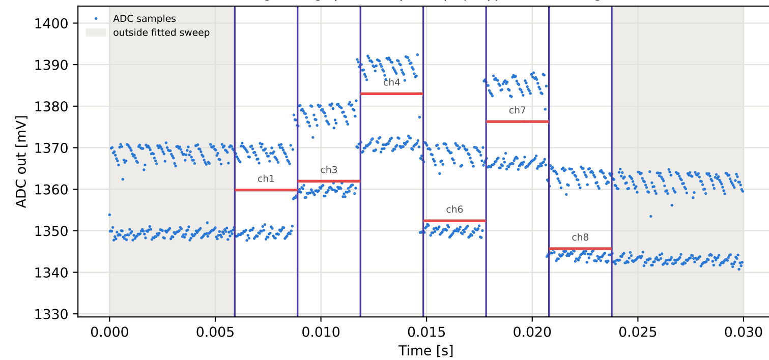
Tag4 &lt;- Tag15 | 935 MHz | run 0 | rep 1 | phase 78.35 deg
