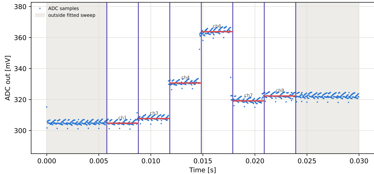
Tag7 &lt;- Tag6 | 935 MHz | run 0 | rep 1 | phase 82.18 deg
