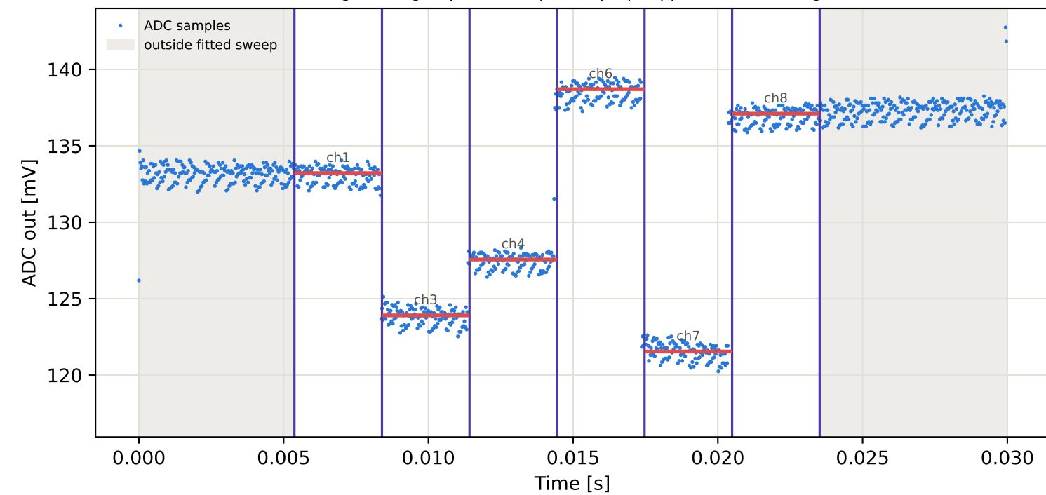
Tag5 &lt;- Tag2 | 785 MHz | run 0 | rep 1 | phase -105.31 deg
