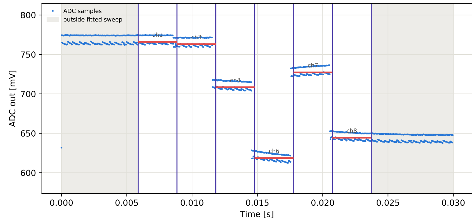
Tag9 &lt;- Tag8 | 875 MHz | run 0 | rep 1 | phase 20.78 deg
