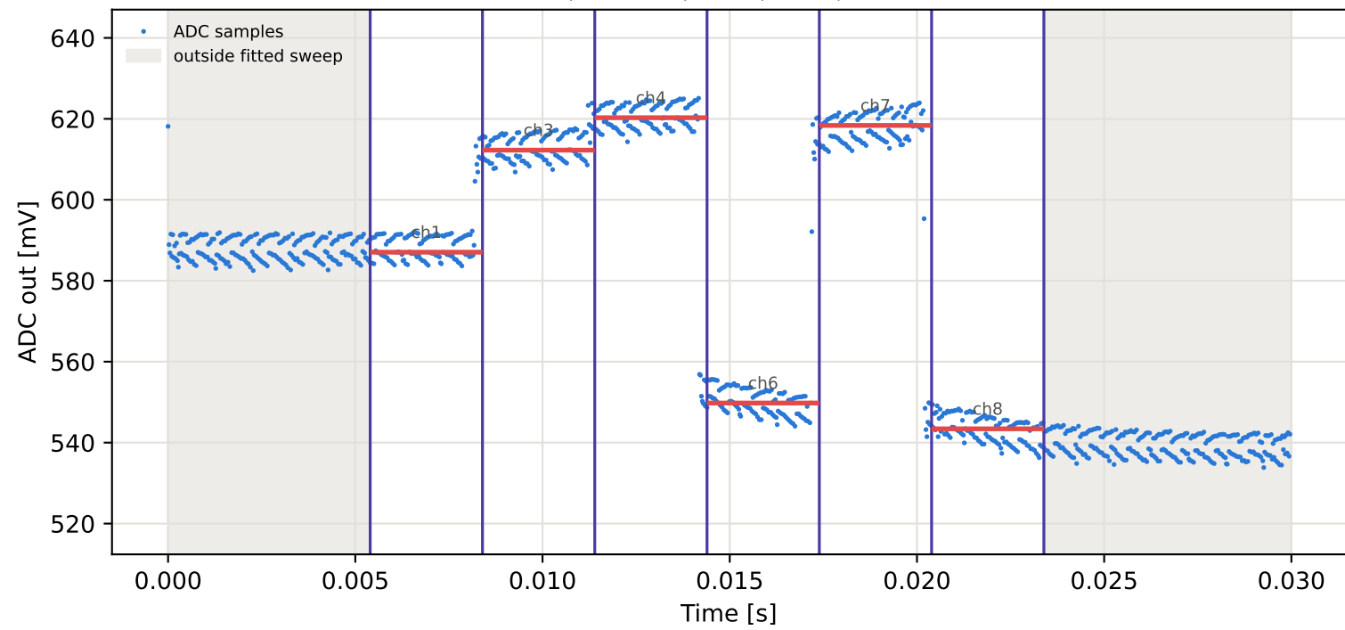
Tag7 &lt;- Tag6 | 905 MHz | run 0 | rep 1 | phase -31.53 deg
