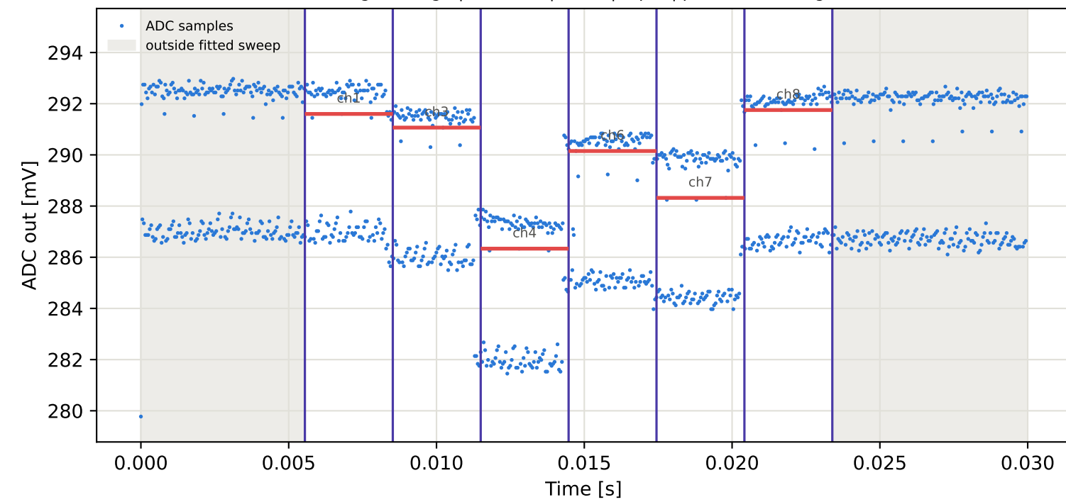
Tag1 &lt;- Tag7 | 995 MHz | run 0 | rep 1 | phase -131.29 deg
