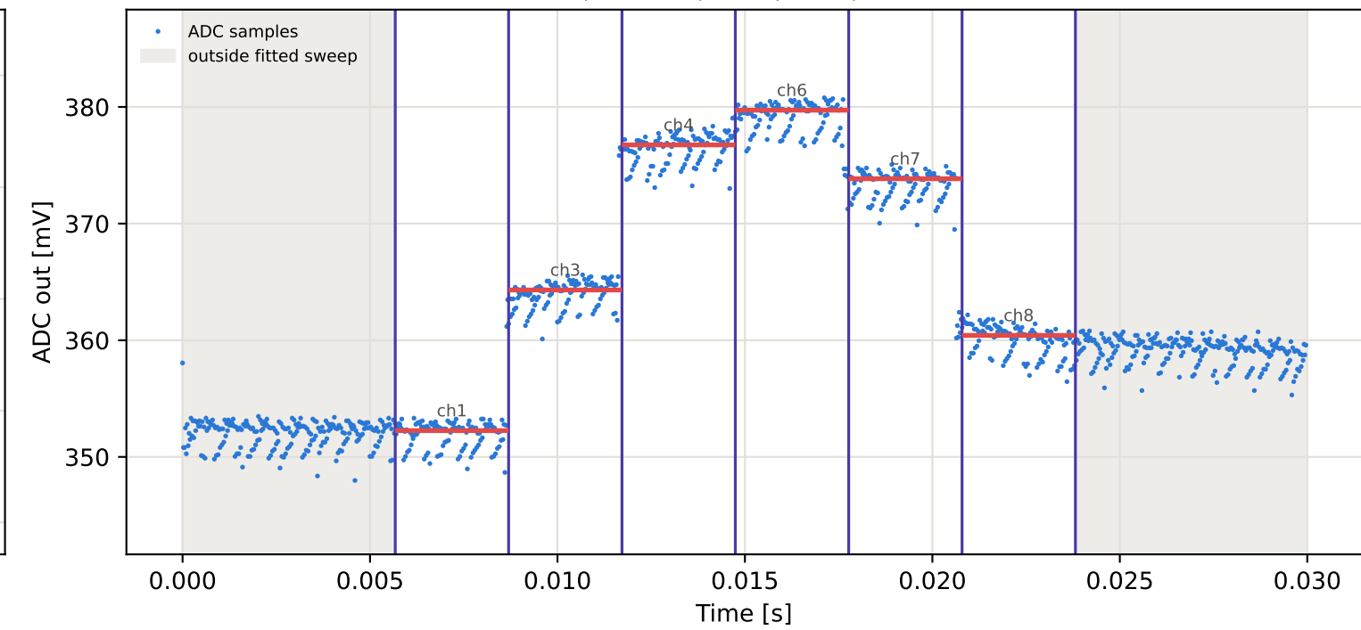
Tag7 &lt;- Tag15 | 895 MHz | run 0 | rep 1 | phase -119.56 deg
