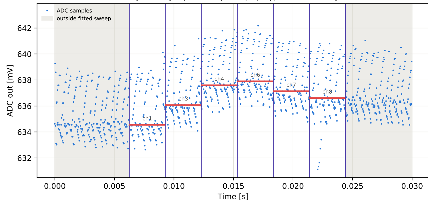
Tag15 &lt;- Tag10 | 865 MHz | run 0 | rep 1 | phase -122.26 deg
