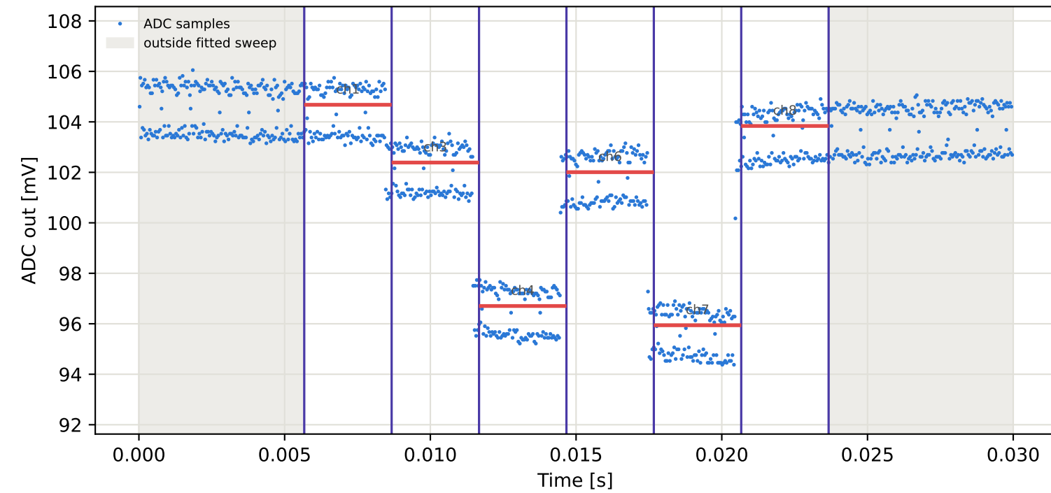
Tag5 &lt;- Tag3 | 775 MHz | run 0 | rep 1 | phase 74.74 deg
