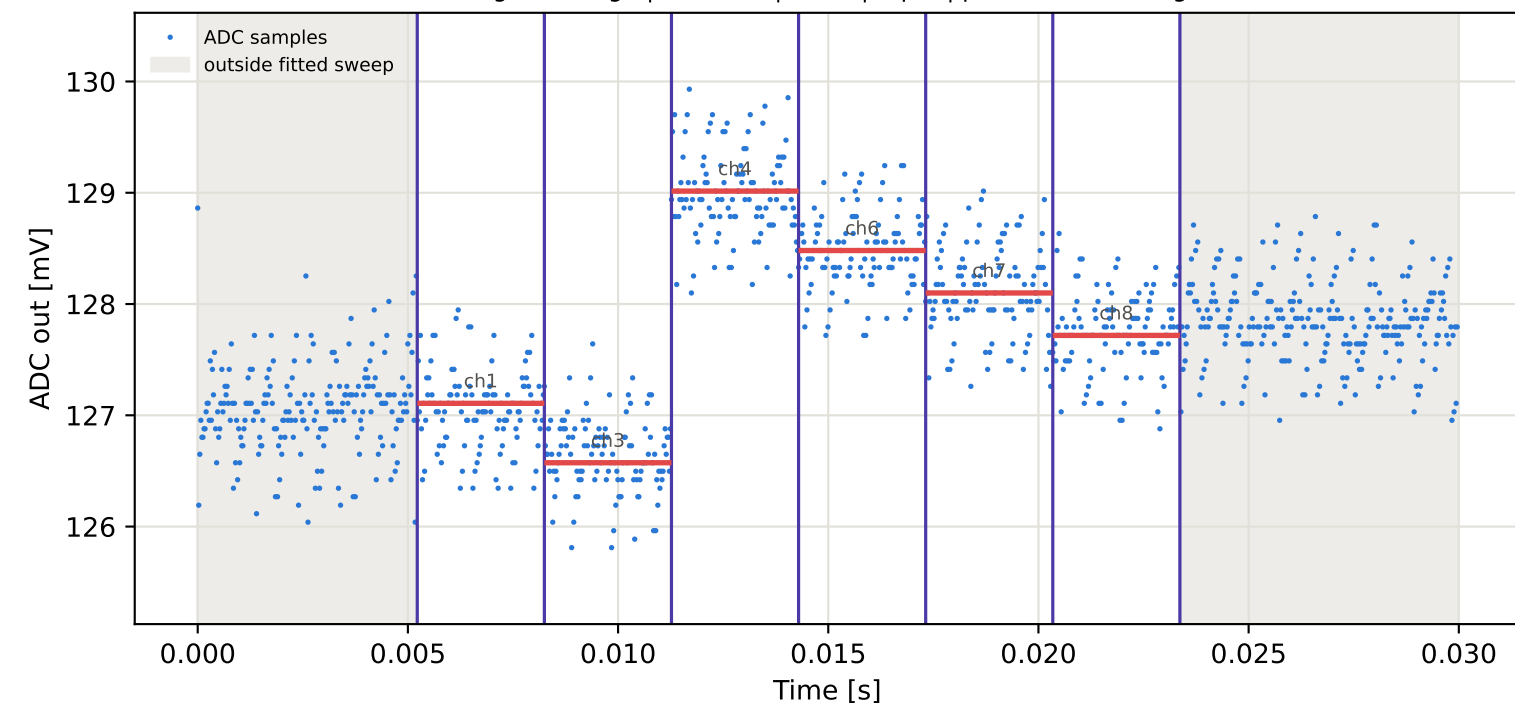
Tag16 &lt;- Tag7 | 775 MHz | run 0 | rep 1 | phase -115.26 deg
