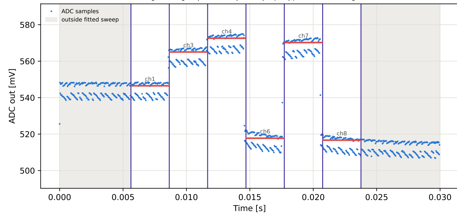
Tag6 &lt;- Tag10 | 915 MHz | run 0 | rep 1 | phase -30.78 deg
