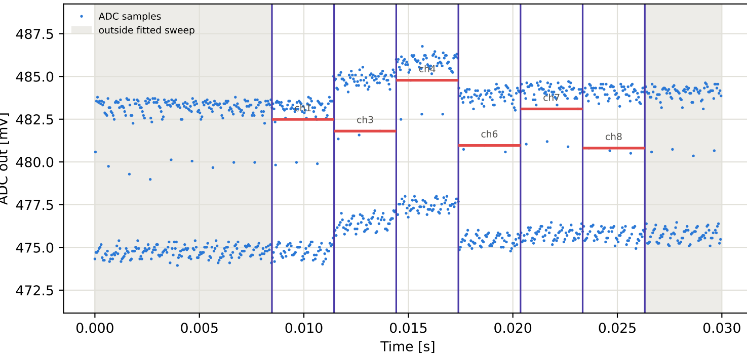
Tag7 &lt;- Tag10 | 975 MHz | run 0 | rep 1 | phase -77.51 deg
