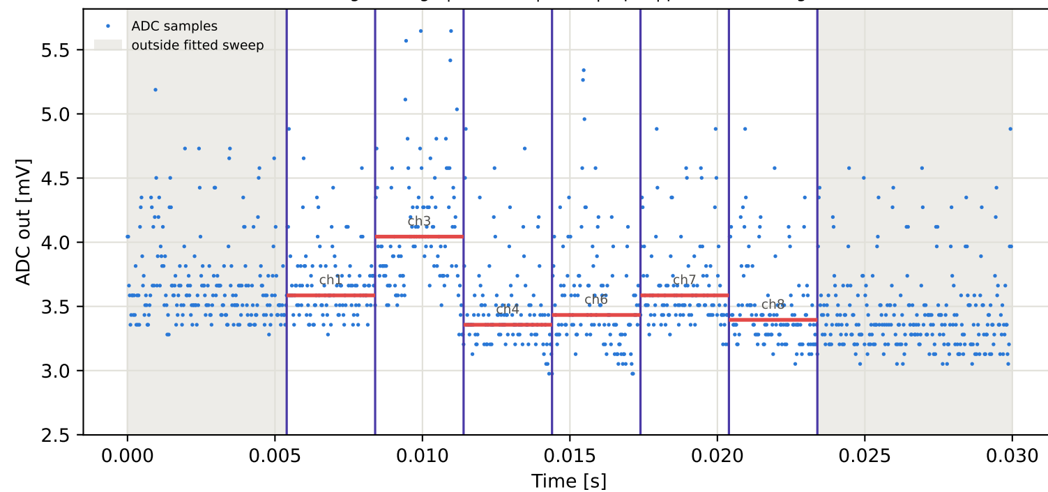
Tag2 &lt;- Tag7 | 795 MHz | run 0 | rep 1 | phase 43.27 deg
