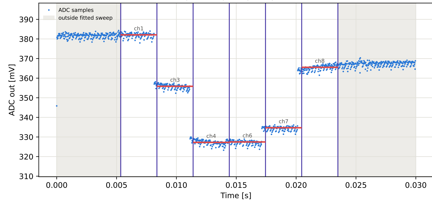
Tag1 &lt;- Tag3 | 885 MHz | run 0 | rep 1 | phase 62.94 deg
