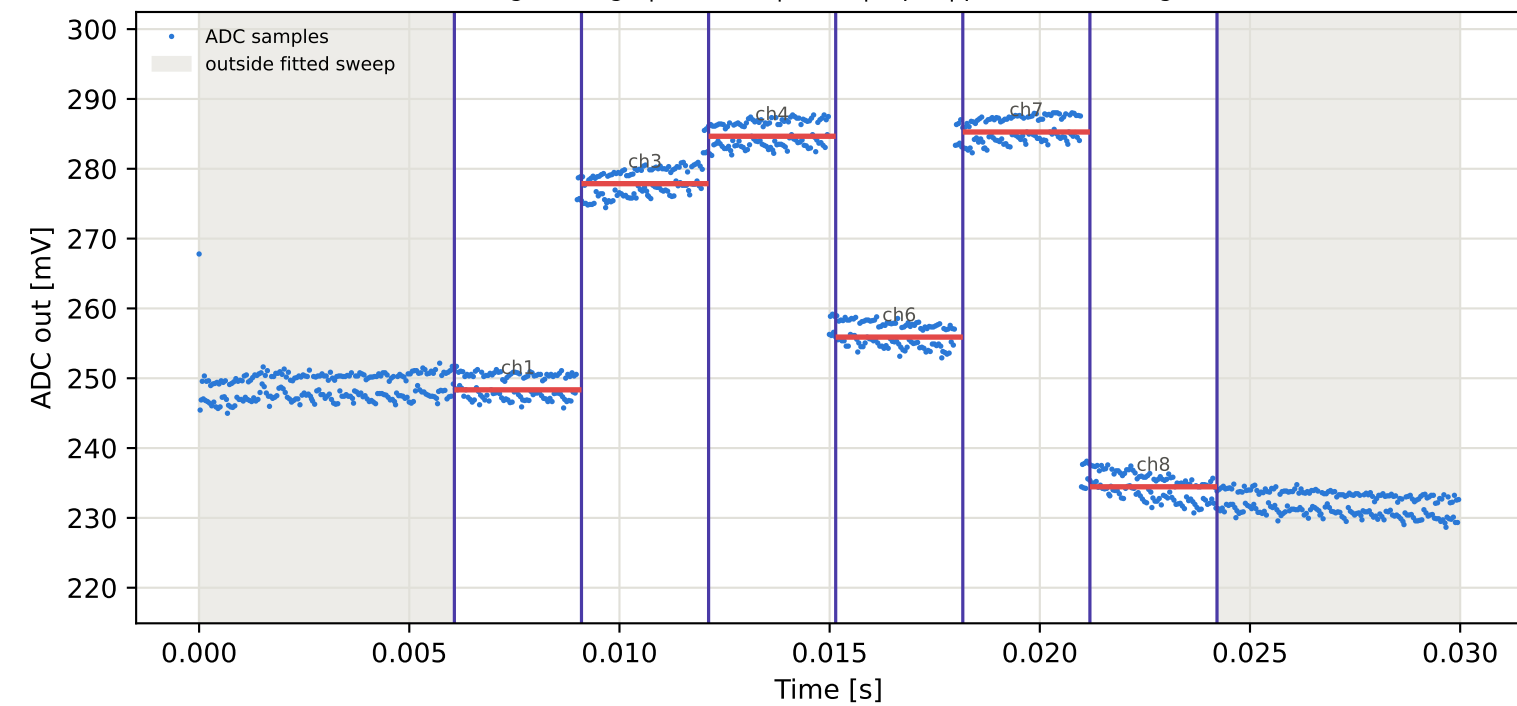
Tag2 &lt;- Tag5 | 865 MHz | run 0 | rep 1 | phase 47.28 deg
