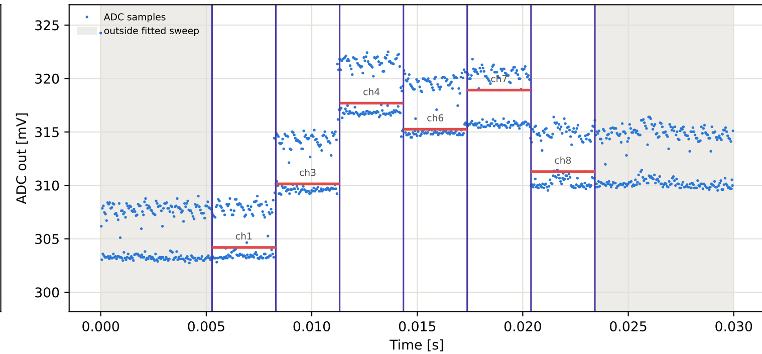
Tag2 &lt;- Tag16 | 845 MHz | run 0 | rep 1 | phase -151.57 deg
