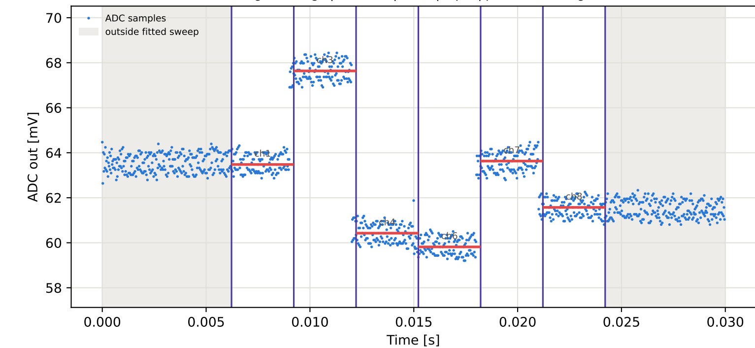
Tag16 &lt;- Tag6 | 785 MHz | run 0 | rep 1 | phase -61.97 deg
