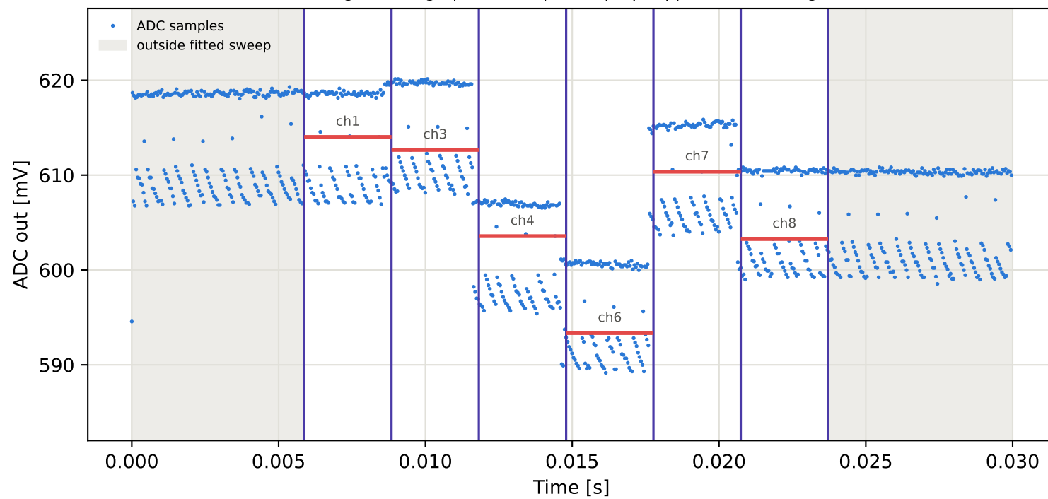
Tag15 &lt;- Tag9 | 985 MHz | run 0 | rep 1 | phase -158.61 deg
