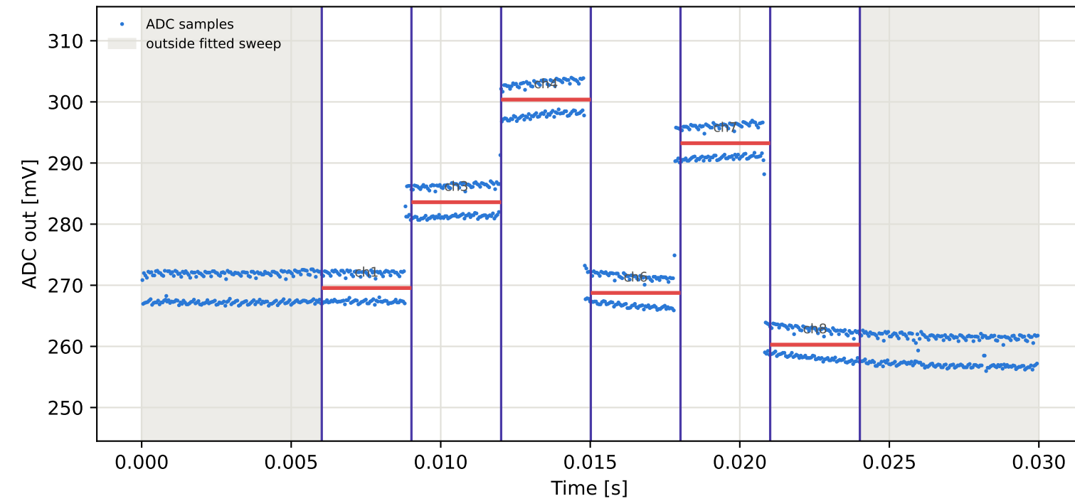
Tag3 &lt;- Tag8 | 935 MHz | run 0 | rep 1 | phase -36.13 deg
