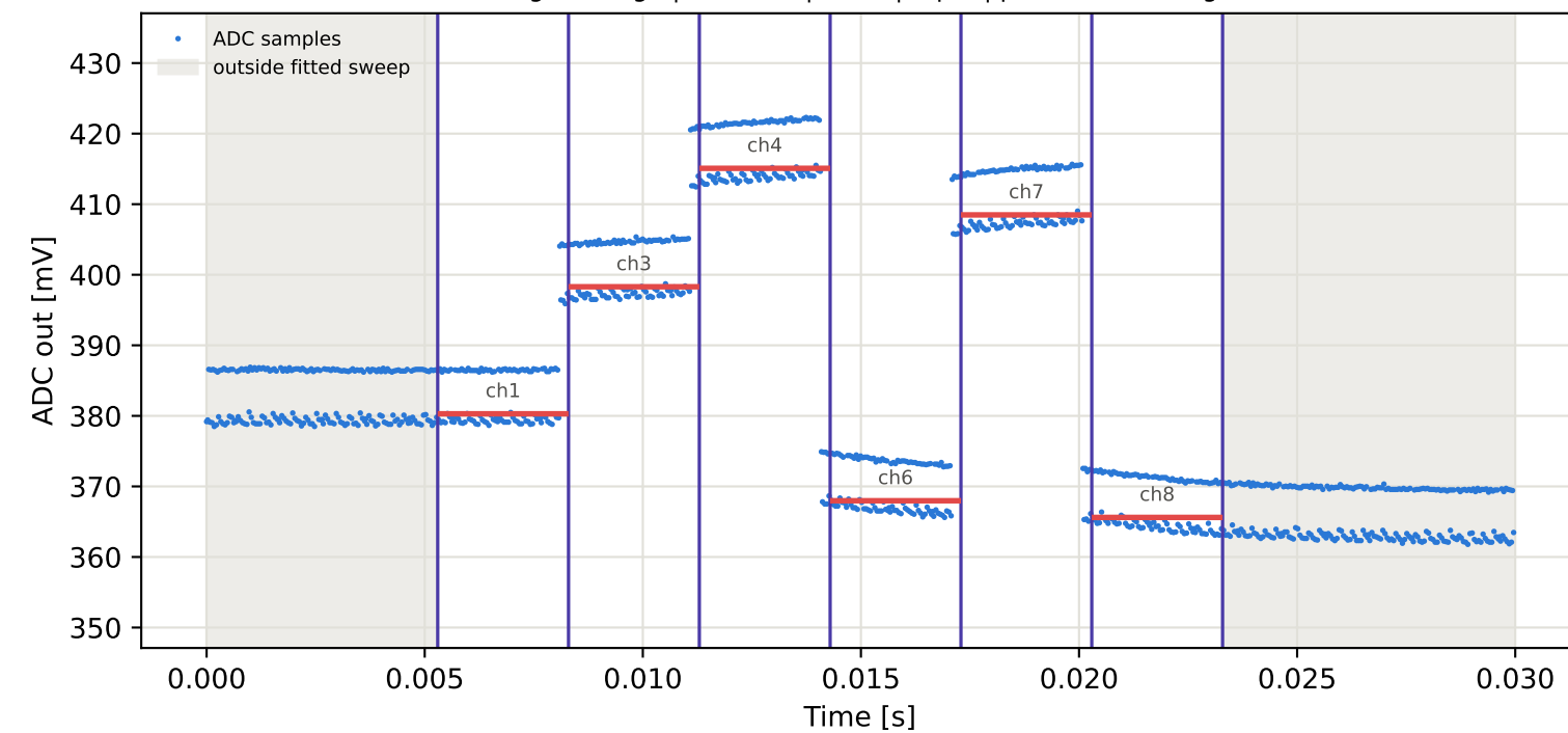
Tag1 &lt;- Tag9 | 945 MHz | run 0 | rep 1 | phase -55.30 deg
