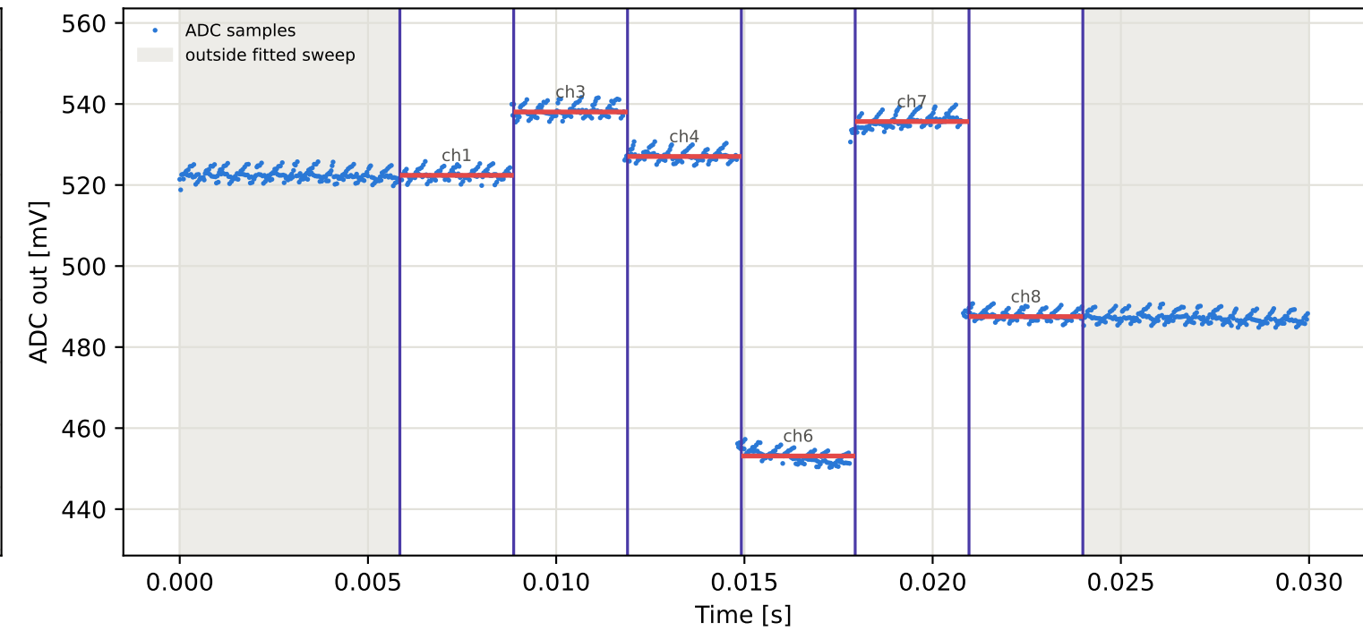
Tag9 &lt;- Tag2 | 965 MHz | run 0 | rep 1 | phase 91.42 deg
