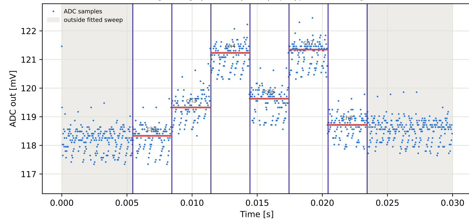
Tag9 &lt;- Tag10 | 785 MHz | run 0 | rep 1 | phase -102.04 deg
