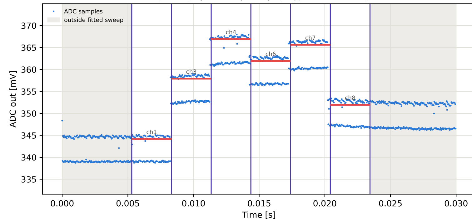
Tag9 &lt;- Tag5 | 845 MHz | run 0 | rep 1 | phase 173.08 deg
