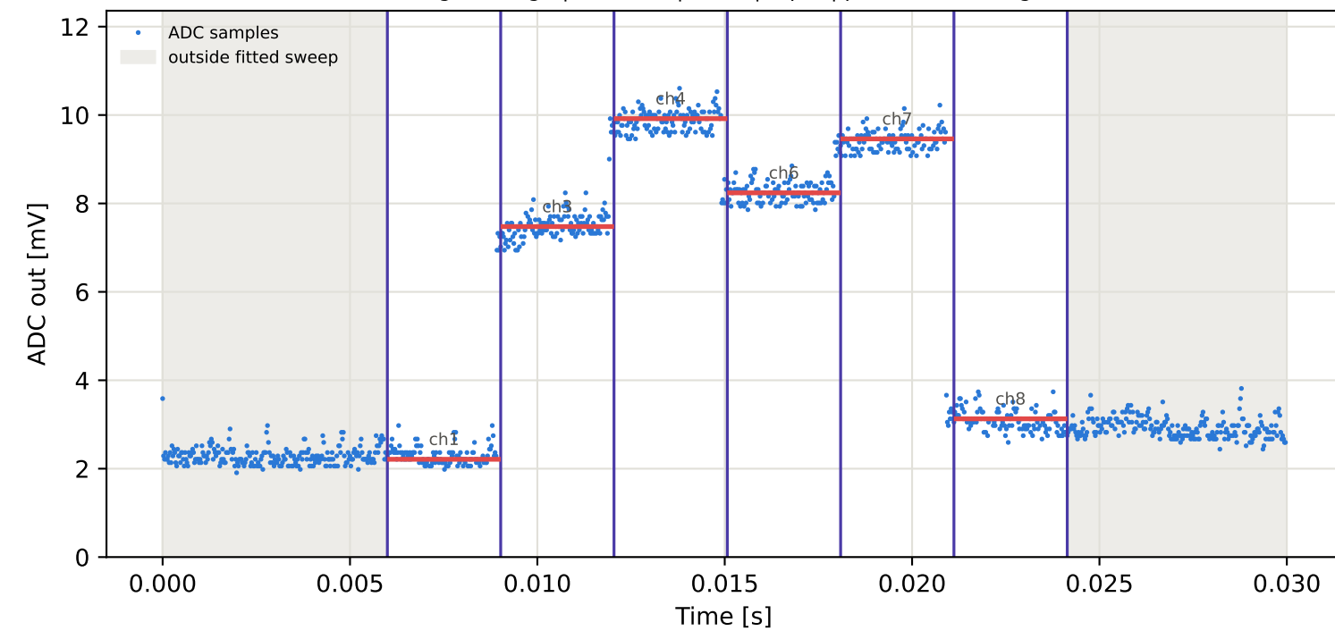
Tag1 &lt;- Tag7 | 875 MHz | run 0 | rep 1 | phase 122.32 deg
