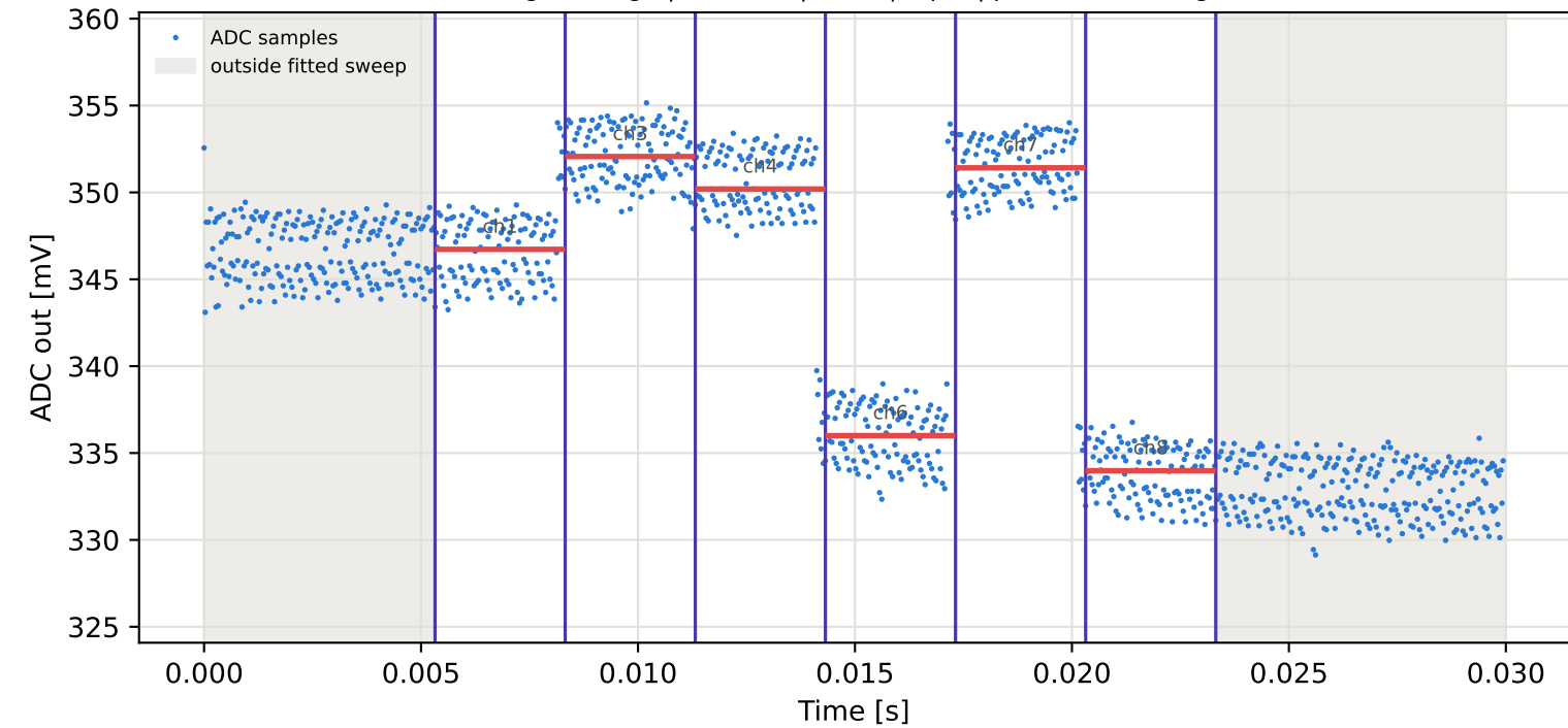
Tag1 &lt;- Tag8 | 885 MHz | run 0 | rep 1 | phase -101.94 deg
