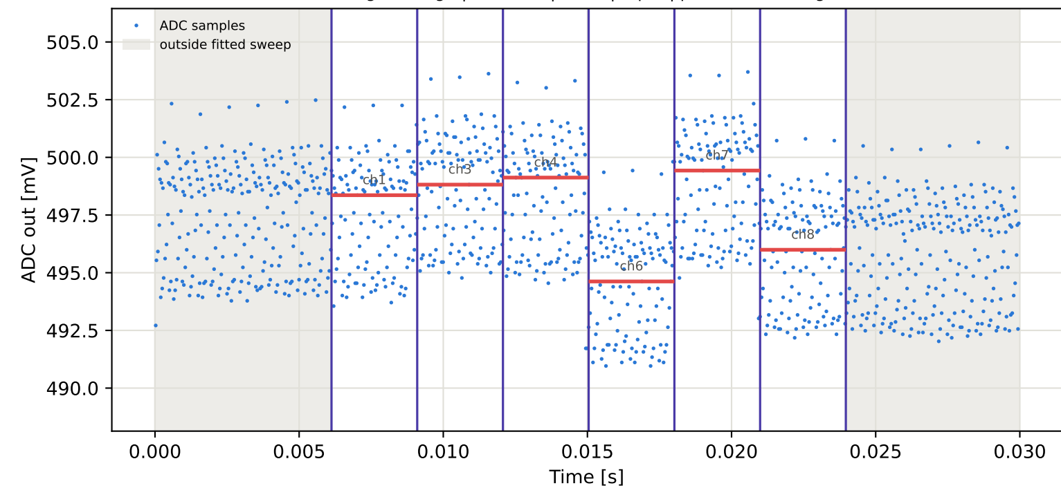
Tag1 &lt;- Tag9 | 965 MHz | run 0 | rep 1 | phase -22.78 deg
