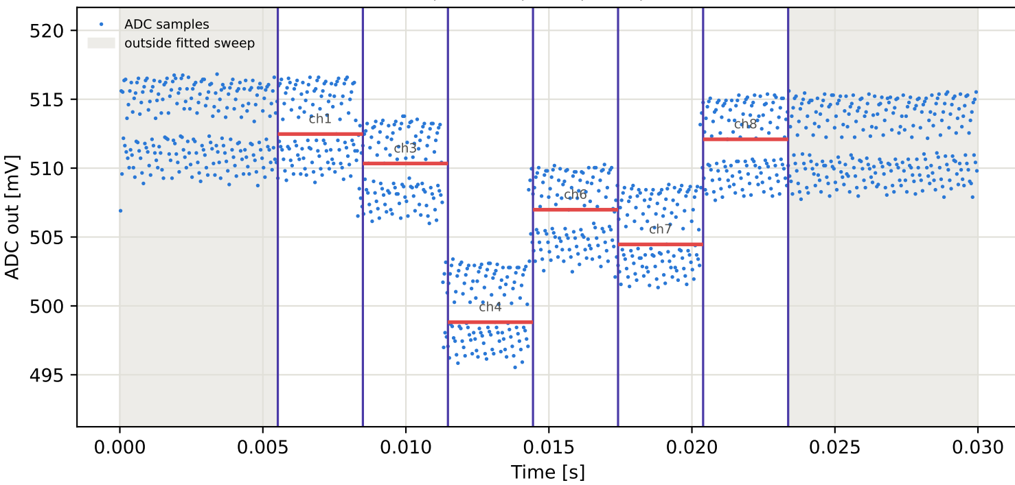
Tag3 &lt;- Tag16 | 975 MHz | run 0 | rep 1 | phase 68.84 deg
