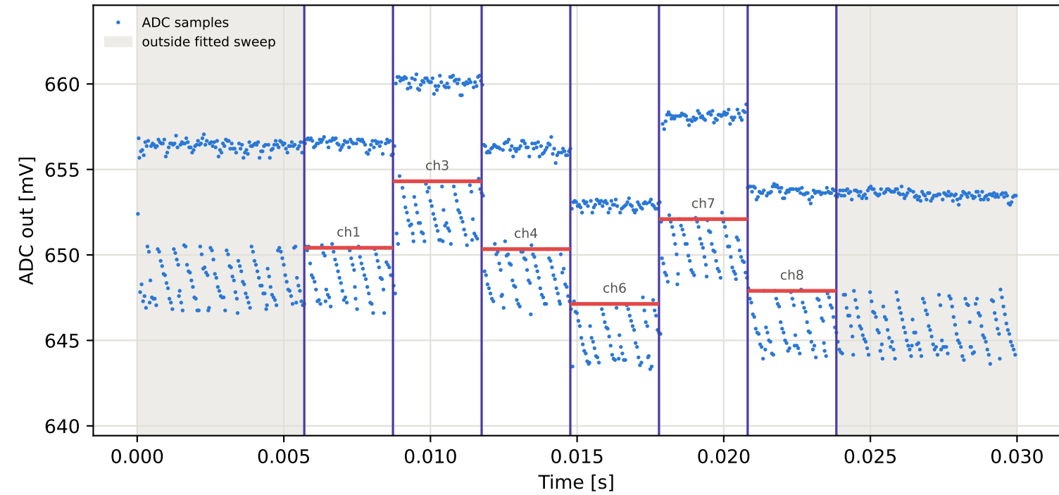
Tag8 &lt;- Tag7 | 825 MHz | run 0 | rep 1 | phase 114.05 deg
