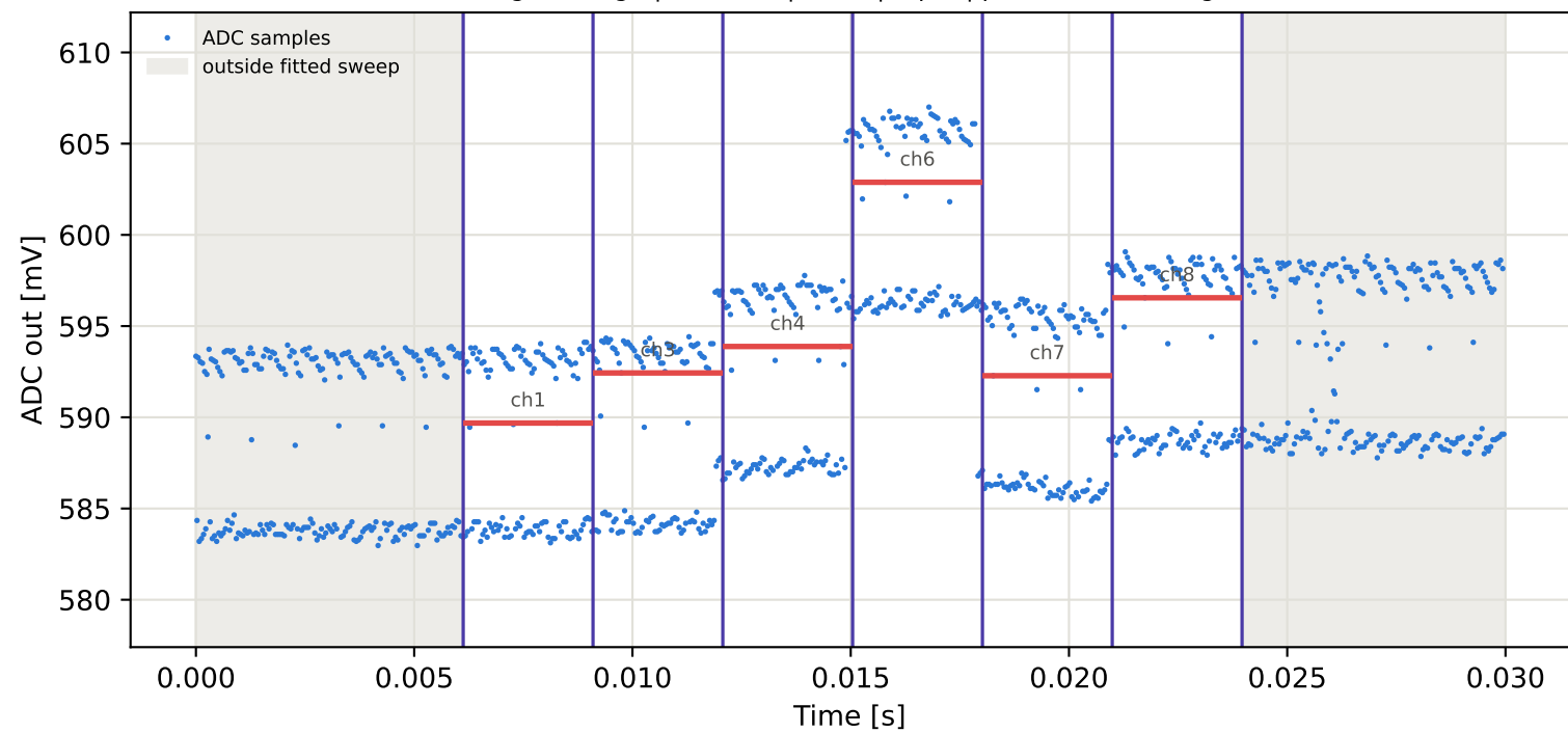
Tag7 &lt;- Tag4 | 905 MHz | run 0 | rep 1 | phase 158.40 deg
