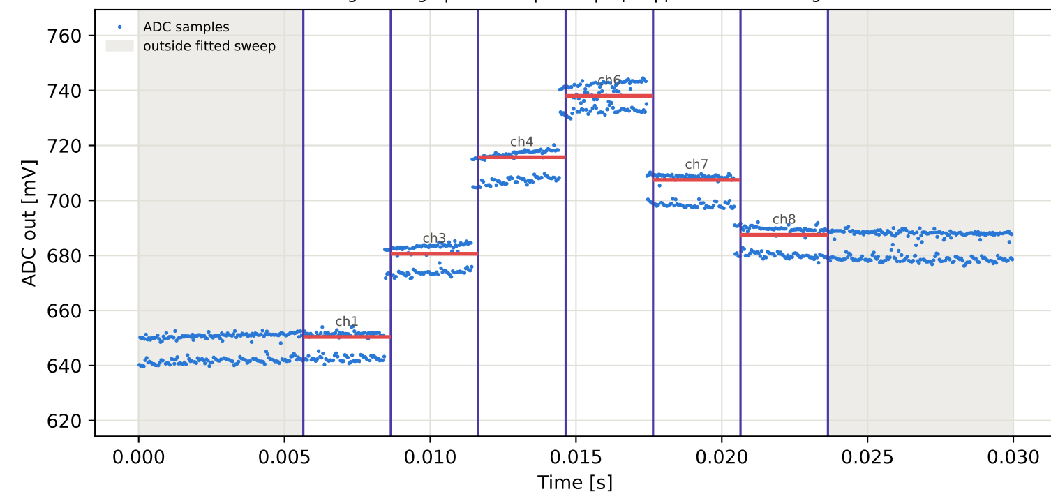
Tag4 &lt;- Tag7 | 885 MHz | run 0 | rep 1 | phase -114.67 deg
