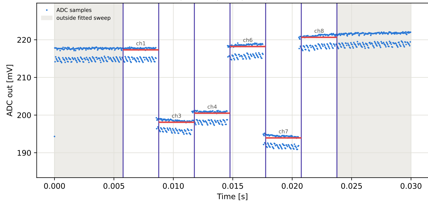
Tag3 &lt;- Tag8 | 805 MHz | run 0 | rep 1 | phase 147.34 deg
