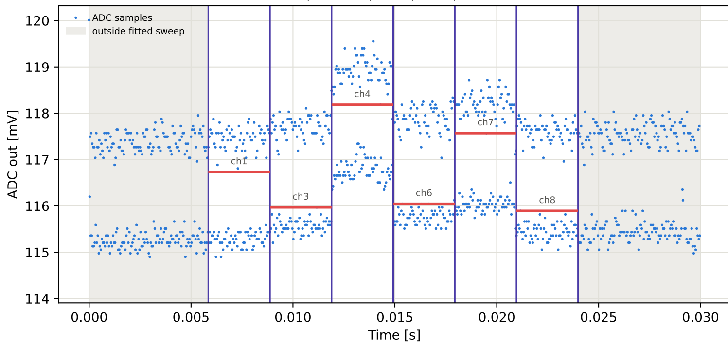
Tag5 &lt;- Tag8 | 995 MHz | run 0 | rep 1 | phase 128.30 deg
