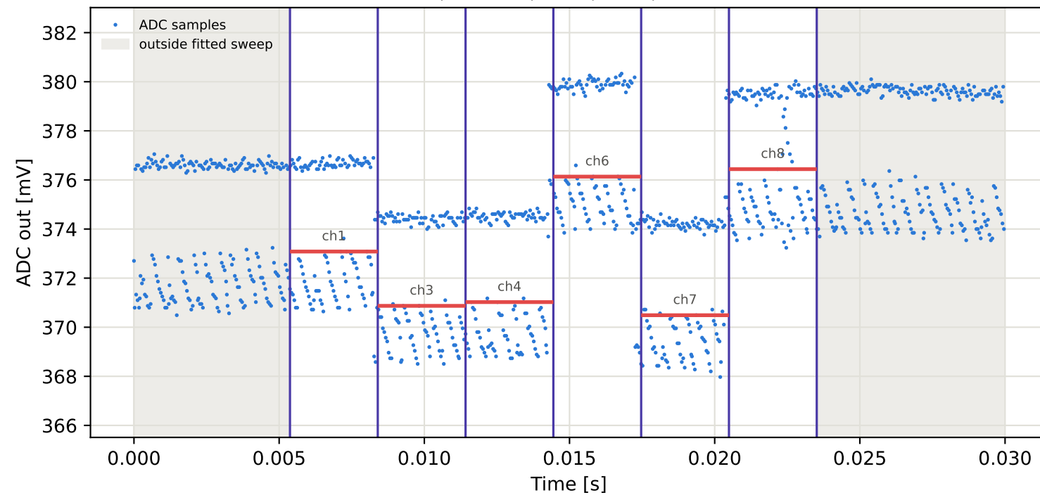
Tag4 &lt;- Tag2 | 825 MHz | run 0 | rep 1 | phase 161.22 deg
