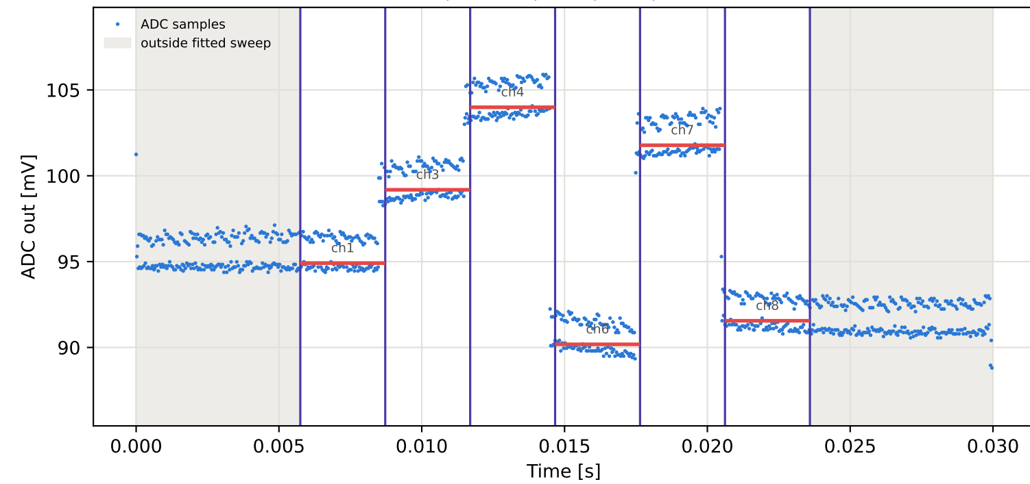
Tag10 &lt;- Tag4 | 965 MHz | run 0 | rep 1 | phase -52.78 deg
