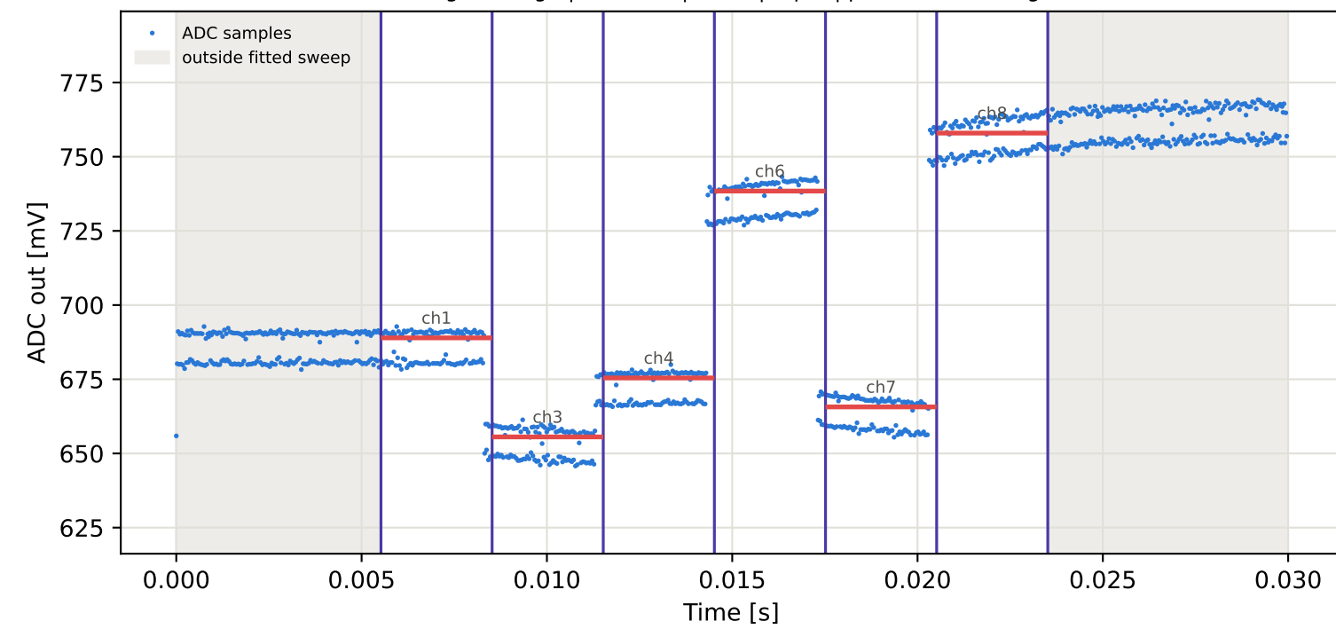
Tag4 &lt;- Tag9 | 885 MHz | run 0 | rep 1 | phase 167.48 deg
