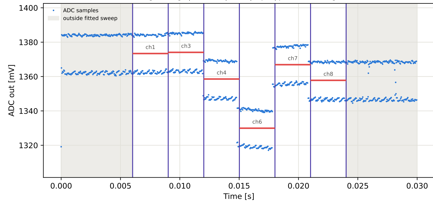
Tag4 &lt;- Tag8 | 935 MHz | run 0 | rep 1 | phase -57.70 deg
