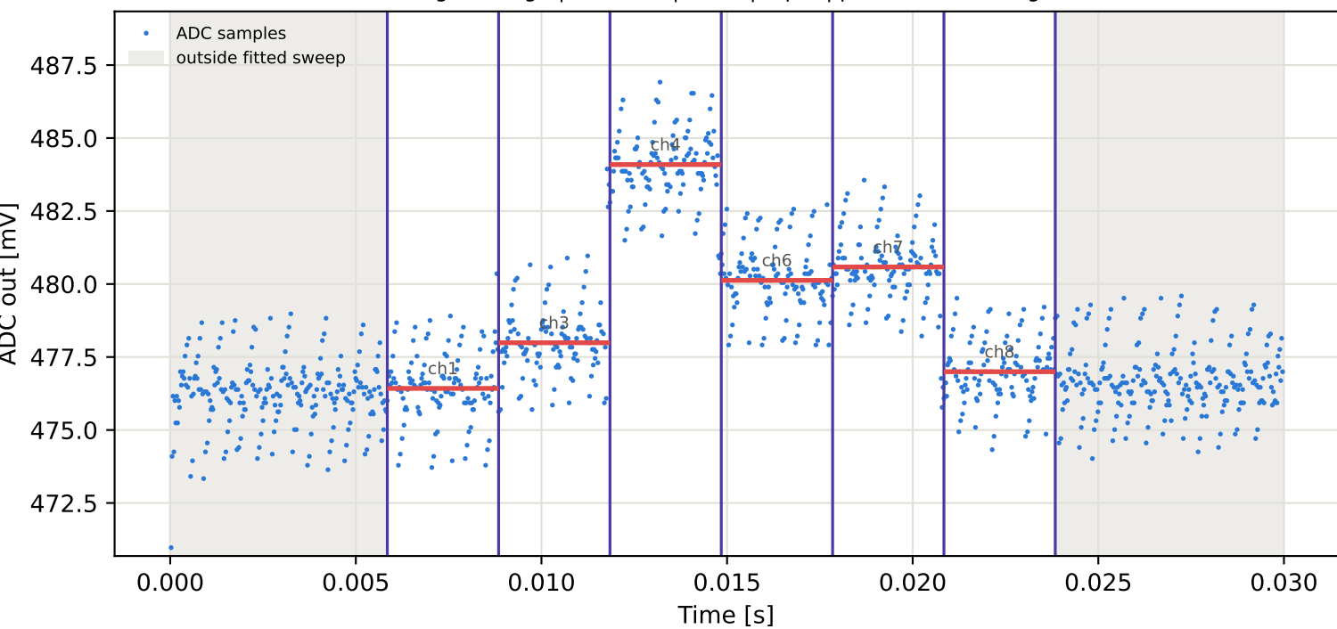
Tag7 &lt;- Tag5 | 975 MHz | run 0 | rep 1 | phase -116.36 deg
