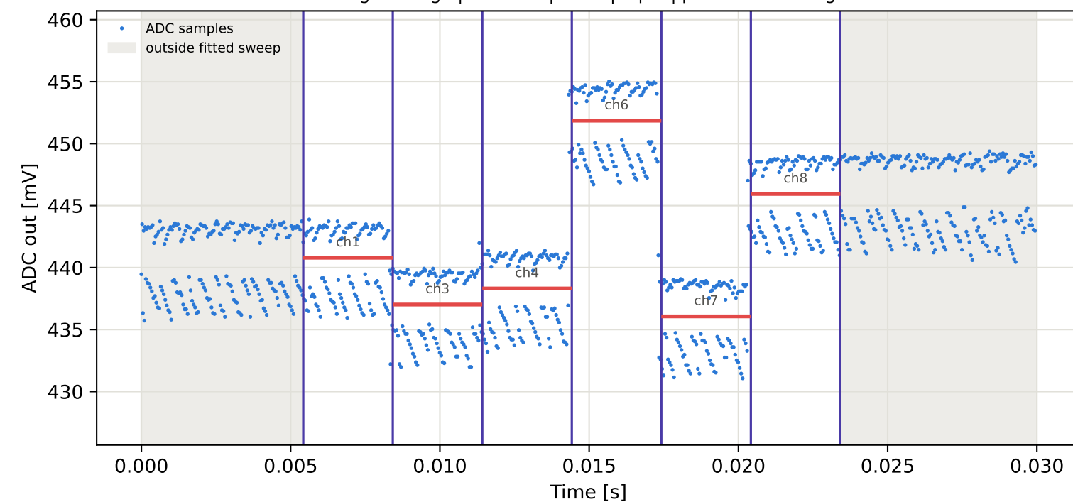
Tag7 &lt;- Tag5 | 985 MHz | run 0 | rep 1 | phase -39.64 deg
