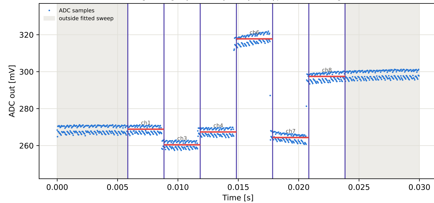
Tag1 &lt;- Tag16 | 915 MHz | run 0 | rep 1 | phase -82.50 deg
