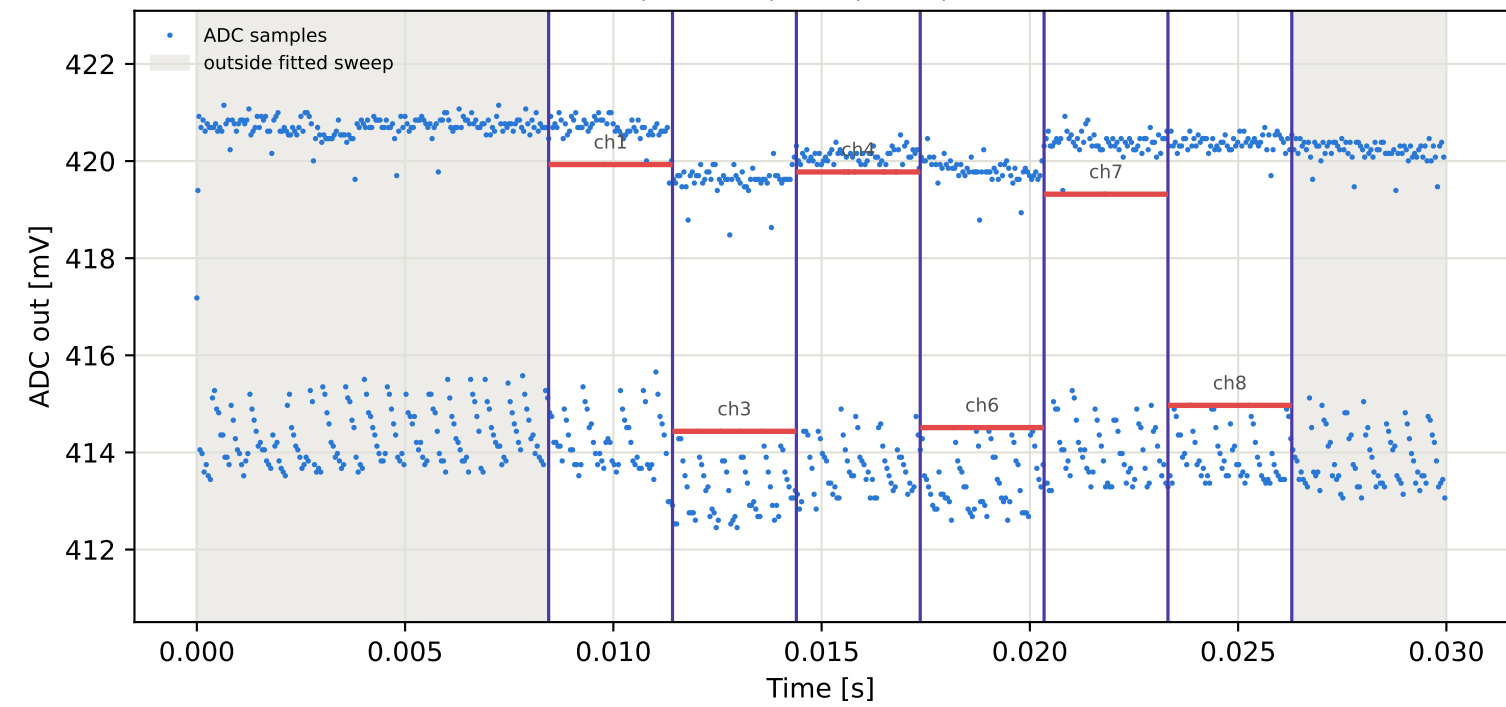
Tag5 &lt;- Tag1 | 825 MHz | run 0 | rep 1 | phase -39.98 deg
