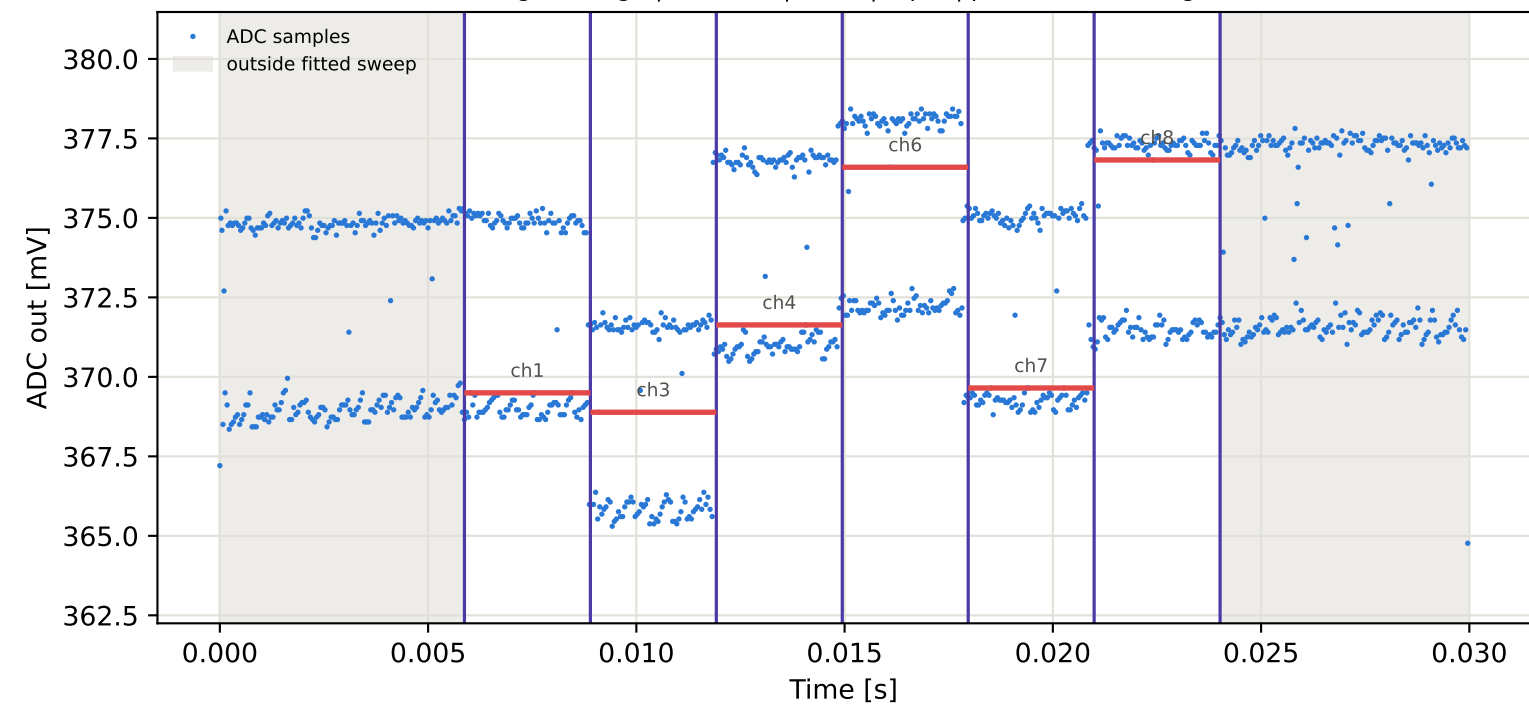
Tag9 &lt;- Tag15 | 835 MHz | run 0 | rep 1 | phase -149.50 deg
