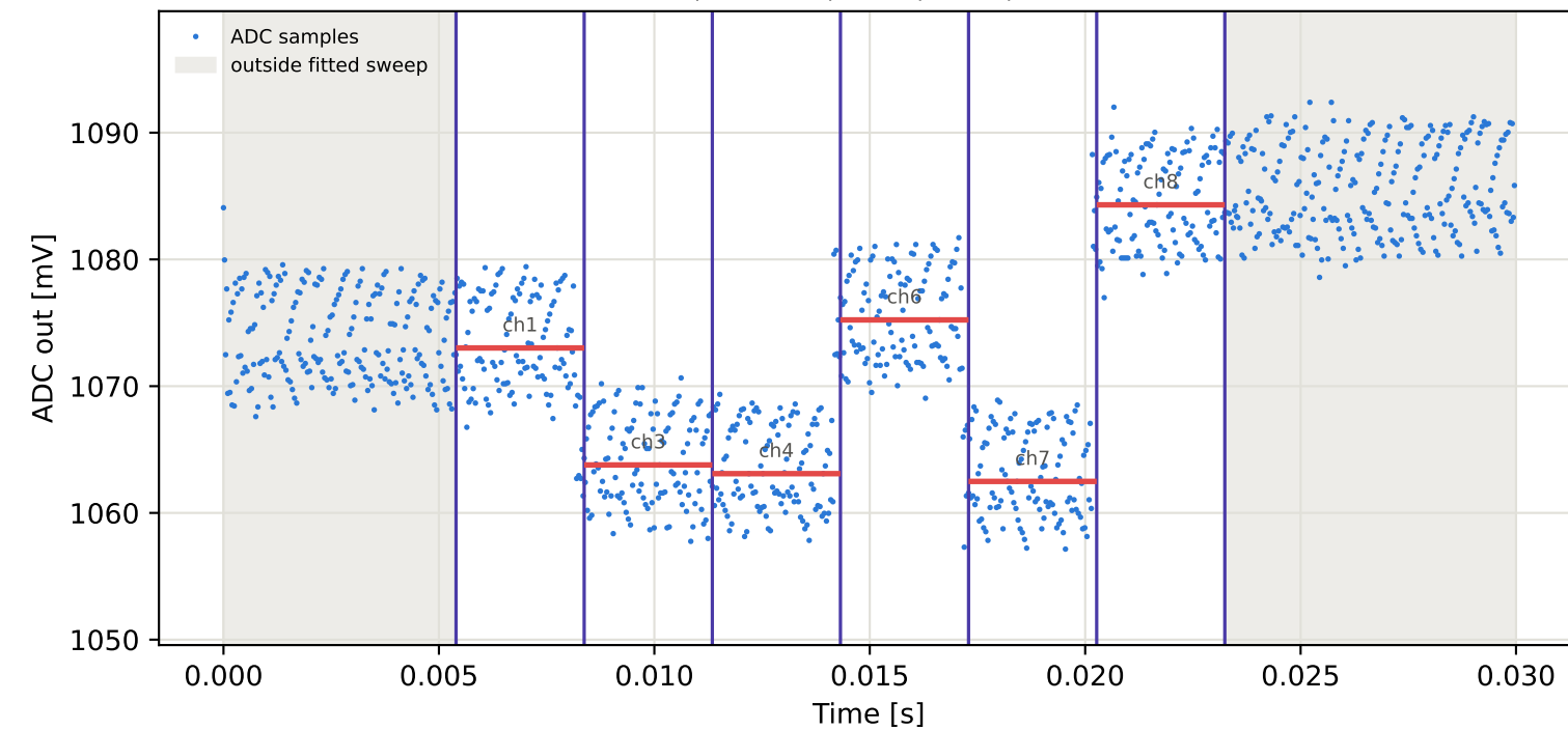
Tag16 &lt;- Tag10 | 885 MHz | run 0 | rep 1 | phase 136.00 deg
