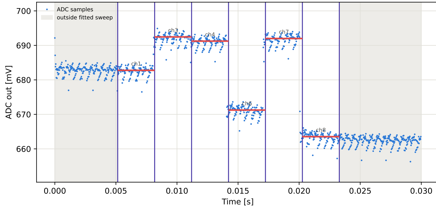
Tag15 &lt;- Tag1 | 885 MHz | run 0 | rep 1 | phase 142.16 deg
