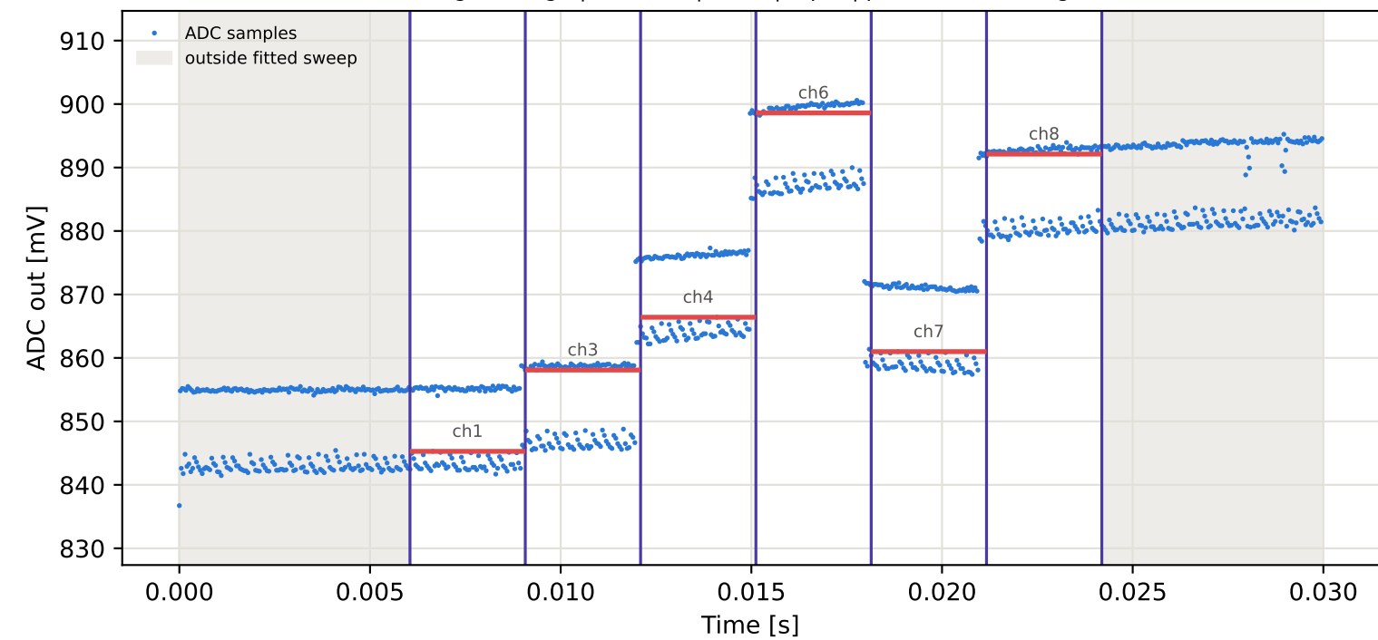
Tag3 &lt;- Tag7 | 875 MHz | run 0 | rep 1 | phase 90.85 deg
