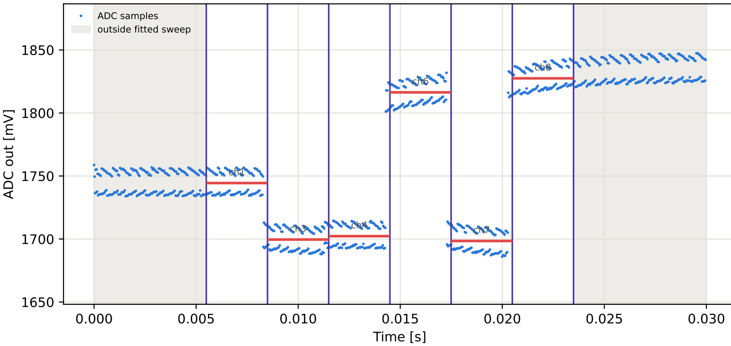
Tag8 &lt;- Tag15 | 905 MHz | run 0 | rep 1 | phase 159.31 deg
