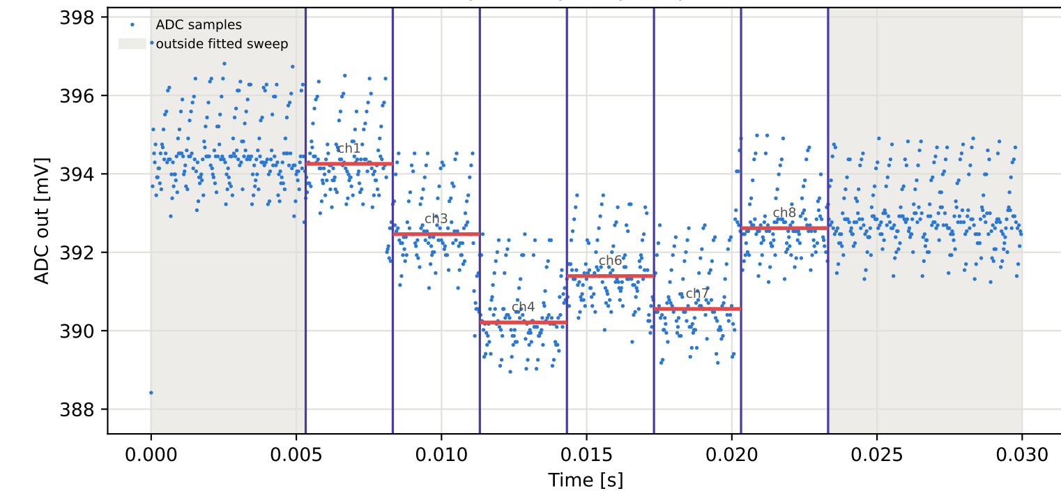
Tag15 &lt;- Tag6 | 835 MHz | run 0 | rep 1 | phase 78.38 deg
