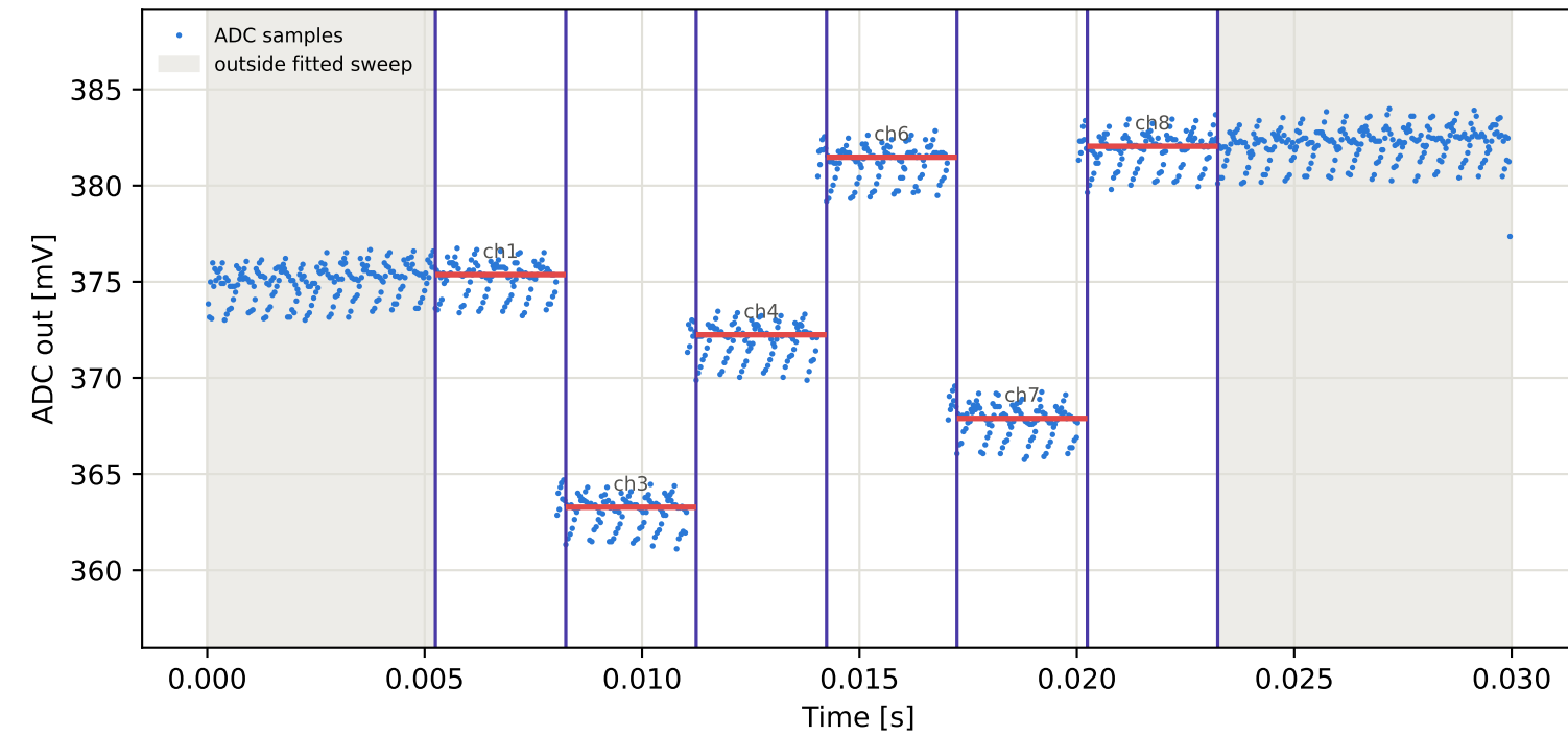
Tag9 &lt;- Tag16 | 835 MHz | run 0 | rep 1 | phase 165.90 deg
