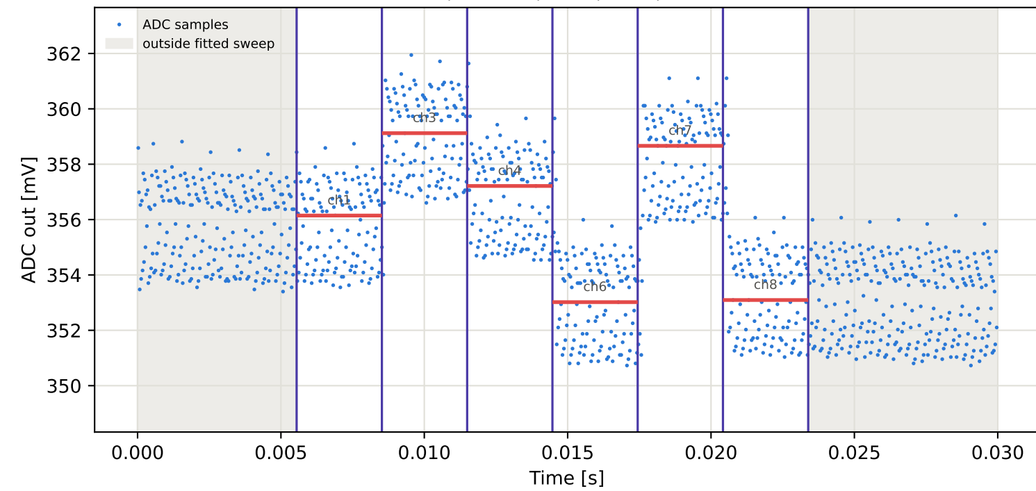
Tag3 &lt;- Tag9 | 825 MHz | run 0 | rep 1 | phase -3.99 deg
