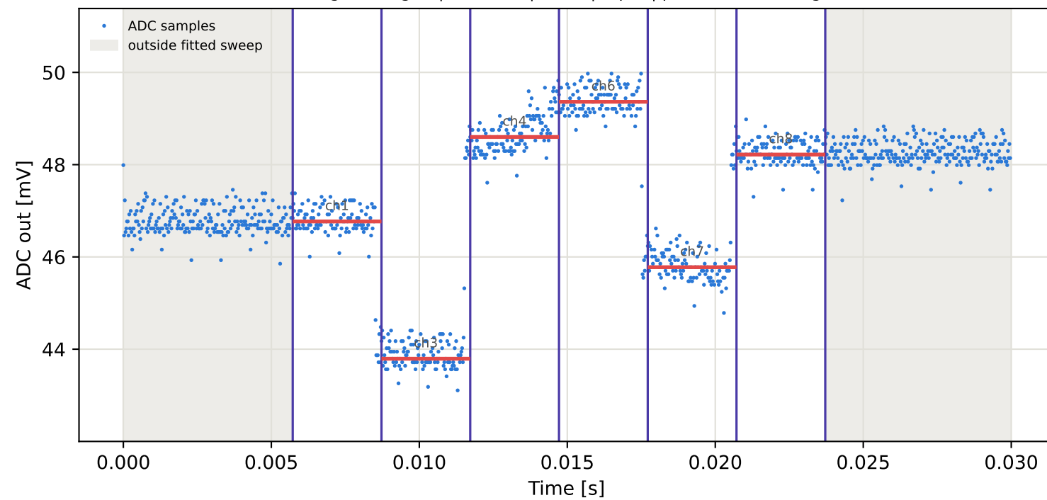
Tag1 &lt;- Tag16 | 775 MHz | run 0 | rep 1 | phase -122.26 deg
