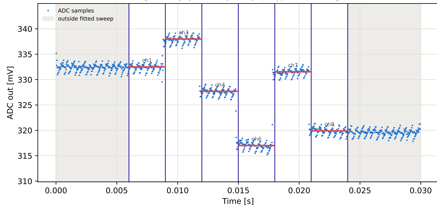
Tag10 &lt;- Tag9 | 865 MHz | run 0 | rep 1 | phase 144.76 deg
