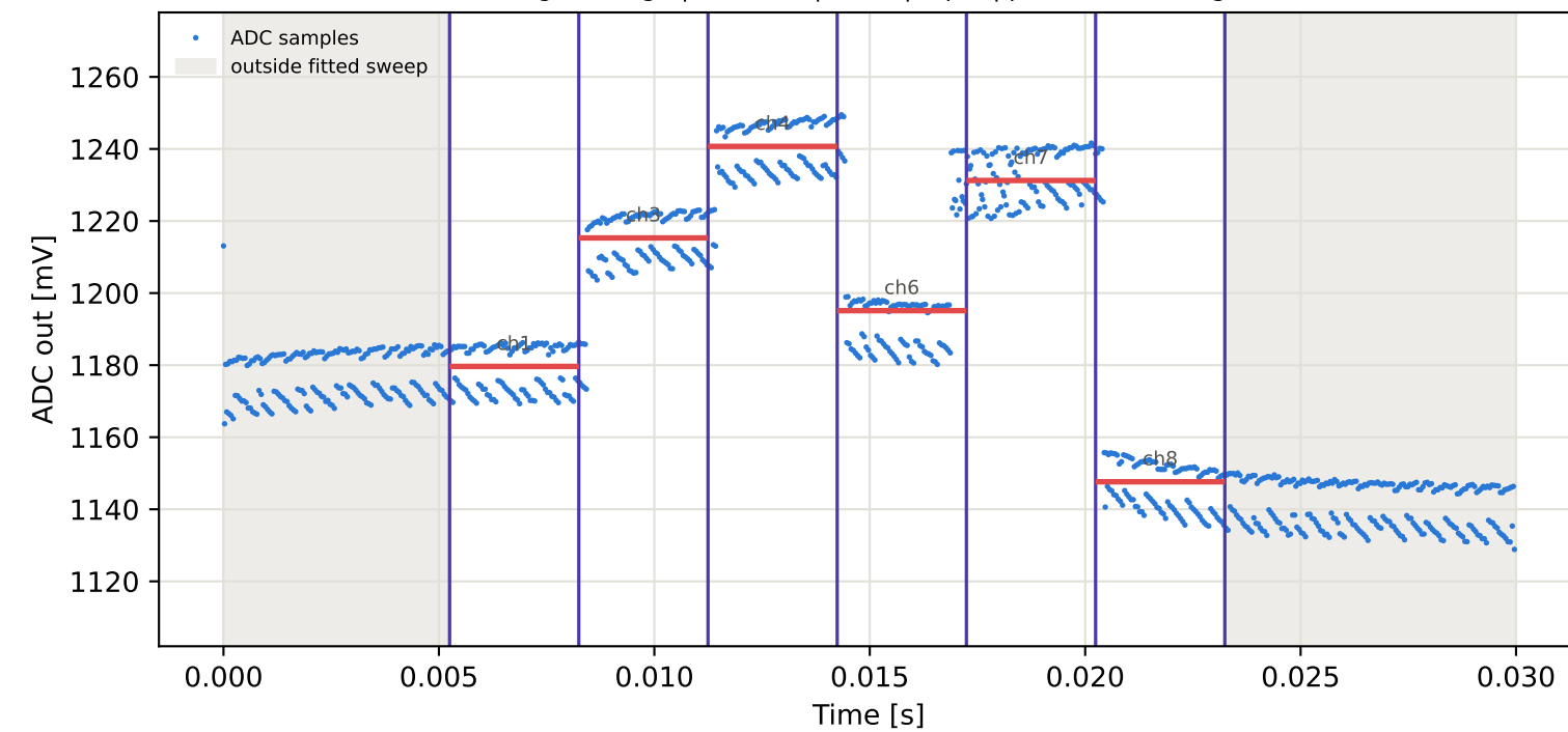
Tag4 &lt;- Tag7 | 905 MHz | run 0 | rep 1 | phase -155.36 deg
