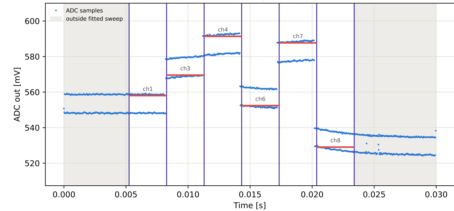
Tag6 &lt;- Tag10 | 905 MHz | run 0 | rep 1 | phase -63.19 deg
