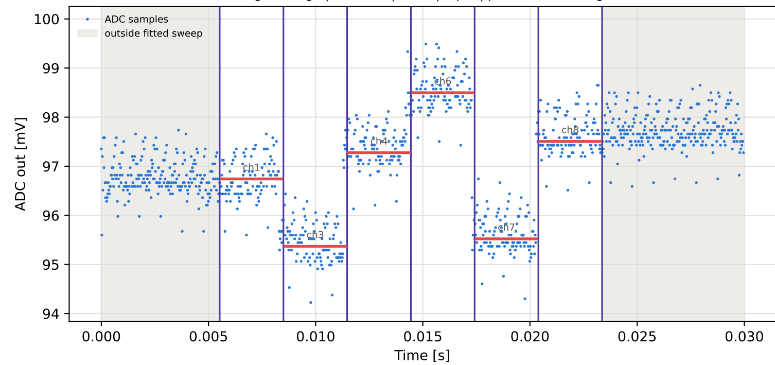
Tag5 &lt;- Tag1 | 775 MHz | run 0 | rep 1 | phase -158.73 deg
