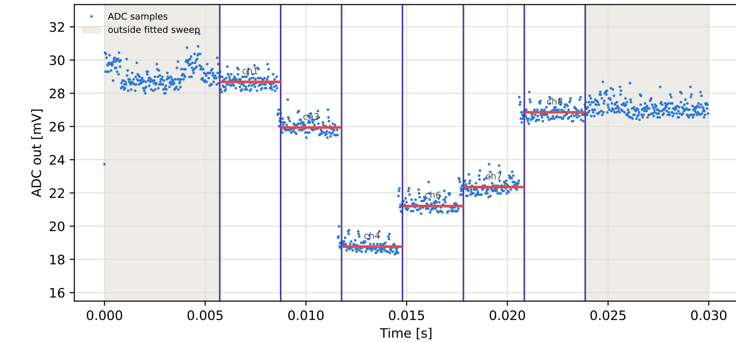
Tag2 &lt;- Tag15 | 965 MHz | run 0 | rep 1 | phase -67.58 deg
