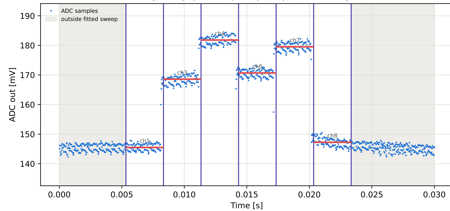
Tag6 &lt;- Tag9 | 885 MHz | run 0 | rep 1 | phase -47.77 deg
