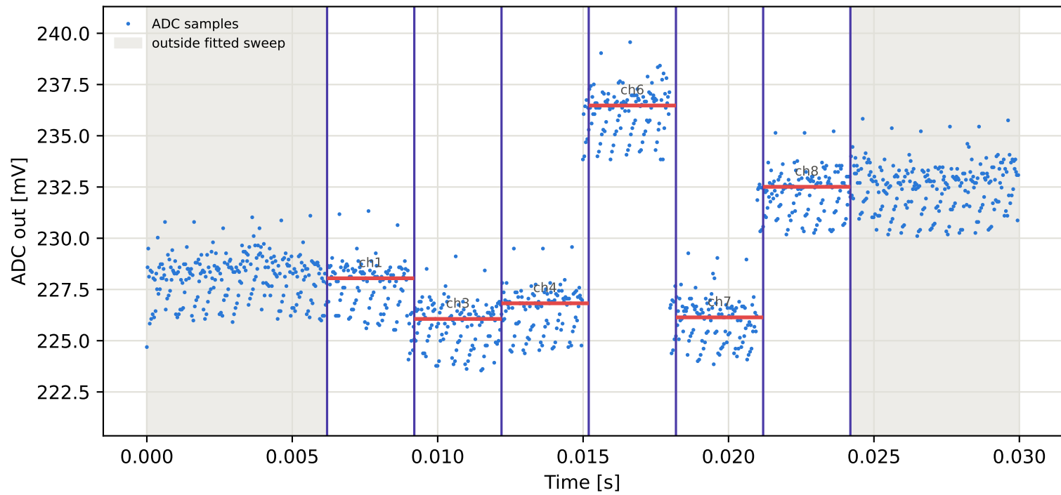
Tag2 &lt;- Tag16 | 925 MHz | run 0 | rep 1 | phase 128.98 deg
