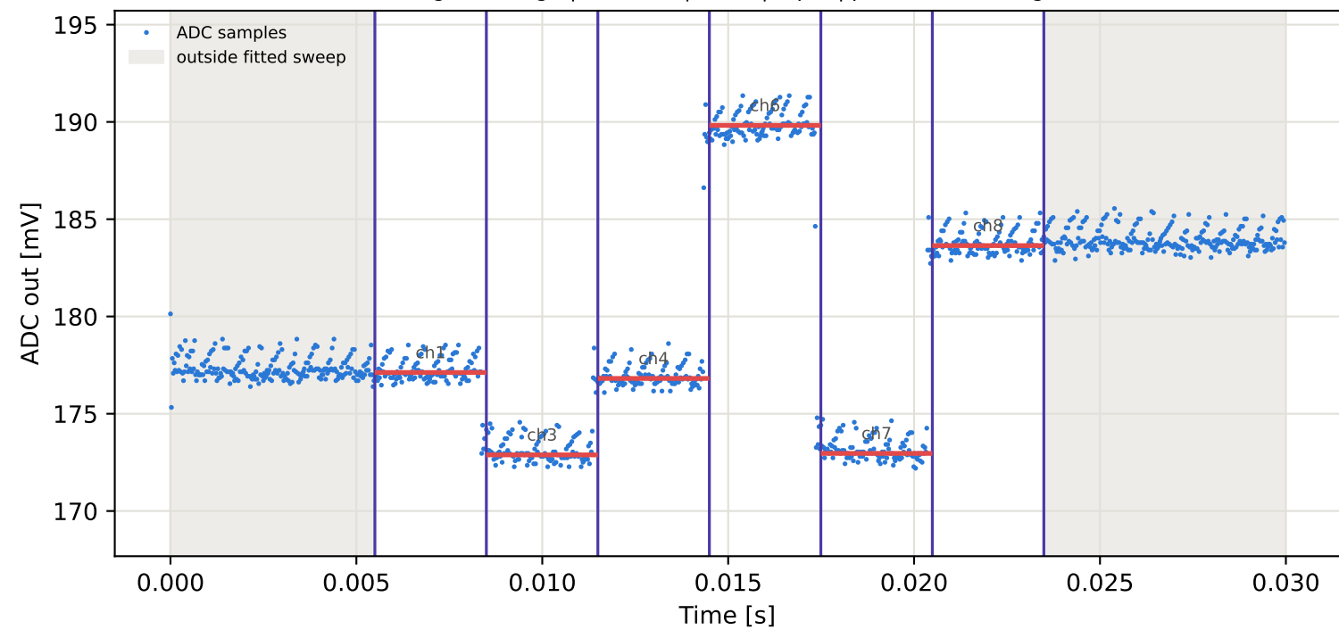
Tag10 &lt;- Tag8 | 985 MHz | run 0 | rep 1 | phase -5.13 deg
