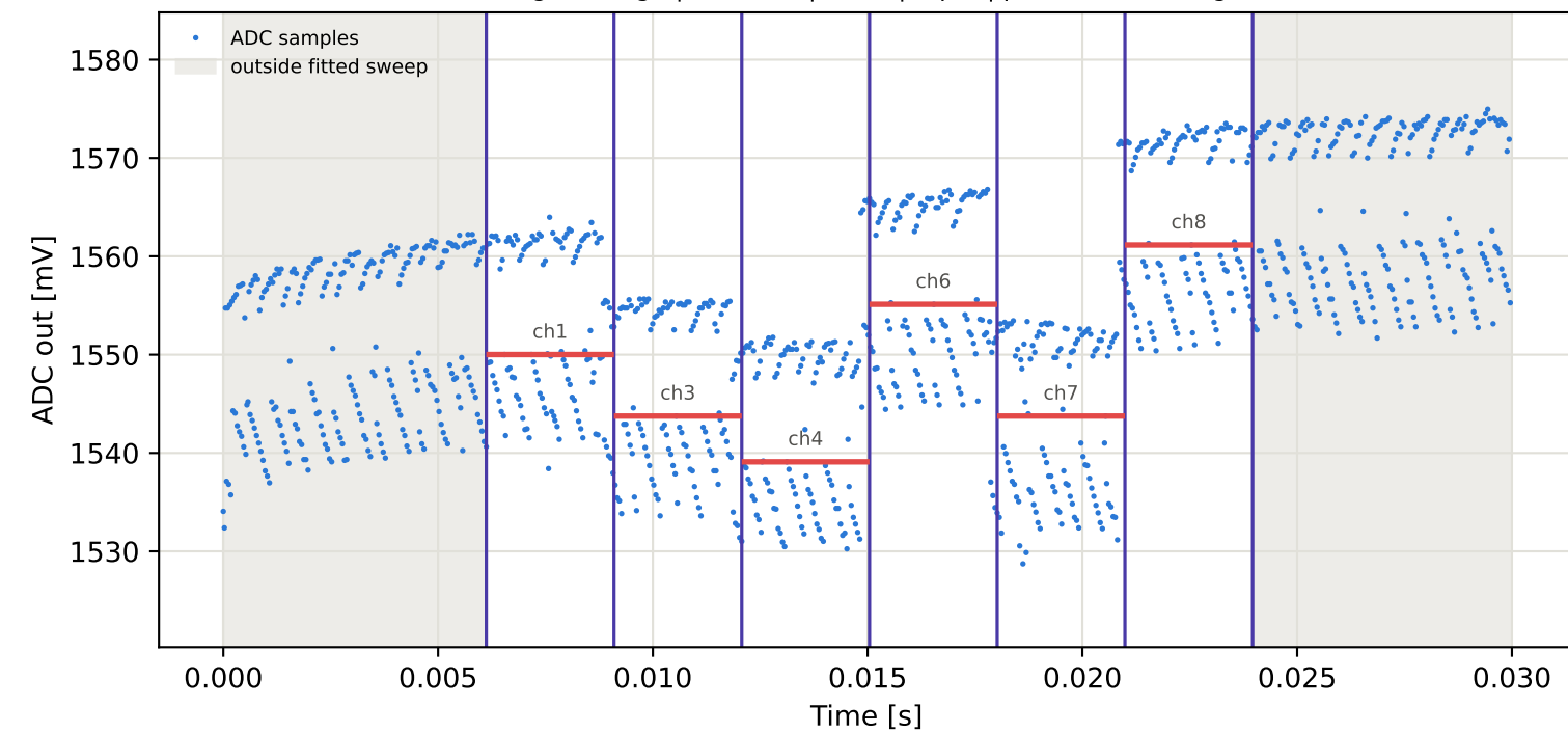
Tag9 &lt;- Tag10 | 915 MHz | run 0 | rep 1 | phase 121.61 deg
