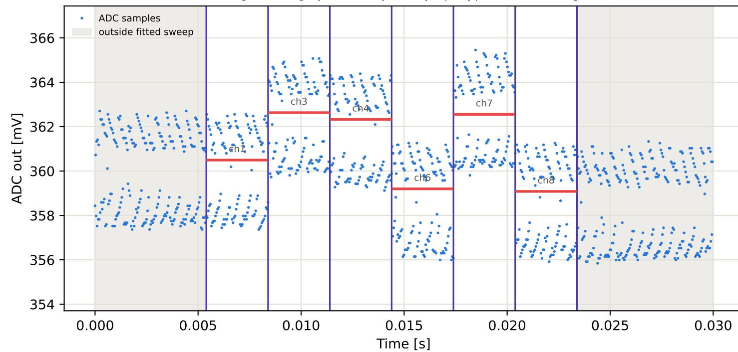
Tag15 &lt;- Tag9 | 825 MHz | run 0 | rep 1 | phase -170.58 deg
