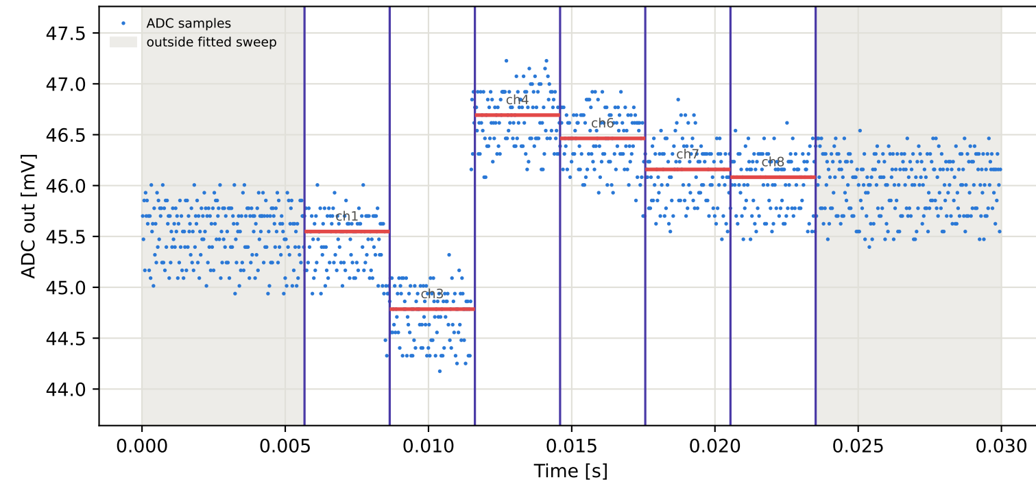
Tag1 &lt;- Tag3 | 775 MHz | run 0 | rep 1 | phase -75.42 deg
