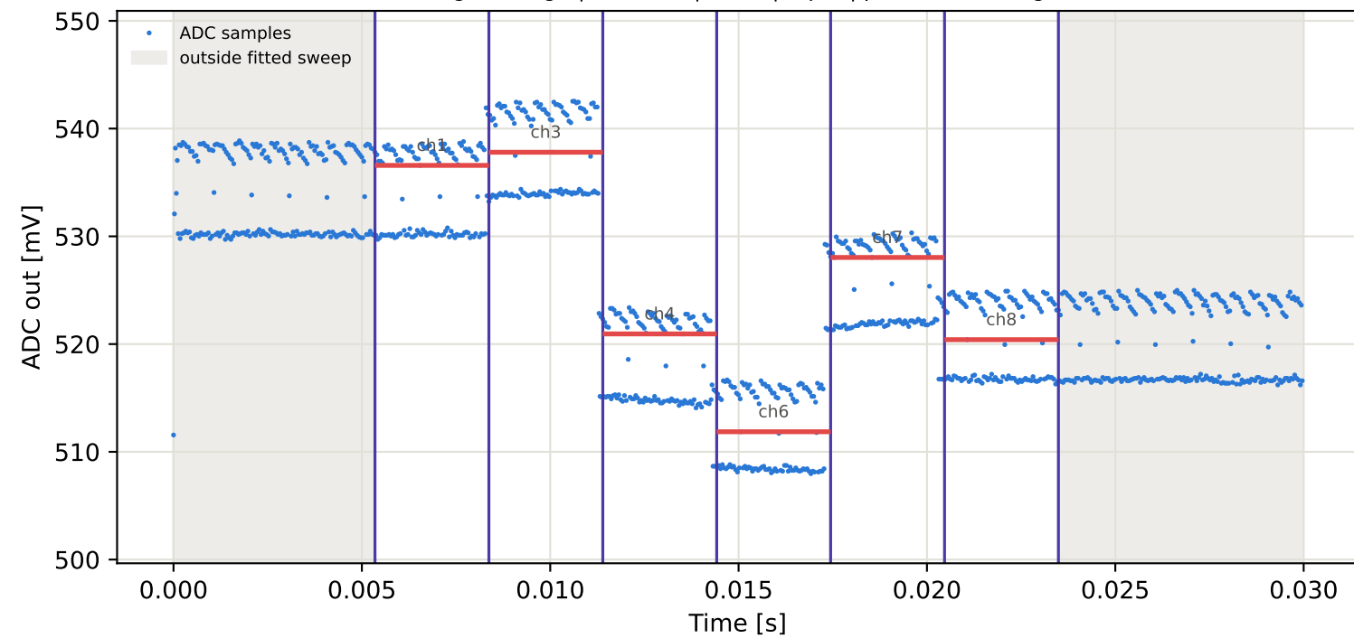
Tag8 &lt;- Tag10 | 845 MHz | run 0 | rep 1 | phase -106.60 deg
