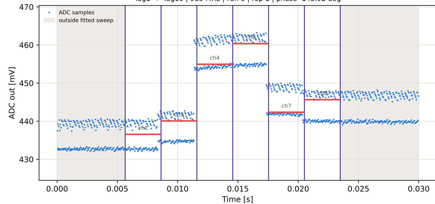
Tag1 &lt;- Tag16 | 985 MHz | run 0 | rep 1 | phase -35.73 deg
