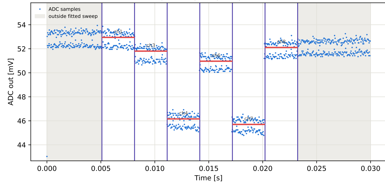
Tag1 &lt;- Tag4 | 775 MHz | run 0 | rep 1 | phase 103.03 deg
