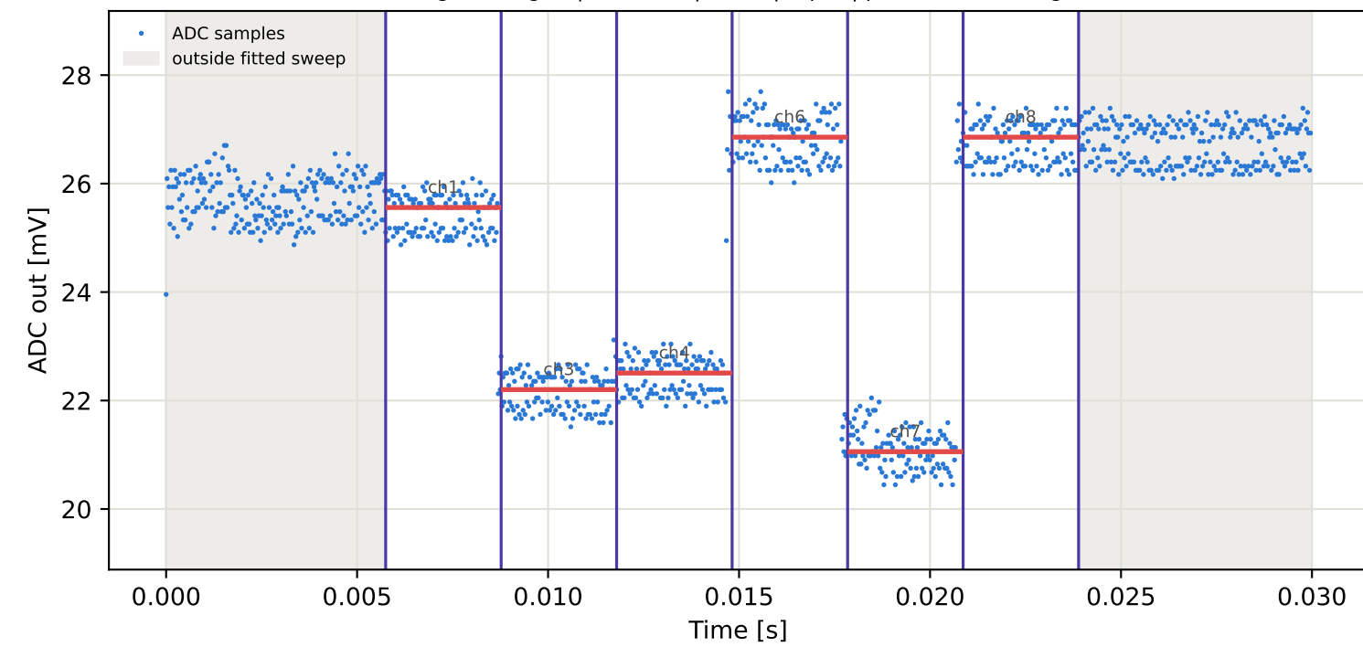
Tag5 &lt;- Tag2 | 805 MHz | run 0 | rep 1 | phase 22.77 deg
