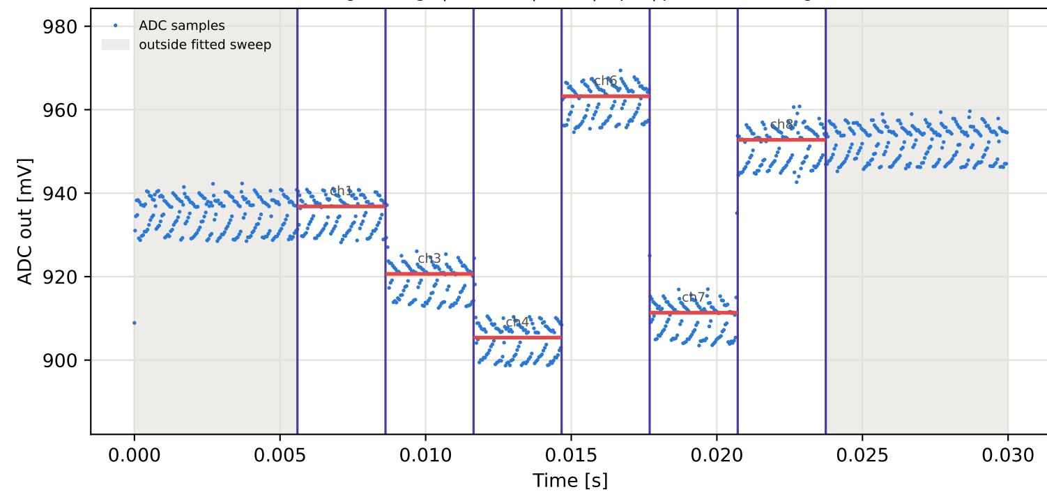
Tag8 &lt;- Tag5 | 965 MHz | run 0 | rep 1 | phase -159.62 deg
