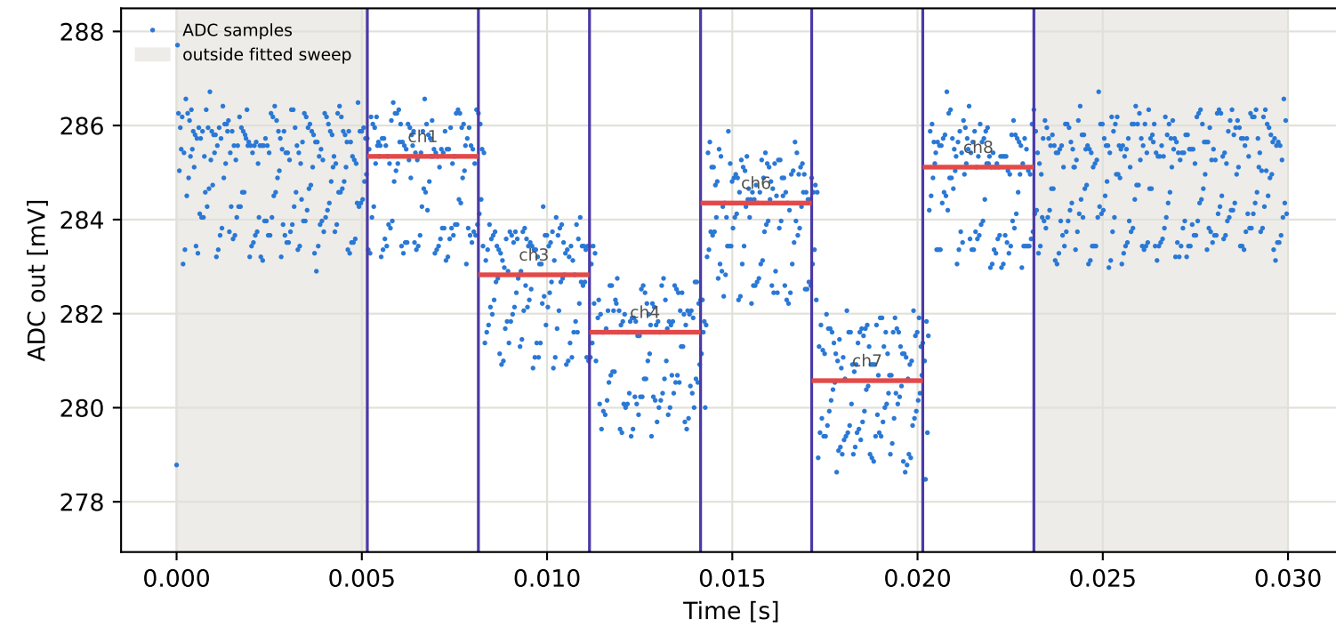
Tag2 &lt;- Tag15 | 825 MHz | run 0 | rep 1 | phase 136.15 deg
