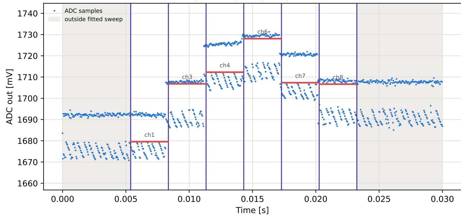
Tag8 &lt;- Tag7 | 885 MHz | run 0 | rep 1 | phase -135.59 deg
