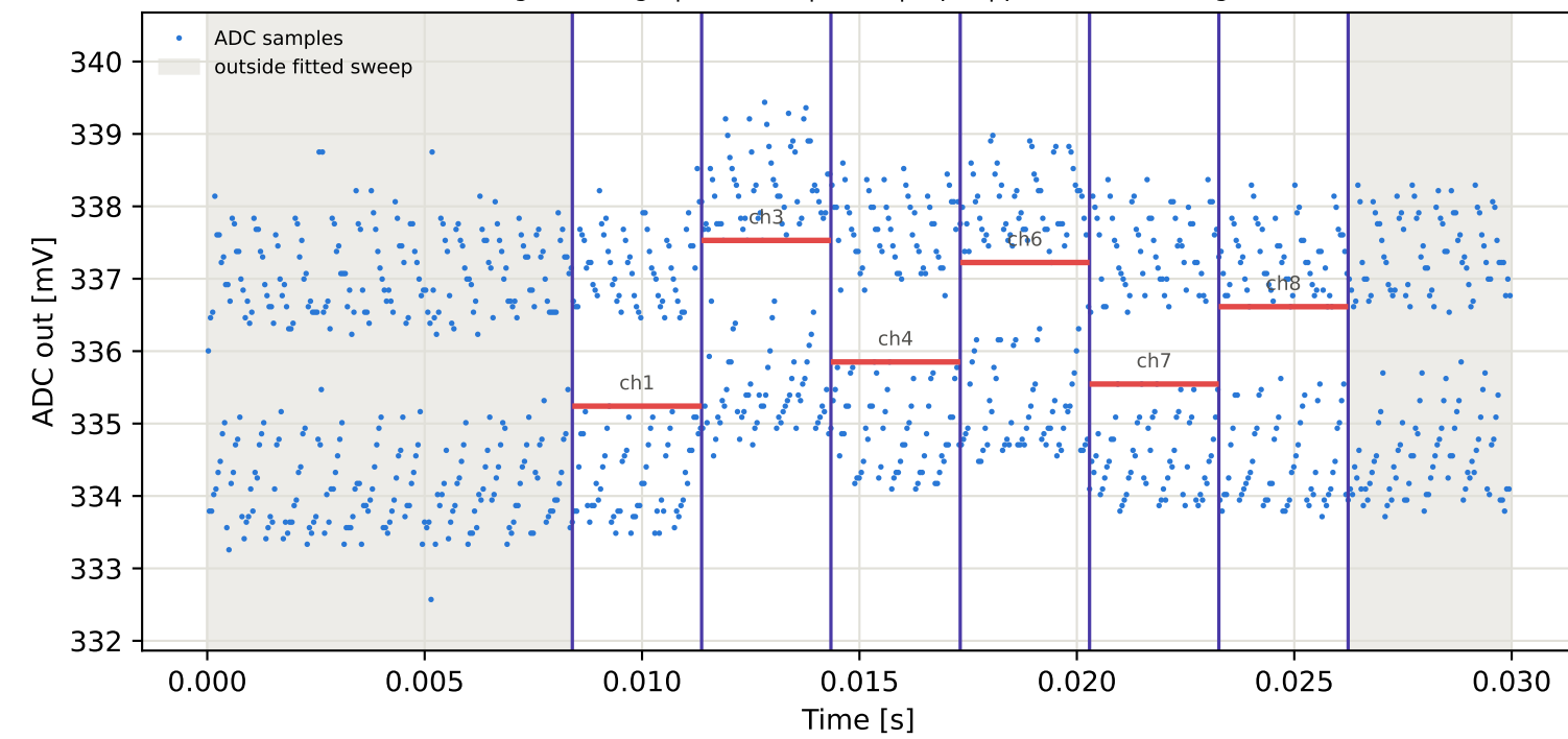
Tag15 &lt;- Tag9 | 775 MHz | run 0 | rep 1 | phase 45.85 deg
