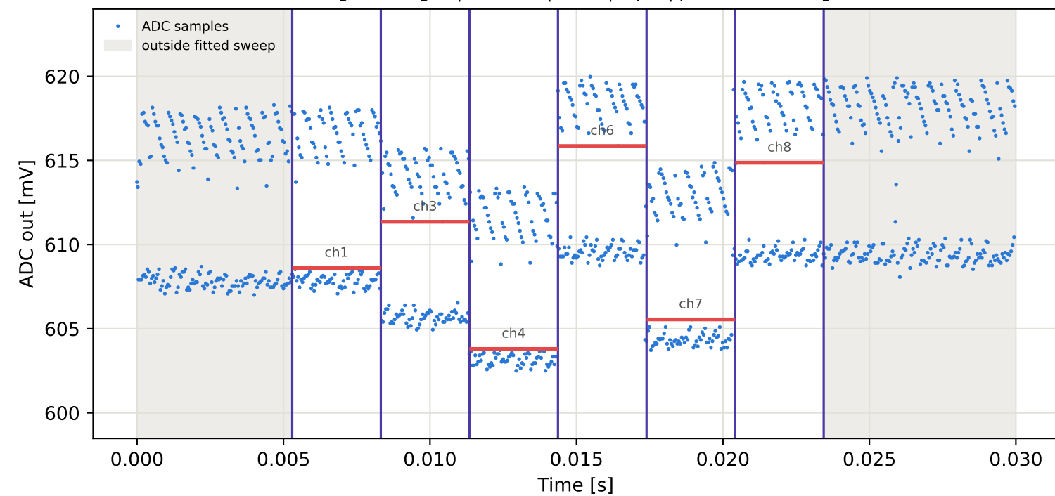
Tag15 &lt;- Tag10 | 985 MHz | run 0 | rep 1 | phase 124.08 deg
