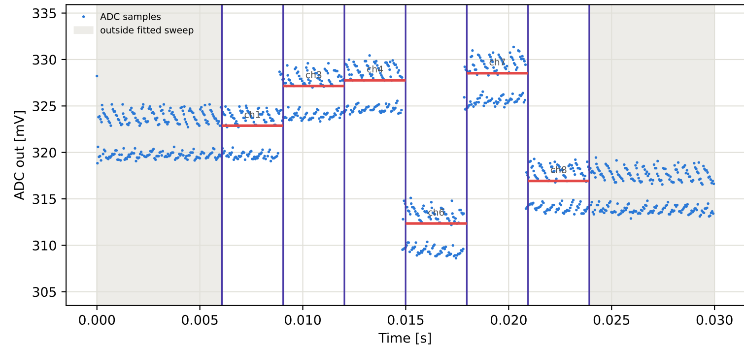
Tag7 &lt;- Tag15 | 995 MHz | run 0 | rep 1 | phase 77.48 deg
