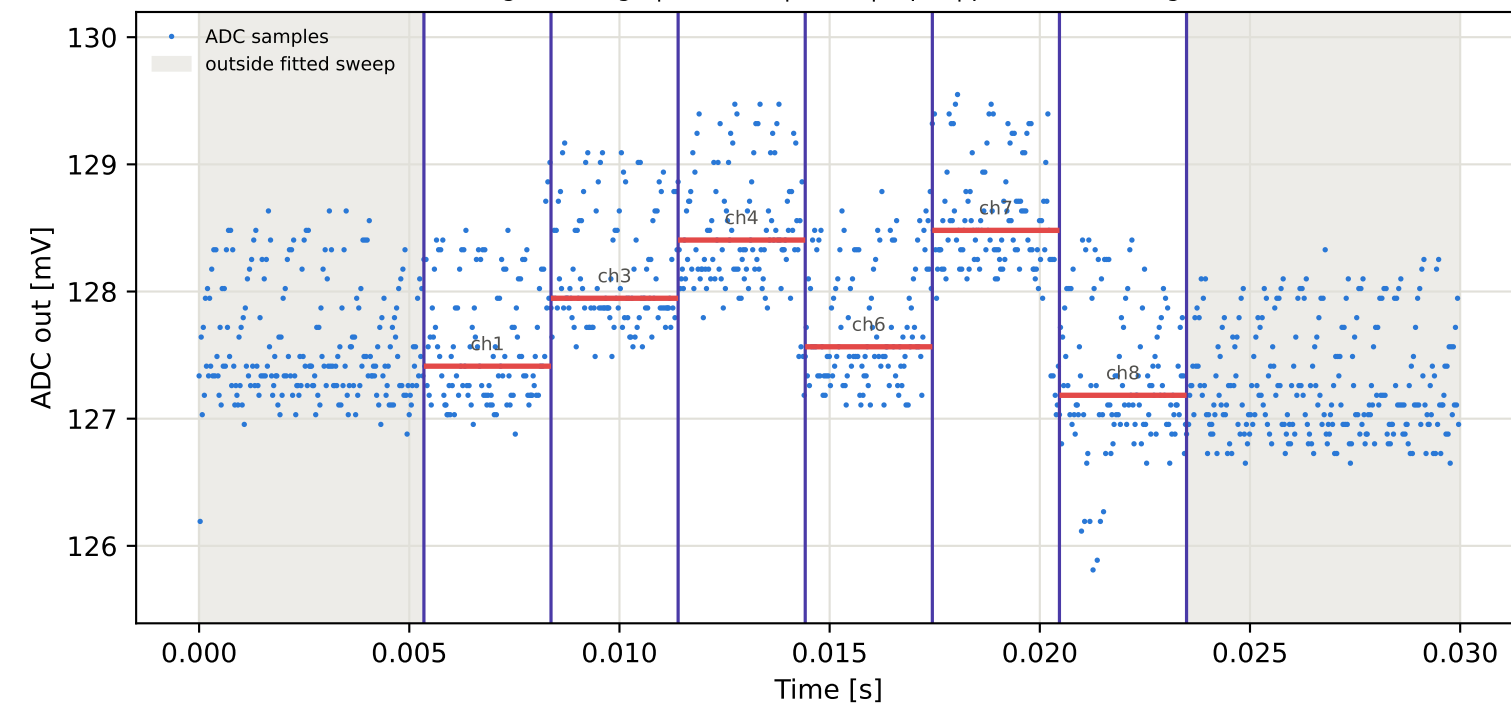
Tag16 &lt;- Tag4 | 775 MHz | run 0 | rep 1 | phase 9.25 deg
