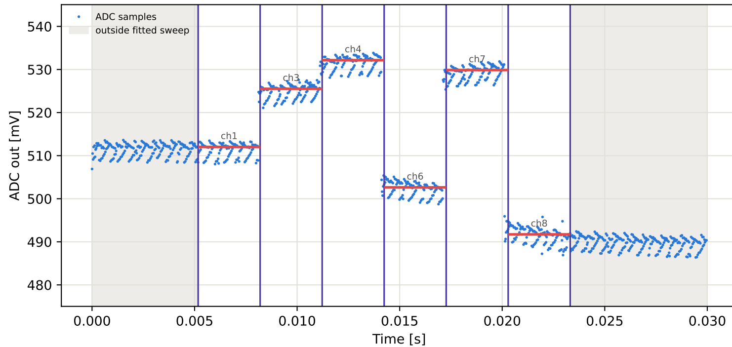
Tag15 &lt;- Tag1 | 905 MHz | run 0 | rep 1 | phase -61.61 deg
