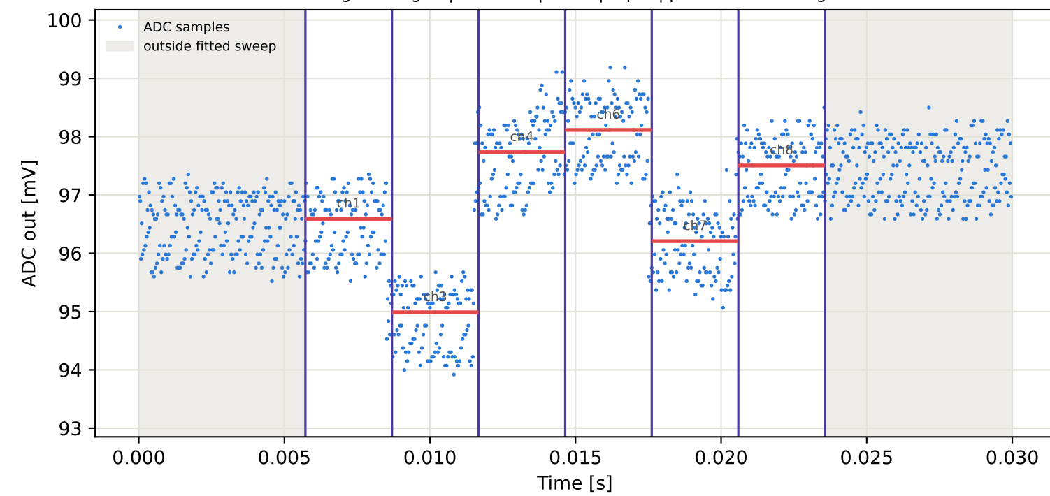
Tag5 &lt;- Tag16 | 775 MHz | run 0 | rep 1 | phase 105.83 deg
