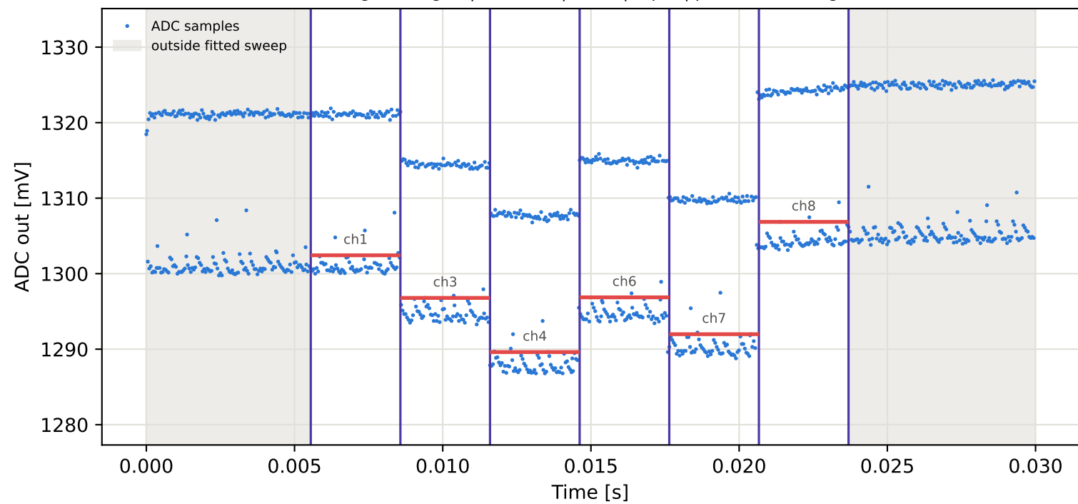
Tag4 &lt;- Tag16 | 915 MHz | run 0 | rep 1 | phase 3.93 deg
