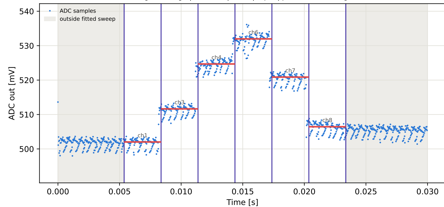
Tag10 &lt;- Tag5 | 905 MHz | run 0 | rep 1 | phase -162.74 deg
