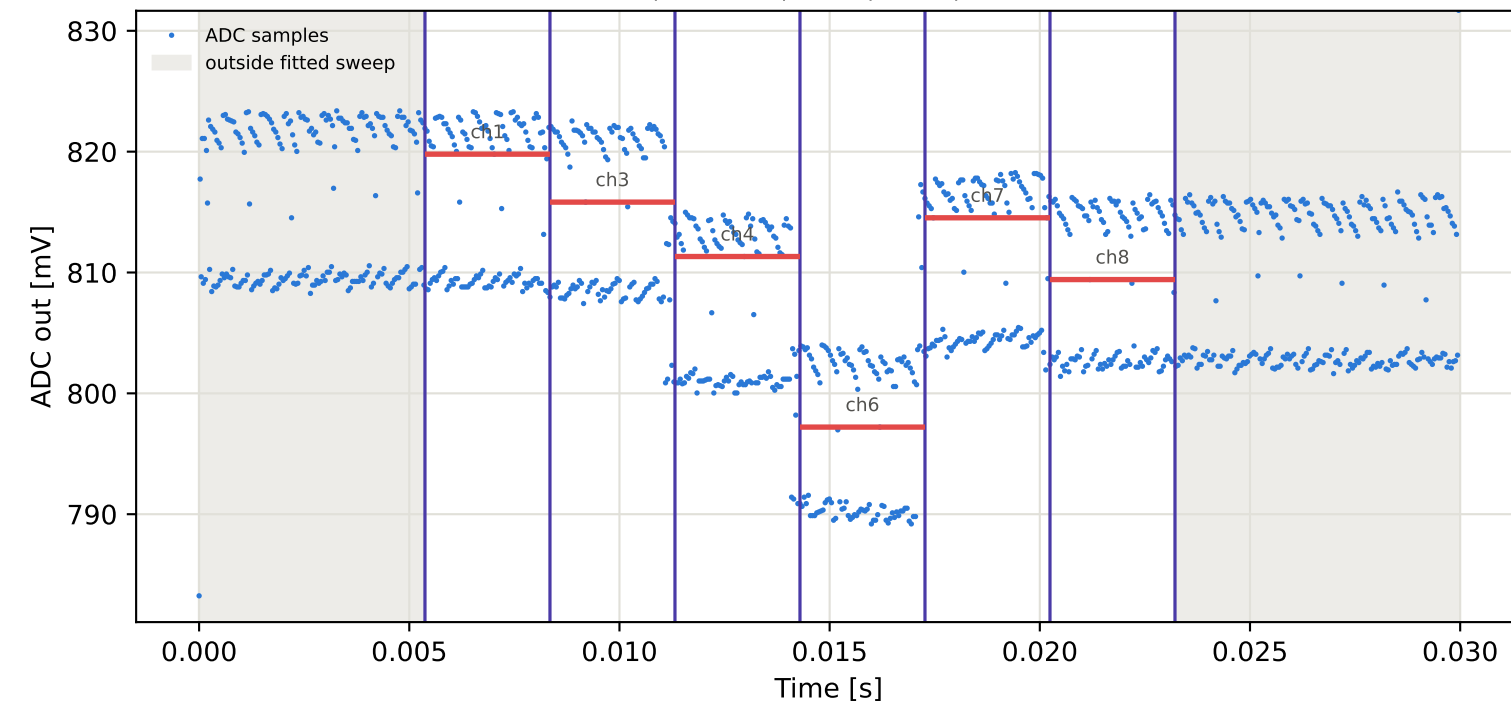
Tag9 &lt;- Tag7 | 925 MHz | run 0 | rep 1 | phase 21.52 deg
