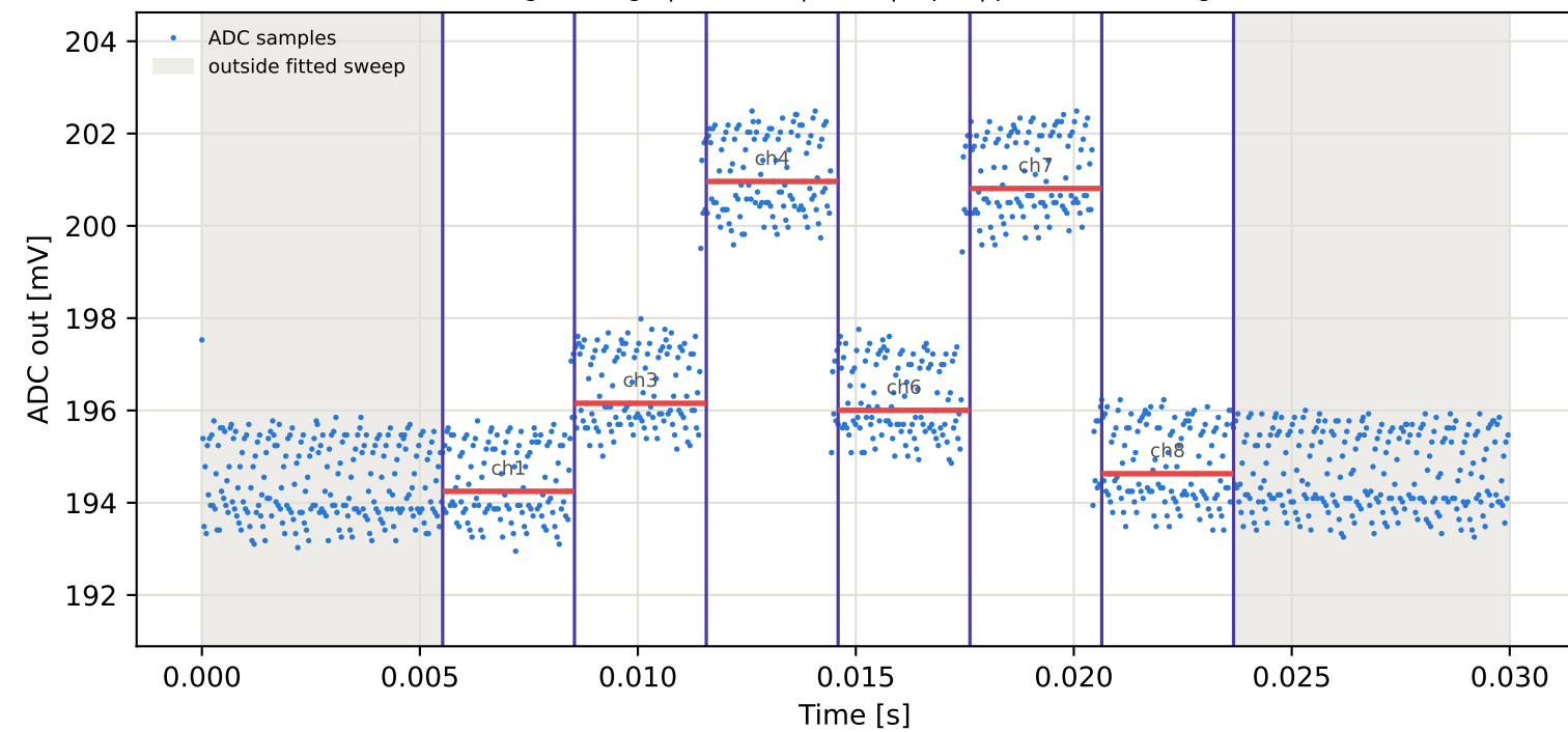
Tag3 &lt;- Tag15 | 805 MHz | run 0 | rep 1 | phase -91.69 deg
