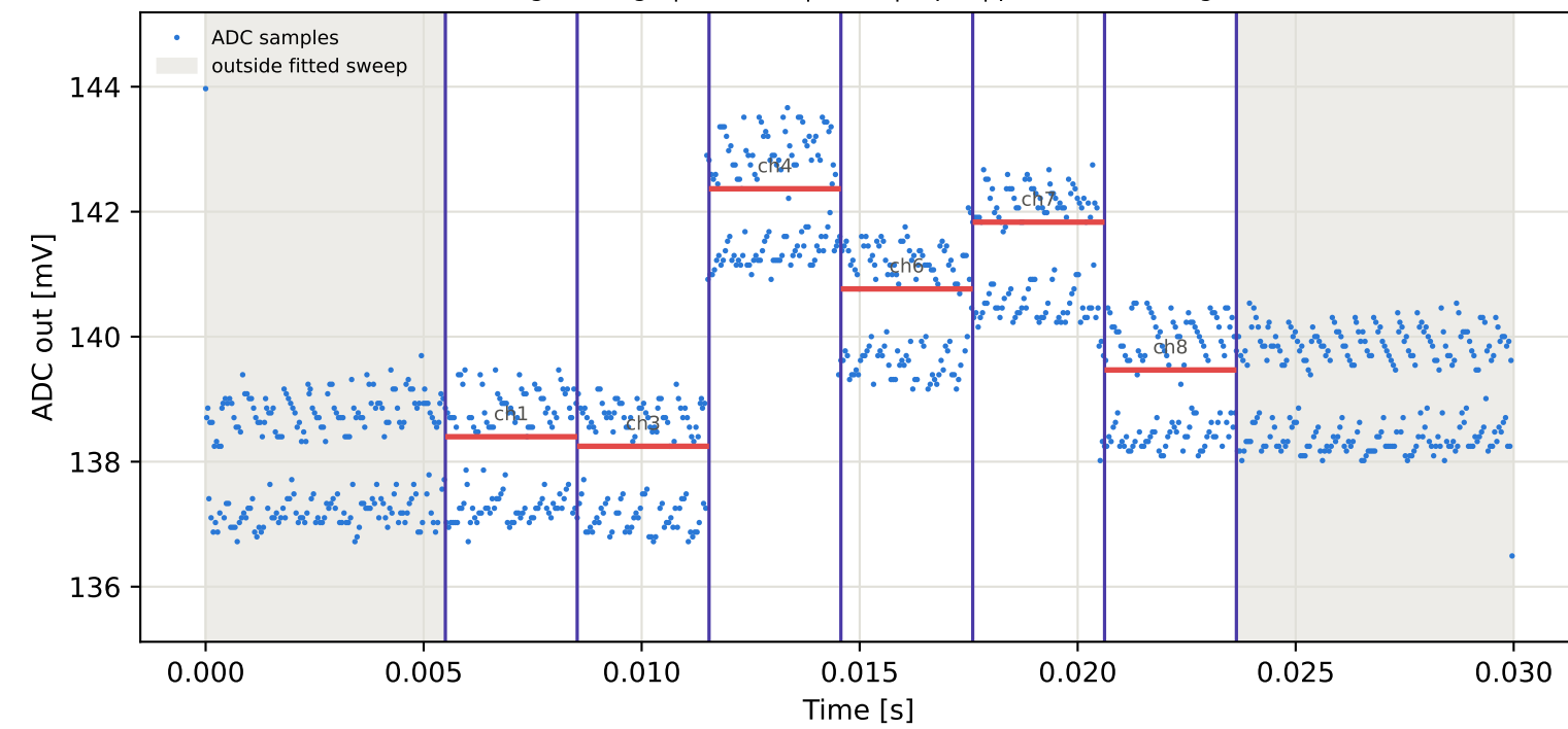
Tag9 &lt;- Tag10 | 775 MHz | run 0 | rep 1 | phase -171.93 deg
