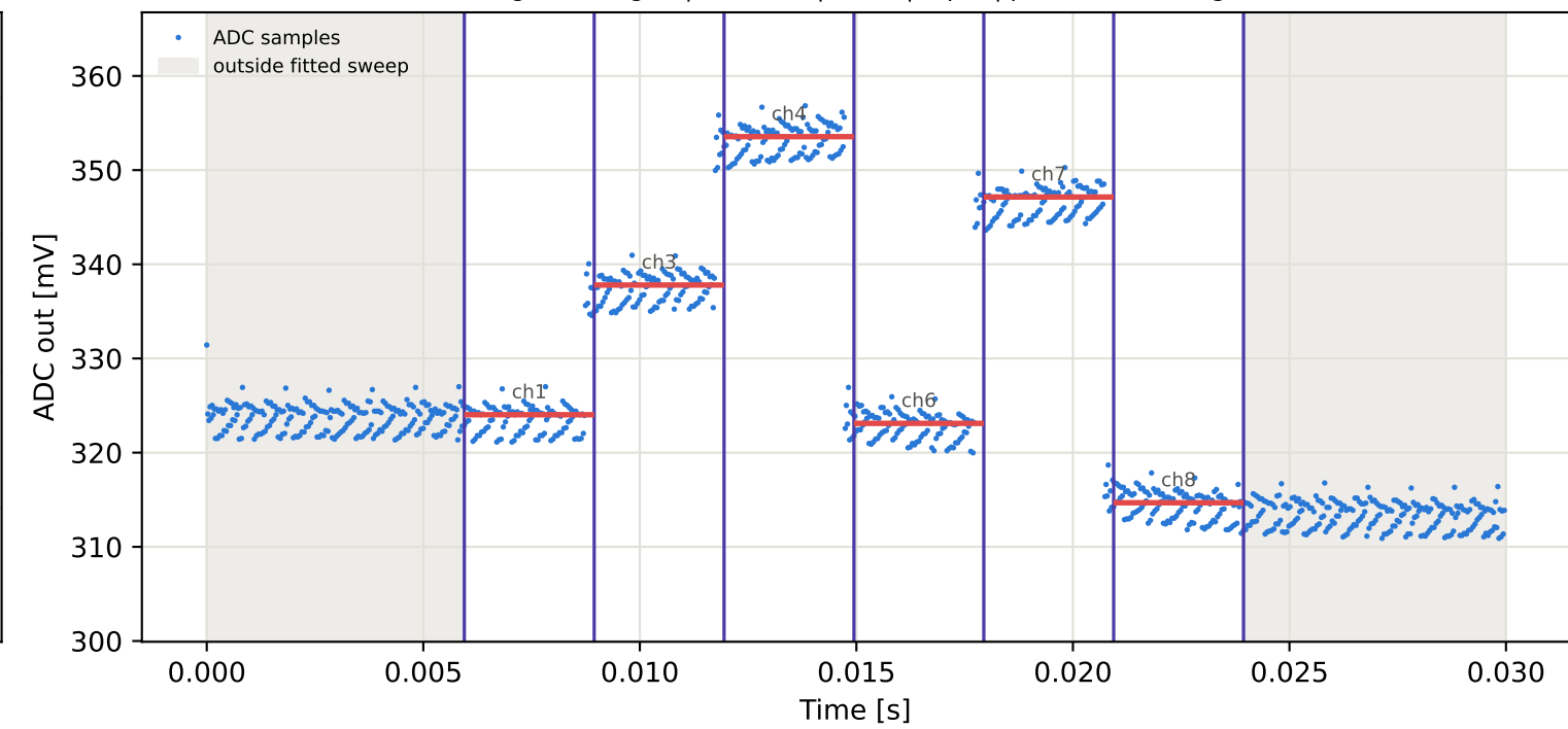
Tag10 &lt;- Tag3 | 935 MHz | run 0 | rep 1 | phase -176.45 deg
