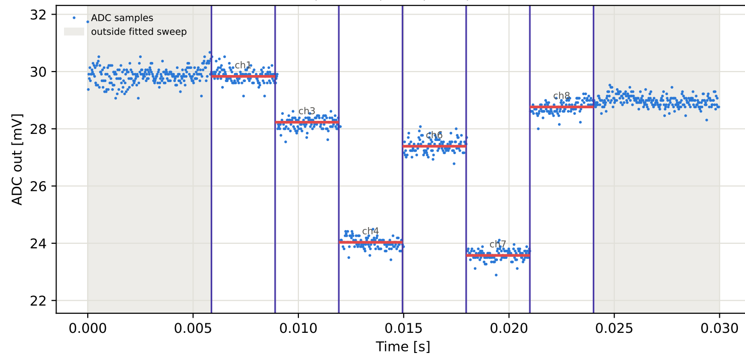
Tag6 &lt;- Tag4 | 795 MHz | run 0 | rep 1 | phase 97.72 deg
