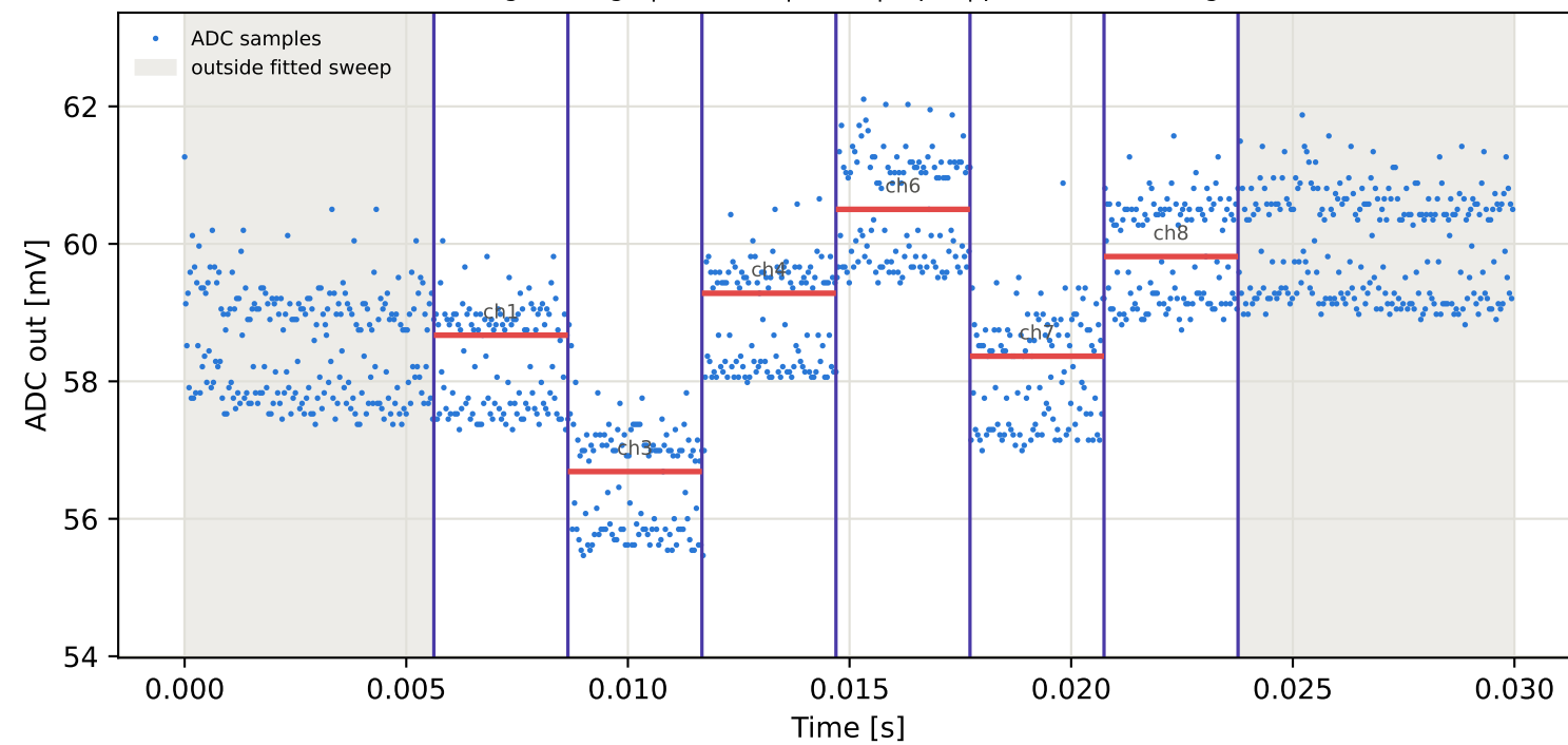
Tag3 &lt;- Tag10 | 805 MHz | run 0 | rep 1 | phase 63.89 deg
