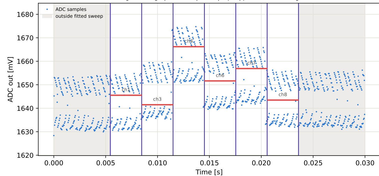
Tag16 &lt;- Tag6 | 975 MHz | run 0 | rep 1 | phase -115.58 deg
