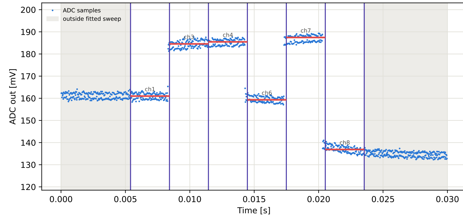
Tag7 &lt;- Tag10 | 885 MHz | run 0 | rep 1 | phase -79.11 deg
