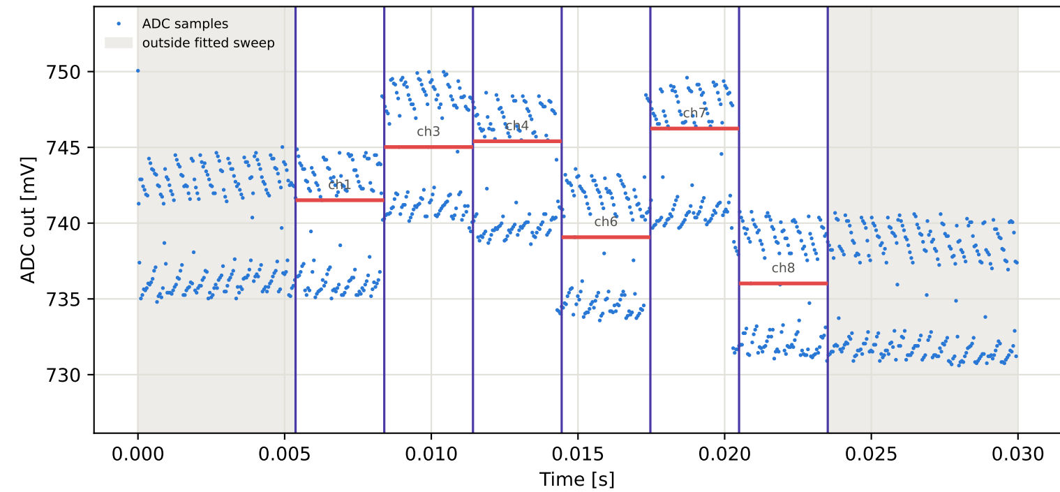
Tag16 &lt;- Tag7 | 865 MHz | run 0 | rep 1 | phase -8.80 deg
