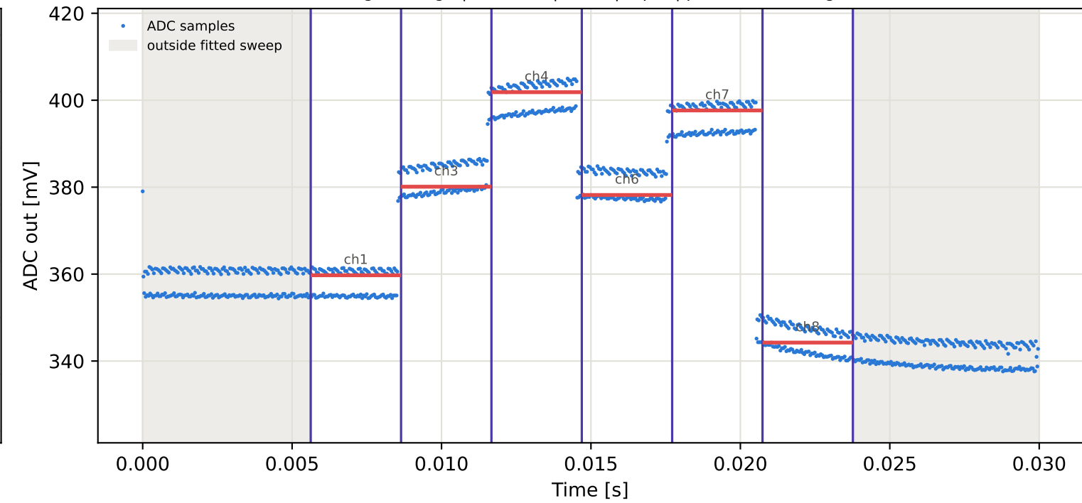
Tag1 &lt;- Tag8 | 895 MHz | run 0 | rep 1 | phase -95.52 deg
