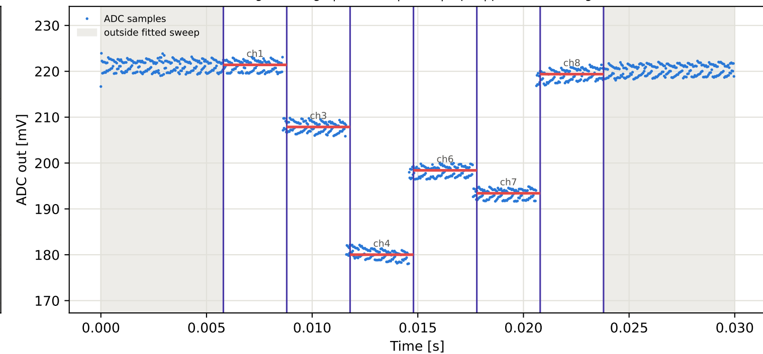
Tag10 &lt;- Tag1 | 945 MHz | run 0 | rep 1 | phase 72.01 deg
