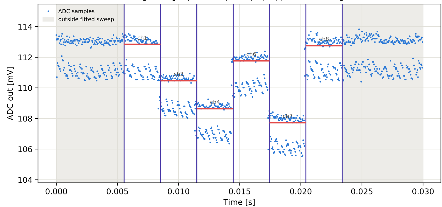
Tag6 &lt;- Tag3 | 785 MHz | run 0 | rep 1 | phase 118.07 deg
