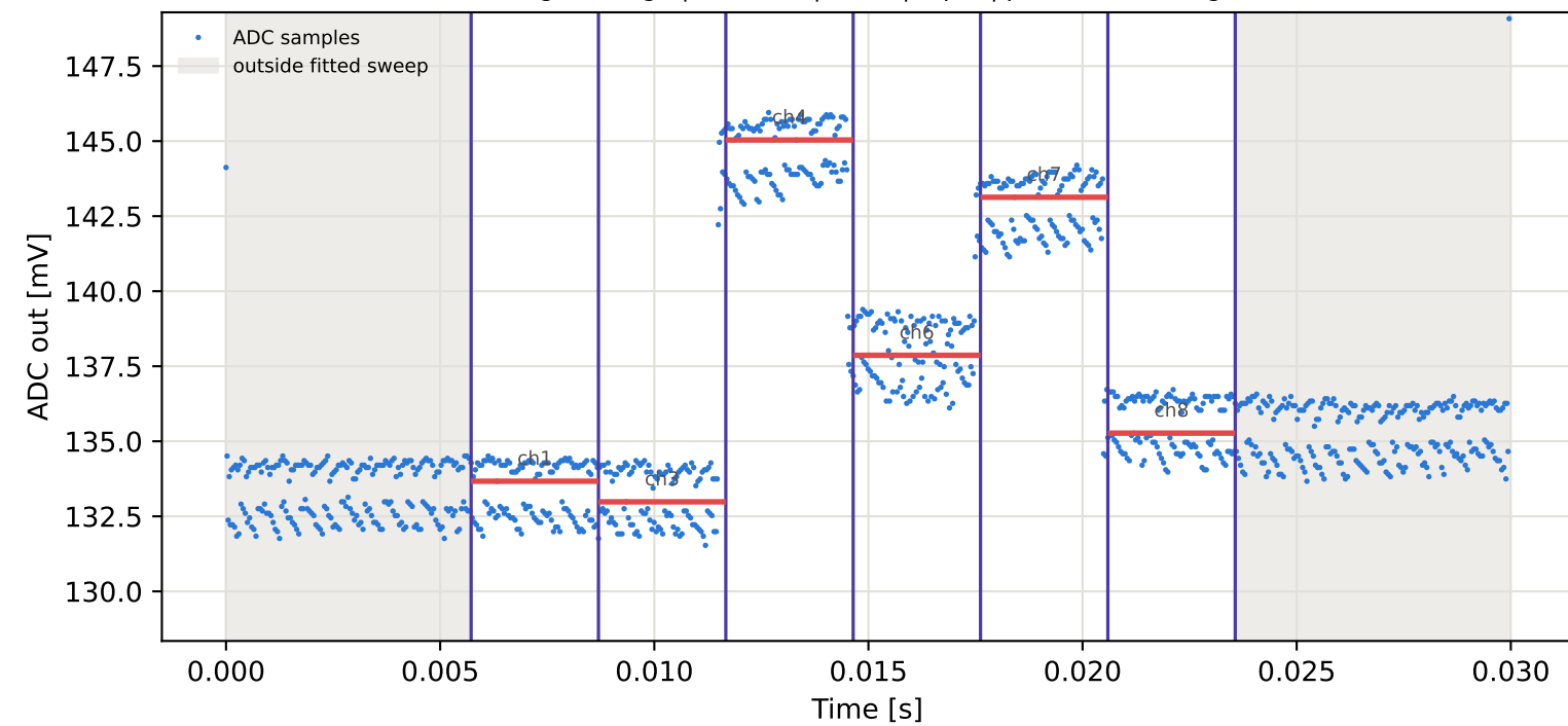
Tag8 &lt;- Tag5 | 775 MHz | run 0 | rep 1 | phase 170.24 deg
