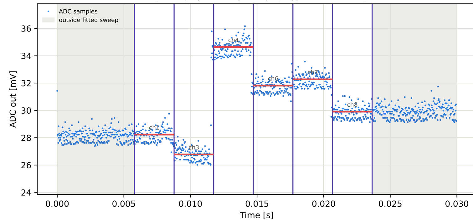
Tag2 &lt;- Tag5 | 775 MHz | run 0 | rep 1 | phase 51.44 deg
