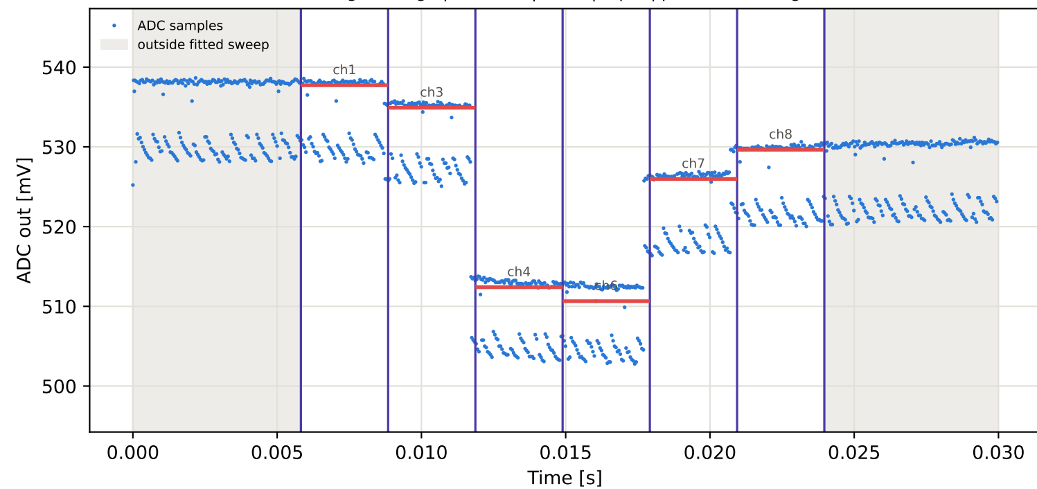
Tag9 &lt;- Tag8 | 965 MHz | run 0 | rep 1 | phase 57.32 deg
