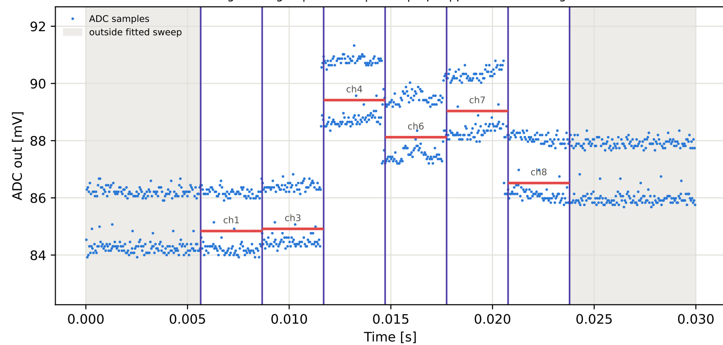
Tag1 &lt;- Tag2 | 825 MHz | run 0 | rep 1 | phase 46.84 deg
