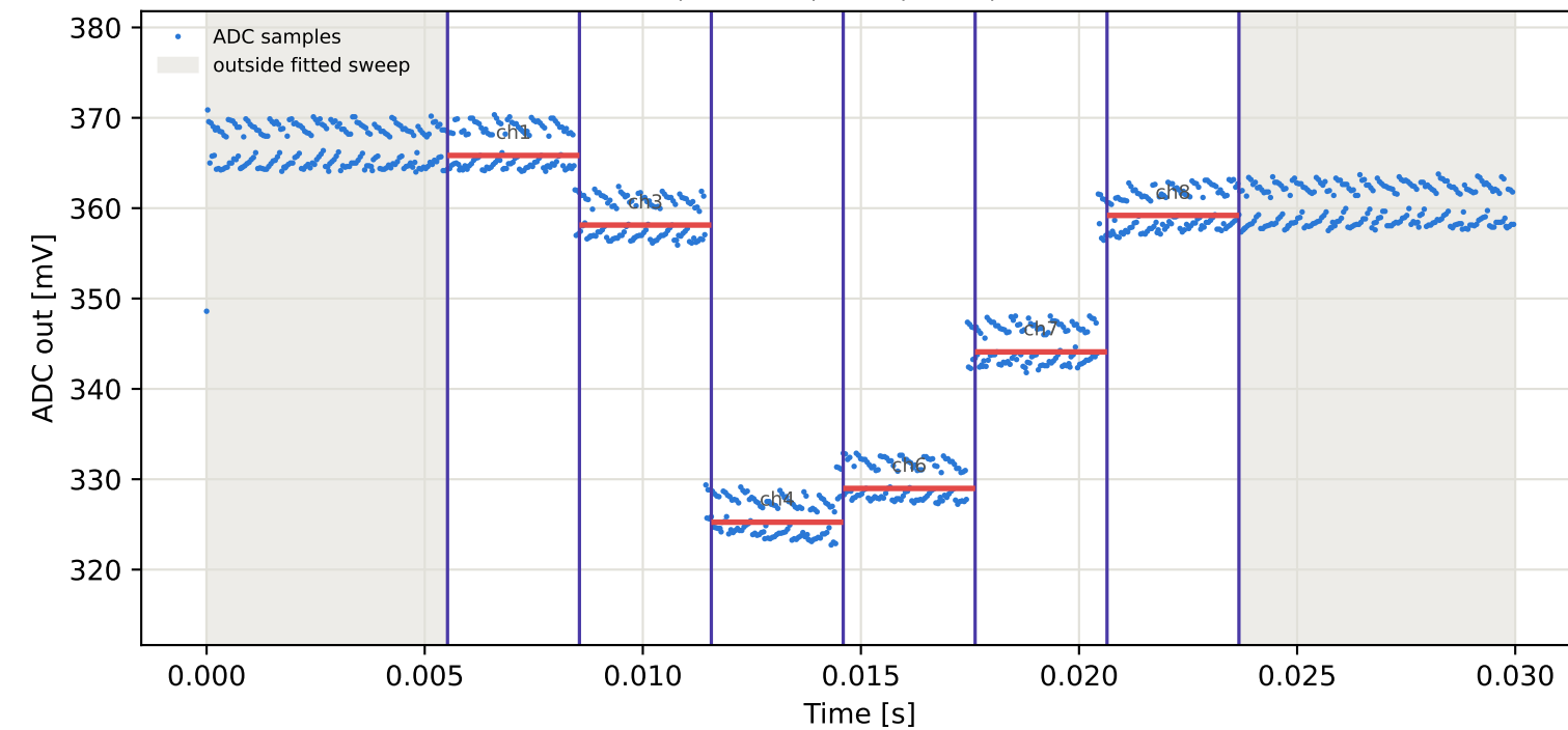
Tag5 &lt;- Tag3 | 955 MHz | run 0 | rep 1 | phase 50.23 deg
