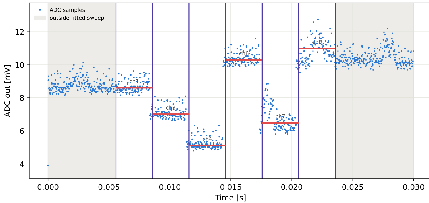
Tag2 &lt;- Tag5 | 955 MHz | run 0 | rep 1 | phase 122.84 deg
