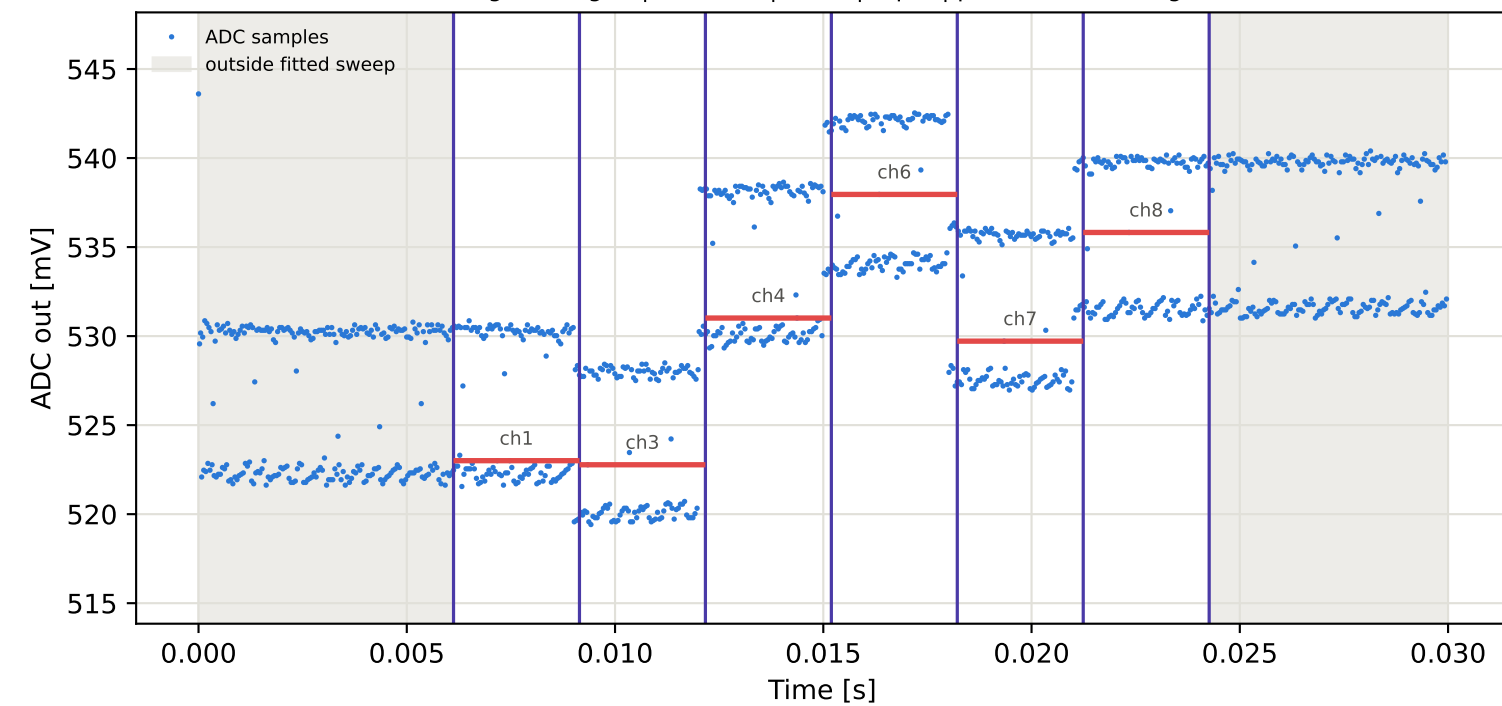
Tag5 &lt;- Tag3 | 835 MHz | run 0 | rep 1 | phase -139.29 deg
