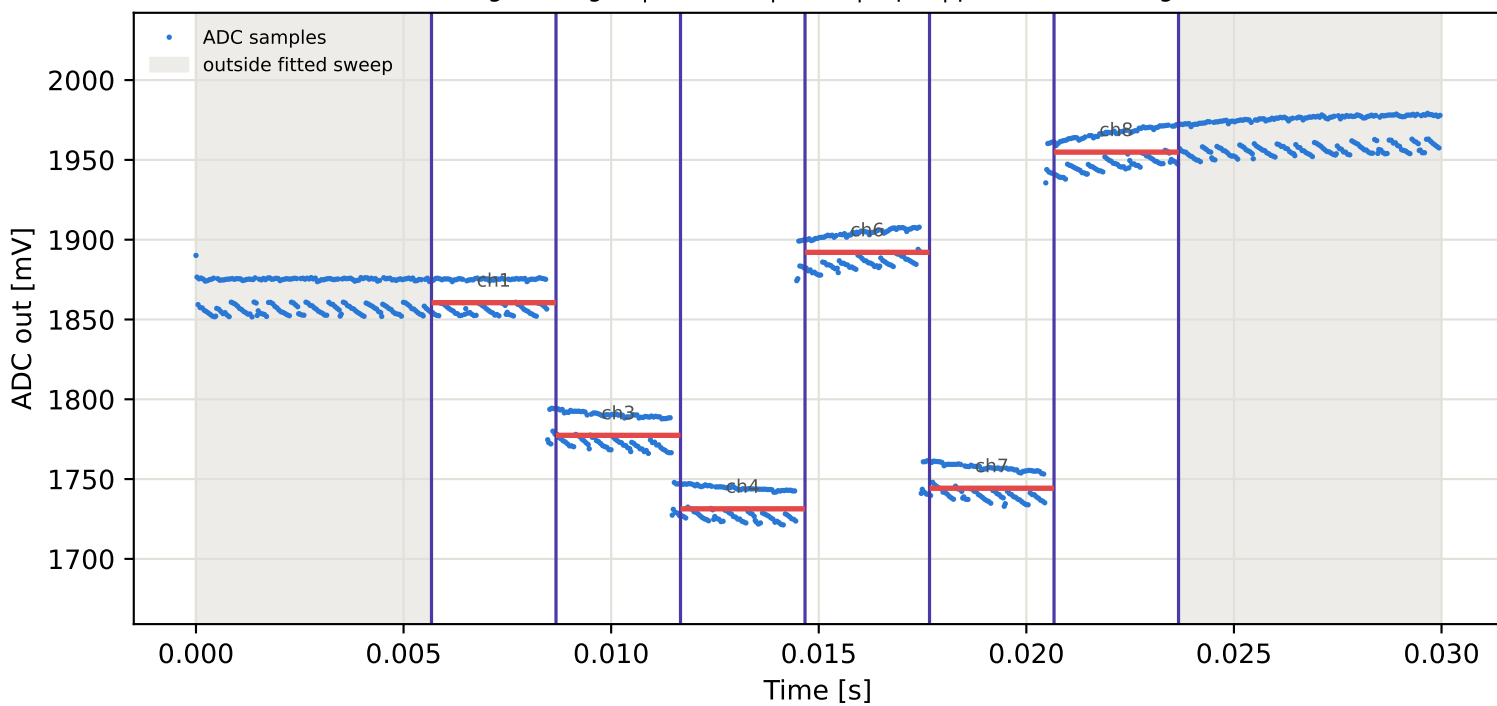
Tag8 &lt;- Tag16 | 895 MHz | run 0 | rep 1 | phase 127.81 deg
