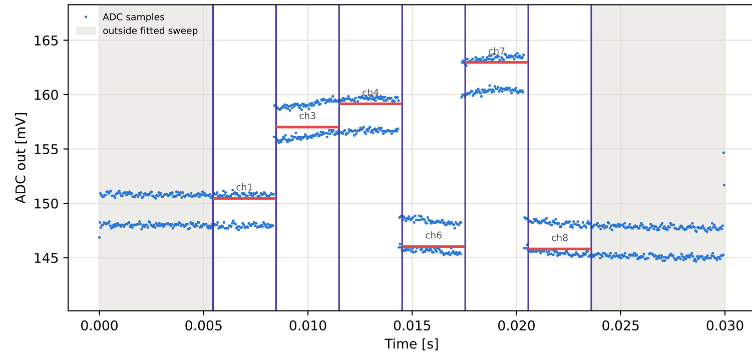
Tag4 &lt;- Tag2 | 795 MHz | run 0 | rep 1 | phase -119.20 deg
