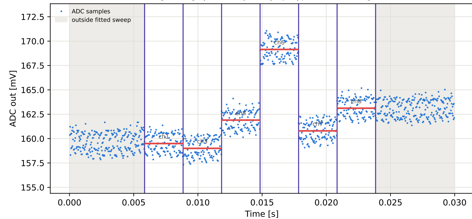
Tag2 &lt;- Tag5 | 935 MHz | run 0 | rep 1 | phase 59.63 deg
