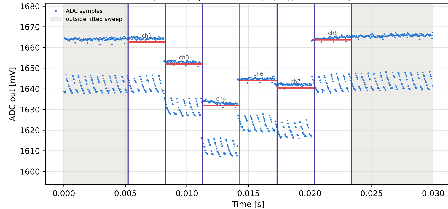
Tag16 &lt;- Tag10 | 935 MHz | run 0 | rep 1 | phase 94.30 deg
