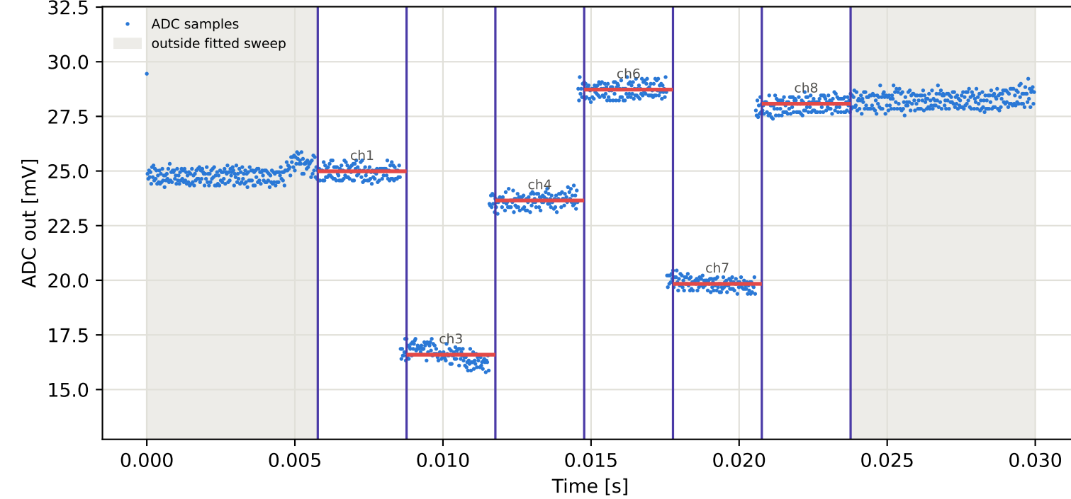
Tag5 &lt;- Tag3 | 805 MHz | run 0 | rep 1 | phase 115.50 deg
