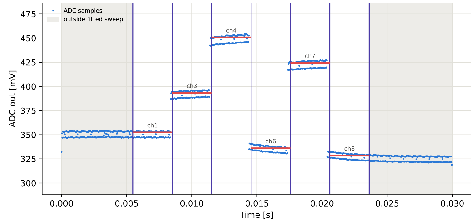
Tag5 &lt;- Tag1 | 975 MHz | run 0 | rep 1 | phase -167.26 deg
