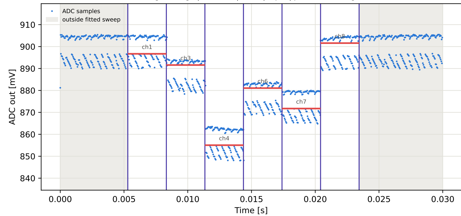
Tag8 &lt;- Tag5 | 955 MHz | run 0 | rep 1 | phase -166.00 deg
