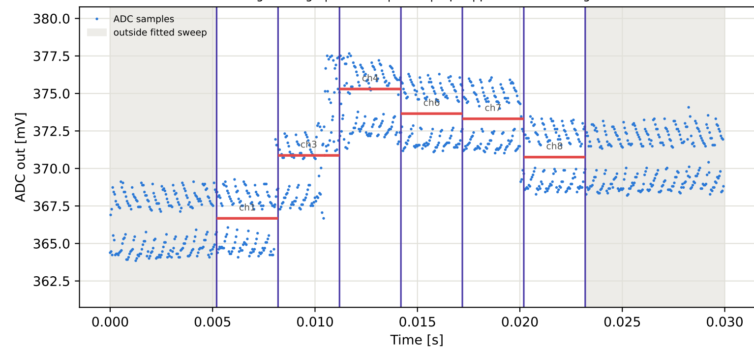
Tag9 &lt;- Tag5 | 835 MHz | run 0 | rep 1 | phase 93.34 deg
