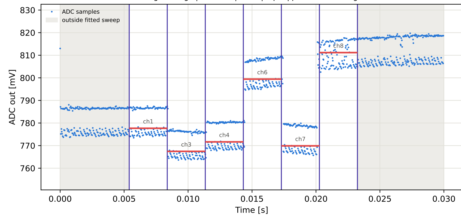
Tag3 &lt;- Tag7 | 885 MHz | run 0 | rep 1 | phase 104.31 deg
