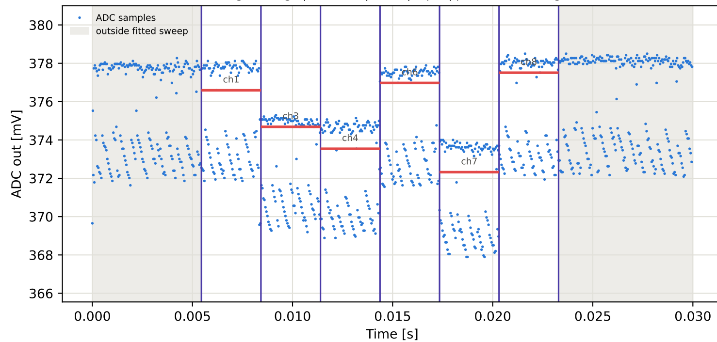
Tag4 &lt;- Tag15 | 825 MHz | run 0 | rep 1 | phase 75.10 deg
