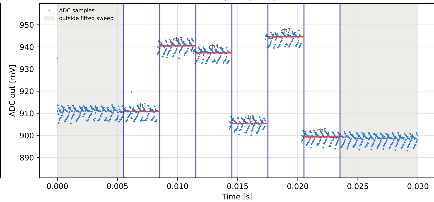
Tag2 &lt;- Tag10 | 845 MHz | run 0 | rep 1 | phase -103.97 deg
