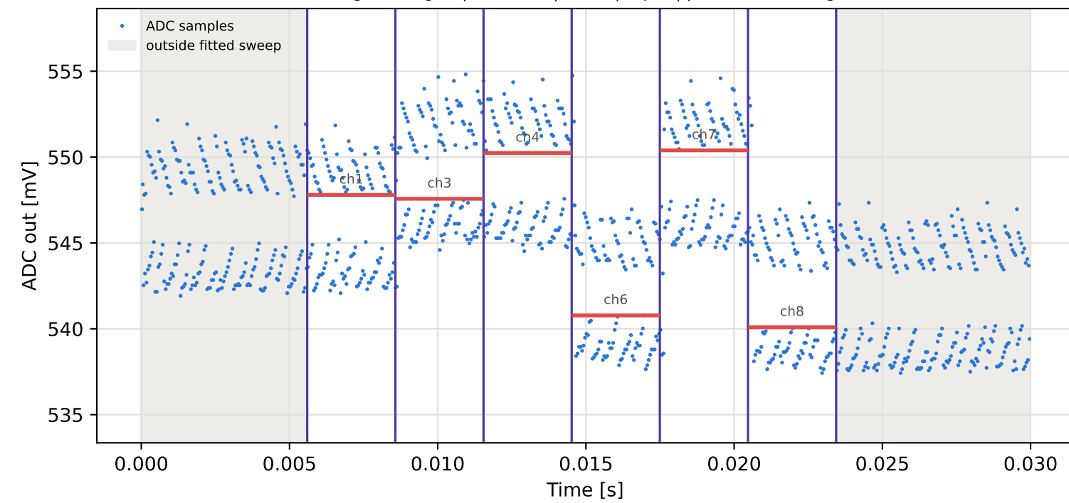
Tag6 &lt;- Tag2 | 915 MHz | run 0 | rep 1 | phase 18.99 deg
