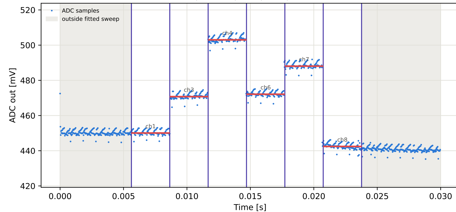
Tag6 &lt;- Tag4 | 935 MHz | run 0 | rep 1 | phase -96.61 deg
