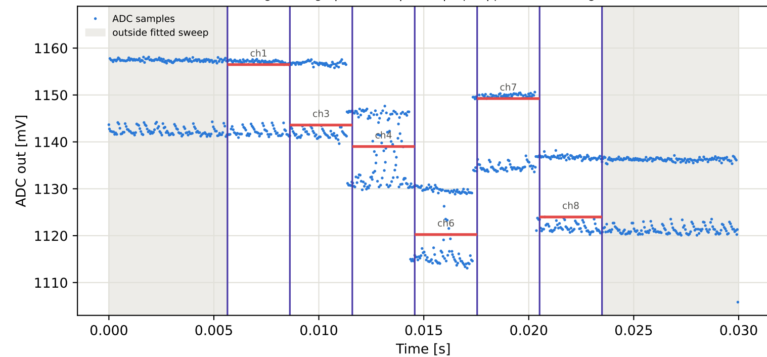
Tag8 &lt;- Tag6 | 875 MHz | run 0 | rep 1 | phase -57.78 deg
