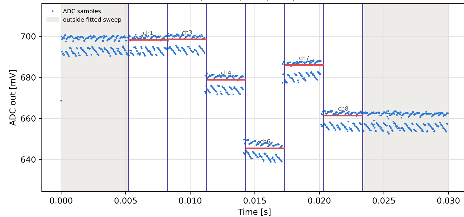
Tag9 &lt;- Tag5 | 885 MHz | run 0 | rep 1 | phase -128.24 deg
