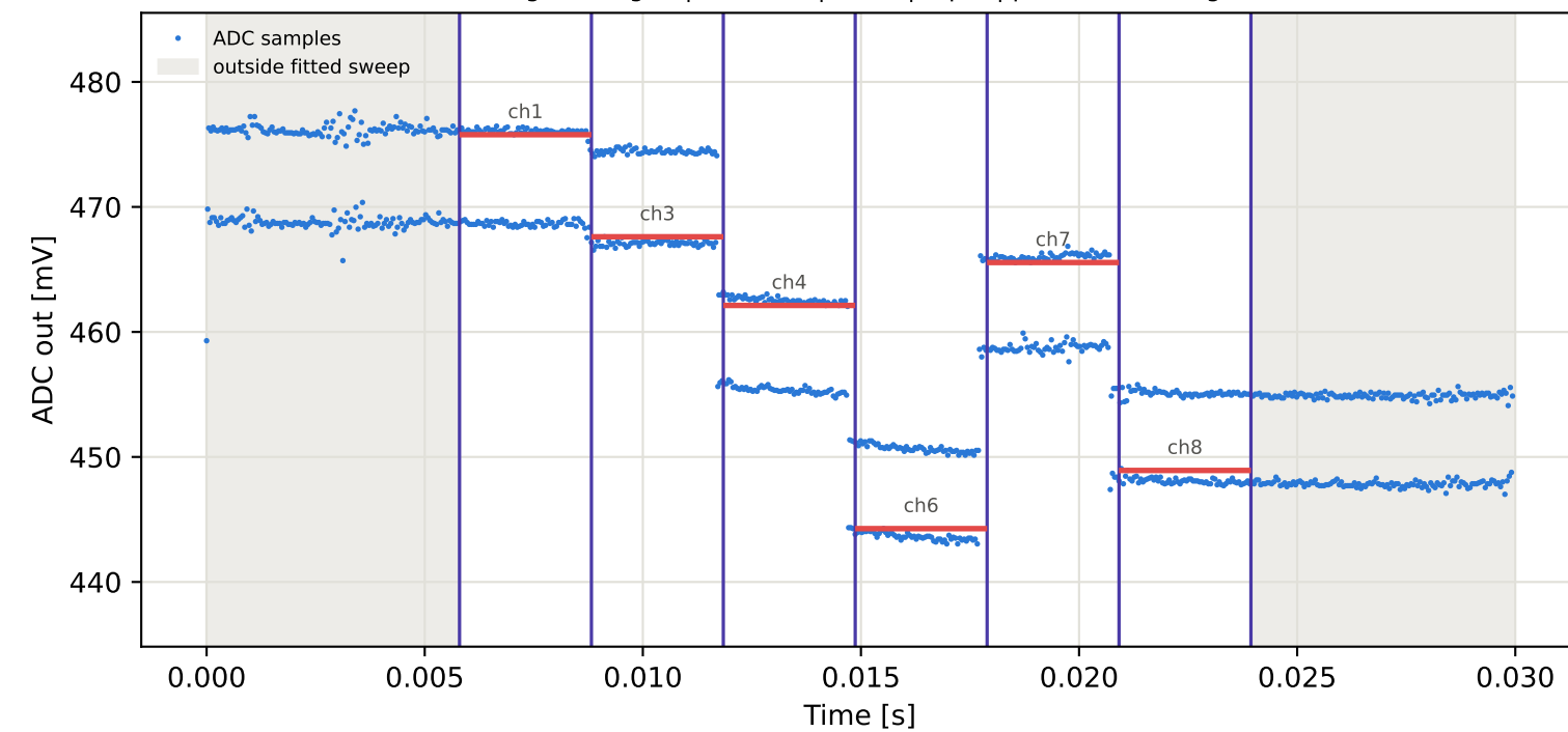
Tag4 &lt;- Tag2 | 875 MHz | run 0 | rep 1 | phase 41.24 deg
