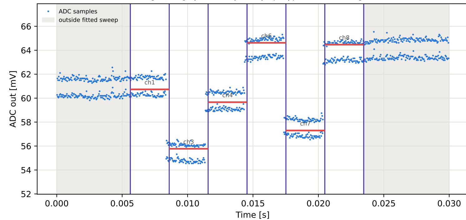
Tag1 &lt;- Tag7 | 835 MHz | run 0 | rep 1 | phase 42.01 deg
