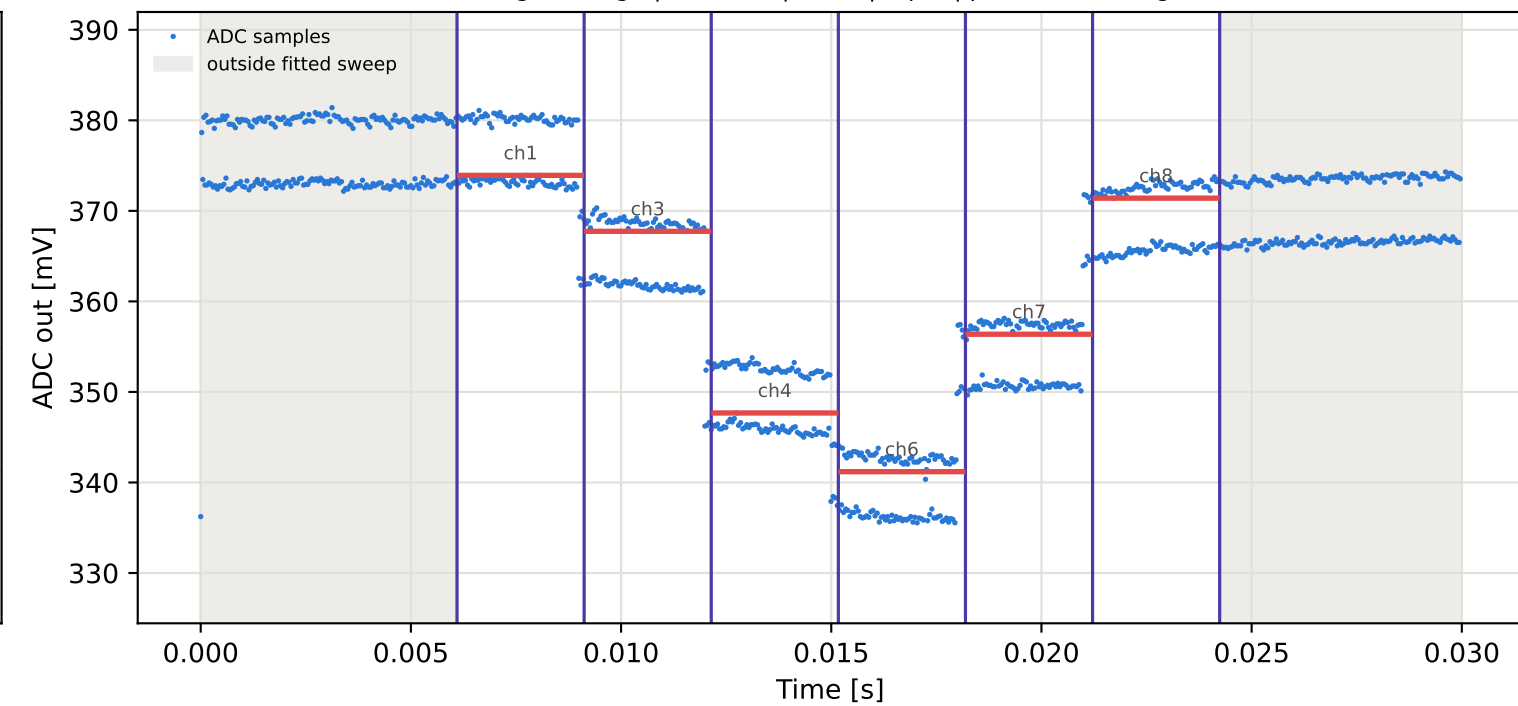
Tag2 &lt;- Tag6 | 905 MHz | run 0 | rep 1 | phase -176.32 deg
