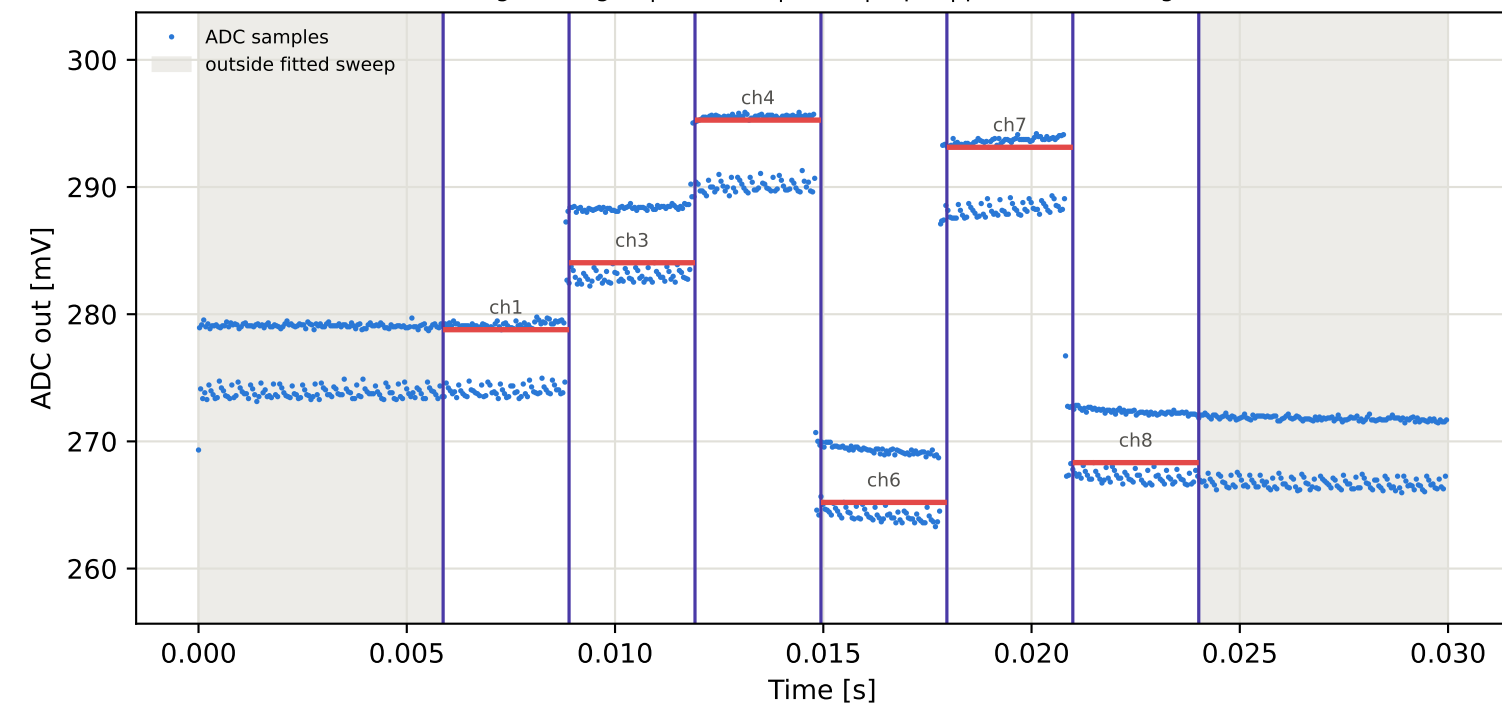
Tag1 &lt;- Tag3 | 995 MHz | run 0 | rep 1 | phase 101.28 deg
