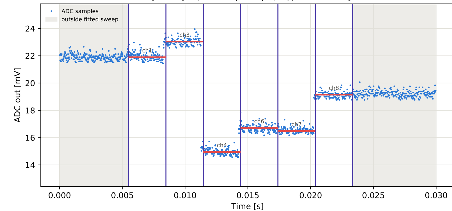
Tag9 &lt;- Tag16 | 795 MHz | run 0 | rep 1 | phase 68.06 deg
