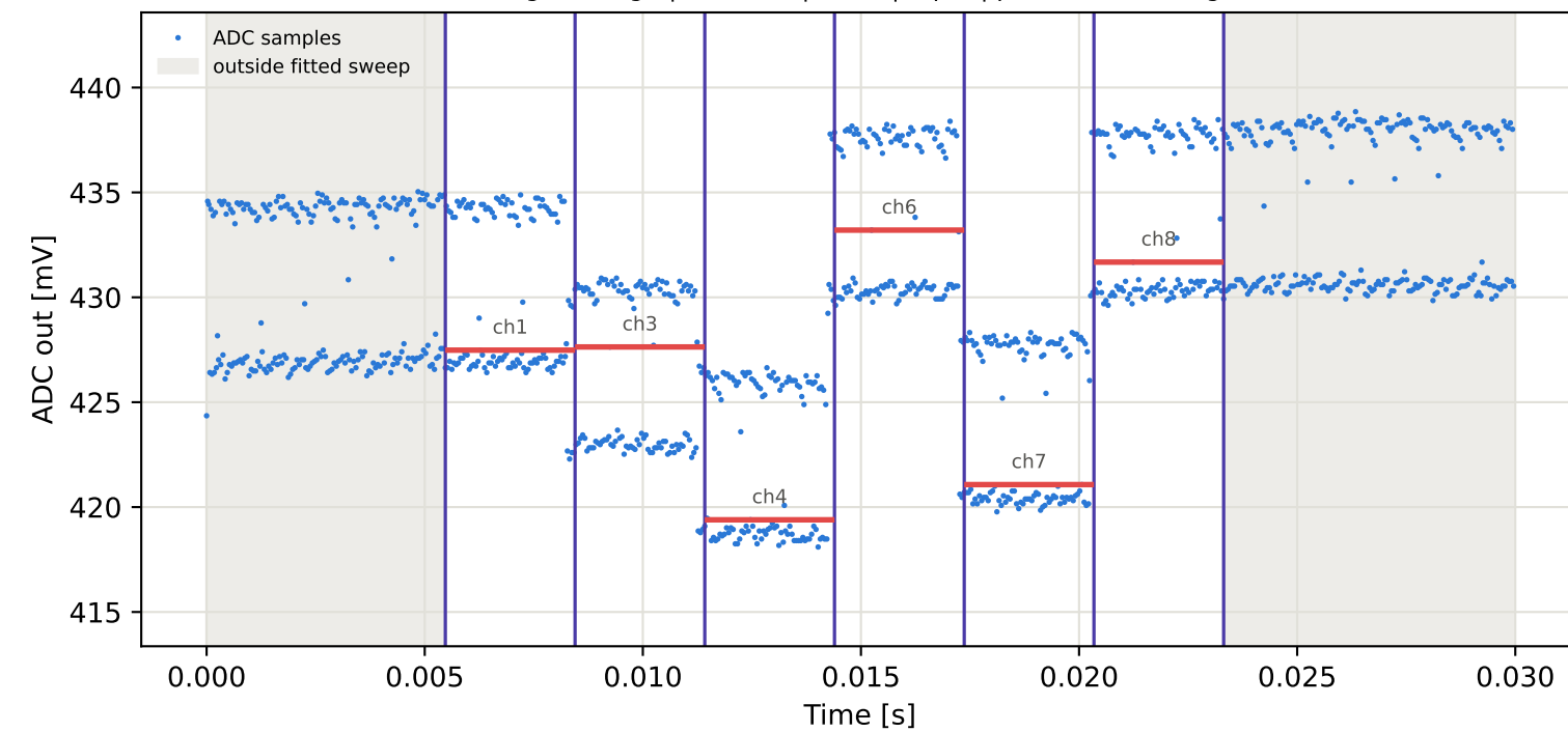
Tag4 &lt;- Tag15 | 985 MHz | run 0 | rep 1 | phase -149.69 deg
