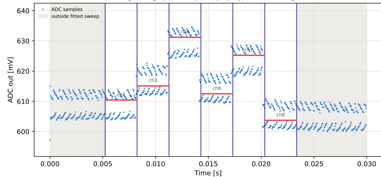
Tag7 &lt;- Tag5 | 945 MHz | run 0 | rep 1 | phase -88.15 deg
