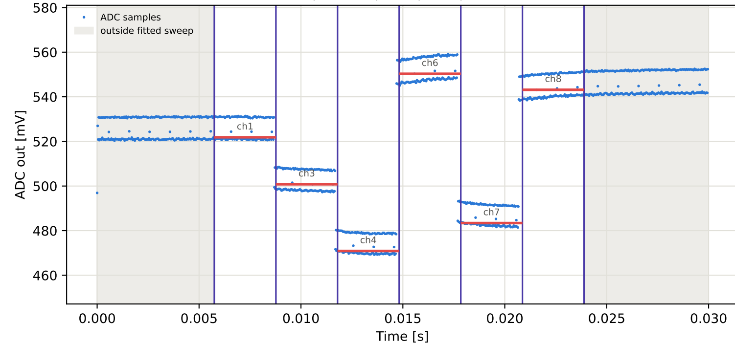
Tag1 &lt;- Tag3 | 965 MHz | run 0 | rep 1 | phase 124.93 deg
