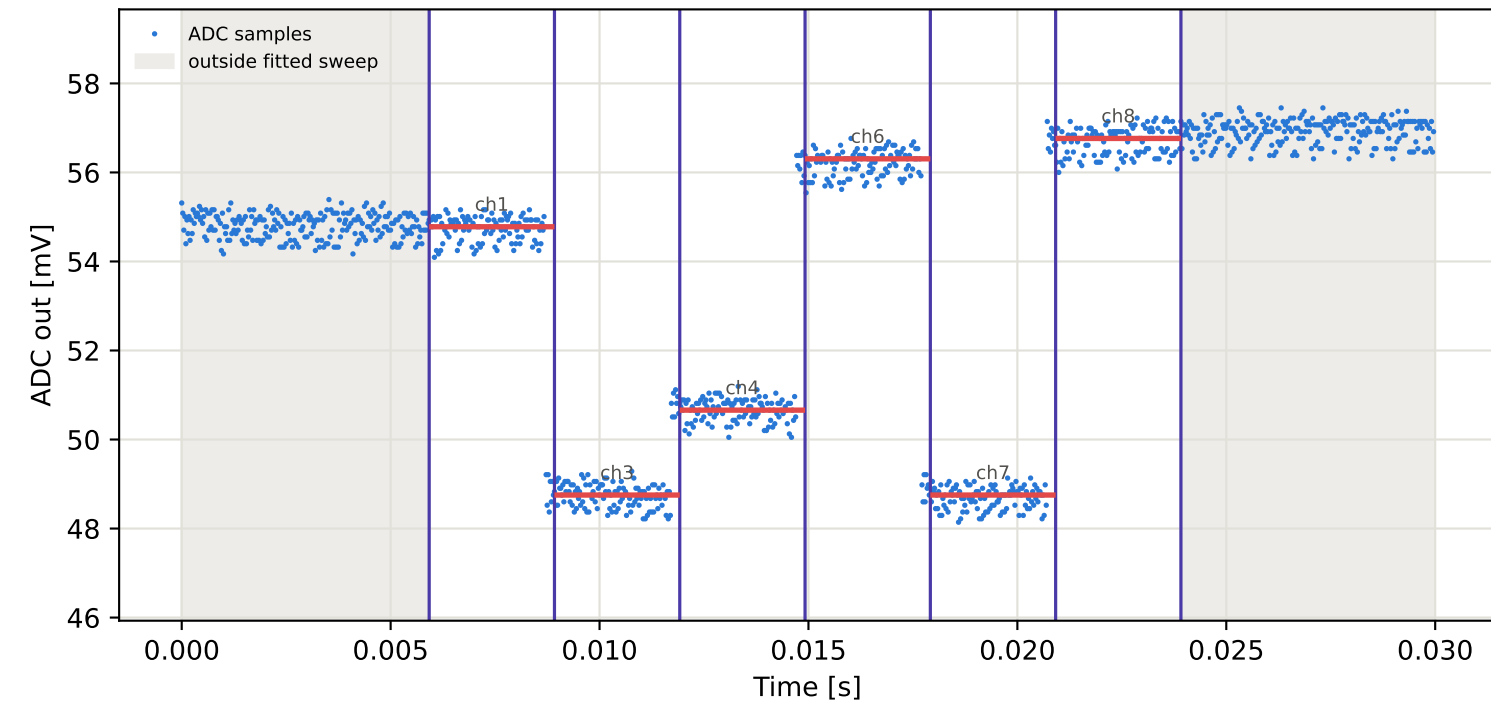
Tag15 &lt;- Tag10 | 805 MHz | run 0 | rep 1 | phase -58.52 deg
