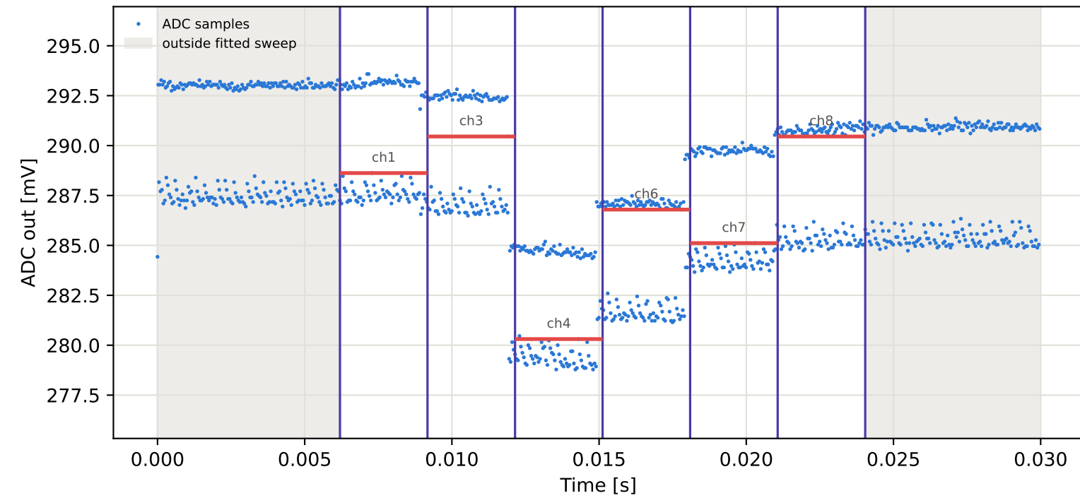
Tag10 &lt;- Tag1 | 995 MHz | run 0 | rep 1 | phase -168.57 deg
