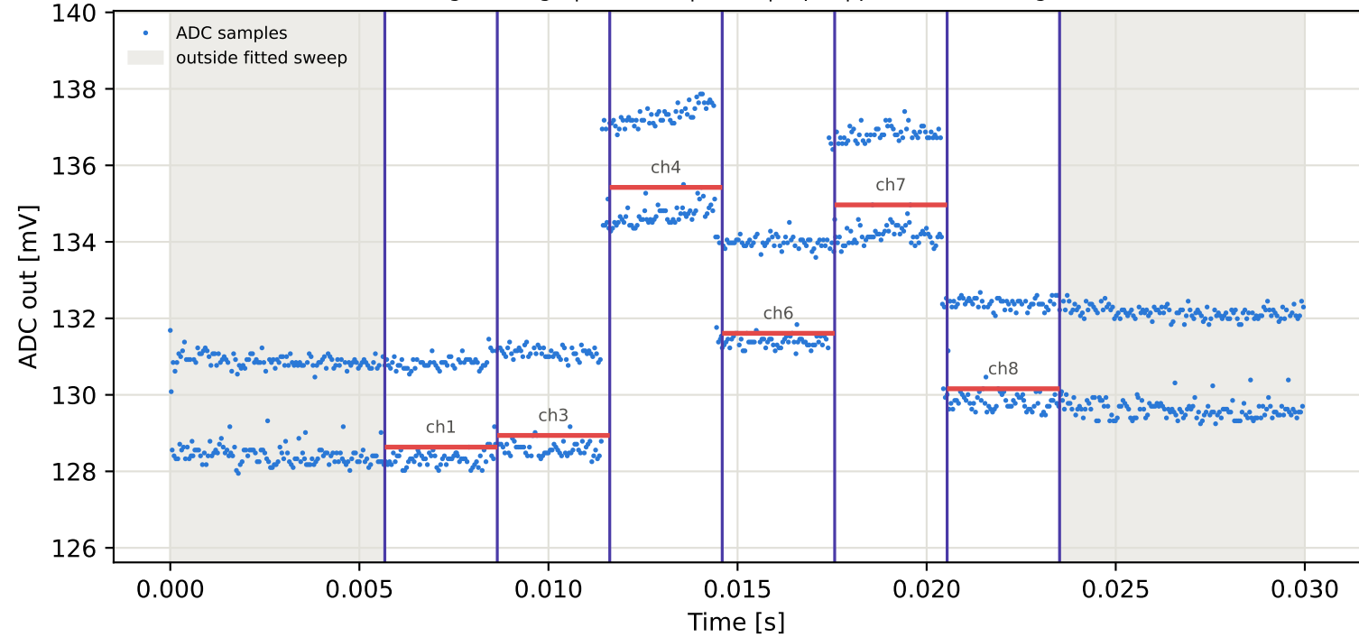
Tag7 &lt;- Tag1 | 775 MHz | run 0 | rep 1 | phase 157.67 deg
