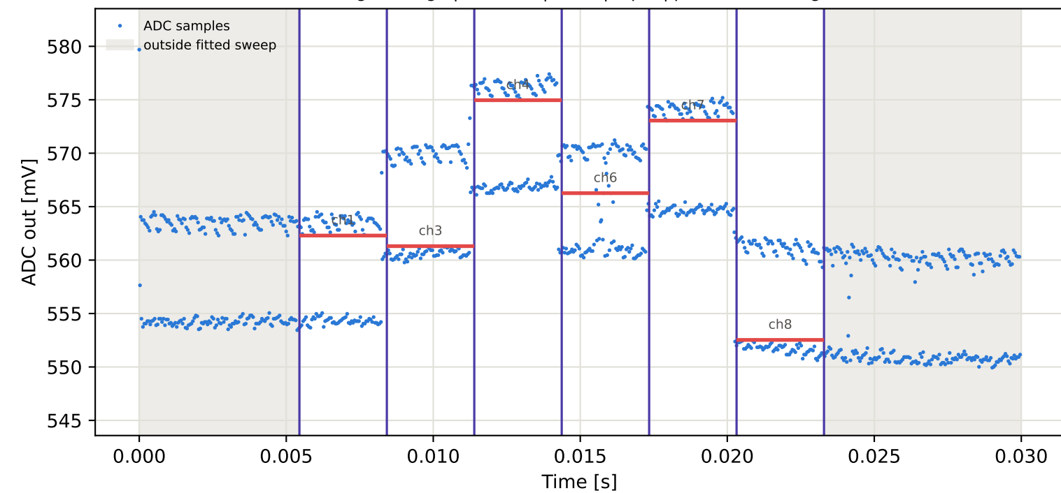
Tag6 &lt;- Tag4 | 895 MHz | run 0 | rep 1 | phase -138.33 deg
