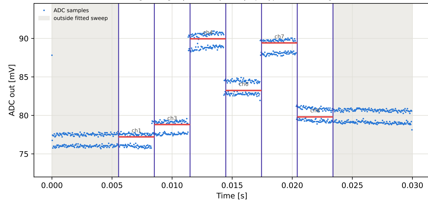
Tag1 &lt;- Tag16 | 795 MHz | run 0 | rep 1 | phase 64.48 deg
