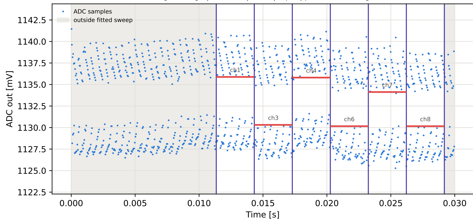
Tag8 &lt;- Tag15 | 875 MHz | run 0 | rep 1 | phase 123.03 deg
