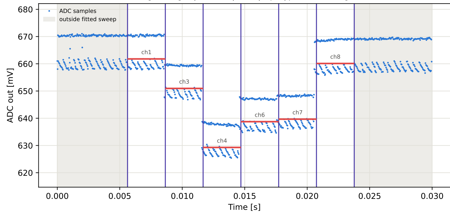
Tag6 &lt;- Tag2 | 955 MHz | run 0 | rep 1 | phase -169.58 deg
