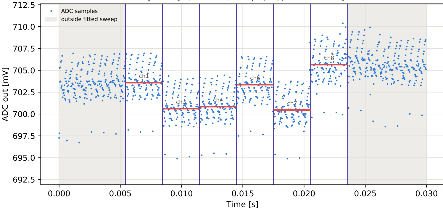
Tag6 &lt;- Tag1 | 875 MHz | run 0 | rep 1 | phase 131.79 deg
