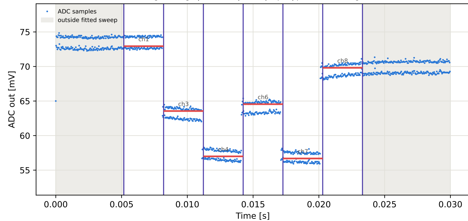
Tag1 &lt;- Tag8 | 835 MHz | run 0 | rep 1 | phase 89.94 deg
