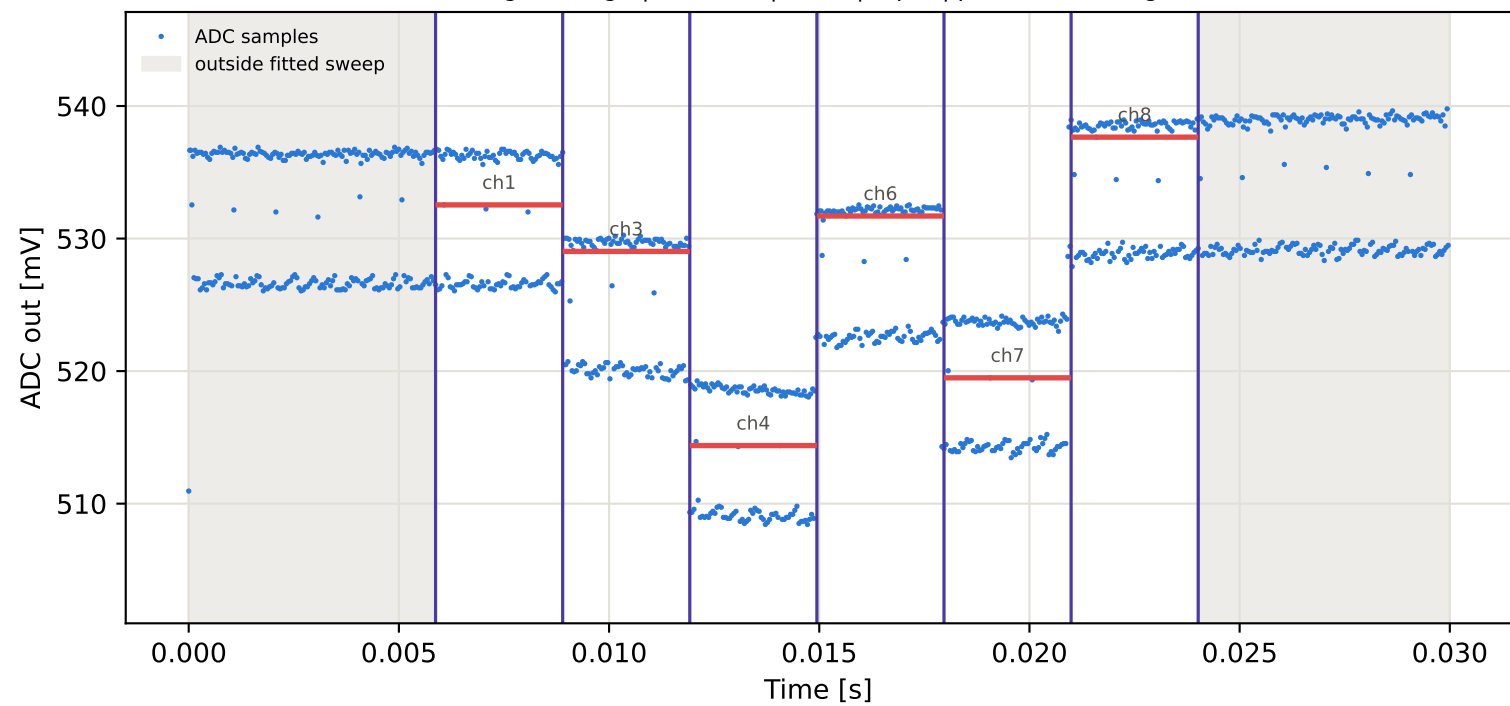
Tag5 &lt;- Tag9 | 945 MHz | run 0 | rep 1 | phase -3.48 deg
