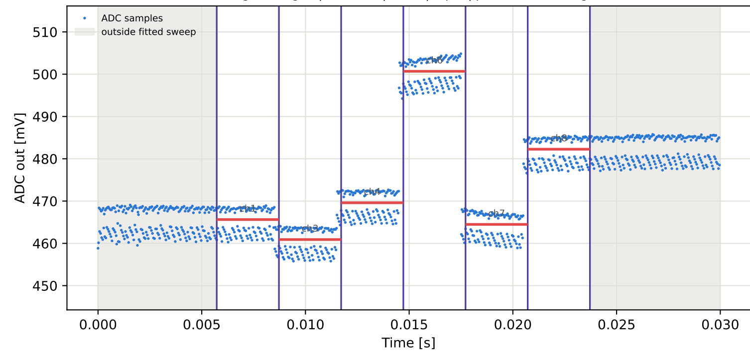
Tag1 &lt;- Tag2 | 955 MHz | run 0 | rep 1 | phase 124.24 deg
