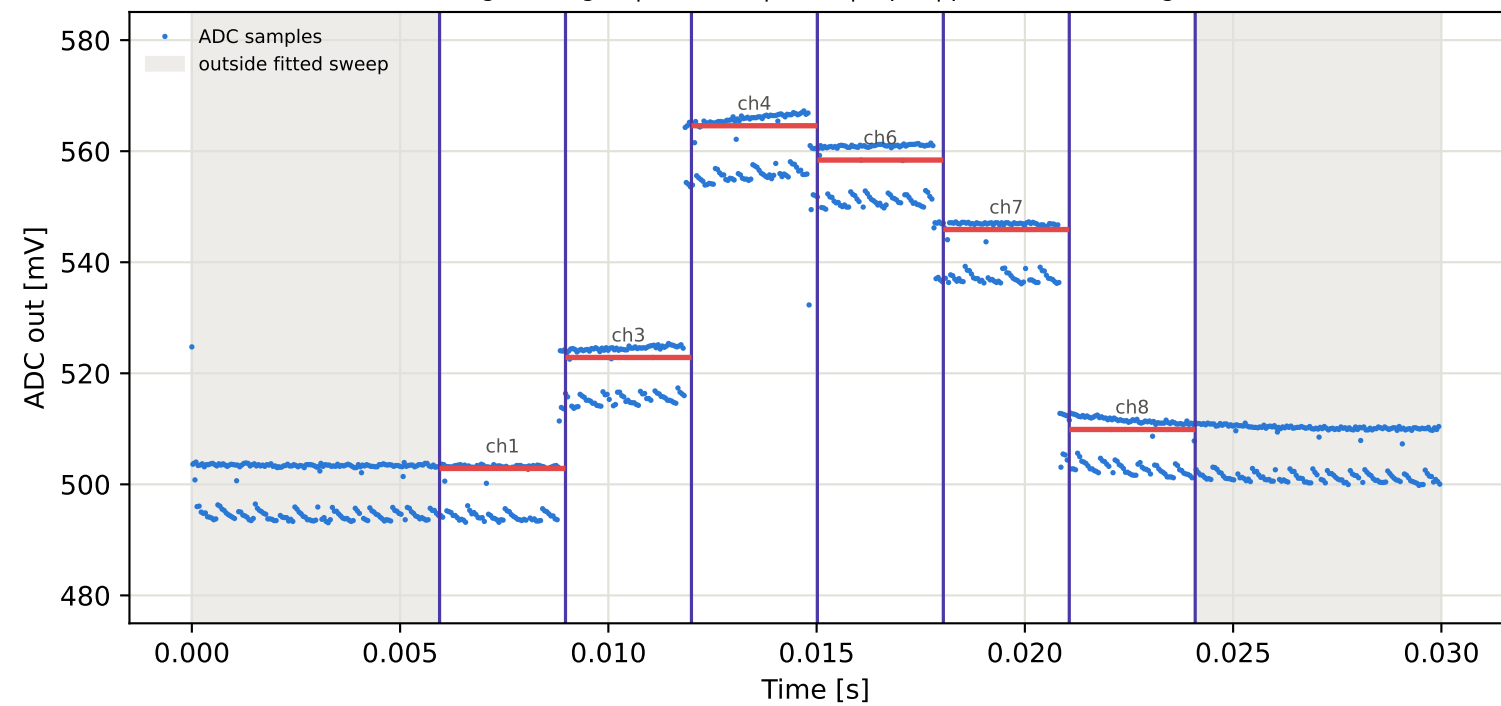
Tag5 &lt;- Tag2 | 945 MHz | run 0 | rep 1 | phase -56.07 deg
