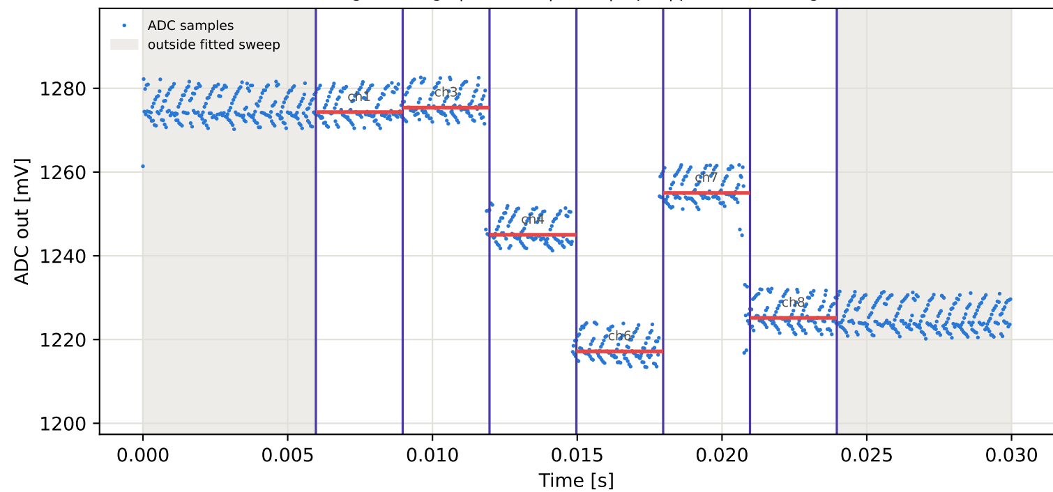
Tag2 &lt;- Tag10 | 875 MHz | run 0 | rep 1 | phase -56.43 deg
