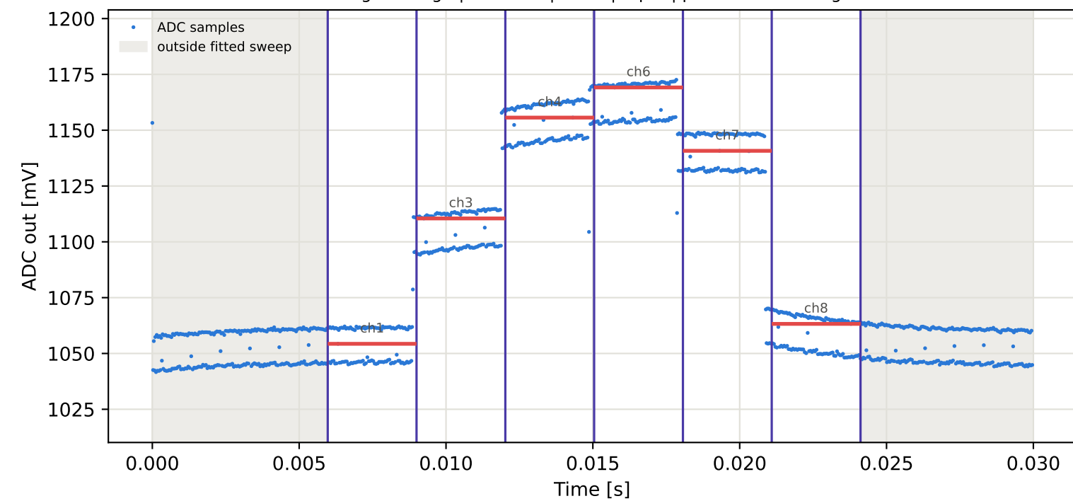
Tag4 &lt;- Tag7 | 895 MHz | run 0 | rep 1 | phase -85.69 deg
