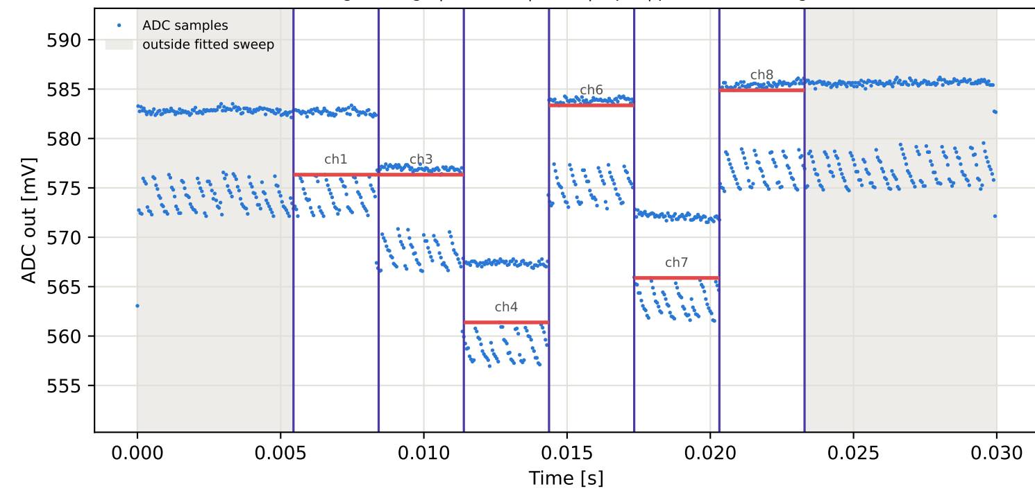
Tag7 &lt;- Tag1 | 975 MHz | run 0 | rep 1 | phase -175.92 deg
