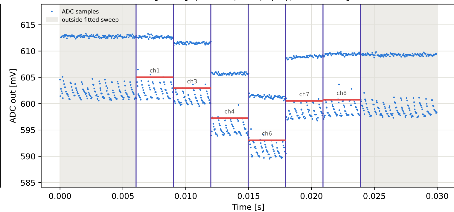
Tag5 &lt;- Tag9 | 935 MHz | run 0 | rep 1 | phase 27.15 deg
