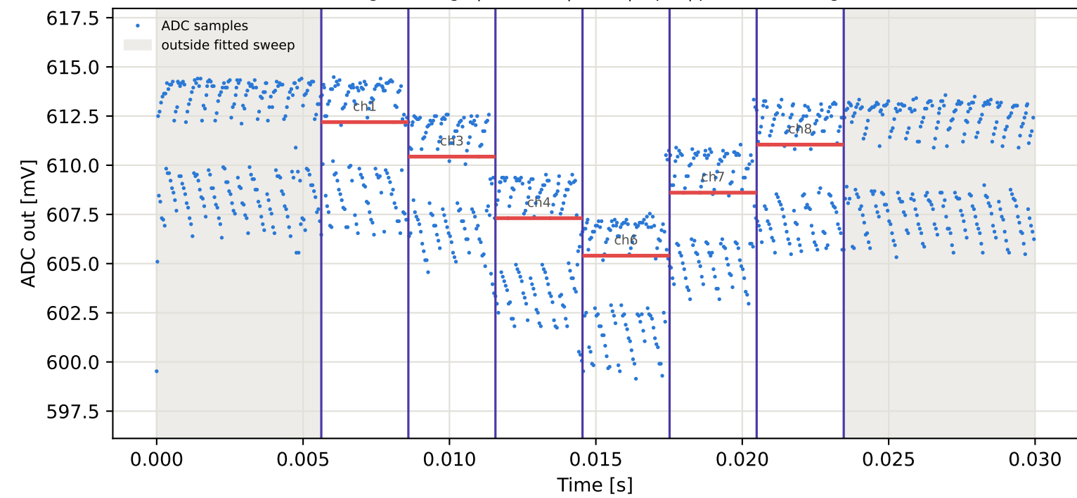
Tag15 &lt;- Tag4 | 855 MHz | run 0 | rep 1 | phase 145.69 deg
