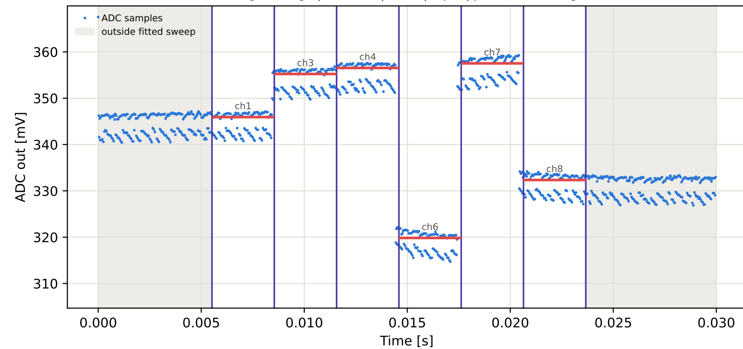
Tag5 &lt;- Tag8 | 955 MHz | run 0 | rep 1 | phase 123.75 deg
