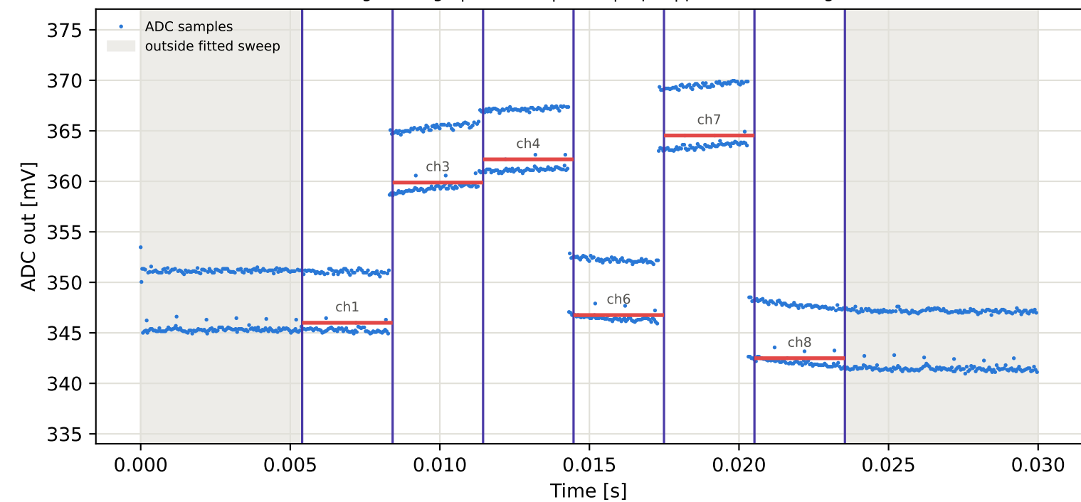
Tag3 &lt;- Tag9 | 845 MHz | run 0 | rep 1 | phase -48.41 deg
