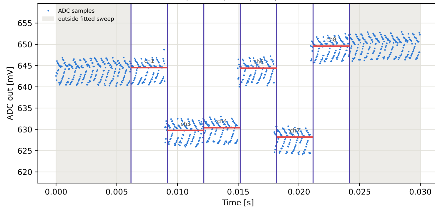
Tag15 &lt;- Tag9 | 865 MHz | run 0 | rep 1 | phase -69.72 deg
