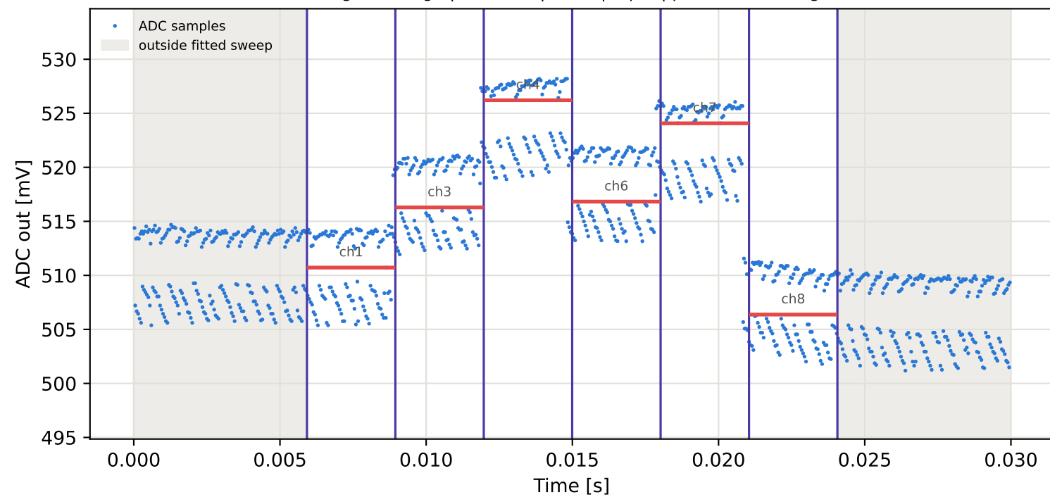
Tag15 &lt;- Tag10 | 915 MHz | run 0 | rep 1 | phase 154.84 deg
