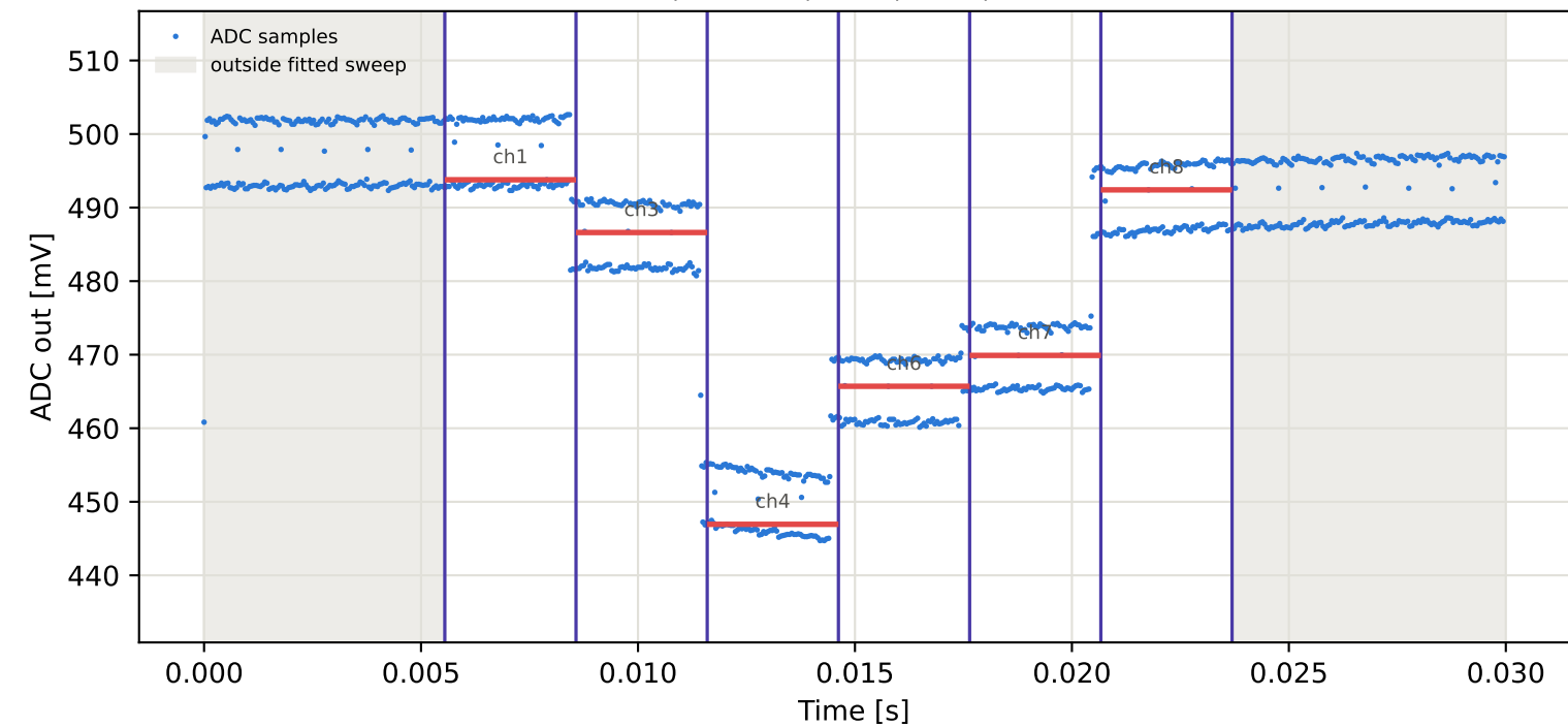
Tag9 &lt;- Tag8 | 955 MHz | run 0 | rep 1 | phase 60.30 deg
