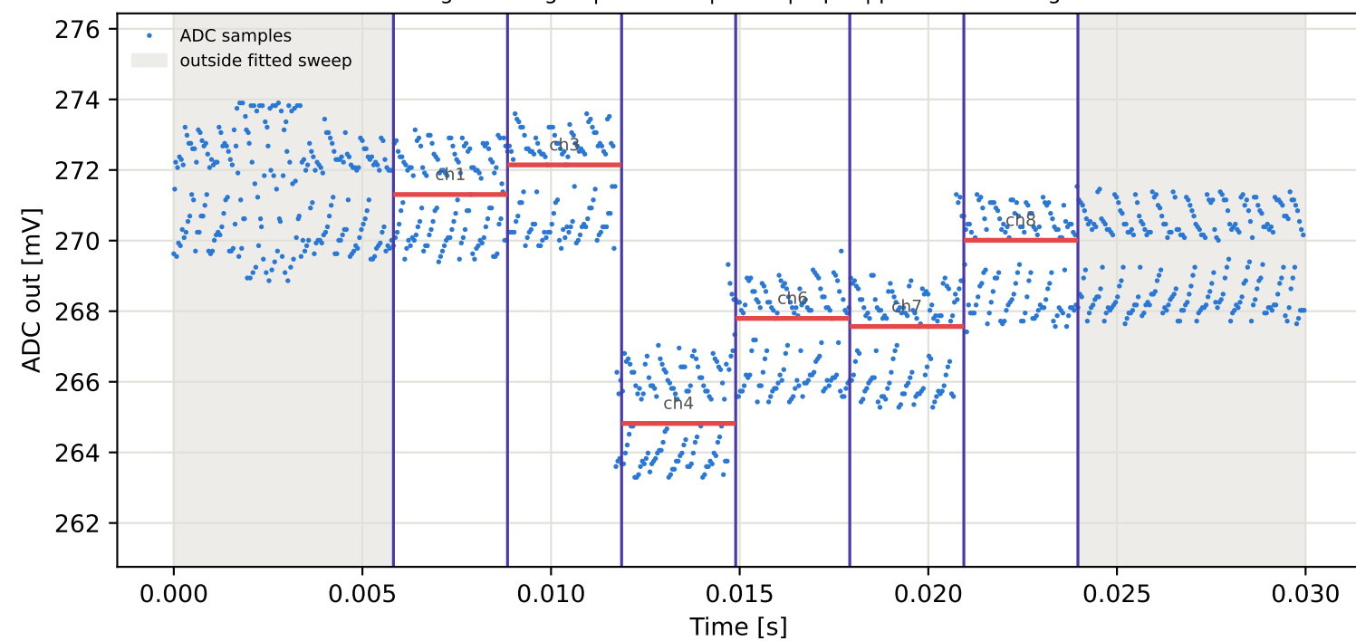
Tag16 &lt;- Tag15 | 805 MHz | run 0 | rep 1 | phase 73.51 deg
