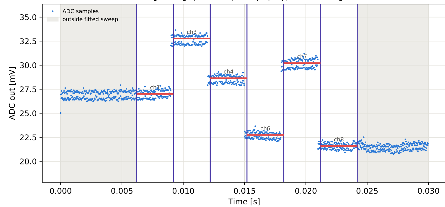
Tag1 &lt;- Tag7 | 855 MHz | run 0 | rep 1 | phase -171.83 deg
