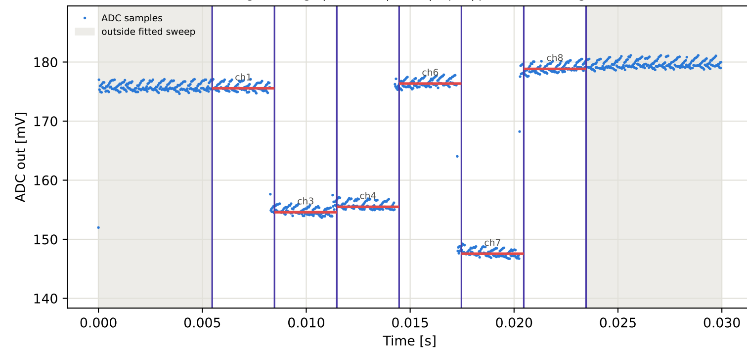
Tag2 &lt;- Tag1 | 795 MHz | run 0 | rep 1 | phase 30.03 deg
