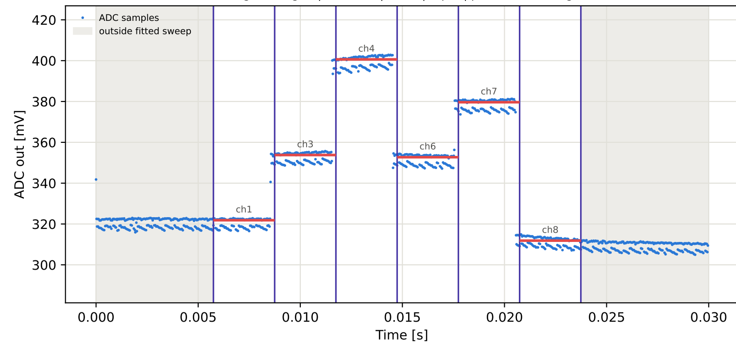
Tag5 &lt;- Tag2 | 955 MHz | run 0 | rep 1 | phase -18.24 deg
