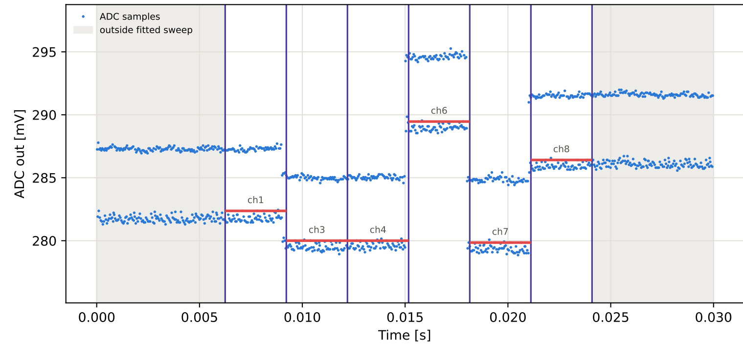
Tag3 &lt;- Tag9 | 935 MHz | run 0 | rep 1 | phase 103.47 deg
