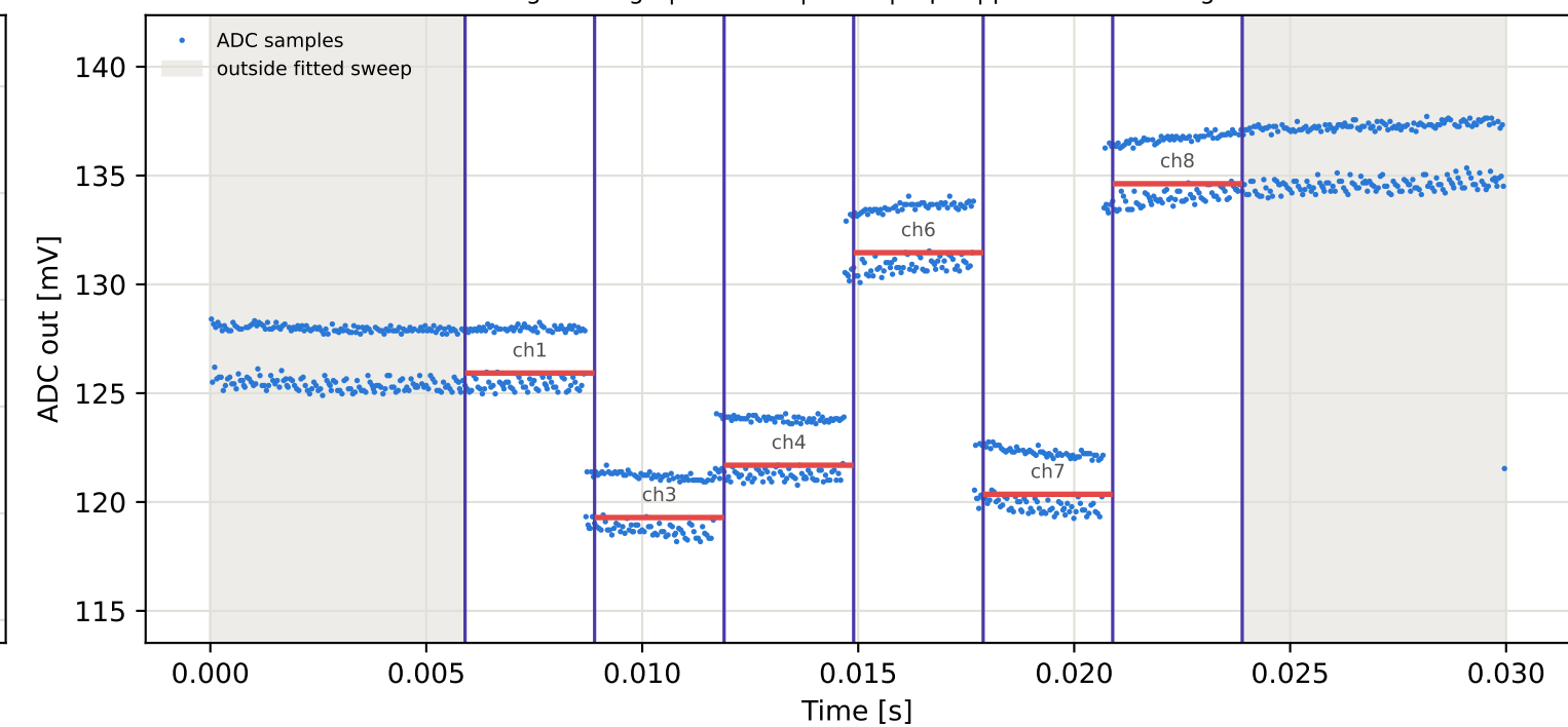
Tag1 &lt;- Tag4 | 865 MHz | run 0 | rep 1 | phase 161.12 deg
