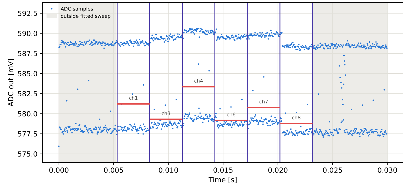
Tag6 &lt;- Tag4 | 945 MHz | run 0 | rep 1 | phase -72.15 deg
