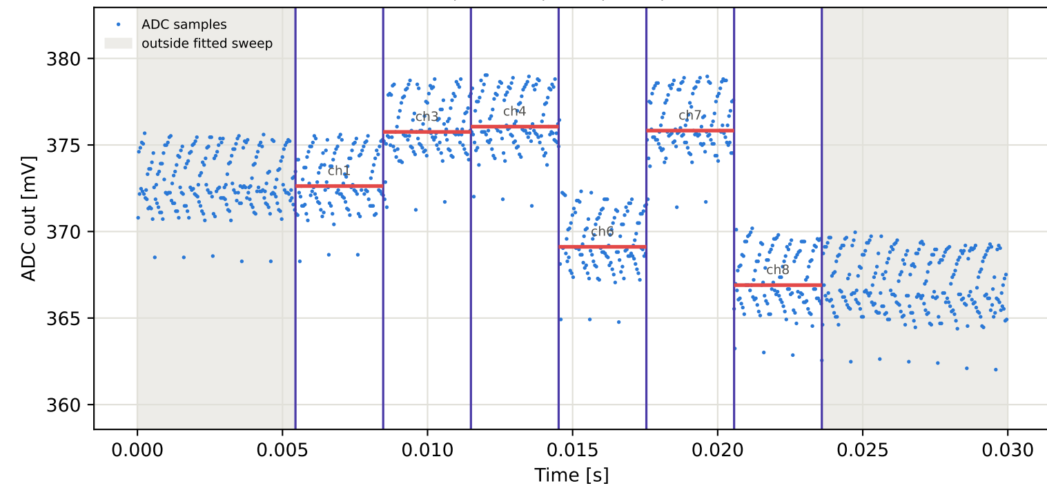
Tag7 &lt;- Tag10 | 895 MHz | run 0 | rep 1 | phase -30.16 deg
