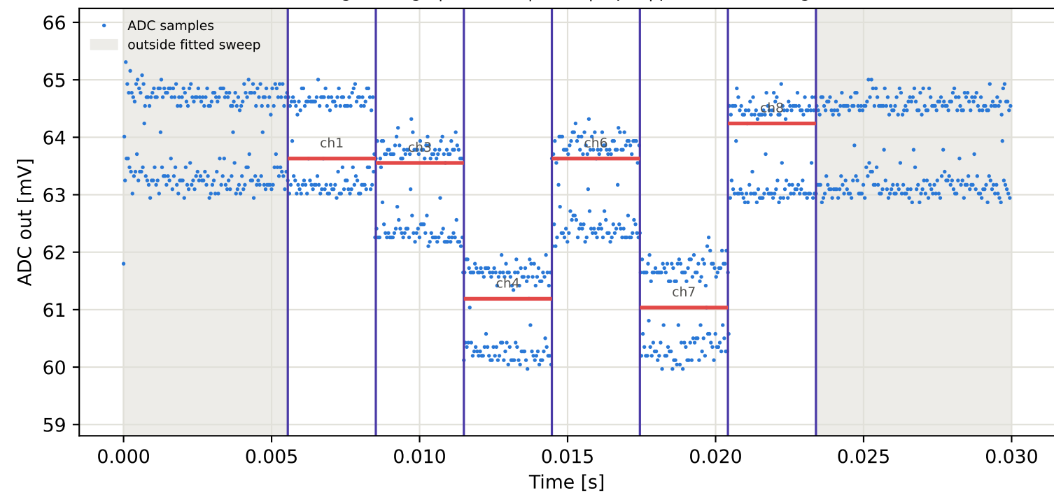
Tag9 &lt;- Tag15 | 805 MHz | run 0 | rep 1 | phase -172.65 deg
