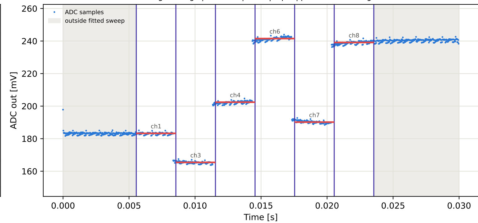
Tag9 &lt;- Tag6 | 855 MHz | run 0 | rep 1 | phase 11.57 deg
