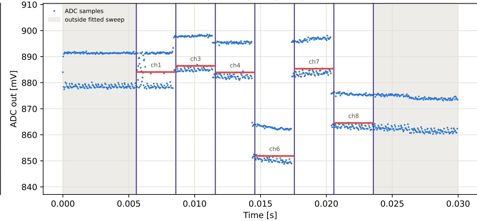
Tag3 &lt;- Tag2 | 875 MHz | run 0 | rep 1 | phase 3.39 deg
