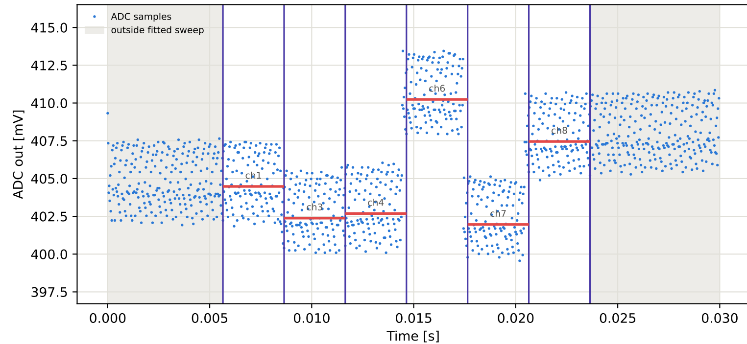
Tag3 &lt;- Tag2 | 985 MHz | run 0 | rep 1 | phase 0.83 deg
