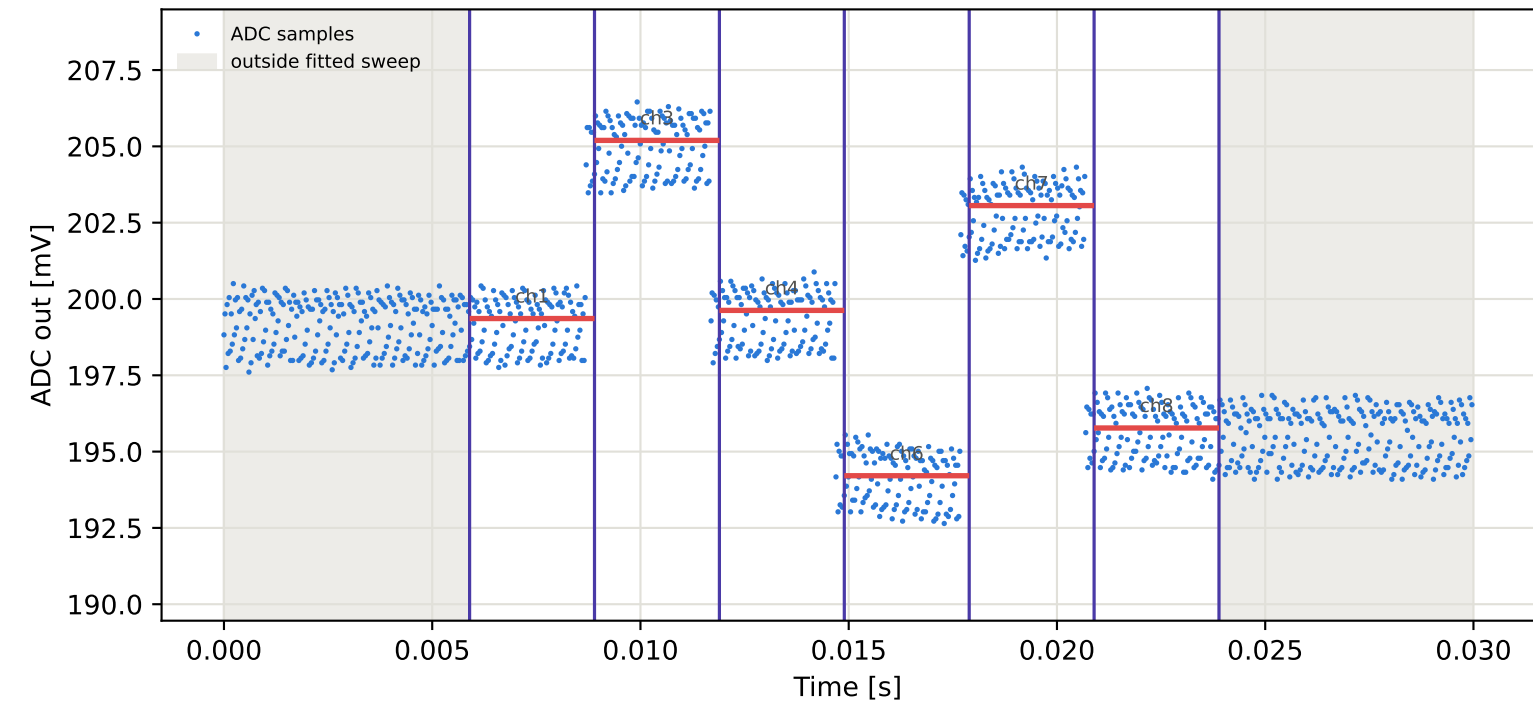
Tag3 &lt;- Tag8 | 805 MHz | run 0 | rep 1 | phase 147.34 deg
