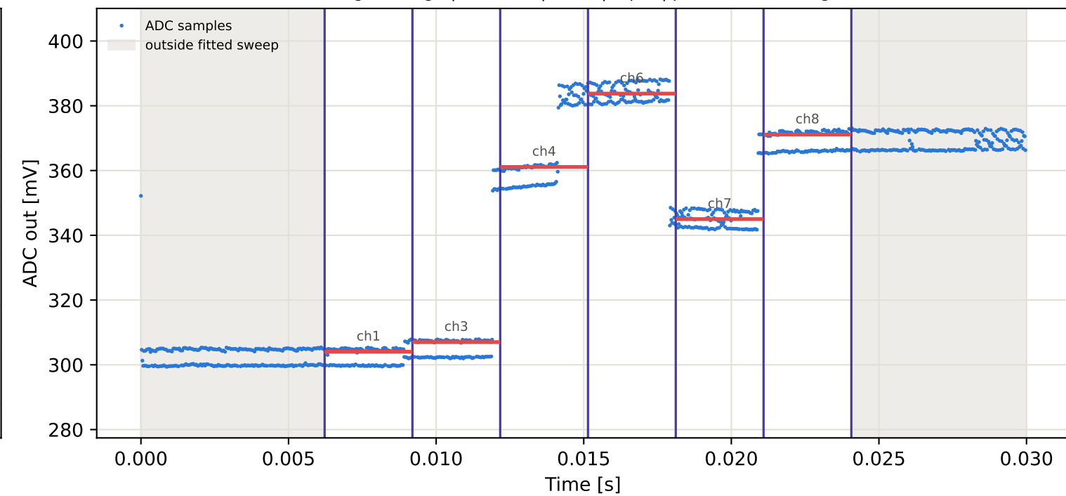
Tag9 &lt;- Tag6 | 845 MHz | run 0 | rep 1 | phase -1.12 deg
