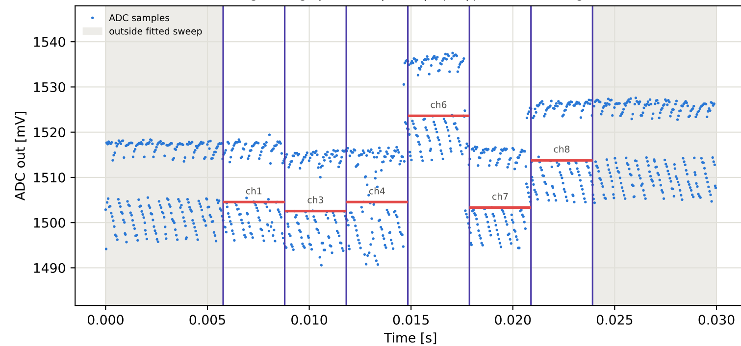
Tag8 &lt;- Tag4 | 925 MHz | run 0 | rep 1 | phase 76.45 deg
