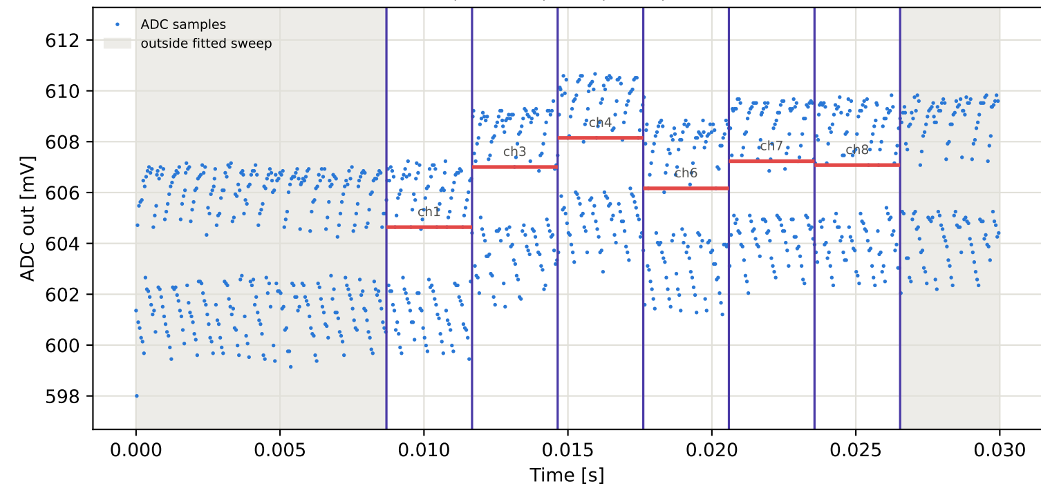
Tag15 &lt;- Tag10 | 855 MHz | run 0 | rep 1 | phase -87.46 deg
