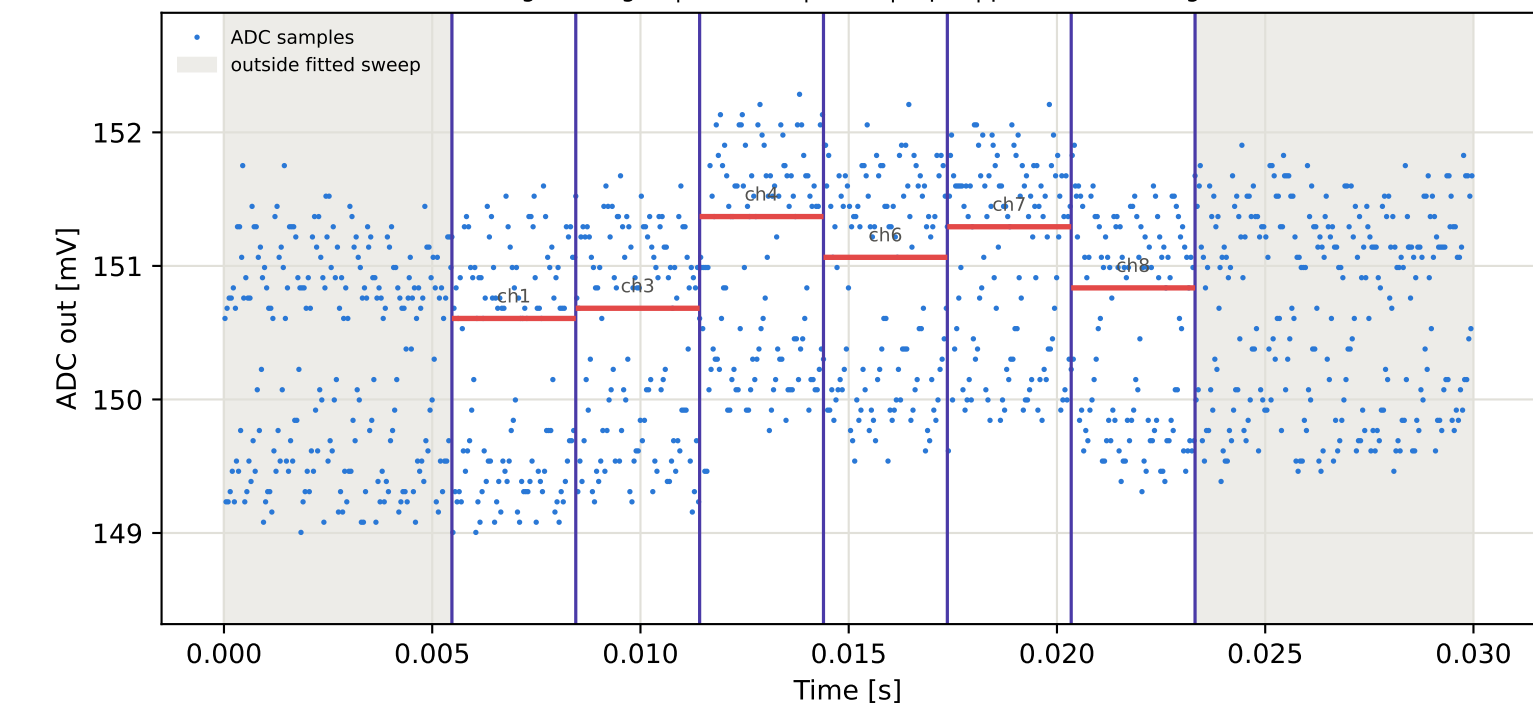
Tag7 &lt;- Tag10 | 805 MHz | run 0 | rep 1 | phase -99.36 deg
