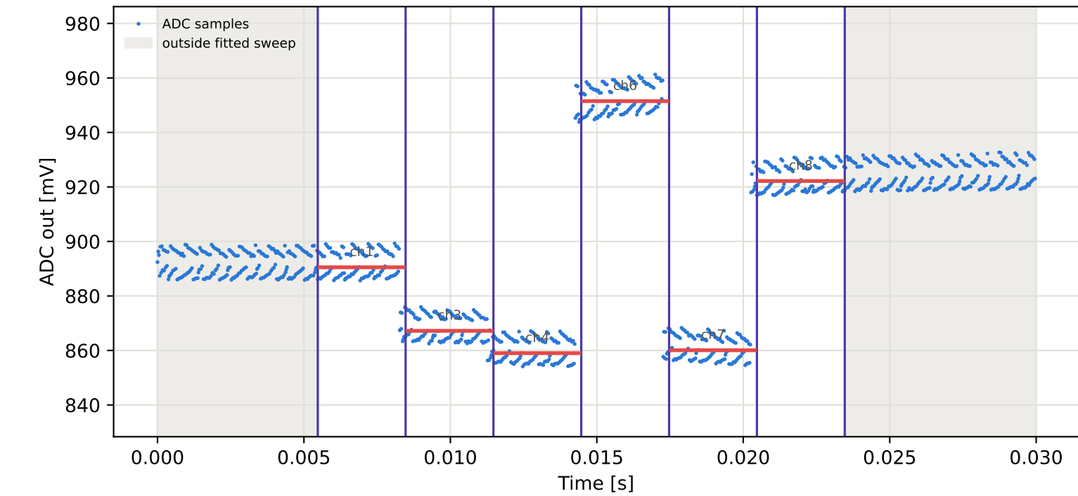
Tag8 &lt;- Tag6 | 955 MHz | run 0 | rep 1 | phase -167.49 deg
