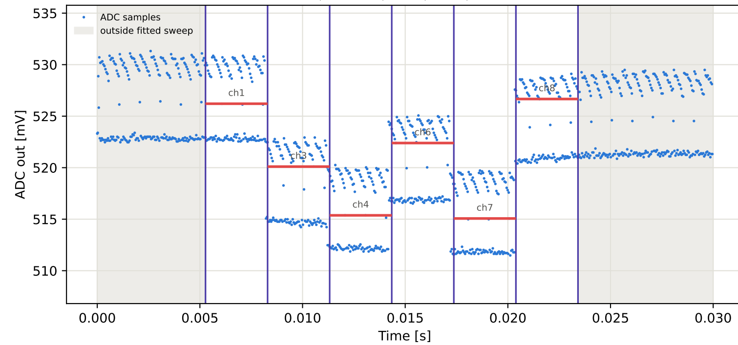
Tag7 &lt;- Tag10 | 845 MHz | run 0 | rep 1 | phase 106.68 deg
