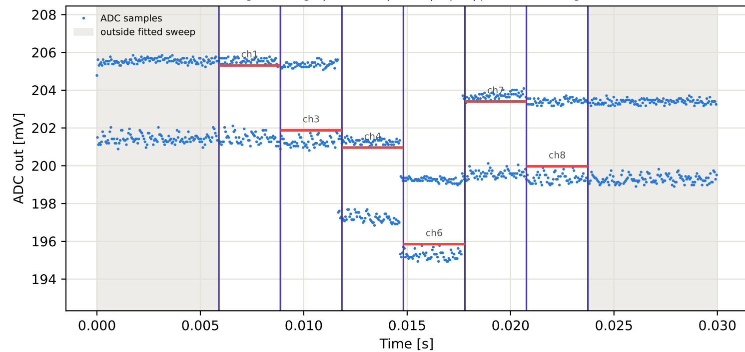
Tag10 &lt;- Tag9 | 955 MHz | run 0 | rep 1 | phase -115.42 deg
