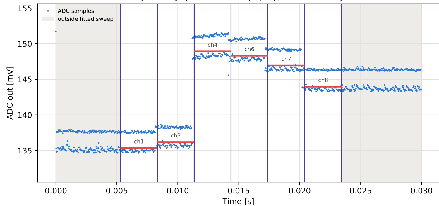
Tag10 &lt;- Tag4 | 825 MHz | run 0 | rep 1 | phase -120.28 deg
