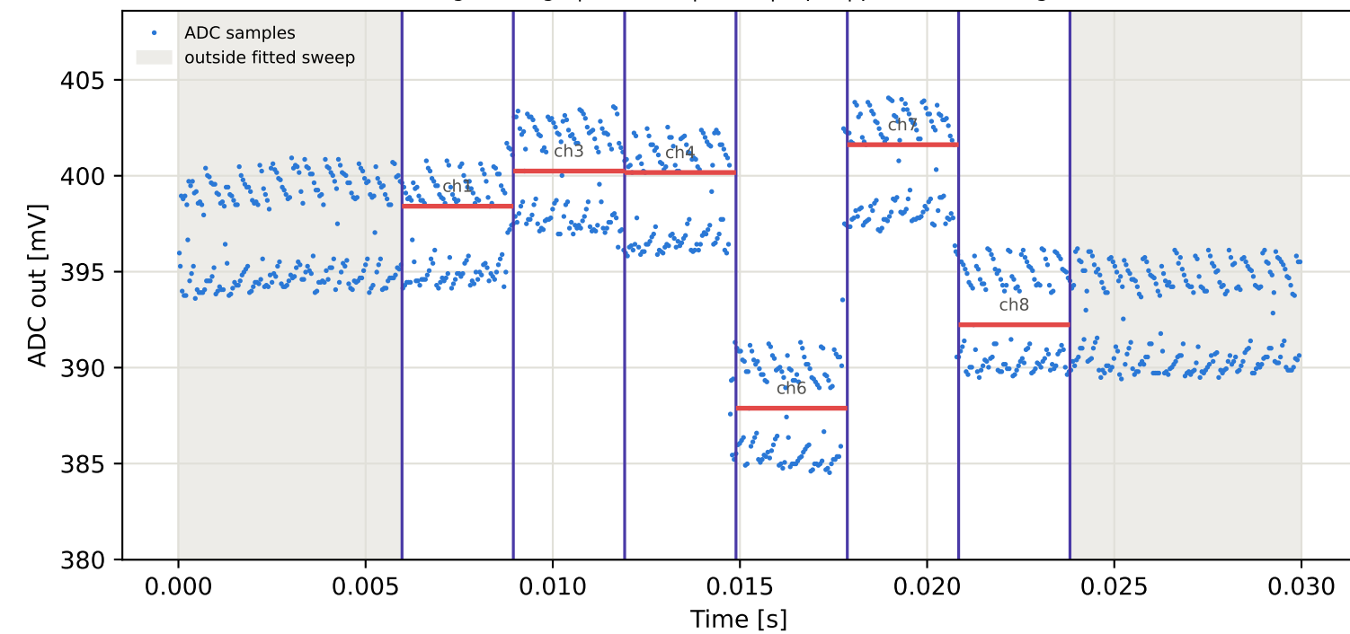
Tag4 &lt;- Tag7 | 975 MHz | run 0 | rep 1 | phase -24.13 deg
