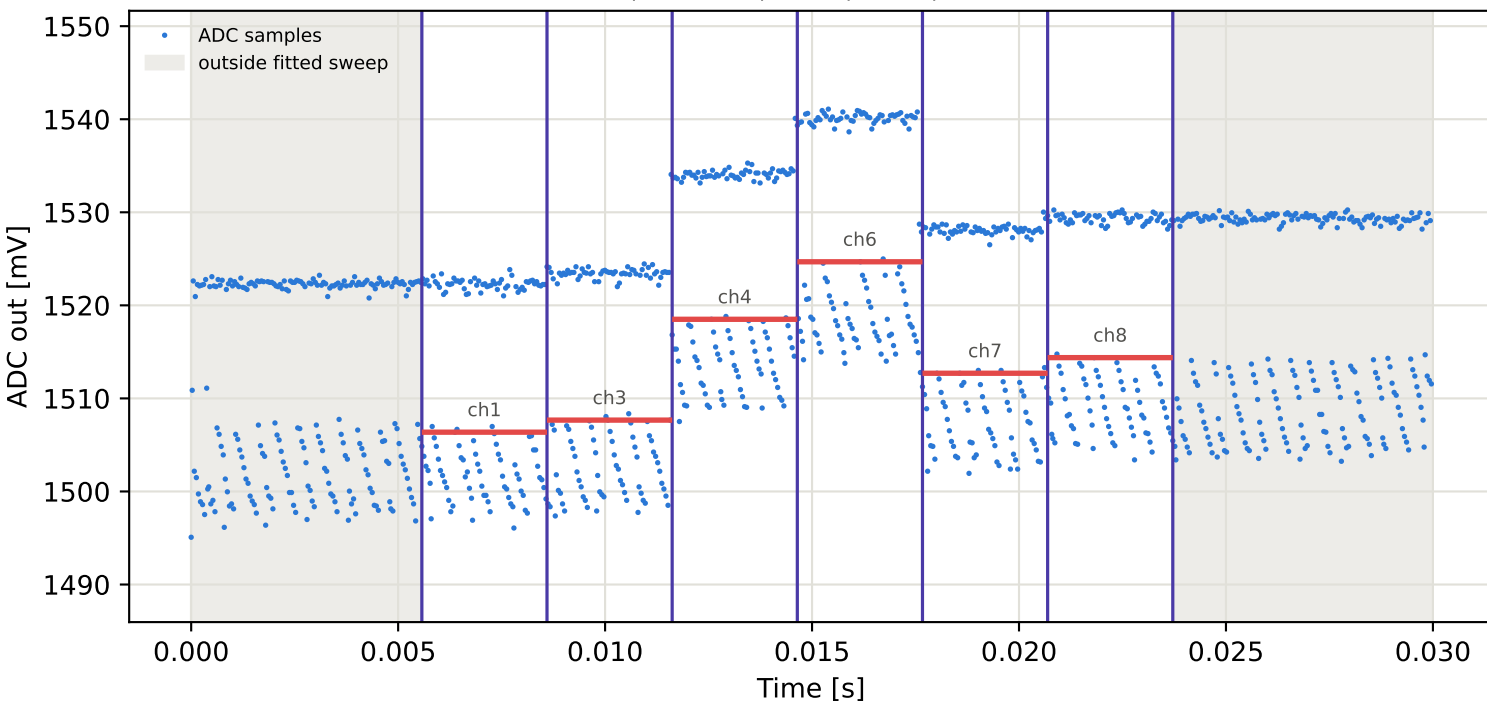
Tag15 &lt;- Tag1 | 965 MHz | run 0 | rep 1 | phase -147.86 deg
