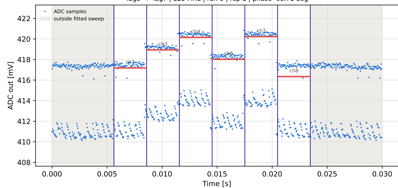
Tag5 &lt;- Tag9 | 825 MHz | run 0 | rep 1 | phase -85.58 deg
