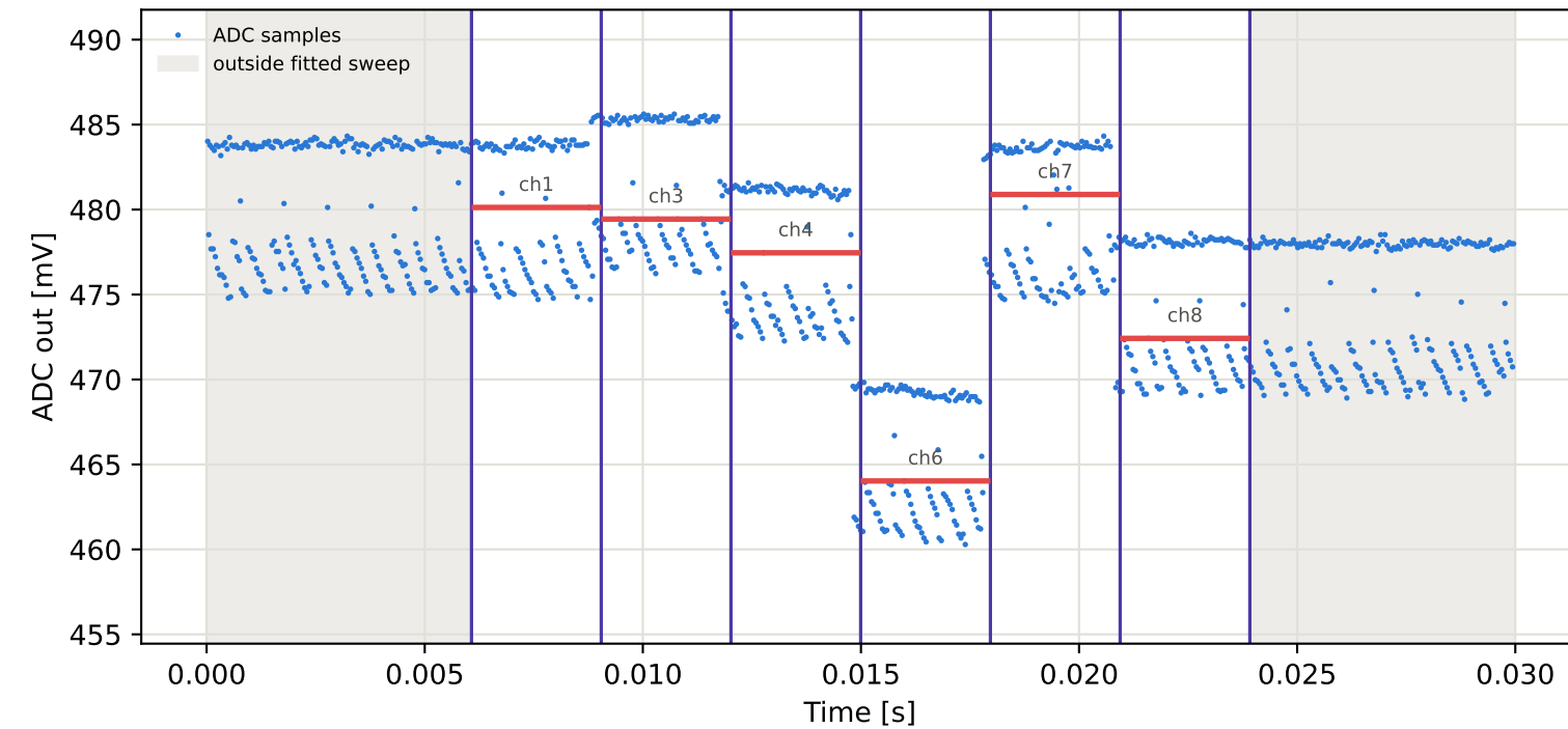
Tag9 &lt;- Tag7 | 955 MHz | run 0 | rep 1 | phase 0.30 deg
