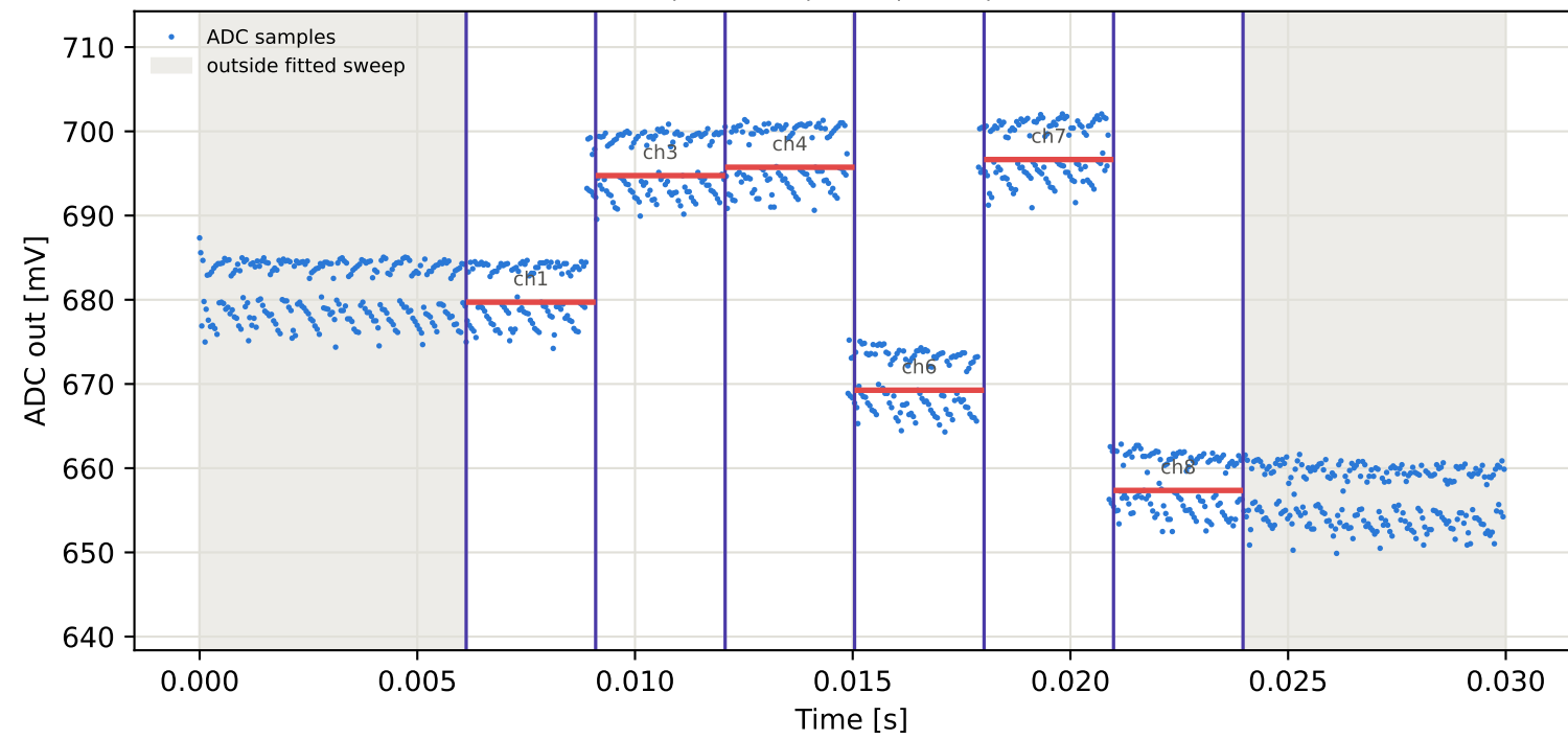
Tag10 &lt;- Tag4 | 885 MHz | run 0 | rep 1 | phase -35.37 deg
