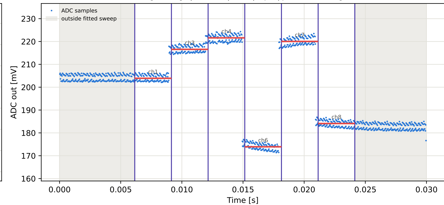
Tag1 &lt;- Tag8 | 925 MHz | run 0 | rep 1 | phase -11.24 deg
