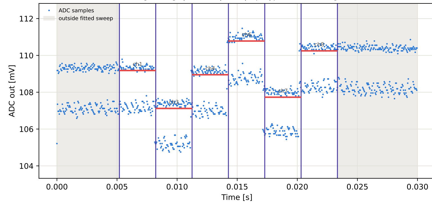
Tag6 &lt;- Tag9 | 785 MHz | run 0 | rep 1 | phase -99.07 deg
