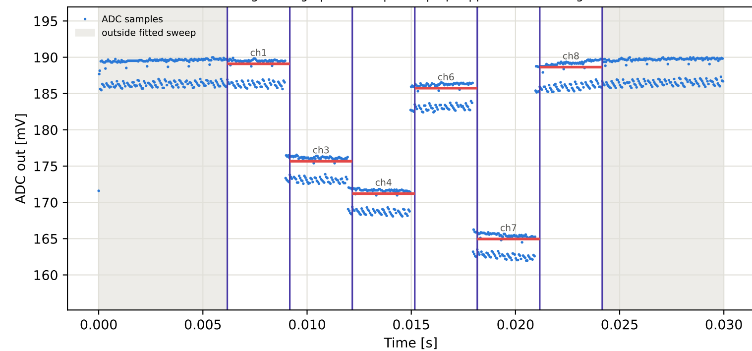
Tag3 &lt;- Tag6 | 795 MHz | run 0 | rep 1 | phase 39.27 deg
