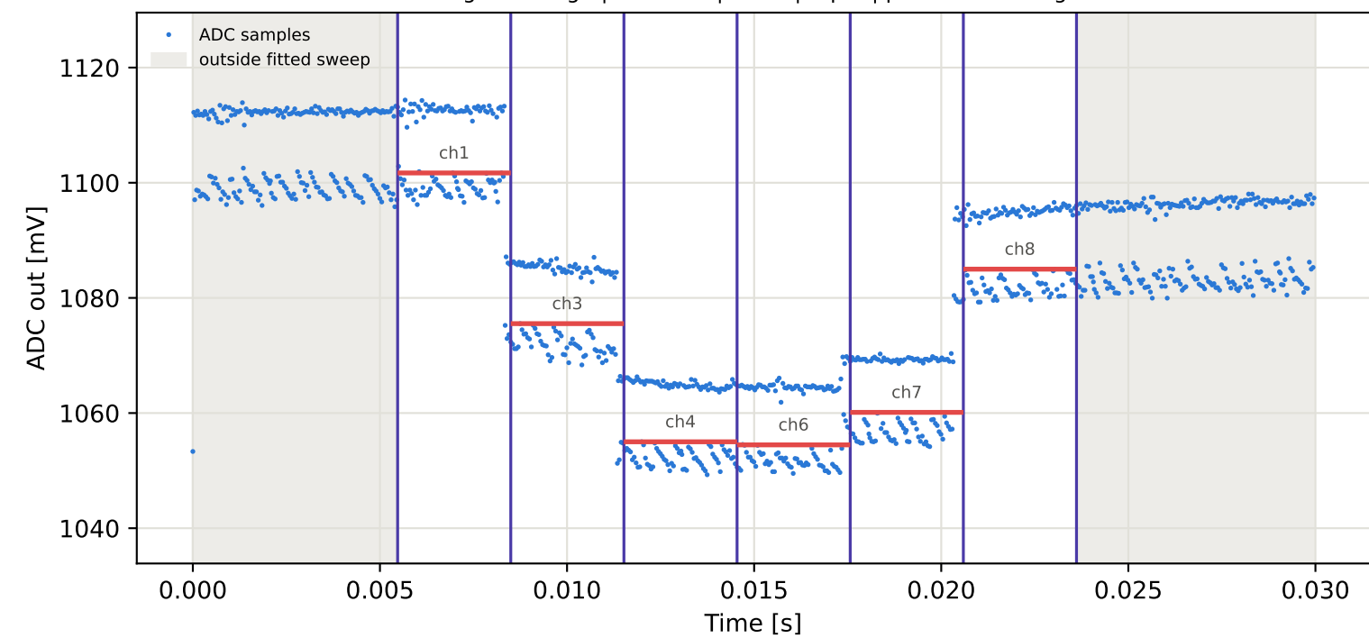
Tag2 &lt;- Tag10 | 885 MHz | run 0 | rep 1 | phase -88.80 deg
