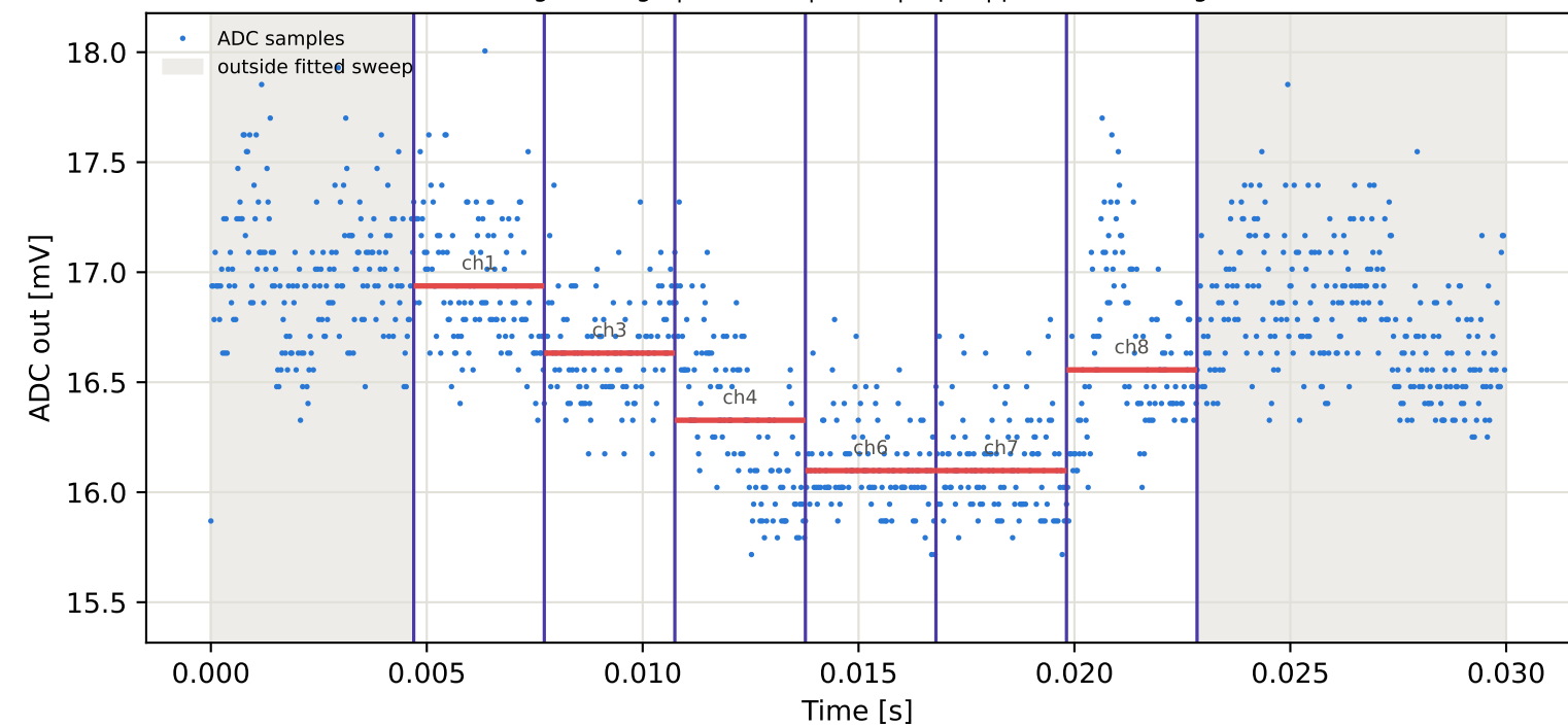
Tag9 &lt;- Tag2 | 795 MHz | run 0 | rep 1 | phase 66.57 deg
