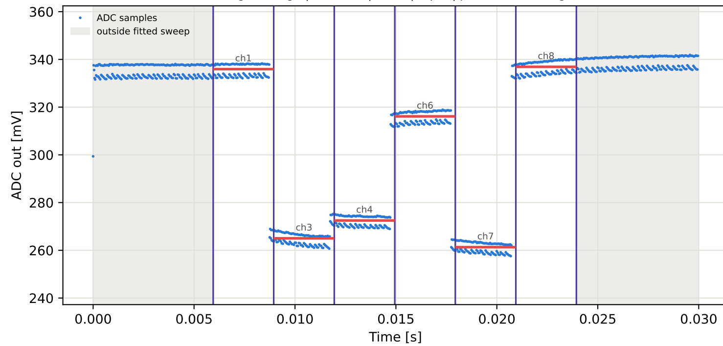
Tag3 &lt;- Tag6 | 835 MHz | run 0 | rep 1 | phase 74.13 deg
