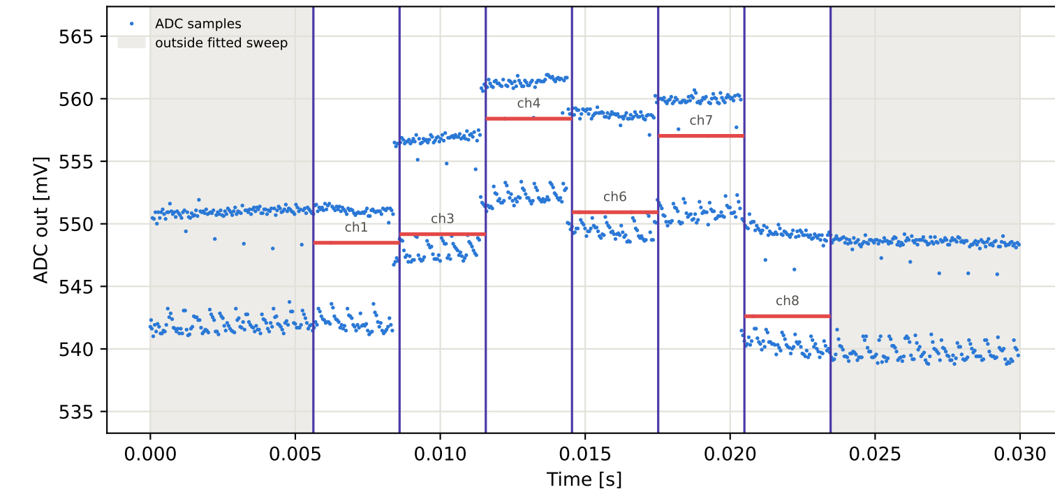
Tag2 &lt;- Tag15 | 895 MHz | run 0 | rep 1 | phase -130.67 deg
