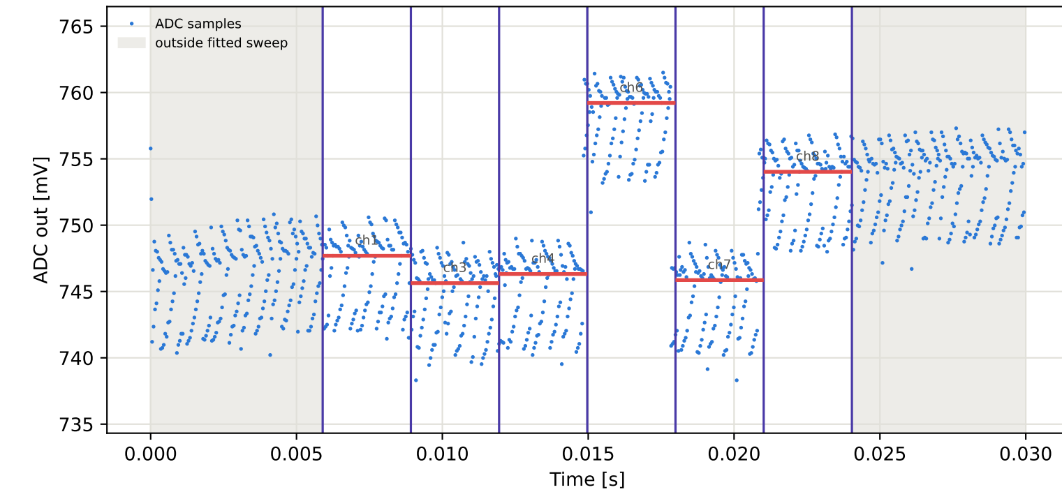
Tag9 &lt;- Tag16 | 935 MHz | run 0 | rep 1 | phase -94.79 deg
