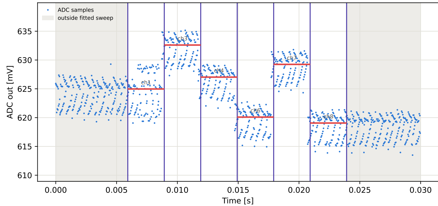
Tag4 &lt;- Tag2 | 855 MHz | run 0 | rep 1 | phase -136.25 deg
