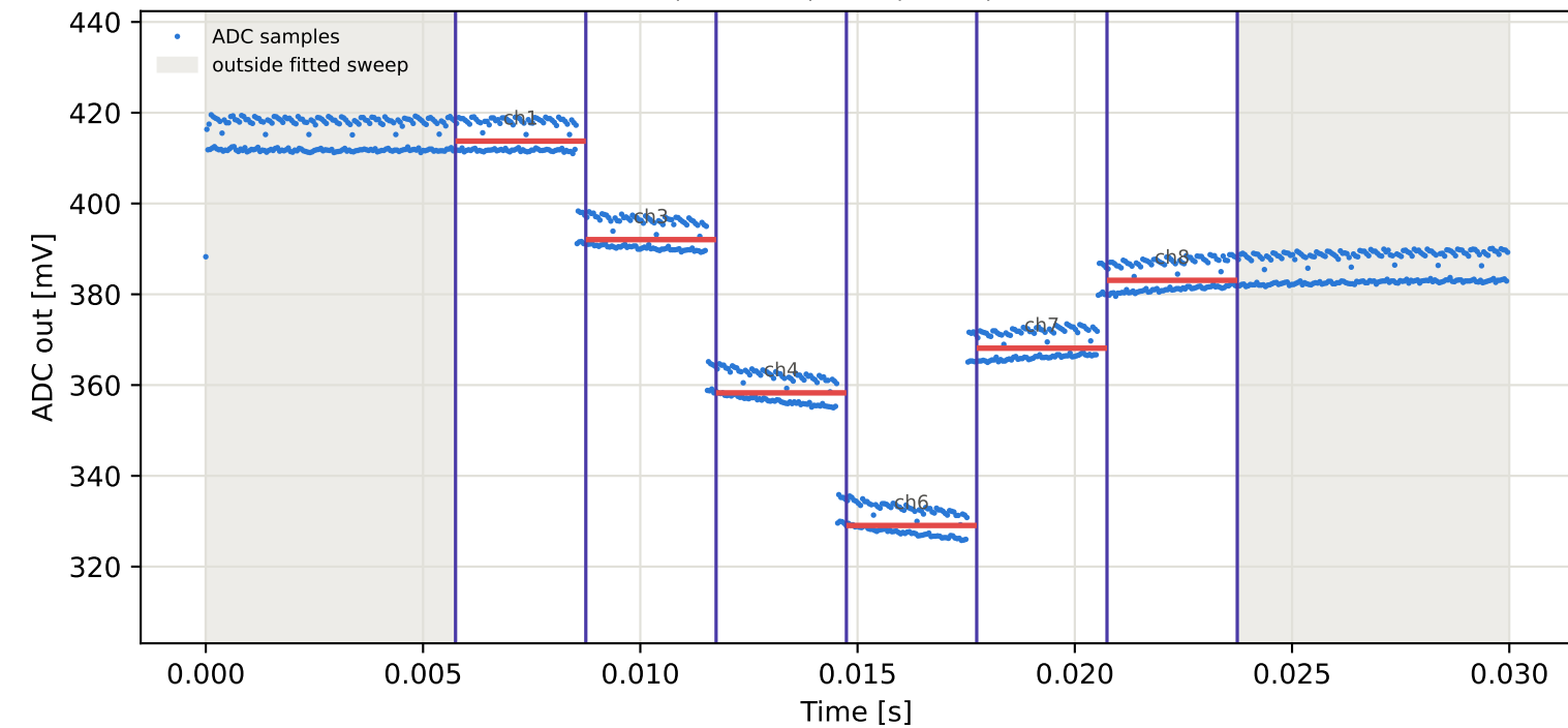
Tag1 &lt;- Tag3 | 895 MHz | run 0 | rep 1 | phase 43.63 deg
