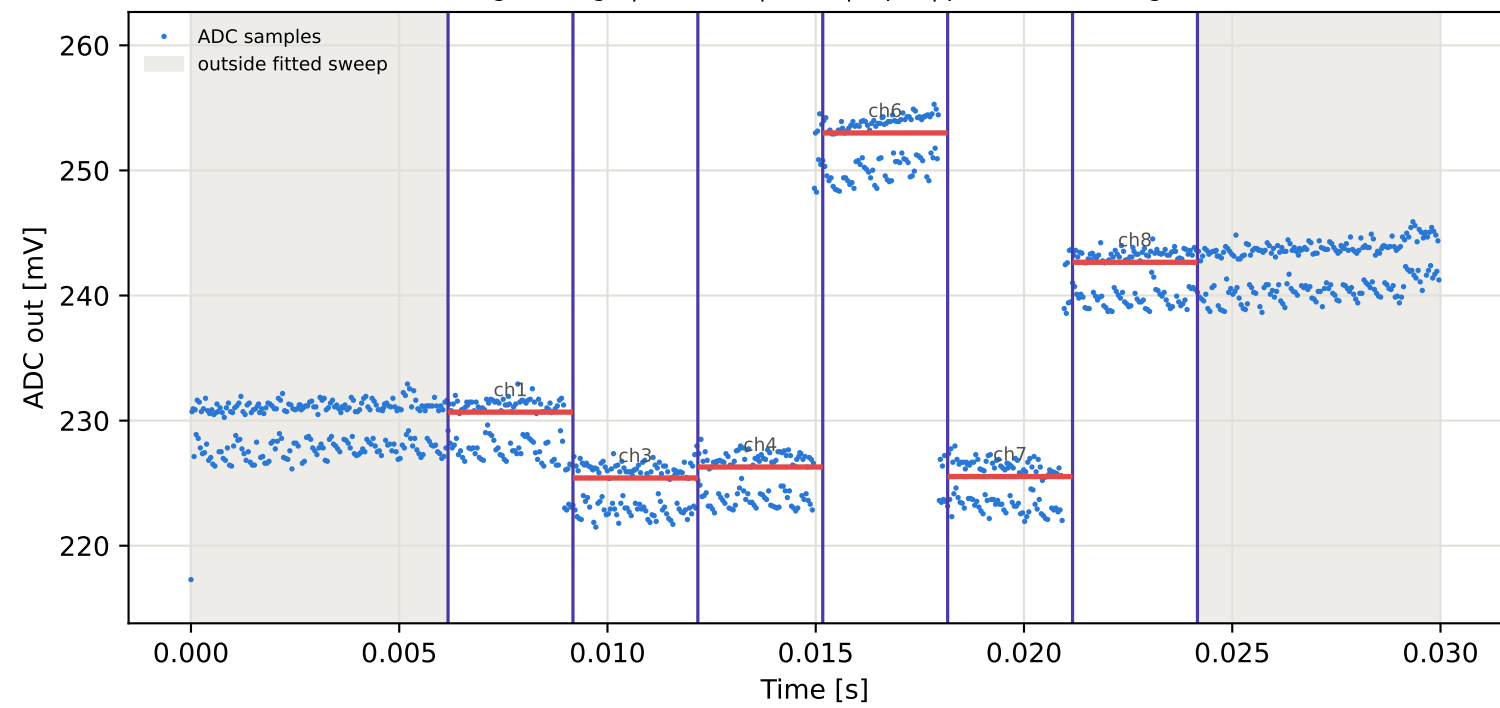
Tag2 &lt;- Tag5 | 925 MHz | run 0 | rep 1 | phase -5.07 deg
