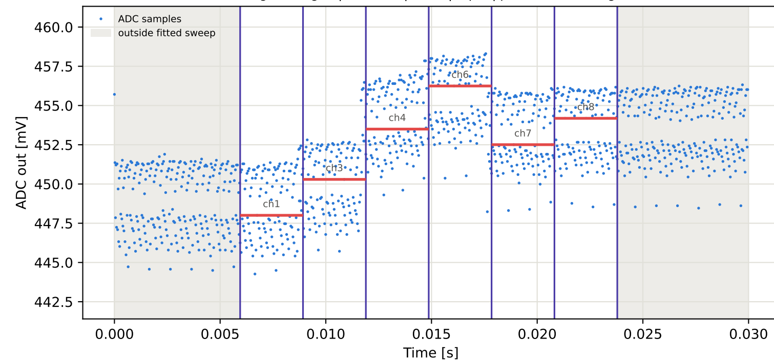
Tag3 &lt;- Tag16 | 855 MHz | run 0 | rep 1 | phase -60.32 deg
