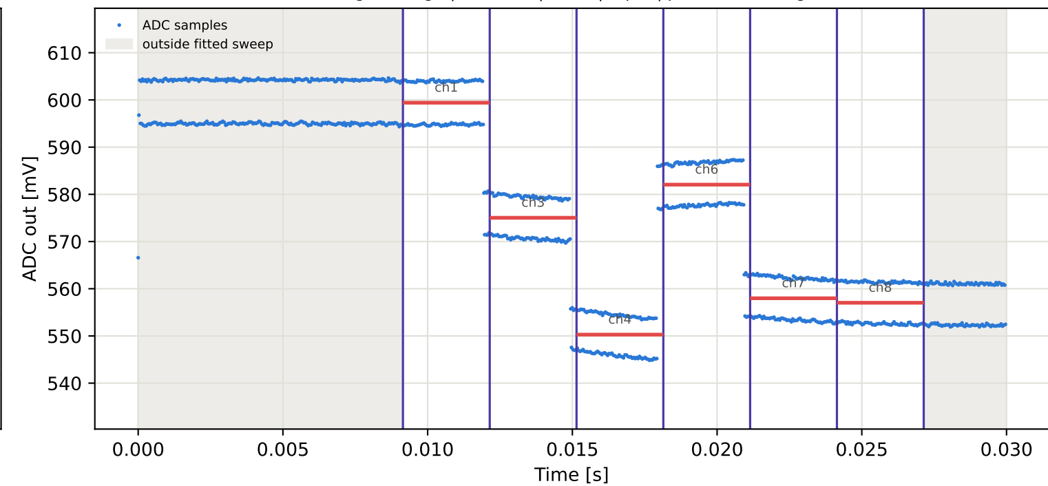
Tag7 &lt;- Tag1 | 865 MHz | run 0 | rep 1 | phase -36.65 deg
