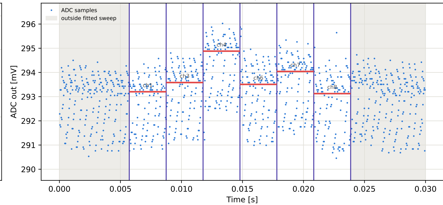
Tag15 &lt;- Tag10 | 995 MHz | run 0 | rep 1 | phase -101.19 deg
