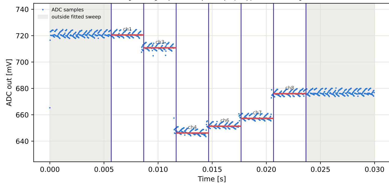
Tag8 &lt;- Tag16 | 825 MHz | run 0 | rep 1 | phase 61.77 deg
