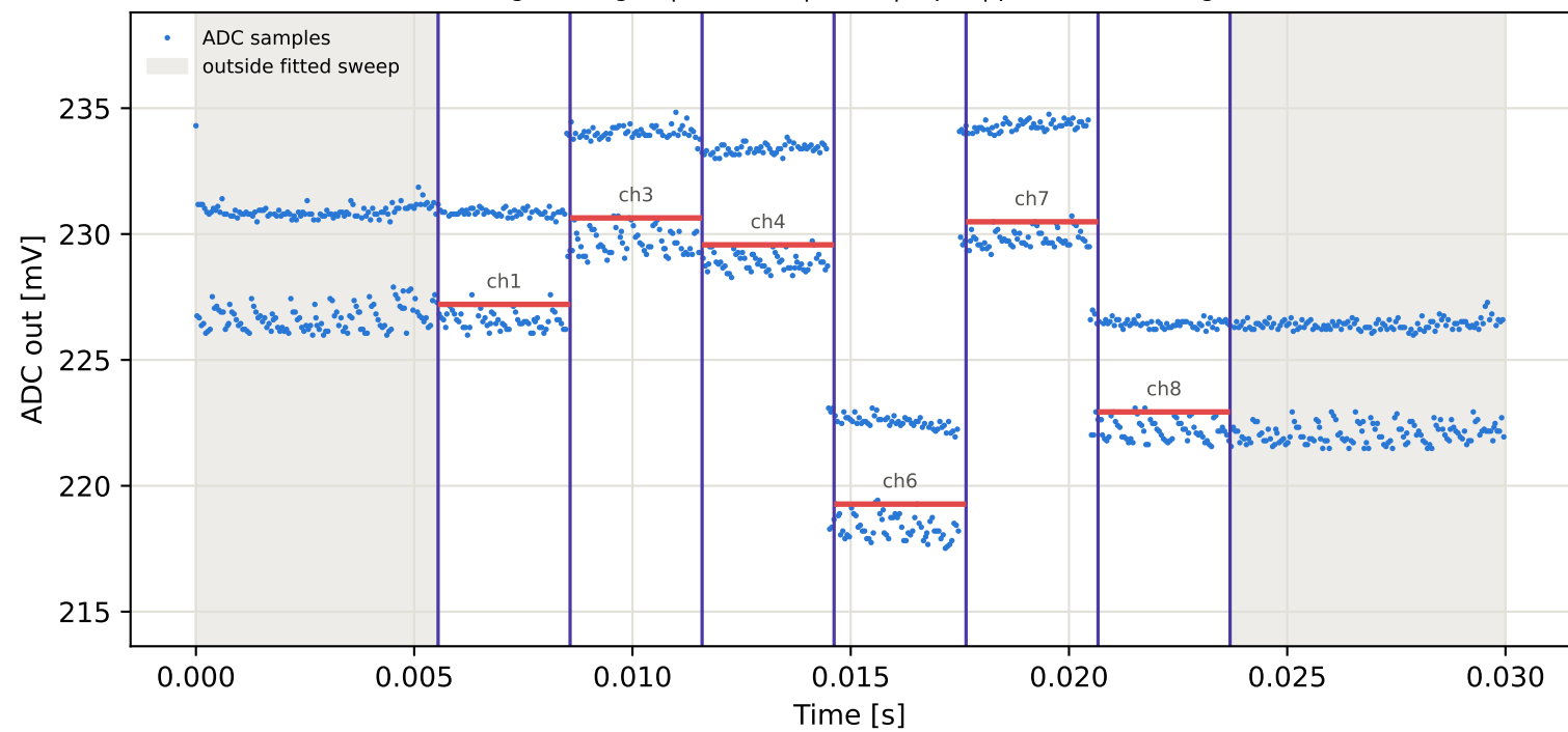
Tag5 &lt;- Tag2 | 985 MHz | run 0 | rep 1 | phase 24.29 deg
