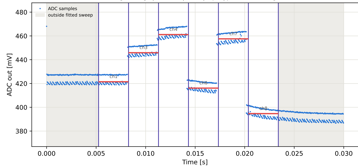
Tag1 &lt;- Tag8 | 905 MHz | run 0 | rep 1 | phase -86.51 deg
