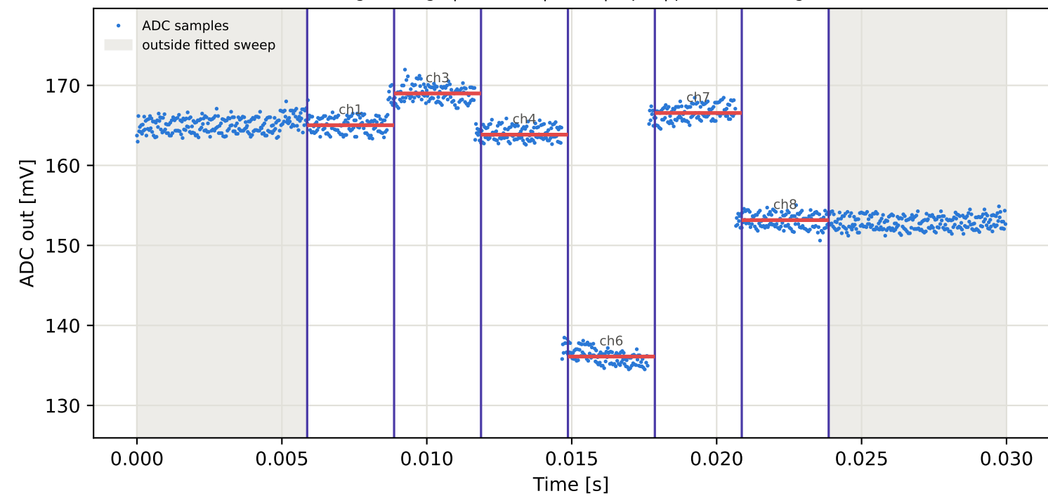
Tag2 &lt;- Tag6 | 935 MHz | run 0 | rep 1 | phase -125.31 deg
