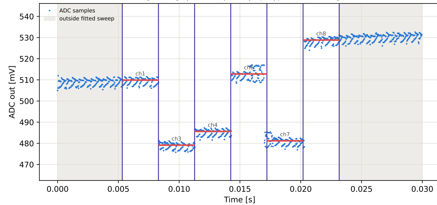
Tag4 &lt;- Tag7 | 865 MHz | run 0 | rep 1 | phase 179.19 deg
