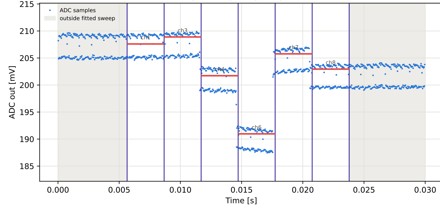
Tag10 &lt;- Tag4 | 945 MHz | run 0 | rep 1 | phase 22.23 deg
