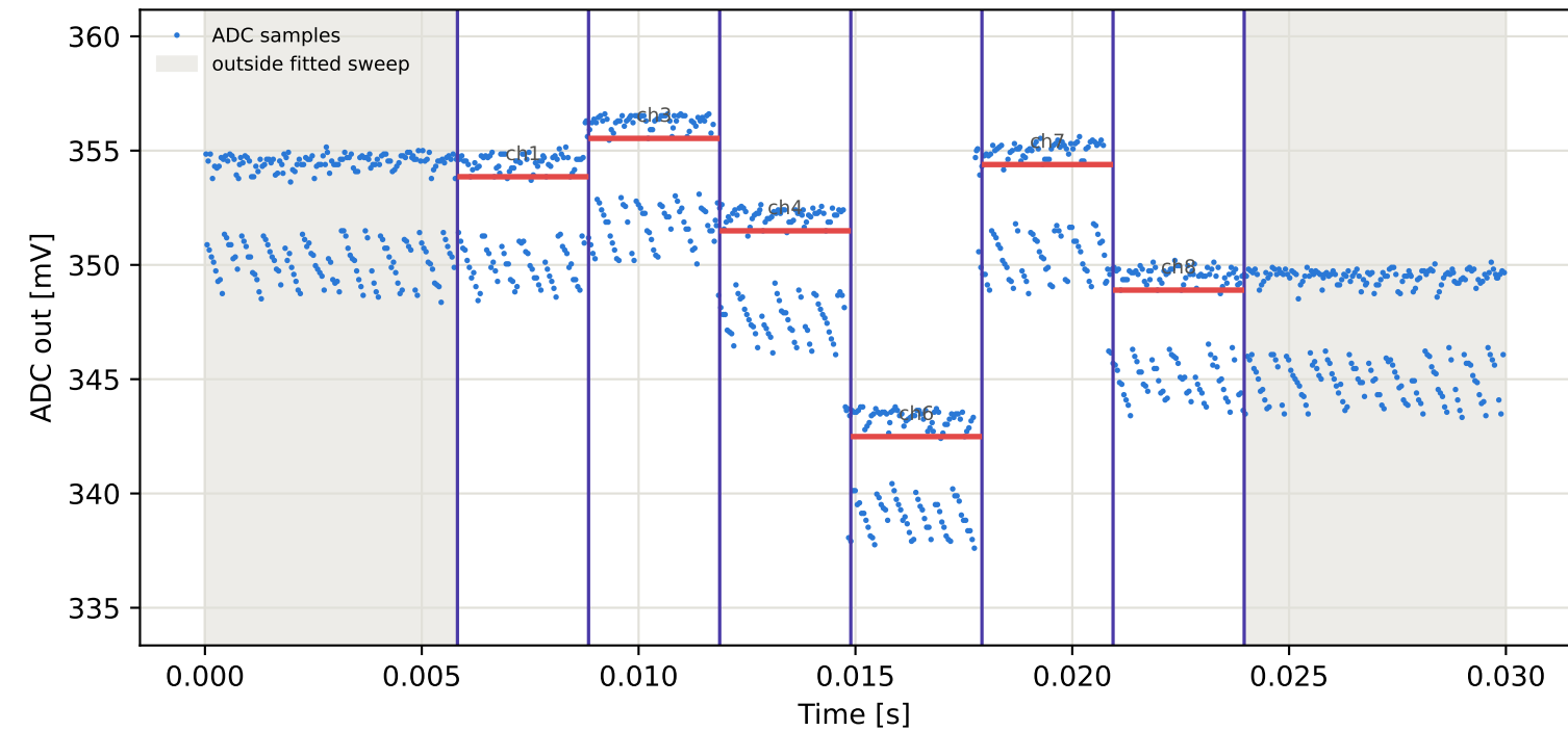
Tag6 &lt;- Tag10 | 955 MHz | run 0 | rep 1 | phase 58.69 deg
