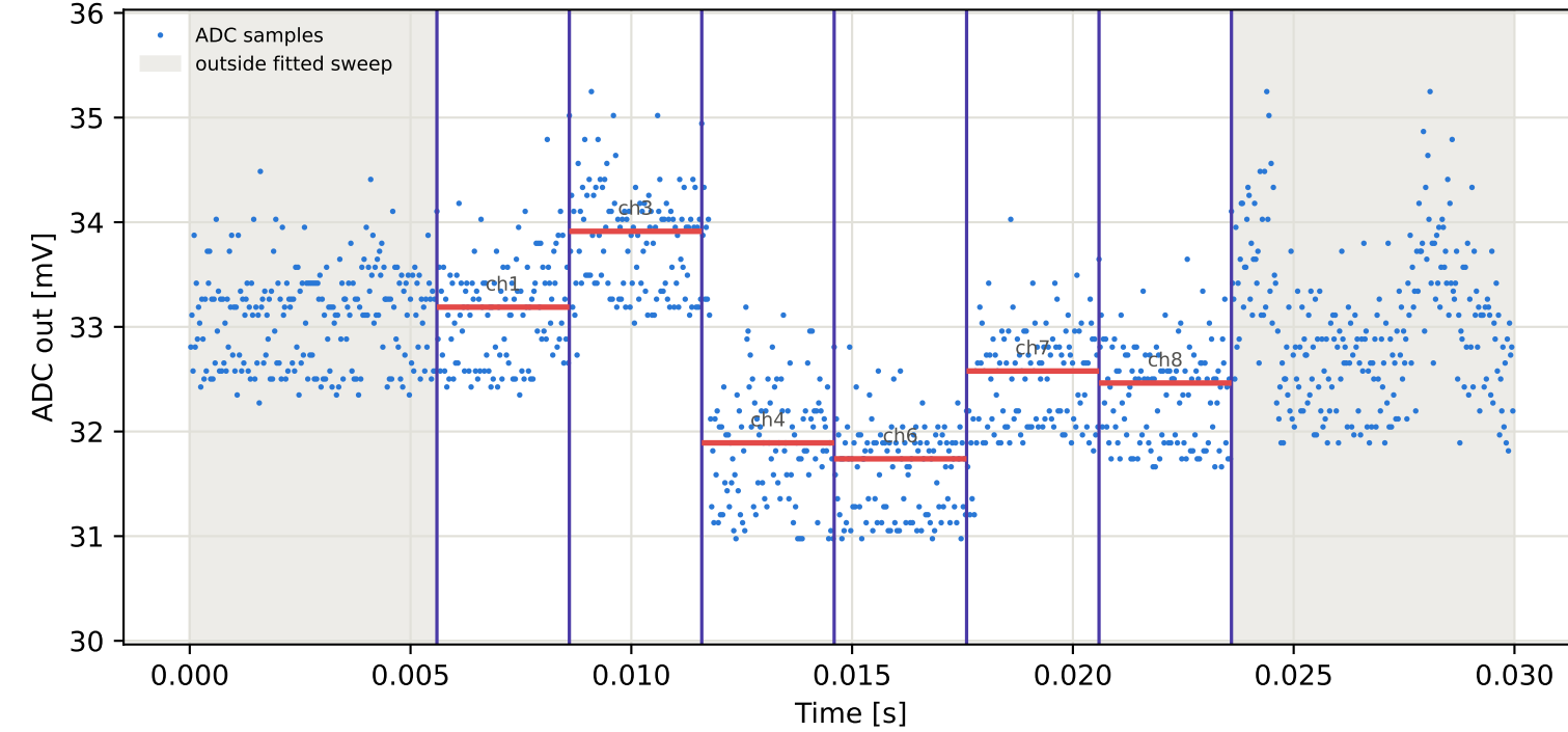
Tag2 &lt;- Tag7 | 775 MHz | run 0 | rep 1 | phase 70.79 deg
