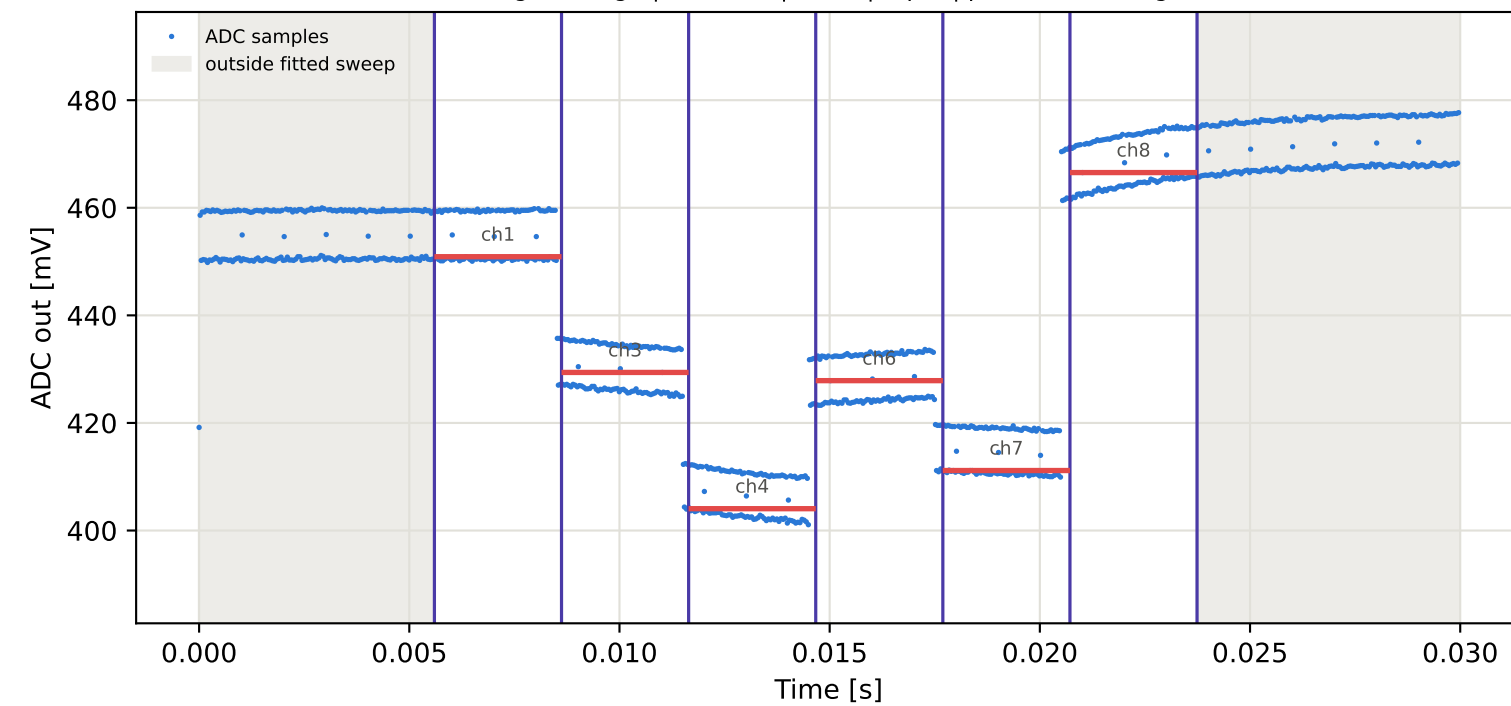
Tag1 &lt;- Tag7 | 905 MHz | run 0 | rep 1 | phase -163.94 deg
