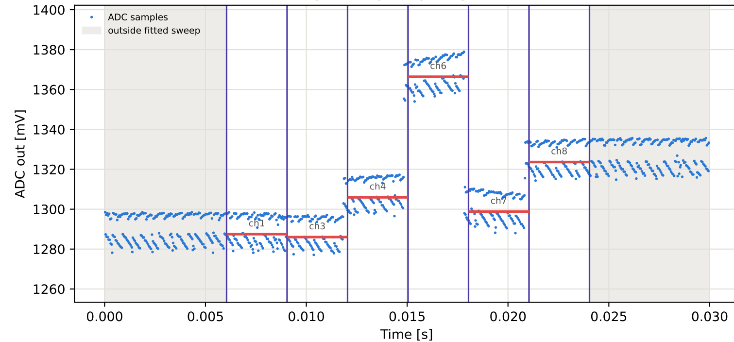
Tag4 &lt;- Tag9 | 915 MHz | run 0 | rep 1 | phase -163.37 deg
