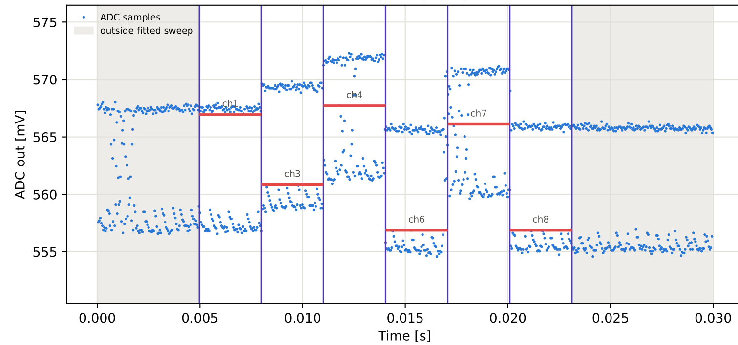
Tag7 &lt;- Tag5 | 965 MHz | run 0 | rep 1 | phase -38.91 deg
