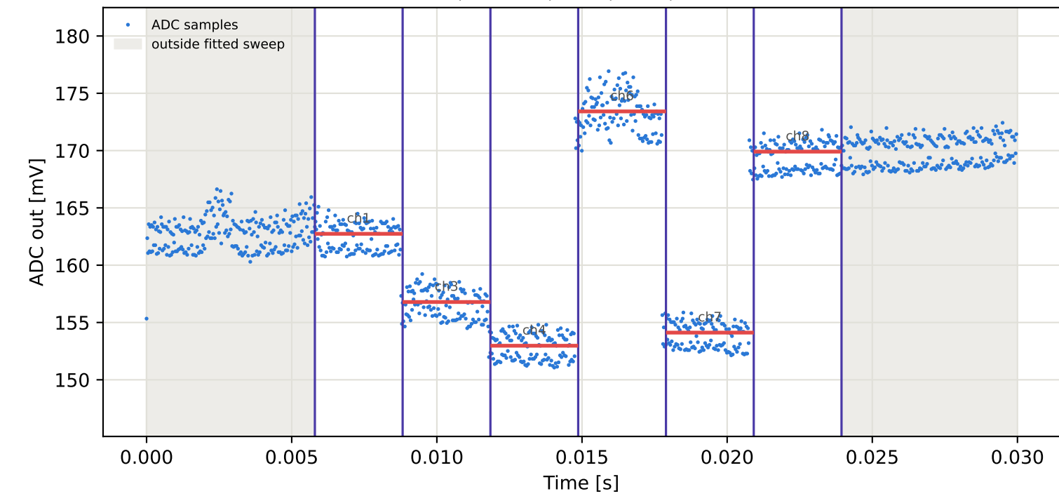
Tag2 &lt;- Tag16 | 935 MHz | run 0 | rep 1 | phase 145.37 deg
