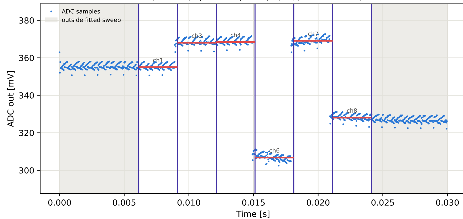
Tag15 &lt;- Tag1 | 925 MHz | run 0 | rep 1 | phase 69.02 deg
