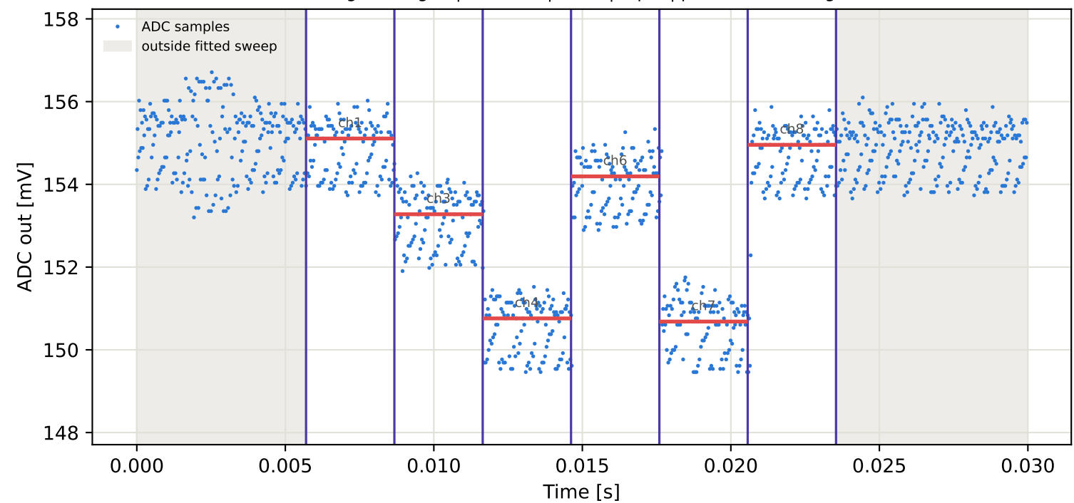
Tag7 &lt;- Tag15 | 805 MHz | run 0 | rep 1 | phase 112.68 deg
