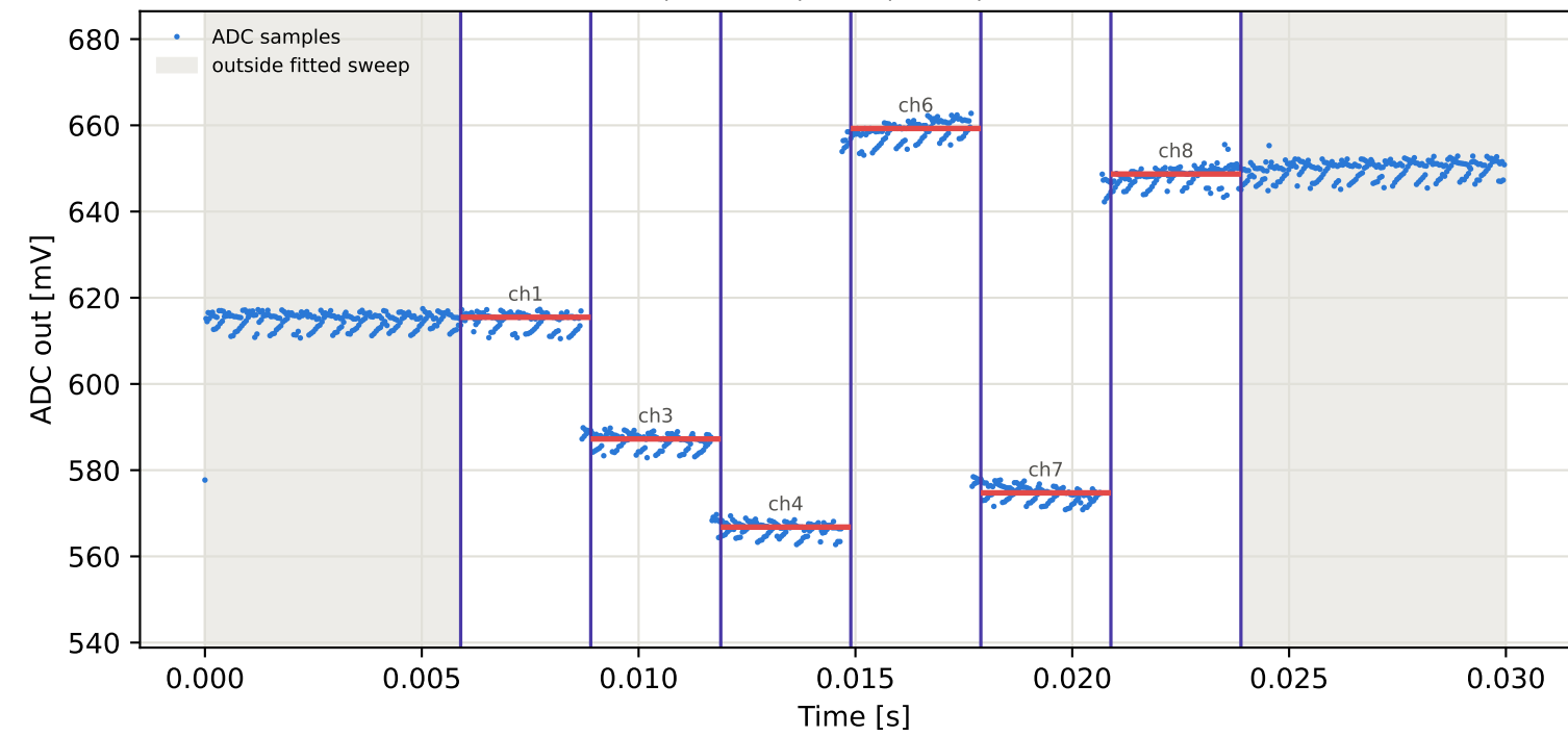
Tag5 &lt;- Tag4 | 935 MHz | run 0 | rep 1 | phase 142.14 deg
