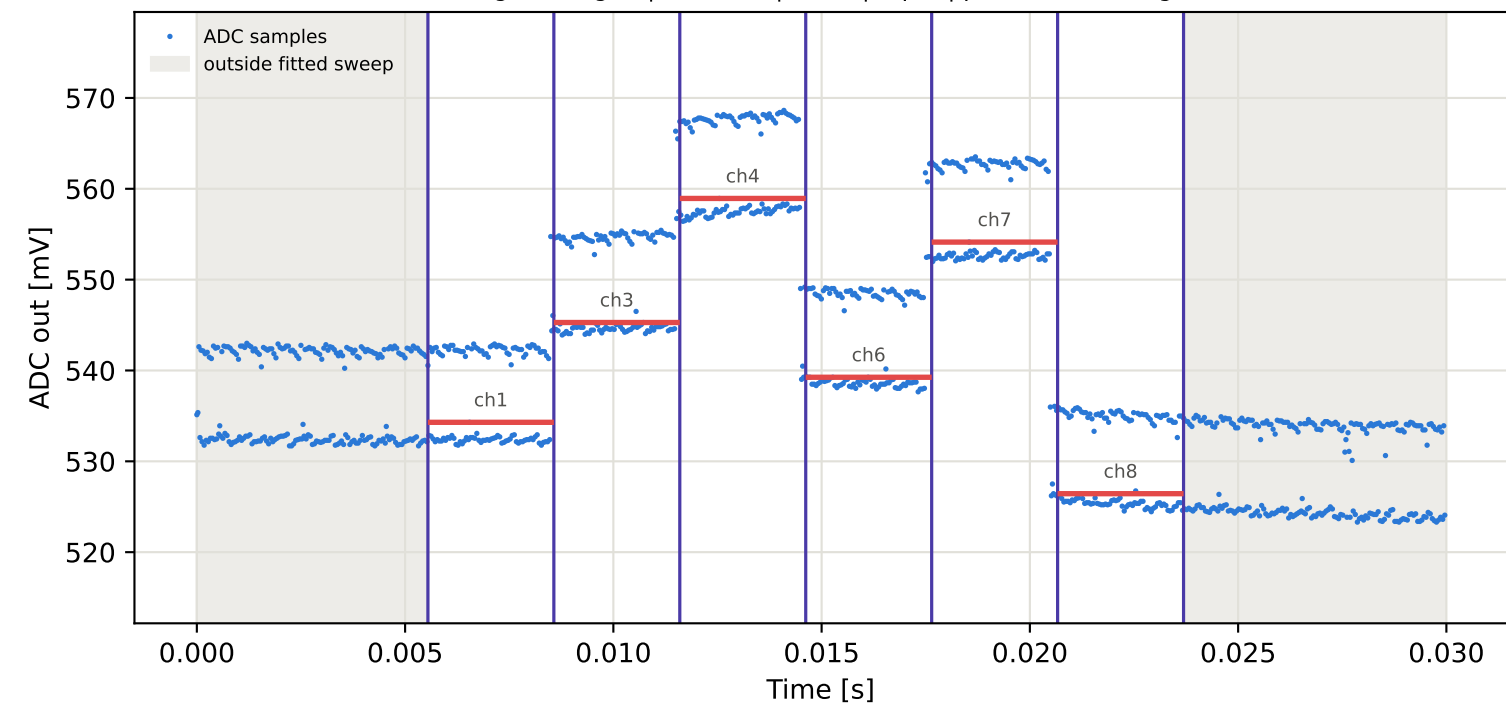
Tag6 &lt;- Tag3 | 915 MHz | run 0 | rep 1 | phase 63.51 deg
