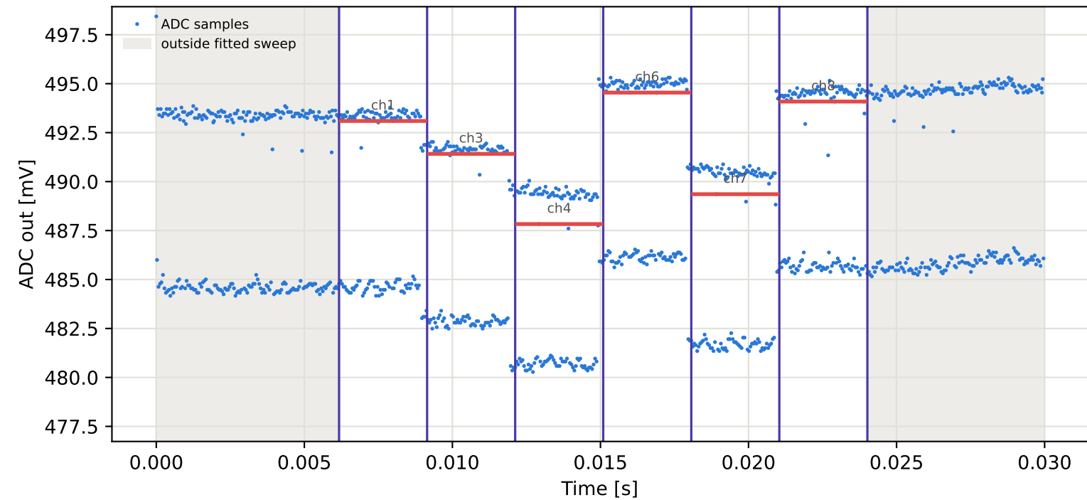
Tag8 &lt;- Tag16 | 995 MHz | run 0 | rep 1 | phase -111.59 deg
