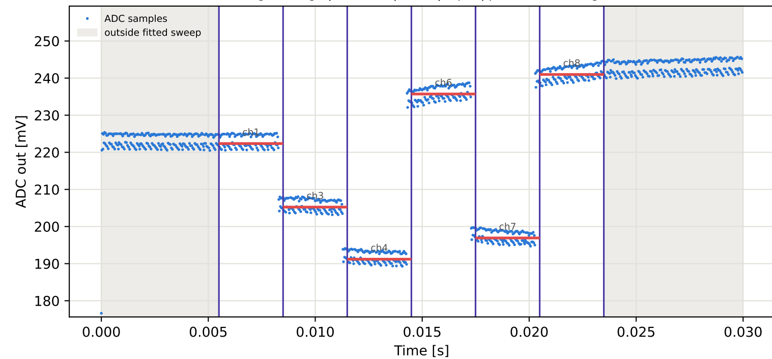
Tag1 &lt;- Tag7 | 925 MHz | run 0 | rep 1 | phase -83.88 deg
