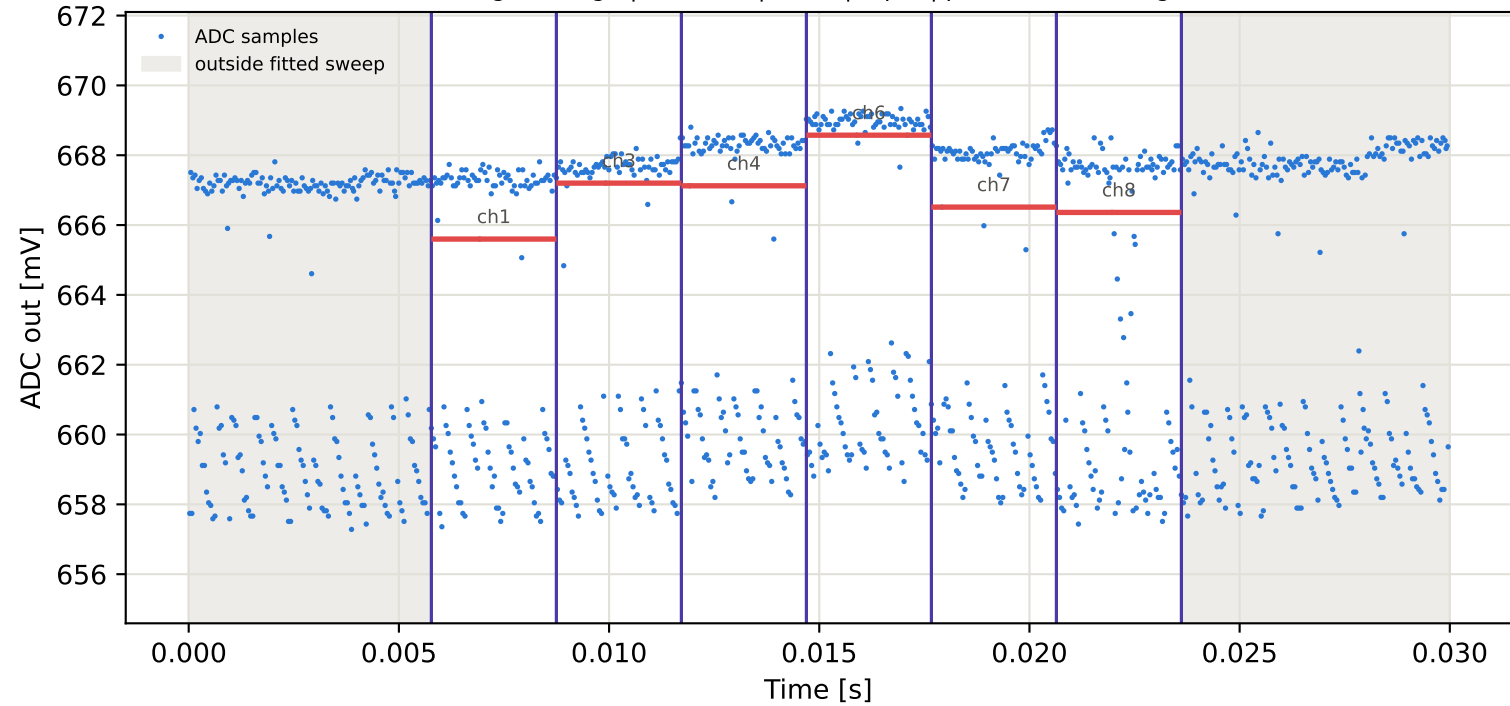
Tag7 &lt;- Tag4 | 865 MHz | run 0 | rep 1 | phase 78.72 deg
