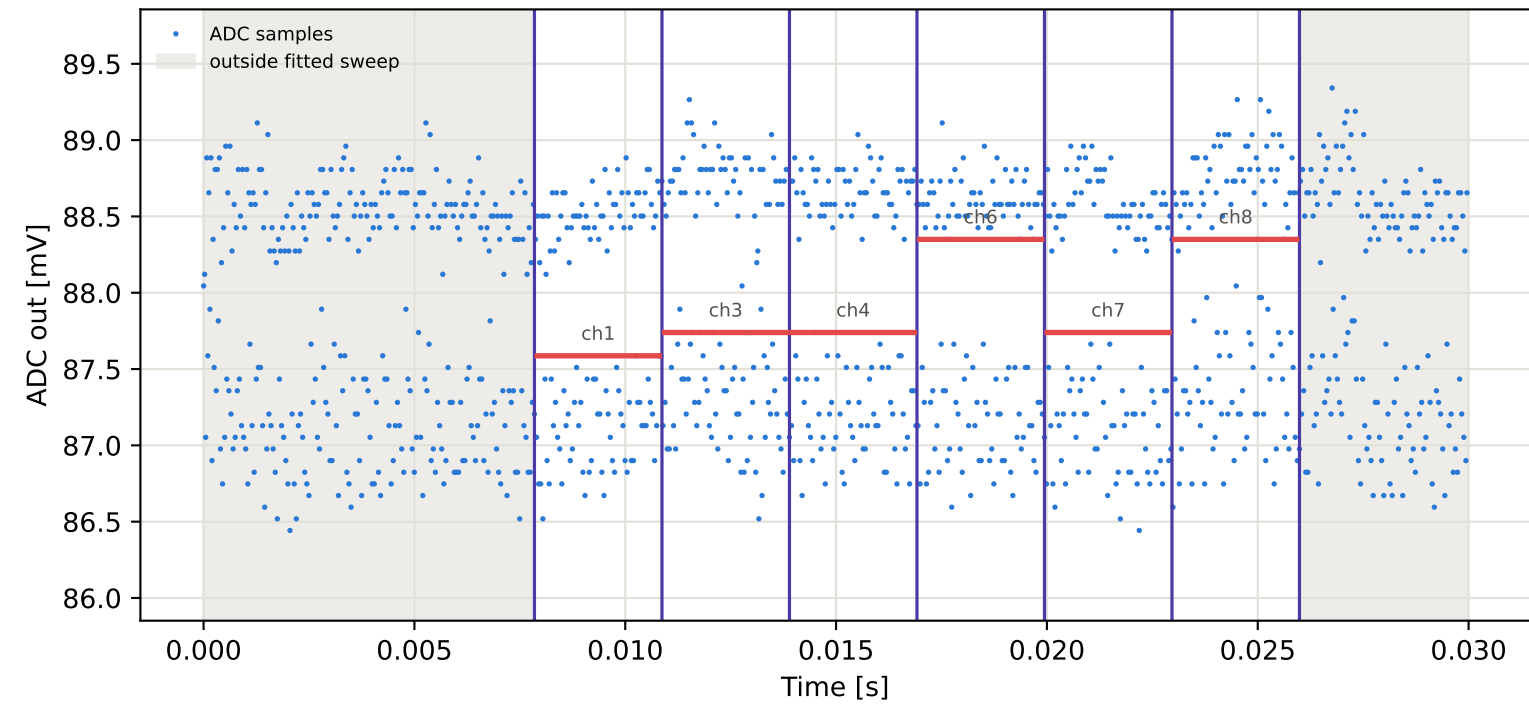
Tag1 &lt;- Tag4 | 795 MHz | run 0 | rep 1 | phase 131.55 deg
