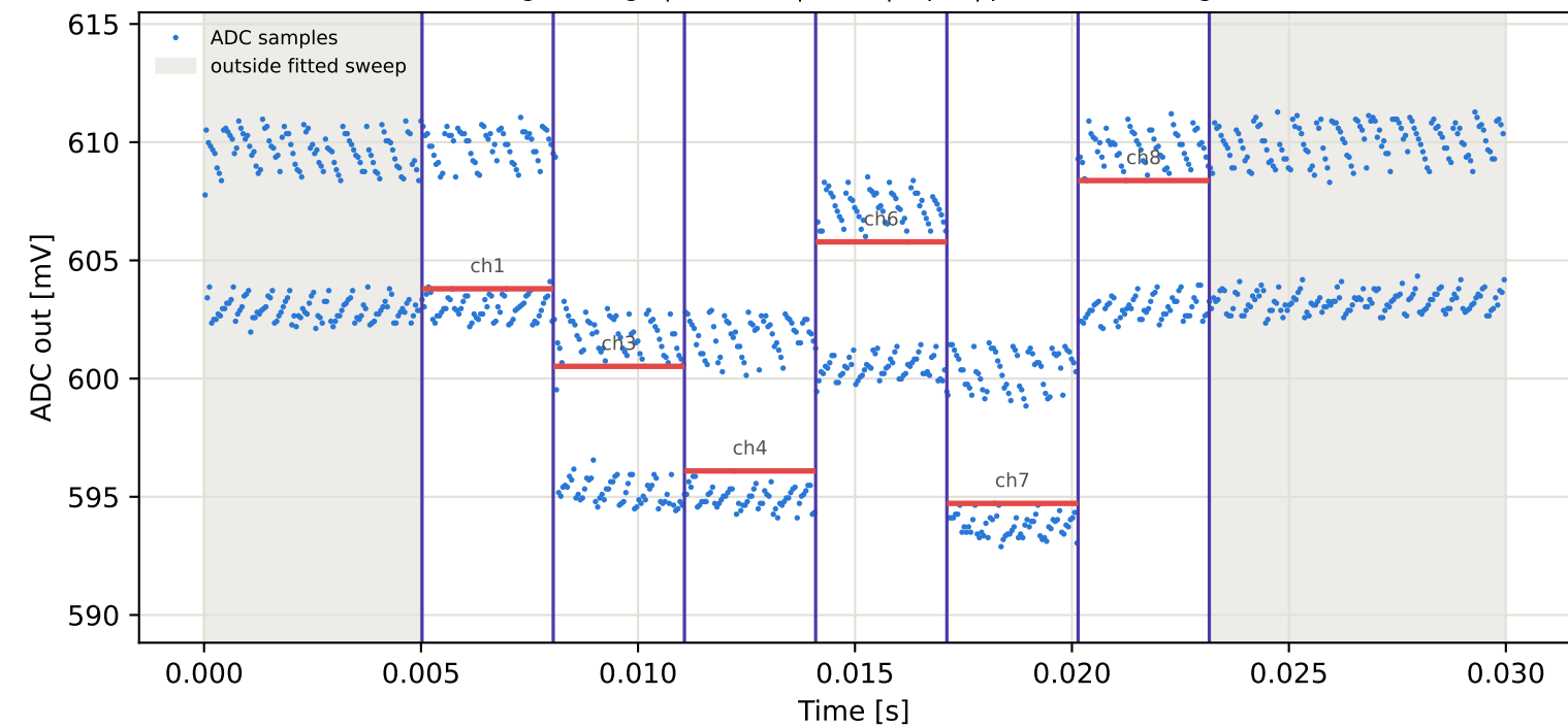
Tag4 &lt;- Tag8 | 835 MHz | run 0 | rep 1 | phase -150.41 deg
