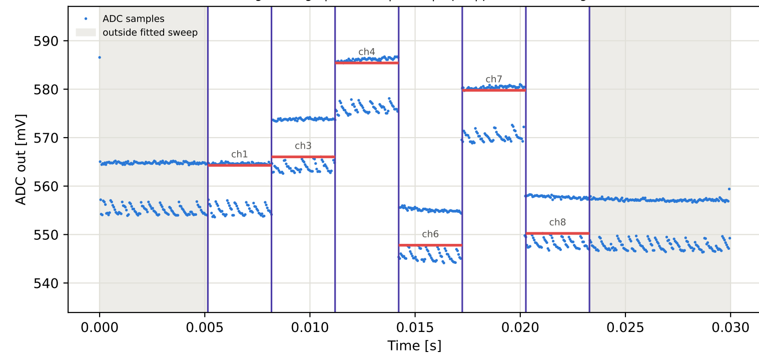
Tag6 &lt;- Tag4 | 975 MHz | run 0 | rep 1 | phase -58.05 deg
