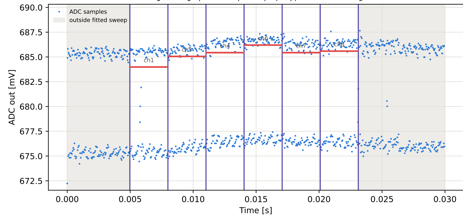
Tag9 &lt;- Tag15 | 875 MHz | run 0 | rep 1 | phase -64.80 deg
