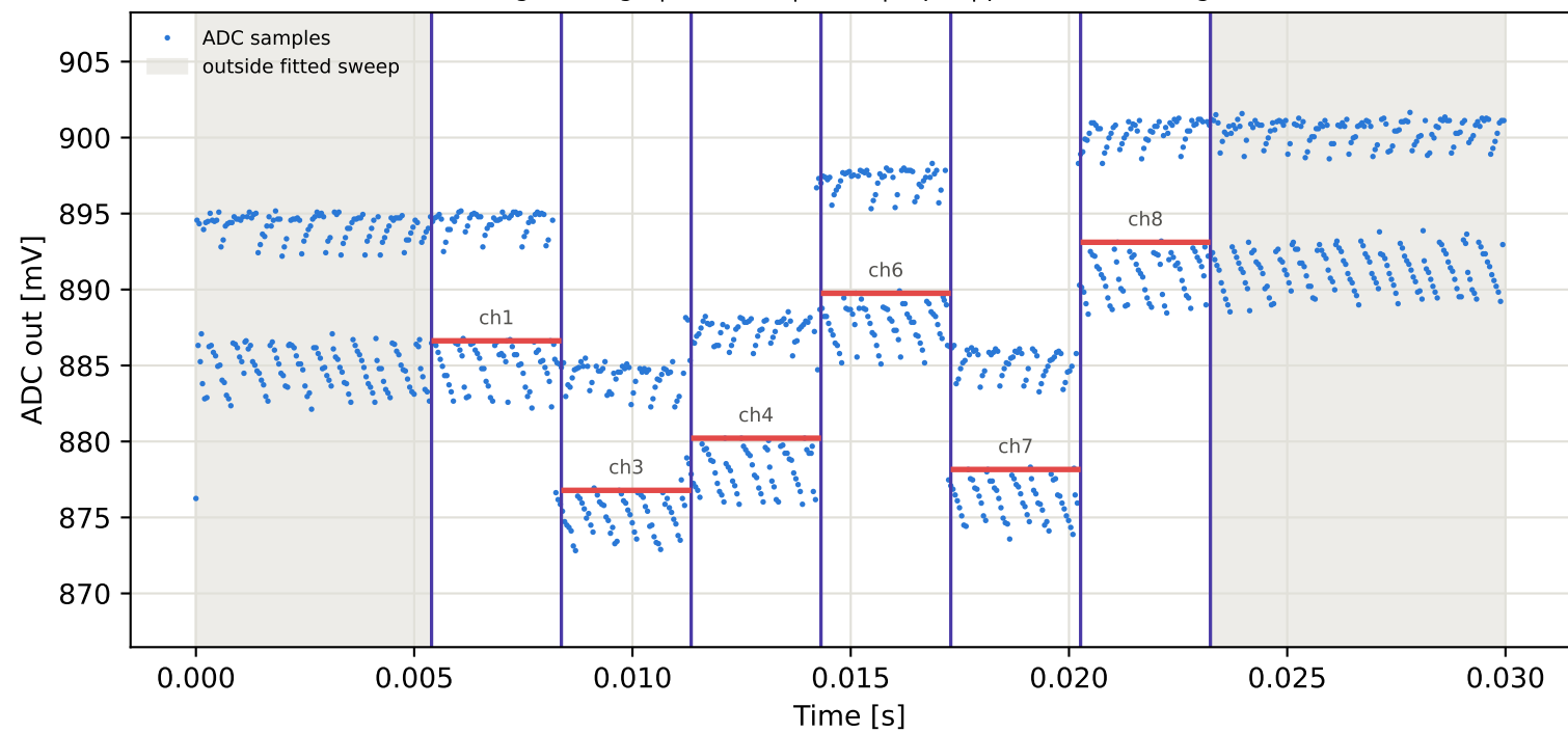
Tag8 &lt;- Tag5 | 845 MHz | run 0 | rep 1 | phase -168.39 deg
