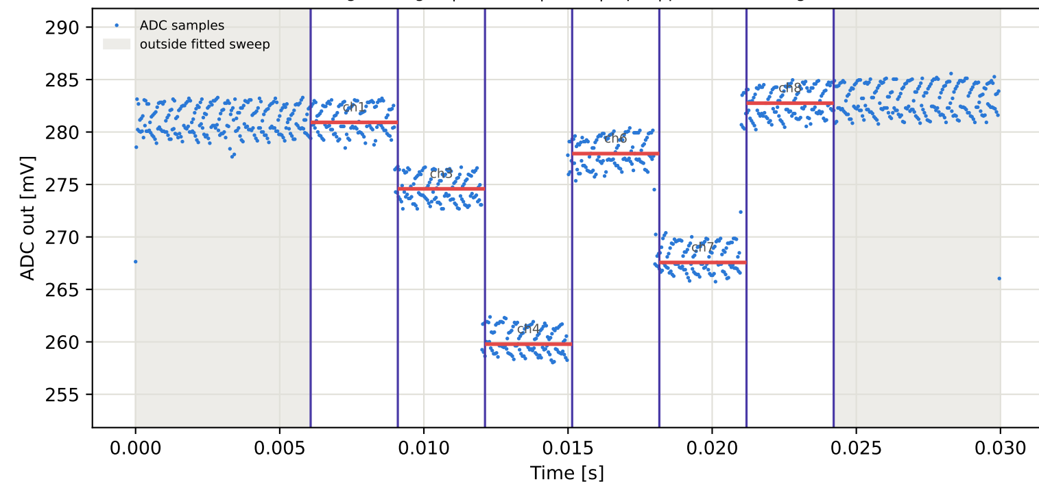
Tag9 &lt;- Tag2 | 995 MHz | run 0 | rep 1 | phase -106.66 deg
