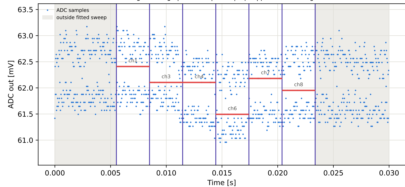
Tag16 &lt;- Tag4 | 785 MHz | run 0 | rep 1 | phase 42.22 deg
