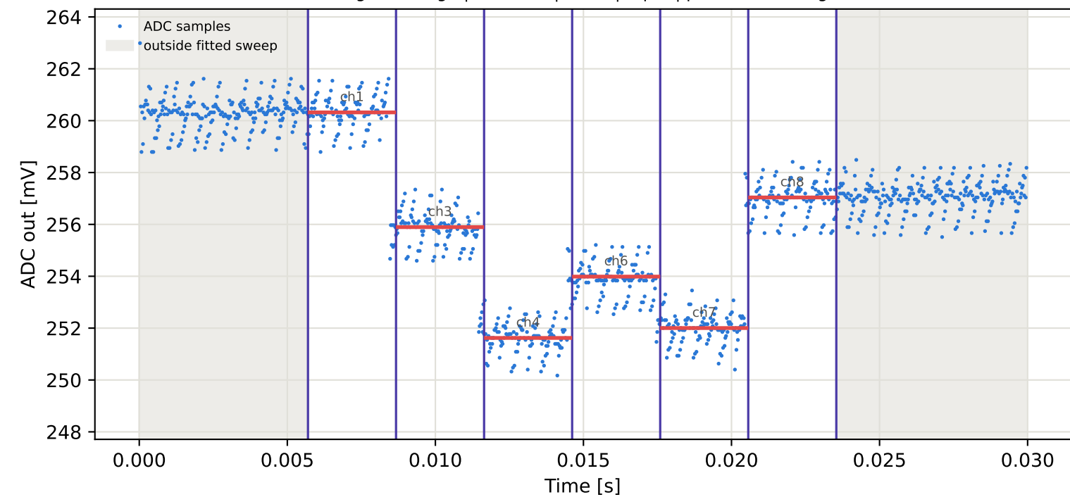
Tag10 &lt;- Tag5 | 845 MHz | run 0 | rep 1 | phase 79.03 deg
