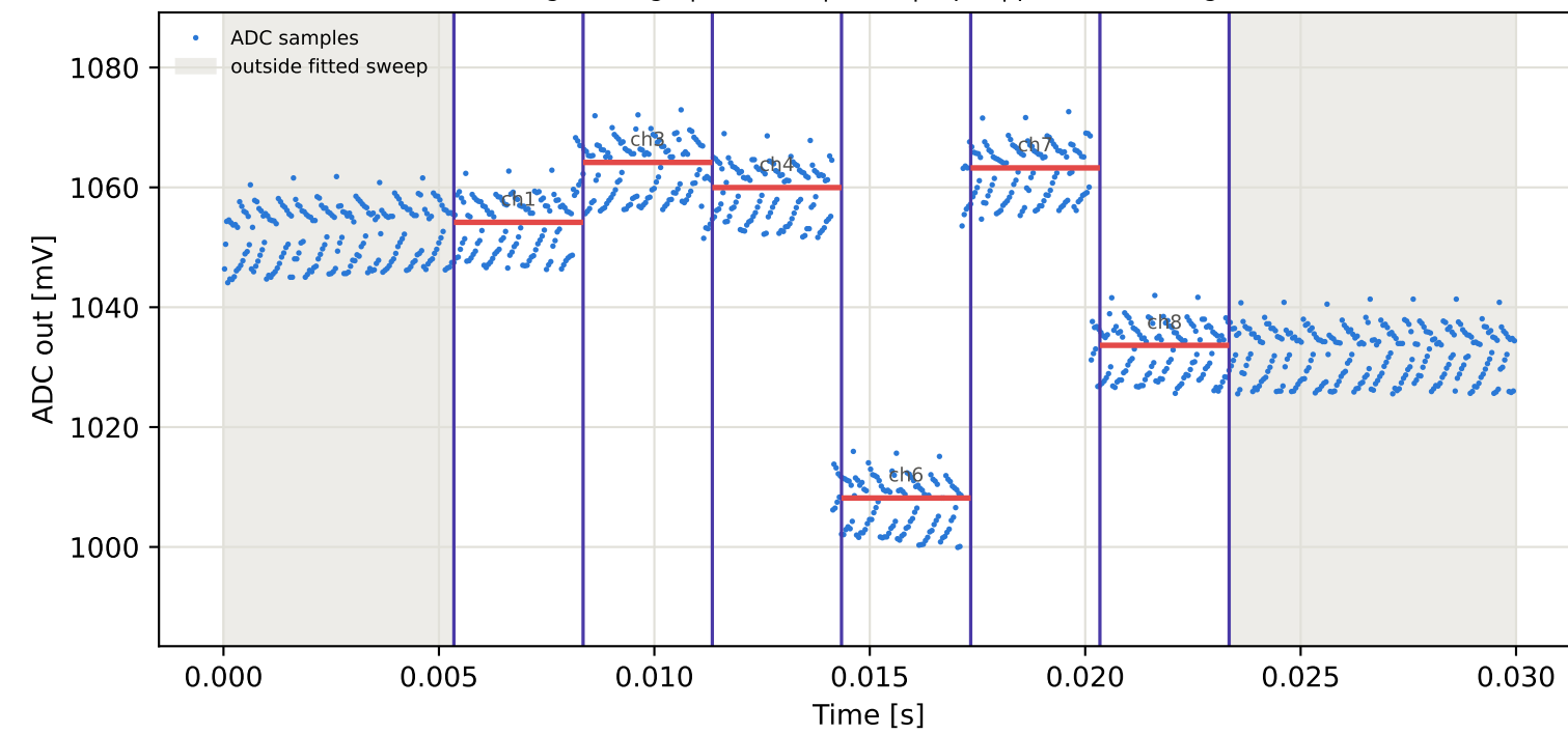
Tag4 &lt;- Tag7 | 945 MHz | run 0 | rep 1 | phase -117.42 deg
