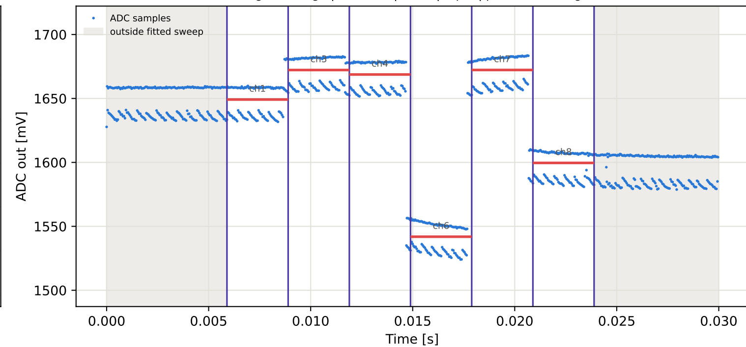
Tag15 &lt;- Tag6 | 935 MHz | run 0 | rep 1 | phase -2.61 deg
