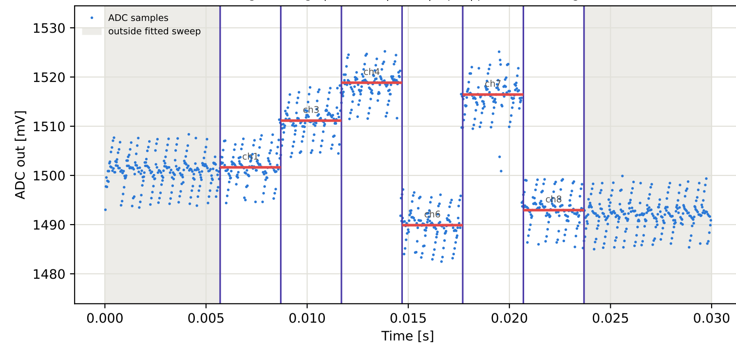
Tag15 &lt;- Tag9 | 955 MHz | run 0 | rep 1 | phase 142.87 deg
