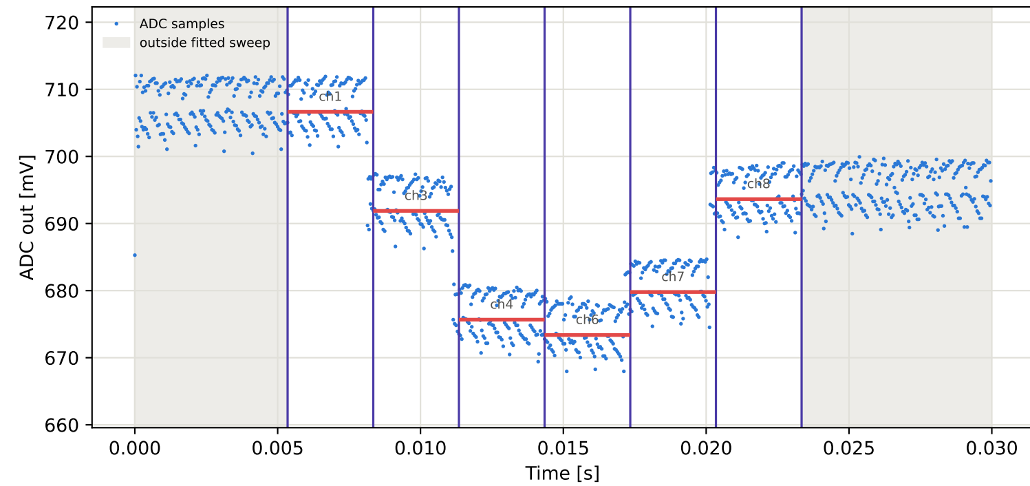
Tag10 &lt;- Tag9 | 885 MHz | run 0 | rep 1 | phase -119.01 deg
