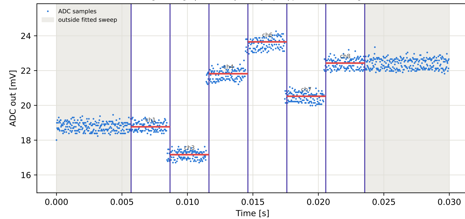
Tag1 &lt;- Tag7 | 845 MHz | run 0 | rep 1 | phase 86.86 deg
