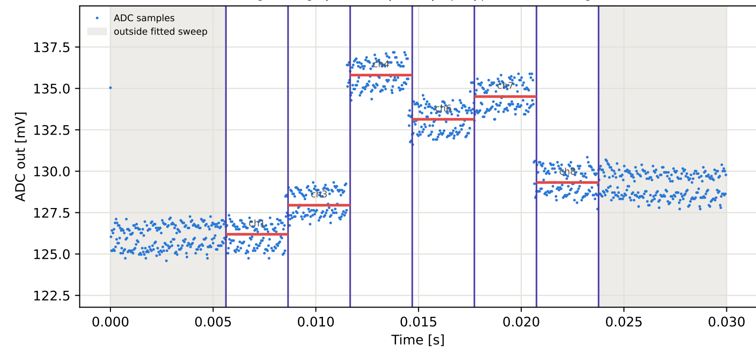
Tag6 &lt;- Tag9 | 805 MHz | run 0 | rep 1 | phase -84.76 deg
