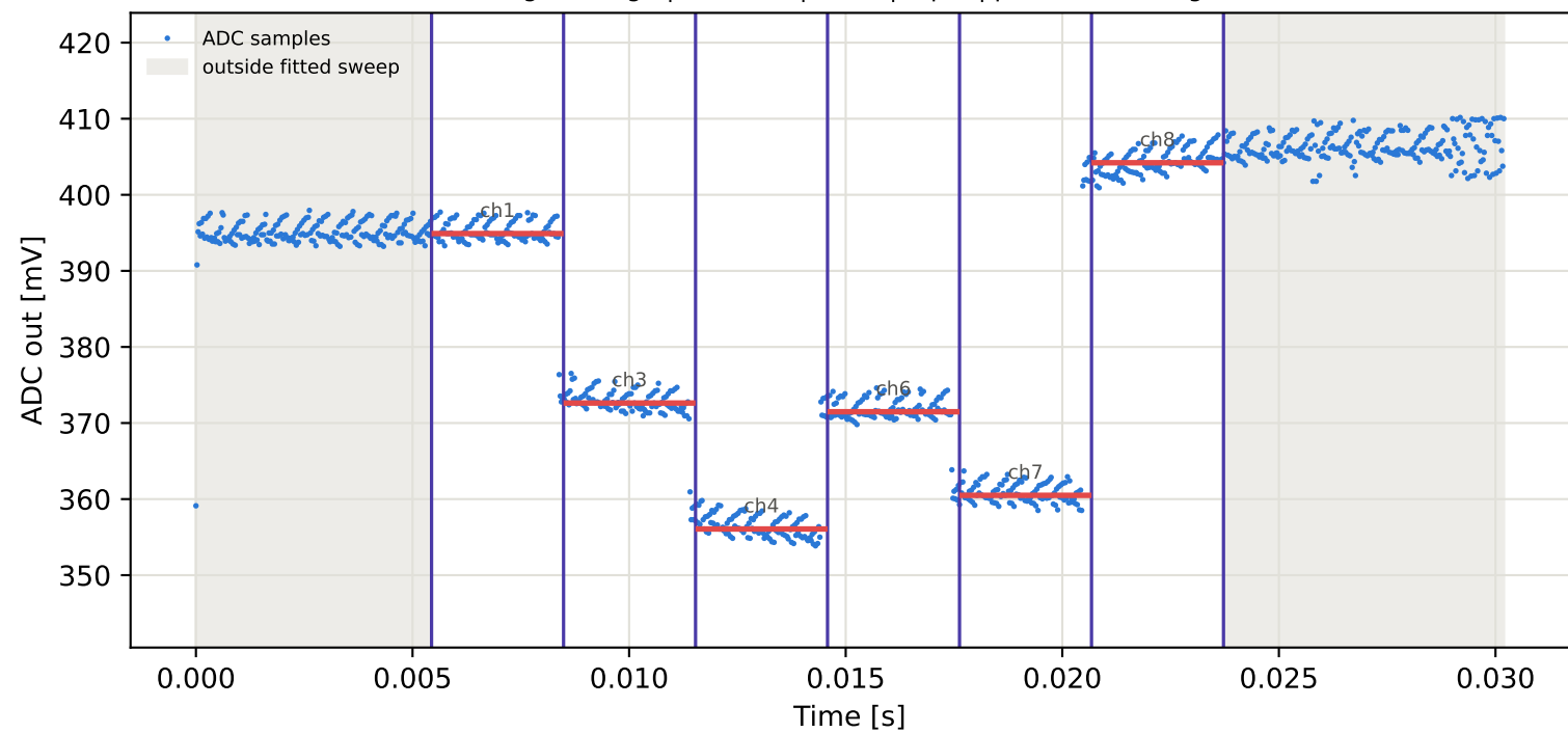
Tag7 &lt;- Tag6 | 895 MHz | run 0 | rep 1 | phase -153.77 deg
