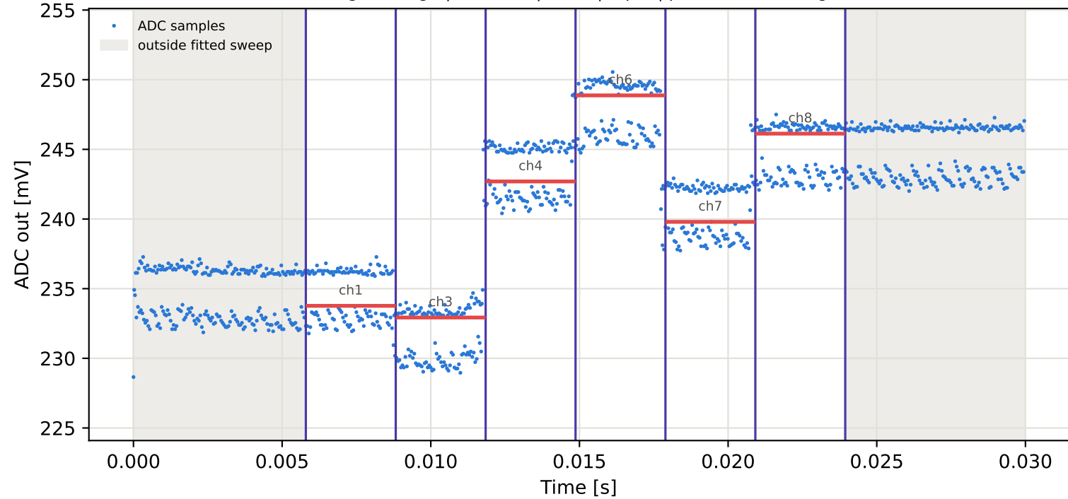
Tag2 &lt;- Tag6 | 835 MHz | run 0 | rep 1 | phase -77.22 deg
