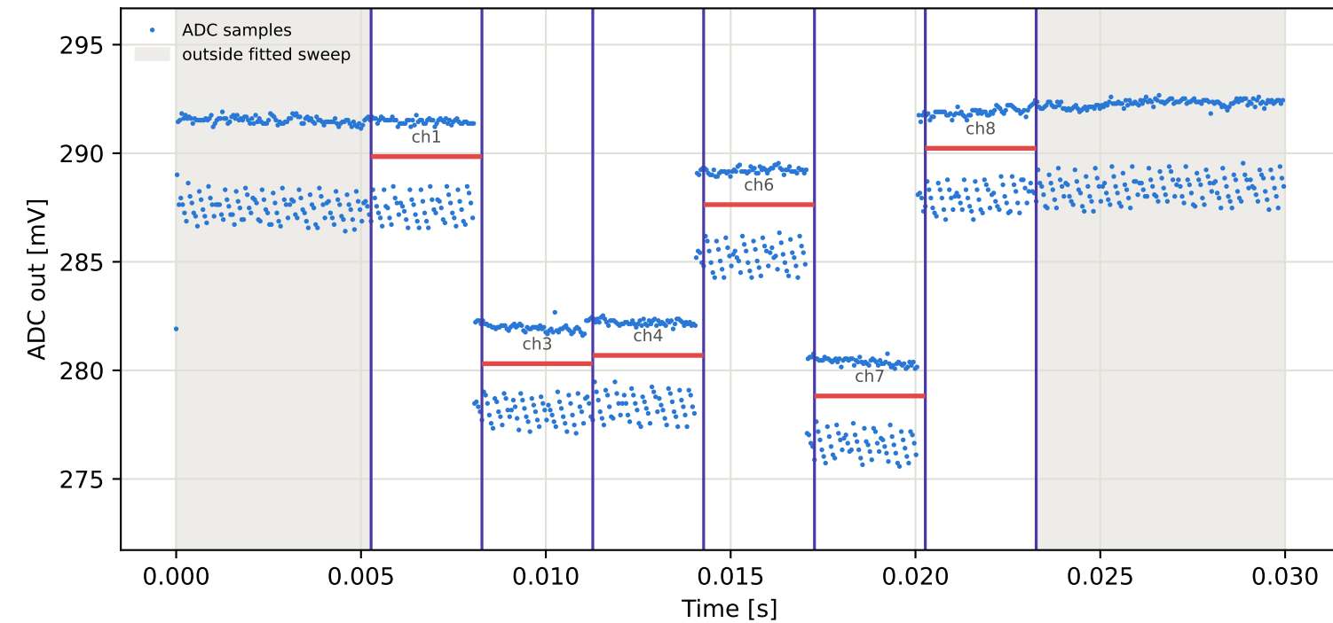
Tag3 &lt;- Tag16 | 835 MHz | run 0 | rep 1 | phase -100.91 deg
