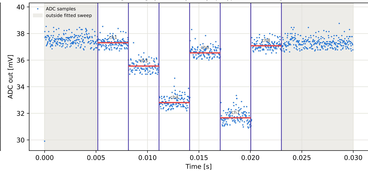
Tag2 &lt;- Tag6 | 775 MHz | run 0 | rep 1 | phase 29.70 deg
