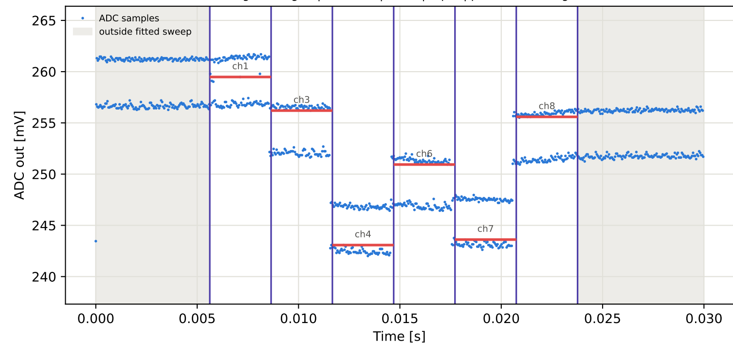
Tag6 &lt;- Tag10 | 825 MHz | run 0 | rep 1 | phase 85.97 deg
