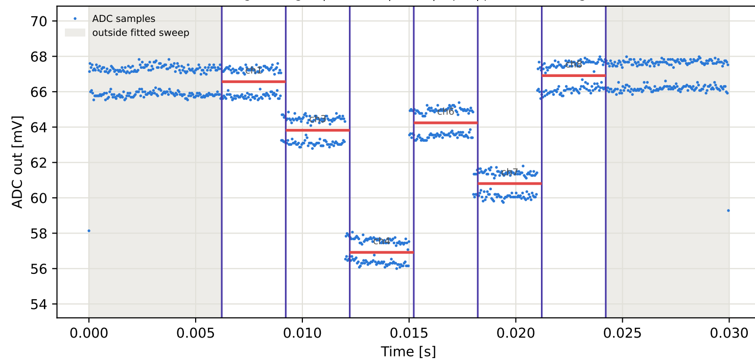
Tag6 &lt;- Tag2 | 995 MHz | run 0 | rep 1 | phase -47.22 deg
