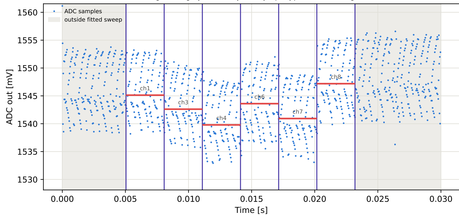
Tag5 &lt;- Tag4 | 895 MHz | run 0 | rep 1 | phase 50.89 deg
