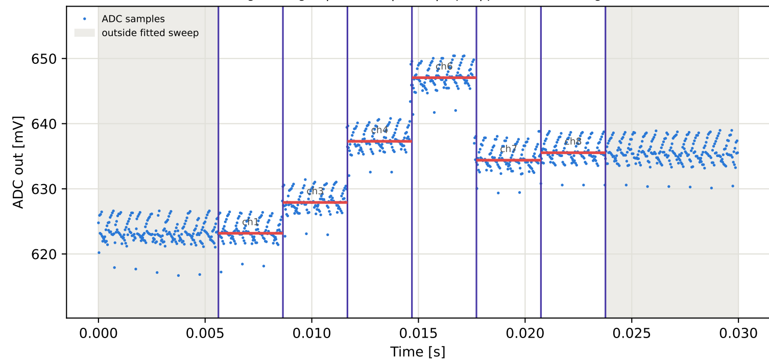
Tag9 &lt;- Tag2 | 895 MHz | run 0 | rep 1 | phase 148.81 deg
