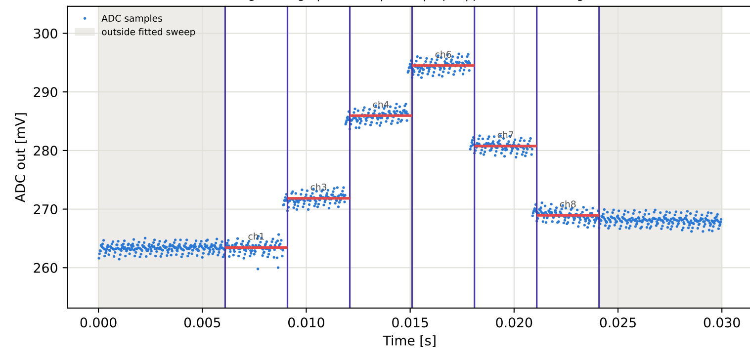
Tag1 &lt;- Tag9 | 915 MHz | run 0 | rep 1 | phase -130.02 deg
