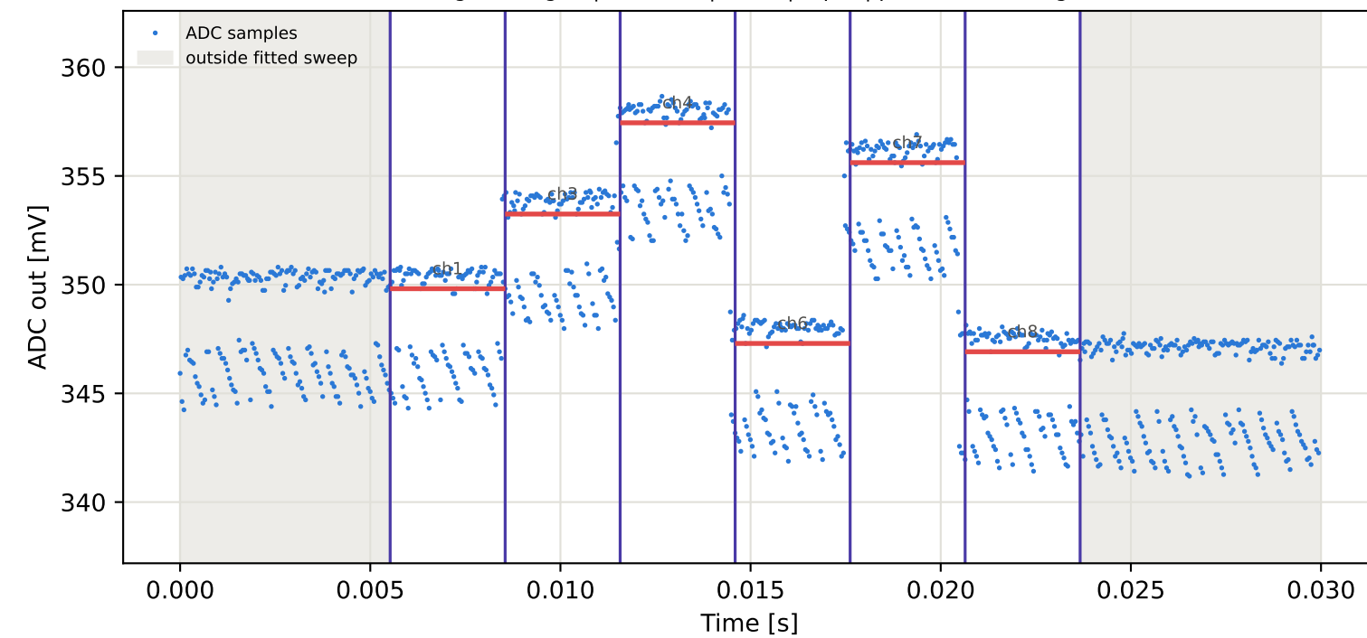
Tag5 &lt;- Tag16 | 955 MHz | run 0 | rep 1 | phase -18.81 deg
