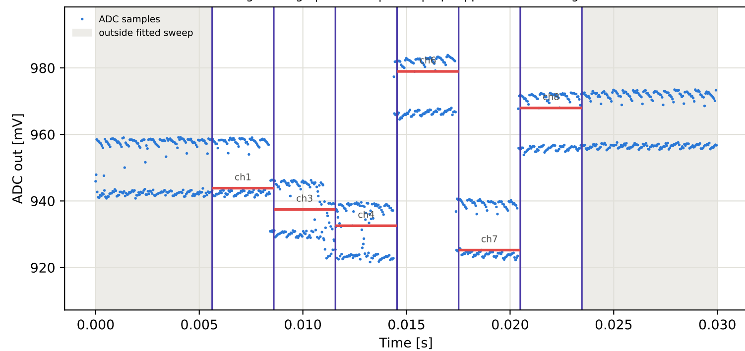
Tag8 &lt;- Tag5 | 975 MHz | run 0 | rep 1 | phase -164.57 deg
