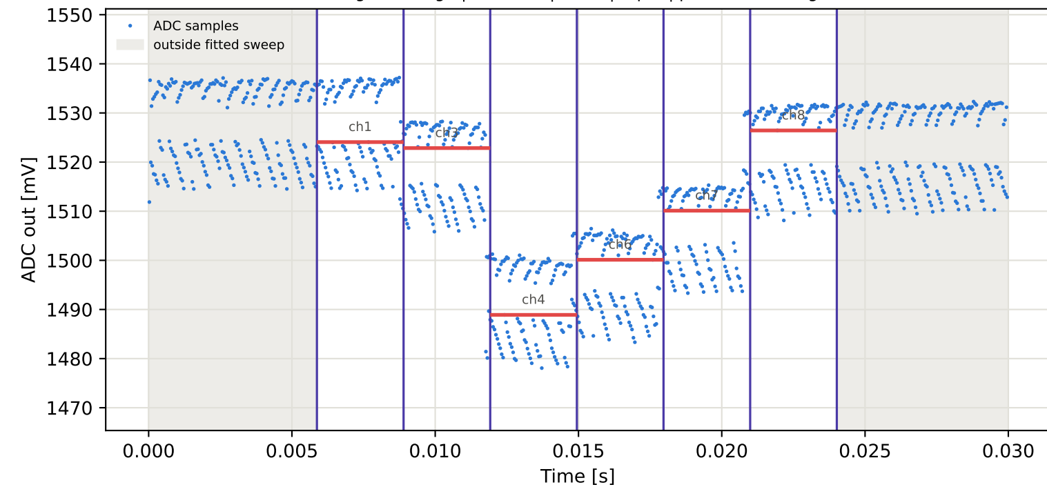
Tag15 &lt;- Tag5 | 955 MHz | run 0 | rep 1 | phase 55.06 deg
