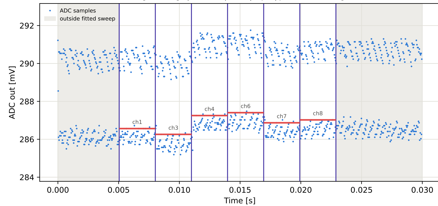
Tag15 &lt;- Tag9 | 785 MHz | run 0 | rep 1 | phase 81.47 deg
