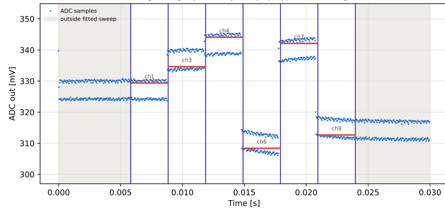
Tag1 &lt;- Tag3 | 935 MHz | run 0 | rep 1 | phase 81.96 deg
