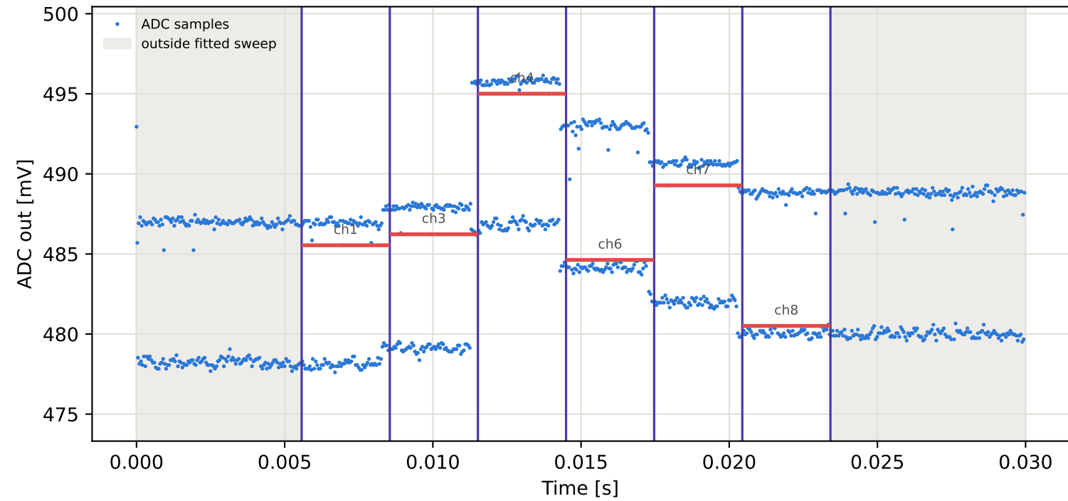
Tag8 &lt;- Tag7 | 995 MHz | run 0 | rep 1 | phase 88.27 deg
