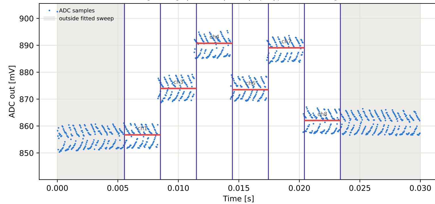
Tag9 &lt;- Tag10 | 845 MHz | run 0 | rep 1 | phase -140.53 deg
