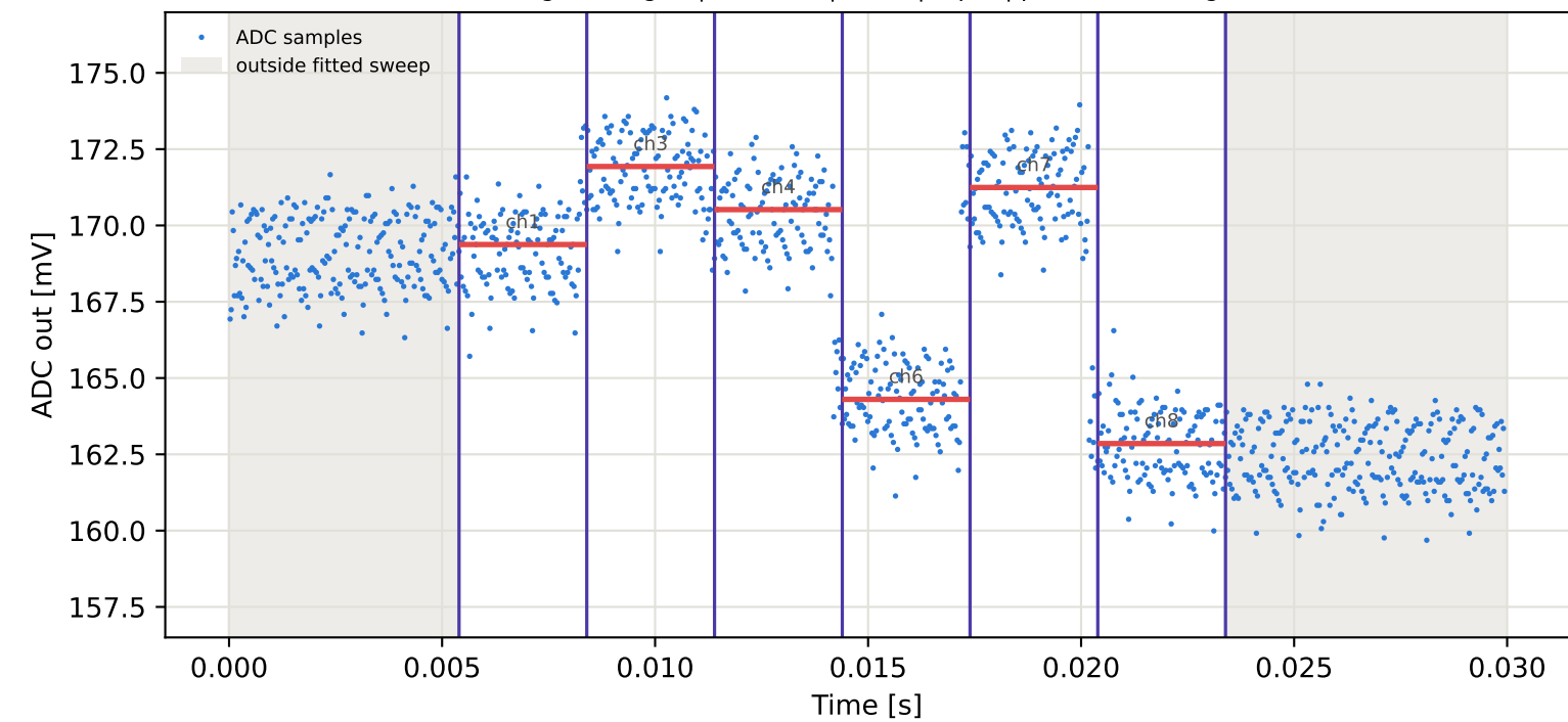
Tag6 &lt;- Tag2 | 885 MHz | run 0 | rep 1 | phase 148.12 deg
