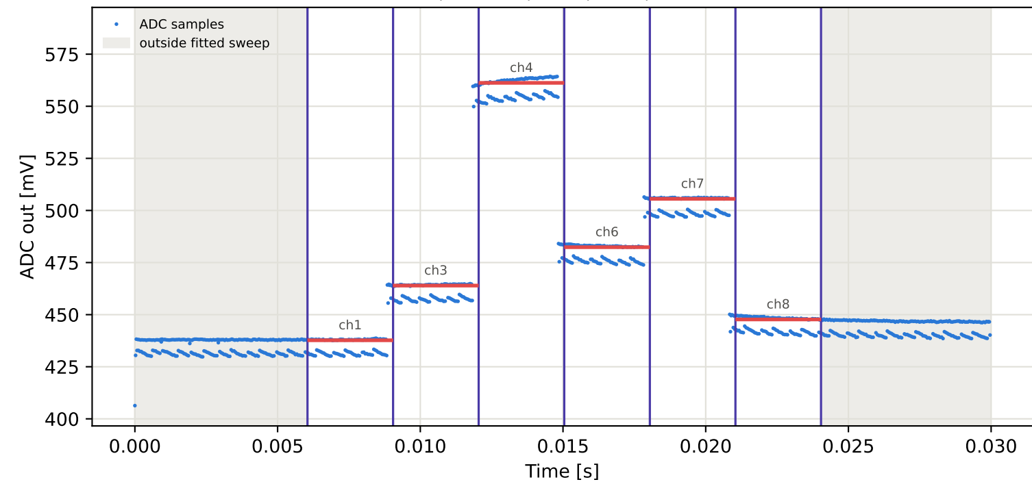
Tag8 &lt;- Tag16 | 995 MHz | run 0 | rep 1 | phase -111.59 deg
