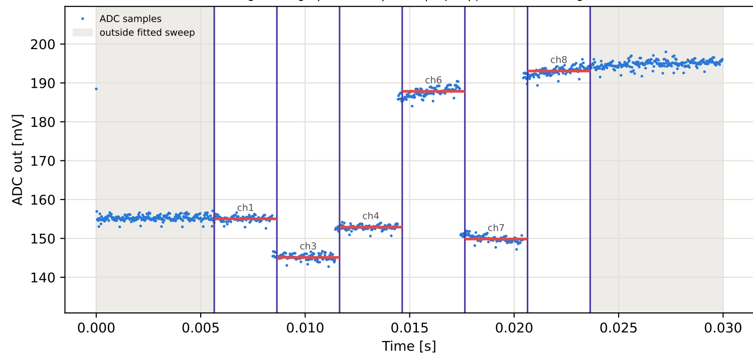
Tag6 &lt;- Tag5 | 885 MHz | run 0 | rep 1 | phase 172.87 deg
