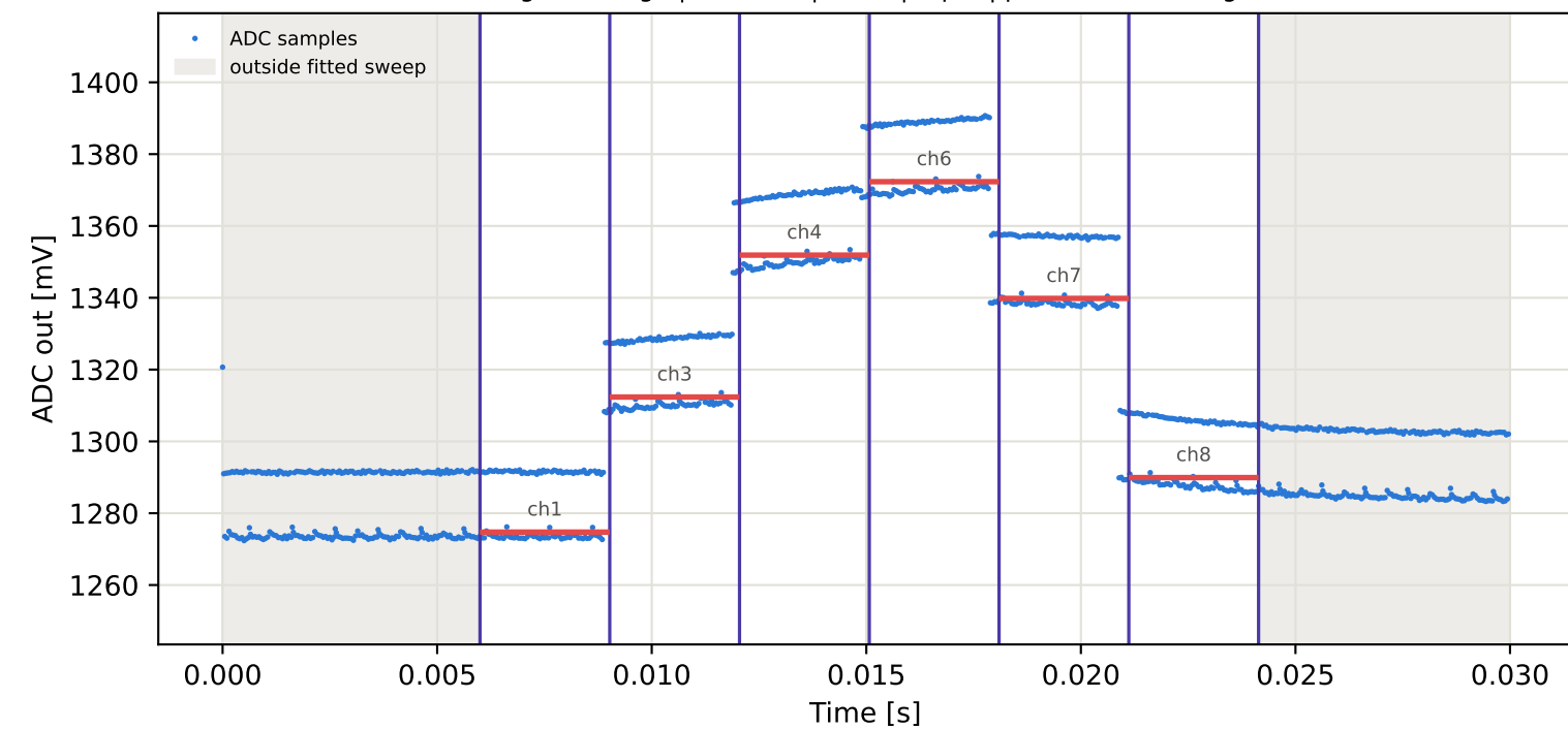
Tag15 &lt;- Tag5 | 895 MHz | run 0 | rep 1 | phase -124.23 deg
