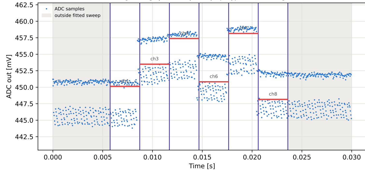
Tag3 &lt;- Tag15 | 855 MHz | run 0 | rep 1 | phase -23.77 deg
