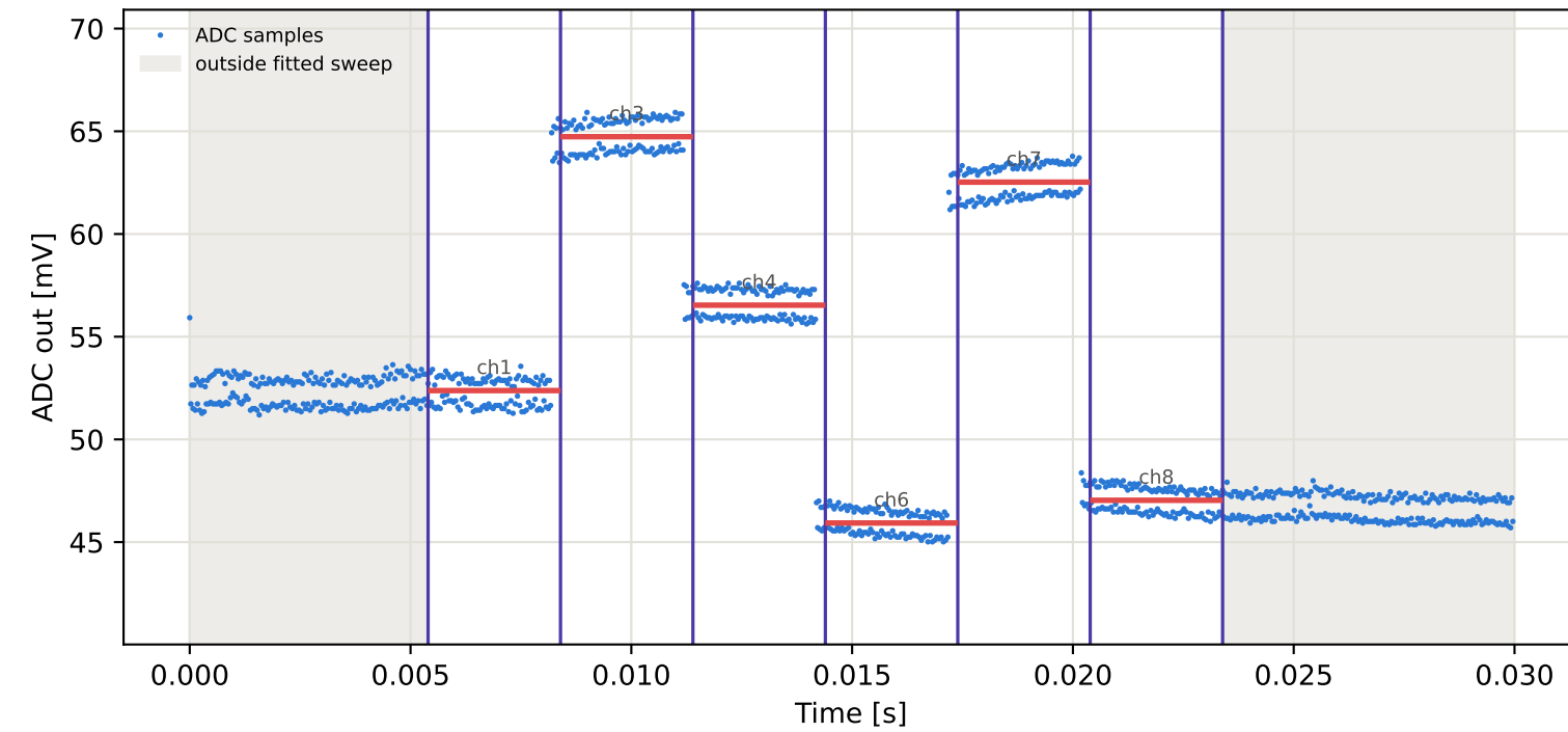
Tag6 &lt;- Tag1 | 795 MHz | run 0 | rep 1 | phase 52.48 deg
