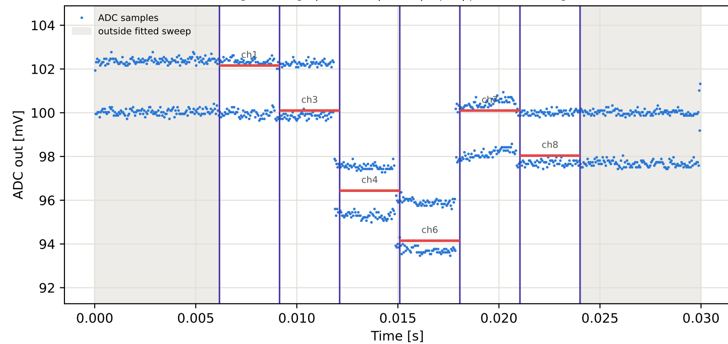
Tag10 &lt;- Tag9 | 965 MHz | run 0 | rep 1 | phase -145.38 deg
