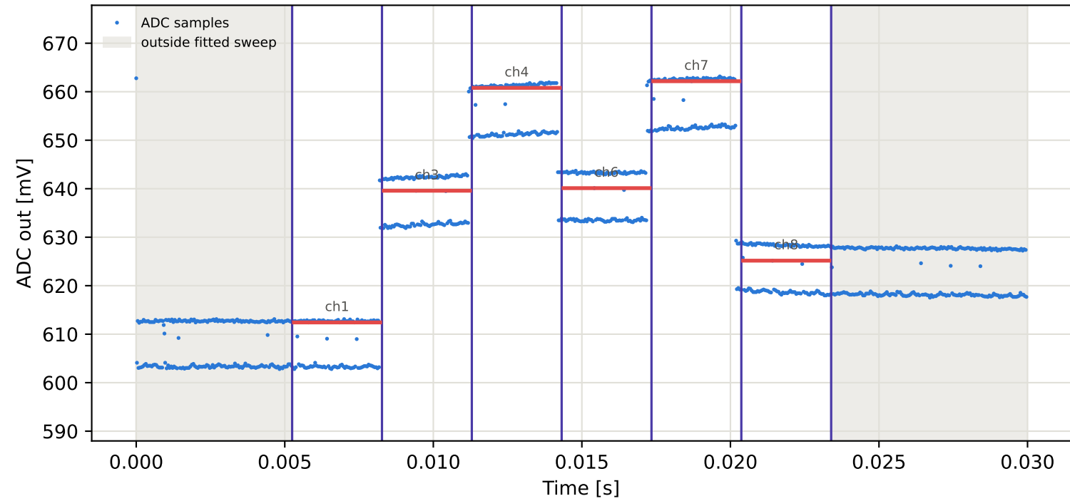
Tag8 &lt;- Tag6 | 825 MHz | run 0 | rep 1 | phase 89.44 deg
