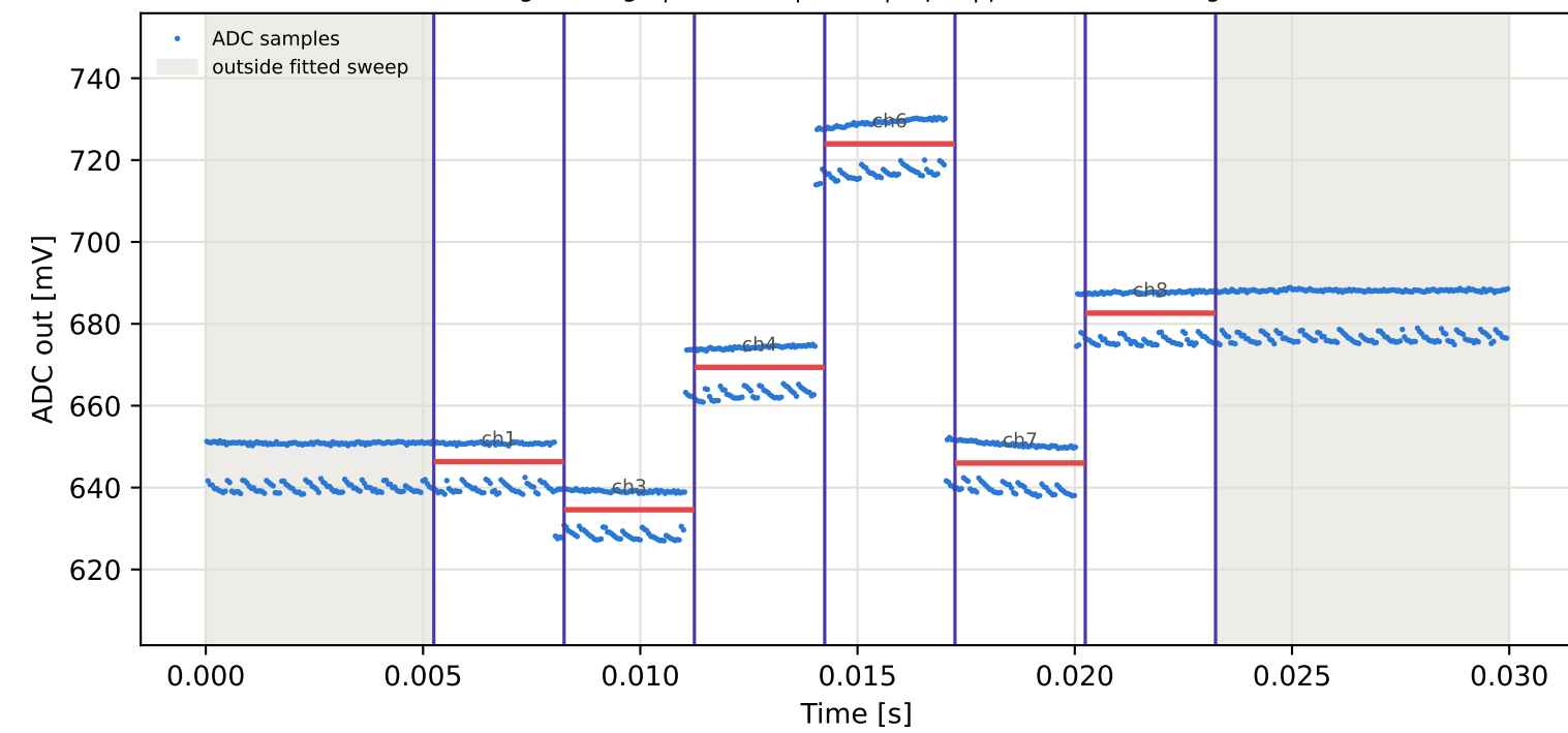
Tag4 &lt;- Tag9 | 965 MHz | run 0 | rep 1 | phase -166.57 deg
