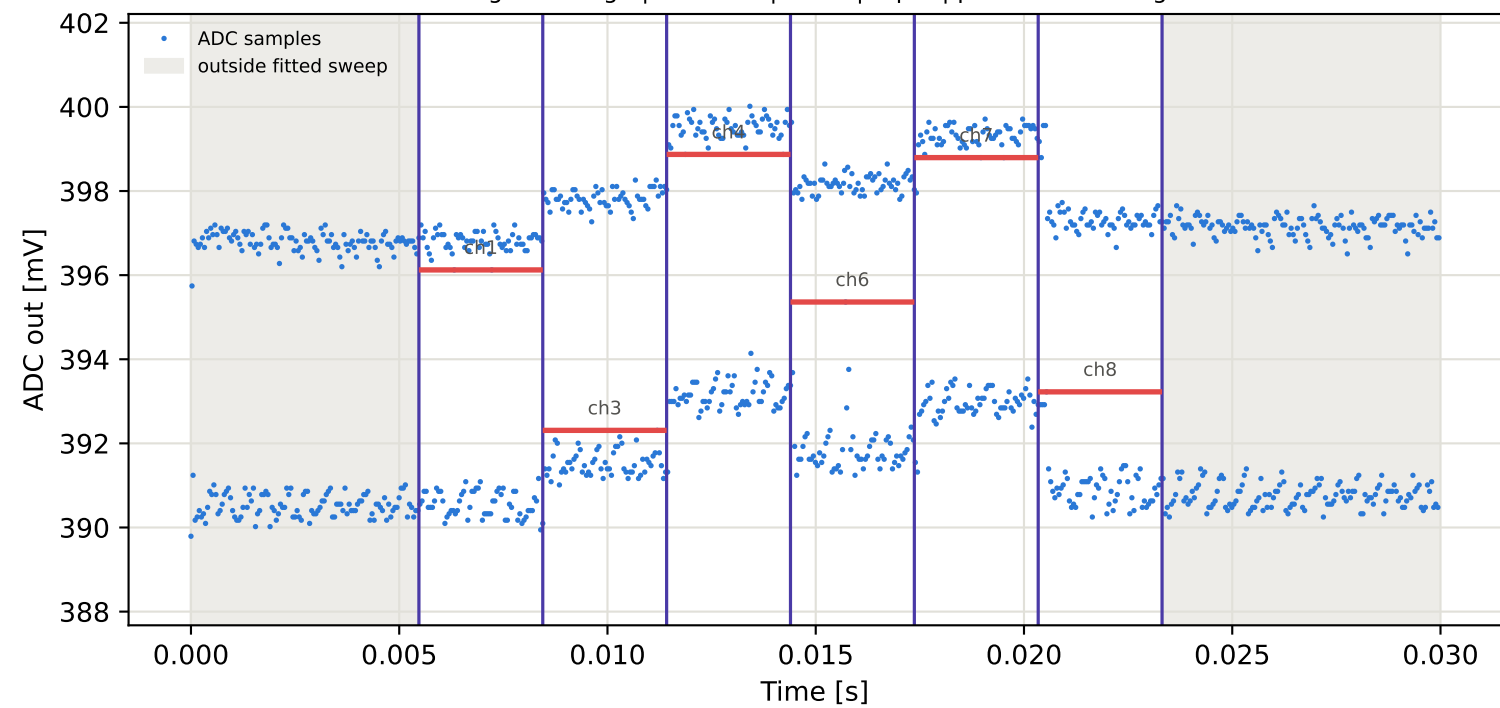
Tag15 &lt;- Tag9 | 805 MHz | run 0 | rep 1 | phase 117.46 deg
