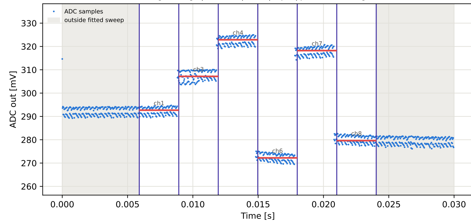
Tag3 &lt;- Tag6 | 995 MHz | run 0 | rep 1 | phase 128.52 deg
