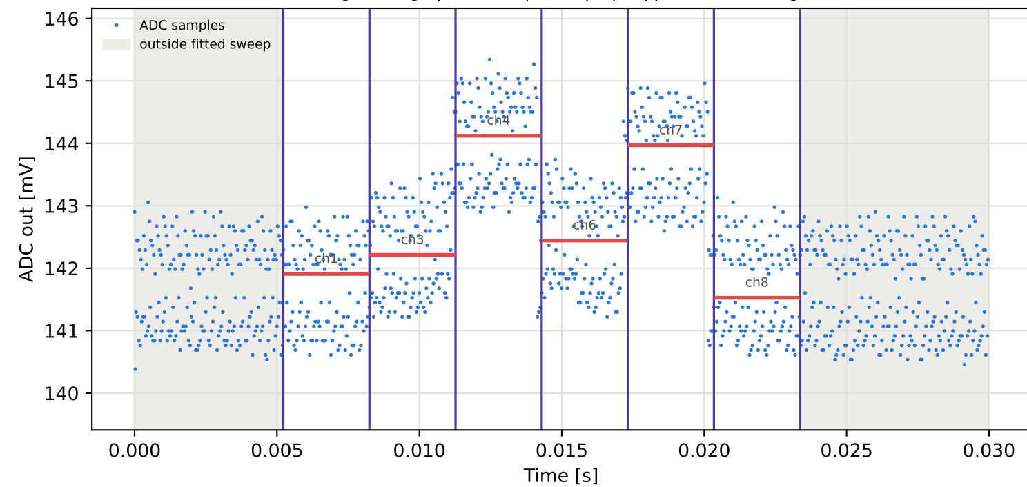
Tag3 &lt;- Tag15 | 785 MHz | run 0 | rep 1 | phase -143.89 deg
