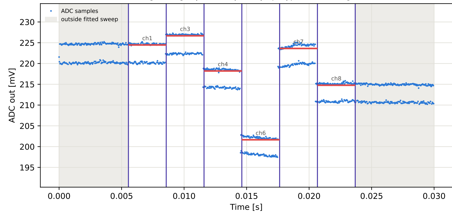
Tag5 &lt;- Tag2 | 975 MHz | run 0 | rep 1 | phase 149.48 deg
