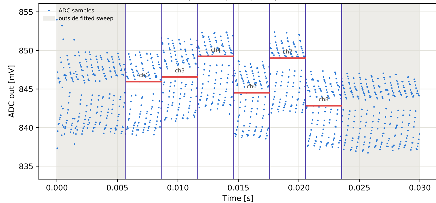
Tag16 &lt;- Tag5 | 915 MHz | run 0 | rep 1 | phase 125.38 deg
