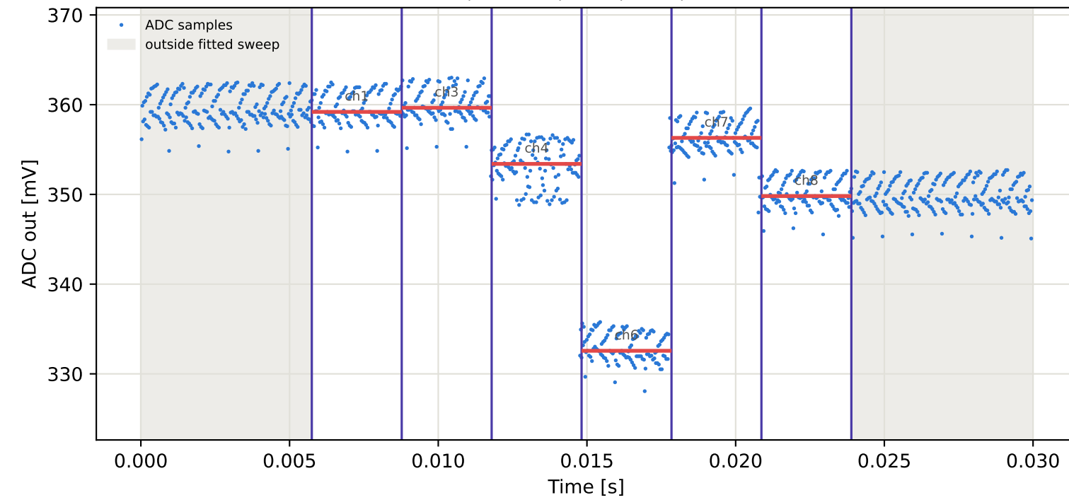
Tag10 &lt;- Tag4 | 925 MHz | run 0 | rep 1 | phase 16.67 deg
