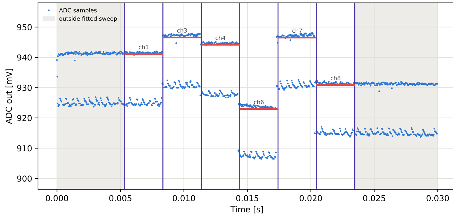
Tag8 &lt;- Tag15 | 975 MHz | run 0 | rep 1 | phase -91.87 deg
