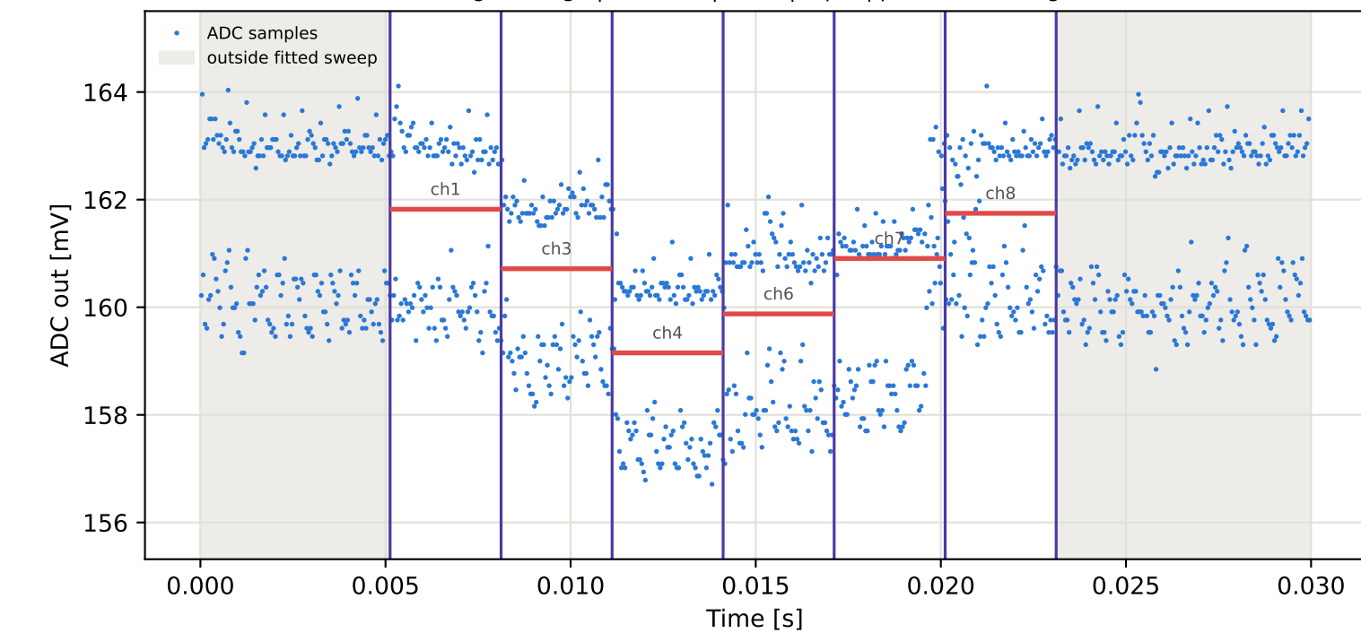
Tag2 &lt;- Tag7 | 935 MHz | run 0 | rep 1 | phase 72.78 deg
