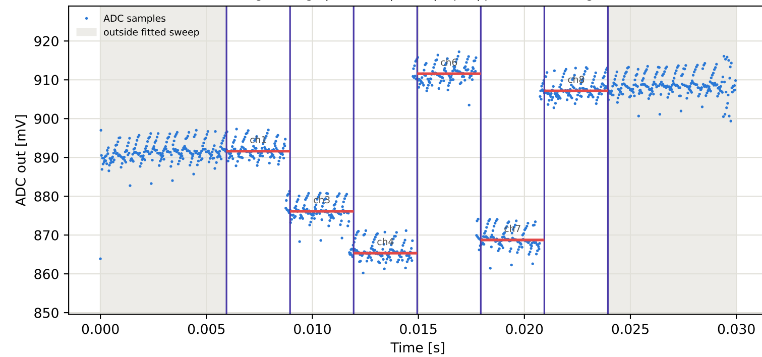
Tag9 &lt;- Tag10 | 955 MHz | run 0 | rep 1 | phase -112.34 deg
