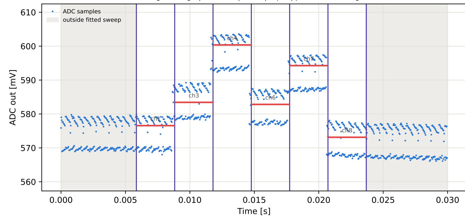
Tag6 &lt;- Tag1 | 945 MHz | run 0 | rep 1 | phase -92.53 deg
