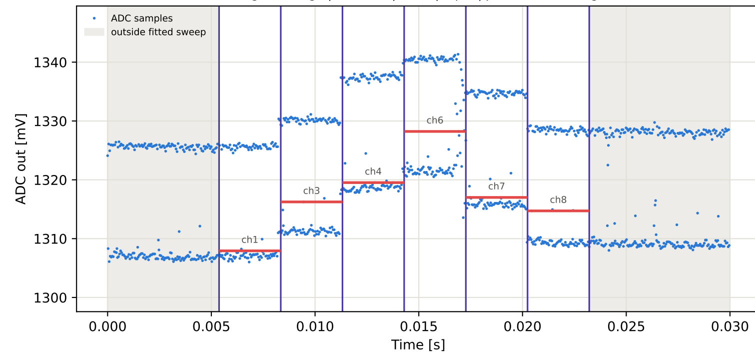
Tag16 &lt;- Tag4 | 895 MHz | run 0 | rep 1 | phase -121.46 deg
