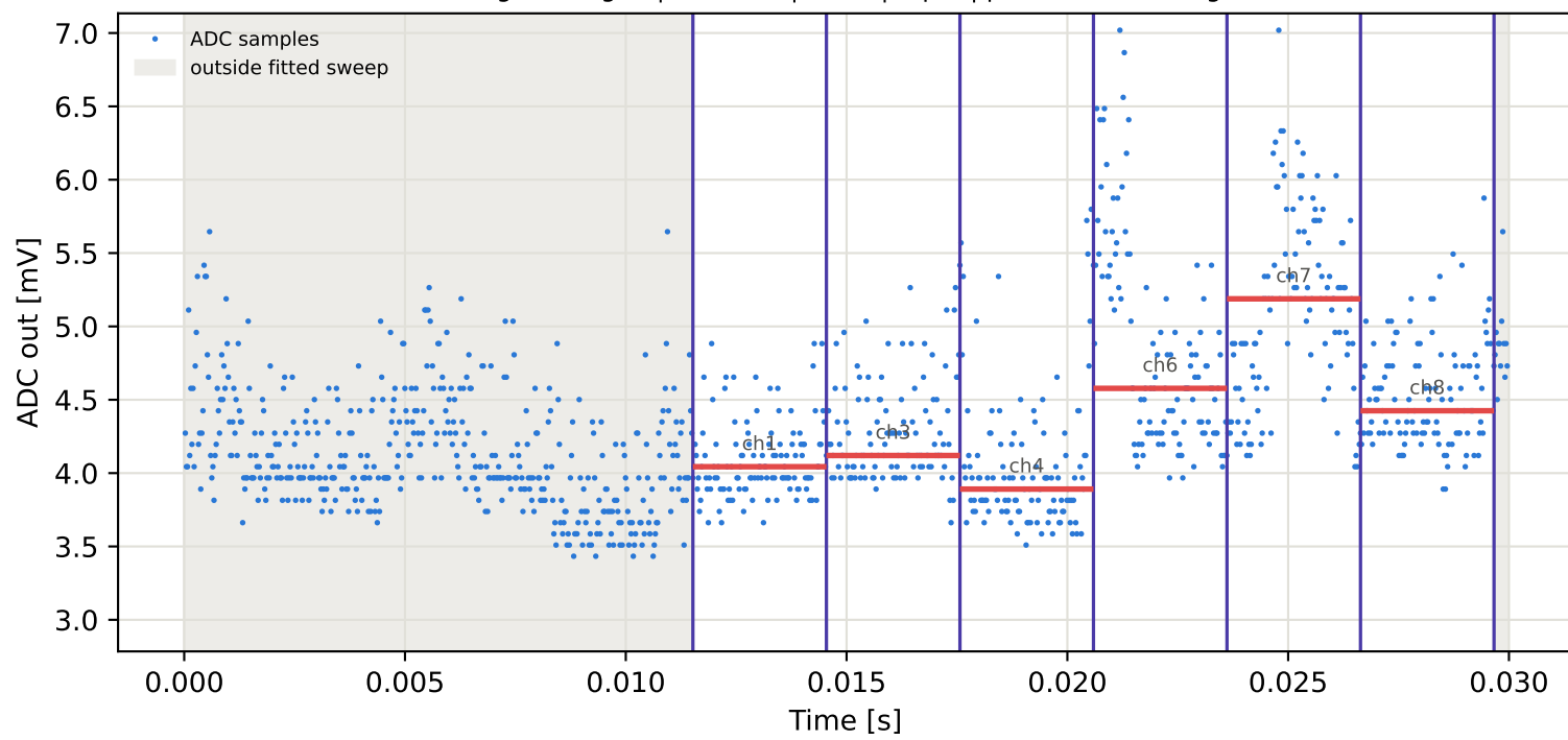
Tag2 &lt;- Tag16 | 785 MHz | run 0 | rep 1 | phase -113.16 deg
