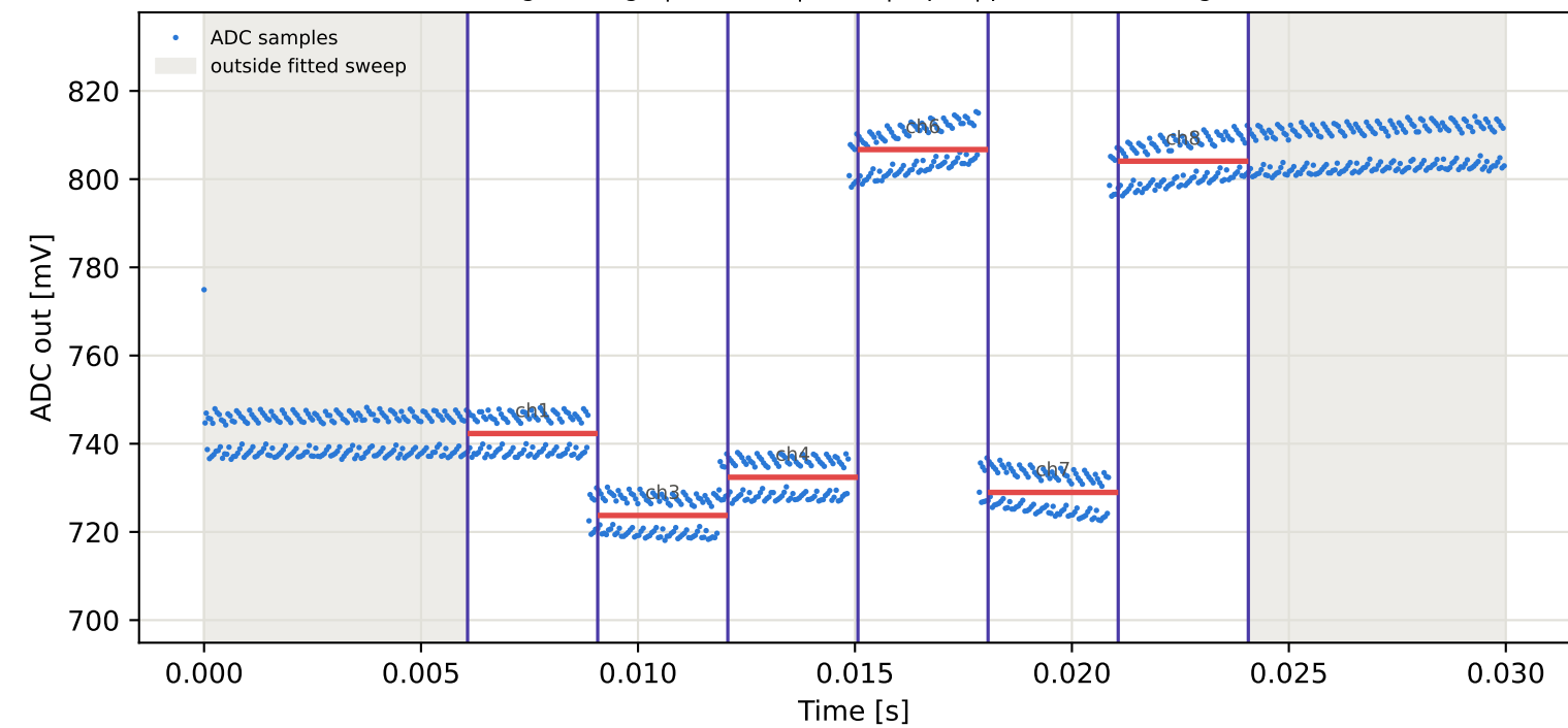
Tag3 &lt;- Tag7 | 895 MHz | run 0 | rep 1 | phase 94.06 deg
