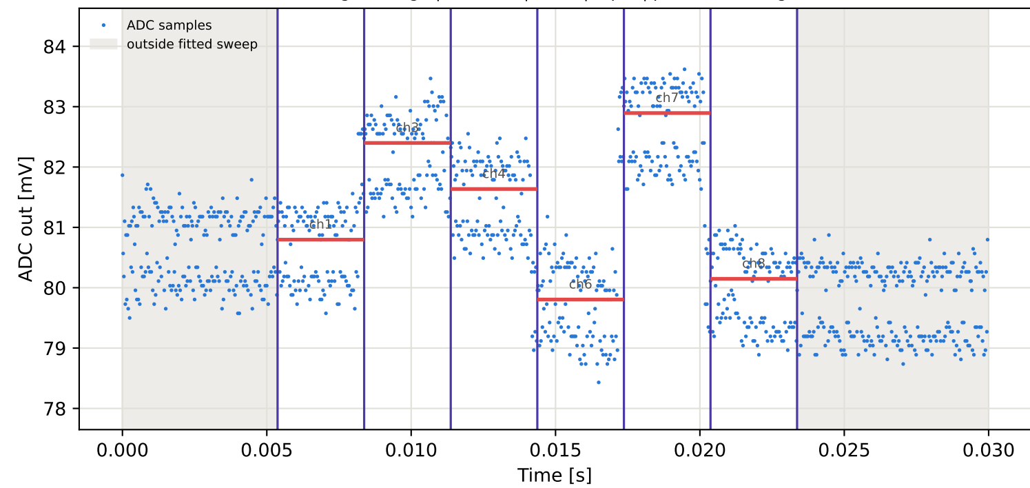
Tag9 &lt;- Tag15 | 785 MHz | run 0 | rep 1 | phase 93.70 deg
