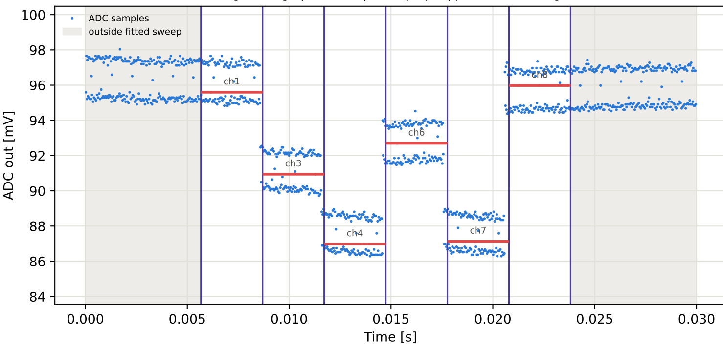
Tag1 &lt;- Tag9 | 825 MHz | run 0 | rep 1 | phase 108.15 deg
