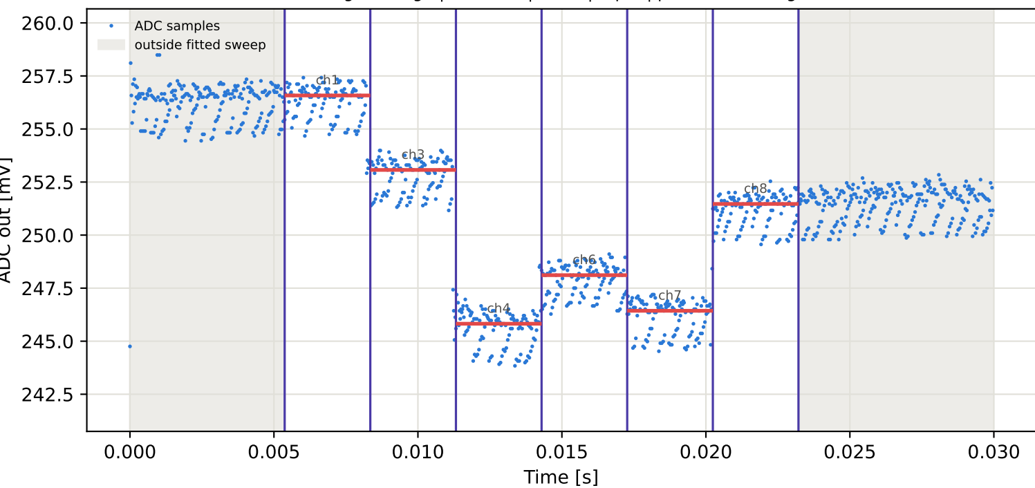
Tag6 &lt;- Tag4 | 825 MHz | run 0 | rep 1 | phase 73.44 deg
