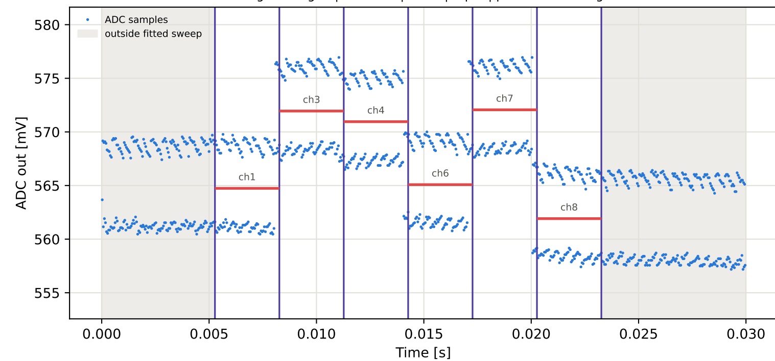
Tag6 &lt;- Tag2 | 865 MHz | run 0 | rep 1 | phase -3.40 deg
