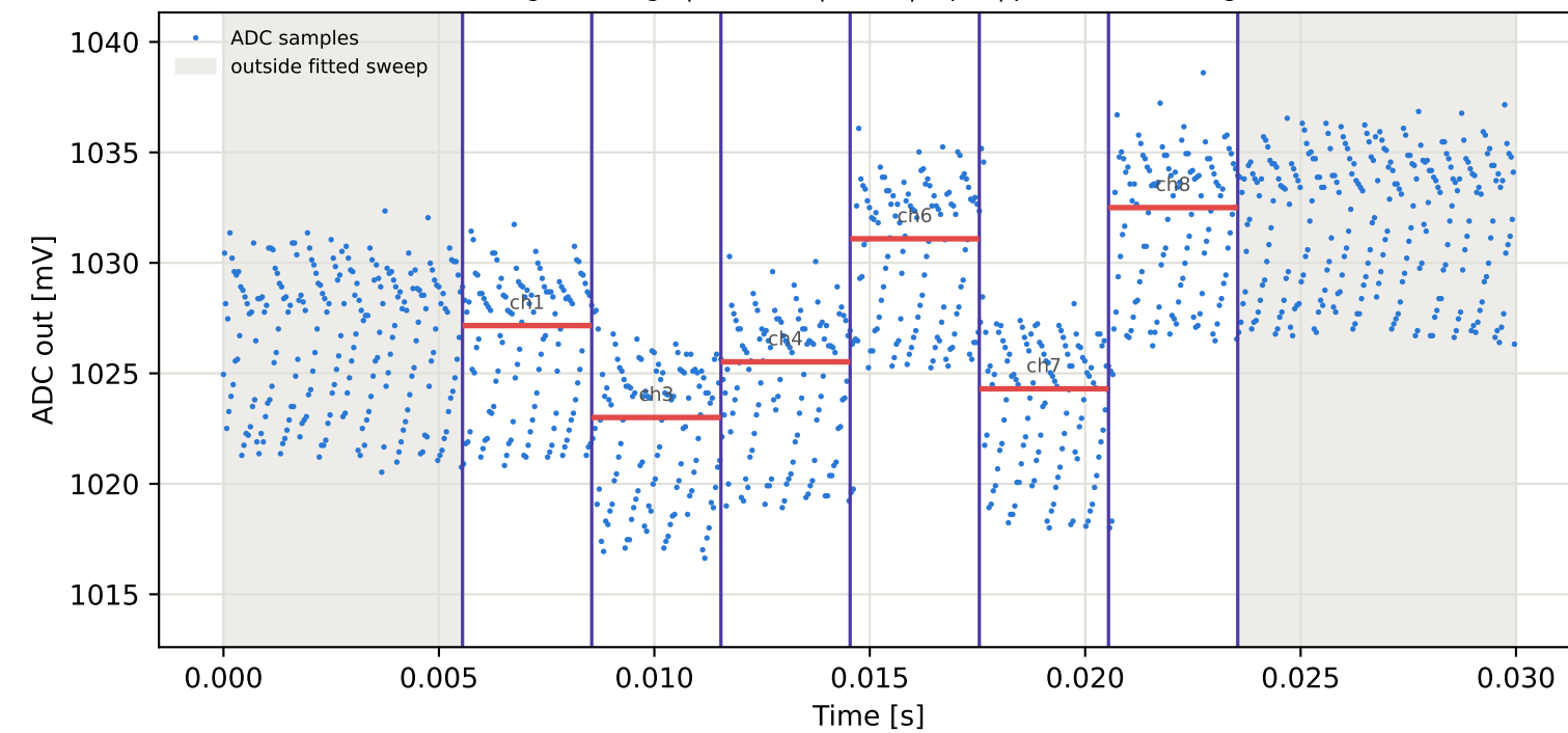
Tag15 &lt;- Tag9 | 875 MHz | run 0 | rep 1 | phase -41.23 deg
