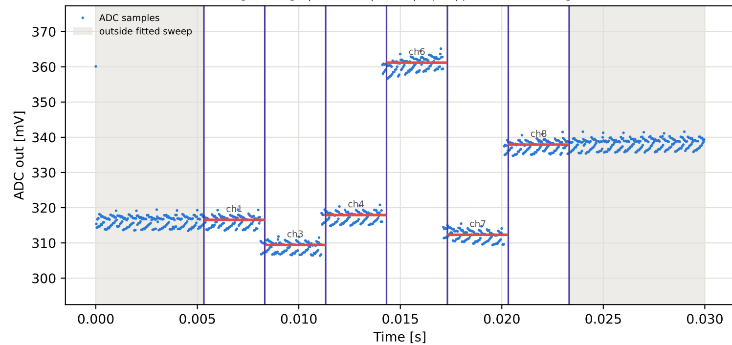
Tag8 &lt;- Tag10 | 935 MHz | run 0 | rep 1 | phase -9.28 deg
