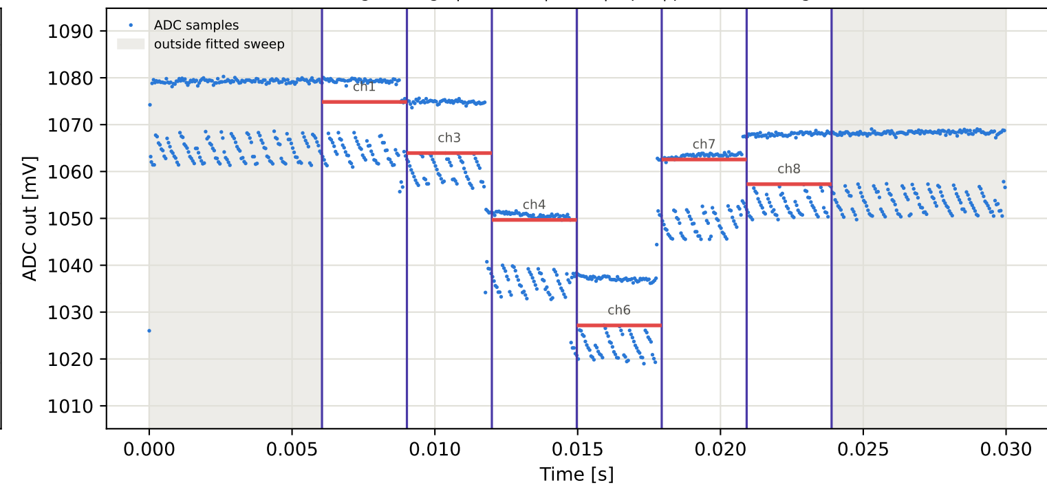
Tag4 &lt;- Tag8 | 945 MHz | run 0 | rep 1 | phase -78.65 deg
