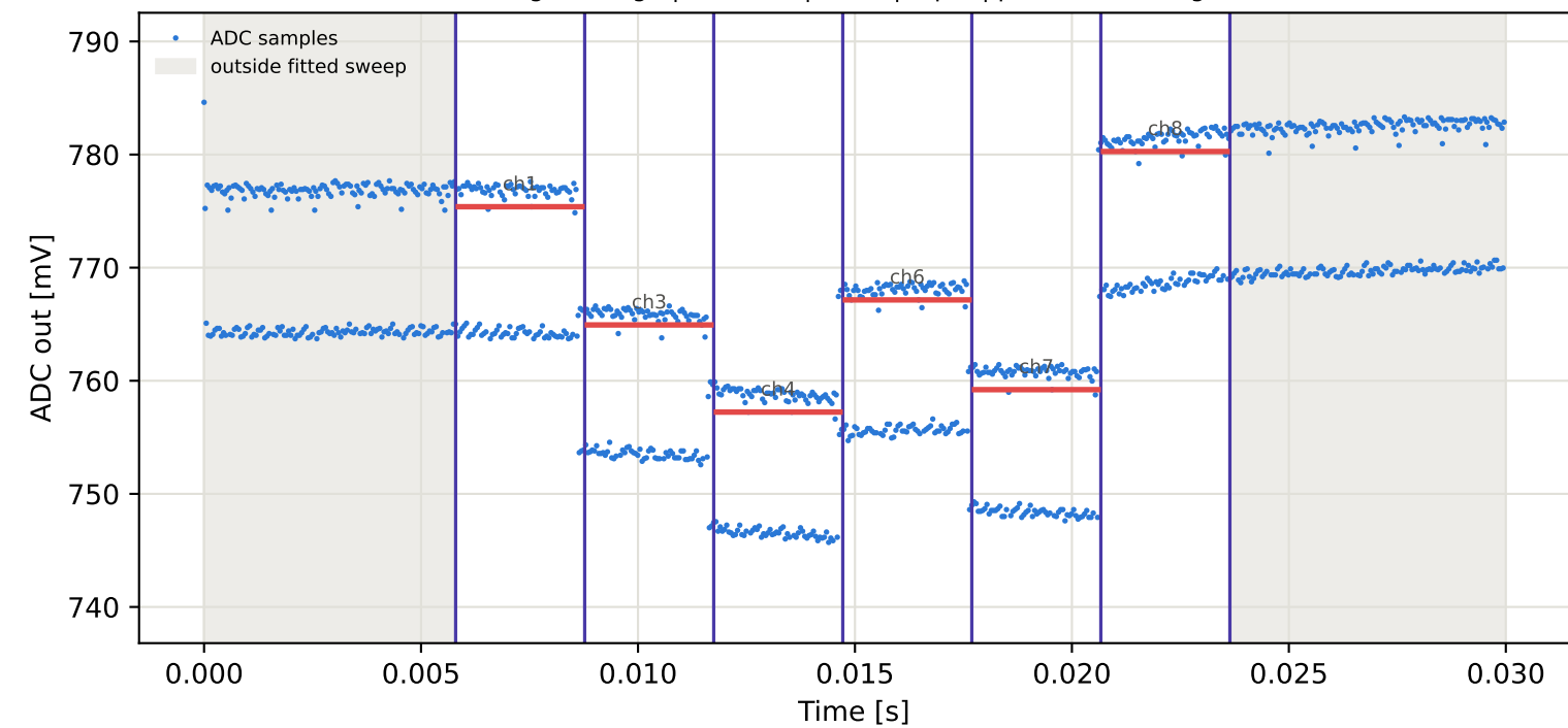
Tag3 &lt;- Tag9 | 895 MHz | run 0 | rep 1 | phase 12.34 deg
