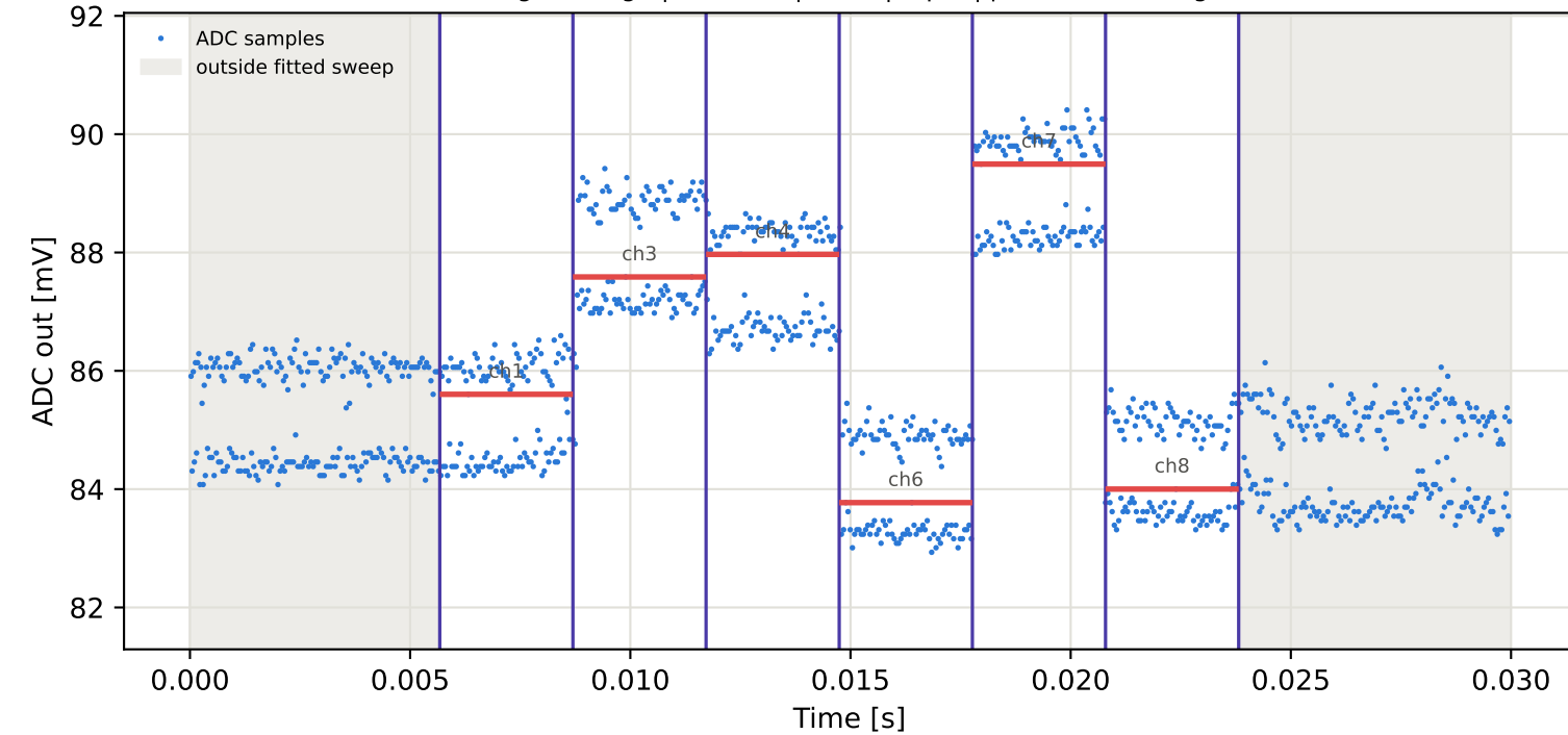
Tag9 &lt;- Tag7 | 775 MHz | run 0 | rep 1 | phase 174.25 deg
