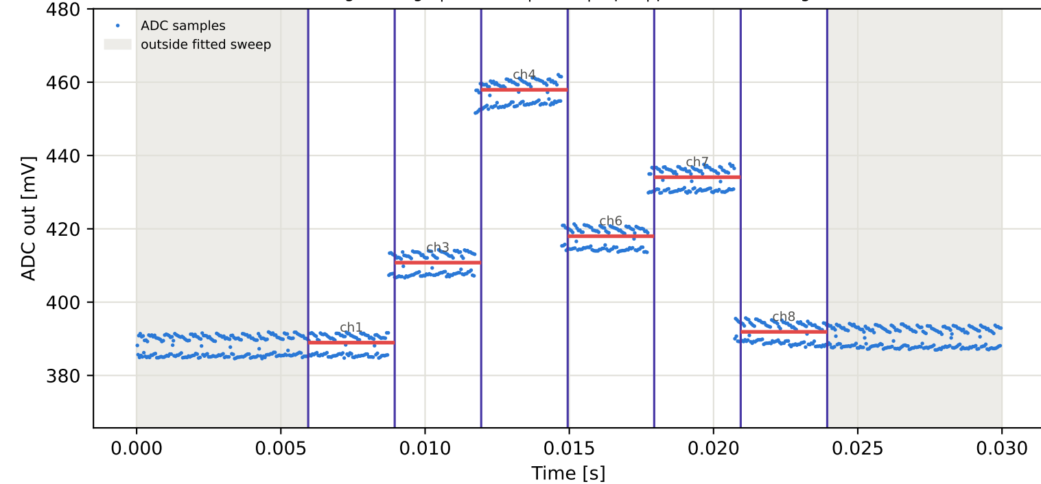
Tag4 &lt;- Tag9 | 985 MHz | run 0 | rep 1 | phase -106.62 deg
