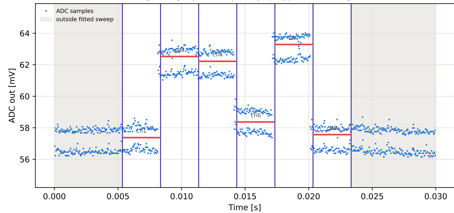
Tag1 &lt;- Tag2 | 835 MHz | run 0 | rep 1 | phase 145.36 deg
