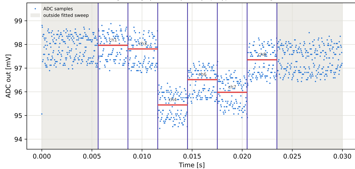
Tag5 &lt;- Tag8 | 775 MHz | run 0 | rep 1 | phase -57.35 deg
