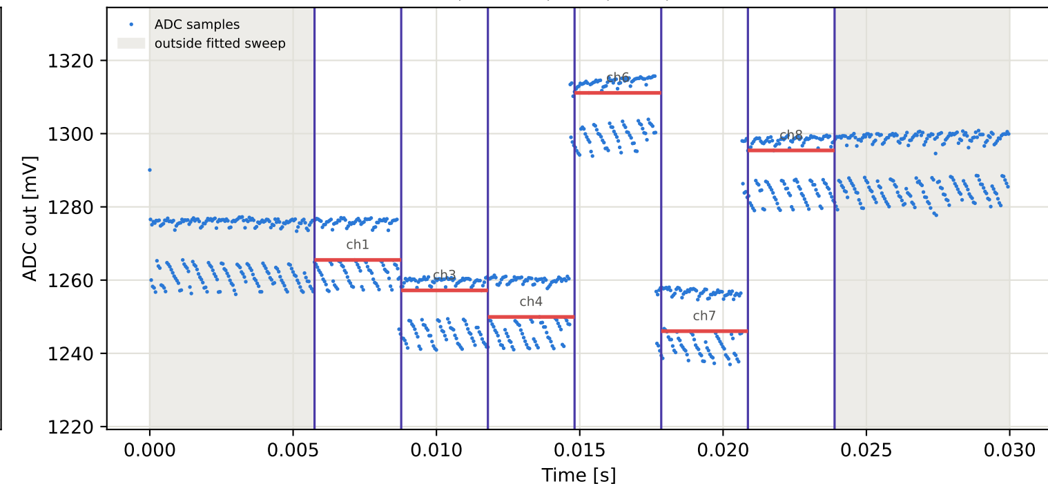
Tag16 &lt;- Tag7 | 955 MHz | run 0 | rep 1 | phase 158.22 deg
