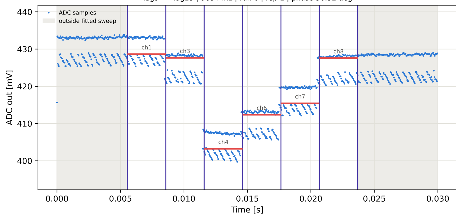
Tag9 &lt;- Tag2 | 985 MHz | run 0 | rep 1 | phase -105.96 deg
