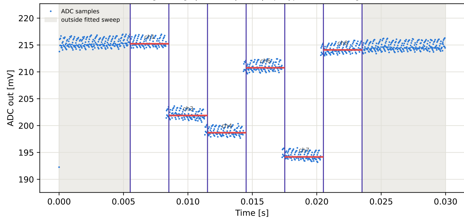
Tag3 &lt;- Tag6 | 805 MHz | run 0 | rep 1 | phase 10.29 deg
