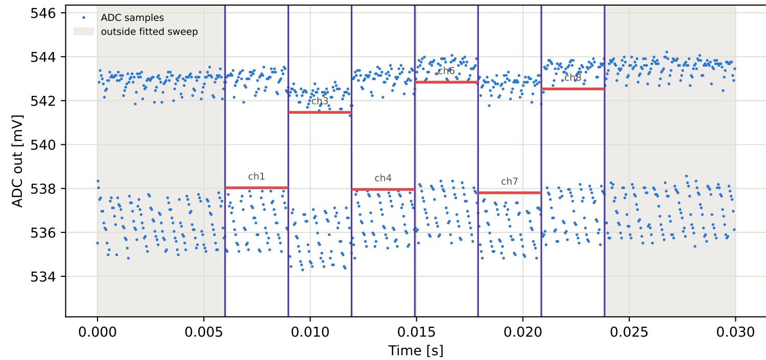
Tag4 &lt;- Tag15 | 845 MHz | run 0 | rep 1 | phase -0.75 deg
