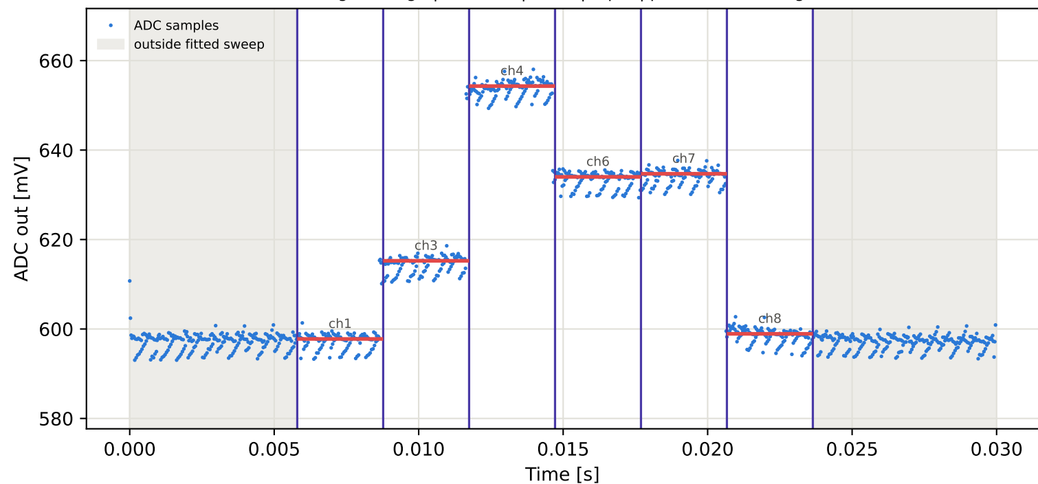
Tag7 &lt;- Tag6 | 945 MHz | run 0 | rep 1 | phase 105.79 deg
