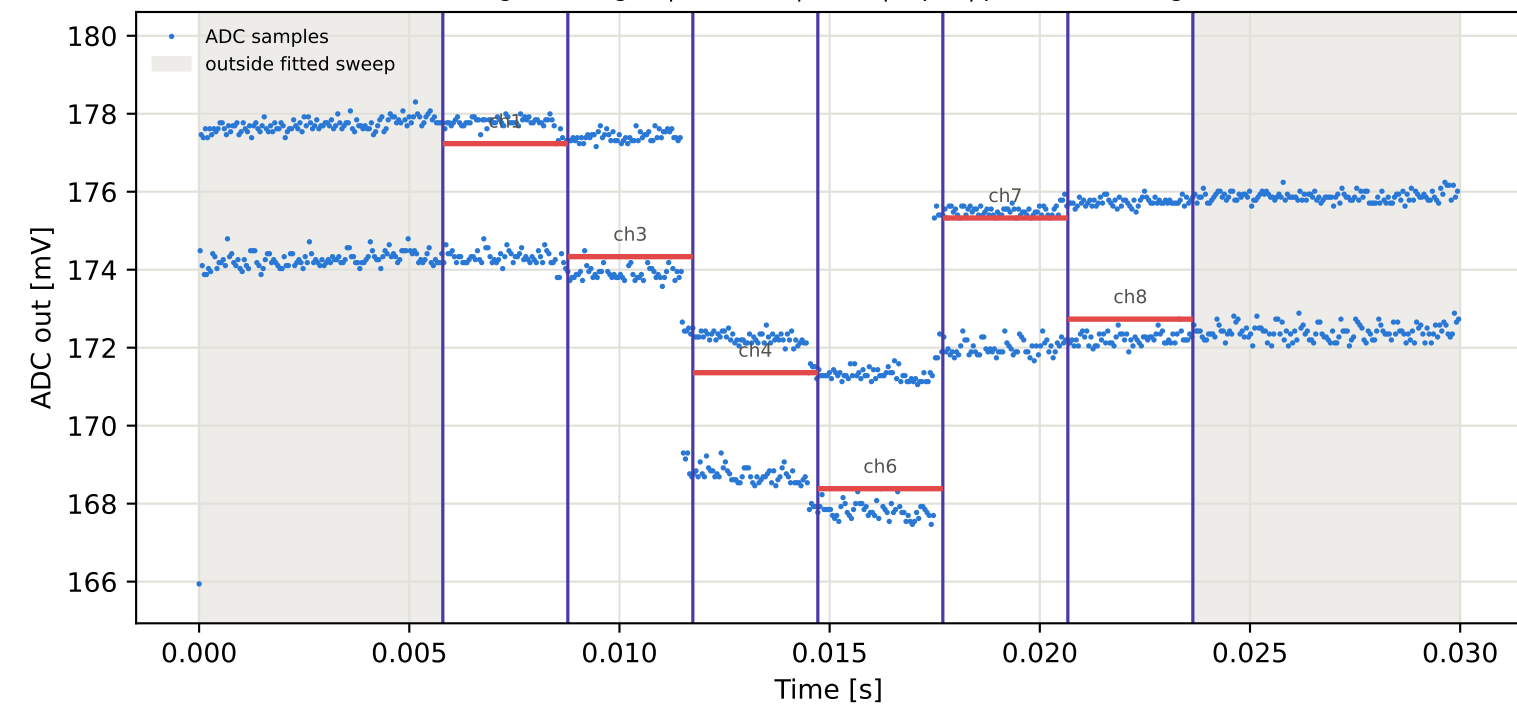
Tag10 &lt;- Tag2 | 985 MHz | run 0 | rep 1 | phase -111.24 deg
