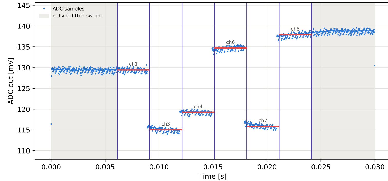
Tag1 &lt;- Tag9 | 865 MHz | run 0 | rep 1 | phase -24.46 deg
