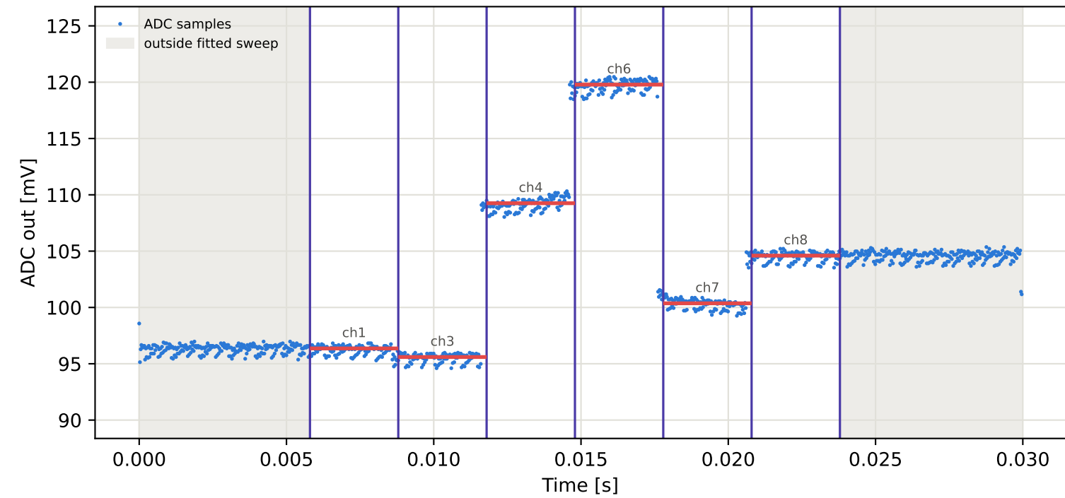
Tag10 &lt;- Tag5 | 965 MHz | run 0 | rep 1 | phase -44.93 deg
