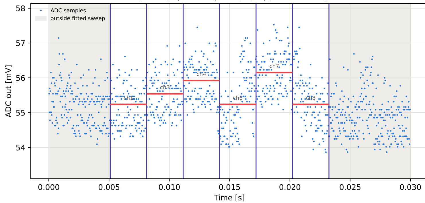
Tag3 &lt;- Tag10 | 945 MHz | run 0 | rep 1 | phase 132.19 deg
