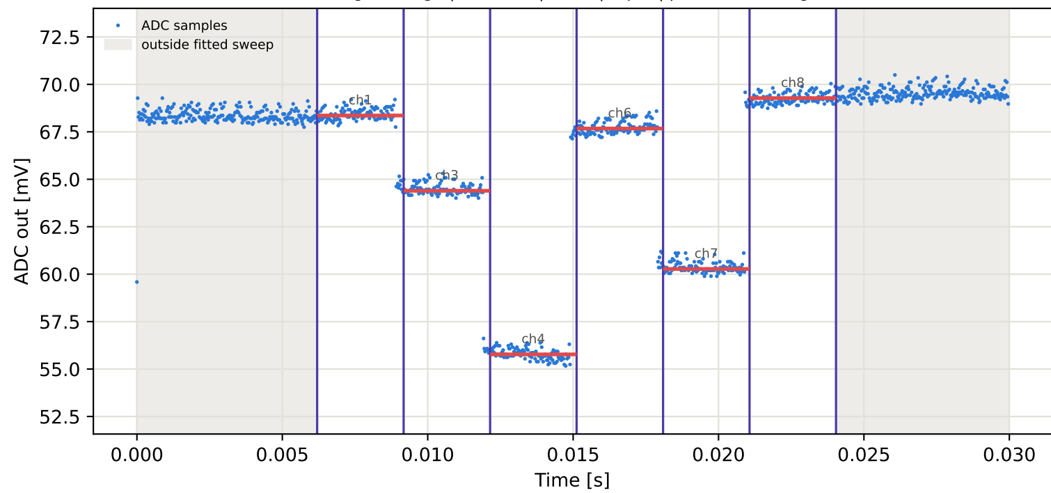
Tag7 &lt;- Tag1 | 995 MHz | run 0 | rep 1 | phase -25.14 deg
