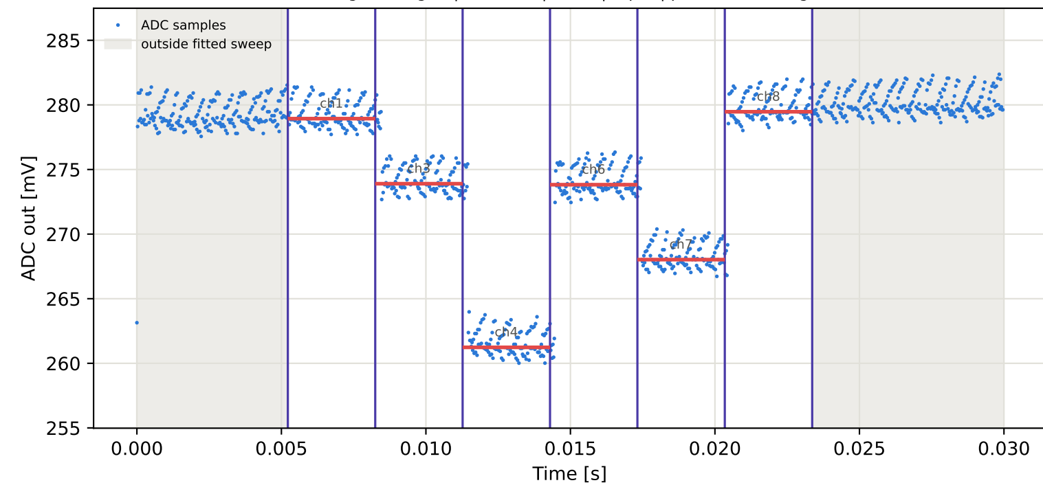
Tag6 &lt;- Tag2 | 985 MHz | run 0 | rep 1 | phase -86.59 deg
