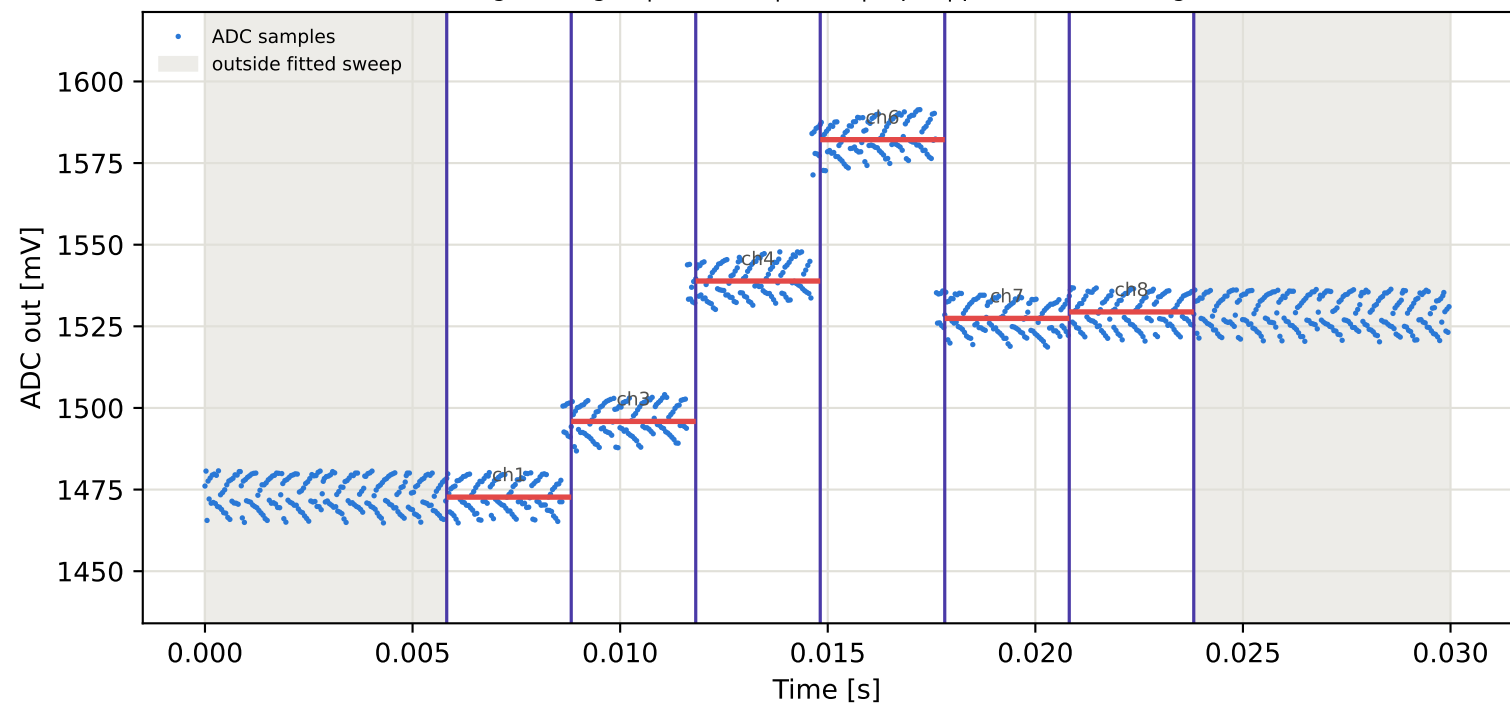
Tag5 &lt;- Tag2 | 895 MHz | run 0 | rep 1 | phase 97.26 deg
