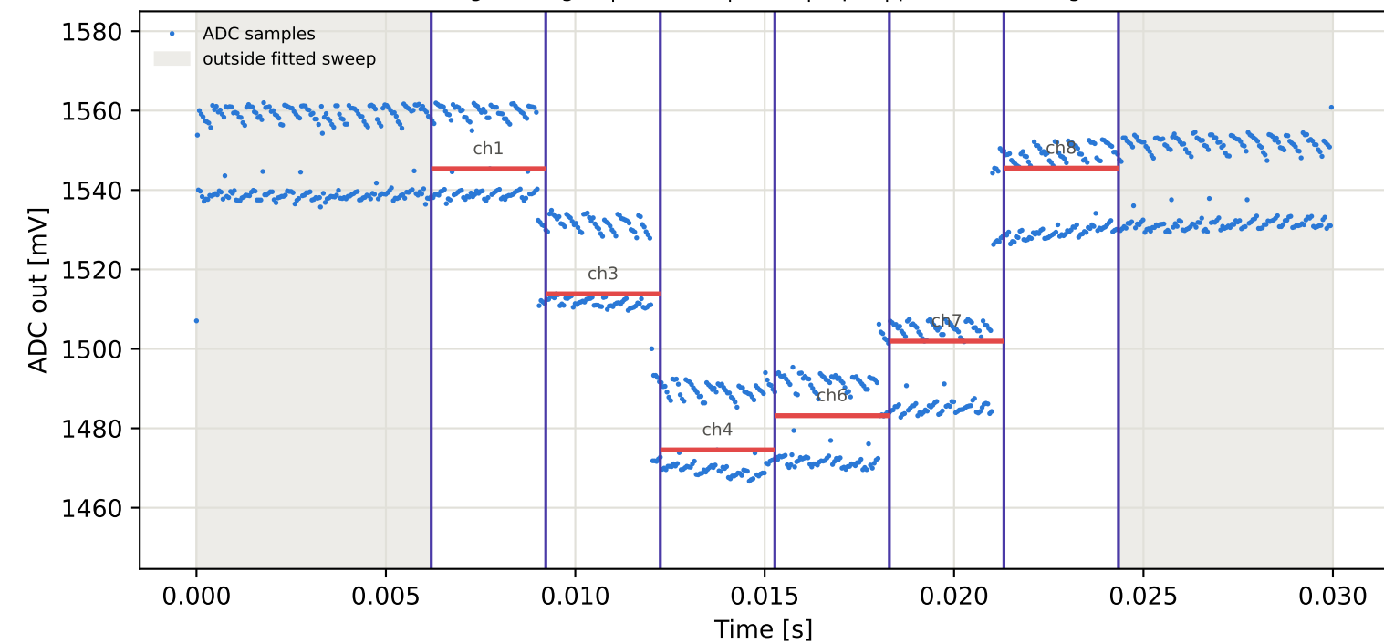
Tag4 &lt;- Tag2 | 925 MHz | run 0 | rep 1 | phase 100.38 deg
