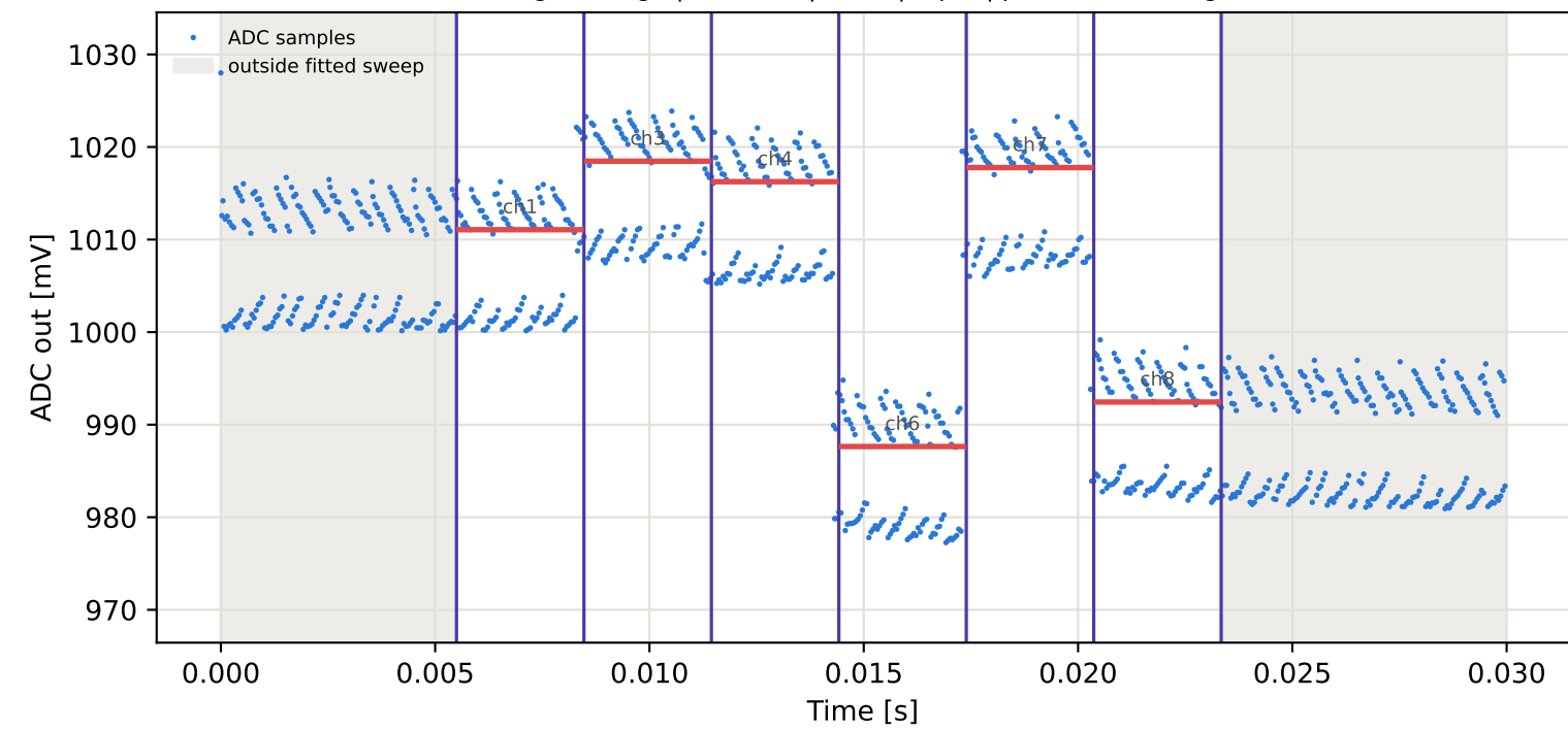
Tag5 &lt;- Tag9 | 905 MHz | run 0 | rep 1 | phase 56.15 deg
