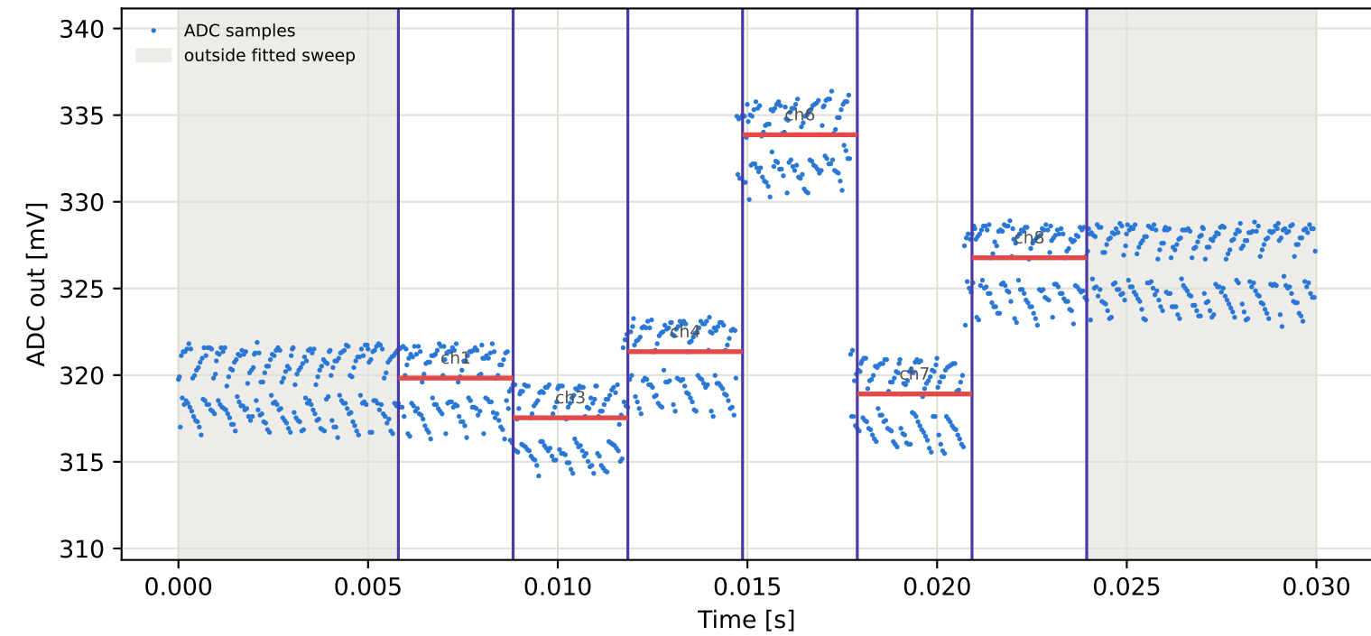
Tag7 &lt;- Tag15 | 935 MHz | run 0 | rep 1 | phase -59.11 deg
