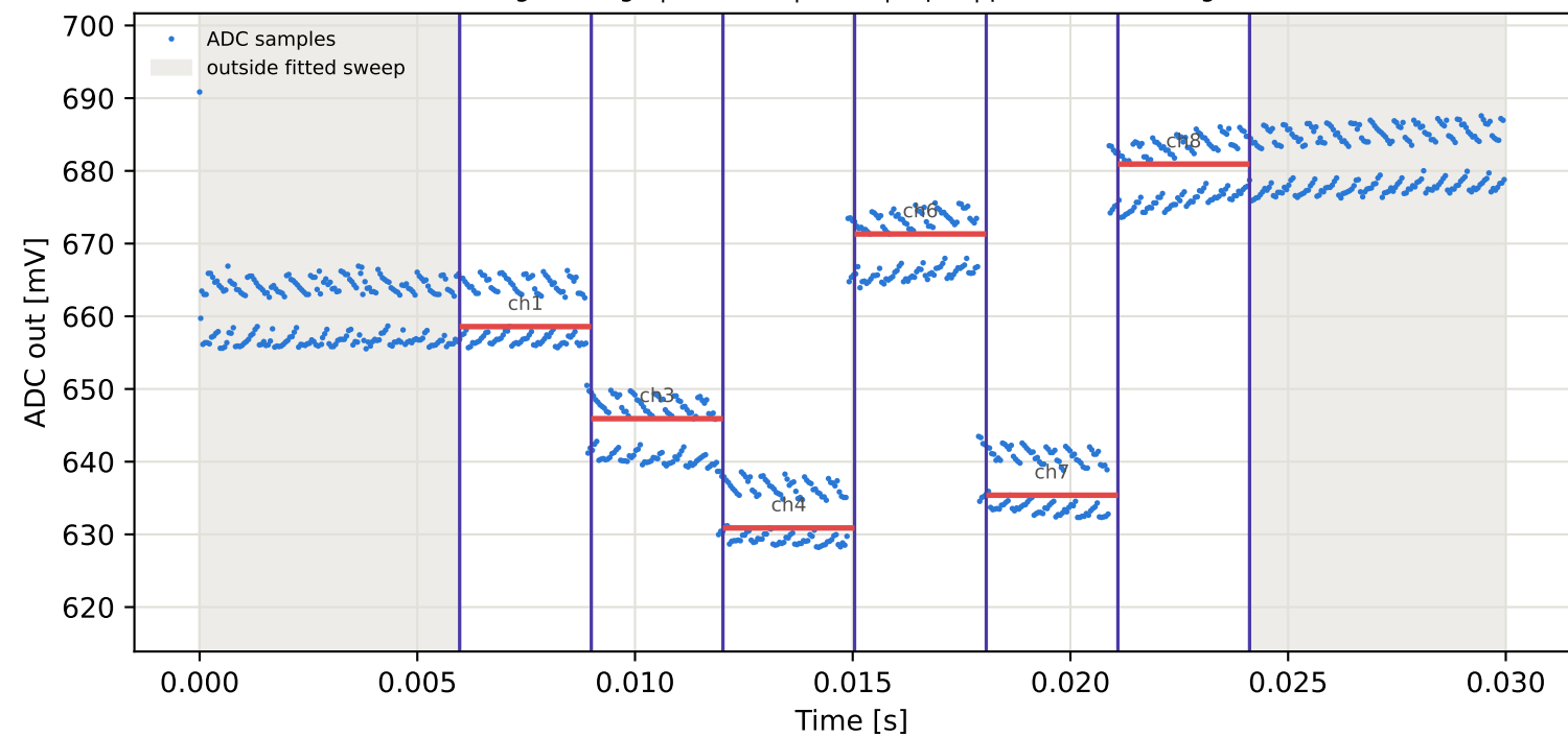
Tag7 &lt;- Tag5 | 915 MHz | run 0 | rep 1 | phase 126.62 deg
