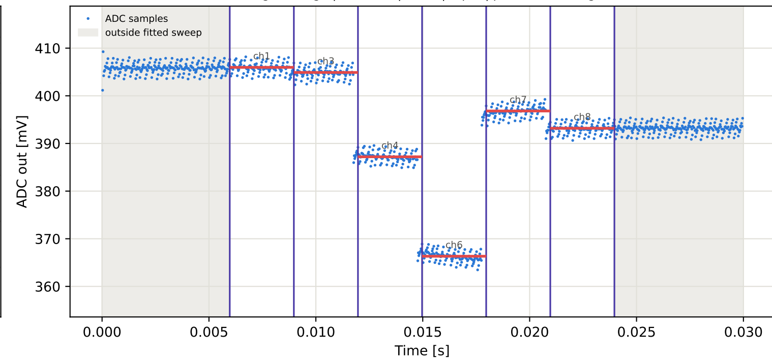
Tag1 &lt;- Tag8 | 945 MHz | run 0 | rep 1 | phase -55.99 deg
