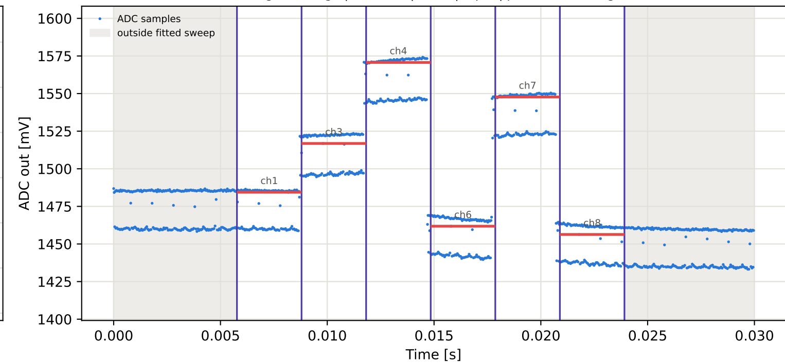
Tag16 &lt;- Tag1 | 965 MHz | run 0 | rep 1 | phase 80.30 deg
