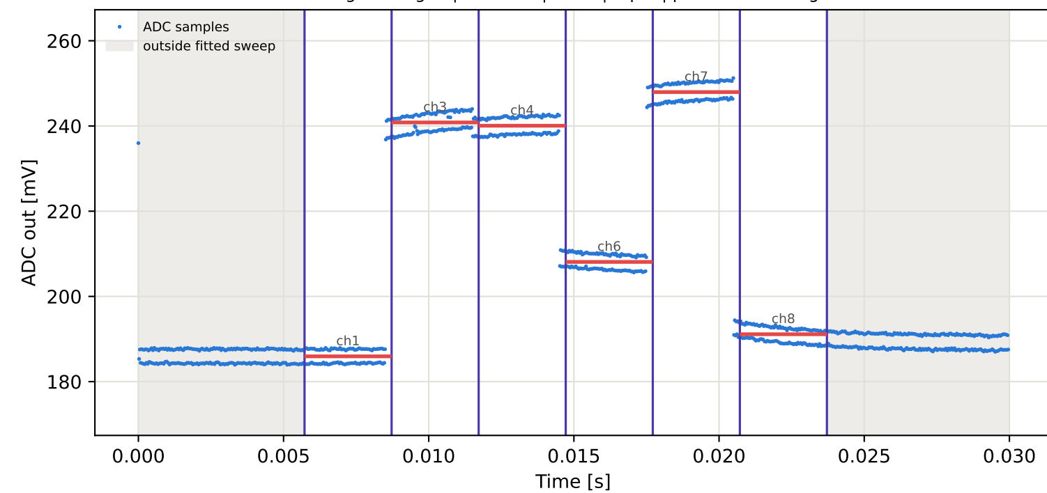
Tag7 &lt;- Tag3 | 825 MHz | run 0 | rep 1 | phase 16.90 deg
