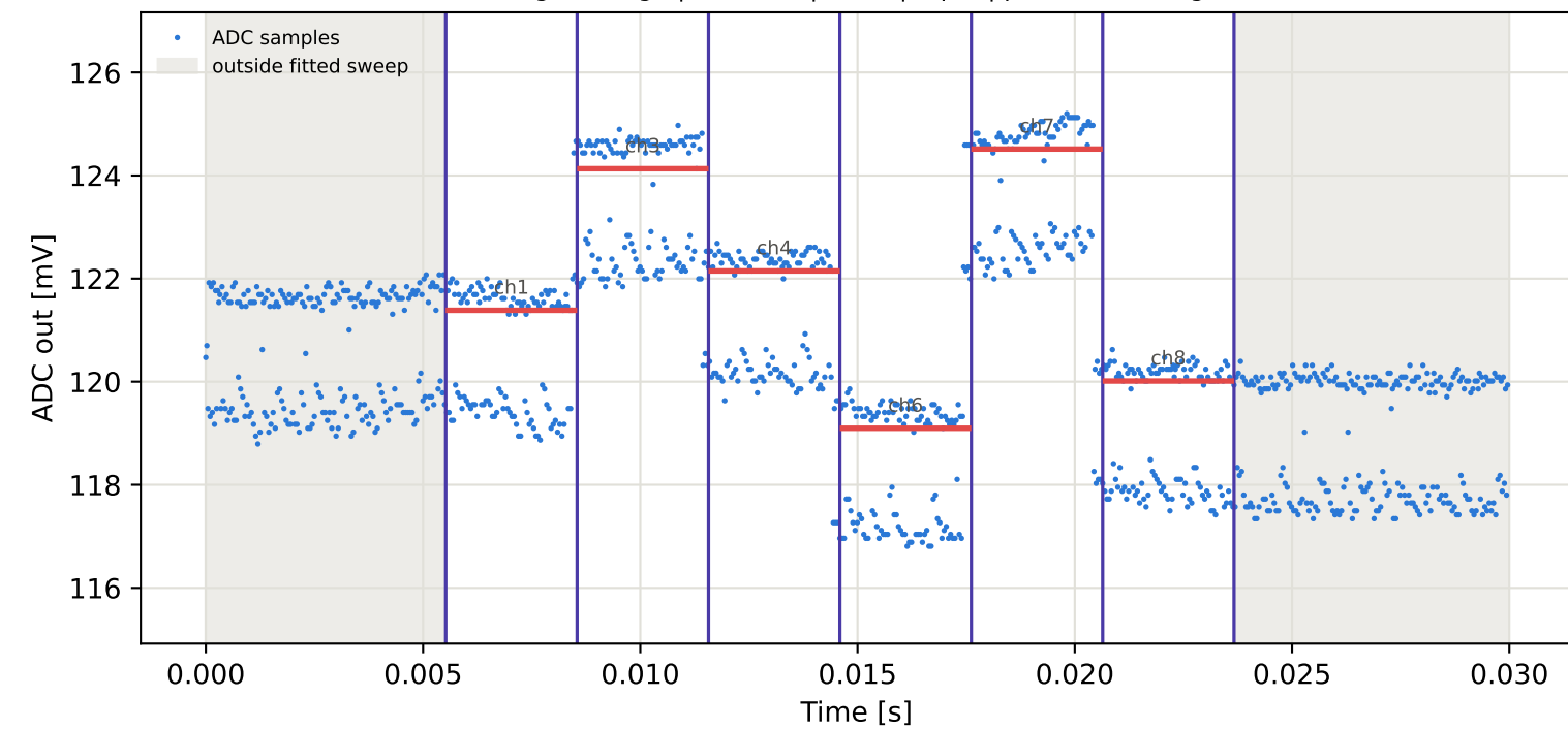
Tag4 &lt;- Tag15 | 805 MHz | run 0 | rep 1 | phase 41.95 deg
