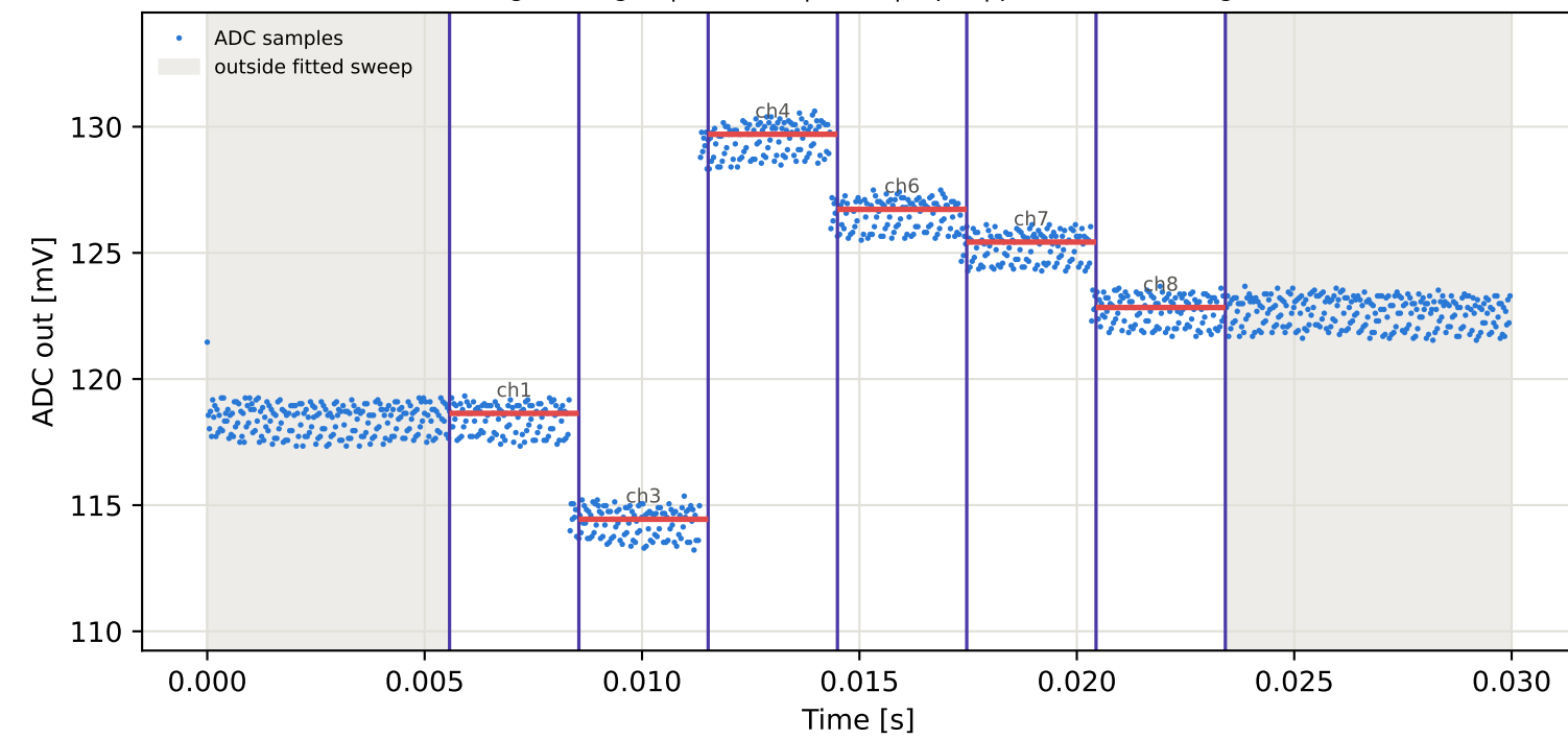
Tag1 &lt;- Tag16 | 785 MHz | run 0 | rep 1 | phase 54.30 deg
