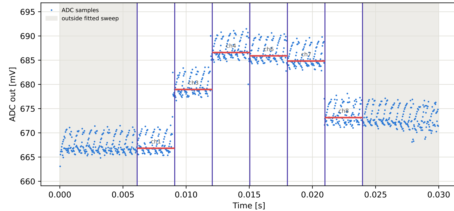
Tag9 &lt;- Tag7 | 875 MHz | run 0 | rep 1 | phase -7.57 deg
