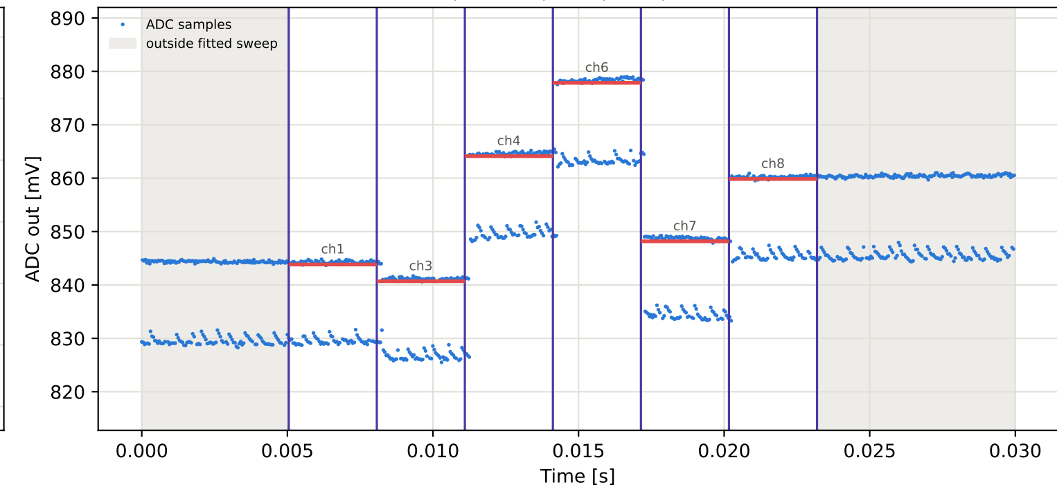
Tag16 &lt;- Tag7 | 995 MHz | run 0 | rep 1 | phase -157.74 deg
