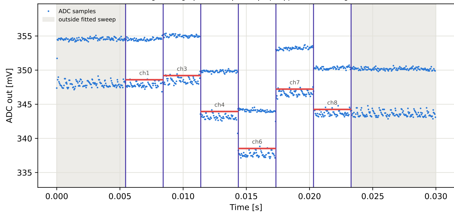
Tag5 &lt;- Tag1 | 955 MHz | run 0 | rep 1 | phase 22.44 deg
