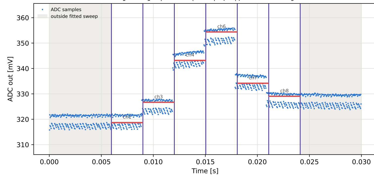
Tag1 &lt;- Tag16 | 935 MHz | run 0 | rep 1 | phase -34.59 deg
