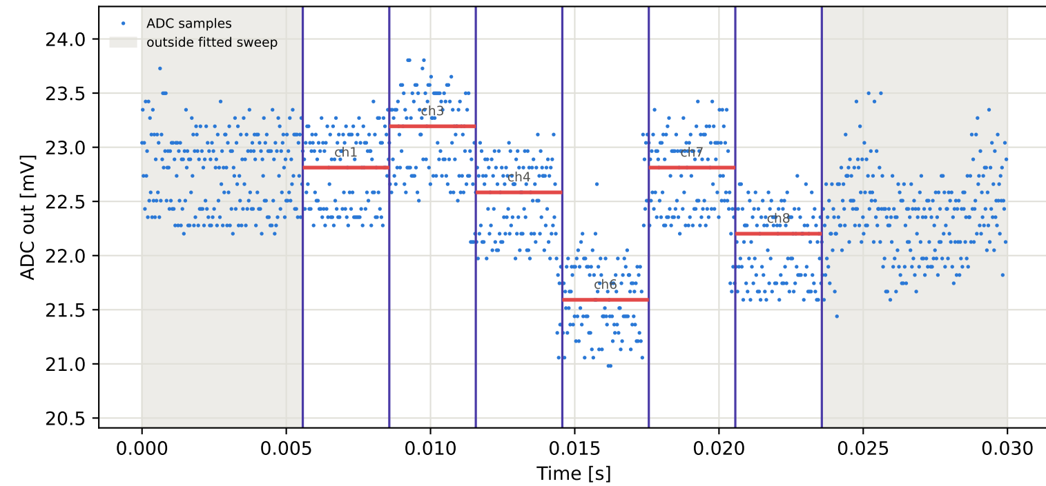
Tag5 &lt;- Tag4 | 805 MHz | run 0 | rep 1 | phase -76.14 deg
