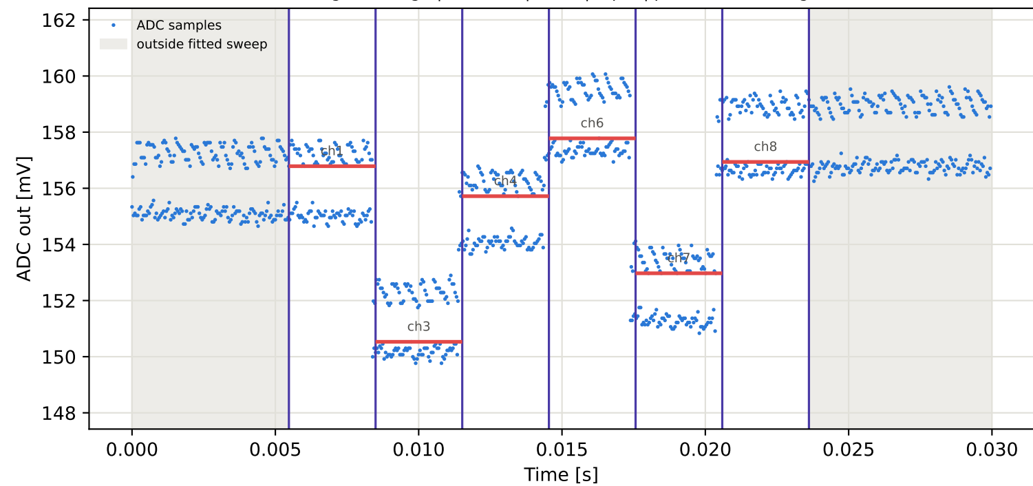
Tag16 &lt;- Tag5 | 795 MHz | run 0 | rep 1 | phase -141.12 deg
