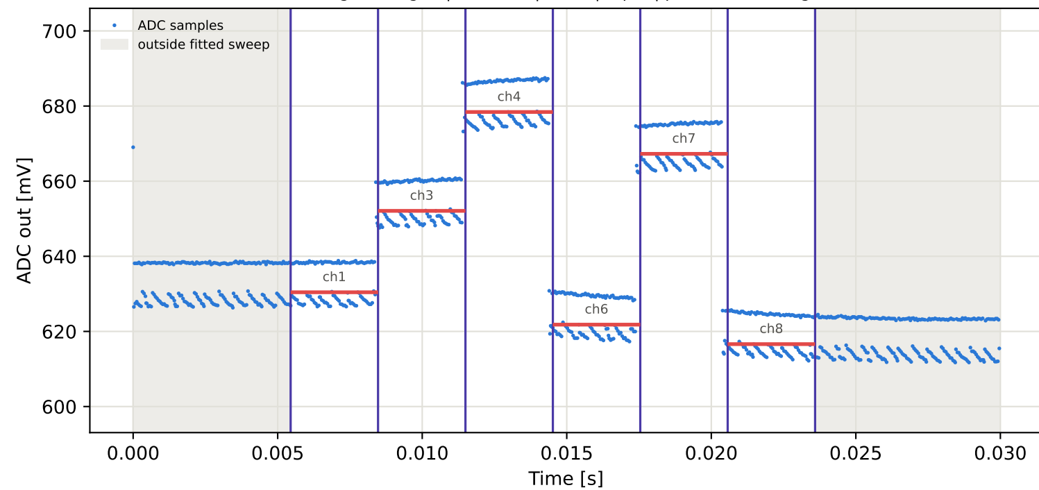
Tag6 &lt;- Tag3 | 955 MHz | run 0 | rep 1 | phase 63.37 deg
