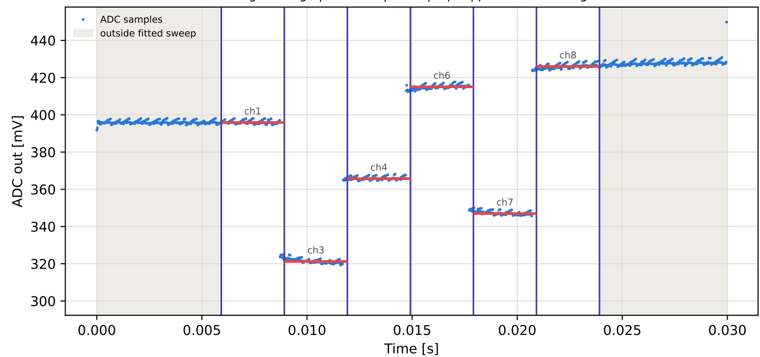
Tag9 &lt;- Tag6 | 835 MHz | run 0 | rep 1 | phase 2.26 deg
