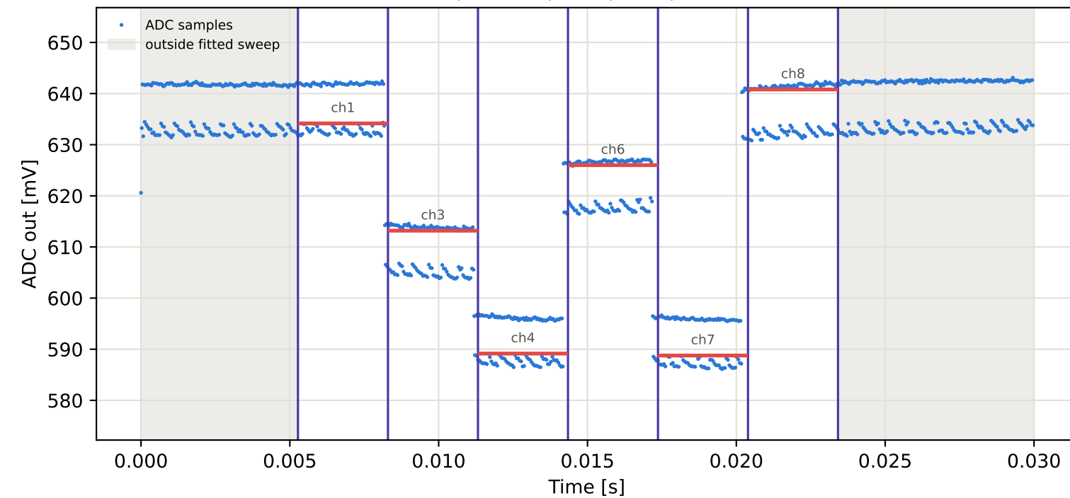
Tag4 &lt;- Tag9 | 835 MHz | run 0 | rep 1 | phase 112.54 deg
