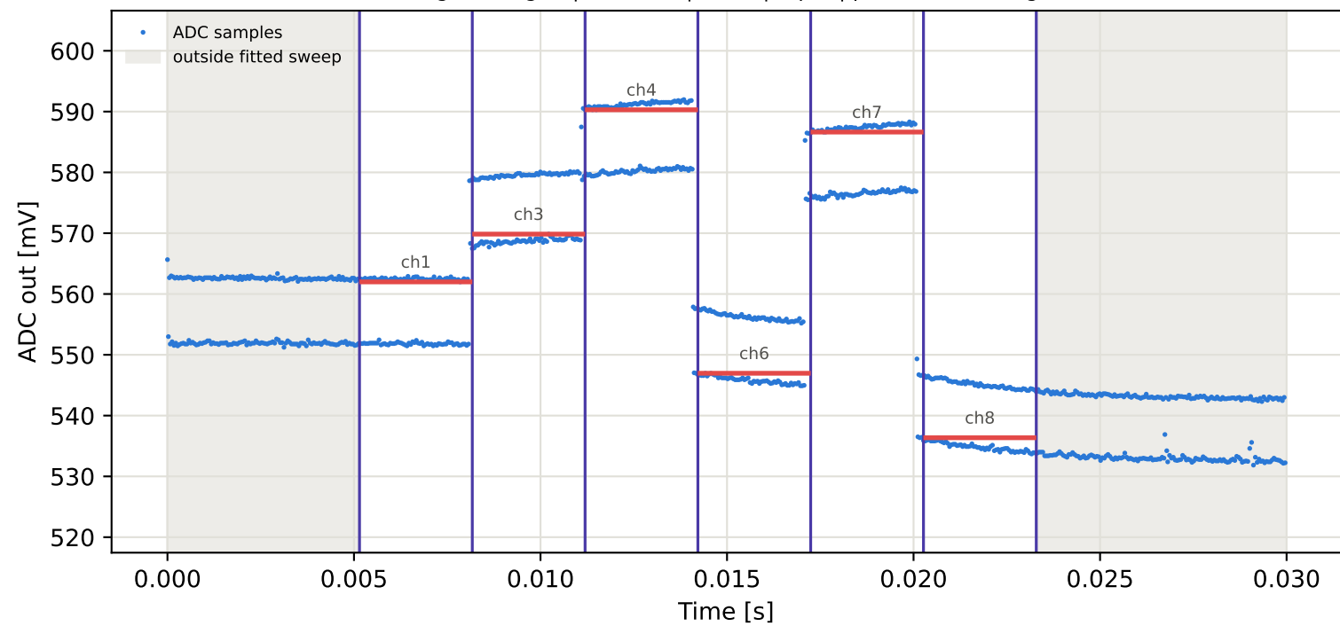
Tag6 &lt;- Tag3 | 905 MHz | run 0 | rep 1 | phase 32.39 deg
