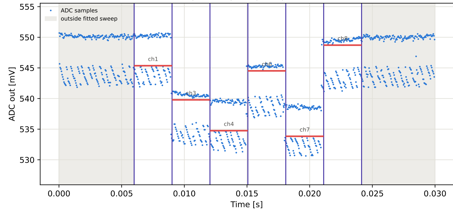
Tag6 &lt;- Tag5 | 855 MHz | run 0 | rep 1 | phase 116.07 deg
