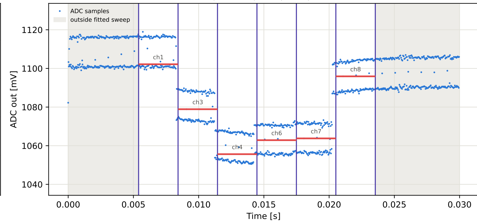
Tag16 &lt;- Tag15 | 885 MHz | run 0 | rep 1 | phase 72.81 deg
