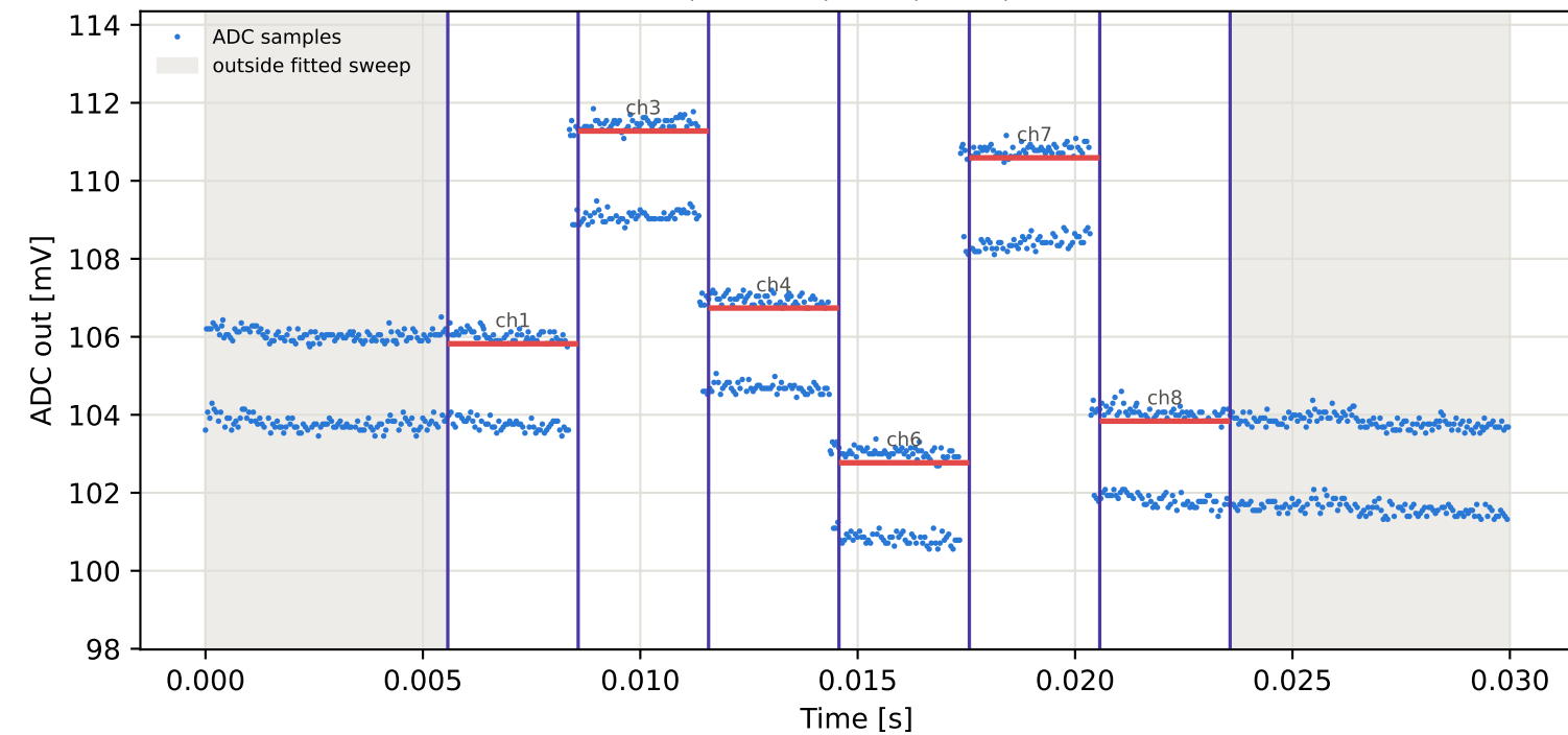
Tag6 &lt;- Tag10 | 785 MHz | run 0 | rep 1 | phase 7.45 deg
