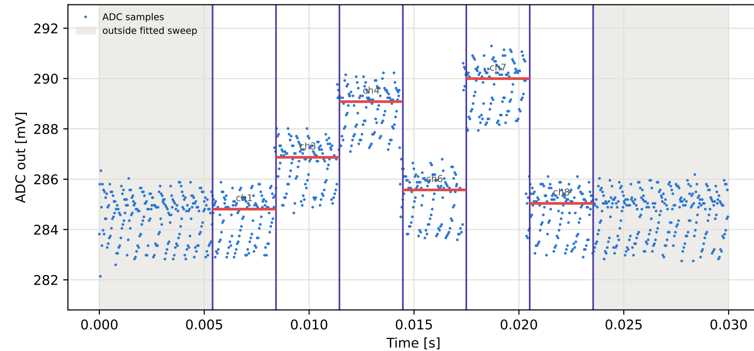
Tag15 &lt;- Tag5 | 785 MHz | run 0 | rep 1 | phase -13.61 deg
