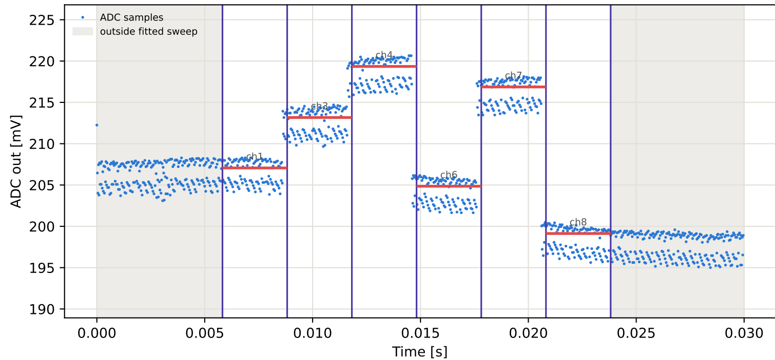
Tag1 &lt;- Tag4 | 925 MHz | run 0 | rep 1 | phase -52.03 deg
