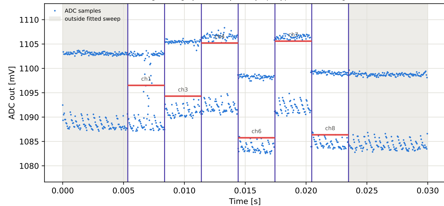
Tag5 &lt;- Tag4 | 875 MHz | run 0 | rep 1 | phase 89.34 deg
