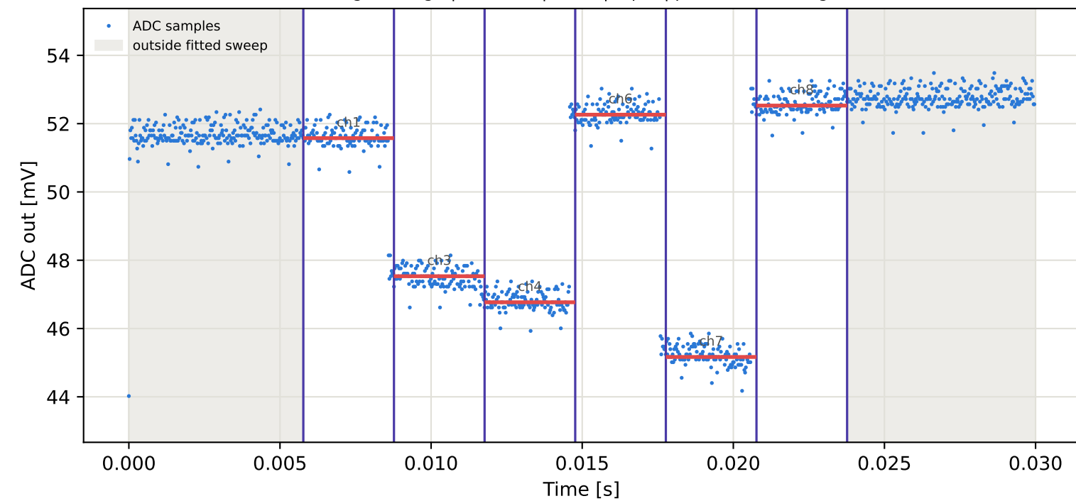
Tag1 &lt;- Tag8 | 775 MHz | run 0 | rep 1 | phase 131.38 deg
