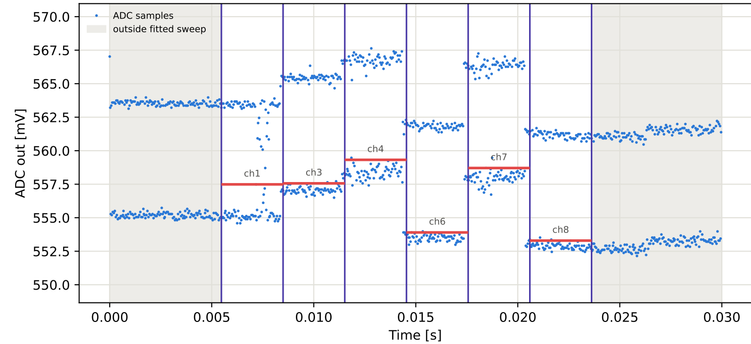
Tag10 &lt;- Tag4 | 875 MHz | run 0 | rep 1 | phase 3.13 deg
