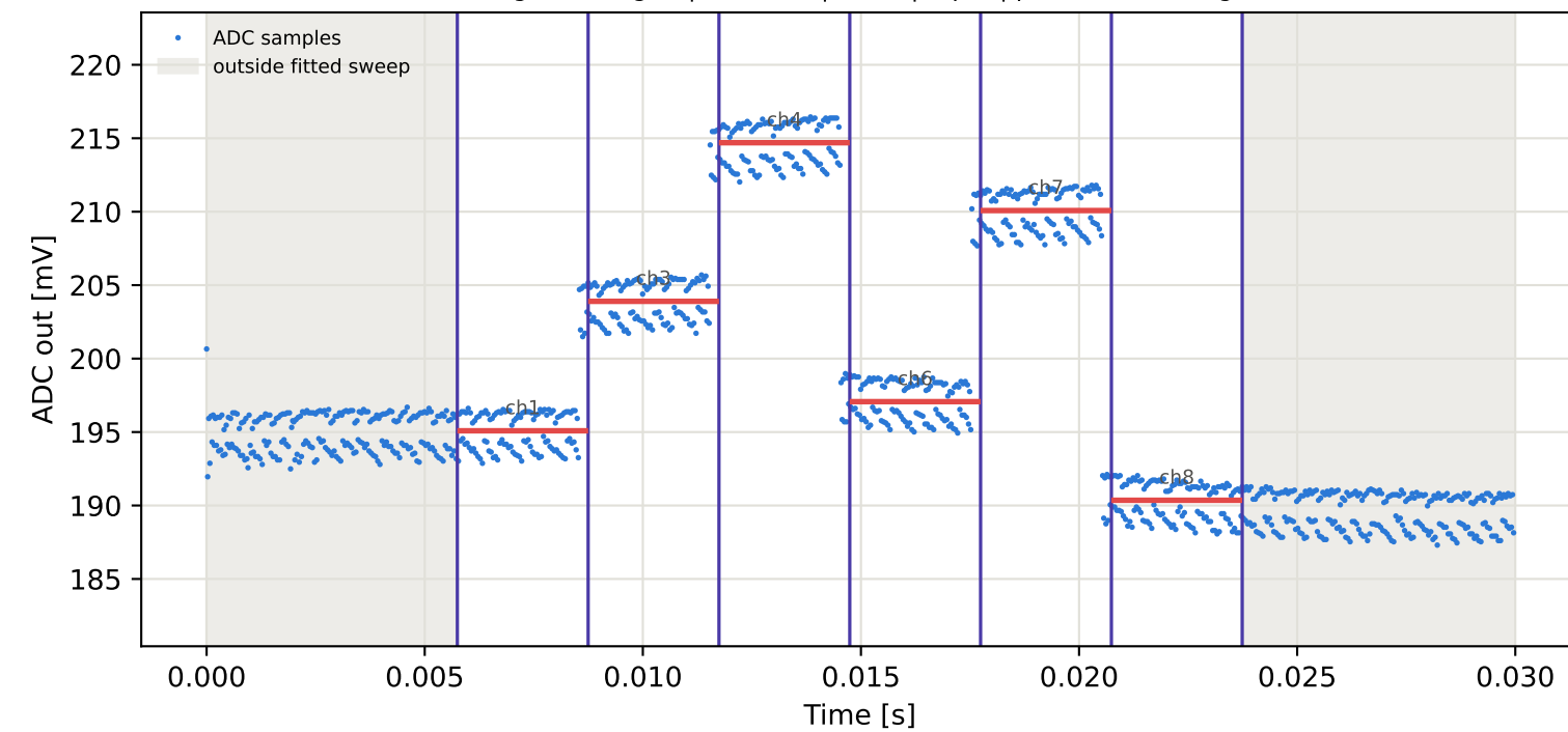
Tag10 &lt;- Tag2 | 955 MHz | run 0 | rep 1 | phase 114.01 deg
