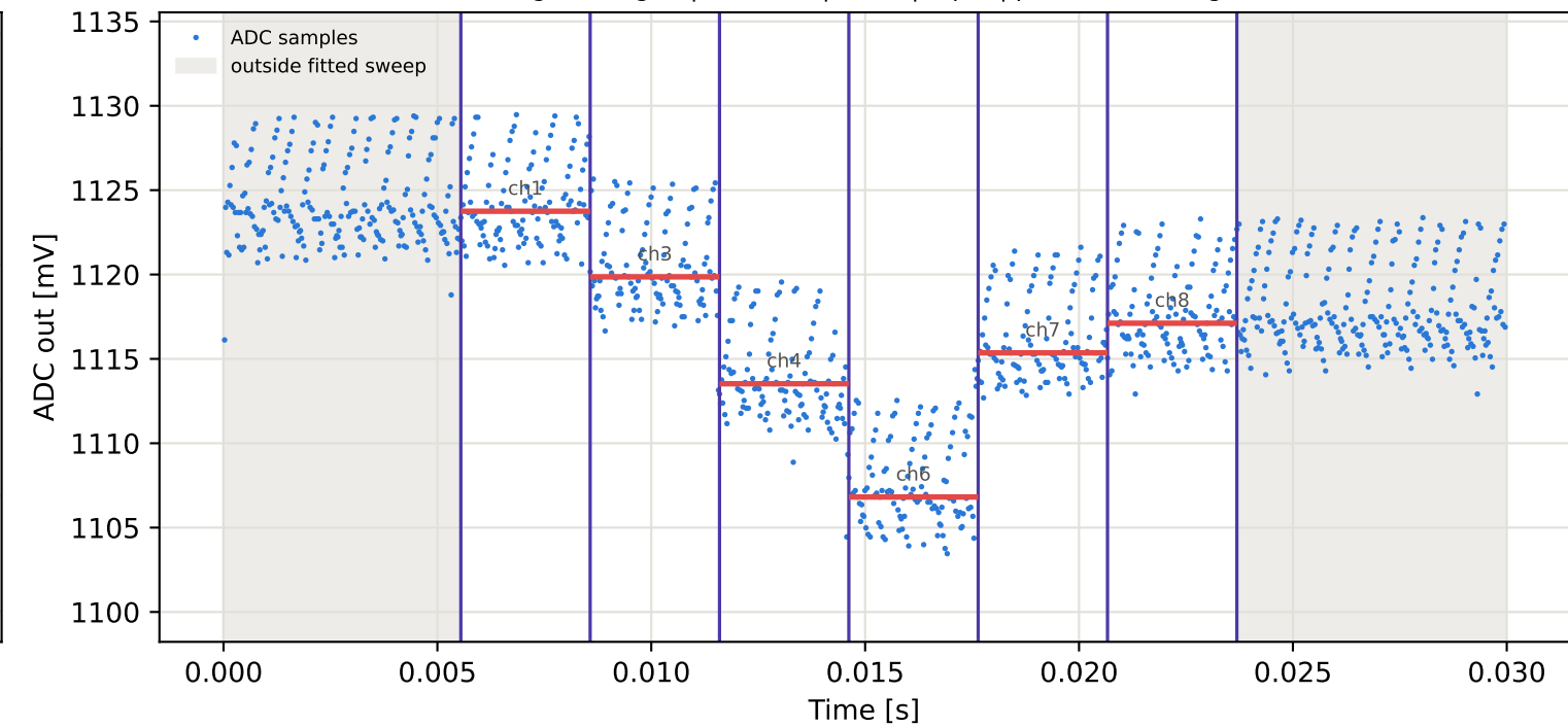
Tag4 &lt;- Tag16 | 895 MHz | run 0 | rep 1 | phase 7.01 deg
