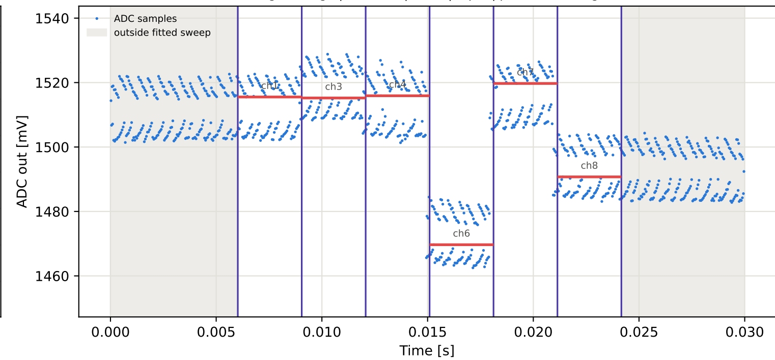
Tag4 &lt;- Tag8 | 925 MHz | run 0 | rep 1 | phase -84.91 deg
