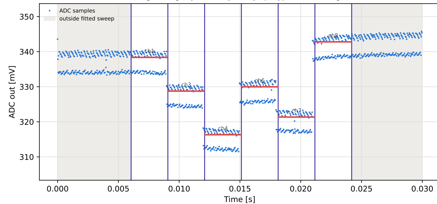
Tag3 &lt;- Tag16 | 925 MHz | run 0 | rep 1 | phase 42.40 deg
