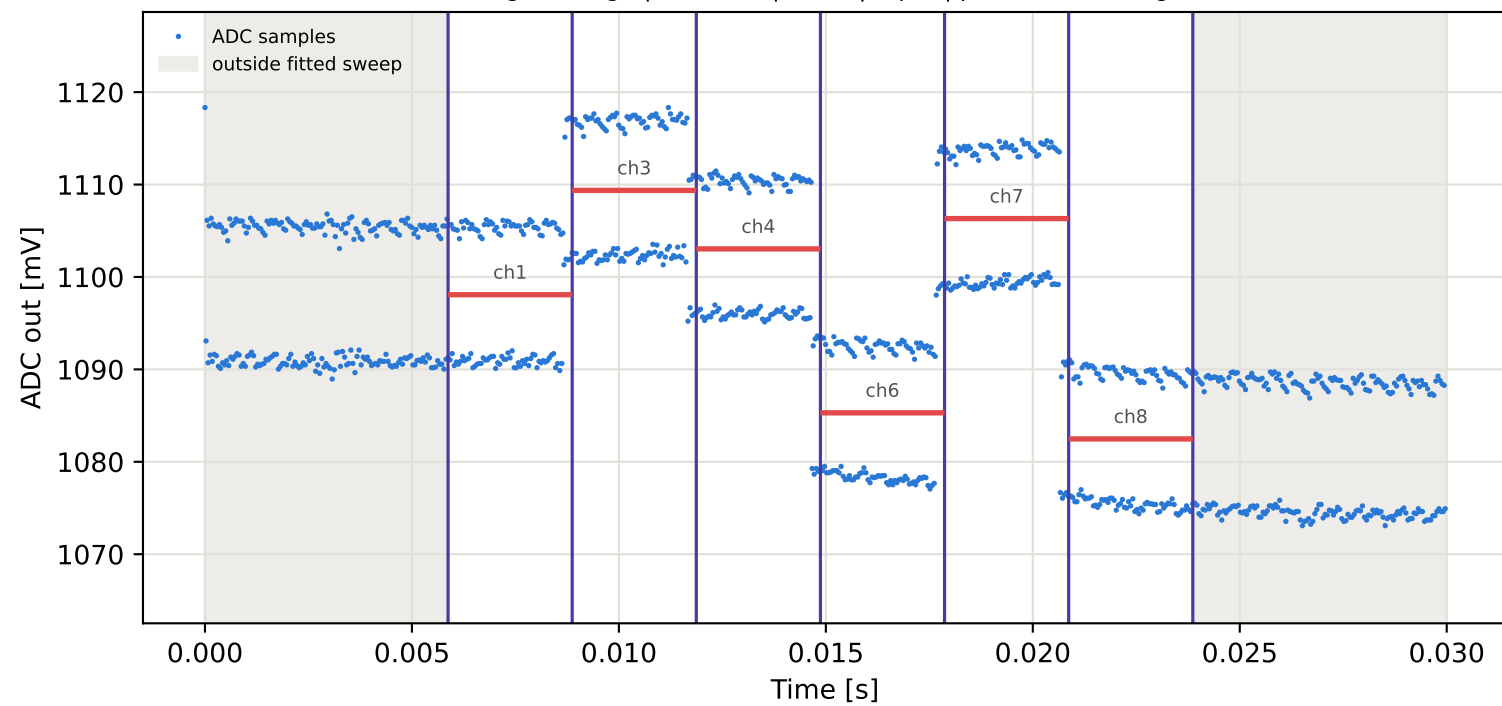
Tag5 &lt;- Tag9 | 875 MHz | run 0 | rep 1 | phase 1.78 deg
