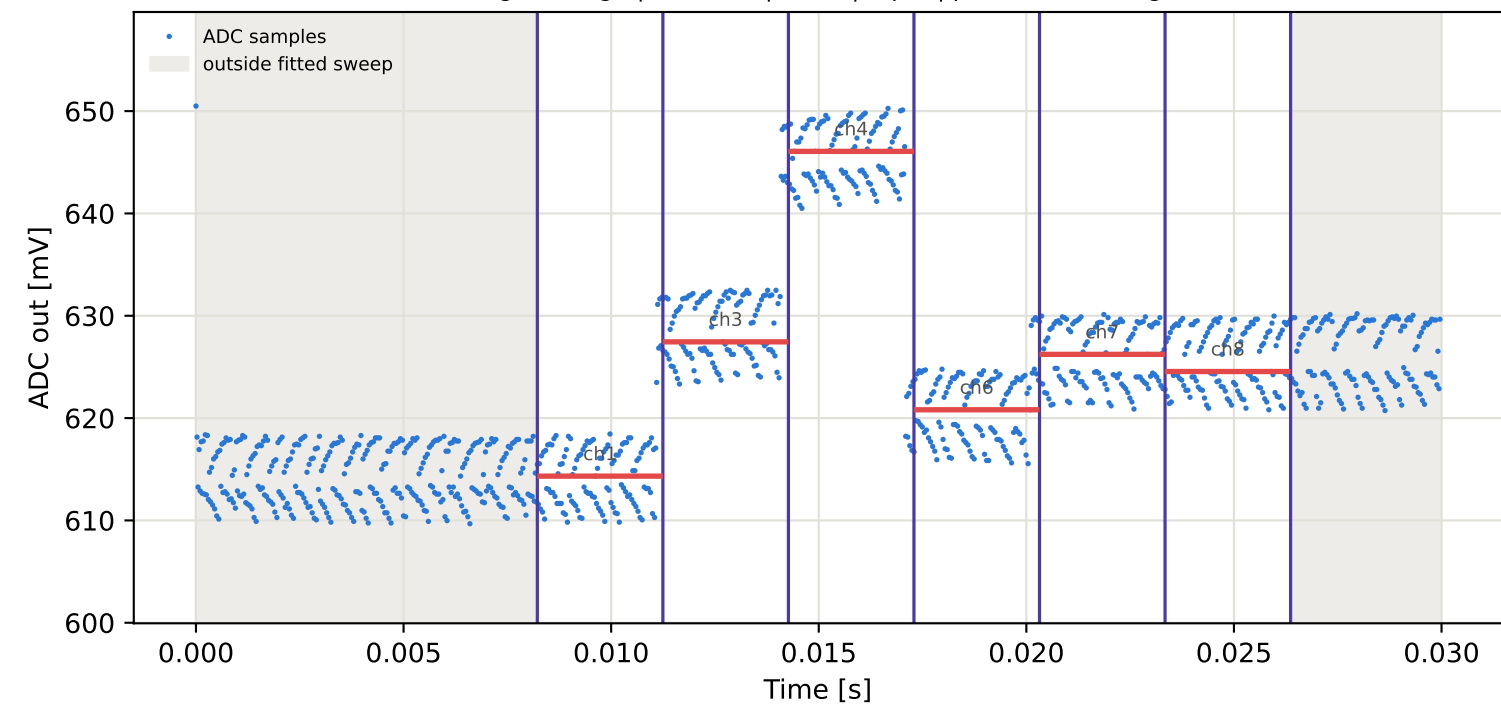
Tag8 &lt;- Tag10 | 945 MHz | run 0 | rep 1 | phase 86.89 deg
