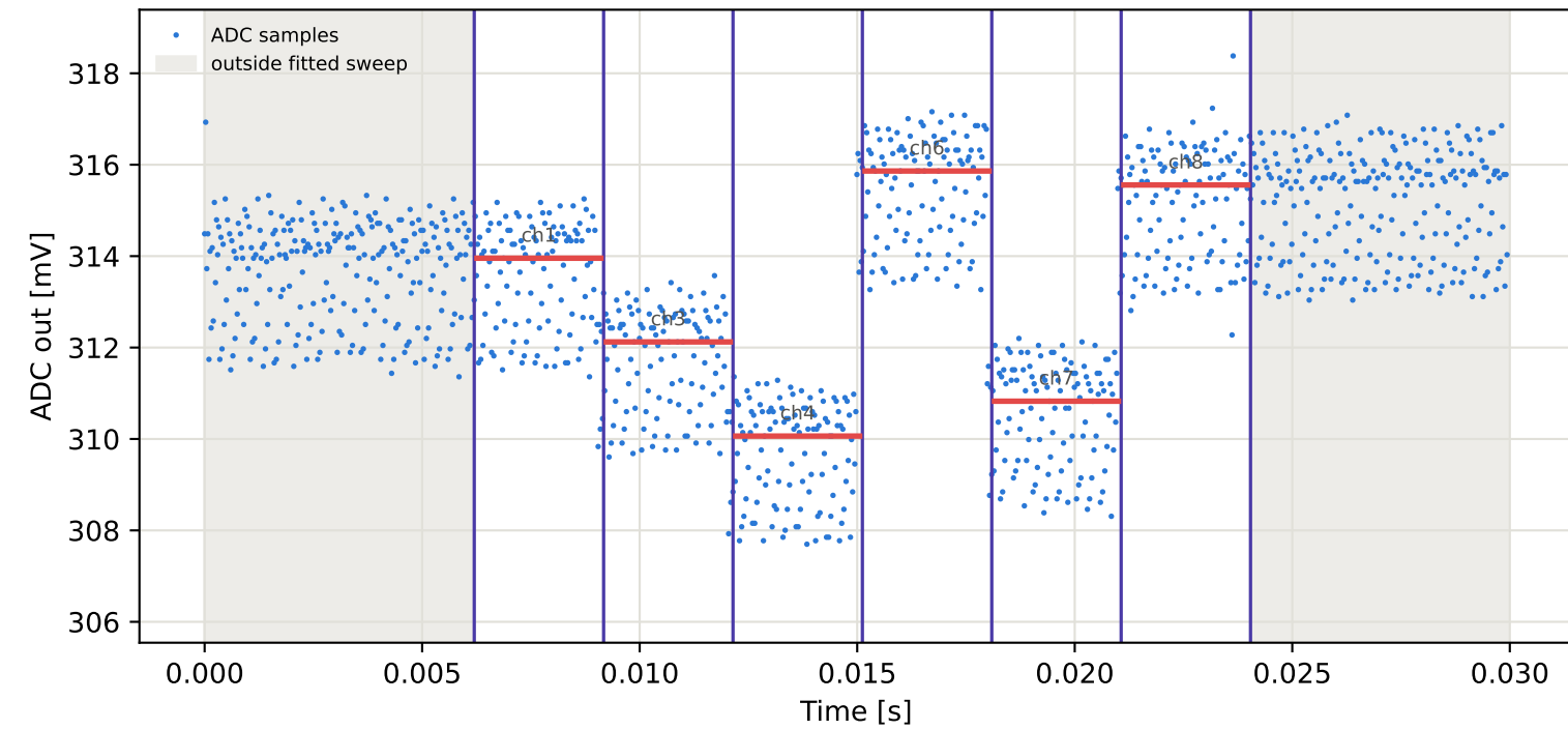
Tag3 &lt;- Tag2 | 995 MHz | run 0 | rep 1 | phase 114.15 deg
