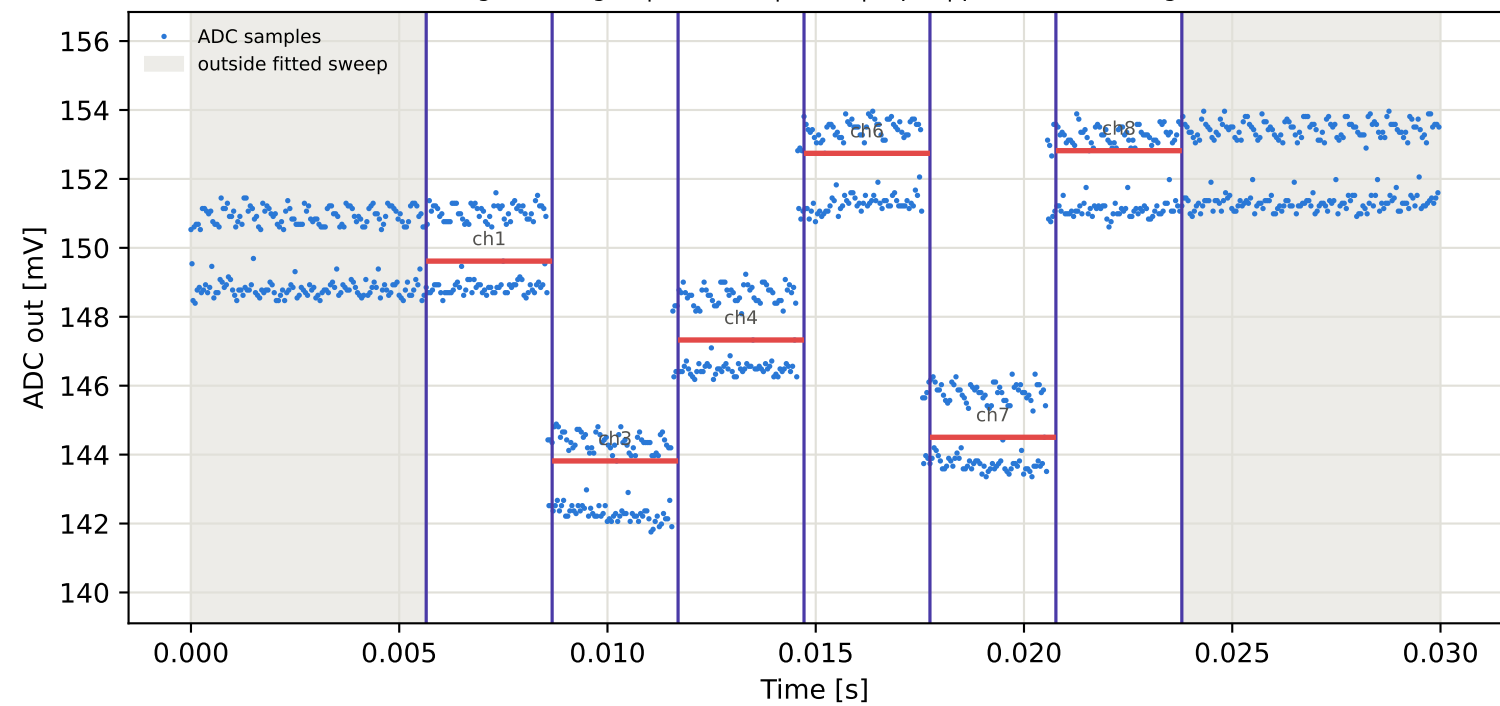
Tag10 &lt;- Tag2 | 825 MHz | run 0 | rep 1 | phase -39.72 deg
