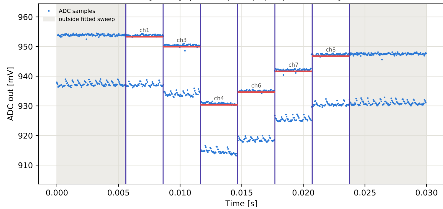
Tag8 &lt;- Tag7 | 975 MHz | run 0 | rep 1 | phase 47.59 deg
