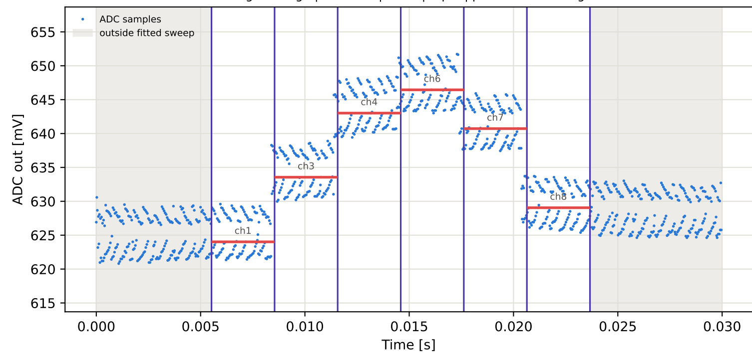
Tag9 &lt;- Tag15 | 895 MHz | run 0 | rep 1 | phase -141.14 deg
