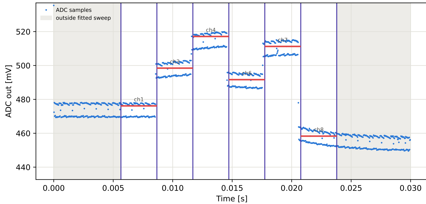
Tag10 &lt;- Tag8 | 895 MHz | run 0 | rep 1 | phase -45.94 deg
