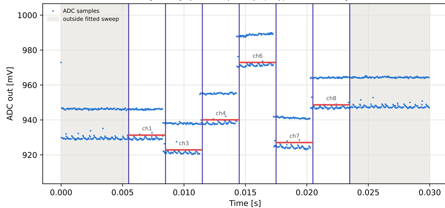
Tag8 &lt;- Tag6 | 975 MHz | run 0 | rep 1 | phase -107.97 deg
