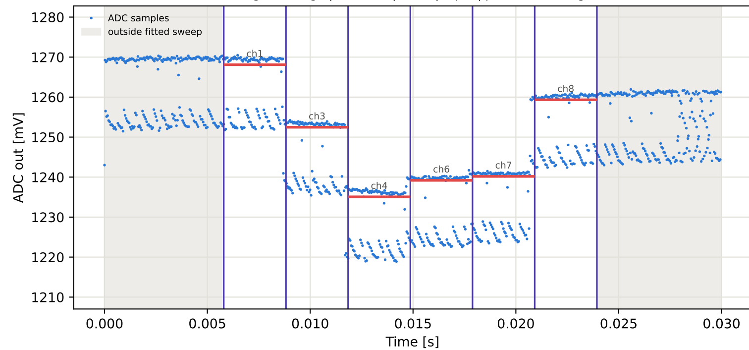
Tag16 &lt;- Tag5 | 875 MHz | run 0 | rep 1 | phase 2.81 deg
