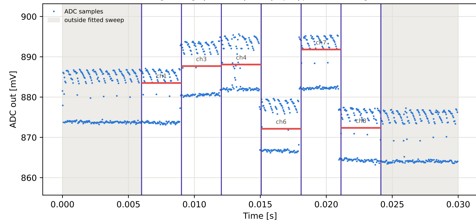
Tag8 &lt;- Tag4 | 845 MHz | run 0 | rep 1 | phase -52.46 deg
