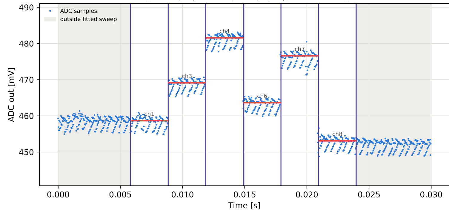
Tag6 &lt;- Tag3 | 925 MHz | run 0 | rep 1 | phase 10.18 deg
