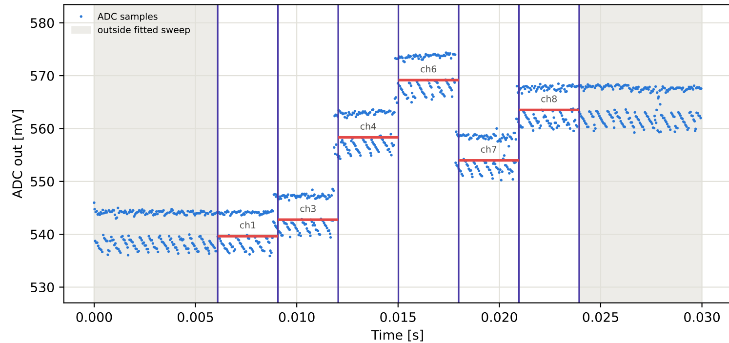
Tag15 &lt;- Tag10 | 875 MHz | run 0 | rep 1 | phase -33.89 deg
