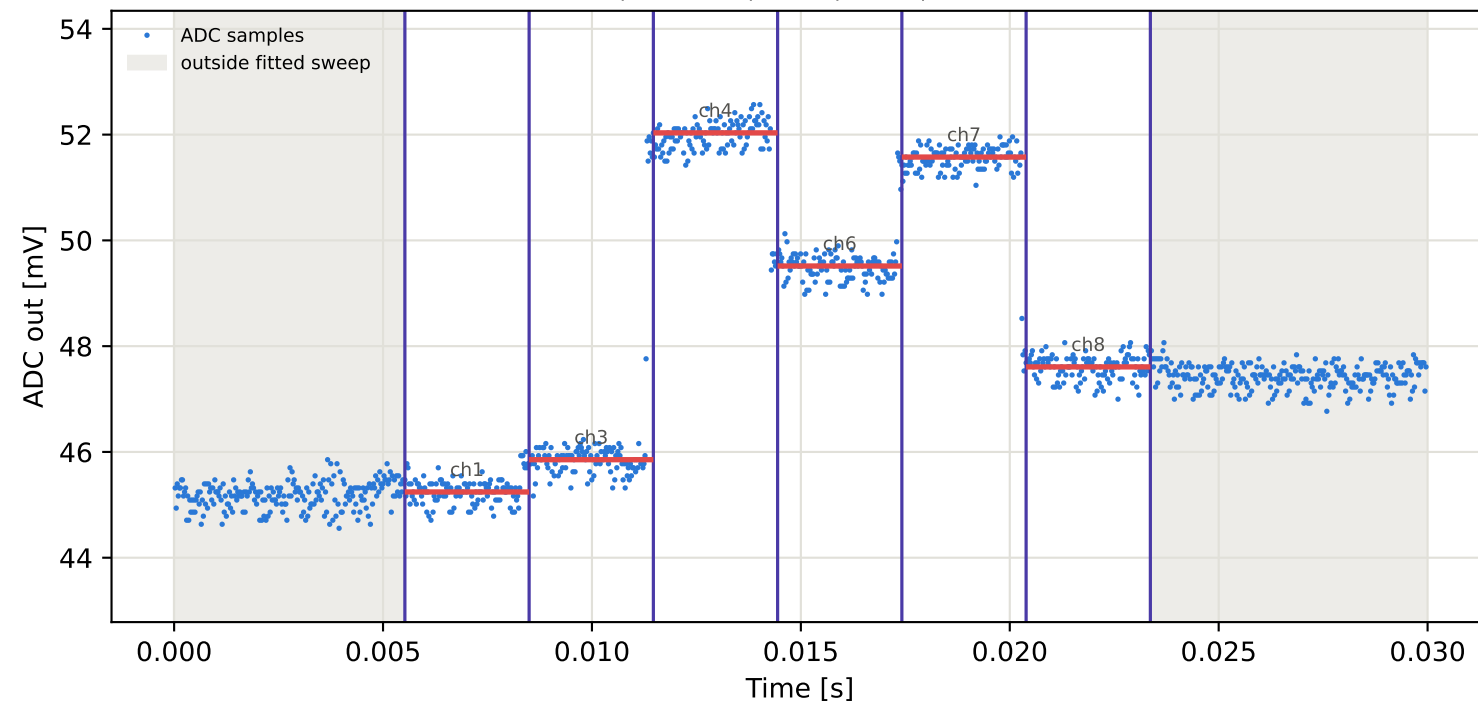
Tag10 &lt;- Tag4 | 805 MHz | run 0 | rep 1 | phase -102.12 deg
