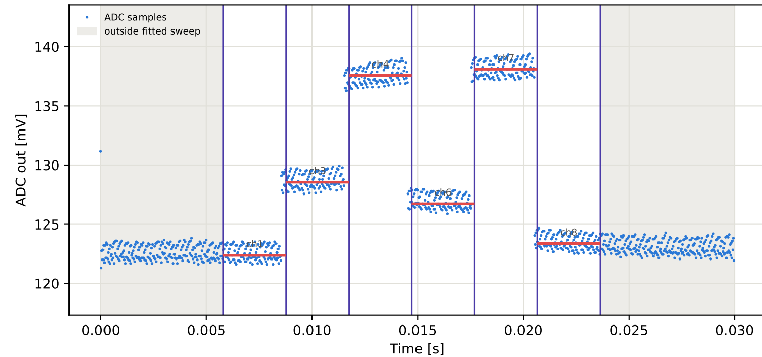
Tag3 &lt;- Tag8 | 775 MHz | run 0 | rep 1 | phase 104.93 deg
