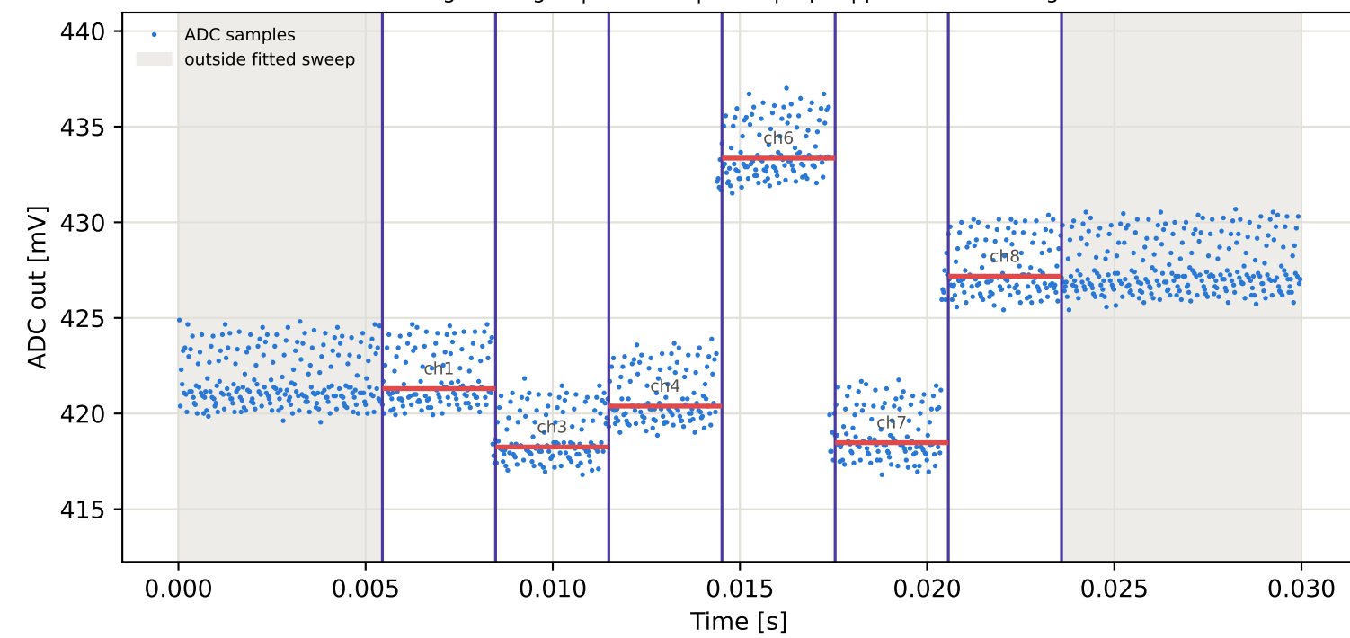
Tag1 &lt;- Tag16 | 975 MHz | run 0 | rep 1 | phase -40.53 deg
