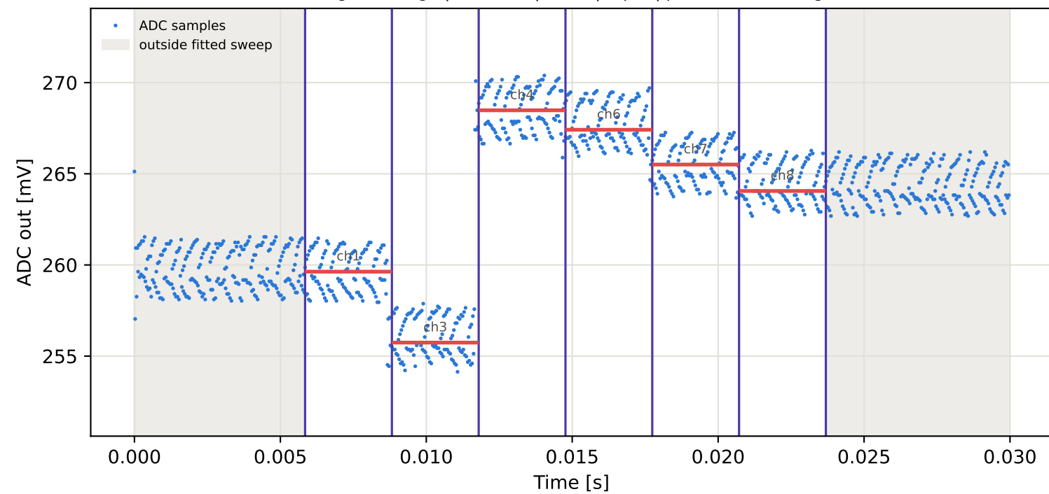
Tag16 &lt;- Tag5 | 805 MHz | run 0 | rep 1 | phase -80.42 deg
