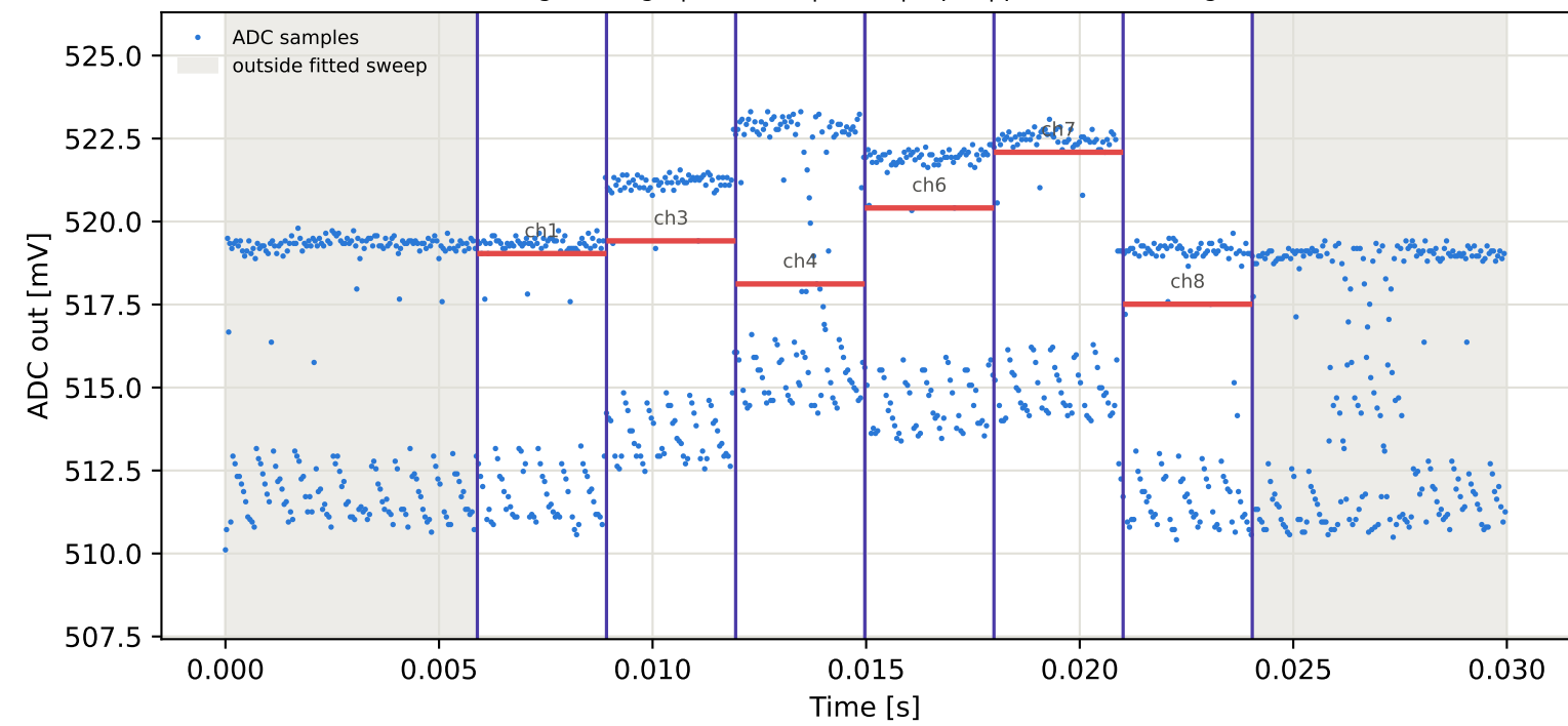
Tag7 &lt;- Tag4 | 845 MHz | run 0 | rep 1 | phase 47.61 deg
