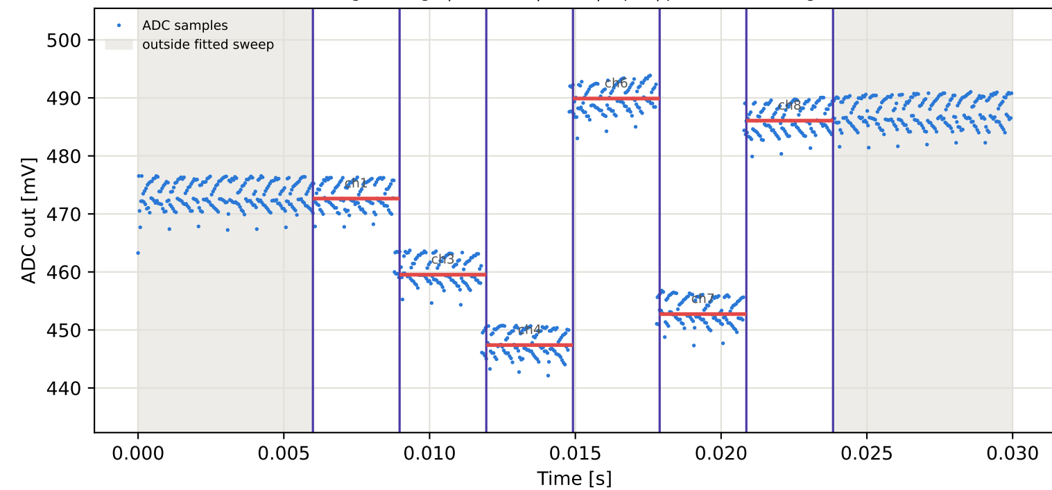
Tag9 &lt;- Tag5 | 945 MHz | run 0 | rep 1 | phase -23.29 deg
