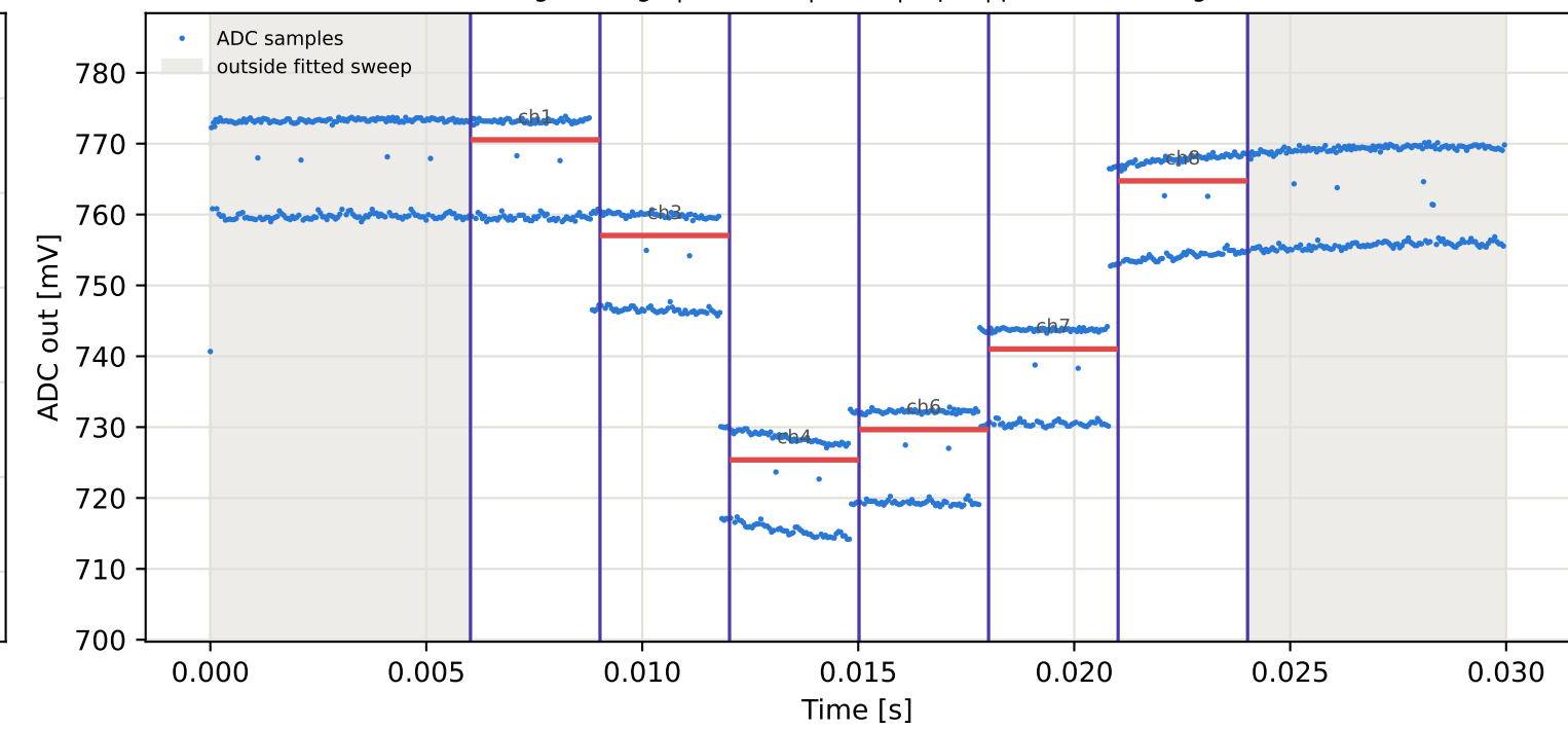
Tag9 &lt;- Tag8 | 935 MHz | run 0 | rep 1 | phase 56.45 deg
