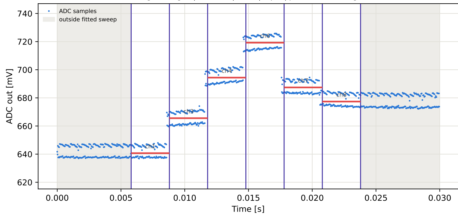
Tag6 &lt;- Tag3 | 875 MHz | run 0 | rep 1 | phase -128.89 deg
