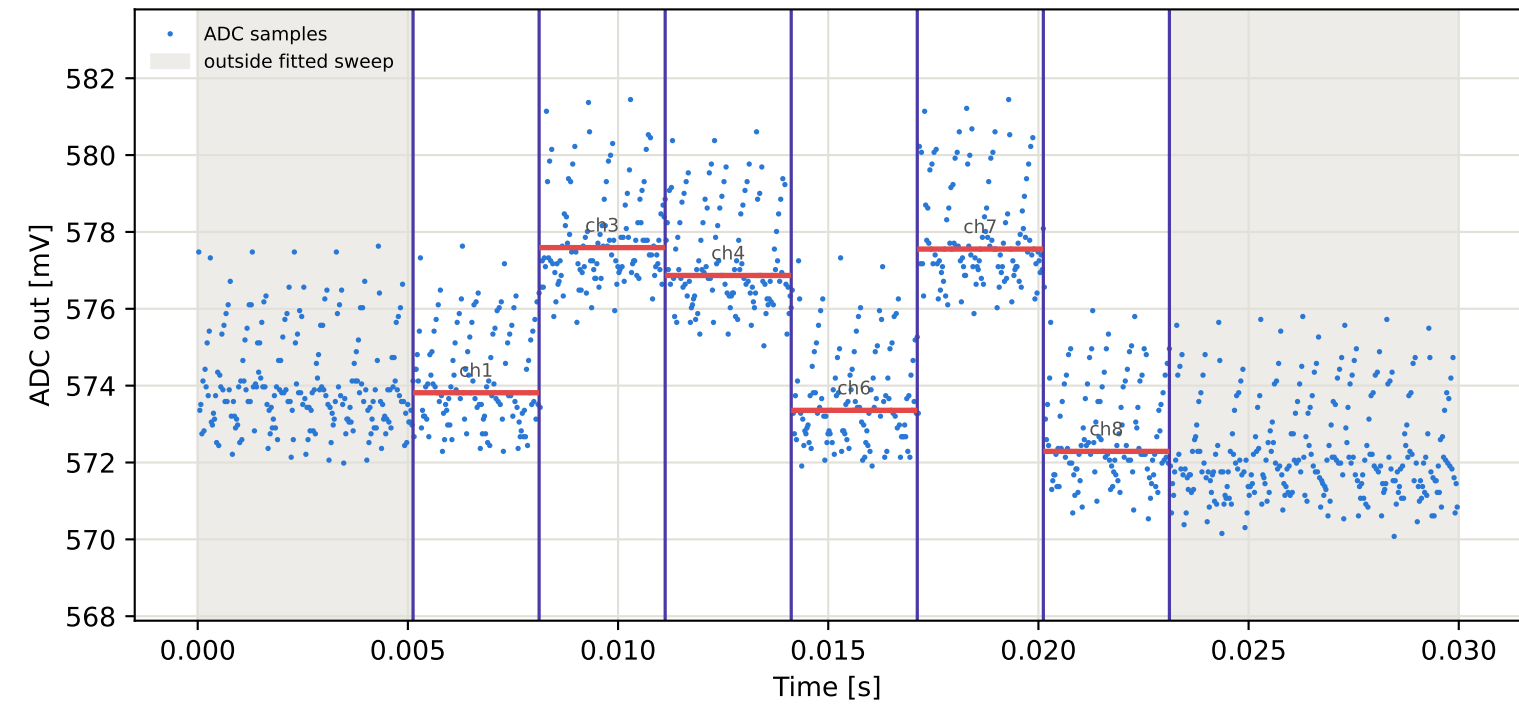
Tag6 &lt;- Tag10 | 865 MHz | run 0 | rep 1 | phase 175.70 deg
