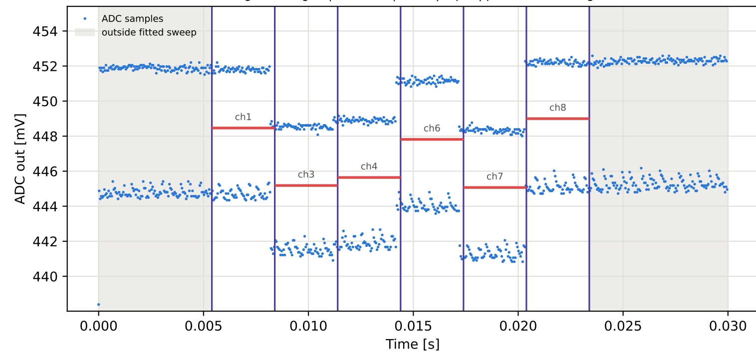
Tag15 &lt;- Tag10 | 845 MHz | run 0 | rep 1 | phase 135.50 deg
