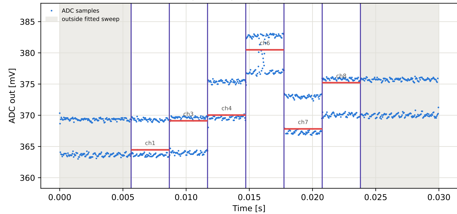
Tag9 &lt;- Tag2 | 835 MHz | run 0 | rep 1 | phase -158.91 deg
