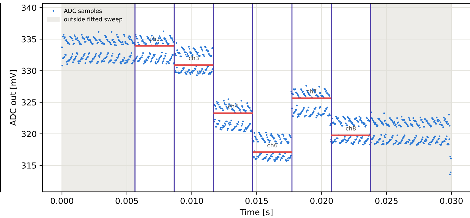
Tag10 &lt;- Tag1 | 865 MHz | run 0 | rep 1 | phase 34.54 deg
