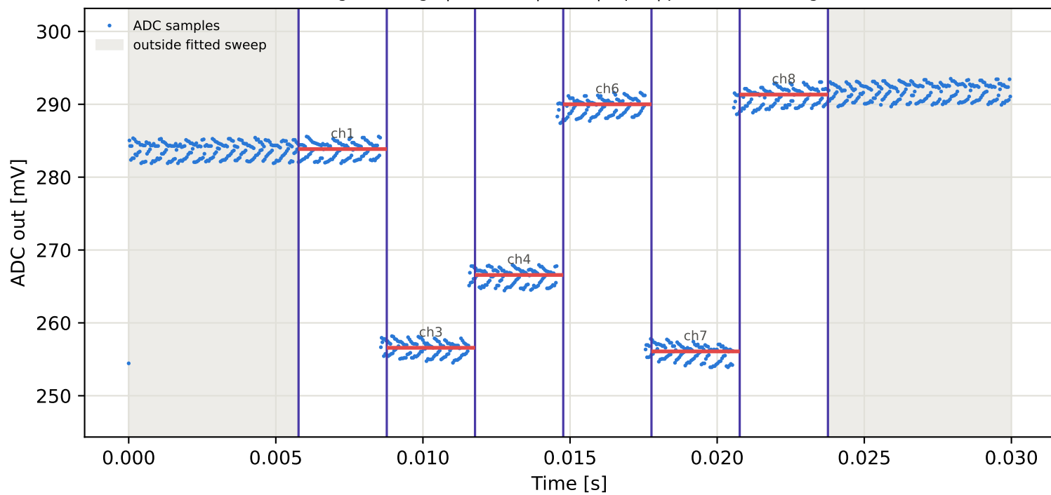
Tag2 &lt;- Tag1 | 805 MHz | run 0 | rep 1 | phase -149.77 deg
