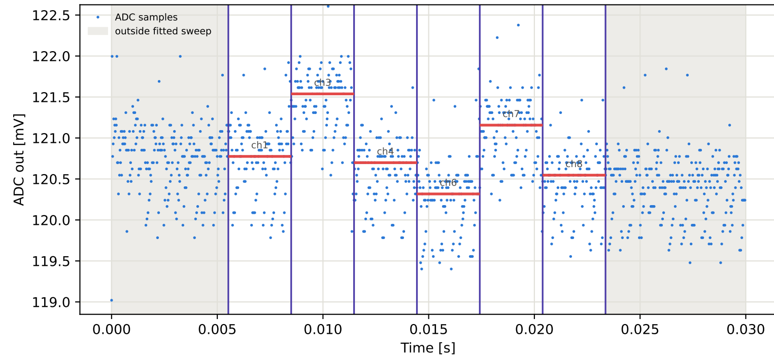
Tag8 &lt;- Tag16 | 785 MHz | run 0 | rep 1 | phase 25.88 deg
