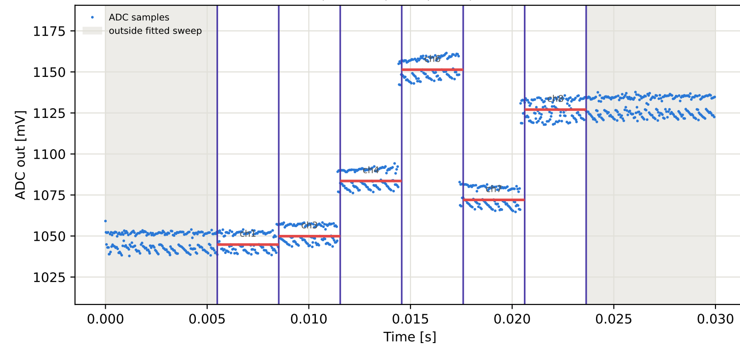
Tag15 &lt;- Tag5 | 885 MHz | run 0 | rep 1 | phase -161.25 deg
