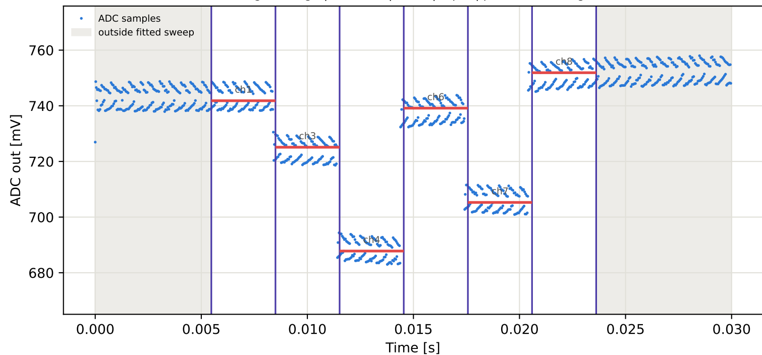
Tag4 &lt;- Tag8 | 955 MHz | run 0 | rep 1 | phase -78.73 deg
