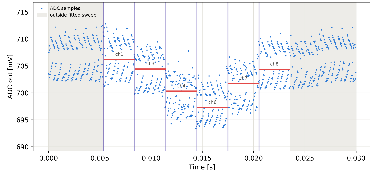
Tag6 &lt;- Tag4 | 875 MHz | run 0 | rep 1 | phase 108.65 deg
