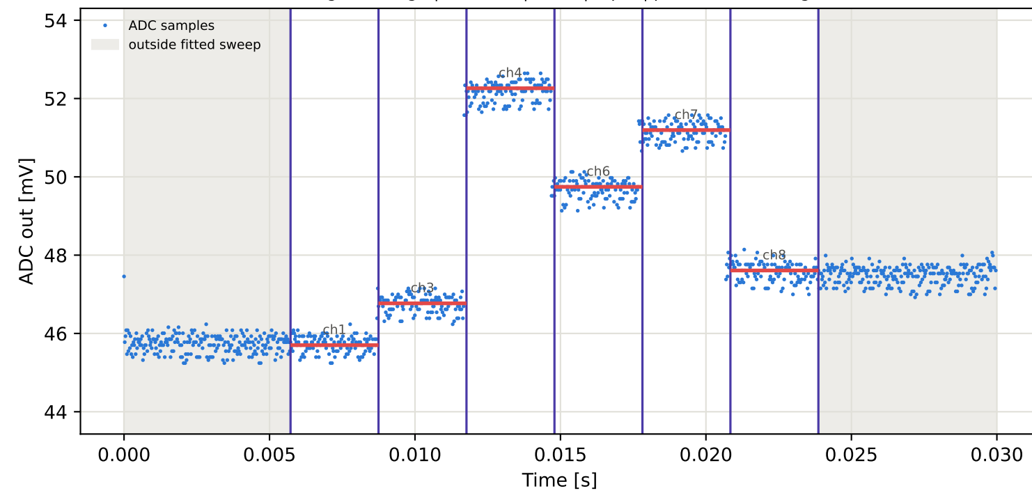
Tag10 &lt;- Tag8 | 805 MHz | run 0 | rep 1 | phase 146.54 deg
