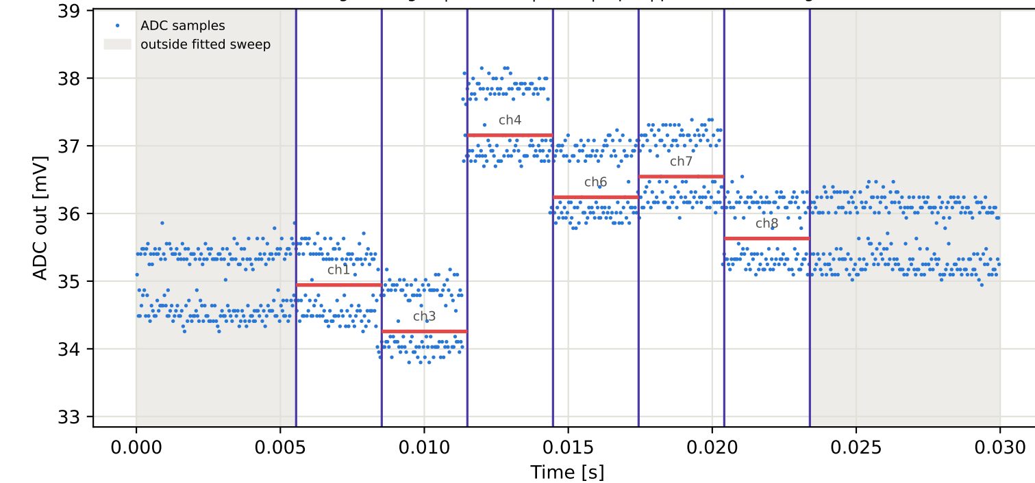
Tag7 &lt;- Tag10 | 785 MHz | run 0 | rep 1 | phase -107.81 deg
