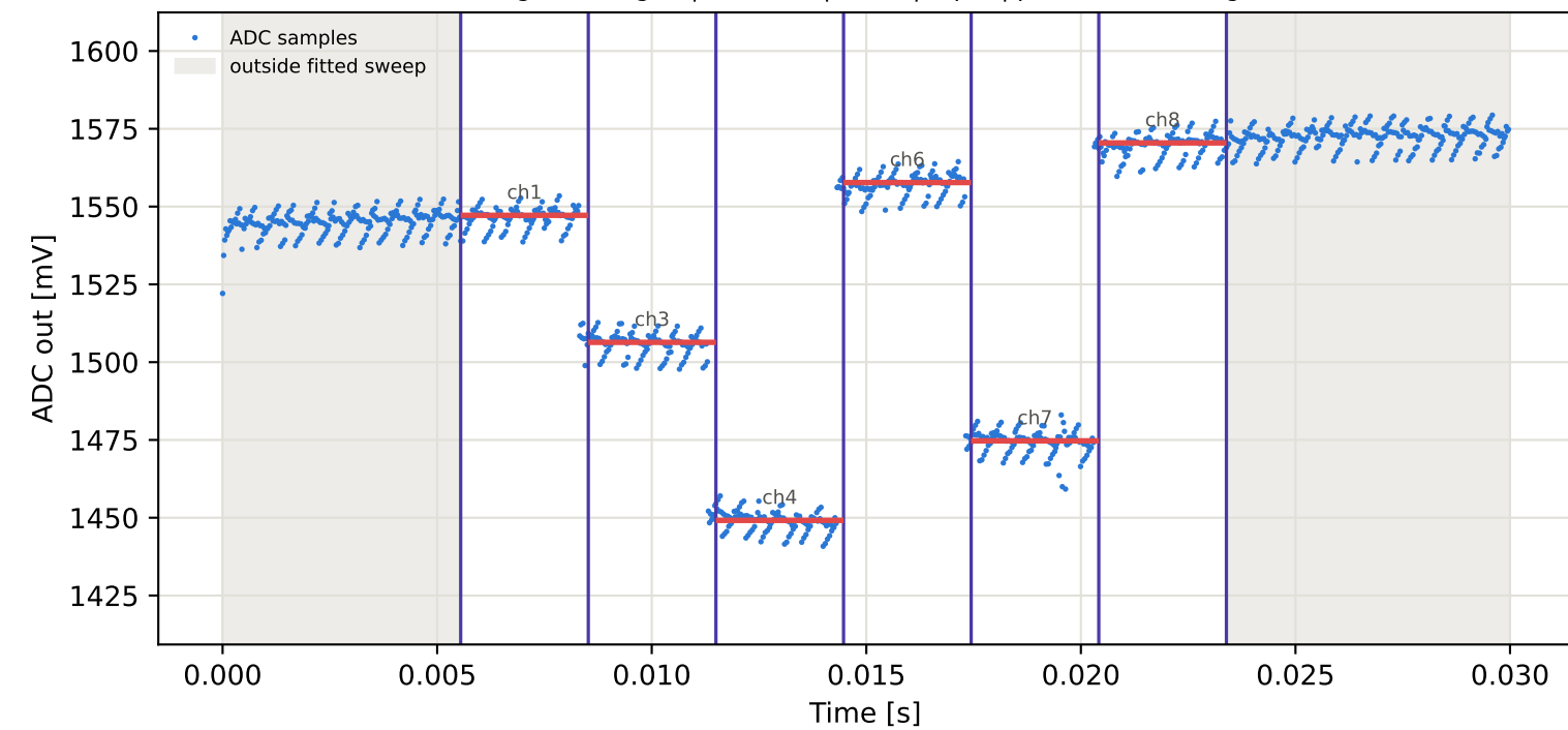
Tag15 &lt;- Tag3 | 955 MHz | run 0 | rep 1 | phase -35.11 deg
