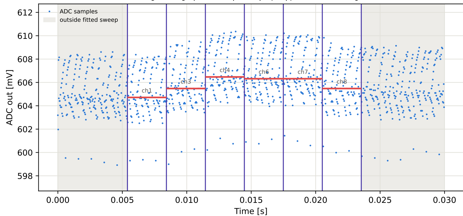
Tag7 &lt;- Tag6 | 855 MHz | run 0 | rep 1 | phase -112.65 deg
