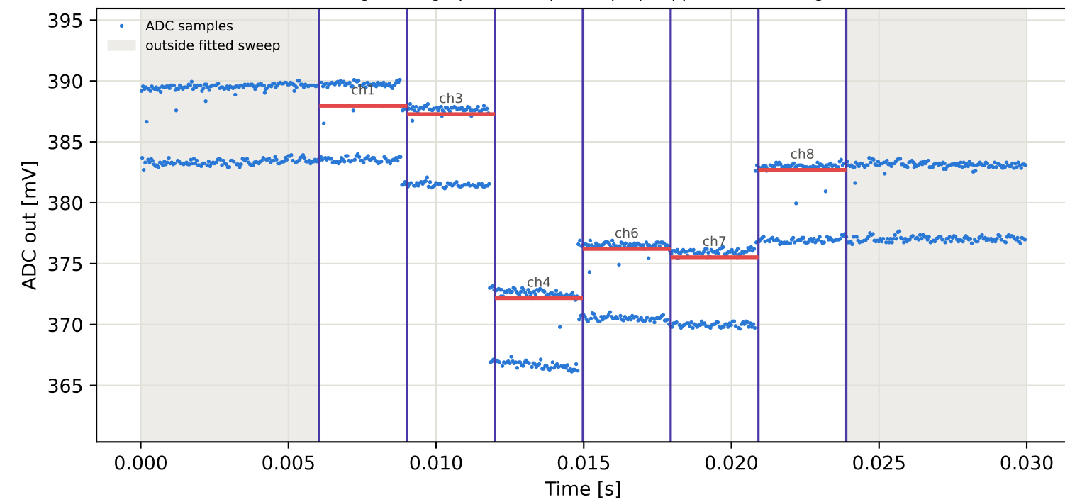
Tag4 &lt;- Tag7 | 825 MHz | run 0 | rep 1 | phase 51.66 deg
