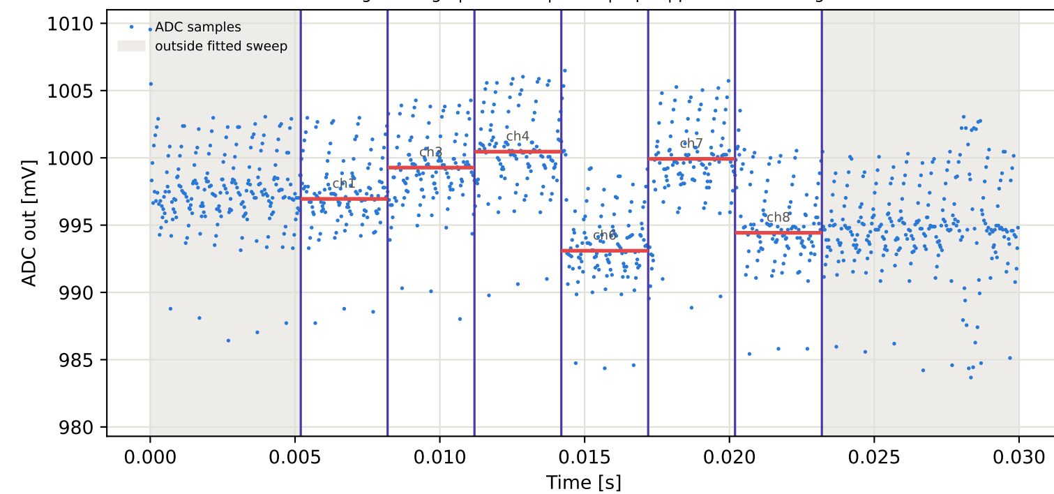
Tag8 &lt;- Tag4 | 945 MHz | run 0 | rep 1 | phase 146.13 deg
