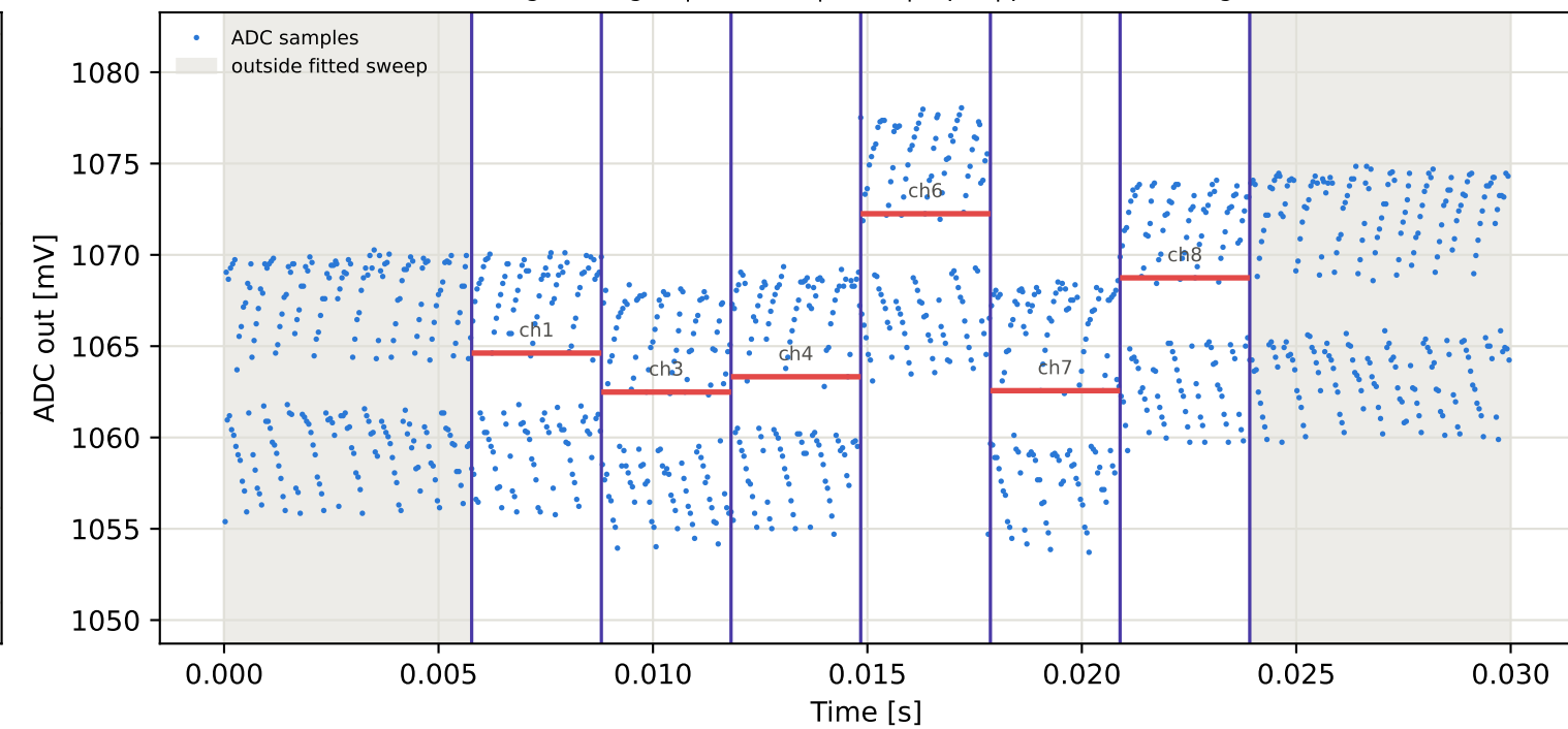
Tag4 &lt;- Tag16 | 945 MHz | run 0 | rep 1 | phase -3.74 deg
