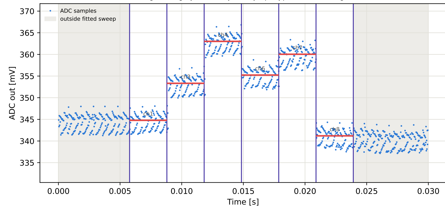
Tag9 &lt;- Tag7 | 915 MHz | run 0 | rep 1 | phase 23.18 deg
