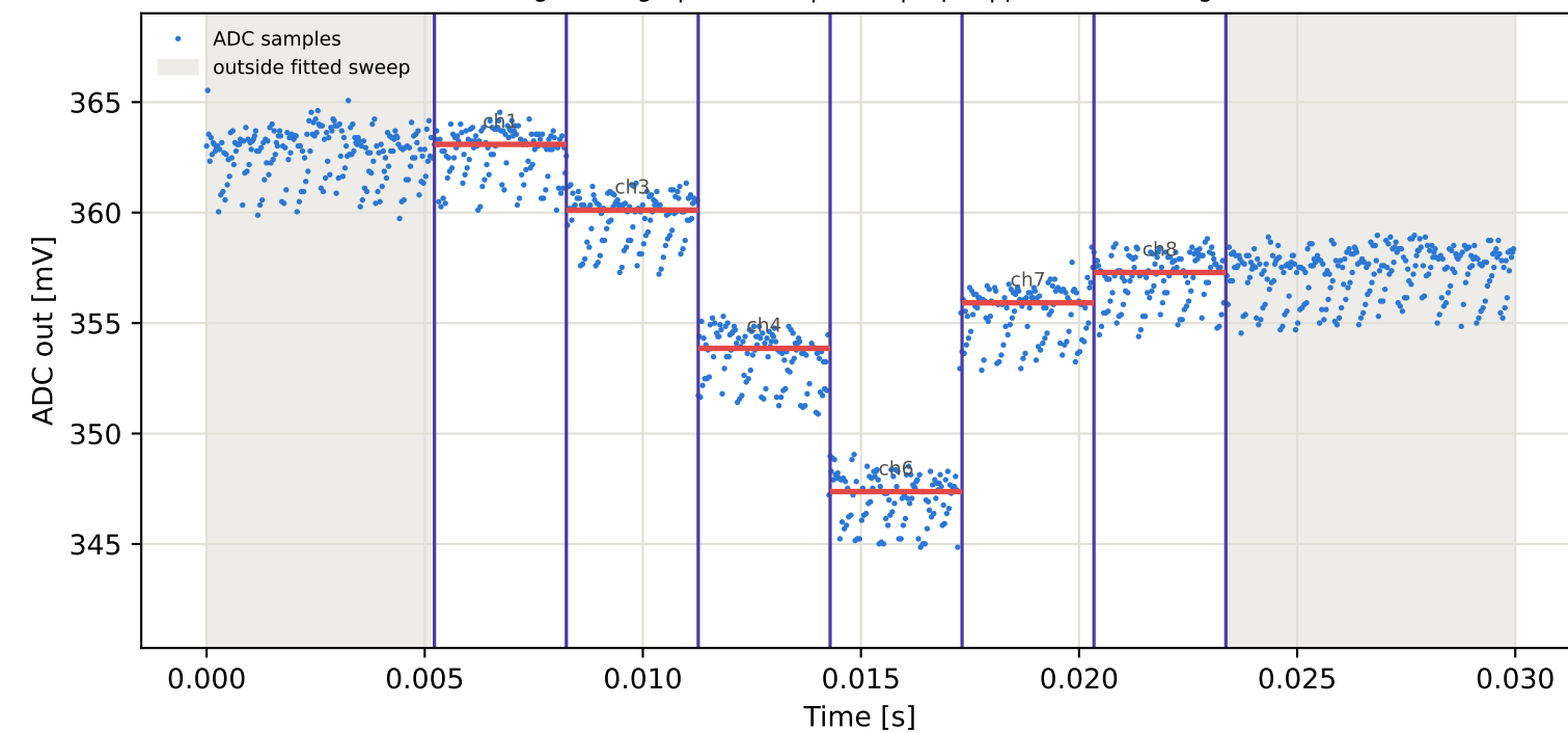
Tag2 &lt;- Tag7 | 905 MHz | run 0 | rep 1 | phase 38.39 deg
