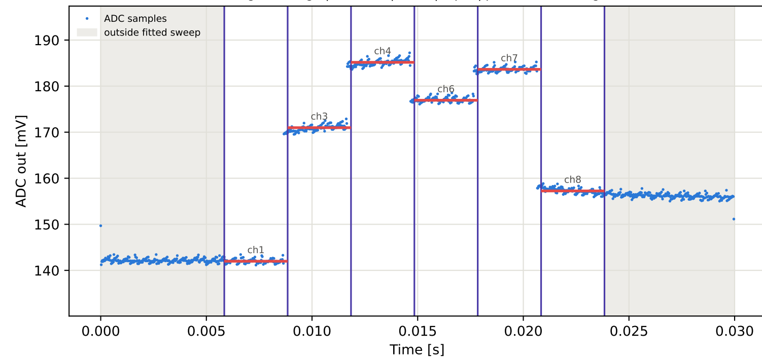
Tag10 &lt;- Tag8 | 855 MHz | run 0 | rep 1 | phase -91.28 deg
