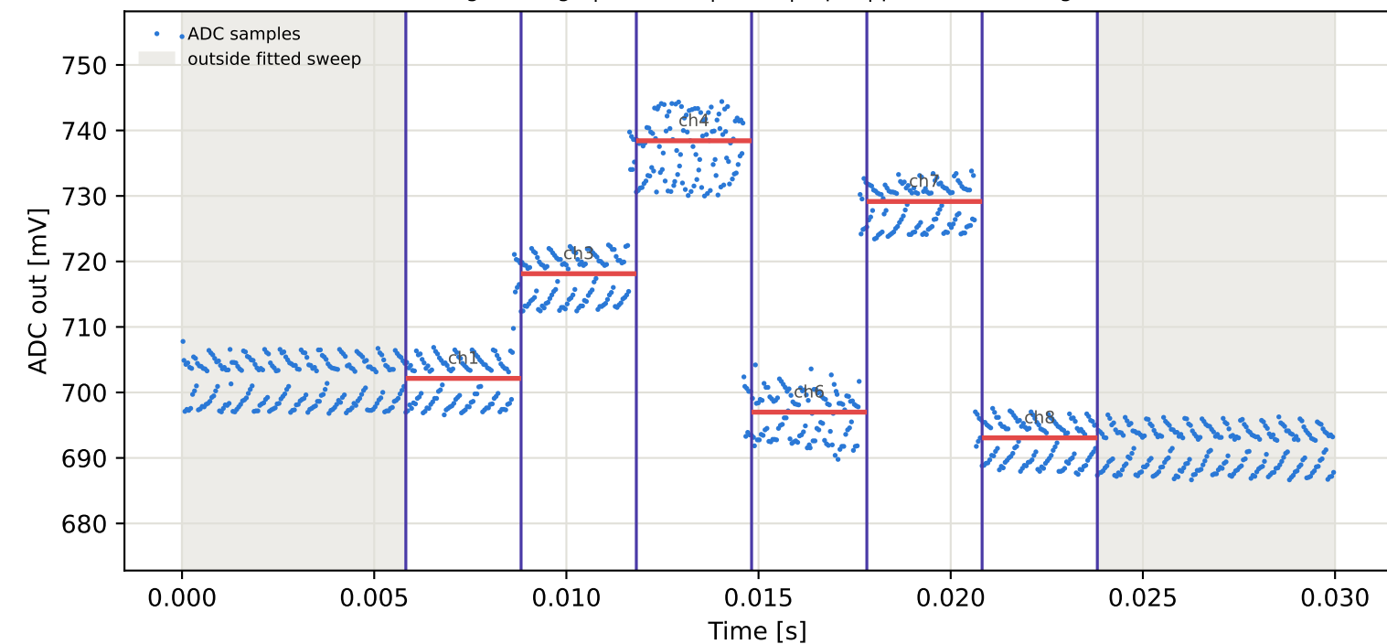
Tag4 &lt;- Tag9 | 955 MHz | run 0 | rep 1 | phase -171.85 deg
