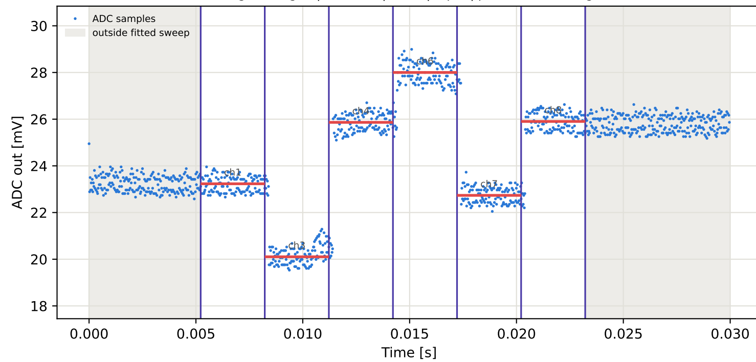
Tag6 &lt;- Tag2 | 795 MHz | run 0 | rep 1 | phase 176.30 deg
