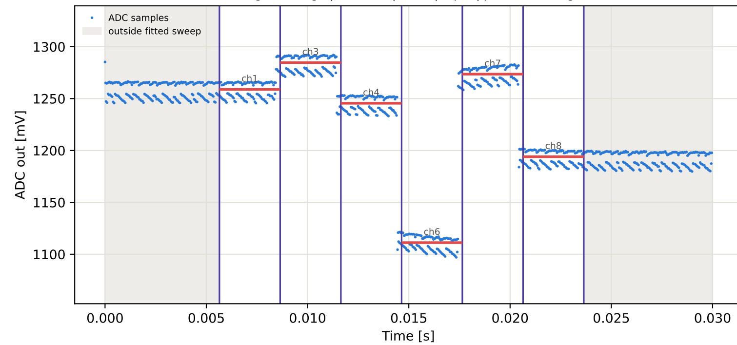
Tag2 &lt;- Tag1 | 955 MHz | run 0 | rep 1 | phase -25.08 deg
