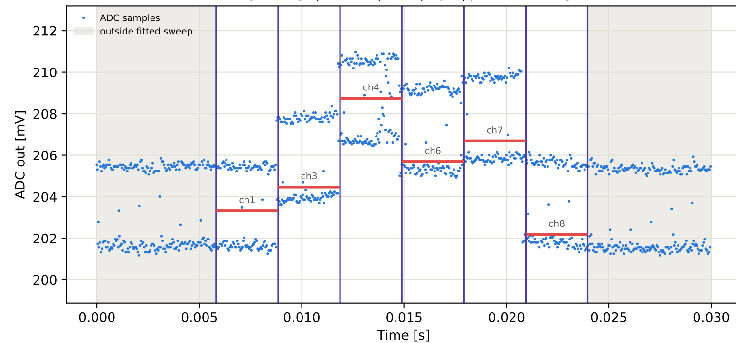
Tag6 &lt;- Tag4 | 835 MHz | run 0 | rep 1 | phase 88.53 deg
