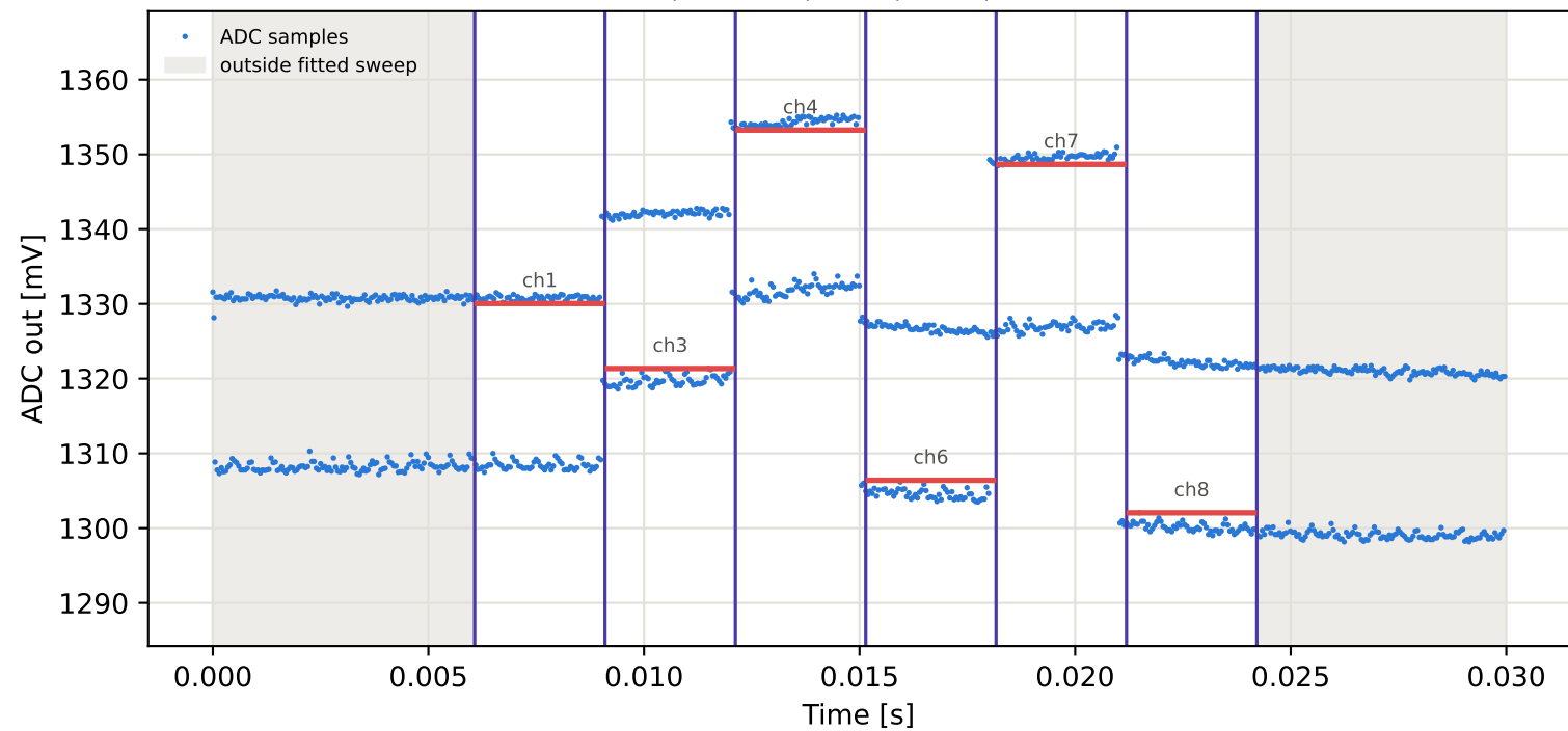
Tag8 &lt;- Tag7 | 935 MHz | run 0 | rep 1 | phase -61.70 deg
