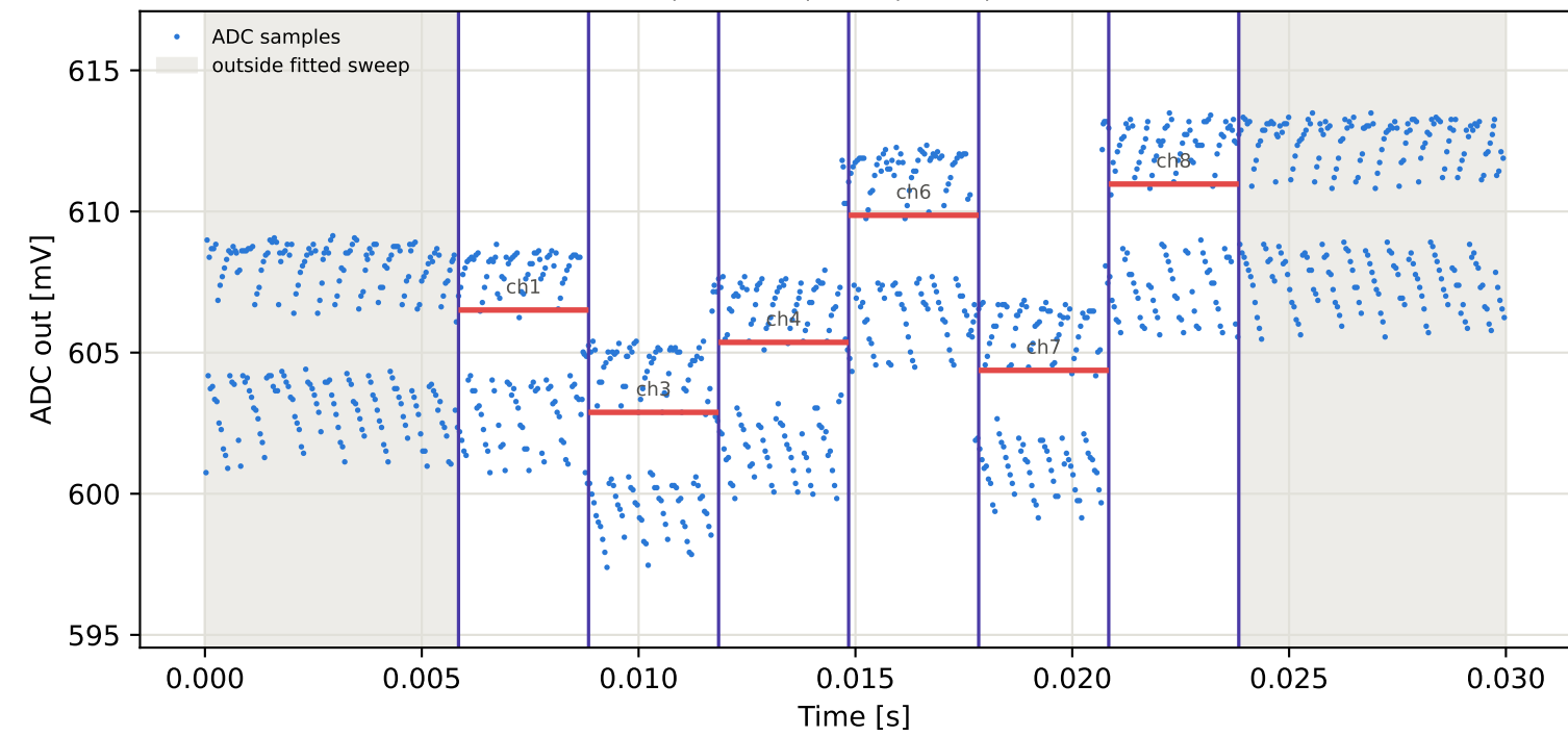
Tag15 &lt;- Tag6 | 855 MHz | run 0 | rep 1 | phase 173.05 deg
