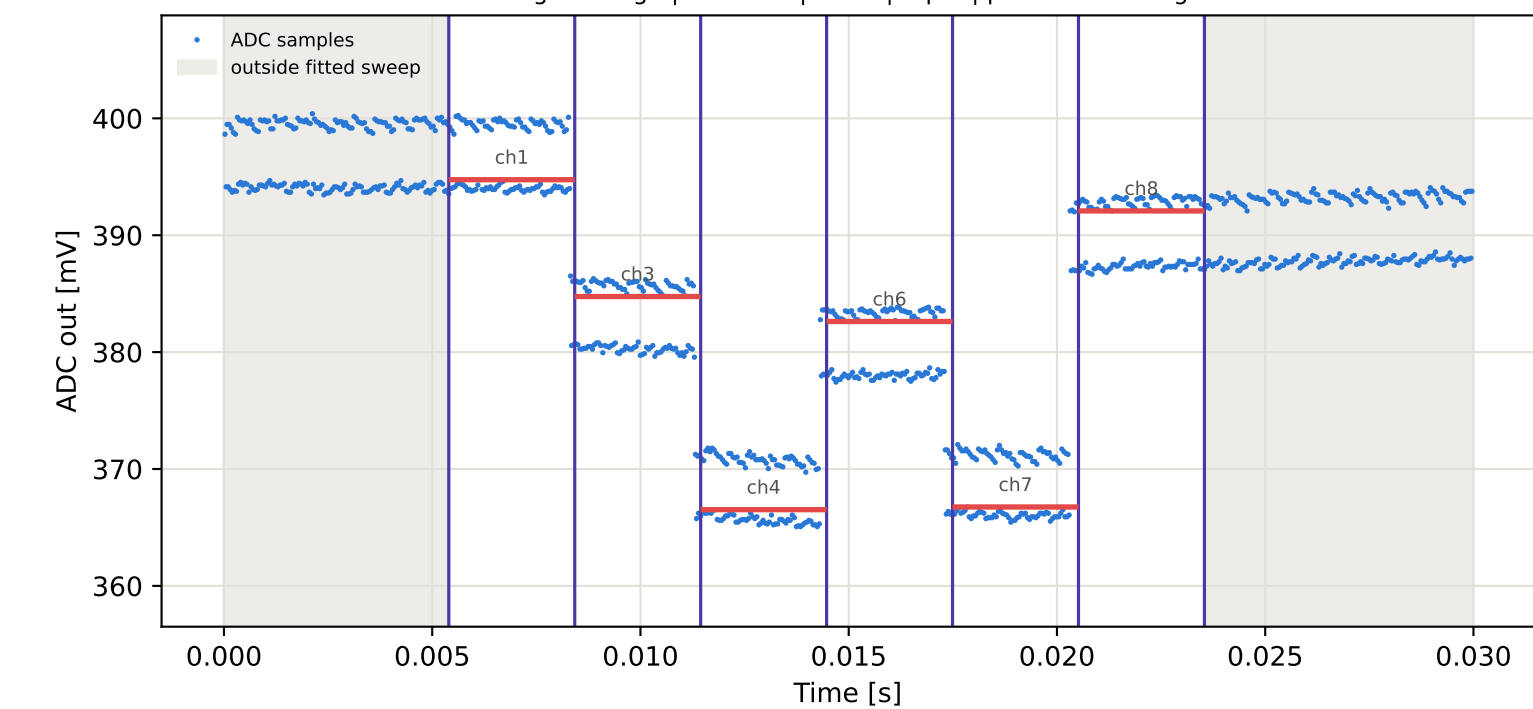
Tag9 &lt;- Tag7 | 835 MHz | run 0 | rep 1 | phase -155.58 deg
