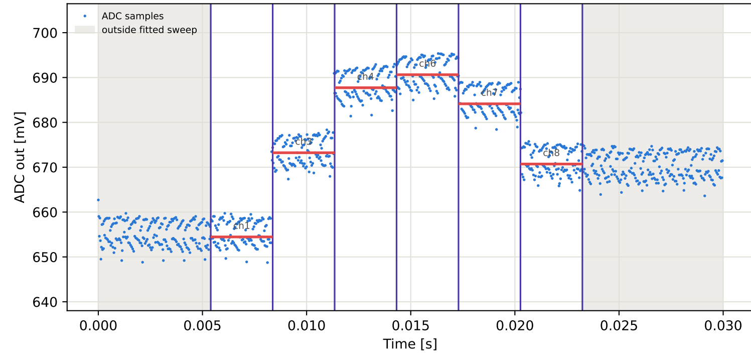
Tag15 &lt;- Tag10 | 885 MHz | run 0 | rep 1 | phase 41.00 deg
