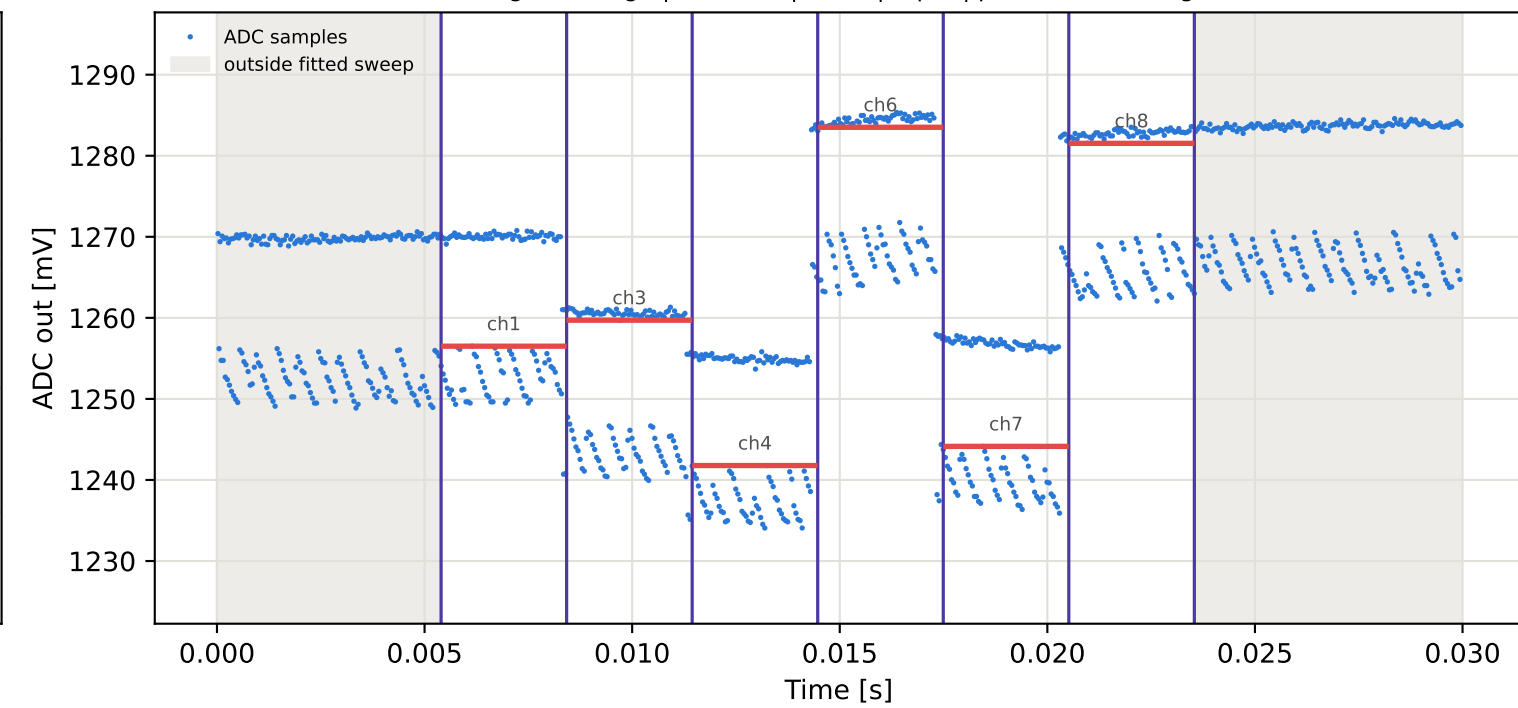
Tag16 &lt;- Tag7 | 925 MHz | run 0 | rep 1 | phase 138.40 deg
