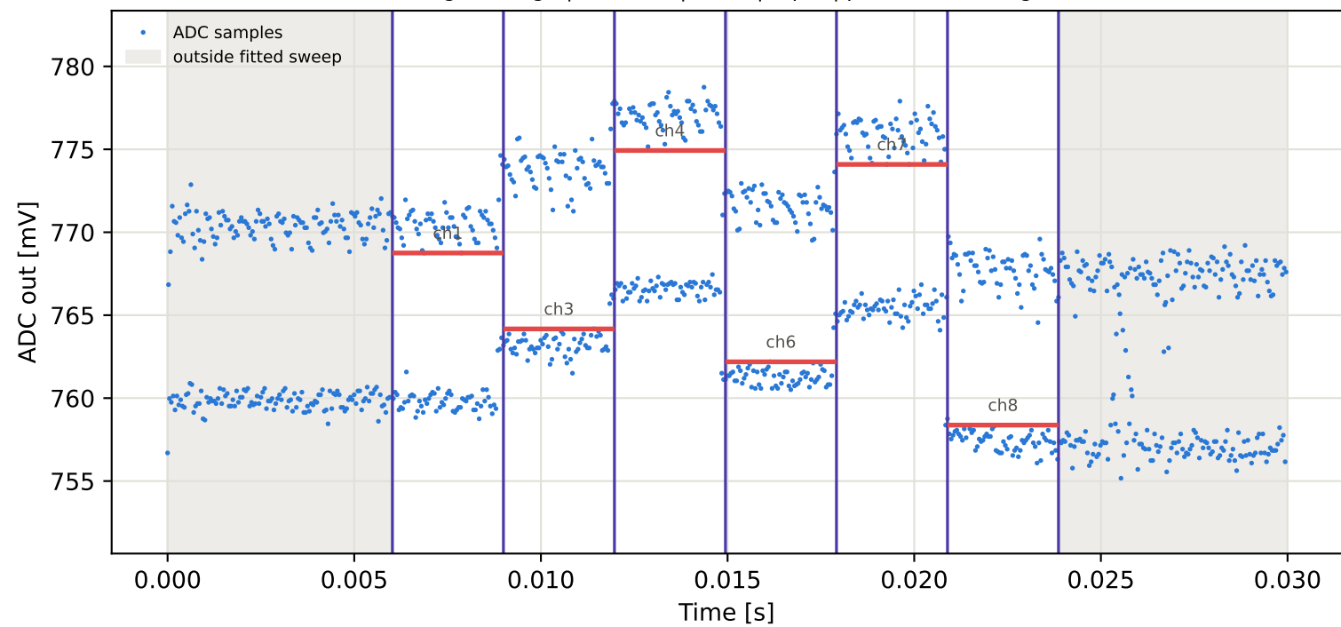
Tag7 &lt;- Tag4 | 885 MHz | run 0 | rep 1 | phase 52.18 deg
