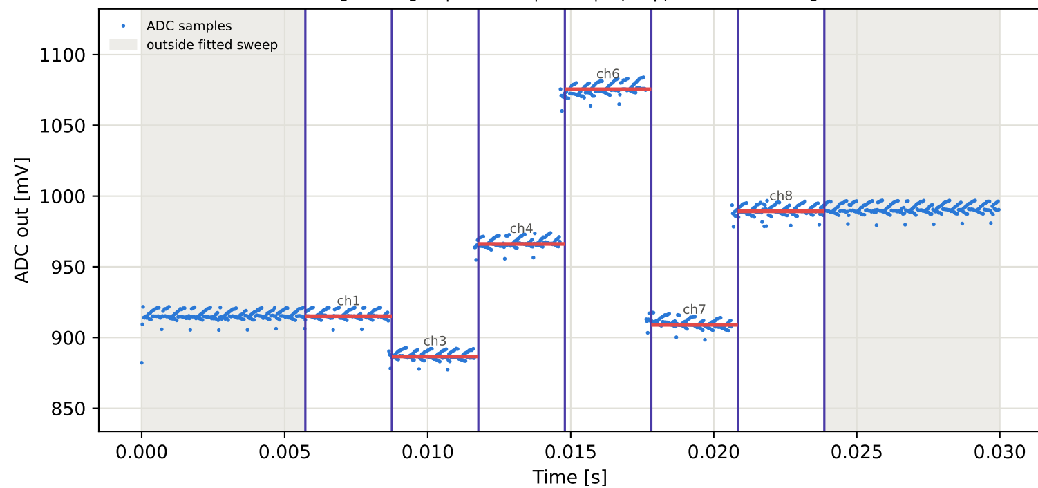
Tag8 &lt;- Tag16 | 965 MHz | run 0 | rep 1 | phase -166.61 deg
