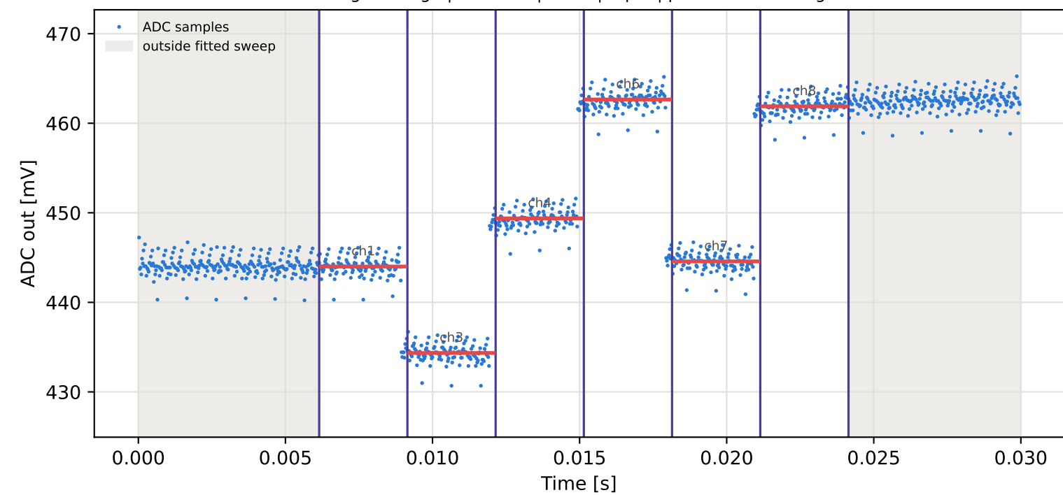
Tag3 &lt;- Tag7 | 855 MHz | run 0 | rep 1 | phase 28.27 deg
