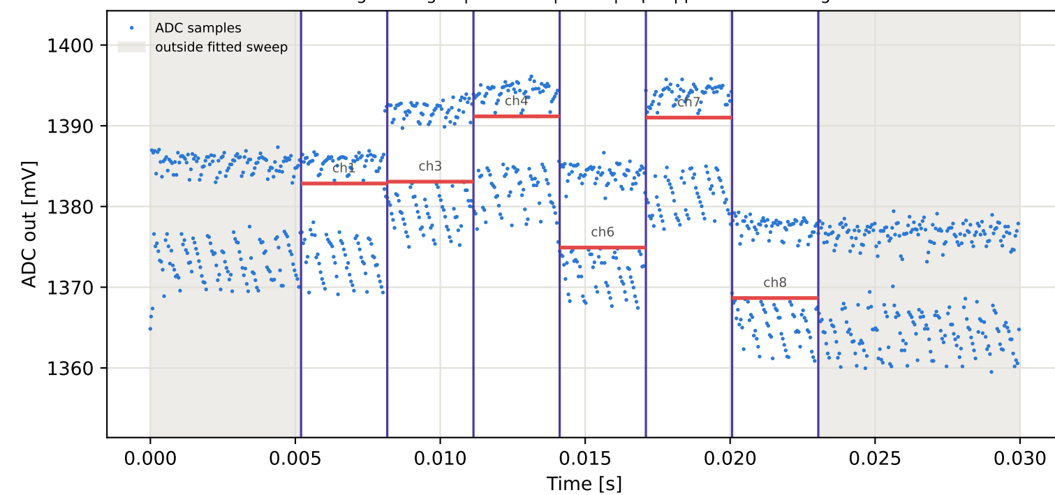
Tag5 &lt;- Tag3 | 885 MHz | run 0 | rep 1 | phase -59.83 deg
