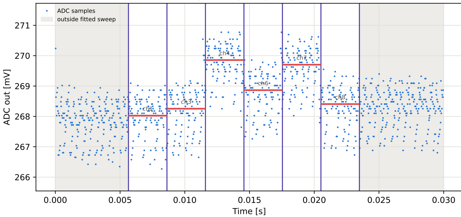
Tag15 &lt;- Tag10 | 795 MHz | run 0 | rep 1 | phase -90.43 deg
