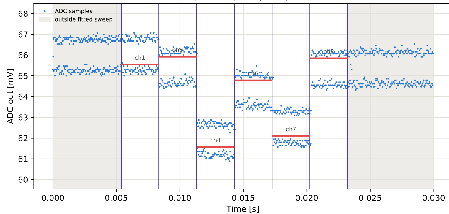
Tag10 &lt;- Tag2 | 795 MHz | run 0 | rep 1 | phase 9.58 deg
