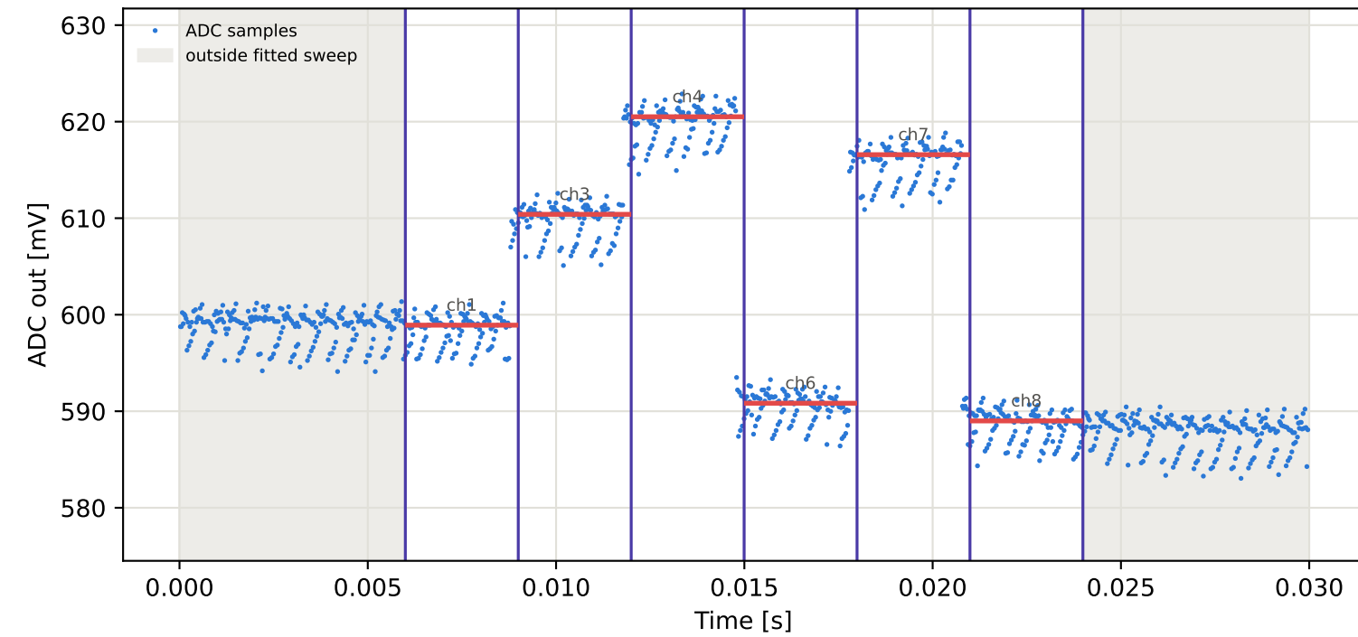
Tag5 &lt;- Tag3 | 935 MHz | run 0 | rep 1 | phase -5.51 deg
