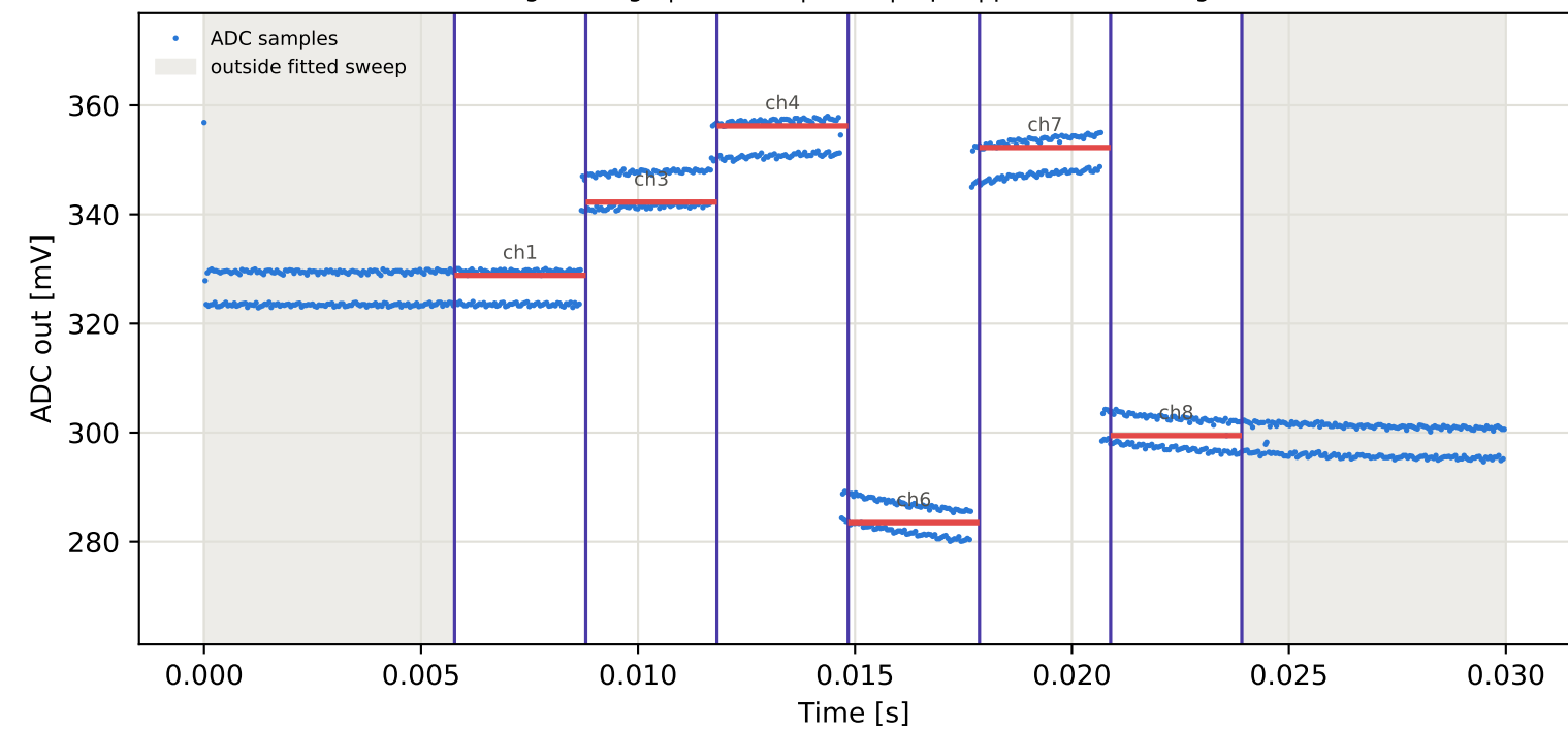
Tag1 &lt;- Tag4 | 935 MHz | run 0 | rep 1 | phase -27.01 deg
