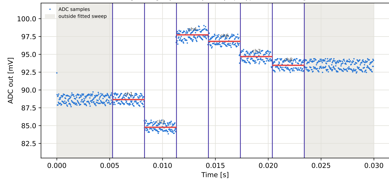
Tag7 &lt;- Tag3 | 795 MHz | run 0 | rep 1 | phase -79.77 deg
