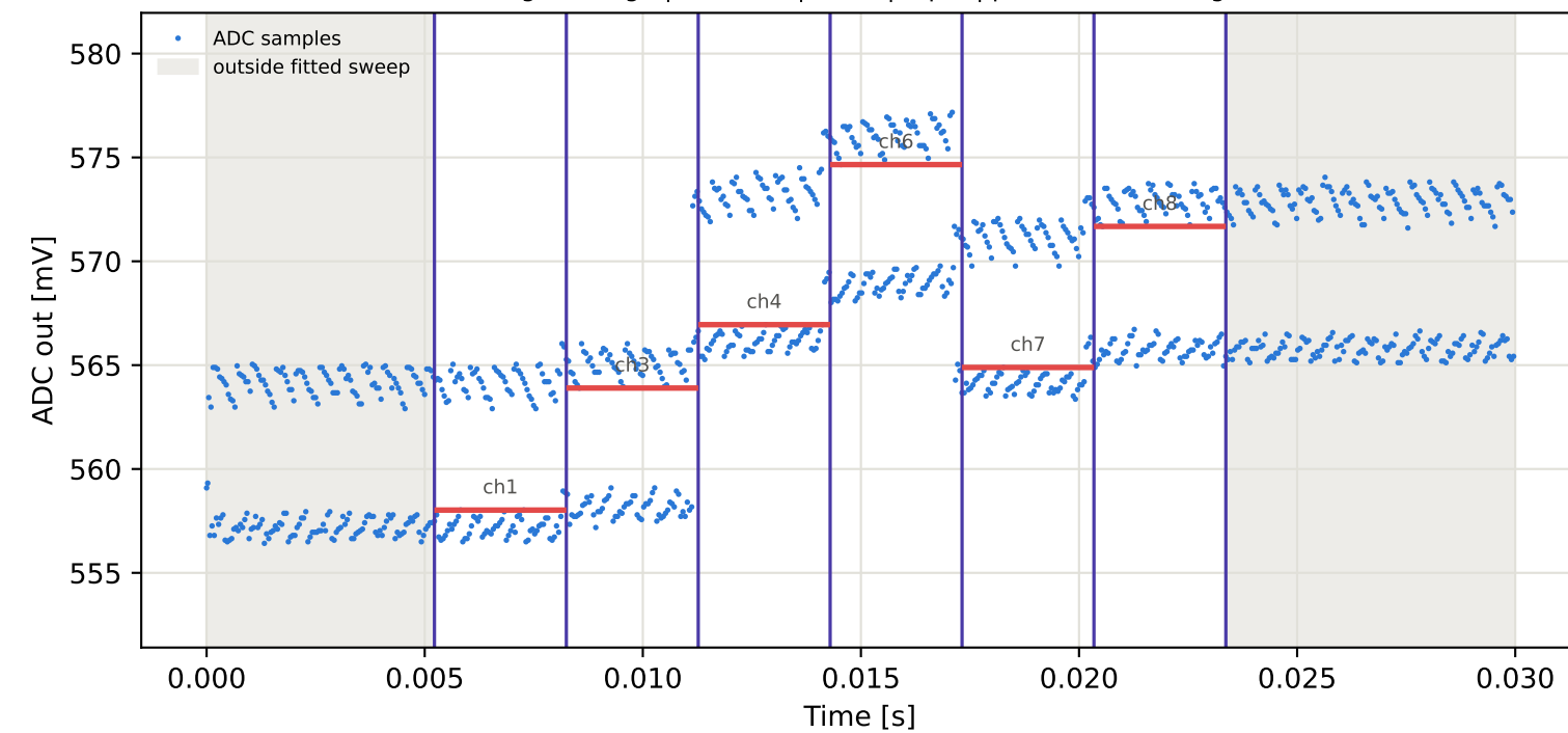
Tag7 &lt;- Tag10 | 865 MHz | run 0 | rep 1 | phase 170.45 deg
