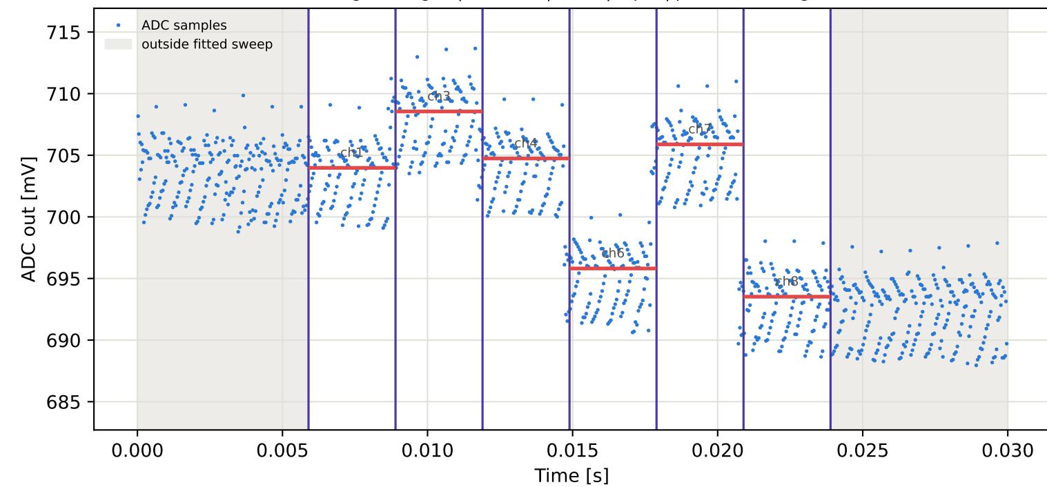
Tag6 &lt;- Tag2 | 875 MHz | run 0 | rep 1 | phase 47.79 deg
