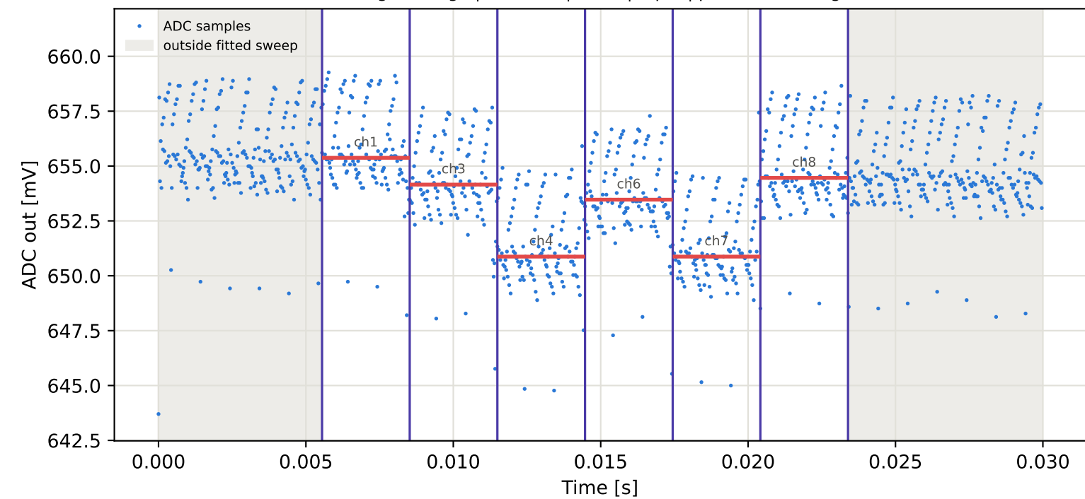
Tag8 &lt;- Tag15 | 825 MHz | run 0 | rep 1 | phase 92.43 deg
