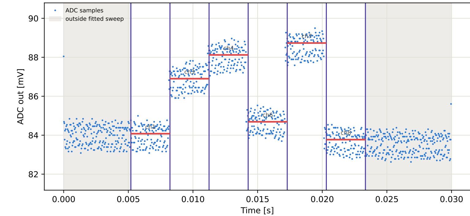
Tag1 &lt;- Tag9 | 795 MHz | run 0 | rep 1 | phase 144.68 deg
