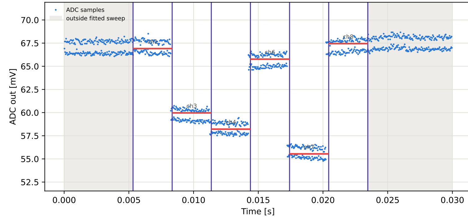
Tag5 &lt;- Tag3 | 795 MHz | run 0 | rep 1 | phase 99.75 deg
