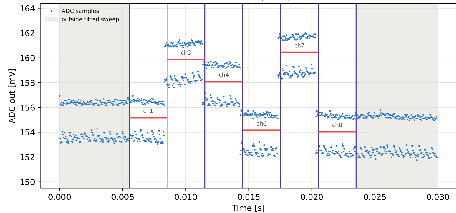
Tag4 &lt;- Tag16 | 795 MHz | run 0 | rep 1 | phase 144.96 deg
