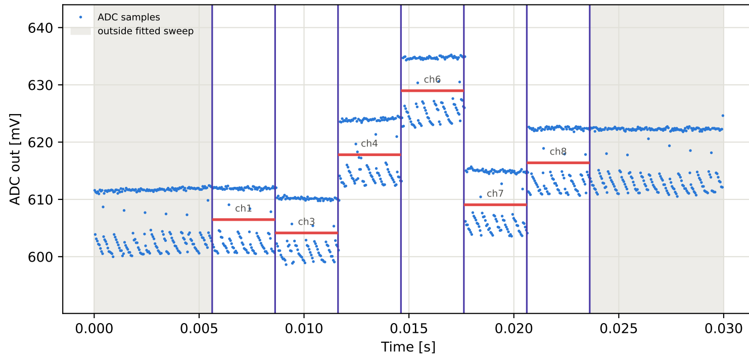
Tag16 &lt;- Tag10 | 985 MHz | run 0 | rep 1 | phase 151.22 deg
