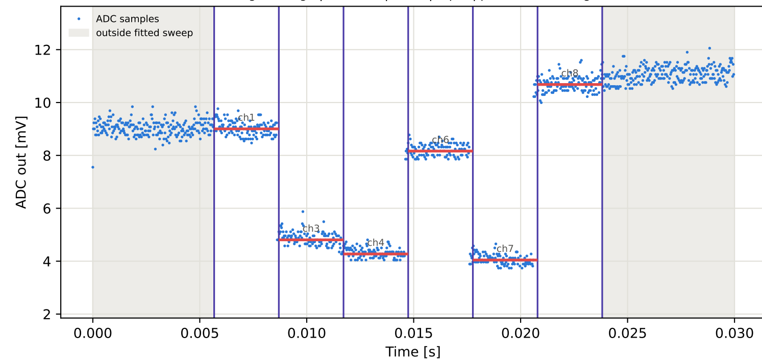
Tag1 &lt;- Tag9 | 875 MHz | run 0 | rep 1 | phase 45.79 deg
