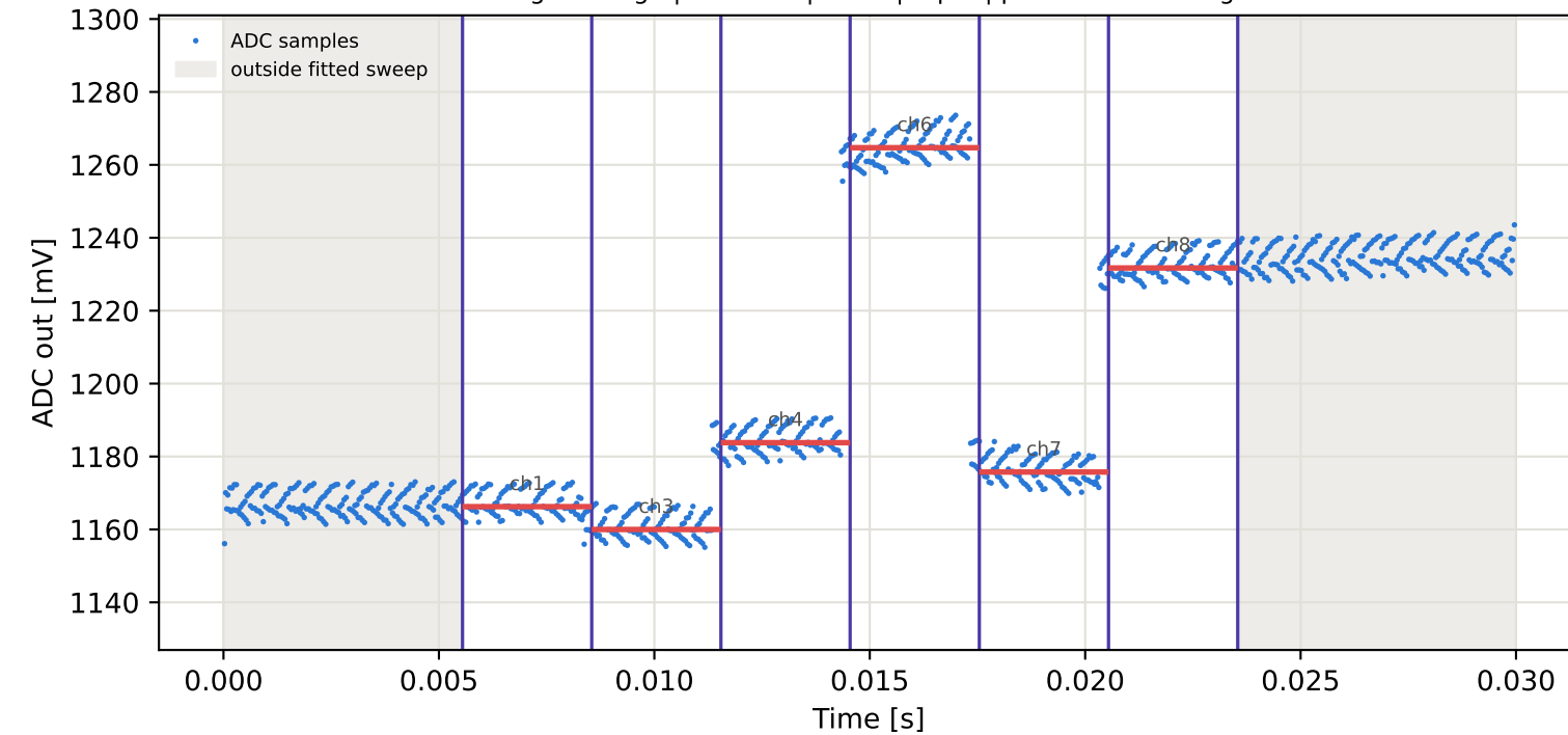
Tag4 &lt;- Tag9 | 905 MHz | run 0 | rep 1 | phase -169.97 deg
