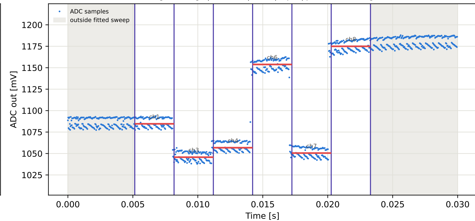
Tag16 &lt;- Tag1 | 885 MHz | run 0 | rep 1 | phase 16.63 deg
