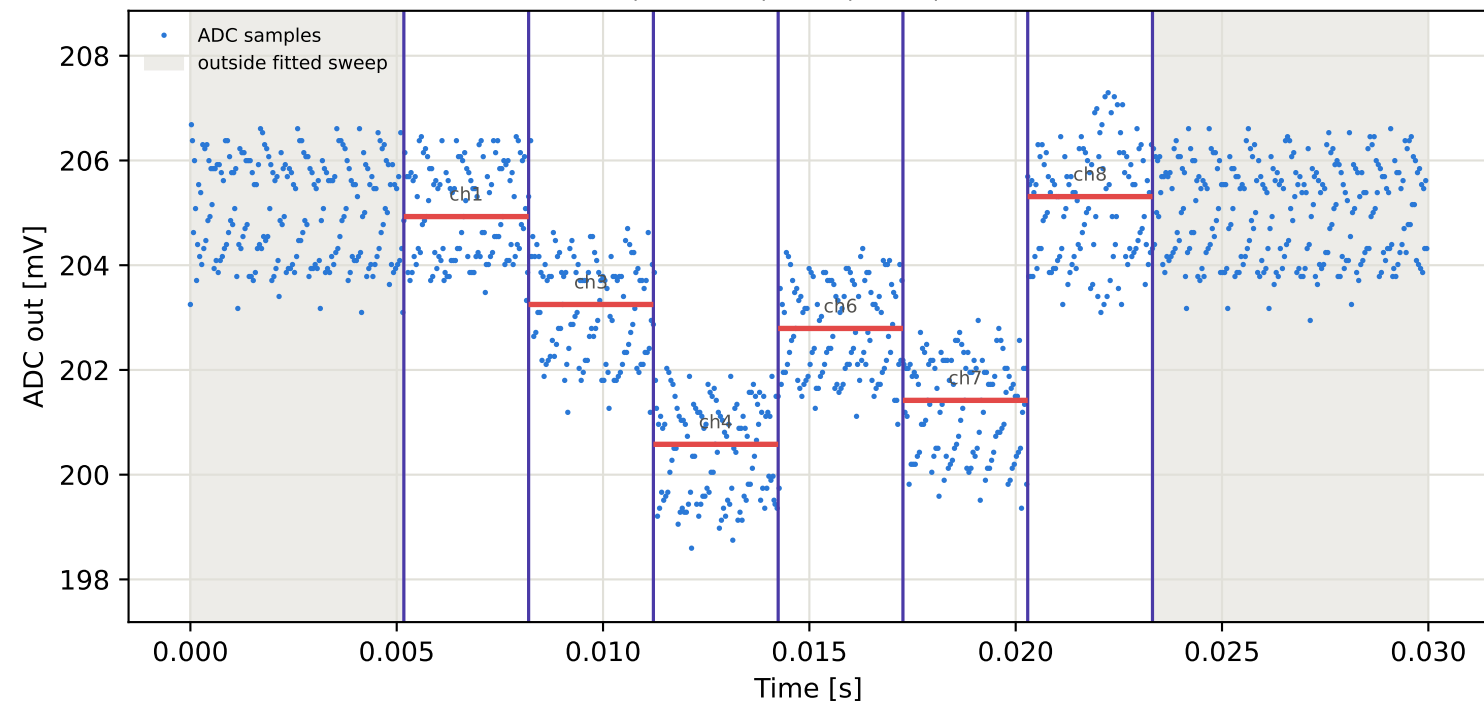
Tag4 &lt;- Tag2 | 775 MHz | run 0 | rep 1 | phase 97.22 deg
