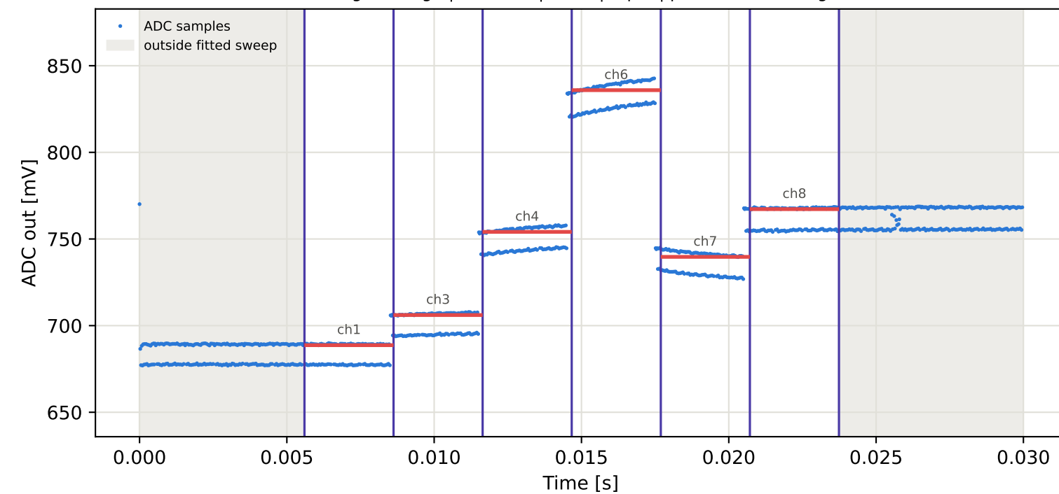
Tag3 &lt;- Tag8 | 895 MHz | run 0 | rep 1 | phase -151.21 deg
