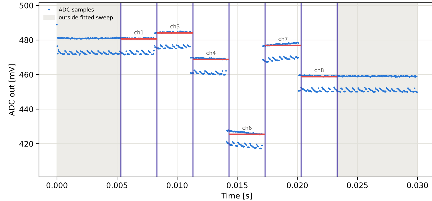
Tag7 &lt;- Tag10 | 935 MHz | run 0 | rep 1 | phase 174.87 deg
