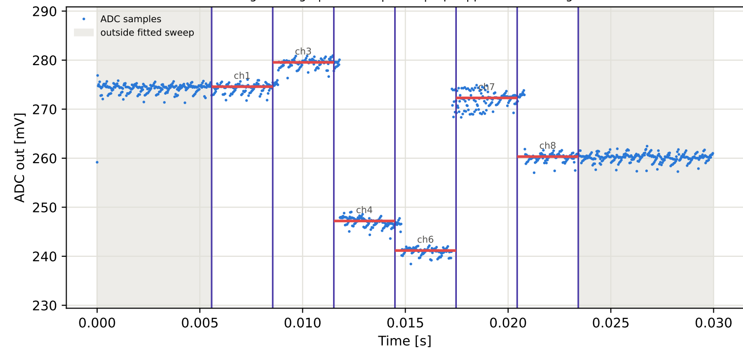
Tag9 &lt;- Tag6 | 995 MHz | run 0 | rep 1 | phase 125.74 deg
