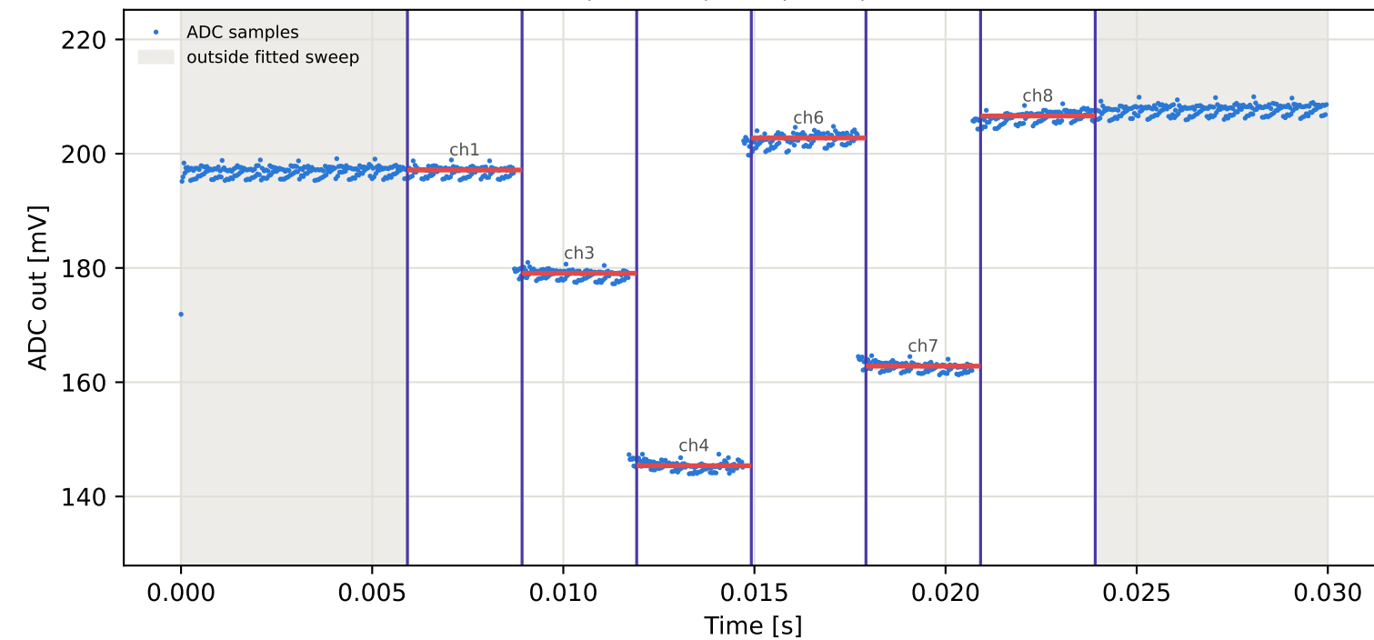
Tag5 &lt;- Tag3 | 965 MHz | run 0 | rep 1 | phase 102.22 deg
