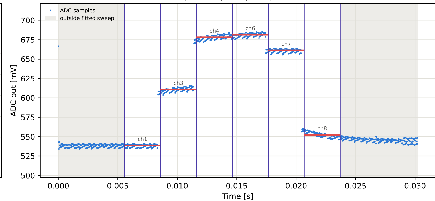
Tag9 &lt;- Tag6 | 895 MHz | run 0 | rep 1 | phase 141.25 deg
