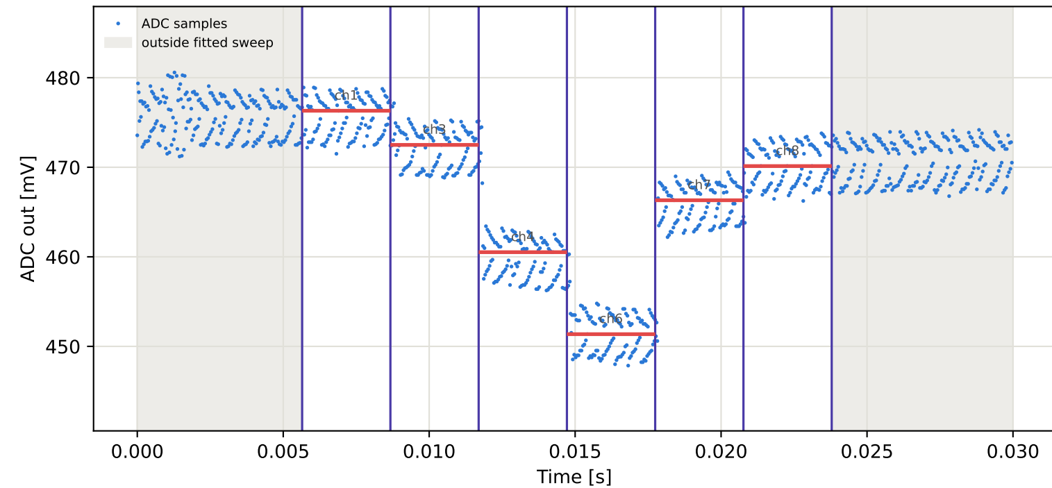
Tag6 &lt;- Tag5 | 935 MHz | run 0 | rep 1 | phase -23.73 deg
