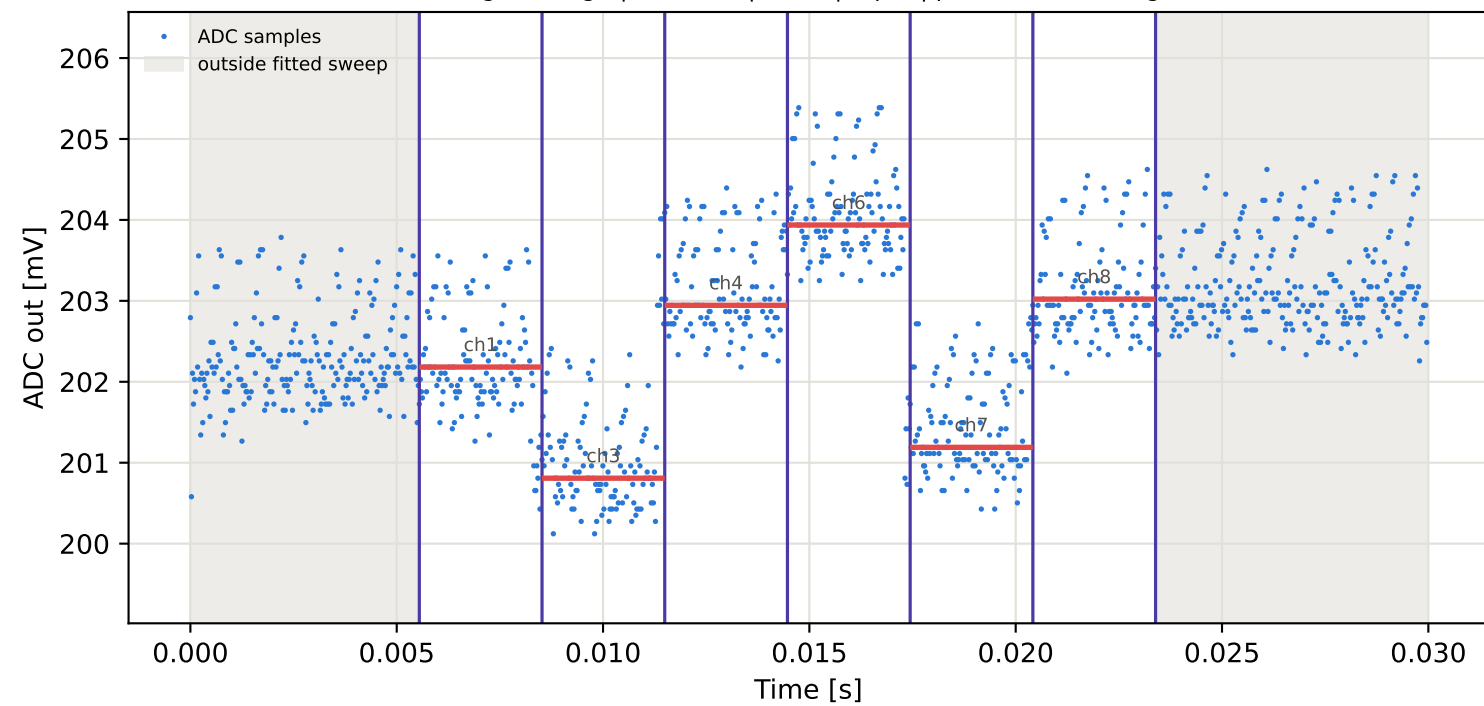
Tag4 &lt;- Tag15 | 775 MHz | run 0 | rep 1 | phase -56.92 deg
