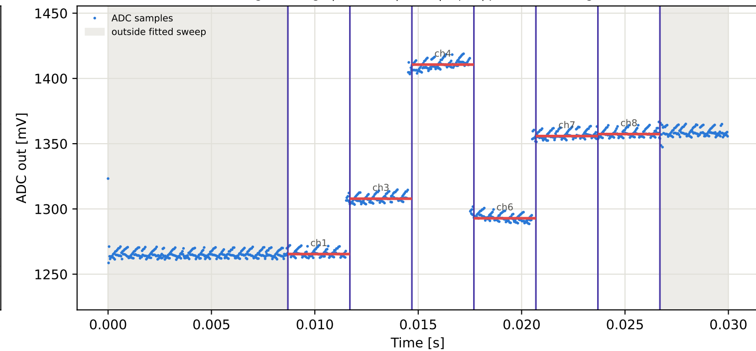
Tag16 &lt;- Tag1 | 895 MHz | run 0 | rep 1 | phase 132.62 deg
