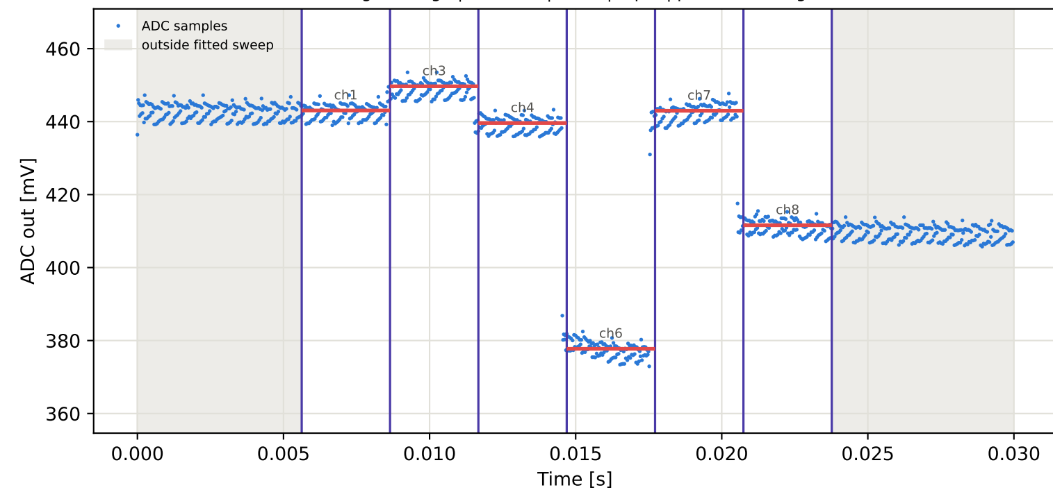
Tag2 &lt;- Tag8 | 915 MHz | run 0 | rep 1 | phase 6.19 deg
