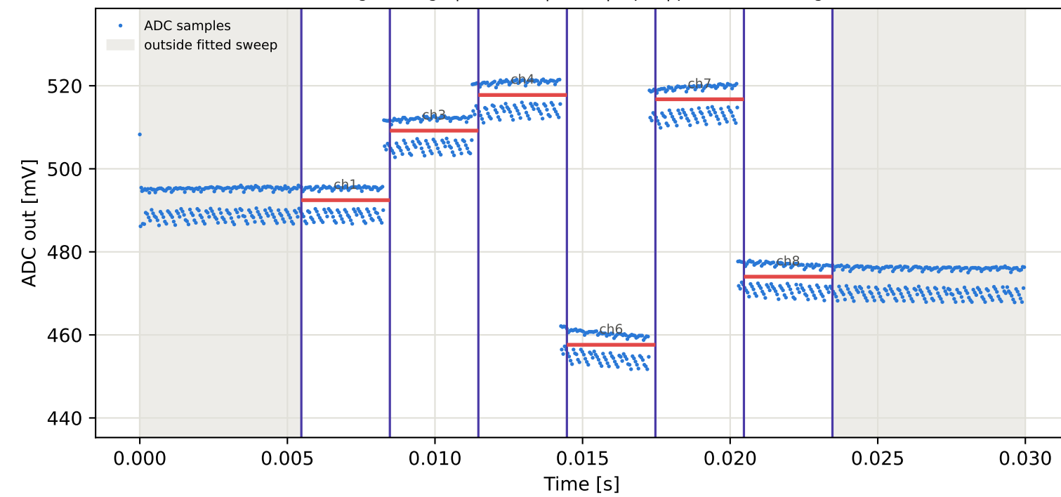
Tag3 &lt;- Tag6 | 975 MHz | run 0 | rep 1 | phase 48.09 deg
