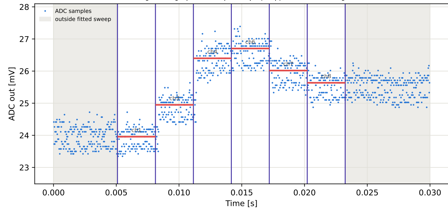
Tag1 &lt;- Tag4 | 855 MHz | run 0 | rep 1 | phase -124.57 deg
