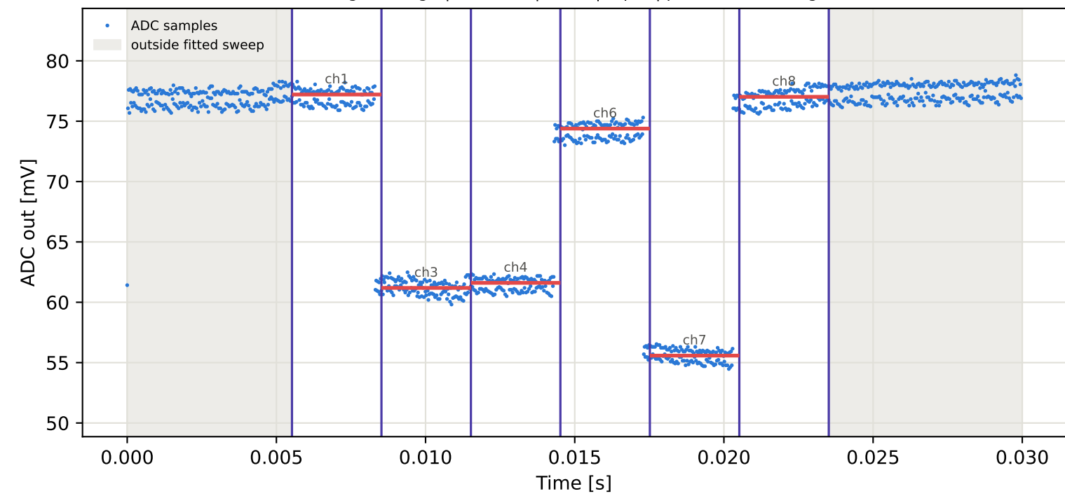
Tag9 &lt;- Tag6 | 805 MHz | run 0 | rep 1 | phase -67.73 deg
