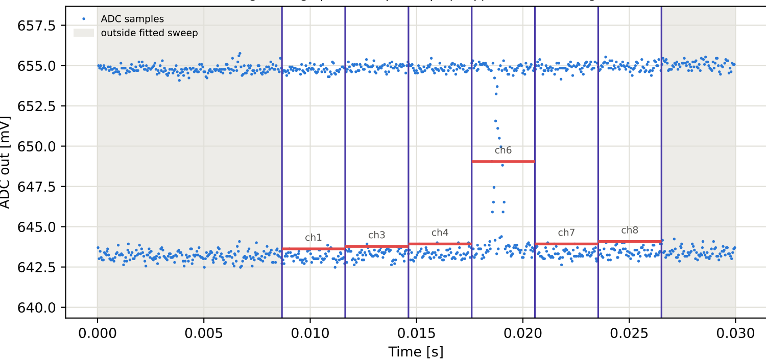
Tag6 &lt;- Tag4 | 955 MHz | run 0 | rep 1 | phase -71.84 deg
