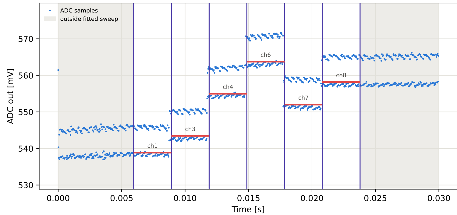
Tag10 &lt;- Tag2 | 875 MHz | run 0 | rep 1 | phase -32.27 deg
