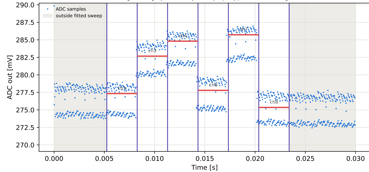
Tag3 &lt;- Tag9 | 835 MHz | run 0 | rep 1 | phase -52.78 deg
