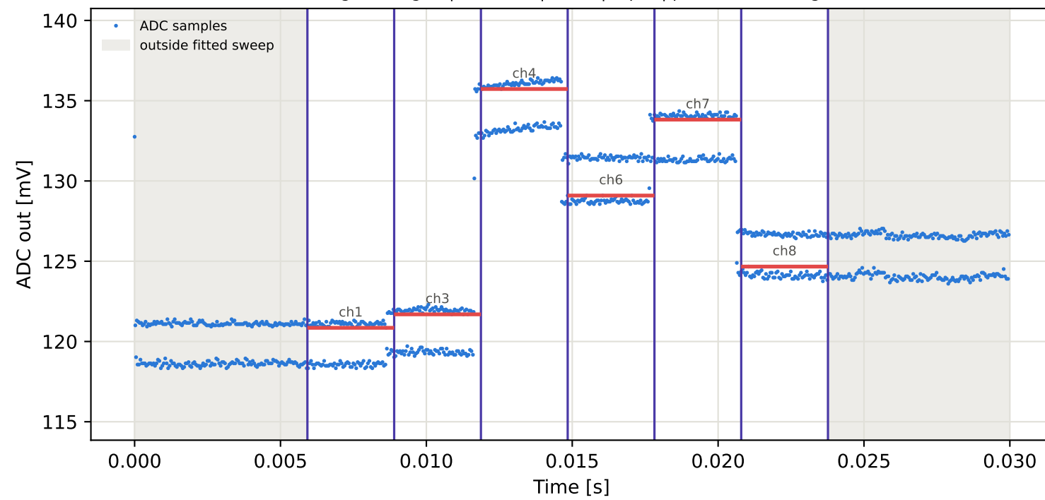
Tag1 &lt;- Tag16 | 805 MHz | run 0 | rep 1 | phase 87.27 deg
