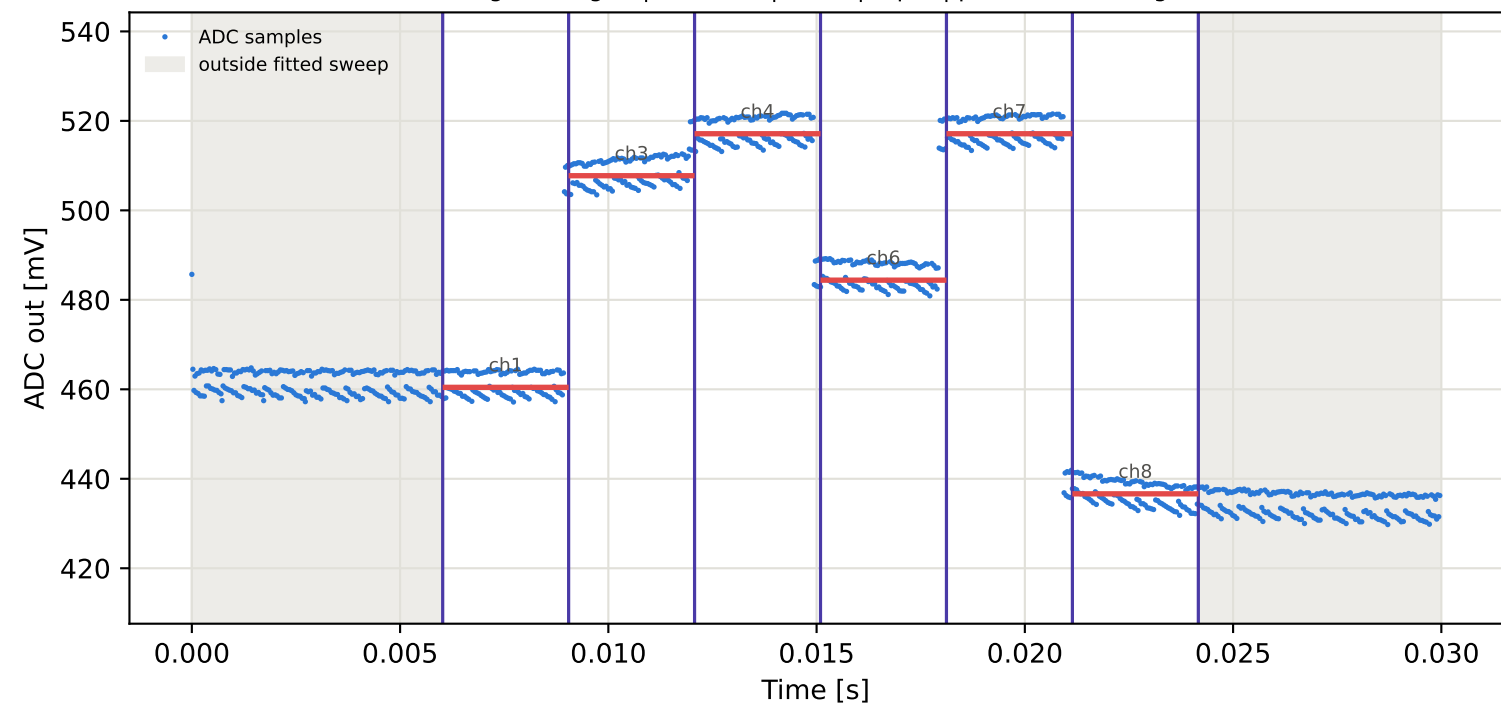
Tag4 &lt;- Tag3 | 865 MHz | run 0 | rep 1 | phase 43.41 deg
