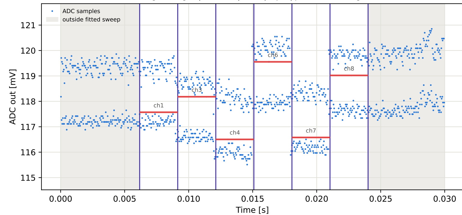
Tag5 &lt;- Tag16 | 995 MHz | run 0 | rep 1 | phase 87.93 deg
