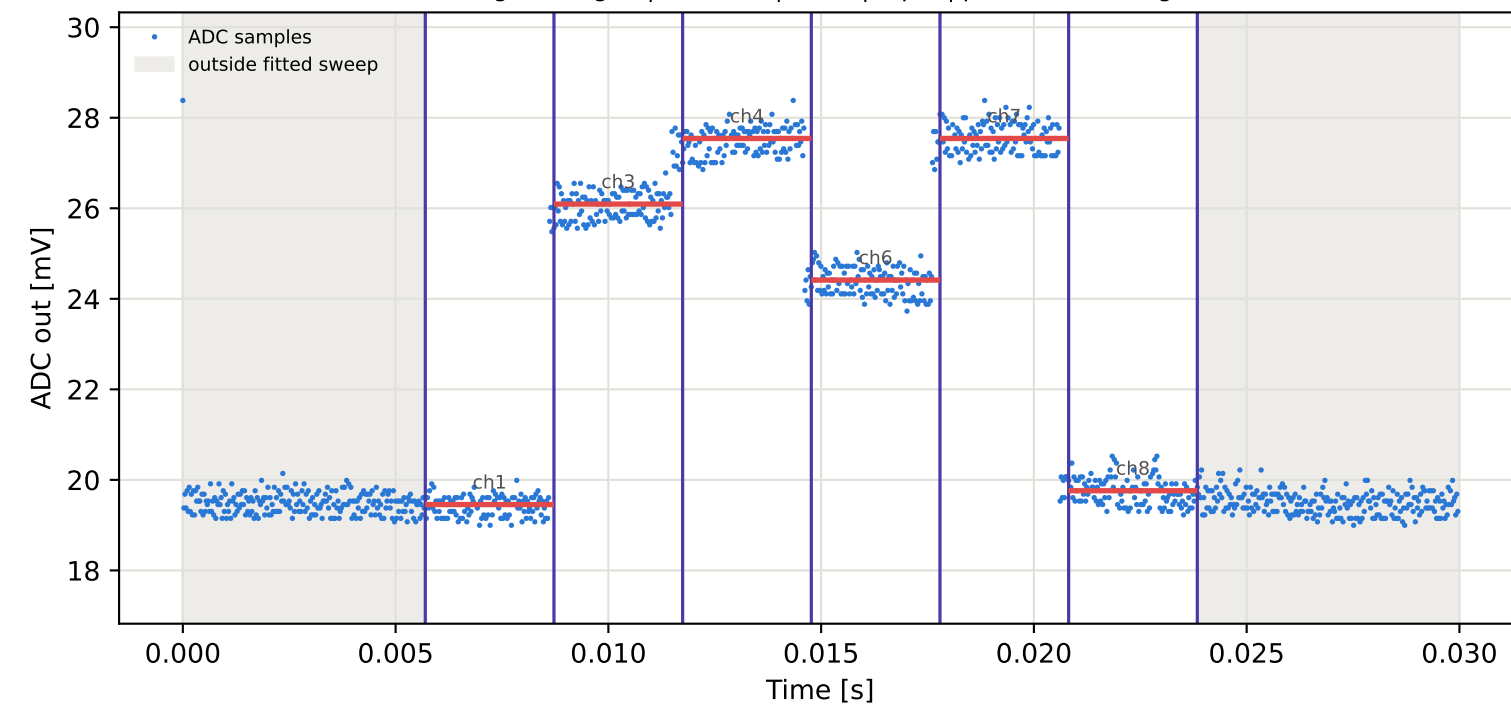
Tag1 &lt;- Tag3 | 855 MHz | run 0 | rep 1 | phase 46.06 deg
