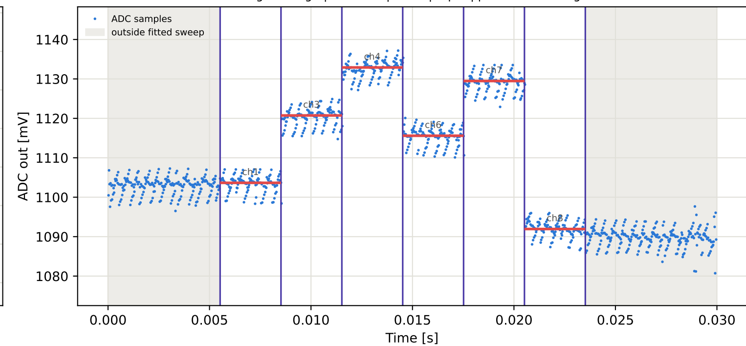
Tag4 &lt;- Tag8 | 895 MHz | run 0 | rep 1 | phase -119.85 deg
