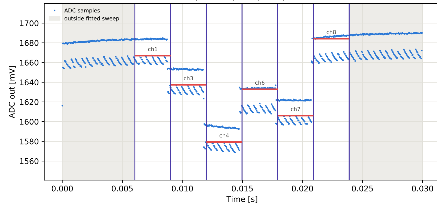
Tag15 &lt;- Tag3 | 935 MHz | run 0 | rep 1 | phase -165.02 deg
