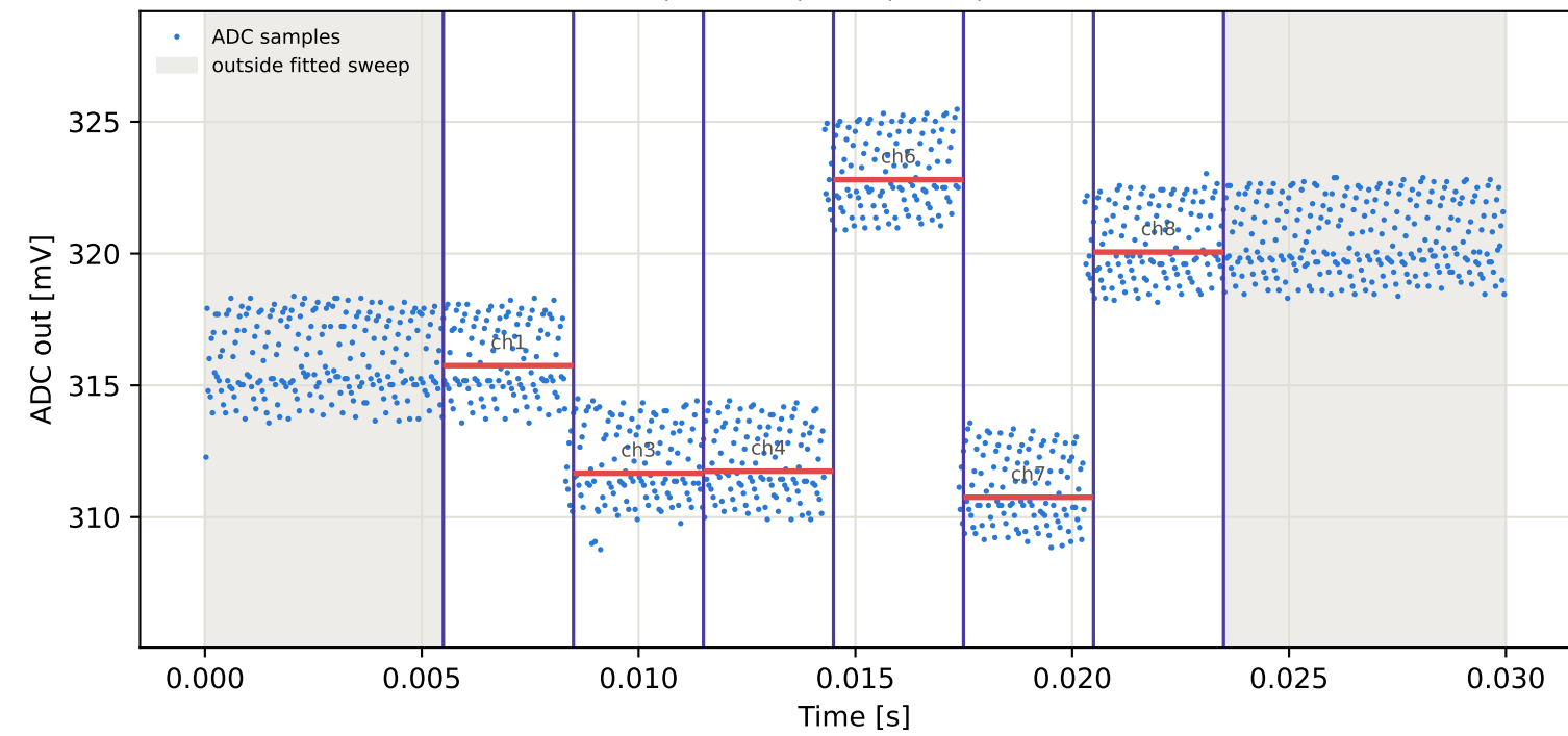
Tag3 &lt;- Tag9 | 995 MHz | run 0 | rep 1 | phase 154.36 deg
