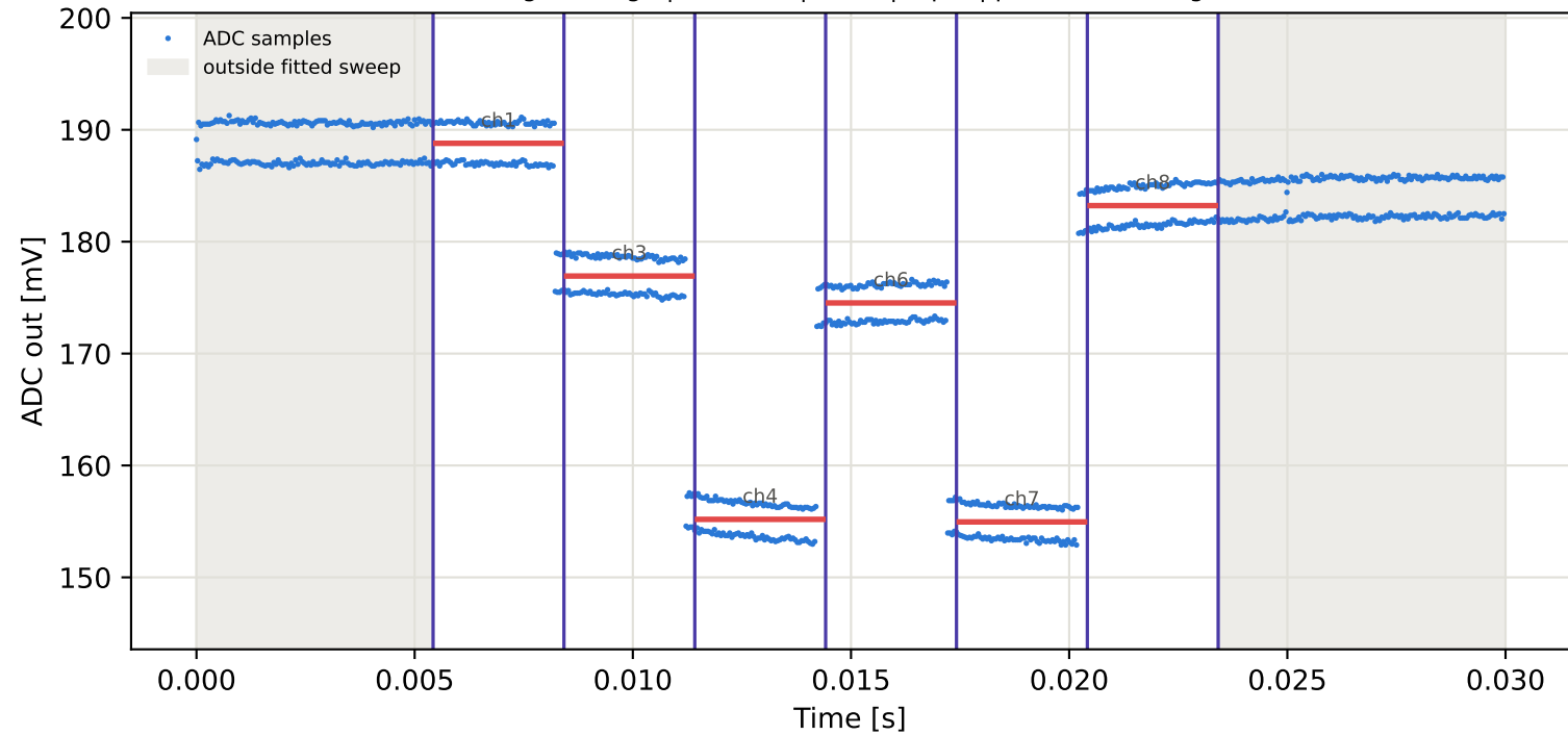
Tag5 &lt;- Tag1 | 795 MHz | run 0 | rep 1 | phase -51.03 deg
