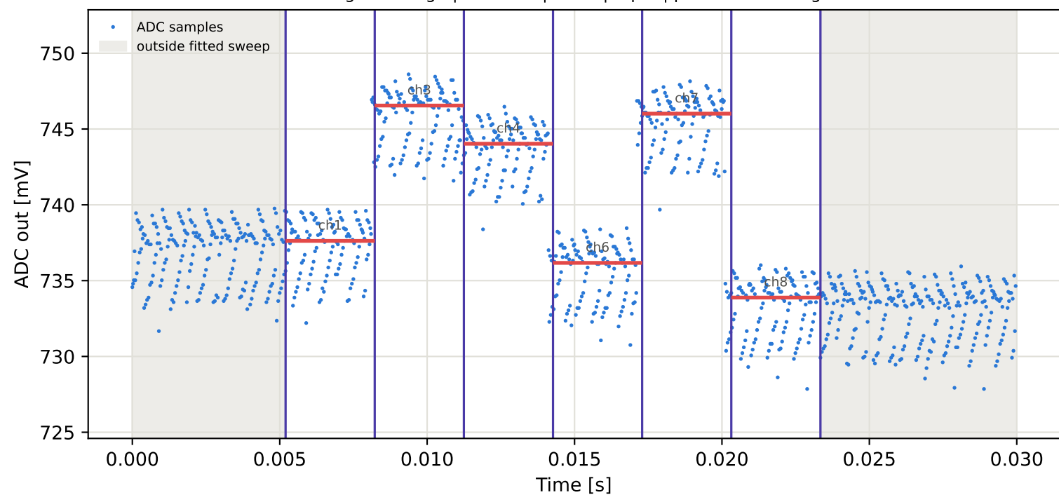
Tag2 &lt;- Tag10 | 865 MHz | run 0 | rep 1 | phase -94.56 deg
