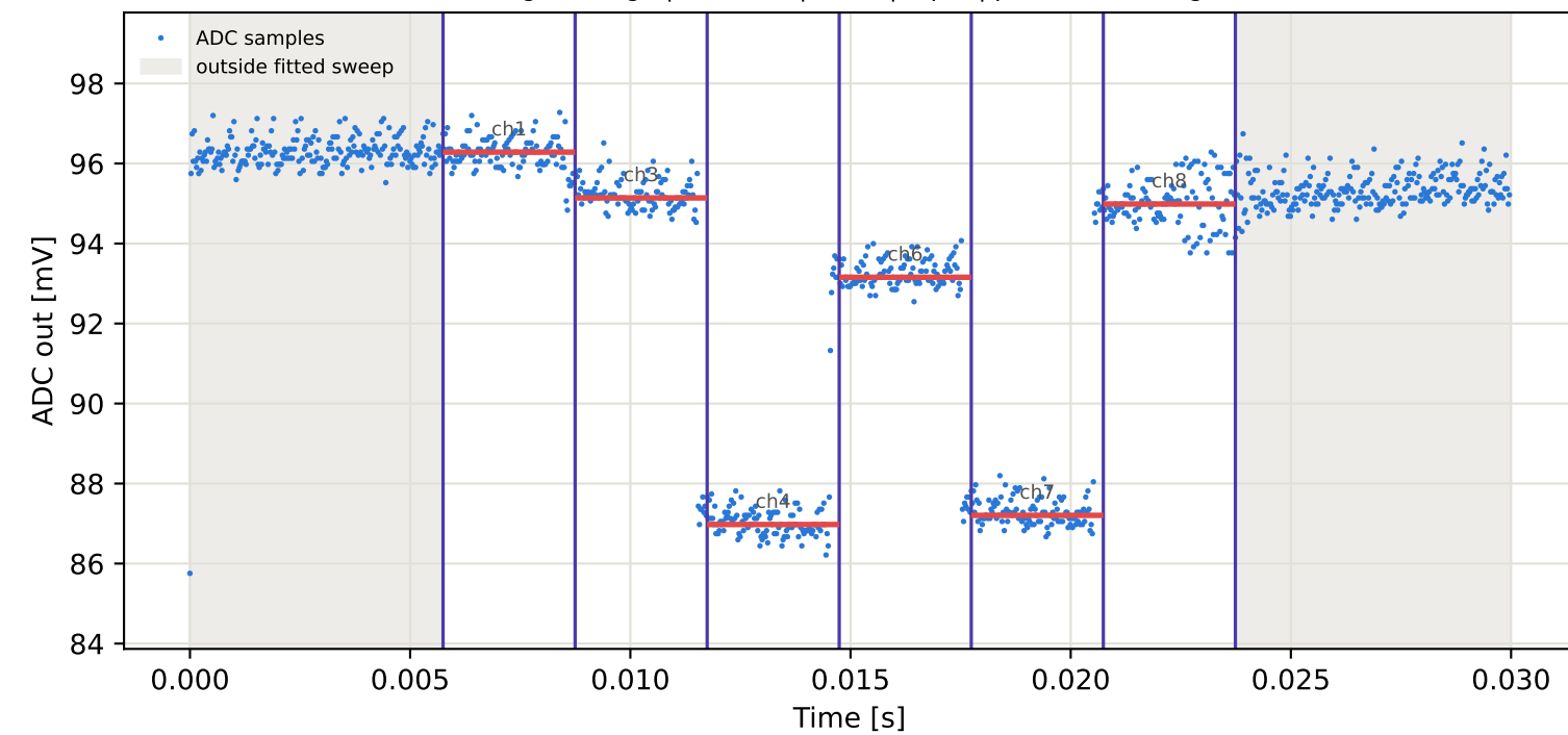
Tag9 &lt;- Tag5 | 775 MHz | run 0 | rep 1 | phase -24.00 deg
