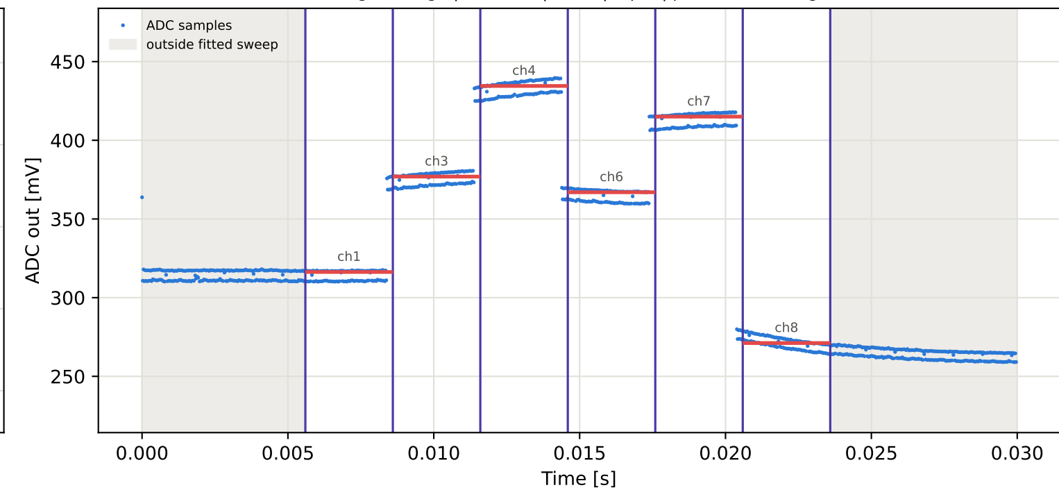
Tag9 &lt;- Tag6 | 915 MHz | run 0 | rep 1 | phase -147.91 deg
