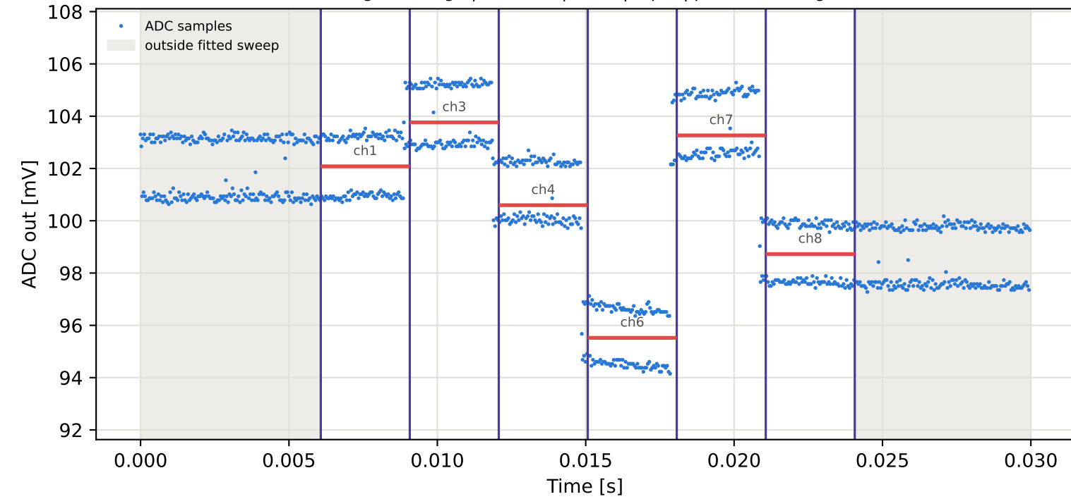
Tag15 &lt;- Tag1 | 995 MHz | run 0 | rep 1 | phase 76.82 deg
