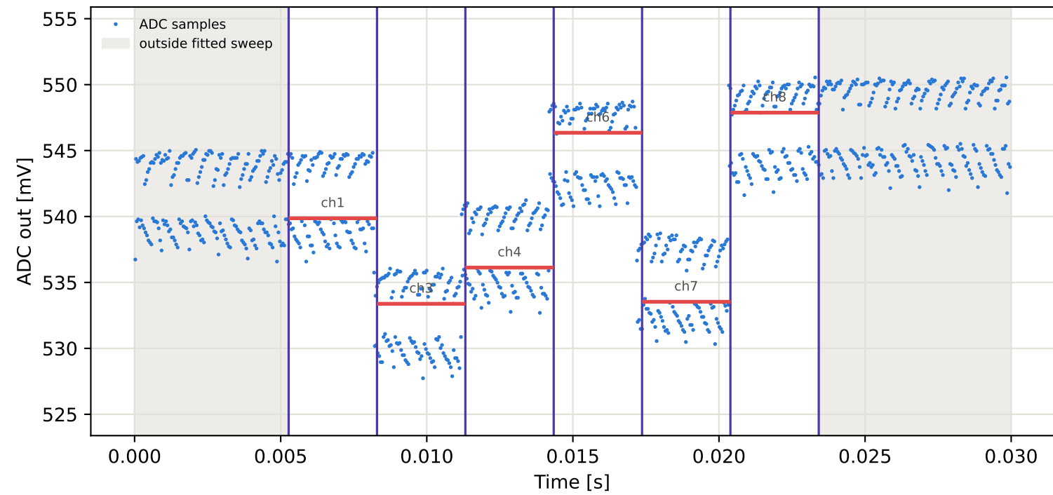
Tag4 &lt;- Tag16 | 845 MHz | run 0 | rep 1 | phase -95.29 deg
