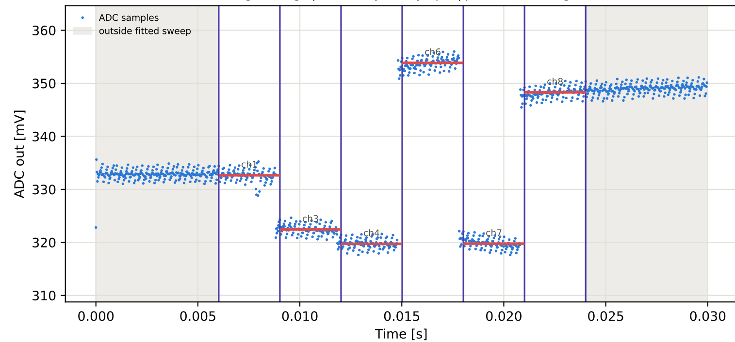
Tag3 &lt;- Tag15 | 925 MHz | run 0 | rep 1 | phase 48.38 deg
