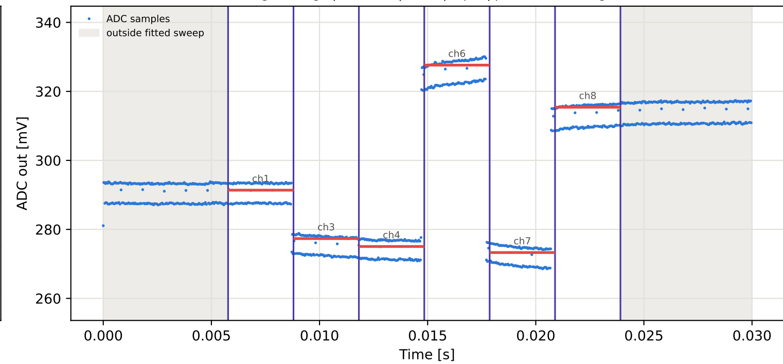
Tag3 &lt;- Tag15 | 935 MHz | run 0 | rep 1 | phase 76.09 deg
