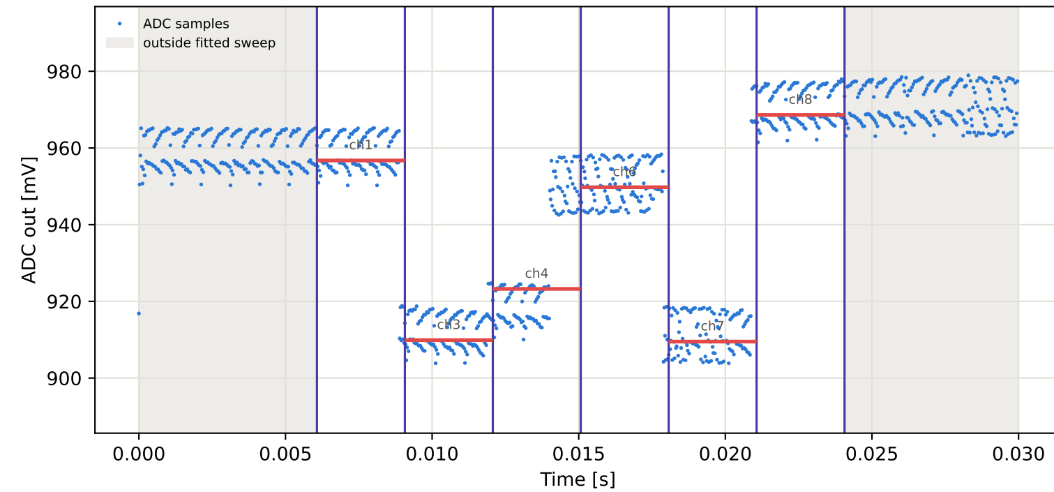
Tag16 &lt;- Tag6 | 845 MHz | run 0 | rep 1 | phase 112.77 deg
