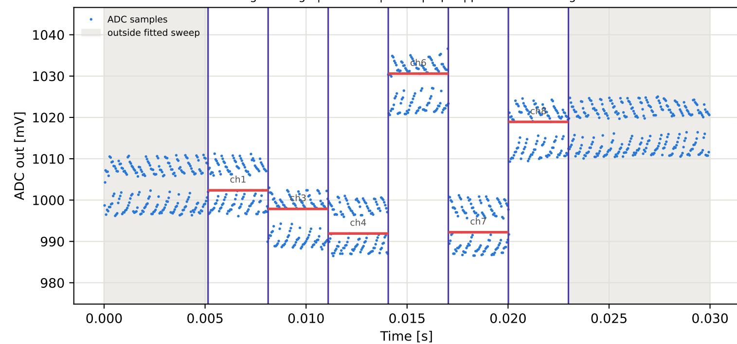
Tag8 &lt;- Tag7 | 945 MHz | run 0 | rep 1 | phase -38.25 deg
