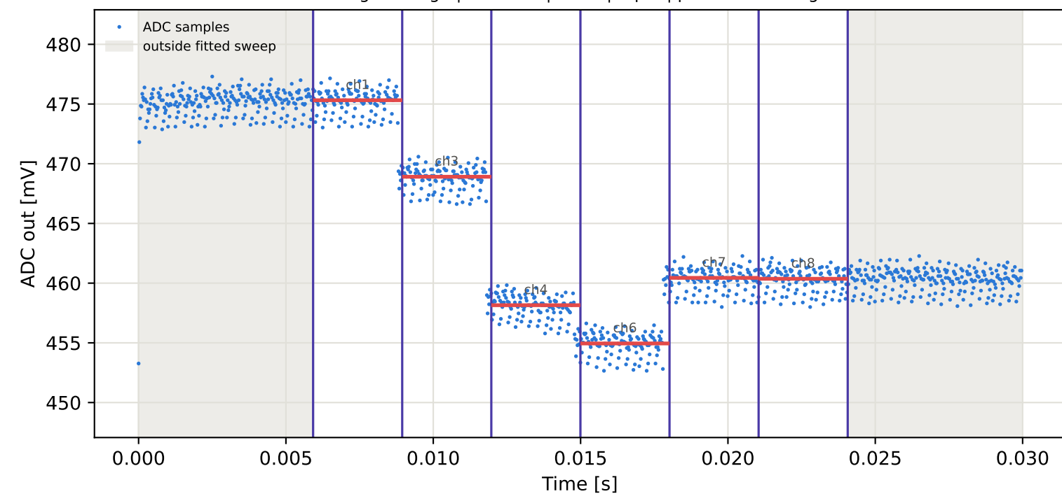
Tag3 &lt;- Tag15 | 865 MHz | run 0 | rep 1 | phase -28.51 deg
