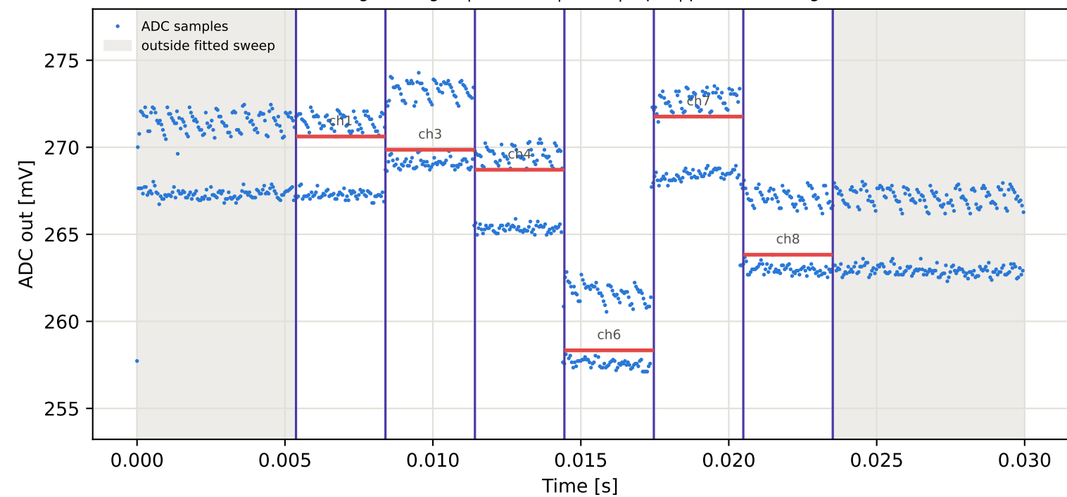
Tag6 &lt;- Tag10 | 985 MHz | run 0 | rep 1 | phase 1.30 deg
