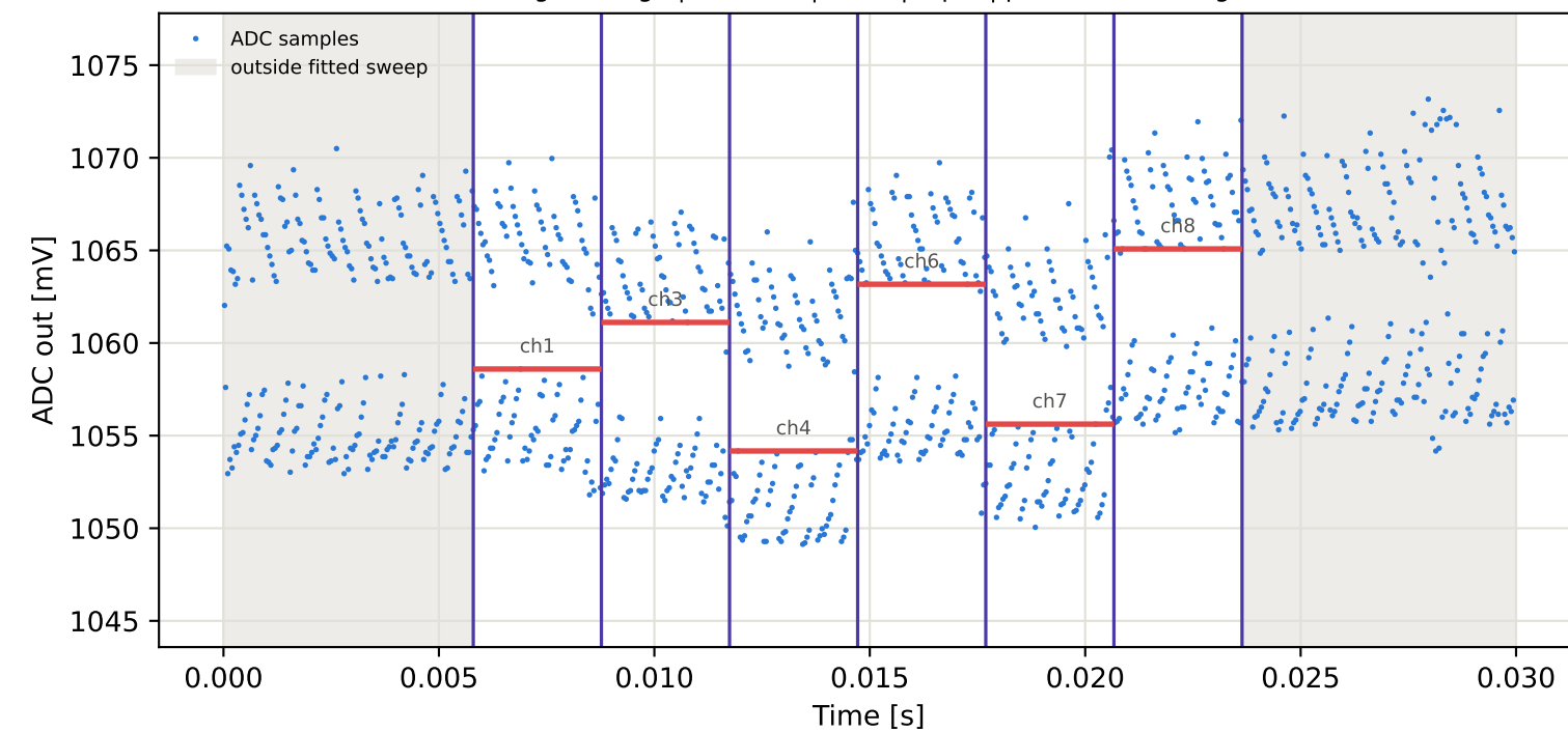
Tag4 &lt;- Tag2 | 945 MHz | run 0 | rep 1 | phase 112.43 deg
