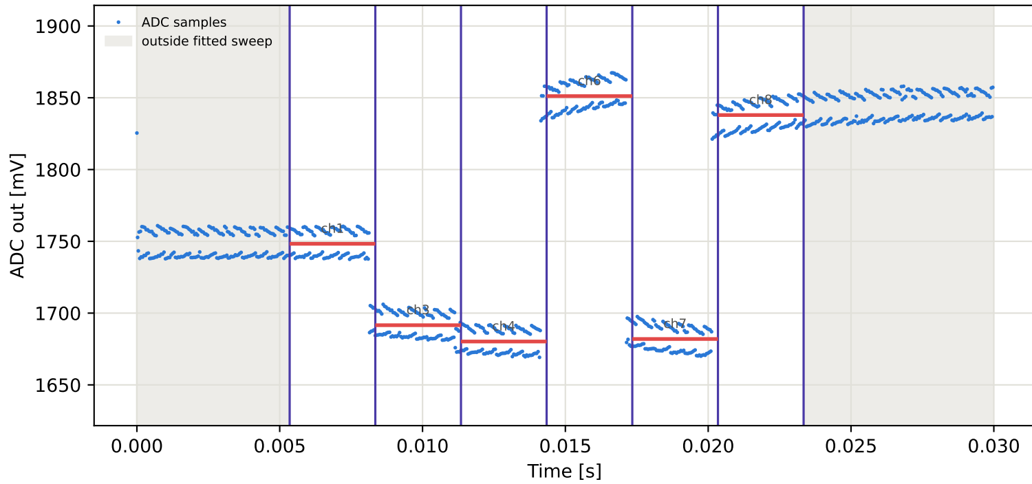
Tag8 &lt;- Tag16 | 905 MHz | run 0 | rep 1 | phase 154.83 deg
