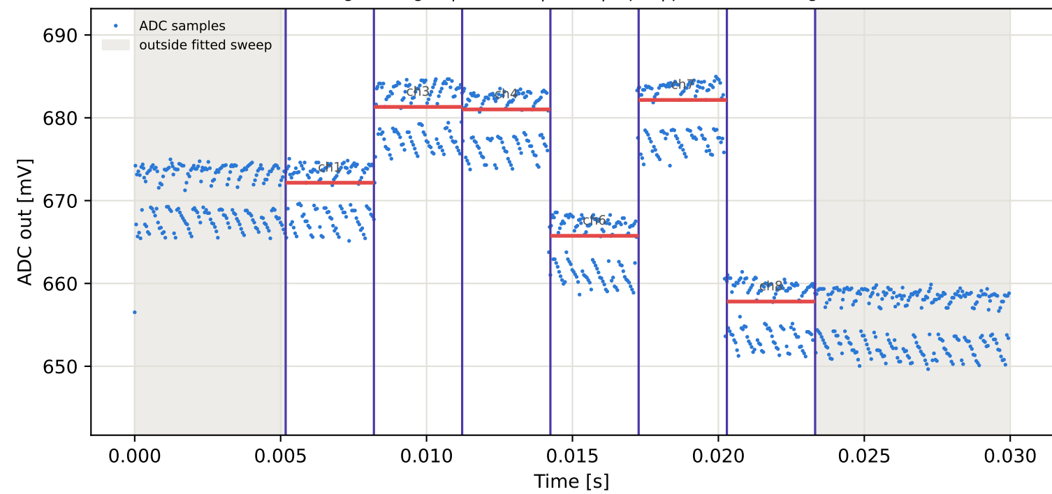
Tag9 &lt;- Tag2 | 885 MHz | run 0 | rep 1 | phase -17.77 deg
