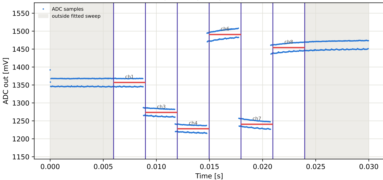
Tag8 &lt;- Tag16 | 935 MHz | run 0 | rep 1 | phase 144.87 deg
