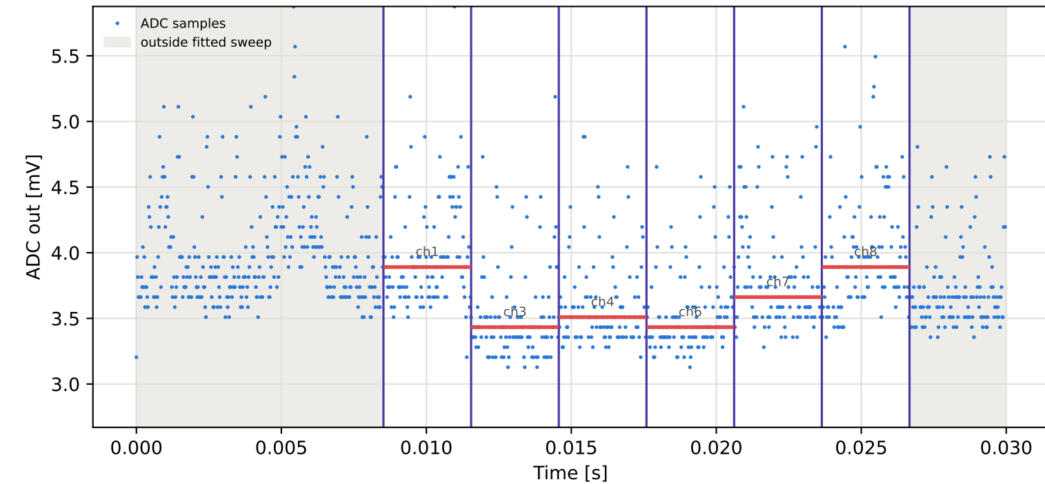
Tag2 &lt;- Tag16 | 795 MHz | run 0 | rep 1 | phase 173.23 deg
