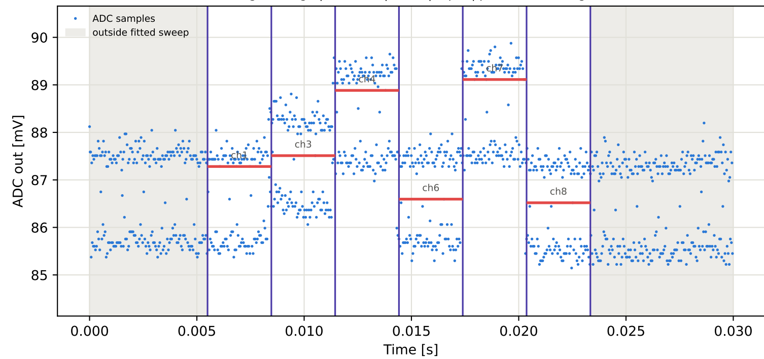
Tag9 &lt;- Tag15 | 775 MHz | run 0 | rep 1 | phase 91.21 deg
