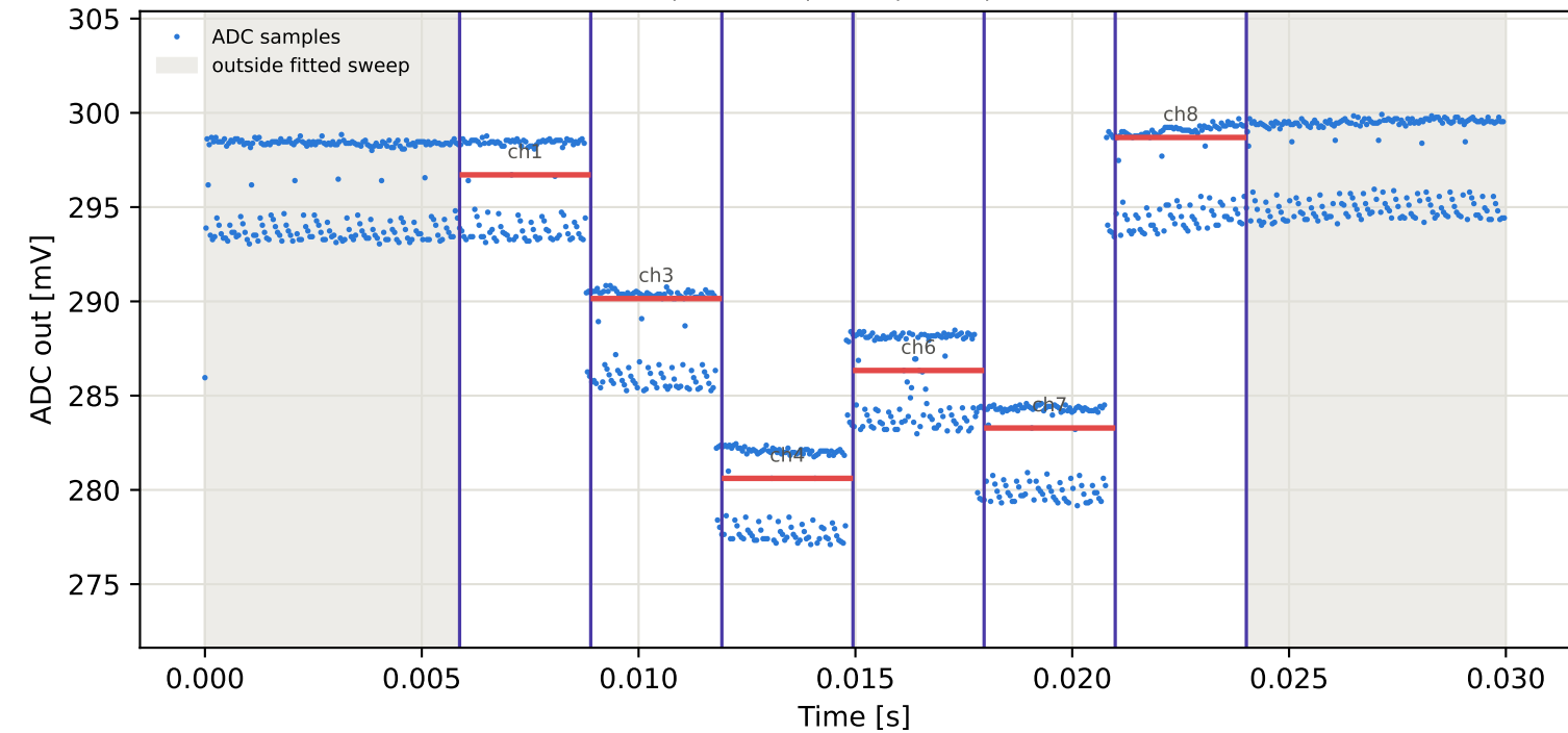
Tag3 &lt;- Tag2 | 835 MHz | run 0 | rep 1 | phase 84.69 deg
