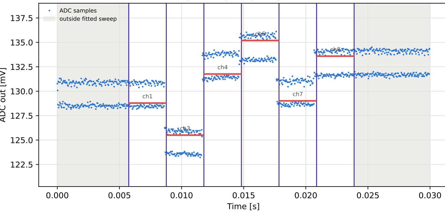
Tag1 &lt;- Tag3 | 805 MHz | run 0 | rep 1 | phase -151.70 deg
