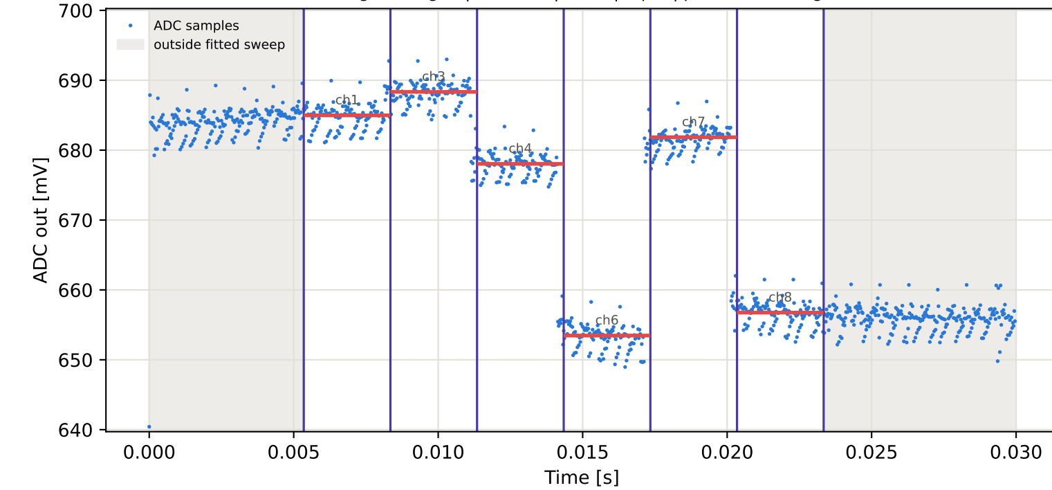
Tag9 &lt;- Tag16 | 885 MHz | run 0 | rep 1 | phase -94.29 deg
