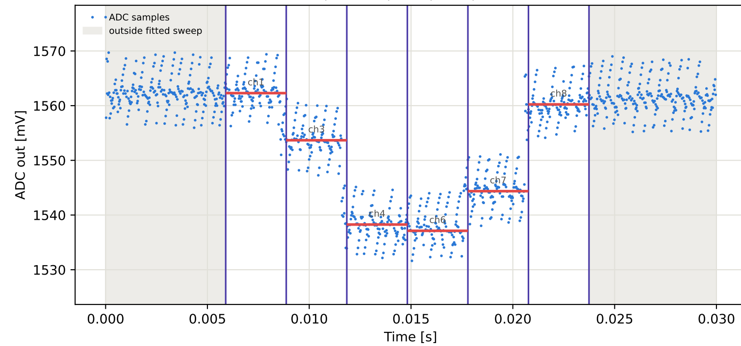
Tag8 &lt;- Tag6 | 915 MHz | run 0 | rep 1 | phase 58.19 deg
