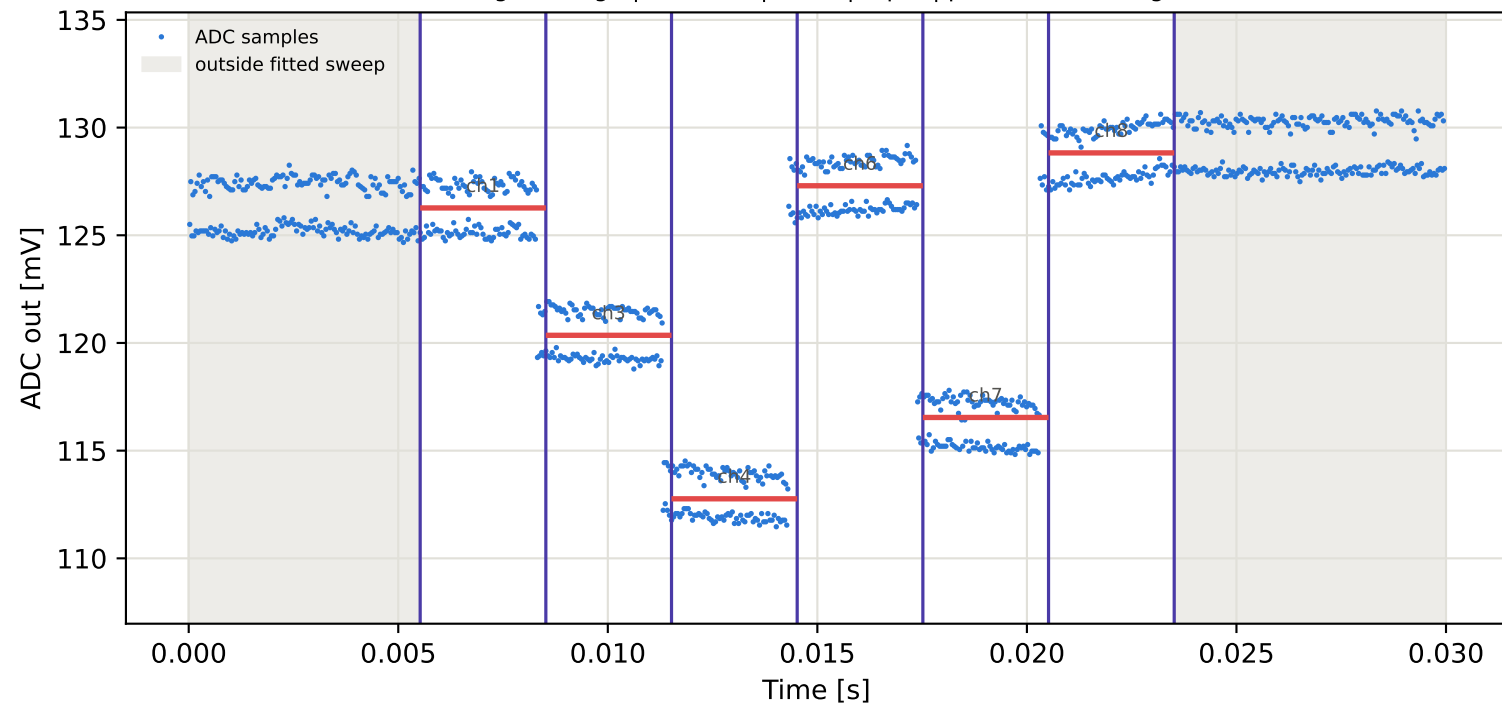
Tag6 &lt;- Tag10 | 995 MHz | run 0 | rep 1 | phase -8.52 deg
