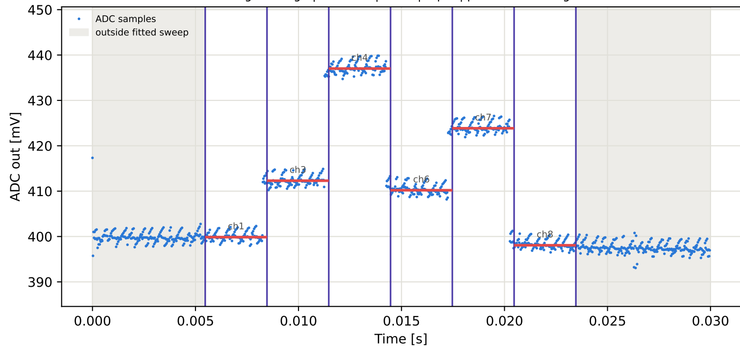
Tag9 &lt;- Tag15 | 985 MHz | run 0 | rep 1 | phase 56.52 deg
