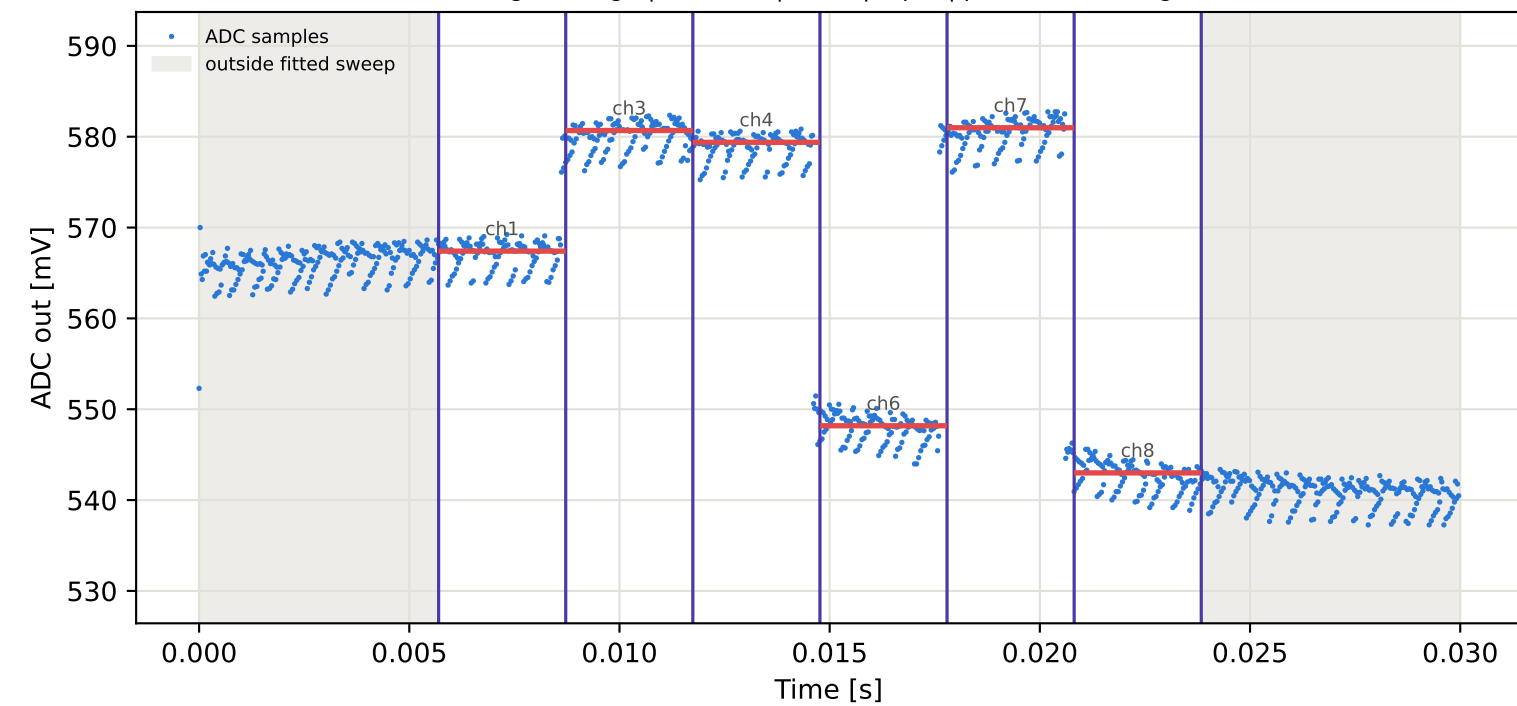
Tag6 &lt;- Tag9 | 895 MHz | run 0 | rep 1 | phase -0.99 deg
