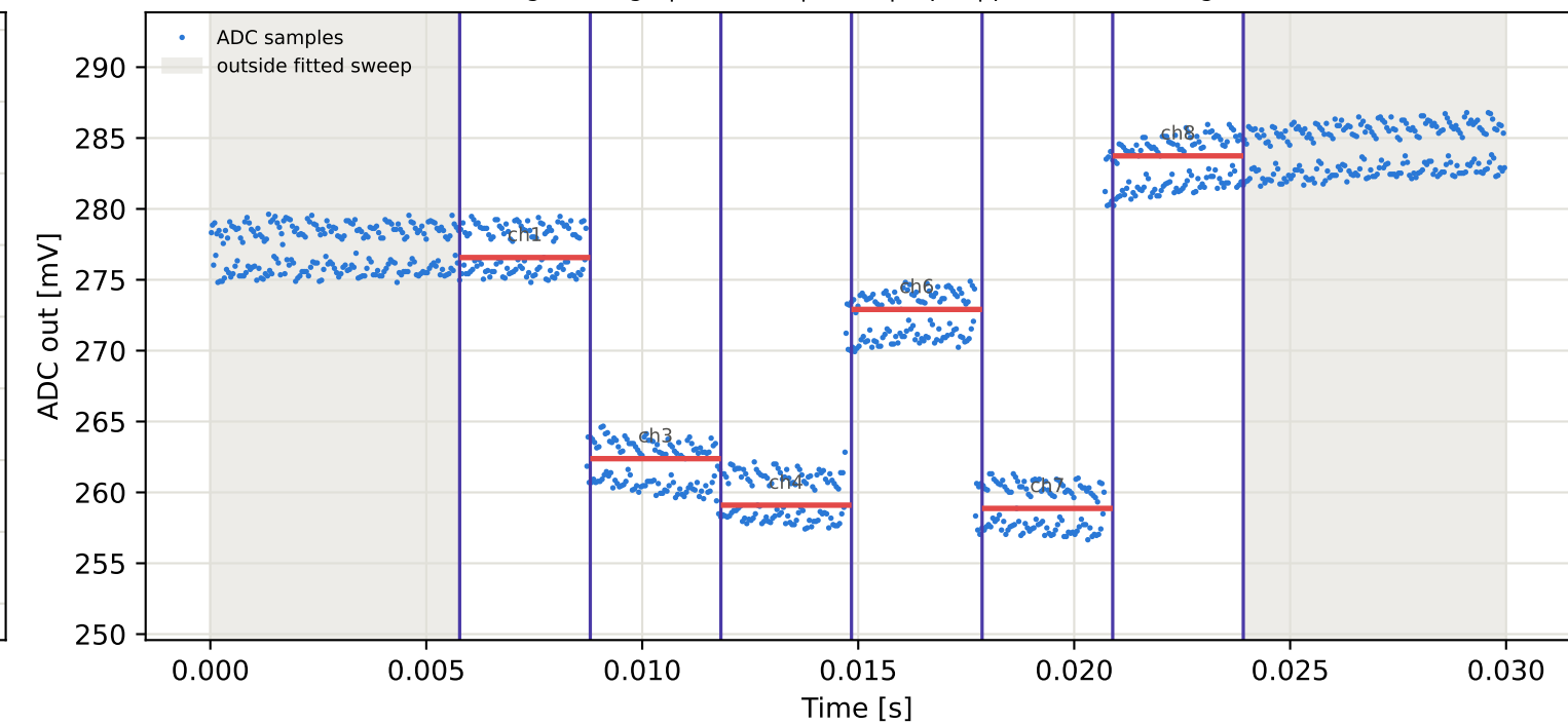
Tag2 &lt;- Tag6 | 865 MHz | run 0 | rep 1 | phase -134.31 deg
