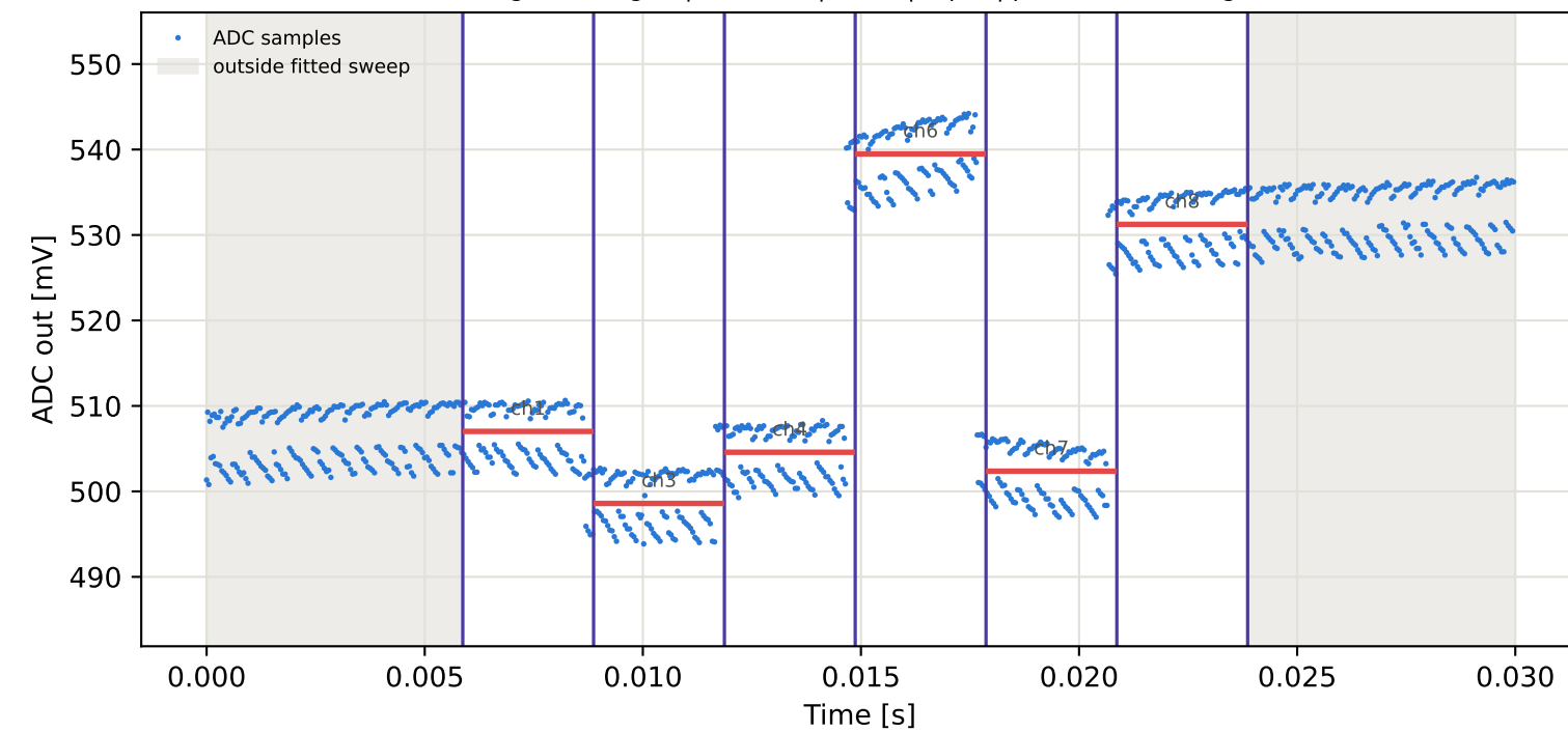
Tag10 &lt;- Tag2 | 915 MHz | run 0 | rep 1 | phase -27.06 deg
