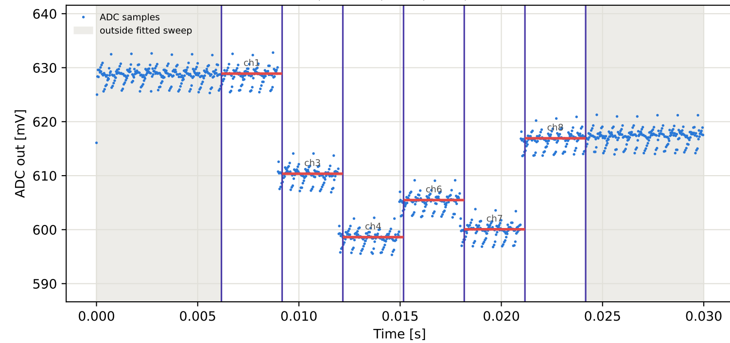
Tag15 &lt;- Tag5 | 855 MHz | run 0 | rep 1 | phase 78.44 deg
