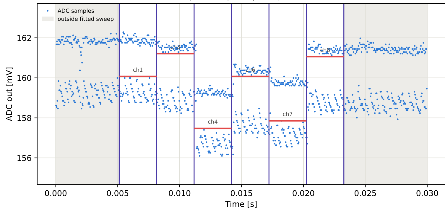
Tag4 &lt;- Tag8 | 795 MHz | run 0 | rep 1 | phase 97.89 deg
