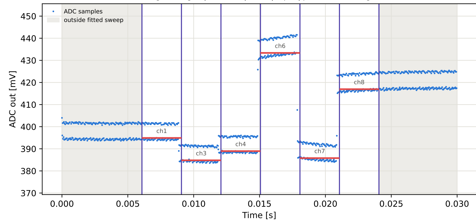
Tag1 &lt;- Tag2 | 945 MHz | run 0 | rep 1 | phase 9.82 deg
