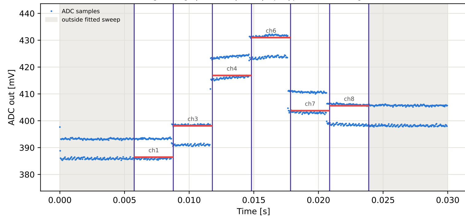
Tag3 &lt;- Tag15 | 945 MHz | run 0 | rep 1 | phase 115.59 deg
