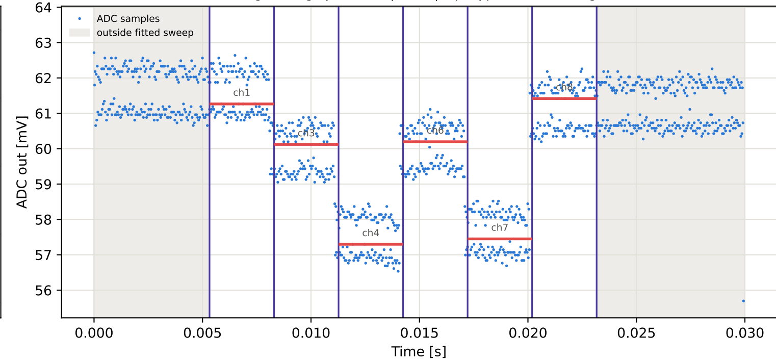
Tag5 &lt;- Tag9 | 795 MHz | run 0 | rep 1 | phase -173.90 deg
