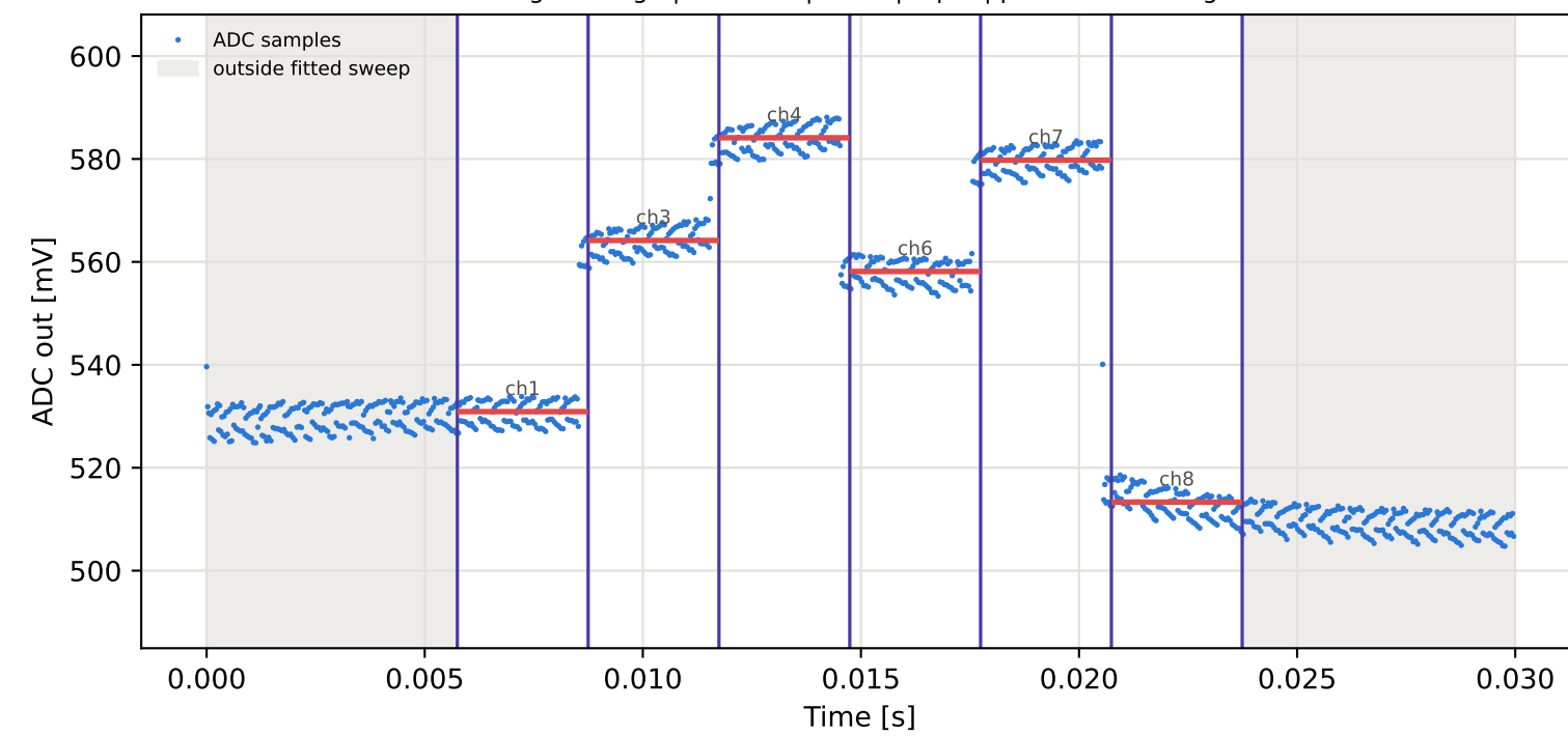
Tag2 &lt;- Tag5 | 895 MHz | run 0 | rep 1 | phase 155.42 deg
