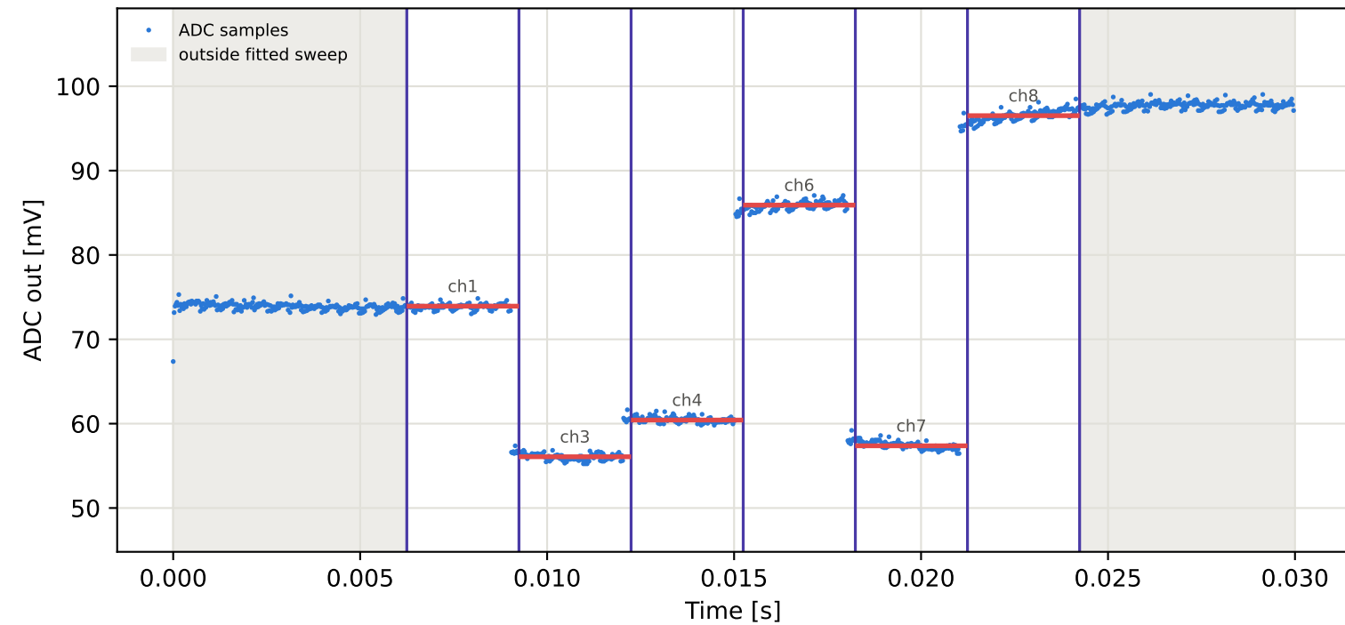
Tag9 &lt;- Tag8 | 865 MHz | run 0 | rep 1 | phase 30.57 deg
