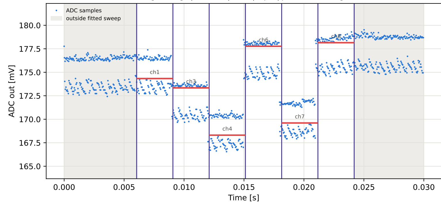
Tag5 &lt;- Tag9 | 965 MHz | run 0 | rep 1 | phase 35.39 deg
