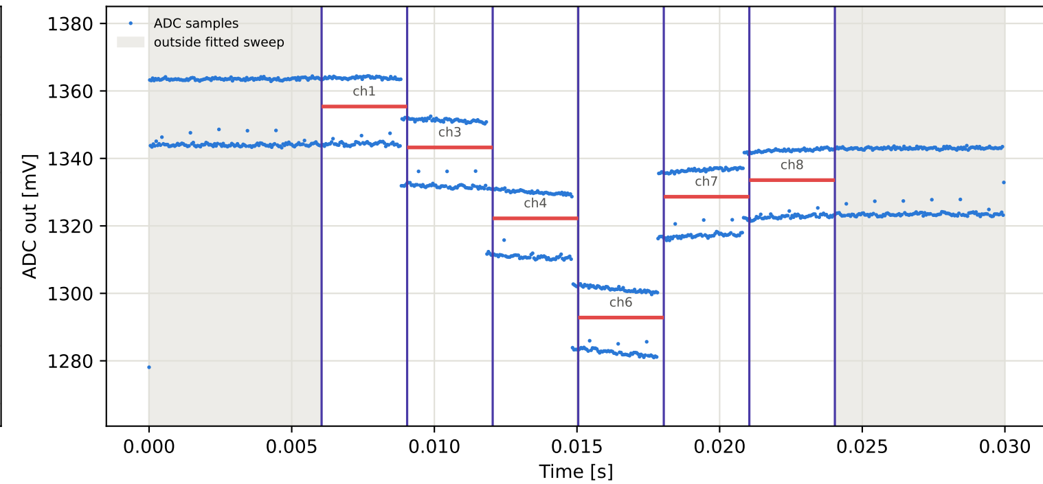
Tag16 &lt;- Tag7 | 895 MHz | run 0 | rep 1 | phase 70.30 deg
