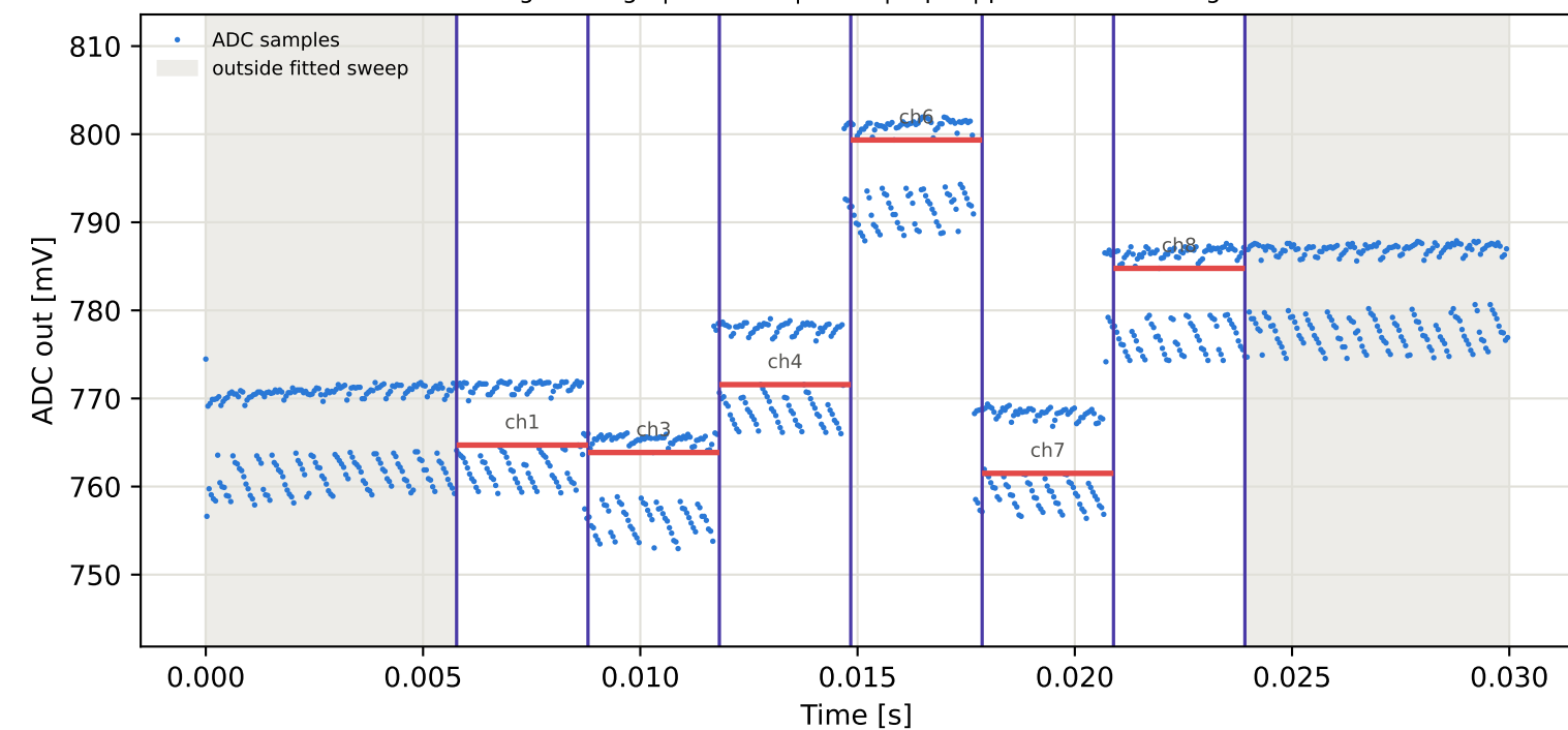
Tag9 &lt;- Tag10 | 985 MHz | run 0 | rep 1 | phase -117.69 deg
