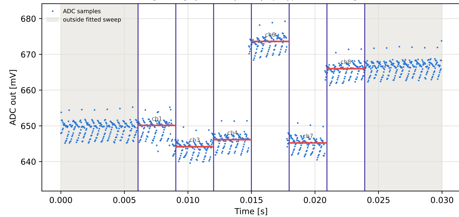
Tag8 &lt;- Tag10 | 915 MHz | run 0 | rep 1 | phase -149.23 deg
