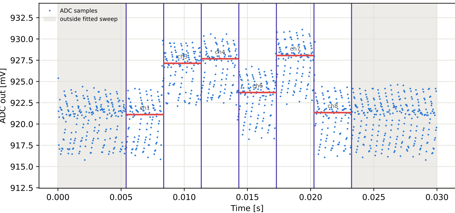
Tag16 &lt;- Tag10 | 845 MHz | run 0 | rep 1 | phase -61.67 deg
