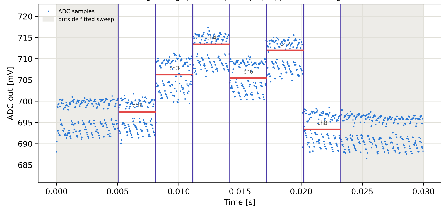
Tag4 &lt;- Tag8 | 885 MHz | run 0 | rep 1 | phase -129.95 deg
