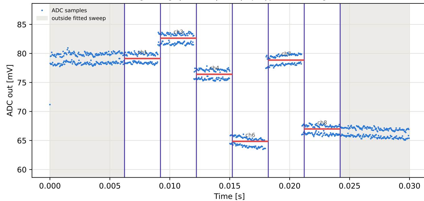
Tag9 &lt;- Tag5 | 865 MHz | run 0 | rep 1 | phase -111.03 deg
