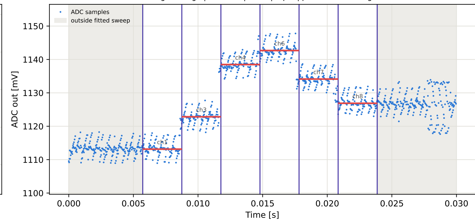
Tag8 &lt;- Tag5 | 875 MHz | run 0 | rep 1 | phase -53.11 deg
