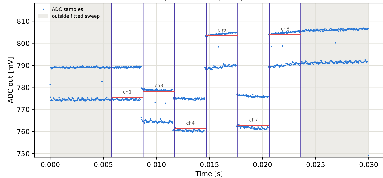
Tag5 &lt;- Tag16 | 915 MHz | run 0 | rep 1 | phase -27.59 deg
