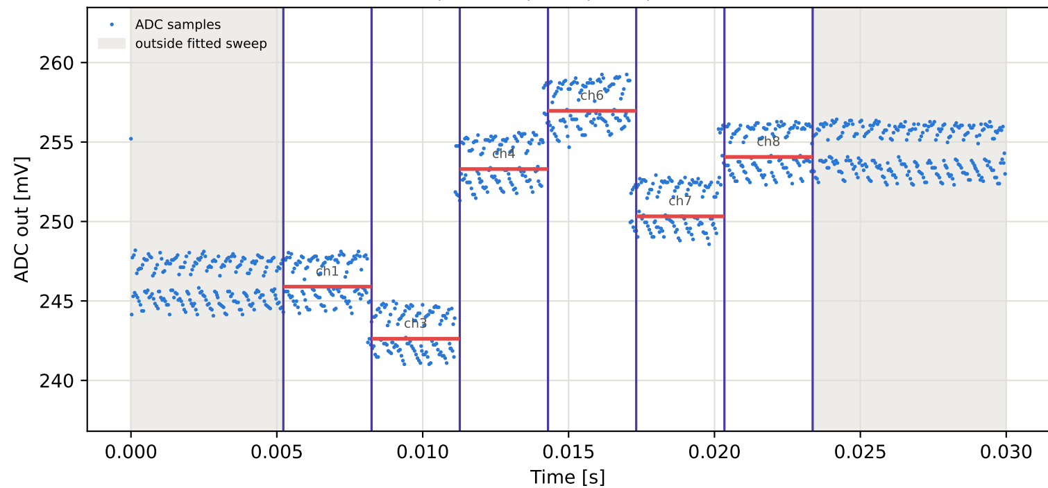
Tag7 &lt;- Tag6 | 835 MHz | run 0 | rep 1 | phase -142.36 deg
