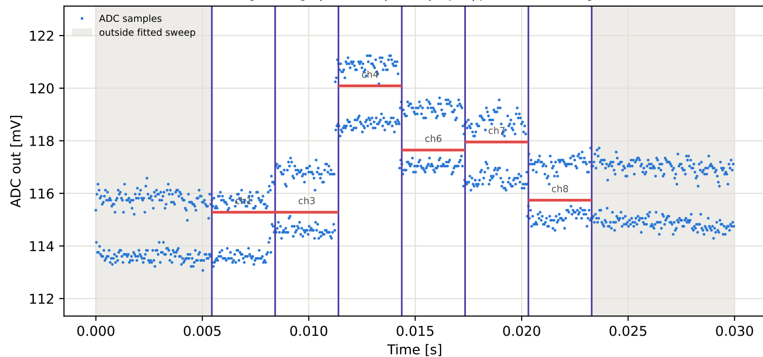
Tag5 &lt;- Tag9 | 995 MHz | run 0 | rep 1 | phase 103.99 deg
