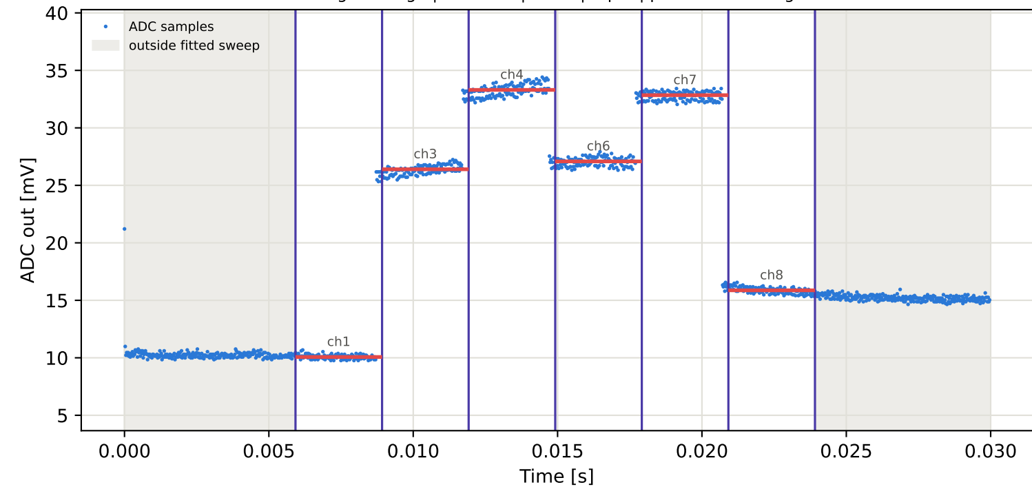
Tag1 &lt;- Tag8 | 855 MHz | run 0 | rep 1 | phase -105.86 deg
