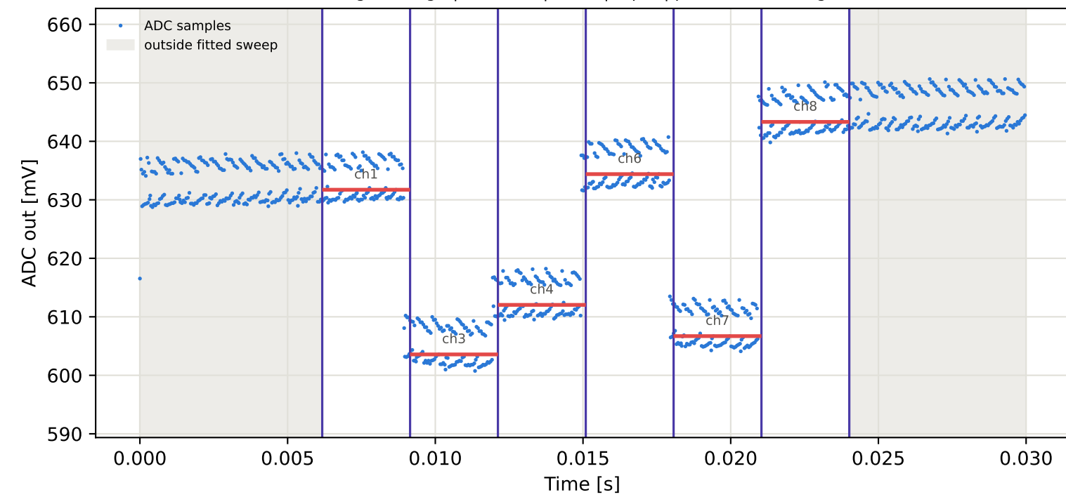
Tag4 &lt;- Tag7 | 855 MHz | run 0 | rep 1 | phase 158.55 deg
