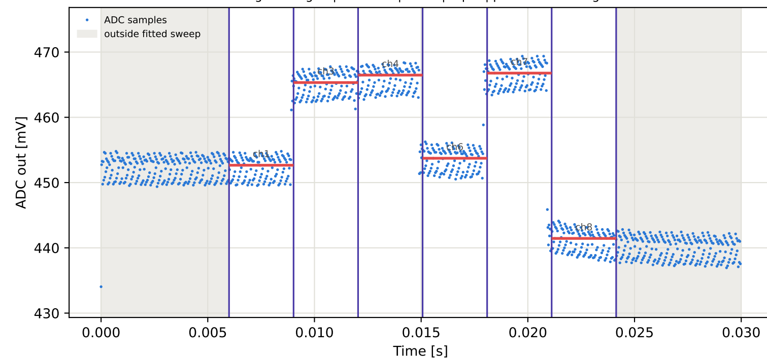
Tag3 &lt;- Tag16 | 865 MHz | run 0 | rep 1 | phase -52.47 deg
