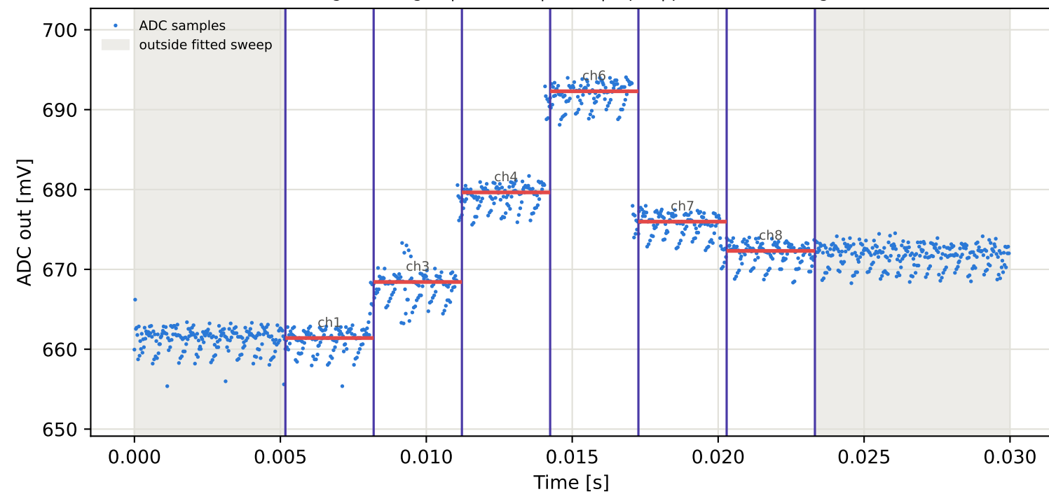
Tag10 &lt;- Tag3 | 885 MHz | run 0 | rep 1 | phase -173.20 deg
