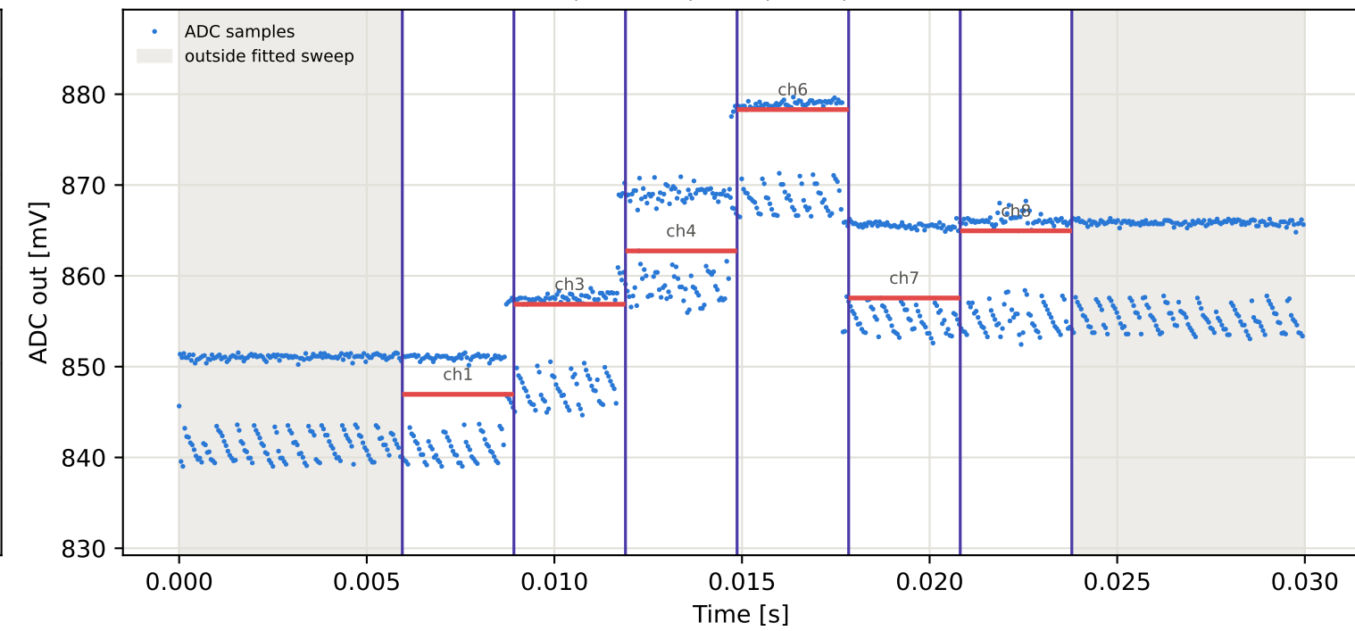
Tag7 &lt;- Tag6 | 875 MHz | run 0 | rep 1 | phase -149.06 deg
