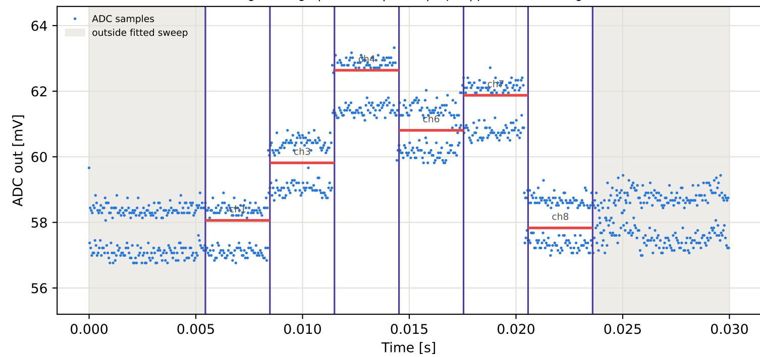
Tag9 &lt;- Tag2 | 805 MHz | run 0 | rep 1 | phase -91.48 deg
