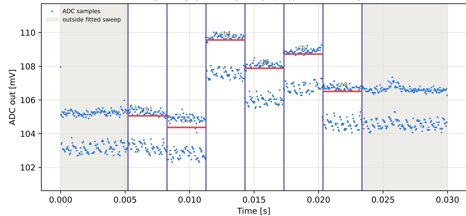
Tag7 &lt;- Tag1 | 785 MHz | run 0 | rep 1 | phase -35.10 deg
