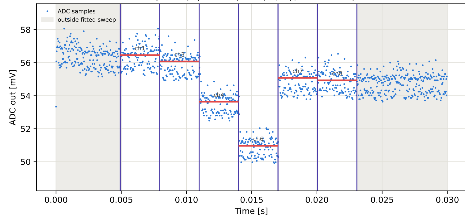
Tag2 &lt;- Tag7 | 945 MHz | run 0 | rep 1 | phase 86.39 deg
