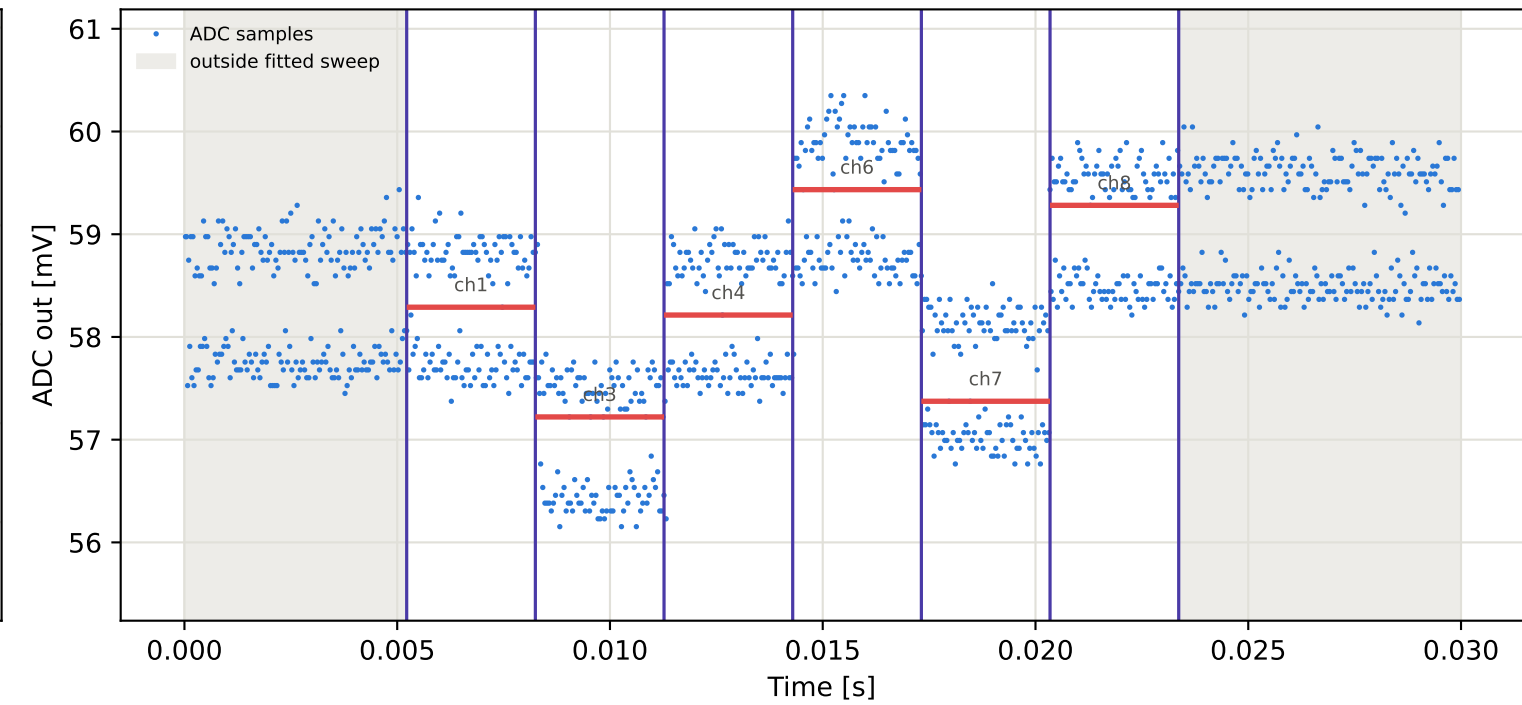
Tag6 &lt;- Tag10 | 795 MHz | run 0 | rep 1 | phase 51.60 deg
