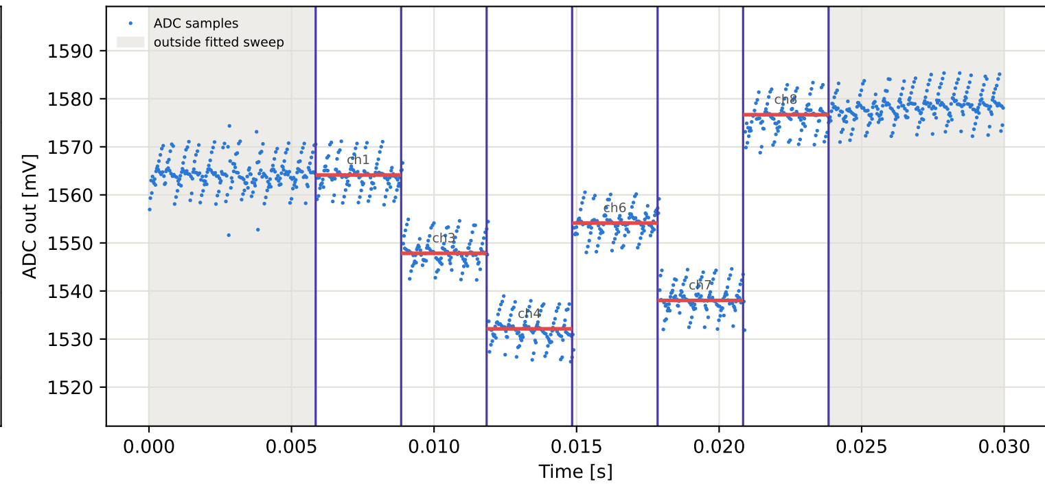
Tag8 &lt;- Tag7 | 915 MHz | run 0 | rep 1 | phase -56.16 deg
