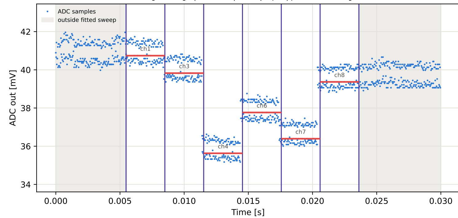
Tag7 &lt;- Tag6 | 785 MHz | run 0 | rep 1 | phase 83.44 deg
