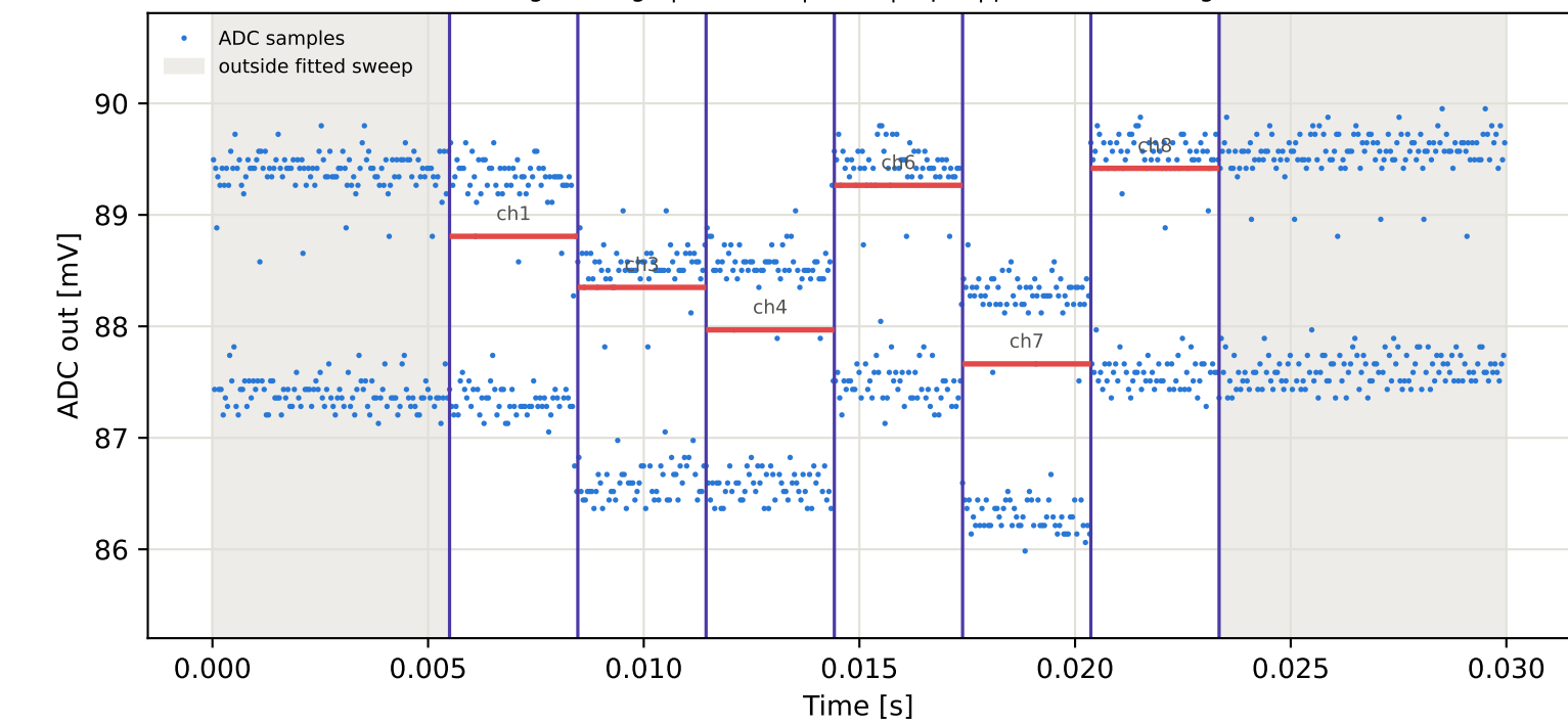
Tag1 &lt;- Tag9 | 795 MHz | run 0 | rep 1 | phase 144.68 deg
