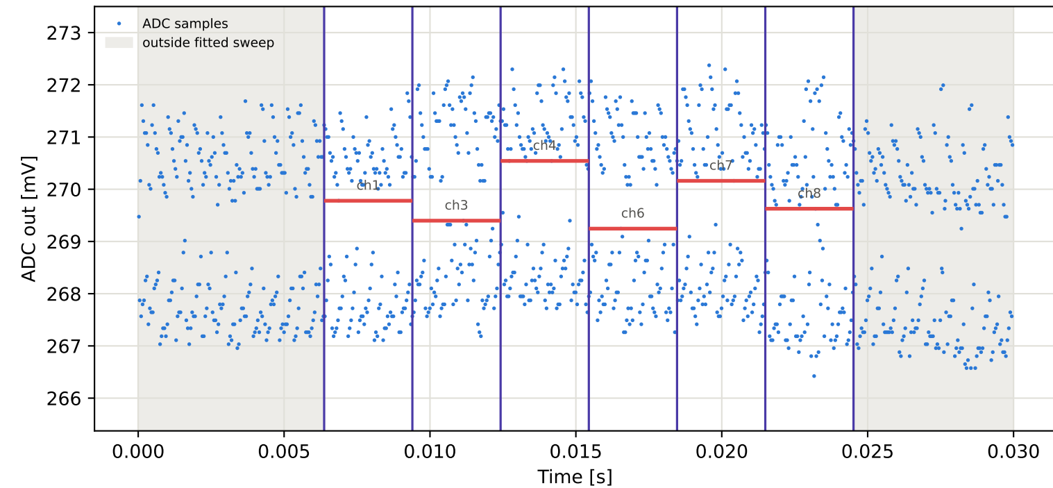
Tag6 &lt;- Tag4 | 985 MHz | run 0 | rep 1 | phase -108.69 deg
