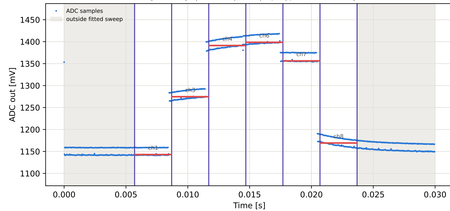
Tag2 &lt;- Tag1 | 895 MHz | run 0 | rep 1 | phase -87.52 deg
