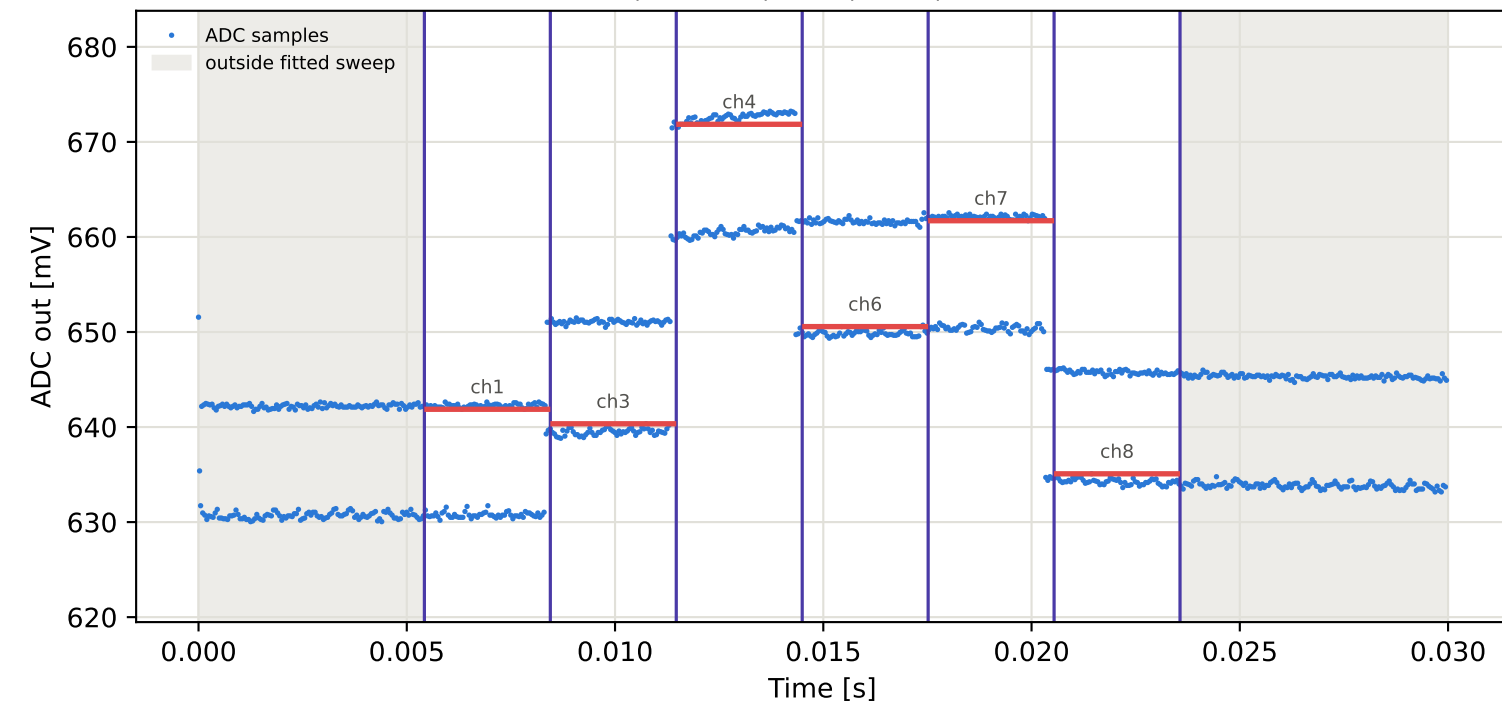
Tag6 &lt;- Tag1 | 955 MHz | run 0 | rep 1 | phase -104.87 deg
