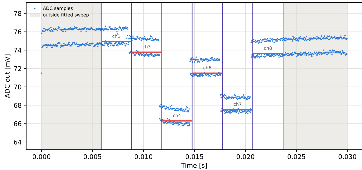
Tag10 &lt;- Tag2 | 775 MHz | run 0 | rep 1 | phase -94.52 deg
