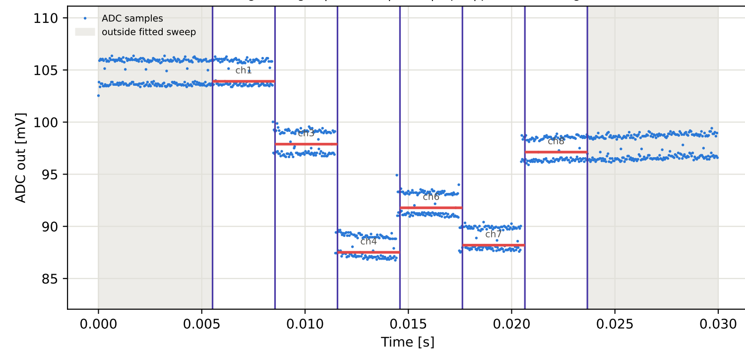
Tag1 &lt;- Tag3 | 825 MHz | run 0 | rep 1 | phase -155.65 deg
