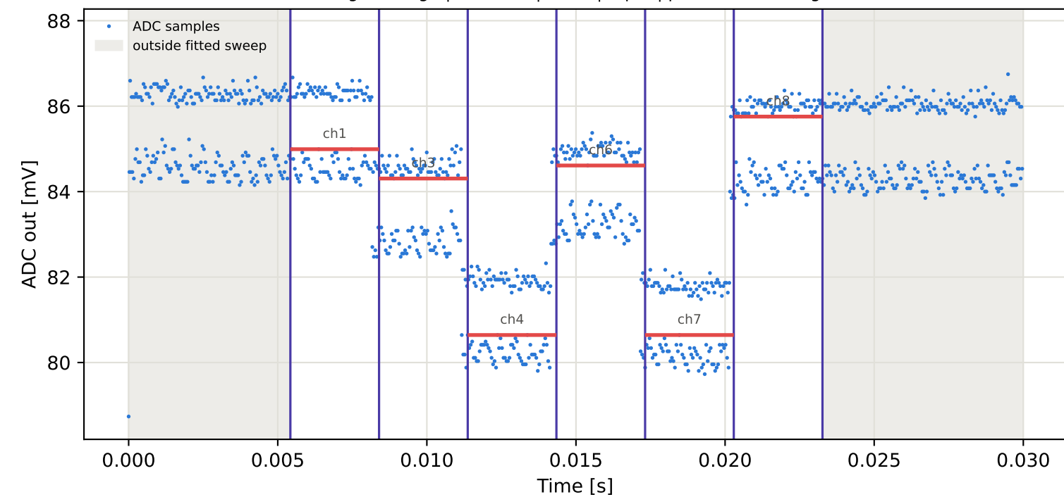
Tag9 &lt;- Tag7 | 785 MHz | run 0 | rep 1 | phase 109.98 deg
