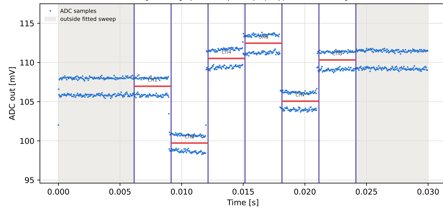
Tag10 &lt;- Tag4 | 785 MHz | run 0 | rep 1 | phase -145.61 deg
