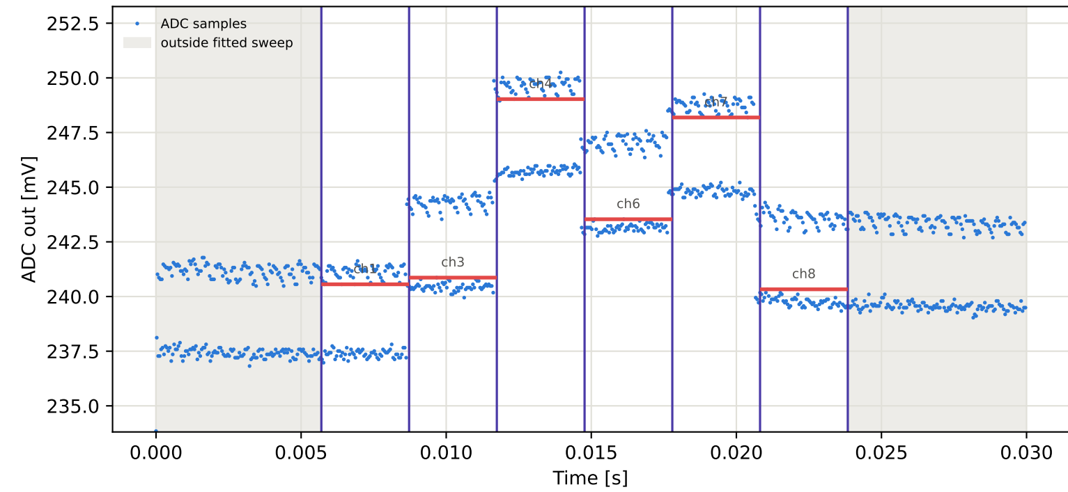
Tag7 &lt;- Tag10 | 825 MHz | run 0 | rep 1 | phase 82.14 deg
