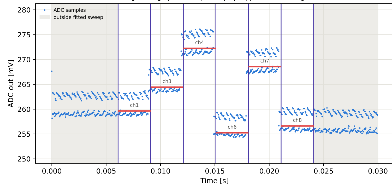
Tag9 &lt;- Tag5 | 995 MHz | run 0 | rep 1 | phase 93.15 deg
