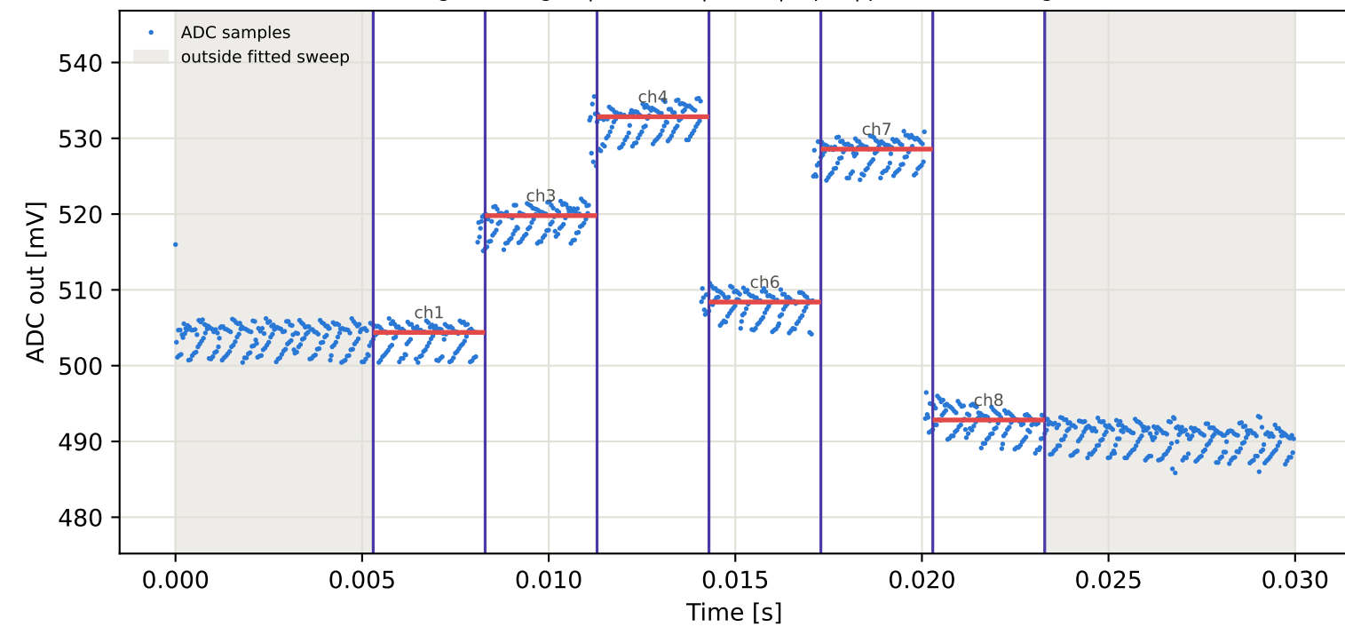
Tag10 &lt;- Tag3 | 905 MHz | run 0 | rep 1 | phase -127.60 deg
