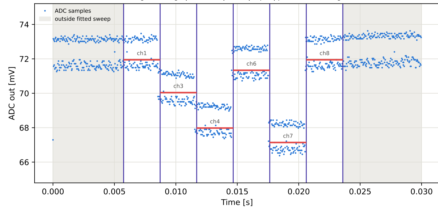
Tag15 &lt;- Tag10 | 775 MHz | run 0 | rep 1 | phase 99.47 deg
