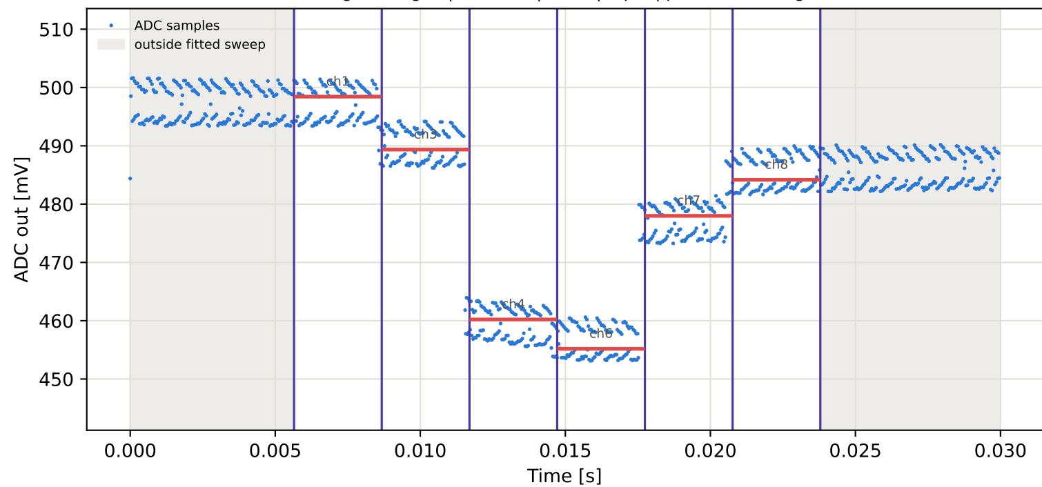
Tag9 &lt;- Tag2 | 975 MHz | run 0 | rep 1 | phase -64.87 deg
