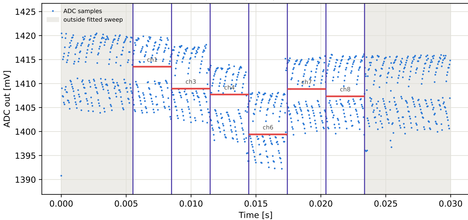
Tag15 &lt;- Tag10 | 905 MHz | run 0 | rep 1 | phase 29.28 deg
