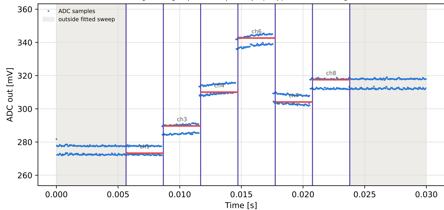
Tag2 &lt;- Tag16 | 875 MHz | run 0 | rep 1 | phase -146.00 deg
