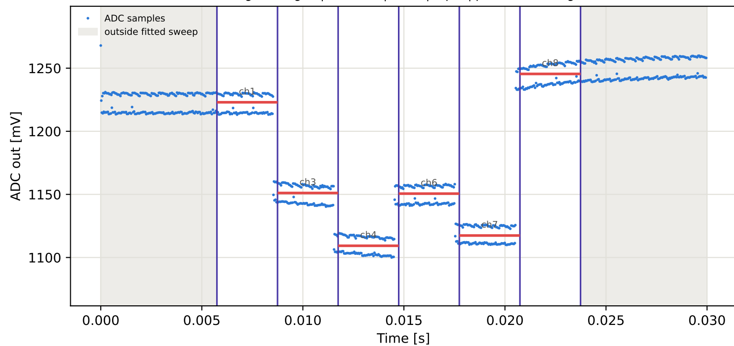
Tag8 &lt;- Tag16 | 875 MHz | run 0 | rep 1 | phase 91.76 deg
