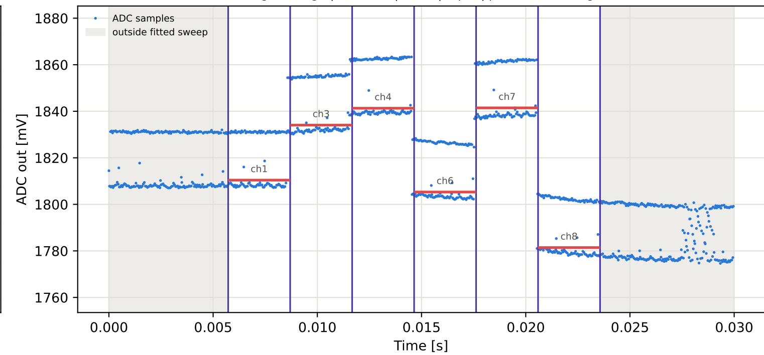
Tag8 &lt;- Tag5 | 895 MHz | run 0 | rep 1 | phase 34.61 deg
