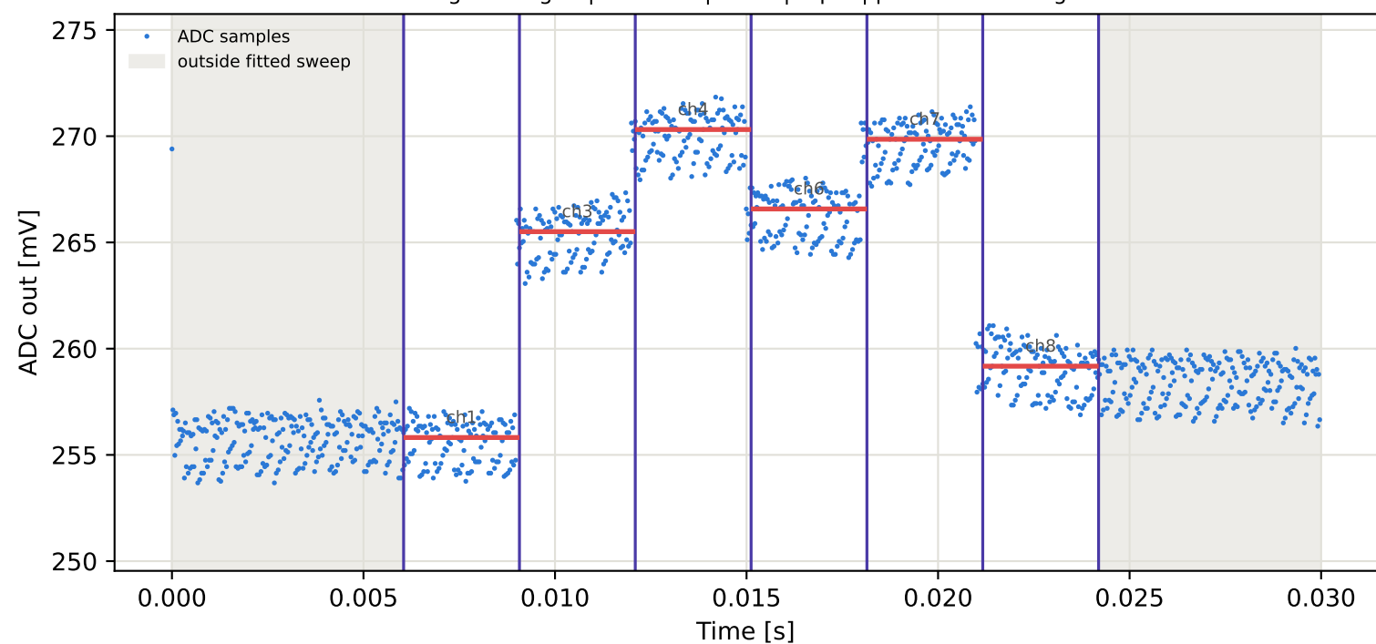
Tag2 &lt;- Tag16 | 865 MHz | run 0 | rep 1 | phase -142.66 deg
