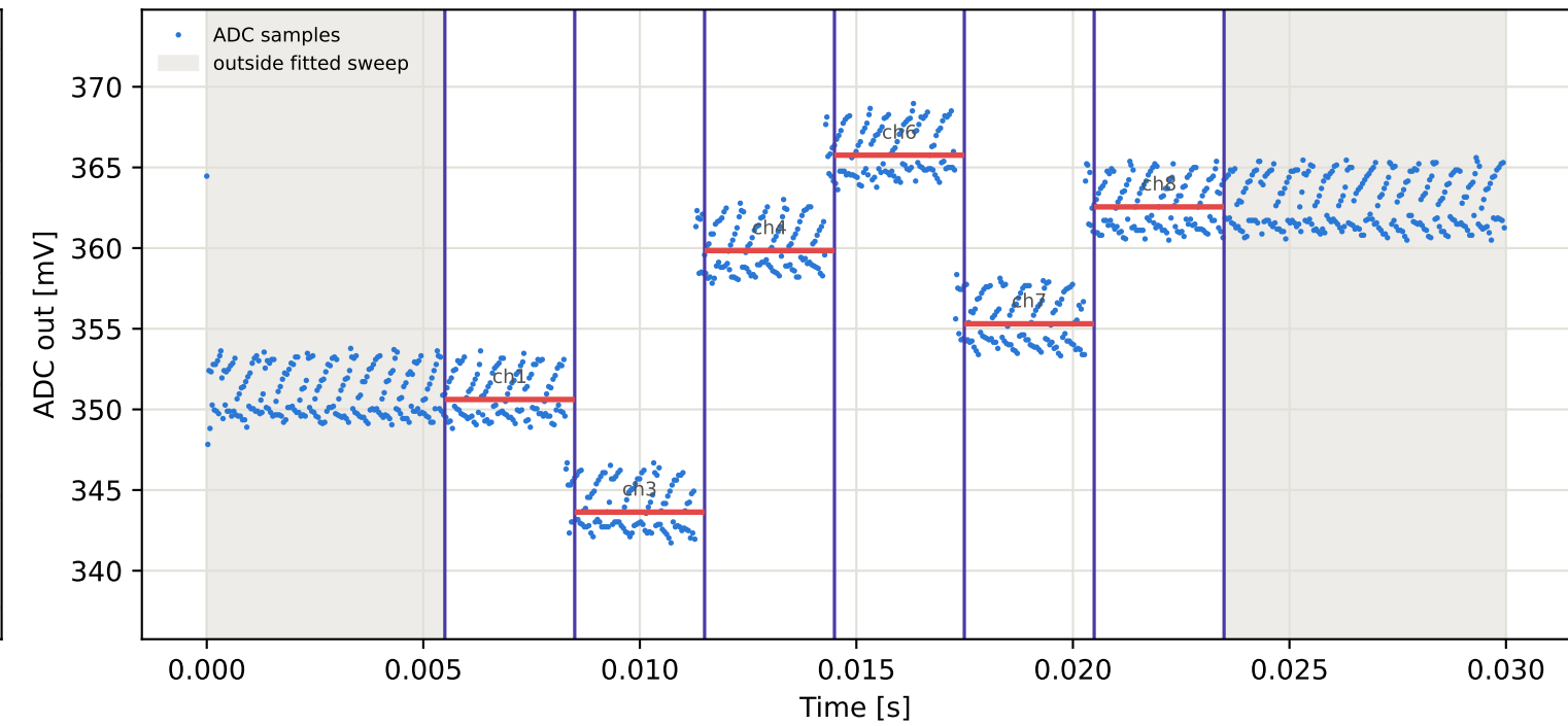
Tag9 &lt;- Tag2 | 845 MHz | run 0 | rep 1 | phase -33.62 deg
