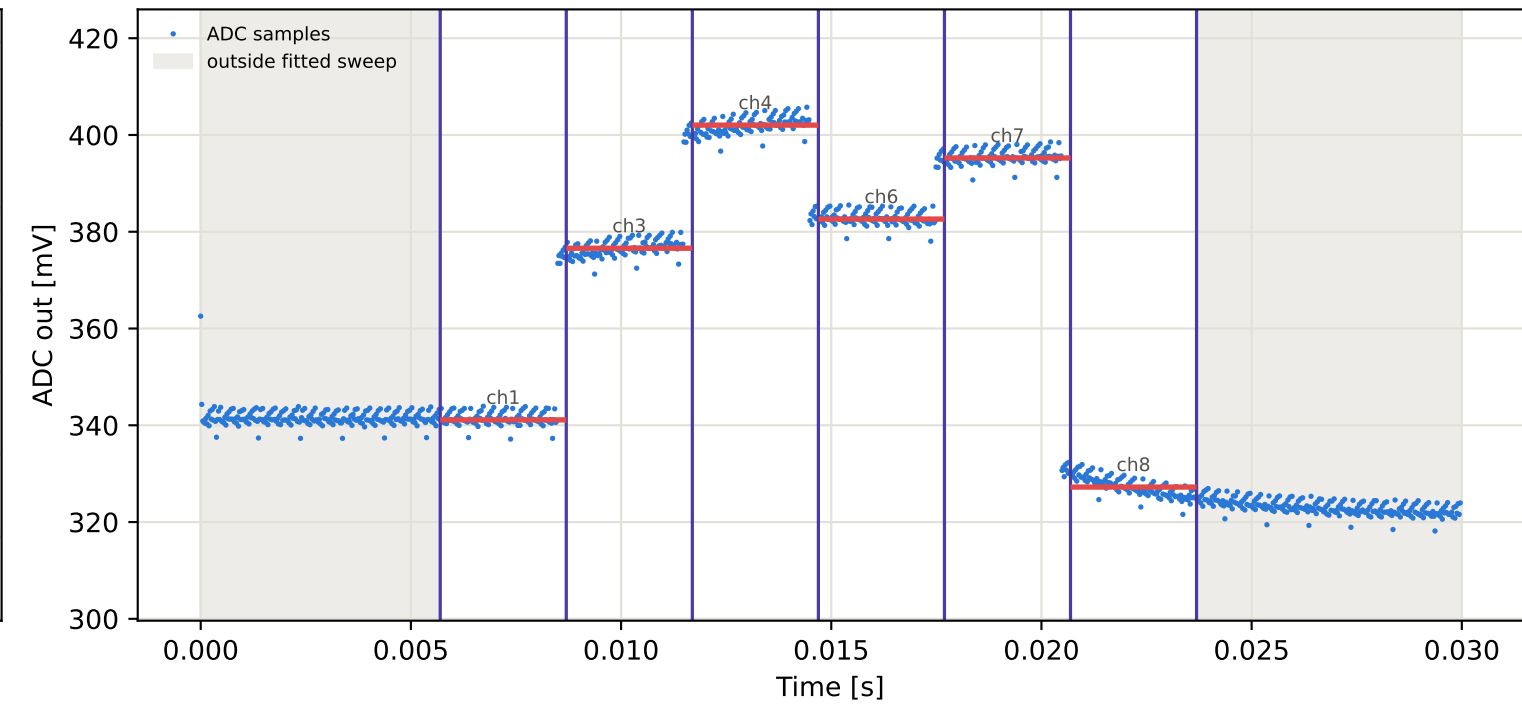
Tag10 &lt;- Tag1 | 895 MHz | run 0 | rep 1 | phase 24.99 deg
