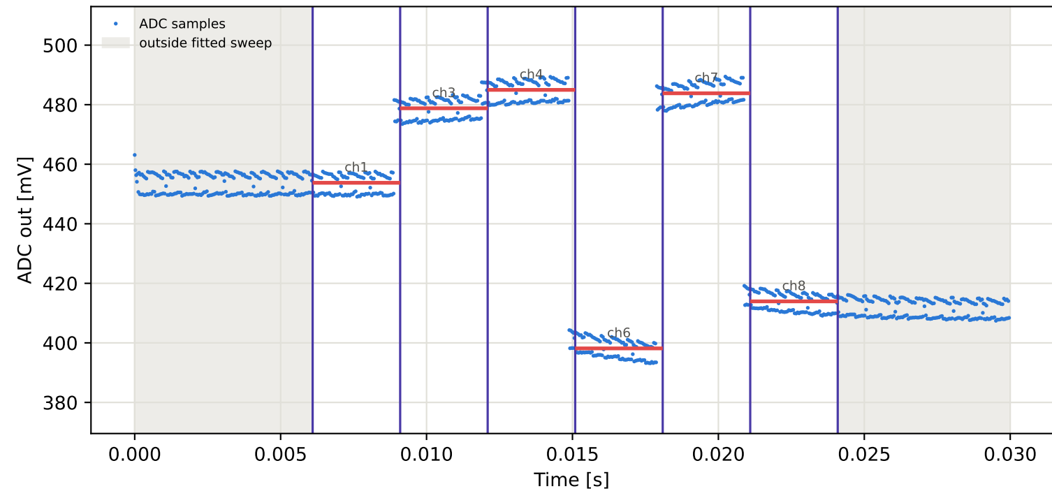
Tag9 &lt;- Tag2 | 945 MHz | run 0 | rep 1 | phase 103.92 deg
