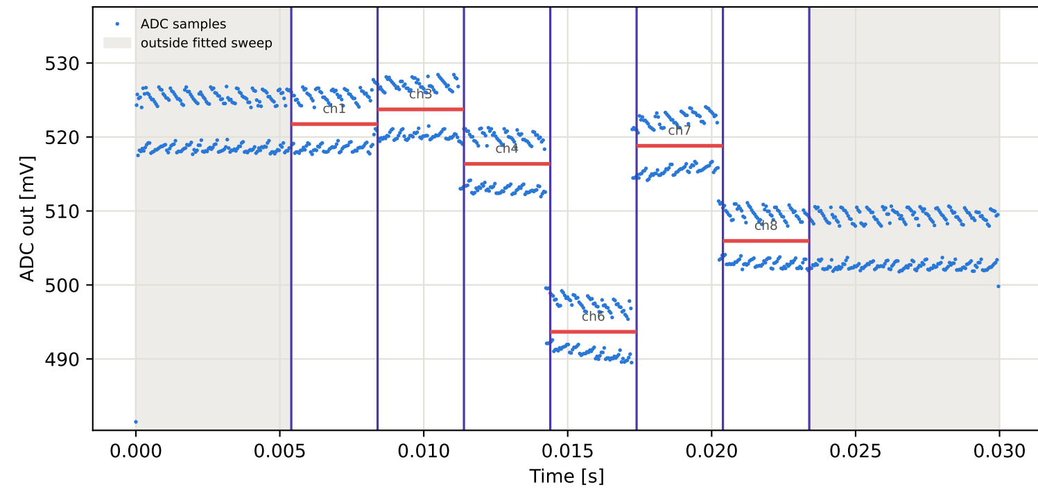
Tag10 &lt;- Tag9 | 905 MHz | run 0 | rep 1 | phase -103.40 deg
