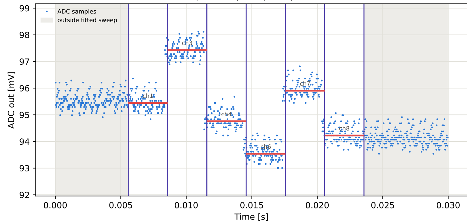
Tag8 &lt;- Tag10 | 795 MHz | run 0 | rep 1 | phase 118.41 deg
