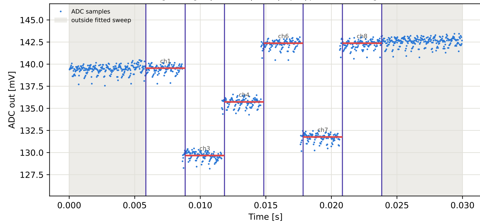
Tag6 &lt;- Tag3 | 805 MHz | run 0 | rep 1 | phase -116.89 deg
