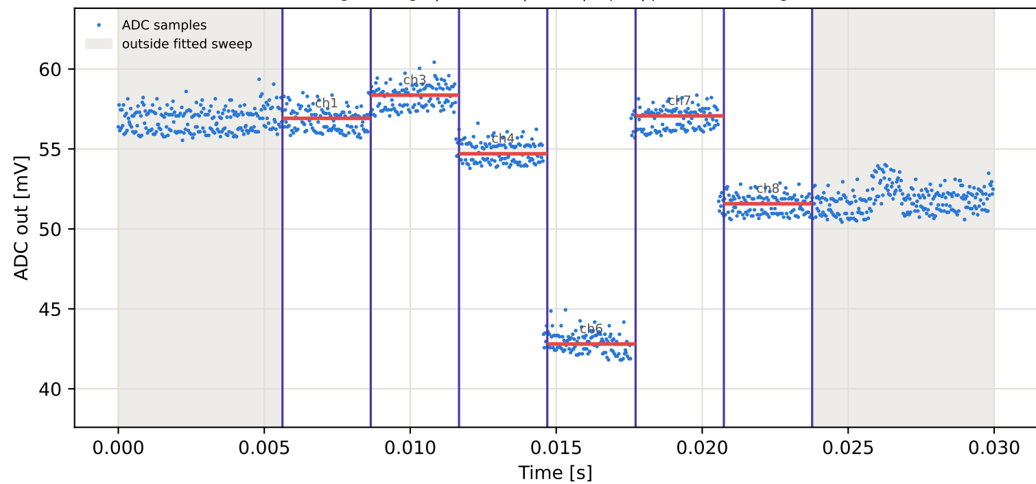
Tag2 &lt;- Tag6 | 945 MHz | run 0 | rep 1 | phase -51.16 deg
