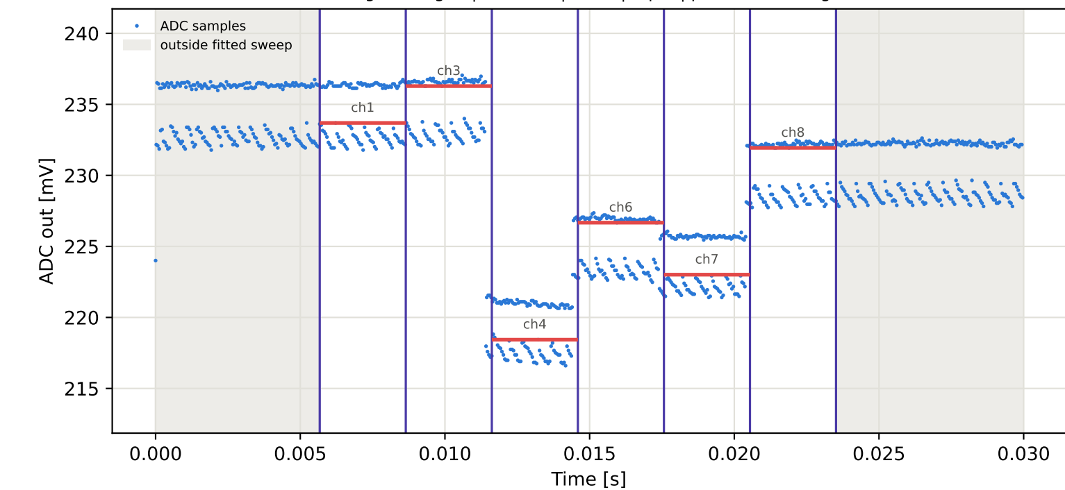
Tag8 &lt;- Tag15 | 795 MHz | run 0 | rep 1 | phase 79.95 deg
