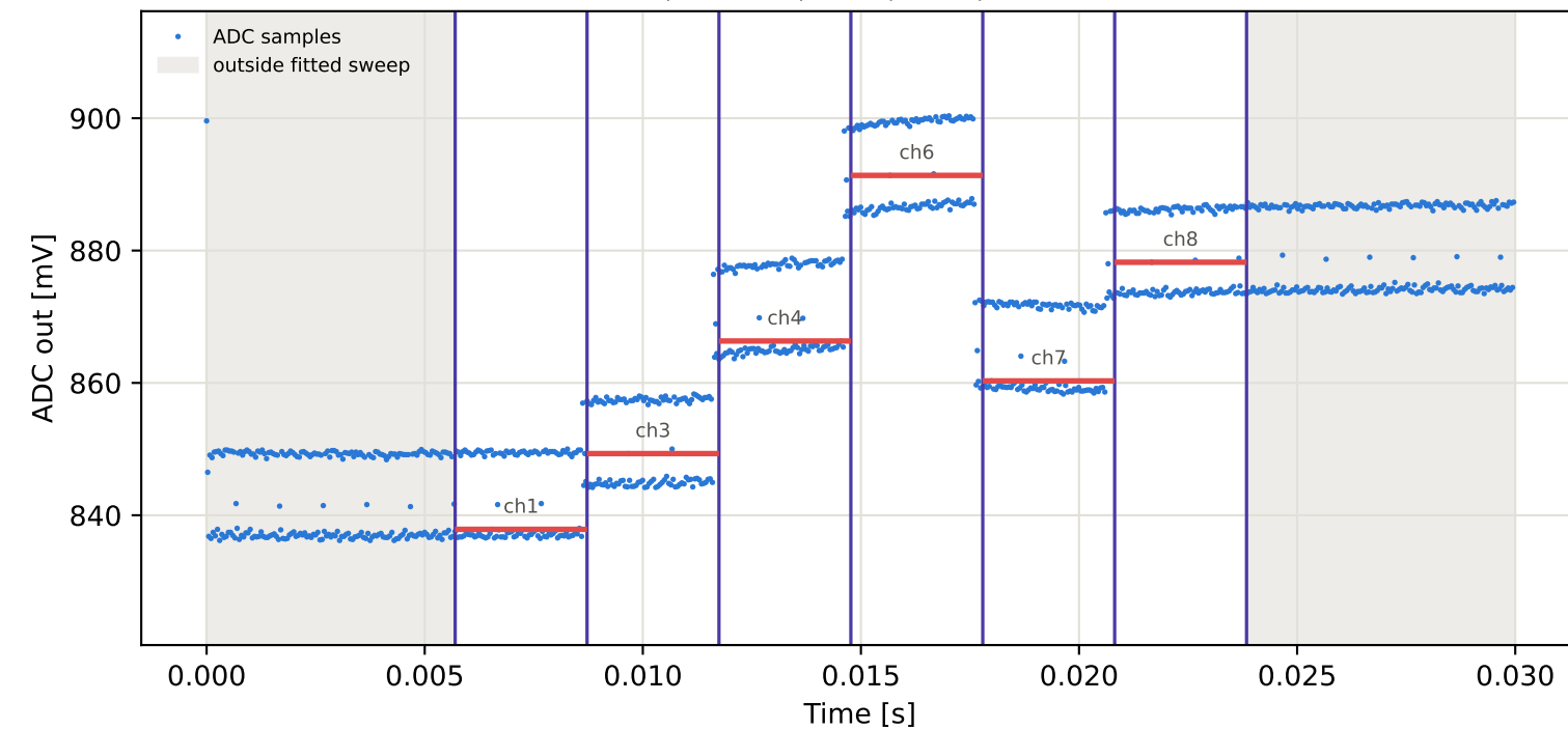
Tag3 &lt;- Tag8 | 875 MHz | run 0 | rep 1 | phase -149.67 deg
