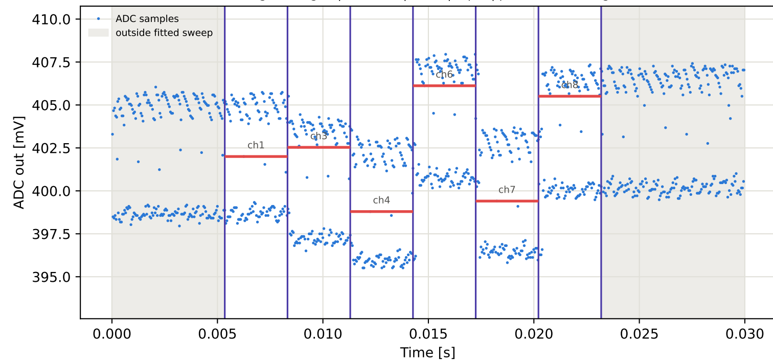
Tag4 &lt;- Tag16 | 975 MHz | run 0 | rep 1 | phase 4.39 deg
