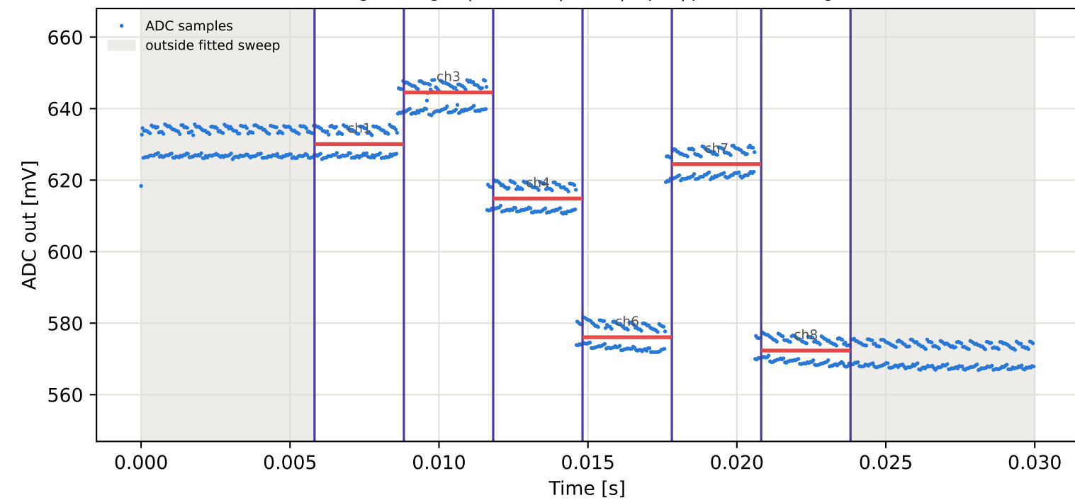
Tag7 &lt;- Tag3 | 855 MHz | run 0 | rep 1 | phase 139.82 deg
