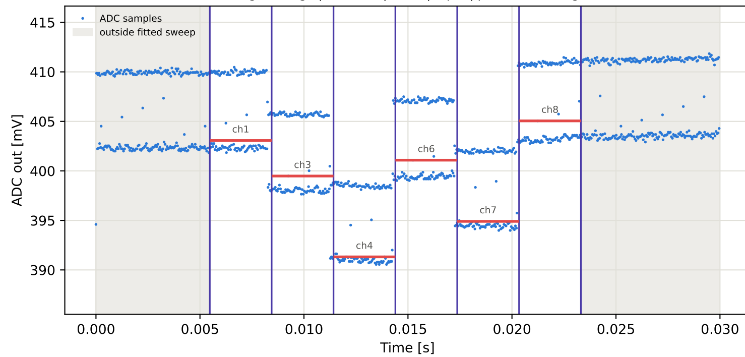
Tag4 &lt;- Tag15 | 975 MHz | run 0 | rep 1 | phase 163.04 deg
