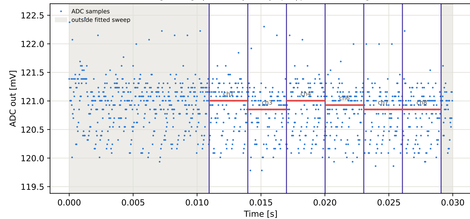
Tag8 &lt;- Tag4 | 785 MHz | run 0 | rep 1 | phase -154.66 deg
