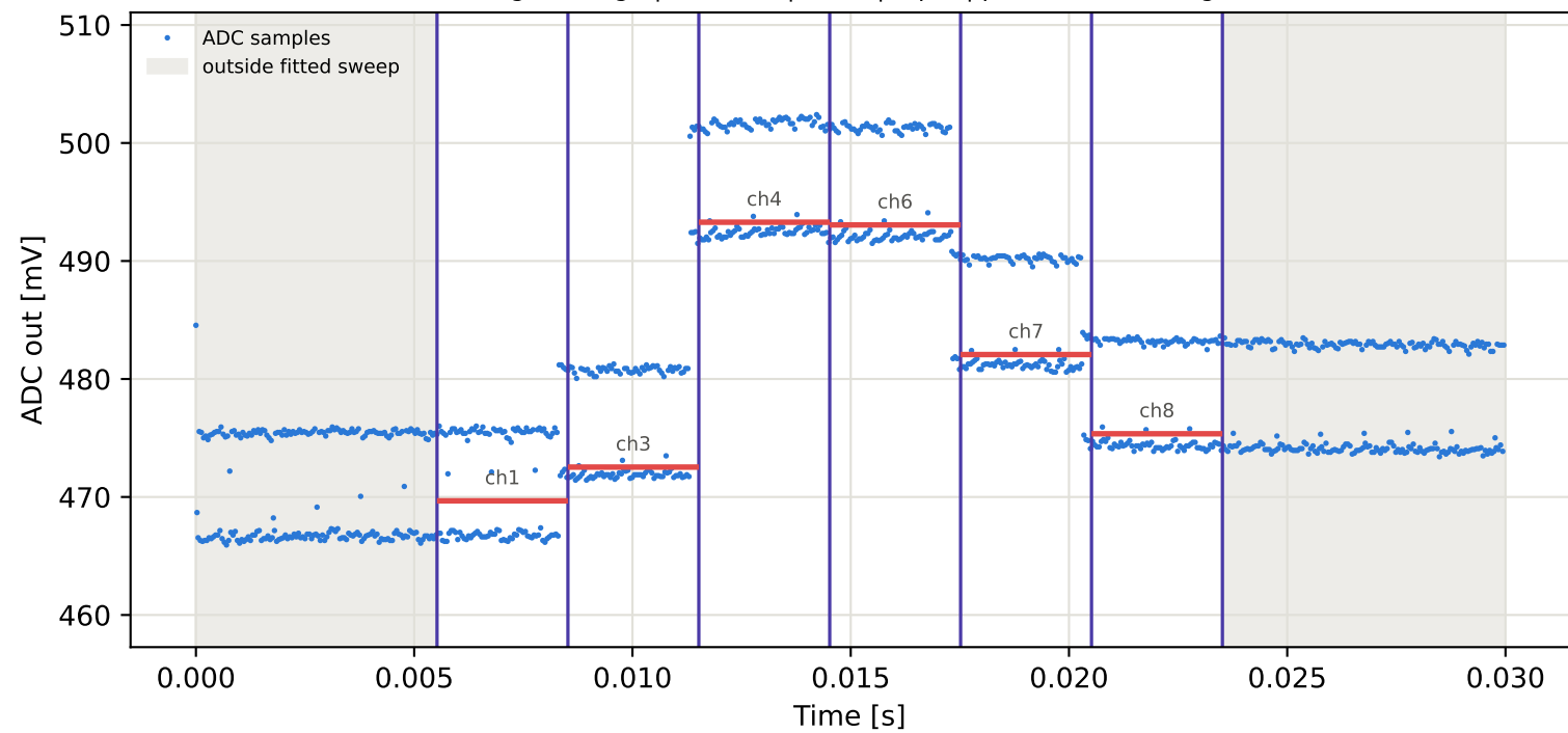
Tag9 &lt;- Tag15 | 975 MHz | run 0 | rep 1 | phase 42.99 deg
