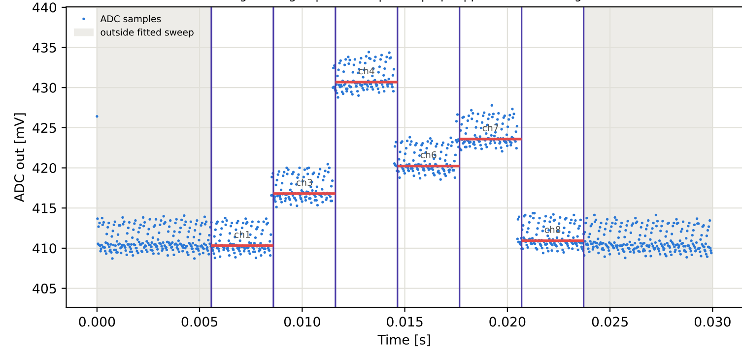
Tag1 &lt;- Tag2 | 975 MHz | run 0 | rep 1 | phase 74.71 deg
