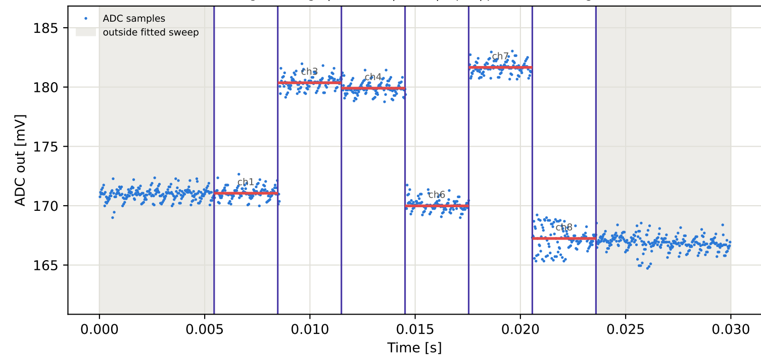
Tag10 &lt;- Tag9 | 855 MHz | run 0 | rep 1 | phase -82.91 deg
