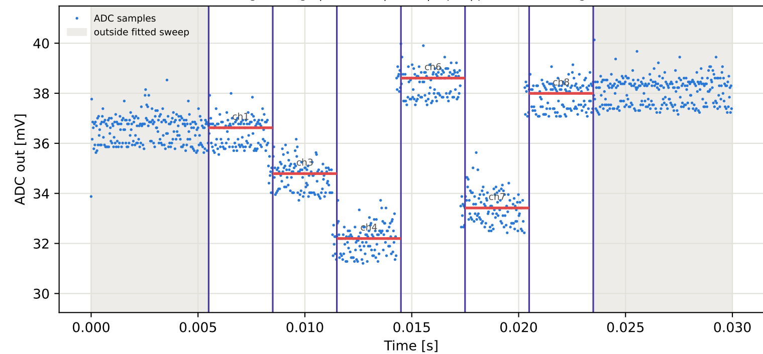
Tag2 &lt;- Tag6 | 975 MHz | run 0 | rep 1 | phase 156.61 deg
