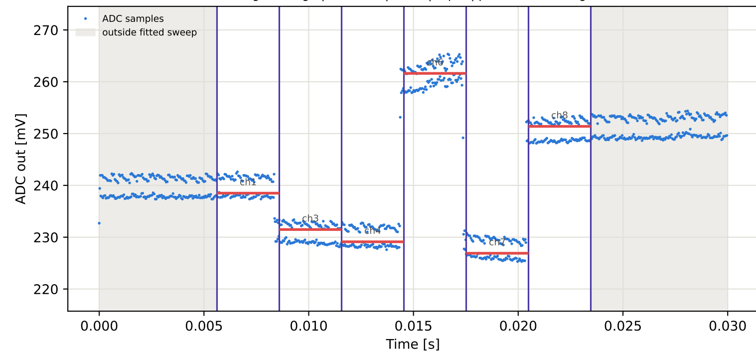
Tag5 &lt;- Tag3 | 985 MHz | run 0 | rep 1 | phase 156.04 deg
