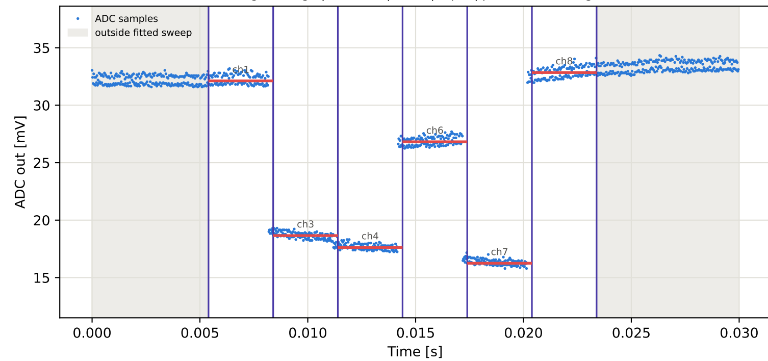
Tag1 &lt;- Tag8 | 845 MHz | run 0 | rep 1 | phase 125.29 deg
