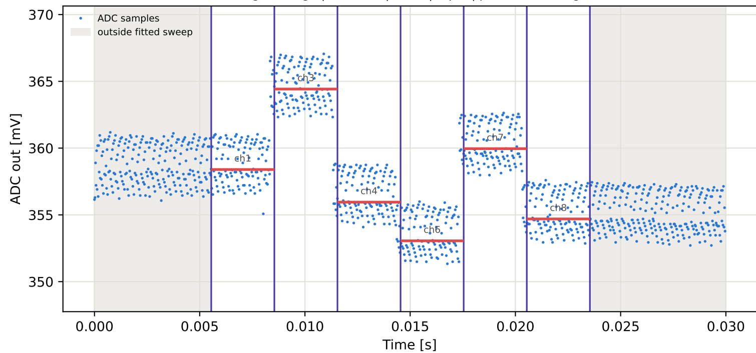
Tag3 &lt;- Tag15 | 825 MHz | run 0 | rep 1 | phase -57.53 deg
