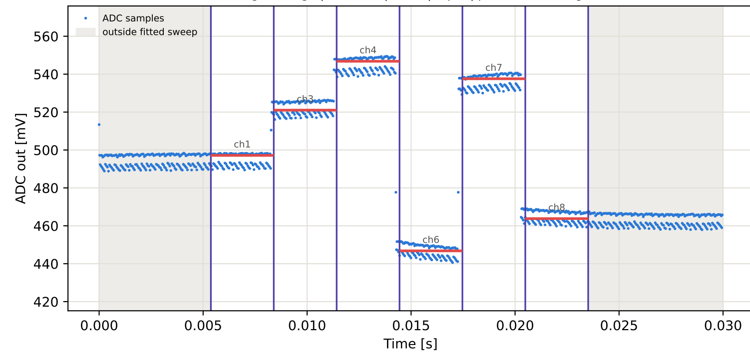
Tag3 &lt;- Tag6 | 955 MHz | run 0 | rep 1 | phase -15.71 deg
