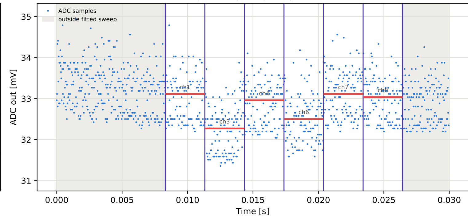
Tag2 &lt;- Tag8 | 775 MHz | run 0 | rep 1 | phase -42.52 deg
