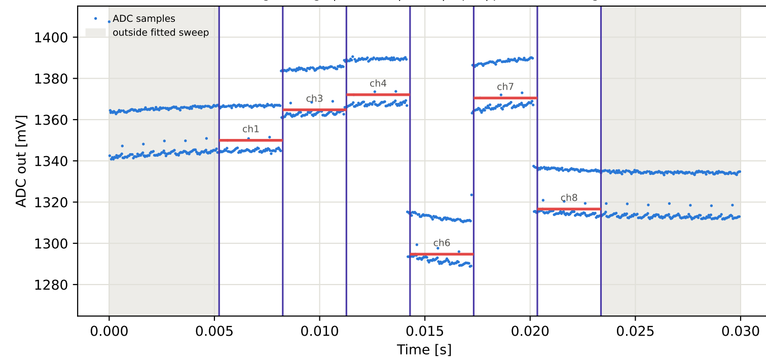
Tag4 &lt;- Tag7 | 935 MHz | run 0 | rep 1 | phase -161.57 deg
