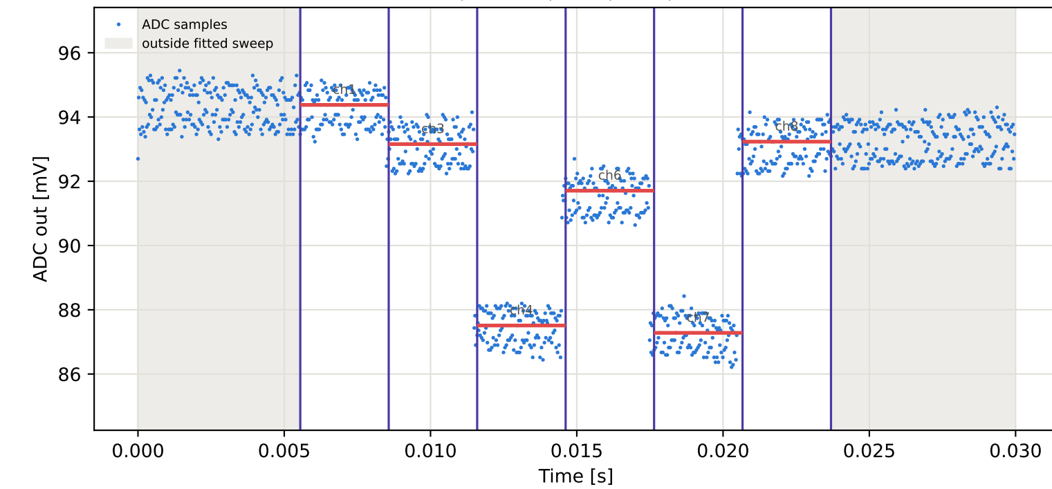
Tag9 &lt;- Tag16 | 775 MHz | run 0 | rep 1 | phase 98.50 deg
