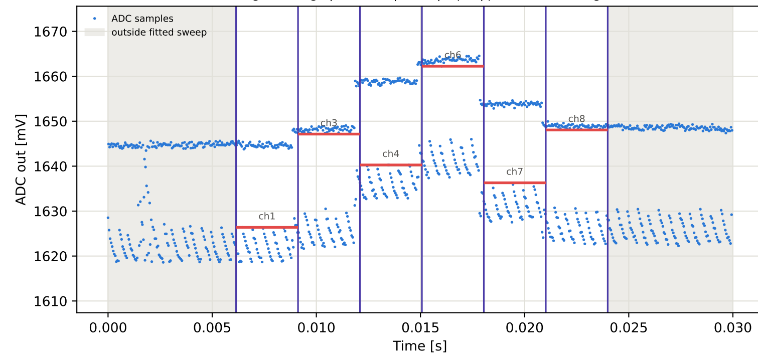
Tag15 &lt;- Tag5 | 935 MHz | run 0 | rep 1 | phase 17.46 deg
