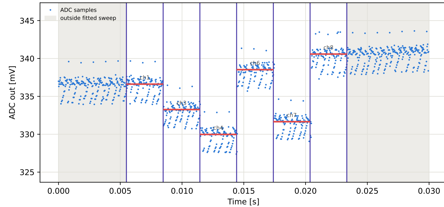
Tag10 &lt;- Tag4 | 935 MHz | run 0 | rep 1 | phase -17.70 deg
