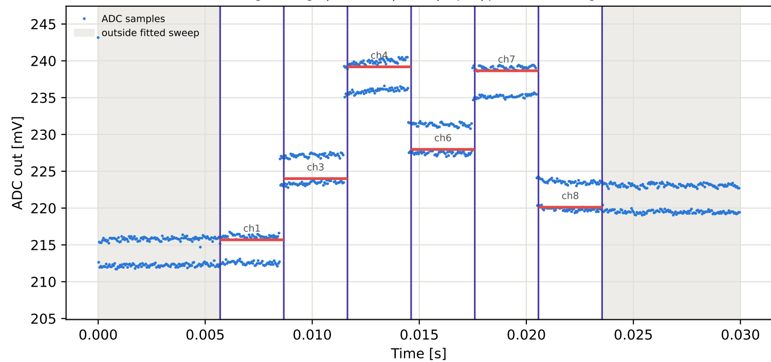
Tag8 &lt;- Tag1 | 825 MHz | run 0 | rep 1 | phase 93.04 deg
