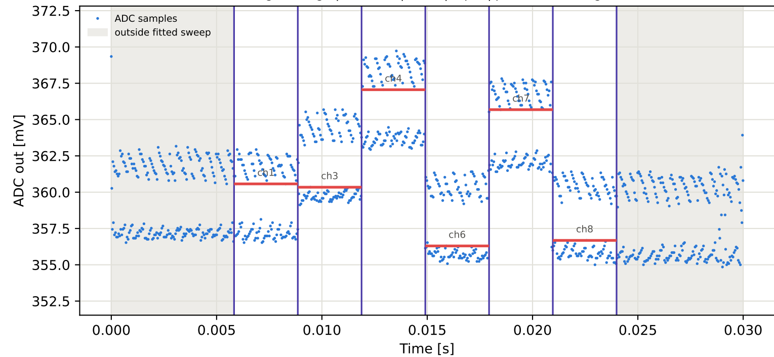
Tag4 &lt;- Tag8 | 995 MHz | run 0 | rep 1 | phase -31.32 deg
