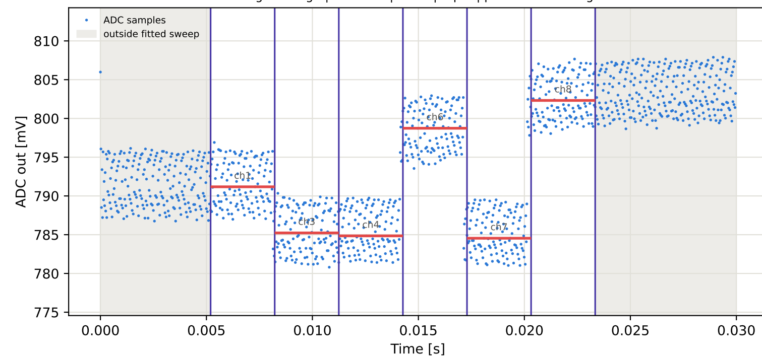
Tag3 &lt;- Tag8 | 885 MHz | run 0 | rep 1 | phase 171.12 deg
