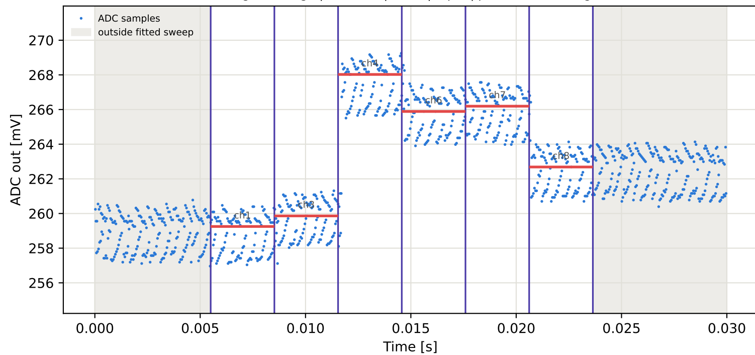
Tag2 &lt;- Tag10 | 805 MHz | run 0 | rep 1 | phase -64.74 deg
