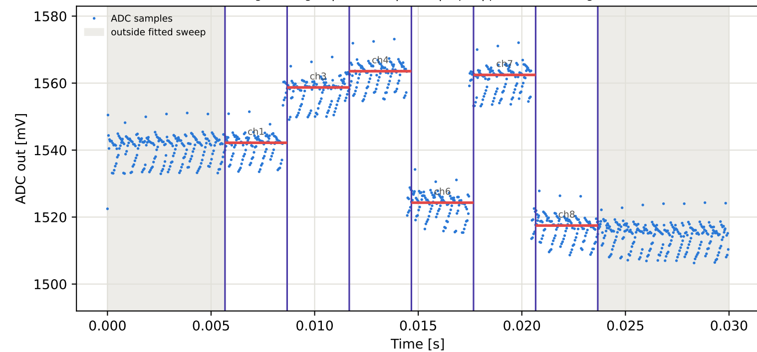
Tag5 &lt;- Tag3 | 895 MHz | run 0 | rep 1 | phase -51.44 deg
