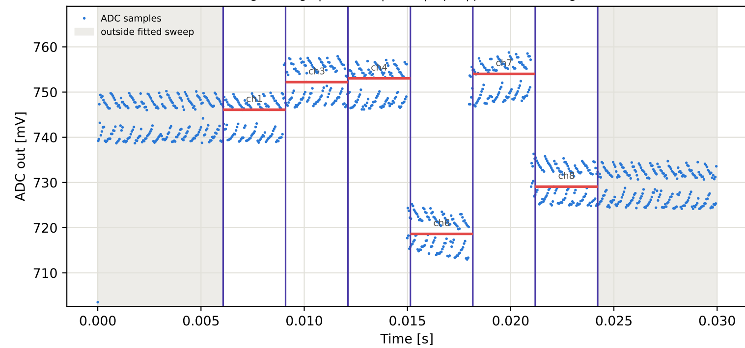
Tag9 &lt;- Tag7 | 935 MHz | run 0 | rep 1 | phase -13.68 deg
