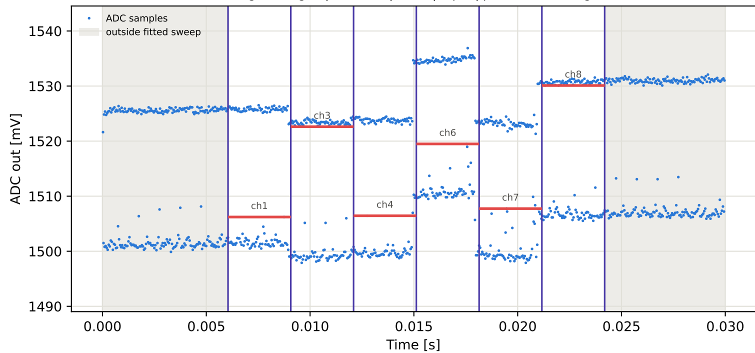
Tag4 &lt;- Tag16 | 925 MHz | run 0 | rep 1 | phase -13.46 deg
