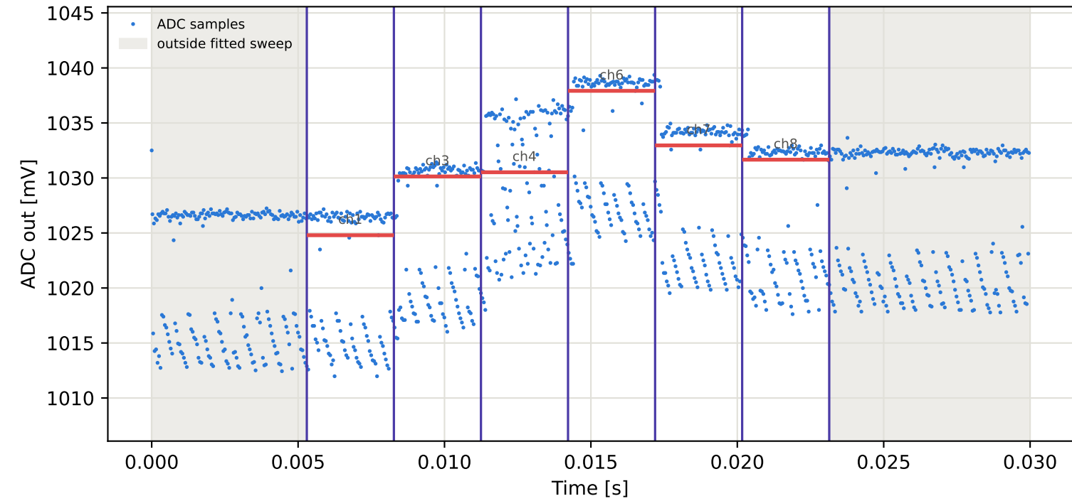
Tag15 &lt;- Tag6 | 875 MHz | run 0 | rep 1 | phase -45.96 deg
