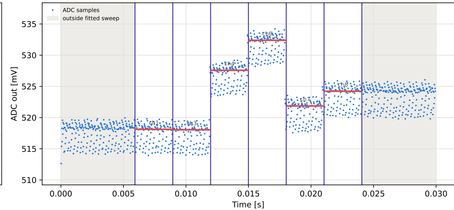
Tag3 &lt;- Tag9 | 965 MHz | run 0 | rep 1 | phase 128.03 deg
