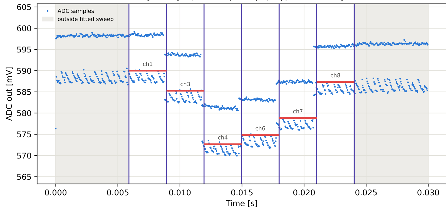
Tag6 &lt;- Tag10 | 945 MHz | run 0 | rep 1 | phase 57.67 deg
