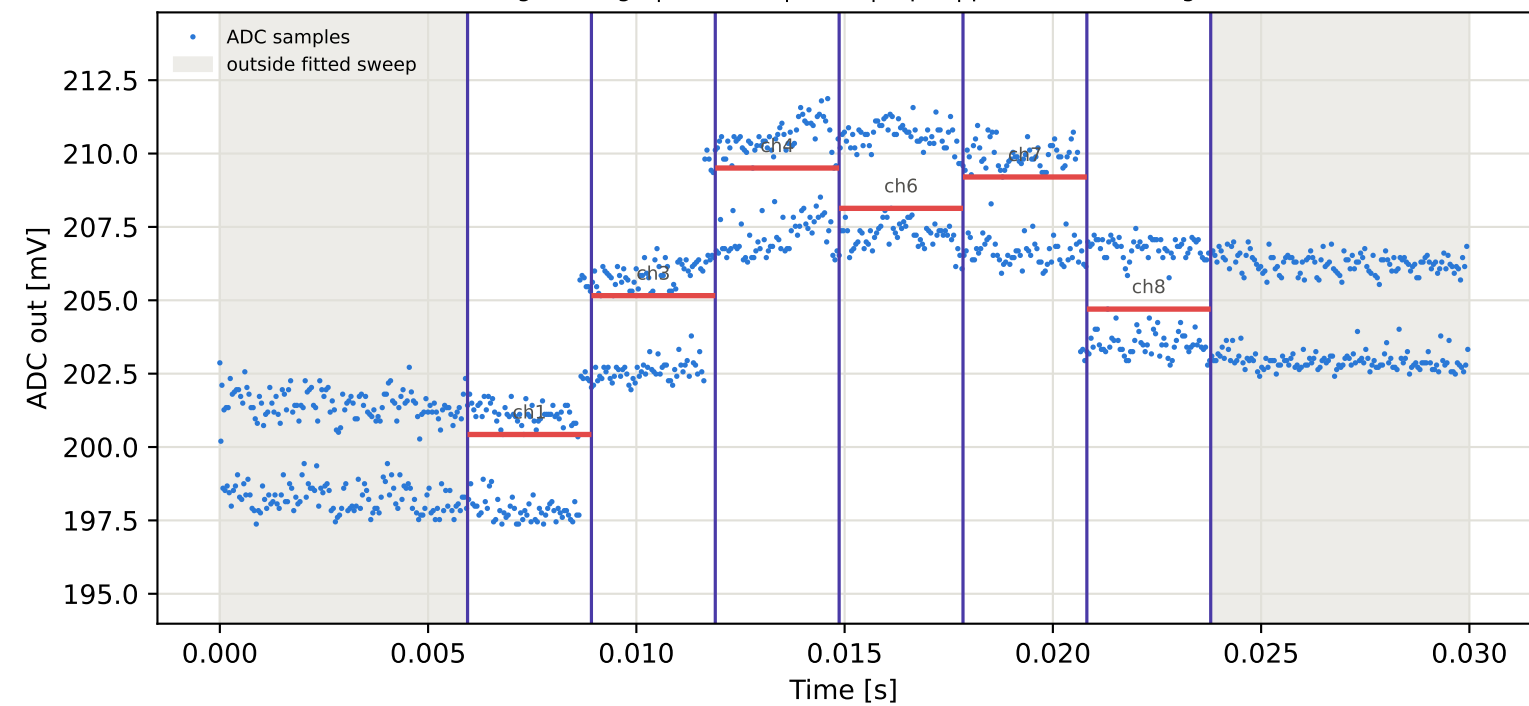
Tag2 &lt;- Tag8 | 855 MHz | run 0 | rep 1 | phase 168.54 deg
