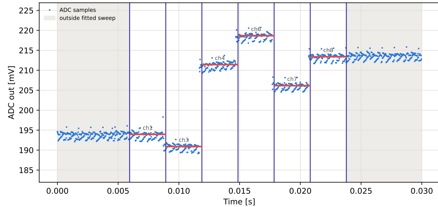
Tag9 &lt;- Tag2 | 855 MHz | run 0 | rep 1 | phase 19.53 deg
