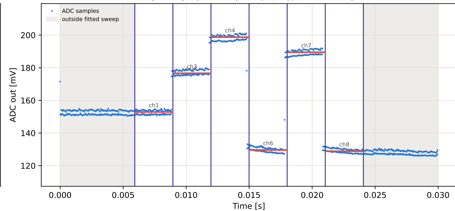
Tag5 &lt;- Tag2 | 965 MHz | run 0 | rep 1 | phase -7.13 deg
