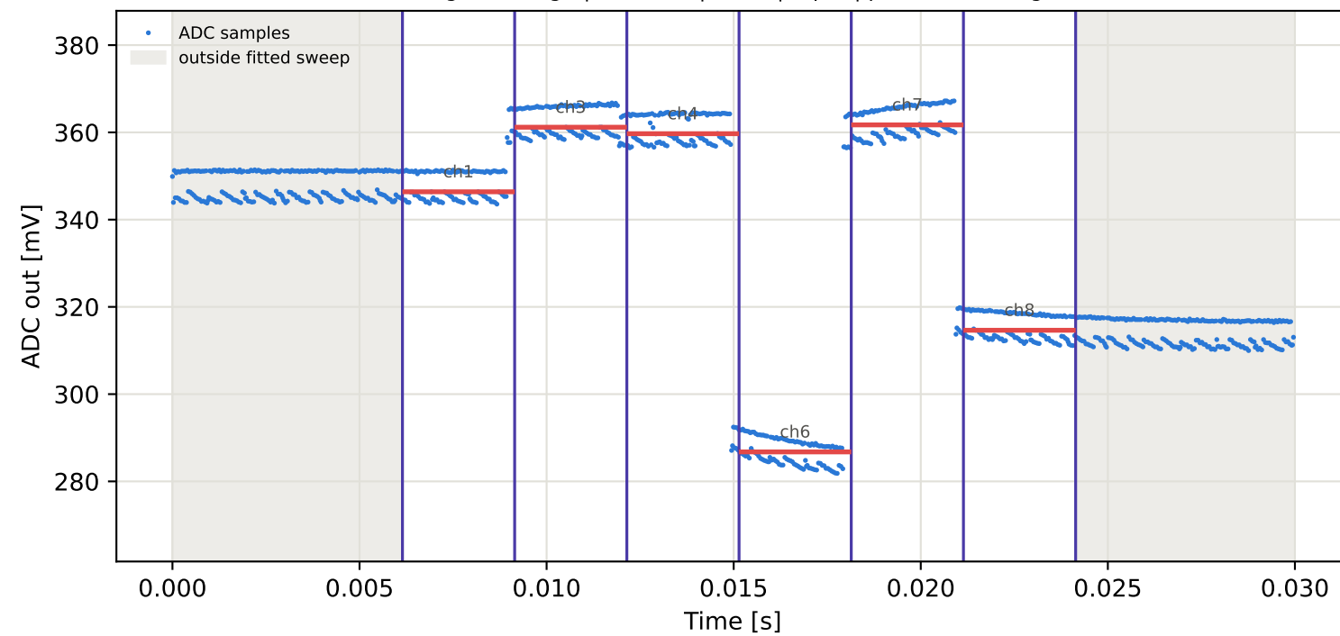
Tag10 &lt;- Tag8 | 925 MHz | run 0 | rep 1 | phase -11.38 deg
