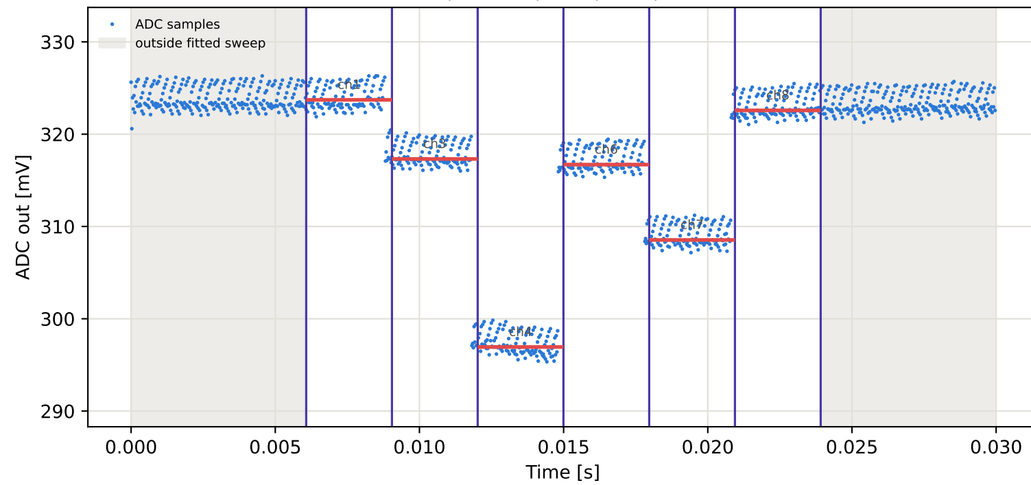
Tag3 &lt;- Tag16 | 995 MHz | run 0 | rep 1 | phase 74.57 deg
