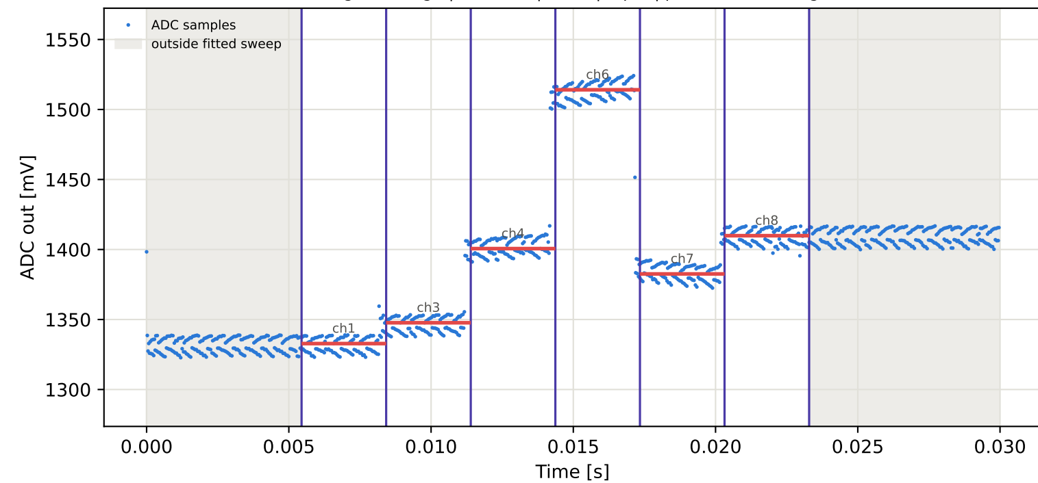
Tag16 &lt;- Tag1 | 905 MHz | run 0 | rep 1 | phase 151.26 deg
