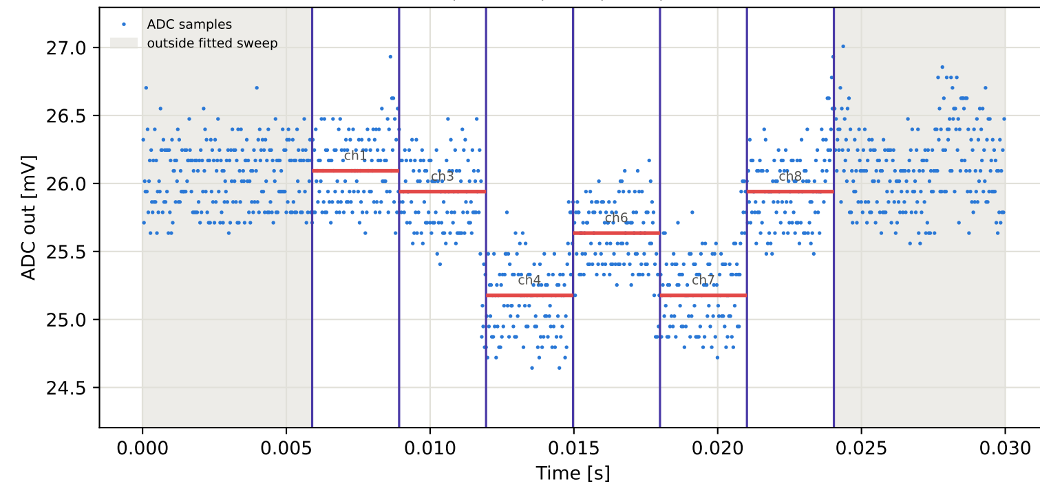
Tag7 &lt;- Tag5 | 775 MHz | run 0 | rep 1 | phase 91.53 deg
