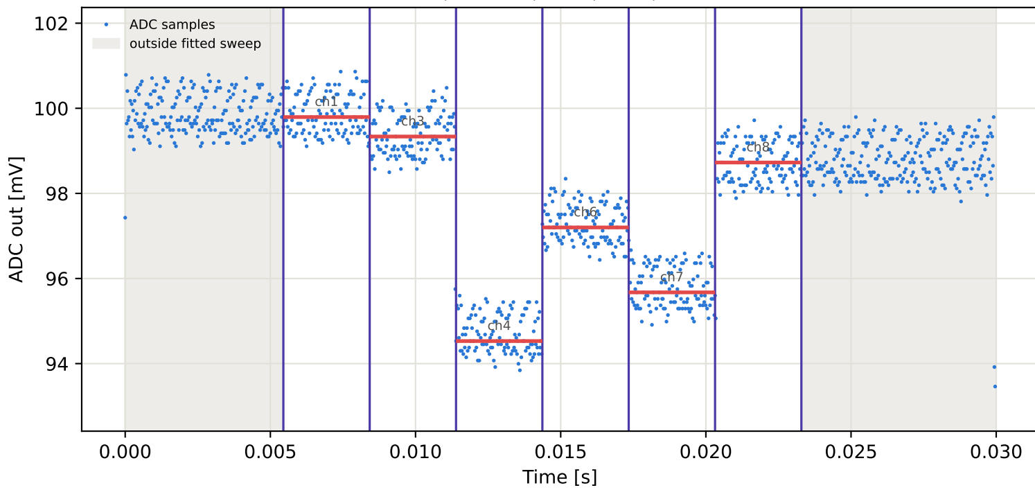
Tag7 &lt;- Tag15 | 795 MHz | run 0 | rep 1 | phase 84.80 deg
