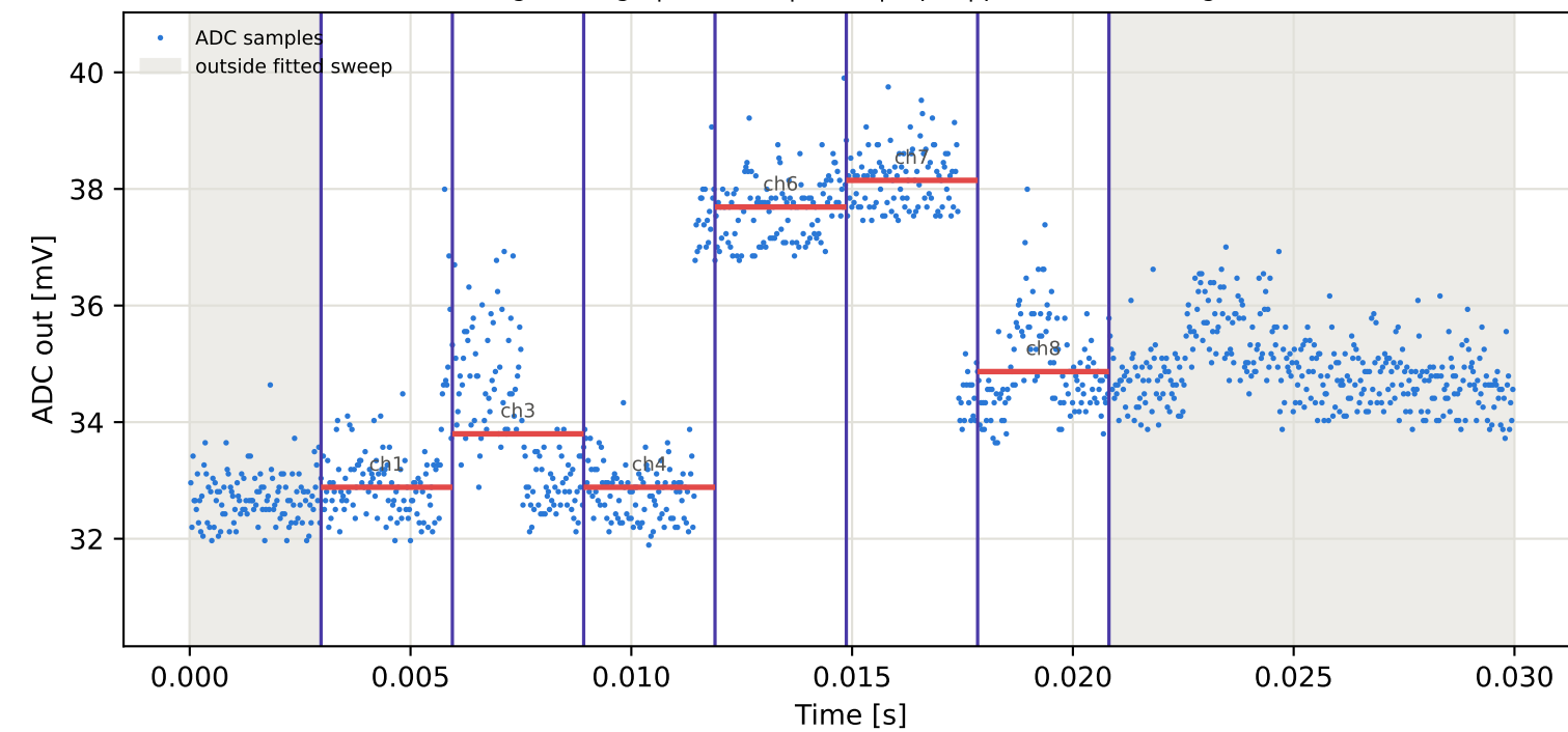
Tag2 &lt;- Tag5 | 975 MHz | run 0 | rep 1 | phase 153.31 deg
