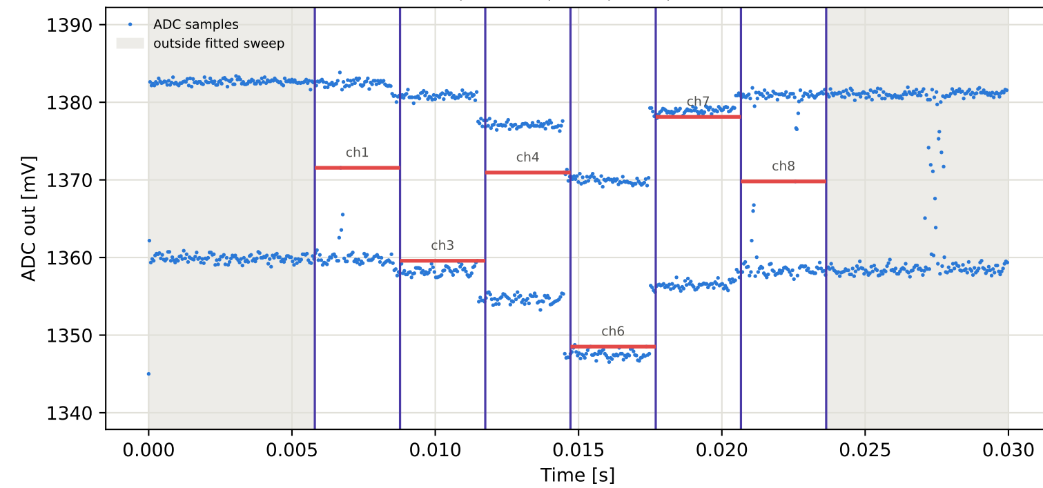
Tag4 &lt;- Tag2 | 935 MHz | run 0 | rep 1 | phase -7.79 deg
