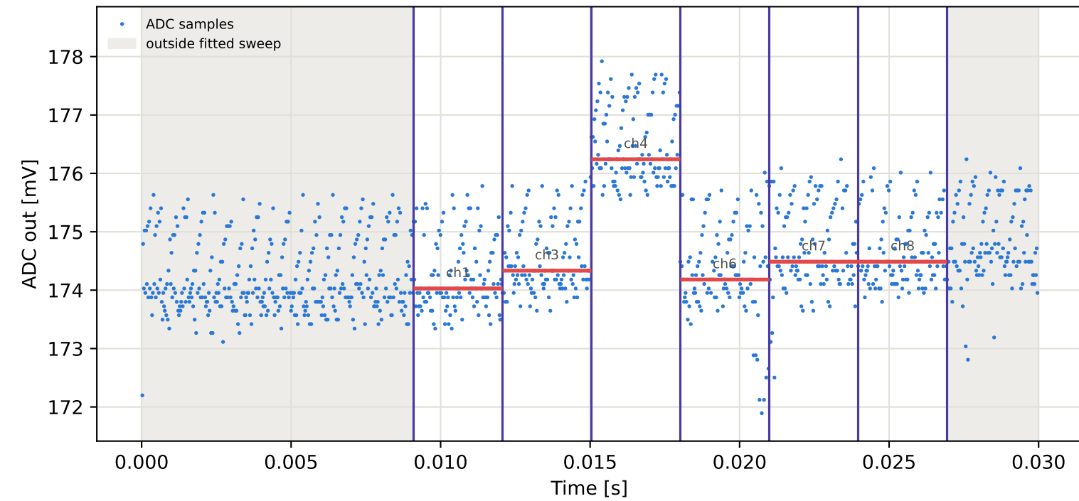
Tag10 &lt;- Tag4 | 985 MHz | run 0 | rep 1 | phase 15.84 deg
