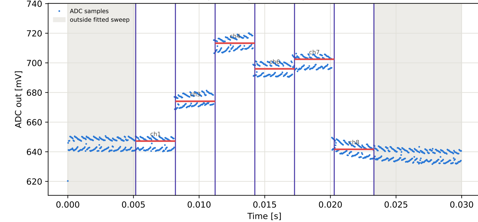
Tag9 &lt;- Tag16 | 905 MHz | run 0 | rep 1 | phase -104.56 deg
