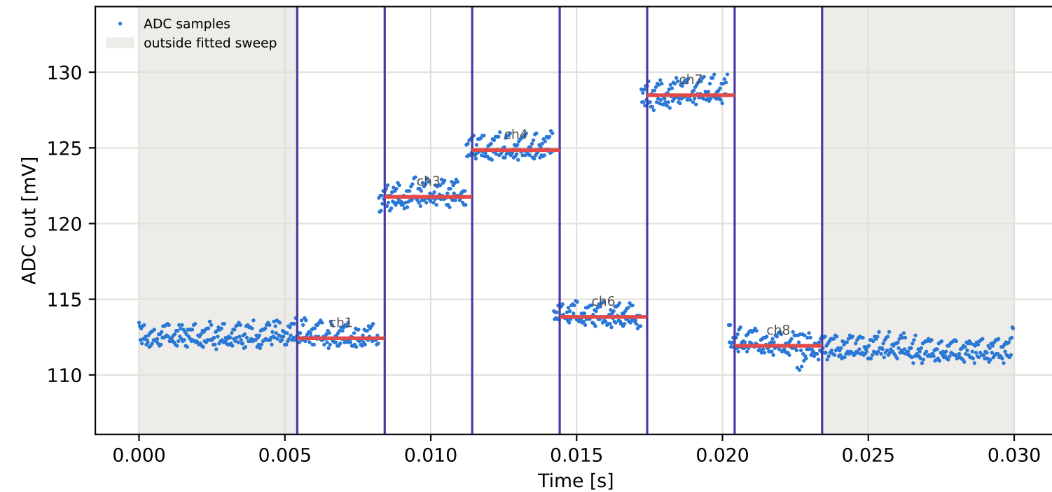
Tag6 &lt;- Tag1 | 785 MHz | run 0 | rep 1 | phase -10.90 deg
