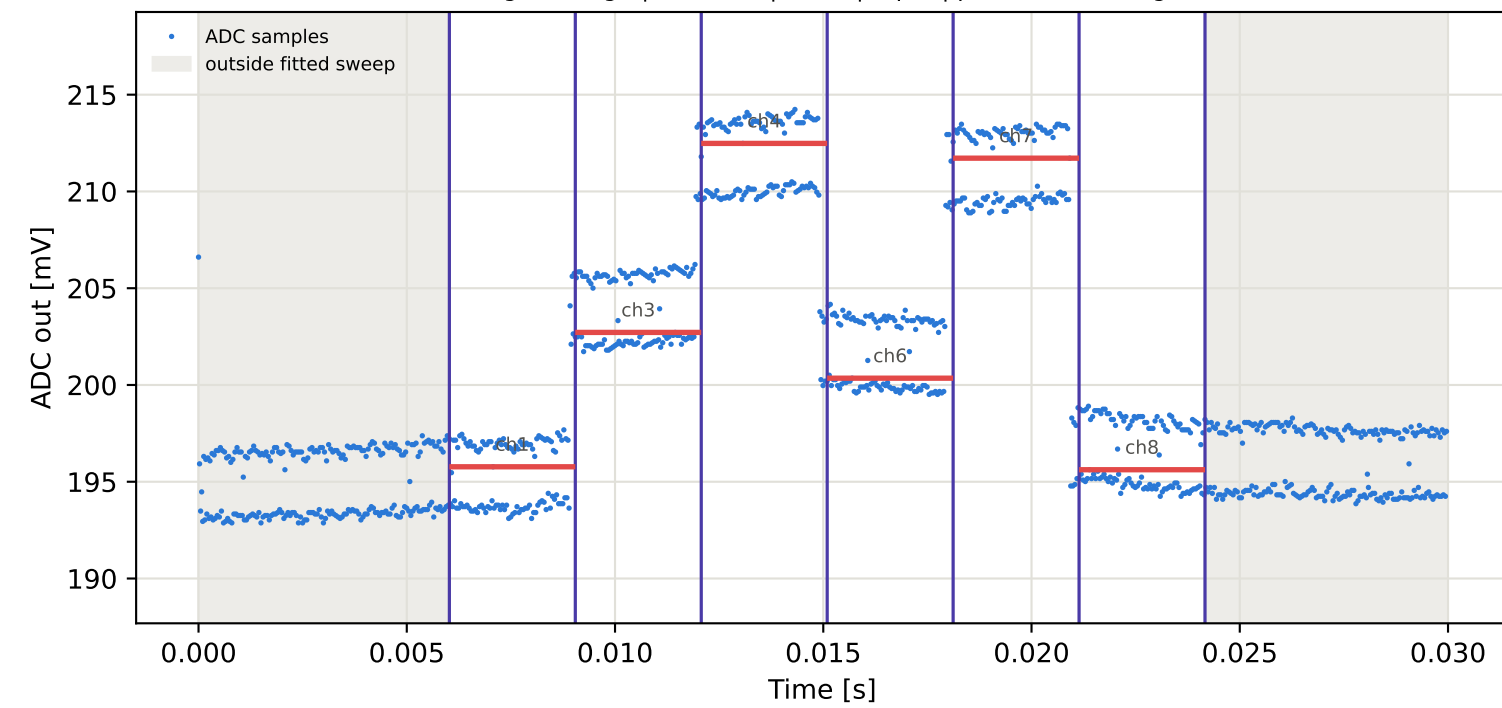
Tag6 &lt;- Tag9 | 835 MHz | run 0 | rep 1 | phase -94.88 deg
