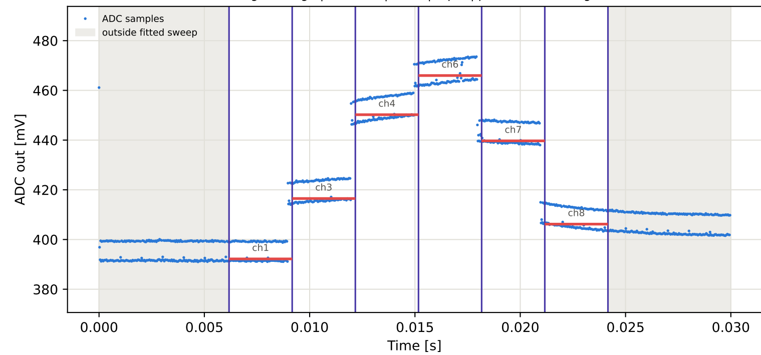
Tag1 &lt;- Tag4 | 905 MHz | run 0 | rep 1 | phase -126.23 deg
