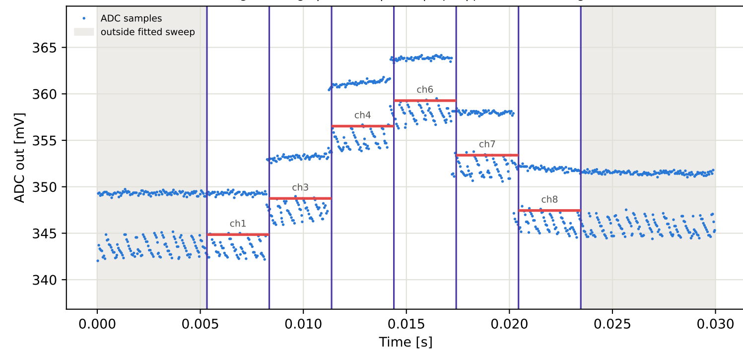
Tag15 &lt;- Tag10 | 925 MHz | run 0 | rep 1 | phase -95.36 deg
