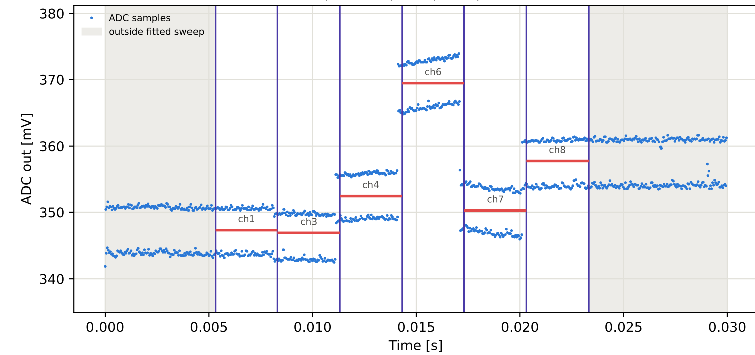
Tag2 &lt;- Tag16 | 905 MHz | run 0 | rep 1 | phase -163.51 deg
