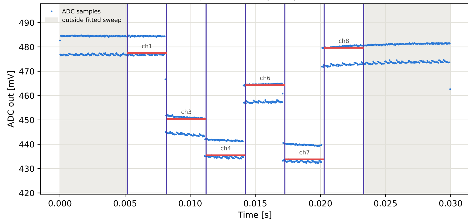
Tag16 &lt;- Tag1 | 845 MHz | run 0 | rep 1 | phase 18.78 deg
