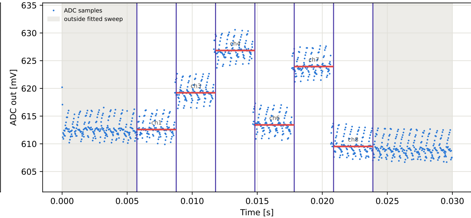
Tag7 &lt;- Tag15 | 945 MHz | run 0 | rep 1 | phase -17.25 deg
