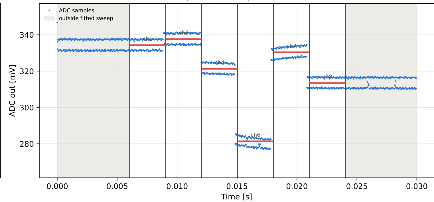
Tag1 &lt;- Tag8 | 935 MHz | run 0 | rep 1 | phase -11.74 deg
