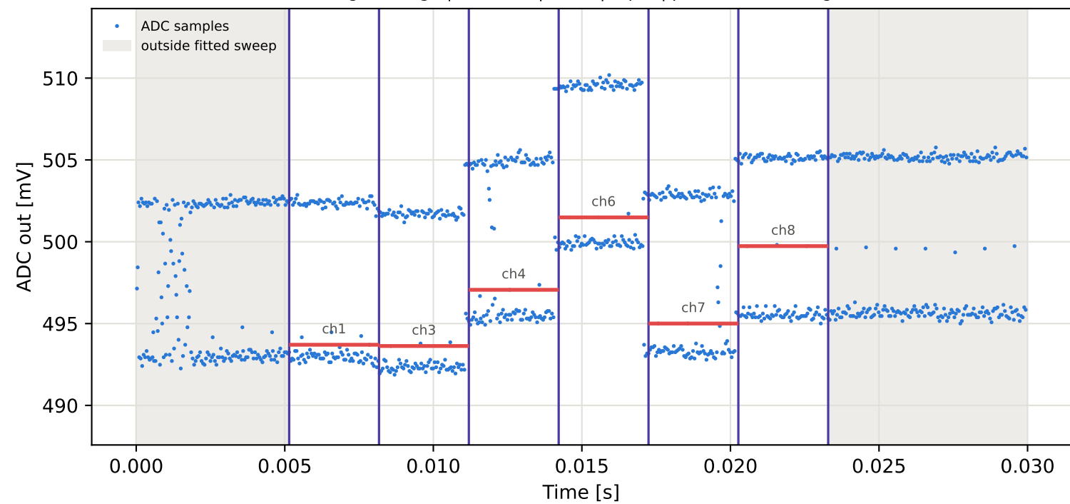
Tag1 &lt;- Tag7 | 965 MHz | run 0 | rep 1 | phase -16.24 deg
