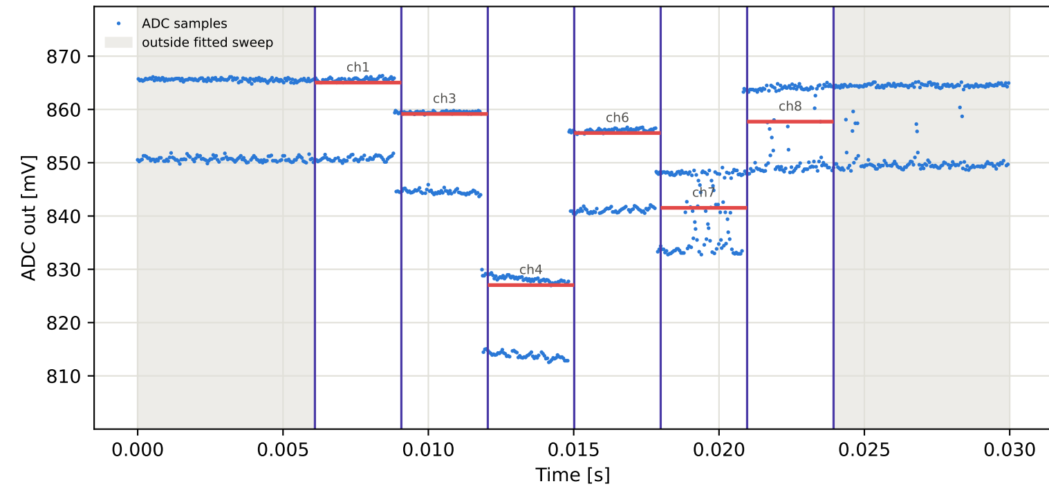
Tag16 &lt;- Tag6 | 995 MHz | run 0 | rep 1 | phase -59.92 deg
