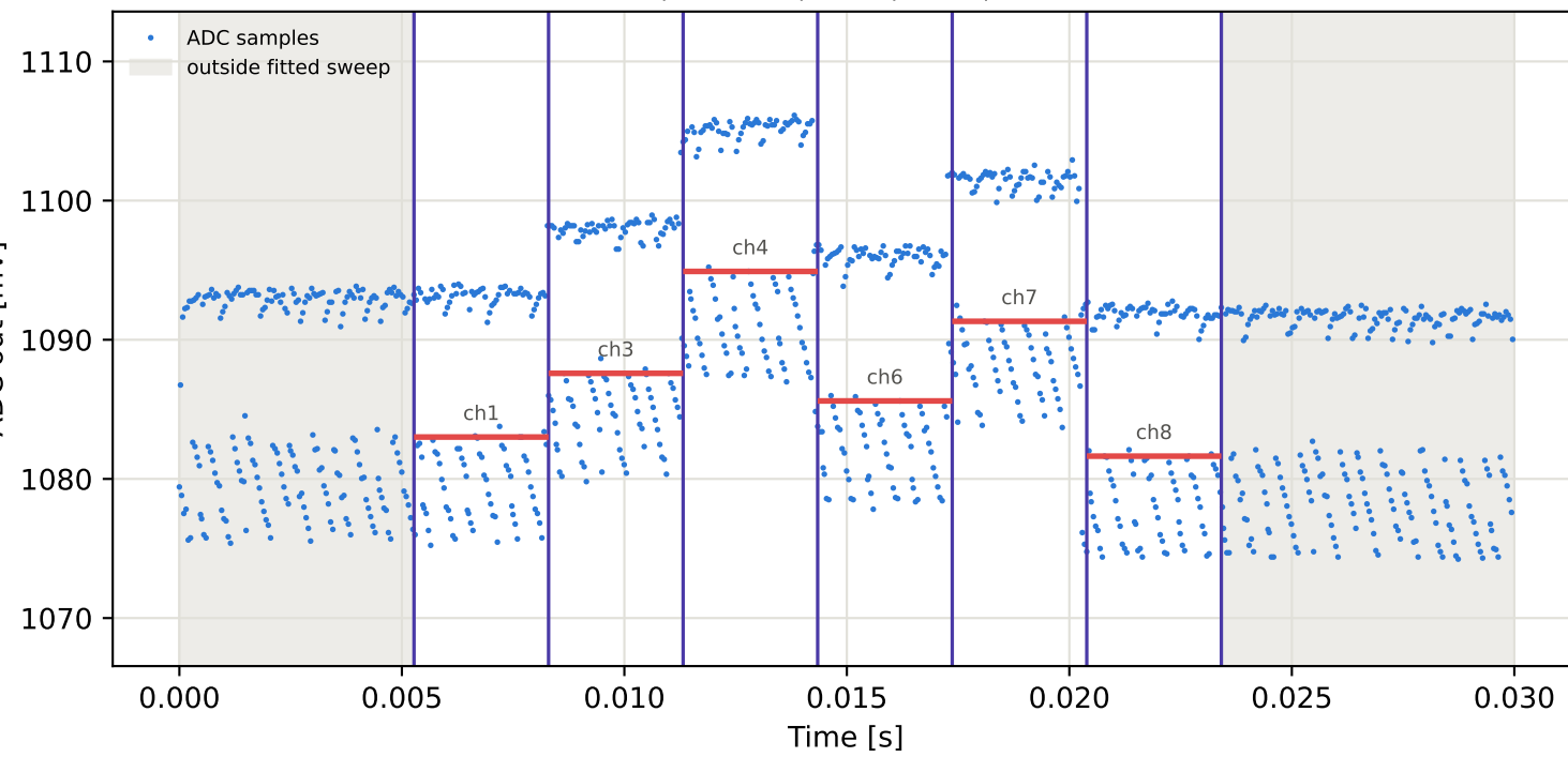
Tag15 &lt;- Tag1 | 975 MHz | run 0 | rep 1 | phase -91.26 deg
