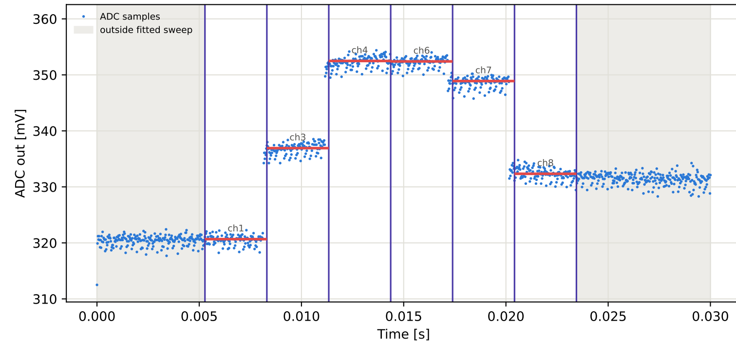
Tag1 &lt;- Tag9 | 885 MHz | run 0 | rep 1 | phase -134.30 deg
