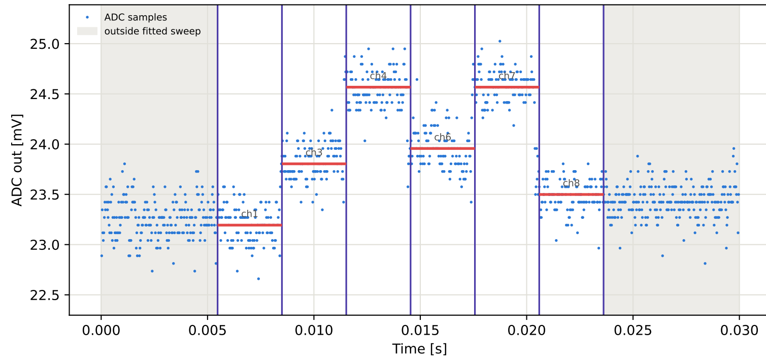
Tag7 &lt;- Tag10 | 795 MHz | run 0 | rep 1 | phase -46.36 deg
