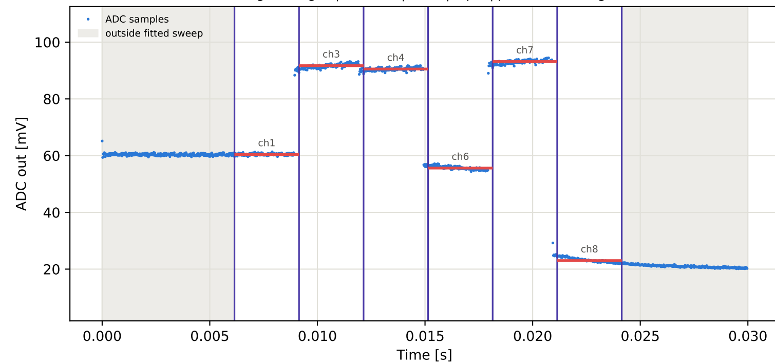
Tag9 &lt;- Tag16 | 865 MHz | run 0 | rep 1 | phase -44.09 deg
