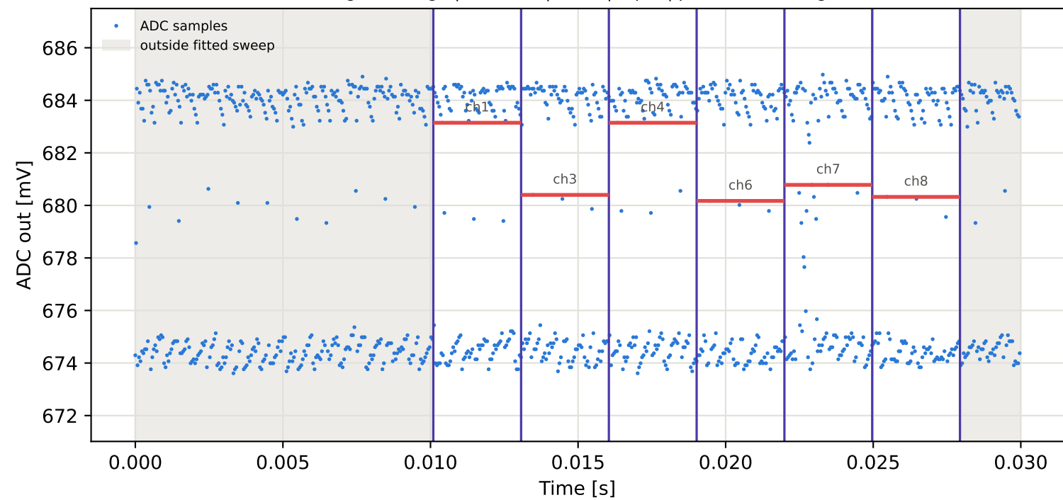
Tag16 &lt;- Tag4 | 825 MHz | run 0 | rep 1 | phase 85.87 deg
