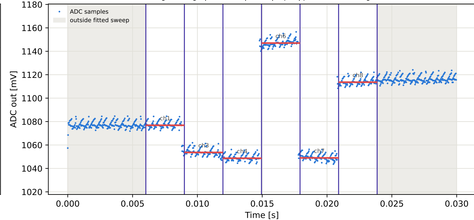
Tag4 &lt;- Tag3 | 945 MHz | run 0 | rep 1 | phase 161.37 deg
