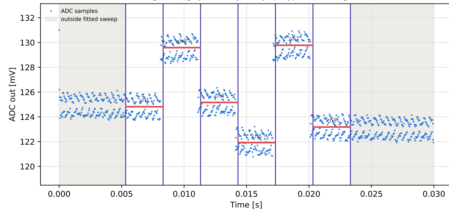
Tag16 &lt;- Tag6 | 775 MHz | run 0 | rep 1 | phase -140.30 deg
