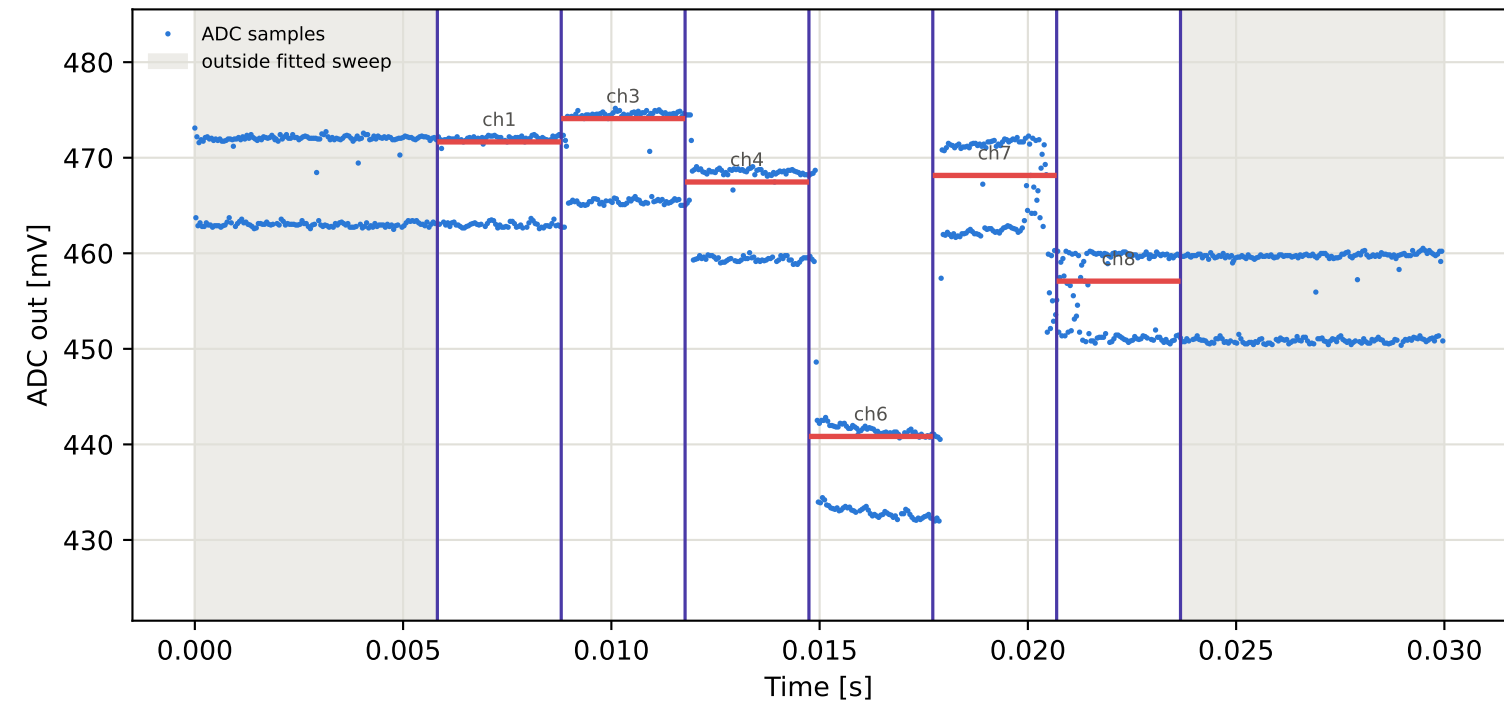
Tag6 &lt;- Tag5 | 925 MHz | run 0 | rep 1 | phase -67.43 deg
