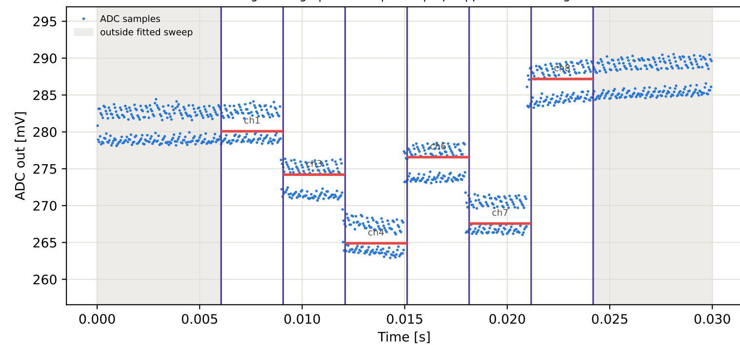
Tag1 &lt;- Tag7 | 915 MHz | run 0 | rep 1 | phase -150.59 deg
