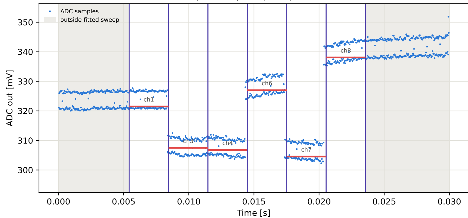
Tag2 &lt;- Tag6 | 875 MHz | run 0 | rep 1 | phase -93.40 deg
