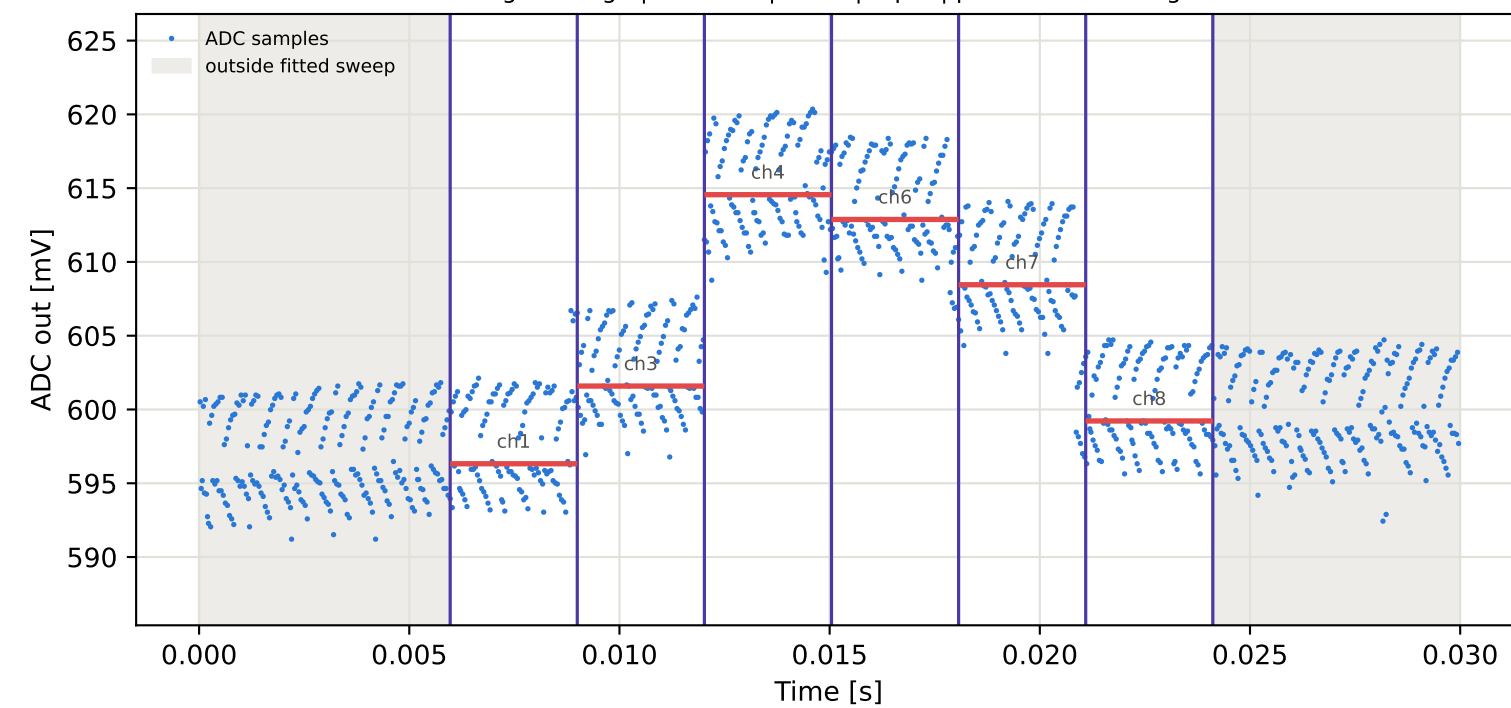
Tag5 &lt;- Tag8 | 935 MHz | run 0 | rep 1 | phase 144.90 deg
