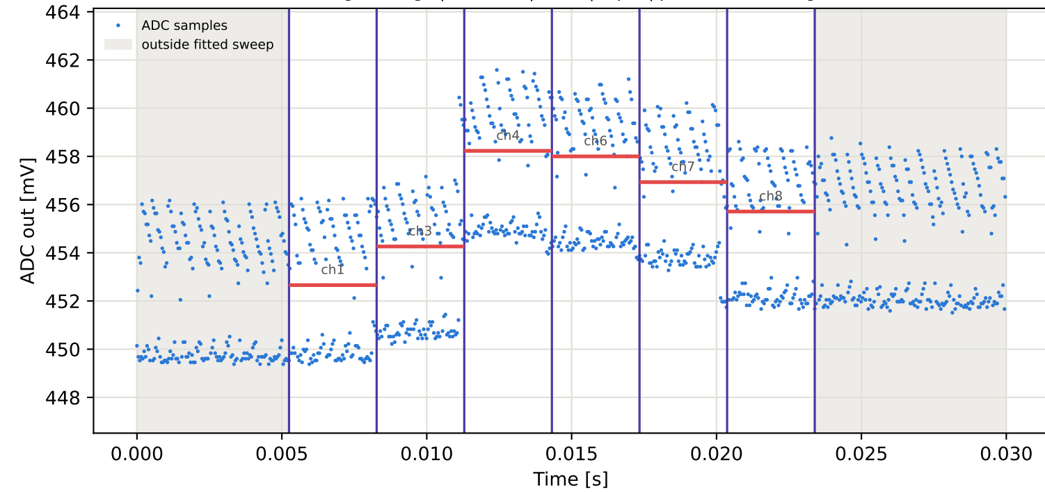
Tag5 &lt;- Tag9 | 845 MHz | run 0 | rep 1 | phase -64.84 deg
