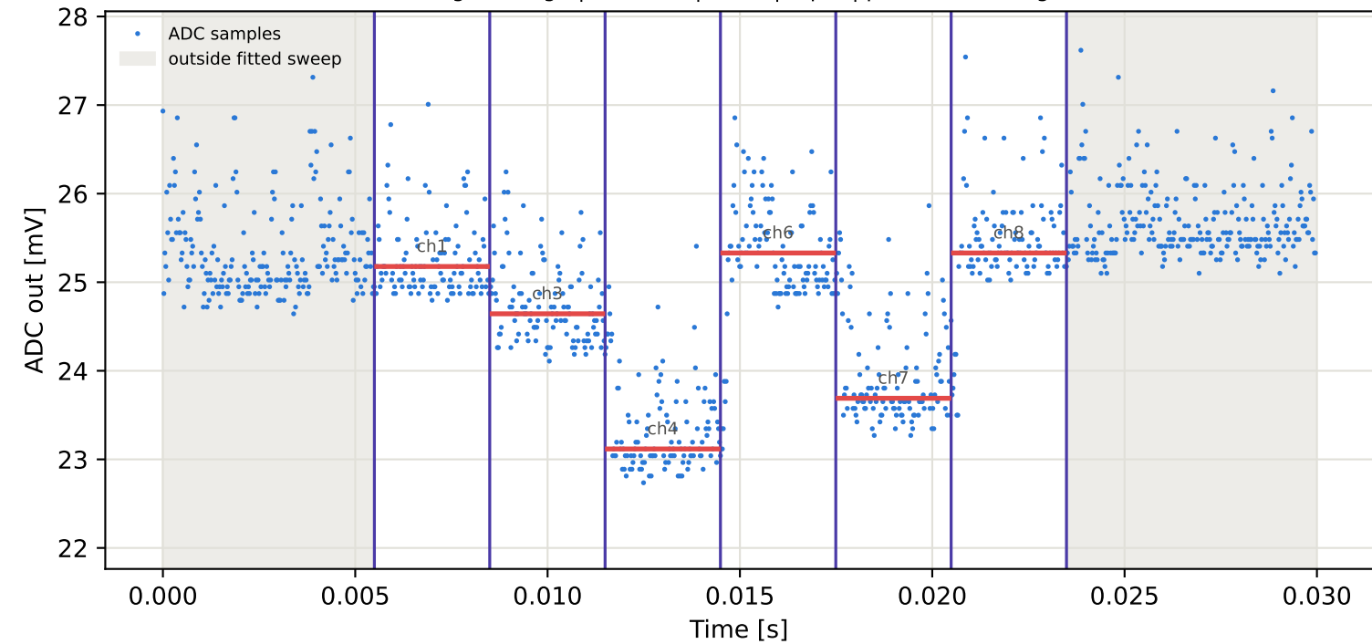
Tag2 &lt;- Tag8 | 965 MHz | run 0 | rep 1 | phase 77.55 deg
