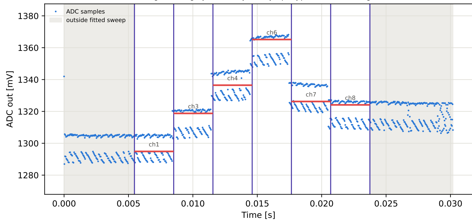
Tag15 &lt;- Tag6 | 895 MHz | run 0 | rep 1 | phase -168.65 deg
