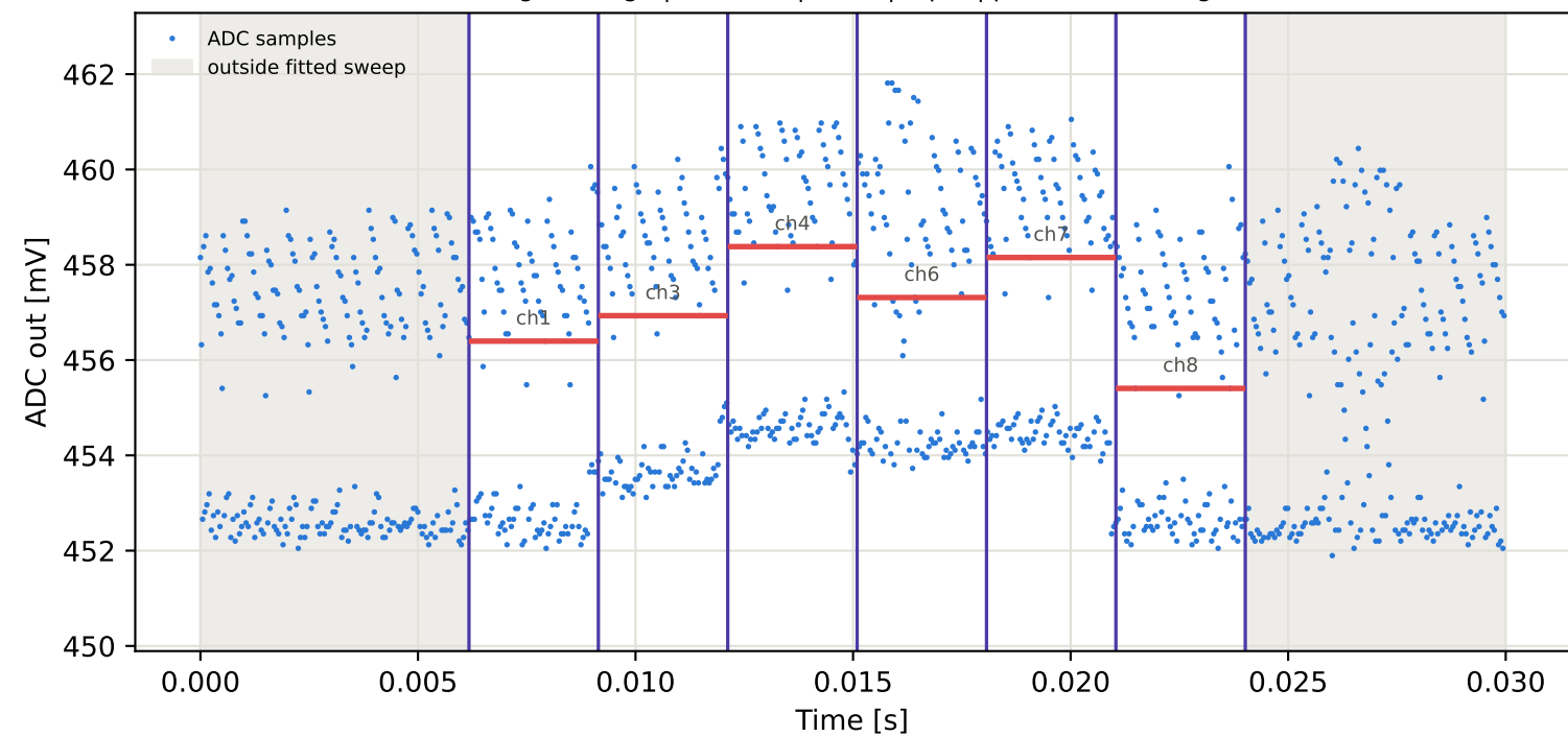
Tag5 &lt;- Tag4 | 845 MHz | run 0 | rep 1 | phase 13.56 deg
