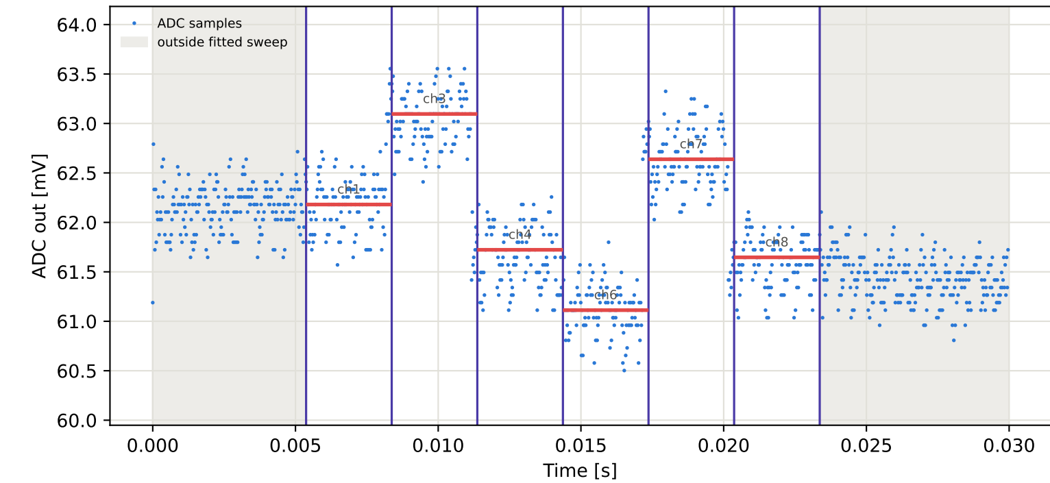
Tag16 &lt;- Tag15 | 785 MHz | run 0 | rep 1 | phase -10.36 deg
