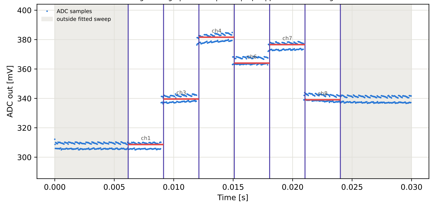
Tag9 &lt;- Tag8 | 835 MHz | run 0 | rep 1 | phase -104.57 deg
