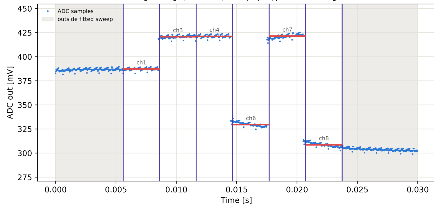
Tag8 &lt;- Tag1 | 895 MHz | run 0 | rep 1 | phase -5.13 deg
