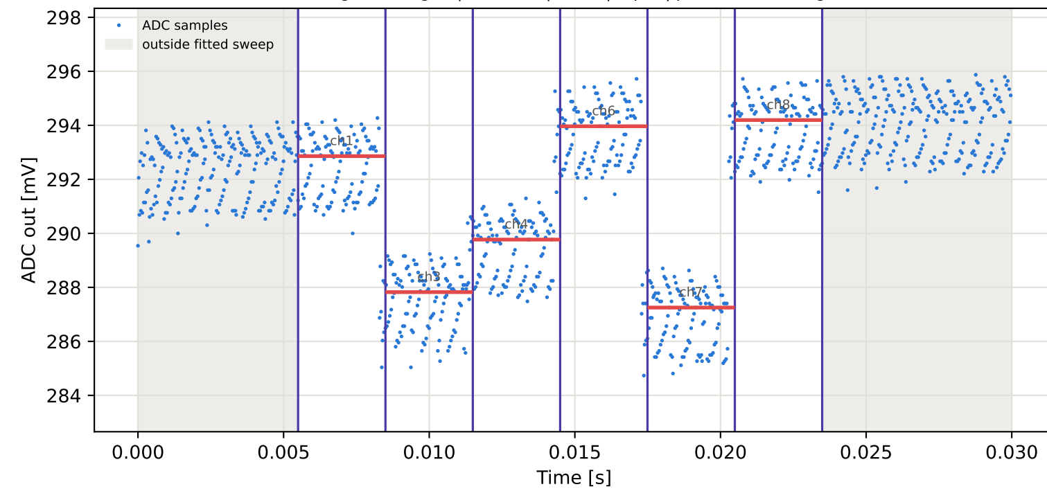
Tag15 &lt;- Tag3 | 785 MHz | run 0 | rep 1 | phase -61.40 deg
