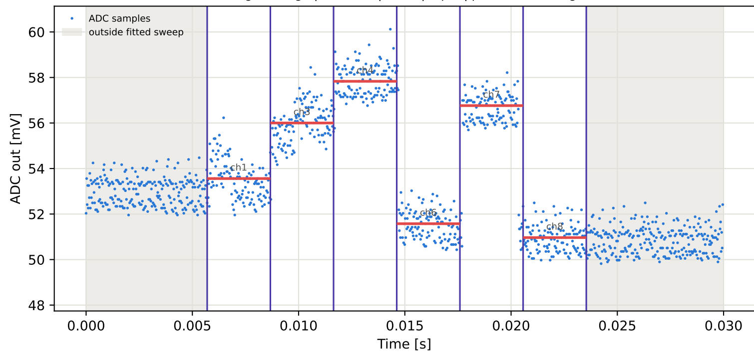
Tag2 &lt;- Tag8 | 945 MHz | run 0 | rep 1 | phase 4.13 deg
