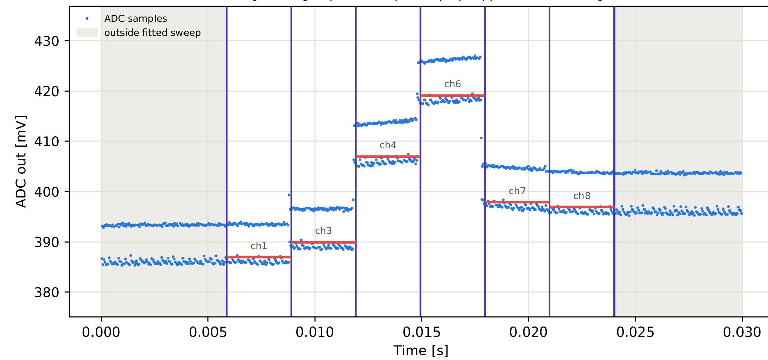
Tag1 &lt;- Tag16 | 945 MHz | run 0 | rep 1 | phase -56.97 deg
