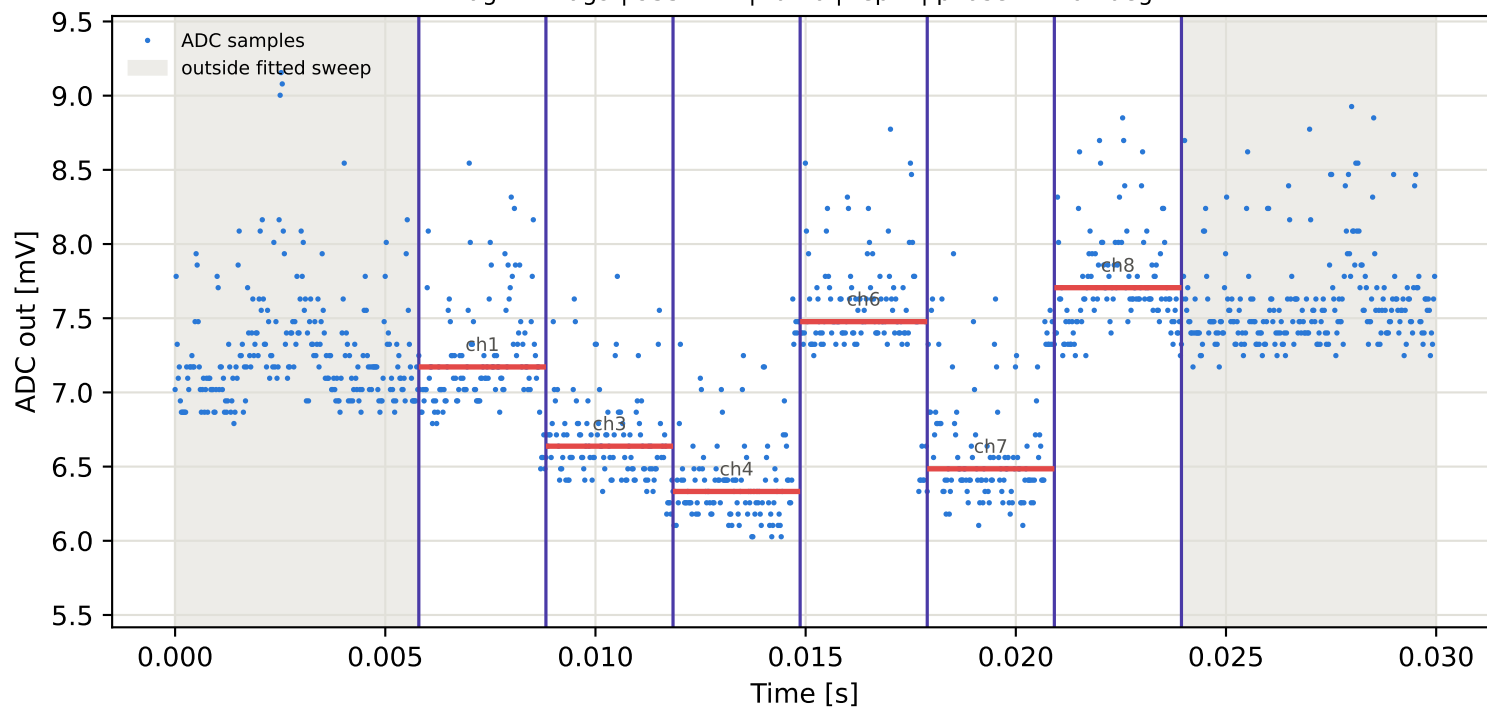
Tag3 &lt;- Tag10 | 955 MHz | run 0 | rep 1 | phase 154.86 deg
