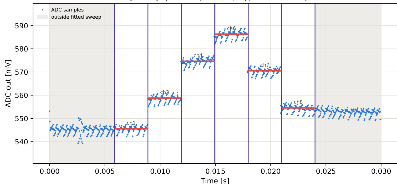
Tag6 &lt;- Tag5 | 895 MHz | run 0 | rep 1 | phase -129.03 deg
