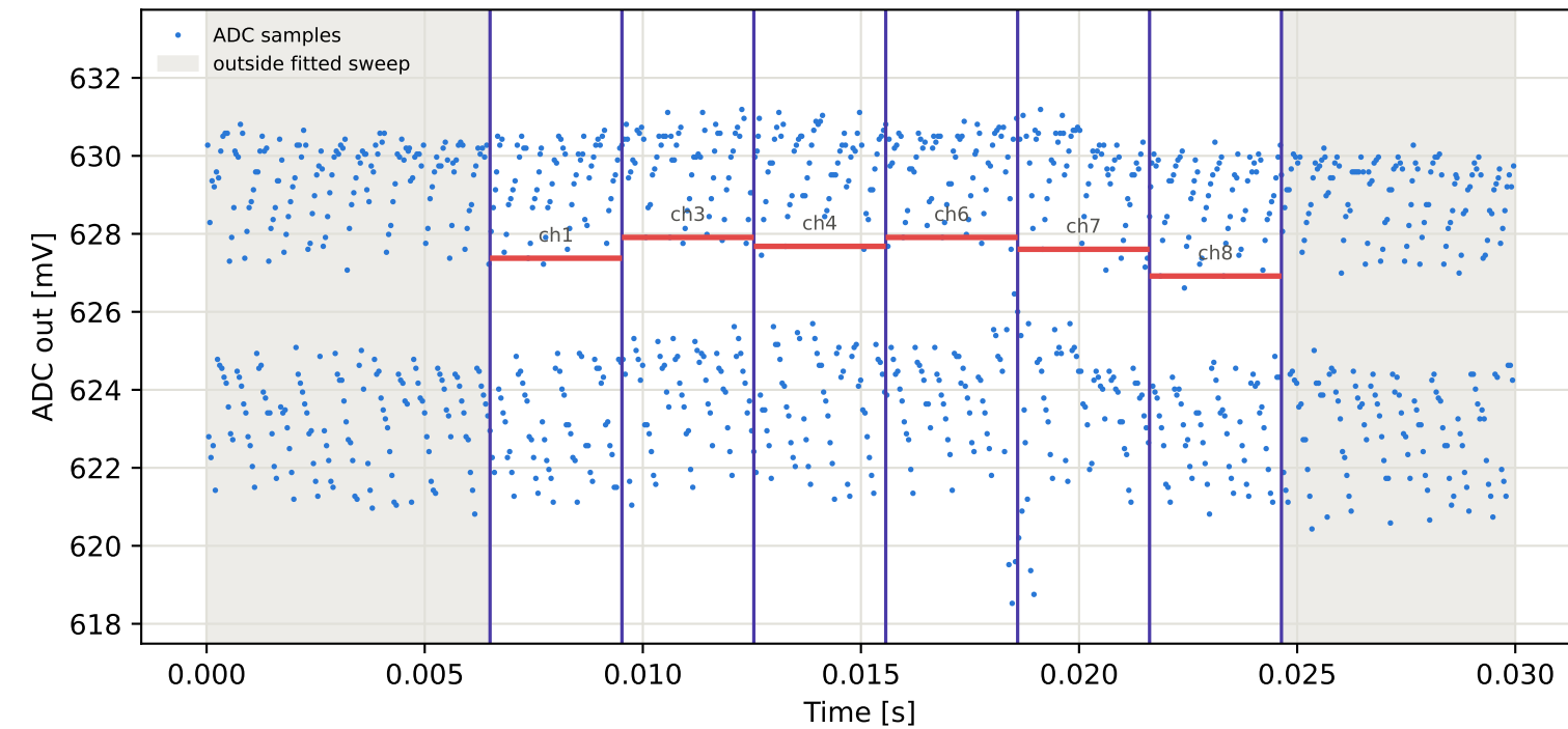
Tag6 &lt;- Tag4 | 965 MHz | run 0 | rep 1 | phase -70.01 deg
