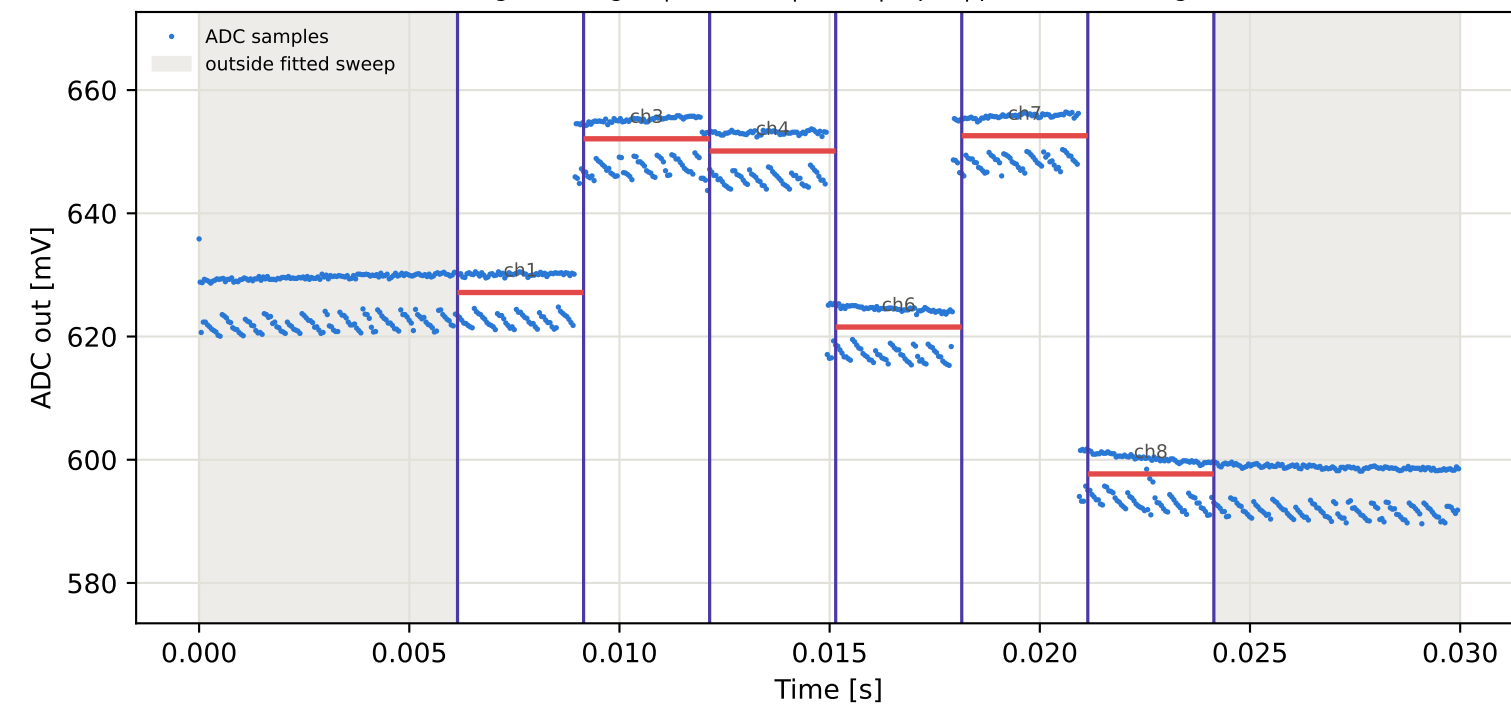
Tag15 &lt;- Tag3 | 865 MHz | run 0 | rep 1 | phase -12.06 deg
