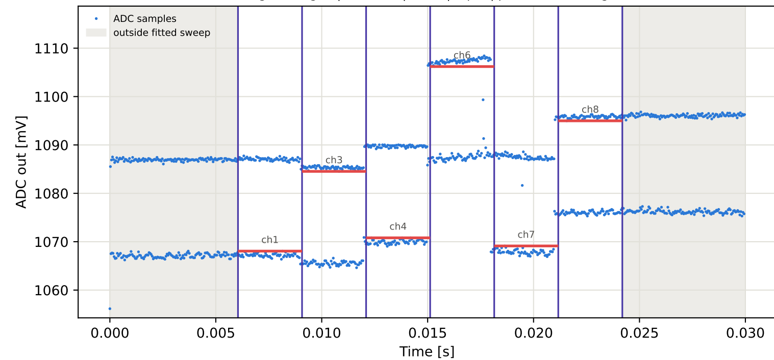
Tag5 &lt;- Tag16 | 925 MHz | run 0 | rep 1 | phase -46.12 deg
