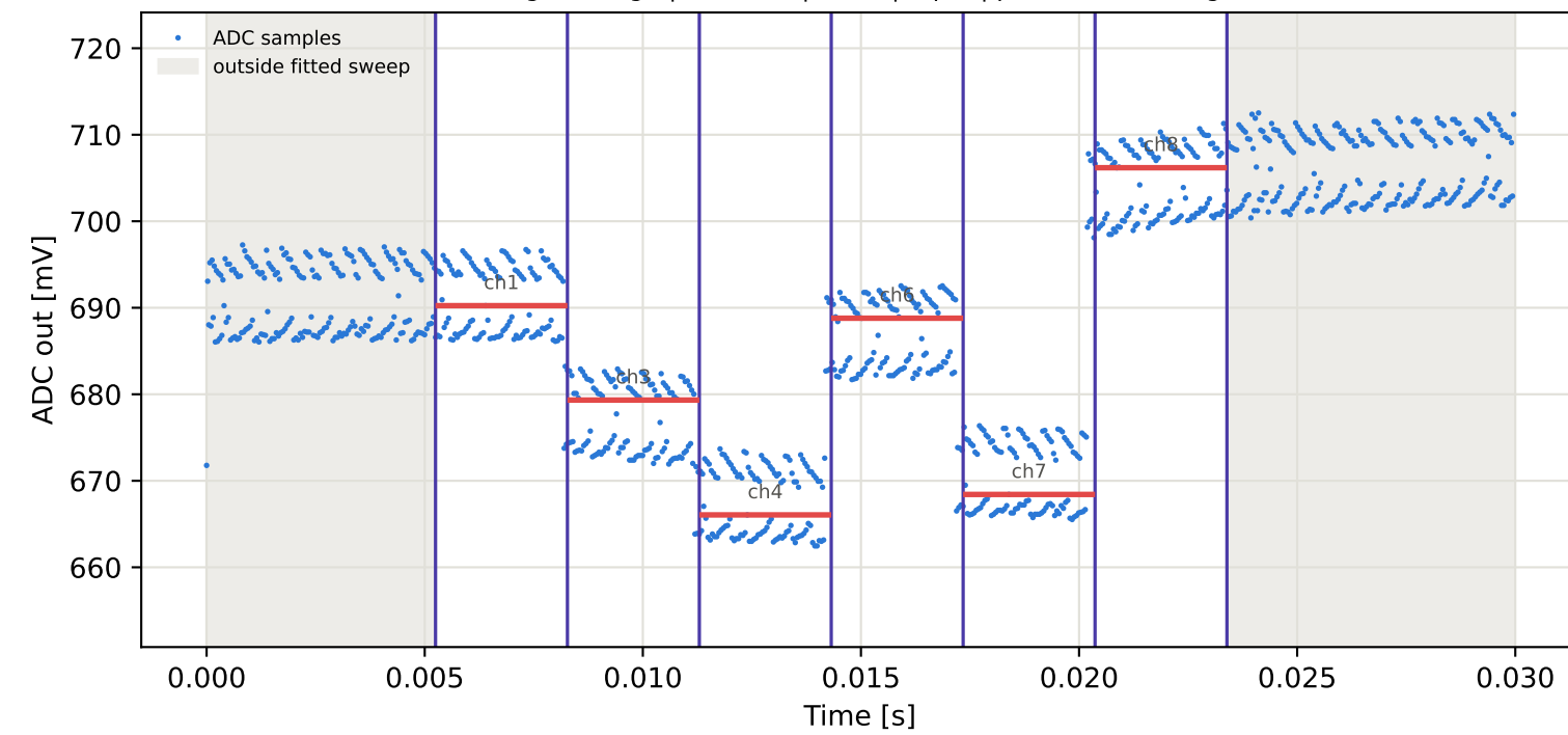
Tag9 &lt;- Tag5 | 905 MHz | run 0 | rep 1 | phase -3.02 deg
