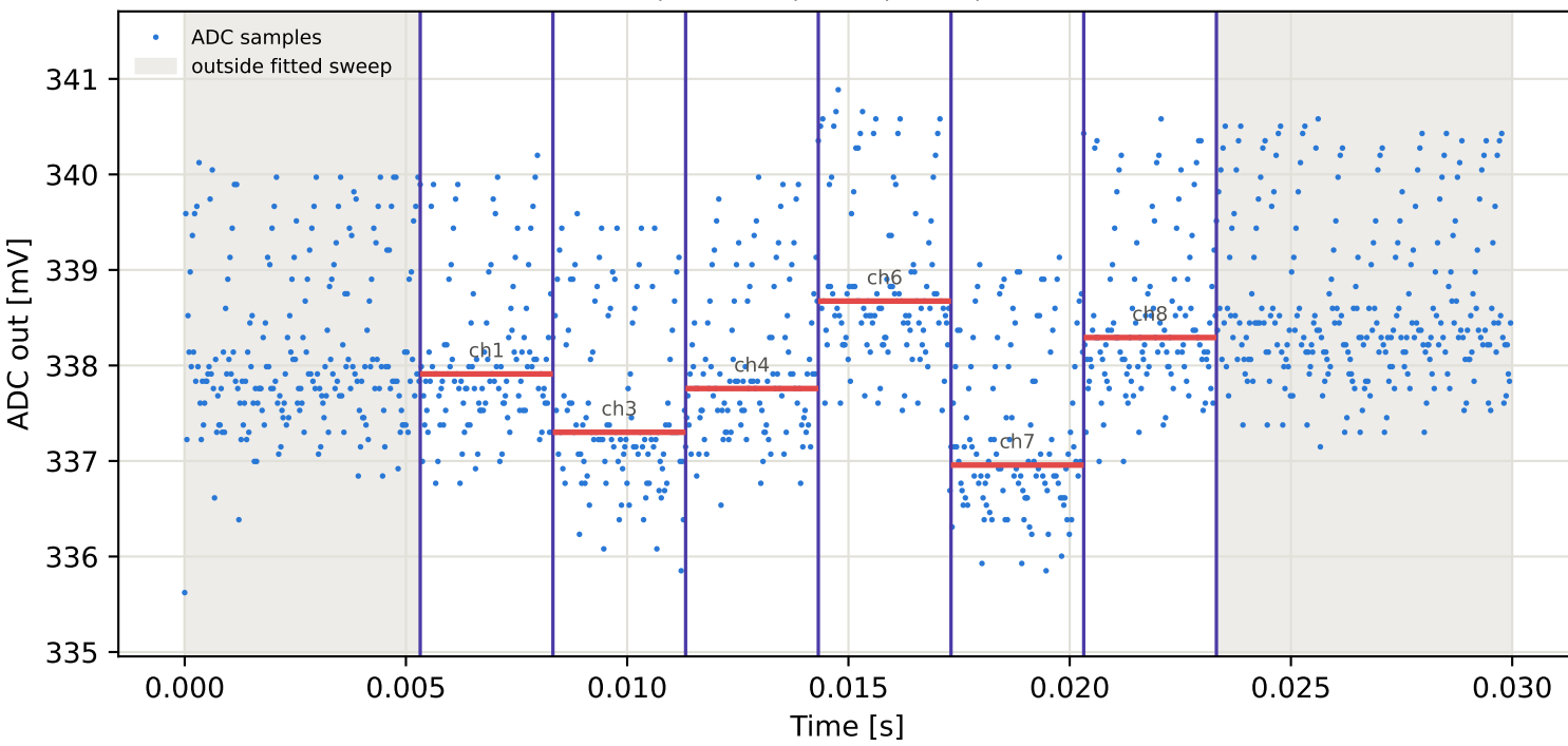
Tag15 &lt;- Tag1 | 775 MHz | run 0 | rep 1 | phase -178.85 deg
