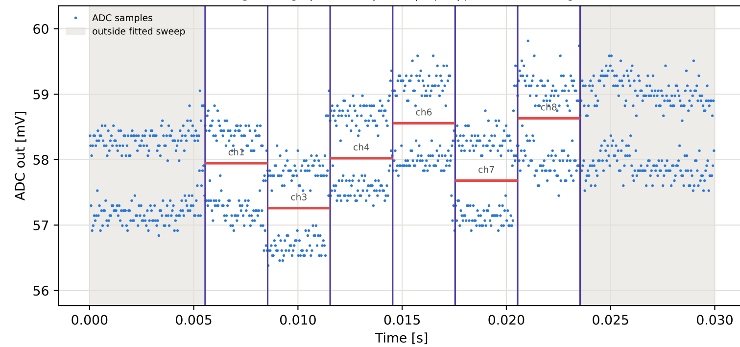
Tag5 &lt;- Tag8 | 795 MHz | run 0 | rep 1 | phase 0.56 deg
