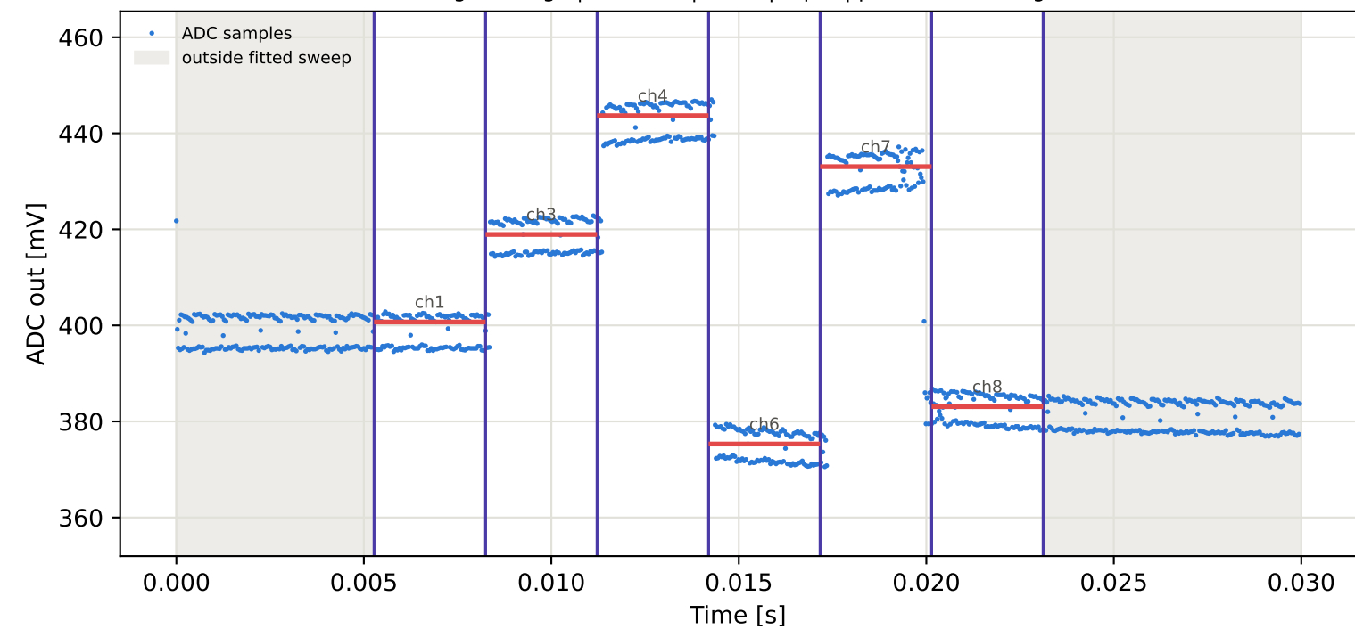
Tag4 &lt;- Tag3 | 985 MHz | run 0 | rep 1 | phase -54.67 deg
