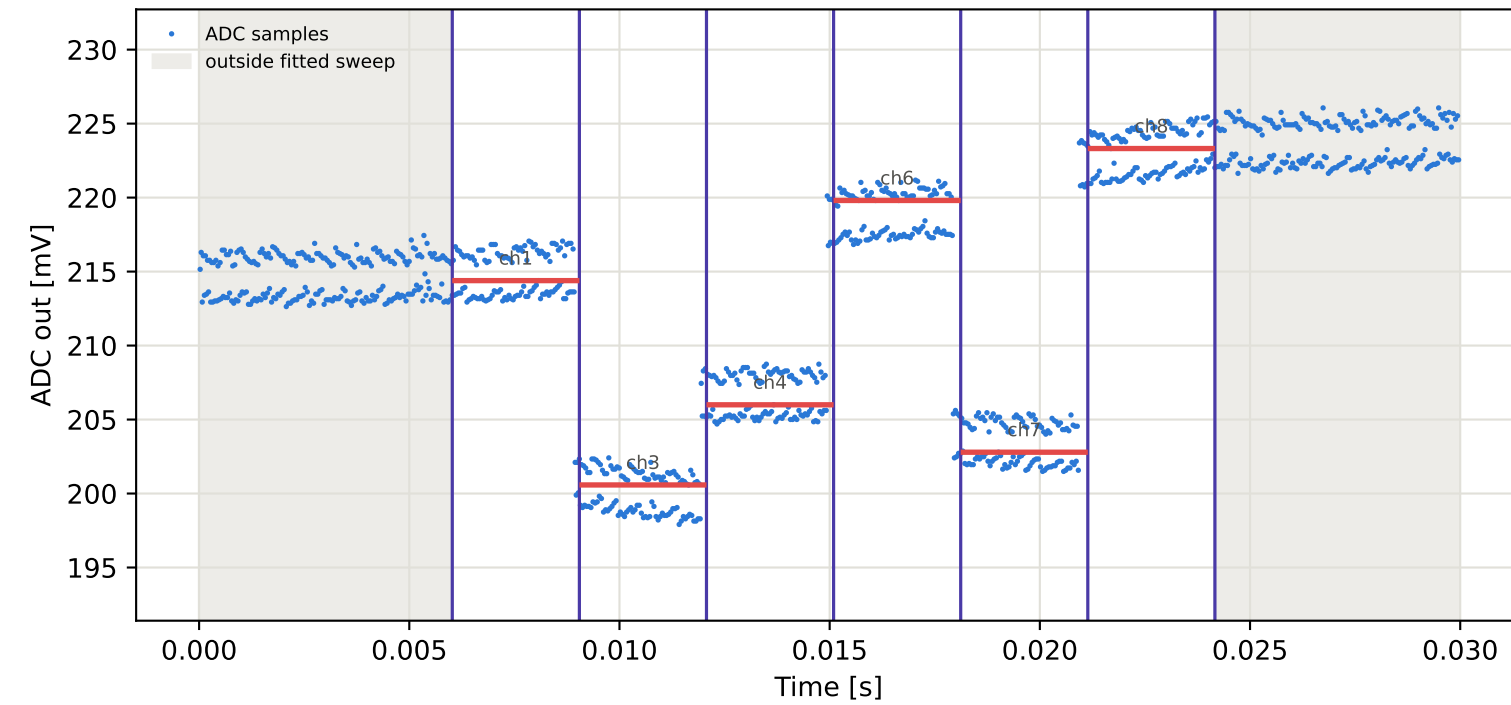
Tag9 &lt;- Tag7 | 855 MHz | run 0 | rep 1 | phase -139.70 deg
