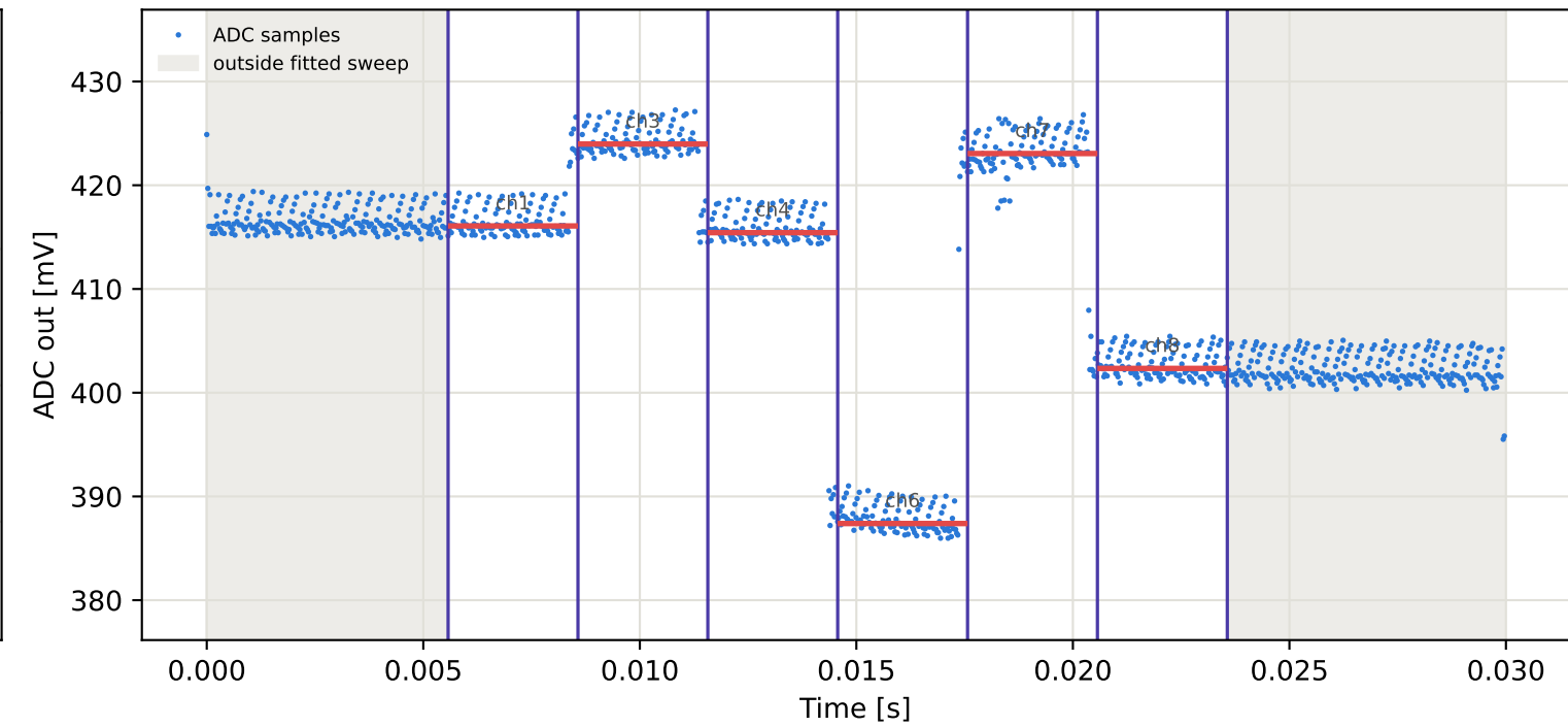
Tag10 &lt;- Tag1 | 975 MHz | run 0 | rep 1 | phase -166.66 deg
