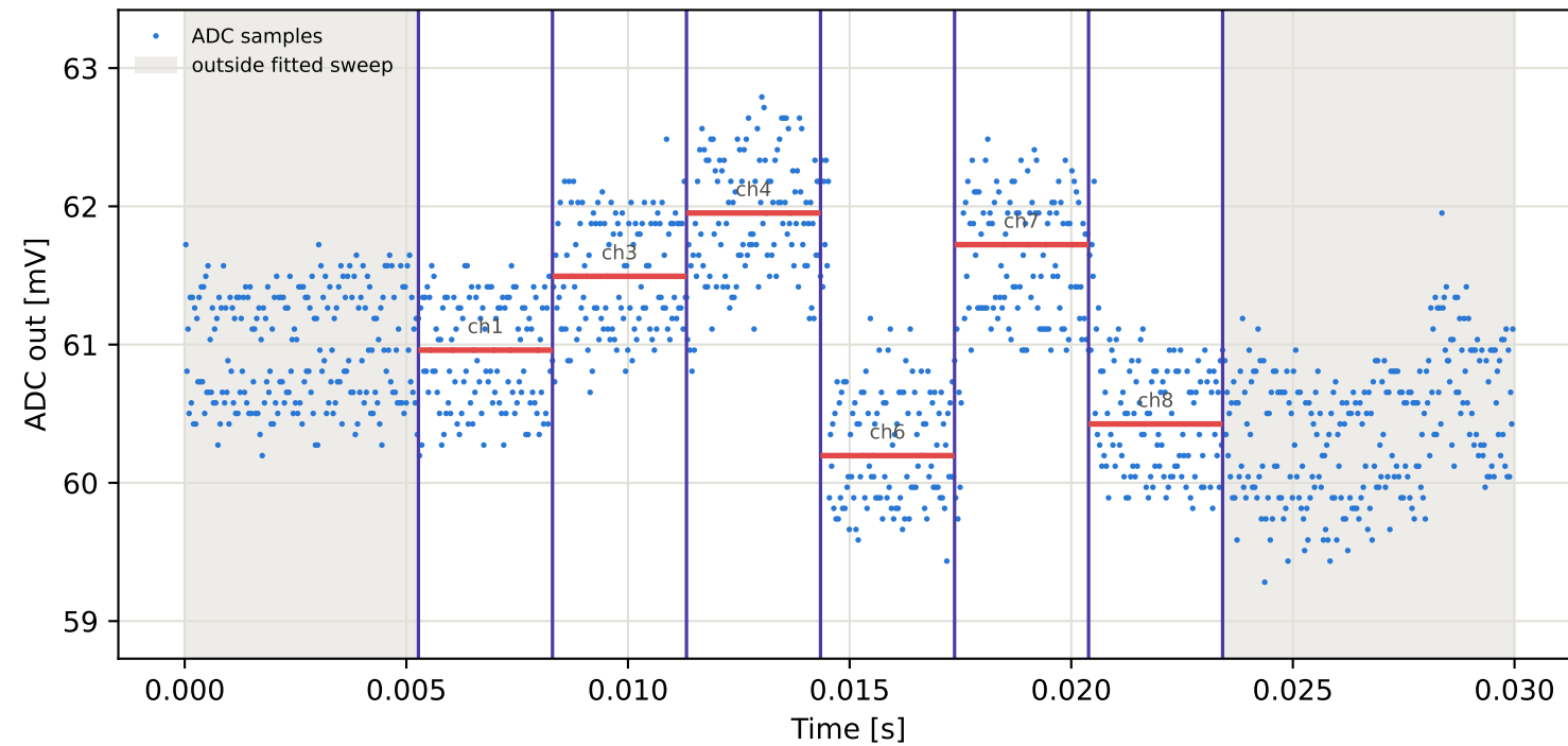
Tag6 &lt;- Tag4 | 995 MHz | run 0 | rep 1 | phase -104.56 deg
