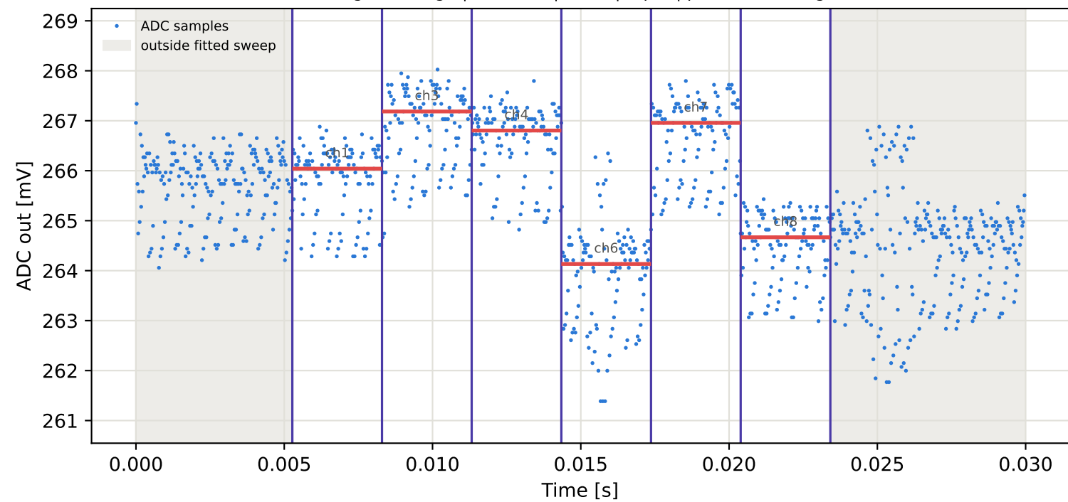
Tag16 &lt;- Tag4 | 805 MHz | run 0 | rep 1 | phase 74.69 deg
