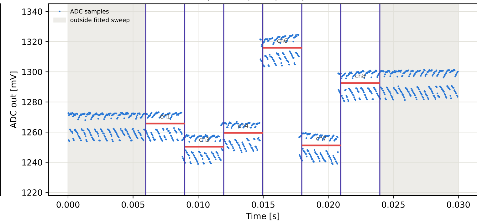
Tag2 &lt;- Tag10 | 955 MHz | run 0 | rep 1 | phase -59.11 deg
