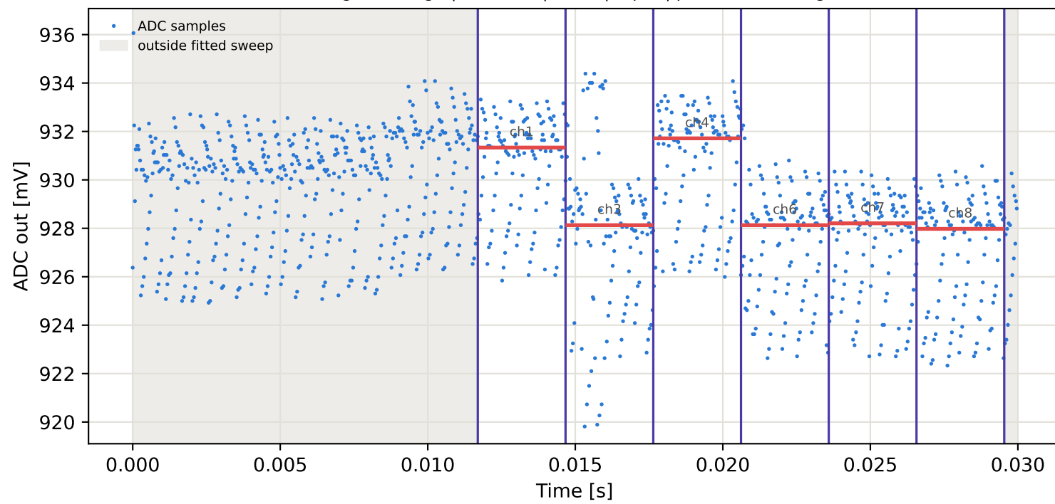
Tag16 &lt;- Tag4 | 835 MHz | run 0 | rep 1 | phase 79.57 deg
