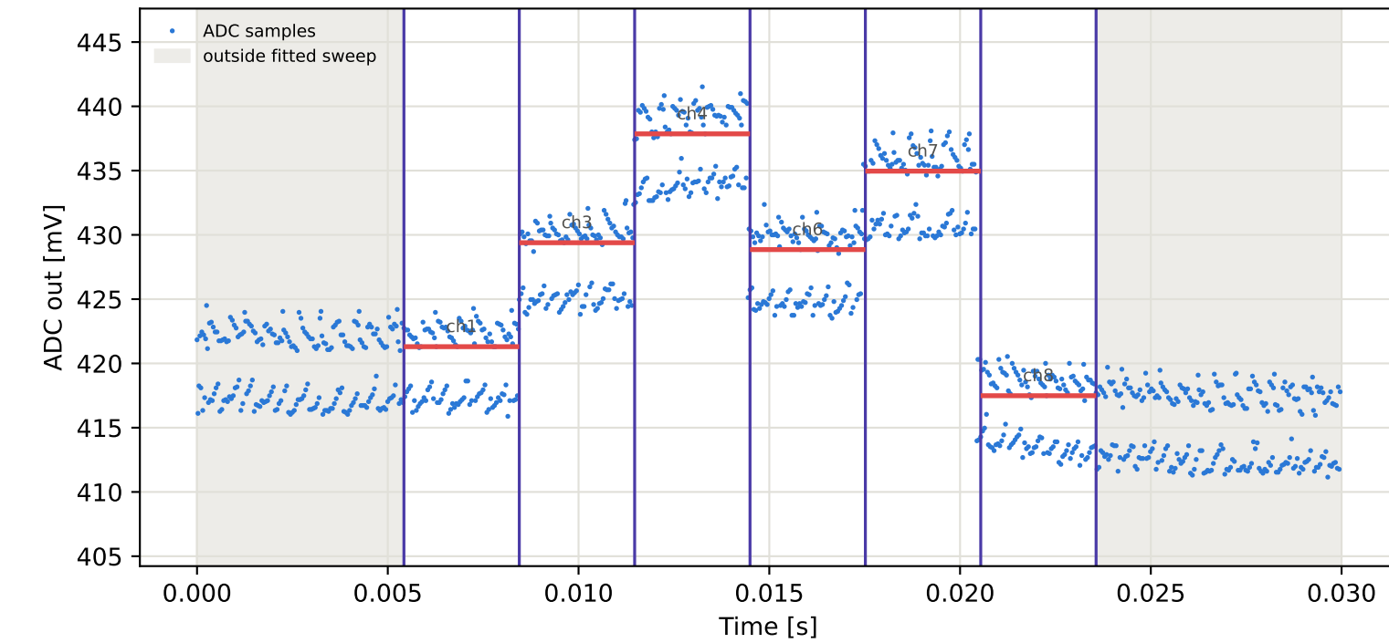
Tag2 &lt;- Tag15 | 915 MHz | run 0 | rep 1 | phase -25.94 deg
