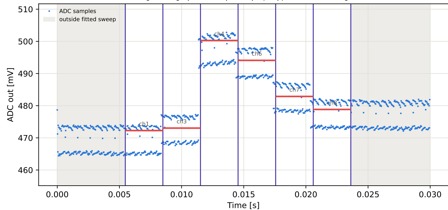
Tag7 &lt;- Tag6 | 975 MHz | run 0 | rep 1 | phase -133.74 deg
