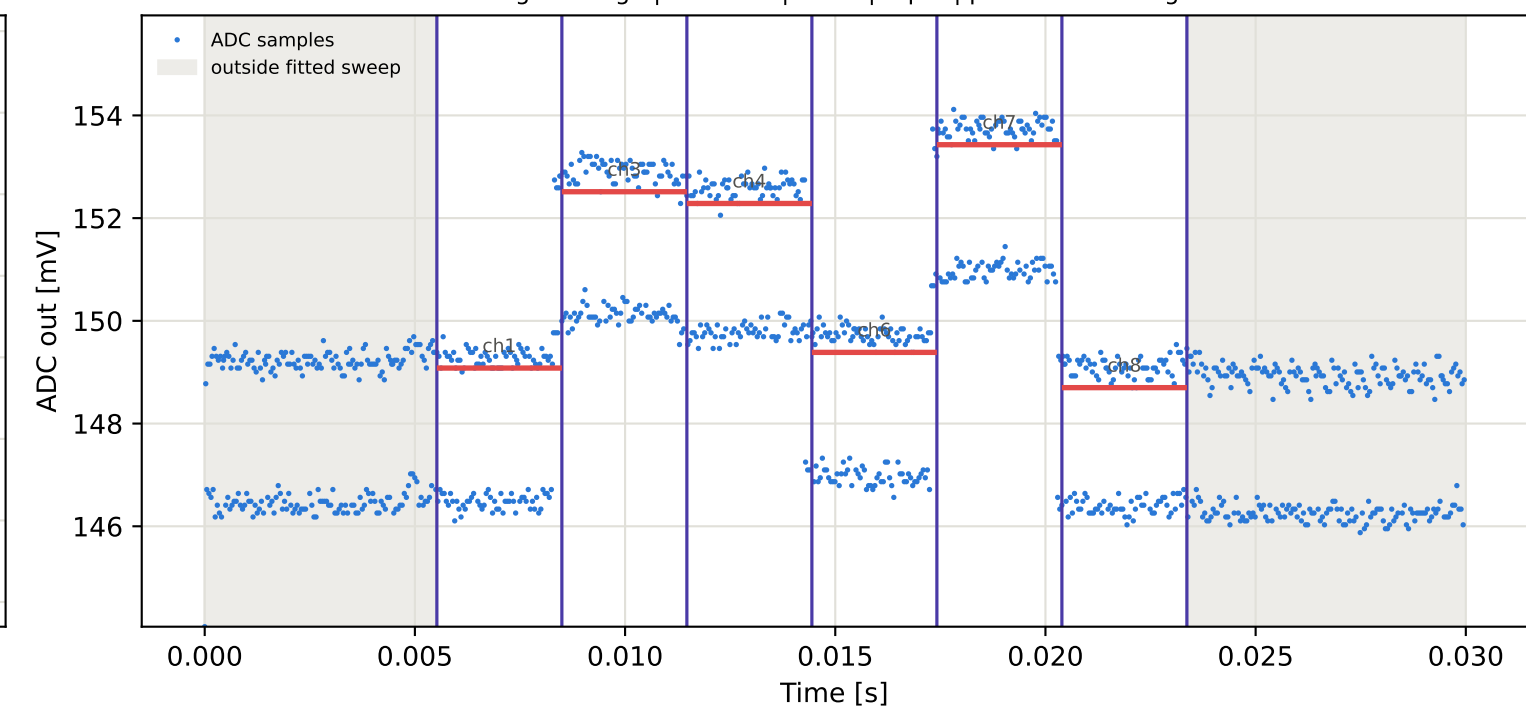
Tag7 &lt;- Tag6 | 805 MHz | run 0 | rep 1 | phase 49.46 deg
