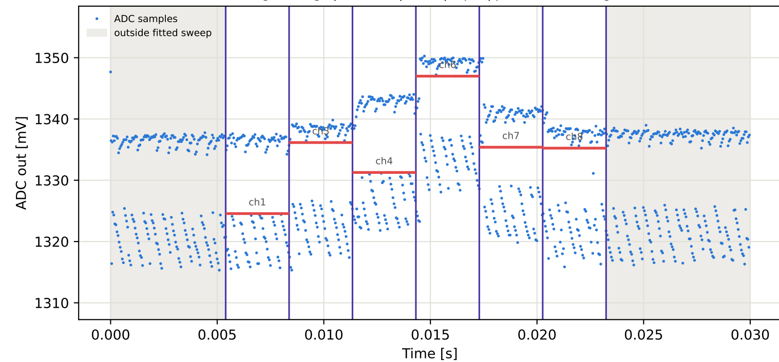
Tag8 &lt;- Tag4 | 935 MHz | run 0 | rep 1 | phase 119.56 deg
