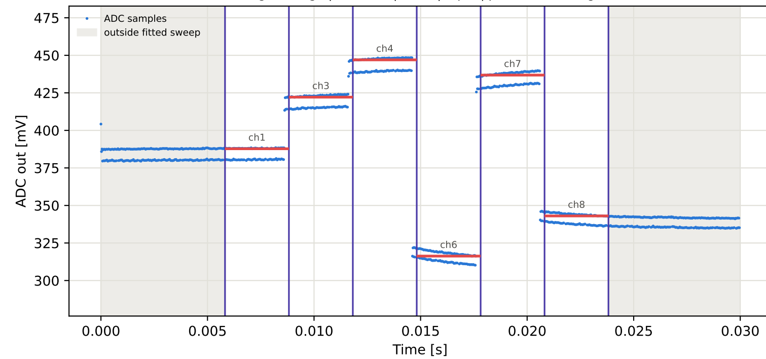
Tag3 &lt;- Tag6 | 945 MHz | run 0 | rep 1 | phase -32.06 deg
