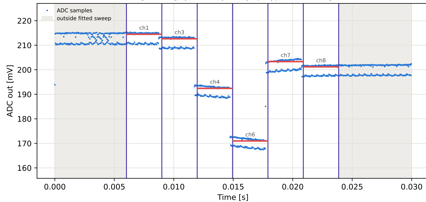
Tag10 &lt;- Tag8 | 945 MHz | run 0 | rep 1 | phase 74.18 deg
