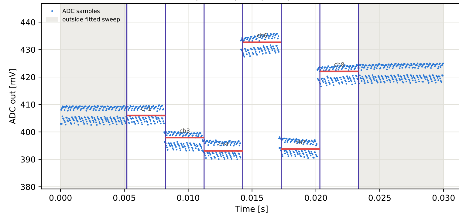
Tag1 &lt;- Tag7 | 945 MHz | run 0 | rep 1 | phase -75.41 deg
