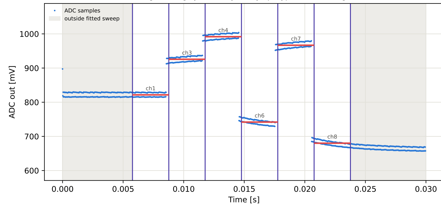
Tag2 &lt;- Tag1 | 915 MHz | run 0 | rep 1 | phase -89.49 deg
