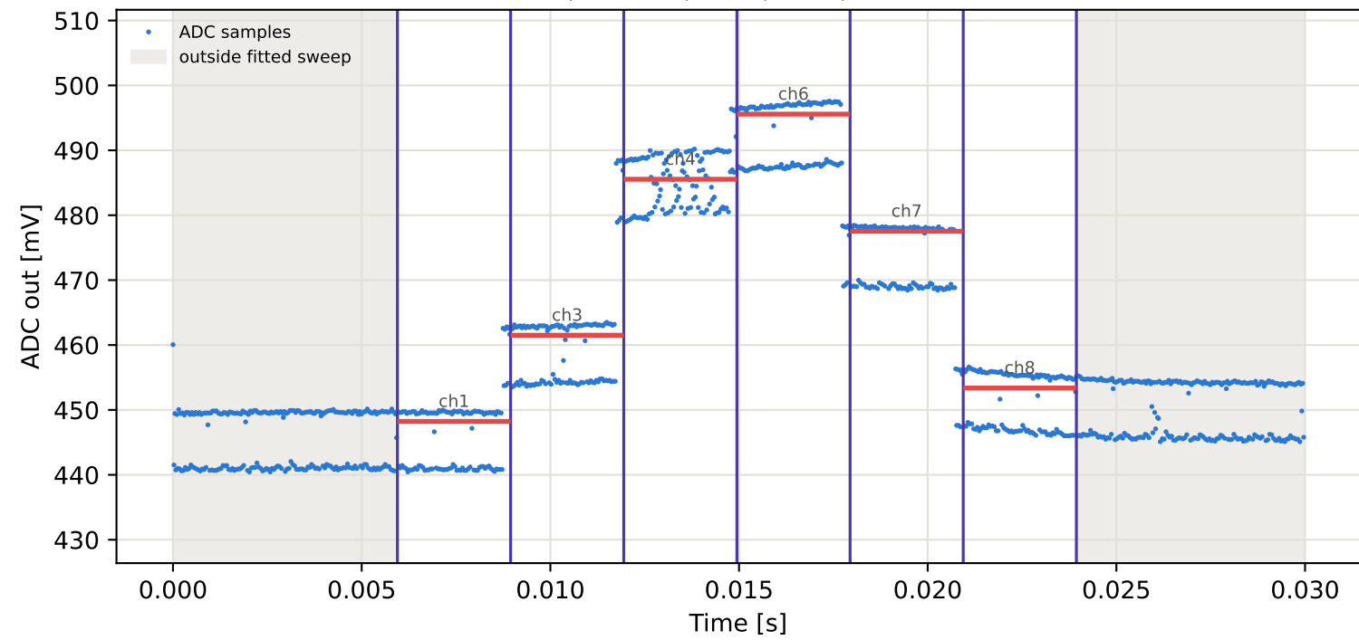
Tag6 &lt;- Tag4 | 925 MHz | run 0 | rep 1 | phase -127.80 deg
