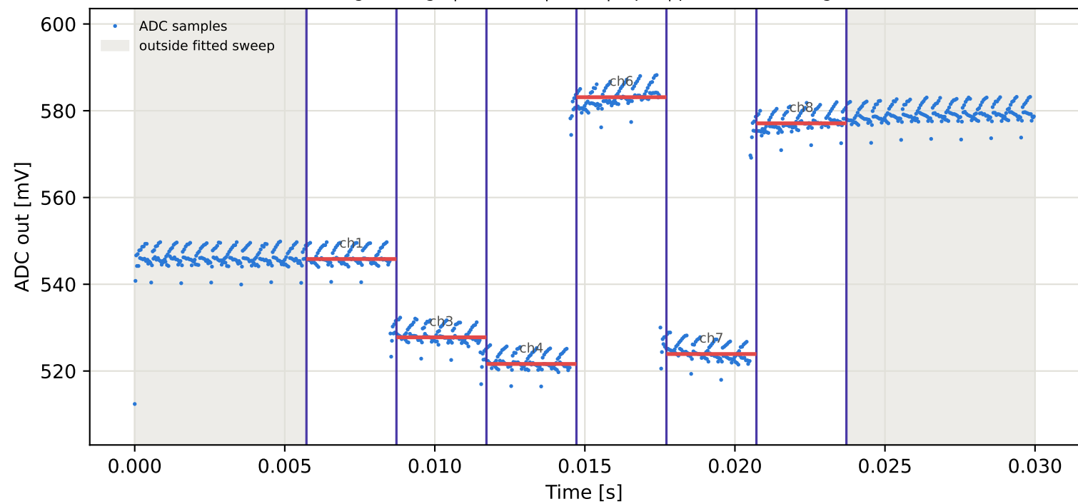
Tag7 &lt;- Tag1 | 915 MHz | run 0 | rep 1 | phase 95.97 deg
