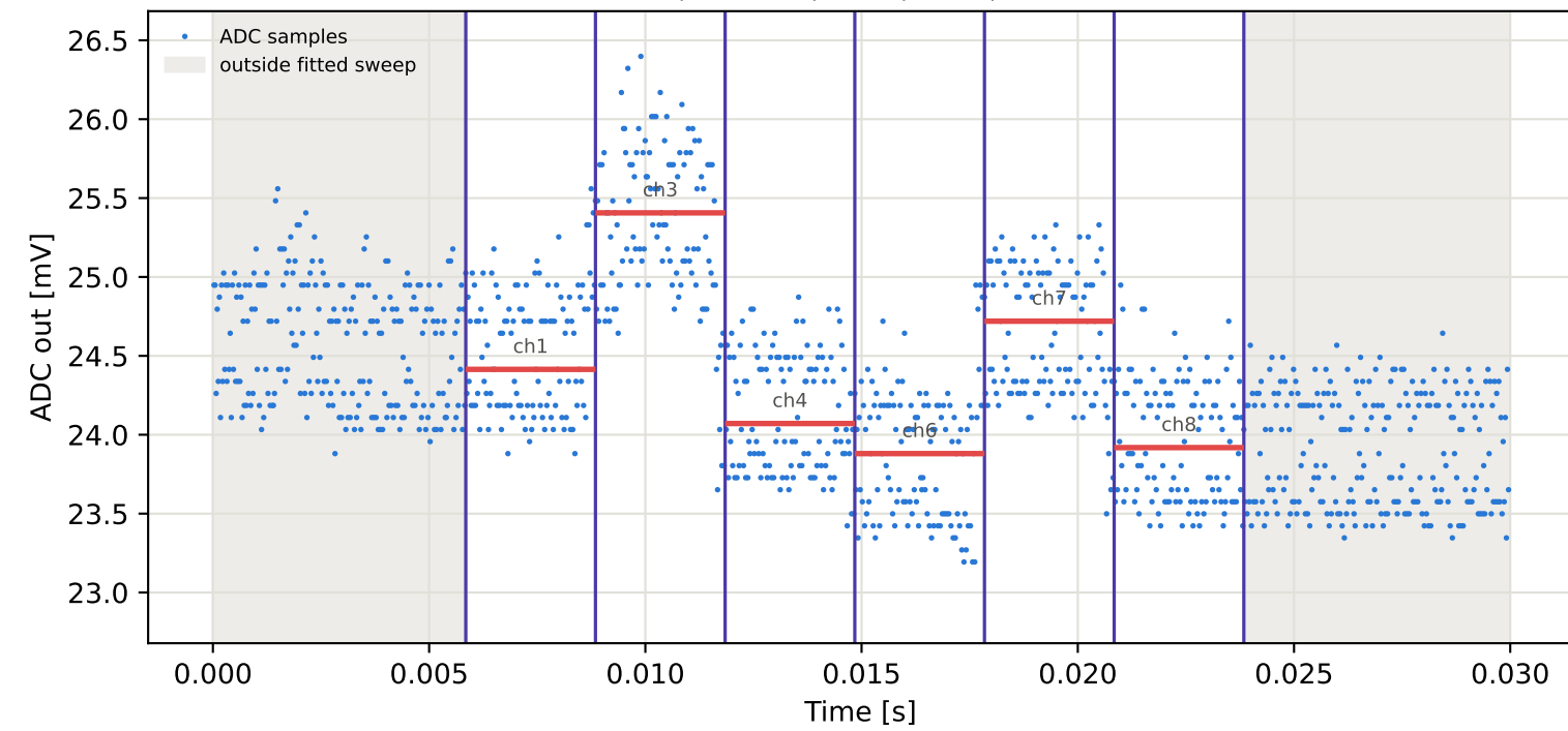
Tag6 &lt;- Tag5 | 795 MHz | run 0 | rep 1 | phase 28.48 deg
