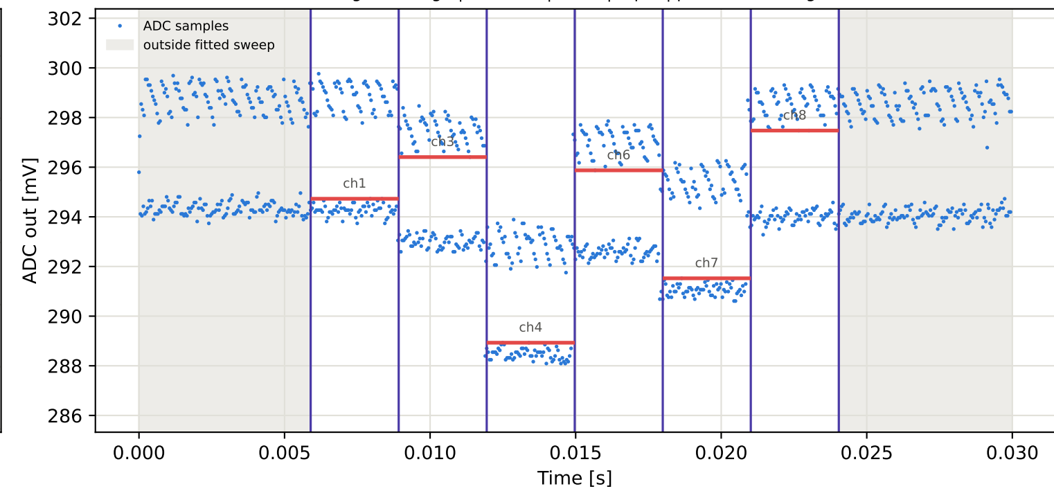
Tag15 &lt;- Tag6 | 995 MHz | run 0 | rep 1 | phase 82.76 deg
