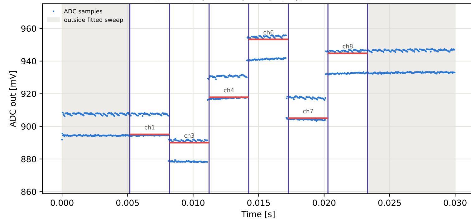
Tag2 &lt;- Tag1 | 845 MHz | run 0 | rep 1 | phase 102.58 deg
