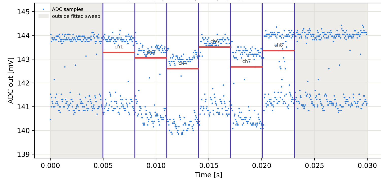
Tag8 &lt;- Tag4 | 775 MHz | run 0 | rep 1 | phase 147.12 deg
