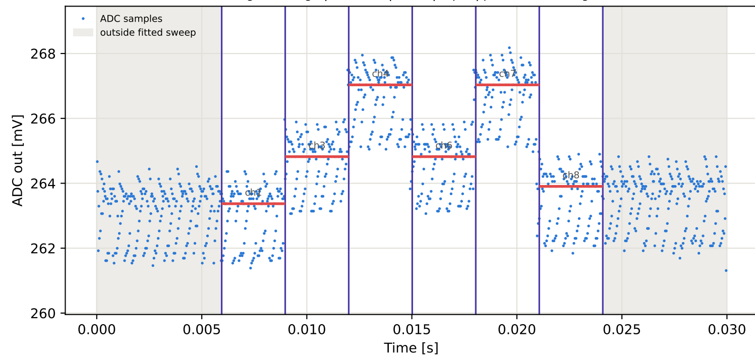
Tag16 &lt;- Tag7 | 805 MHz | run 0 | rep 1 | phase -90.48 deg
