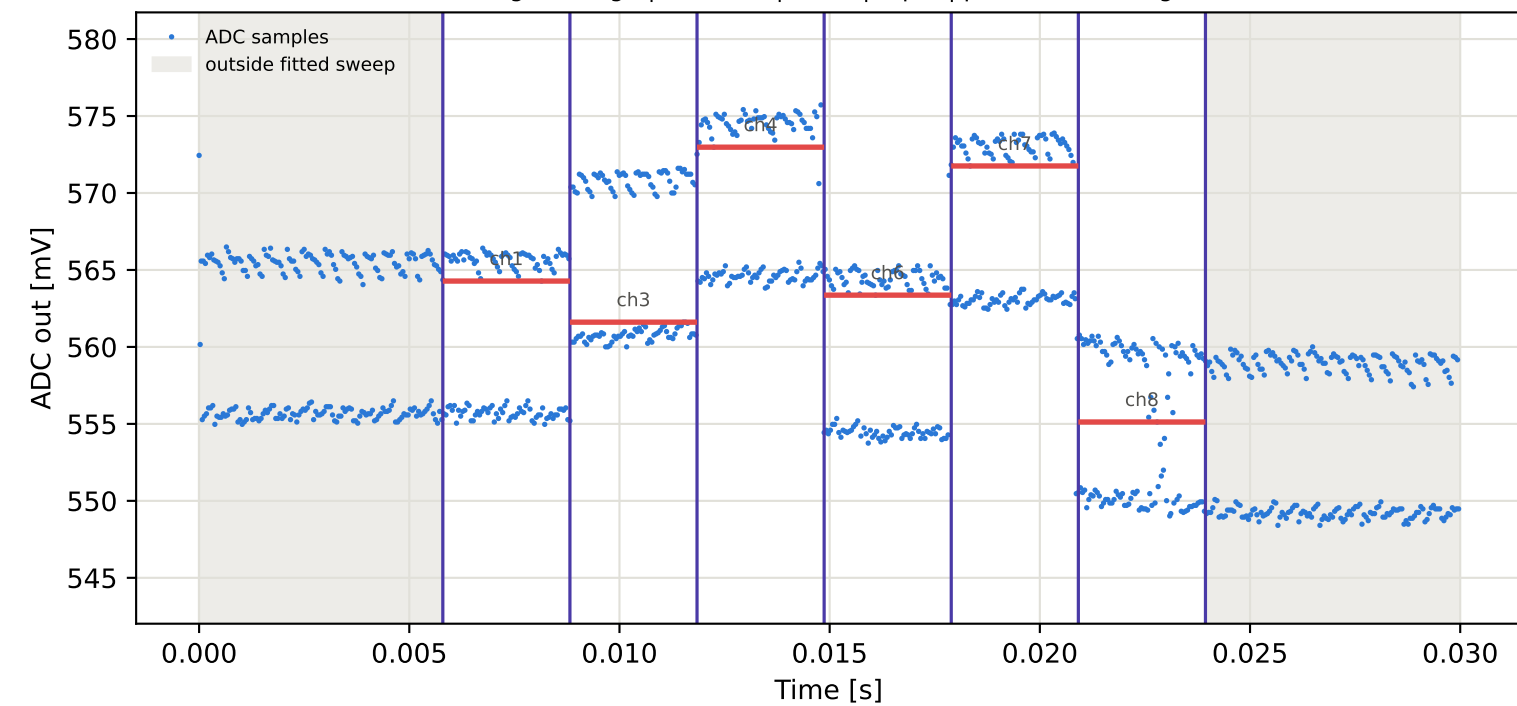
Tag6 &lt;- Tag4 | 905 MHz | run 0 | rep 1 | phase -155.40 deg
