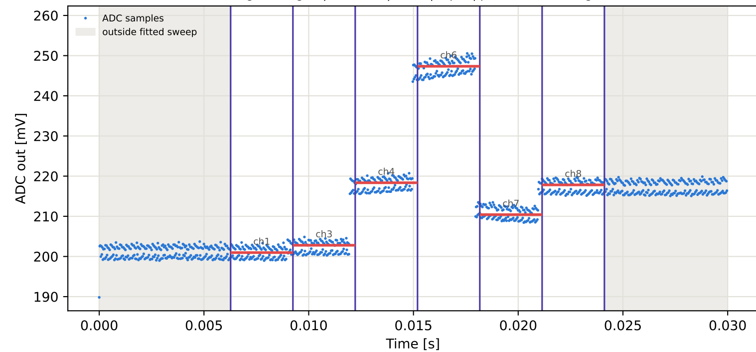
Tag1 &lt;- Tag16 | 925 MHz | run 0 | rep 1 | phase -54.75 deg
