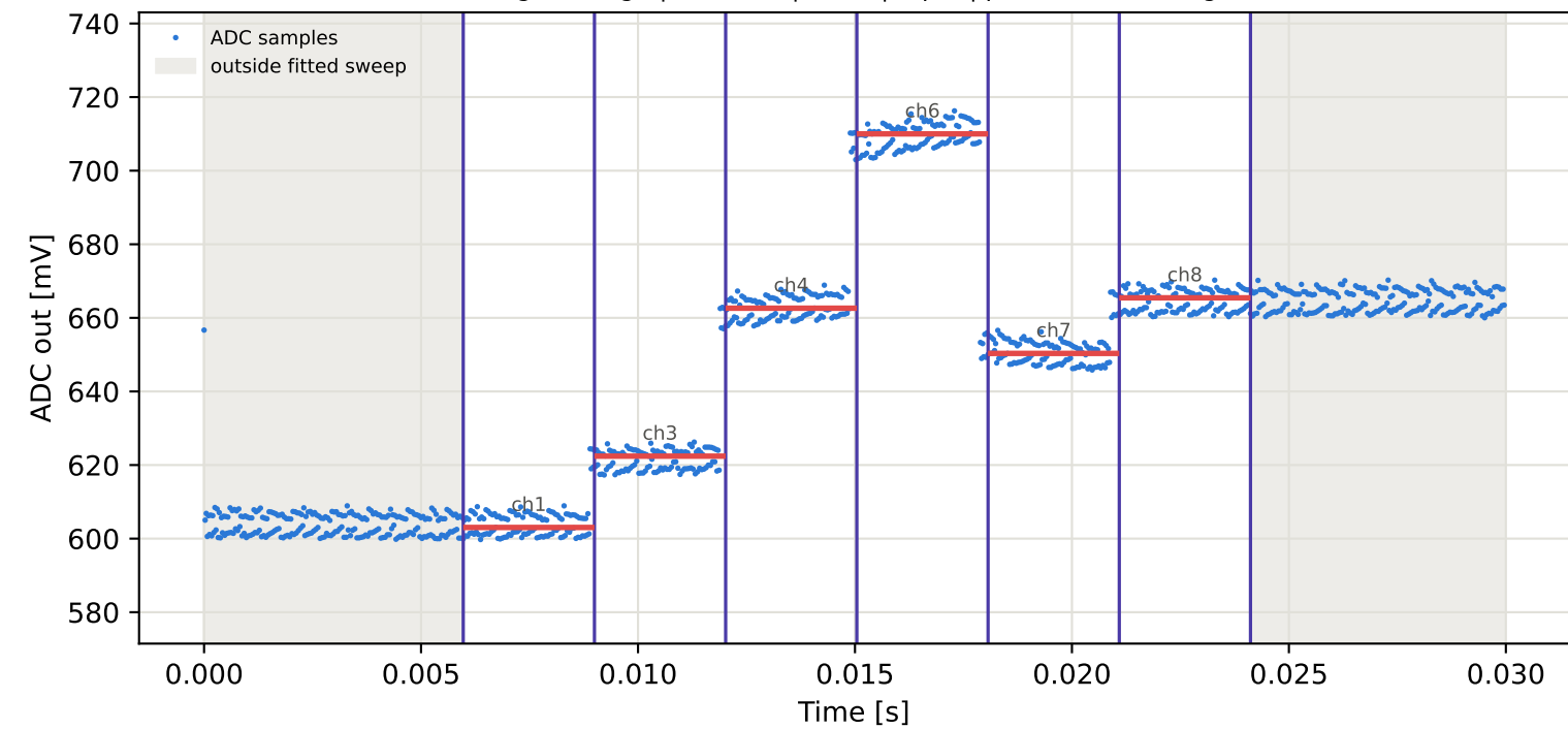
Tag9 &lt;- Tag6 | 885 MHz | run 0 | rep 1 | phase 144.60 deg
