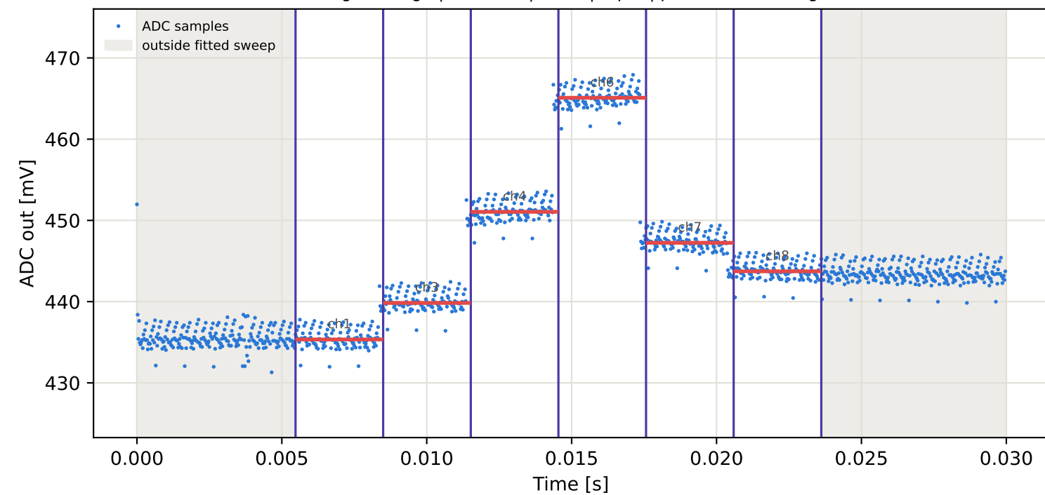
Tag3 &lt;- Tag2 | 855 MHz | run 0 | rep 1 | phase -137.76 deg
