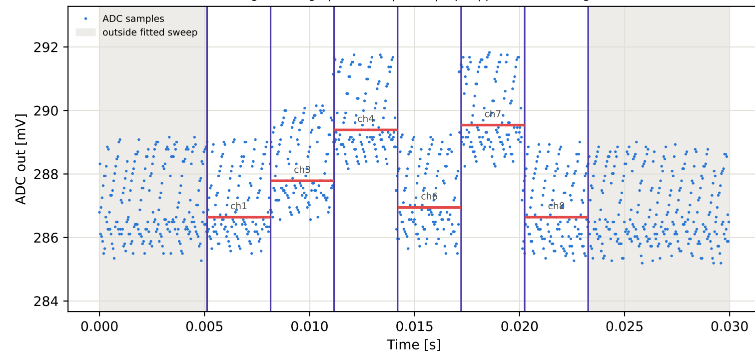
Tag15 &lt;- Tag1 | 785 MHz | run 0 | rep 1 | phase -59.97 deg
