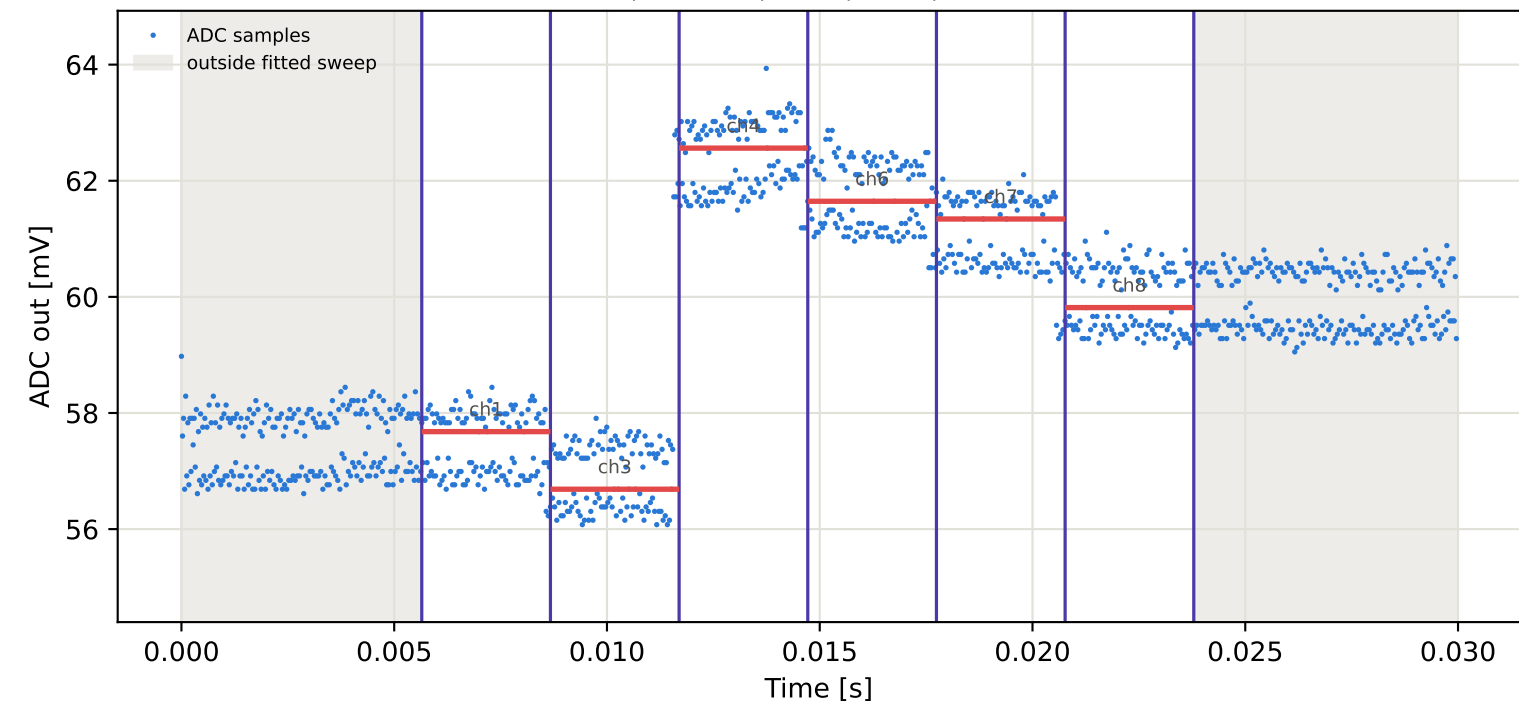
Tag9 &lt;- Tag8 | 805 MHz | run 0 | rep 1 | phase -117.18 deg
