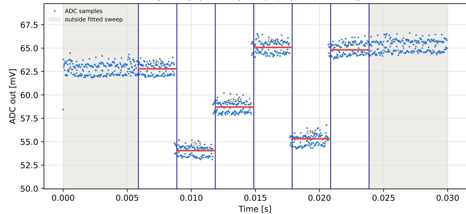
Tag2 &lt;- Tag5 | 805 MHz | run 0 | rep 1 | phase -91.18 deg
