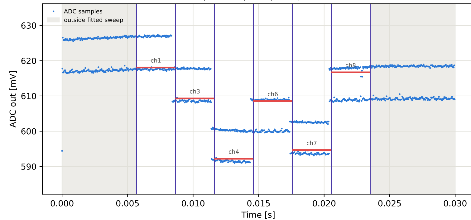
Tag4 &lt;- Tag7 | 835 MHz | run 0 | rep 1 | phase 122.76 deg
