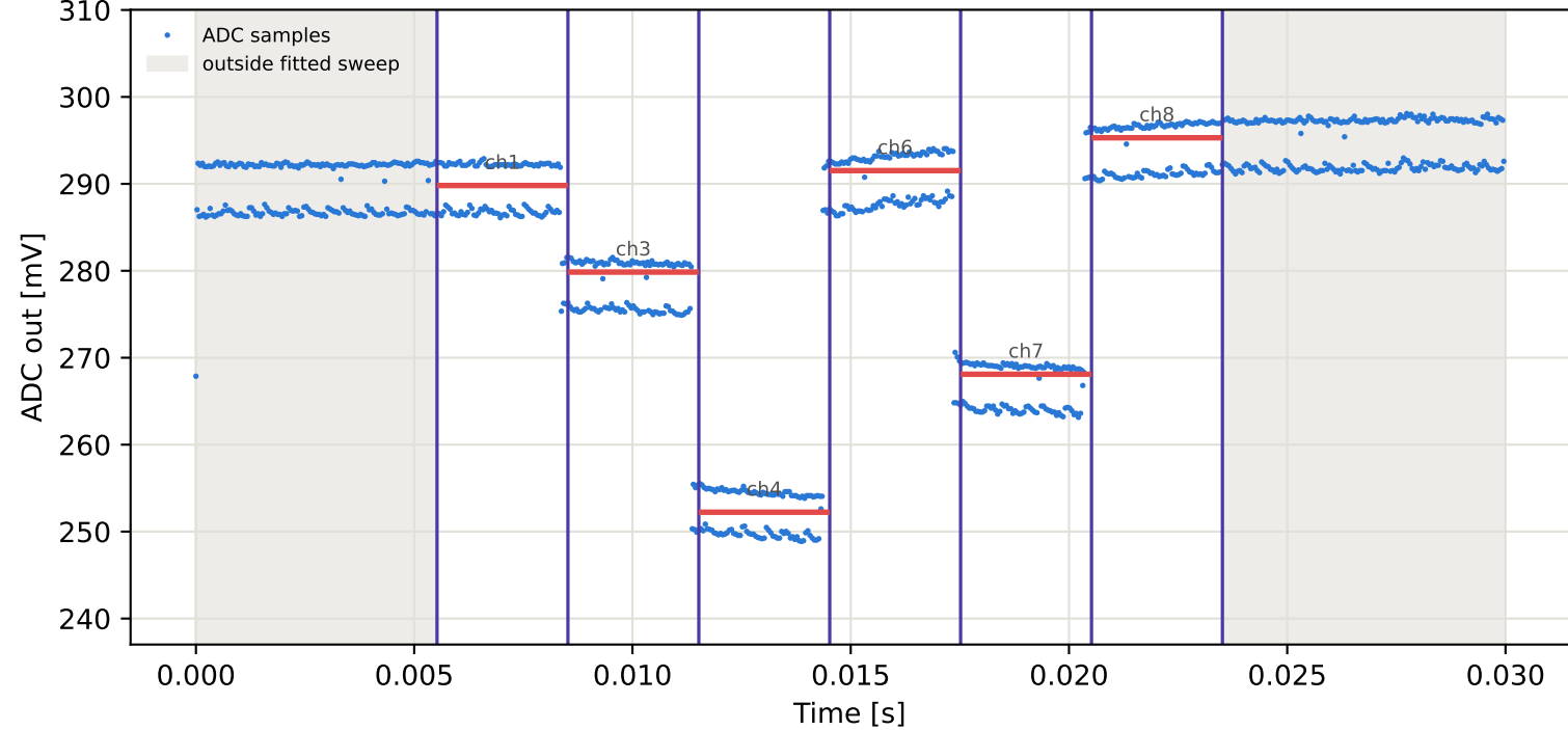
Tag6 &lt;- Tag5 | 985 MHz | run 0 | rep 1 | phase 65.05 deg
