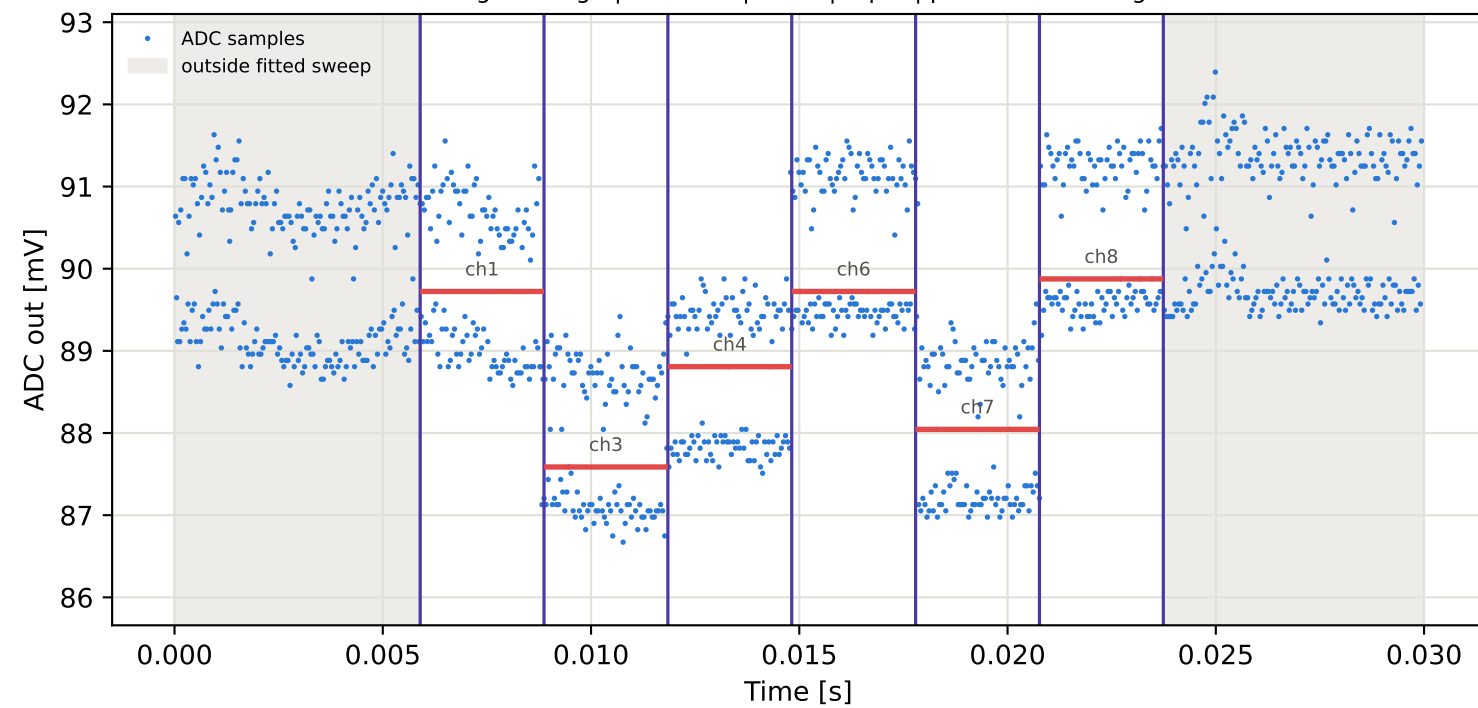
Tag1 &lt;- Tag7 | 825 MHz | run 0 | rep 1 | phase -40.81 deg
