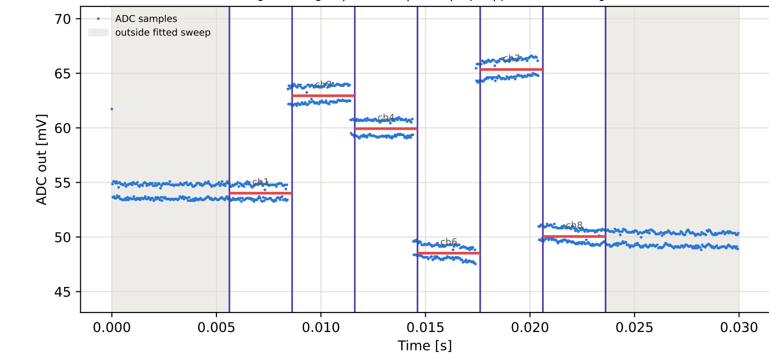
Tag16 &lt;- Tag15 | 785 MHz | run 0 | rep 1 | phase -10.36 deg
