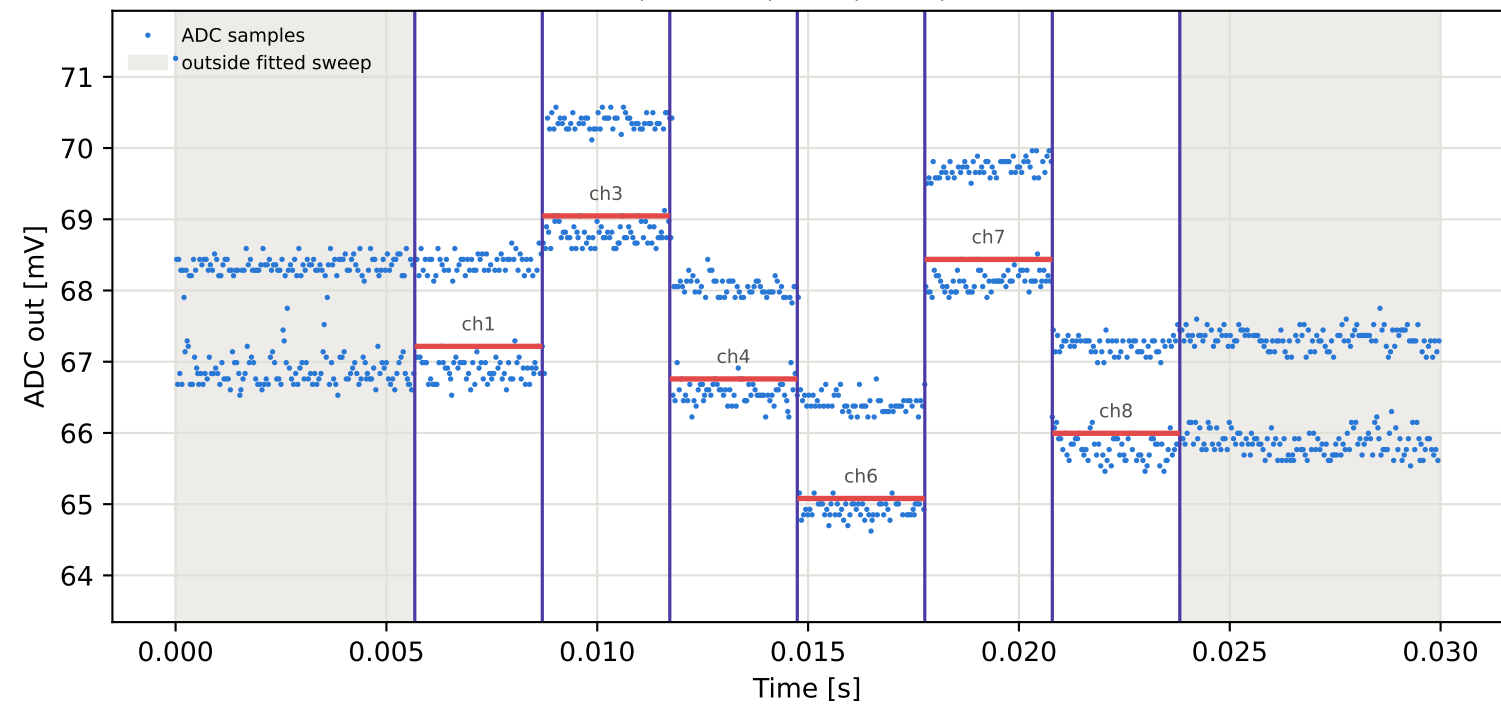
Tag10 &lt;- Tag5 | 775 MHz | run 0 | rep 1 | phase 20.03 deg
