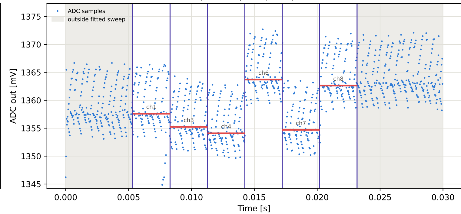
Tag15 &lt;- Tag4 | 915 MHz | run 0 | rep 1 | phase -51.72 deg
