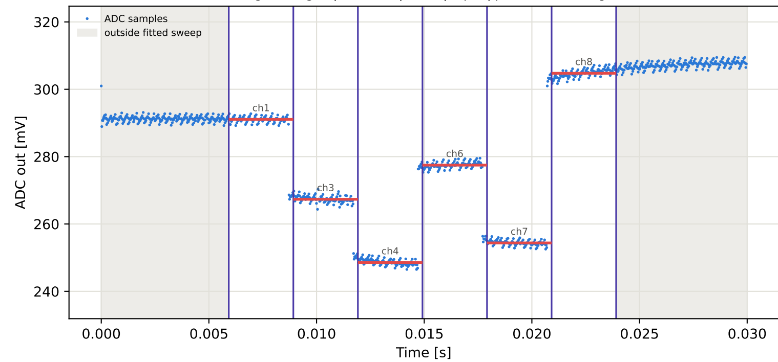
Tag1 &lt;- Tag2 | 915 MHz | run 0 | rep 1 | phase -158.11 deg
