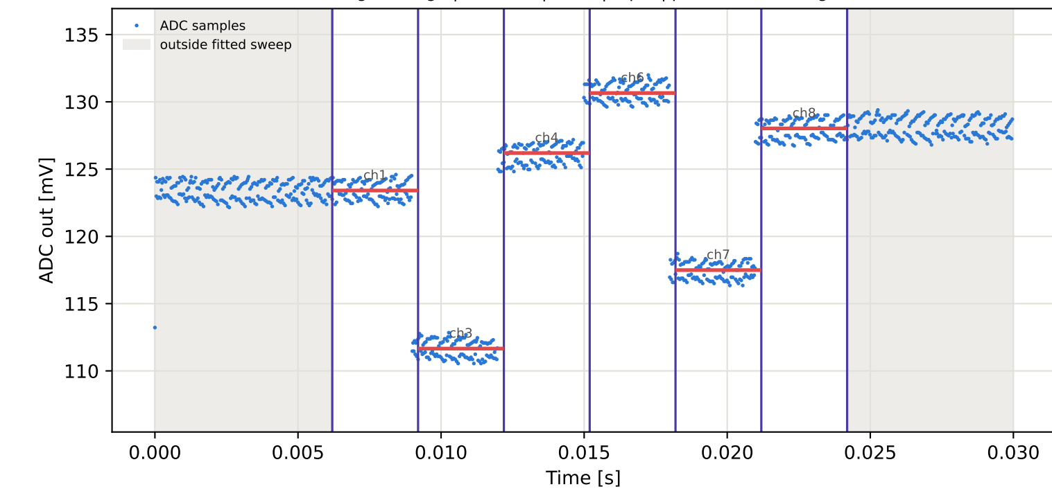
Tag8 &lt;- Tag6 | 785 MHz | run 0 | rep 1 | phase -34.97 deg
