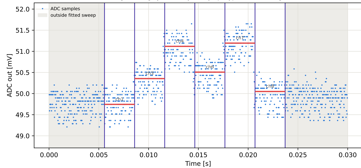
Tag10 &lt;- Tag9 | 805 MHz | run 0 | rep 1 | phase 159.83 deg
