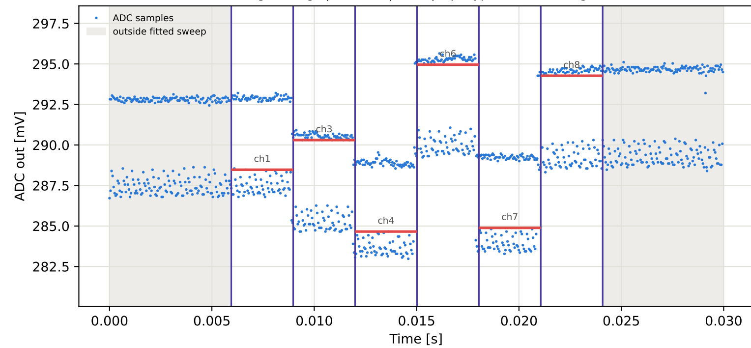
Tag1 &lt;- Tag8 | 995 MHz | run 0 | rep 1 | phase 63.15 deg
