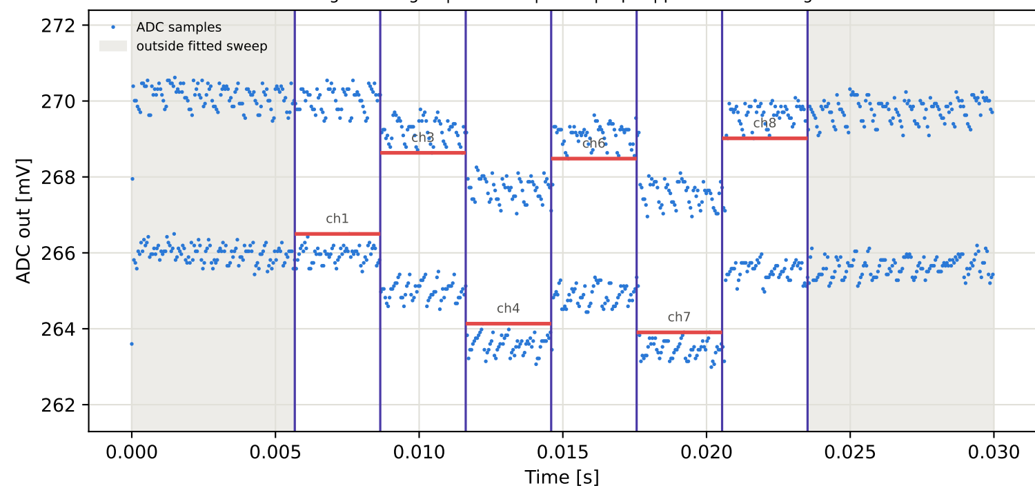
Tag16 &lt;- Tag10 | 805 MHz | run 0 | rep 1 | phase 117.72 deg
