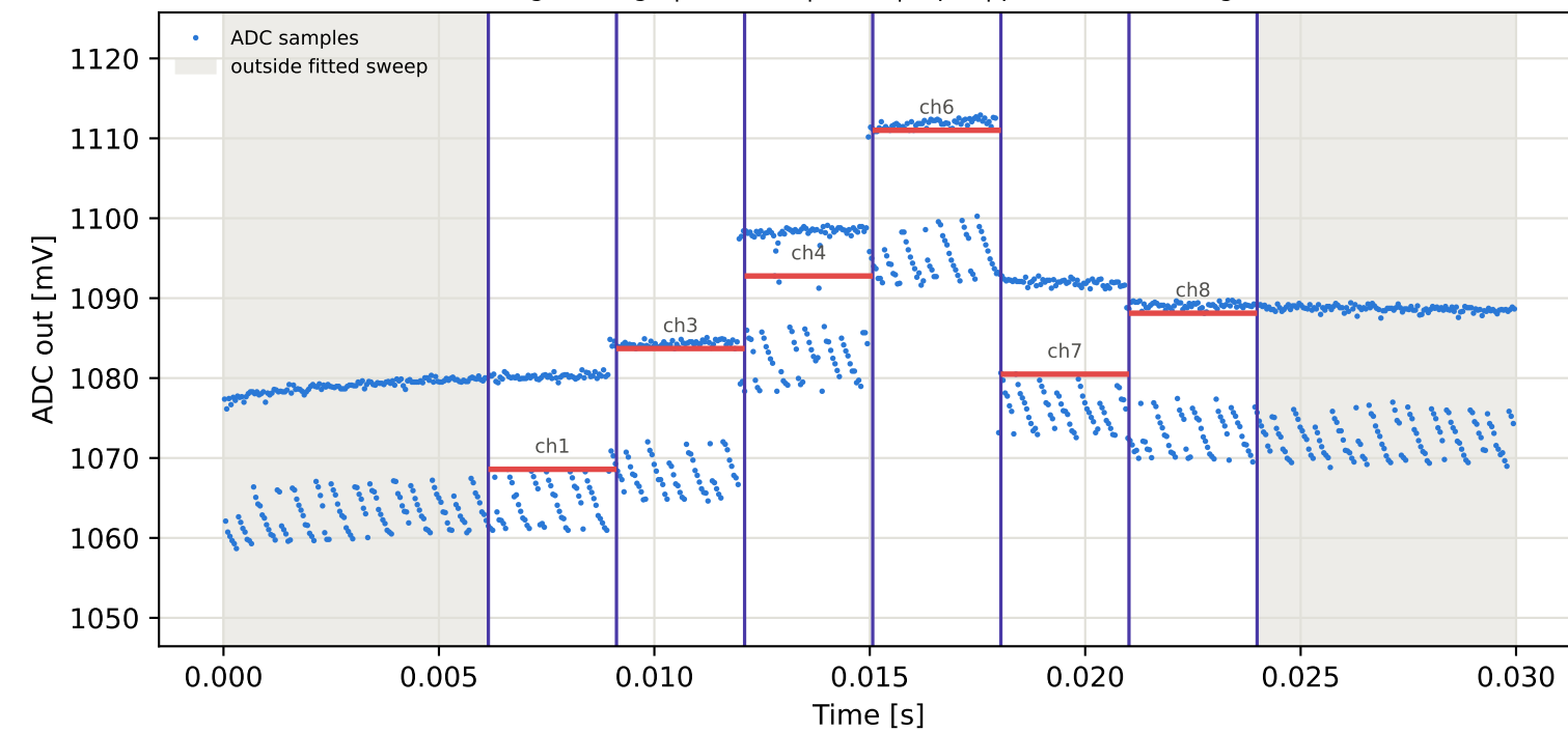
Tag5 &lt;- Tag8 | 925 MHz | run 0 | rep 1 | phase 116.11 deg
