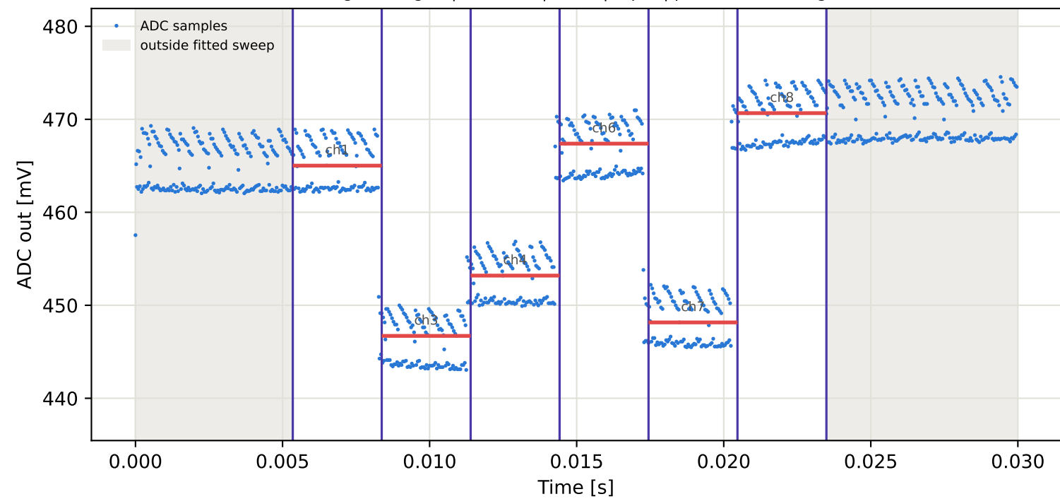
Tag5 &lt;- Tag2 | 845 MHz | run 0 | rep 1 | phase -88.65 deg
