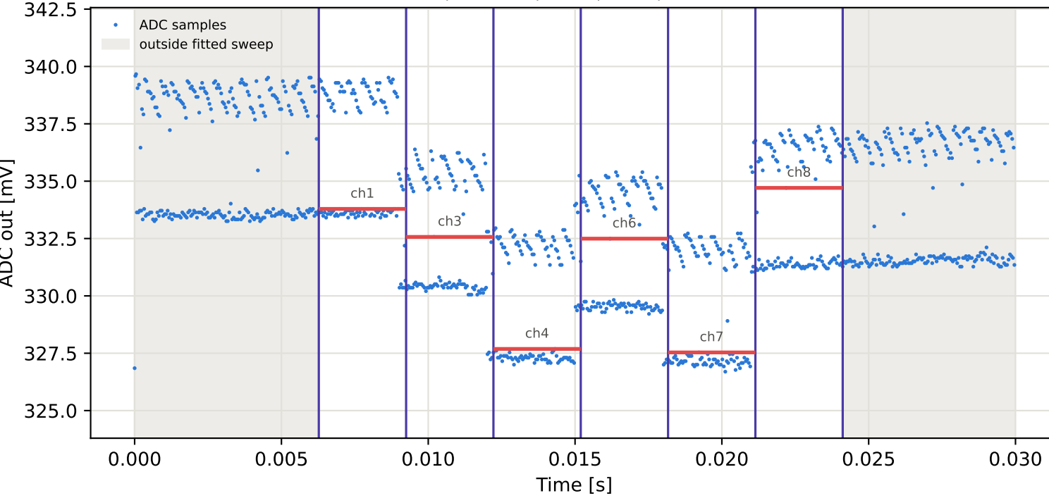
Tag6 &lt;- Tag1 | 845 MHz | run 0 | rep 1 | phase 101.40 deg
