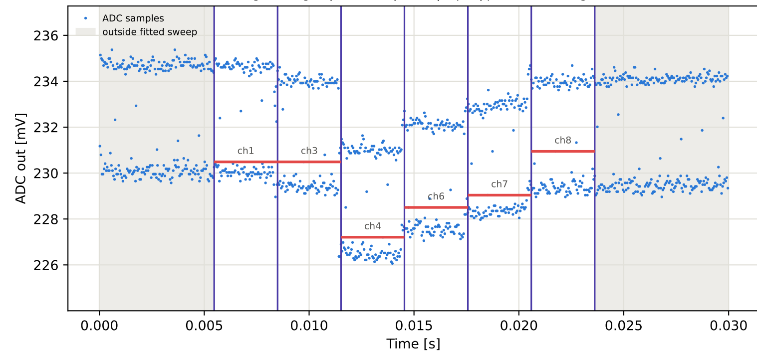
Tag5 &lt;- Tag16 | 985 MHz | run 0 | rep 1 | phase 58.37 deg
