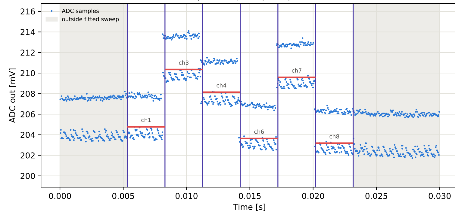
Tag6 &lt;- Tag2 | 835 MHz | run 0 | rep 1 | phase -94.51 deg
