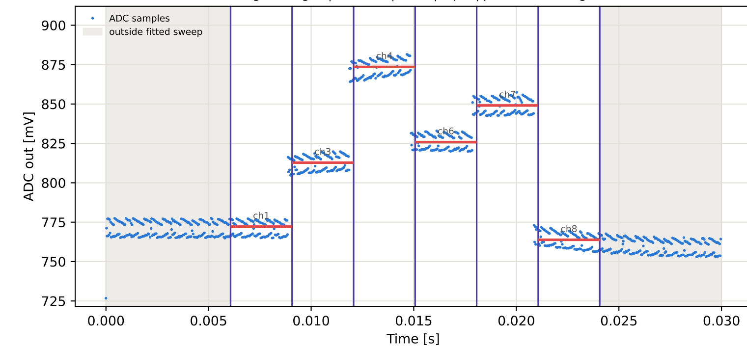
Tag9 &lt;- Tag16 | 925 MHz | run 0 | rep 1 | phase -99.76 deg
