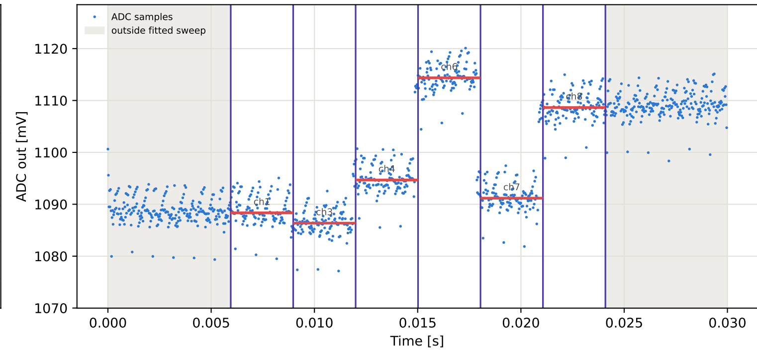
Tag15 &lt;- Tag6 | 885 MHz | run 0 | rep 1 | phase -77.87 deg
