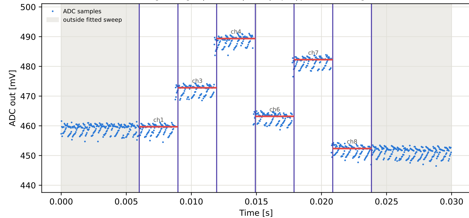
Tag6 &lt;- Tag3 | 935 MHz | run 0 | rep 1 | phase 37.98 deg
