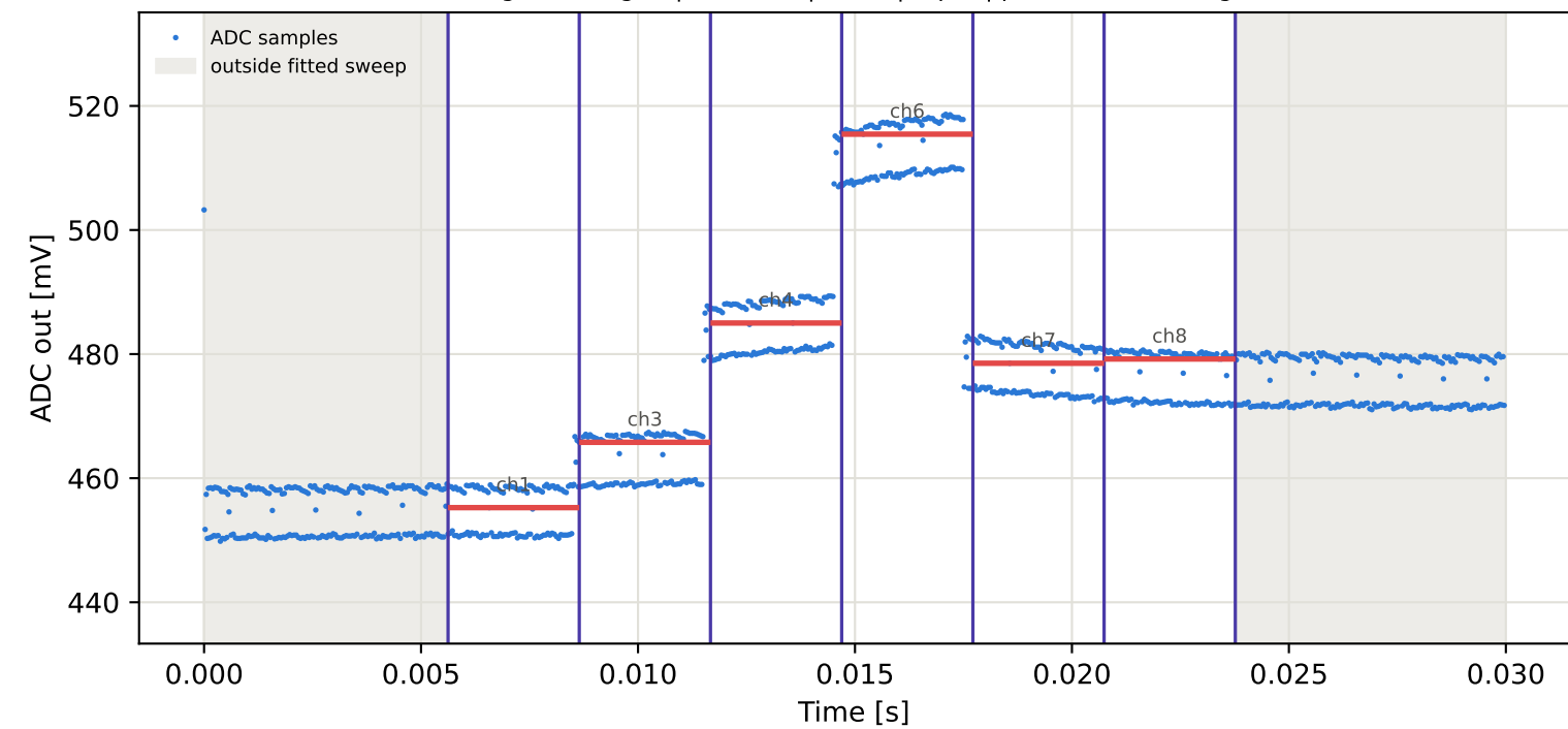
Tag10 &lt;- Tag3 | 895 MHz | run 0 | rep 1 | phase 177.59 deg
