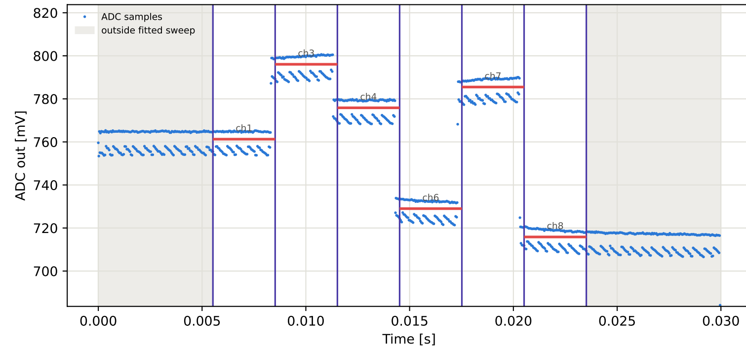
Tag8 &lt;- Tag6 | 855 MHz | run 0 | rep 1 | phase 168.93 deg
