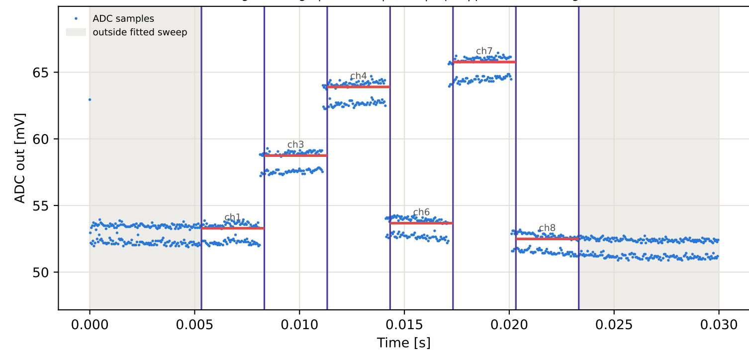
Tag10 &lt;- Tag1 | 795 MHz | run 0 | rep 1 | phase -53.50 deg
