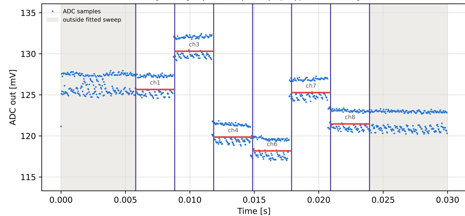
Tag4 &lt;- Tag2 | 805 MHz | run 0 | rep 1 | phase -23.82 deg
