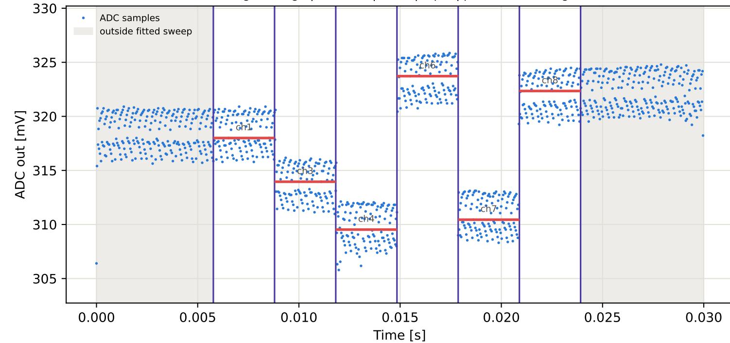
Tag3 &lt;- Tag8 | 995 MHz | run 0 | rep 1 | phase -29.38 deg
