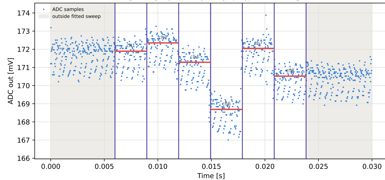
Tag5 &lt;- Tag16 | 965 MHz | run 0 | rep 1 | phase -10.71 deg
