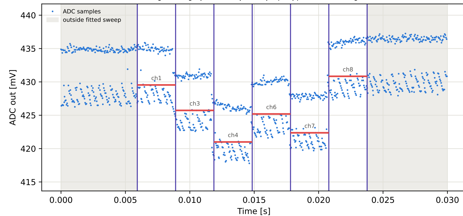
Tag2 &lt;- Tag7 | 915 MHz | run 0 | rep 1 | phase 83.44 deg
