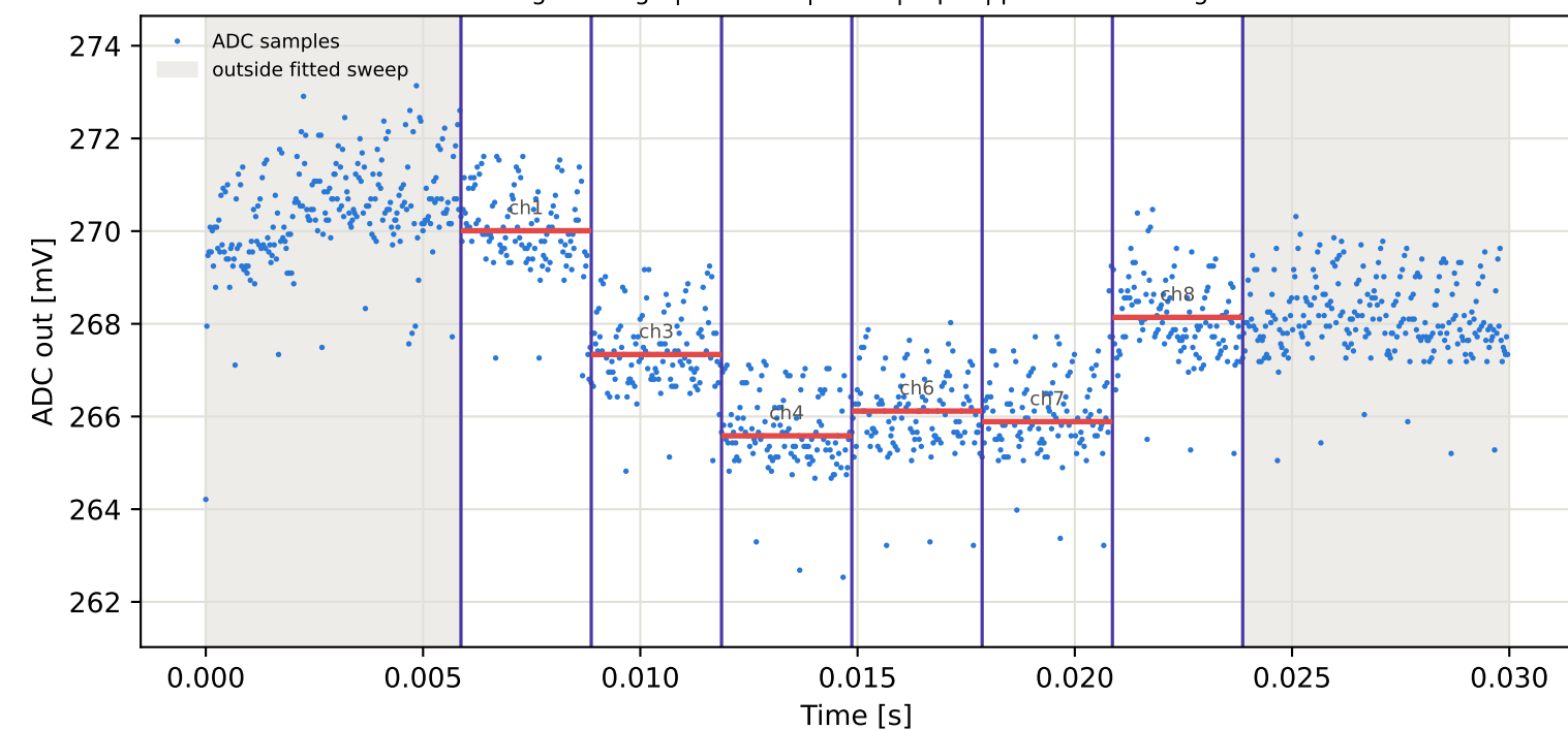
Tag2 &lt;- Tag15 | 865 MHz | run 0 | rep 1 | phase -167.60 deg
