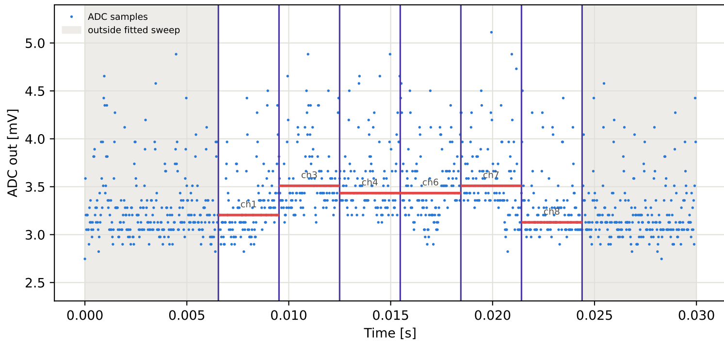
Tag3 &lt;- Tag10 | 795 MHz | run 0 | rep 1 | phase 75.59 deg
