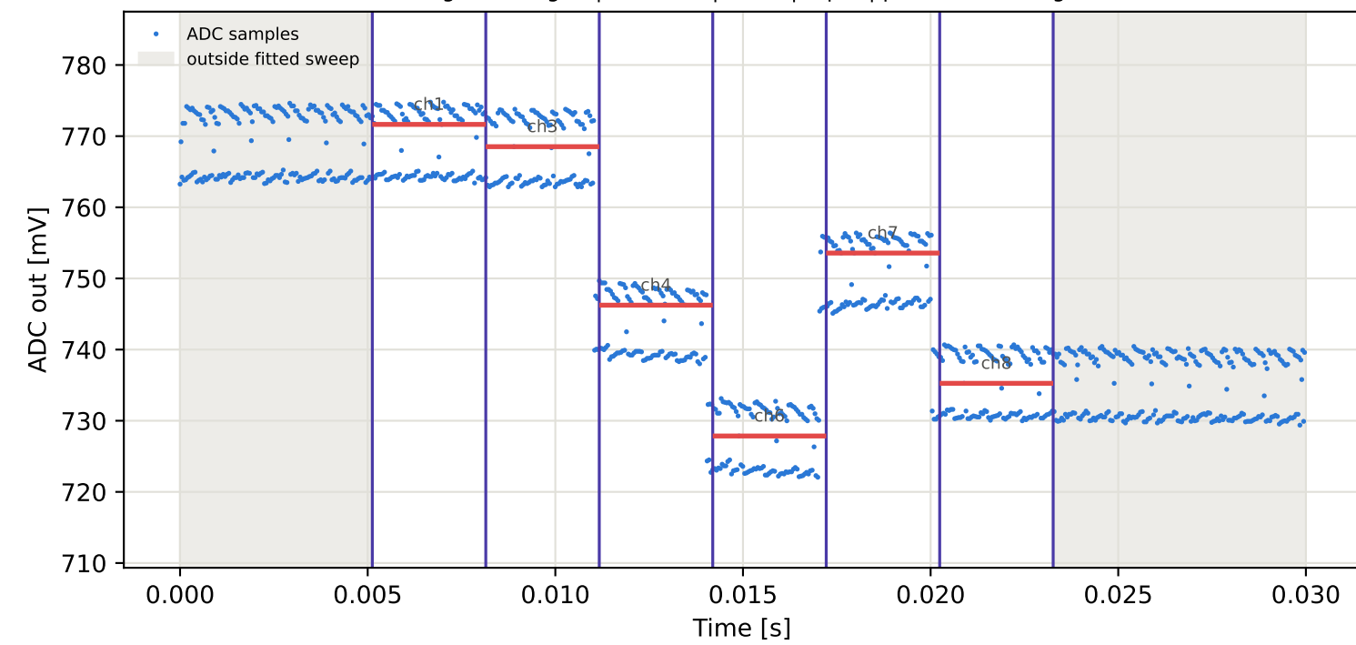
Tag16 &lt;- Tag15 | 865 MHz | run 0 | rep 1 | phase 33.20 deg
