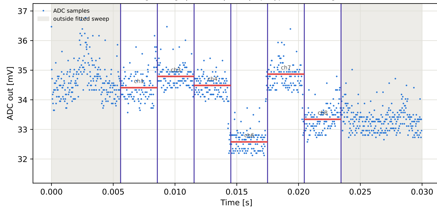
Tag3 &lt;- Tag10 | 995 MHz | run 0 | rep 1 | phase -168.81 deg
