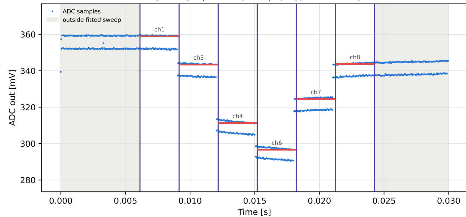
Tag3 &lt;- Tag2 | 925 MHz | run 0 | rep 1 | phase -46.55 deg
