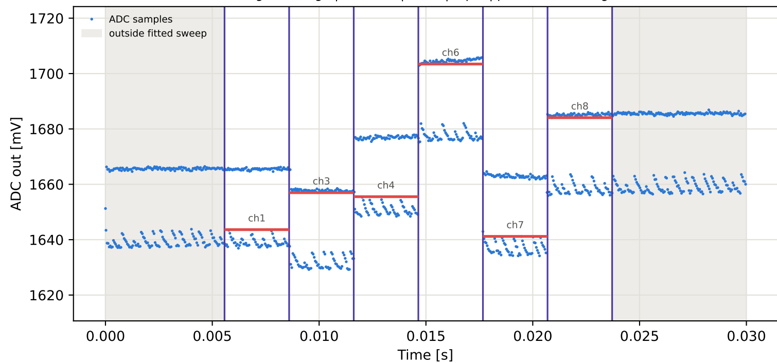
Tag16 &lt;- Tag7 | 975 MHz | run 0 | rep 1 | phase 177.89 deg
