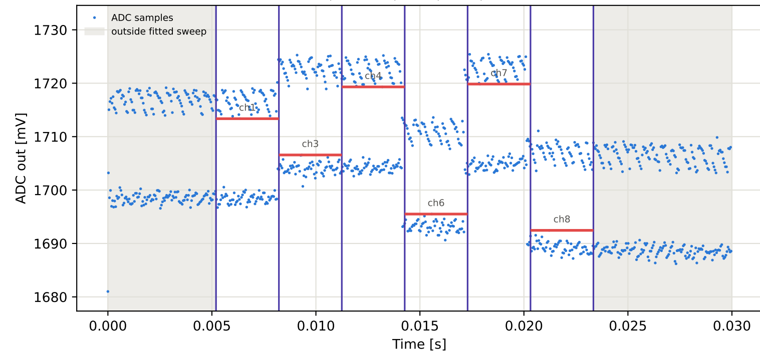
Tag8 &lt;- Tag6 | 885 MHz | run 0 | rep 1 | phase -38.38 deg
