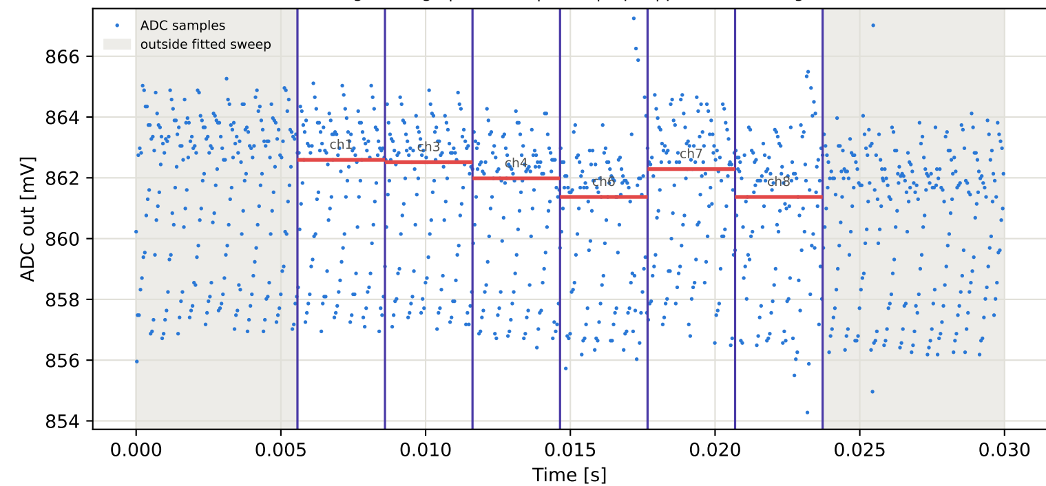
Tag7 &lt;- Tag15 | 875 MHz | run 0 | rep 1 | phase -157.72 deg
