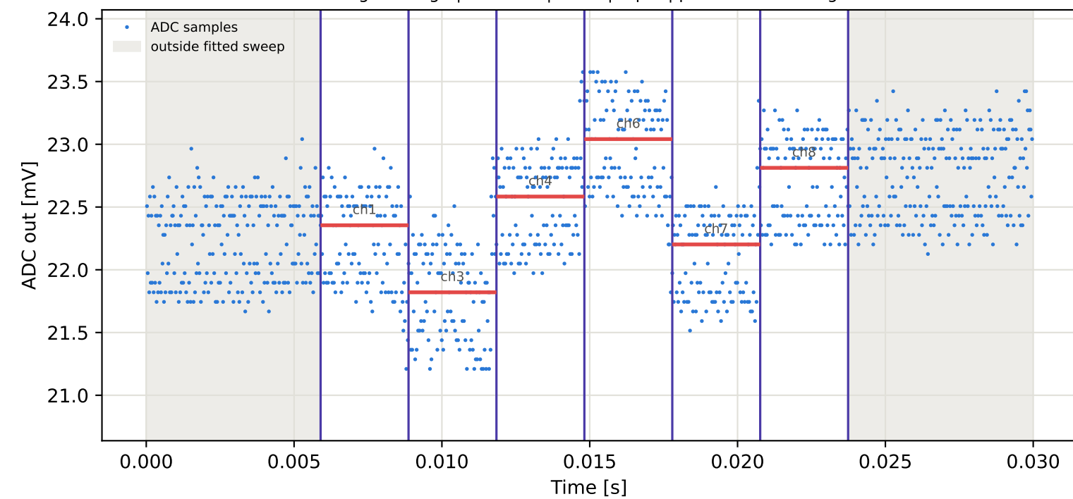
Tag5 &lt;- Tag8 | 805 MHz | run 0 | rep 1 | phase 22.87 deg
