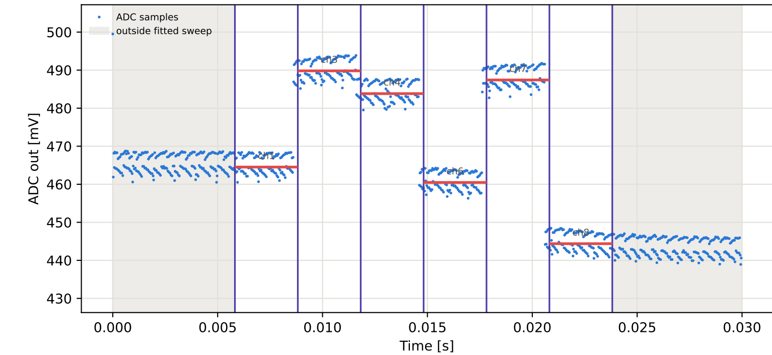
Tag5 &lt;- Tag3 | 855 MHz | run 0 | rep 1 | phase -104.43 deg
