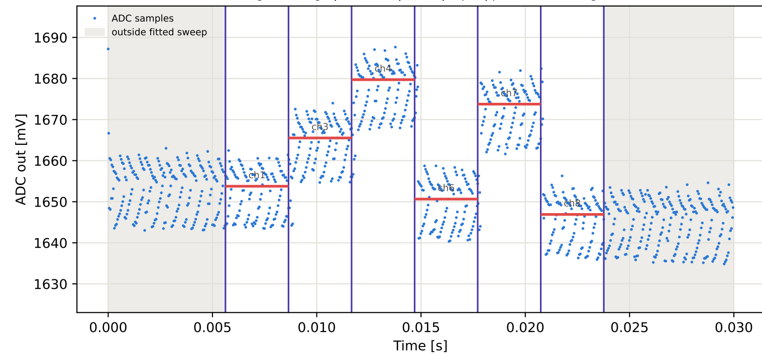
Tag15 &lt;- Tag9 | 945 MHz | run 0 | rep 1 | phase 135.90 deg
