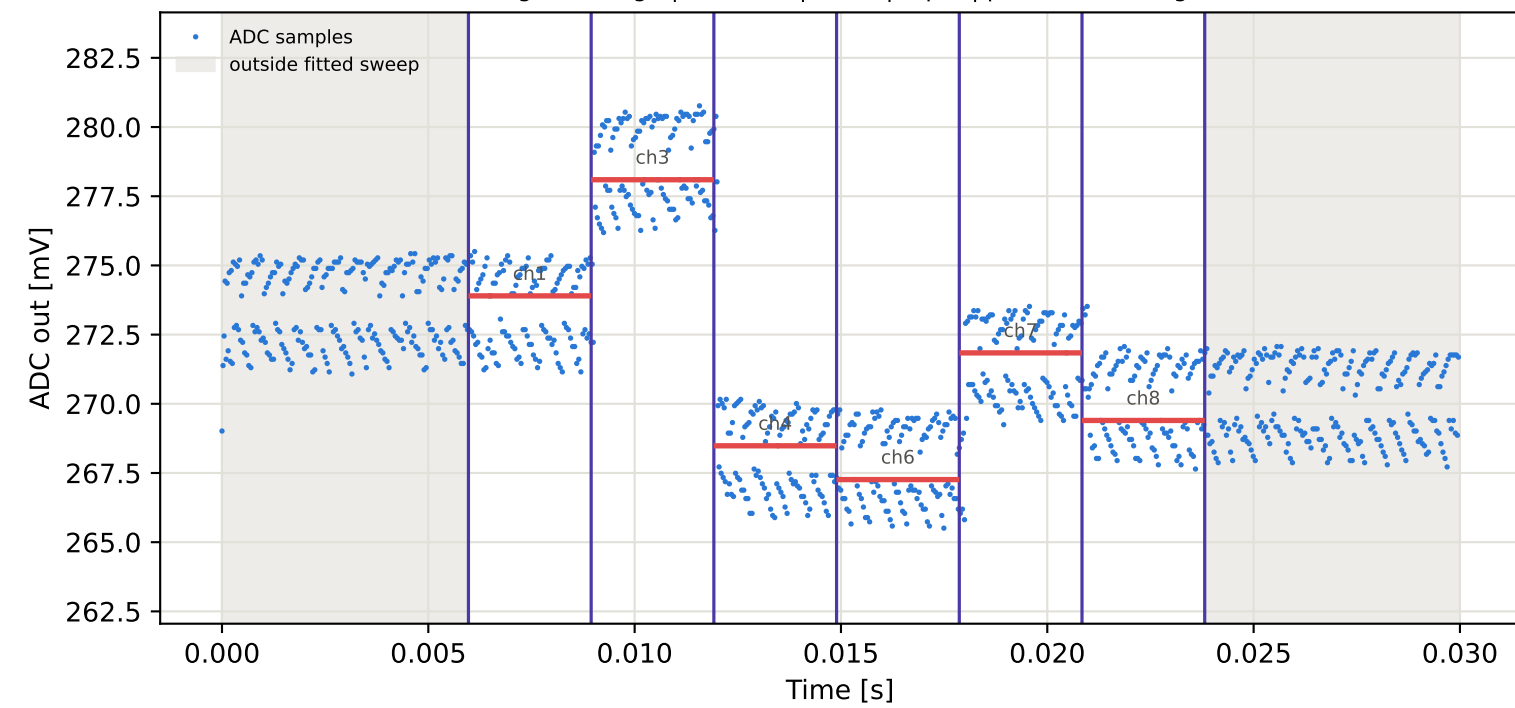
Tag15 &lt;- Tag6 | 795 MHz | run 0 | rep 1 | phase -88.94 deg
