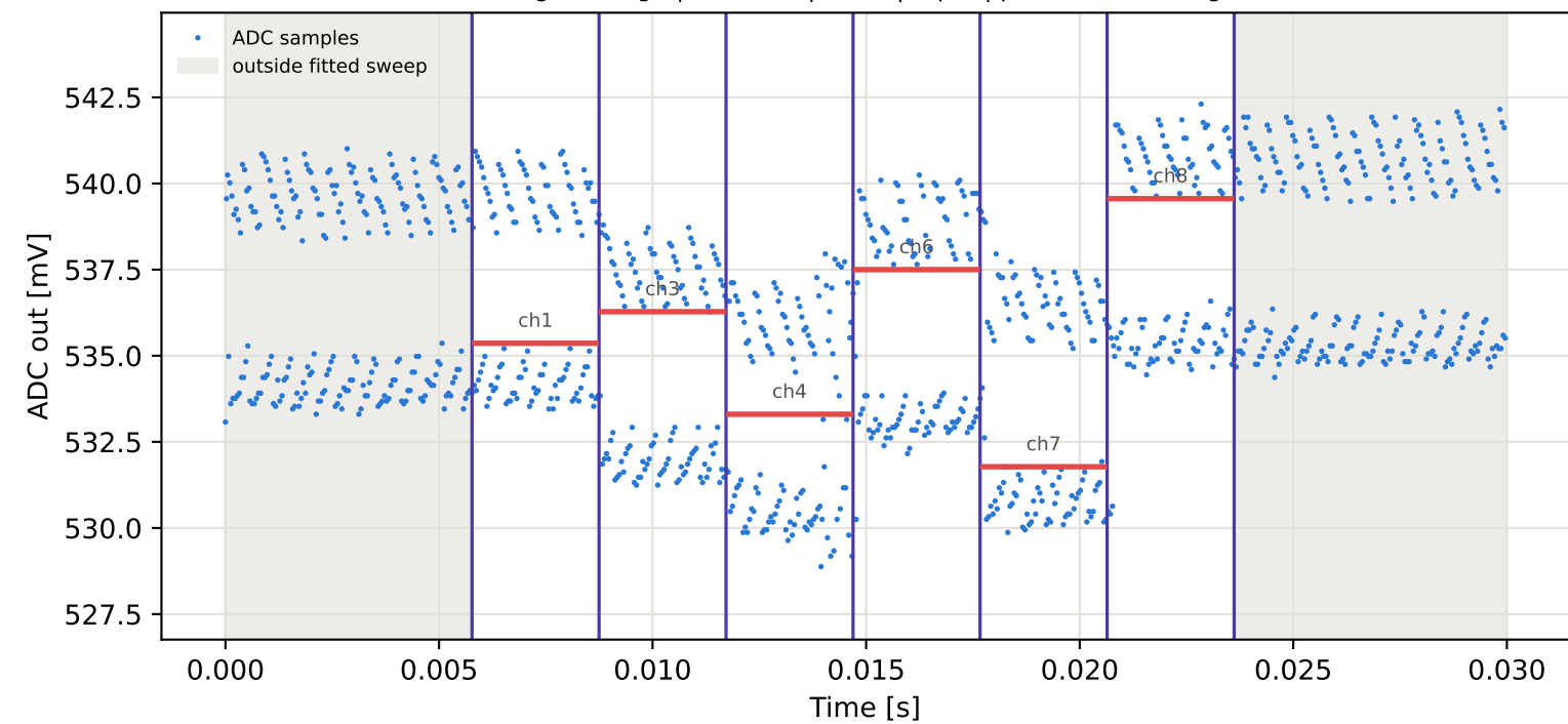
Tag5 &lt;- Tag4 | 835 MHz | run 0 | rep 1 | phase -52.31 deg
