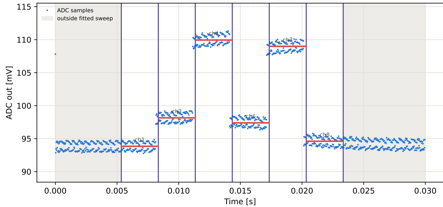
Tag10 &lt;- Tag1 | 785 MHz | run 0 | rep 1 | phase -71.90 deg
