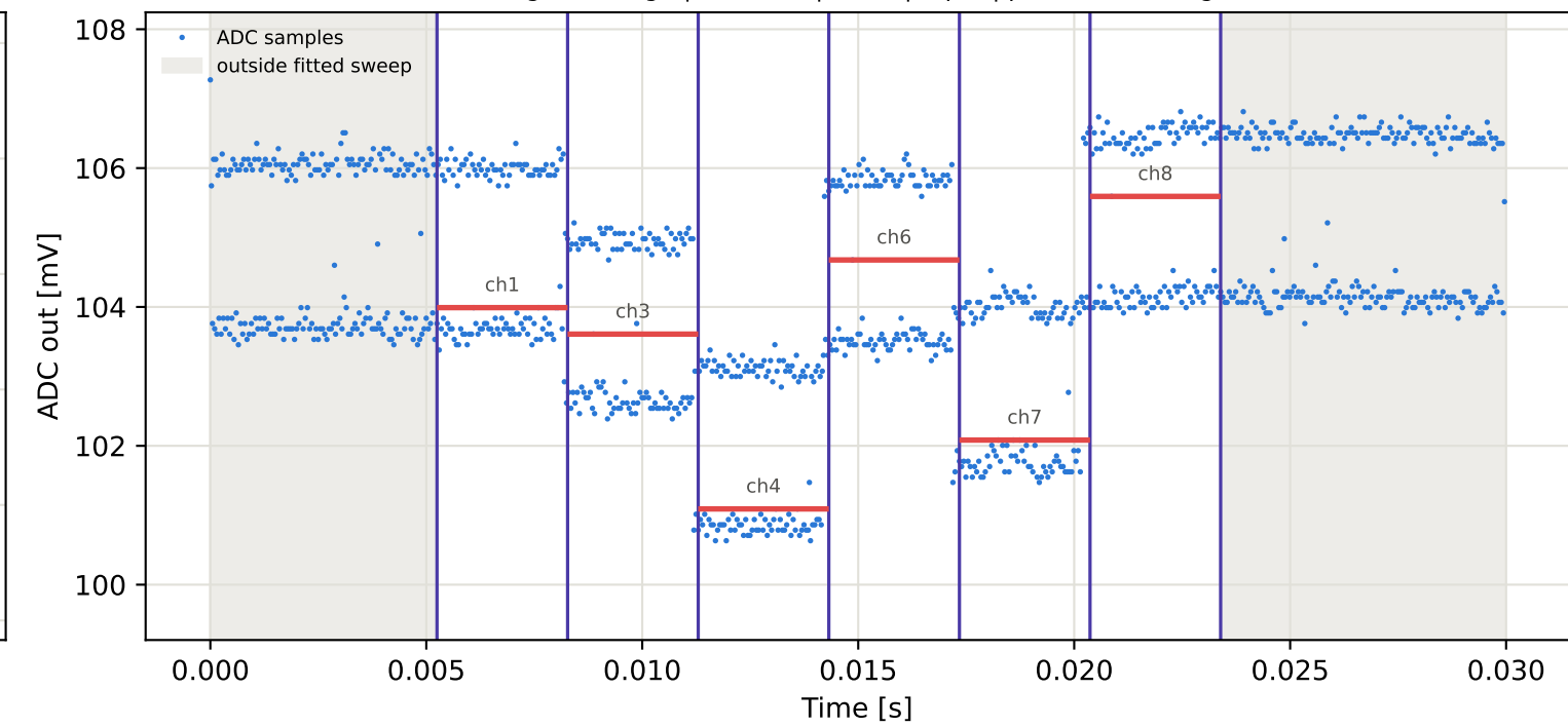
Tag10 &lt;- Tag9 | 995 MHz | run 0 | rep 1 | phase -59.19 deg
