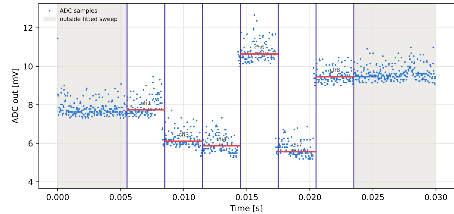
Tag2 &lt;- Tag16 | 955 MHz | run 0 | rep 1 | phase 151.72 deg
