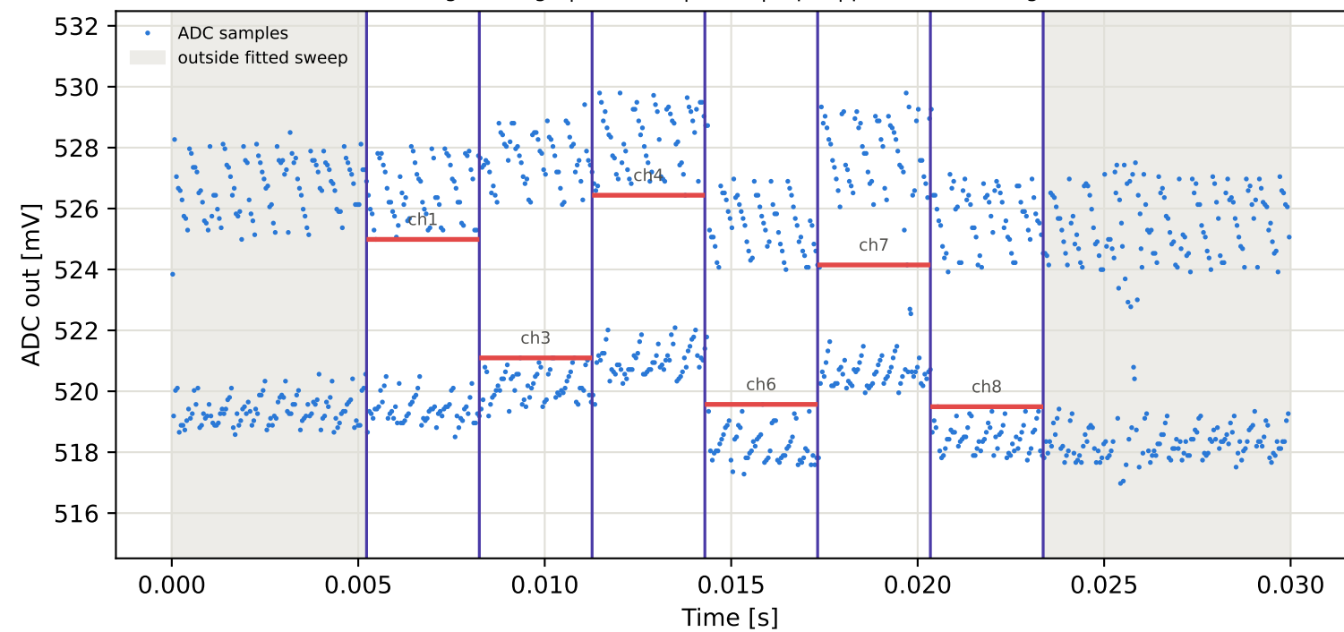
Tag5 &lt;- Tag4 | 945 MHz | run 0 | rep 1 | phase 176.82 deg
