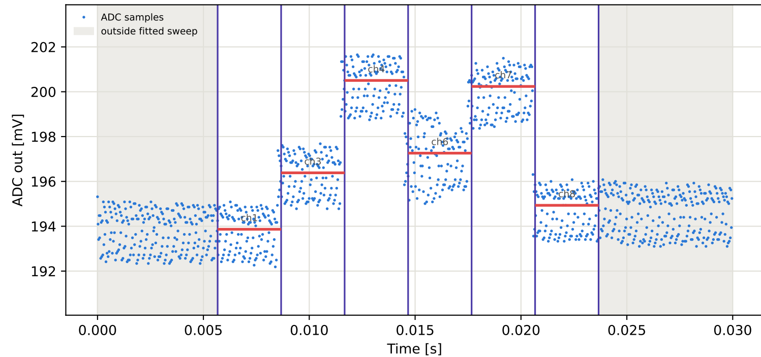
Tag3 &lt;- Tag9 | 805 MHz | run 0 | rep 1 | phase -44.04 deg
