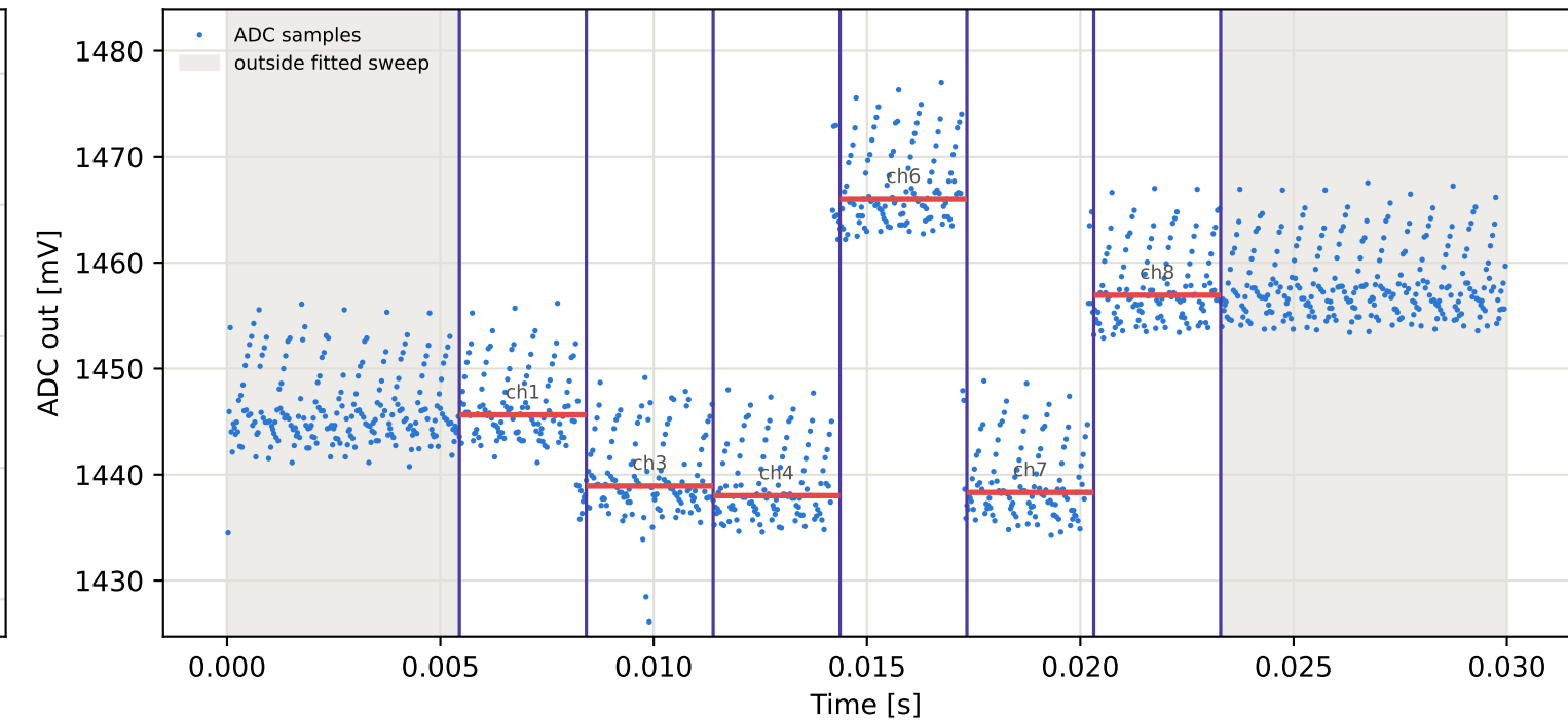
Tag16 &lt;- Tag7 | 935 MHz | run 0 | rep 1 | phase 122.32 deg
