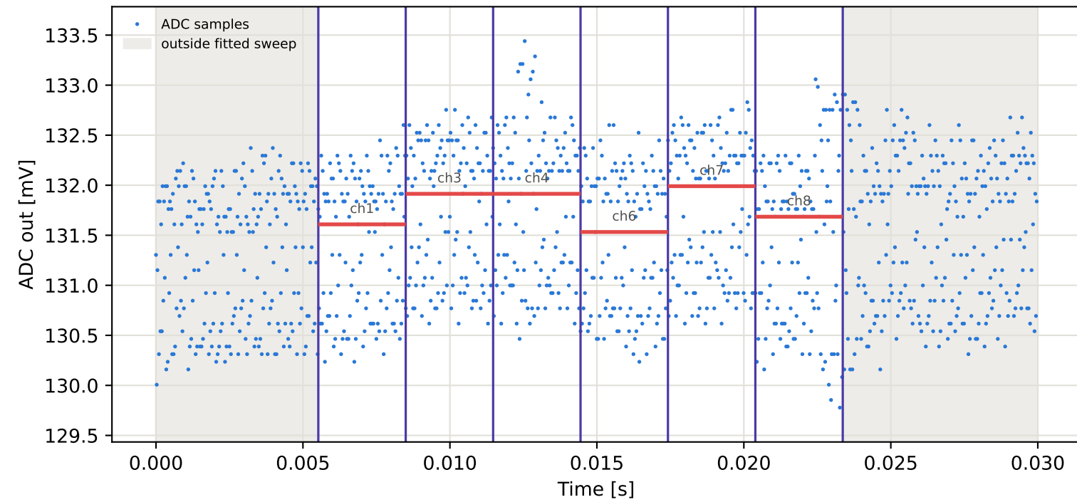
Tag1 &lt;- Tag4 | 805 MHz | run 0 | rep 1 | phase 121.62 deg
