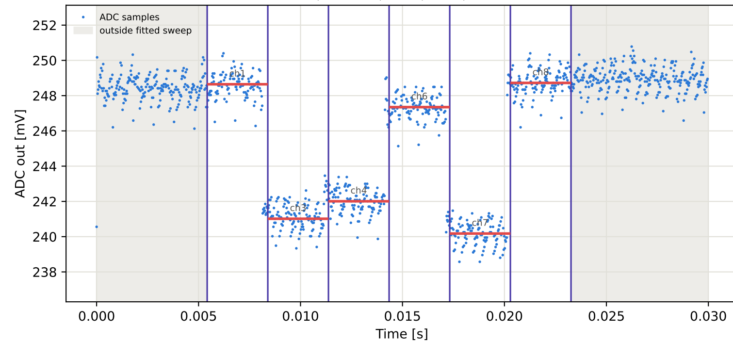
Tag2 &lt;- Tag15 | 835 MHz | run 0 | rep 1 | phase 139.36 deg
