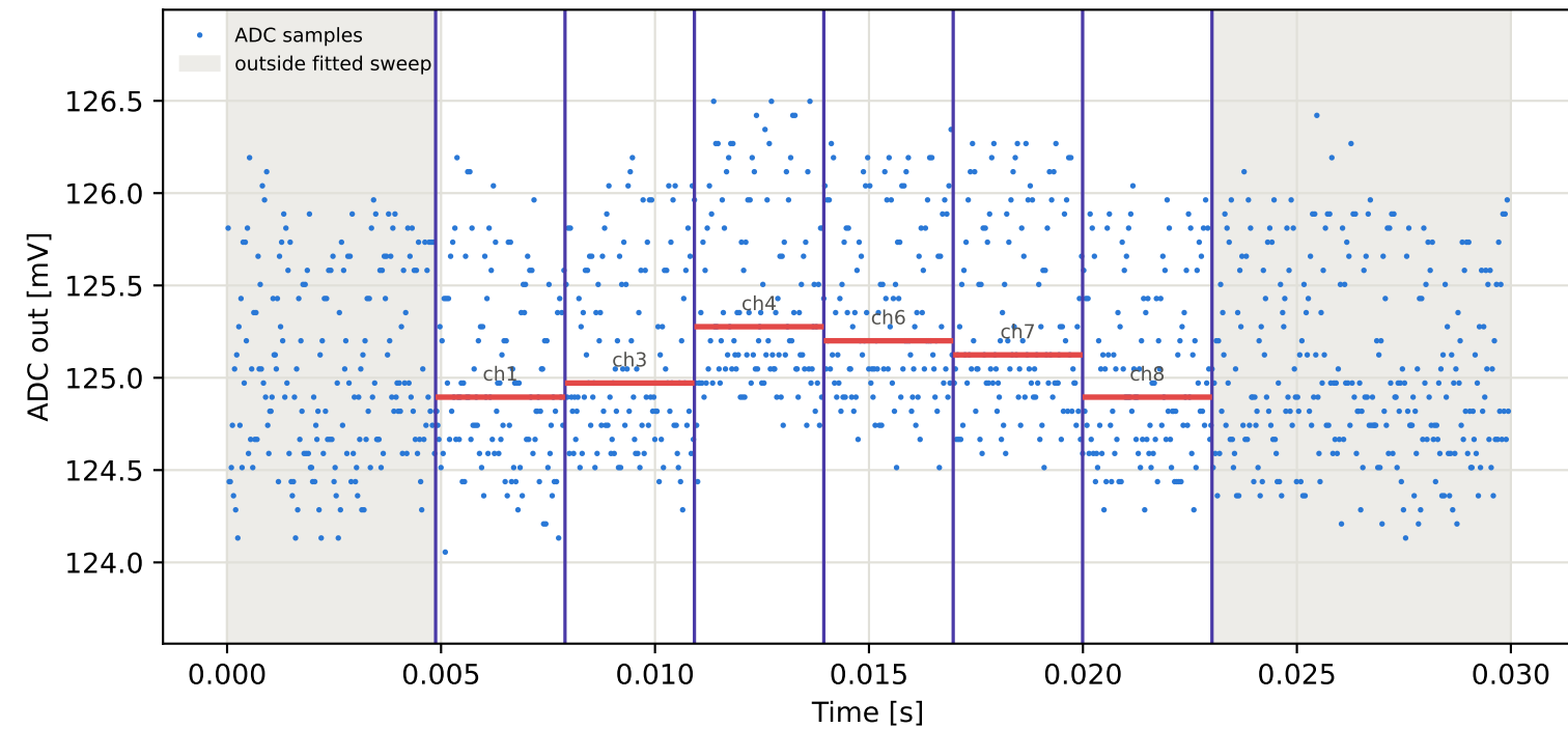
Tag5 &lt;- Tag4 | 785 MHz | run 0 | rep 1 | phase -94.11 deg
