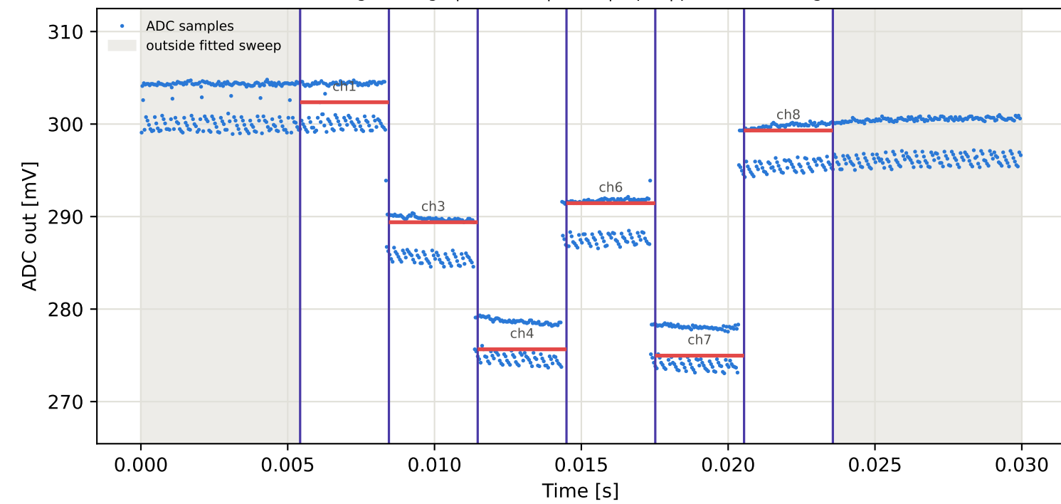
Tag3 &lt;- Tag7 | 835 MHz | run 0 | rep 1 | phase -54.28 deg
