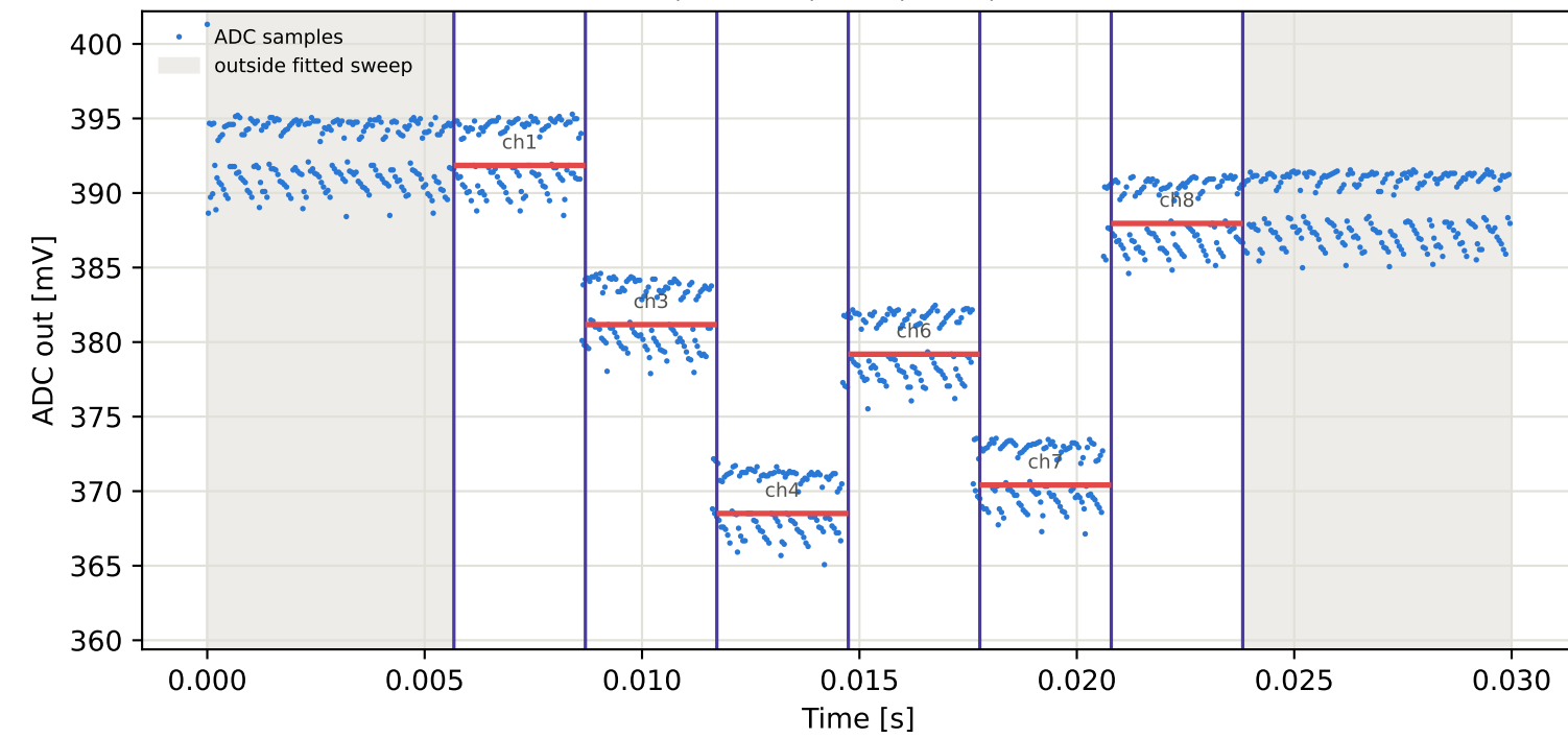
Tag4 &lt;- Tag9 | 825 MHz | run 0 | rep 1 | phase 92.36 deg
