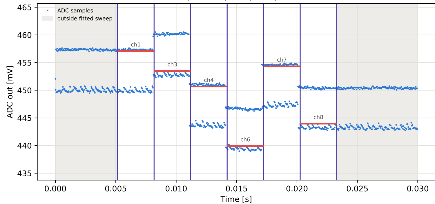
Tag15 &lt;- Tag9 | 845 MHz | run 0 | rep 1 | phase -110.94 deg
