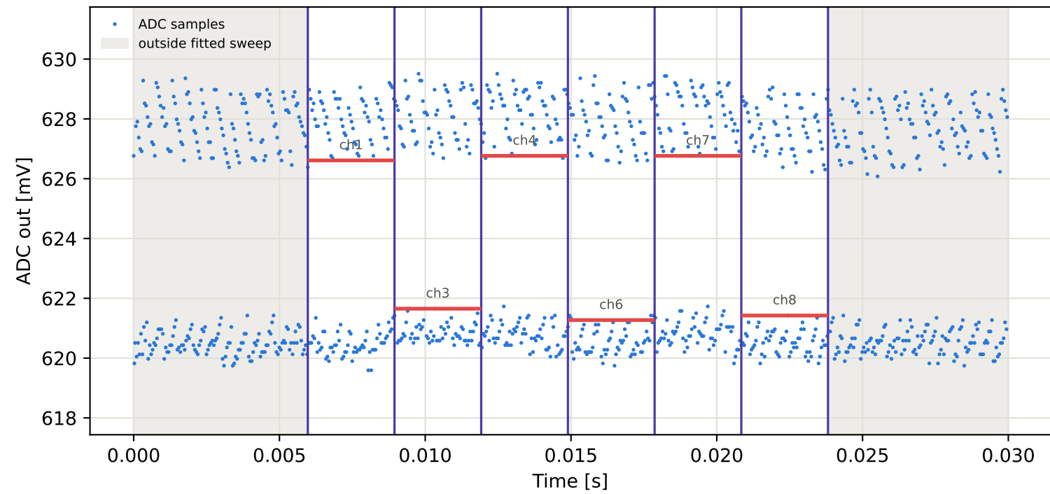
Tag4 &lt;- Tag15 | 855 MHz | run 0 | rep 1 | phase -0.34 deg
