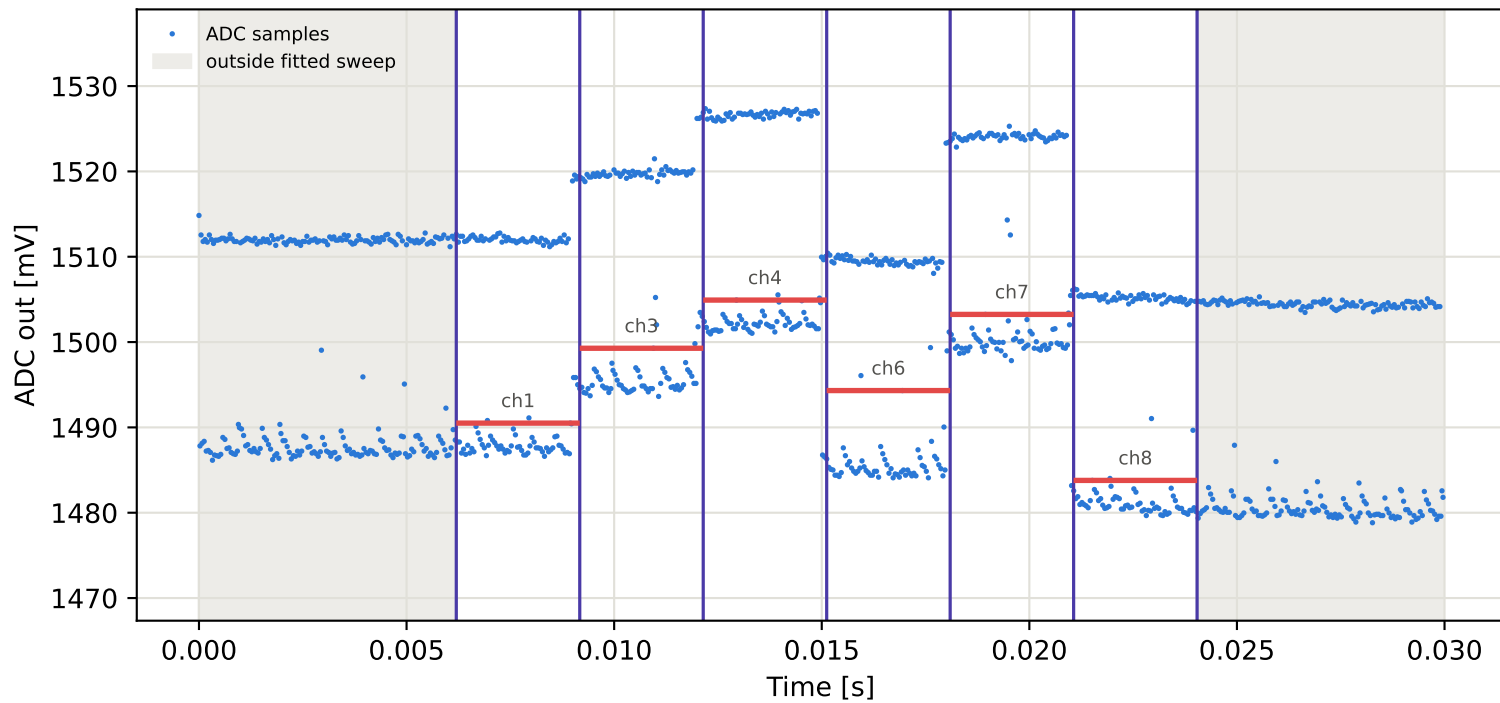
Tag8 &lt;- Tag16 | 925 MHz | run 0 | rep 1 | phase 143.59 deg
