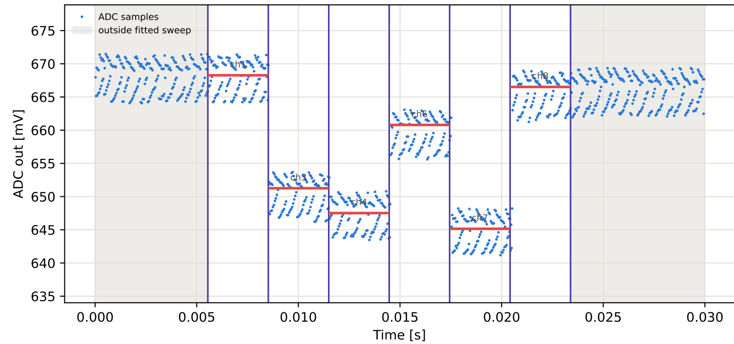
Tag8 &lt;- Tag5 | 825 MHz | run 0 | rep 1 | phase 12.92 deg
