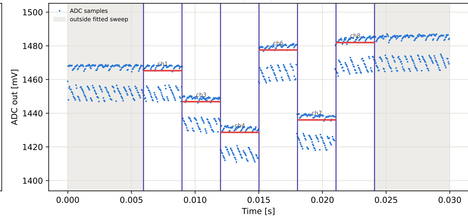
Tag16 &lt;- Tag7 | 935 MHz | run 0 | rep 1 | phase 122.32 deg
