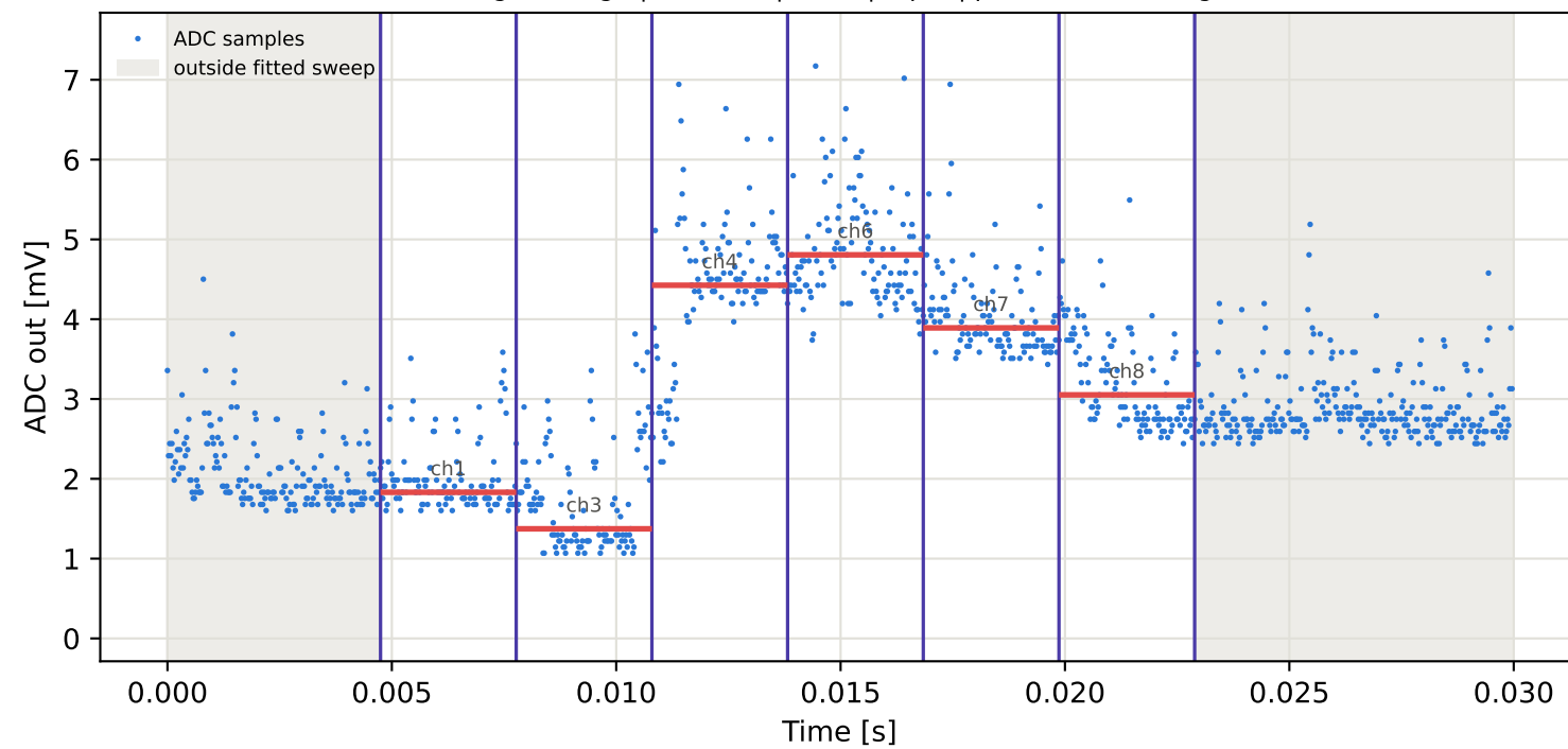
Tag2 &lt;- Tag5 | 795 MHz | run 0 | rep 1 | phase 73.08 deg
