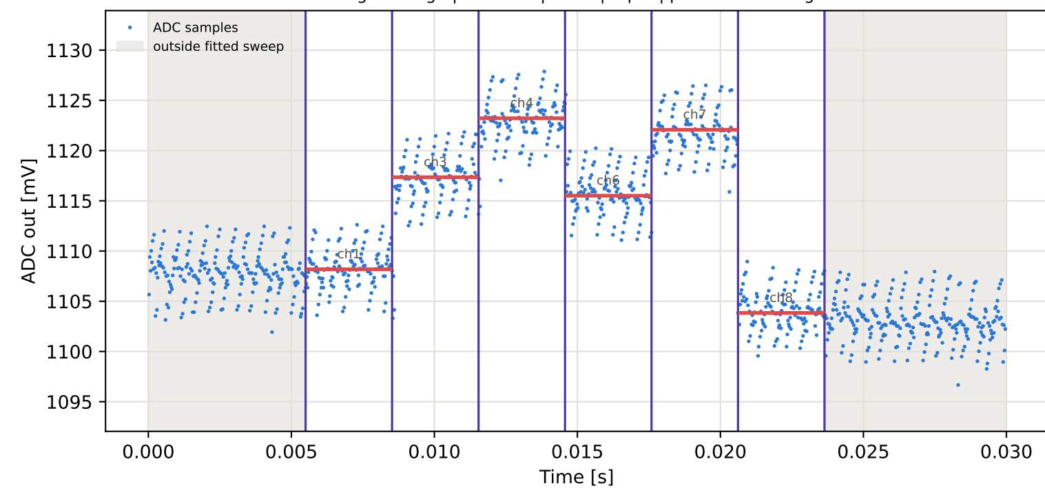
Tag4 &lt;- Tag9 | 895 MHz | run 0 | rep 1 | phase 176.21 deg
