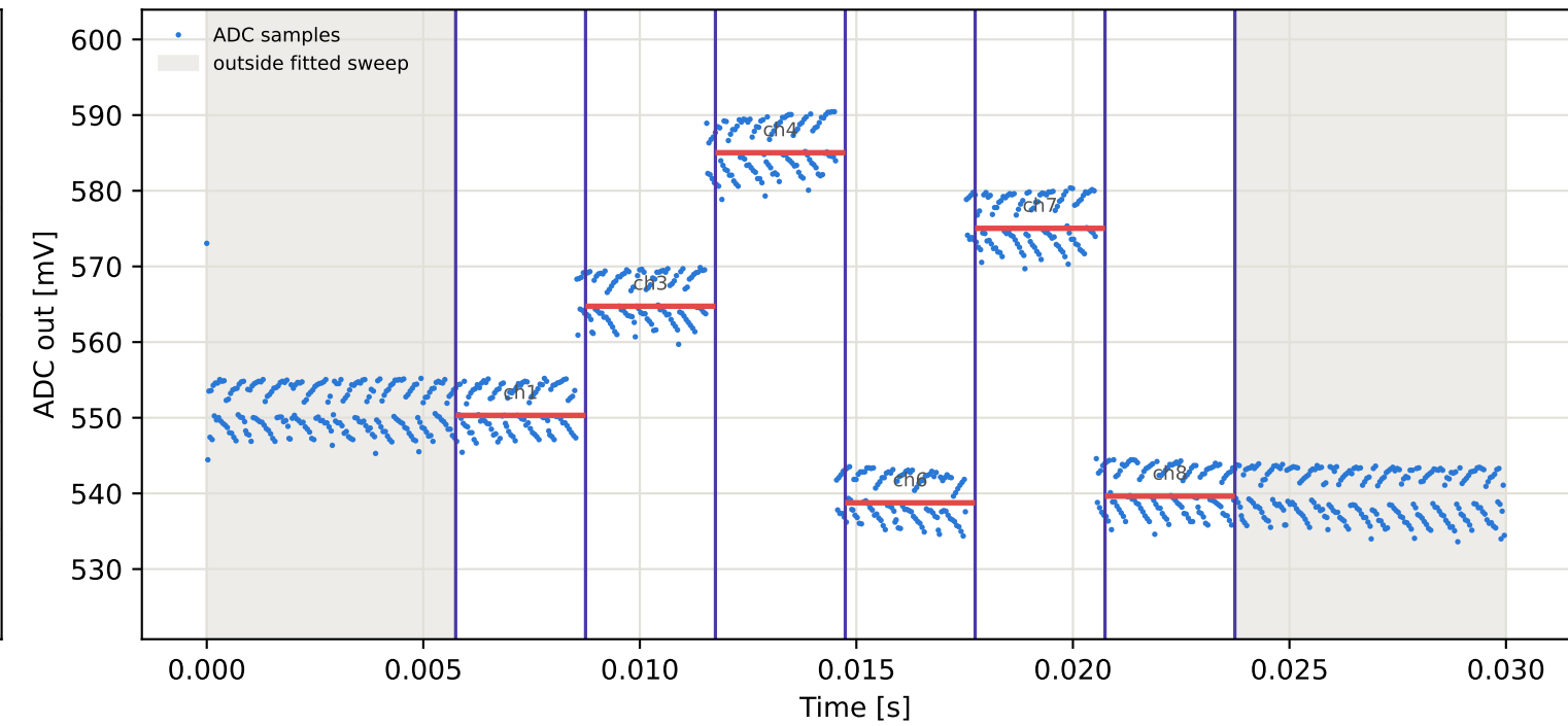
Tag7 &lt;- Tag6 | 965 MHz | run 0 | rep 1 | phase -171.65 deg
