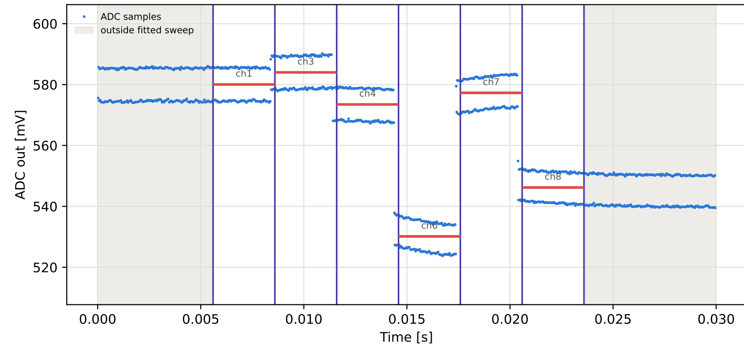
Tag7 &lt;- Tag10 | 905 MHz | run 0 | rep 1 | phase 18.04 deg
