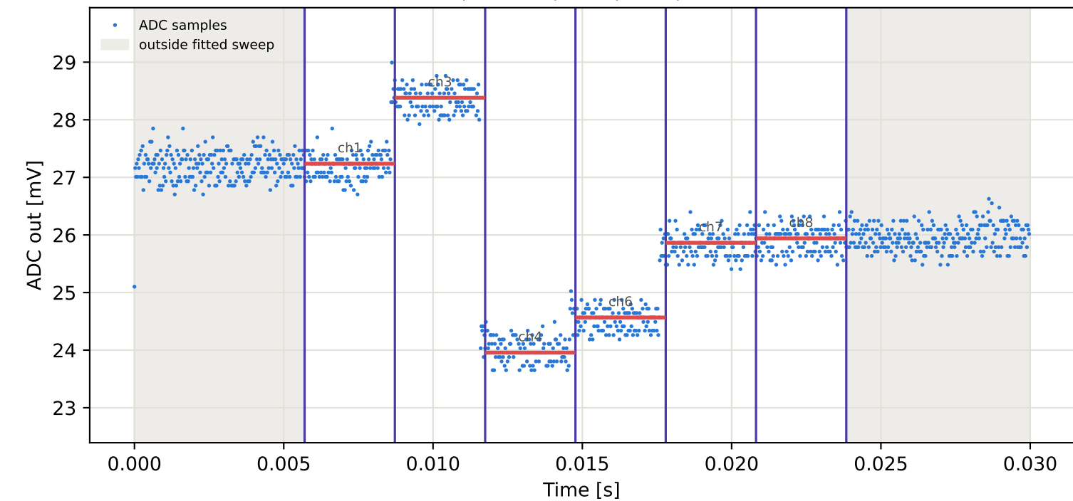
Tag7 &lt;- Tag15 | 775 MHz | run 0 | rep 1 | phase 61.07 deg
