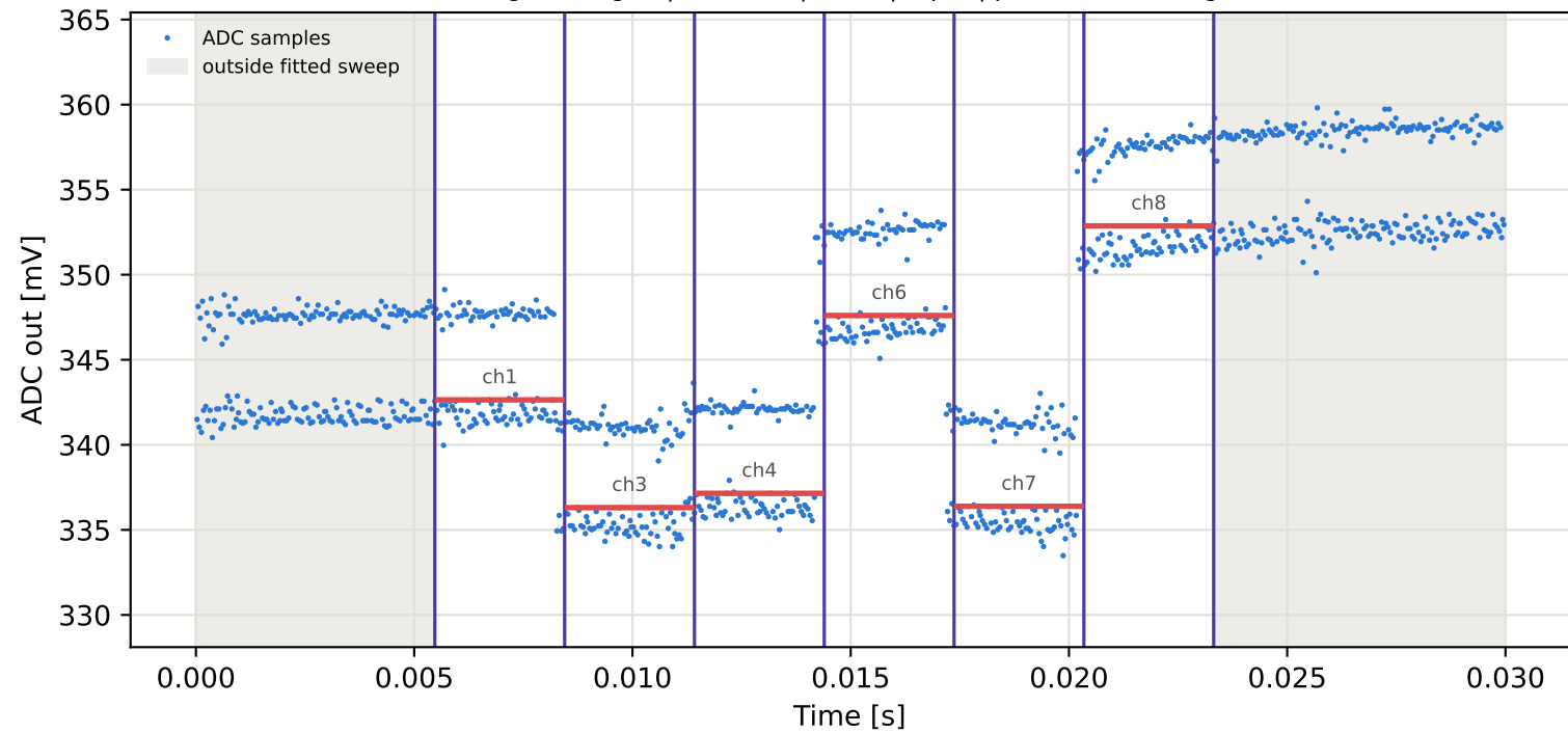
Tag1 &lt;- Tag2 | 885 MHz | run 0 | rep 1 | phase -28.81 deg
