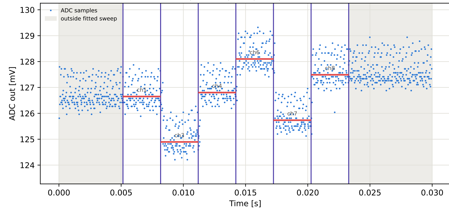
Tag1 &lt;- Tag9 | 785 MHz | run 0 | rep 1 | phase -160.82 deg
