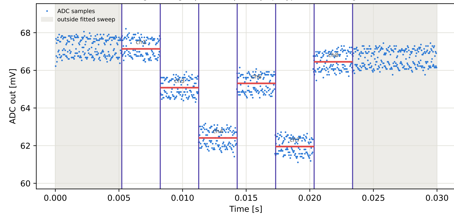
Tag10 &lt;- Tag3 | 795 MHz | run 0 | rep 1 | phase 43.97 deg
