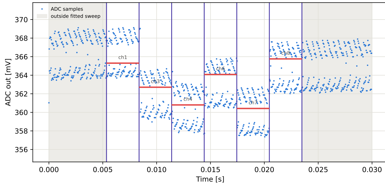
Tag15 &lt;- Tag3 | 825 MHz | run 0 | rep 1 | phase 166.70 deg
