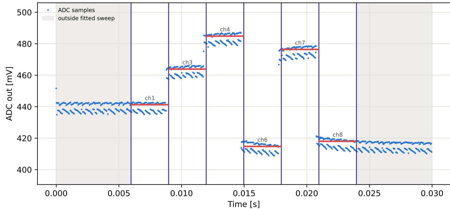
Tag9 &lt;- Tag8 | 945 MHz | run 0 | rep 1 | phase 36.11 deg
