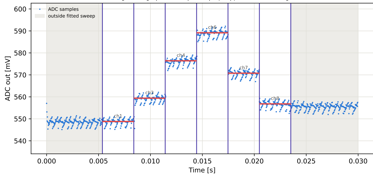
Tag6 &lt;- Tag5 | 905 MHz | run 0 | rep 1 | phase -132.60 deg
