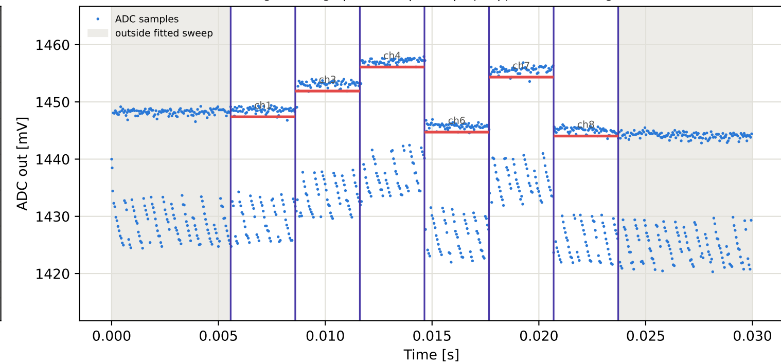
Tag16 &lt;- Tag15 | 935 MHz | run 0 | rep 1 | phase -175.53 deg
