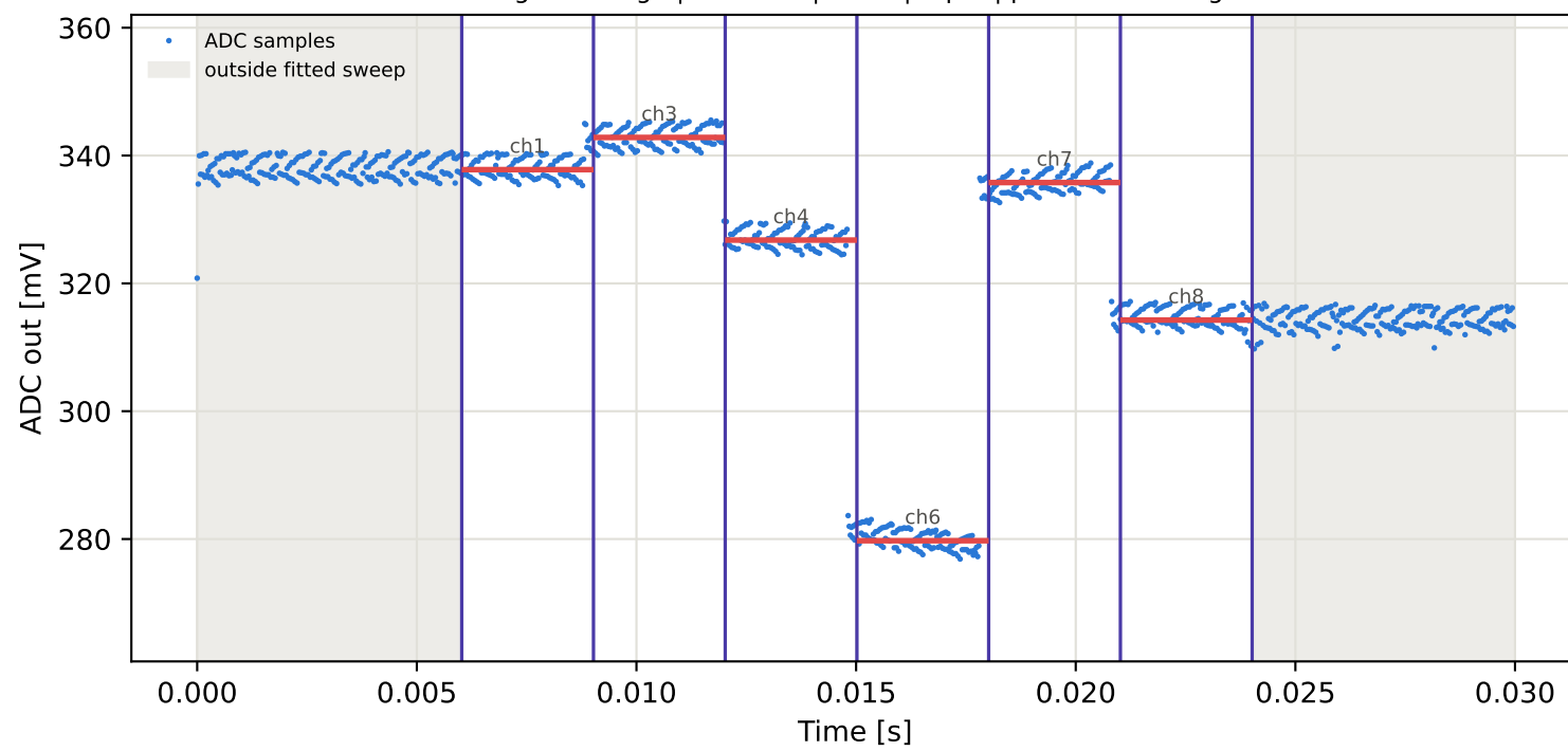
Tag10 &lt;- Tag8 | 935 MHz | run 0 | rep 1 | phase 51.15 deg
