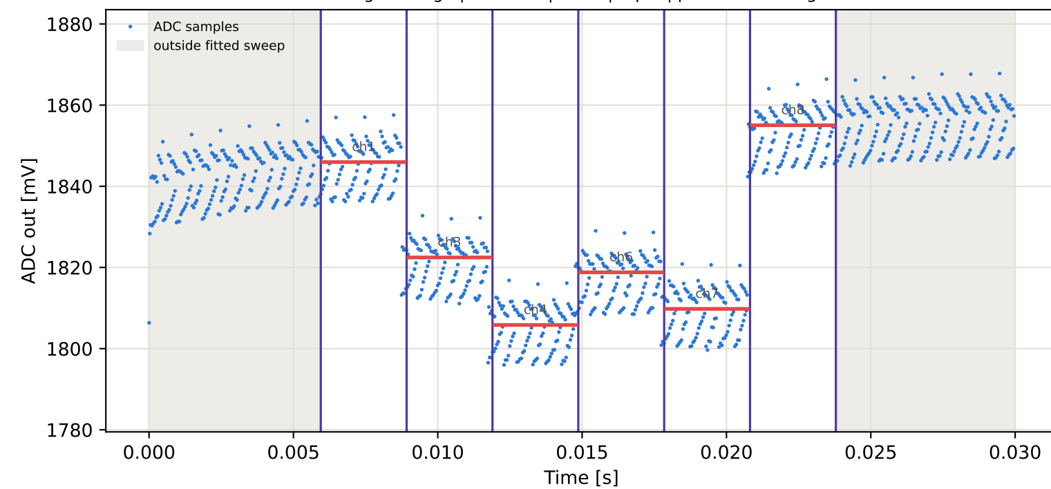
Tag9 &lt;- Tag10 | 895 MHz | run 0 | rep 1 | phase 43.52 deg
