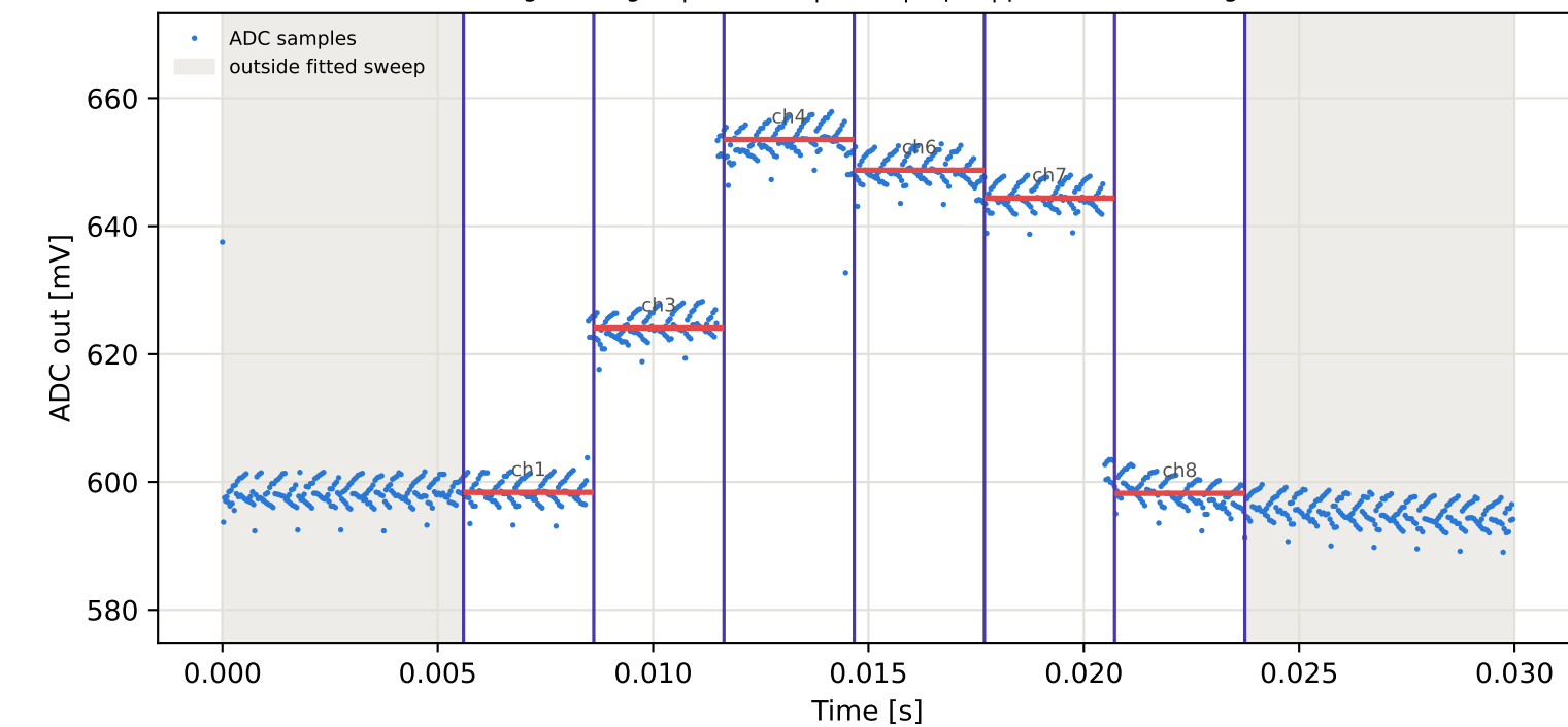
Tag9 &lt;- Tag16 | 895 MHz | run 0 | rep 1 | phase -109.62 deg
