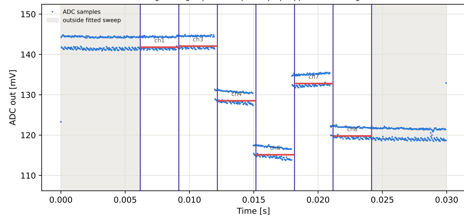
Tag1 &lt;- Tag16 | 865 MHz | run 0 | rep 1 | phase -130.51 deg
