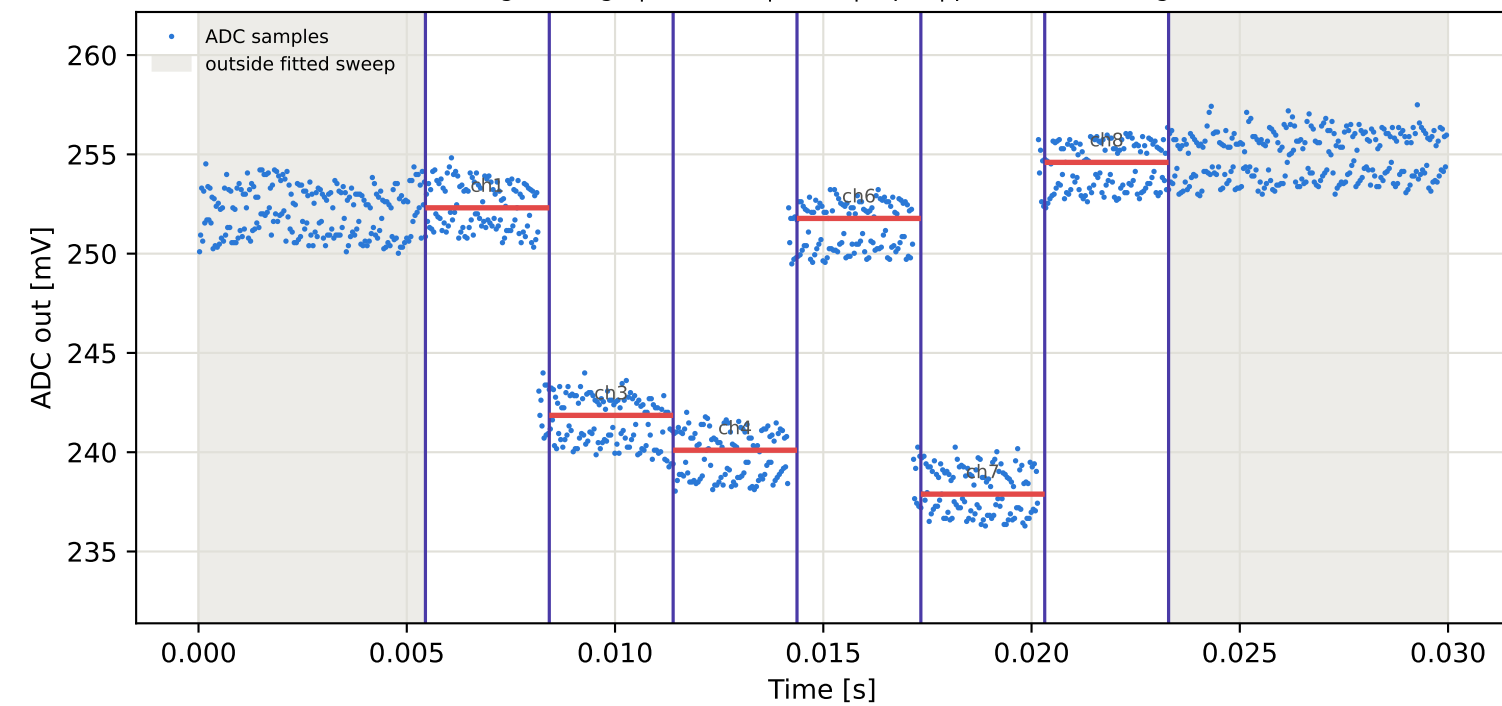
Tag3 &lt;- Tag10 | 835 MHz | run 0 | rep 1 | phase 132.39 deg
