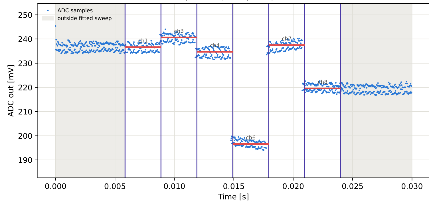
Tag2 &lt;- Tag6 | 925 MHz | run 0 | rep 1 | phase -99.77 deg
