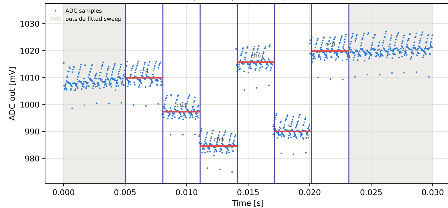
Tag9 &lt;- Tag10 | 945 MHz | run 0 | rep 1 | phase -179.62 deg
