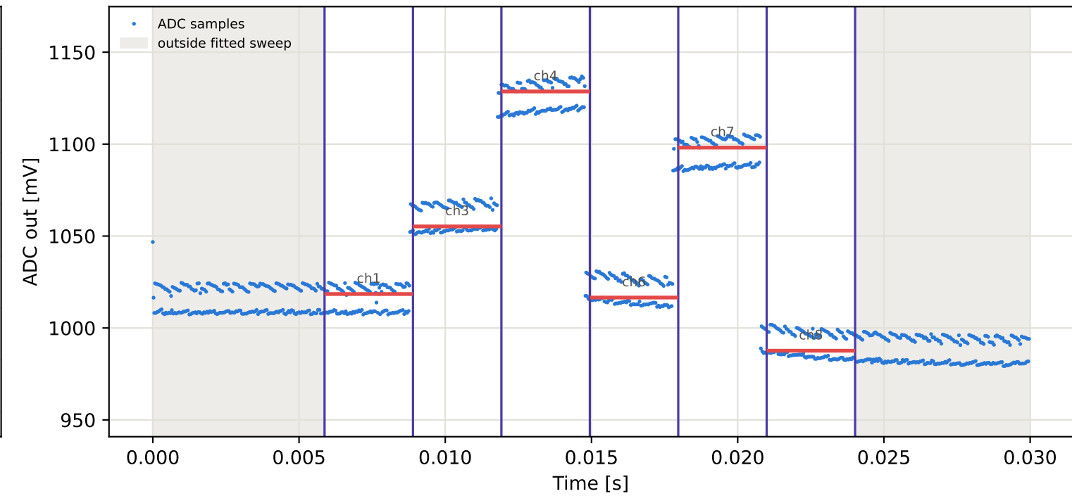
Tag5 &lt;- Tag1 | 945 MHz | run 0 | rep 1 | phase -24.04 deg
