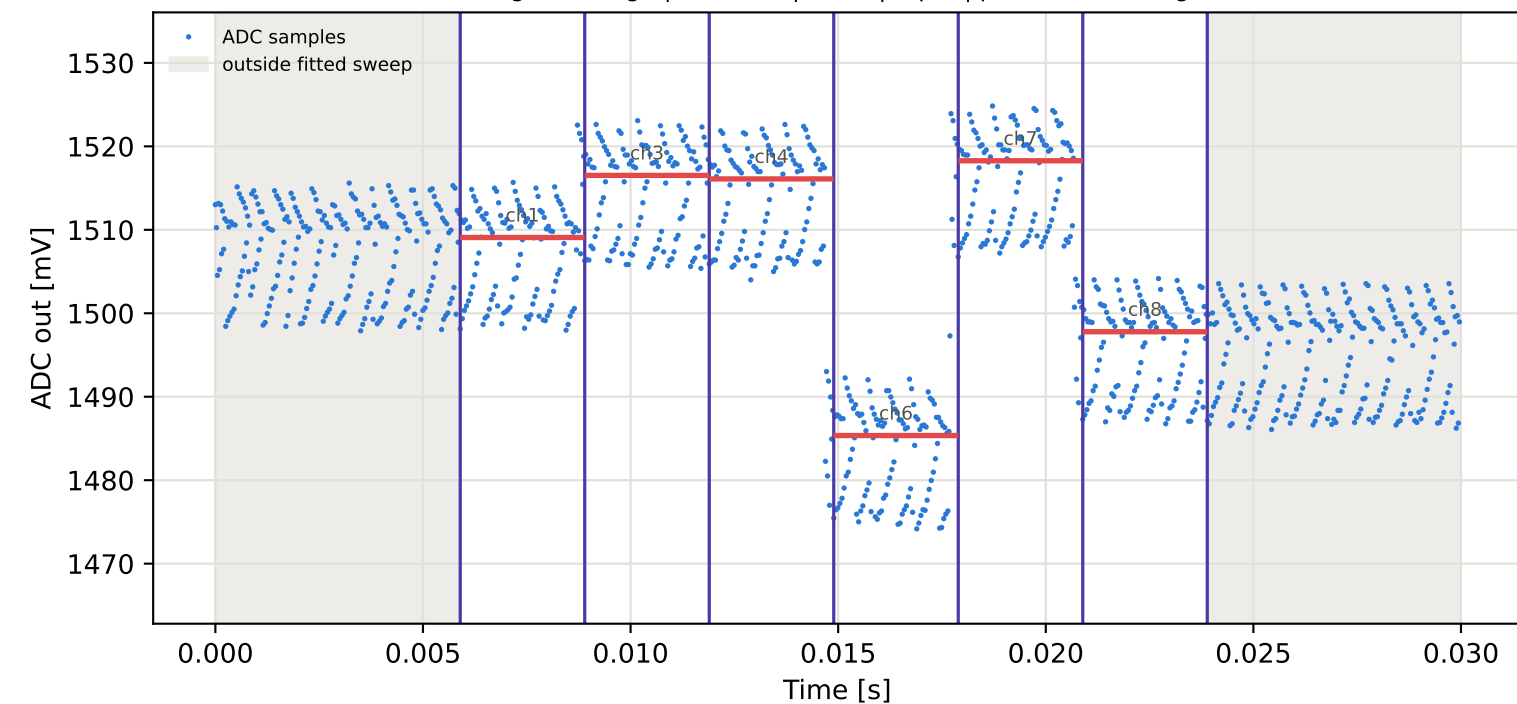
Tag15 &lt;- Tag5 | 965 MHz | run 0 | rep 1 | phase 95.34 deg
