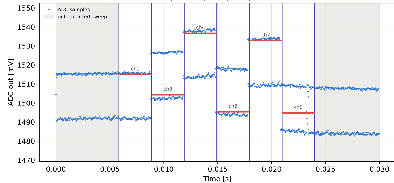
Tag4 &lt;- Tag15 | 925 MHz | run 0 | rep 1 | phase 64.33 deg
