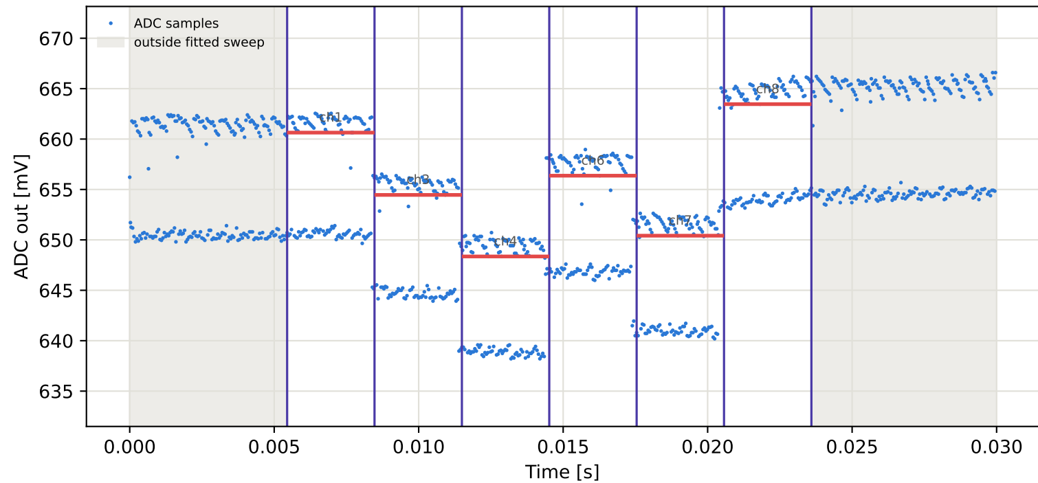
Tag7 &lt;- Tag15 | 915 MHz | run 0 | rep 1 | phase -100.11 deg
