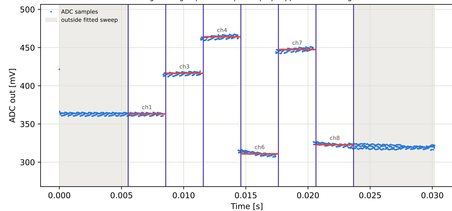
Tag9 &lt;- Tag16 | 985 MHz | run 0 | rep 1 | phase -52.82 deg
