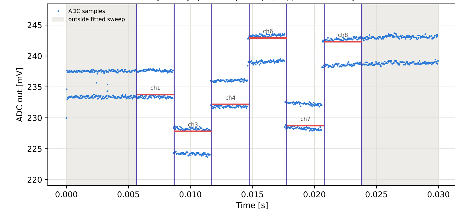
Tag7 &lt;- Tag6 | 825 MHz | run 0 | rep 1 | phase 178.31 deg
