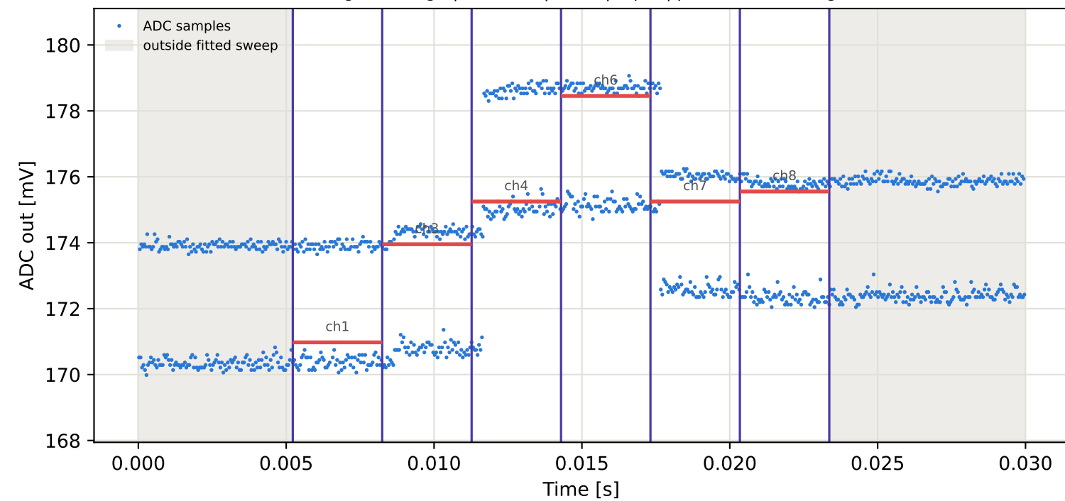
Tag10 &lt;- Tag9 | 985 MHz | run 0 | rep 1 | phase -49.78 deg
