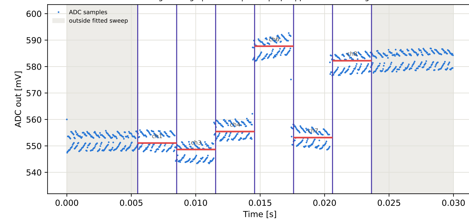
Tag6 &lt;- Tag1 | 895 MHz | run 0 | rep 1 | phase -176.97 deg
