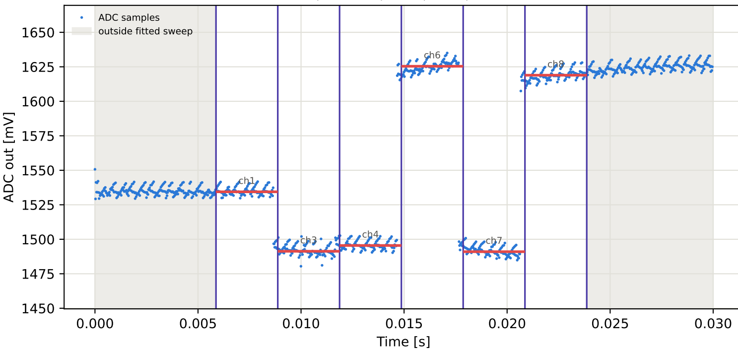
Tag8 &lt;- Tag15 | 915 MHz | run 0 | rep 1 | phase 163.74 deg
