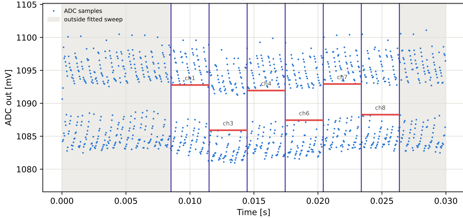
Tag15 &lt;- Tag10 | 975 MHz | run 0 | rep 1 | phase -61.81 deg
