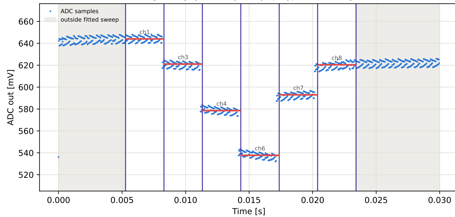
Tag8 &lt;- Tag1 | 905 MHz | run 0 | rep 1 | phase 14.52 deg
