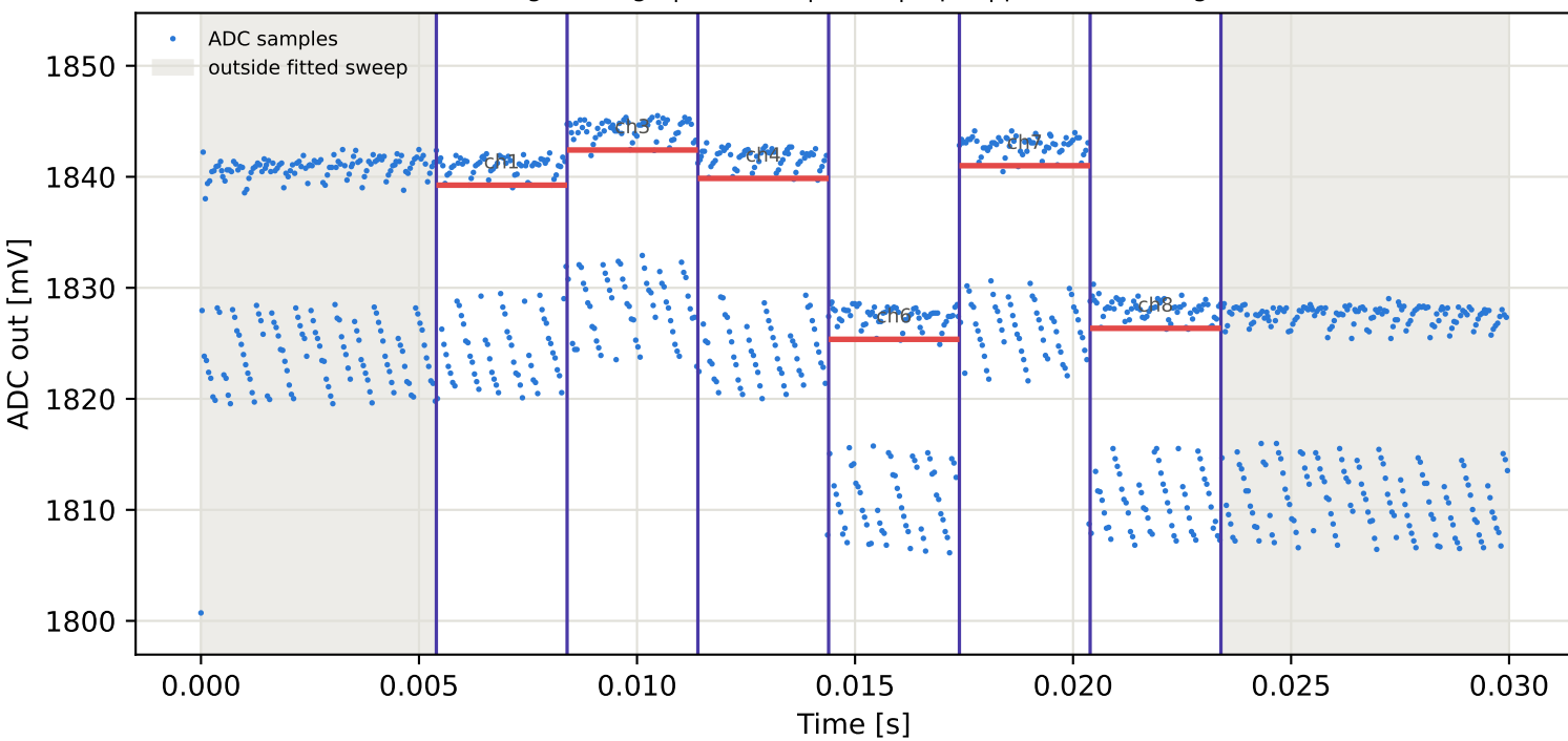
Tag8 &lt;- Tag15 | 895 MHz | run 0 | rep 1 | phase 125.62 deg
