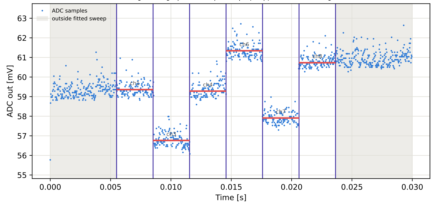
Tag2 &lt;- Tag8 | 805 MHz | run 0 | rep 1 | phase -165.88 deg
