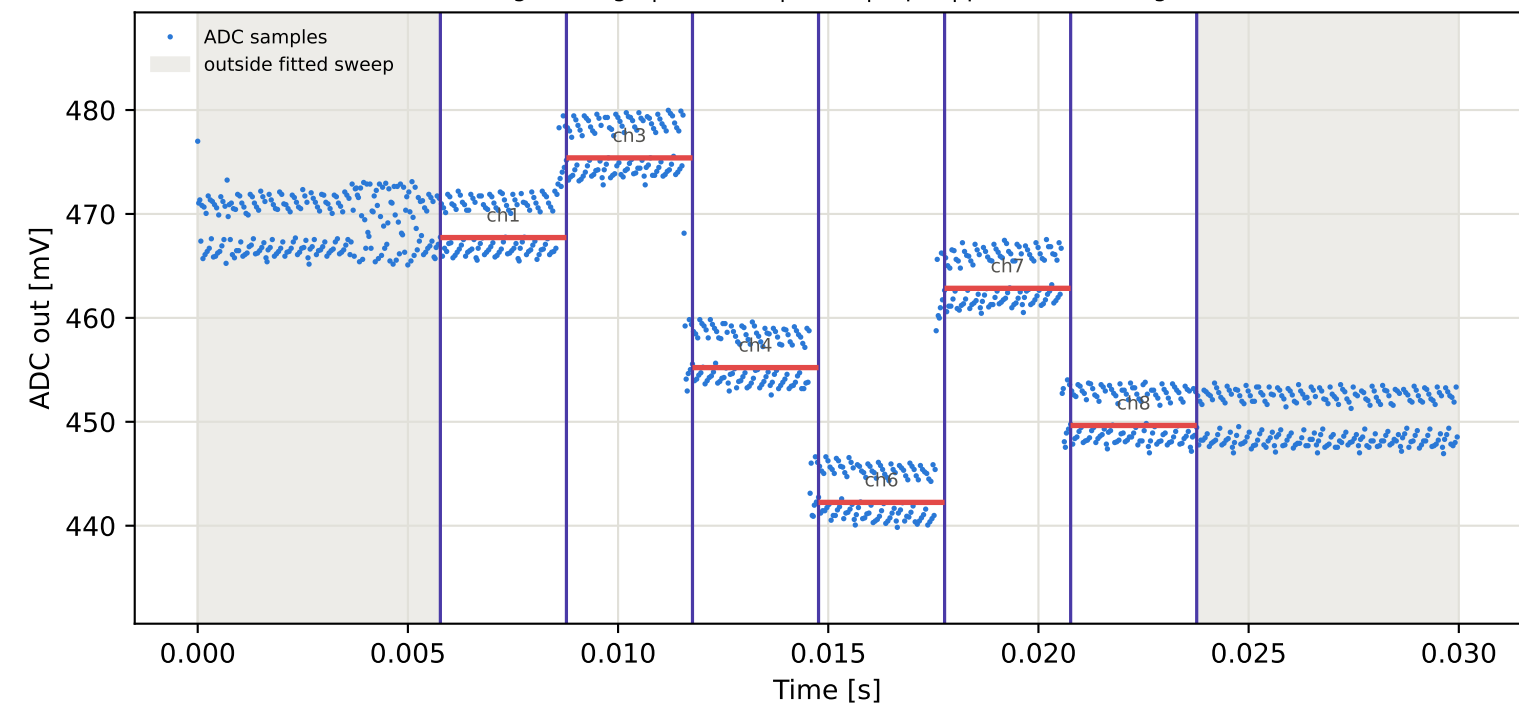
Tag3 &lt;- Tag9 | 855 MHz | run 0 | rep 1 | phase 43.30 deg
