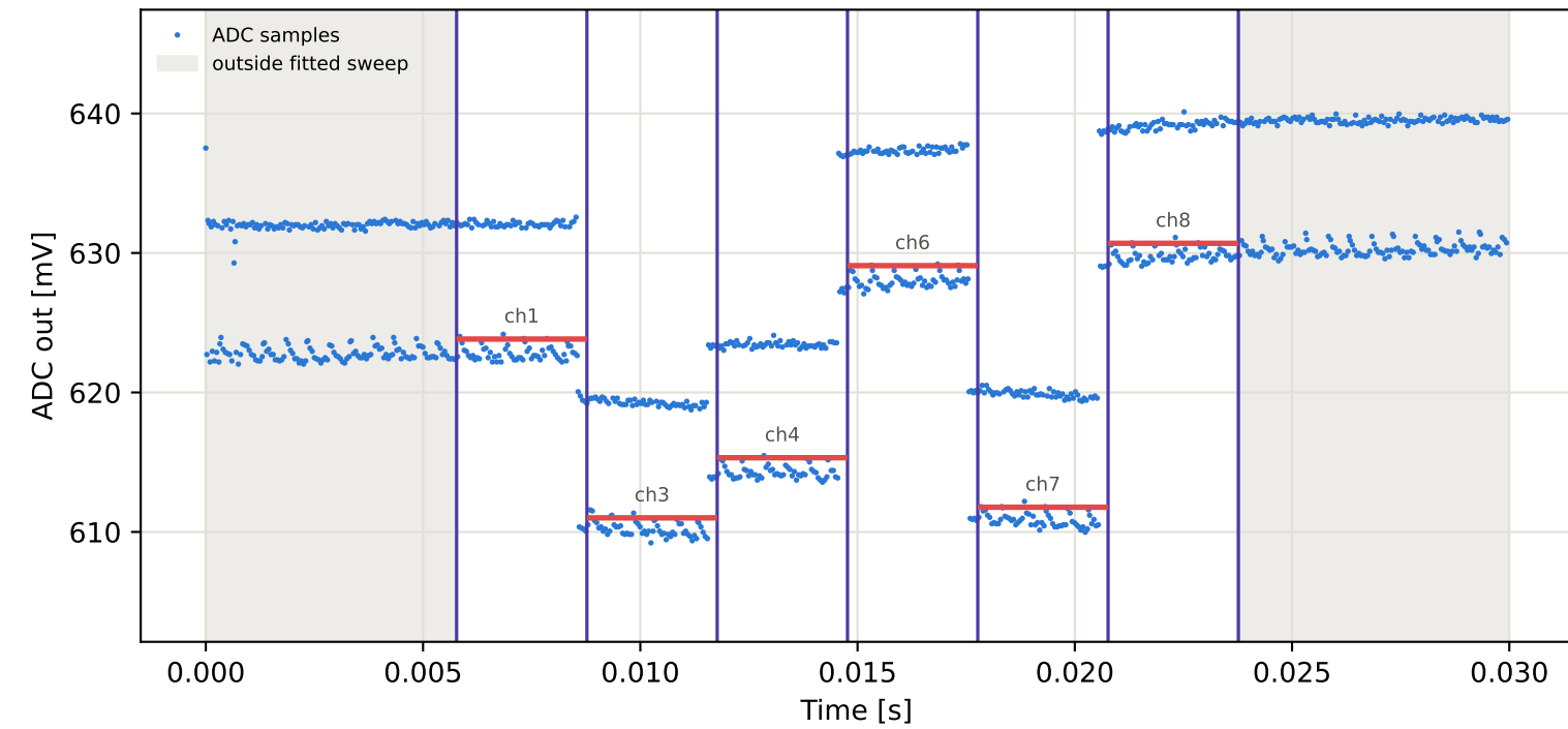
Tag4 &lt;- Tag9 | 855 MHz | run 0 | rep 1 | phase 149.52 deg
