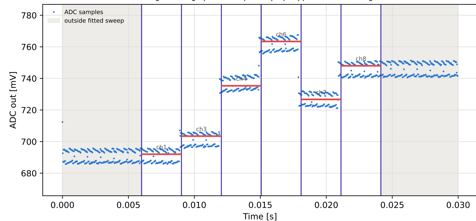
Tag2 &lt;- Tag1 | 865 MHz | run 0 | rep 1 | phase 73.33 deg
