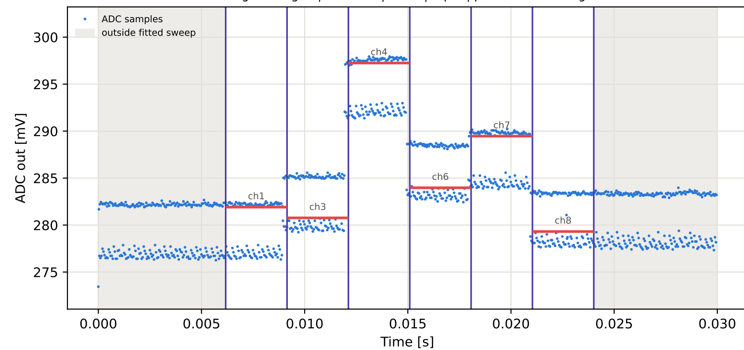
Tag1 &lt;- Tag16 | 995 MHz | run 0 | rep 1 | phase -51.79 deg
