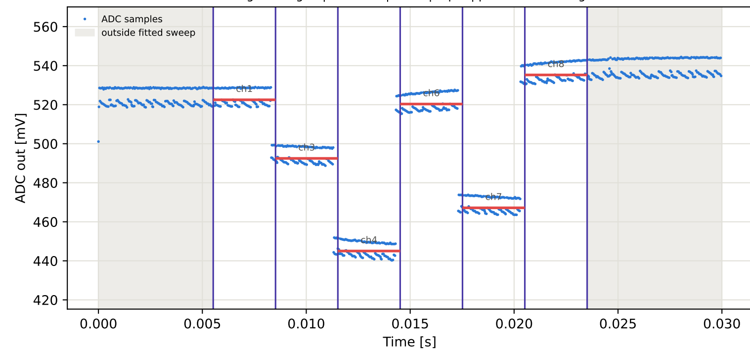
Tag7 &lt;- Tag3 | 955 MHz | run 0 | rep 1 | phase 94.65 deg
