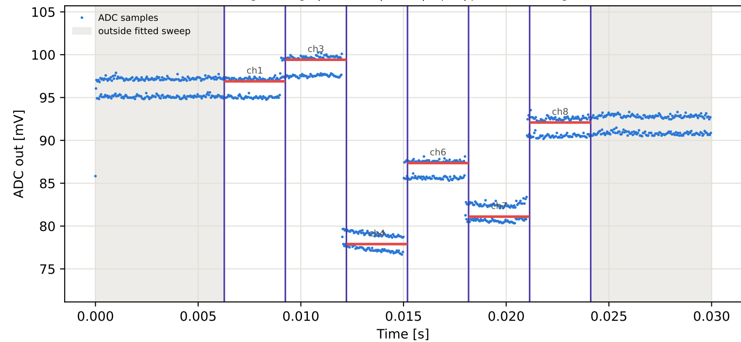
Tag9 &lt;- Tag6 | 785 MHz | run 0 | rep 1 | phase -96.49 deg
