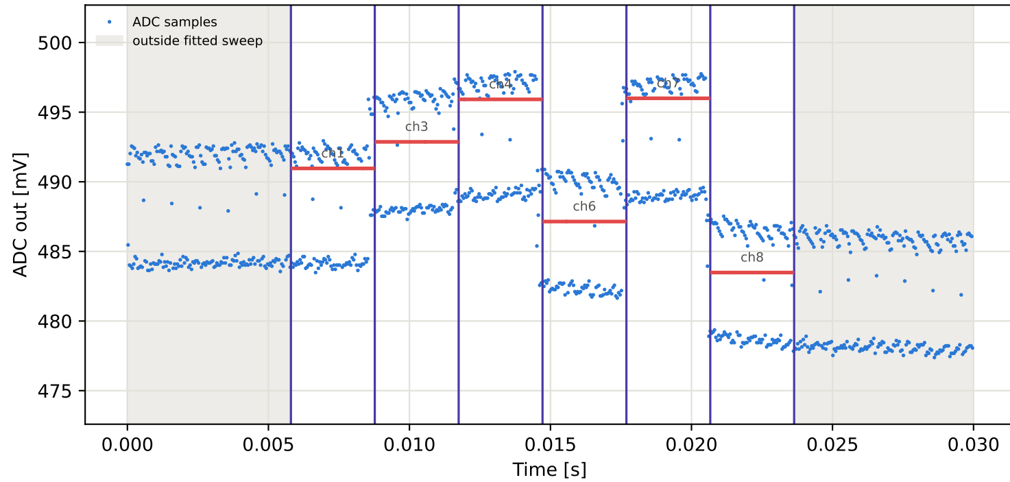
Tag15 &lt;- Tag1 | 895 MHz | run 0 | rep 1 | phase -135.03 deg
