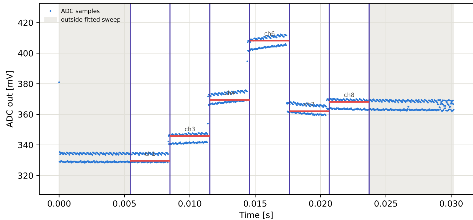
Tag1 &lt;- Tag4 | 895 MHz | run 0 | rep 1 | phase -144.39 deg
