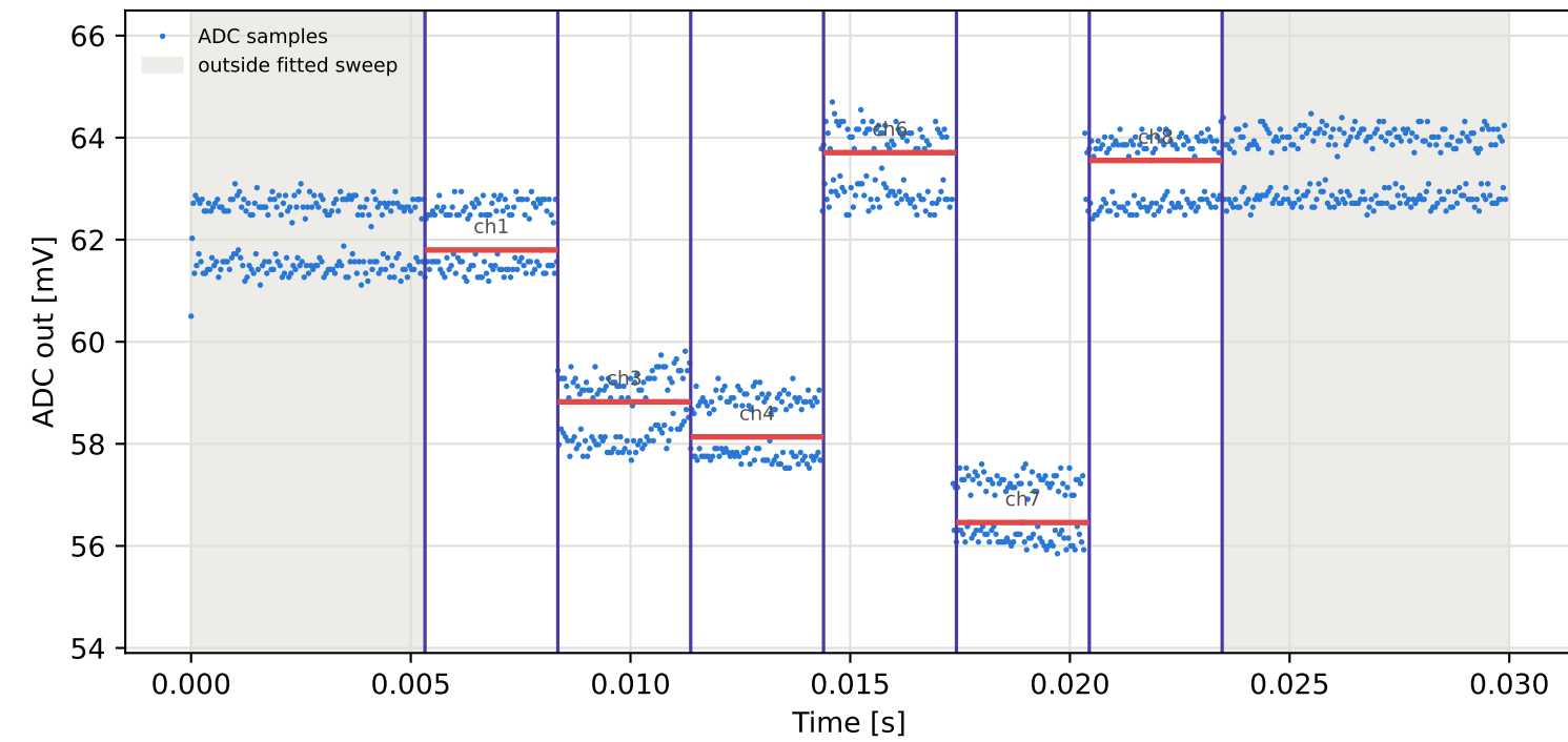
Tag5 &lt;- Tag2 | 795 MHz | run 0 | rep 1 | phase -33.36 deg
