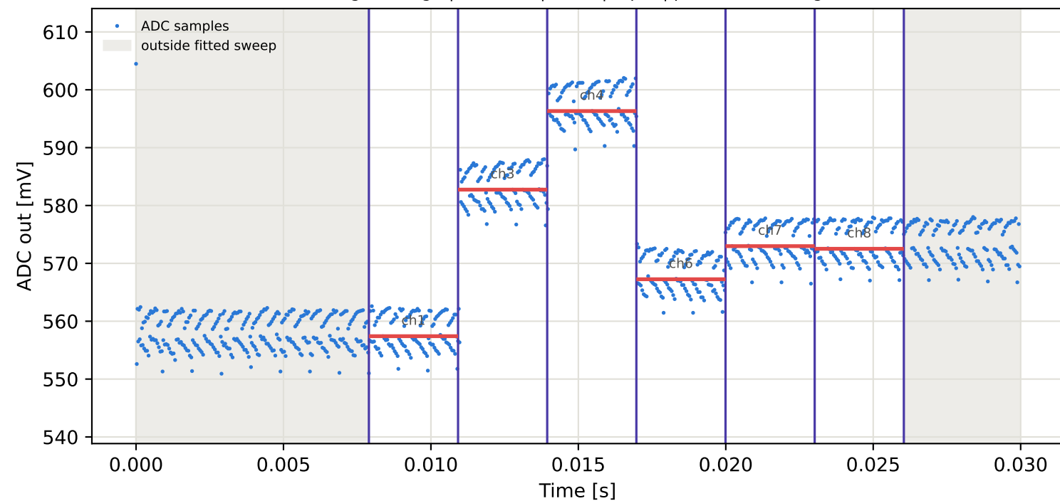
Tag8 &lt;- Tag10 | 965 MHz | run 0 | rep 1 | phase -68.88 deg
