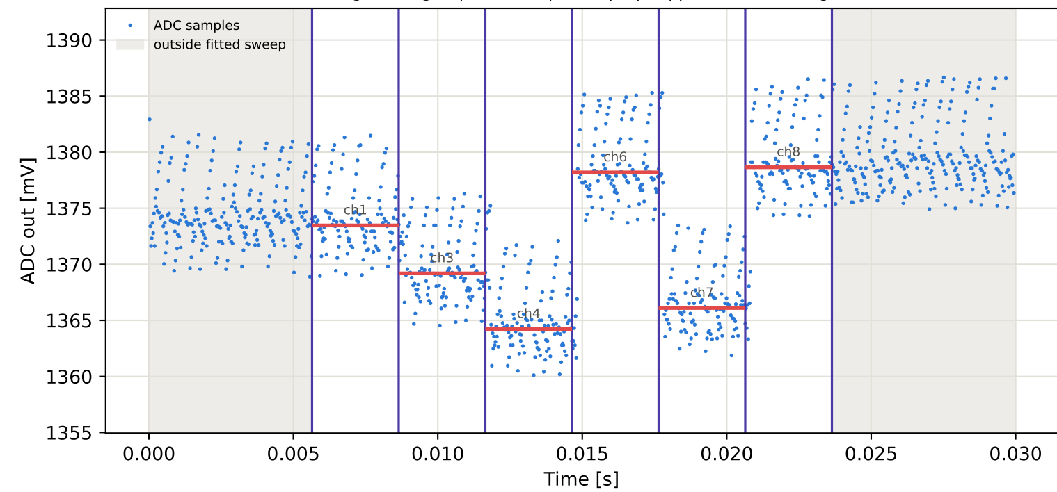
Tag4 &lt;- Tag16 | 935 MHz | run 0 | rep 1 | phase -11.41 deg
