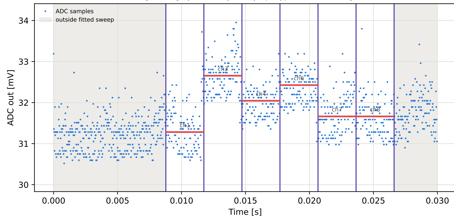
Tag3 &lt;- Tag10 | 775 MHz | run 0 | rep 1 | phase -82.59 deg
