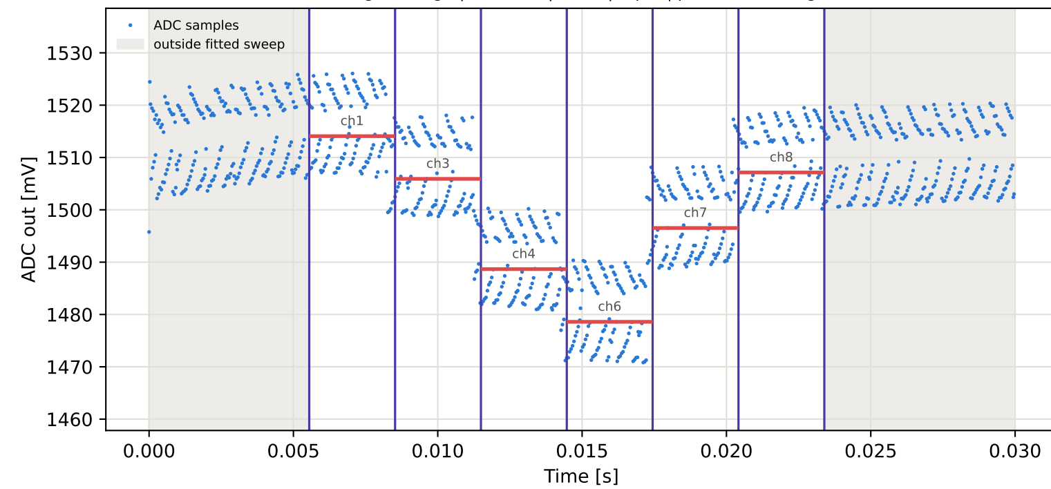
Tag9 &lt;- Tag10 | 925 MHz | run 0 | rep 1 | phase -170.82 deg
