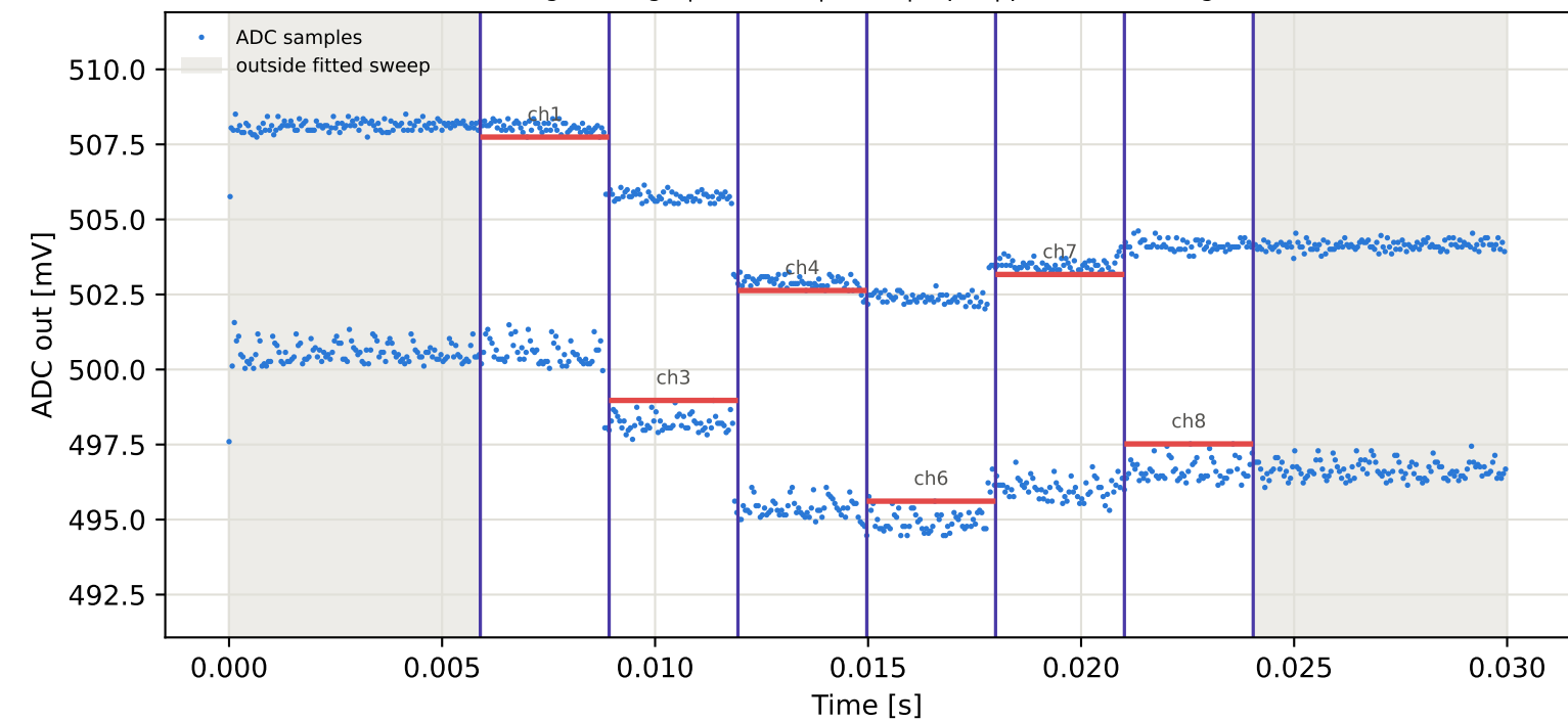
Tag4 &lt;- Tag15 | 865 MHz | run 0 | rep 1 | phase 16.12 deg
