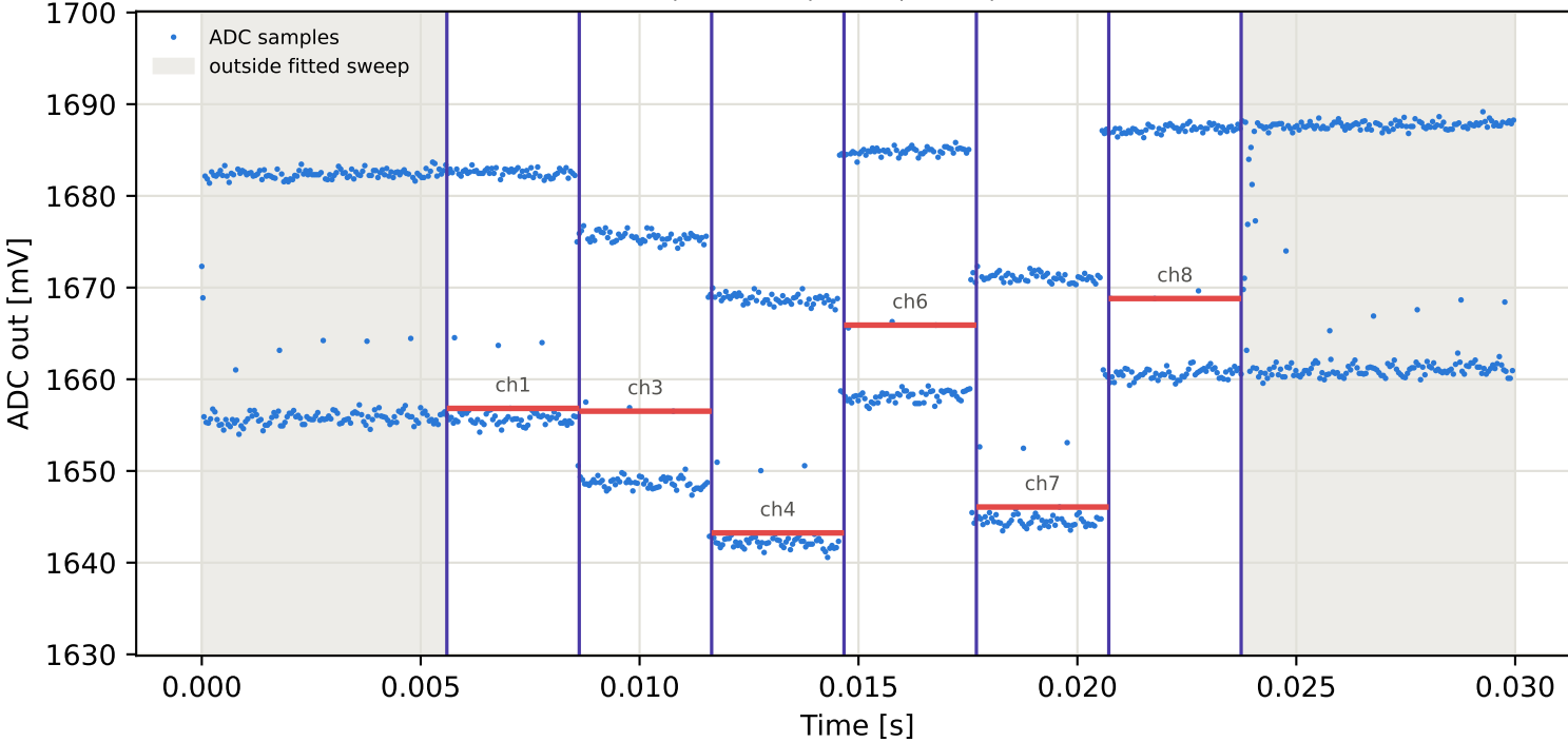
Tag15 &lt;- Tag1 | 945 MHz | run 0 | rep 1 | phase 119.65 deg
