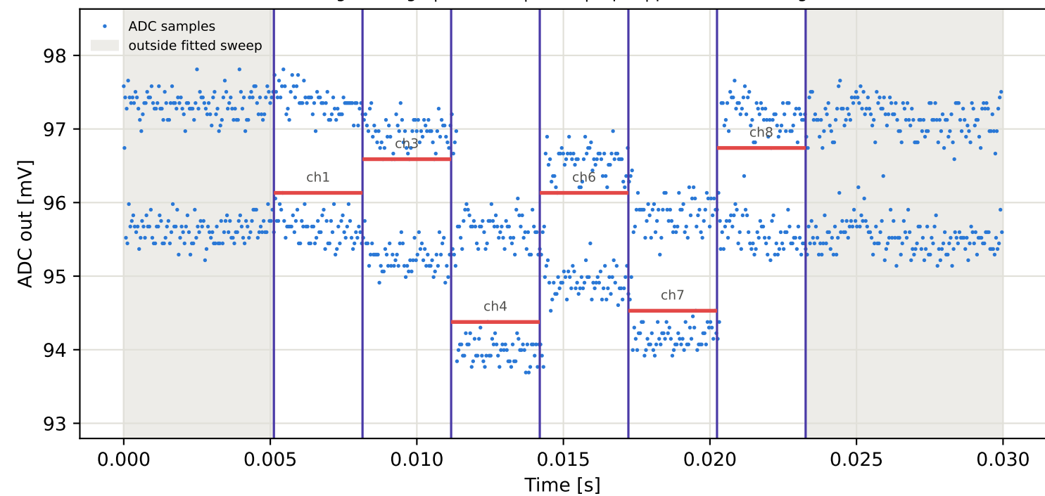
Tag7 &lt;- Tag6 | 795 MHz | run 0 | rep 1 | phase 101.17 deg
