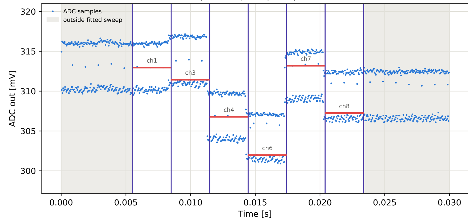
Tag3 &lt;- Tag7 | 995 MHz | run 0 | rep 1 | phase -100.69 deg
