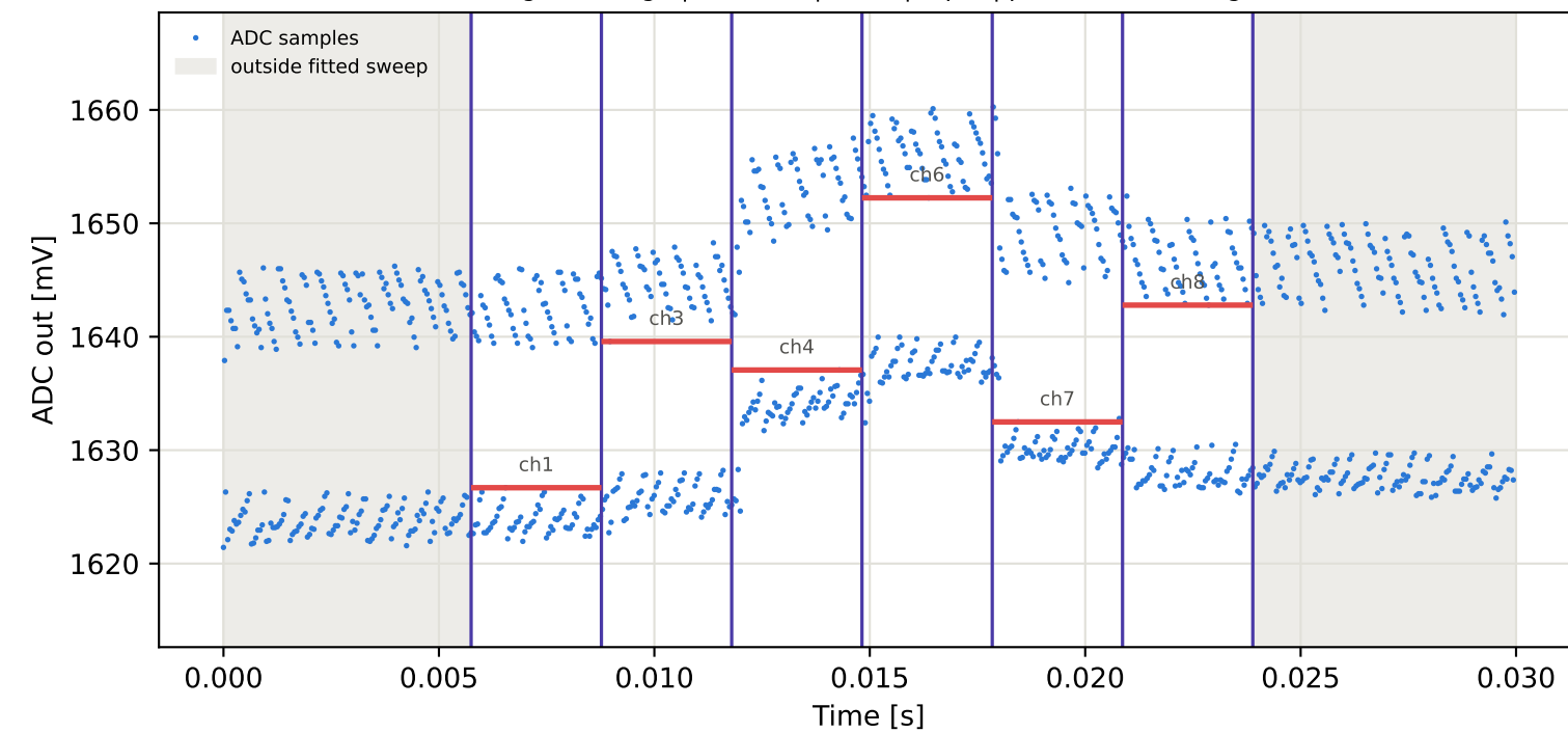
Tag15 &lt;- Tag9 | 935 MHz | run 0 | rep 1 | phase 73.73 deg
