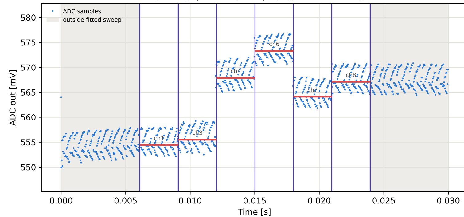
Tag6 &lt;- Tag9 | 865 MHz | run 0 | rep 1 | phase -150.52 deg
