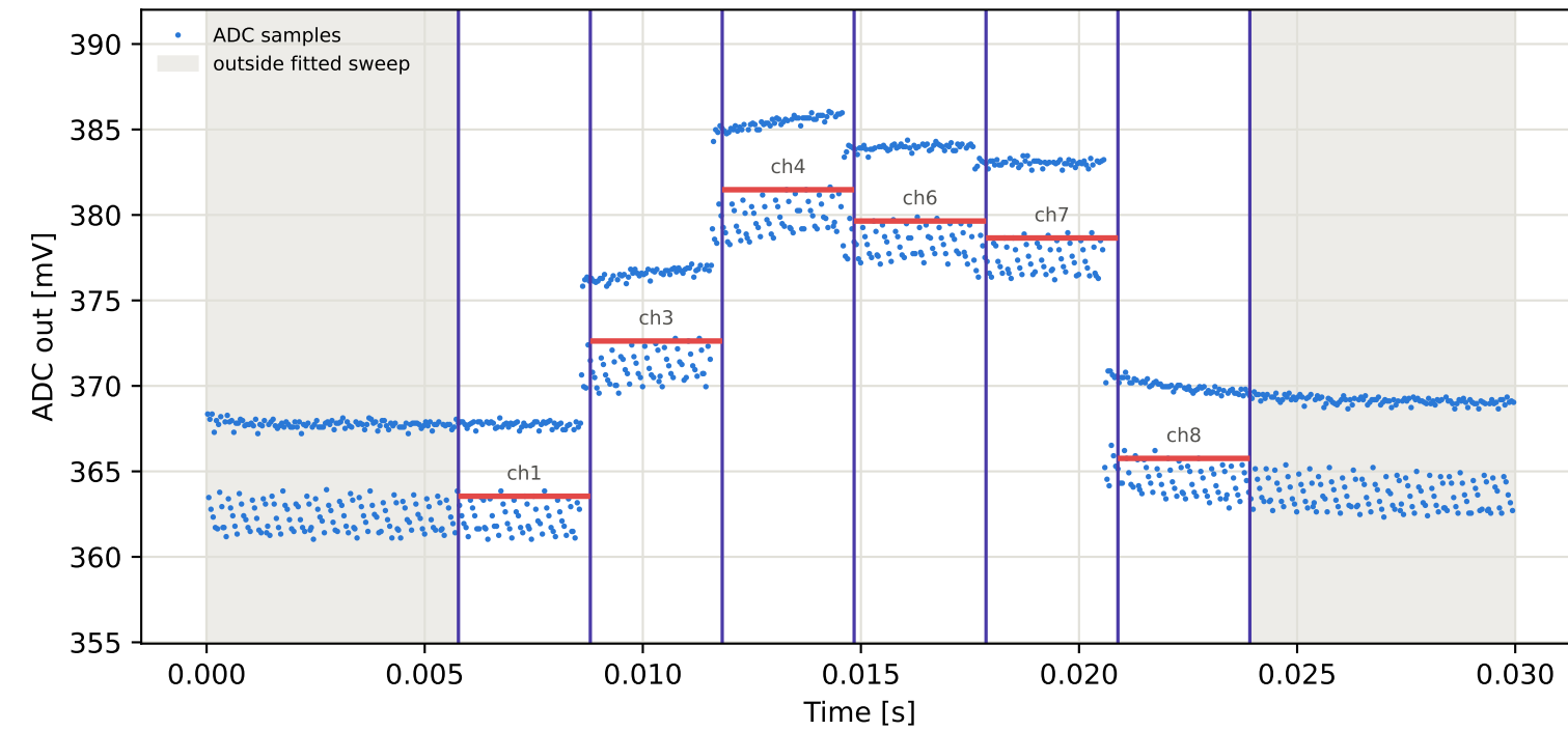
Tag1 &lt;- Tag9 | 895 MHz | run 0 | rep 1 | phase -150.23 deg
