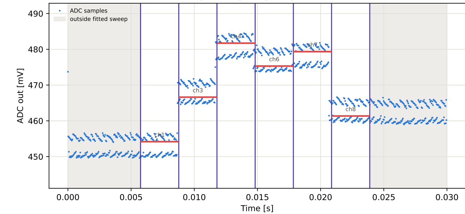
Tag5 &lt;- Tag3 | 855 MHz | run 0 | rep 1 | phase -104.43 deg
