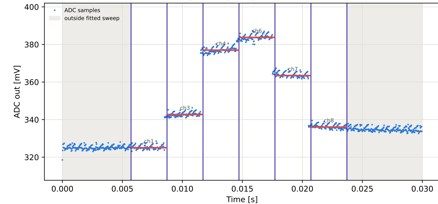
Tag9 &lt;- Tag16 | 915 MHz | run 0 | rep 1 | phase -125.19 deg
