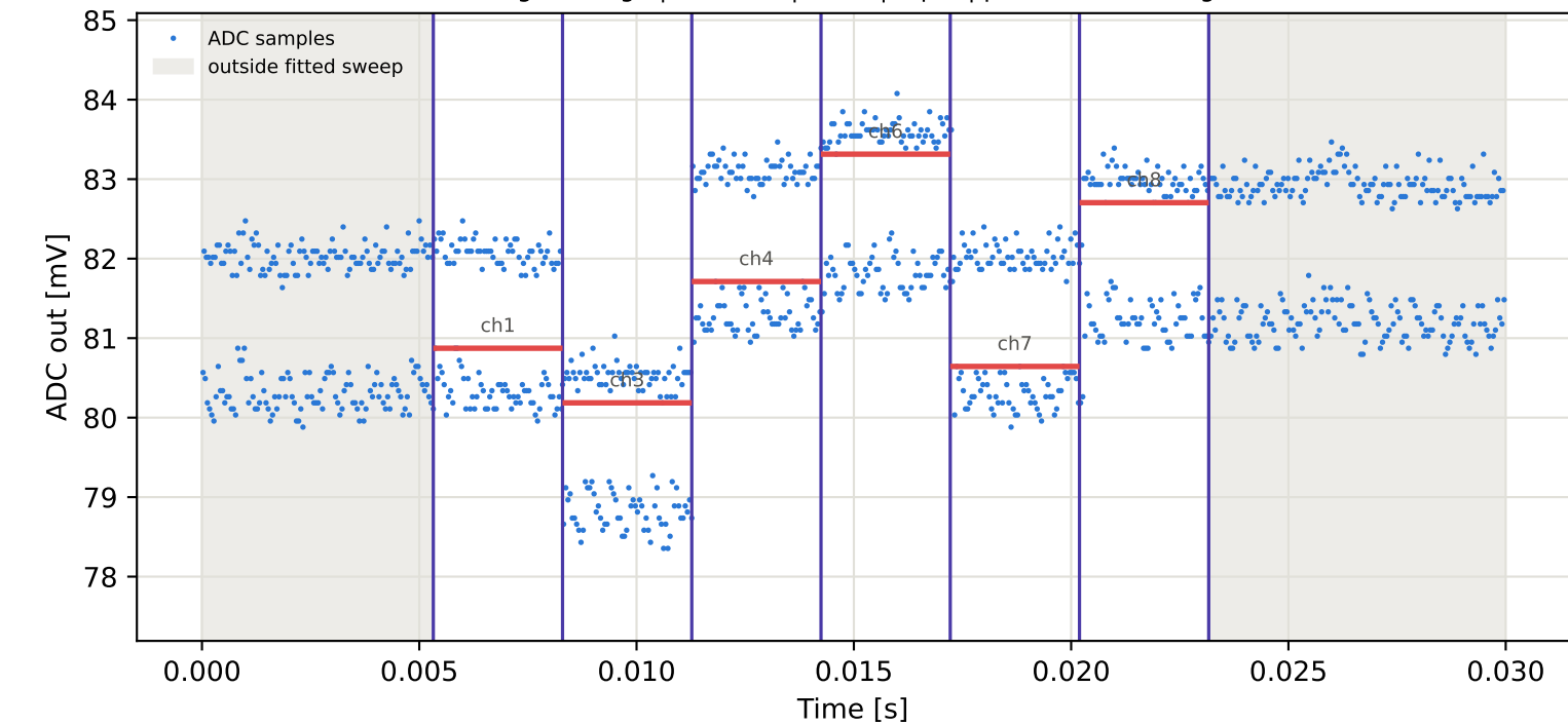
Tag9 &lt;- Tag8 | 785 MHz | run 0 | rep 1 | phase -156.32 deg
