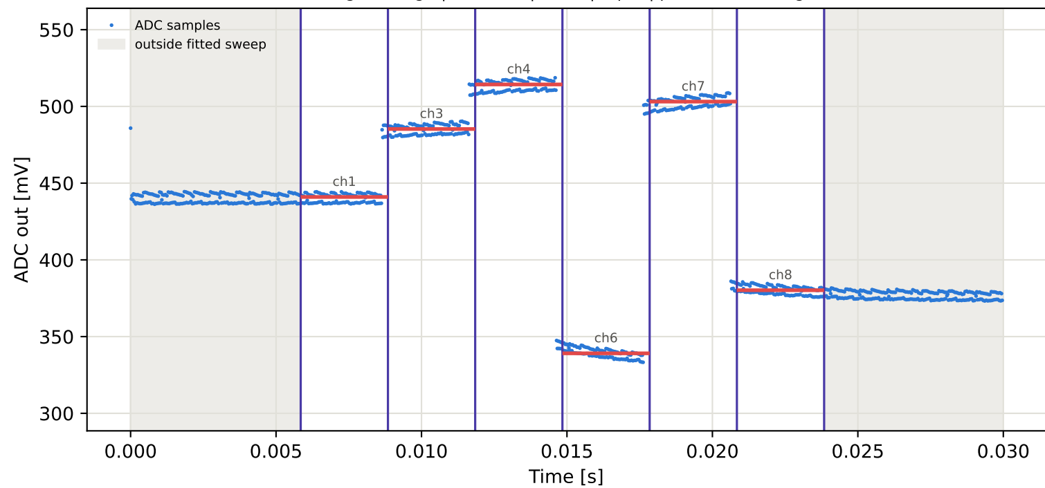
Tag9 &lt;- Tag6 | 945 MHz | run 0 | rep 1 | phase -47.72 deg
