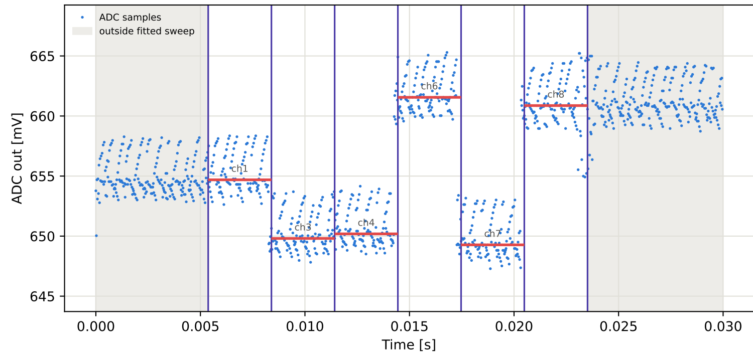
Tag8 &lt;- Tag4 | 825 MHz | run 0 | rep 1 | phase -85.64 deg
