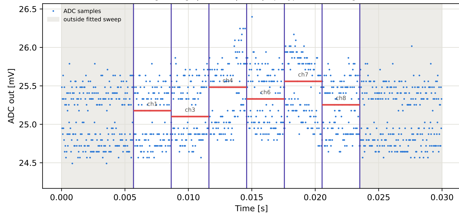
Tag7 &lt;- Tag4 | 775 MHz | run 0 | rep 1 | phase -88.18 deg
