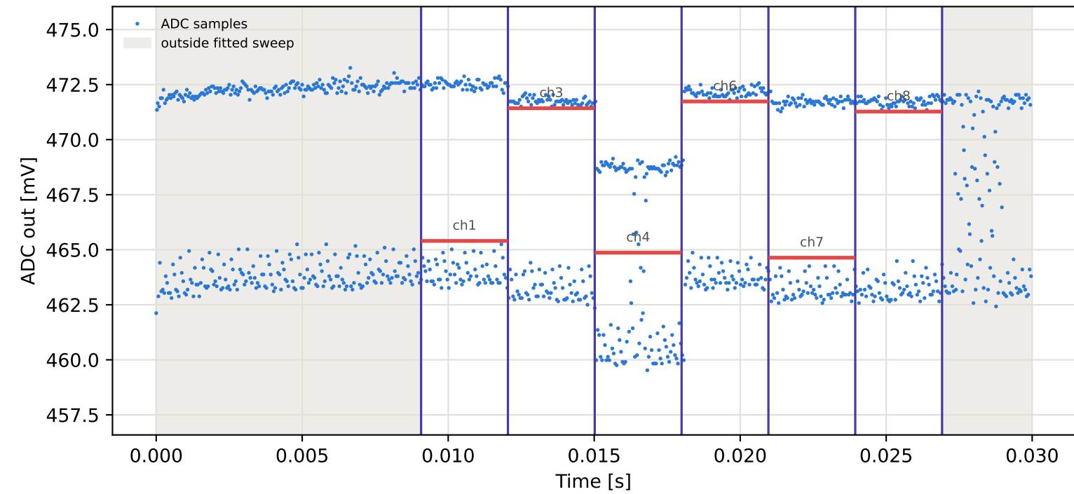
Tag1 &lt;- Tag4 | 955 MHz | run 0 | rep 1 | phase -10.80 deg
