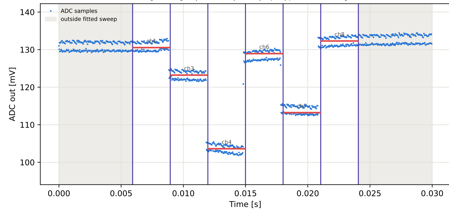
Tag5 &lt;- Tag3 | 995 MHz | run 0 | rep 1 | phase 170.92 deg
