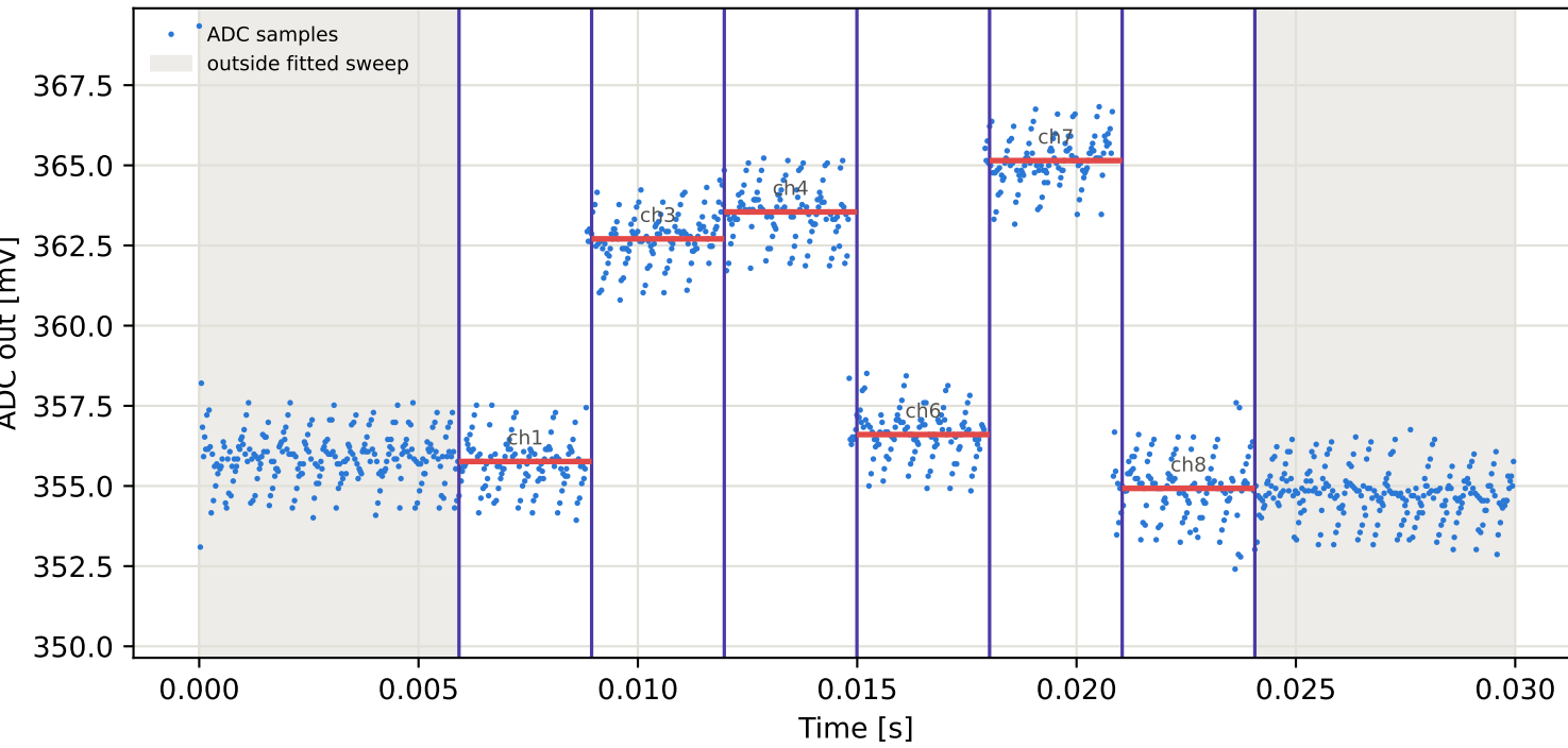
Tag15 &lt;- Tag5 | 825 MHz | run 0 | rep 1 | phase -48.48 deg
