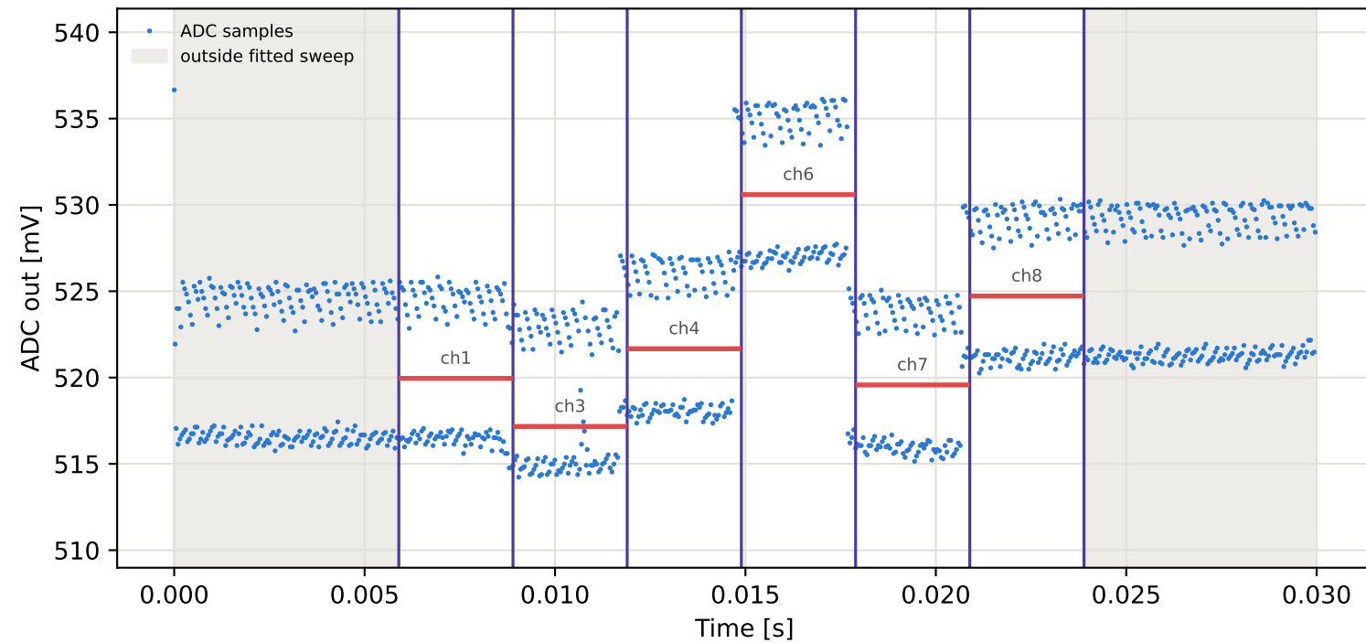
Tag3 &lt;- Tag16 | 965 MHz | run 0 | rep 1 | phase 31.67 deg
