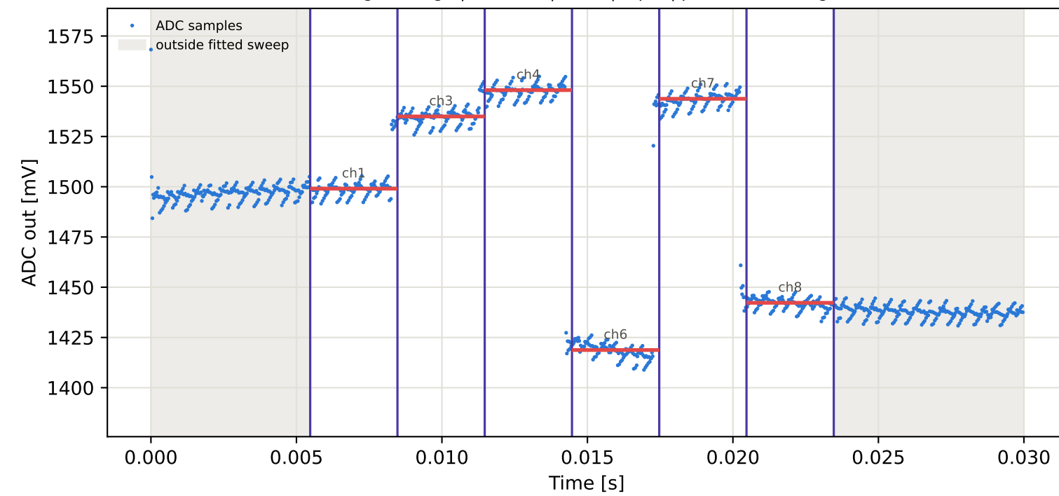
Tag4 &lt;- Tag7 | 925 MHz | run 0 | rep 1 | phase -85.36 deg
