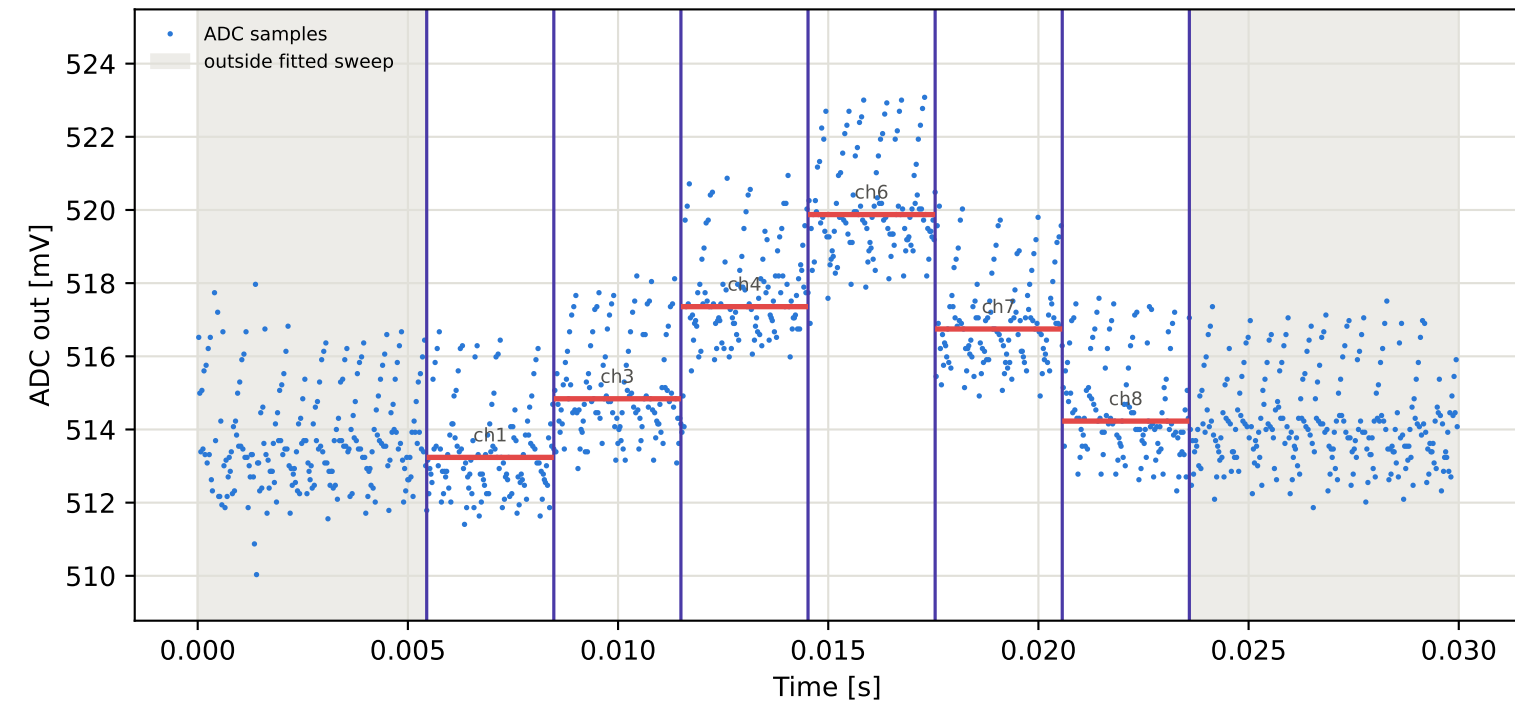
Tag10 &lt;- Tag5 | 915 MHz | run 0 | rep 1 | phase -145.64 deg
