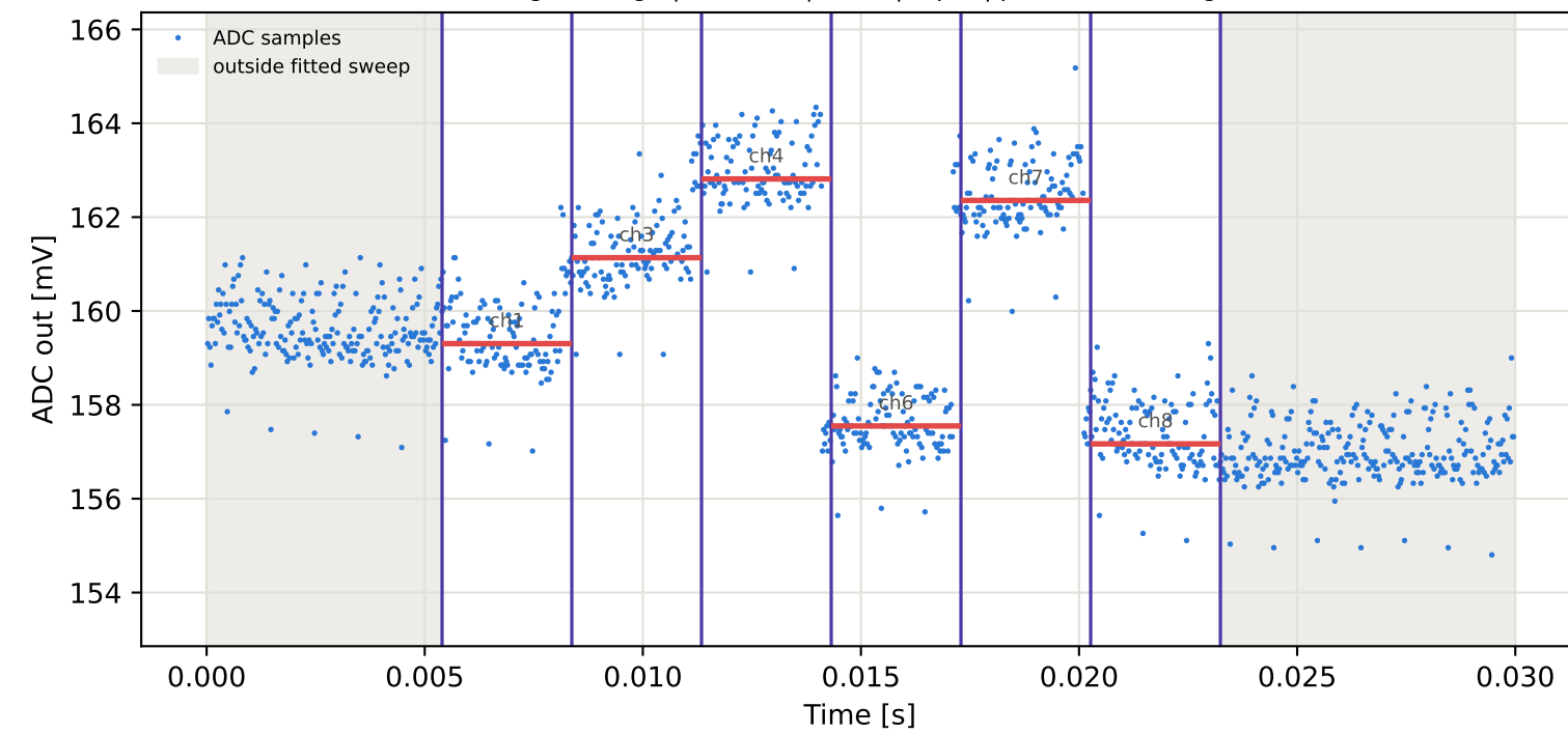
Tag3 &lt;- Tag10 | 935 MHz | run 0 | rep 1 | phase 97.15 deg
