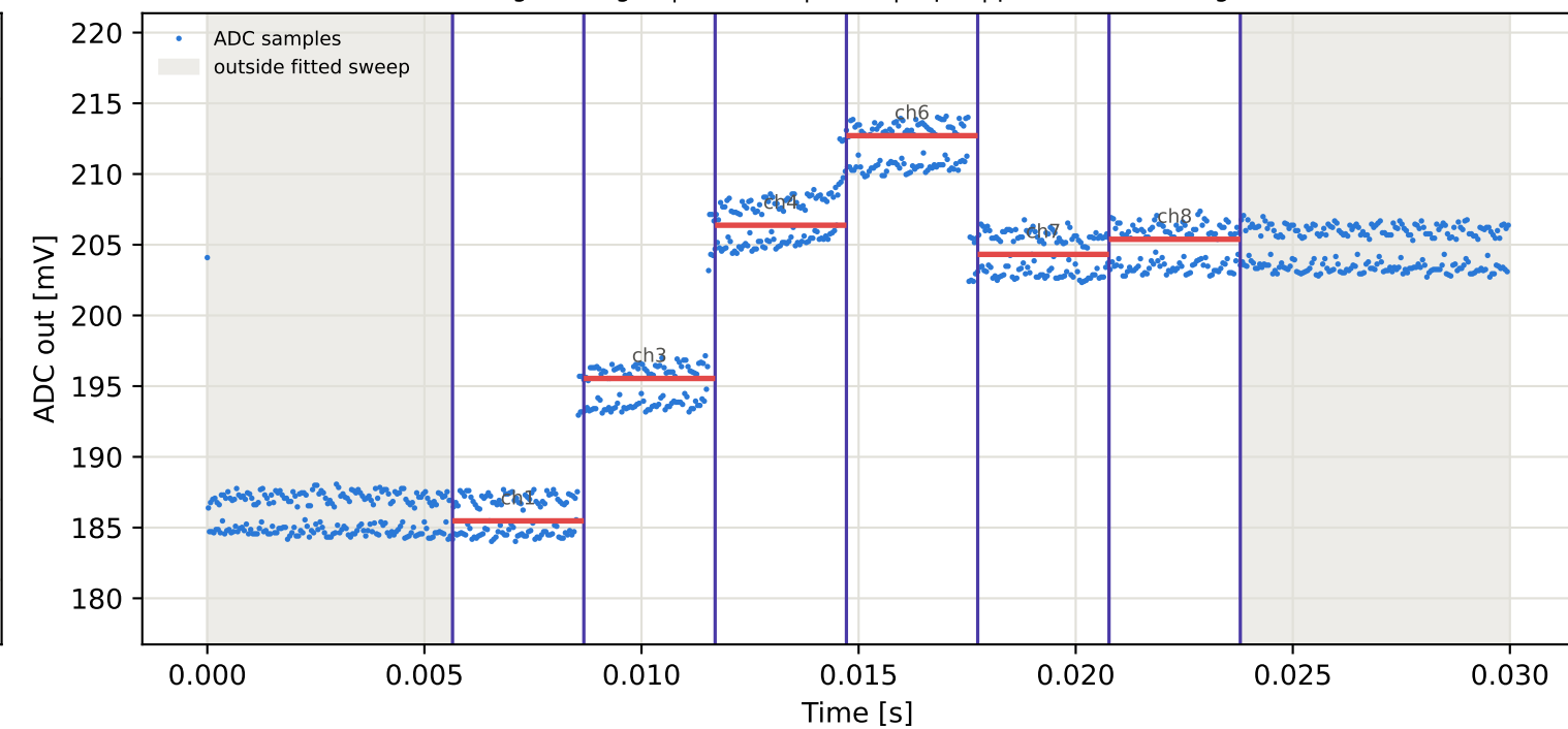
Tag2 &lt;- Tag16 | 855 MHz | run 0 | rep 1 | phase -131.27 deg
