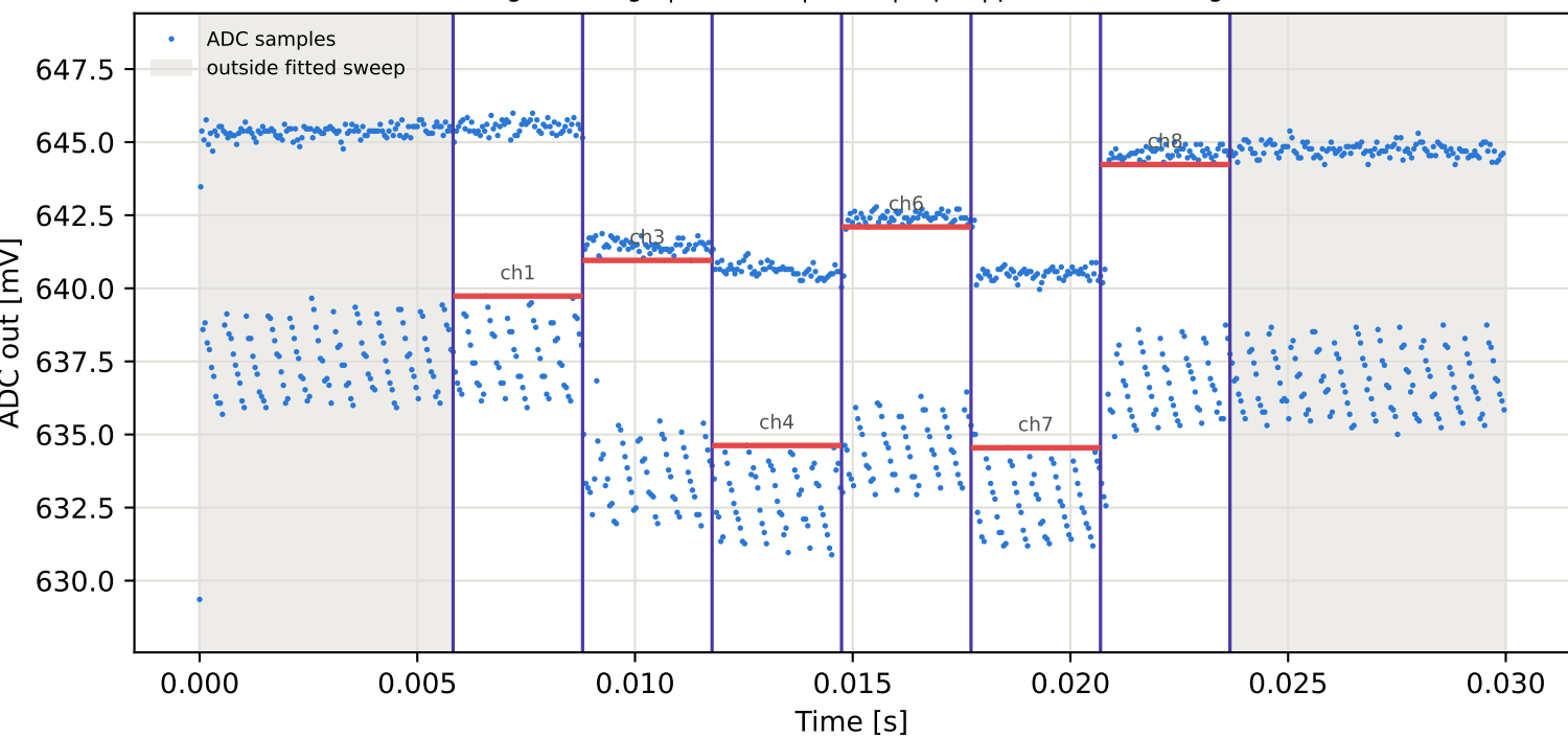
Tag15 &lt;- Tag1 | 865 MHz | run 0 | rep 1 | phase 114.86 deg
