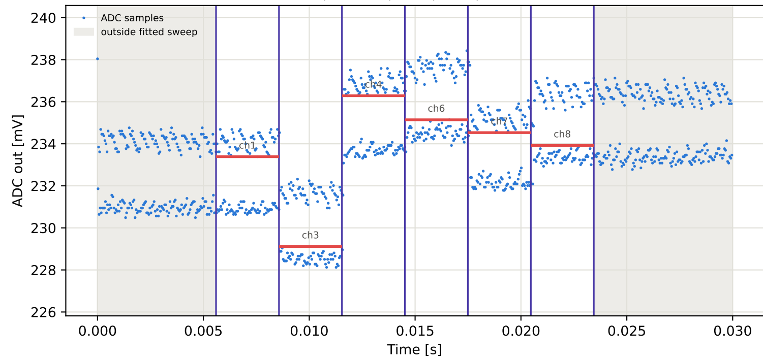
Tag7 &lt;- Tag15 | 825 MHz | run 0 | rep 1 | phase -125.16 deg
