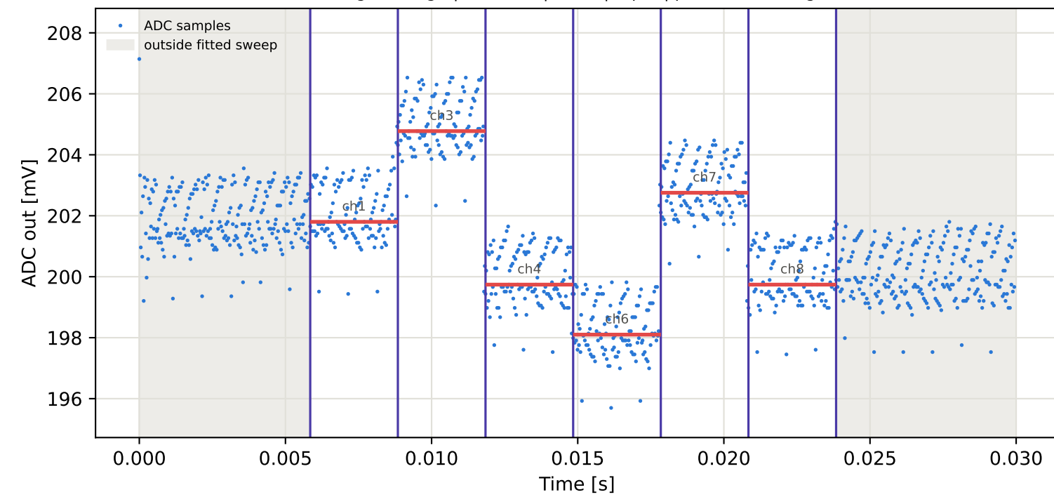
Tag4 &lt;- Tag7 | 775 MHz | run 0 | rep 1 | phase 115.36 deg
