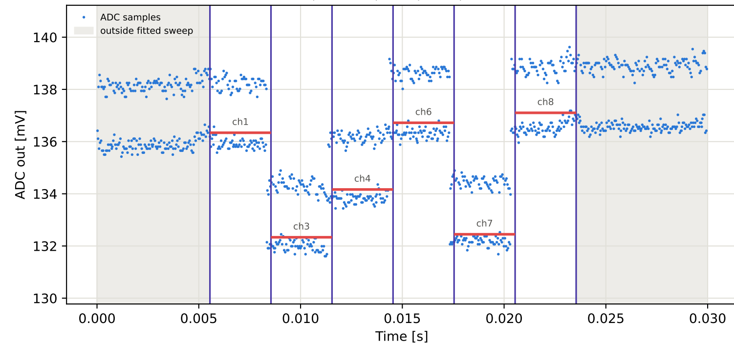
Tag6 &lt;- Tag4 | 805 MHz | run 0 | rep 1 | phase 163.12 deg
