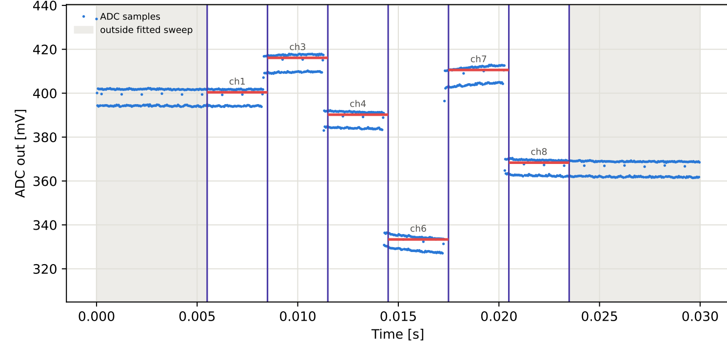
Tag4 &lt;- Tag3 | 975 MHz | run 0 | rep 1 | phase -95.45 deg
