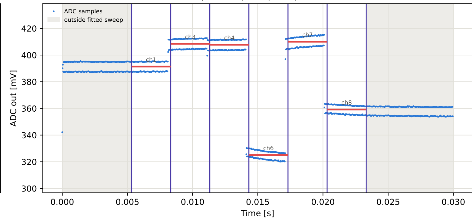
Tag3 &lt;- Tag7 | 945 MHz | run 0 | rep 1 | phase -173.79 deg
