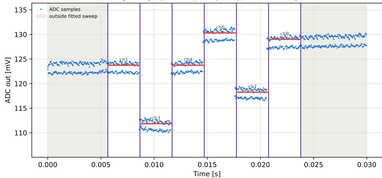
Tag4 &lt;- Tag3 | 805 MHz | run 0 | rep 1 | phase -84.48 deg
