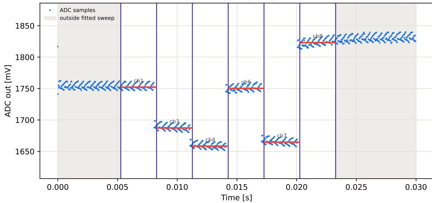
Tag8 &lt;- Tag16 | 885 MHz | run 0 | rep 1 | phase 121.01 deg
