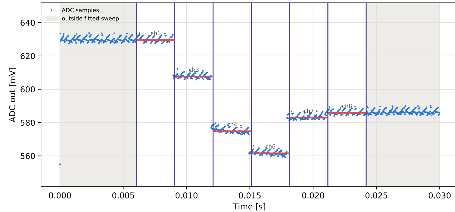
Tag6 &lt;- Tag1 | 865 MHz | run 0 | rep 1 | phase 71.93 deg
