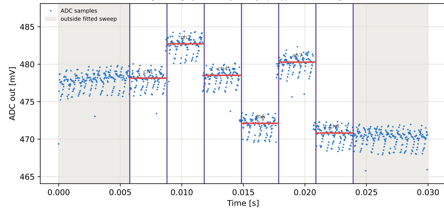
Tag5 &lt;- Tag8 | 855 MHz | run 0 | rep 1 | phase -0.67 deg
