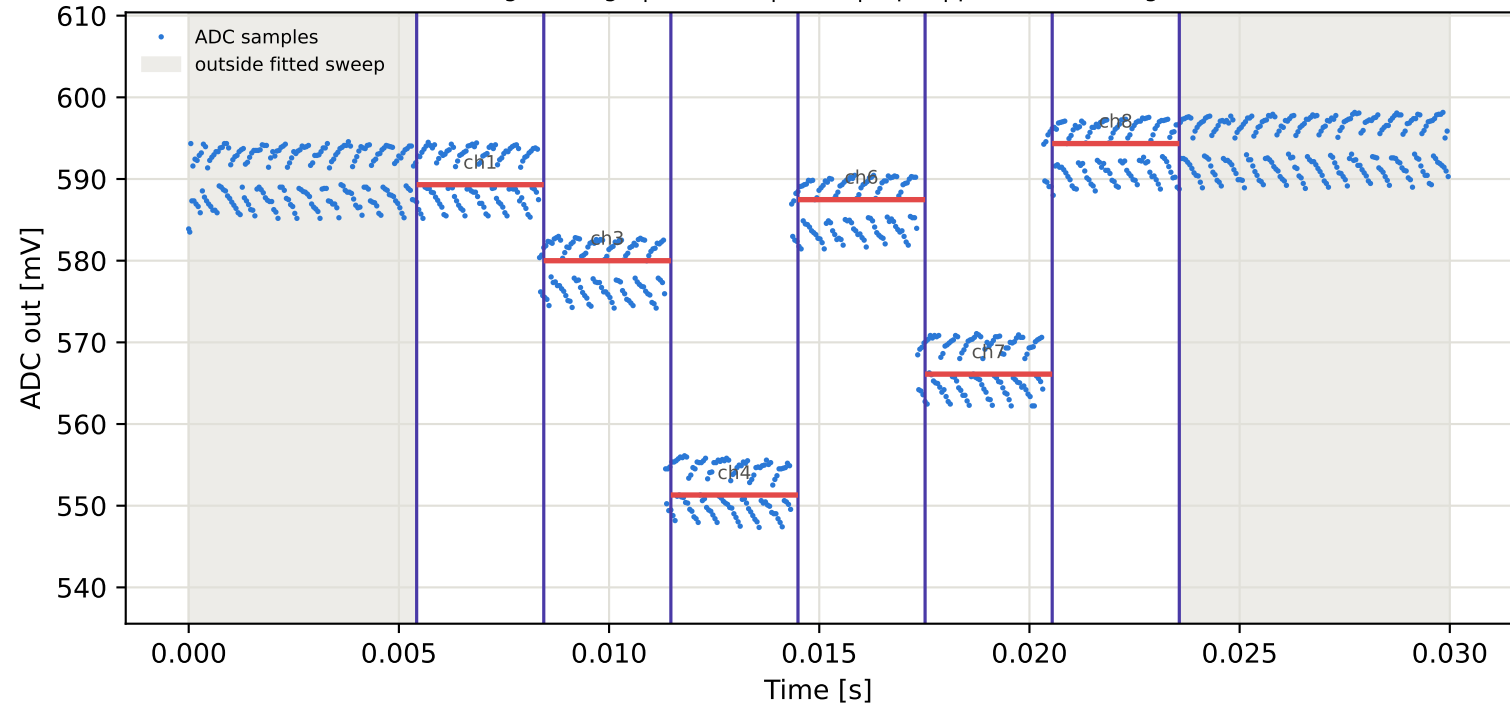
Tag6 &lt;- Tag5 | 975 MHz | run 0 | rep 1 | phase 2.91 deg
