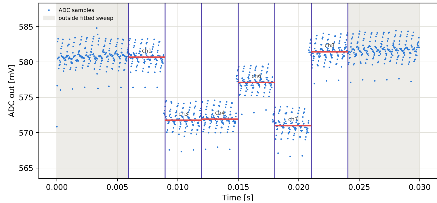
Tag5 &lt;- Tag1 | 865 MHz | run 0 | rep 1 | phase 118.96 deg
