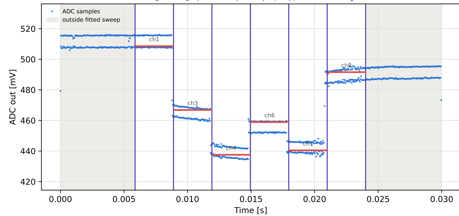
Tag4 &lt;- Tag9 | 875 MHz | run 0 | rep 1 | phase 83.33 deg
