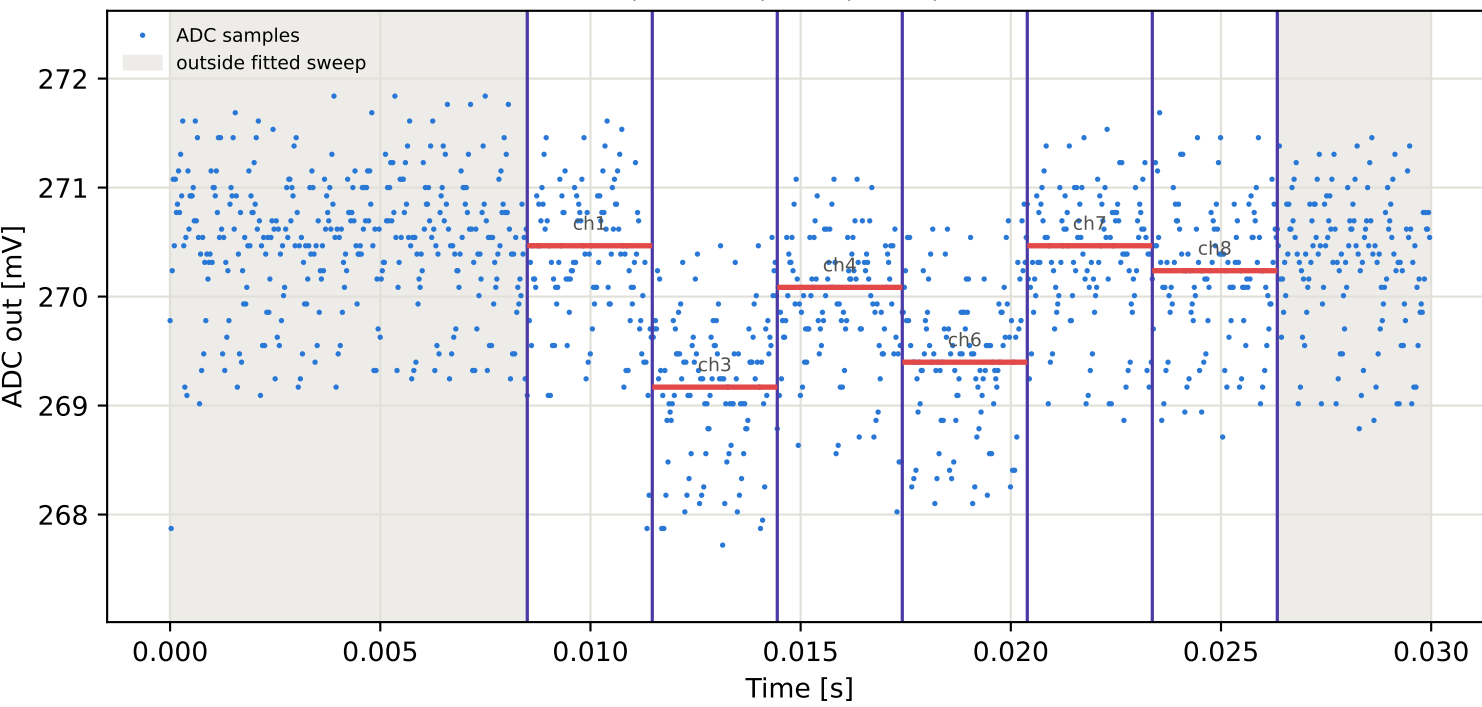
Tag15 &lt;- Tag1 | 795 MHz | run 0 | rep 1 | phase 10.19 deg
