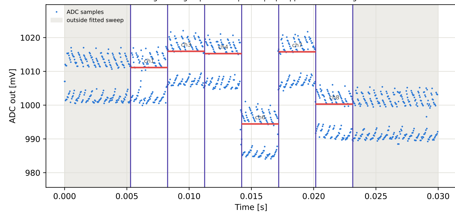
Tag5 &lt;- Tag3 | 905 MHz | run 0 | rep 1 | phase 1.35 deg
