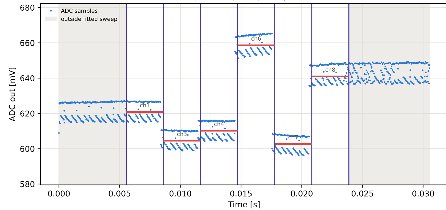
Tag15 &lt;- Tag3 | 985 MHz | run 0 | rep 1 | phase 86.57 deg
