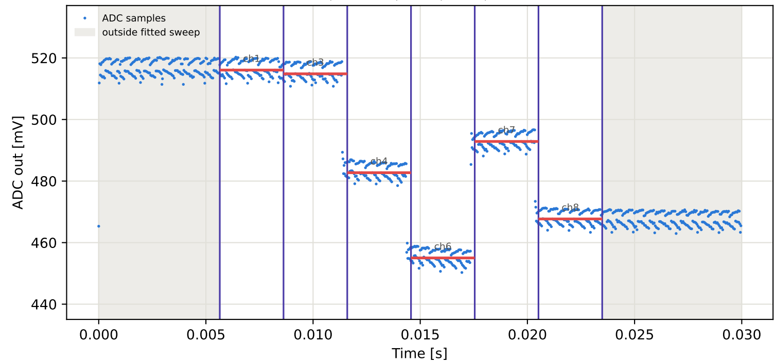
Tag5 &lt;- Tag4 | 855 MHz | run 0 | rep 1 | phase 31.49 deg
