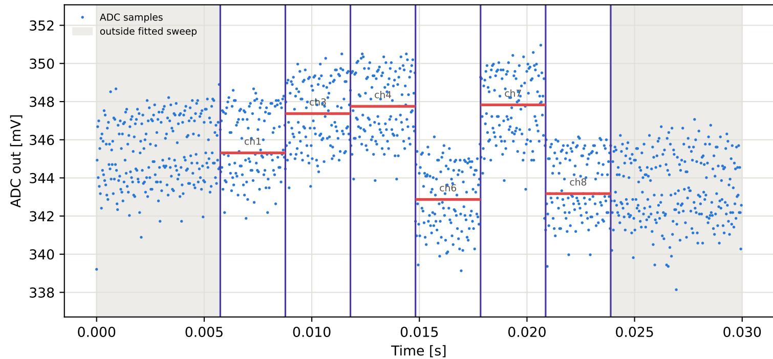
Tag1 &lt;- Tag4 | 885 MHz | run 0 | rep 1 | phase -124.67 deg
