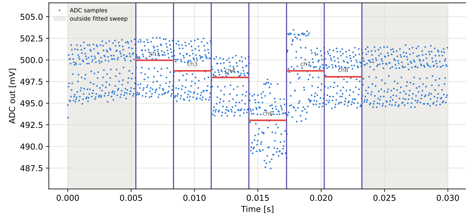
Tag1 &lt;- Tag4 | 965 MHz | run 0 | rep 1 | phase 9.67 deg
