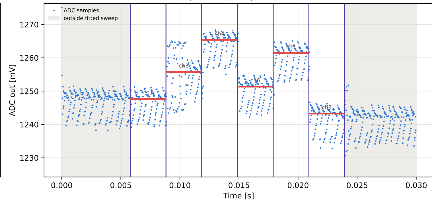
Tag16 &lt;- Tag5 | 925 MHz | run 0 | rep 1 | phase 139.74 deg
