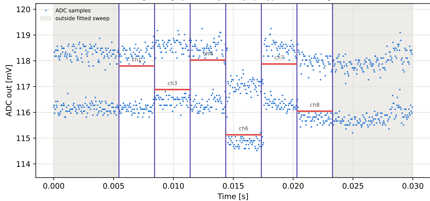
Tag5 &lt;- Tag4 | 995 MHz | run 0 | rep 1 | phase -159.84 deg
