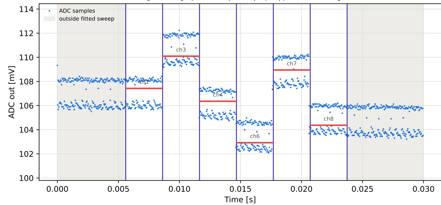
Tag10 &lt;- Tag5 | 785 MHz | run 0 | rep 1 | phase 19.20 deg
