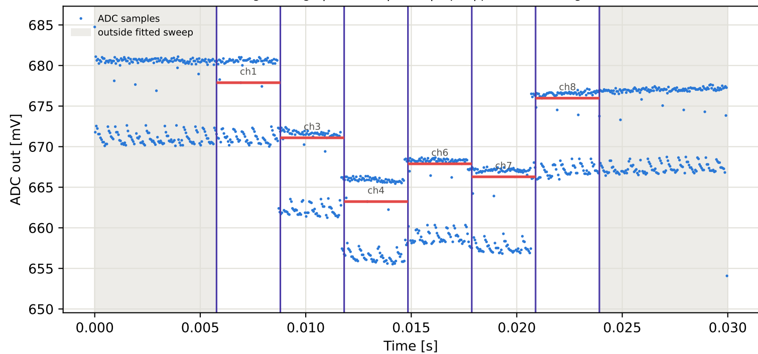
Tag7 &lt;- Tag6 | 865 MHz | run 0 | rep 1 | phase -163.88 deg
