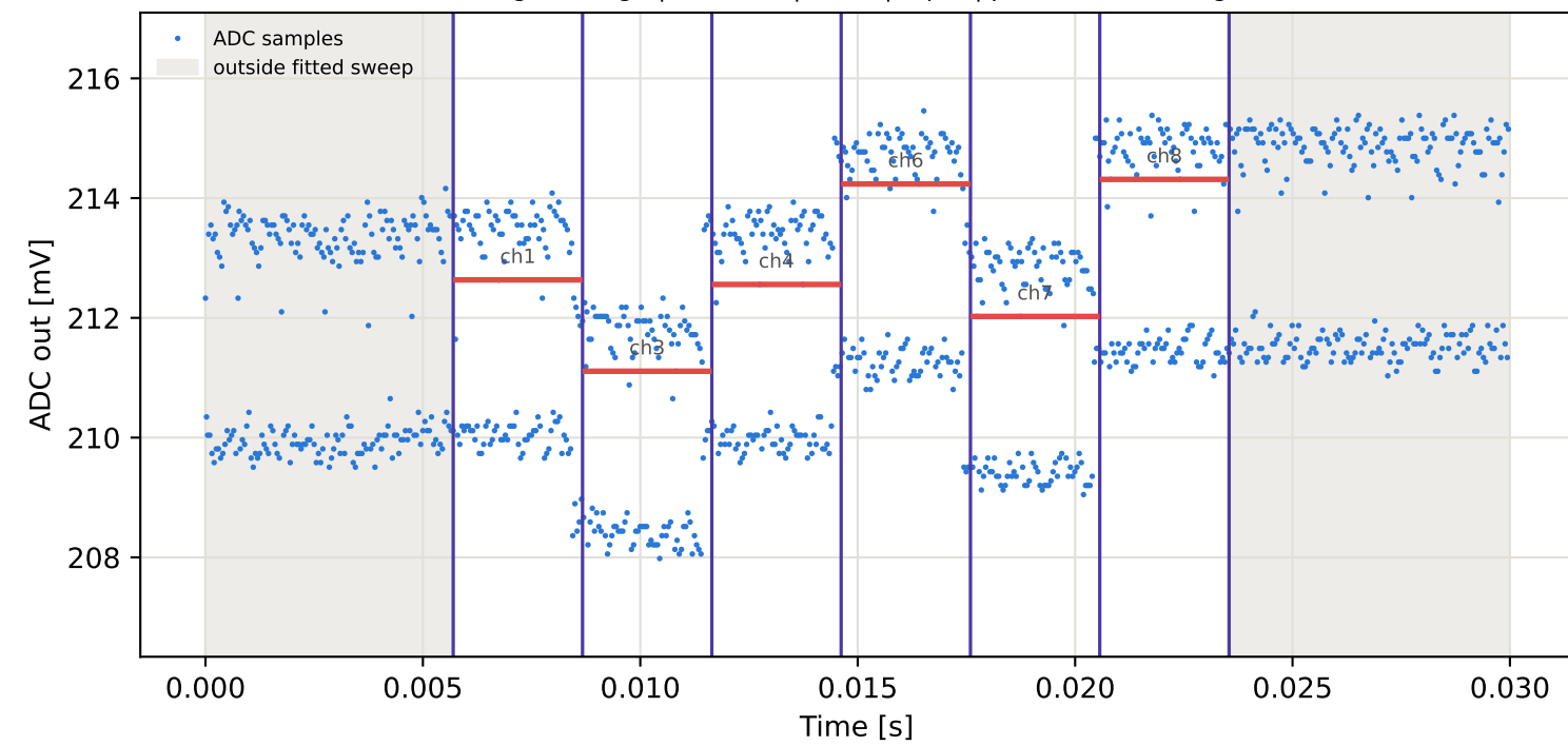
Tag9 &lt;- Tag15 | 855 MHz | run 0 | rep 1 | phase -139.58 deg
