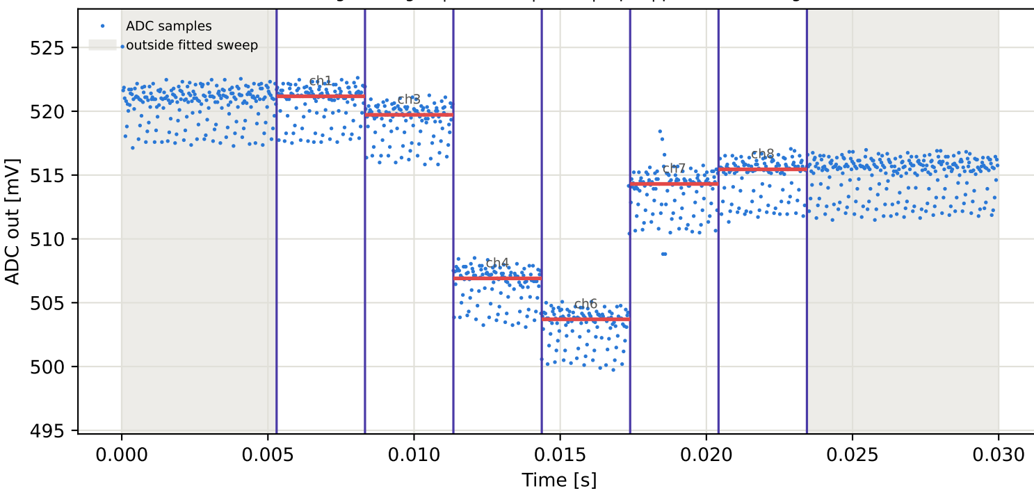
Tag3 &lt;- Tag16 | 955 MHz | run 0 | rep 1 | phase 39.68 deg
