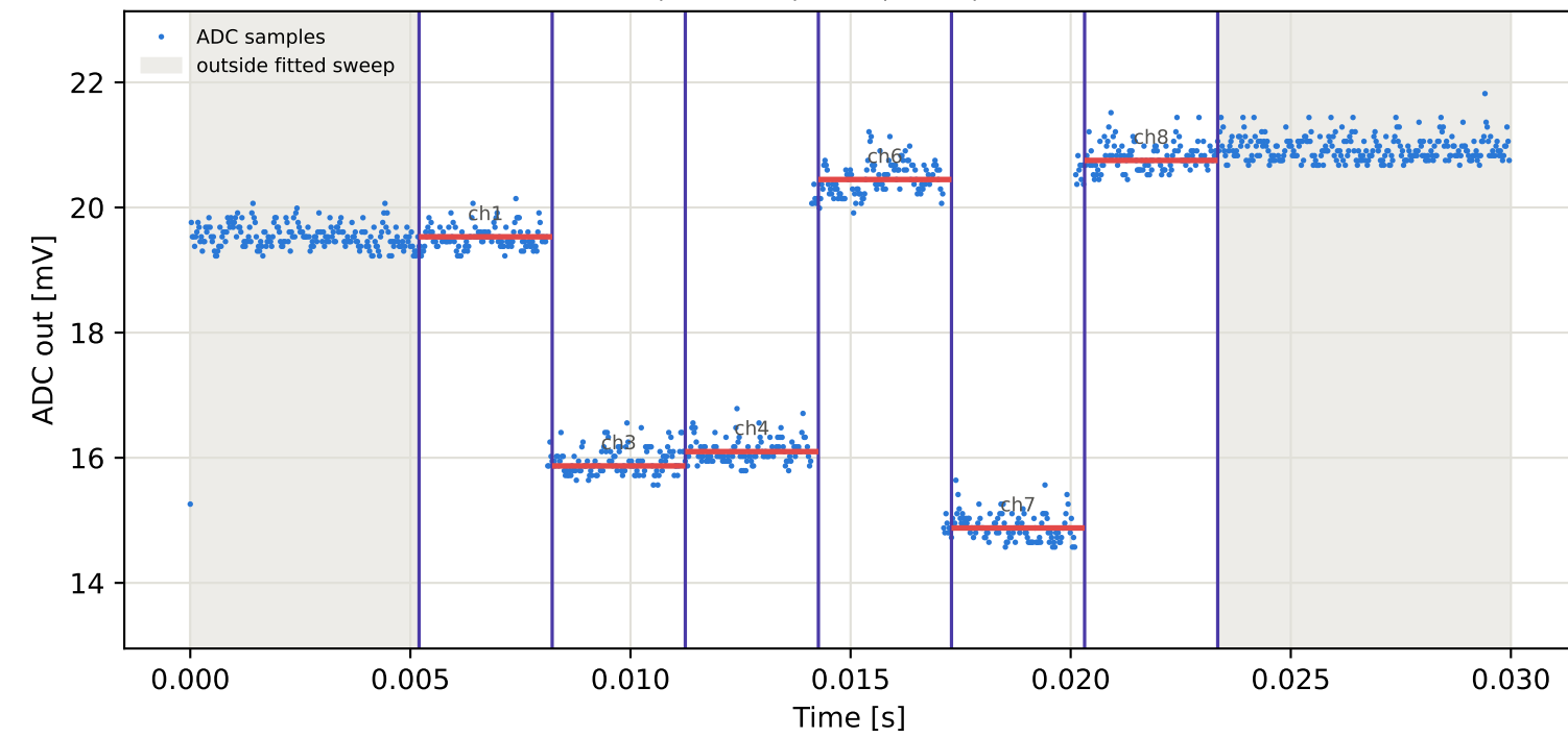
Tag9 &lt;- Tag7 | 795 MHz | run 0 | rep 1 | phase 150.42 deg
