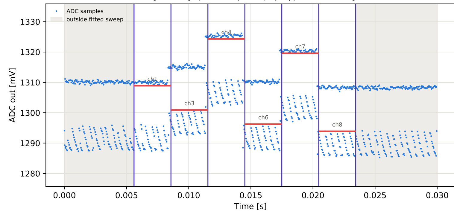
Tag16 &lt;- Tag6 | 985 MHz | run 0 | rep 1 | phase -75.71 deg
