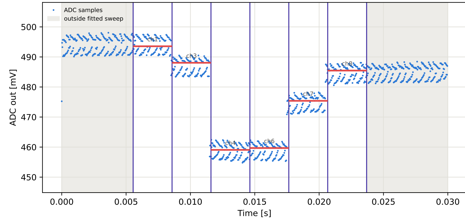
Tag7 &lt;- Tag15 | 975 MHz | run 0 | rep 1 | phase 47.37 deg
