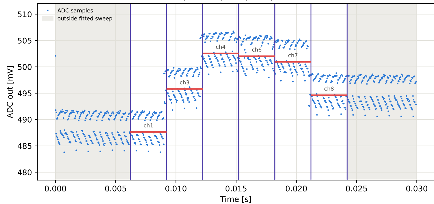
Tag4 &lt;- Tag16 | 865 MHz | run 0 | rep 1 | phase -68.68 deg
