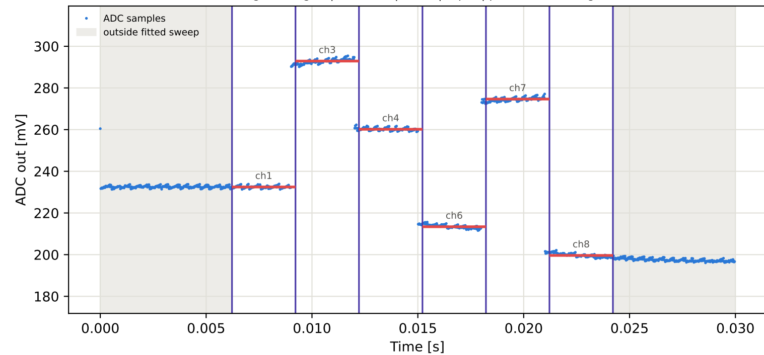
Tag7 &lt;- Tag3 | 835 MHz | run 0 | rep 1 | phase 75.95 deg
