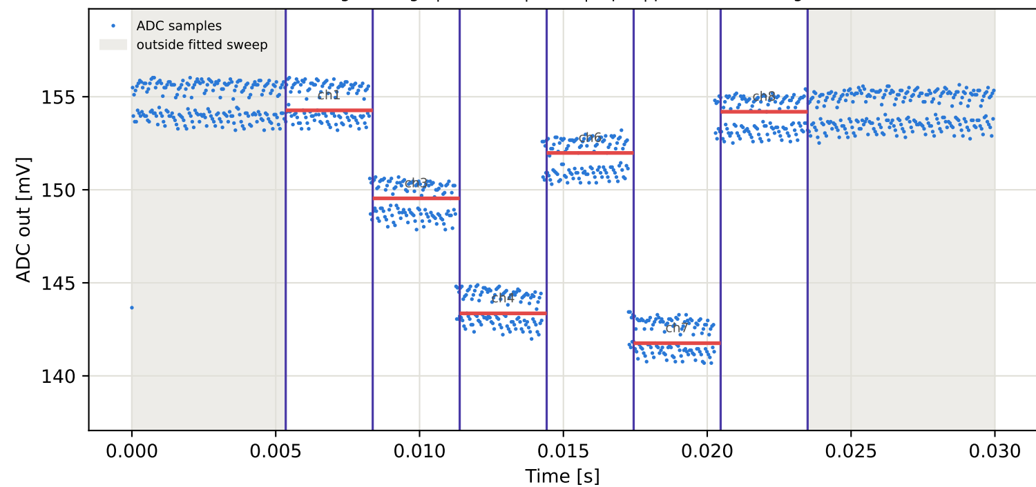
Tag3 &lt;- Tag8 | 785 MHz | run 0 | rep 1 | phase 114.96 deg
