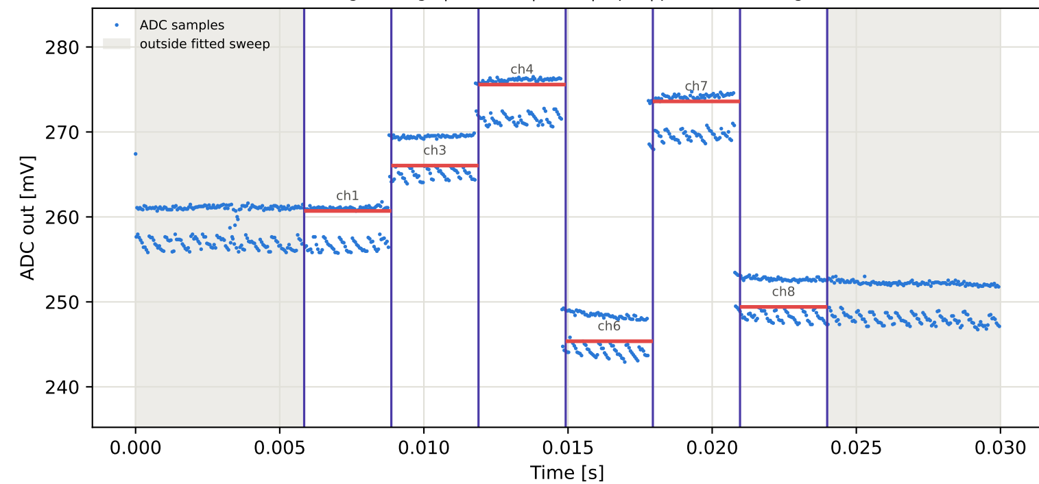
Tag9 &lt;- Tag15 | 995 MHz | run 0 | rep 1 | phase 86.54 deg
