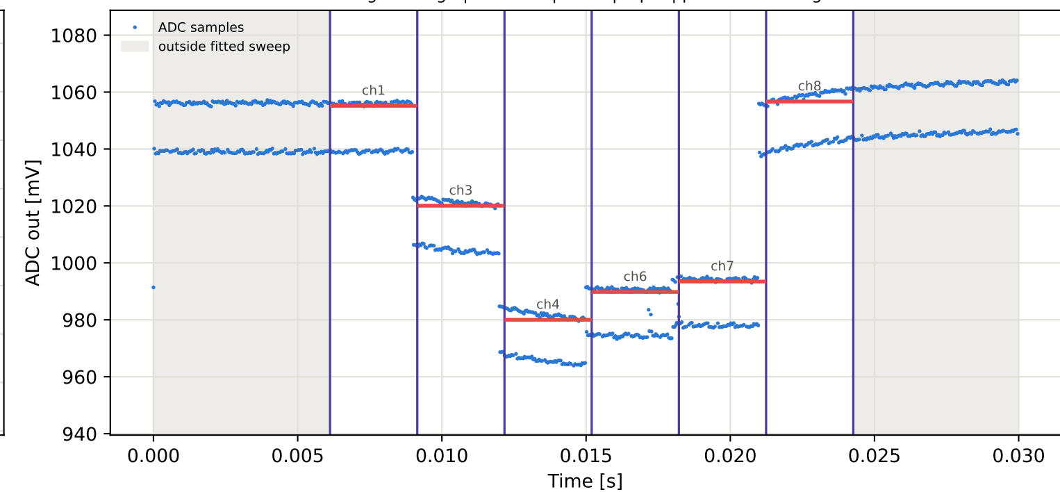
Tag5 &lt;- Tag4 | 905 MHz | run 0 | rep 1 | phase 70.06 deg
