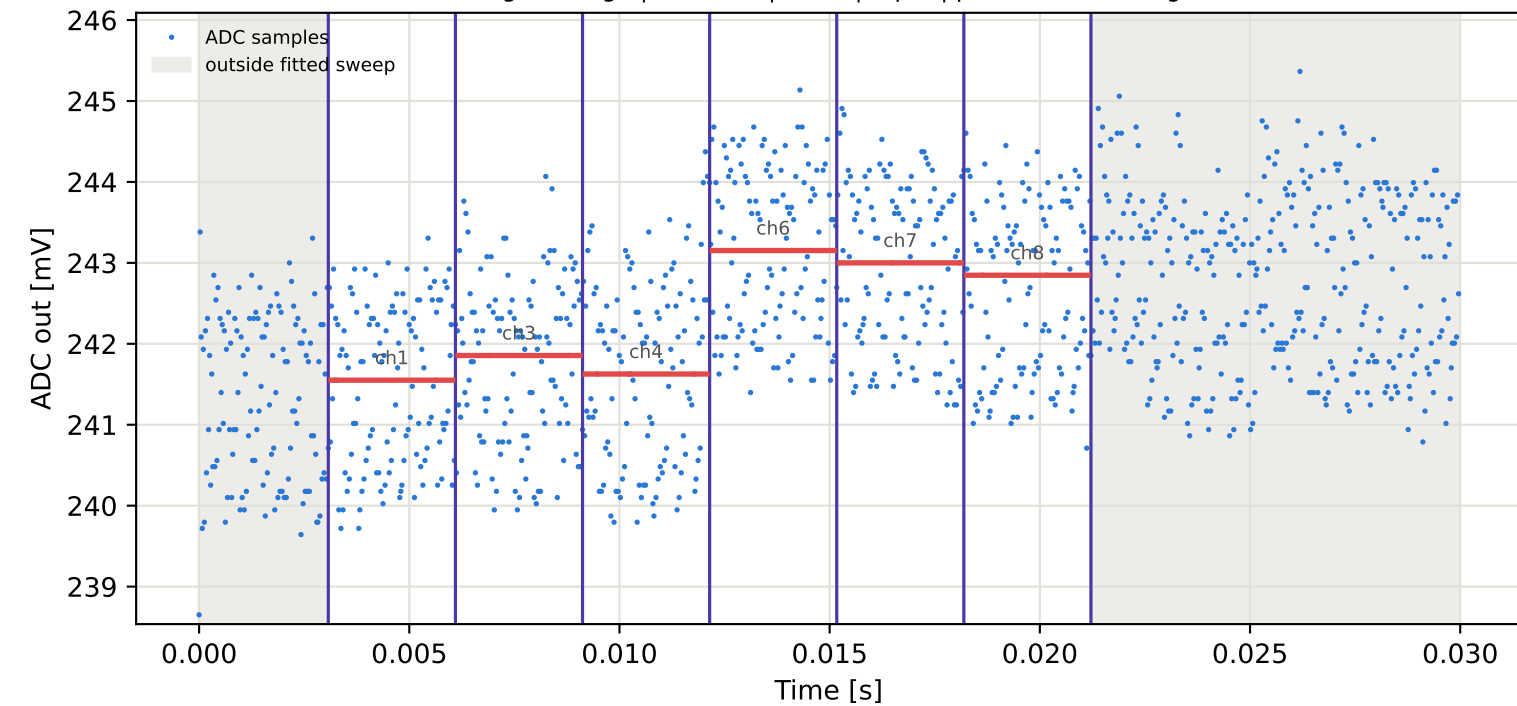
Tag2 &lt;- Tag7 | 835 MHz | run 0 | rep 1 | phase -159.26 deg
