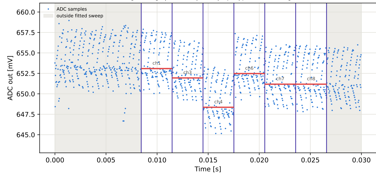
Tag7 &lt;- Tag5 | 915 MHz | run 0 | rep 1 | phase 126.62 deg
