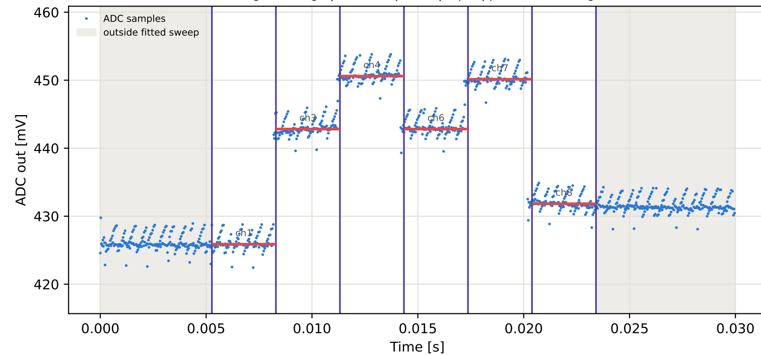
Tag15 &lt;- Tag5 | 845 MHz | run 0 | rep 1 | phase 67.51 deg
