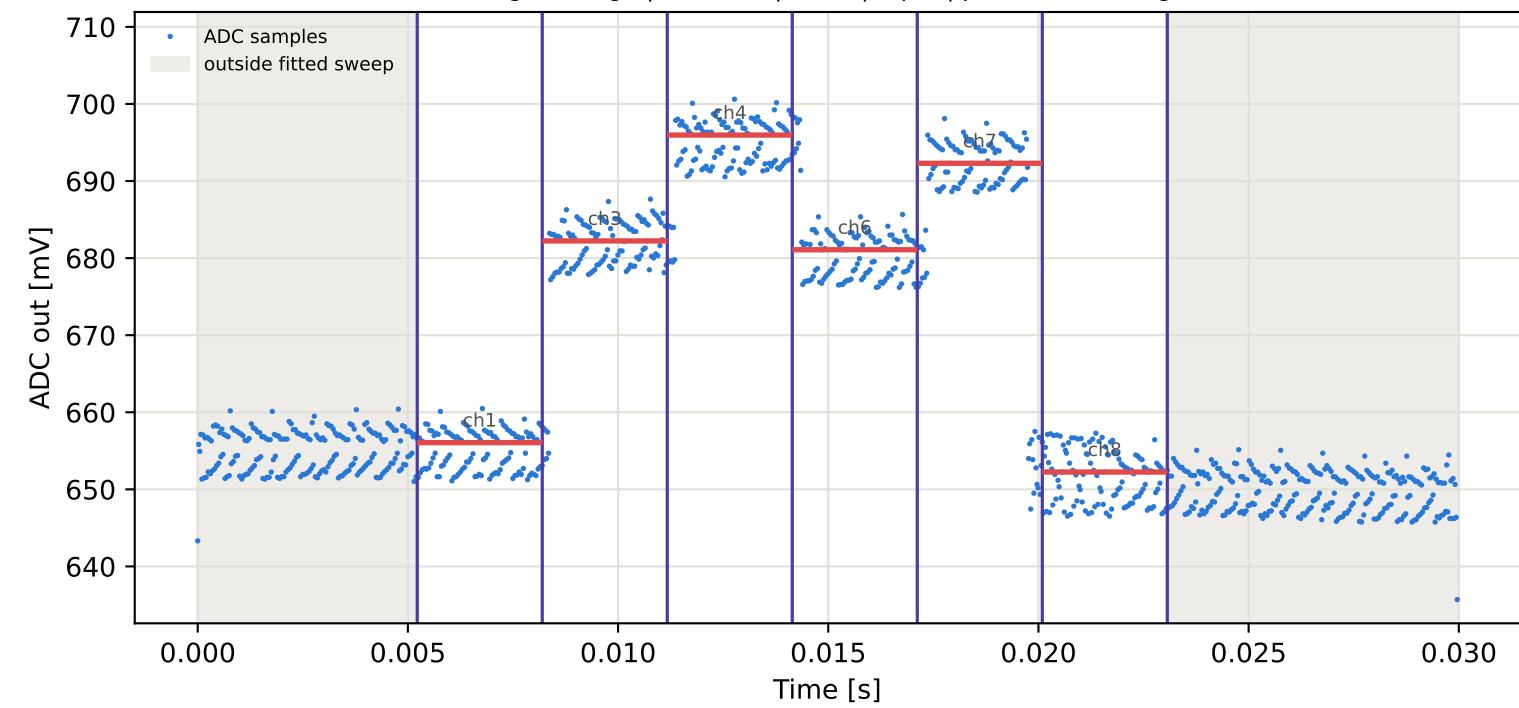
Tag9 &lt;- Tag6 | 875 MHz | run 0 | rep 1 | phase -88.77 deg
