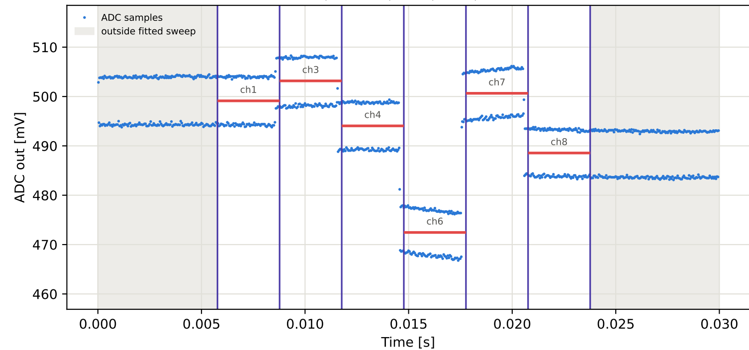
Tag1 &lt;- Tag4 | 965 MHz | run 0 | rep 1 | phase 9.67 deg
