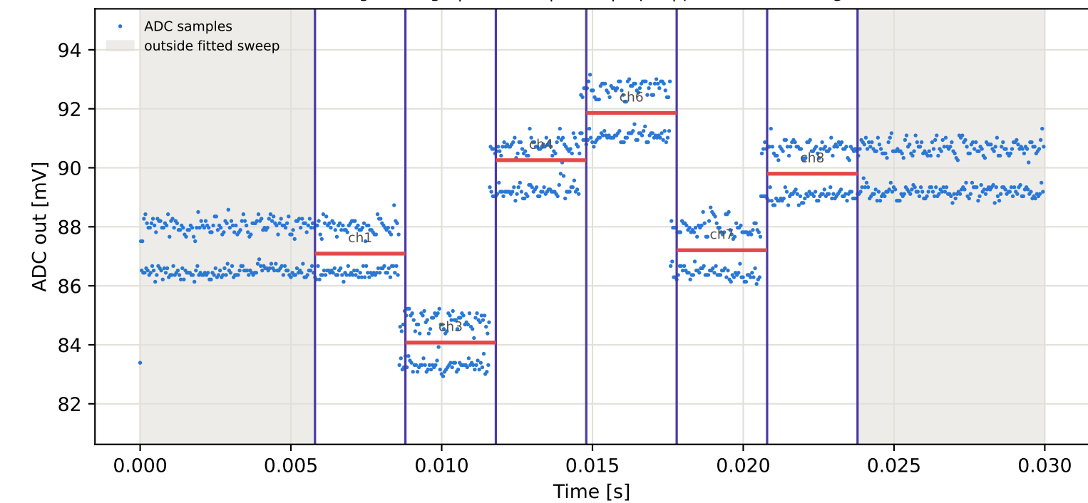
Tag9 &lt;- Tag8 | 775 MHz | run 0 | rep 1 | phase -103.22 deg
