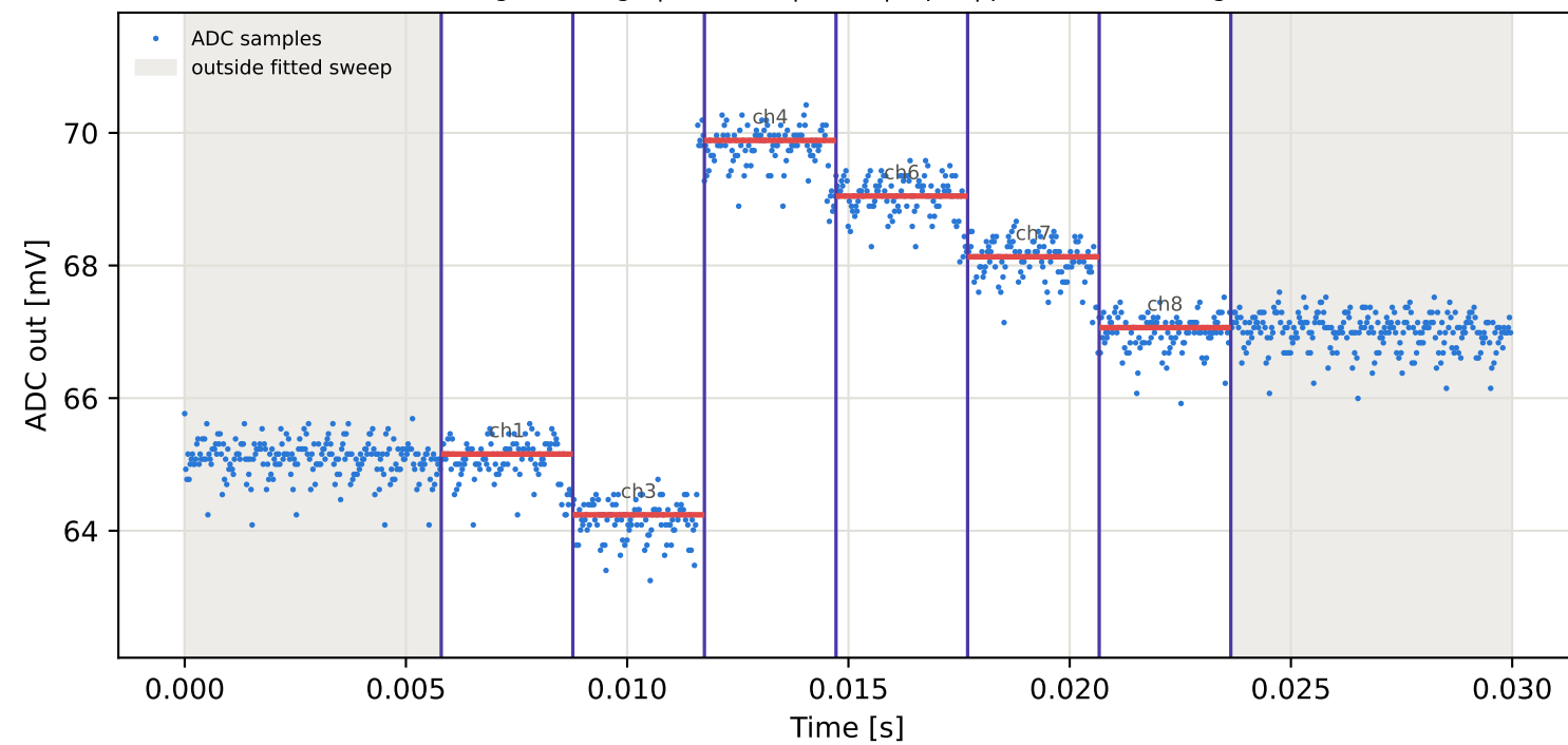
Tag10 &lt;- Tag8 | 775 MHz | run 0 | rep 1 | phase -119.00 deg
