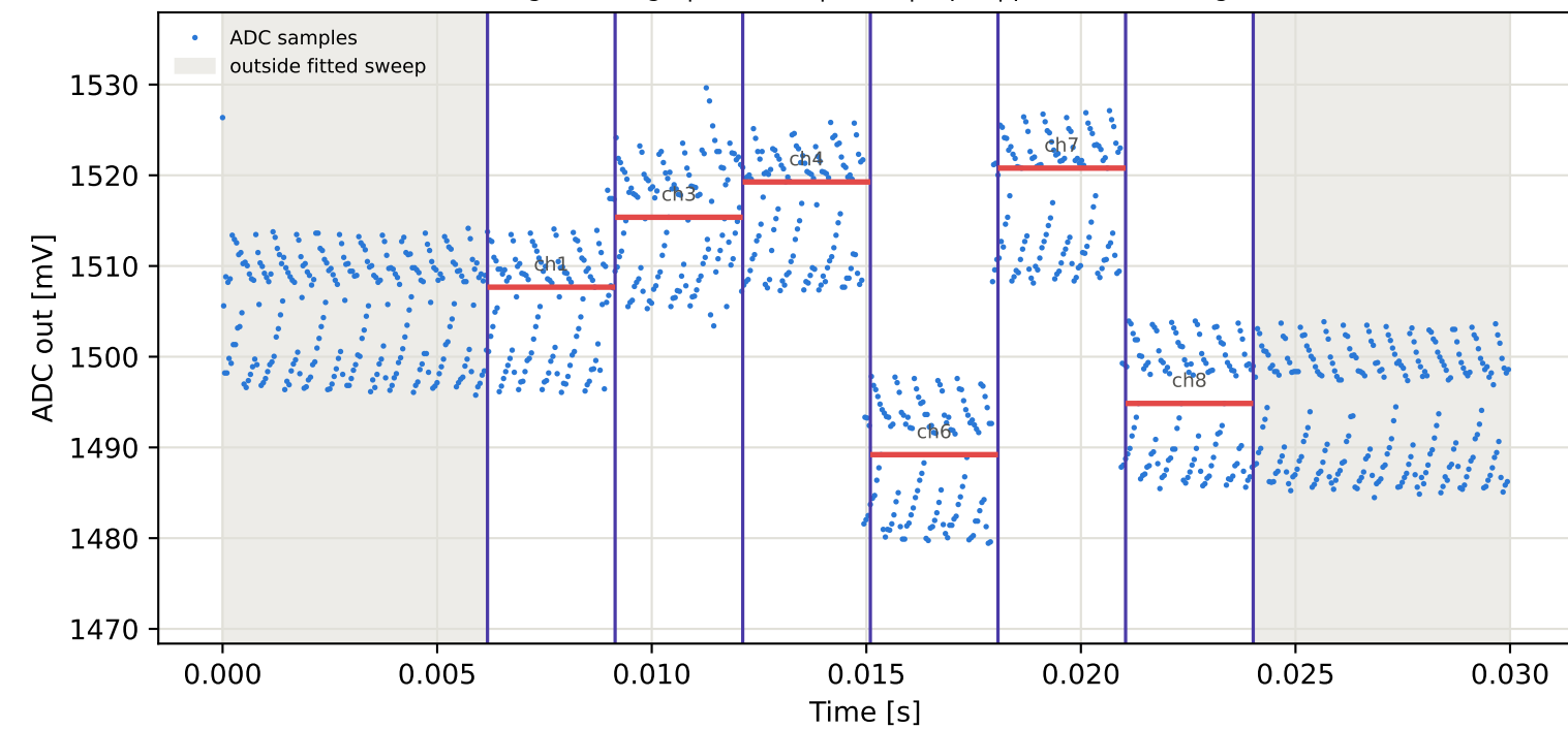
Tag15 &lt;- Tag9 | 965 MHz | run 0 | rep 1 | phase 142.73 deg
