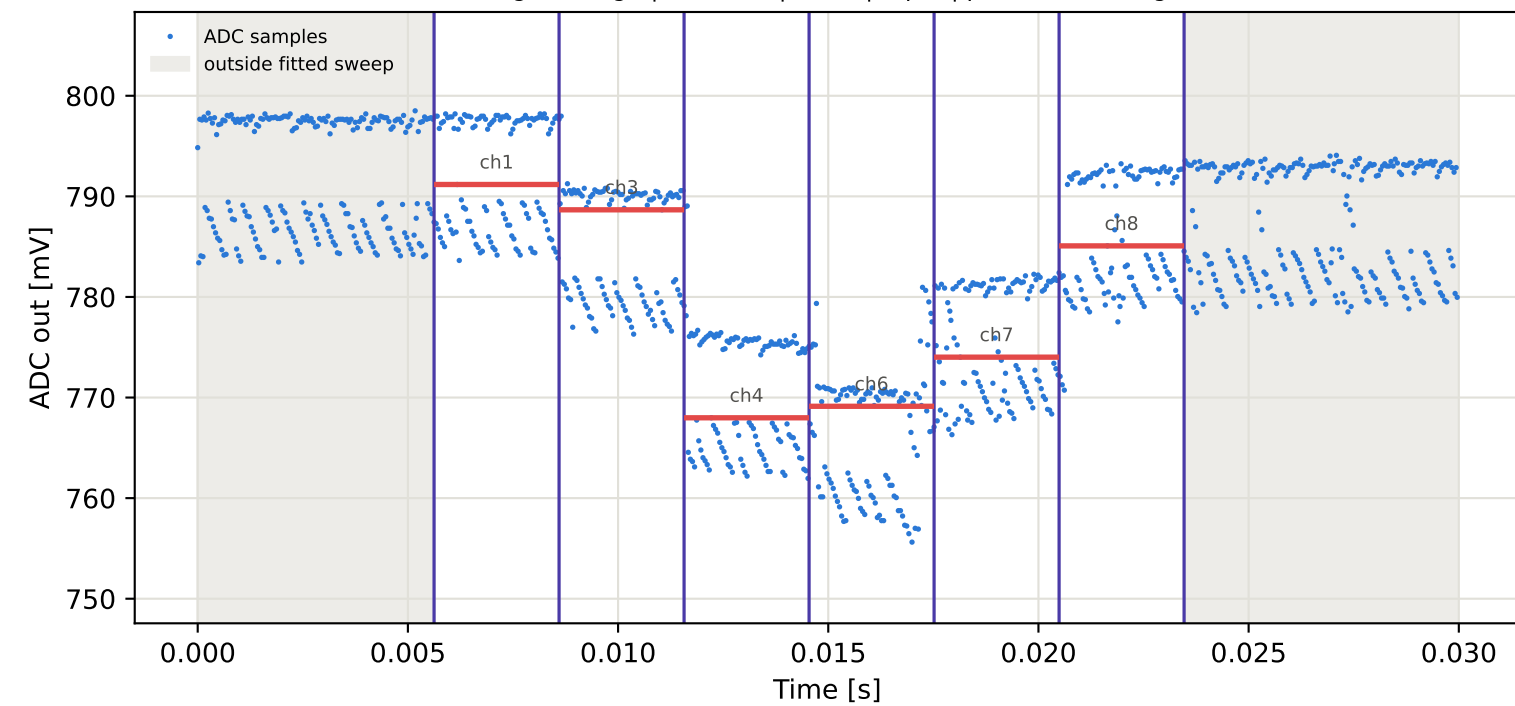
Tag5 &lt;- Tag9 | 915 MHz | run 0 | rep 1 | phase -29.22 deg
