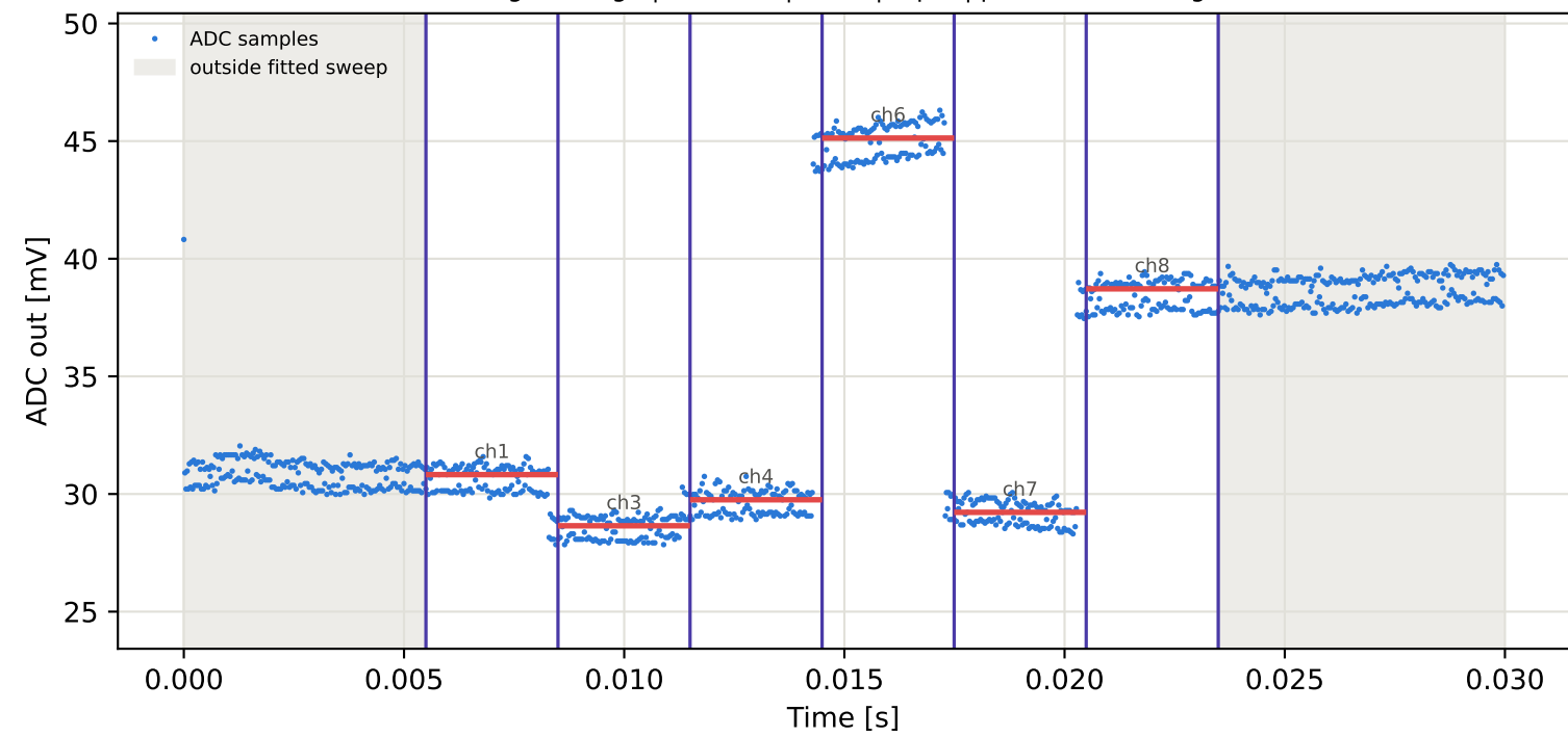
Tag3 &lt;- Tag2 | 915 MHz | run 0 | rep 1 | phase 177.60 deg
