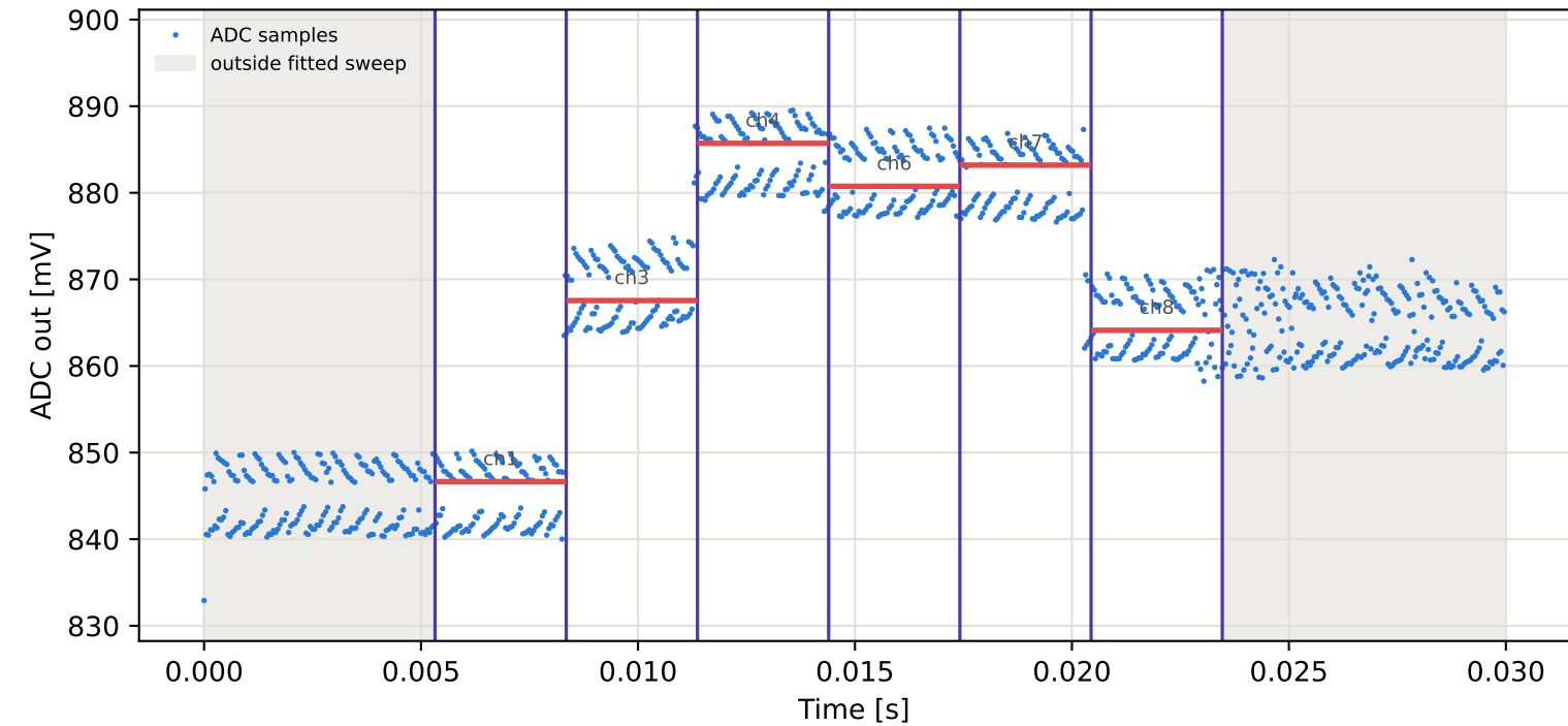
Tag8 &lt;- Tag7 | 865 MHz | run 0 | rep 1 | phase 175.53 deg
