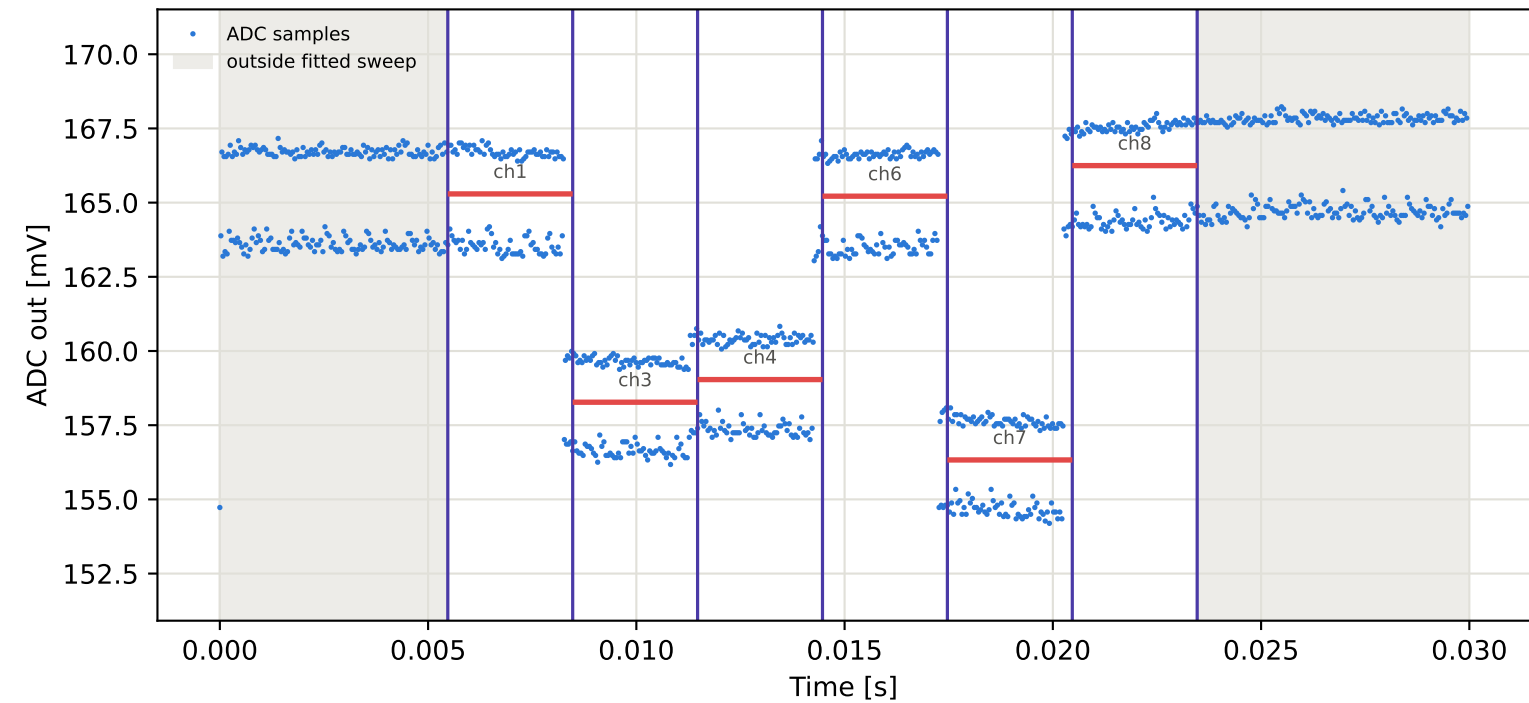
Tag4 &lt;- Tag3 | 795 MHz | run 0 | rep 1 | phase -118.83 deg
