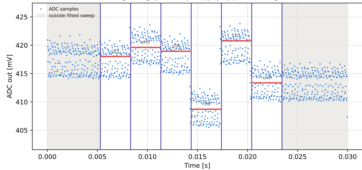
Tag1 &lt;- Tag4 | 975 MHz | run 0 | rep 1 | phase -8.43 deg
