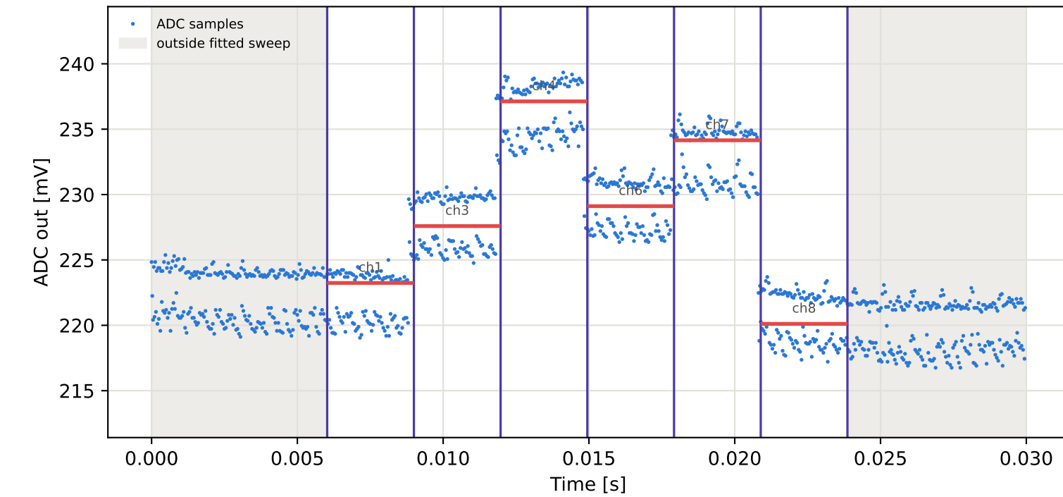
Tag2 &lt;- Tag15 | 925 MHz | run 0 | rep 1 | phase -34.15 deg
