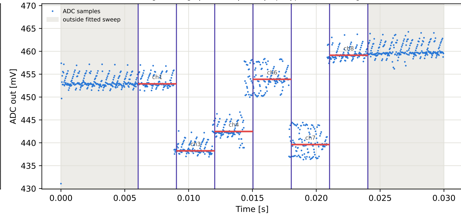
Tag15 &lt;- Tag6 | 845 MHz | run 0 | rep 1 | phase 117.10 deg
