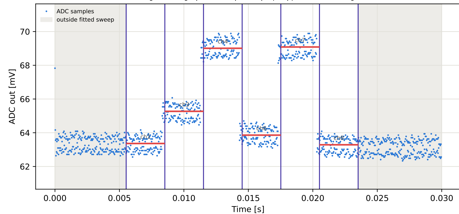
Tag10 &lt;- Tag1 | 775 MHz | run 0 | rep 1 | phase -60.79 deg
