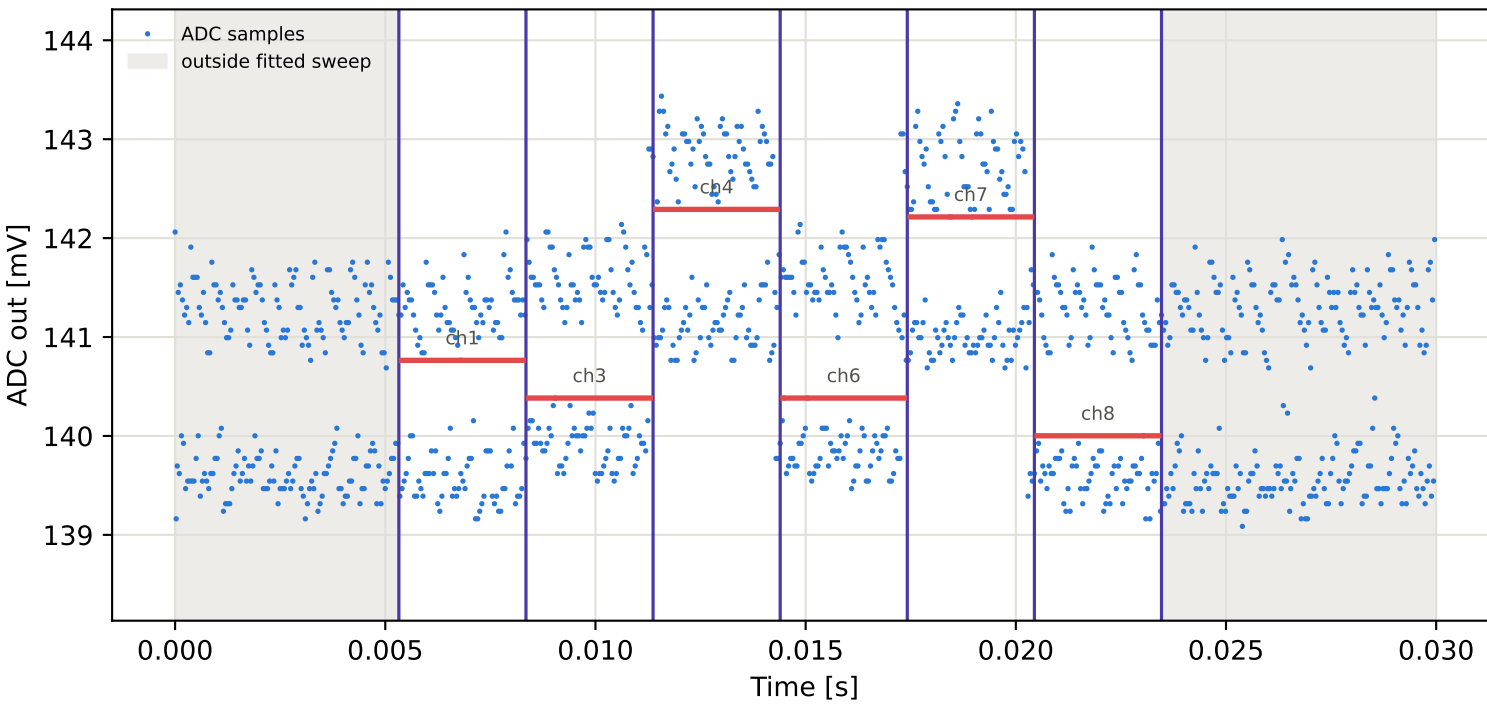
Tag8 &lt;- Tag15 | 775 MHz | run 0 | rep 1 | phase 30.31 deg
