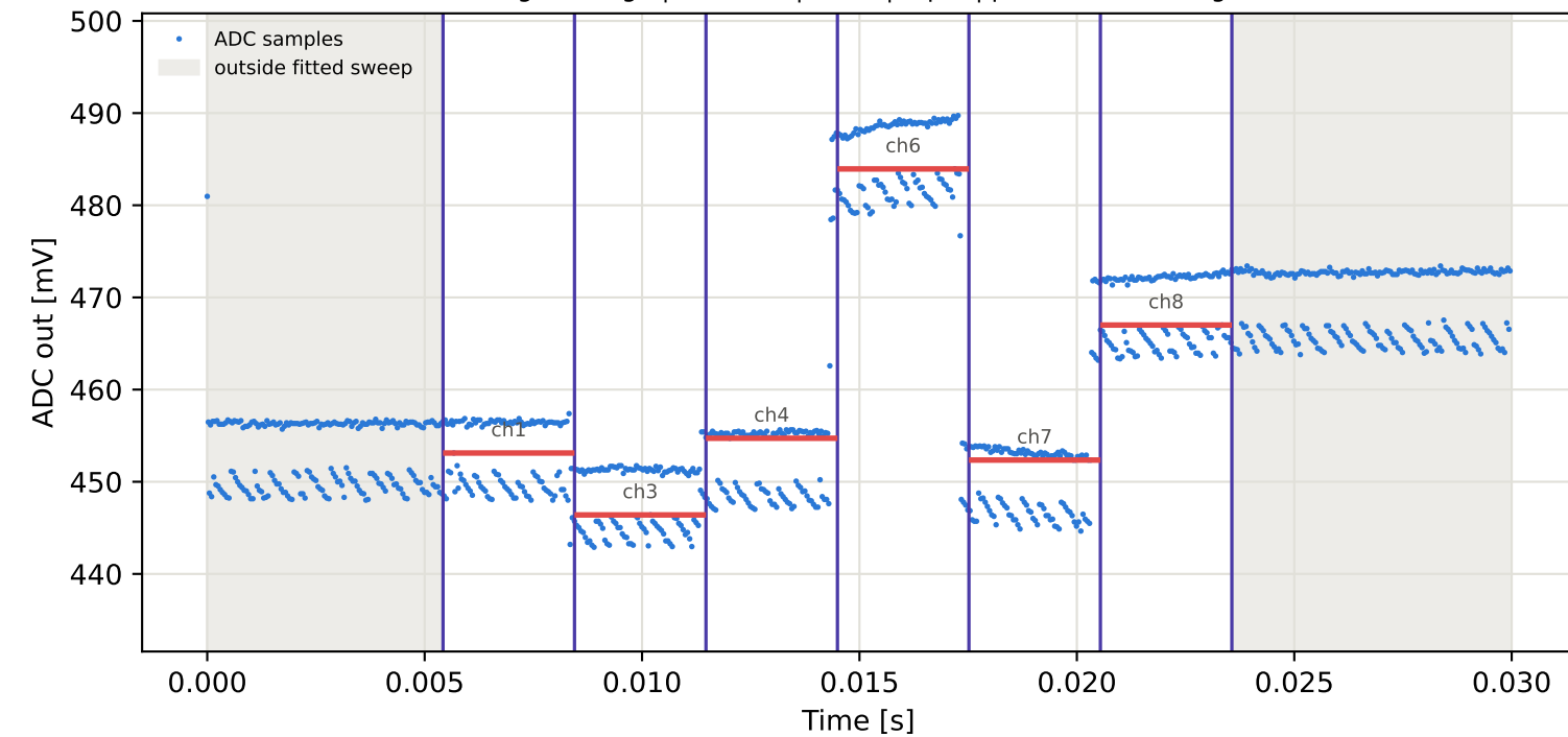
Tag7 &lt;- Tag5 | 925 MHz | run 0 | rep 1 | phase -173.50 deg
