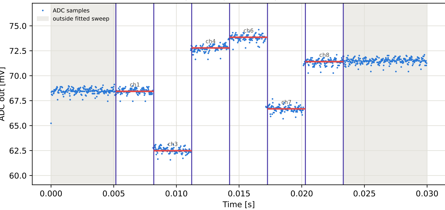
Tag10 &lt;- Tag4 | 775 MHz | run 0 | rep 1 | phase -141.53 deg
