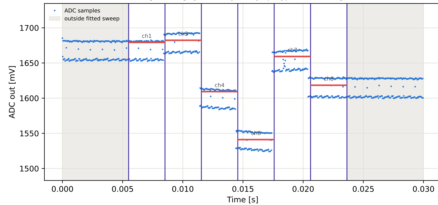
Tag2 &lt;- Tag1 | 975 MHz | run 0 | rep 1 | phase 106.42 deg
