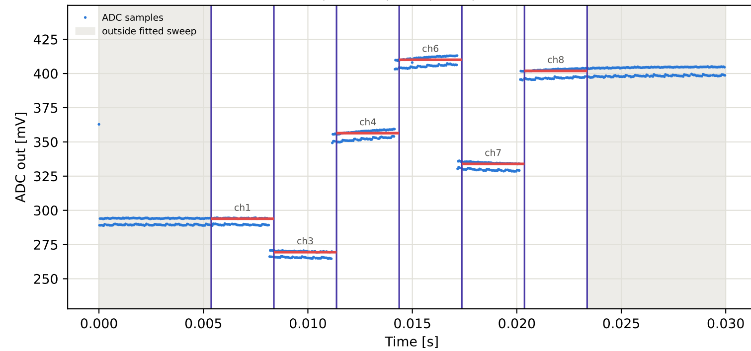
Tag9 &lt;- Tag16 | 845 MHz | run 0 | rep 1 | phase -151.49 deg
