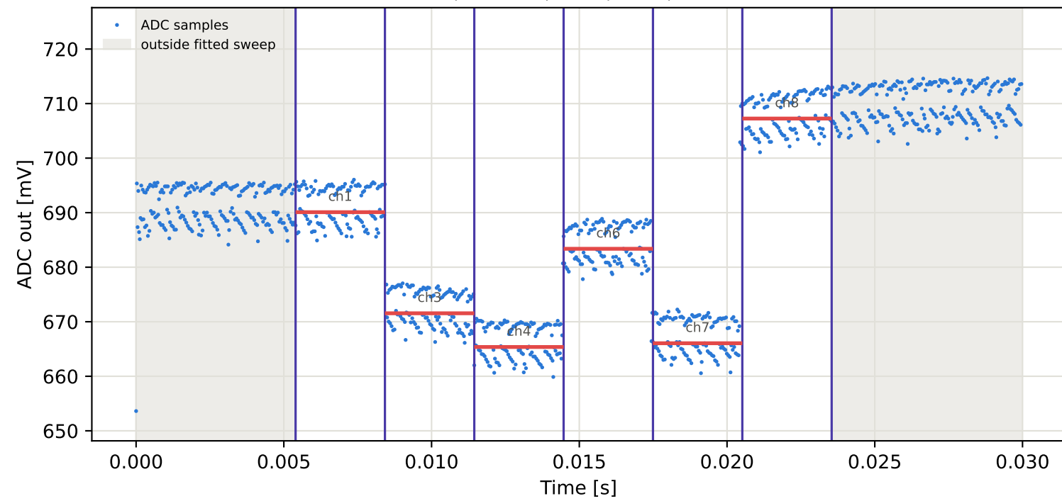
Tag10 &lt;- Tag5 | 885 MHz | run 0 | rep 1 | phase 112.07 deg
