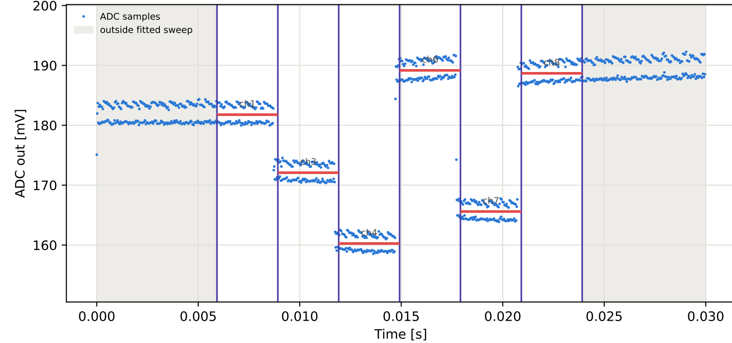
Tag6 &lt;- Tag1 | 965 MHz | run 0 | rep 1 | phase -86.19 deg
