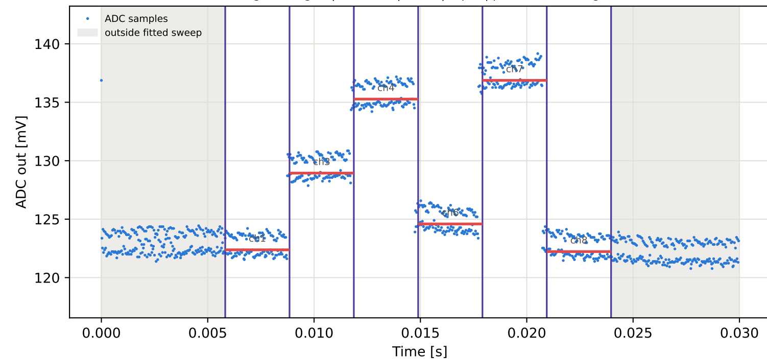
Tag6 &lt;- Tag2 | 805 MHz | run 0 | rep 1 | phase -10.09 deg
