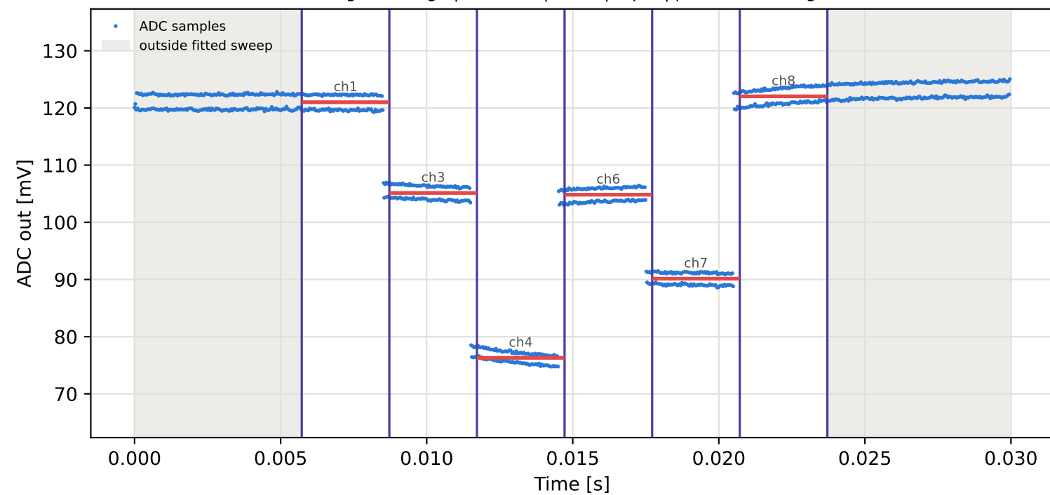
Tag10 &lt;- Tag1 | 965 MHz | run 0 | rep 1 | phase 80.58 deg
