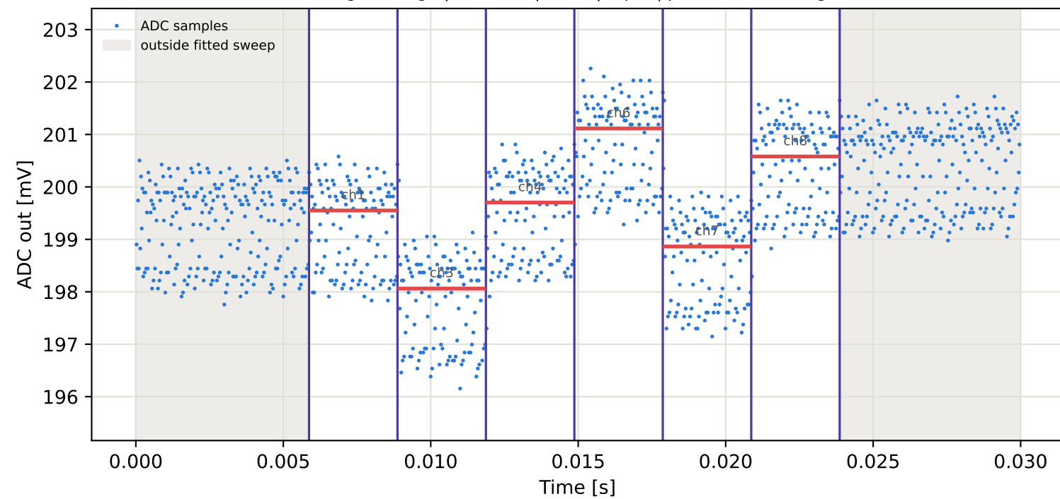
Tag3 &lt;- Tag7 | 805 MHz | run 0 | rep 1 | phase -87.81 deg
