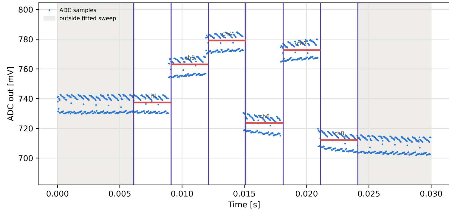
Tag9 &lt;- Tag2 | 935 MHz | run 0 | rep 1 | phase 142.41 deg
