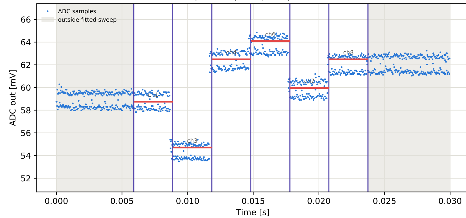
Tag9 &lt;- Tag5 | 805 MHz | run 0 | rep 1 | phase 107.56 deg
