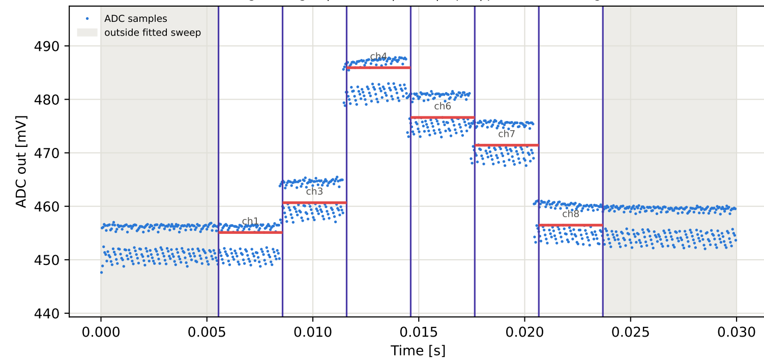
Tag1 &lt;- Tag16 | 955 MHz | run 0 | rep 1 | phase -10.31 deg
