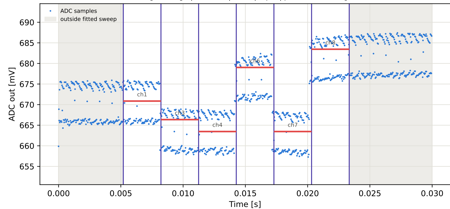
Tag9 &lt;- Tag8 | 885 MHz | run 0 | rep 1 | phase 19.09 deg
