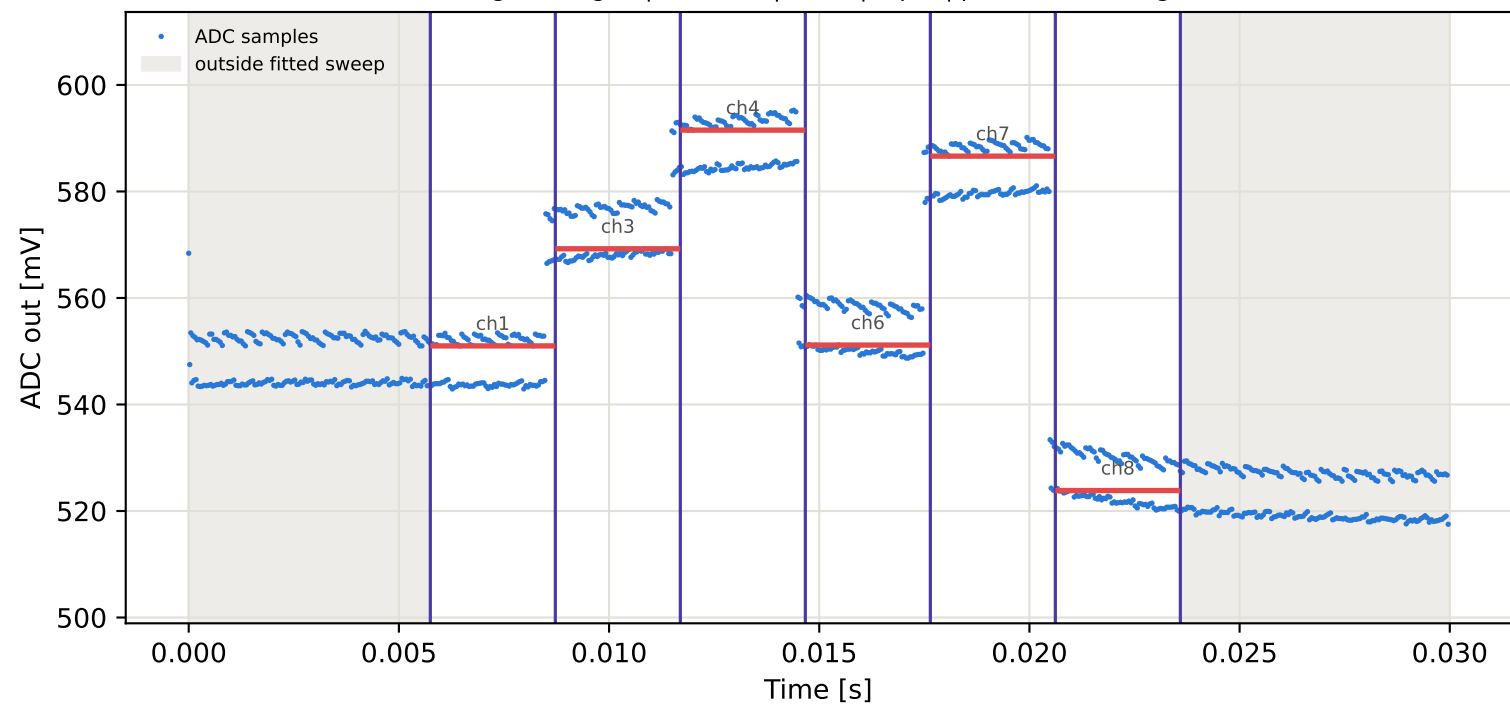
Tag6 &lt;- Tag3 | 895 MHz | run 0 | rep 1 | phase 40.58 deg
