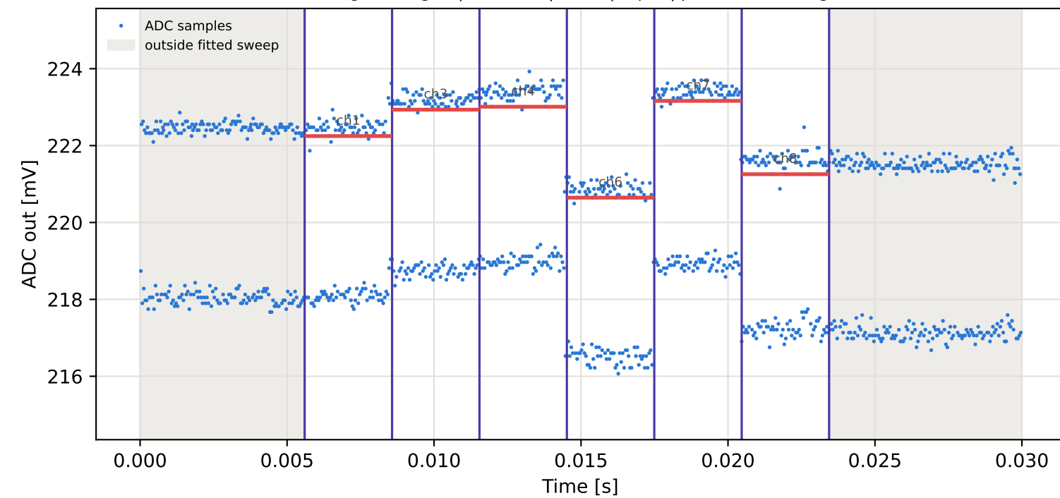
Tag5 &lt;- Tag16 | 975 MHz | run 0 | rep 1 | phase 49.39 deg
