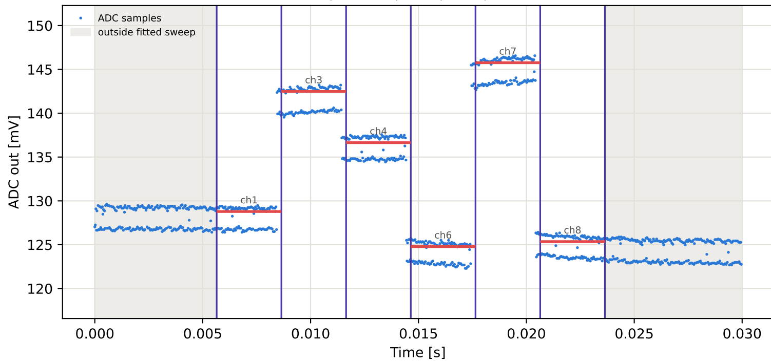
Tag8 &lt;- Tag16 | 775 MHz | run 0 | rep 1 | phase -14.77 deg
