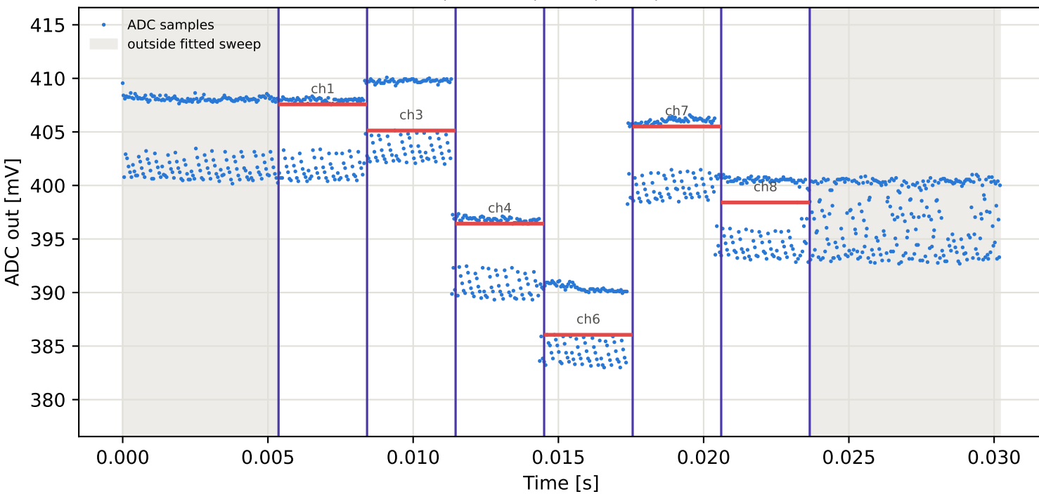
Tag3 &lt;- Tag16 | 985 MHz | run 0 | rep 1 | phase 24.52 deg
