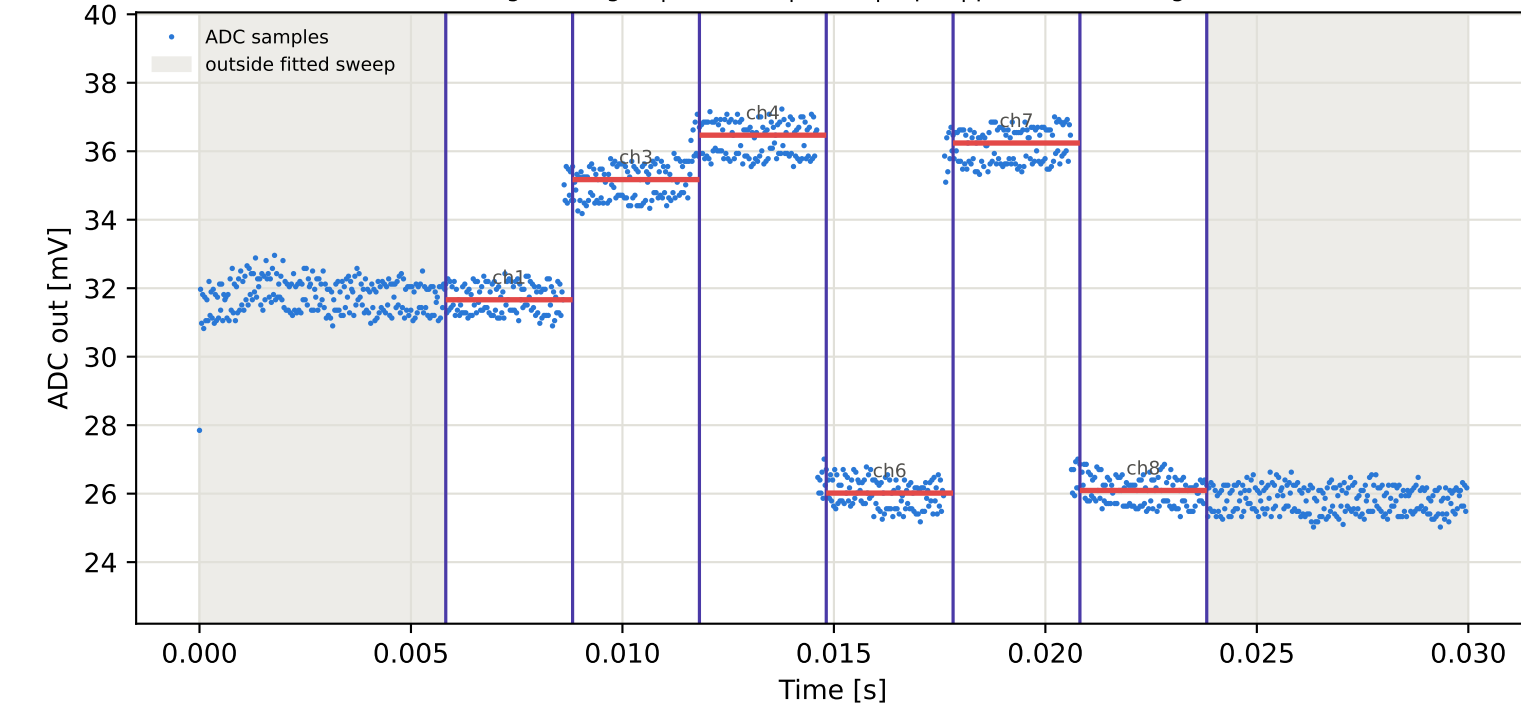
Tag3 &lt;- Tag16 | 915 MHz | run 0 | rep 1 | phase -32.44 deg
