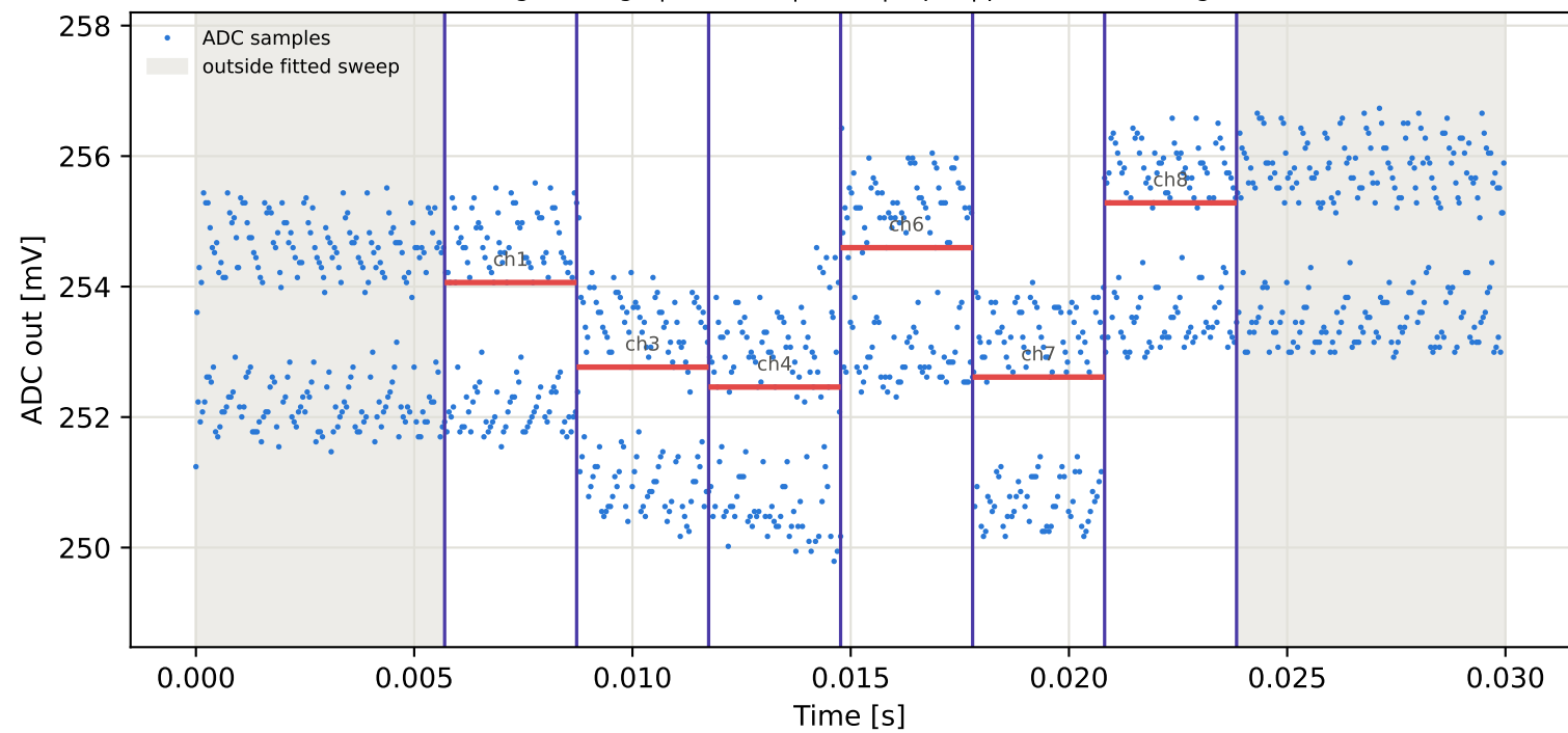
Tag7 &lt;- Tag4 | 835 MHz | run 0 | rep 1 | phase 23.41 deg
