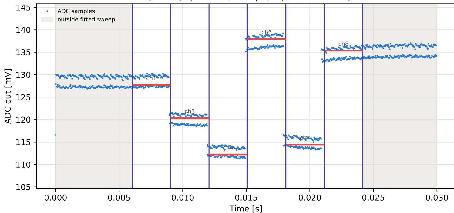
Tag6 &lt;- Tag1 | 995 MHz | run 0 | rep 1 | phase -78.33 deg
