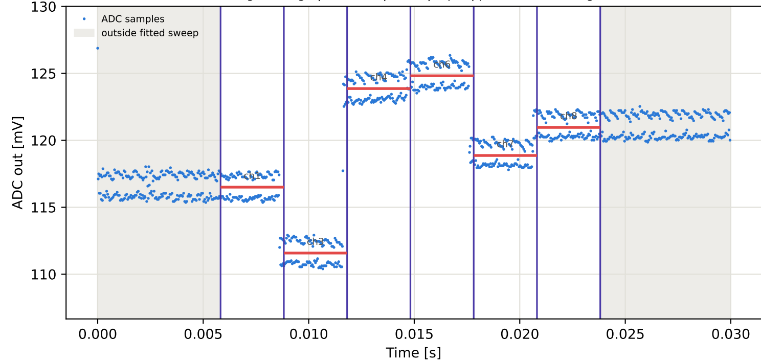
Tag8 &lt;- Tag7 | 785 MHz | run 0 | rep 1 | phase 51.53 deg
