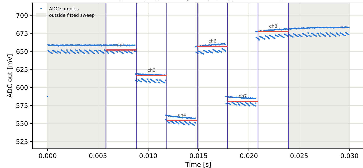
Tag7 &lt;- Tag3 | 945 MHz | run 0 | rep 1 | phase 90.60 deg
