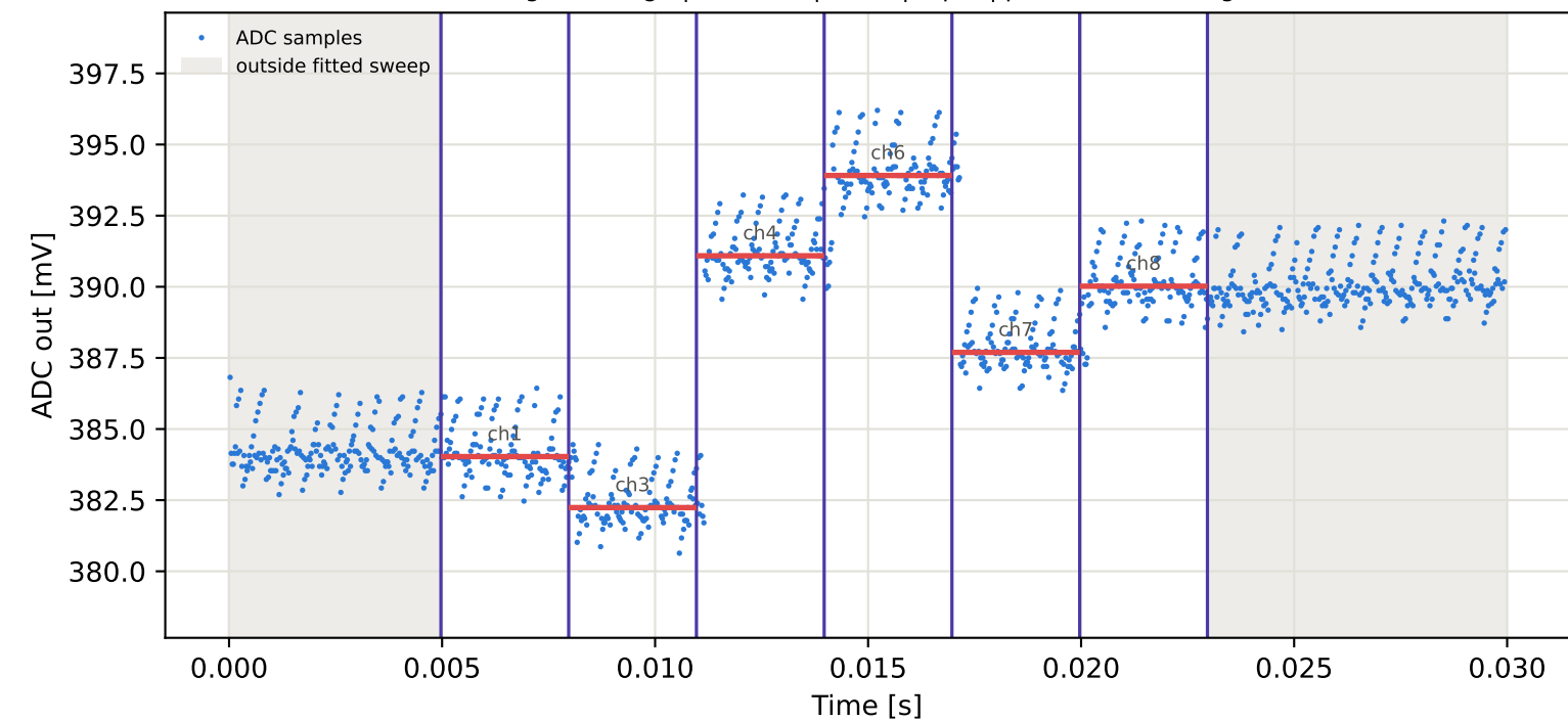
Tag16 &lt;- Tag10 | 835 MHz | run 0 | rep 1 | phase -75.92 deg
