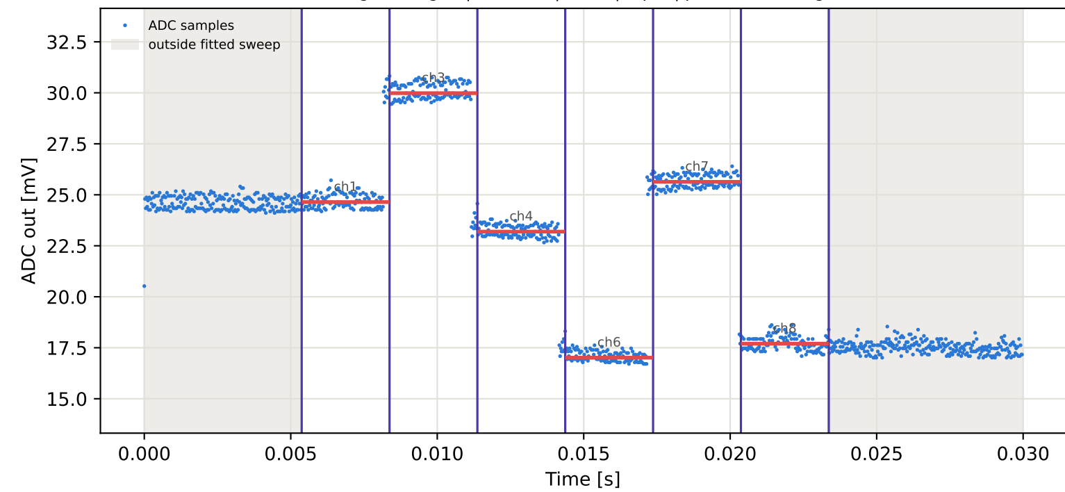
Tag1 &lt;- Tag16 | 845 MHz | run 0 | rep 1 | phase -162.51 deg
