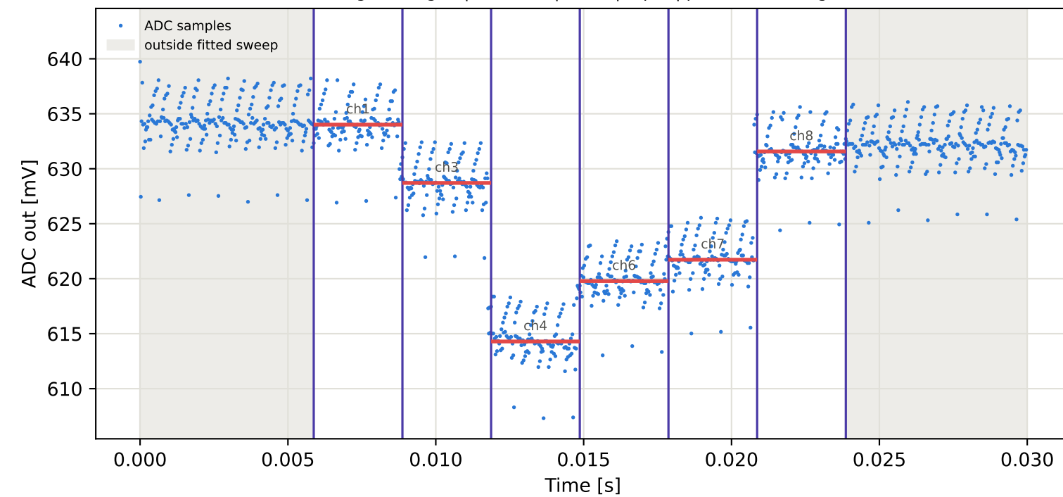
Tag6 &lt;- Tag2 | 965 MHz | run 0 | rep 1 | phase -102.20 deg
