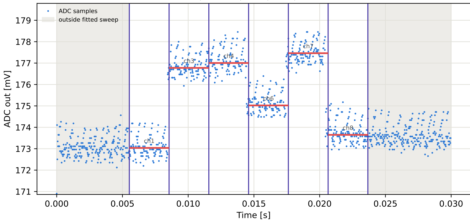
Tag10 &lt;- Tag1 | 855 MHz | run 0 | rep 1 | phase -67.88 deg
