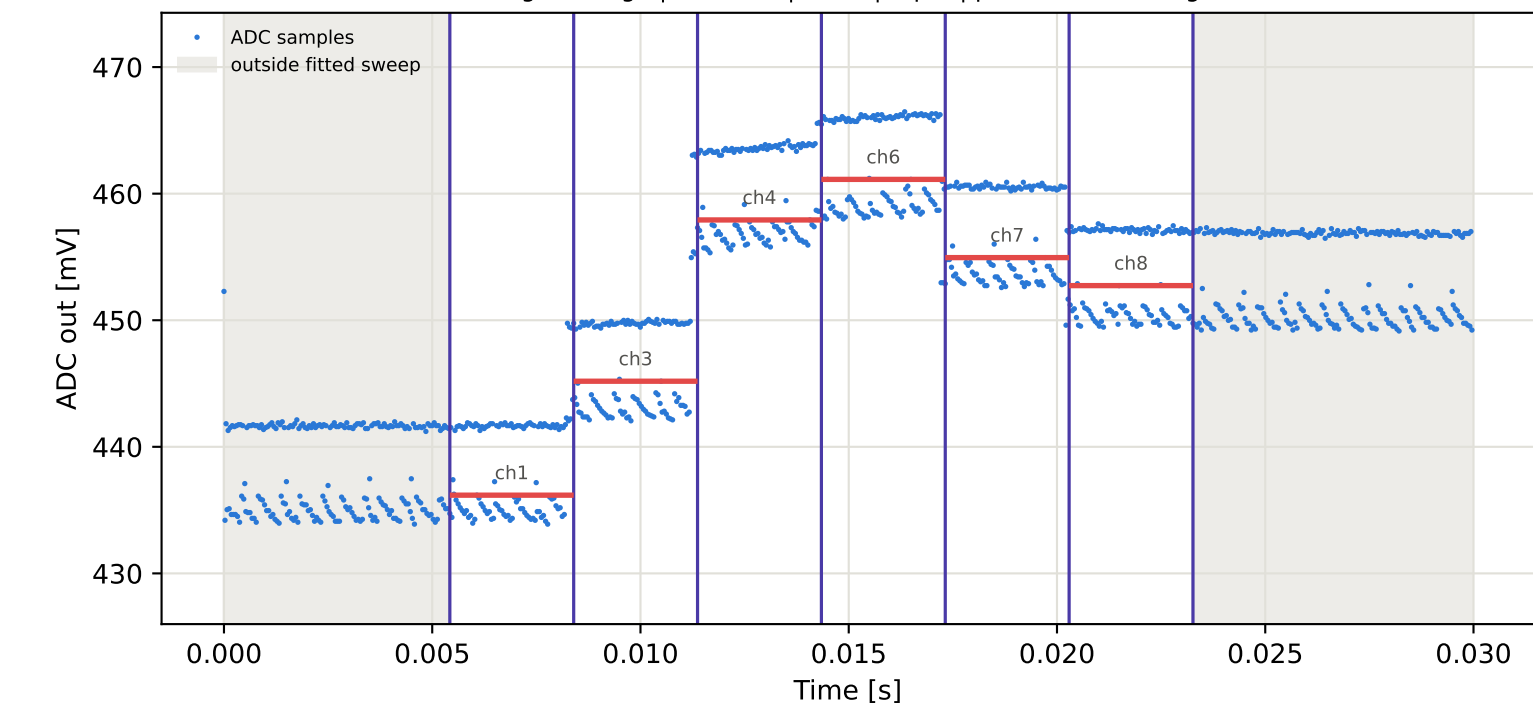
Tag5 &lt;- Tag3 | 845 MHz | run 0 | rep 1 | phase -126.00 deg
