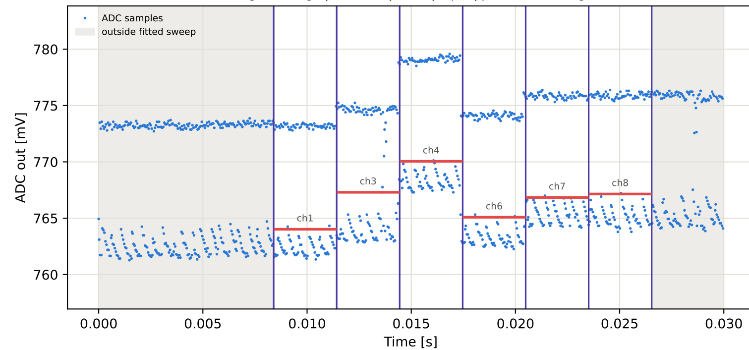
Tag16 &lt;- Tag4 | 855 MHz | run 0 | rep 1 | phase 158.85 deg
