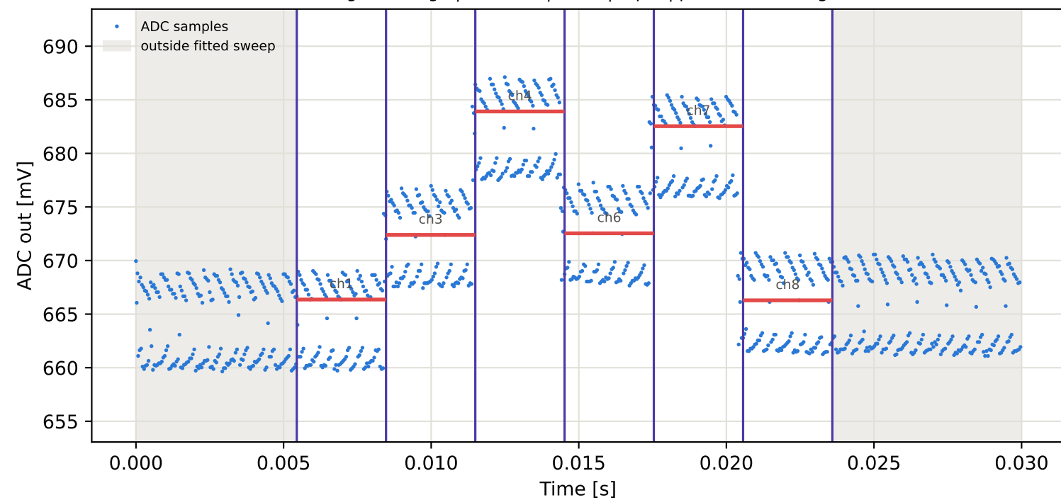
Tag16 &lt;- Tag7 | 825 MHz | run 0 | rep 1 | phase -83.00 deg
