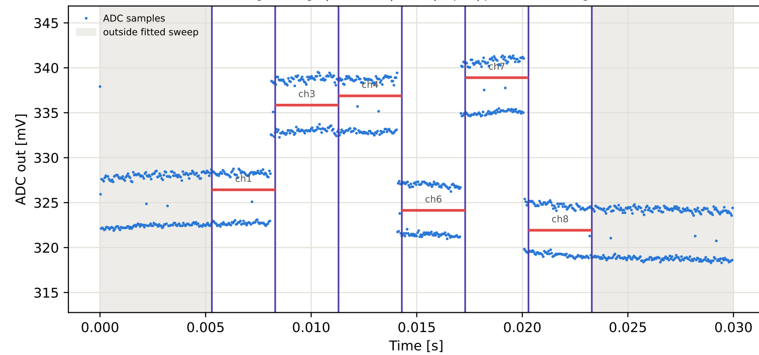
Tag6 &lt;- Tag9 | 845 MHz | run 0 | rep 1 | phase -93.90 deg
