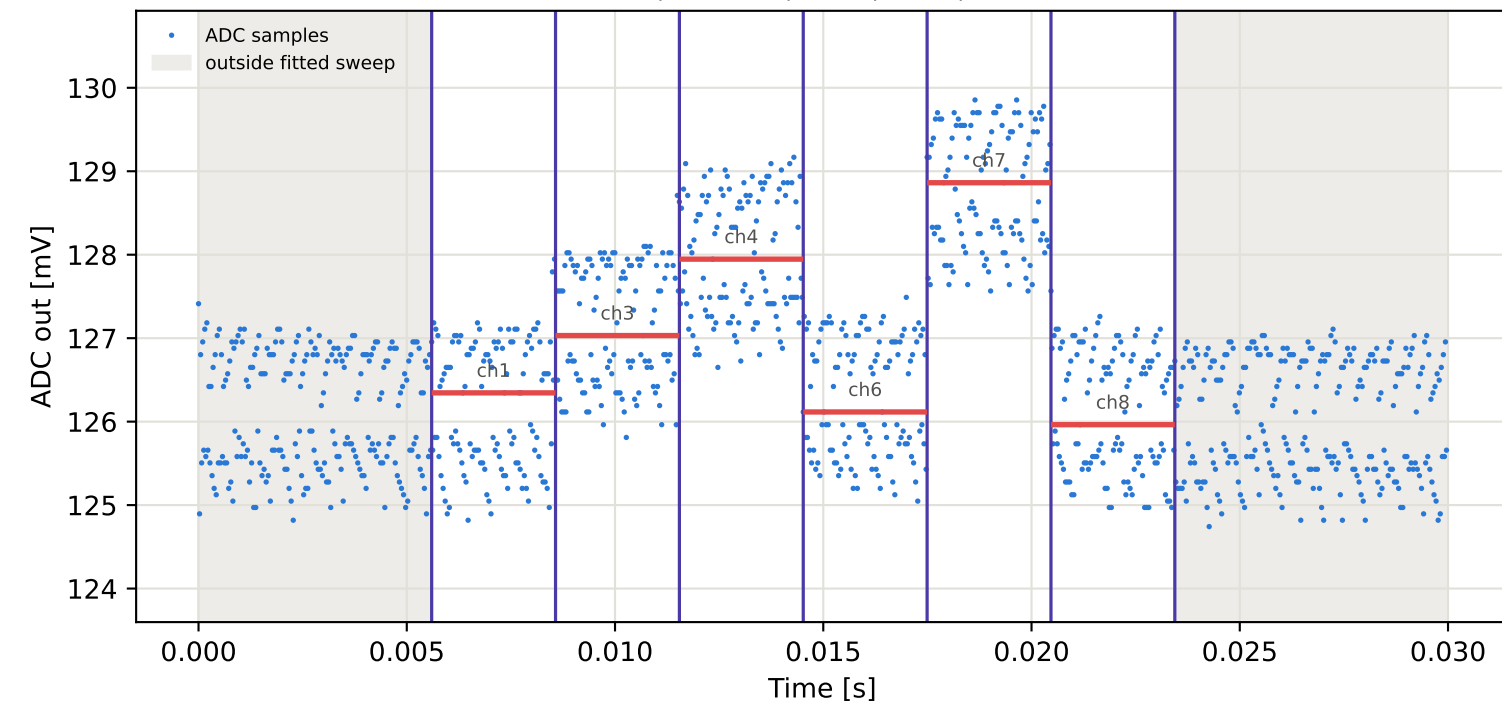
Tag16 &lt;- Tag10 | 775 MHz | run 0 | rep 1 | phase -45.66 deg
