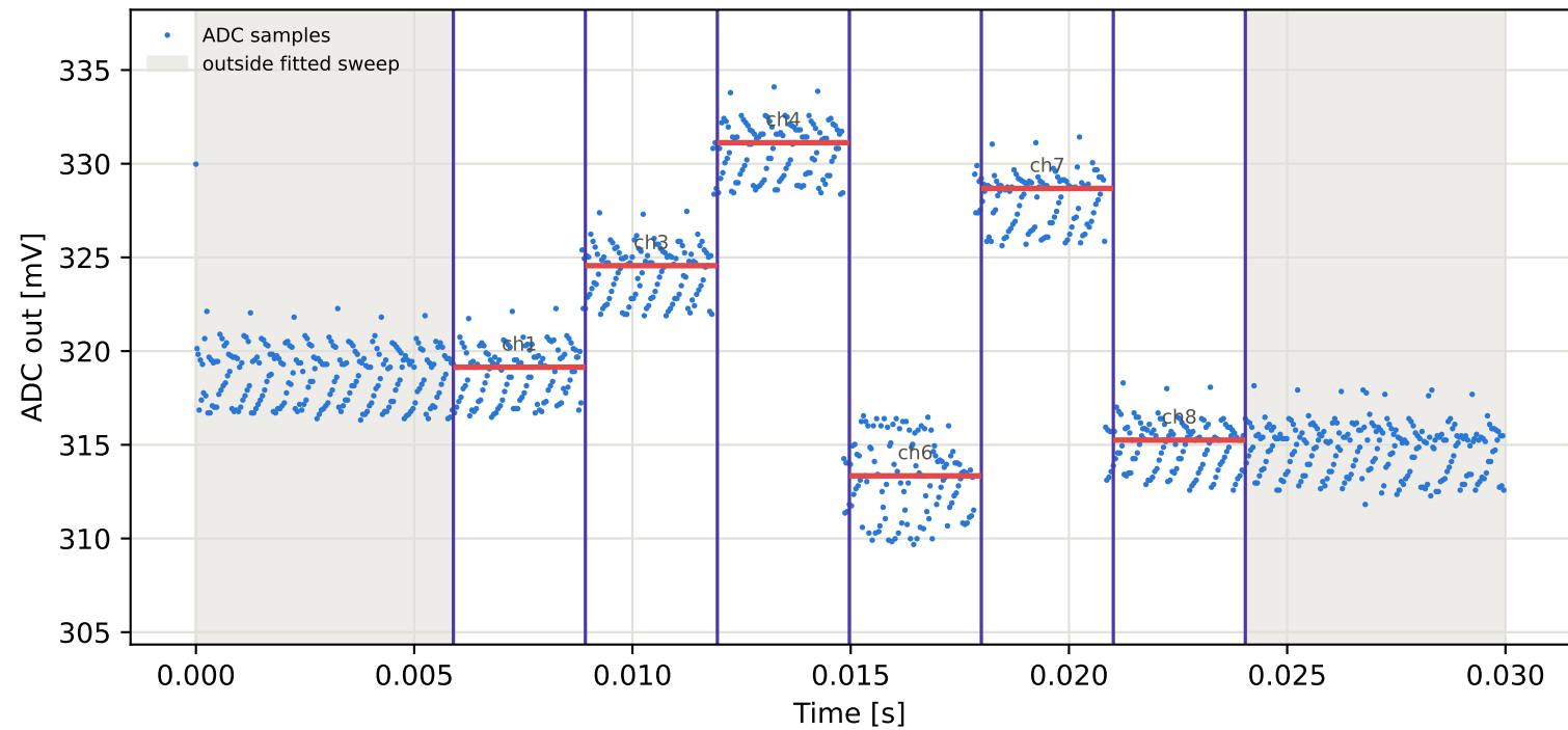
Tag7 &lt;- Tag6 | 995 MHz | run 0 | rep 1 | phase -58.25 deg
