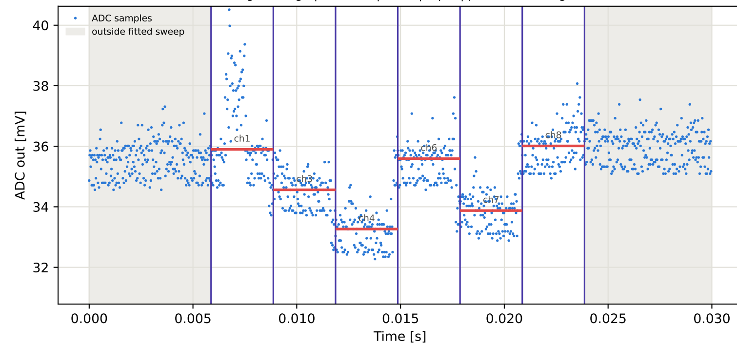
Tag2 &lt;- Tag7 | 975 MHz | run 0 | rep 1 | phase 97.06 deg
