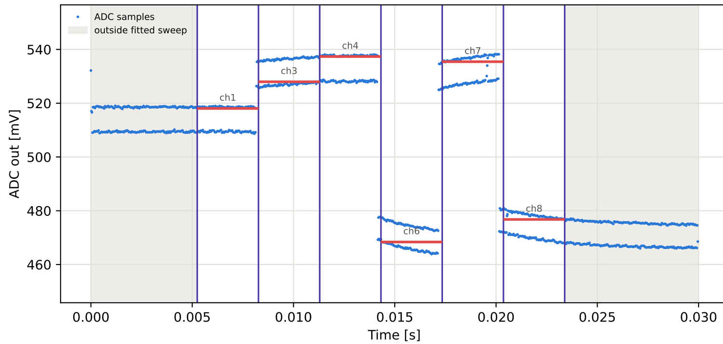
Tag10 &lt;- Tag8 | 905 MHz | run 0 | rep 1 | phase -45.92 deg
