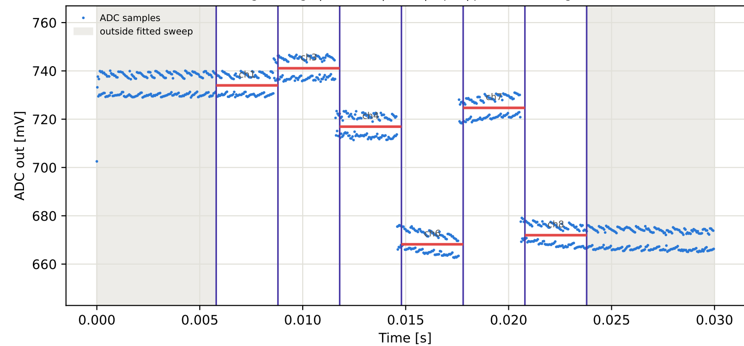
Tag7 &lt;- Tag1 | 875 MHz | run 0 | rep 1 | phase 19.86 deg
