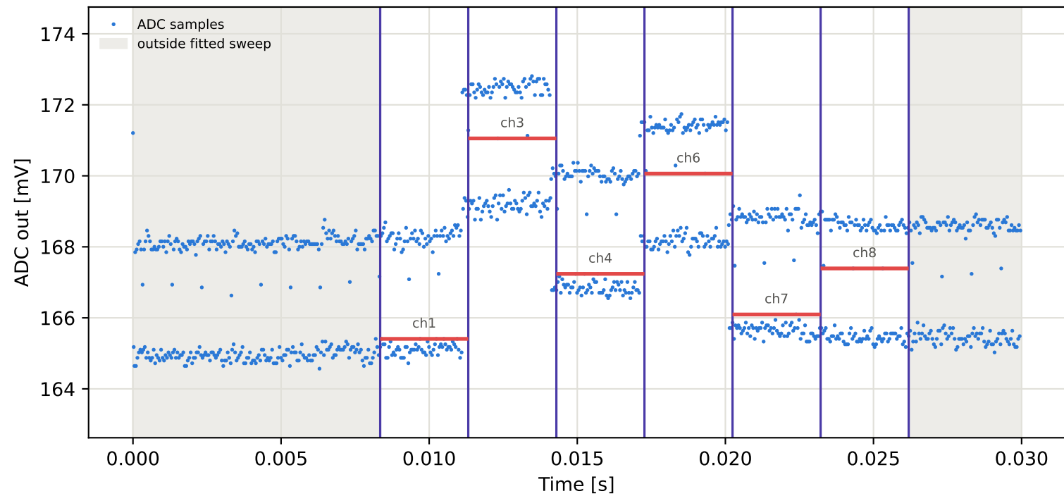
Tag3 &lt;- Tag15 | 795 MHz | run 0 | rep 1 | phase -113.52 deg
