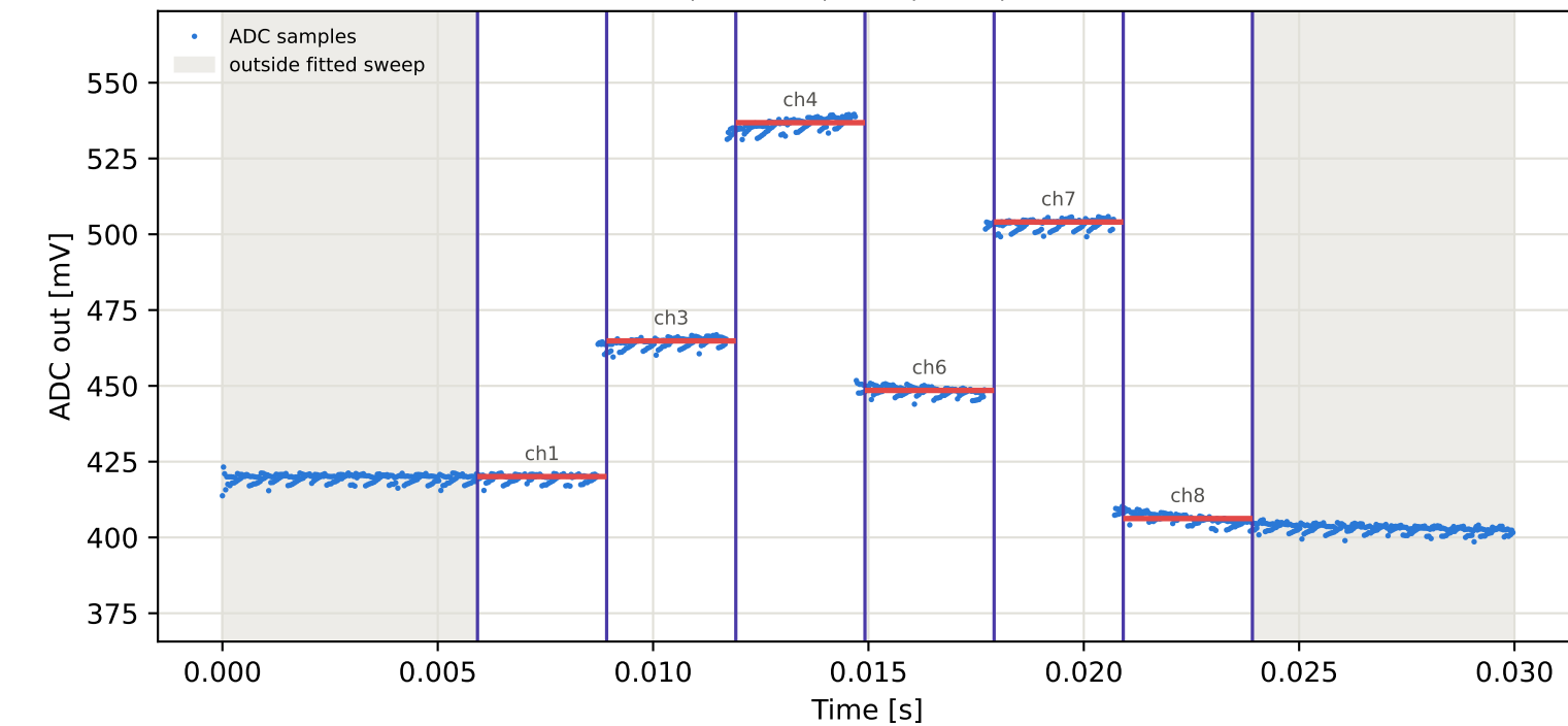
Tag9 &lt;- Tag16 | 945 MHz | run 0 | rep 1 | phase -89.52 deg
