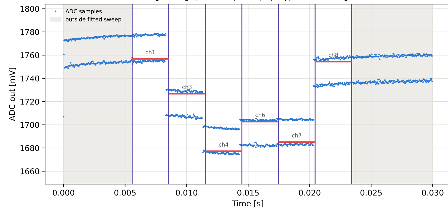
Tag9 &lt;- Tag10 | 885 MHz | run 0 | rep 1 | phase 10.63 deg
