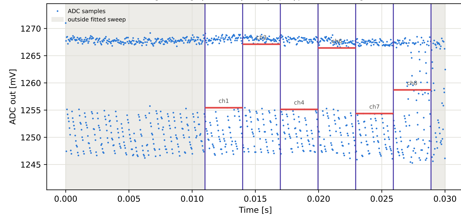
Tag16 &lt;- Tag4 | 955 MHz | run 0 | rep 1 | phase 62.02 deg
