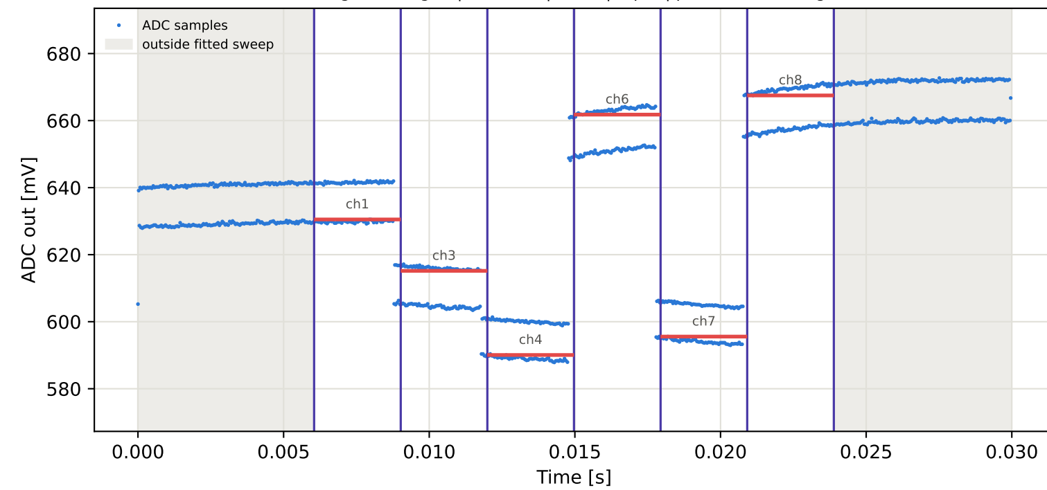
Tag10 &lt;- Tag2 | 935 MHz | run 0 | rep 1 | phase 40.03 deg
