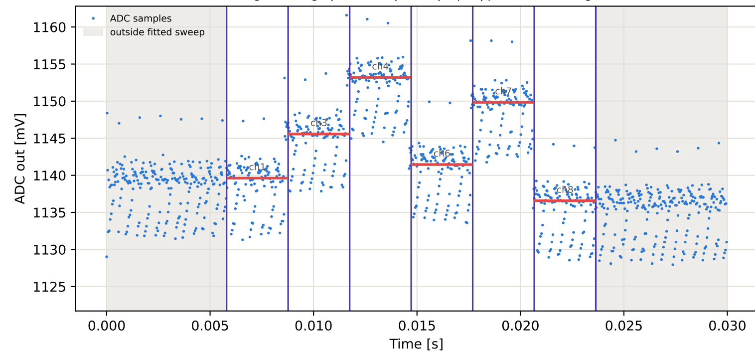
Tag16 &lt;- Tag15 | 955 MHz | run 0 | rep 1 | phase -71.29 deg
