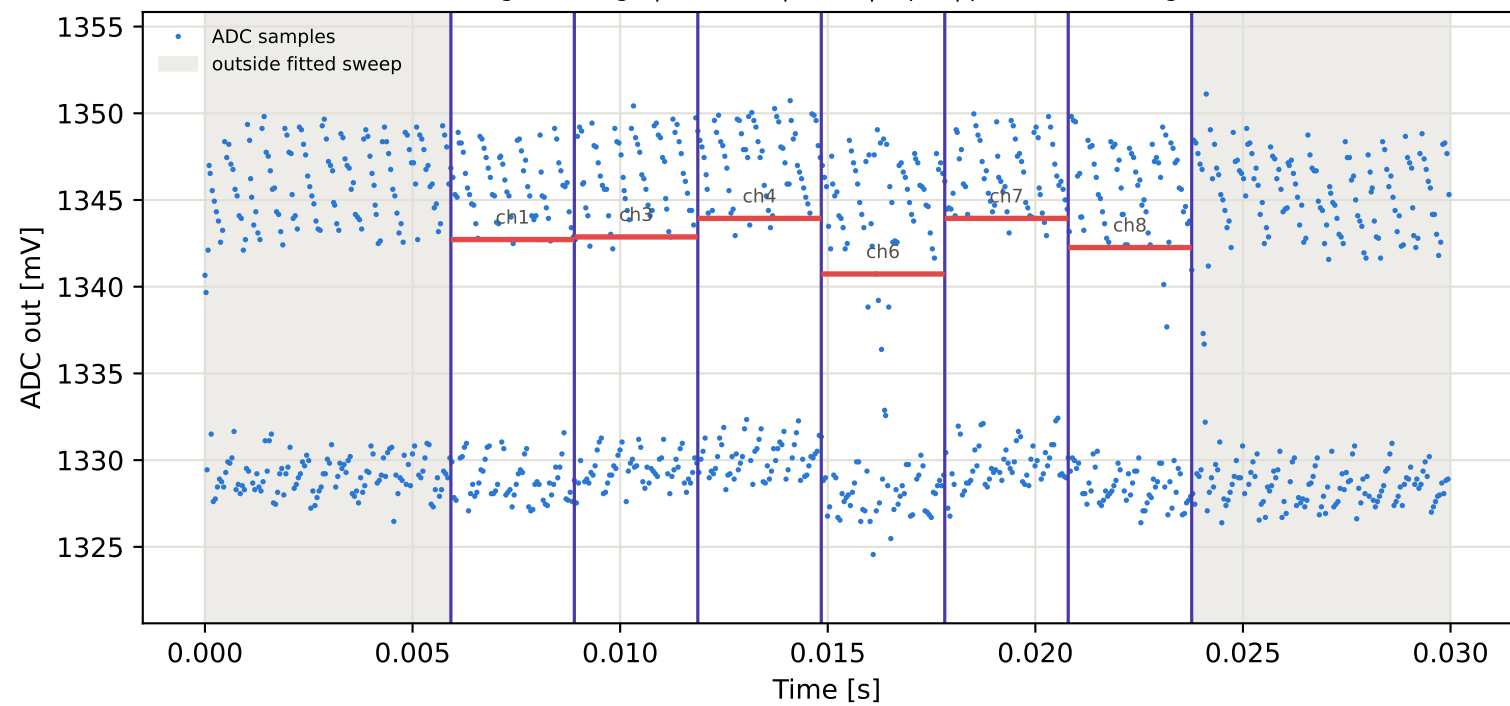
Tag15 &lt;- Tag4 | 955 MHz | run 0 | rep 1 | phase -157.24 deg
