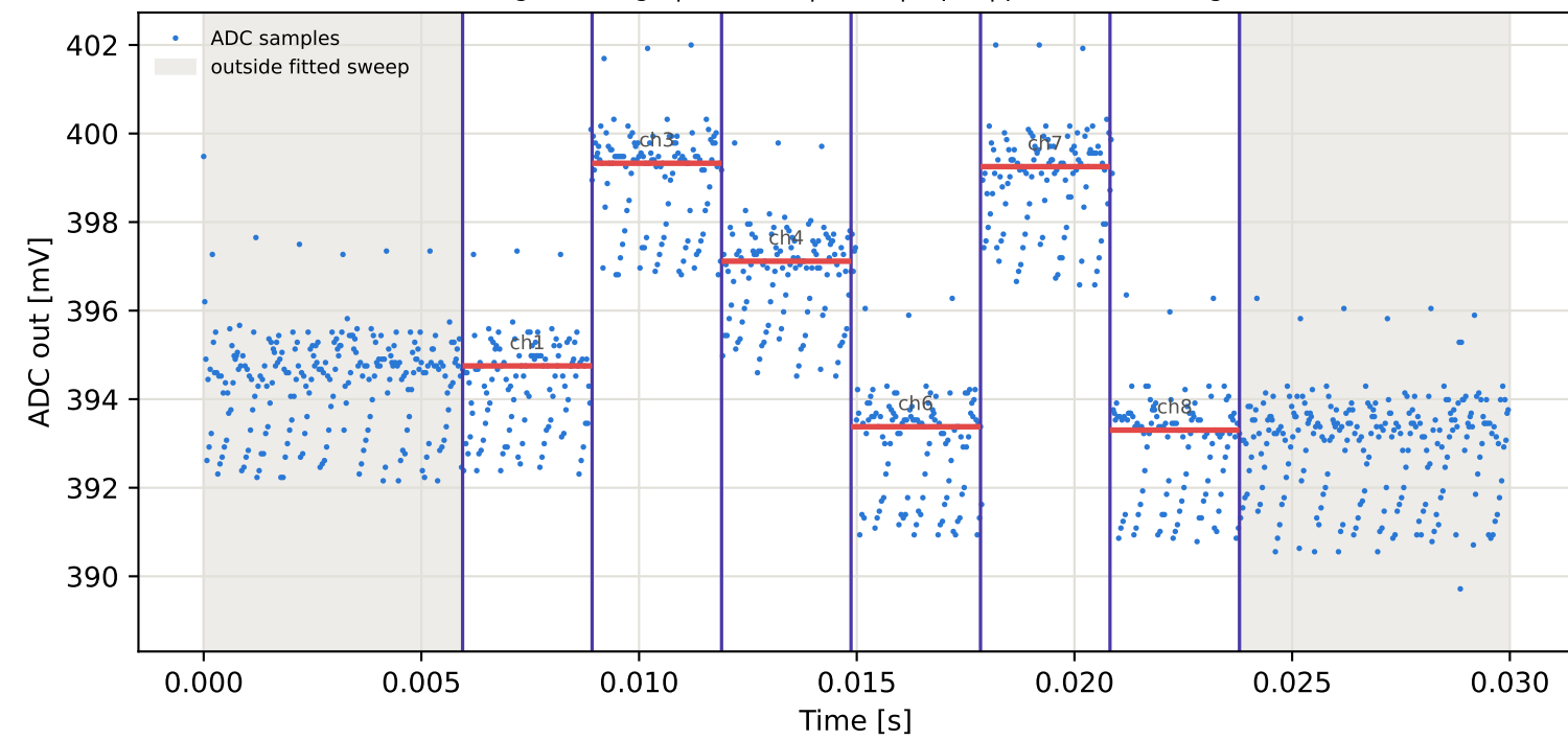
Tag16 &lt;- Tag5 | 805 MHz | run 0 | rep 1 | phase 76.44 deg
