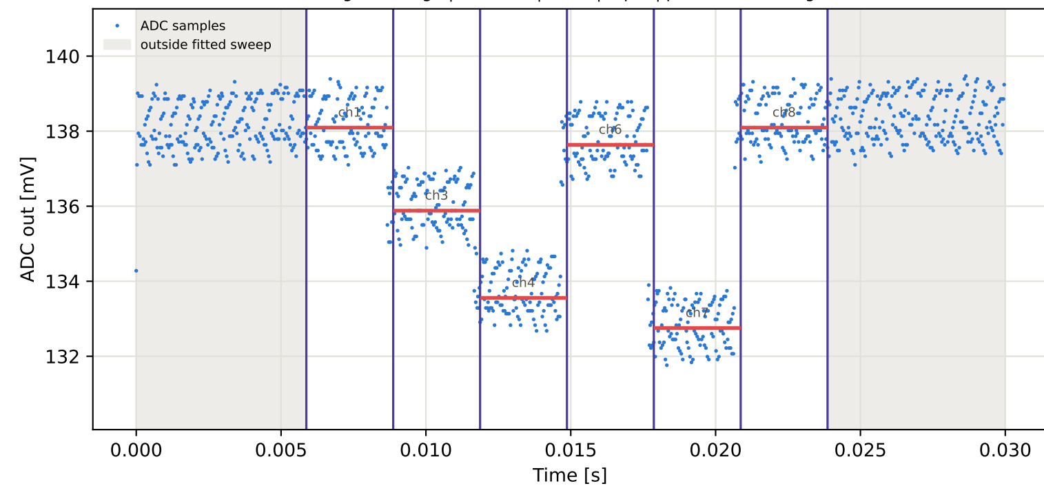
Tag16 &lt;- Tag7 | 775 MHz | run 0 | rep 1 | phase 123.06 deg
