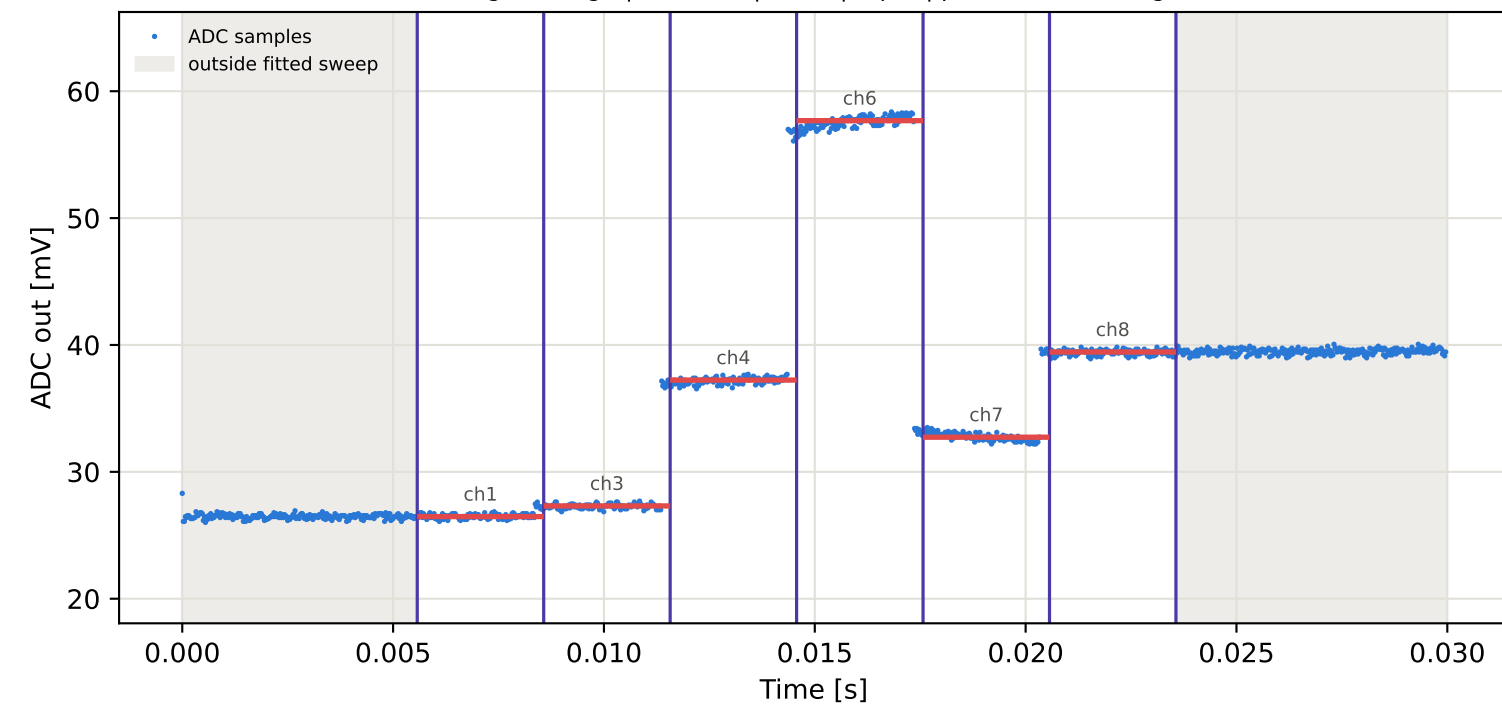
Tag2 &lt;- Tag5 | 915 MHz | run 0 | rep 1 | phase 39.72 deg
