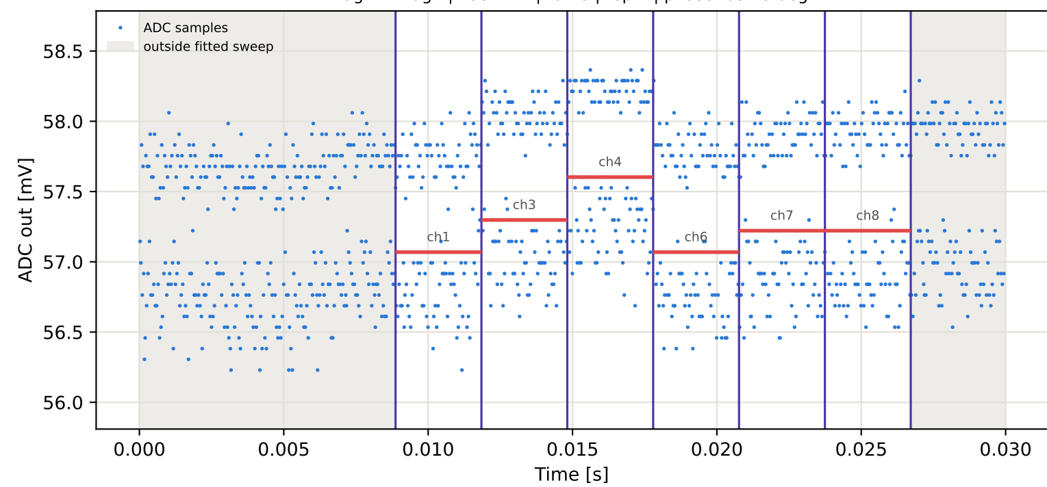
Tag7 &lt;- Tag4 | 795 MHz | run 0 | rep 1 | phase -83.24 deg
