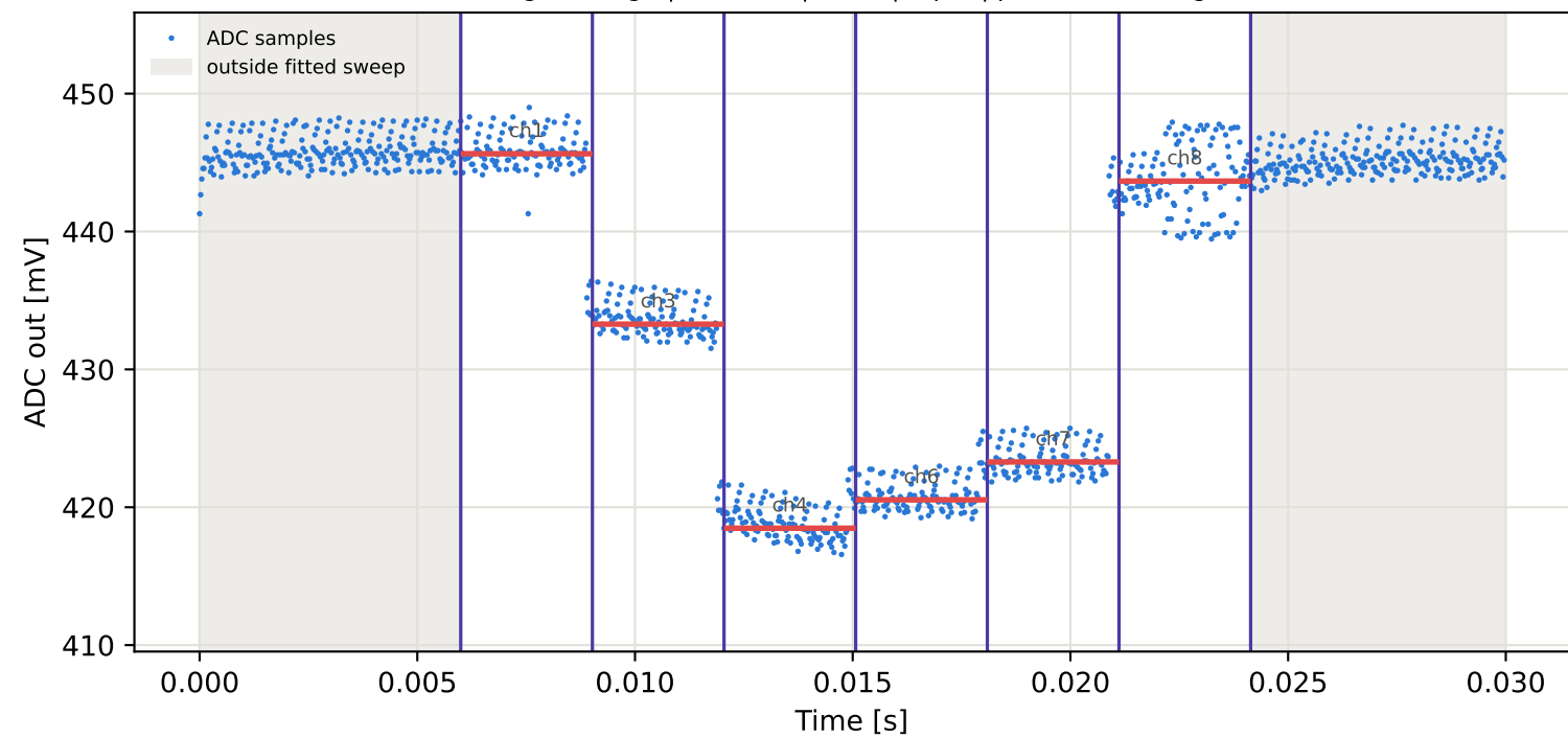
Tag1 &lt;- Tag7 | 895 MHz | run 0 | rep 1 | phase 84.96 deg
