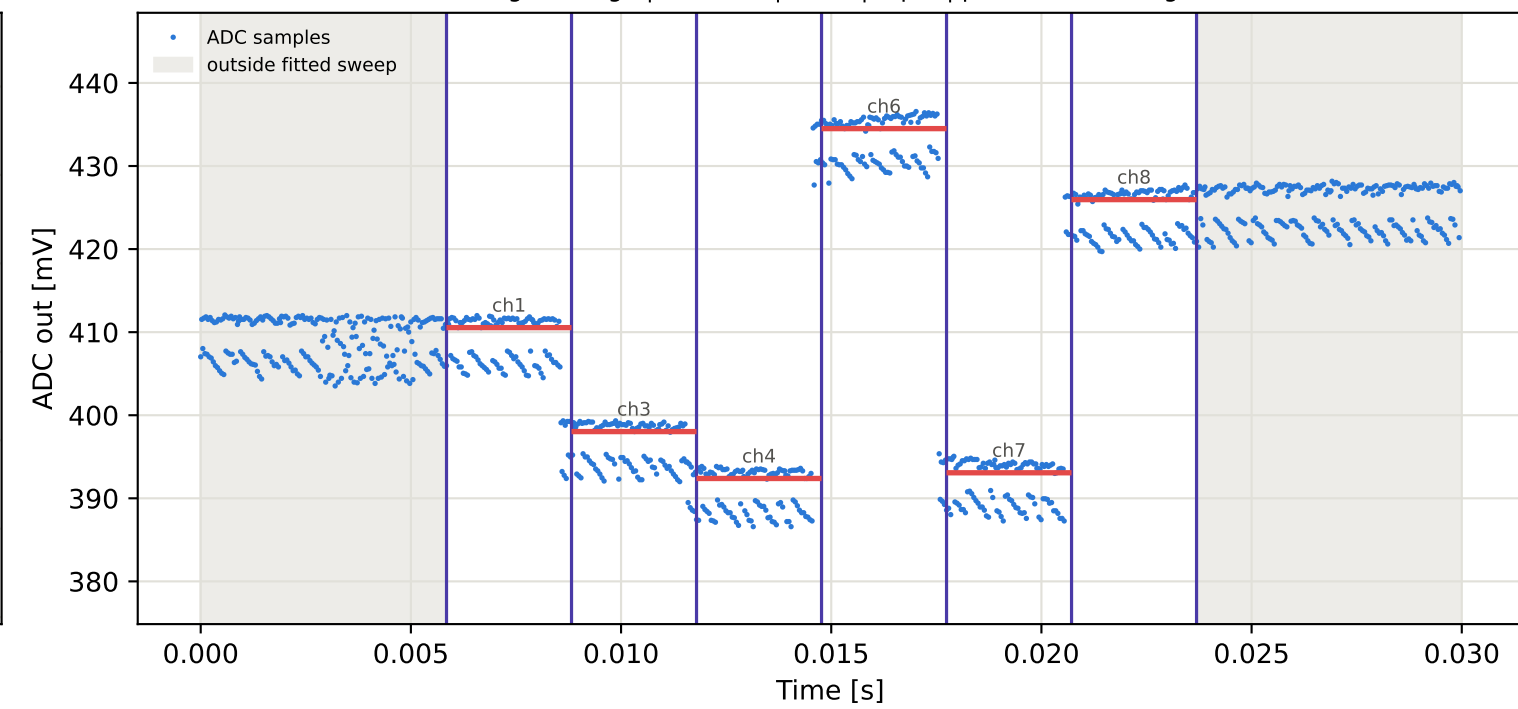
Tag6 &lt;- Tag5 | 965 MHz | run 0 | rep 1 | phase 147.62 deg
