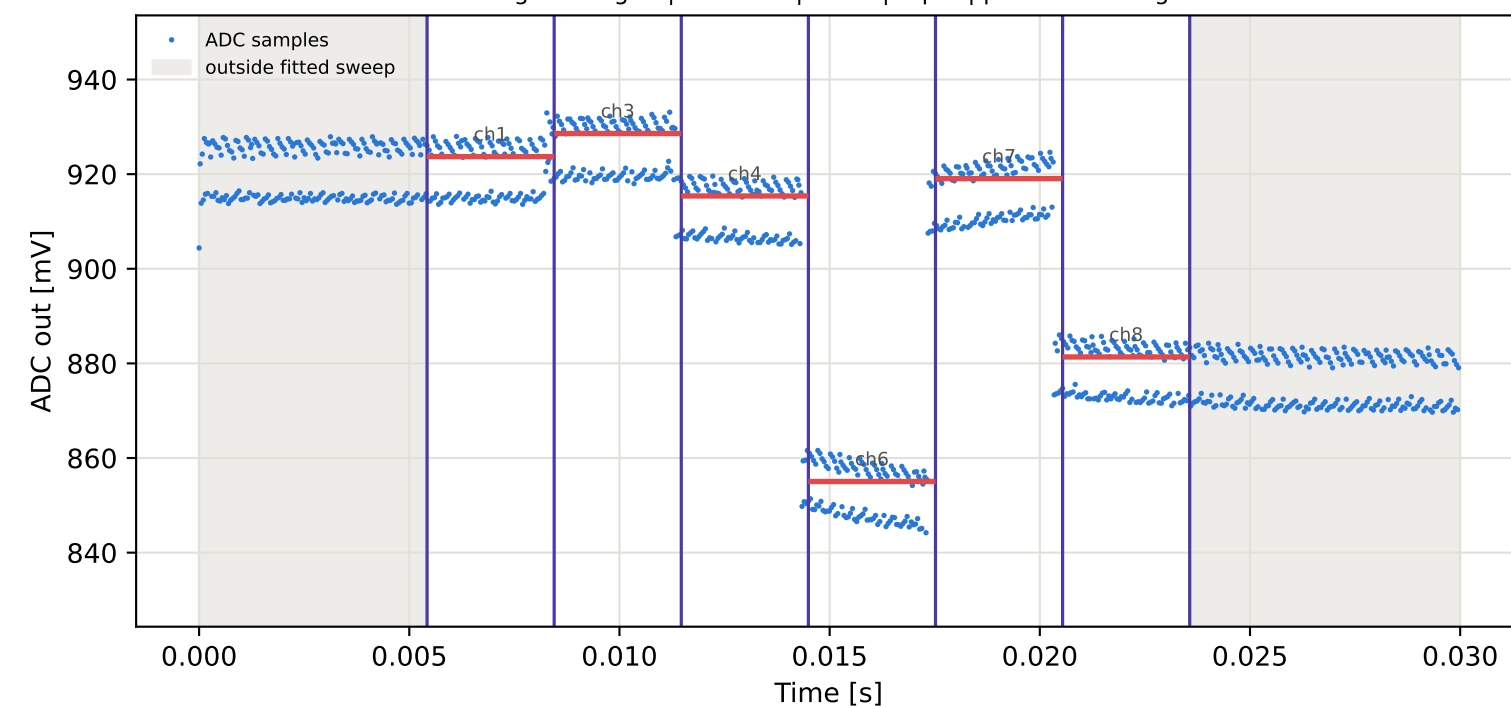
Tag1 &lt;- Tag3 | 905 MHz | run 0 | rep 1 | phase -31.54 deg
