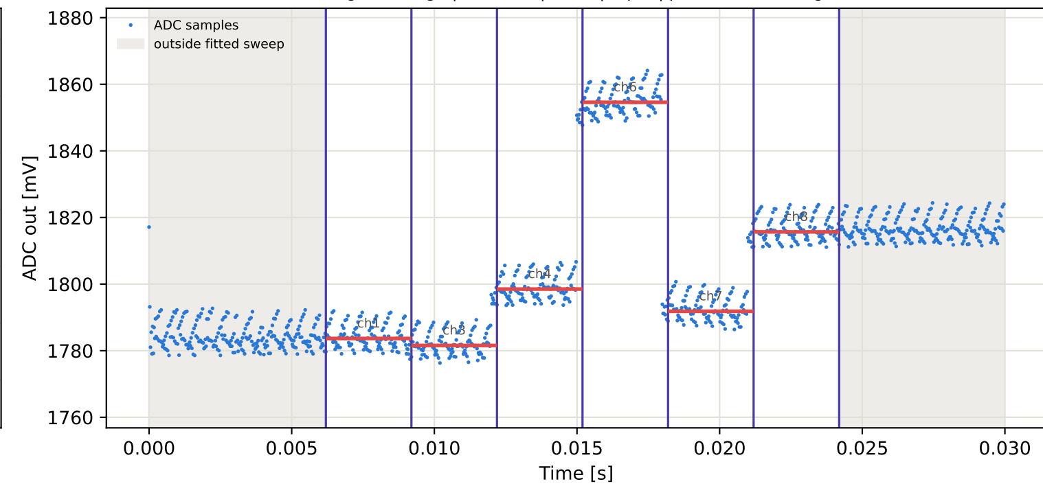
Tag16 &lt;- Tag1 | 915 MHz | run 0 | rep 1 | phase 42.53 deg
