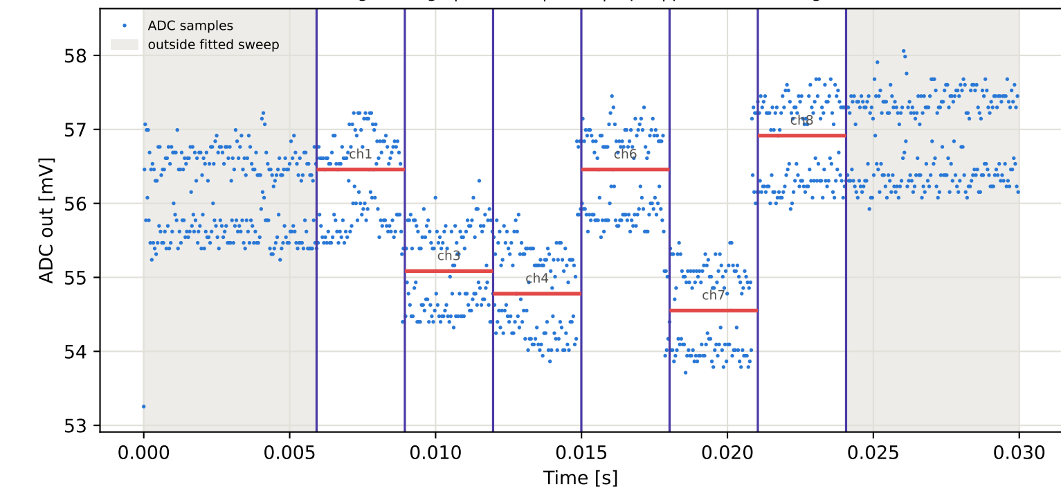
Tag6 &lt;- Tag4 | 795 MHz | run 0 | rep 1 | phase -22.09 deg
