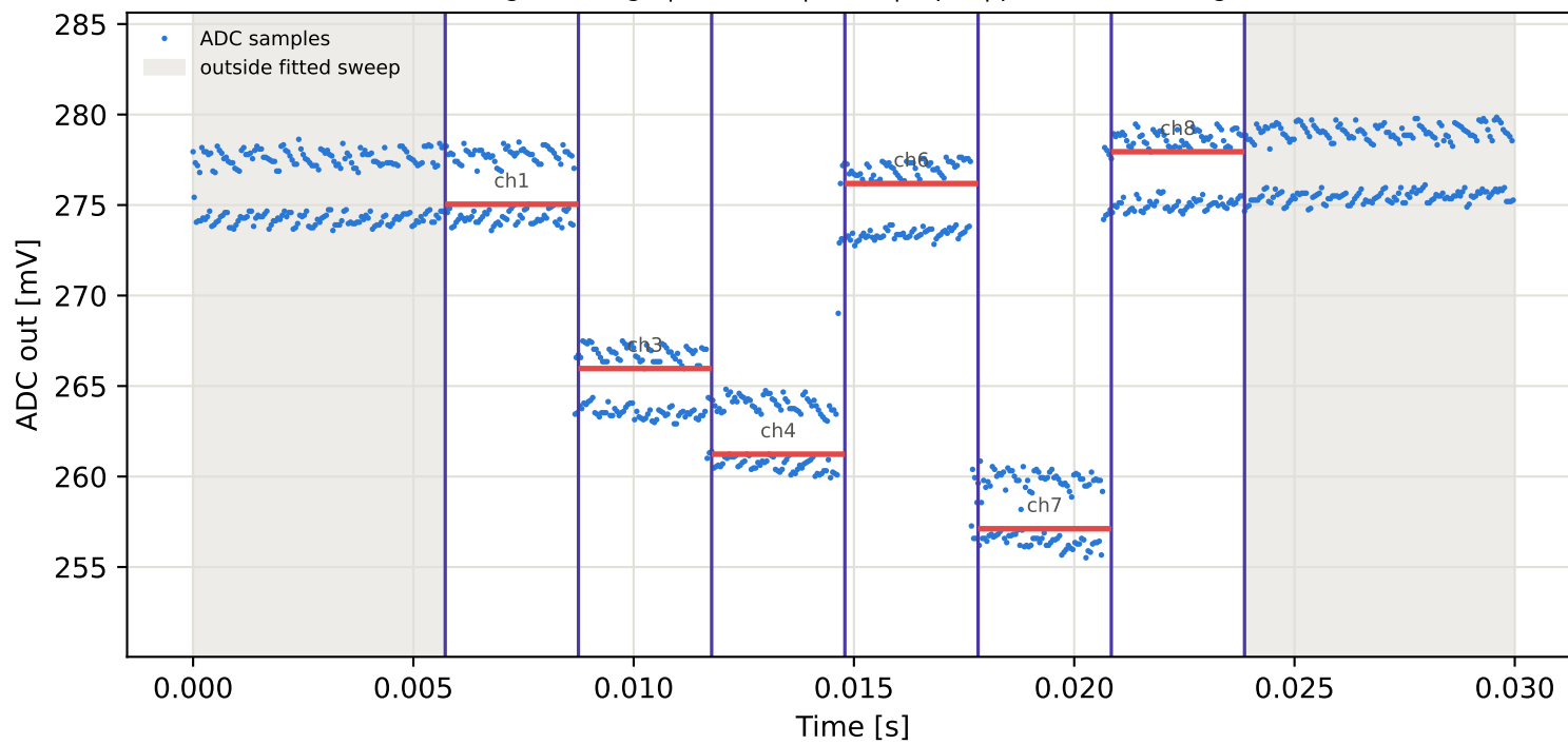
Tag2 &lt;- Tag1 | 795 MHz | run 0 | rep 1 | phase 153.47 deg
