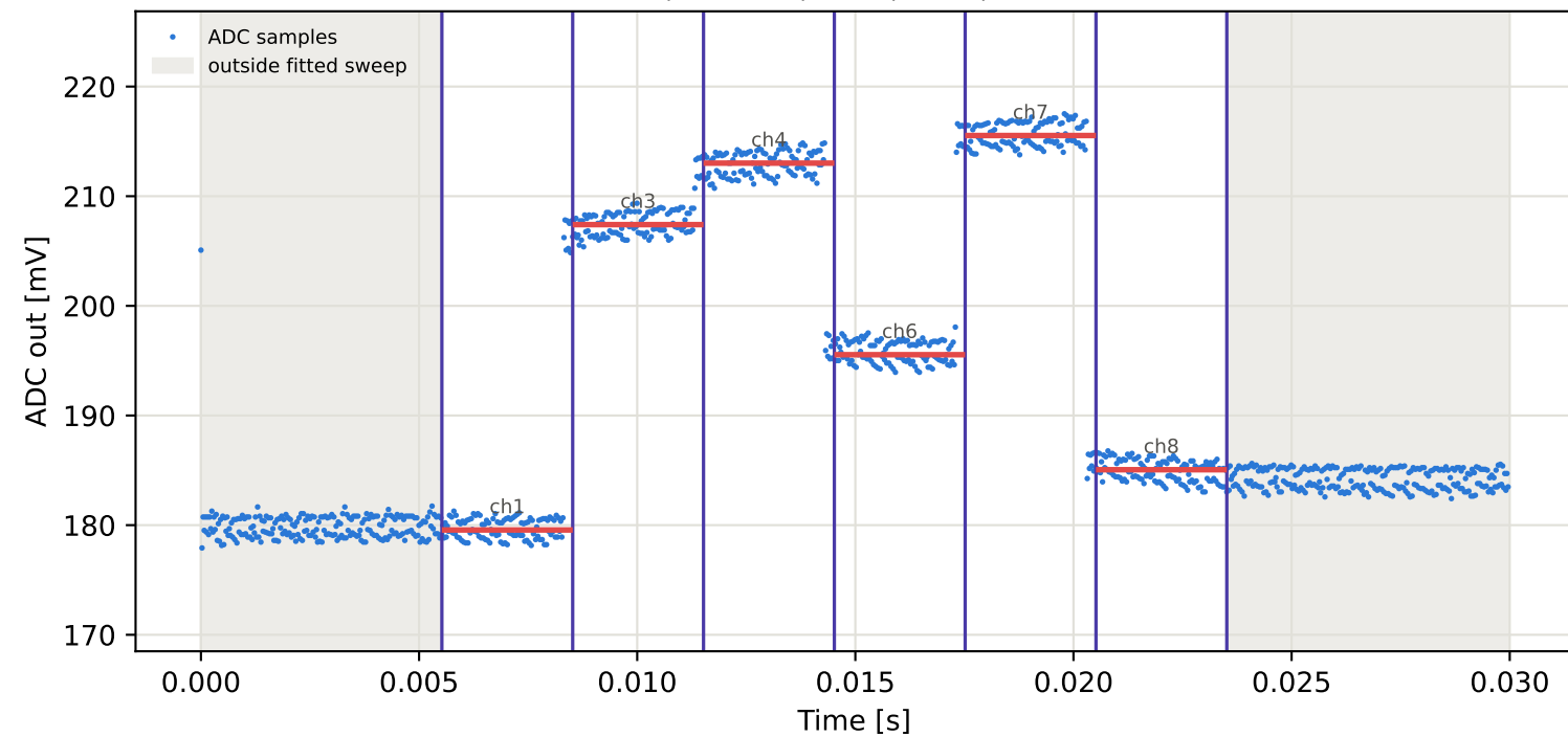
Tag4 &lt;- Tag3 | 835 MHz | run 0 | rep 1 | phase -70.69 deg
