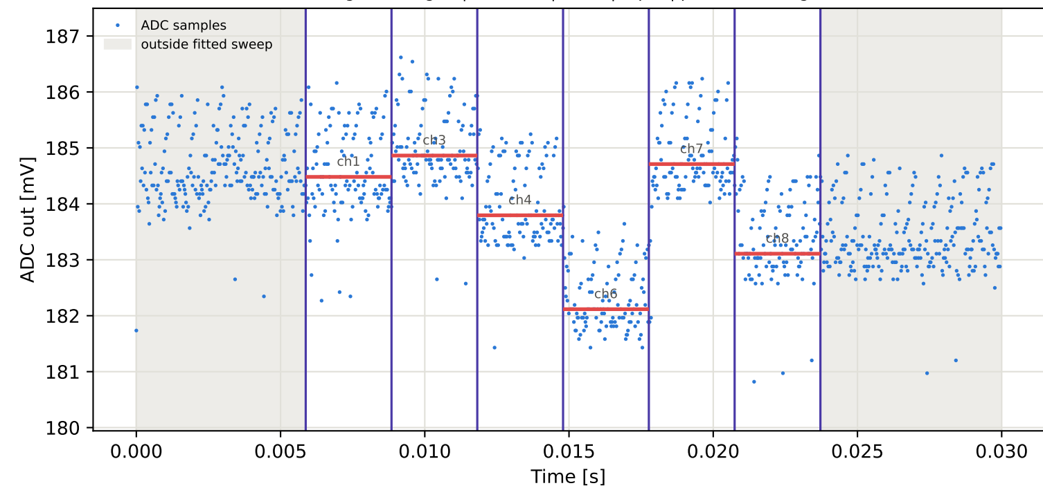
Tag10 &lt;- Tag3 | 995 MHz | run 0 | rep 1 | phase 7.34 deg
