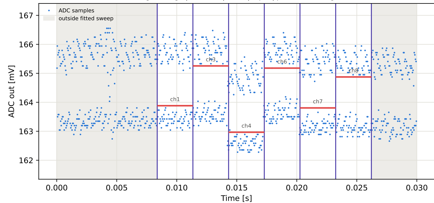
Tag7 &lt;- Tag4 | 995 MHz | run 0 | rep 1 | phase 133.96 deg
