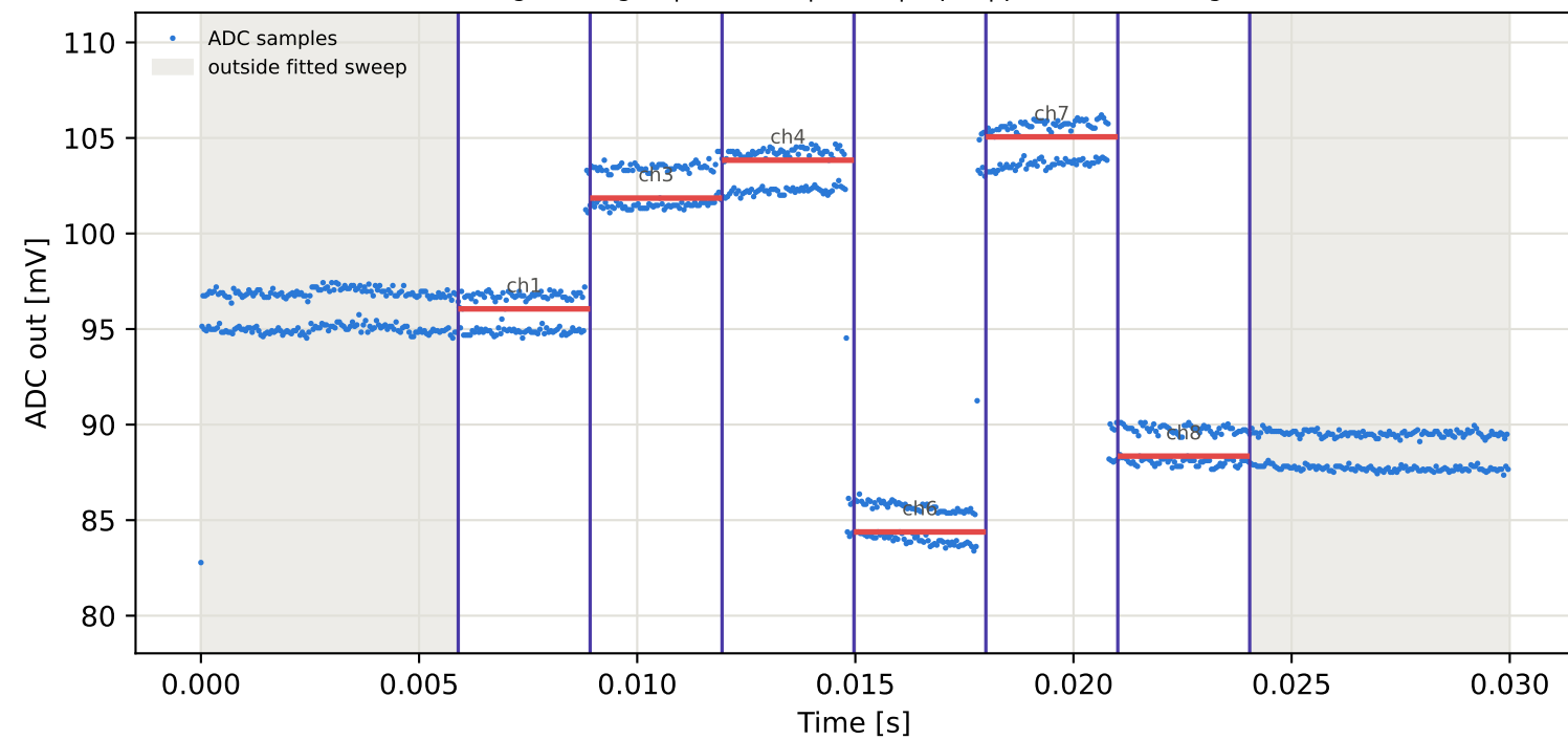
Tag6 &lt;- Tag3 | 995 MHz | run 0 | rep 1 | phase -111.24 deg
