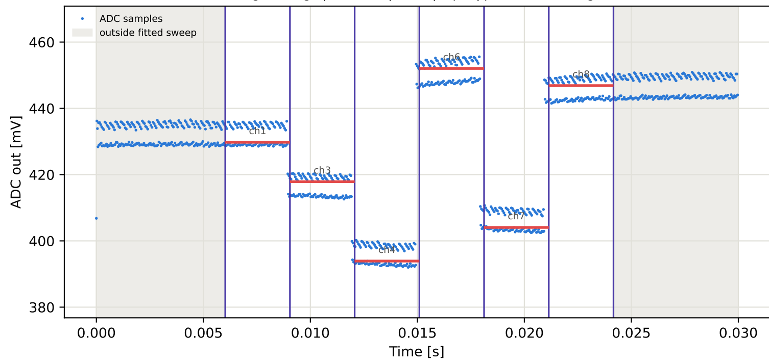
Tag3 &lt;- Tag15 | 985 MHz | run 0 | rep 1 | phase 32.10 deg
