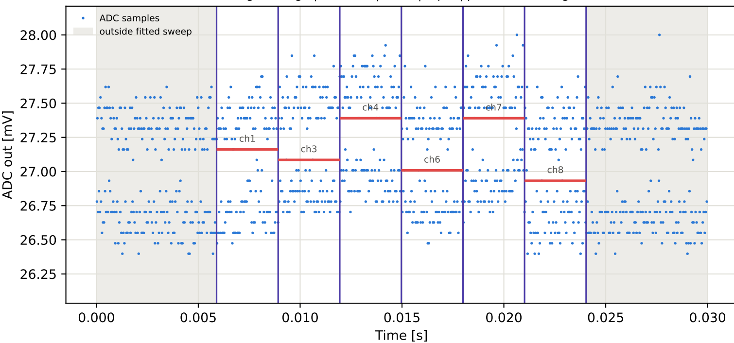
Tag2 &lt;- Tag7 | 805 MHz | run 0 | rep 1 | phase -57.31 deg
