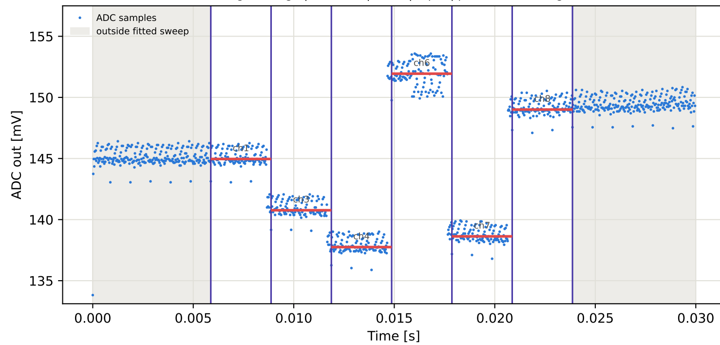
Tag1 &lt;- Tag7 | 995 MHz | run 0 | rep 1 | phase -117.31 deg
