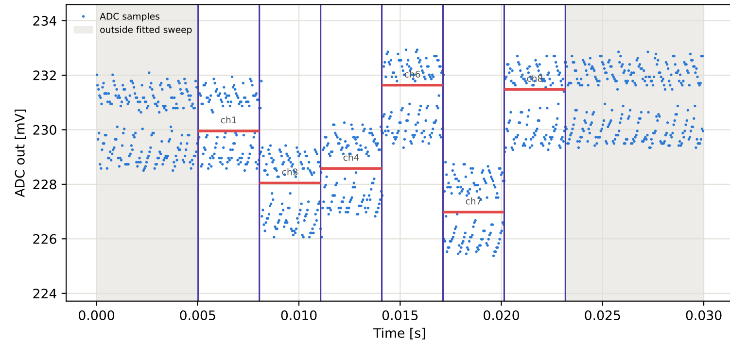
Tag16 &lt;- Tag10 | 775 MHz | run 0 | rep 1 | phase 109.27 deg
