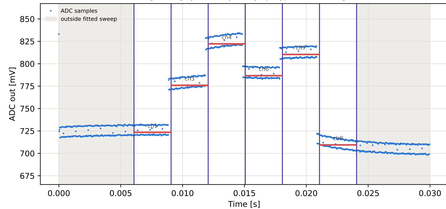
Tag4 &lt;- Tag7 | 895 MHz | run 0 | rep 1 | phase 39.13 deg
