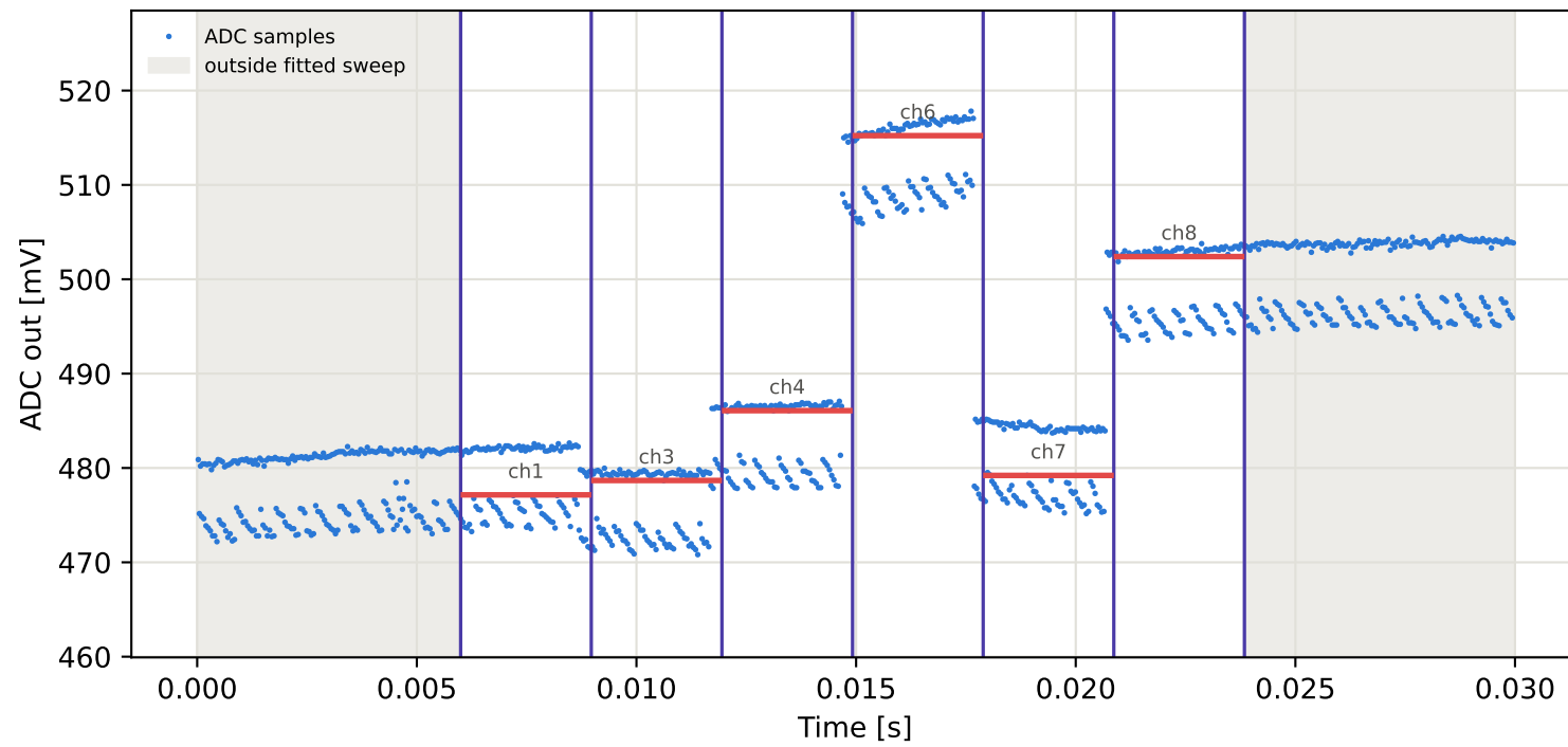
Tag8 &lt;- Tag1 | 905 MHz | run 0 | rep 1 | phase 164.24 deg
