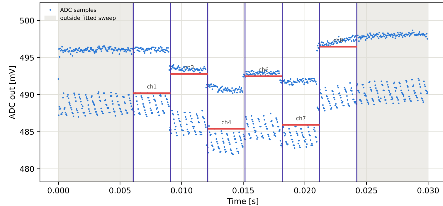
Tag7 &lt;- Tag5 | 905 MHz | run 0 | rep 1 | phase 61.29 deg
