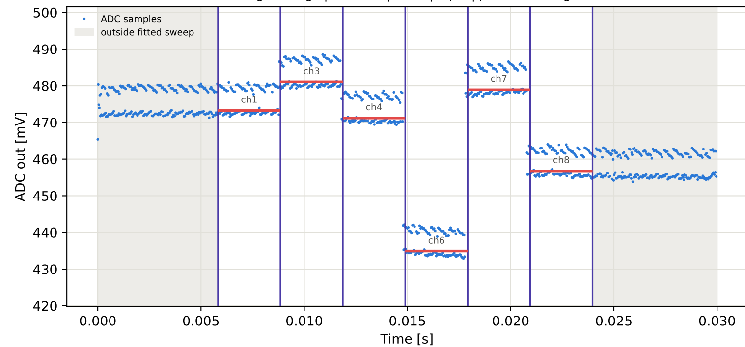
Tag4 &lt;- Tag7 | 975 MHz | run 0 | rep 1 | phase -109.16 deg
