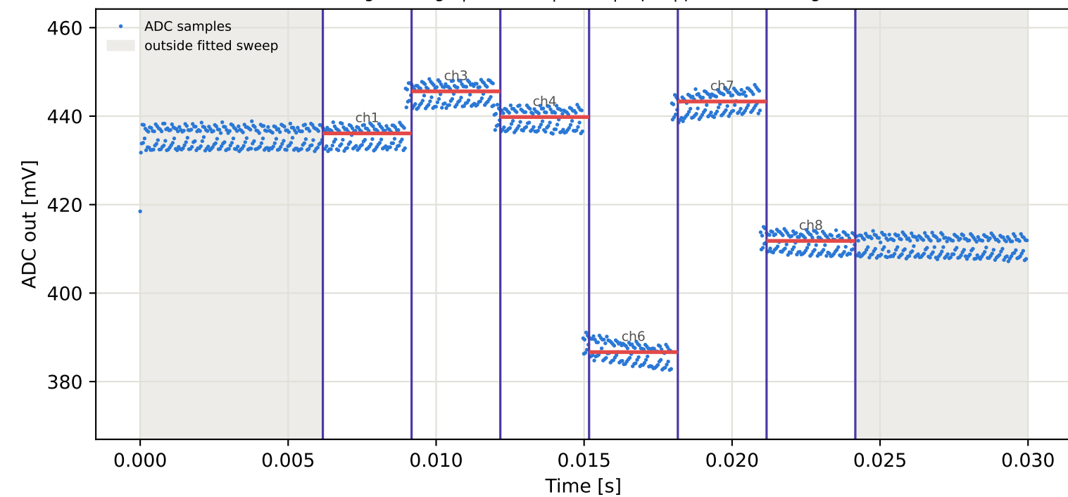
Tag1 &lt;- Tag9 | 935 MHz | run 0 | rep 1 | phase -2.21 deg
