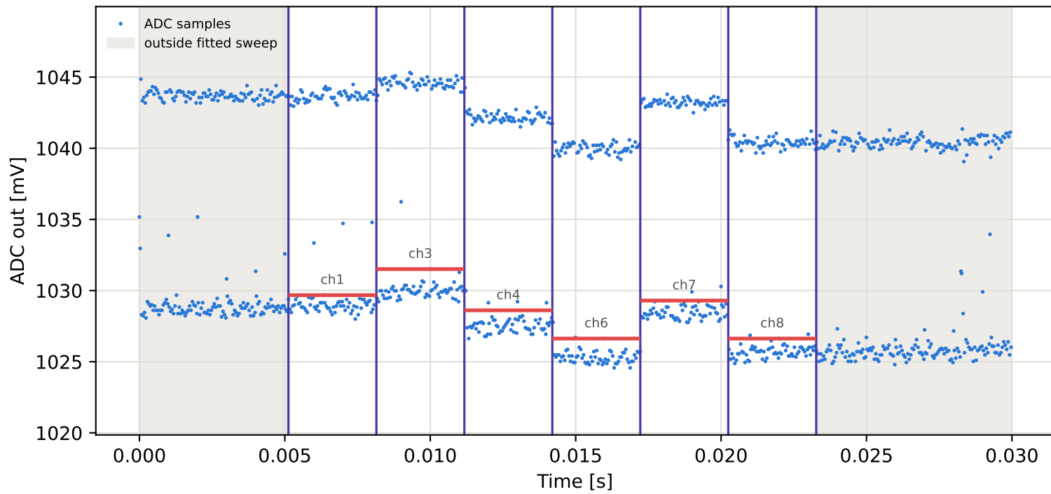
Tag8 &lt;- Tag16 | 855 MHz | run 0 | rep 1 | phase 137.05 deg
