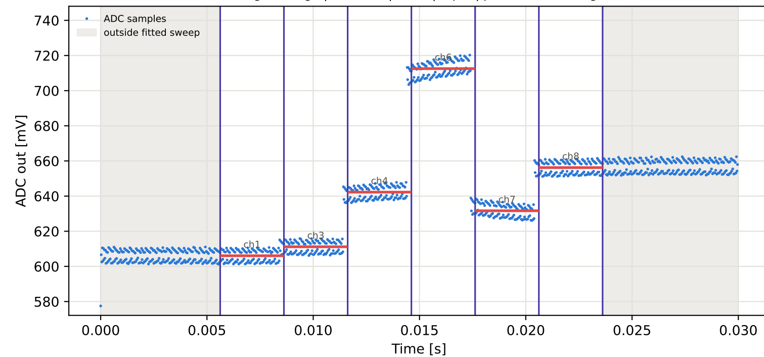
Tag3 &lt;- Tag8 | 905 MHz | run 0 | rep 1 | phase -82.58 deg
