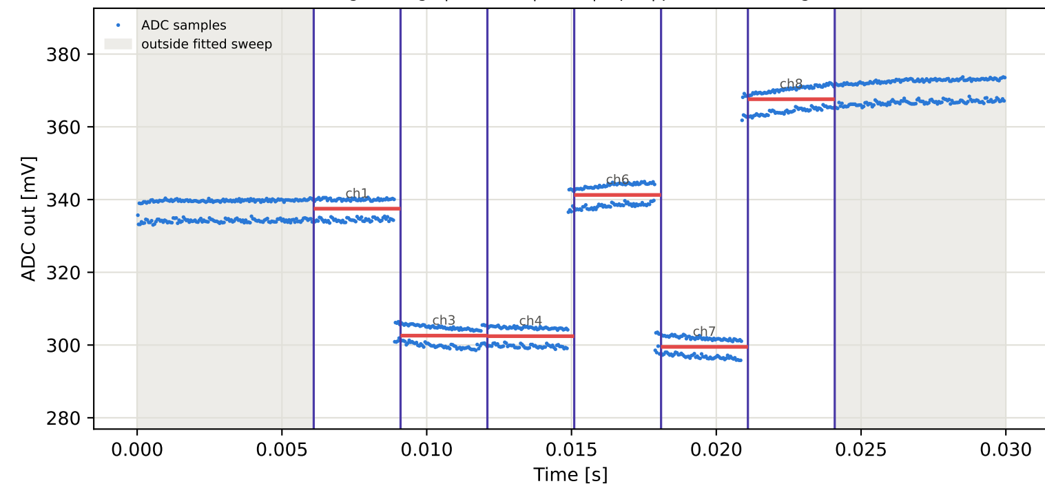
Tag4 &lt;- Tag7 | 865 MHz | run 0 | rep 1 | phase -81.35 deg
