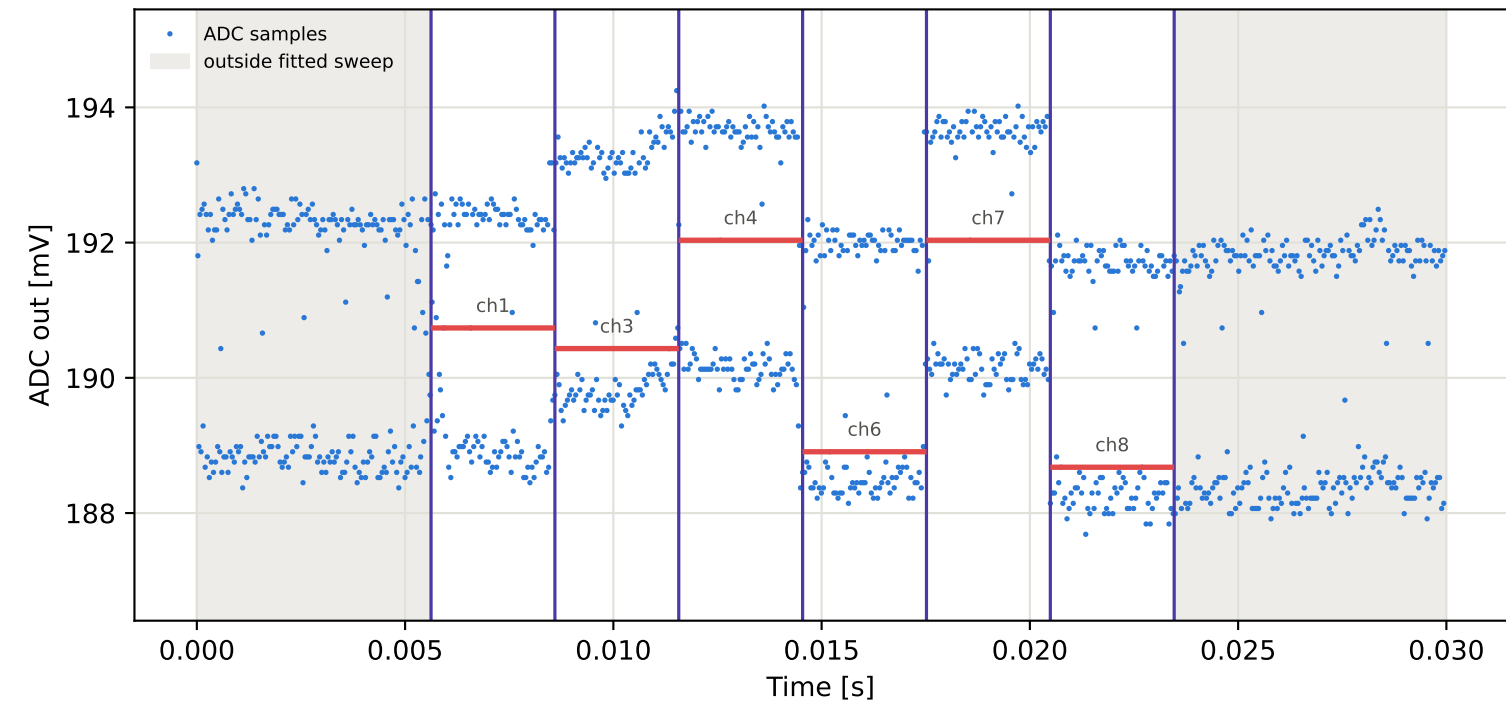
Tag5 &lt;- Tag4 | 775 MHz | run 0 | rep 1 | phase 15.44 deg
