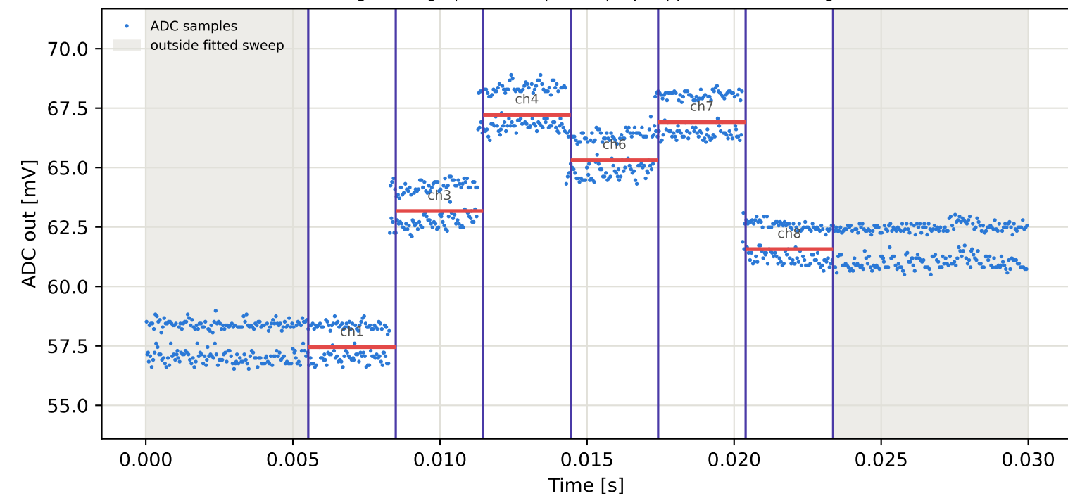
Tag2 &lt;- Tag7 | 845 MHz | run 0 | rep 1 | phase -68.36 deg
