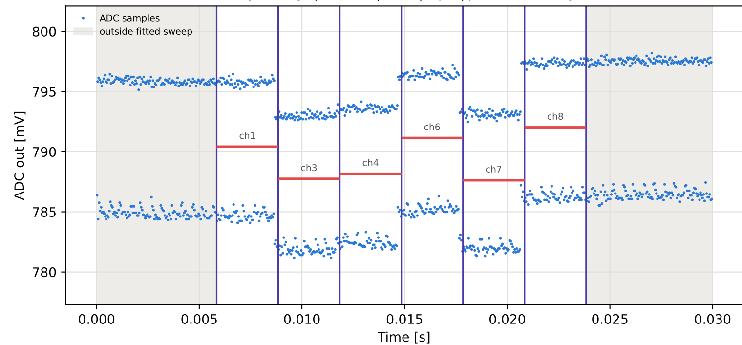
Tag6 &lt;- Tag10 | 865 MHz | run 0 | rep 1 | phase -149.36 deg
