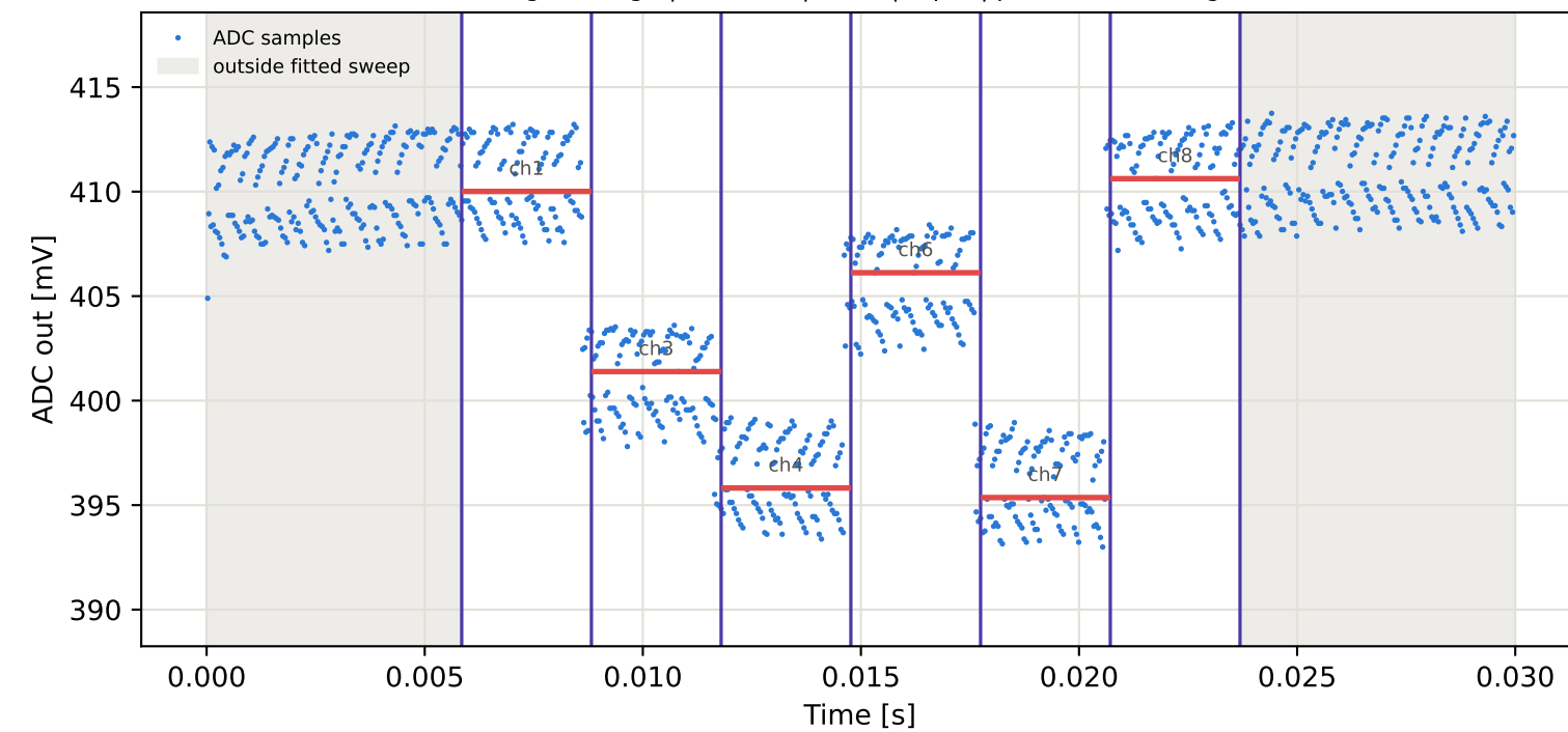
Tag6 &lt;- Tag9 | 855 MHz | run 0 | rep 1 | phase -117.45 deg
