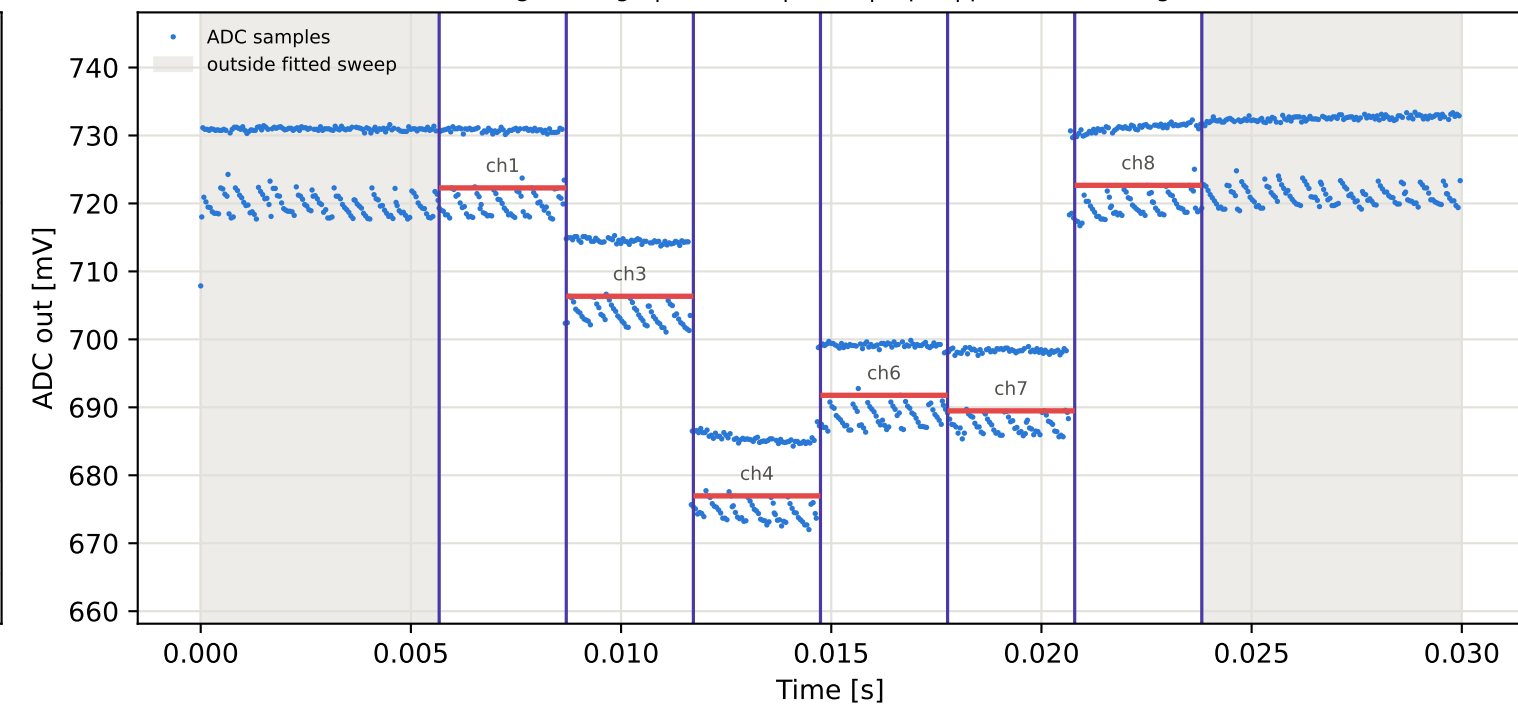
Tag7 &lt;- Tag6 | 935 MHz | run 0 | rep 1 | phase 171.97 deg
