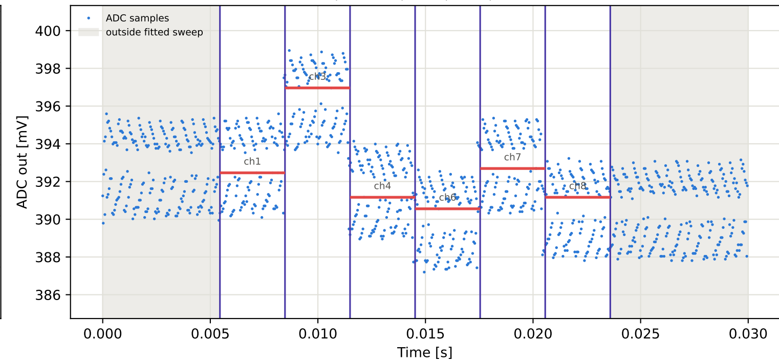
Tag5 &lt;- Tag1 | 835 MHz | run 0 | rep 1 | phase 32.43 deg
