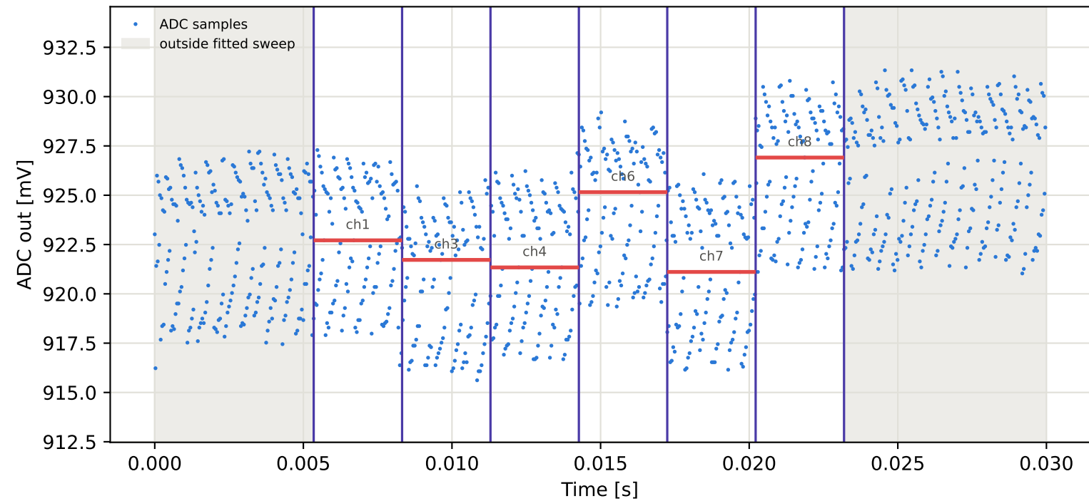
Tag16 &lt;- Tag15 | 875 MHz | run 0 | rep 1 | phase 77.54 deg
