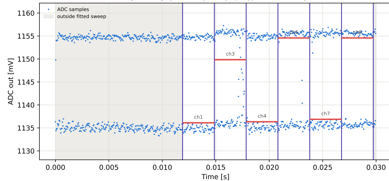
Tag16 &lt;- Tag4 | 955 MHz | run 0 | rep 1 | phase -5.63 deg
