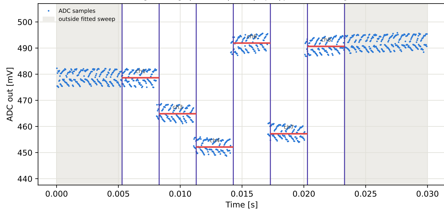
Tag10 &lt;- Tag9 | 945 MHz | run 0 | rep 1 | phase -75.84 deg
