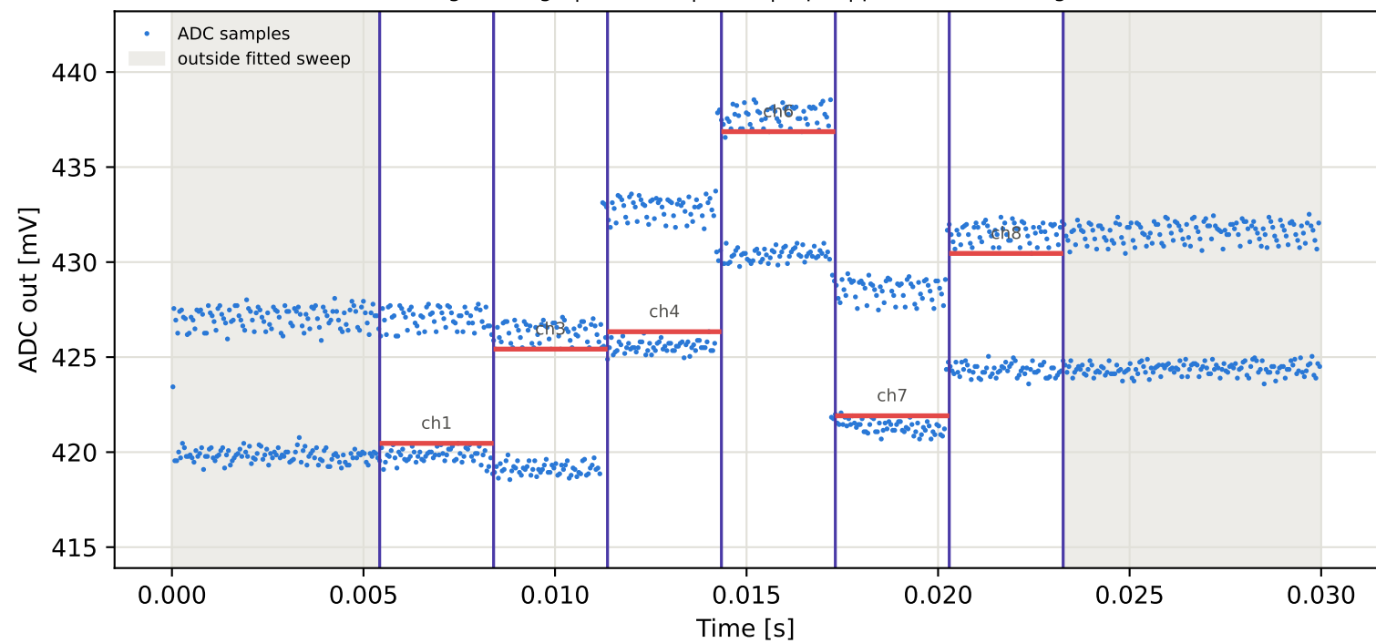
Tag3 &lt;- Tag9 | 965 MHz | run 0 | rep 1 | phase -174.13 deg
