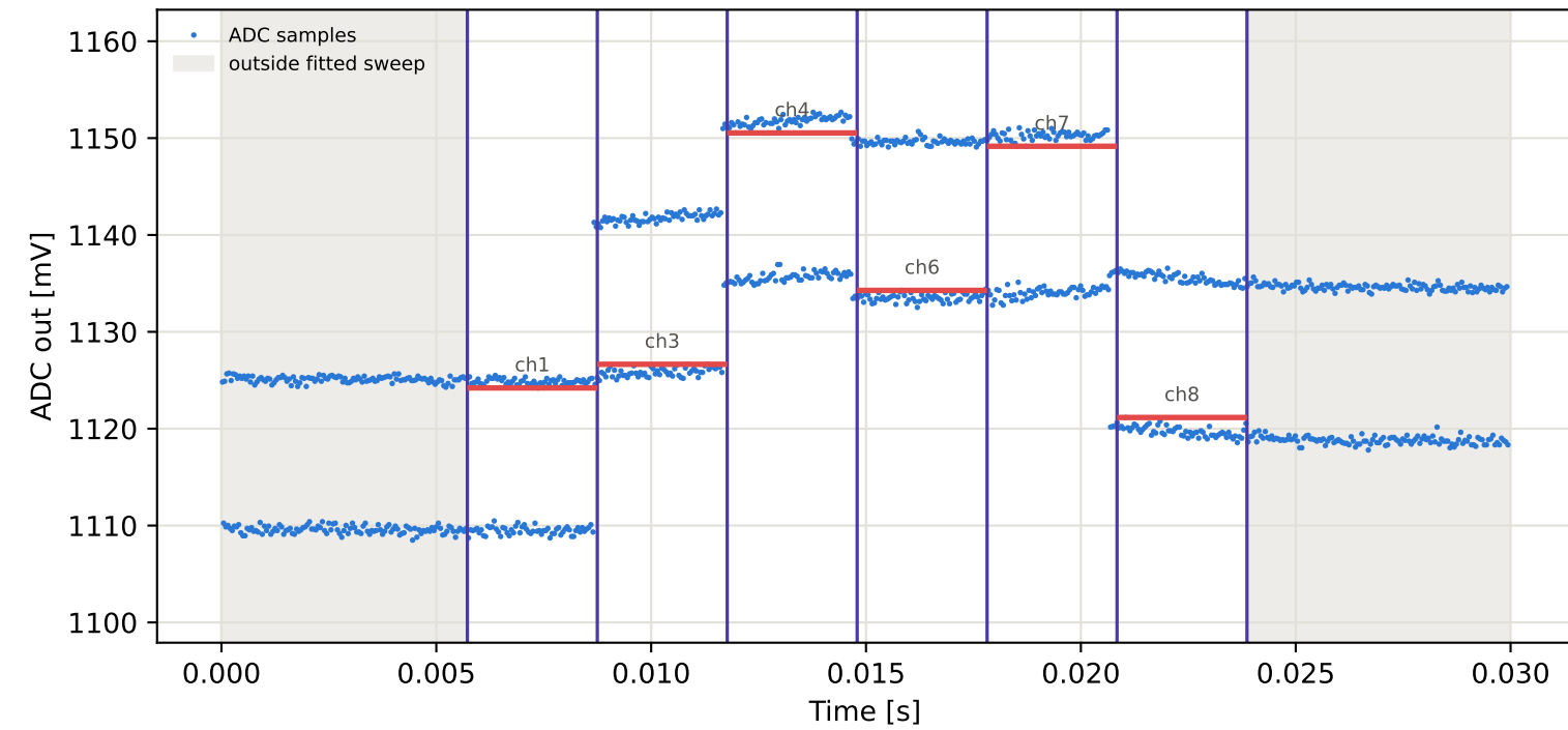
Tag3 &lt;- Tag2 | 875 MHz | run 0 | rep 1 | phase 52.22 deg
