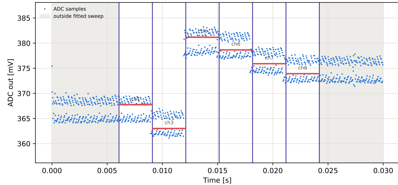
Tag3 &lt;- Tag2 | 835 MHz | run 0 | rep 1 | phase 107.41 deg
