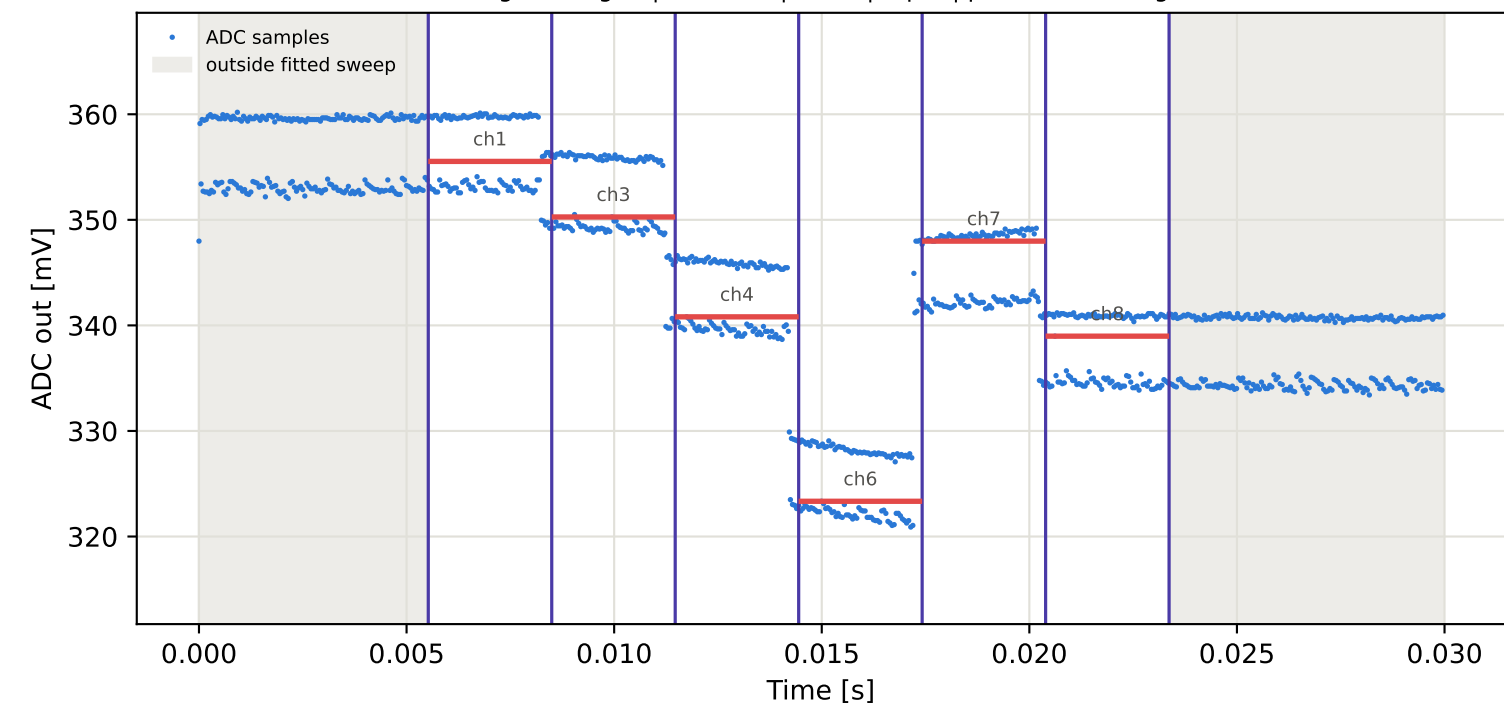
Tag2 &lt;- Tag16 | 895 MHz | run 0 | rep 1 | phase 26.87 deg
