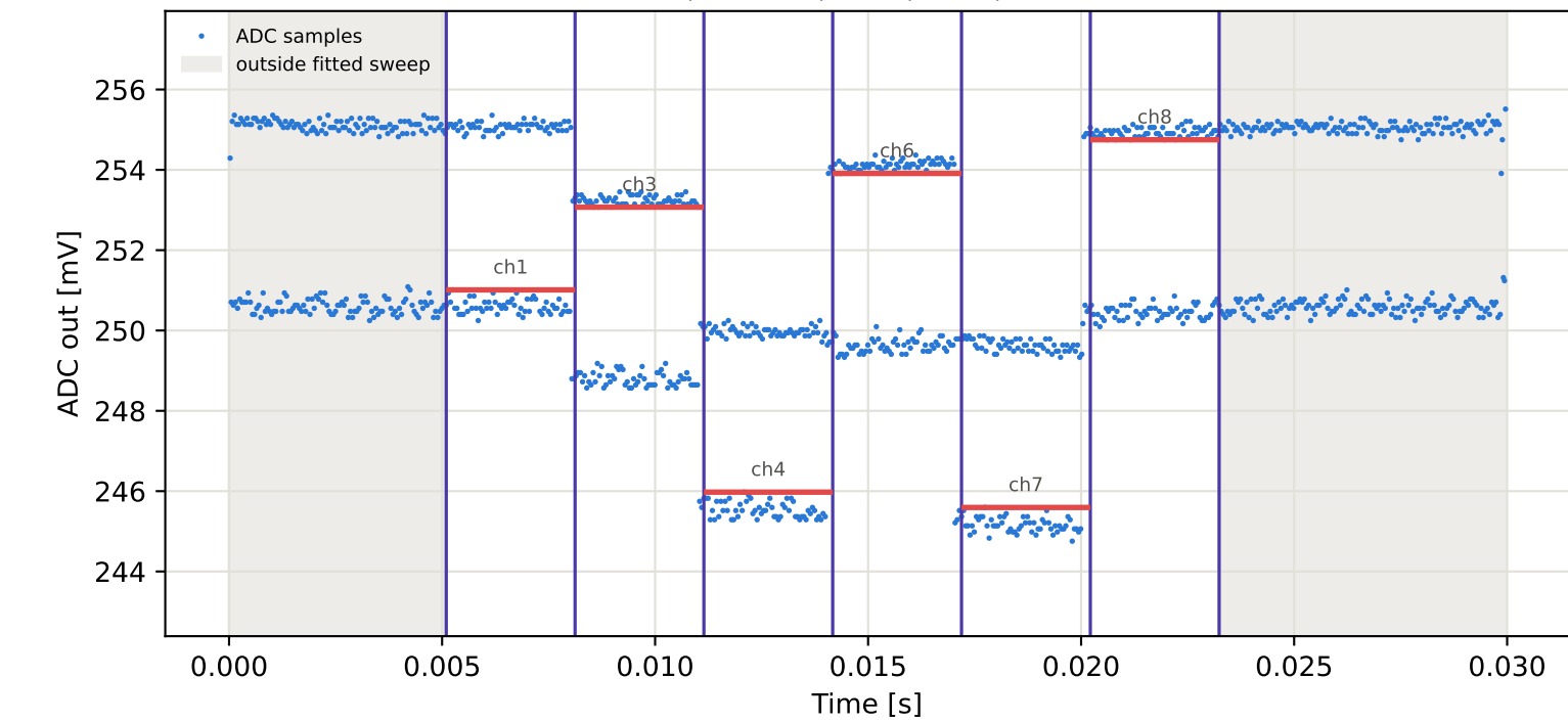
Tag15 &lt;- Tag5 | 785 MHz | run 0 | rep 1 | phase 121.02 deg
