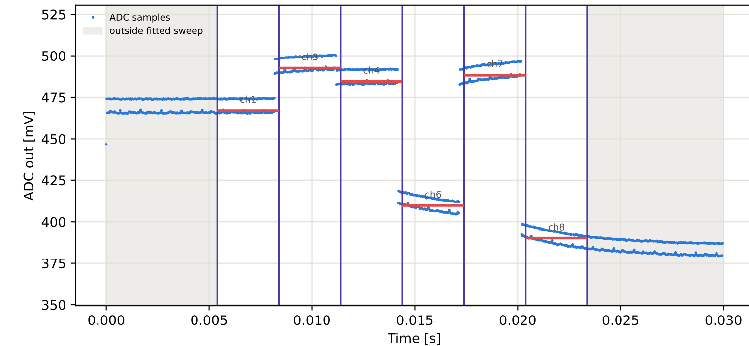
Tag9 &lt;- Tag16 | 895 MHz | run 0 | rep 1 | phase -18.03 deg
