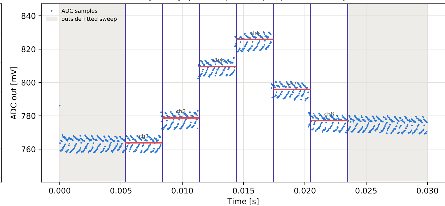
Tag5 &lt;- Tag4 | 925 MHz | run 0 | rep 1 | phase -133.44 deg
