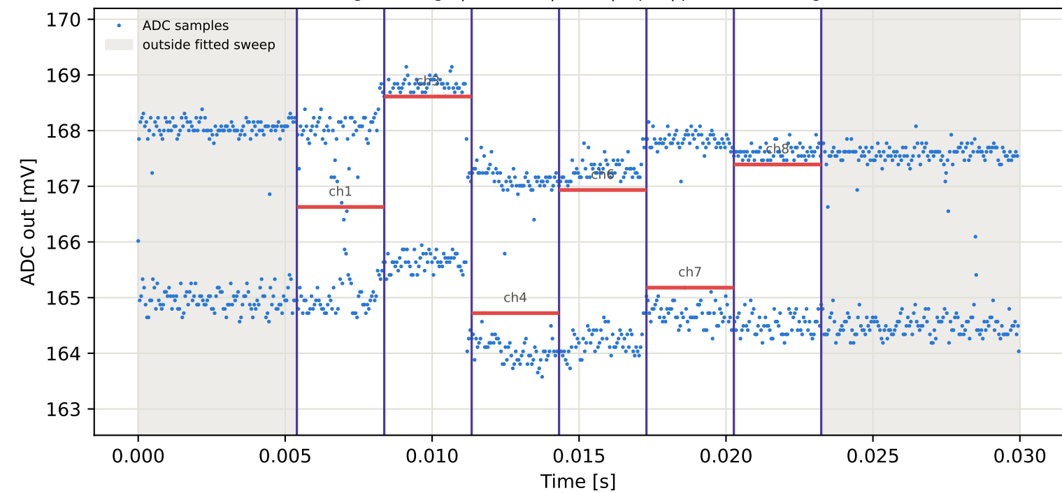
Tag16 &lt;- Tag5 | 785 MHz | run 0 | rep 1 | phase 8.29 deg
