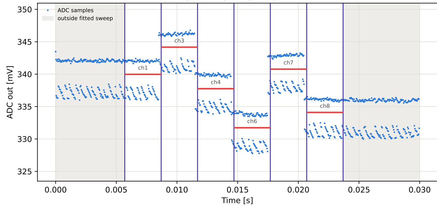
Tag9 &lt;- Tag7 | 835 MHz | run 0 | rep 1 | phase 19.56 deg
