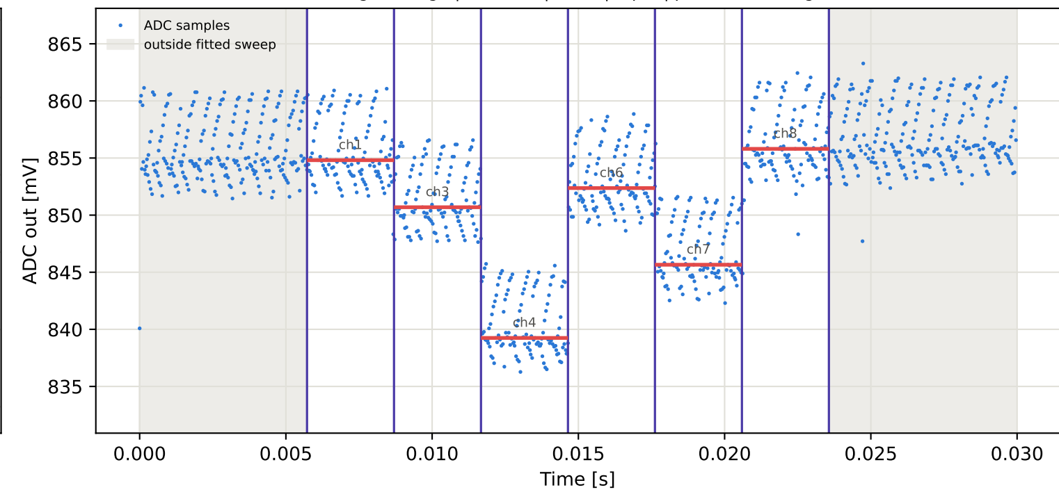
Tag8 &lt;- Tag5 | 975 MHz | run 0 | rep 1 | phase 86.76 deg
