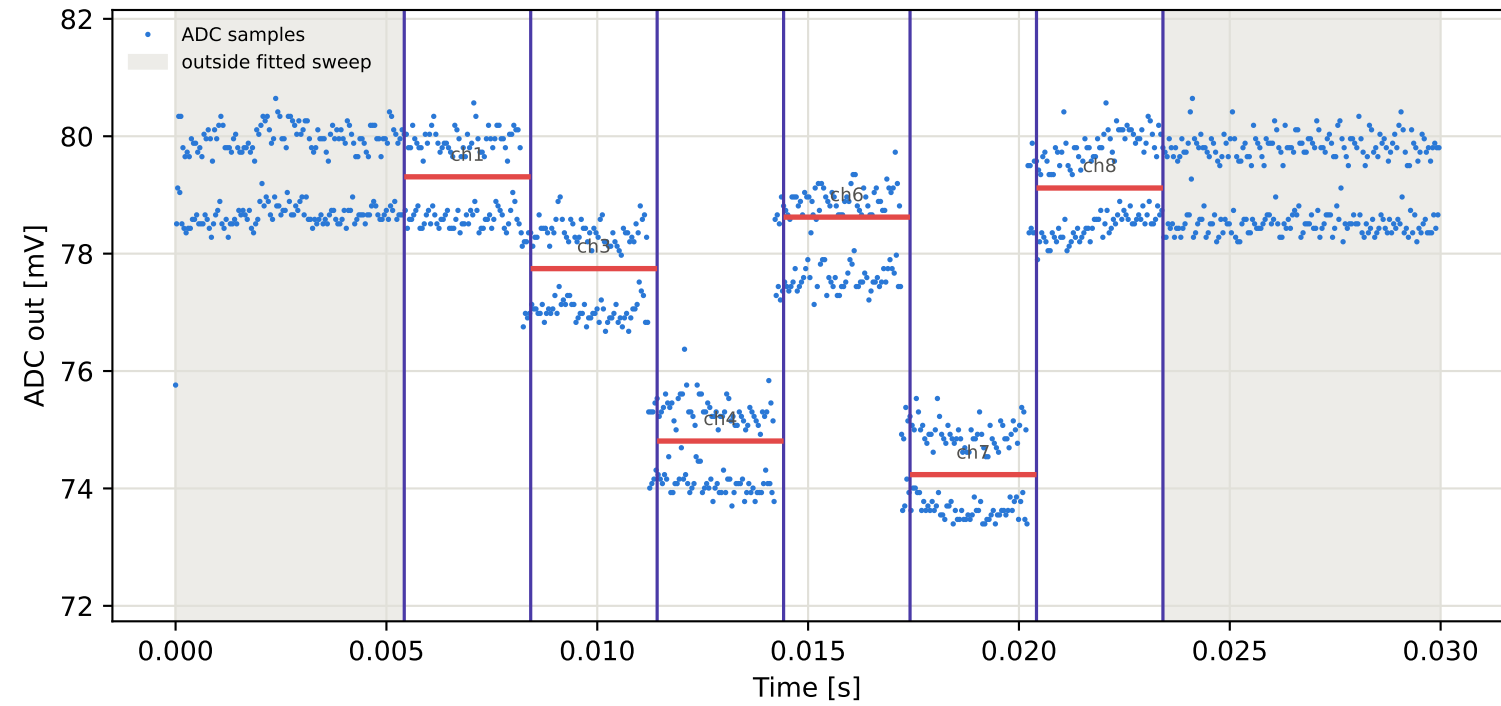
Tag3 &lt;- Tag15 | 795 MHz | run 0 | rep 1 | phase 165.41 deg
