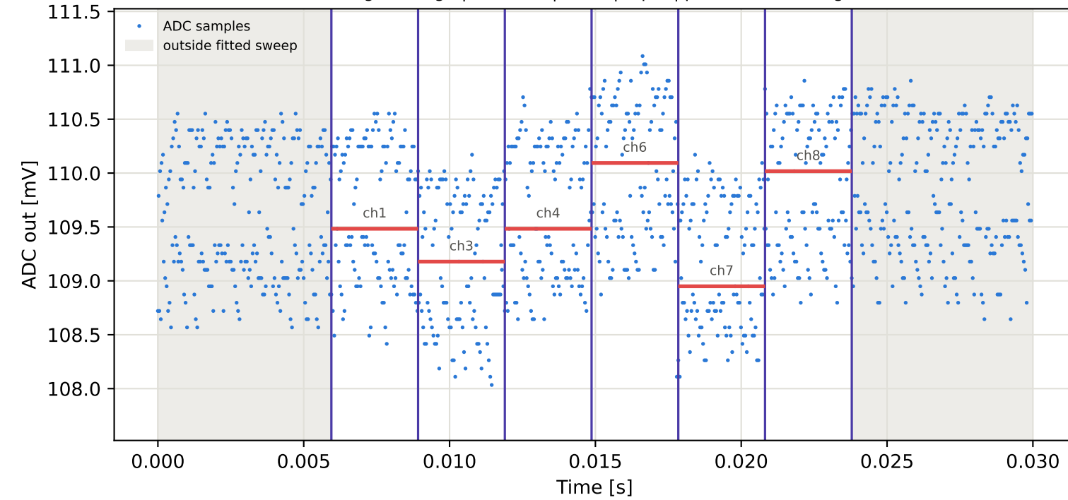
Tag8 &lt;- Tag15 | 775 MHz | run 0 | rep 1 | phase 78.95 deg
