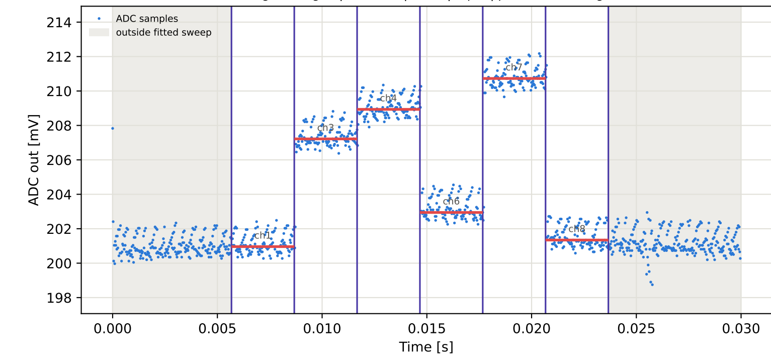
Tag9 &lt;- Tag16 | 805 MHz | run 0 | rep 1 | phase 114.63 deg
