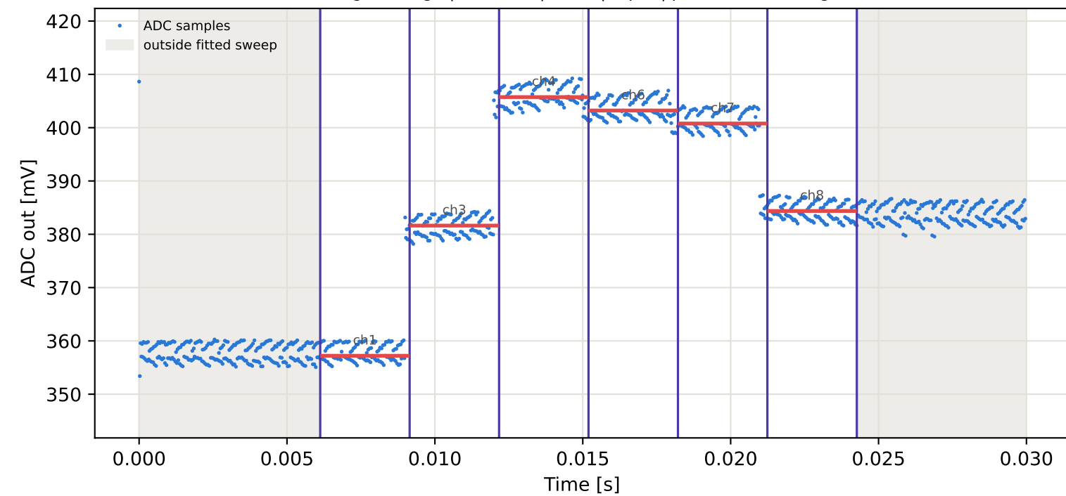
Tag7 &lt;- Tag1 | 855 MHz | run 0 | rep 1 | phase -142.93 deg
