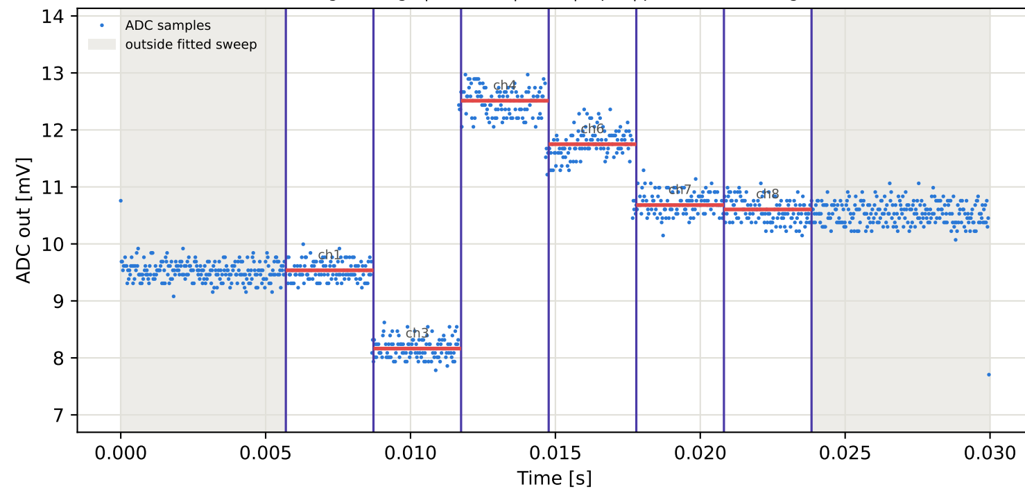
Tag2 &lt;- Tag5 | 775 MHz | run 0 | rep 1 | phase 48.96 deg
