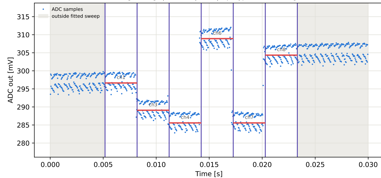
Tag5 &lt;- Tag8 | 985 MHz | run 0 | rep 1 | phase 175.66 deg
