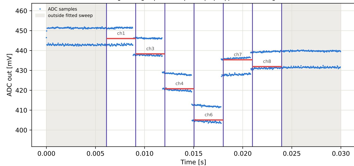
Tag1 &lt;- Tag2 | 935 MHz | run 0 | rep 1 | phase 135.96 deg
