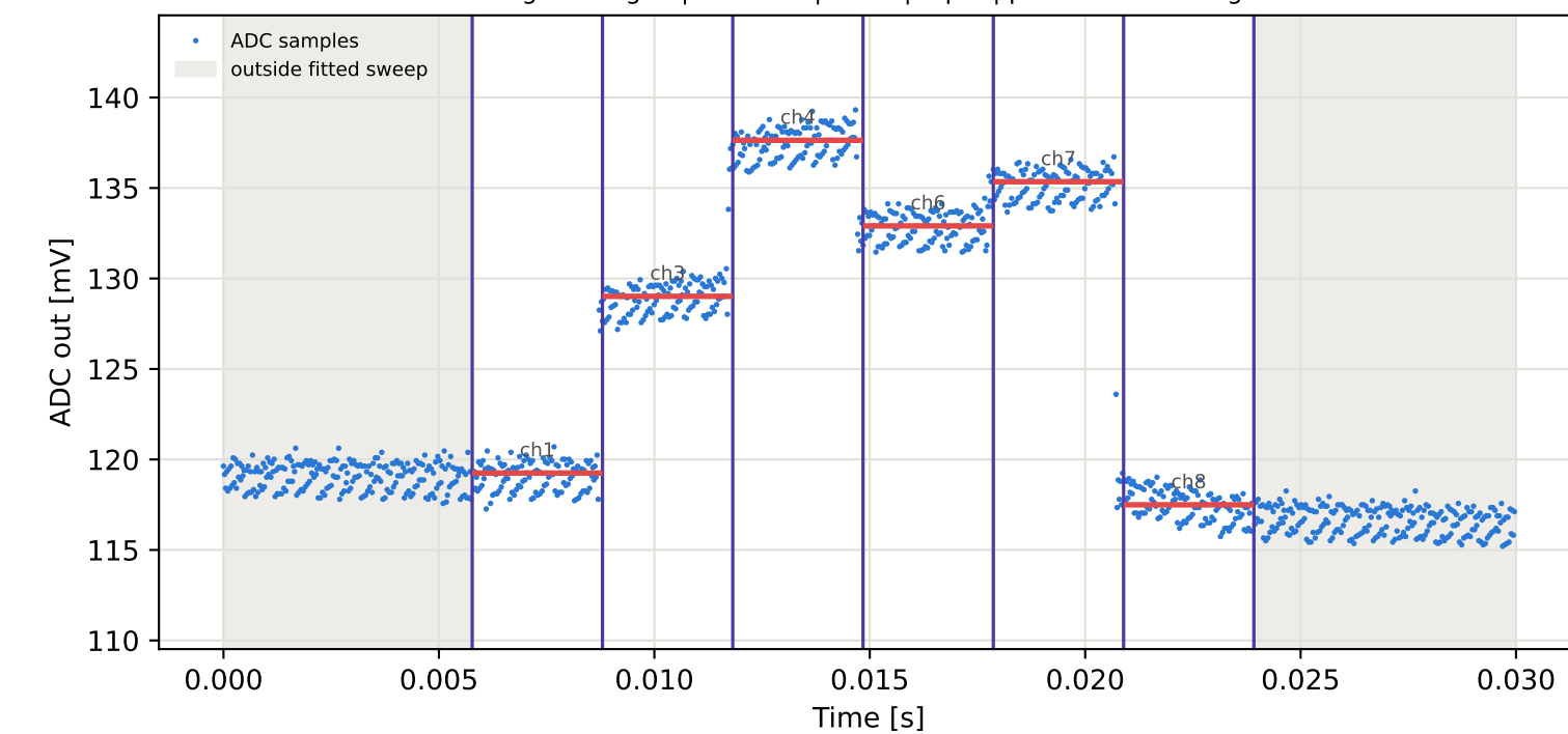
Tag2 &lt;- Tag15 | 905 MHz | run 0 | rep 1 | phase -100.00 deg
