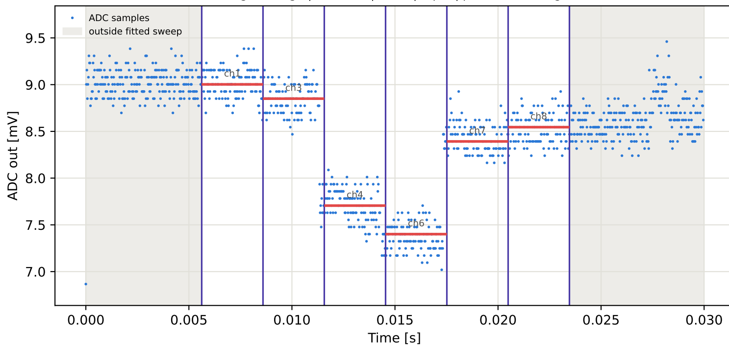
Tag3 &lt;- Tag10 | 955 MHz | run 0 | rep 1 | phase 160.91 deg
