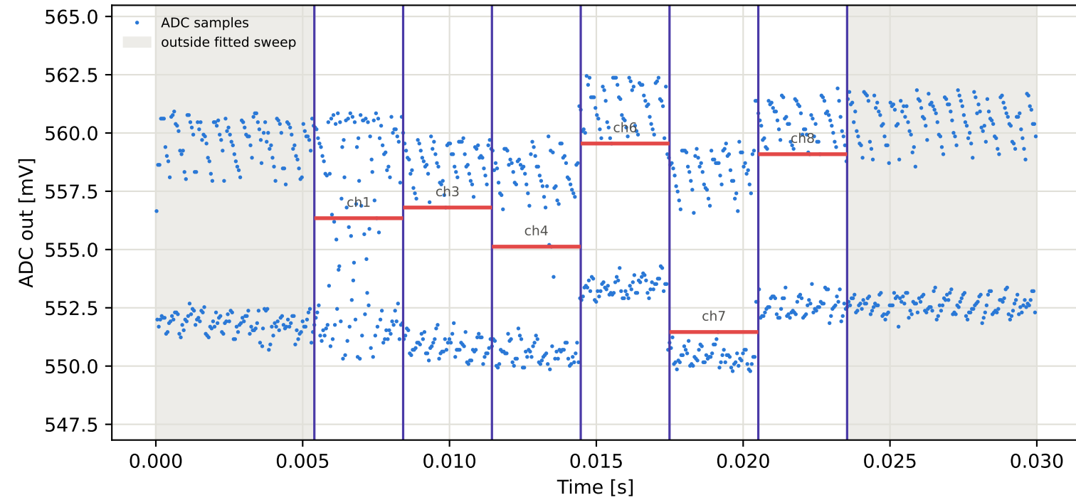
Tag8 &lt;- Tag16 | 995 MHz | run 0 | rep 1 | phase -70.39 deg
