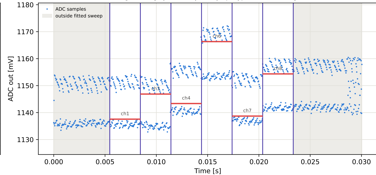
Tag16 &lt;- Tag5 | 955 MHz | run 0 | rep 1 | phase 18.34 deg
