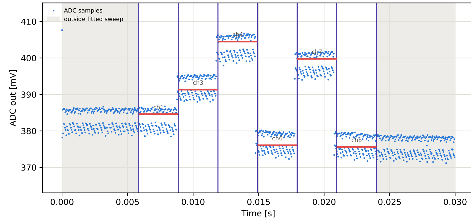
Tag3 &lt;- Tag8 | 955 MHz | run 0 | rep 1 | phase -28.85 deg
