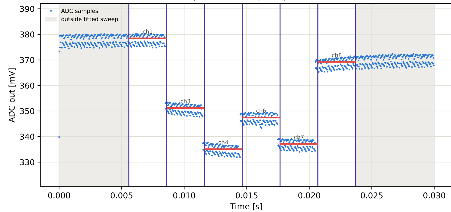
Tag1 &lt;- Tag8 | 865 MHz | run 0 | rep 1 | phase -123.45 deg
