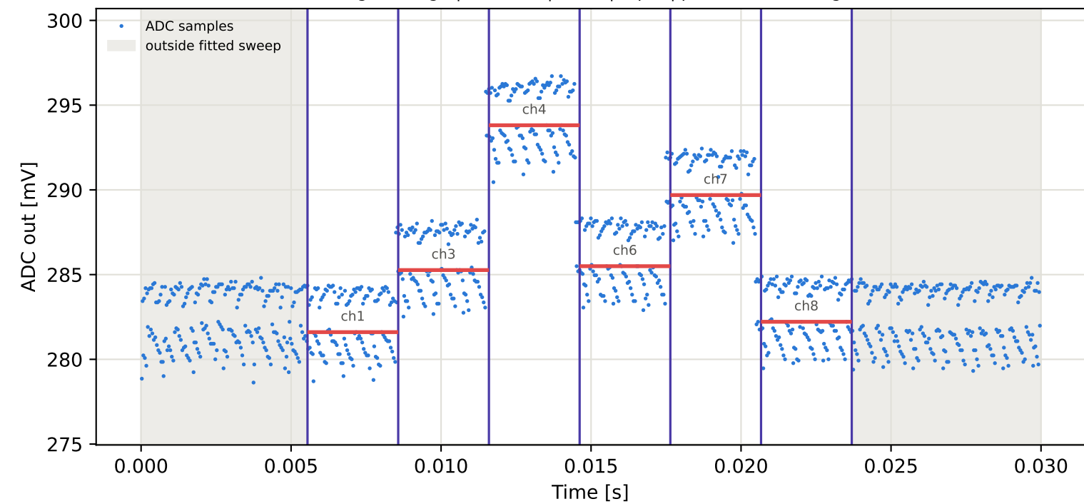
Tag5 &lt;- Tag9 | 985 MHz | run 0 | rep 1 | phase -42.22 deg
