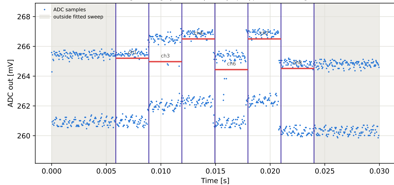
Tag15 &lt;- Tag4 | 795 MHz | run 0 | rep 1 | phase -178.41 deg
