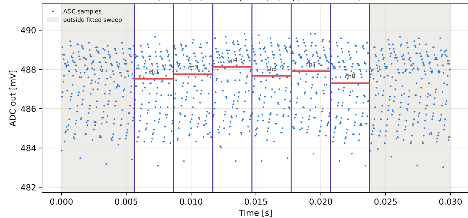
Tag6 &lt;- Tag4 | 865 MHz | run 0 | rep 1 | phase 39.67 deg
