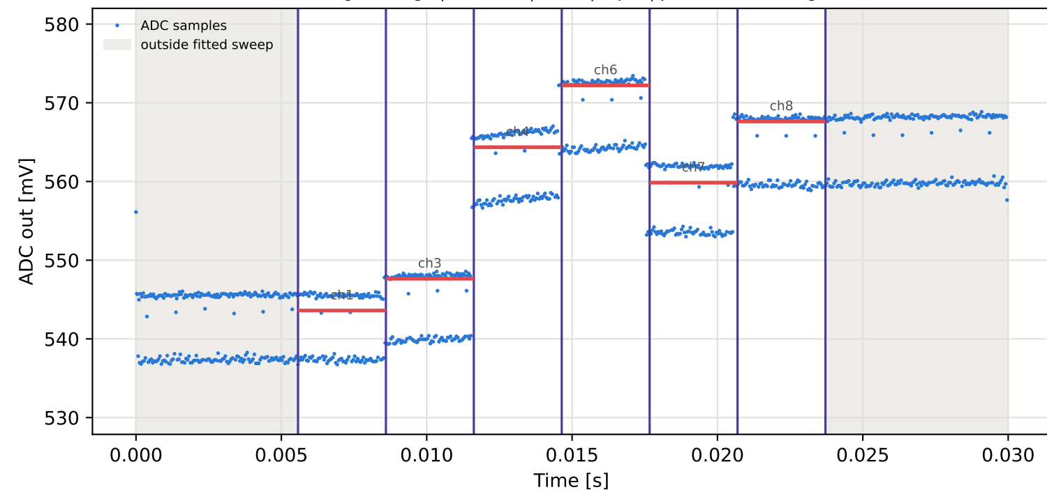
Tag3 &lt;- Tag15 | 855 MHz | run 0 | rep 1 | phase -96.61 deg
