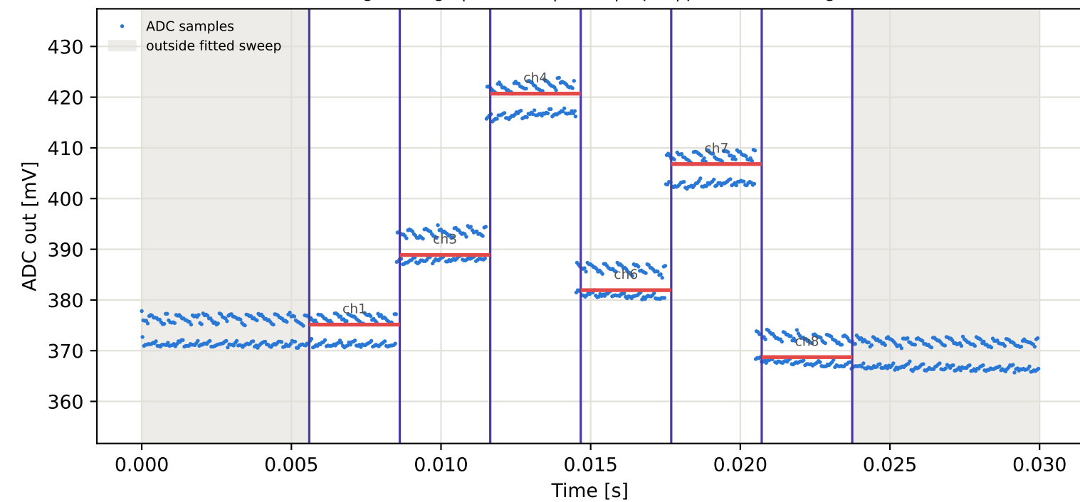
Tag7 &lt;- Tag10 | 965 MHz | run 0 | rep 1 | phase 132.70 deg
