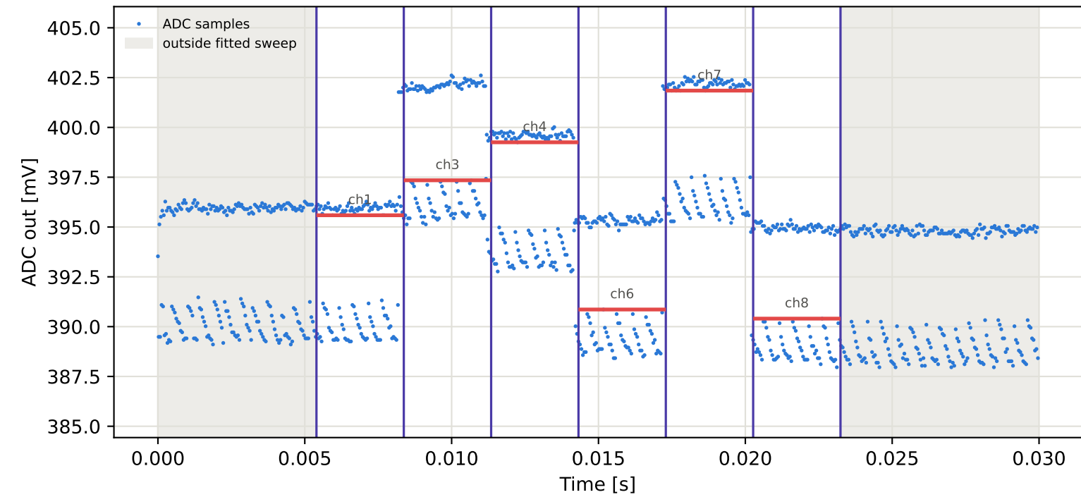
Tag16 &lt;- Tag6 | 805 MHz | run 0 | rep 1 | phase -62.29 deg
