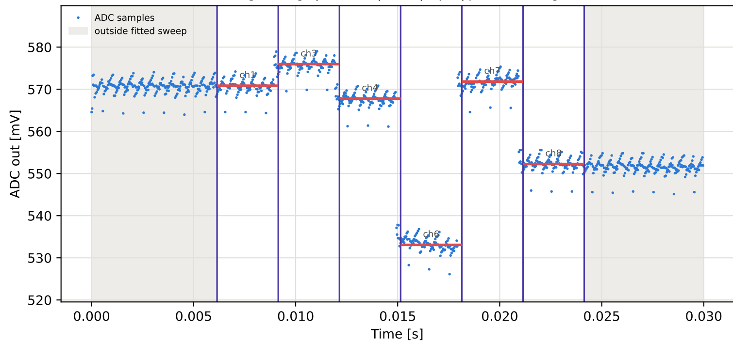
Tag9 &lt;- Tag15 | 925 MHz | run 0 | rep 1 | phase -117.34 deg
