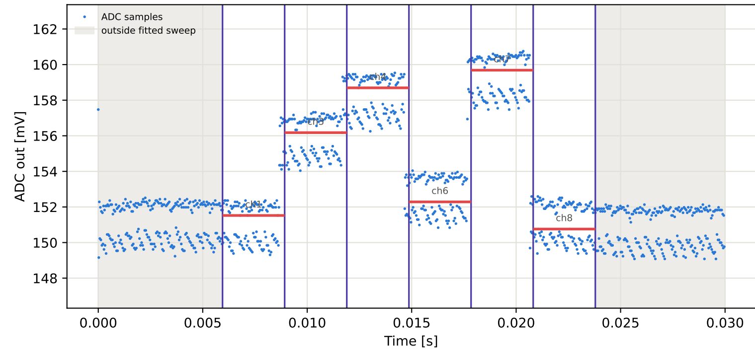
Tag6 &lt;- Tag10 | 795 MHz | run 0 | rep 1 | phase 144.13 deg
