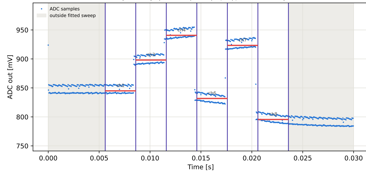
Tag2 &lt;- Tag1 | 925 MHz | run 0 | rep 1 | phase -150.89 deg
