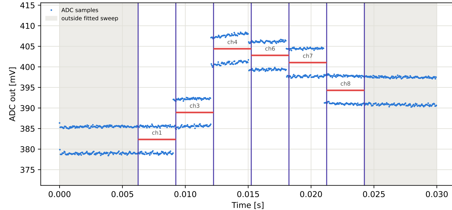
Tag7 &lt;- Tag10 | 855 MHz | run 0 | rep 1 | phase -173.51 deg
