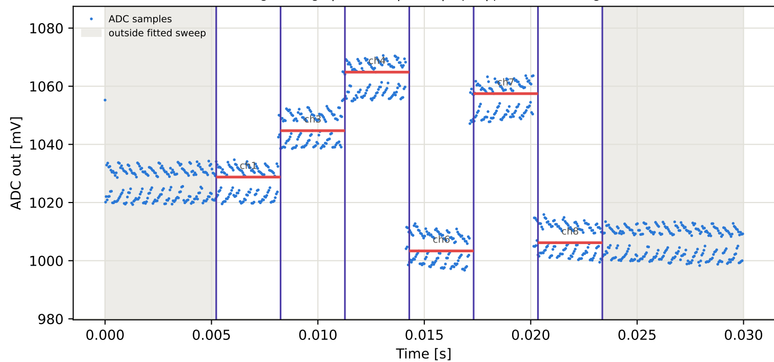
Tag5 &lt;- Tag1 | 945 MHz | run 0 | rep 1 | phase 27.92 deg
