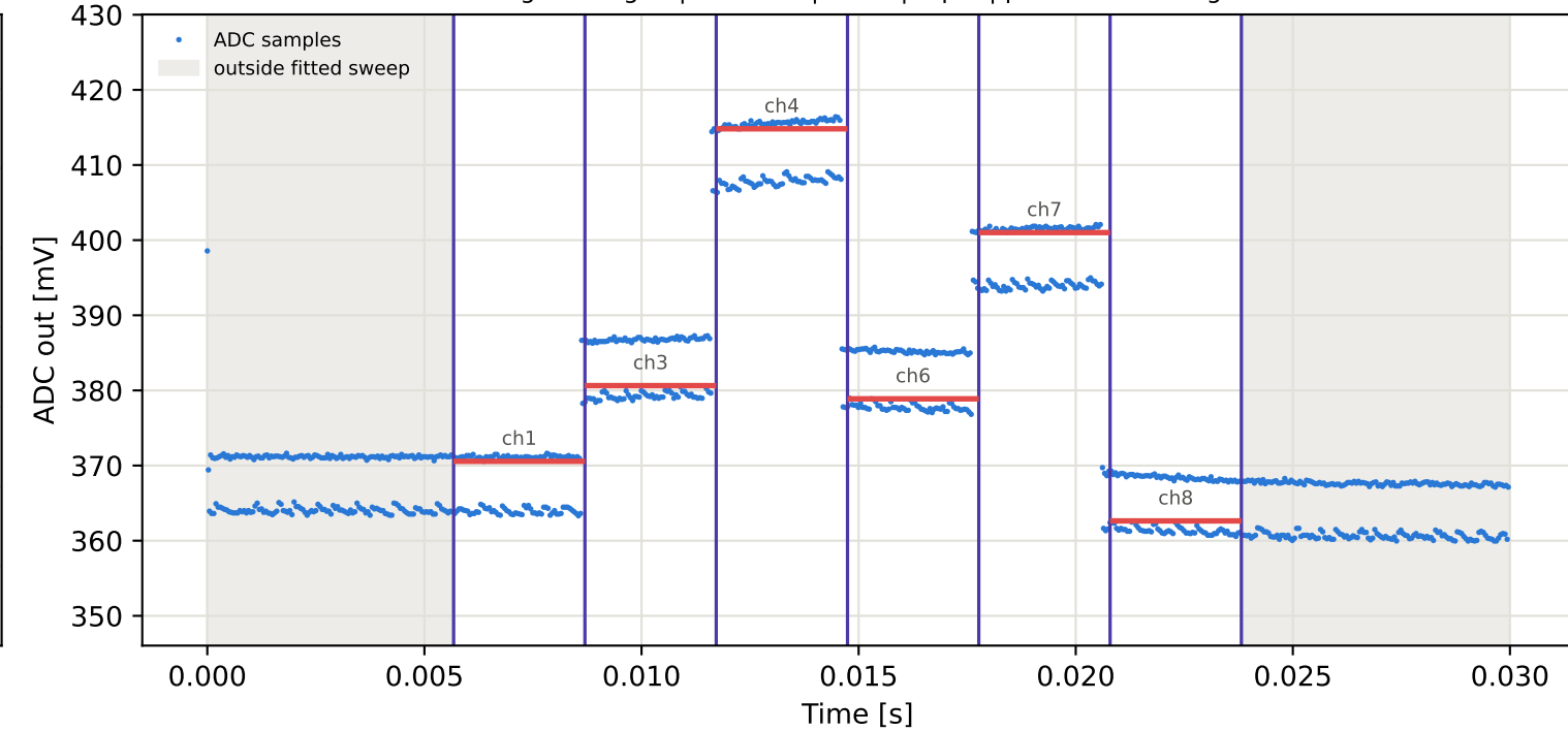
Tag6 &lt;- Tag3 | 955 MHz | run 0 | rep 1 | phase -175.88 deg
