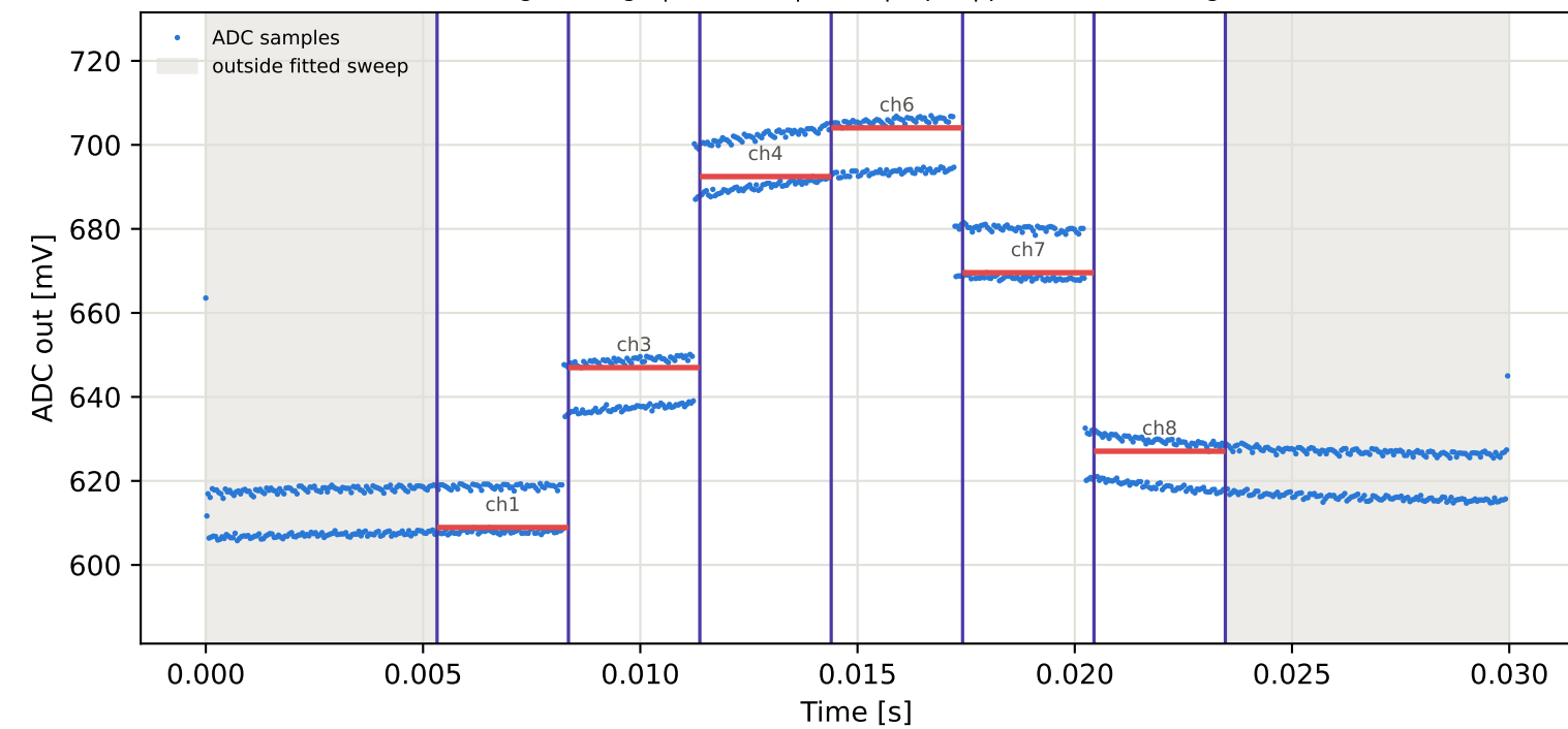
Tag3 &lt;- Tag6 | 925 MHz | run 0 | rep 1 | phase -53.68 deg
