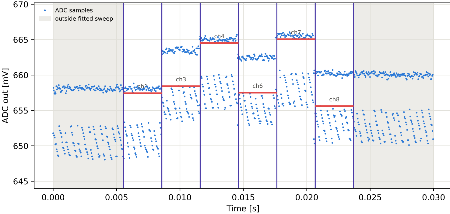
Tag8 &lt;- Tag15 | 845 MHz | run 0 | rep 1 | phase 150.86 deg
