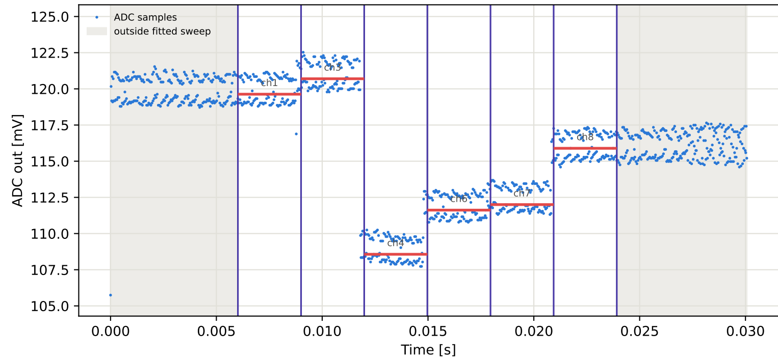
Tag9 &lt;- Tag2 | 795 MHz | run 0 | rep 1 | phase 91.28 deg
