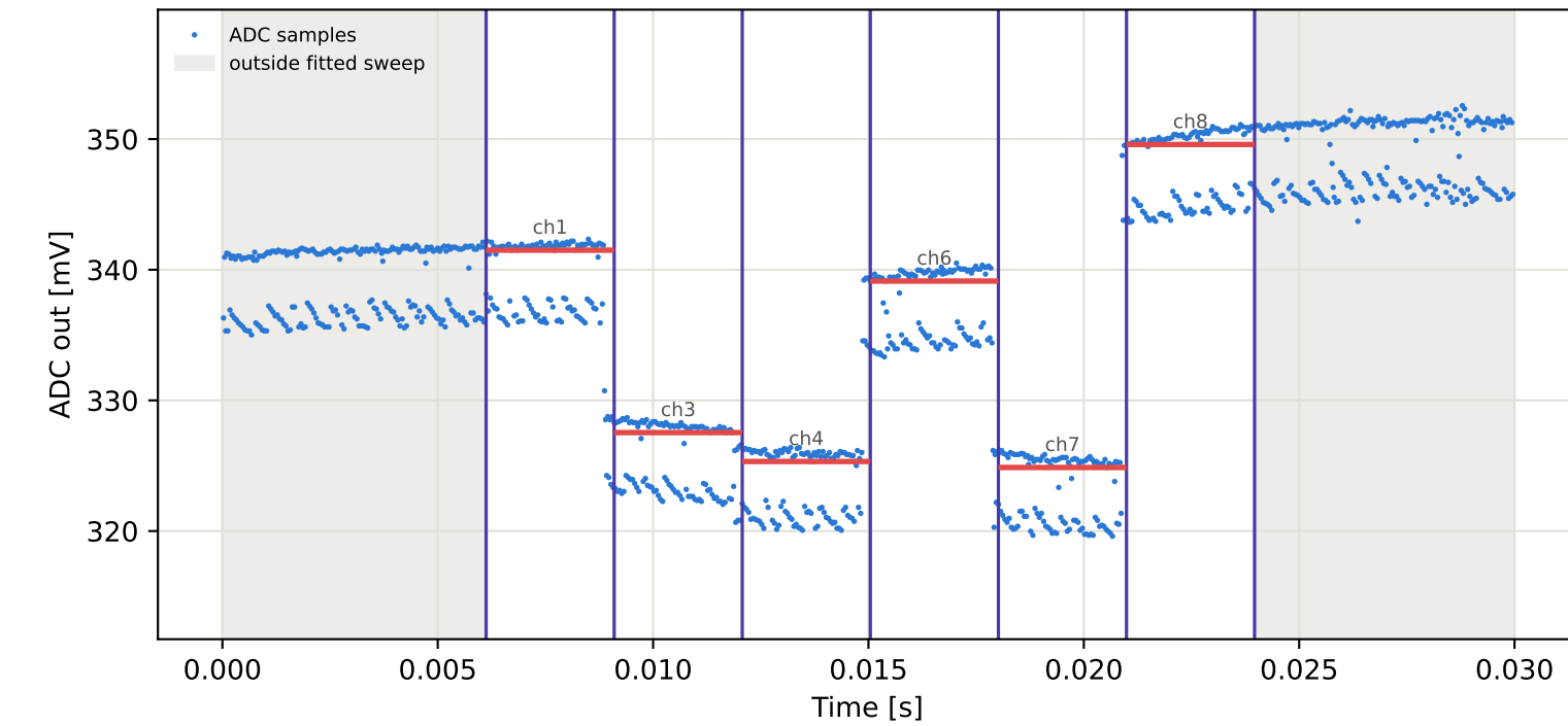
Tag9 &lt;- Tag16 | 875 MHz | run 0 | rep 1 | phase -128.81 deg
