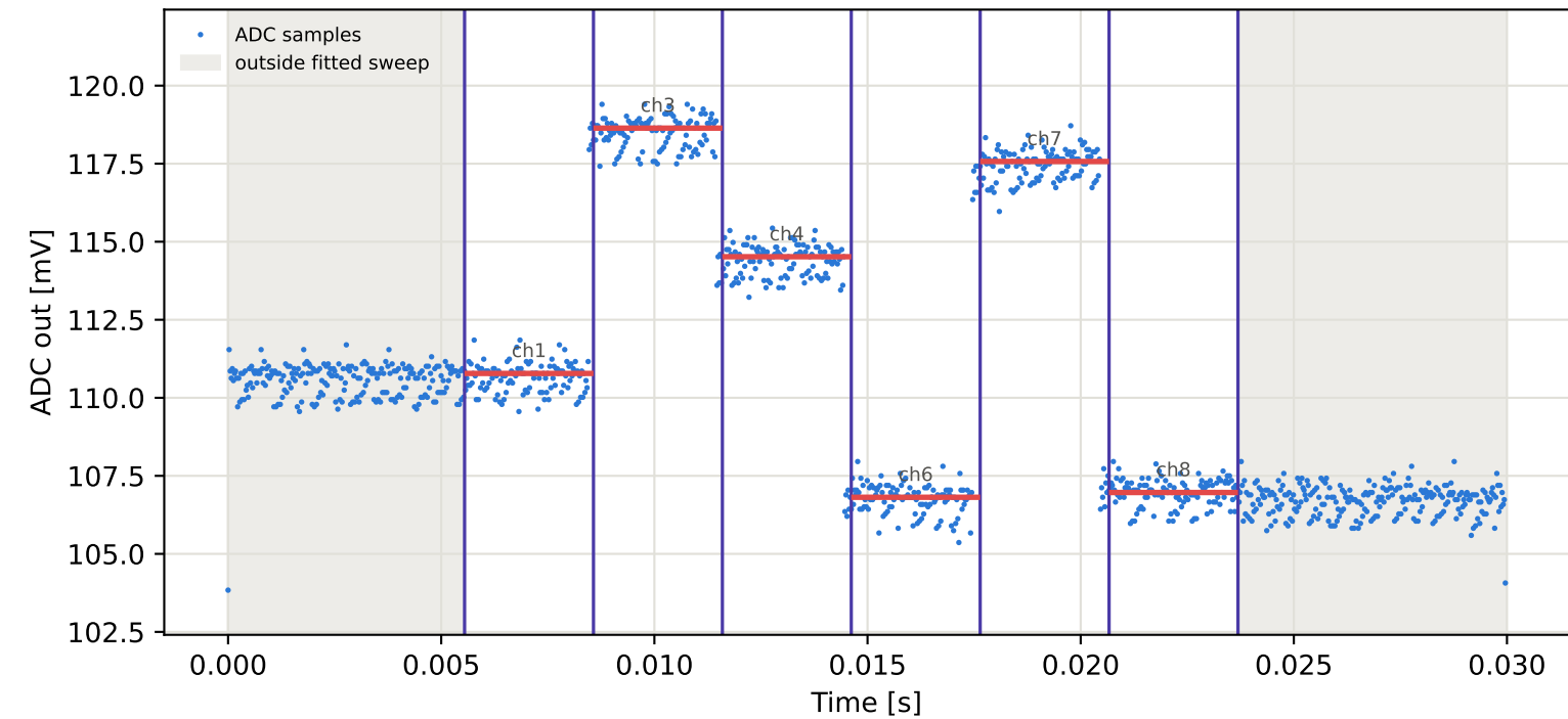
Tag6 &lt;- Tag10 | 805 MHz | run 0 | rep 1 | phase -176.25 deg
