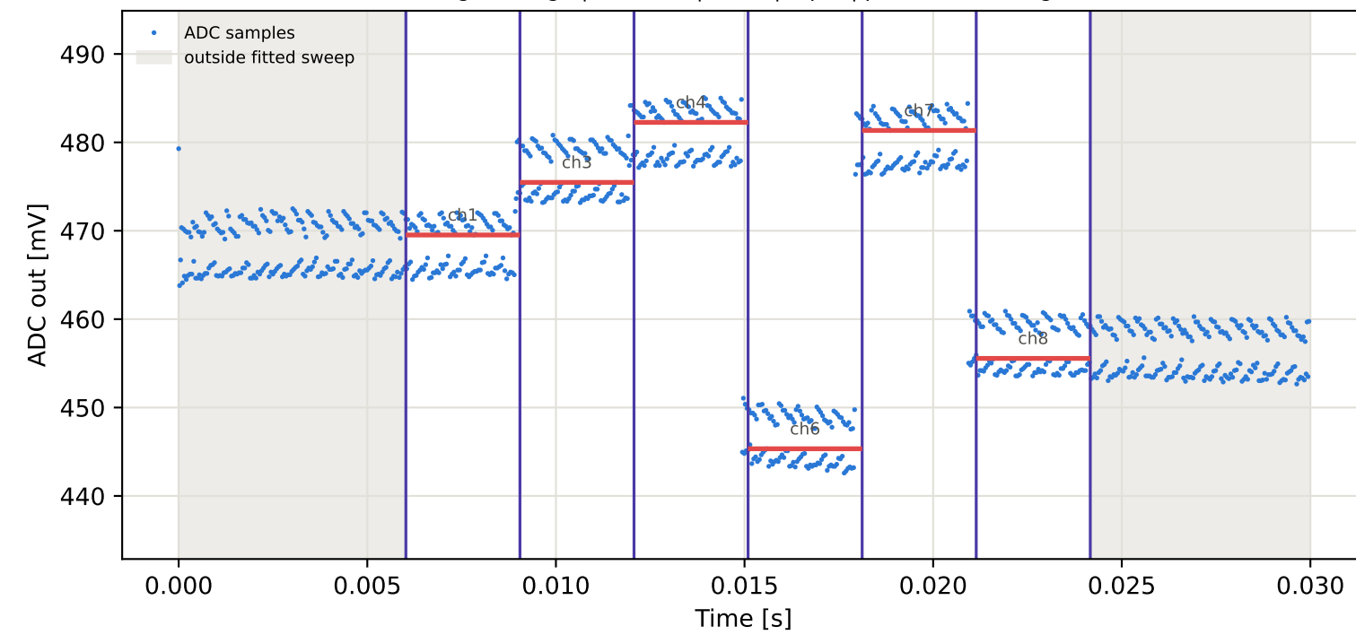
Tag4 &lt;- Tag15 | 985 MHz | run 0 | rep 1 | phase 143.22 deg
