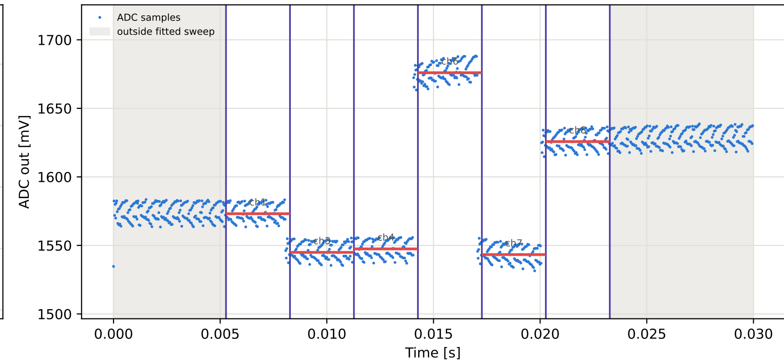
Tag15 &lt;- Tag6 | 945 MHz | run 0 | rep 1 | phase -97.14 deg
