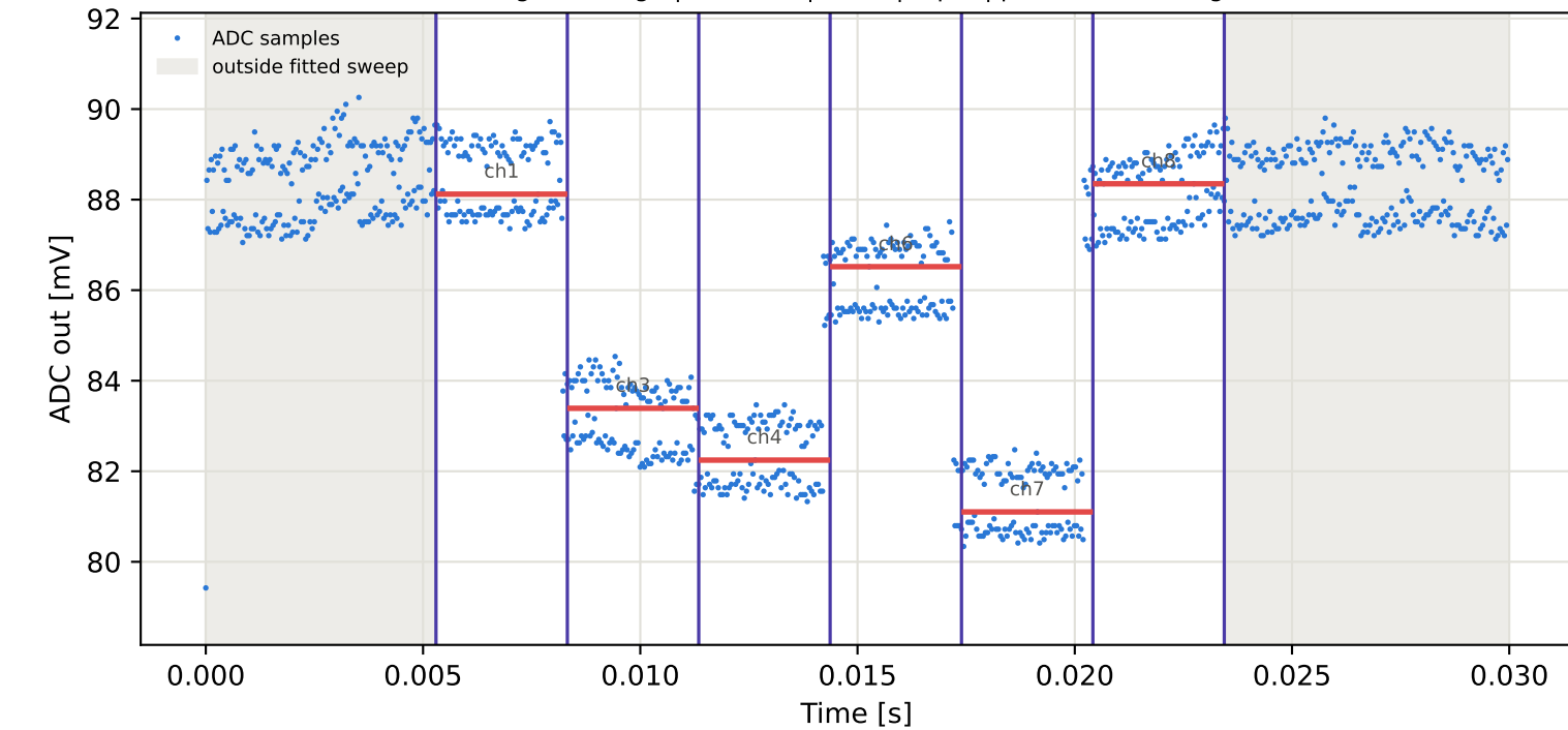
Tag15 &lt;- Tag1 | 825 MHz | run 0 | rep 1 | phase -174.93 deg
