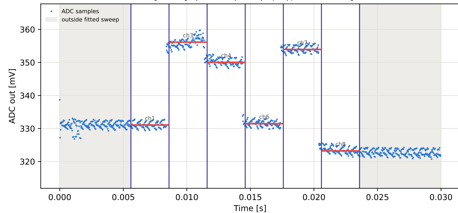
Tag4 &lt;- Tag3 | 845 MHz | run 0 | rep 1 | phase -35.32 deg
