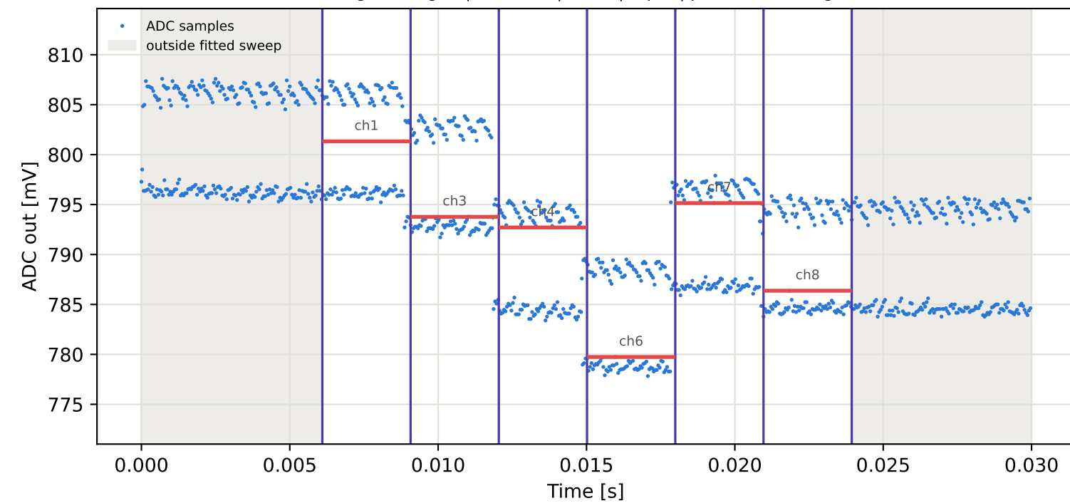
Tag5 &lt;- Tag16 | 865 MHz | run 0 | rep 1 | phase 21.10 deg
