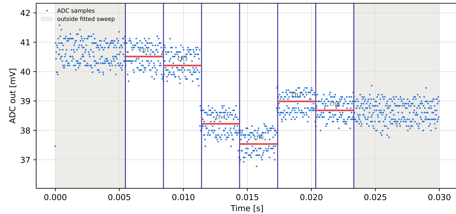
Tag2 &lt;- Tag7 | 865 MHz | run 0 | rep 1 | phase 43.17 deg
