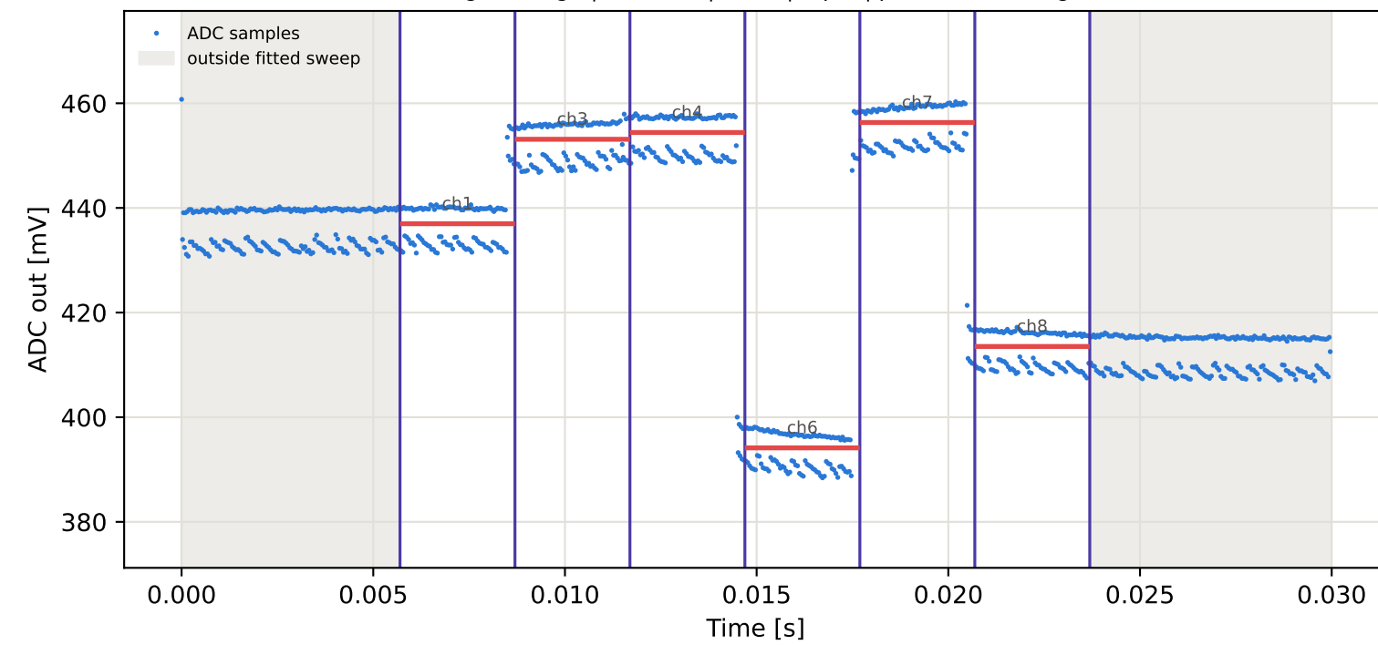
Tag4 &lt;- Tag7 | 965 MHz | run 0 | rep 1 | phase -165.08 deg
