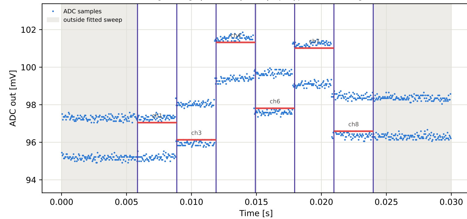
Tag1 &lt;- Tag7 | 805 MHz | run 0 | rep 1 | phase 28.83 deg
