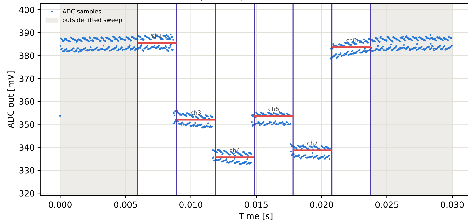
Tag8 &lt;- Tag1 | 875 MHz | run 0 | rep 1 | phase 83.77 deg
