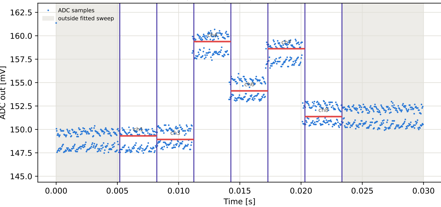
Tag5 &lt;- Tag3 | 795 MHz | run 0 | rep 1 | phase -97.23 deg
