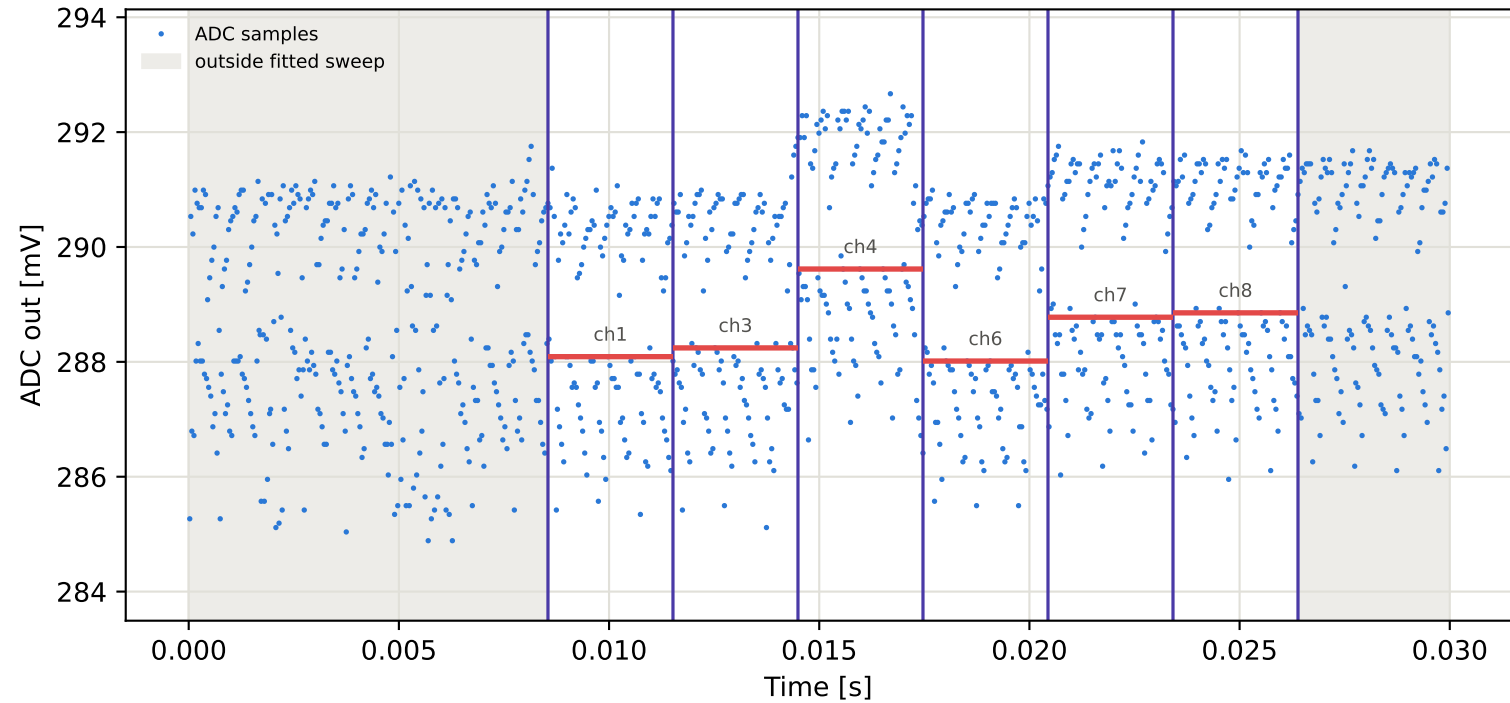
Tag5 &lt;- Tag4 | 985 MHz | run 0 | rep 1 | phase -36.94 deg
