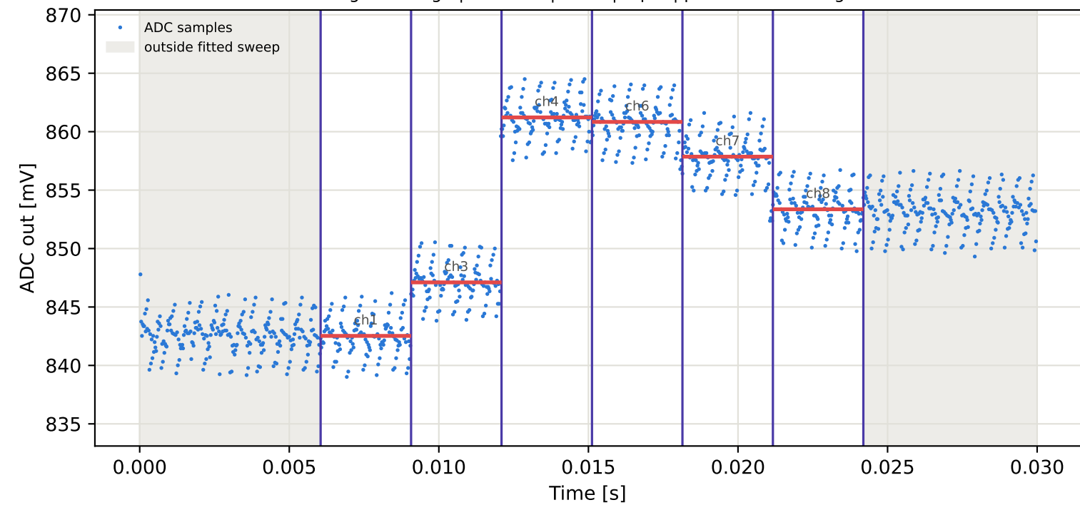
Tag2 &lt;- Tag10 | 855 MHz | run 0 | rep 1 | phase 73.42 deg
