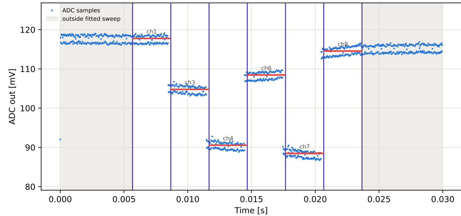
Tag5 &lt;- Tag1 | 805 MHz | run 0 | rep 1 | phase -132.12 deg
