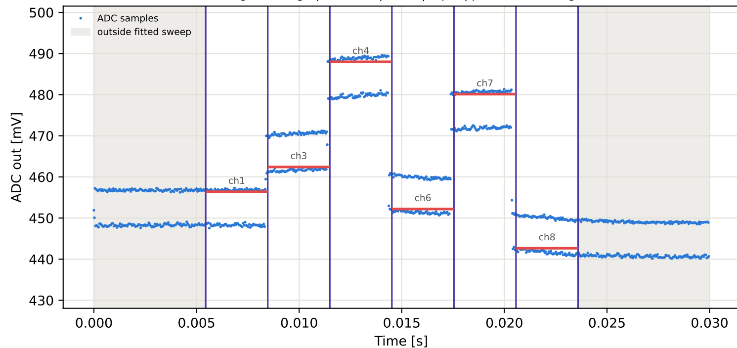
Tag15 &lt;- Tag10 | 945 MHz | run 0 | rep 1 | phase -62.44 deg
