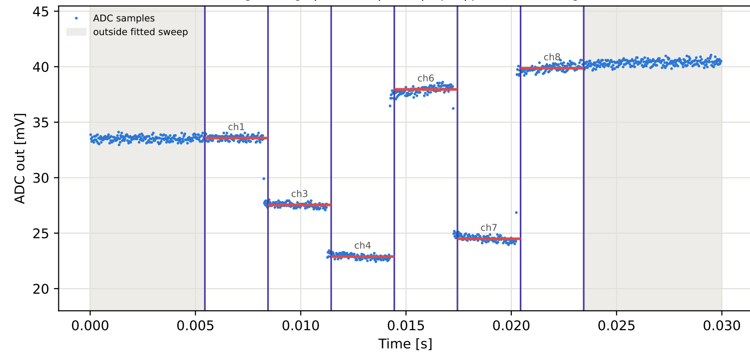
Tag2 &lt;- Tag6 | 925 MHz | run 0 | rep 1 | phase 68.85 deg
