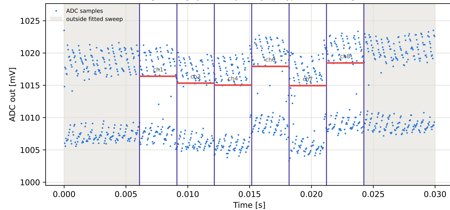
Tag16 &lt;- Tag4 | 915 MHz | run 0 | rep 1 | phase -158.04 deg
