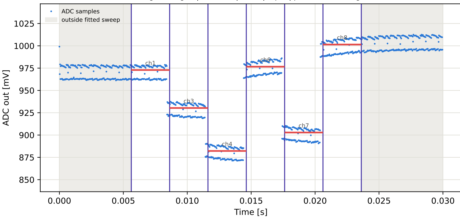
Tag4 &lt;- Tag3 | 935 MHz | run 0 | rep 1 | phase 163.67 deg
