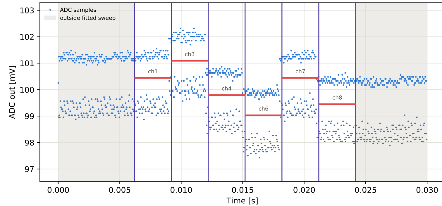
Tag1 &lt;- Tag9 | 805 MHz | run 0 | rep 1 | phase -103.62 deg
