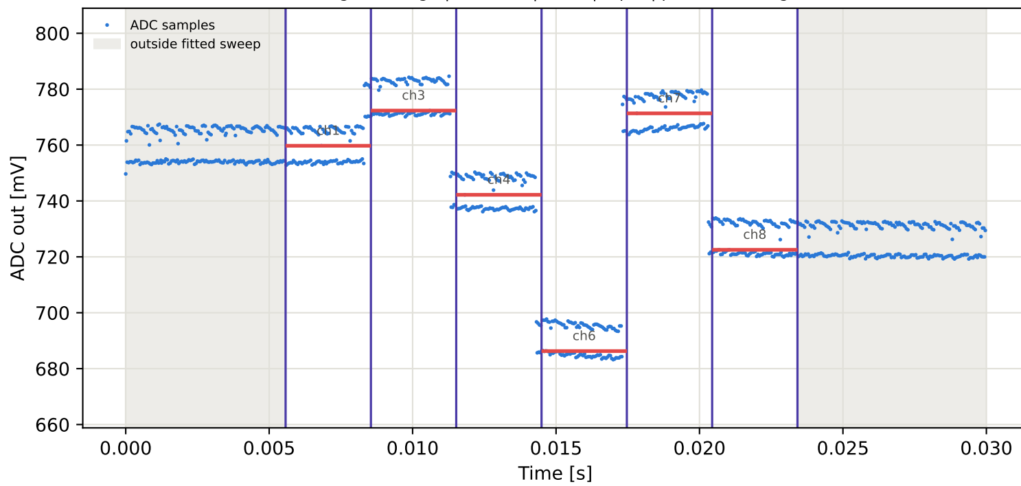
Tag2 &lt;- Tag1 | 995 MHz | run 0 | rep 1 | phase -87.56 deg
