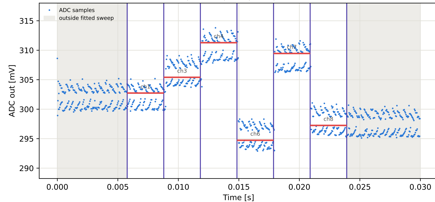
Tag6 &lt;- Tag1 | 985 MHz | run 0 | rep 1 | phase -48.27 deg
