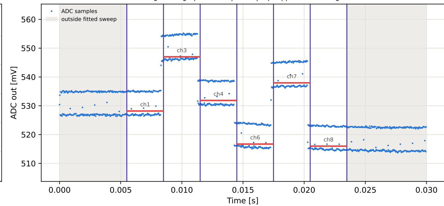
Tag8 &lt;- Tag5 | 835 MHz | run 0 | rep 1 | phase 42.33 deg
