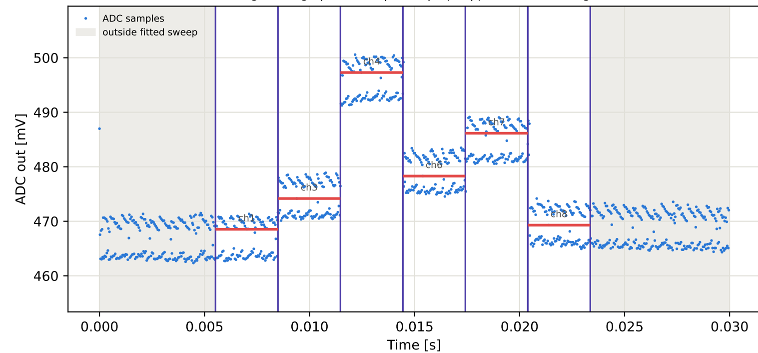
Tag4 &lt;- Tag9 | 975 MHz | run 0 | rep 1 | phase -43.41 deg
