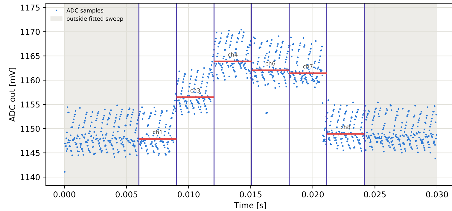
Tag16 &lt;- Tag10 | 895 MHz | run 0 | rep 1 | phase -107.19 deg
