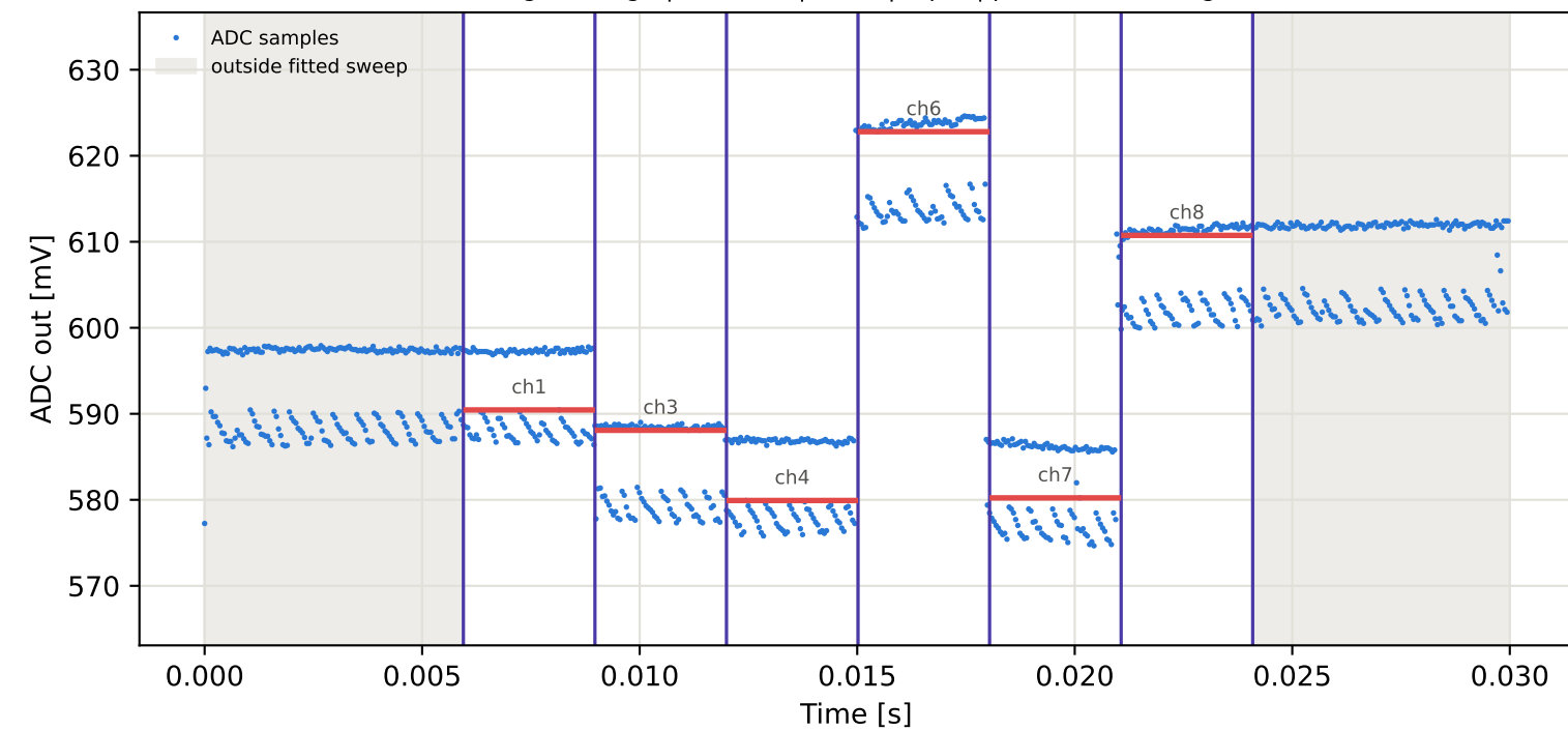
Tag9 &lt;- Tag15 | 975 MHz | run 0 | rep 1 | phase -75.28 deg
