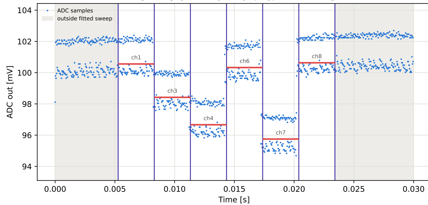
Tag8 &lt;- Tag1 | 775 MHz | run 0 | rep 1 | phase -178.74 deg
