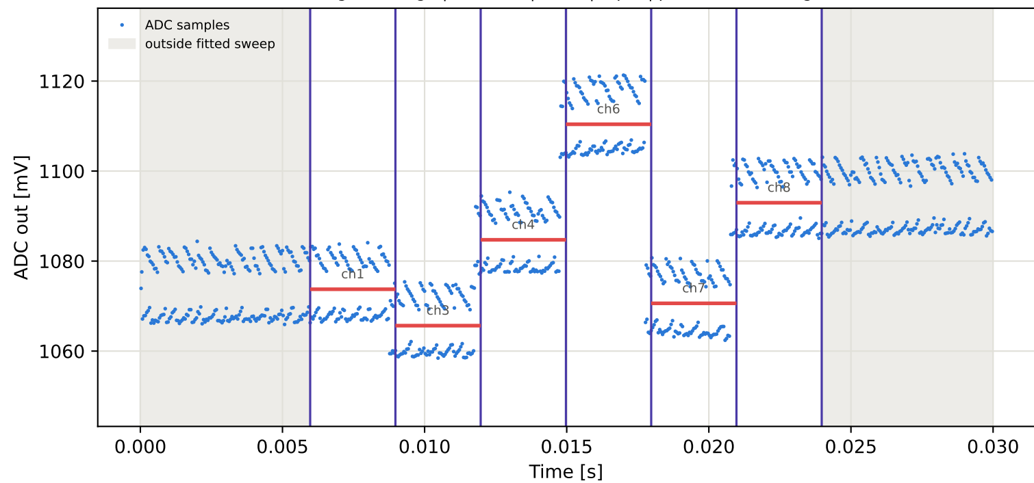
Tag2 &lt;- Tag10 | 985 MHz | run 0 | rep 1 | phase -55.91 deg
