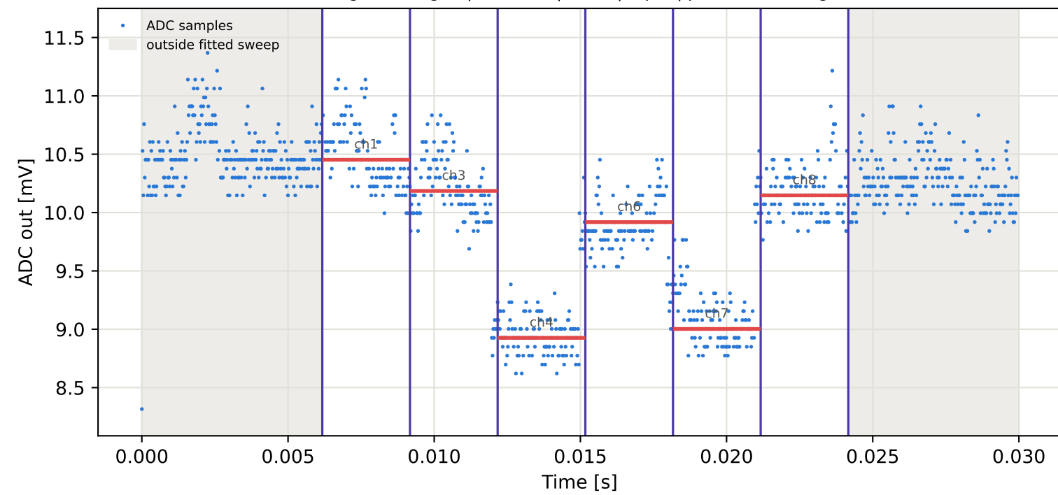
Tag10 &lt;- Tag3 | 775 MHz | run 0 | rep 1 | phase 93.57 deg
