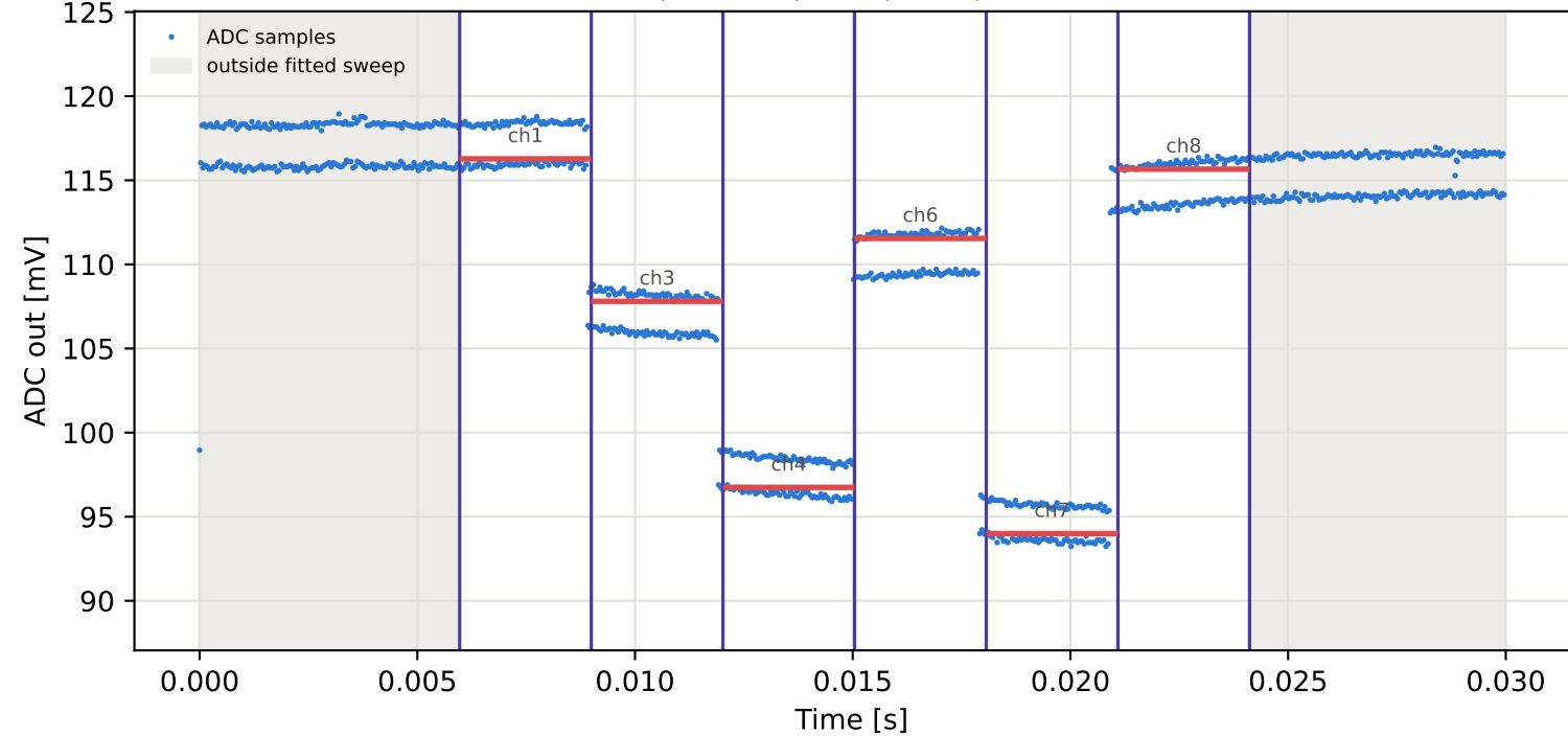
Tag1 &lt;- Tag3 | 805 MHz | run 0 | rep 1 | phase 110.89 deg
