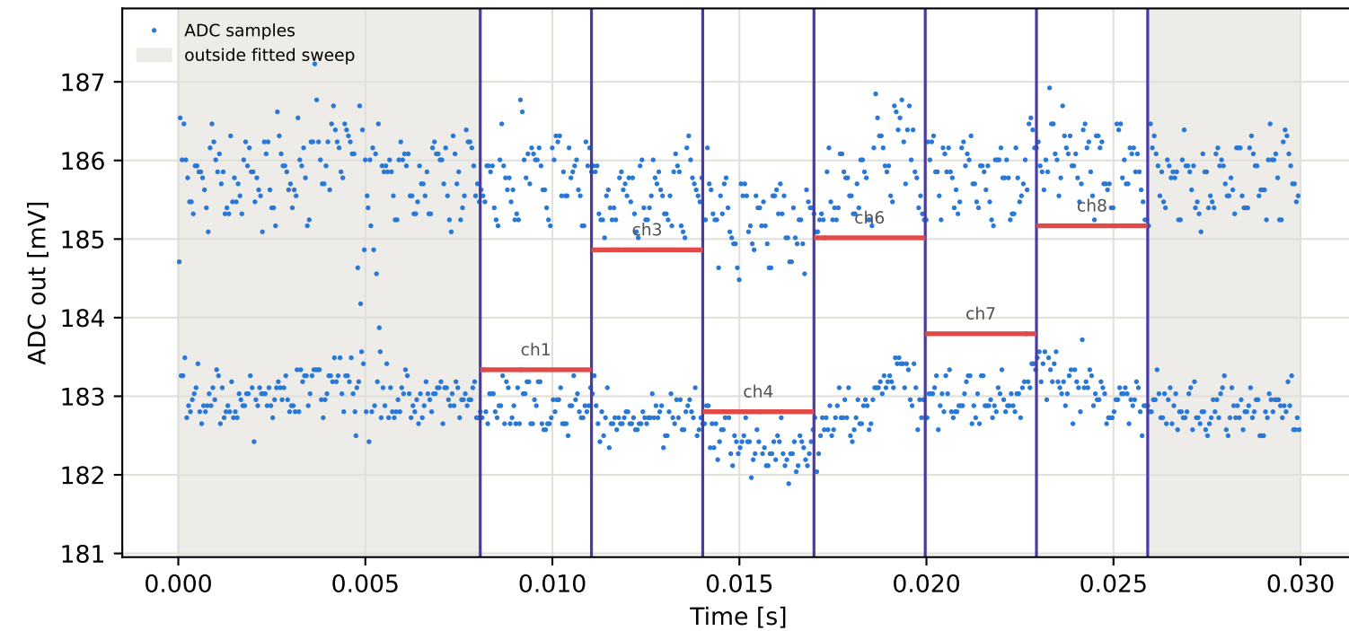
Tag10 &lt;- Tag4 | 995 MHz | run 0 | rep 1 | phase 62.98 deg
