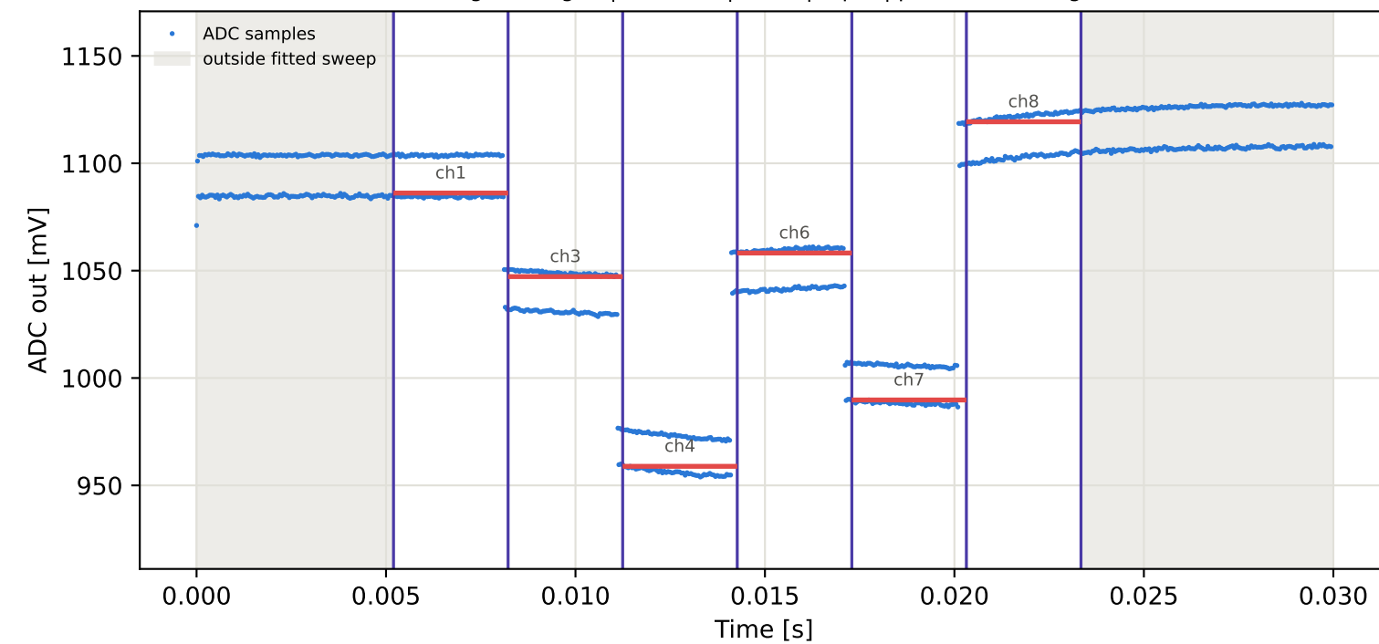
Tag4 &lt;- Tag2 | 945 MHz | run 0 | rep 1 | phase 85.50 deg
