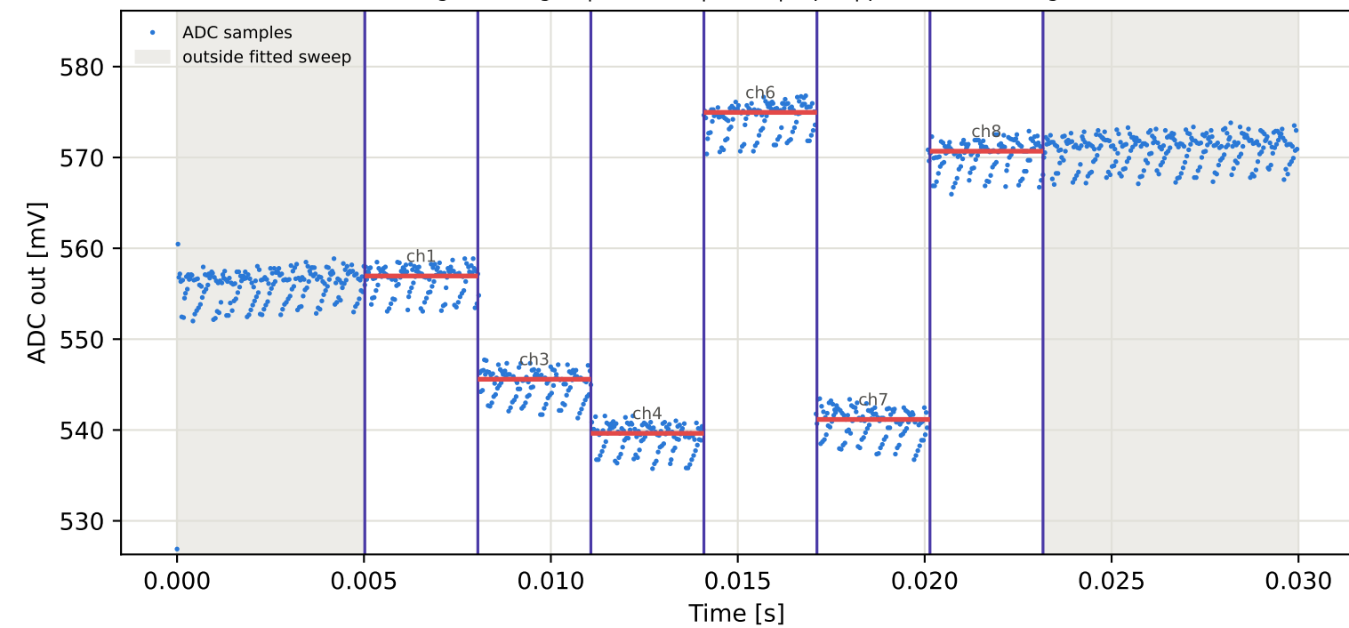
Tag10 &lt;- Tag2 | 955 MHz | run 0 | rep 1 | phase 2.55 deg
