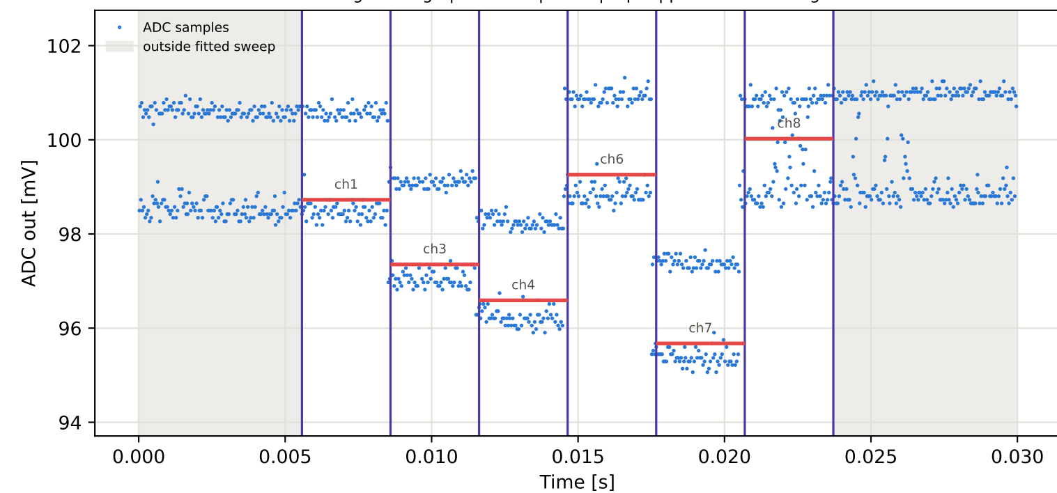
Tag7 &lt;- Tag5 | 775 MHz | run 0 | rep 1 | phase 139.88 deg
