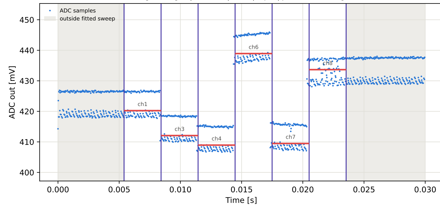
Tag1 &lt;- Tag16 | 965 MHz | run 0 | rep 1 | phase 26.81 deg
