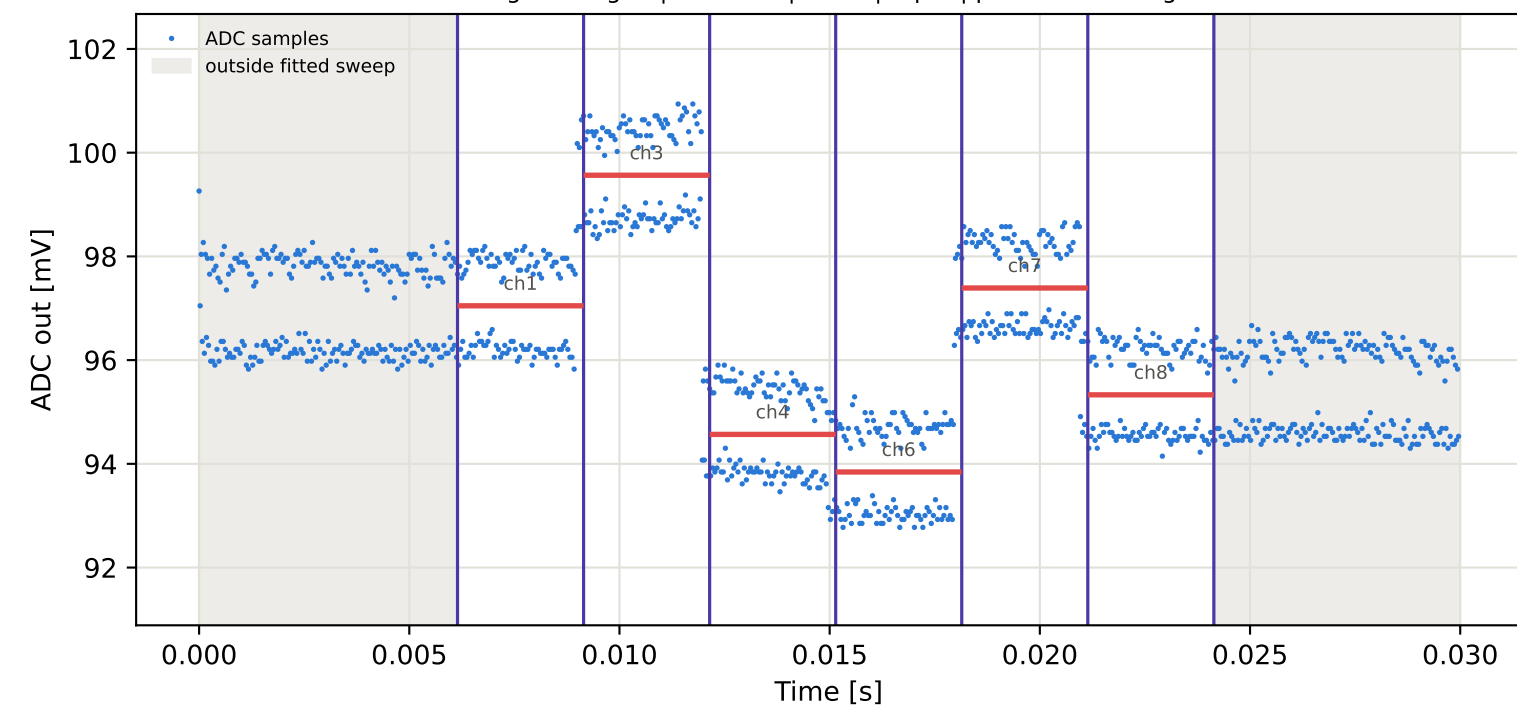
Tag7 &lt;- Tag3 | 775 MHz | run 0 | rep 1 | phase -72.95 deg
