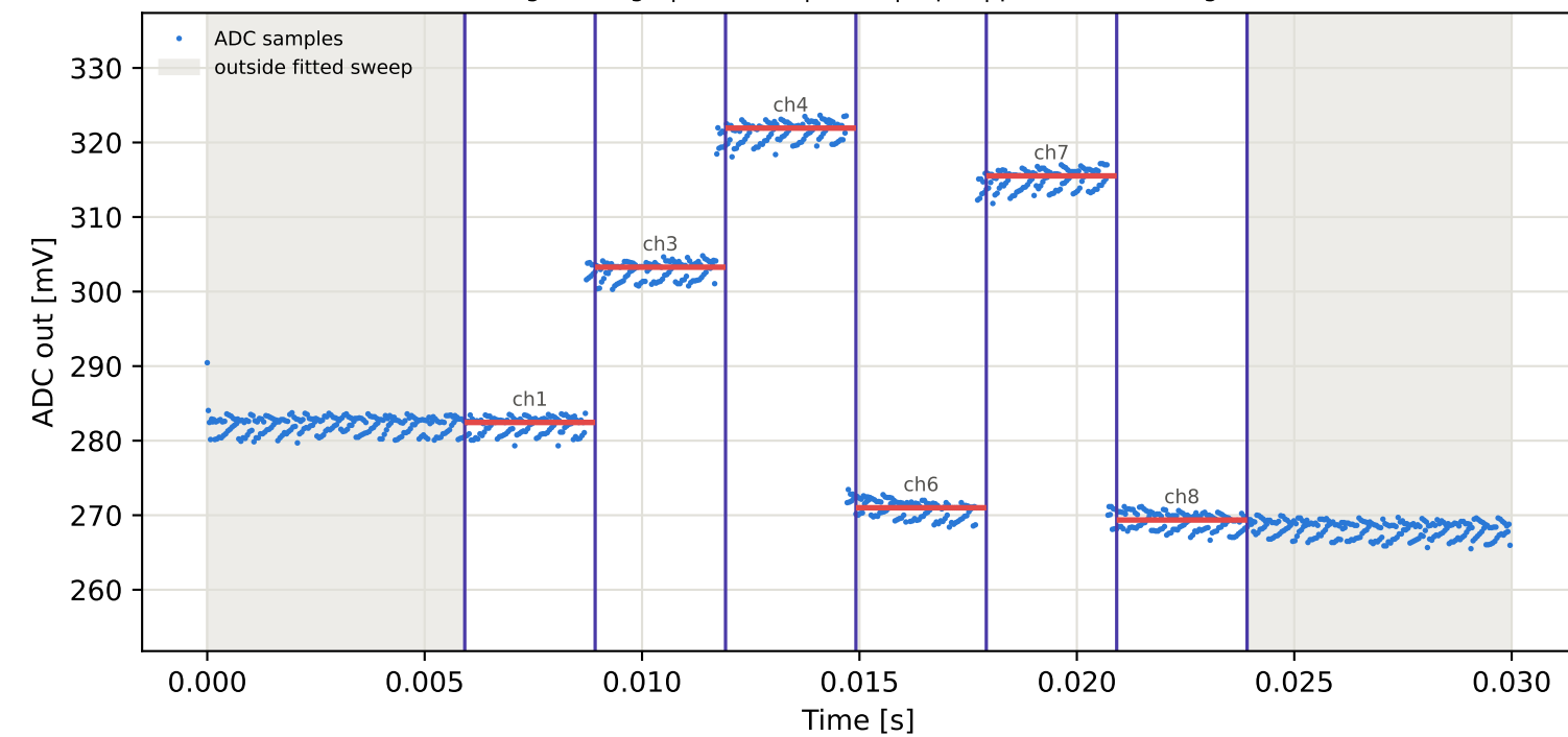
Tag7 &lt;- Tag10 | 985 MHz | run 0 | rep 1 | phase 172.90 deg
