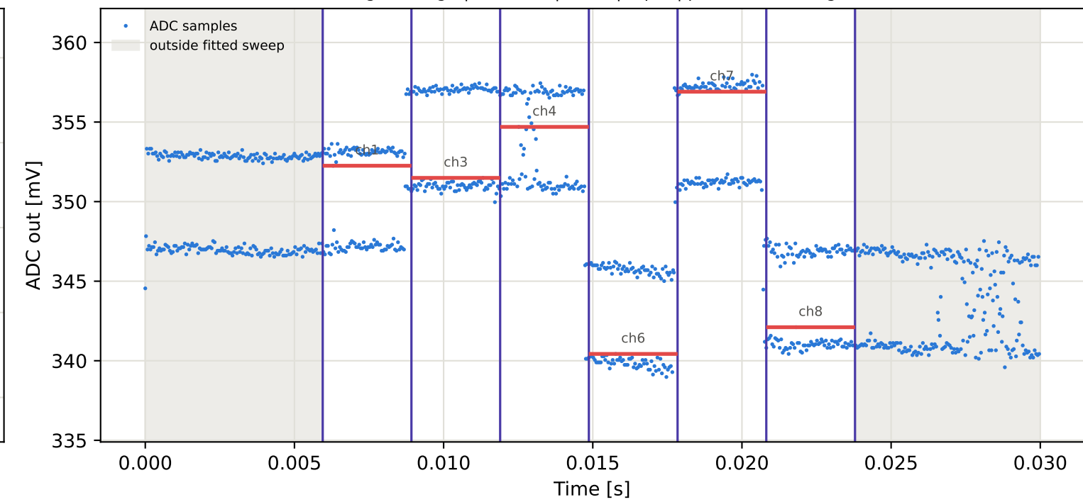
Tag7 &lt;- Tag4 | 875 MHz | run 0 | rep 1 | phase 22.57 deg
