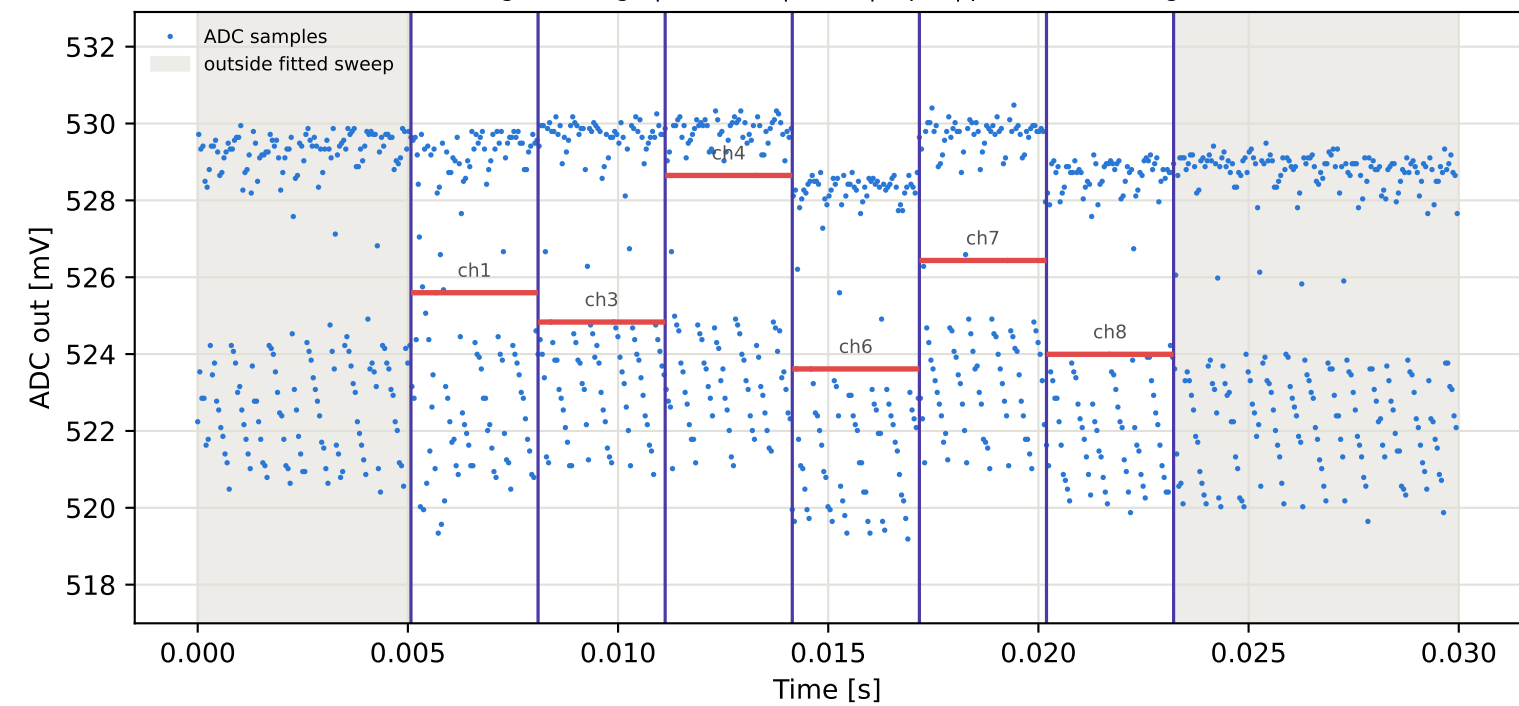
Tag15 &lt;- Tag4 | 995 MHz | run 0 | rep 1 | phase -50.71 deg
