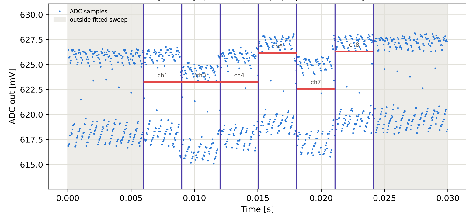
Tag15 &lt;- Tag6 | 845 MHz | run 0 | rep 1 | phase 172.47 deg
