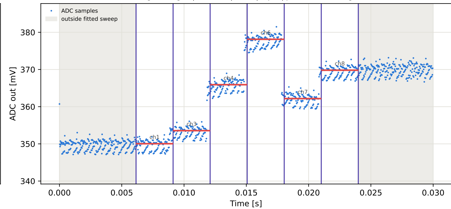
Tag4 &lt;- Tag16 | 875 MHz | run 0 | rep 1 | phase -4.18 deg
