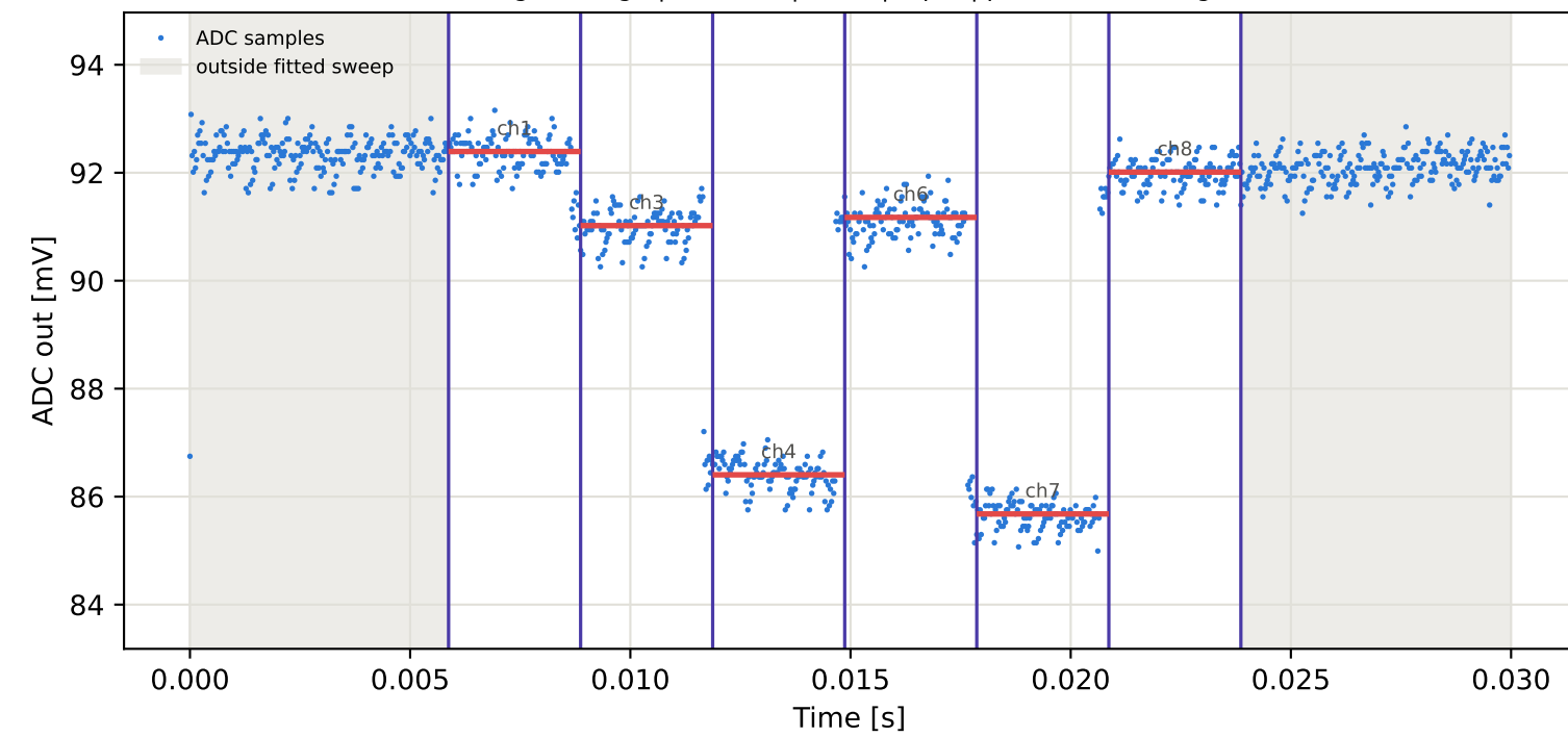
Tag9 &lt;- Tag5 | 775 MHz | run 0 | rep 1 | phase 68.57 deg
