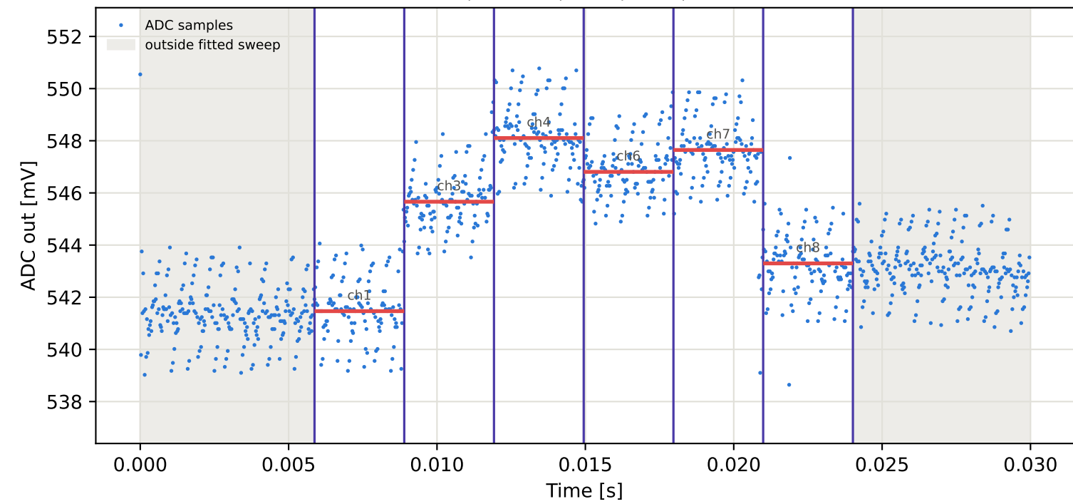
Tag15 &lt;- Tag10 | 865 MHz | run 0 | rep 1 | phase -99.96 deg
