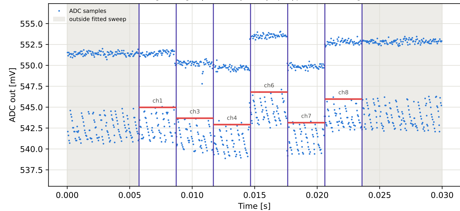
Tag5 &lt;- Tag16 | 975 MHz | run 0 | rep 1 | phase 142.18 deg
