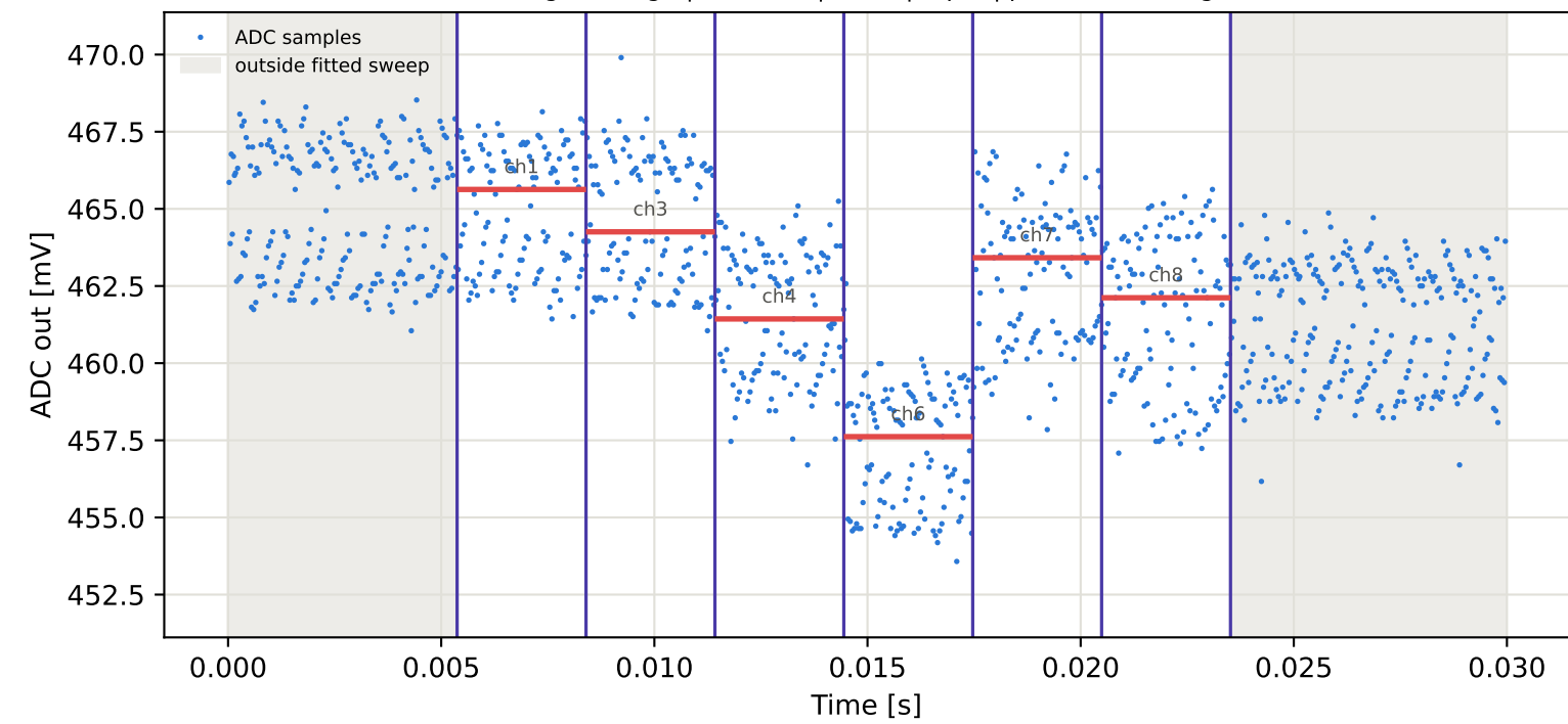
Tag7 &lt;- Tag4 | 885 MHz | run 0 | rep 1 | phase -4.97 deg
