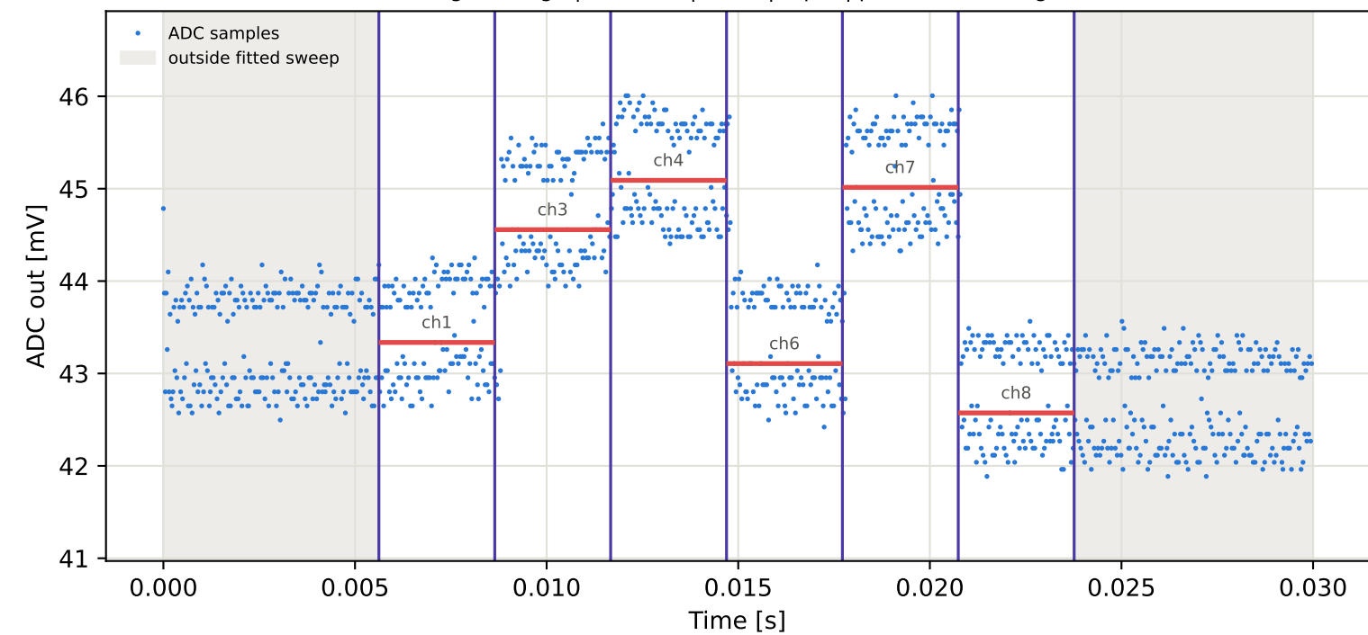
Tag1 &lt;- Tag4 | 795 MHz | run 0 | rep 1 | phase 146.86 deg
