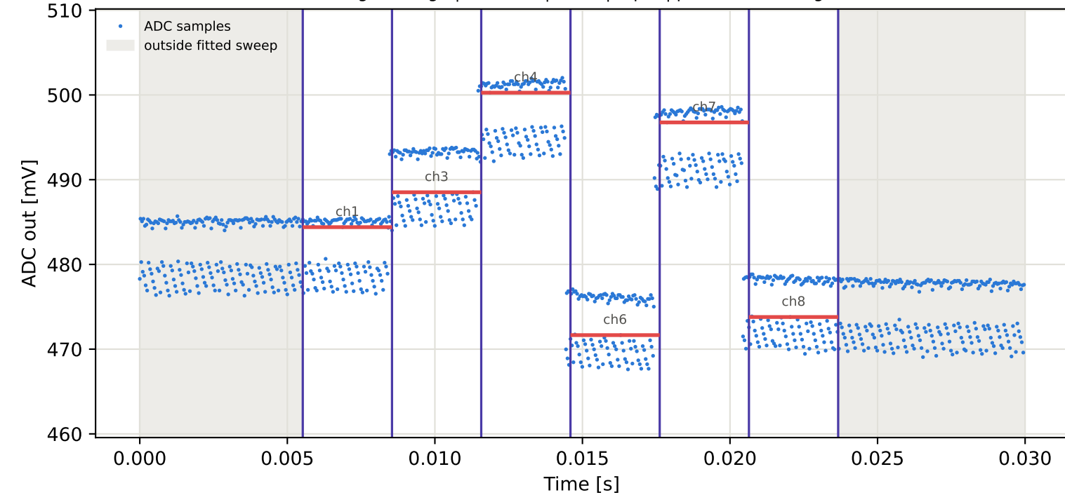
Tag3 &lt;- Tag8 | 975 MHz | run 0 | rep 1 | phase -52.46 deg
