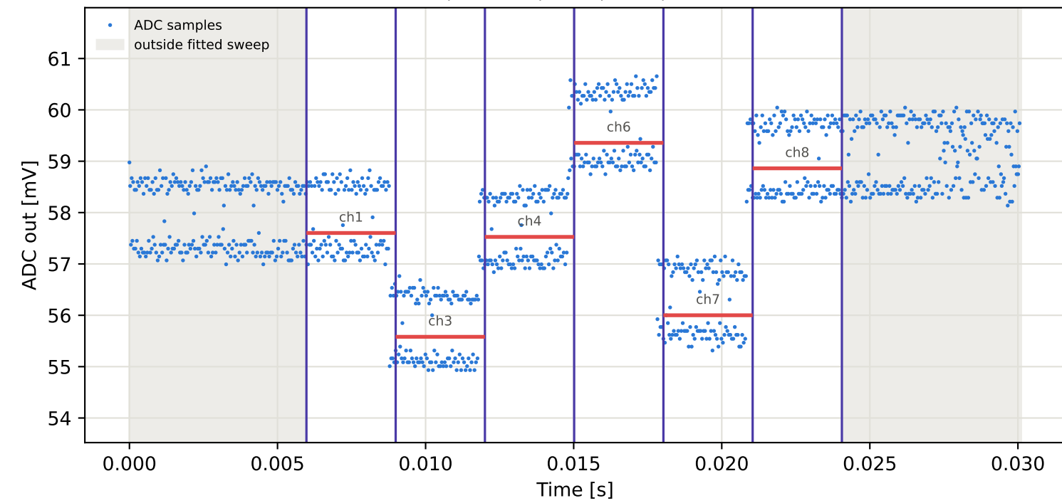
Tag7 &lt;- Tag15 | 795 MHz | run 0 | rep 1 | phase -167.98 deg
