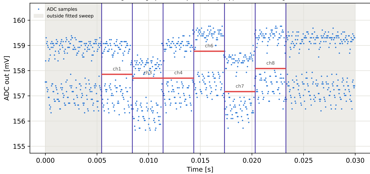
Tag5 &lt;- Tag1 | 795 MHz | run 0 | rep 1 | phase 179.43 deg
