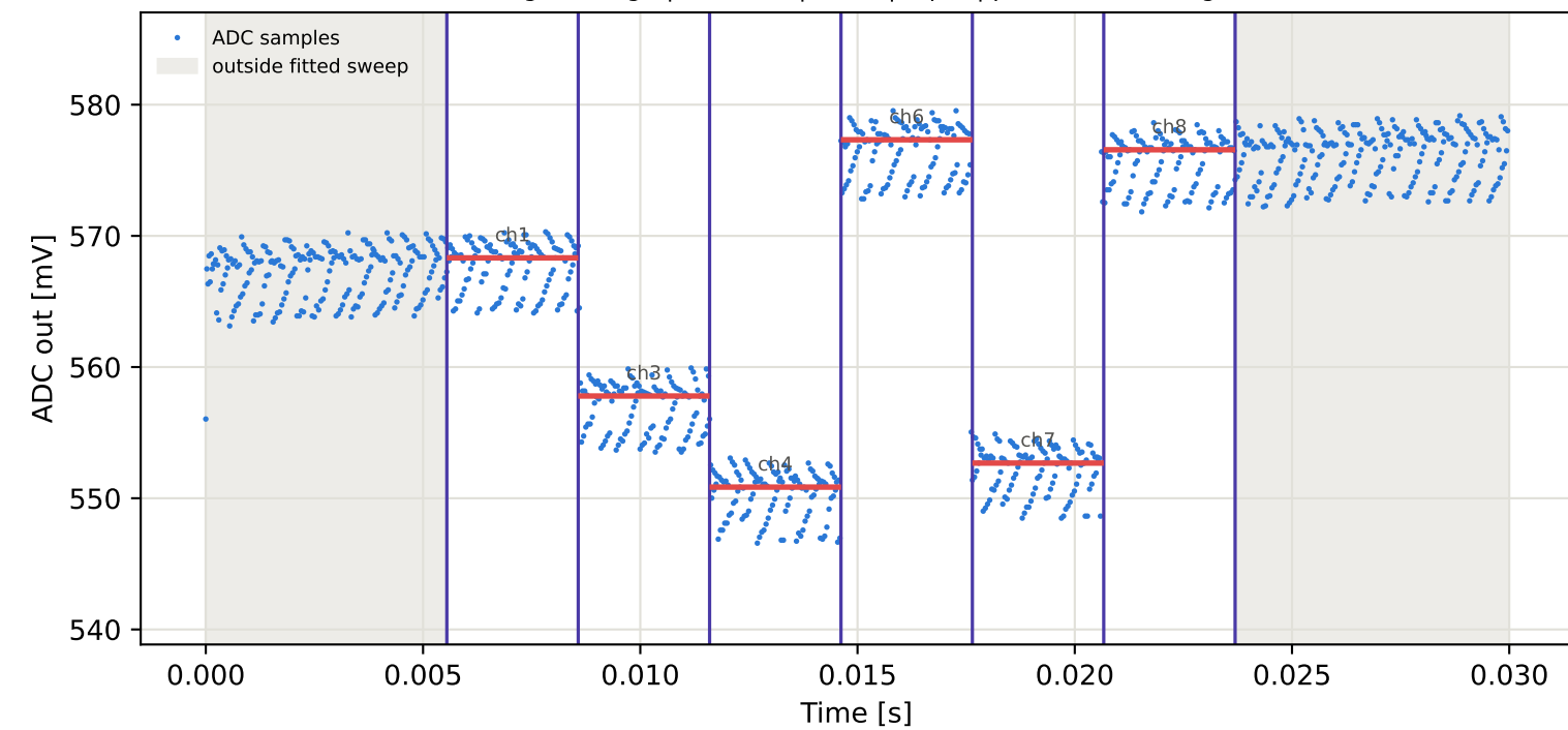
Tag9 &lt;- Tag10 | 995 MHz | run 0 | rep 1 | phase 163.69 deg
