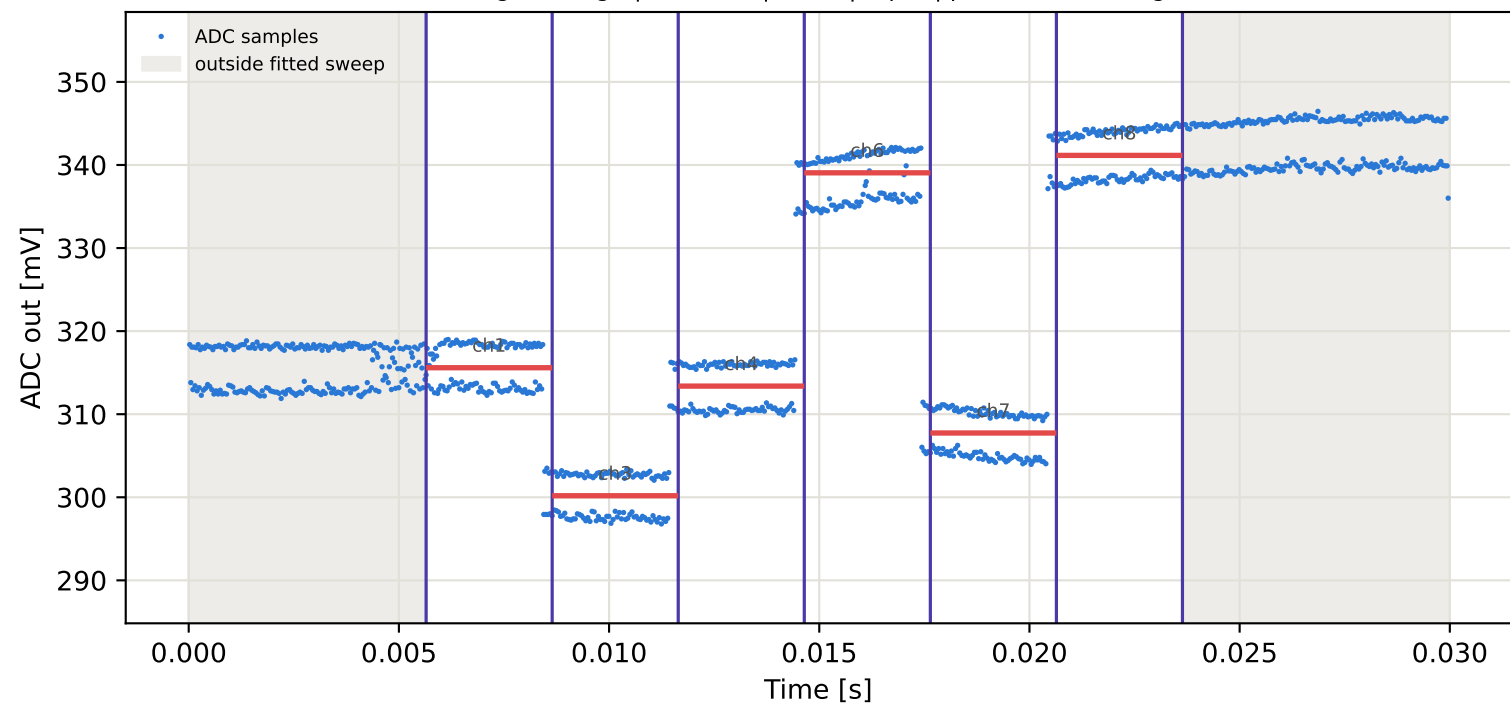
Tag4 &lt;- Tag8 | 865 MHz | run 0 | rep 1 | phase -158.60 deg
