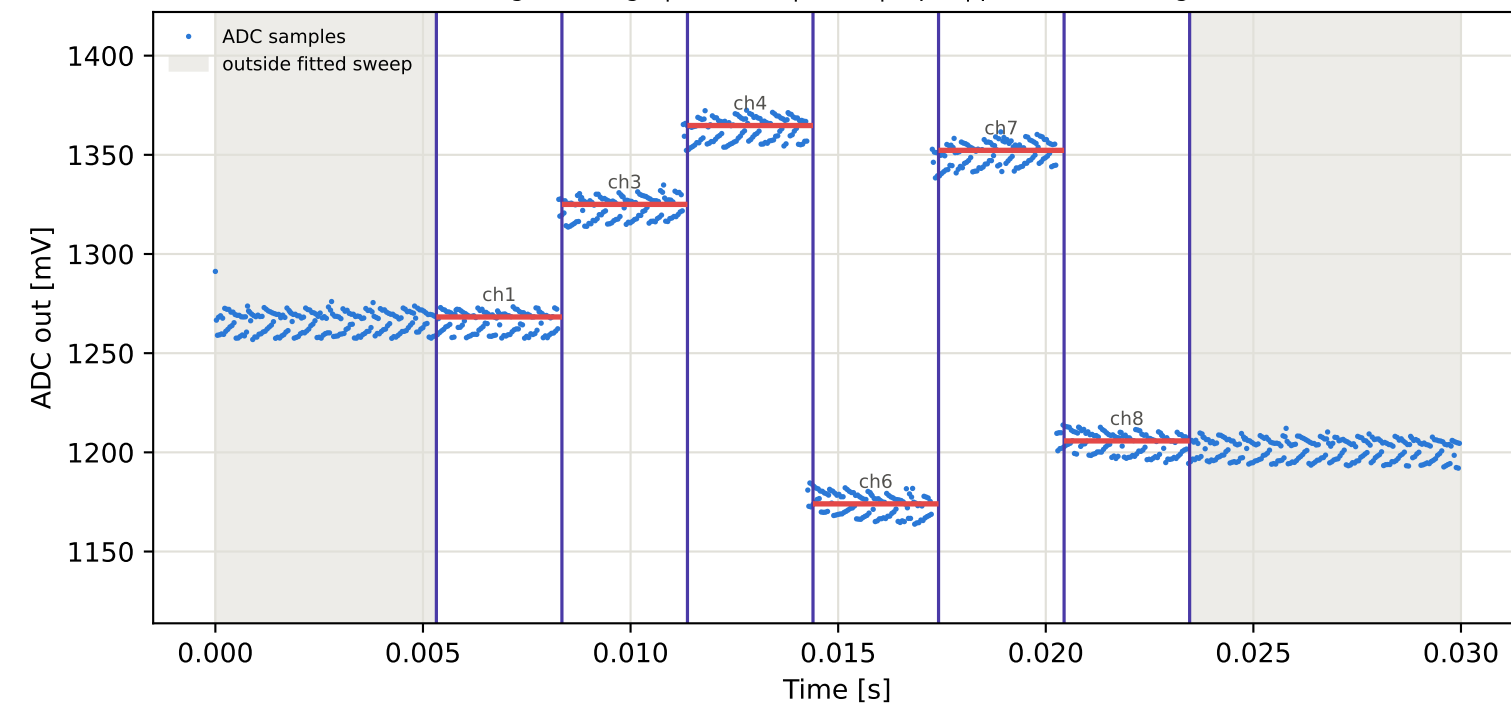
Tag2 &lt;- Tag1 | 965 MHz | run 0 | rep 1 | phase 149.10 deg
