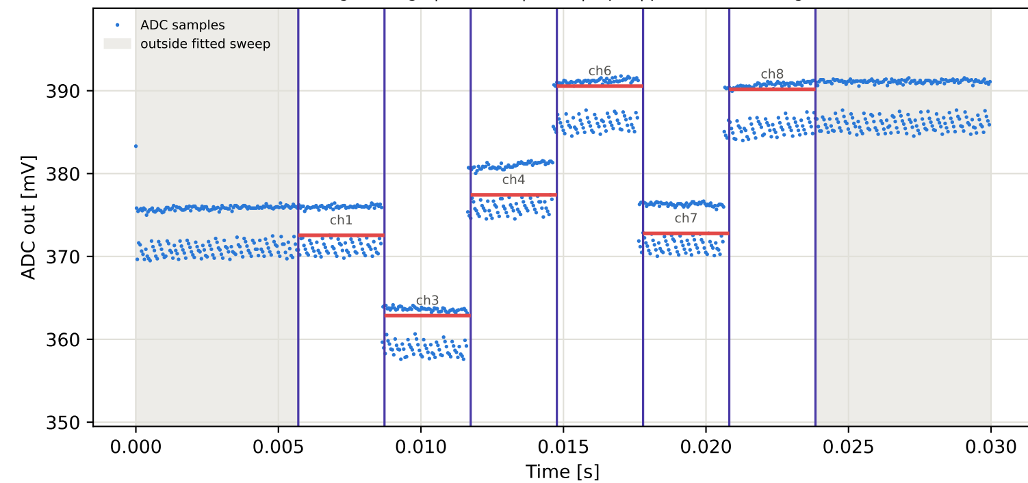
Tag3 &lt;- Tag6 | 835 MHz | run 0 | rep 1 | phase 65.46 deg
