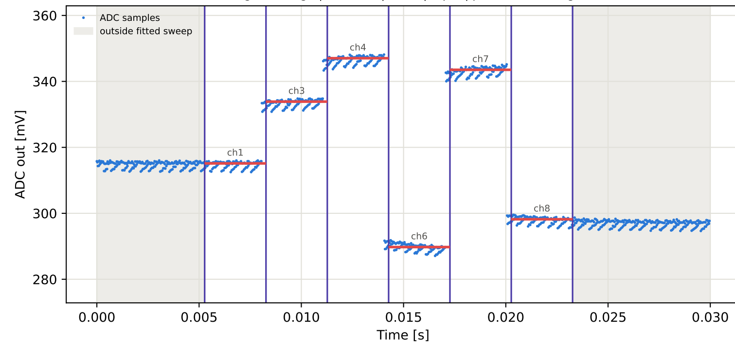
Tag10 &lt;- Tag8 | 985 MHz | run 0 | rep 1 | phase 26.73 deg
