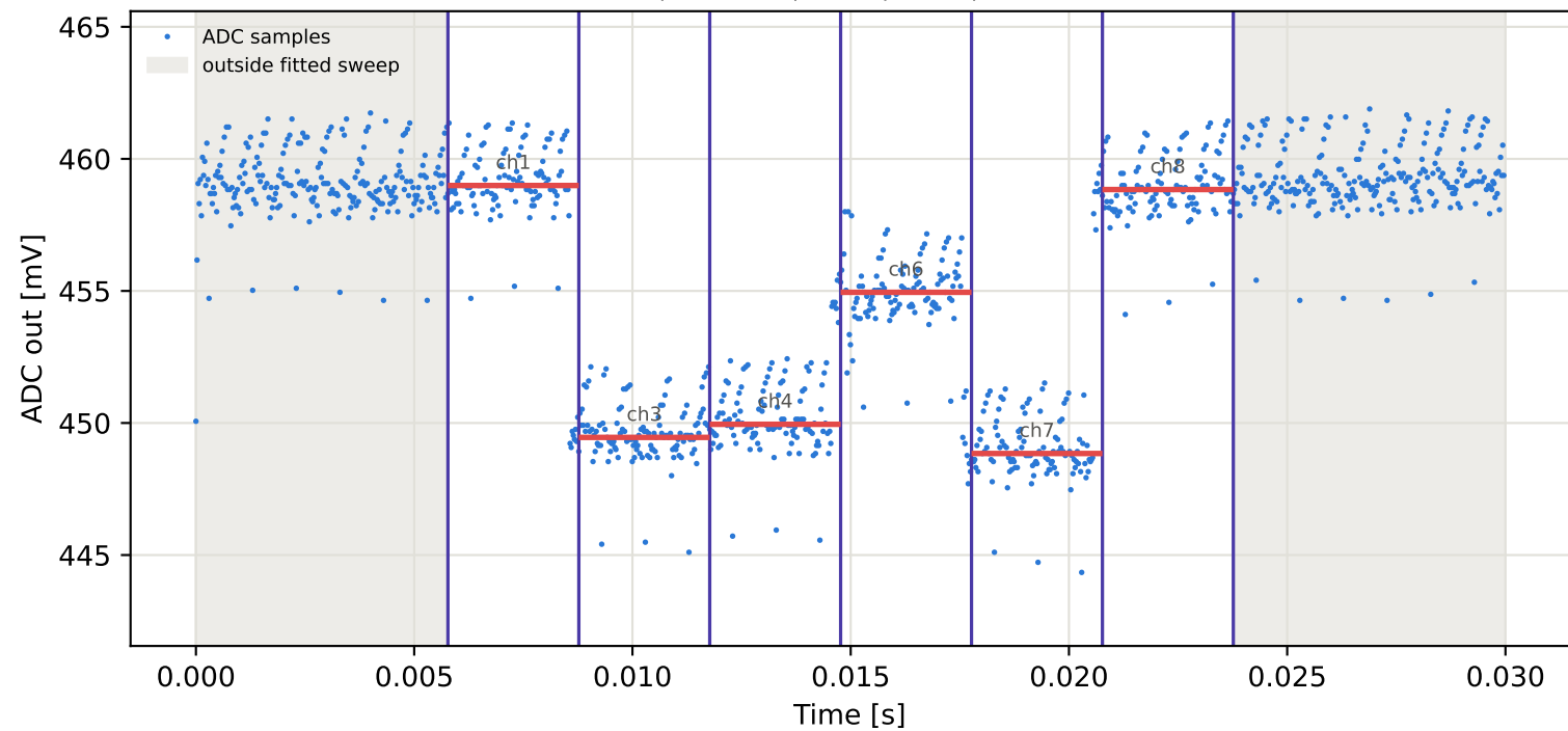
Tag5 &lt;- Tag1 | 855 MHz | run 0 | rep 1 | phase 119.69 deg
