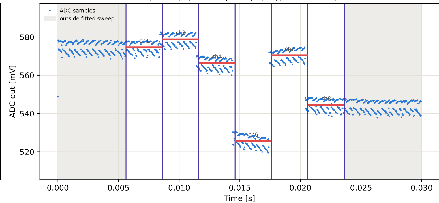
Tag7 &lt;- Tag6 | 895 MHz | run 0 | rep 1 | phase 91.52 deg
