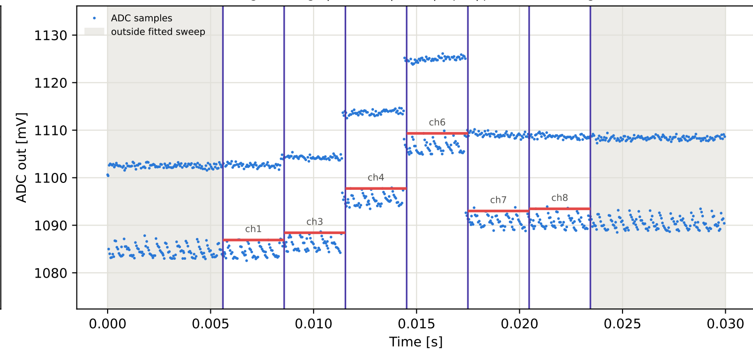
Tag16 &lt;- Tag5 | 945 MHz | run 0 | rep 1 | phase 1.27 deg
