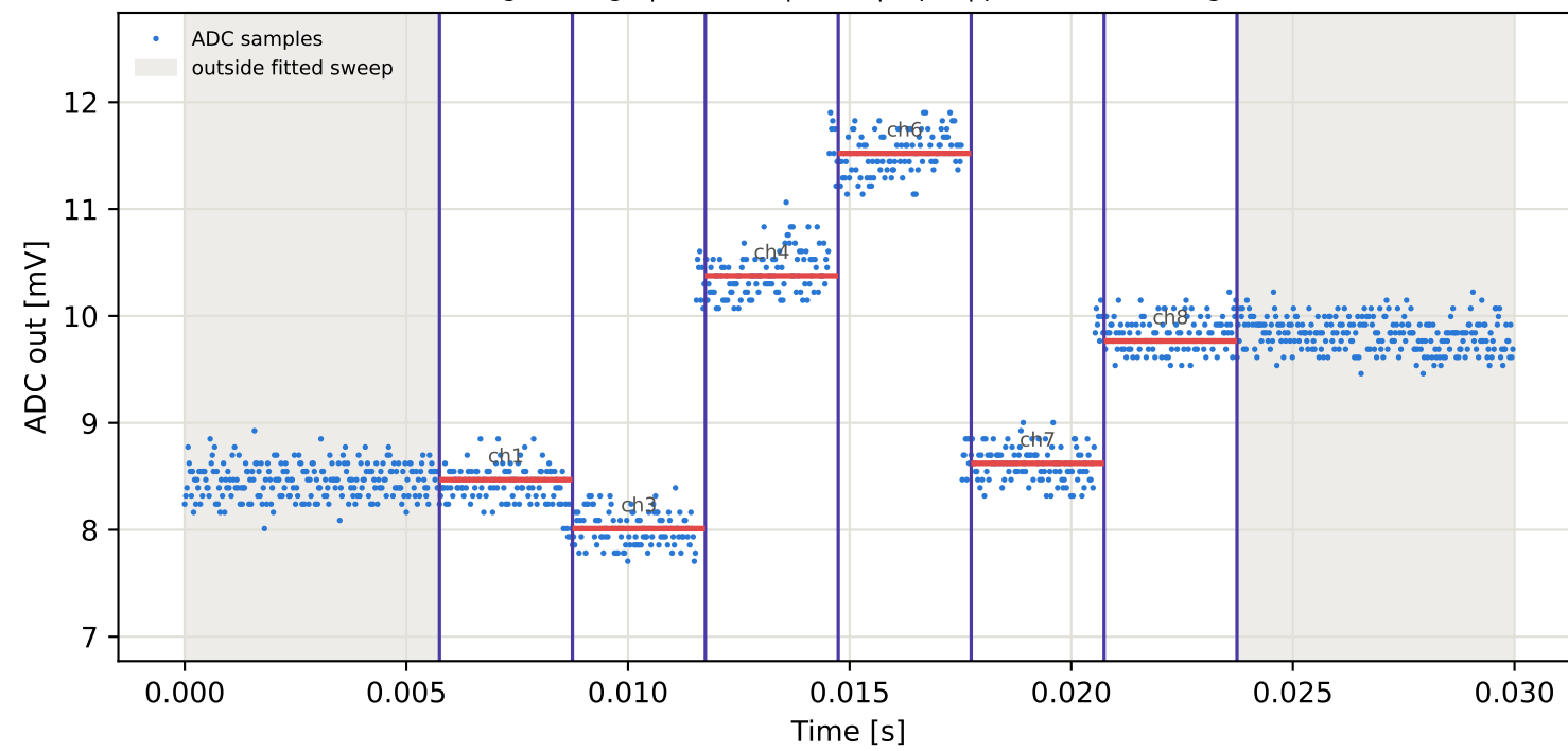
Tag2 &lt;- Tag5 | 995 MHz | run 0 | rep 1 | phase 57.12 deg
