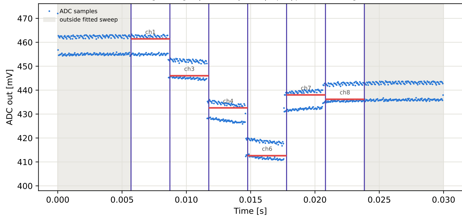
Tag1 &lt;- Tag2 | 895 MHz | run 0 | rep 1 | phase -164.31 deg
