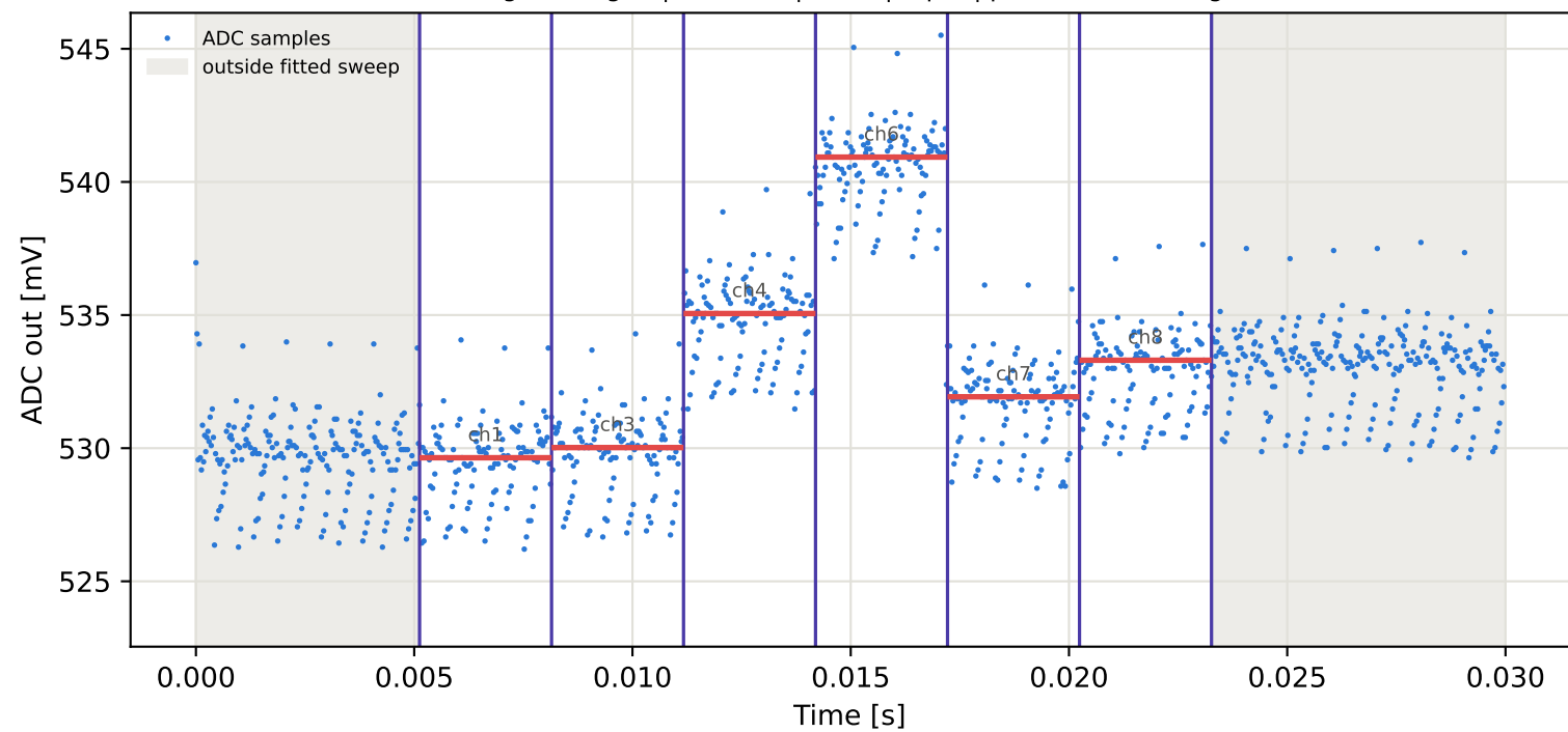
Tag8 &lt;- Tag16 | 955 MHz | run 0 | rep 1 | phase -103.80 deg
