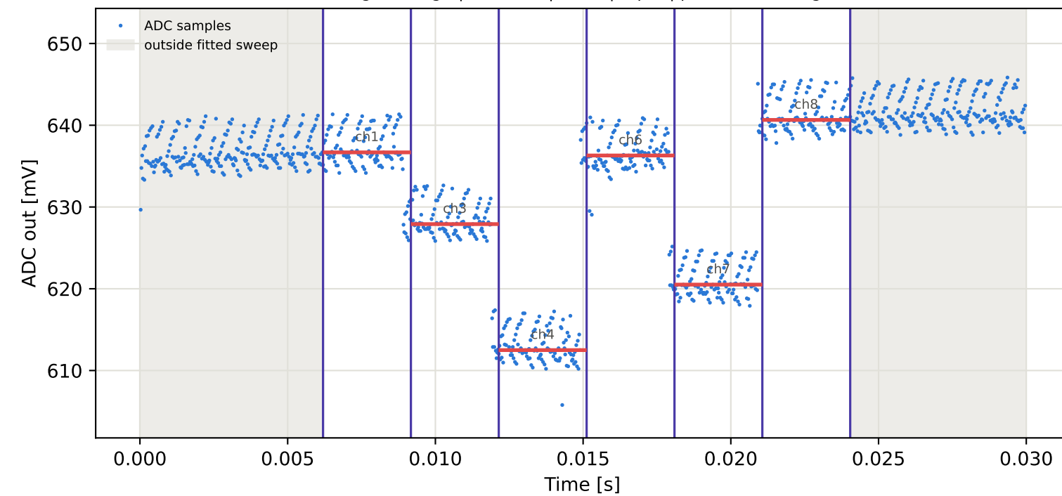
Tag5 &lt;- Tag8 | 965 MHz | run 0 | rep 1 | phase -170.71 deg
