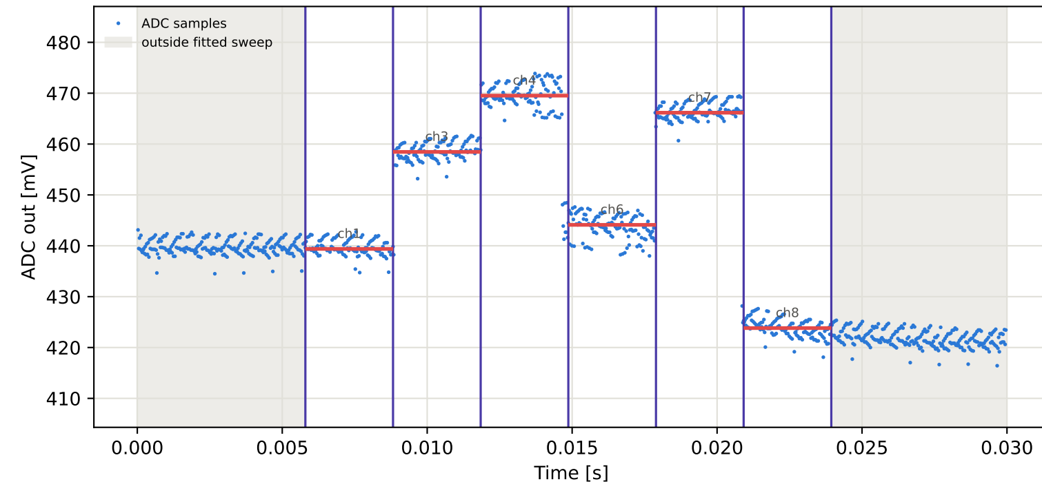
Tag9 &lt;- Tag7 | 895 MHz | run 0 | rep 1 | phase 162.73 deg
