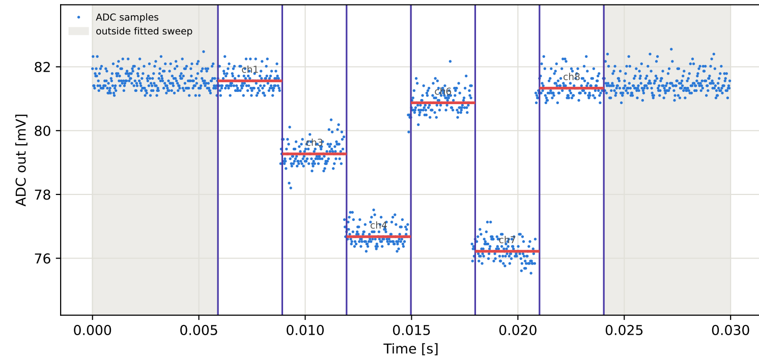
Tag3 &lt;- Tag2 | 785 MHz | run 0 | rep 1 | phase -94.02 deg
