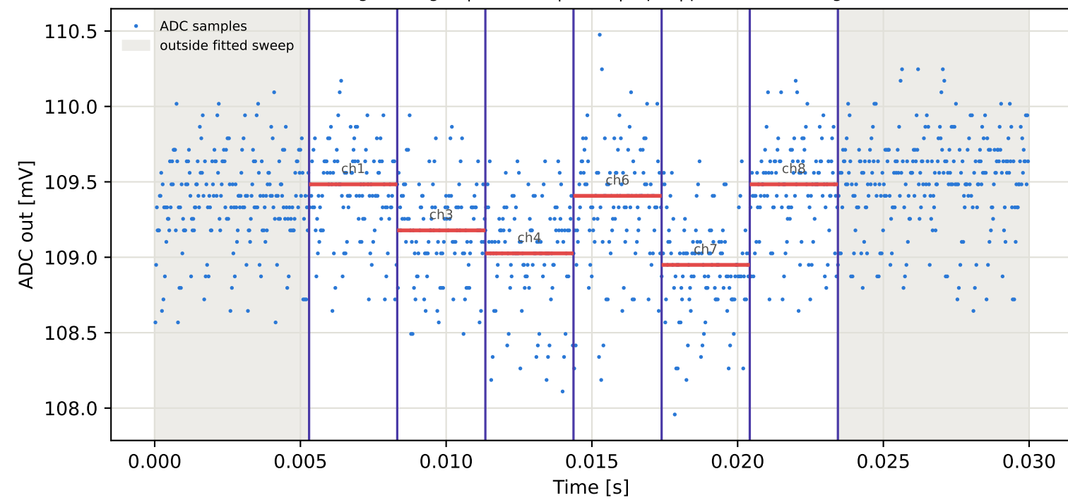
Tag8 &lt;- Tag16 | 775 MHz | run 0 | rep 1 | phase 34.61 deg
