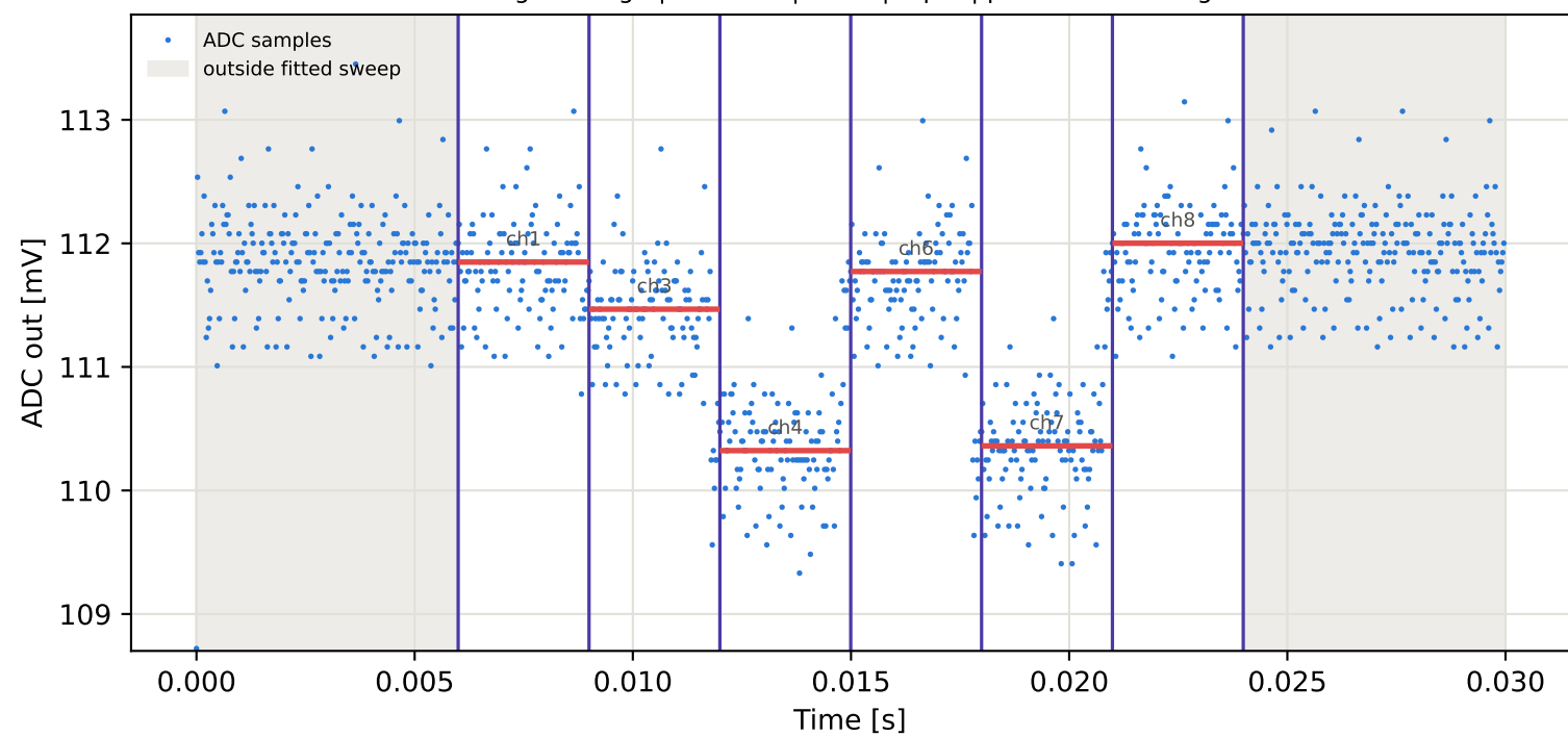
Tag3 &lt;- Tag15 | 775 MHz | run 0 | rep 1 | phase 85.96 deg
