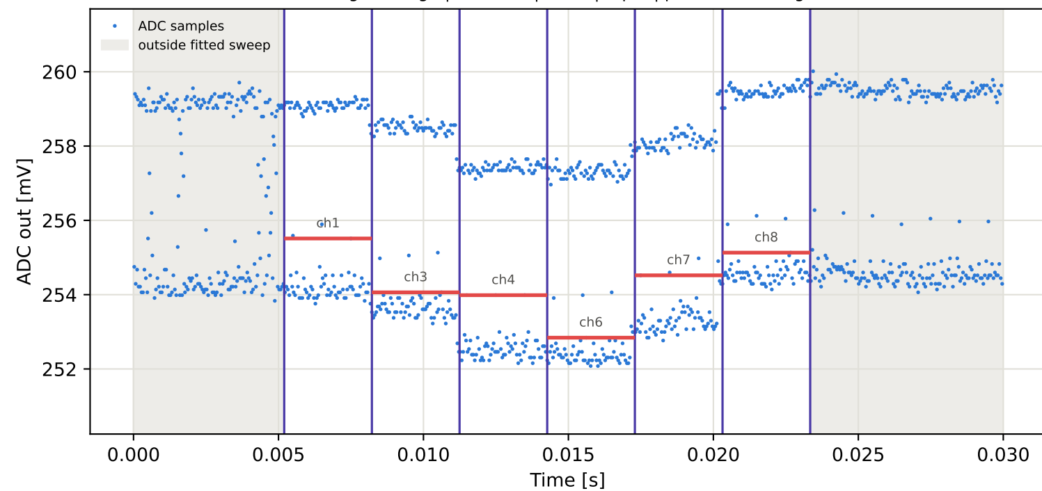
Tag3 &lt;- Tag2 | 995 MHz | run 0 | rep 1 | phase 35.89 deg
