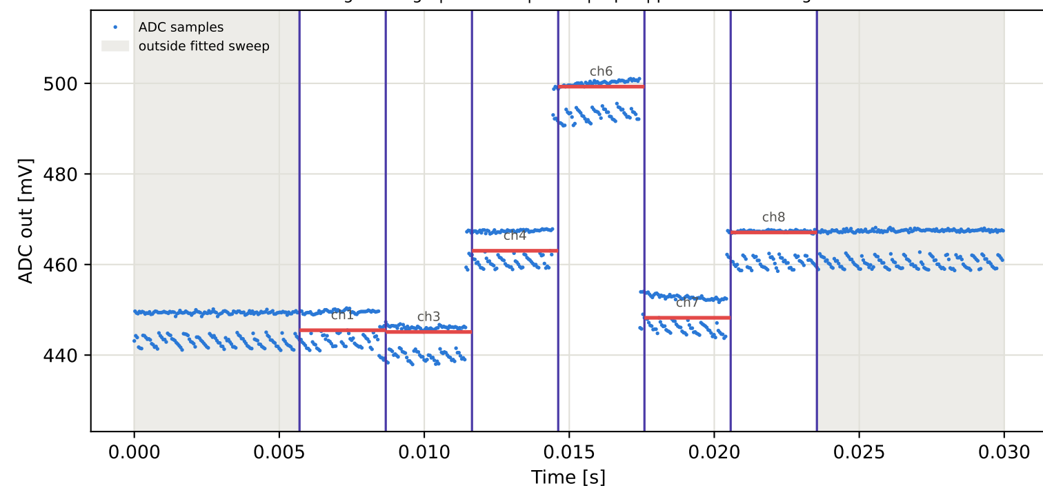
Tag4 &lt;- Tag3 | 965 MHz | run 0 | rep 1 | phase -165.25 deg
