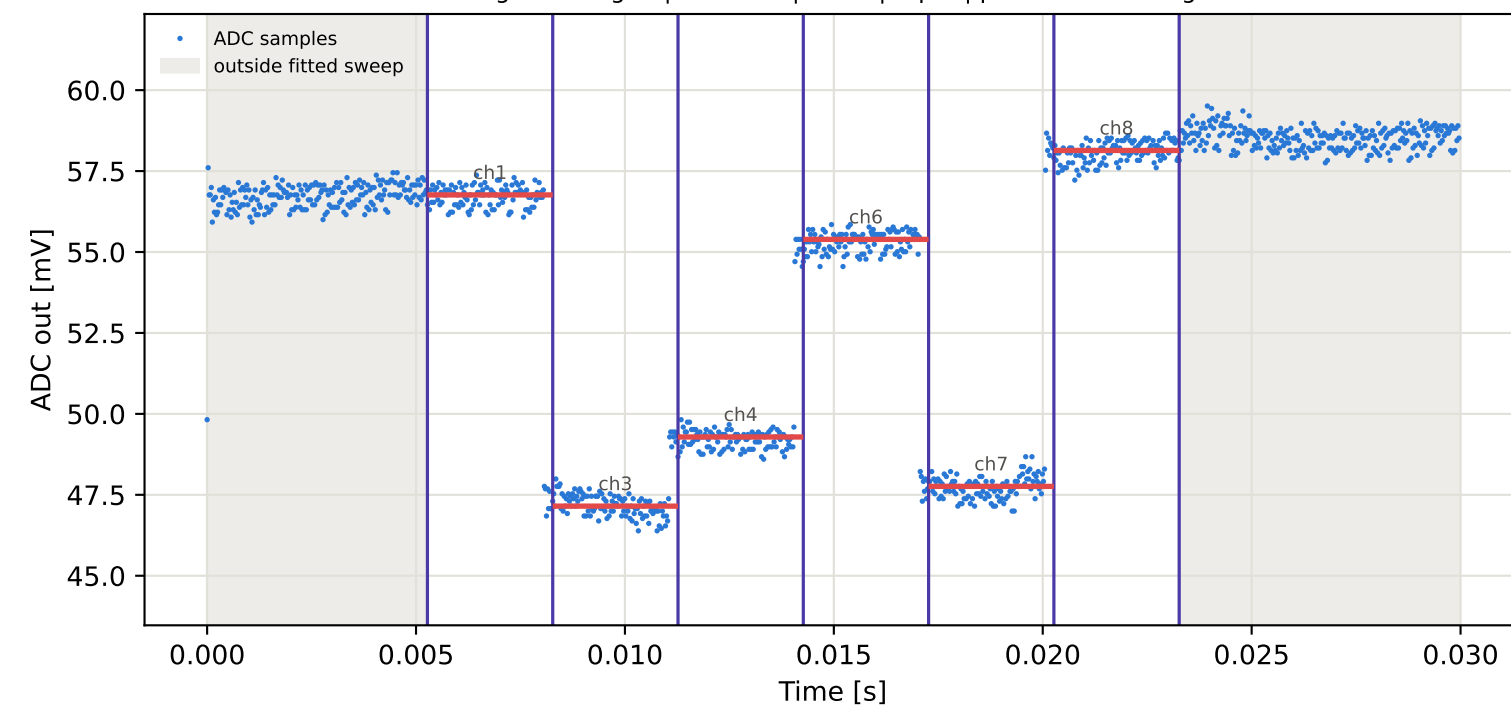
Tag10 &lt;- Tag2 | 855 MHz | run 0 | rep 1 | phase -70.83 deg
