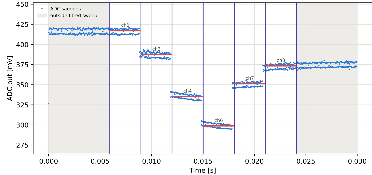
Tag4 &lt;- Tag3 | 885 MHz | run 0 | rep 1 | phase 45.79 deg
