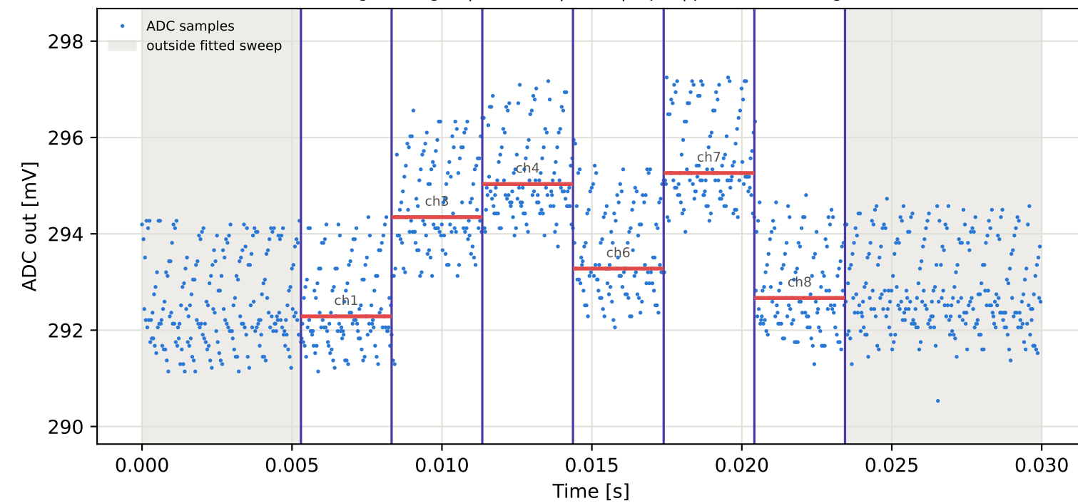
Tag5 &lt;- Tag16 | 825 MHz | run 0 | rep 1 | phase -62.11 deg
