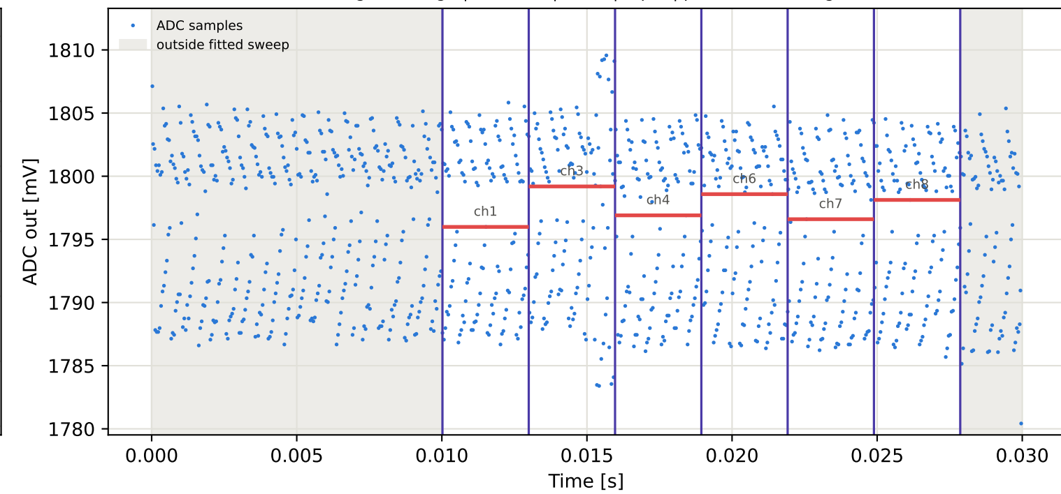
Tag15 &lt;- Tag4 | 915 MHz | run 0 | rep 1 | phase 49.27 deg
