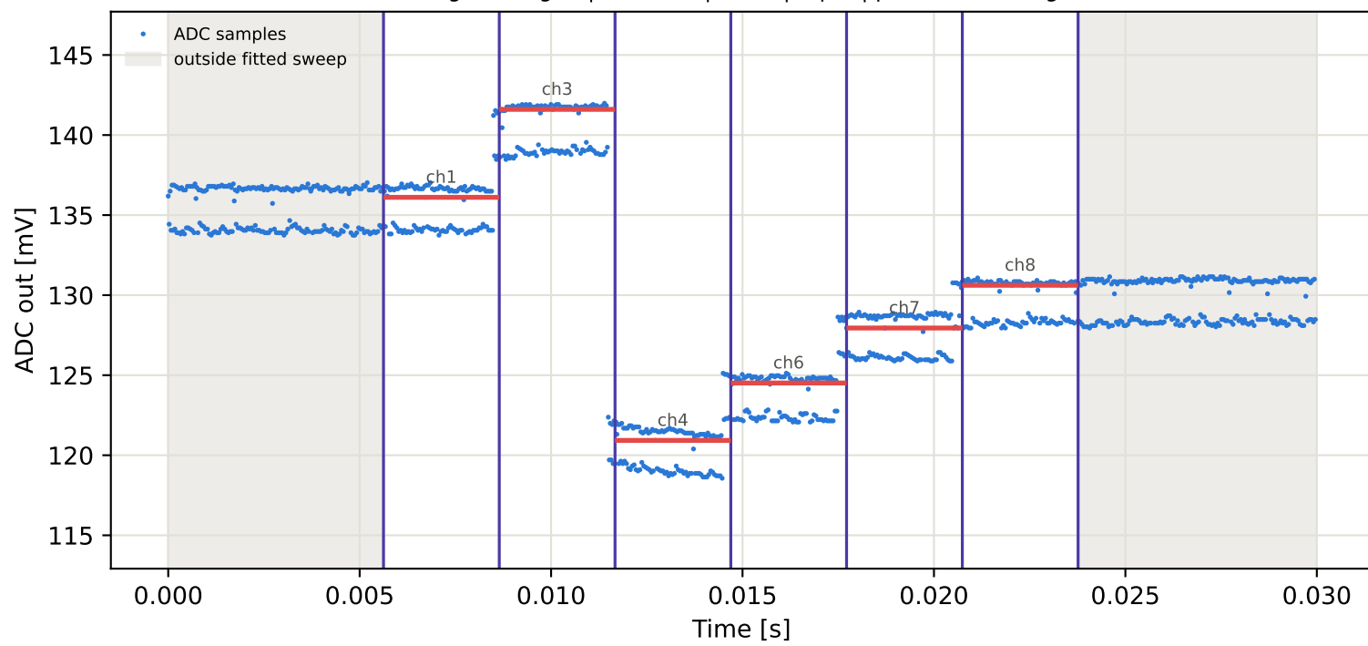
Tag8 &lt;- Tag16 | 785 MHz | run 0 | rep 1 | phase 61.84 deg
