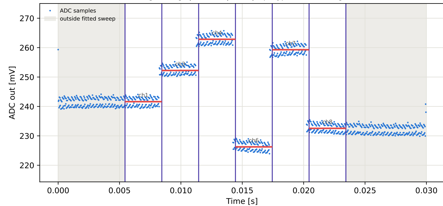
Tag3 &lt;- Tag6 | 995 MHz | run 0 | rep 1 | phase -42.03 deg
