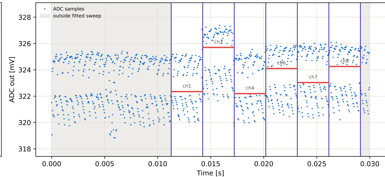
Tag9 &lt;- Tag2 | 995 MHz | run 0 | rep 1 | phase 62.91 deg
