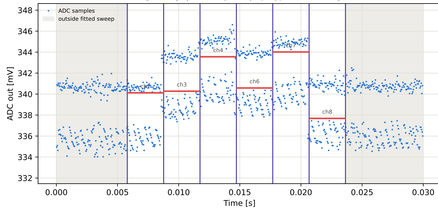
Tag3 &lt;- Tag10 | 885 MHz | run 0 | rep 1 | phase -30.94 deg
