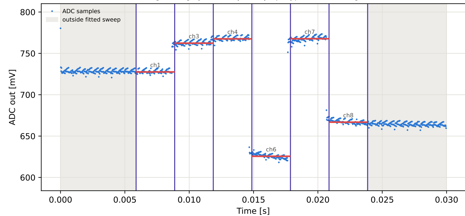
Tag9 &lt;- Tag6 | 935 MHz | run 0 | rep 1 | phase -58.84 deg
