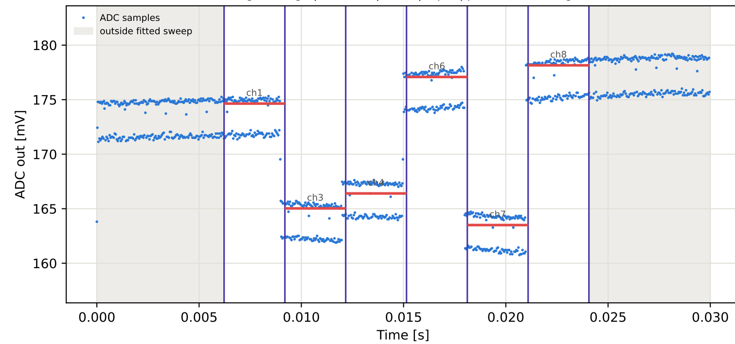
Tag6 &lt;- Tag9 | 805 MHz | run 0 | rep 1 | phase -136.17 deg
