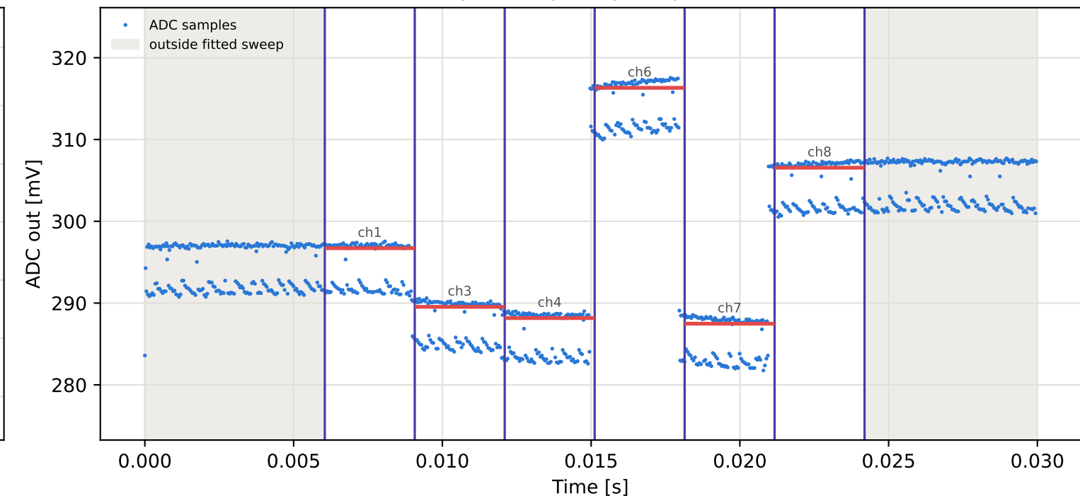
Tag5 &lt;- Tag1 | 985 MHz | run 0 | rep 1 | phase 156.82 deg
