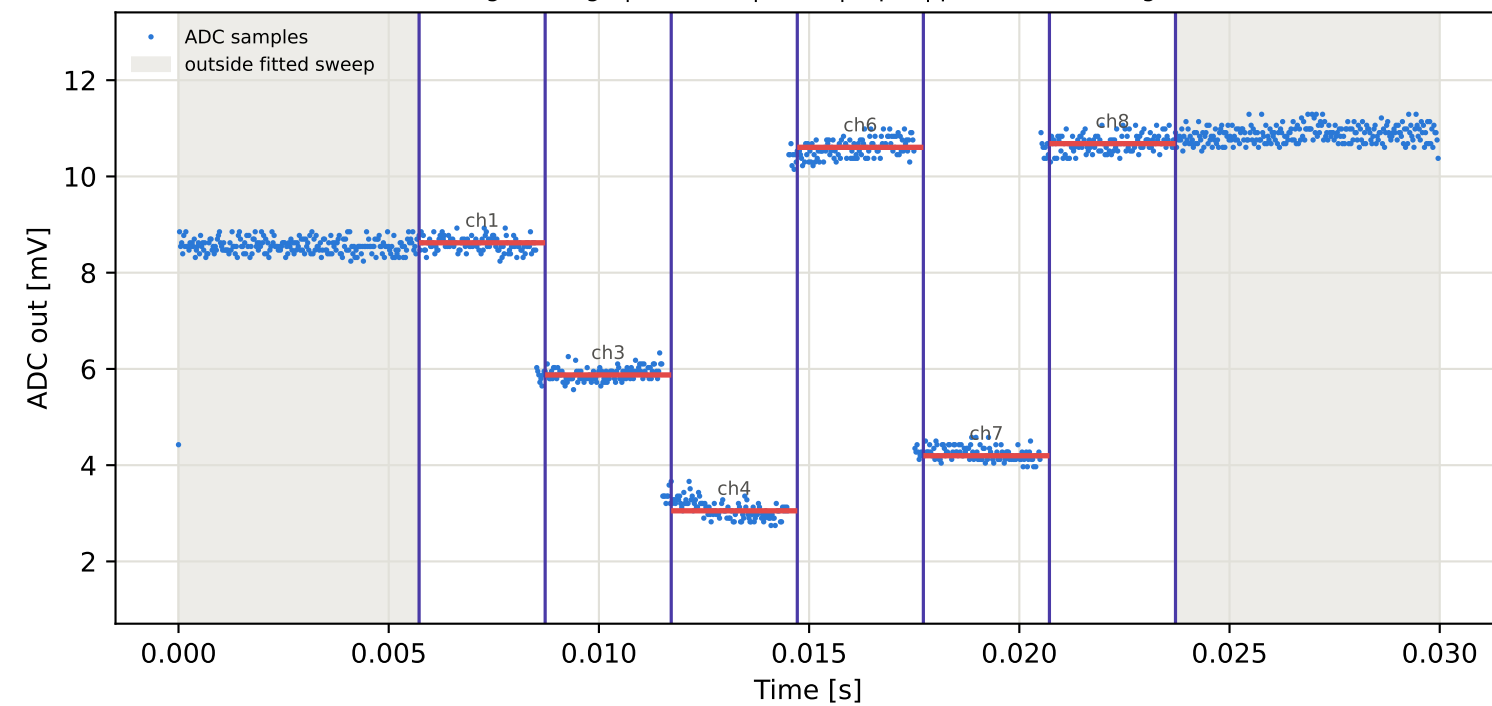
Tag2 &lt;- Tag7 | 965 MHz | run 0 | rep 1 | phase -128.21 deg
