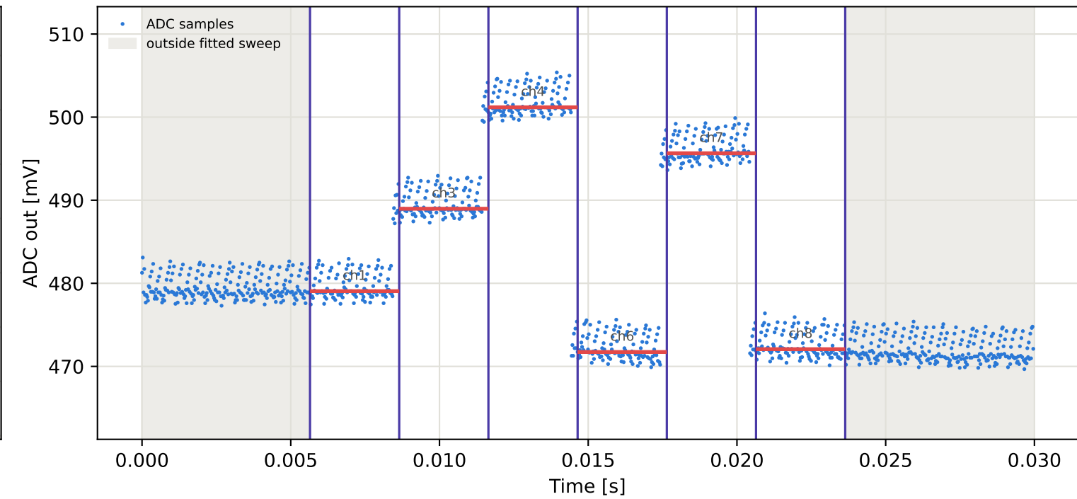
Tag10 &lt;- Tag1 | 975 MHz | run 0 | rep 1 | phase 123.81 deg
