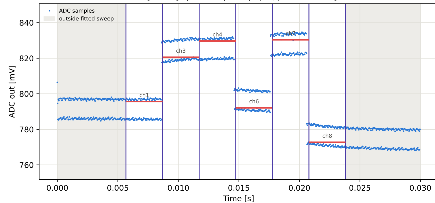
Tag3 &lt;- Tag8 | 865 MHz | run 0 | rep 1 | phase -51.37 deg
