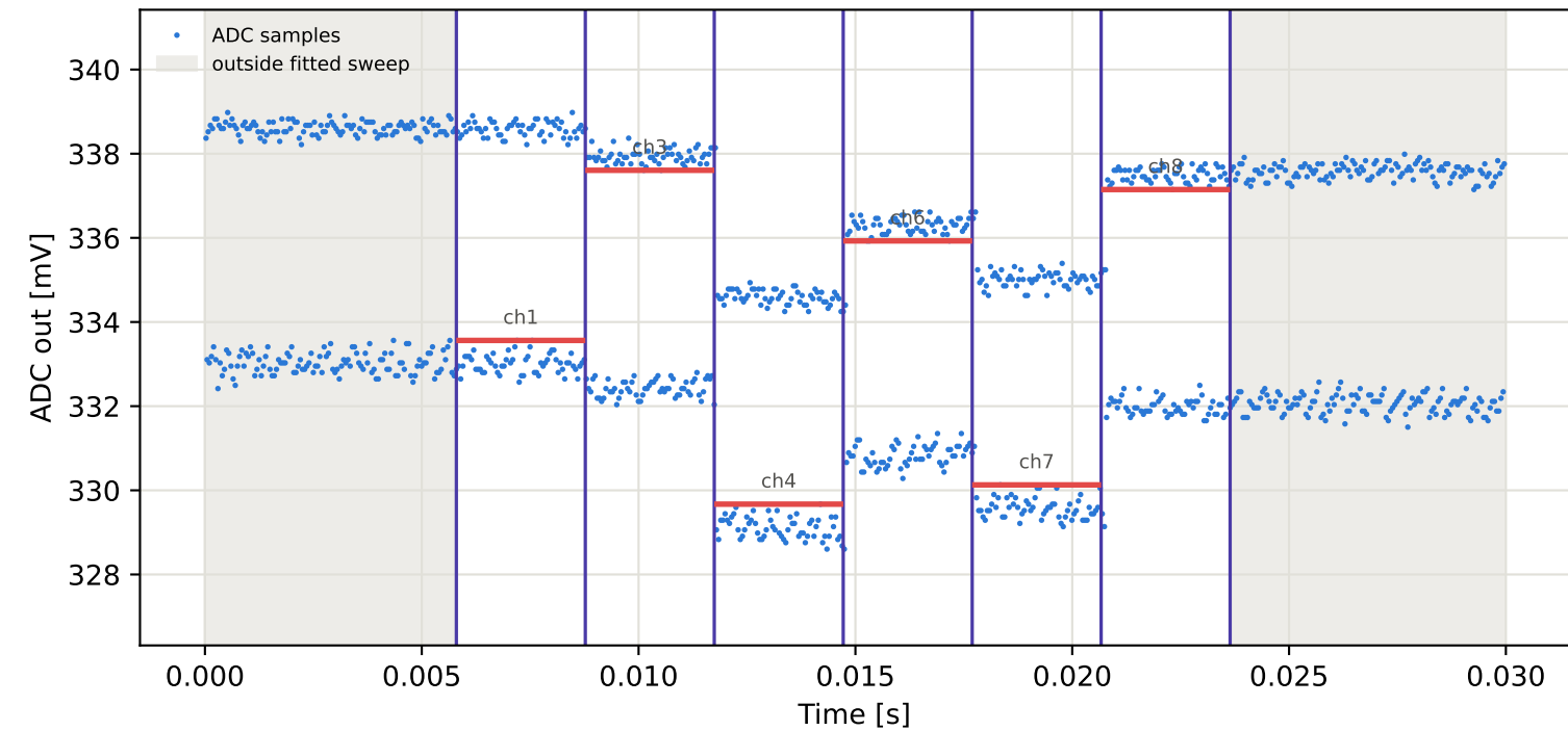
Tag8 &lt;- Tag7 | 805 MHz | run 0 | rep 1 | phase -149.81 deg
