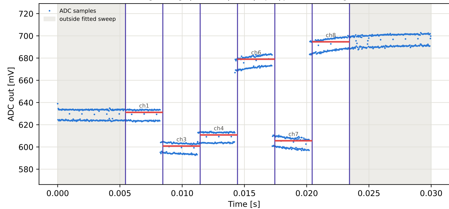
Tag1 &lt;- Tag8 | 885 MHz | run 0 | rep 1 | phase -136.92 deg
