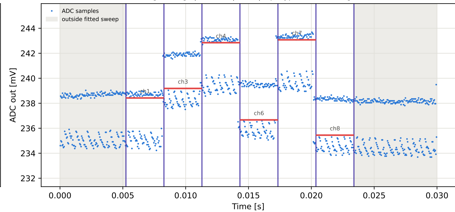
Tag8 &lt;- Tag10 | 825 MHz | run 0 | rep 1 | phase -64.64 deg
