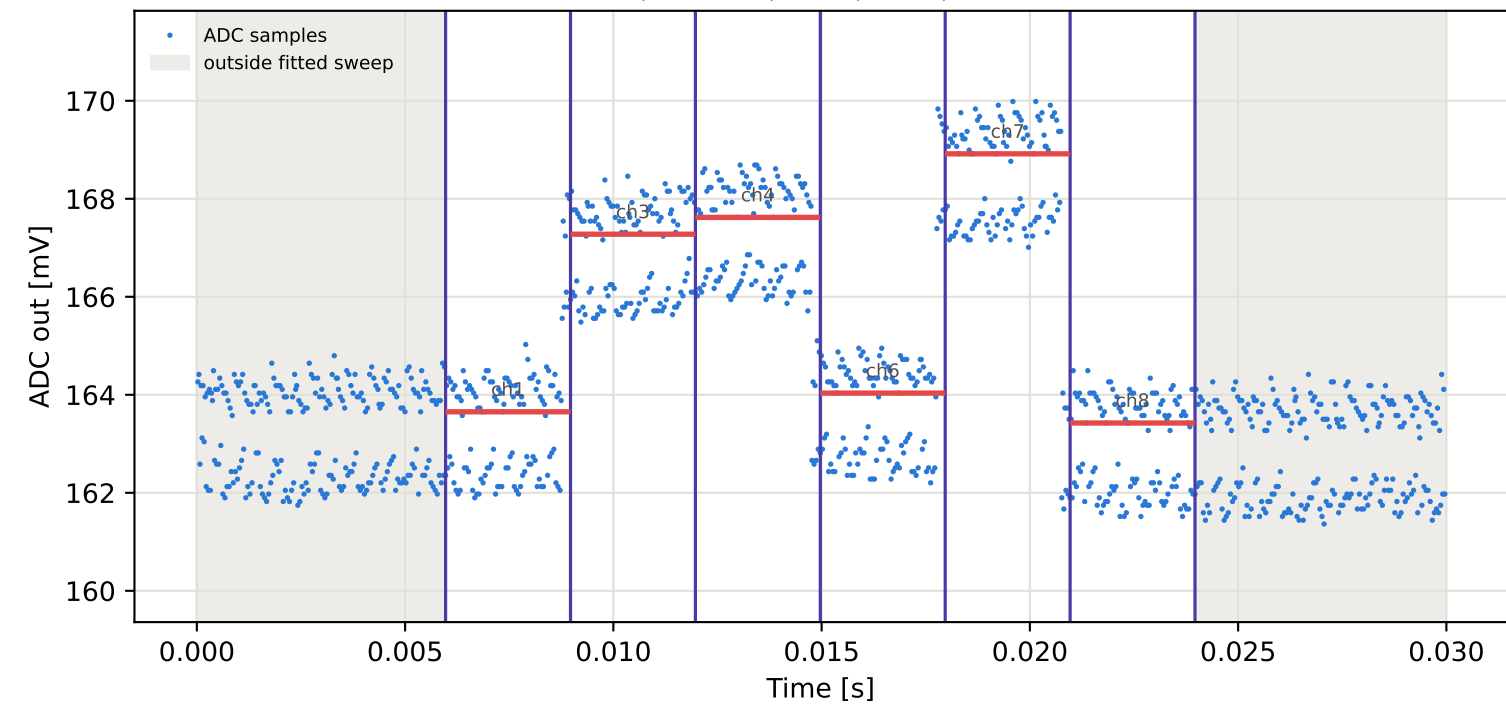
Tag6 &lt;- Tag5 | 805 MHz | run 0 | rep 1 | phase -44.91 deg
