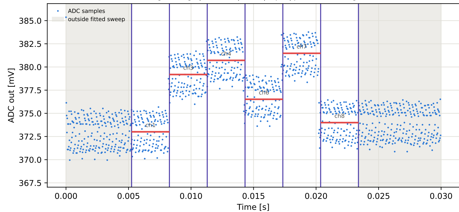
Tag3 &lt;- Tag7 | 835 MHz | run 0 | rep 1 | phase 83.60 deg
