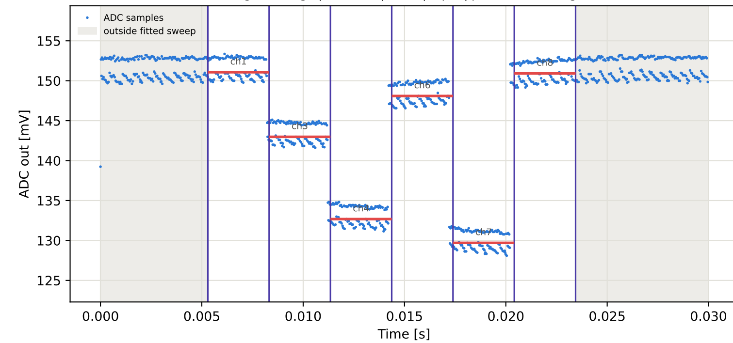
Tag2 &lt;- Tag1 | 775 MHz | run 0 | rep 1 | phase -95.91 deg
