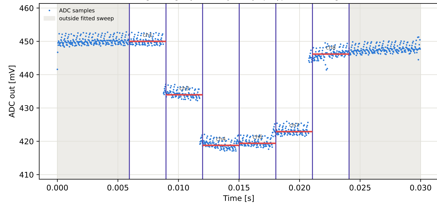
Tag1 &lt;- Tag16 | 895 MHz | run 0 | rep 1 | phase -42.05 deg
