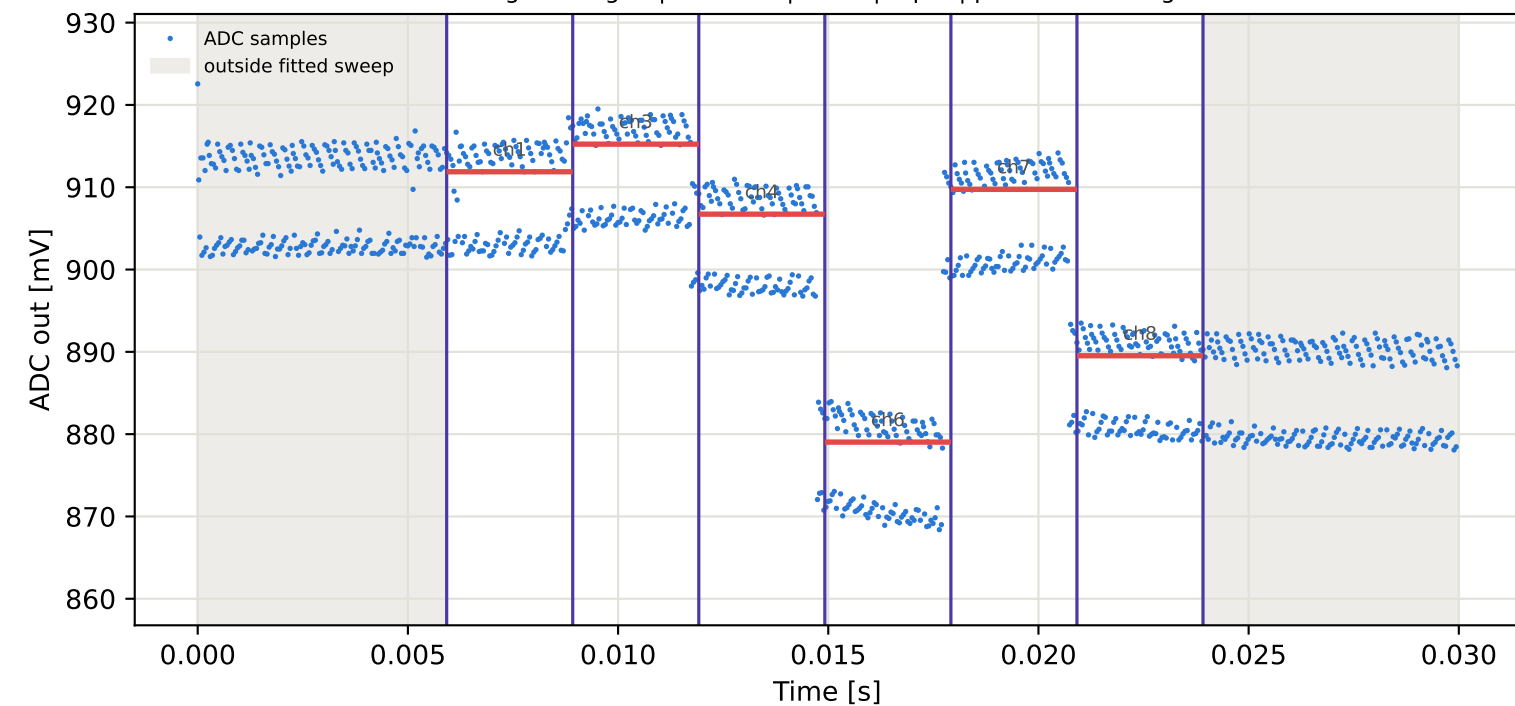
Tag1 &lt;- Tag2 | 905 MHz | run 0 | rep 1 | phase -125.94 deg
