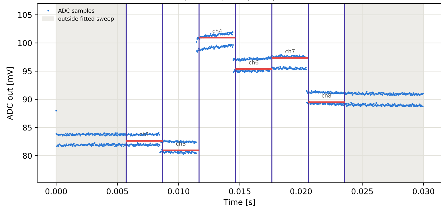
Tag8 &lt;- Tag1 | 805 MHz | run 0 | rep 1 | phase 128.48 deg
