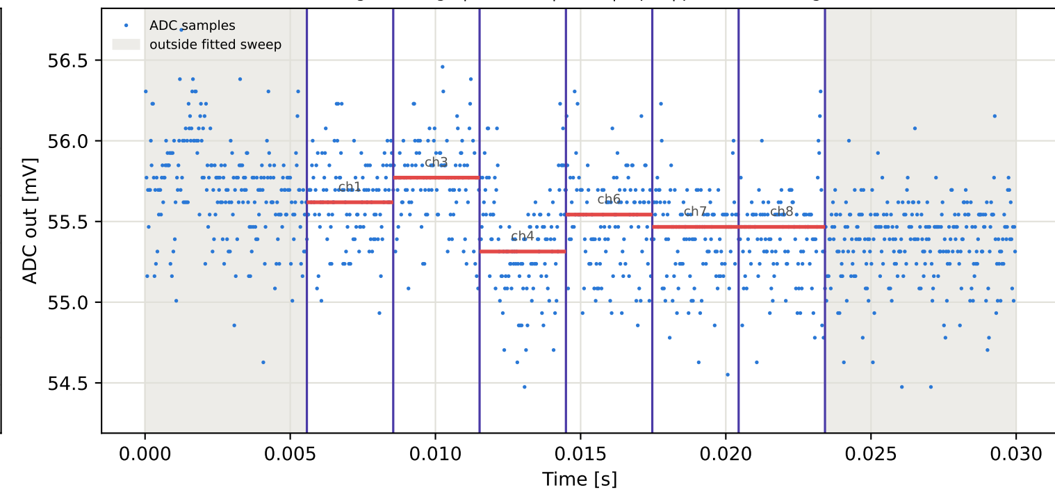
Tag10 &lt;- Tag9 | 785 MHz | run 0 | rep 1 | phase 160.42 deg
