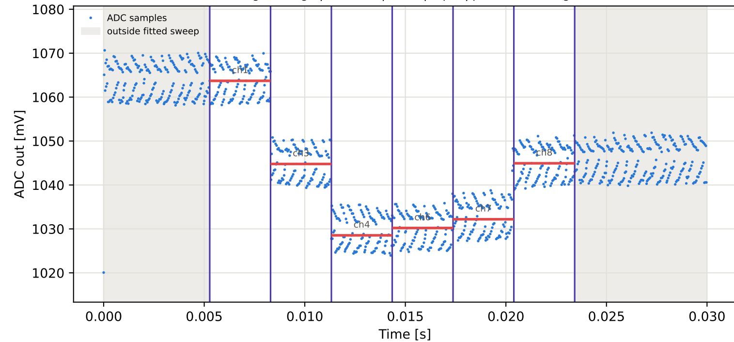
Tag8 &lt;- Tag7 | 855 MHz | run 0 | rep 1 | phase -12.67 deg
