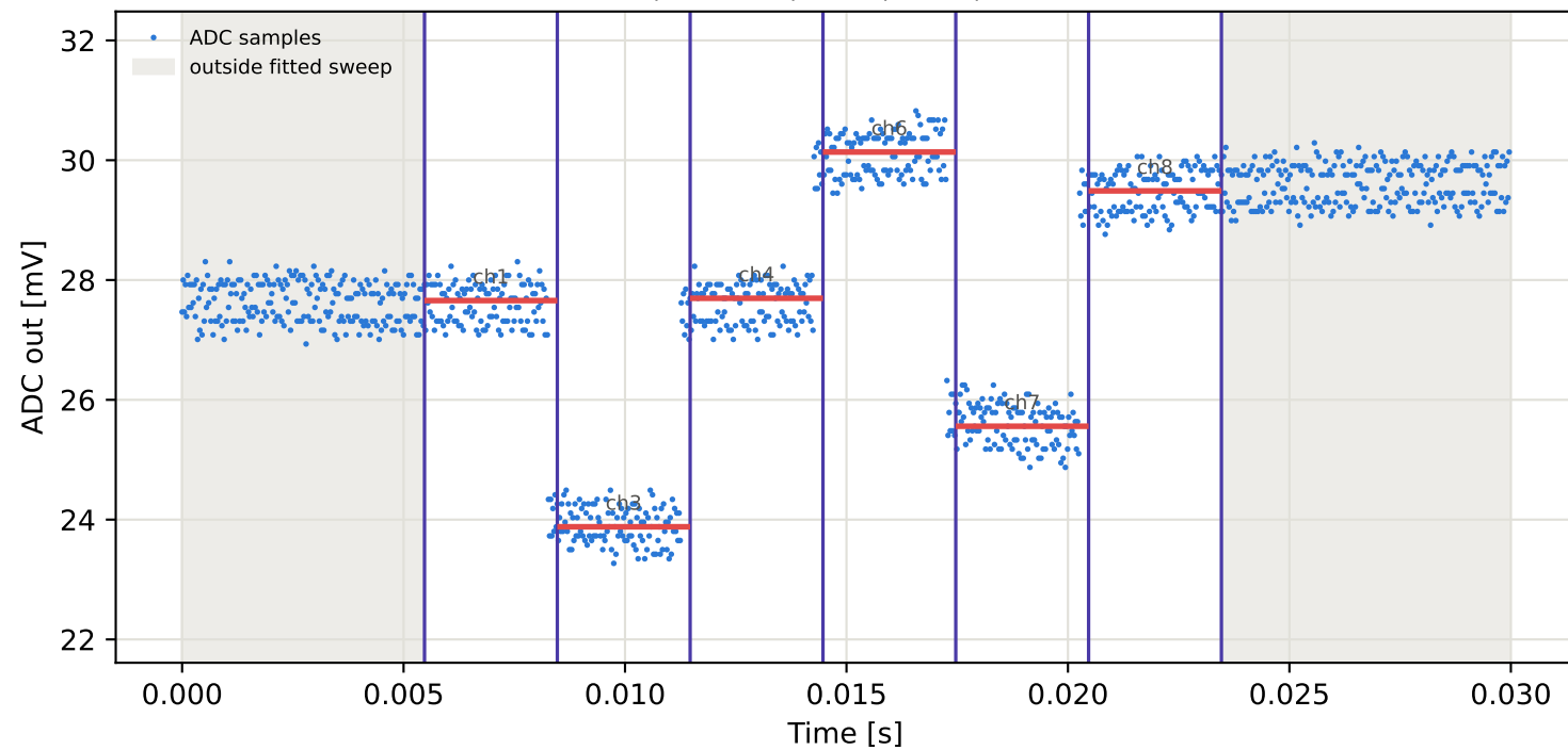
Tag2 &lt;- Tag15 | 825 MHz | run 0 | rep 1 | phase -164.56 deg
