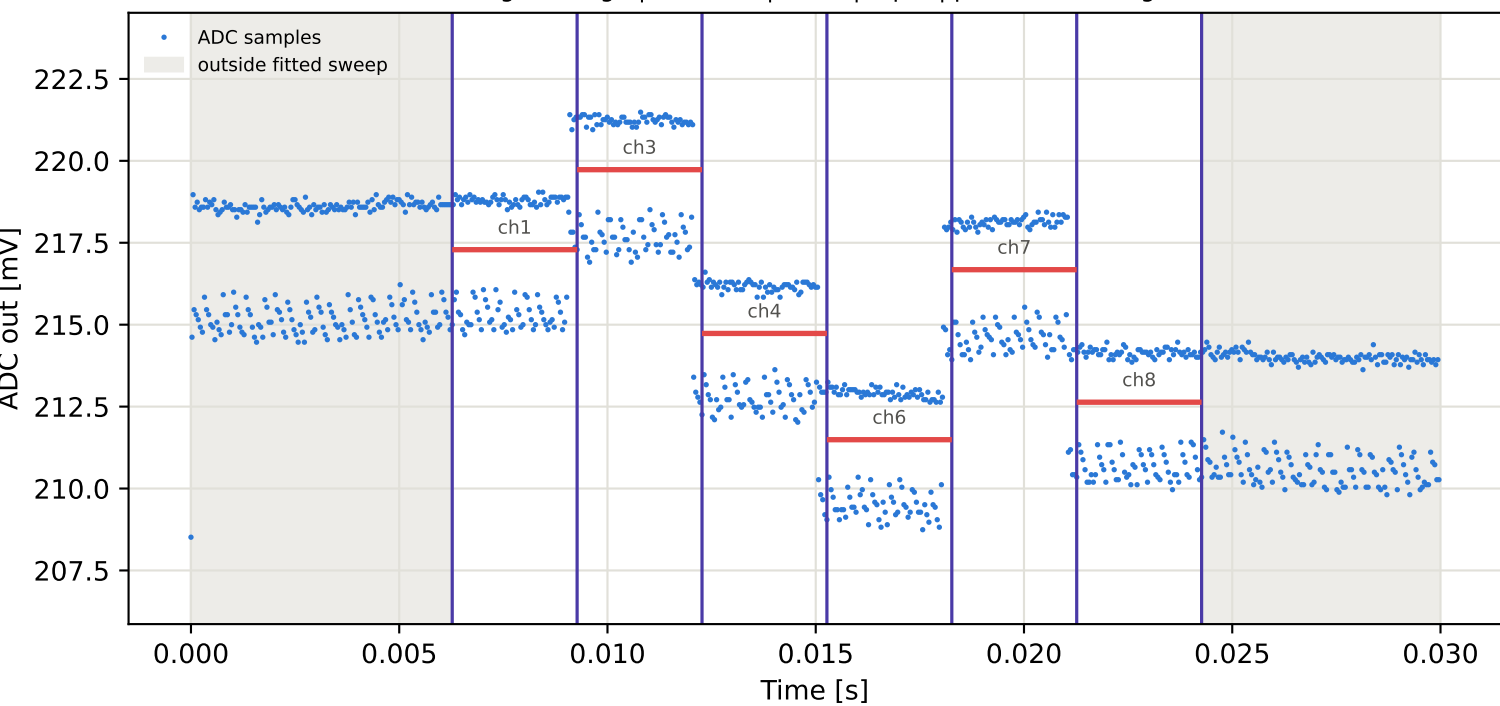
Tag1 &lt;- Tag9 | 855 MHz | run 0 | rep 1 | phase 24.24 deg
