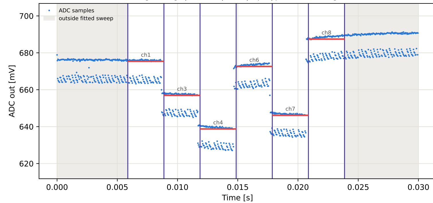
Tag1 &lt;- Tag7 | 925 MHz | run 0 | rep 1 | phase 108.47 deg
