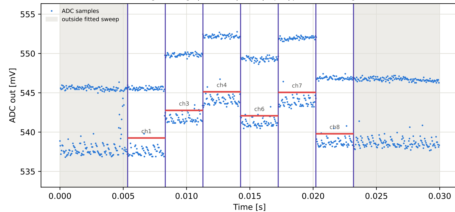
Tag15 &lt;- Tag9 | 865 MHz | run 0 | rep 1 | phase 155.99 deg
