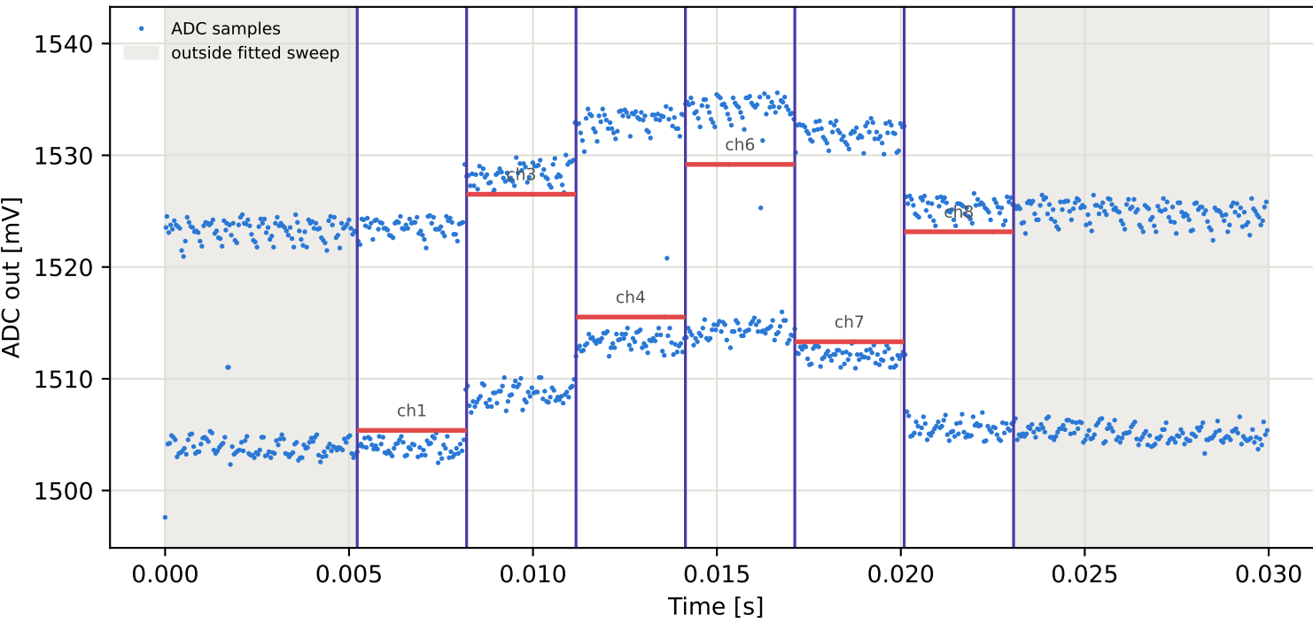
Tag15 &lt;- Tag1 | 895 MHz | run 0 | rep 1 | phase -166.78 deg
