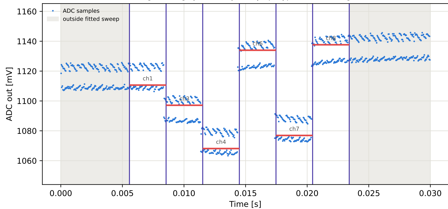
Tag2 &lt;- Tag10 | 945 MHz | run 0 | rep 1 | phase -29.85 deg
