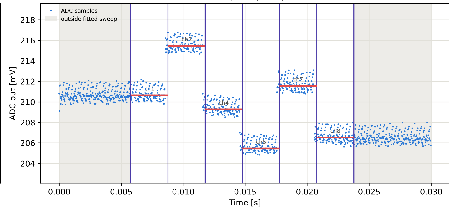
Tag3 &lt;- Tag7 | 825 MHz | run 0 | rep 1 | phase 38.53 deg
