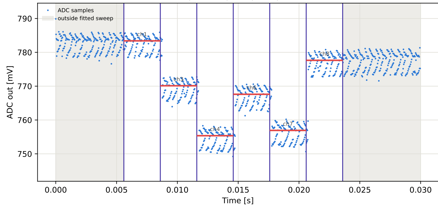
Tag16 &lt;- Tag6 | 835 MHz | run 0 | rep 1 | phase 89.34 deg
