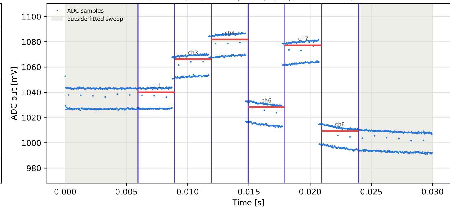
Tag10 &lt;- Tag3 | 915 MHz | run 0 | rep 1 | phase -68.57 deg
