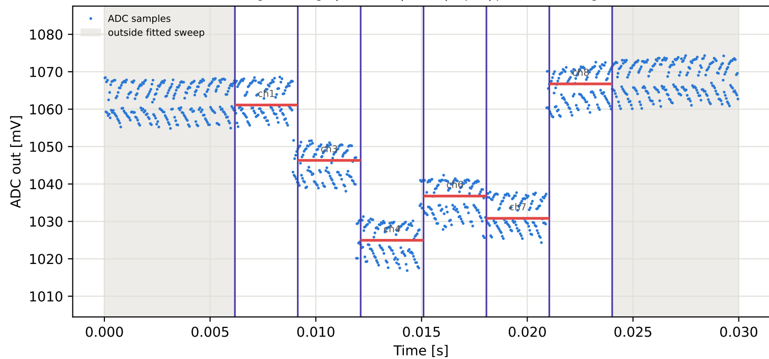
Tag10 &lt;- Tag9 | 915 MHz | run 0 | rep 1 | phase -101.29 deg
