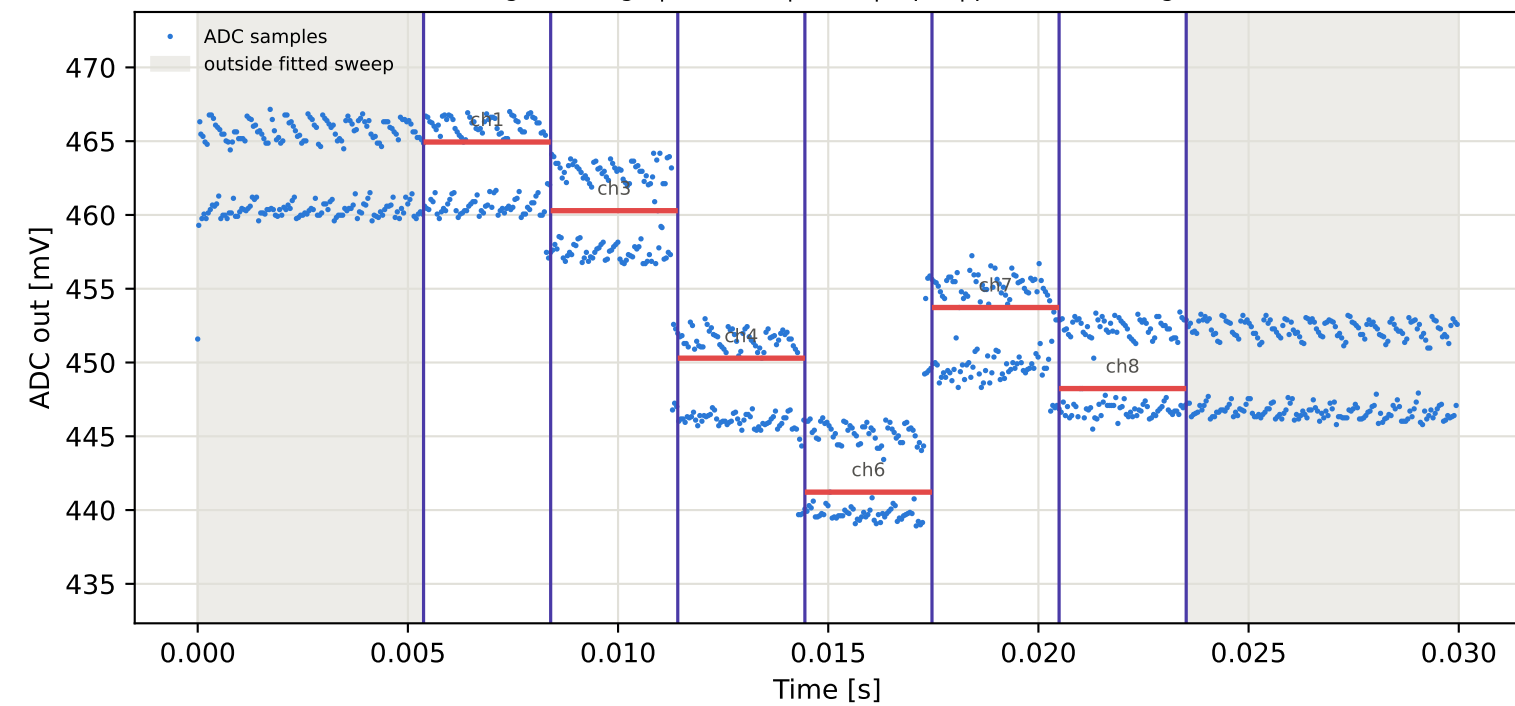
Tag10 &lt;- Tag9 | 875 MHz | run 0 | rep 1 | phase -121.93 deg
