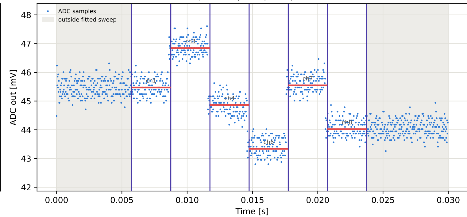
Tag1 &lt;- Tag8 | 795 MHz | run 0 | rep 1 | phase -23.94 deg
