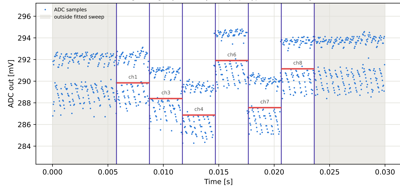
Tag5 &lt;- Tag16 | 985 MHz | run 0 | rep 1 | phase 133.86 deg
