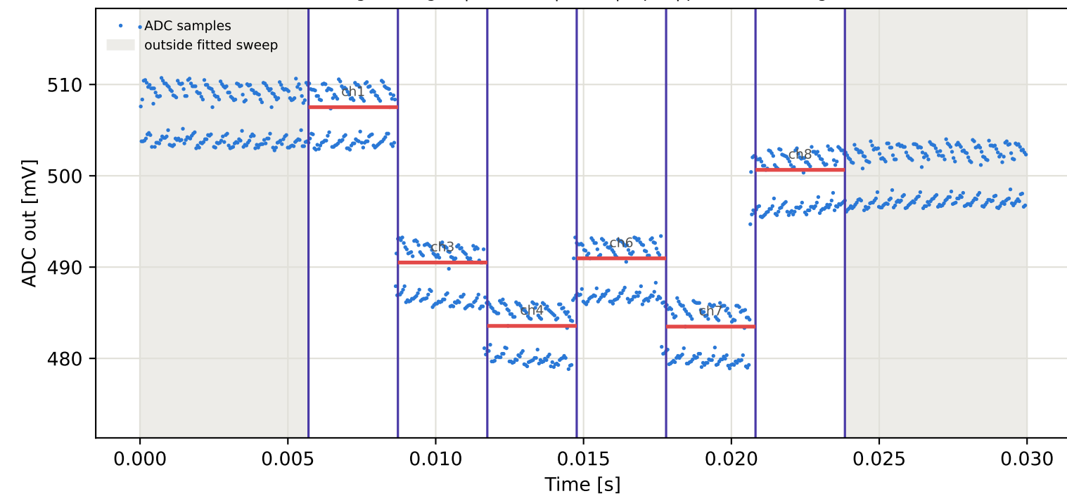
Tag6 &lt;- Tag2 | 865 MHz | run 0 | rep 1 | phase -83.57 deg
