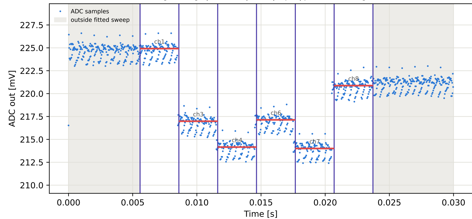
Tag9 &lt;- Tag15 | 855 MHz | run 0 | rep 1 | phase -160.63 deg
