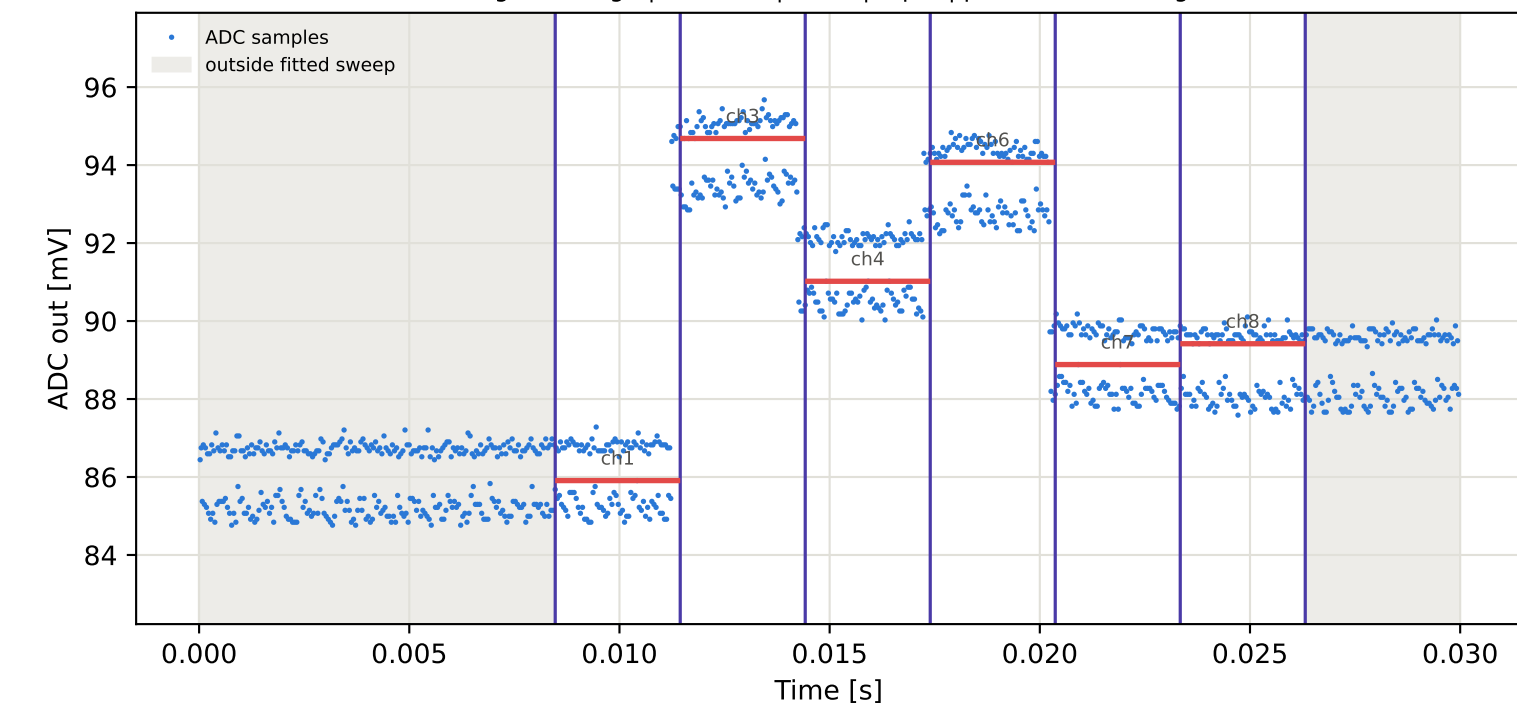
Tag10 &lt;- Tag4 | 805 MHz | run 0 | rep 1 | phase -123.79 deg
