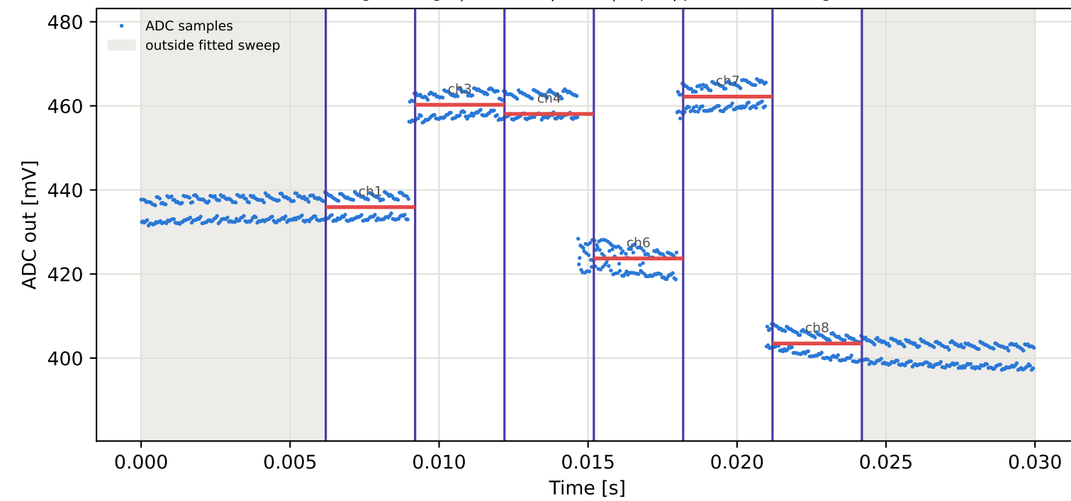
Tag2 &lt;- Tag5 | 875 MHz | run 0 | rep 1 | phase 118.45 deg
