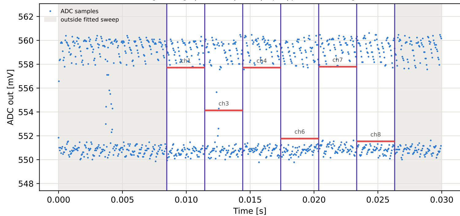
Tag8 &lt;- Tag4 | 995 MHz | run 0 | rep 1 | phase 144.99 deg
