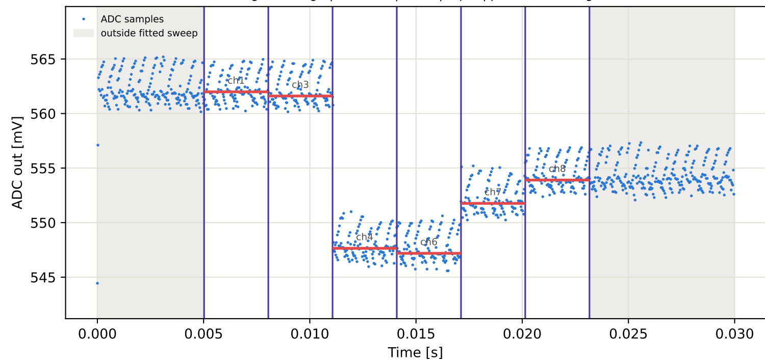
Tag16 &lt;- Tag6 | 825 MHz | run 0 | rep 1 | phase 55.50 deg
