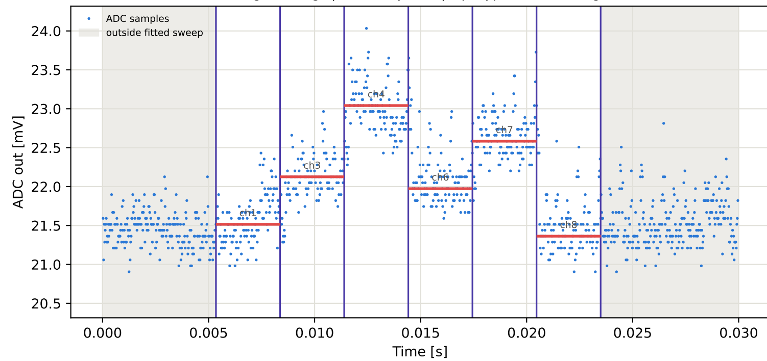
Tag10 &lt;- Tag9 | 845 MHz | run 0 | rep 1 | phase 131.42 deg
