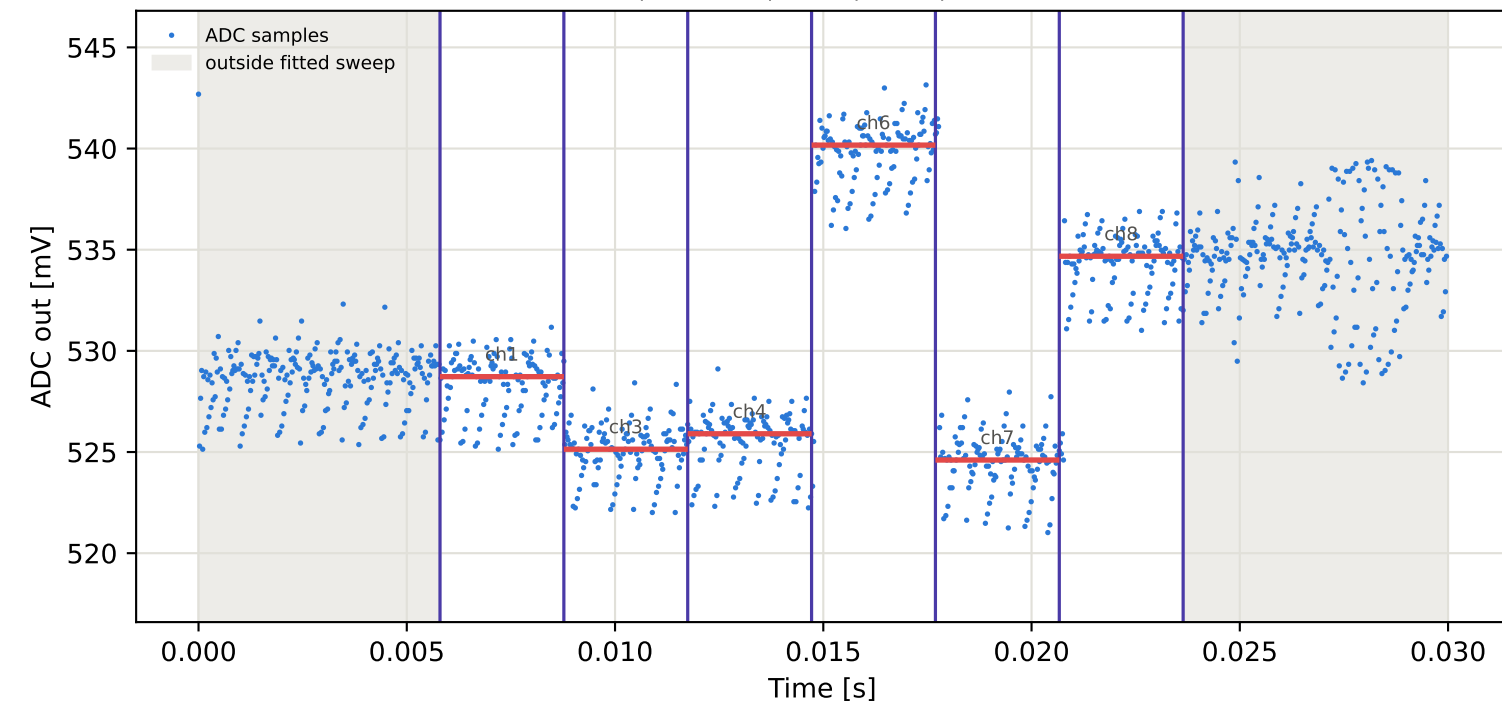
Tag7 &lt;- Tag5 | 975 MHz | run 0 | rep 1 | phase 165.87 deg
