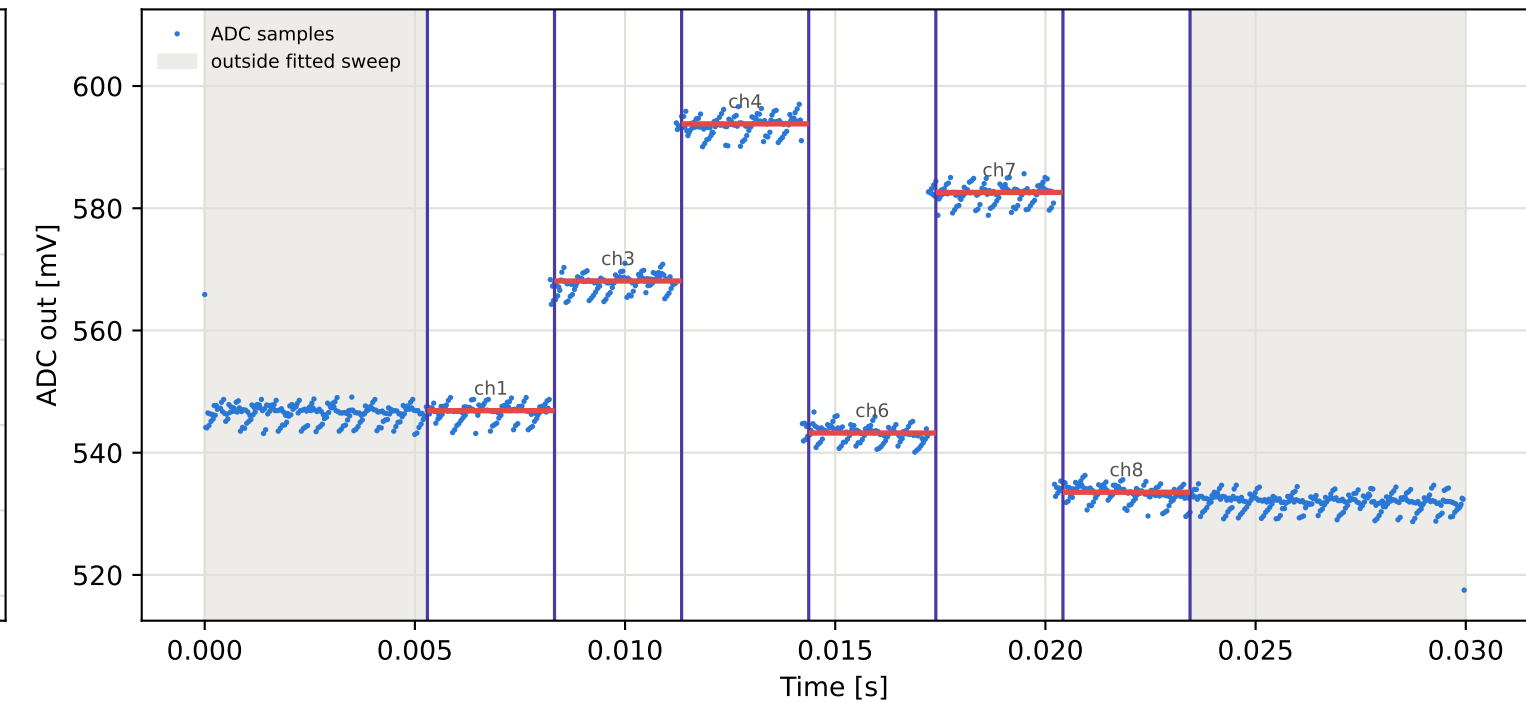
Tag9 &lt;- Tag2 | 965 MHz | run 0 | rep 1 | phase -16.43 deg
