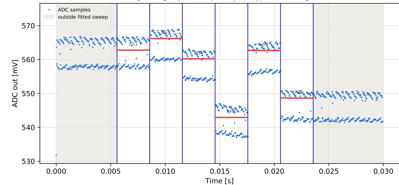
Tag7 &lt;- Tag15 | 895 MHz | run 0 | rep 1 | phase 9.65 deg
