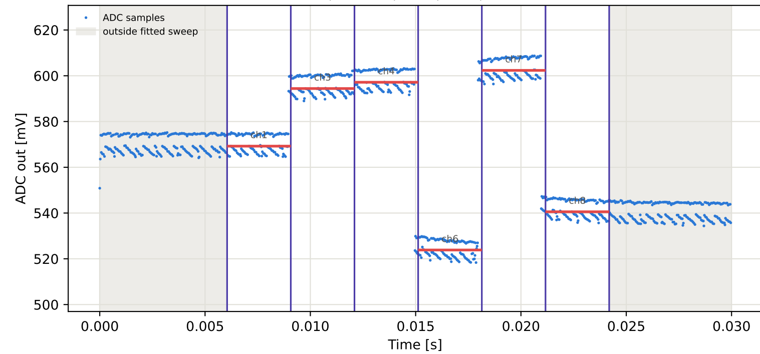
Tag9 &lt;- Tag16 | 985 MHz | run 0 | rep 1 | phase -27.91 deg
