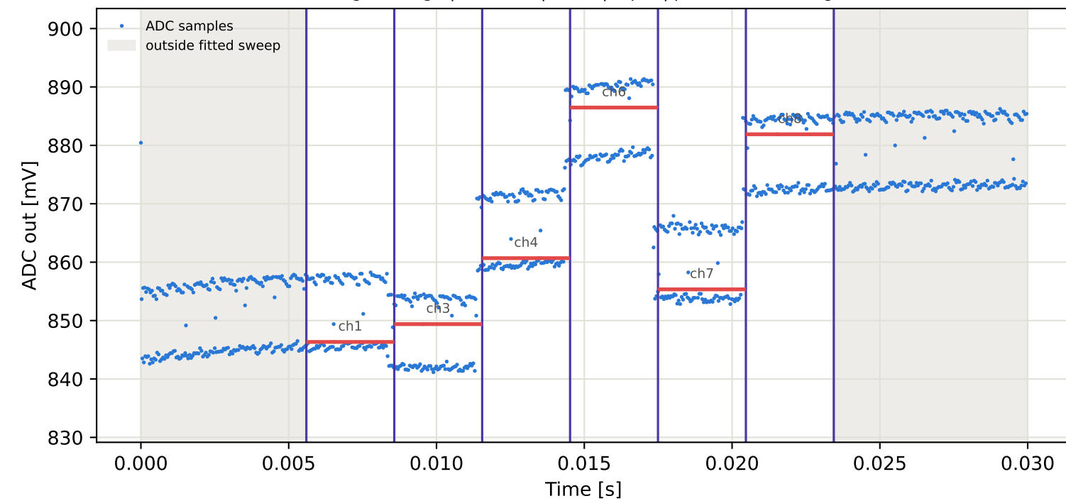
Tag6 &lt;- Tag9 | 875 MHz | run 0 | rep 1 | phase -88.53 deg
