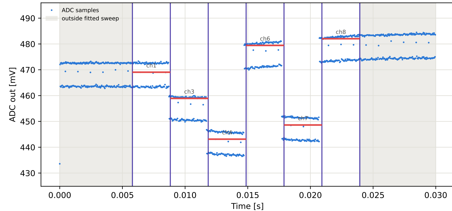
Tag5 &lt;- Tag3 | 945 MHz | run 0 | rep 1 | phase -16.34 deg
