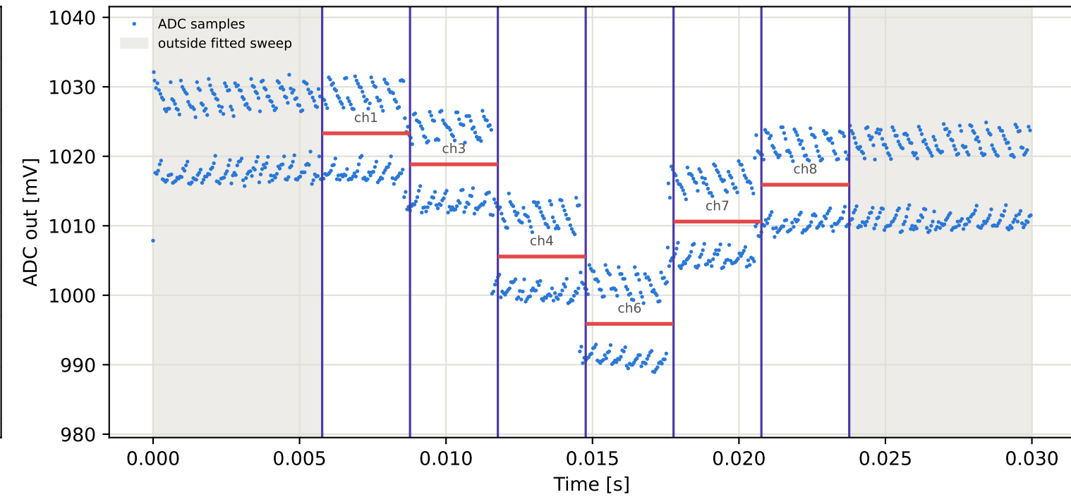
Tag16 &lt;- Tag15 | 915 MHz | run 0 | rep 1 | phase -173.54 deg
