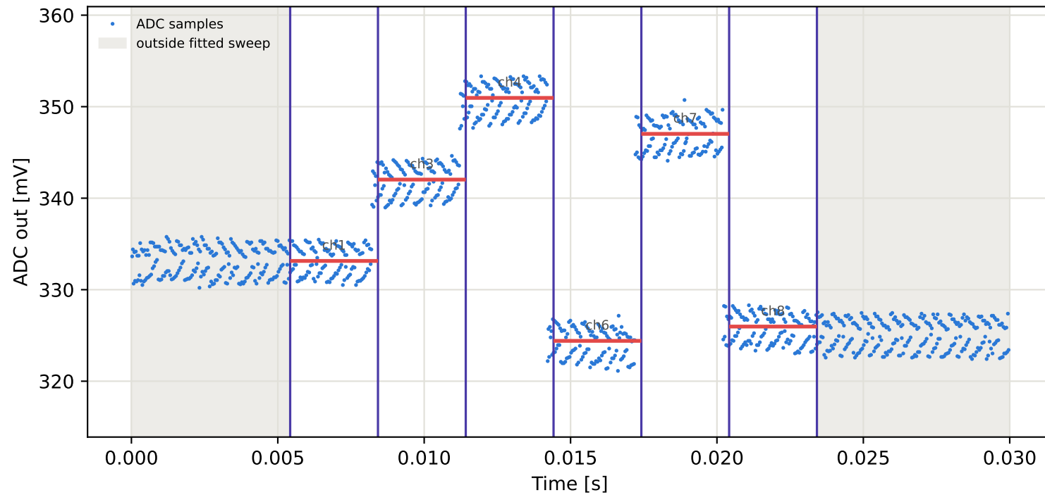
Tag15 &lt;- Tag1 | 965 MHz | run 0 | rep 1 | phase 130.77 deg
