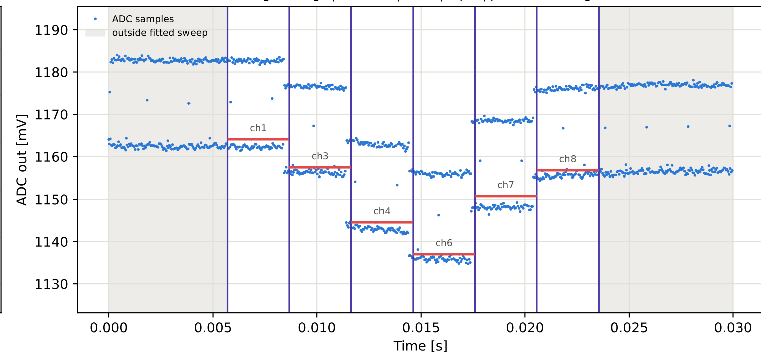
Tag6 &lt;- Tag5 | 915 MHz | run 0 | rep 1 | phase 44.57 deg
