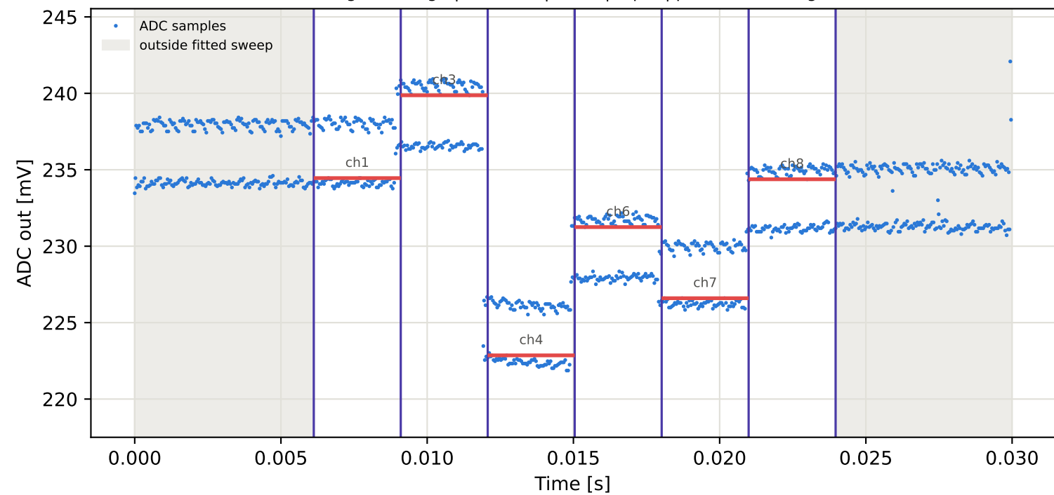
Tag15 &lt;- Tag6 | 775 MHz | run 0 | rep 1 | phase -12.35 deg
