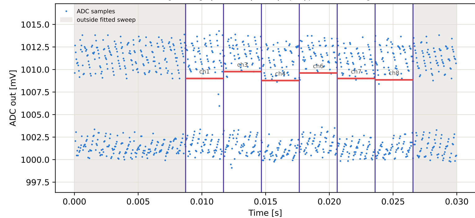
Tag8 &lt;- Tag4 | 865 MHz | run 0 | rep 1 | phase -103.59 deg
