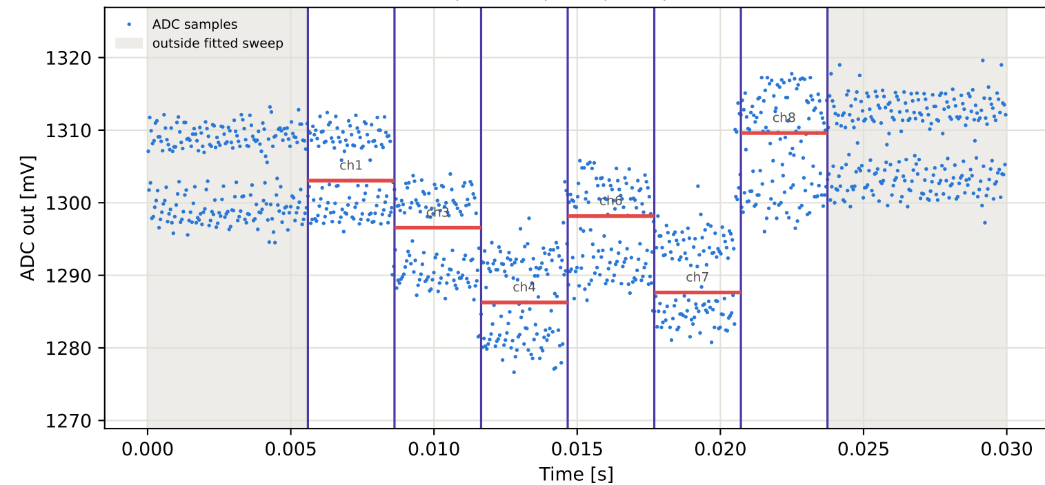
Tag3 &lt;- Tag2 | 885 MHz | run 0 | rep 1 | phase 96.77 deg
