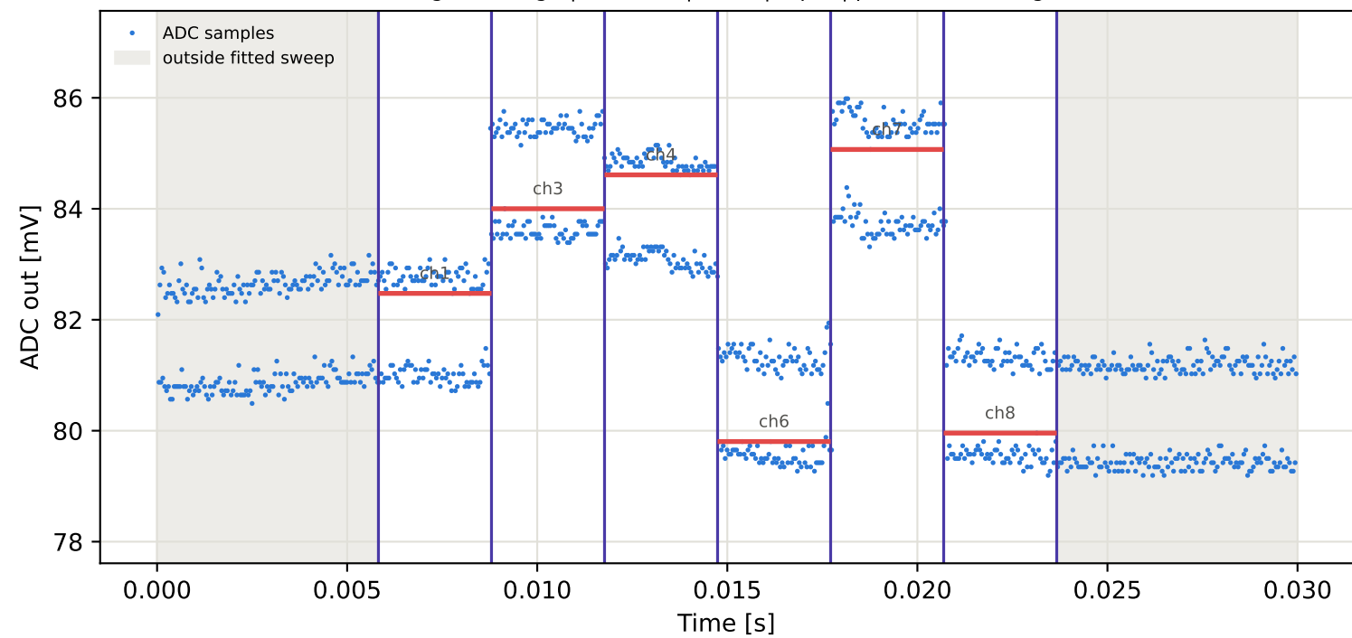
Tag10 &lt;- Tag9 | 825 MHz | run 0 | rep 1 | phase -154.53 deg
