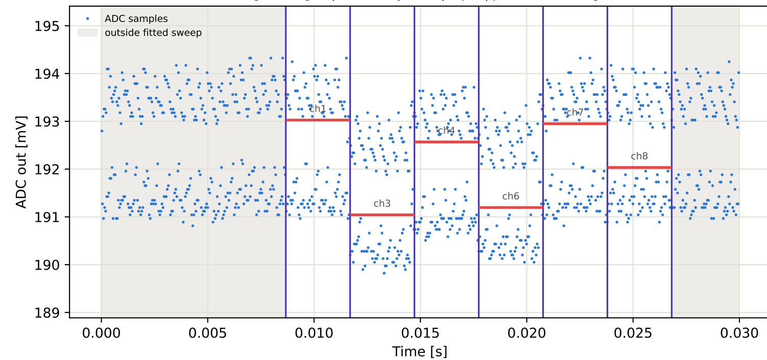
Tag5 &lt;- Tag16 | 775 MHz | run 0 | rep 1 | phase -172.73 deg
