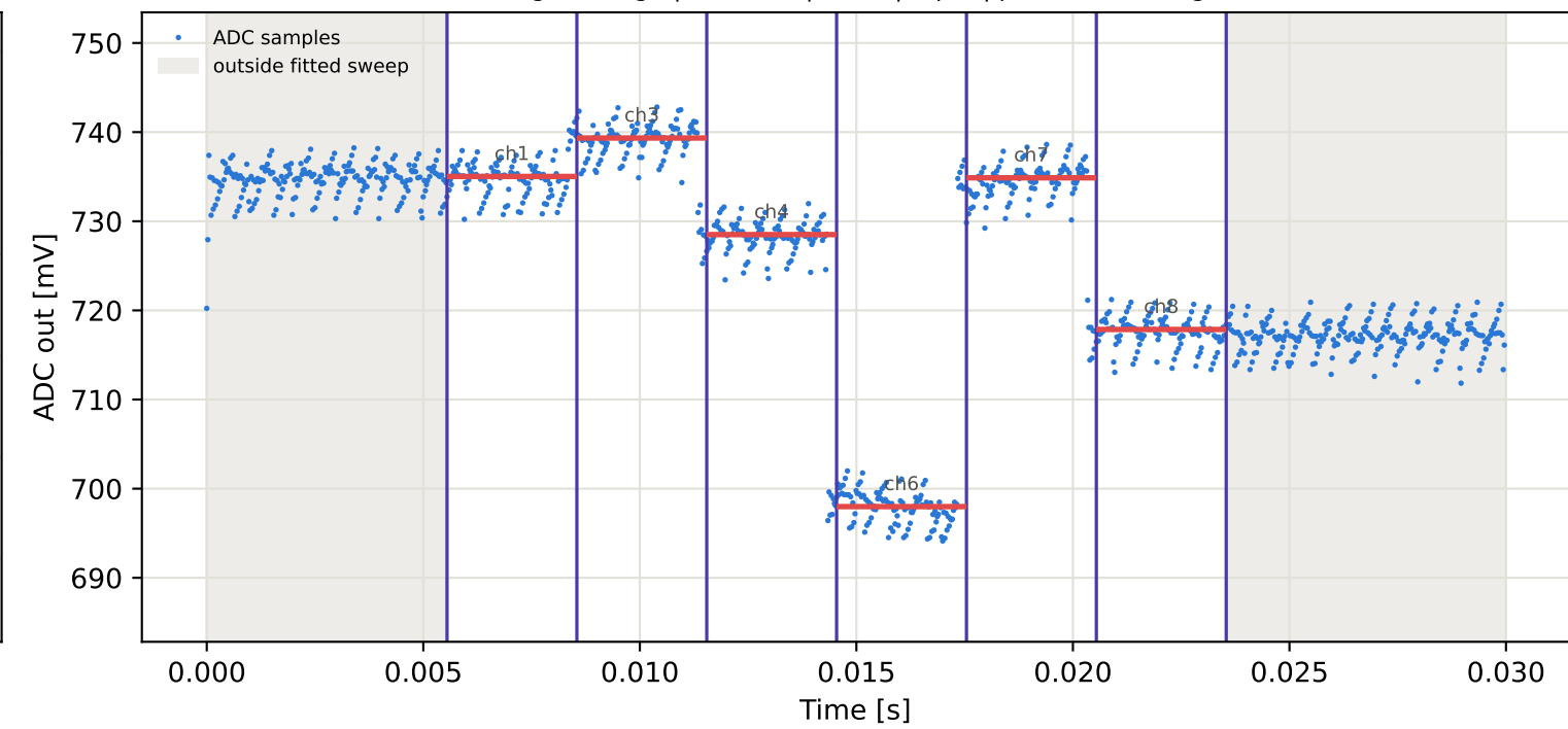
Tag9 &lt;- Tag15 | 935 MHz | run 0 | rep 1 | phase -144.05 deg
