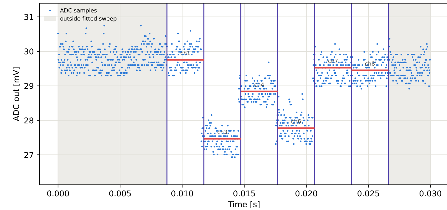
Tag6 &lt;- Tag10 | 775 MHz | run 0 | rep 1 | phase 45.93 deg
