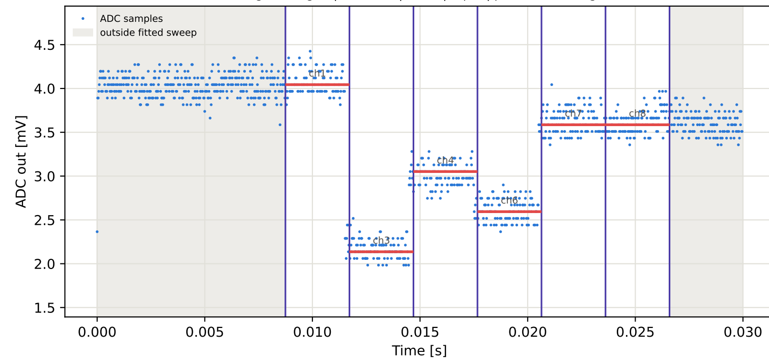
Tag7 &lt;- Tag3 | 785 MHz | run 0 | rep 1 | phase -17.30 deg
