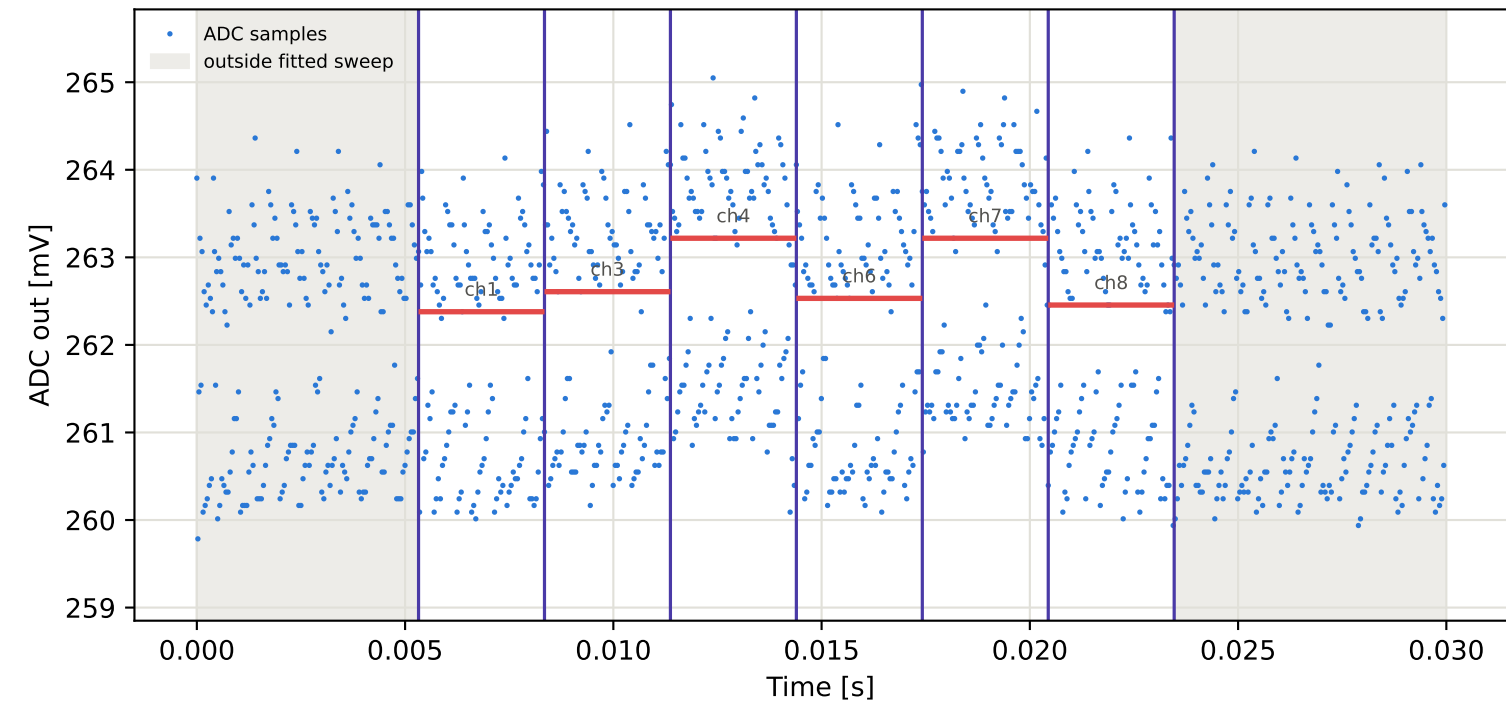
Tag16 &lt;- Tag15 | 795 MHz | run 0 | rep 1 | phase 39.47 deg
