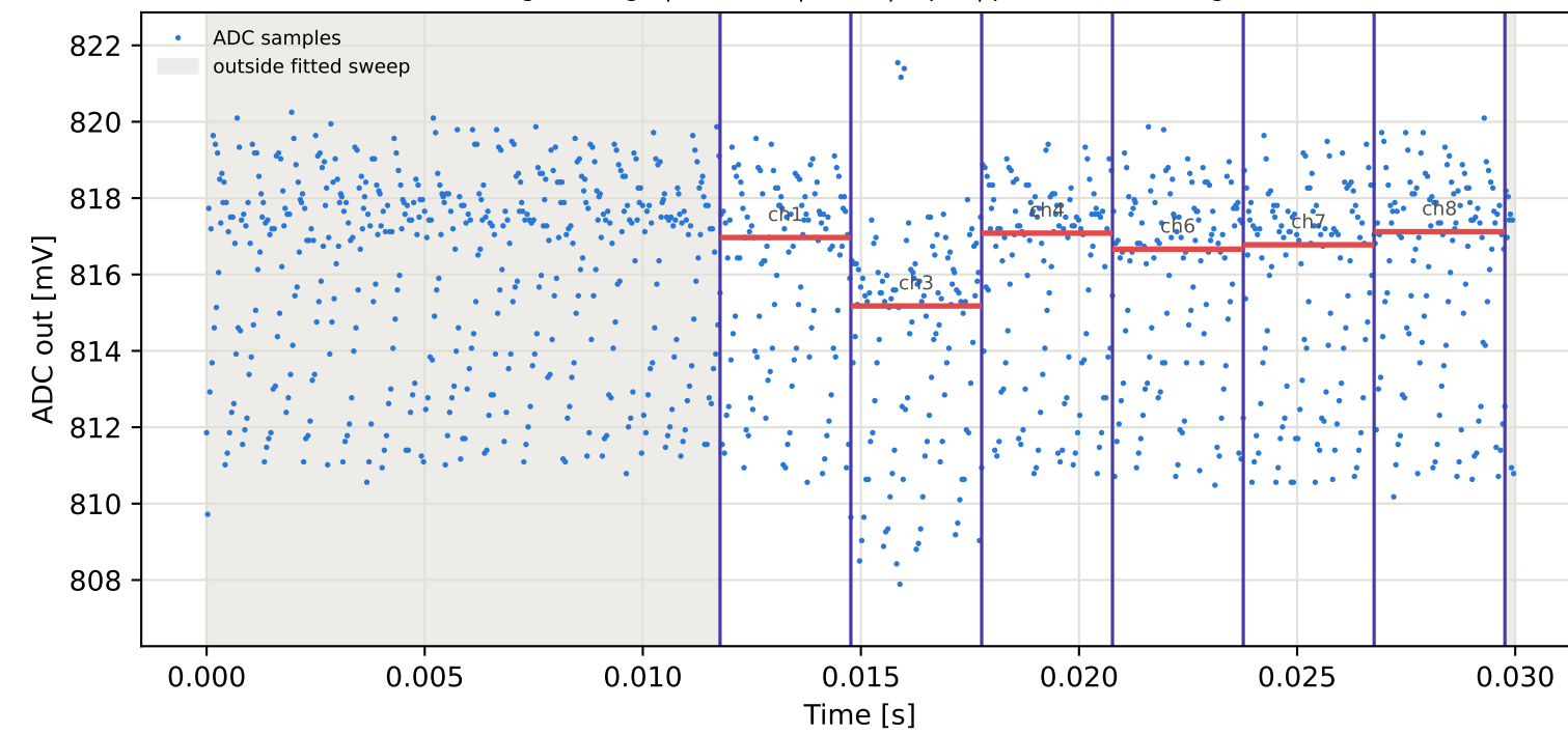
Tag8 &lt;- Tag4 | 935 MHz | run 0 | rep 1 | phase 48.38 deg
