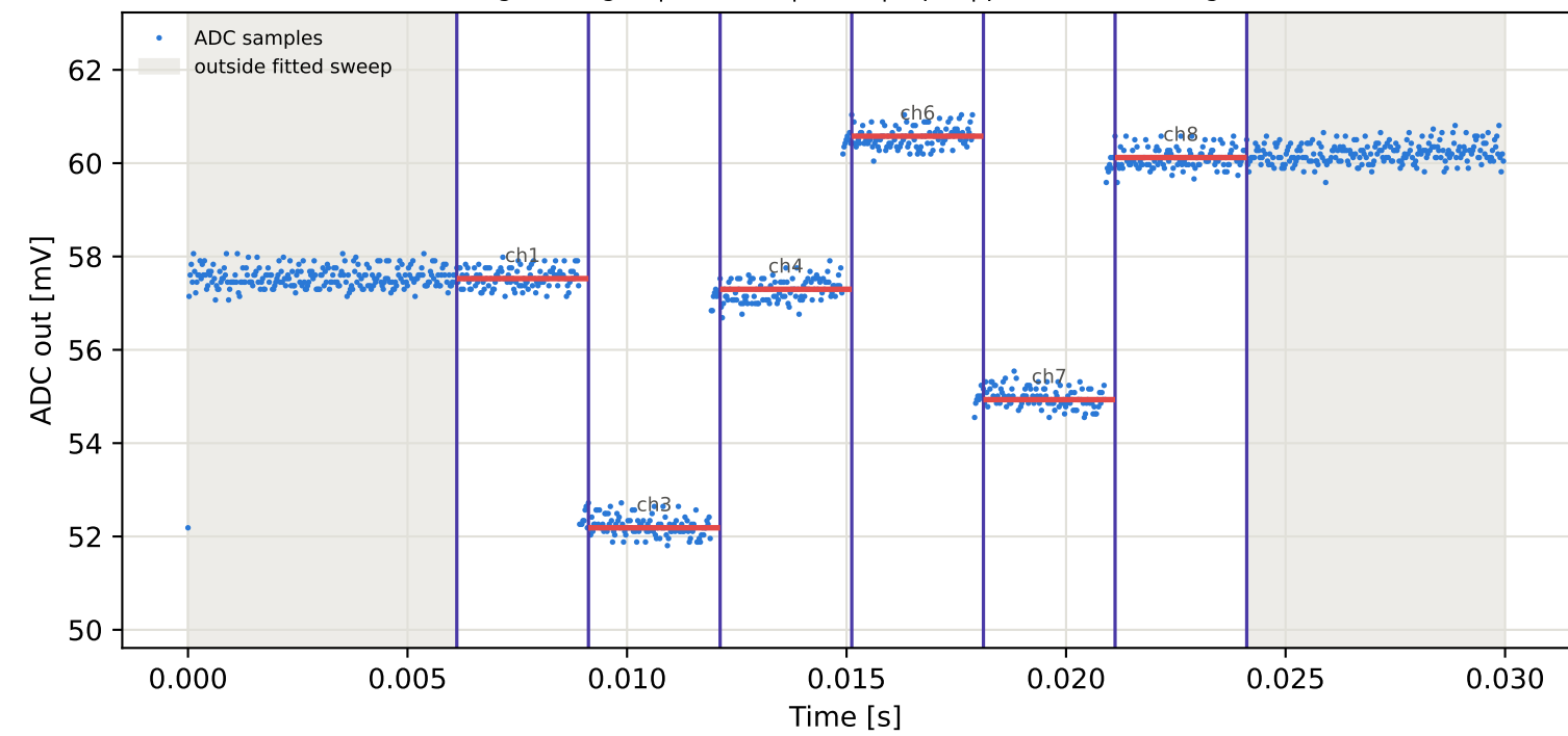
Tag1 &lt;- Tag2 | 835 MHz | run 0 | rep 1 | phase 96.59 deg
