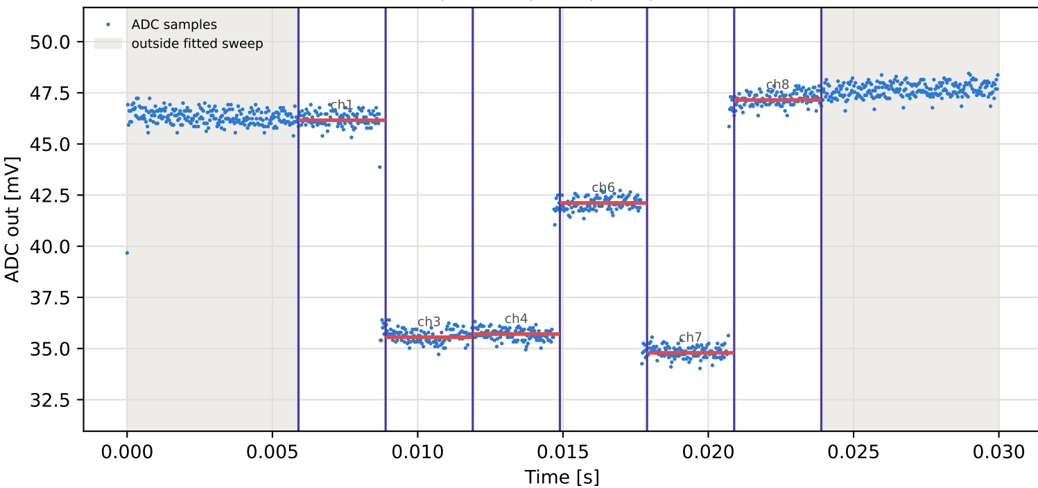
Tag2 &lt;- Tag15 | 865 MHz | run 0 | rep 1 | phase 122.25 deg
