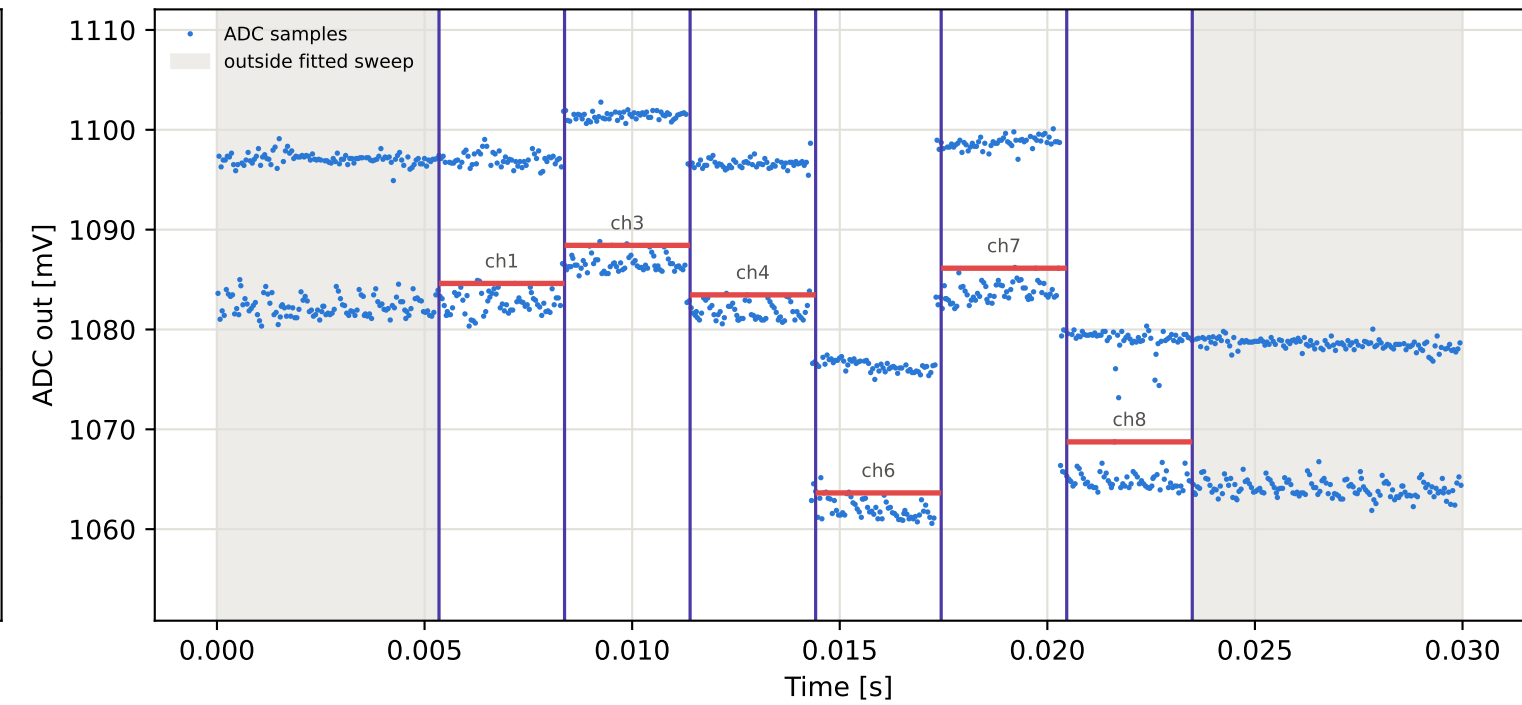
Tag15 &lt;- Tag6 | 885 MHz | run 0 | rep 1 | phase -2.14 deg
