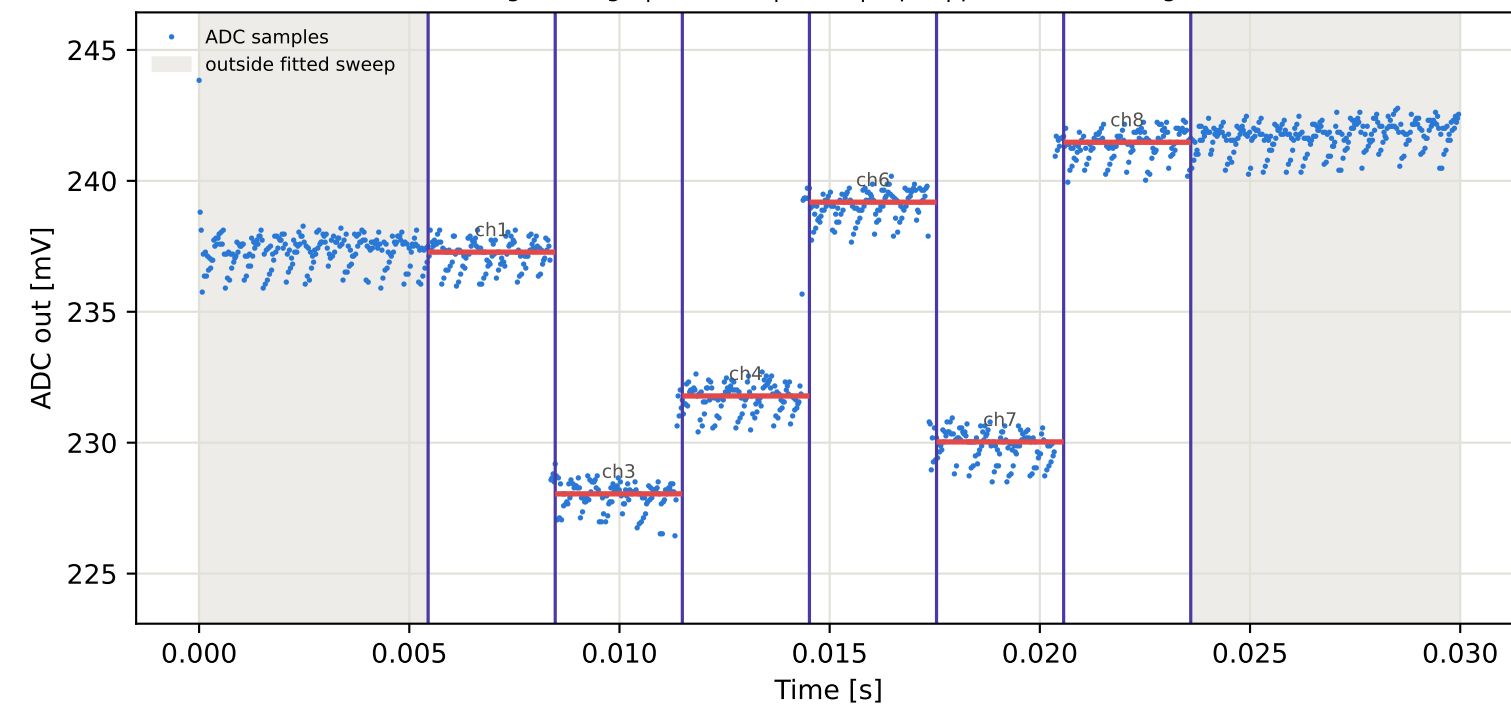
Tag9 &lt;- Tag7 | 845 MHz | run 0 | rep 1 | phase 9.72 deg
