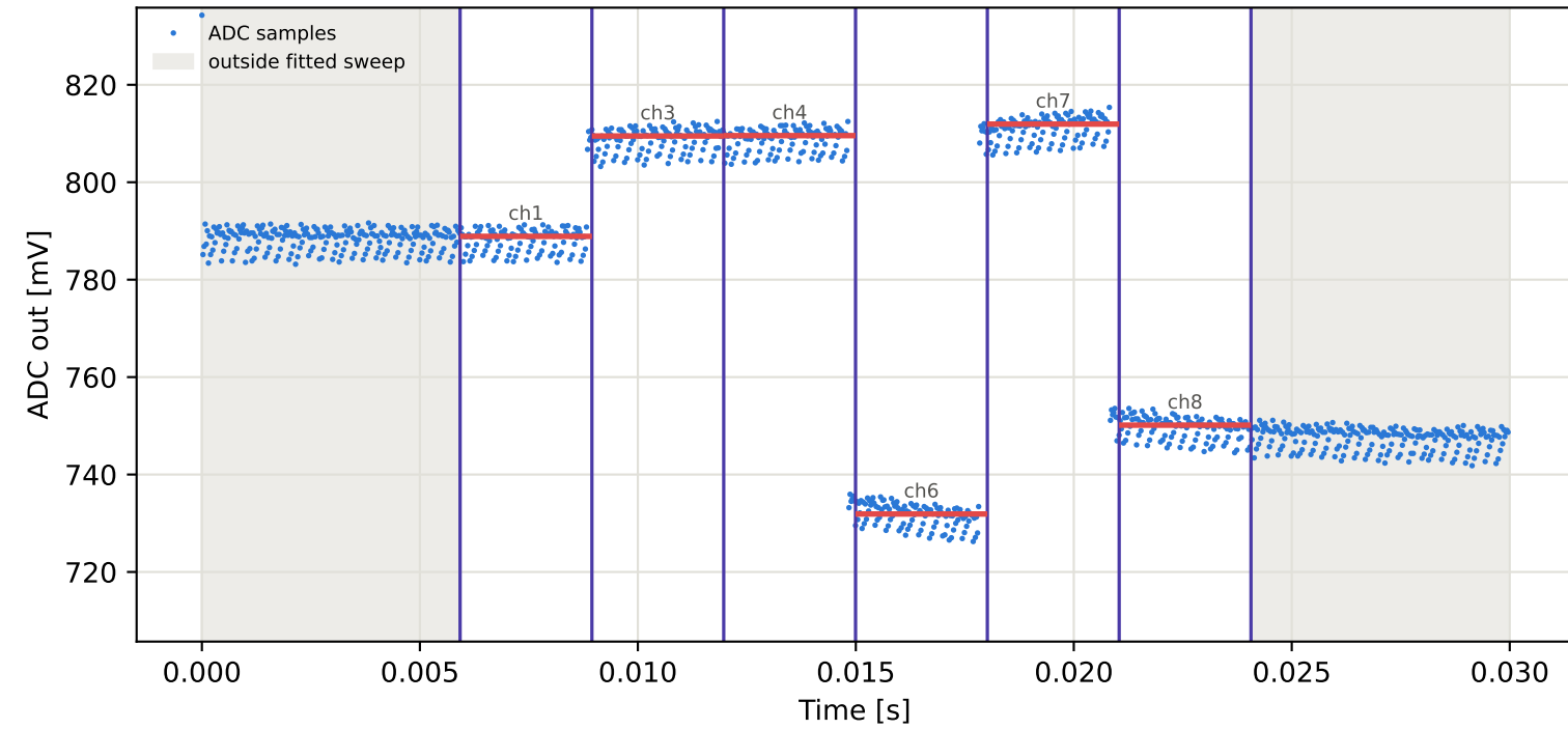
Tag3 &lt;- Tag2 | 935 MHz | run 0 | rep 1 | phase 153.87 deg
