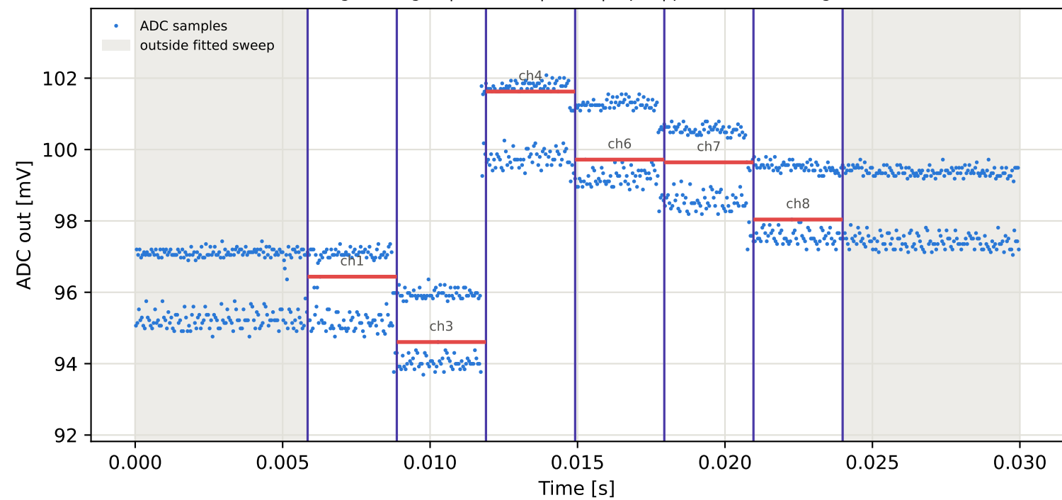
Tag1 &lt;- Tag16 | 805 MHz | run 0 | rep 1 | phase -164.41 deg
