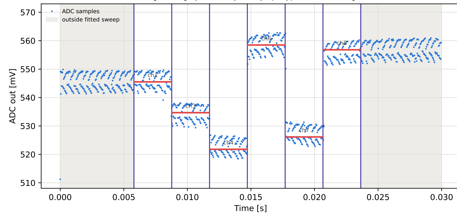
Tag8 &lt;- Tag6 | 955 MHz | run 0 | rep 1 | phase 127.22 deg
