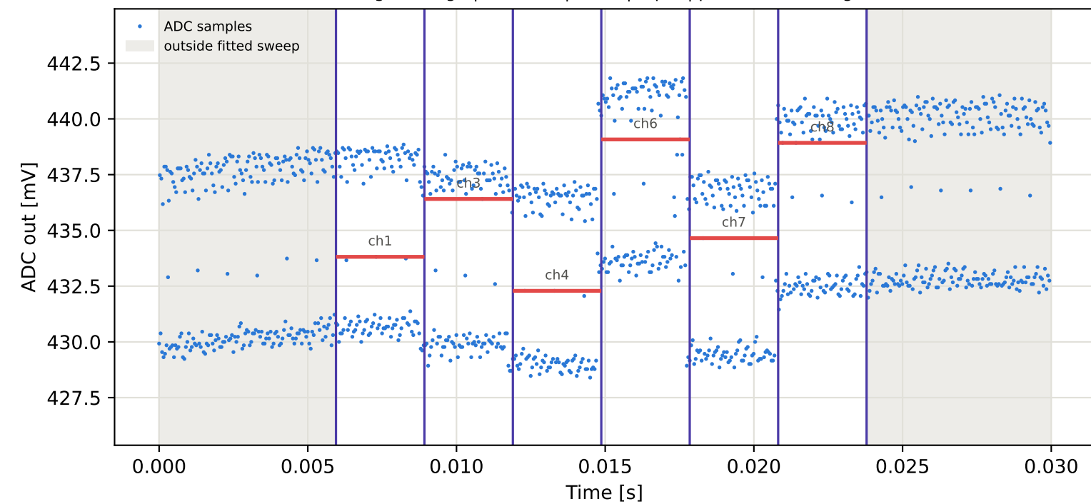
Tag1 &lt;- Tag4 | 935 MHz | run 0 | rep 1 | phase -136.37 deg
