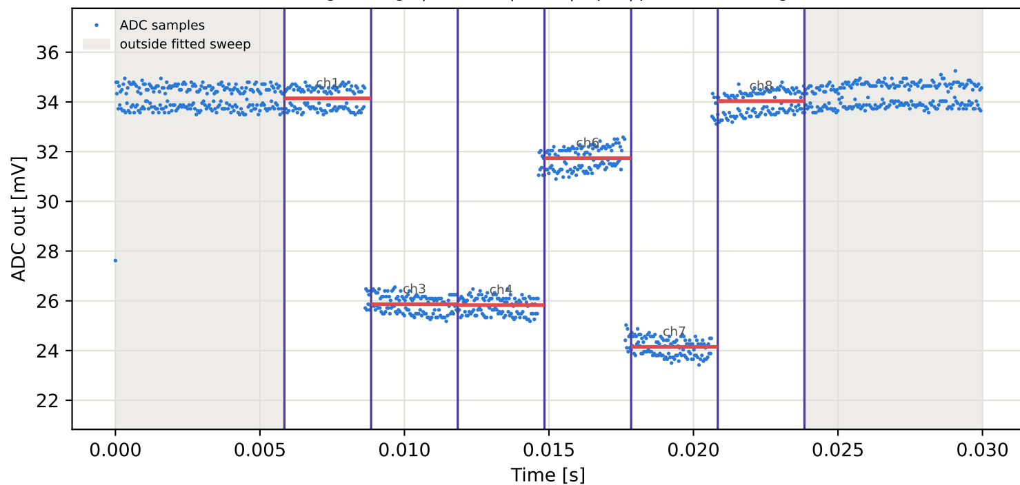
Tag2 &lt;- Tag5 | 825 MHz | run 0 | rep 1 | phase -175.56 deg
