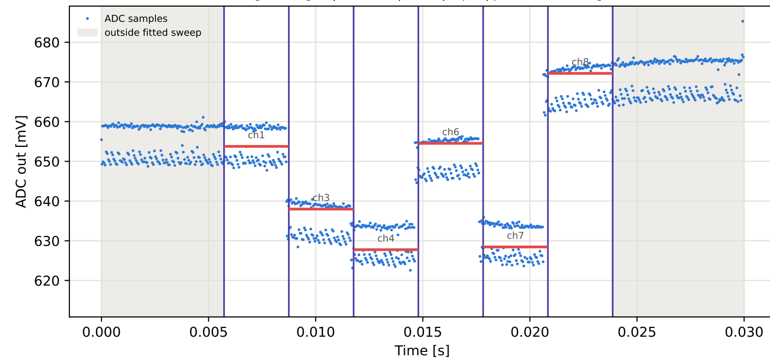
Tag1 &lt;- Tag16 | 885 MHz | run 0 | rep 1 | phase -33.60 deg
