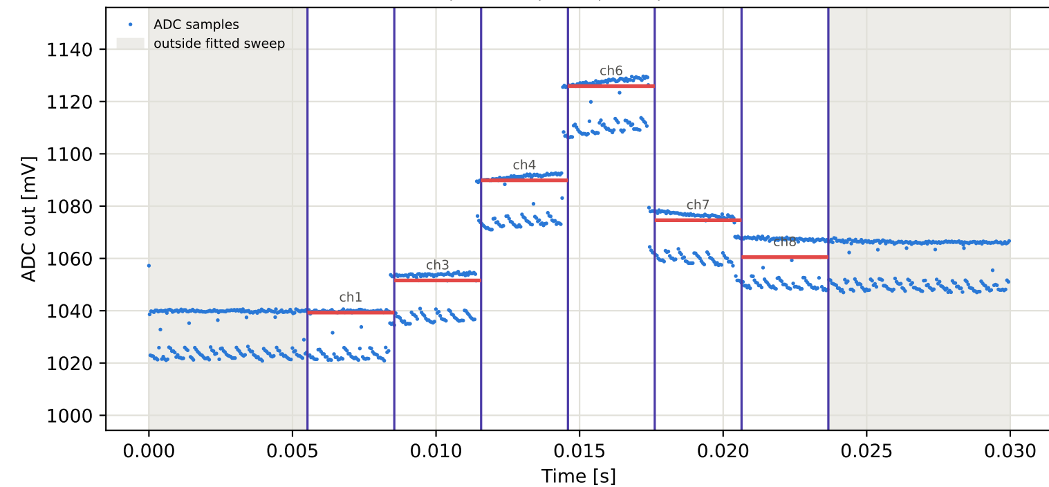
Tag5 &lt;- Tag3 | 915 MHz | run 0 | rep 1 | phase -141.35 deg
