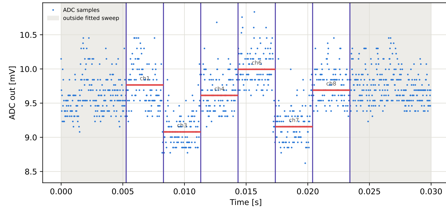
Tag15 &lt;- Tag1 | 775 MHz | run 0 | rep 1 | phase 103.79 deg
