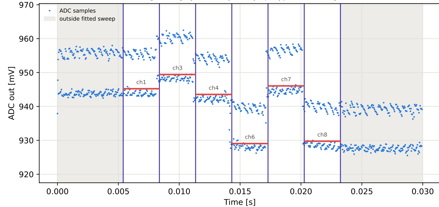
Tag5 &lt;- Tag9 | 885 MHz | run 0 | rep 1 | phase 177.97 deg
