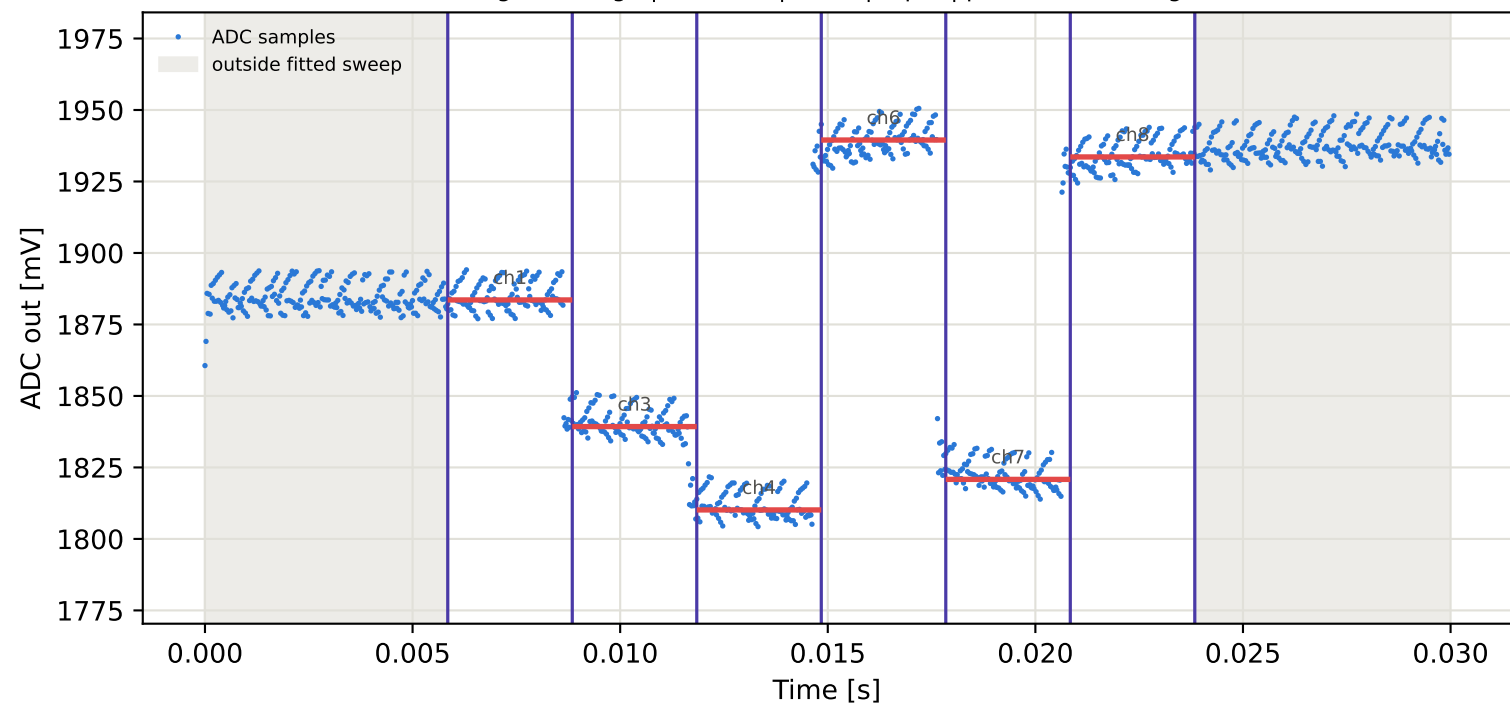
Tag15 &lt;- Tag6 | 935 MHz | run 0 | rep 1 | phase -157.39 deg
