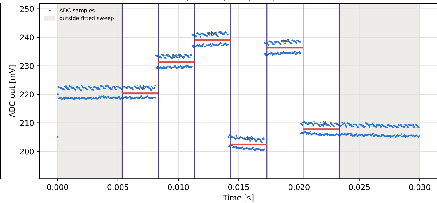
Tag7 &lt;- Tag1 | 945 MHz | run 0 | rep 1 | phase 85.06 deg
