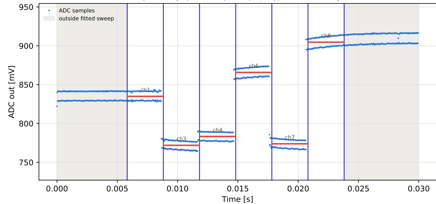
Tag16 &lt;- Tag1 | 875 MHz | run 0 | rep 1 | phase 150.68 deg
