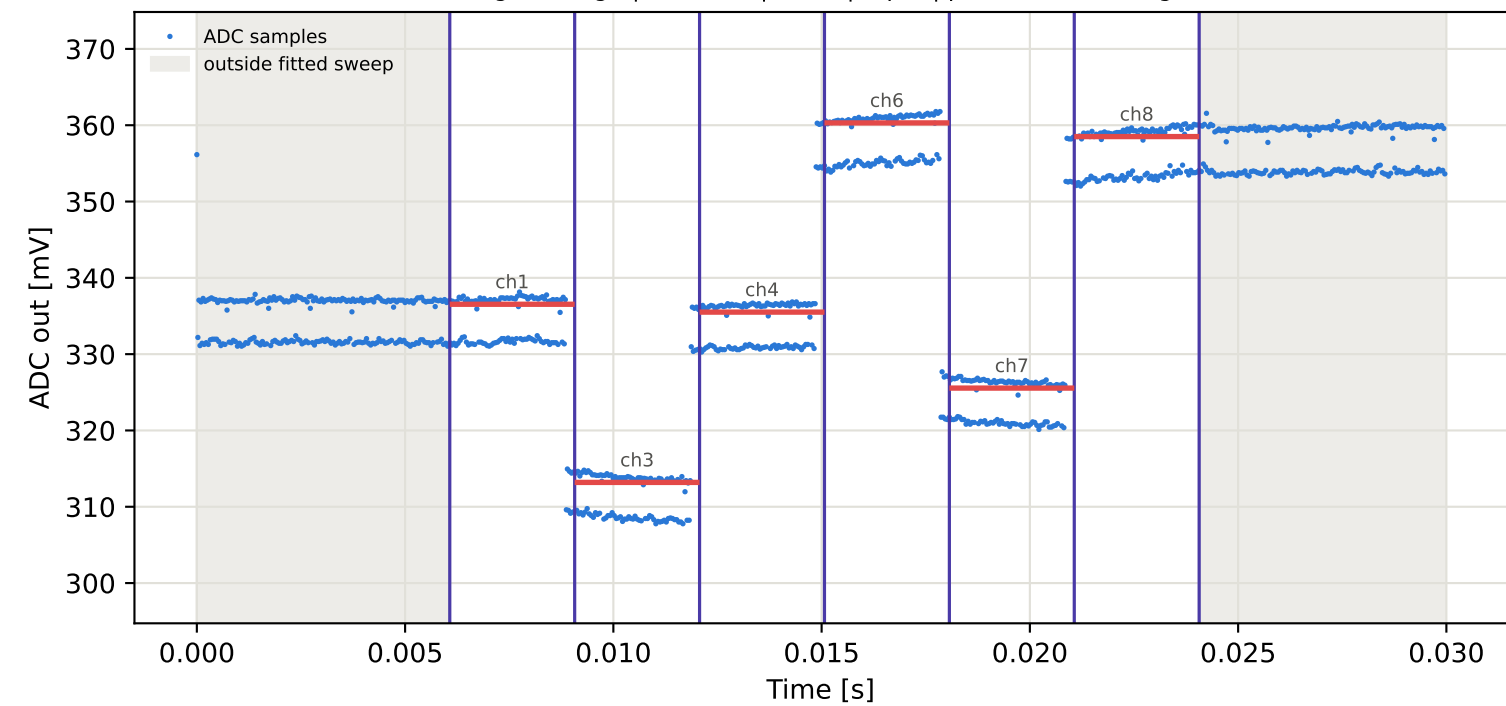
Tag4 &lt;- Tag8 | 845 MHz | run 0 | rep 1 | phase -155.32 deg
