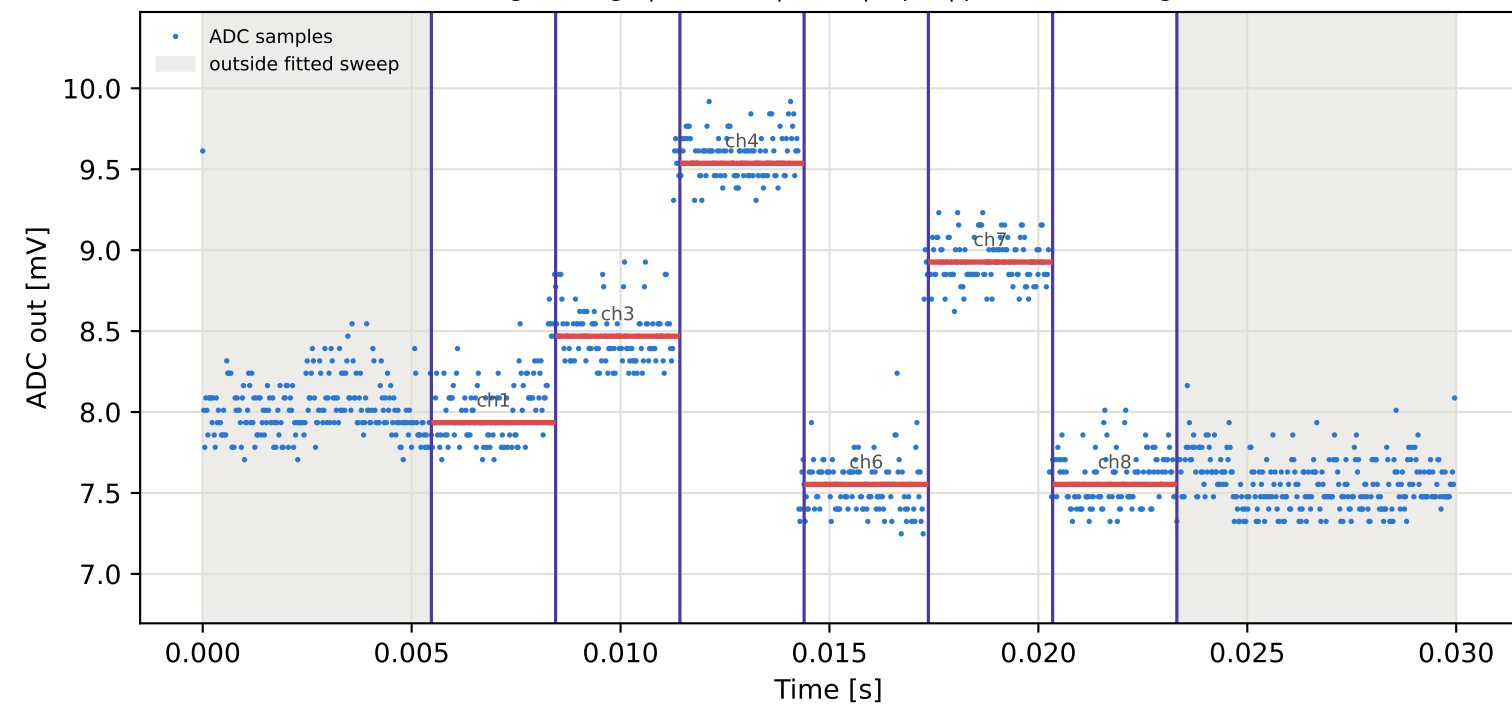
Tag2 &lt;- Tag6 | 995 MHz | run 0 | rep 1 | phase -175.91 deg
