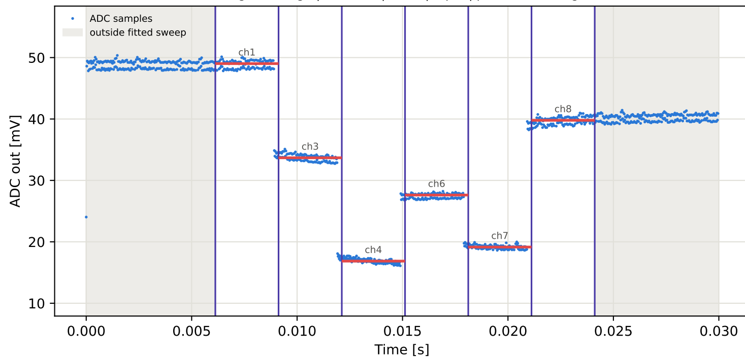
Tag10 &lt;- Tag8 | 845 MHz | run 0 | rep 1 | phase 67.83 deg
