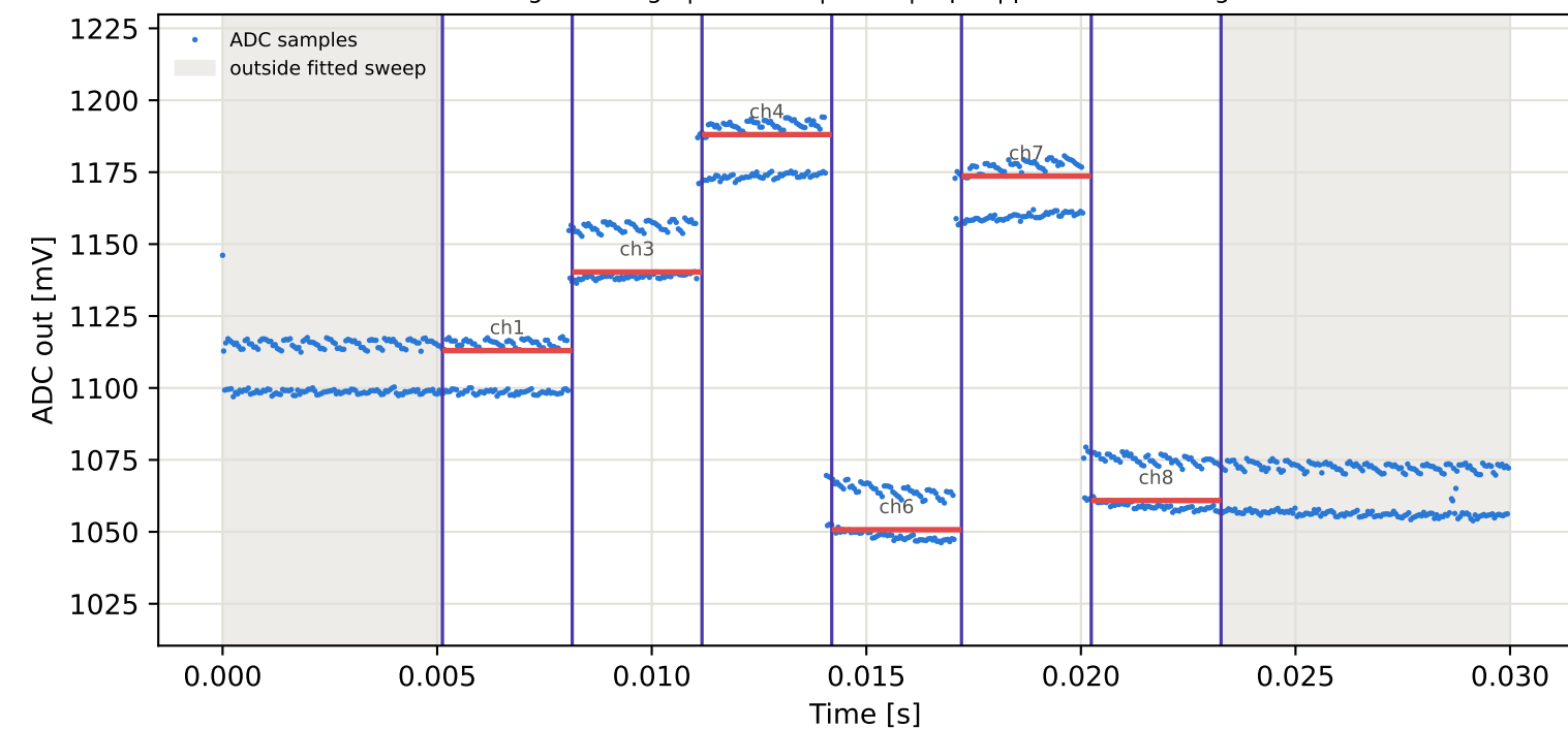
Tag2 &lt;- Tag1 | 955 MHz | run 0 | rep 1 | phase -165.95 deg
