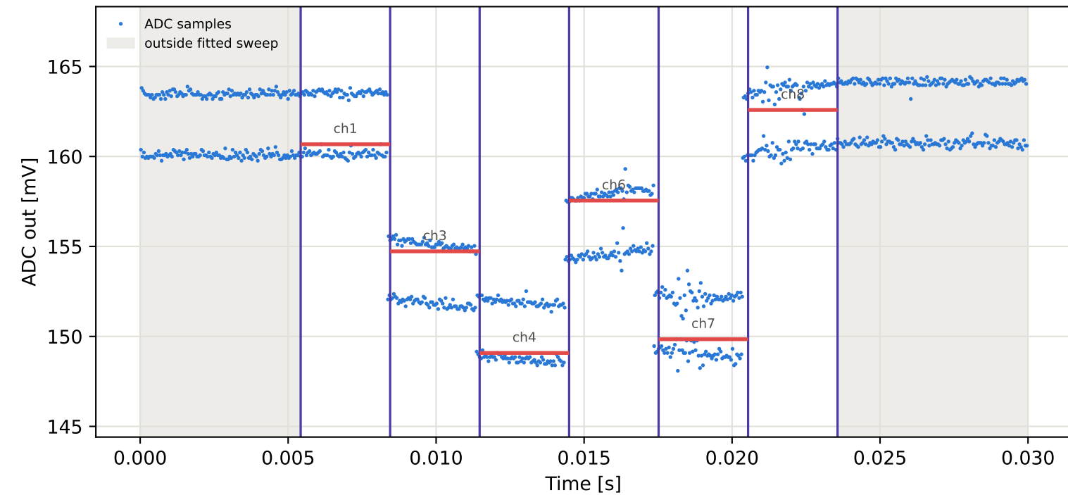
Tag1 &lt;- Tag9 | 875 MHz | run 0 | rep 1 | phase 23.84 deg
