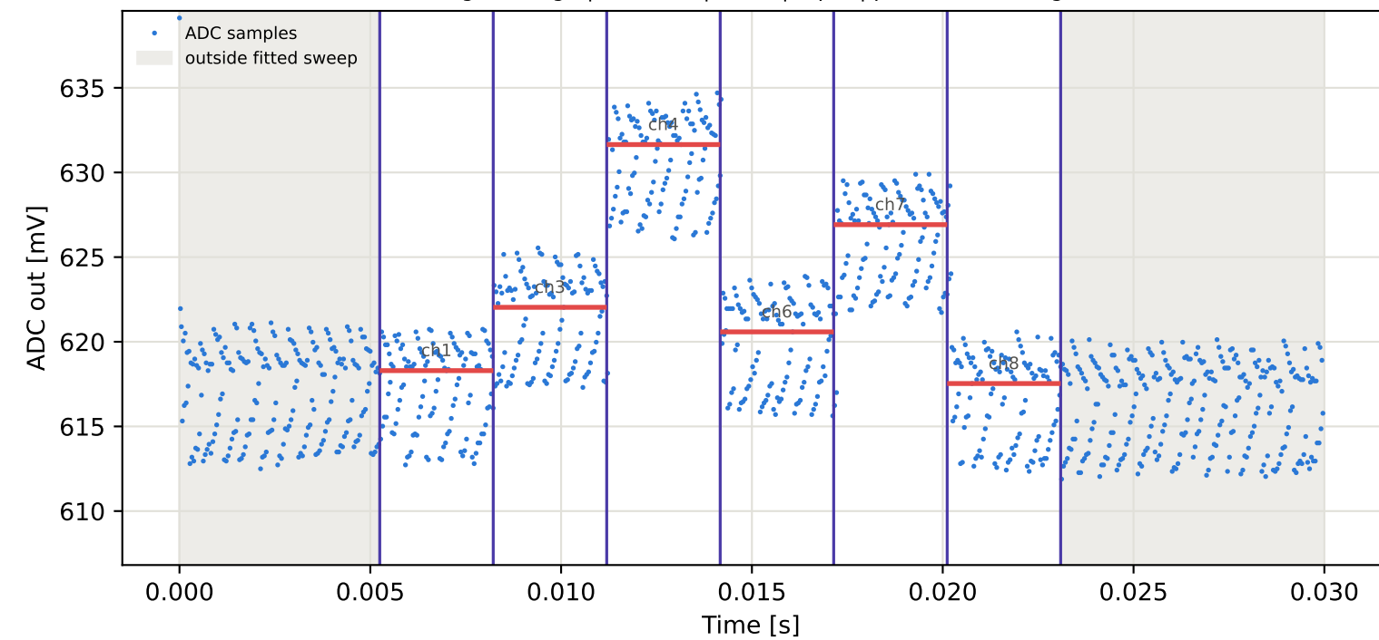
Tag5 &lt;- Tag9 | 965 MHz | run 0 | rep 1 | phase -110.91 deg
