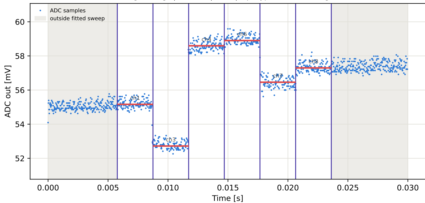
Tag8 &lt;- Tag1 | 795 MHz | run 0 | rep 1 | phase 59.35 deg
