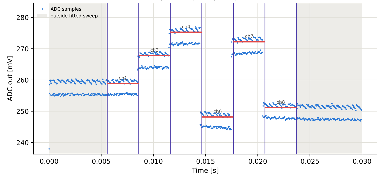
Tag7 &lt;- Tag1 | 975 MHz | run 0 | rep 1 | phase 147.66 deg
