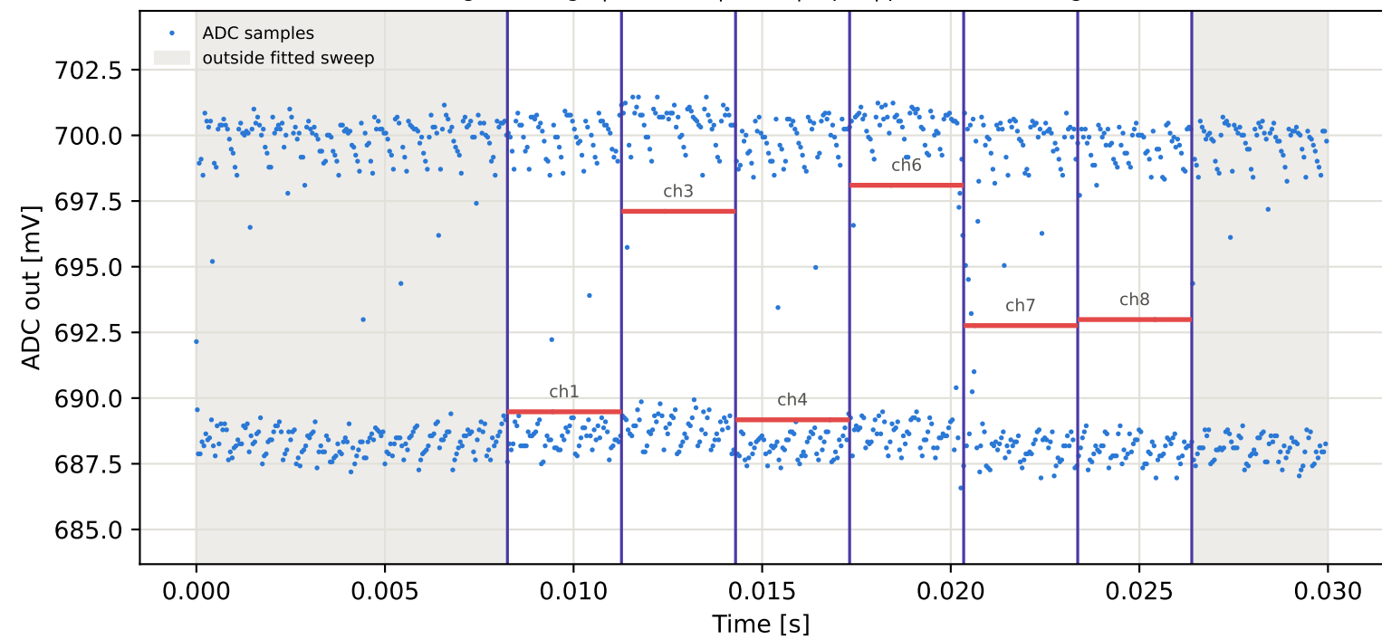
Tag15 &lt;- Tag4 | 985 MHz | run 0 | rep 1 | phase -62.71 deg
