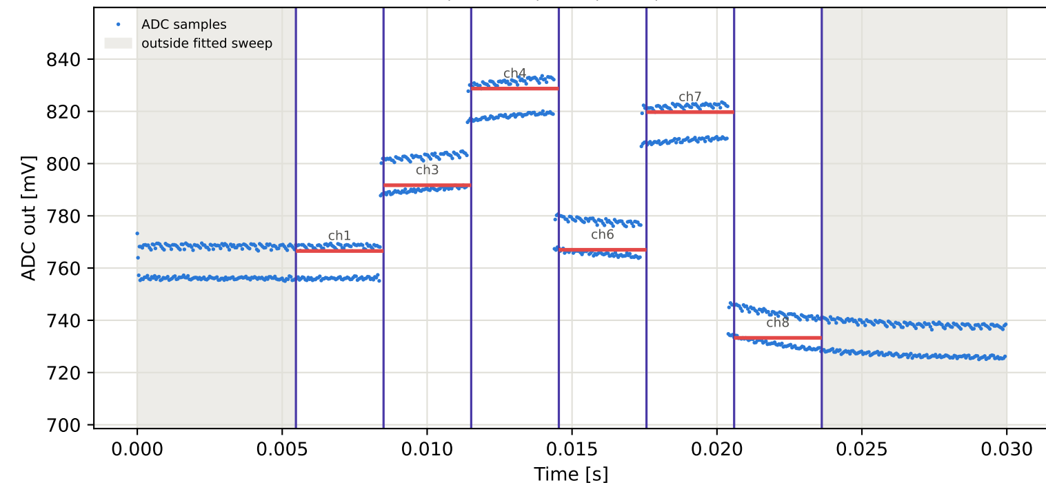
Tag1 &lt;- Tag3 | 915 MHz | run 0 | rep 1 | phase -71.58 deg
