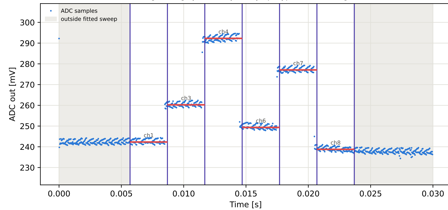
Tag6 &lt;- Tag9 | 975 MHz | run 0 | rep 1 | phase -83.98 deg
