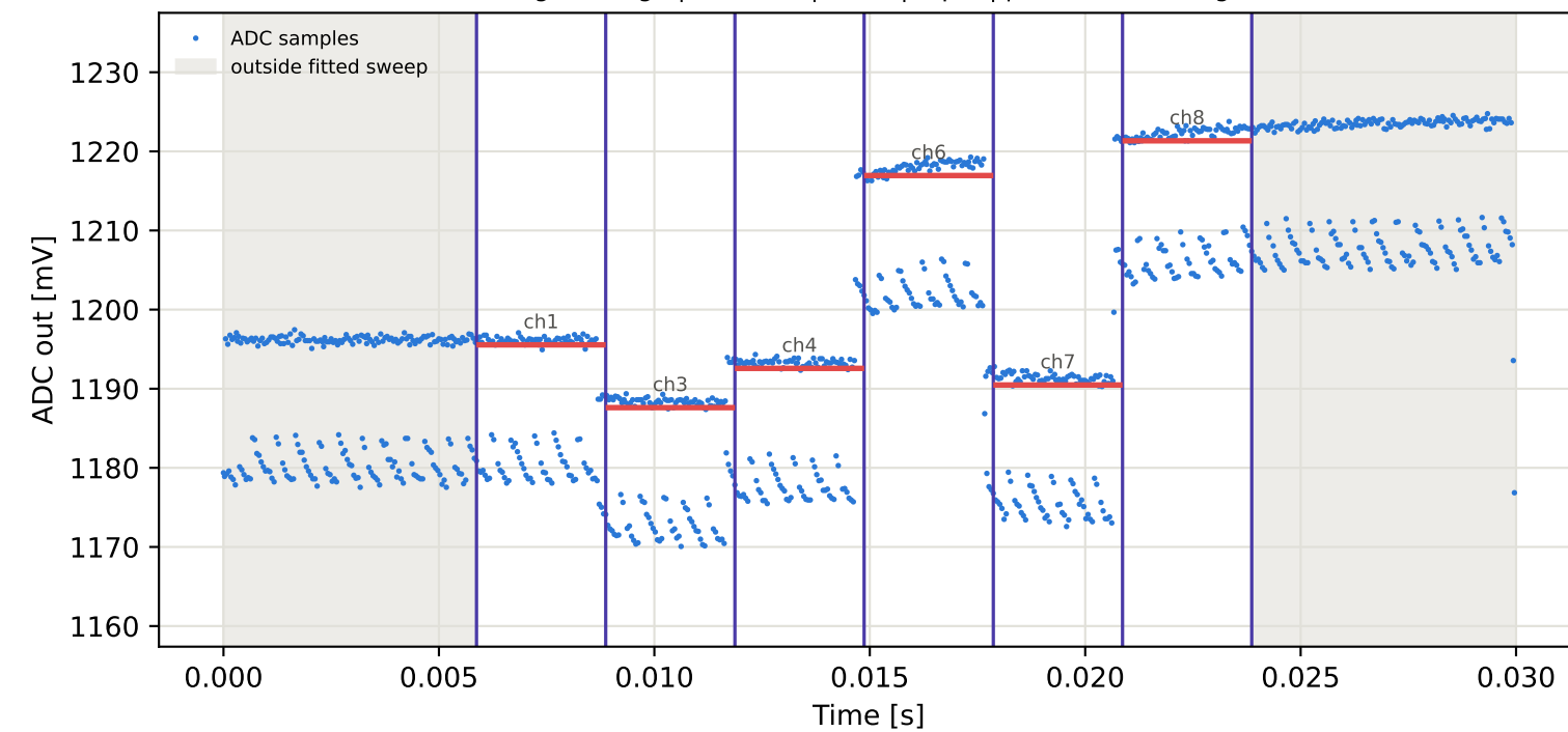
Tag7 &lt;- Tag10 | 895 MHz | run 0 | rep 1 | phase -38.29 deg
