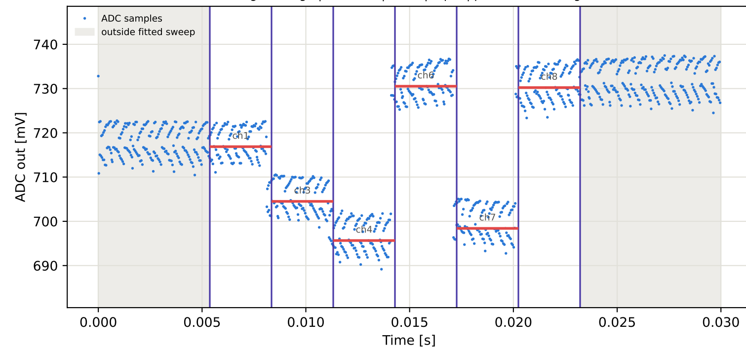
Tag7 &lt;- Tag5 | 935 MHz | run 0 | rep 1 | phase 134.80 deg
