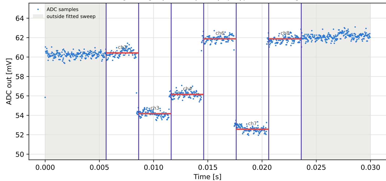
Tag6 &lt;- Tag3 | 795 MHz | run 0 | rep 1 | phase -52.35 deg
