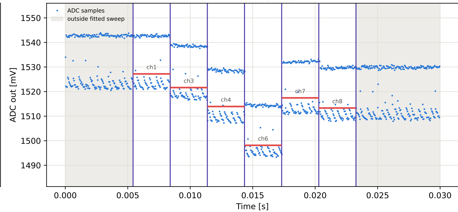
Tag15 &lt;- Tag6 | 895 MHz | run 0 | rep 1 | phase 29.85 deg
