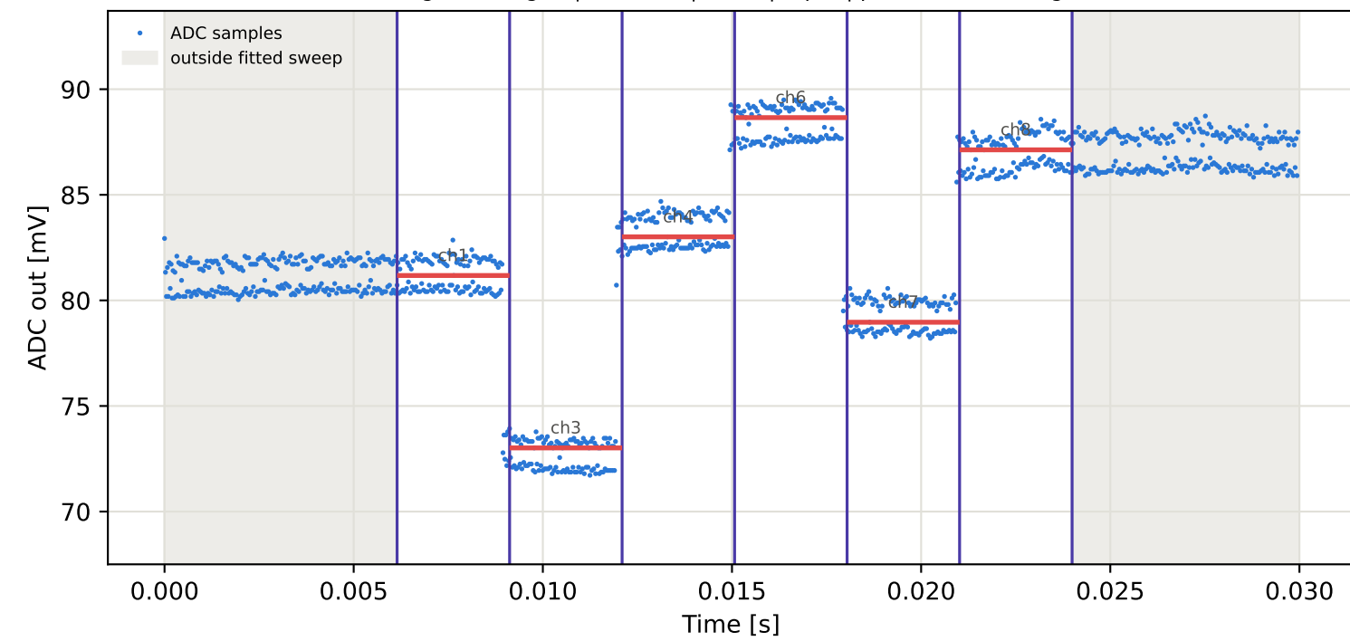
Tag10 &lt;- Tag3 | 825 MHz | run 0 | rep 1 | phase -158.62 deg
