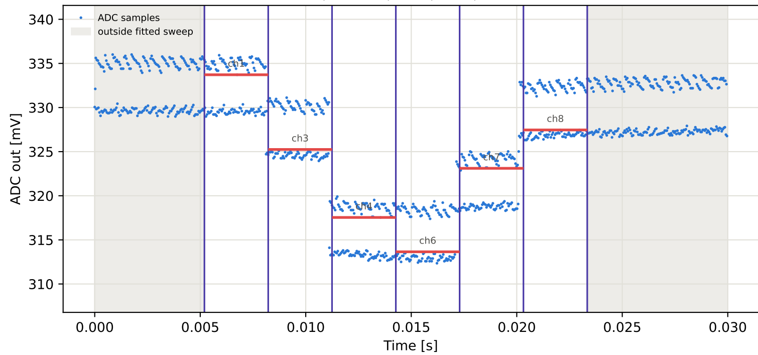
Tag6 &lt;- Tag5 | 935 MHz | run 0 | rep 1 | phase 46.60 deg
