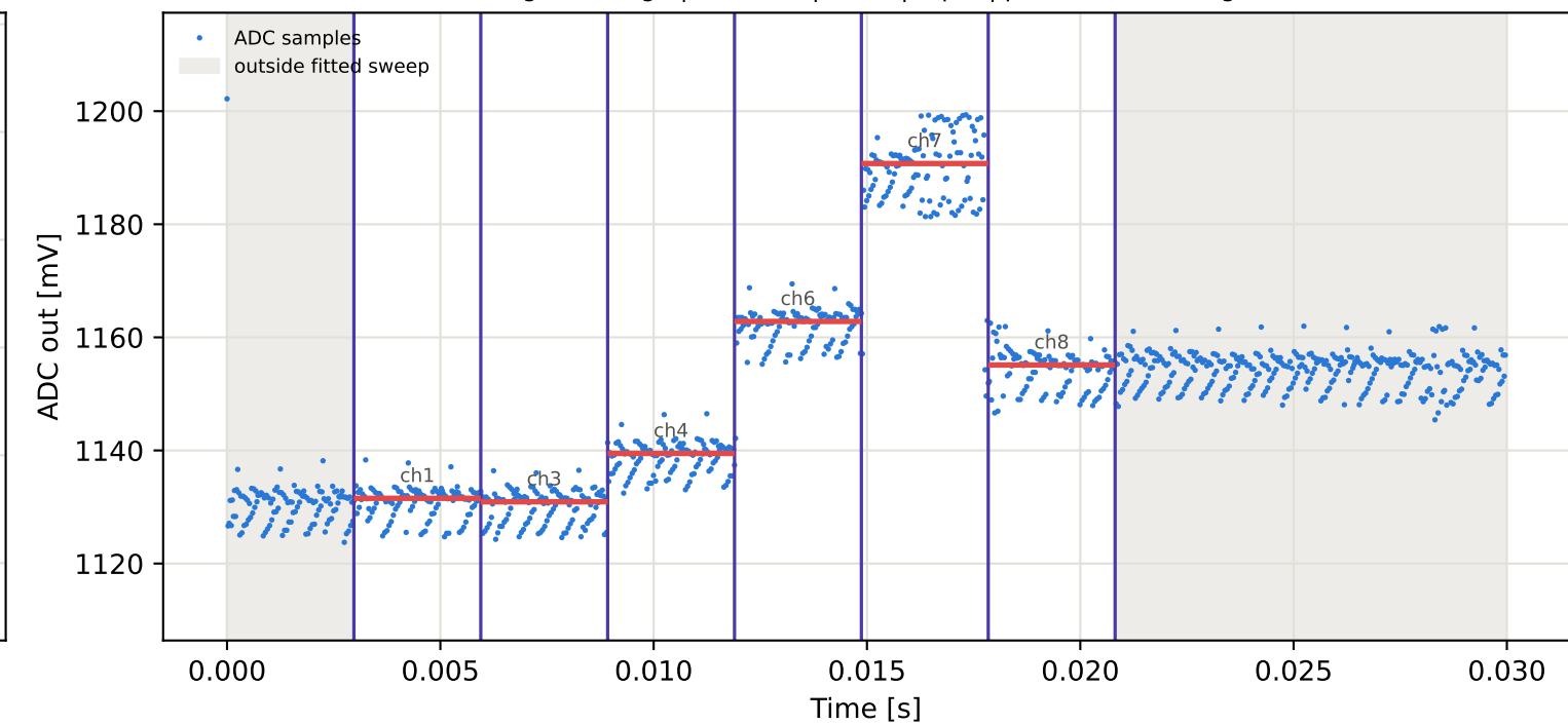
Tag16 &lt;- Tag7 | 895 MHz | run 0 | rep 1 | phase -49.16 deg
