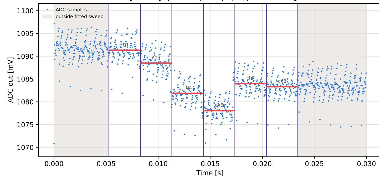
Tag15 &lt;- Tag9 | 885 MHz | run 0 | rep 1 | phase 165.28 deg
