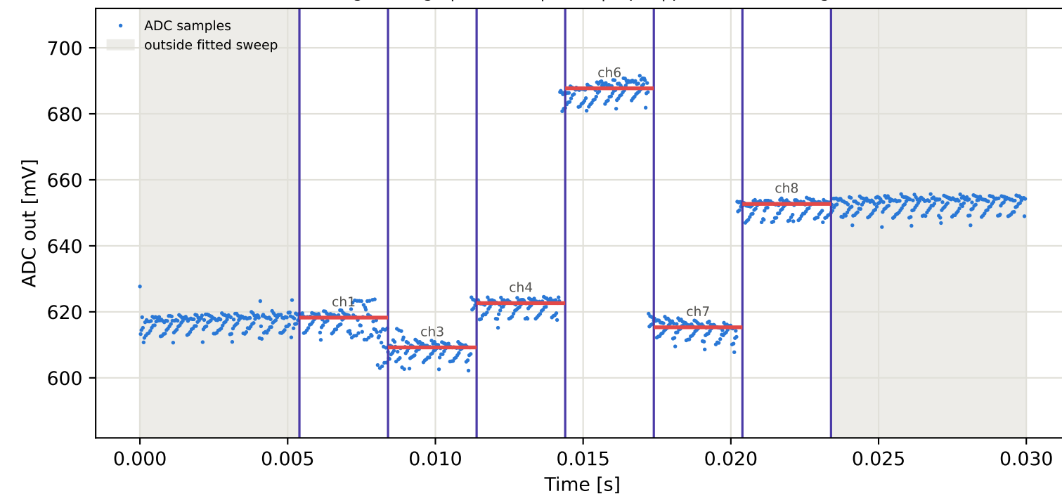
Tag6 &lt;- Tag9 | 925 MHz | run 0 | rep 1 | phase -170.56 deg
