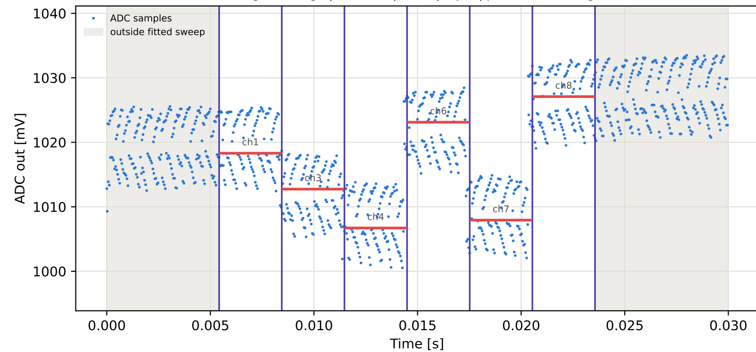
Tag16 &lt;- Tag5 | 915 MHz | run 0 | rep 1 | phase -85.70 deg
