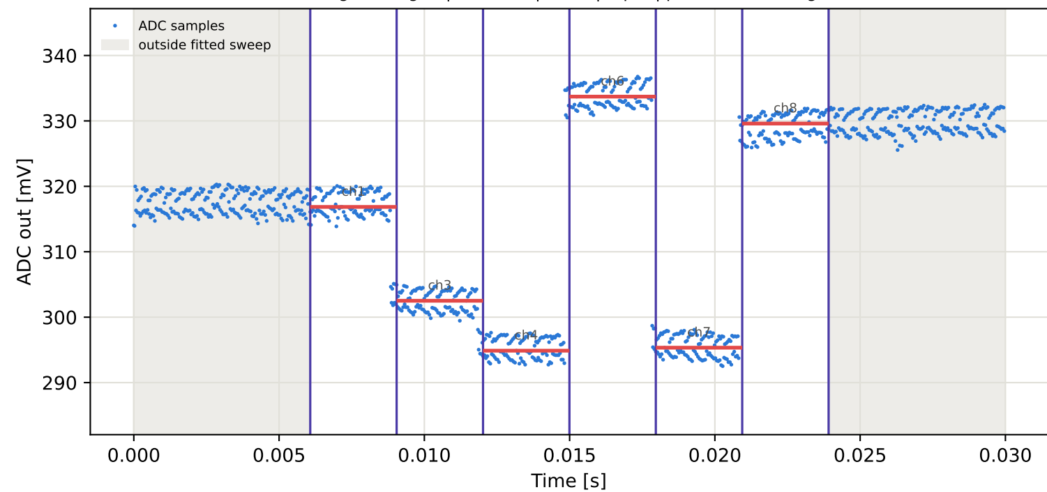
Tag4 &lt;- Tag3 | 995 MHz | run 0 | rep 1 | phase -91.37 deg
