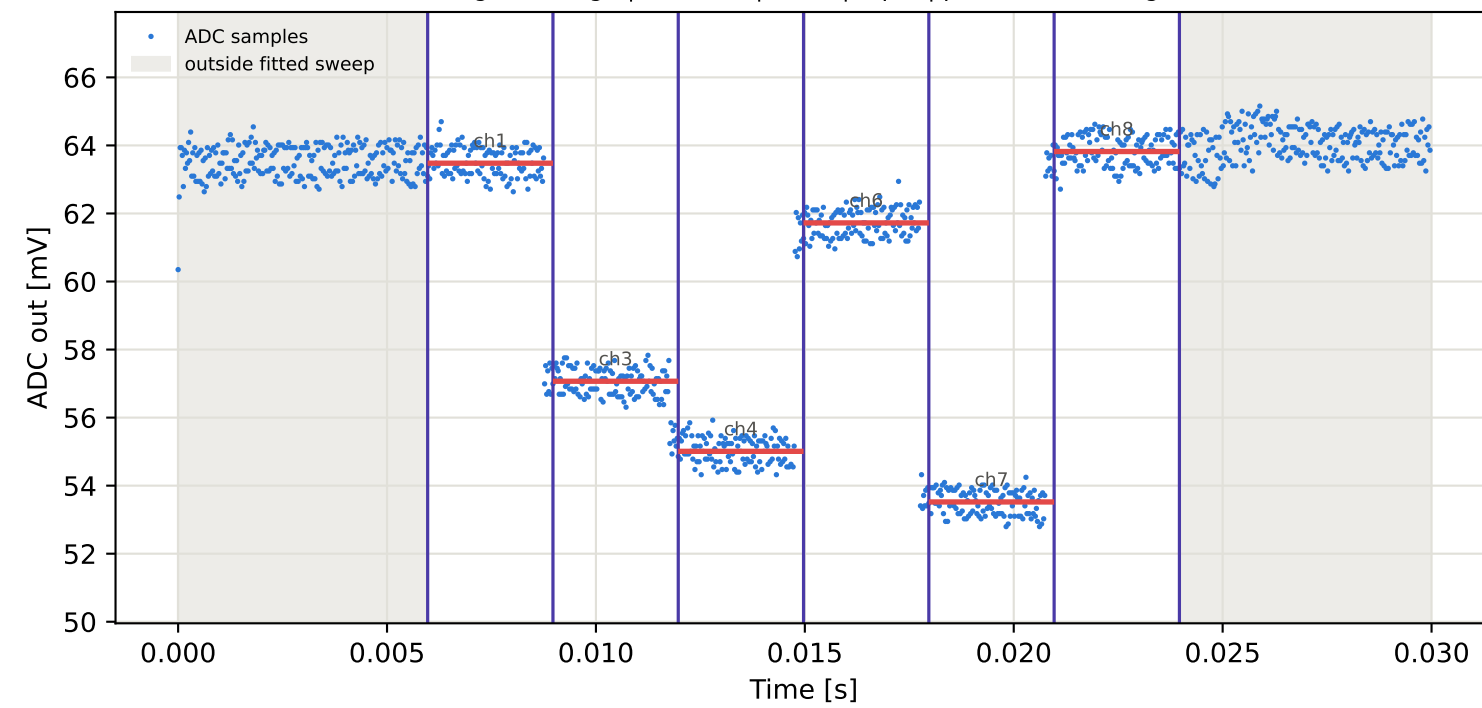
Tag10 &lt;- Tag8 | 785 MHz | run 0 | rep 1 | phase 176.46 deg
