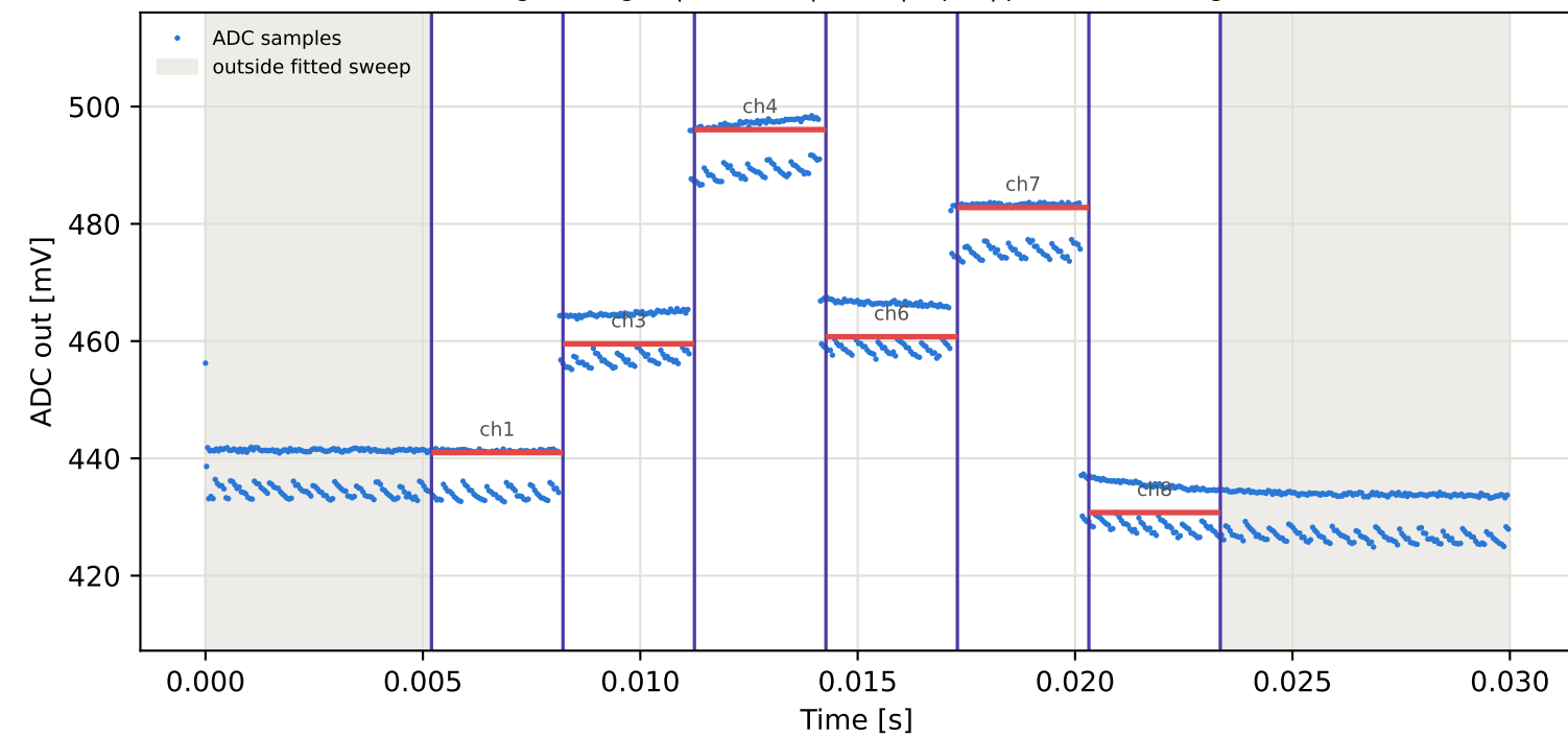
Tag5 &lt;- Tag2 | 945 MHz | run 0 | rep 1 | phase -99.88 deg
