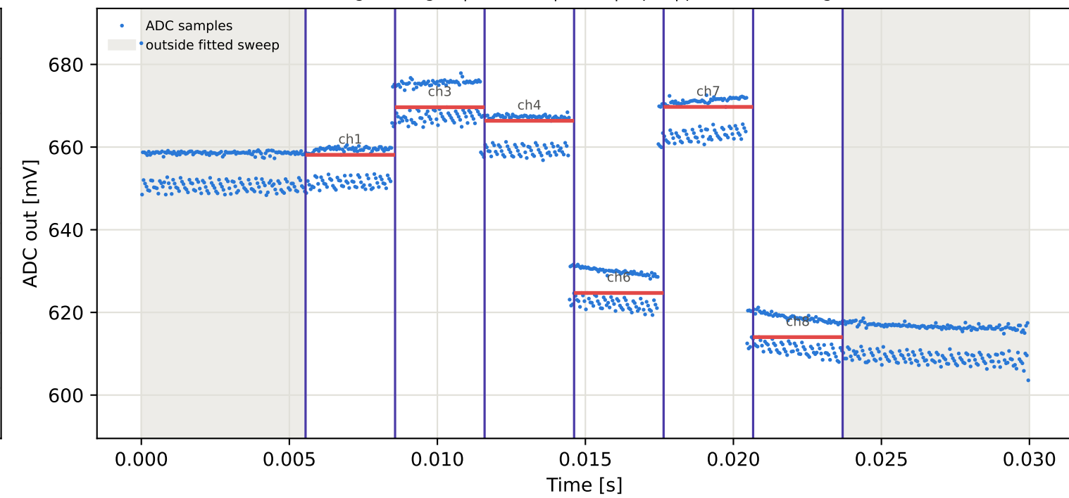
Tag1 &lt;- Tag2 | 885 MHz | run 0 | rep 1 | phase 110.83 deg
