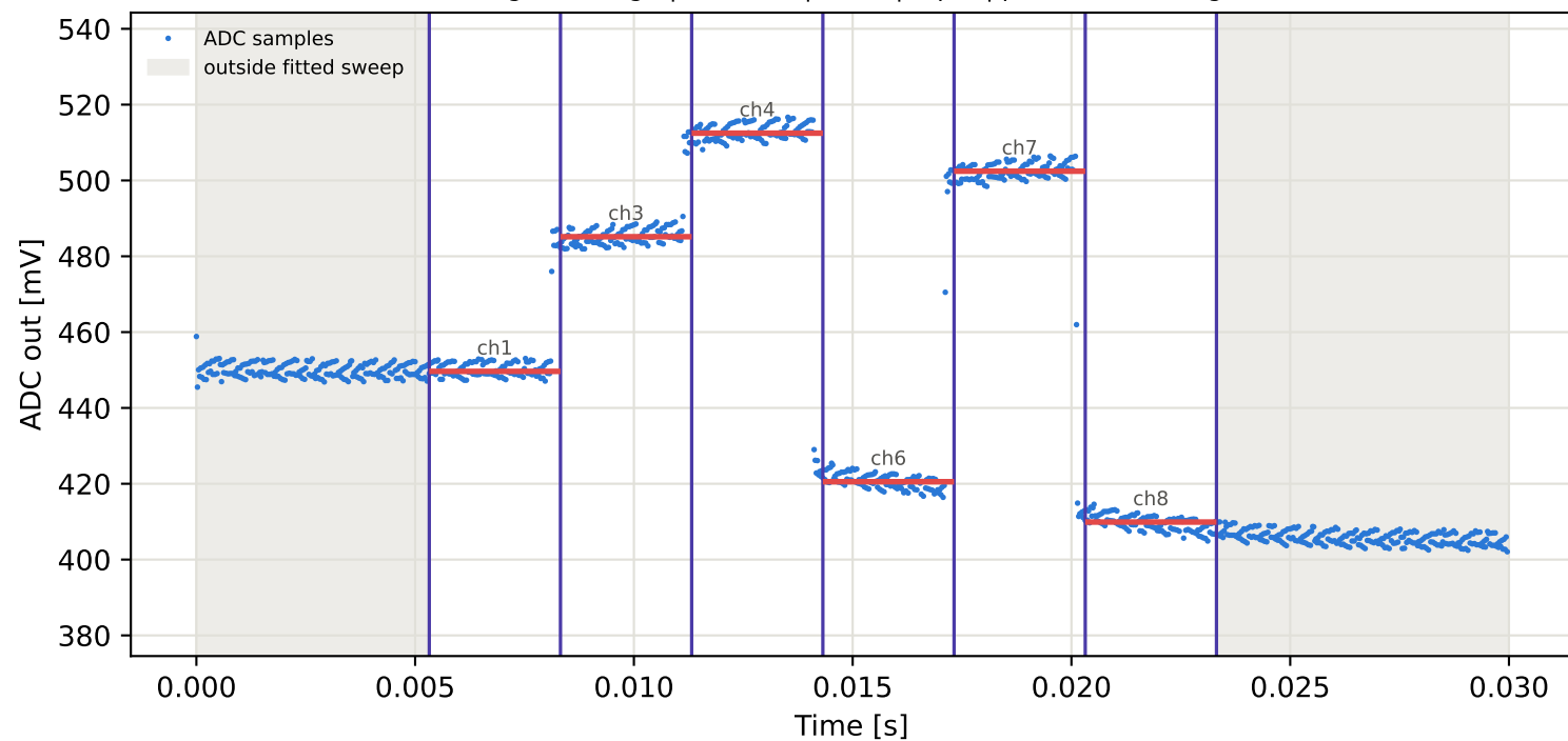
Tag10 &lt;- Tag8 | 925 MHz | run 0 | rep 1 | phase -139.64 deg
