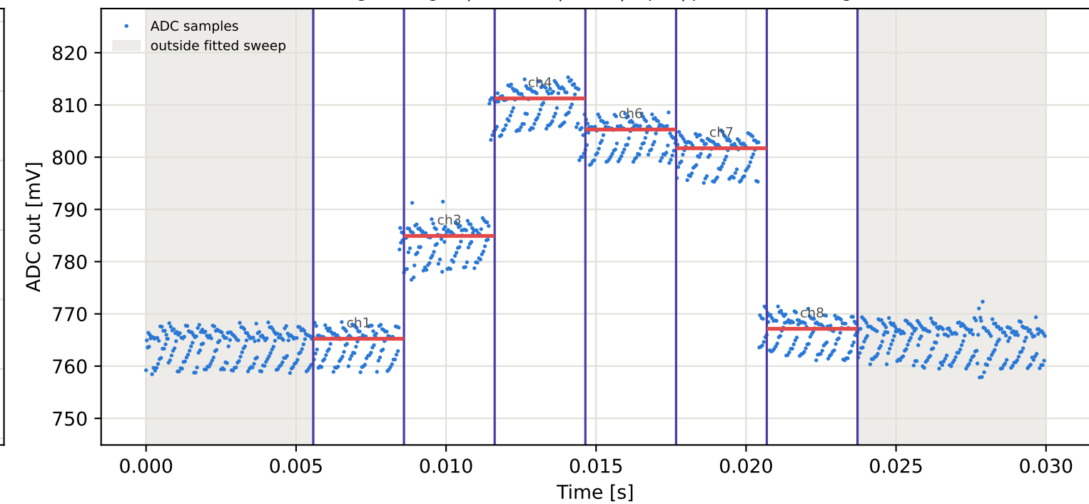
Tag5 &lt;- Tag2 | 925 MHz | run 0 | rep 1 | phase 71.42 deg
