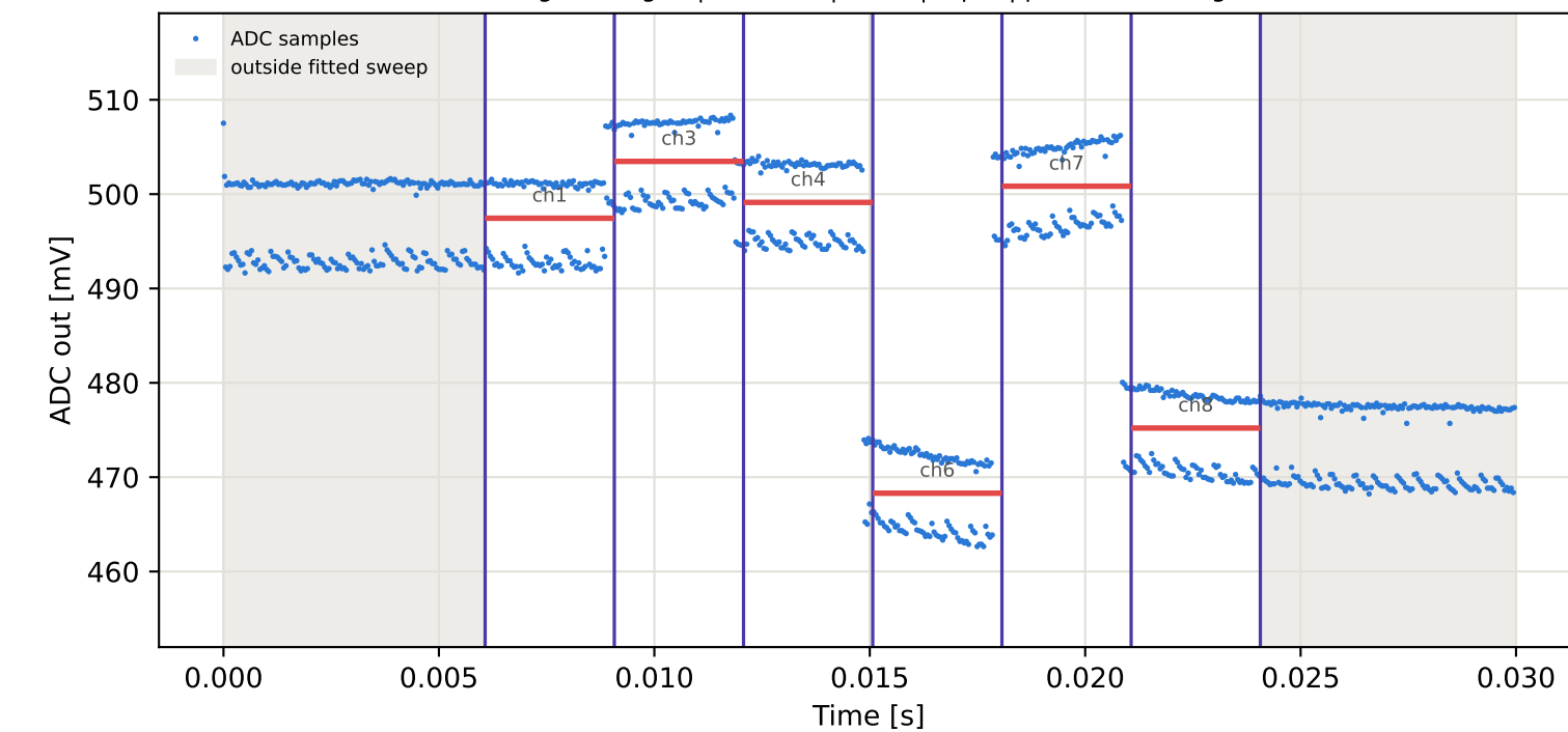
Tag7 &lt;- Tag10 | 905 MHz | run 0 | rep 1 | phase -1.94 deg
