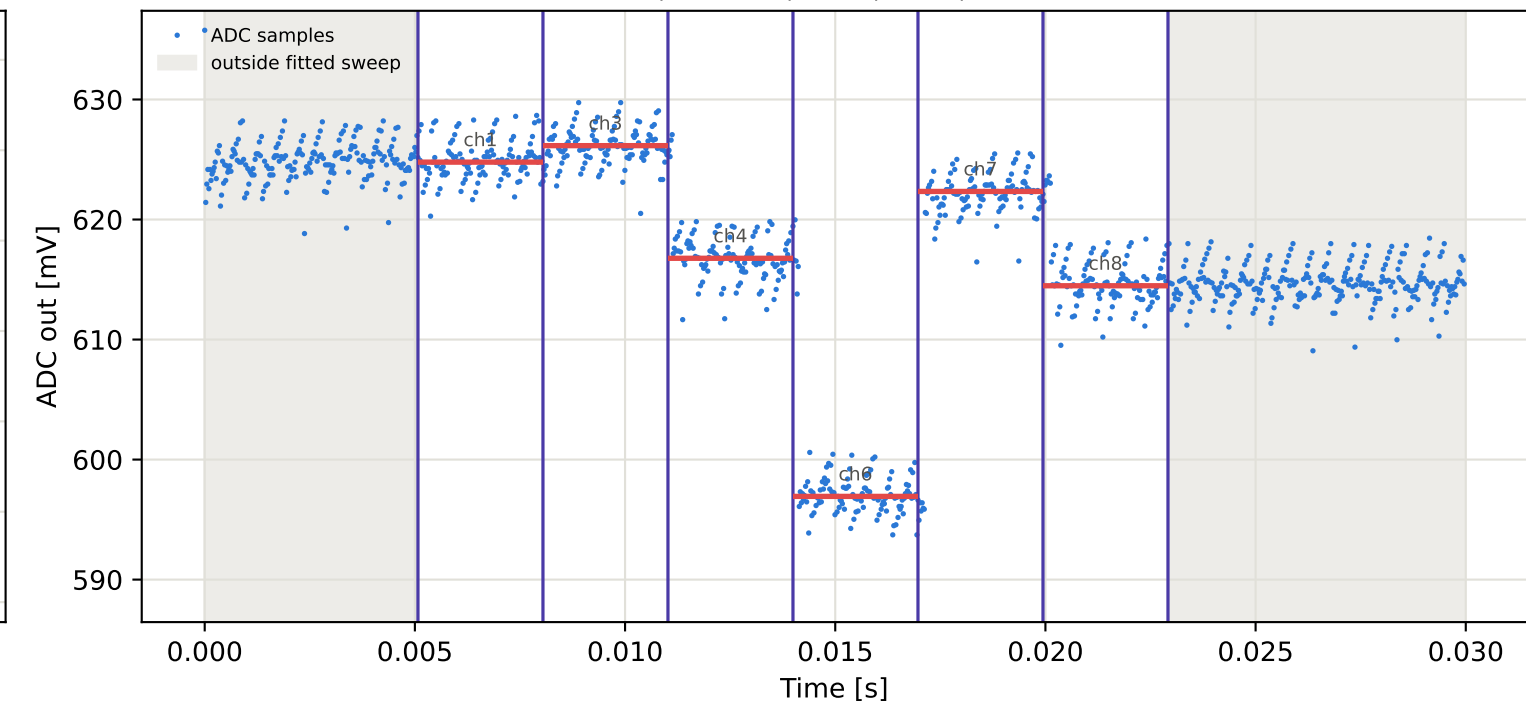
Tag9 &lt;- Tag8 | 945 MHz | run 0 | rep 1 | phase 17.01 deg
