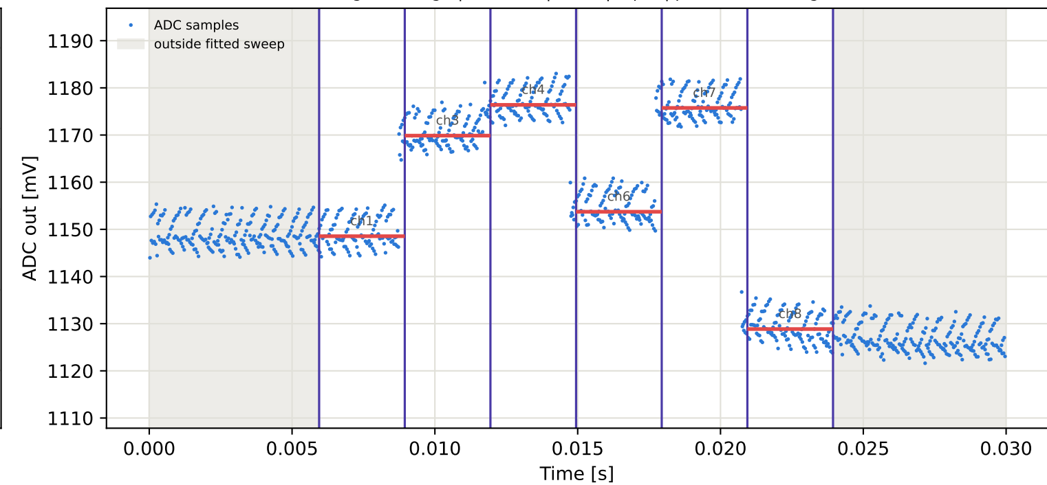
Tag2 &lt;- Tag10 | 895 MHz | run 0 | rep 1 | phase -92.69 deg
