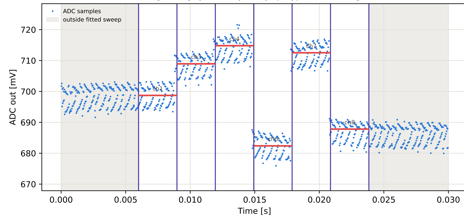
Tag8 &lt;- Tag1 | 935 MHz | run 0 | rep 1 | phase -26.25 deg
