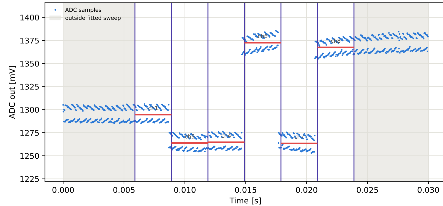
Tag6 &lt;- Tag1 | 905 MHz | run 0 | rep 1 | phase 150.02 deg
