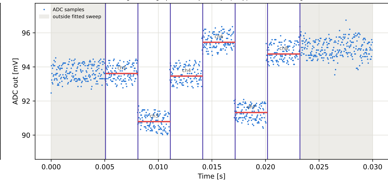
Tag10 &lt;- Tag1 | 805 MHz | run 0 | rep 1 | phase -171.68 deg
