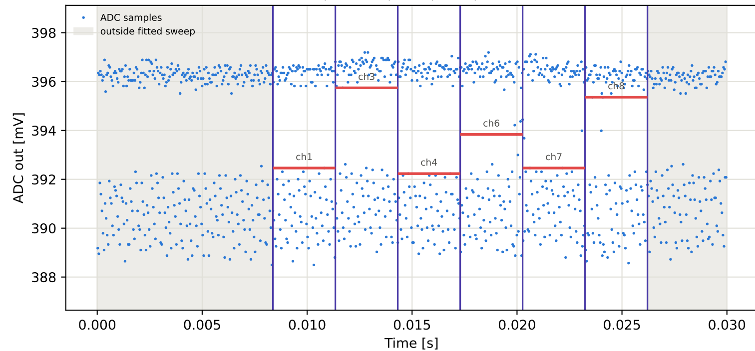
Tag3 &lt;- Tag2 | 955 MHz | run 0 | rep 1 | phase 75.05 deg
