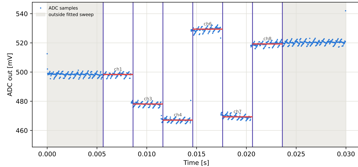
Tag4 &lt;- Tag2 | 985 MHz | run 0 | rep 1 | phase -73.56 deg
