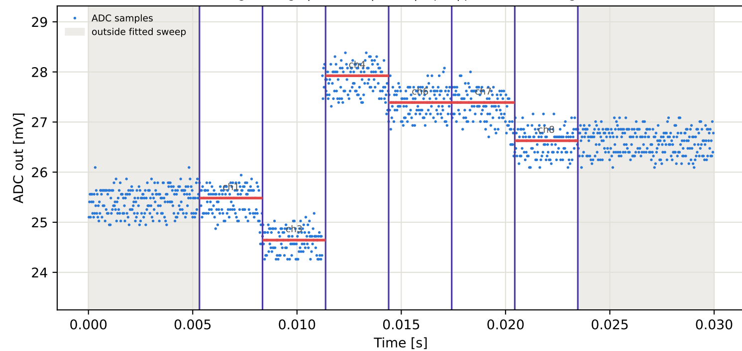
Tag2 &lt;- Tag6 | 805 MHz | run 0 | rep 1 | phase -25.87 deg
