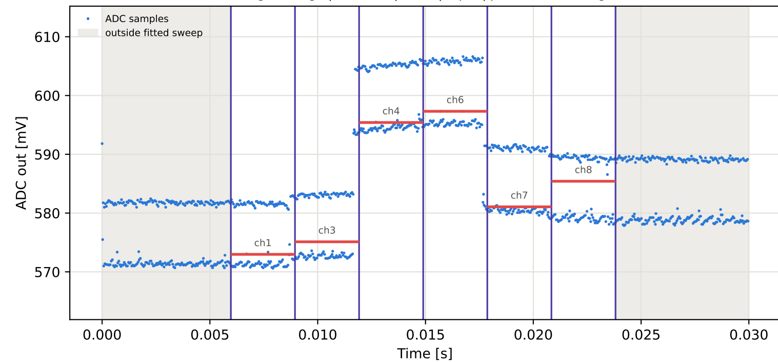
Tag9 &lt;- Tag5 | 975 MHz | run 0 | rep 1 | phase 29.59 deg
