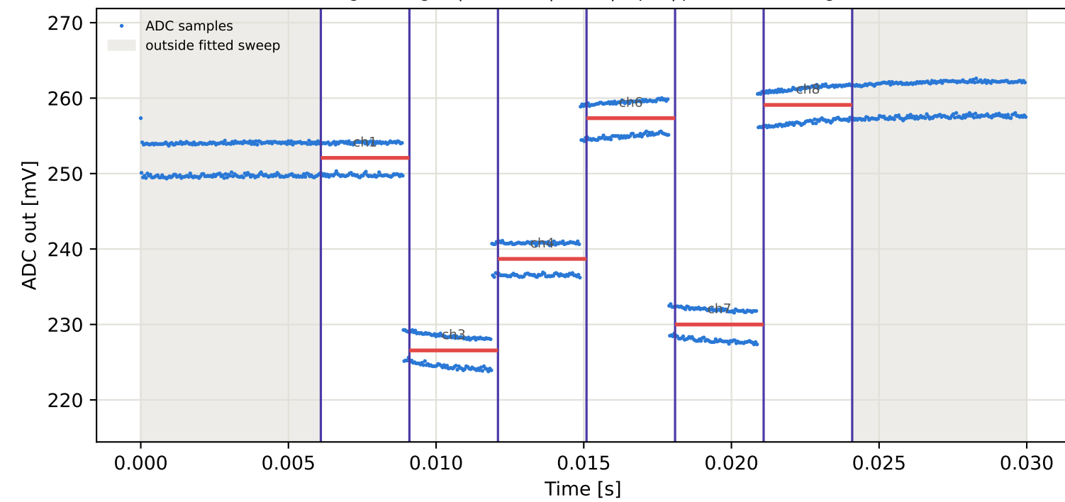
Tag7 &lt;- Tag3 | 825 MHz | run 0 | rep 1 | phase 87.63 deg
