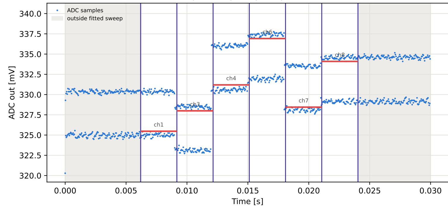
Tag8 &lt;- Tag7 | 805 MHz | run 0 | rep 1 | phase -149.81 deg
