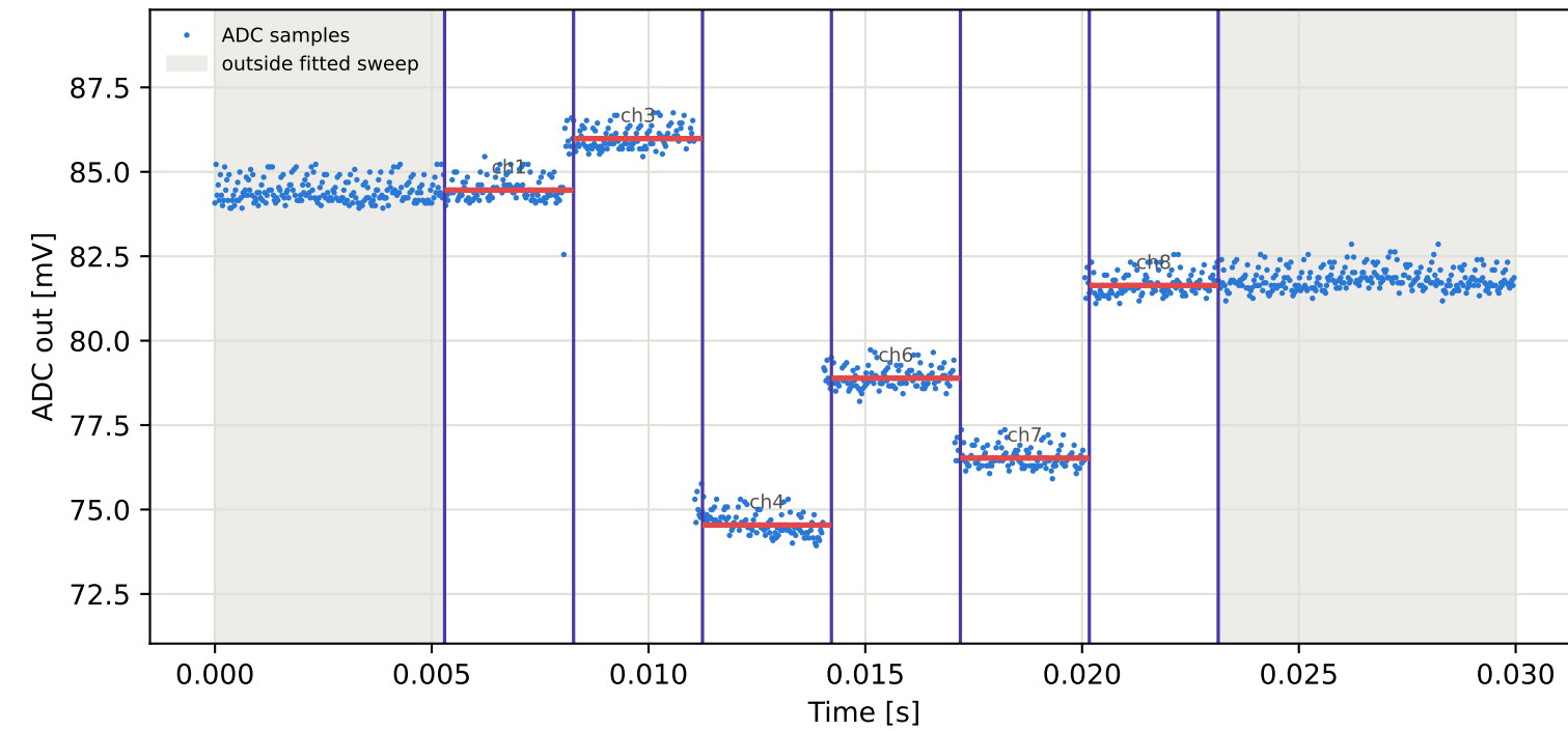
Tag3 &lt;- Tag16 | 785 MHz | run 0 | rep 1 | phase -83.22 deg
