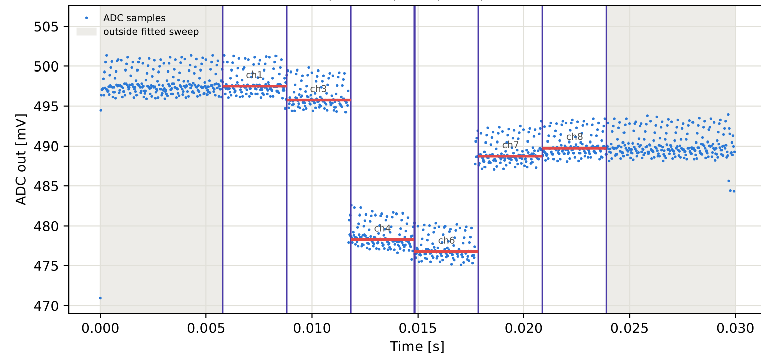
Tag1 &lt;- Tag9 | 975 MHz | run 0 | rep 1 | phase 40.40 deg
