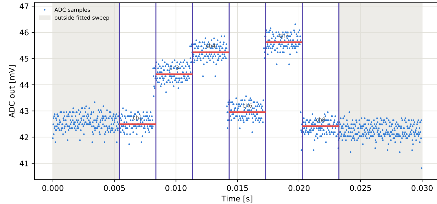
Tag1 &lt;- Tag9 | 795 MHz | run 0 | rep 1 | phase -150.15 deg
