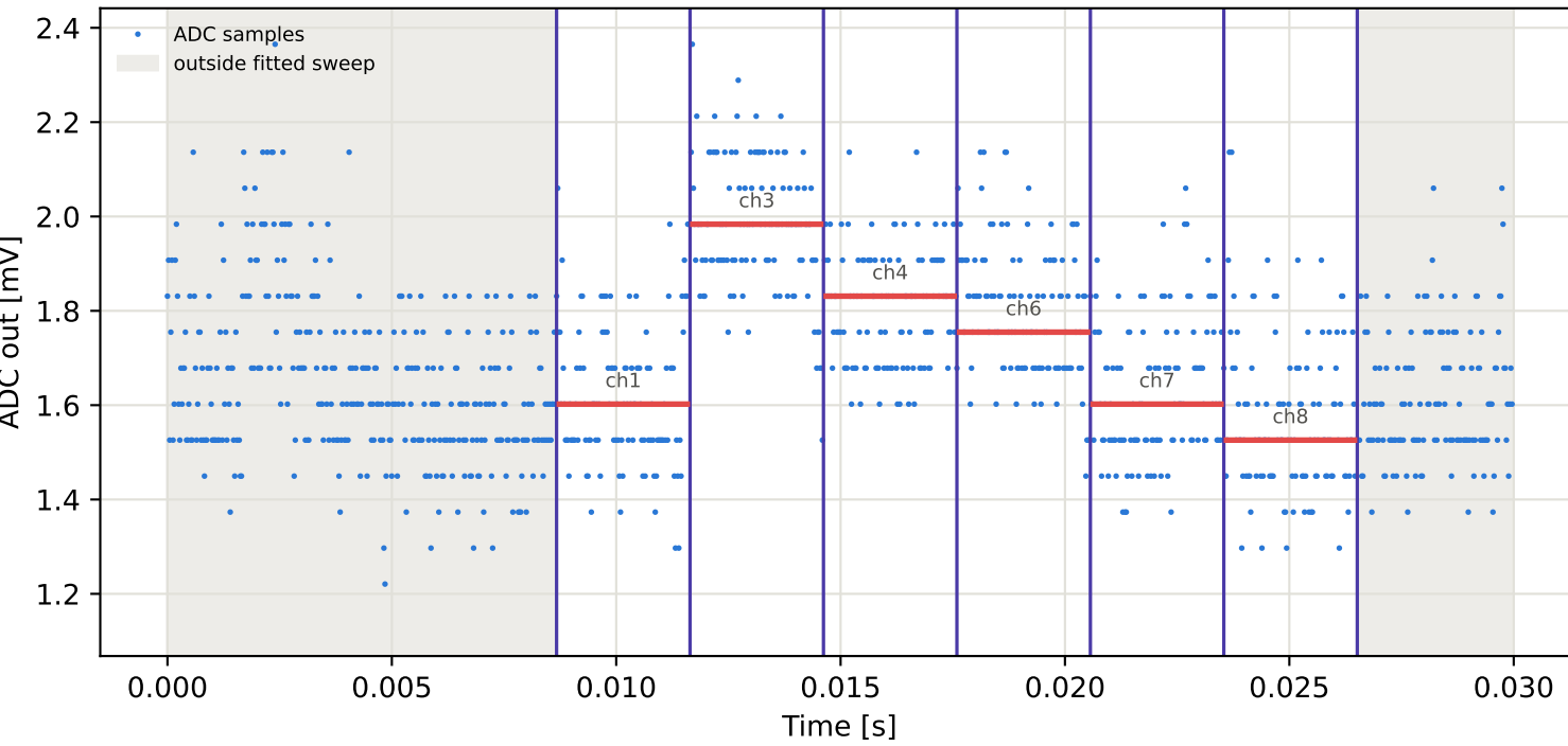
Tag2 &lt;- Tag7 | 985 MHz | run 0 | rep 1 | phase -71.15 deg
