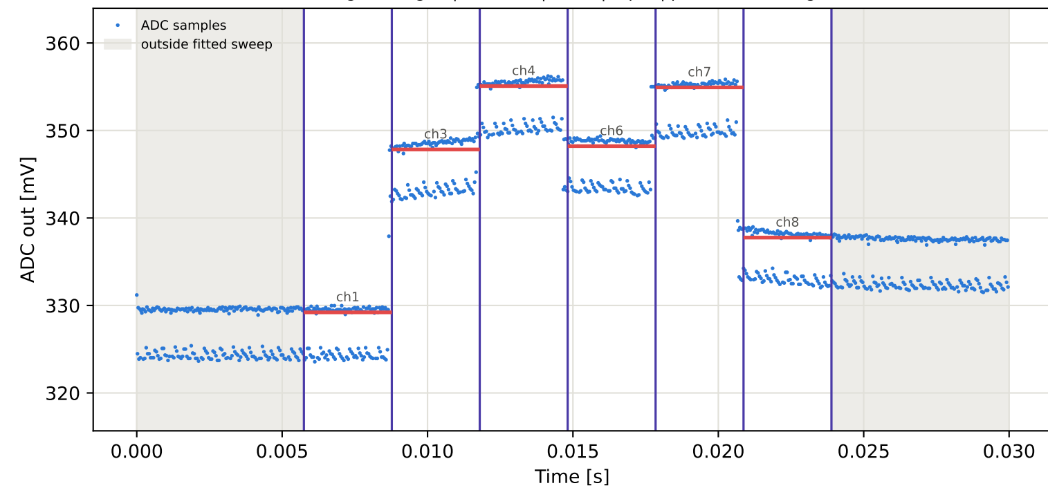
Tag1 &lt;- Tag2 | 865 MHz | run 0 | rep 1 | phase -27.18 deg
