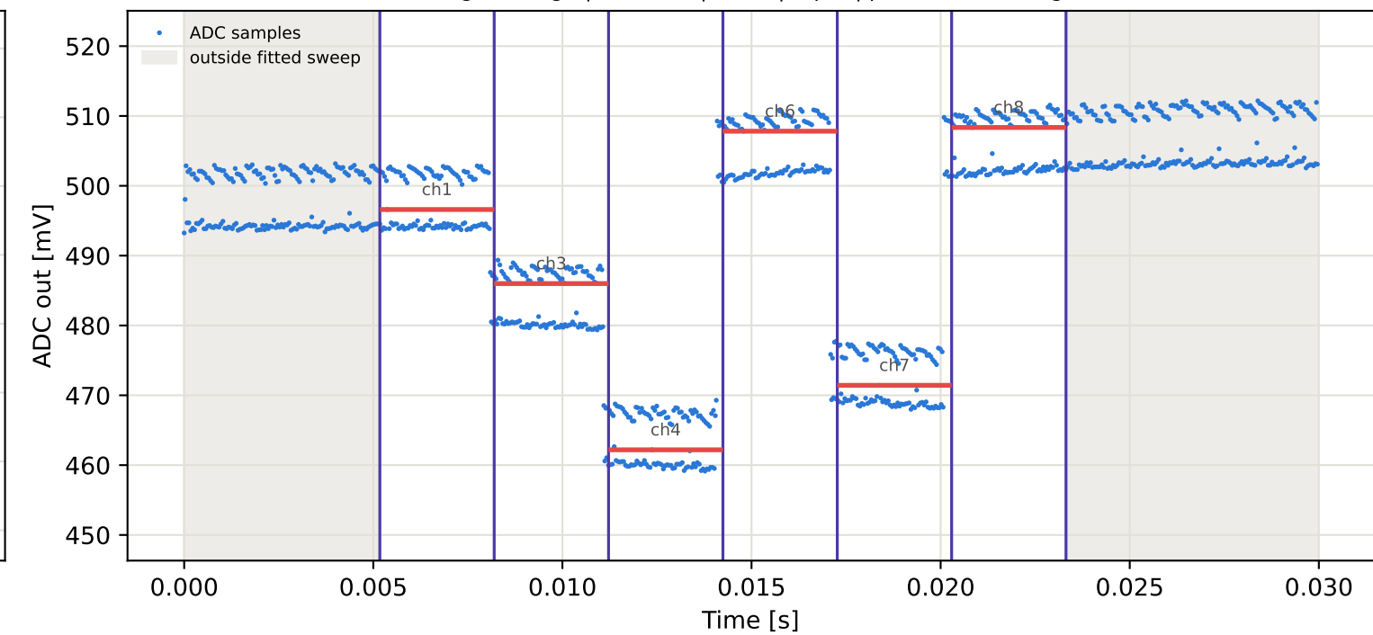
Tag4 &lt;- Tag8 | 985 MHz | run 0 | rep 1 | phase -54.93 deg
