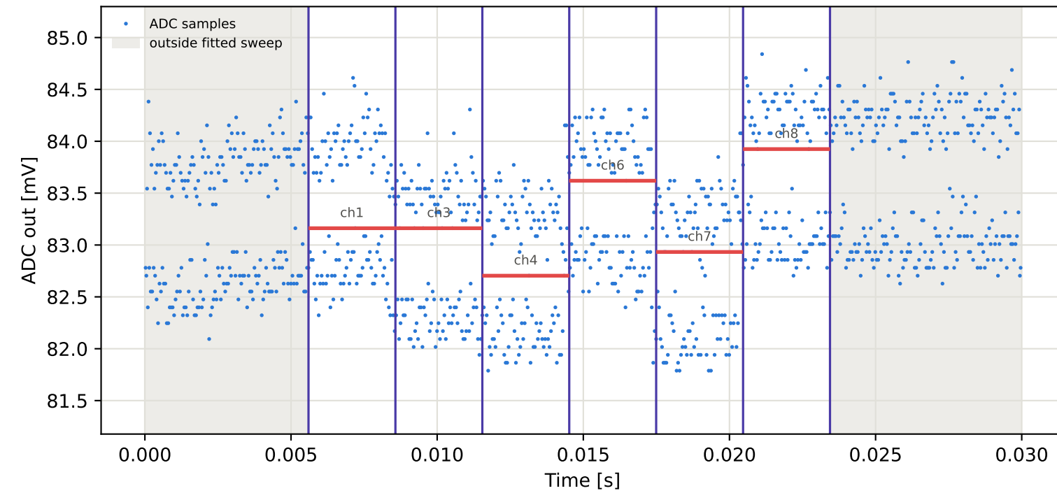
Tag10 &lt;- Tag4 | 825 MHz | run 0 | rep 1 | phase -93.50 deg
