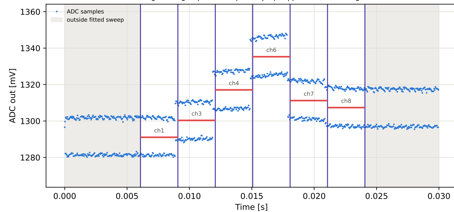
Tag5 &lt;- Tag16 | 905 MHz | run 0 | rep 1 | phase 35.66 deg
