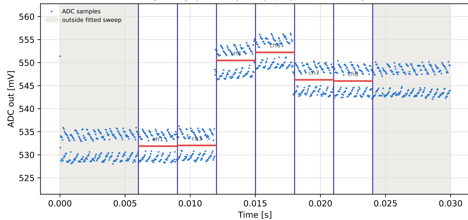
Tag7 &lt;- Tag1 | 835 MHz | run 0 | rep 1 | phase 91.55 deg
