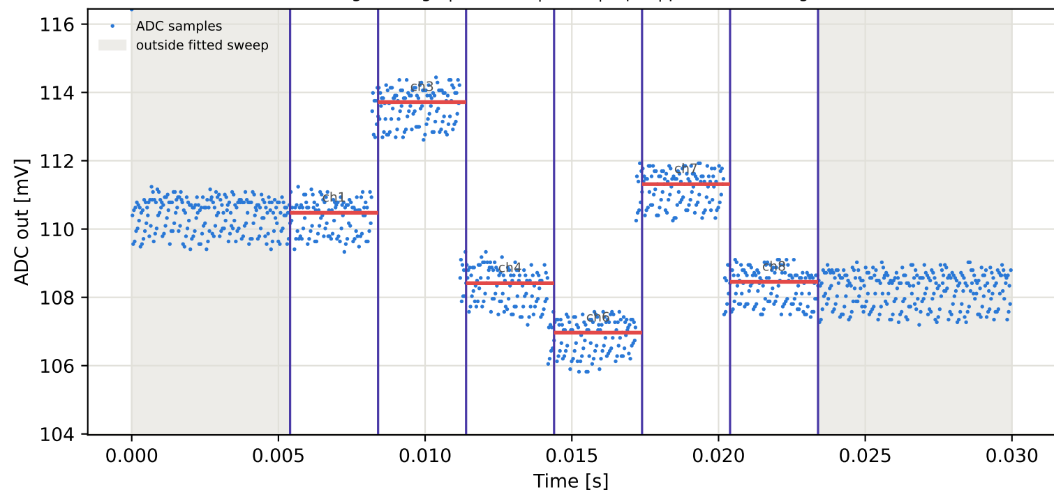
Tag3 &lt;- Tag9 | 775 MHz | run 0 | rep 1 | phase 34.13 deg
