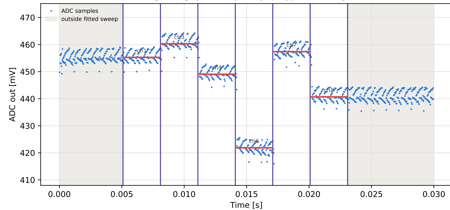
Tag8 &lt;- Tag1 | 965 MHz | run 0 | rep 1 | phase 139.46 deg
