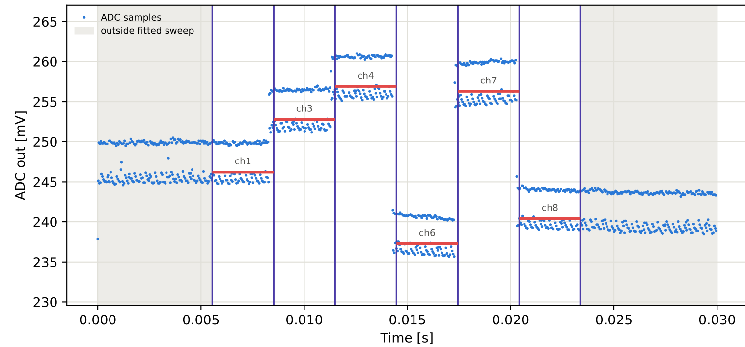
Tag3 &lt;- Tag8 | 995 MHz | run 0 | rep 1 | phase -42.27 deg
