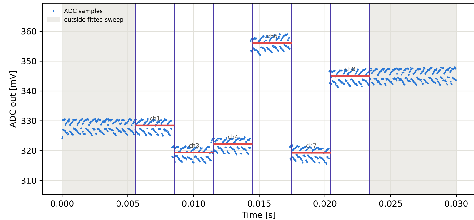
Tag6 &lt;- Tag1 | 935 MHz | run 0 | rep 1 | phase 168.88 deg
