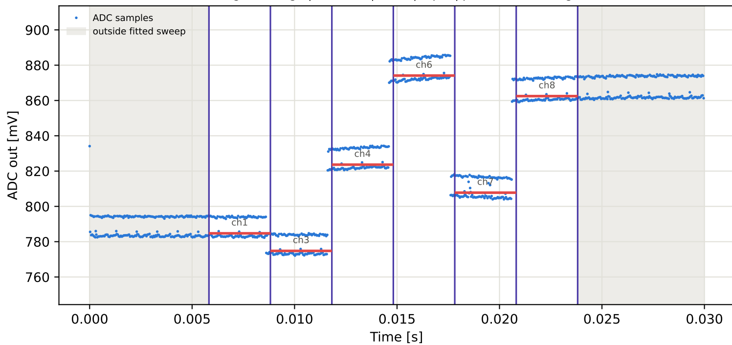
Tag2 &lt;- Tag1 | 865 MHz | run 0 | rep 1 | phase 33.86 deg
