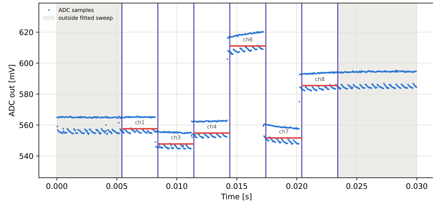
Tag9 &lt;- Tag7 | 925 MHz | run 0 | rep 1 | phase 178.94 deg
