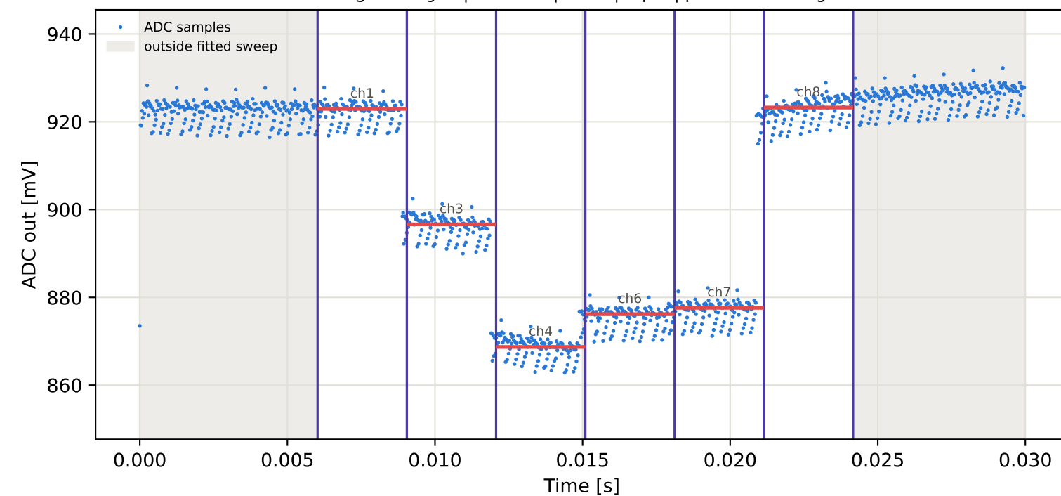
Tag1 &lt;- Tag16 | 905 MHz | run 0 | rep 1 | phase 7.53 deg
