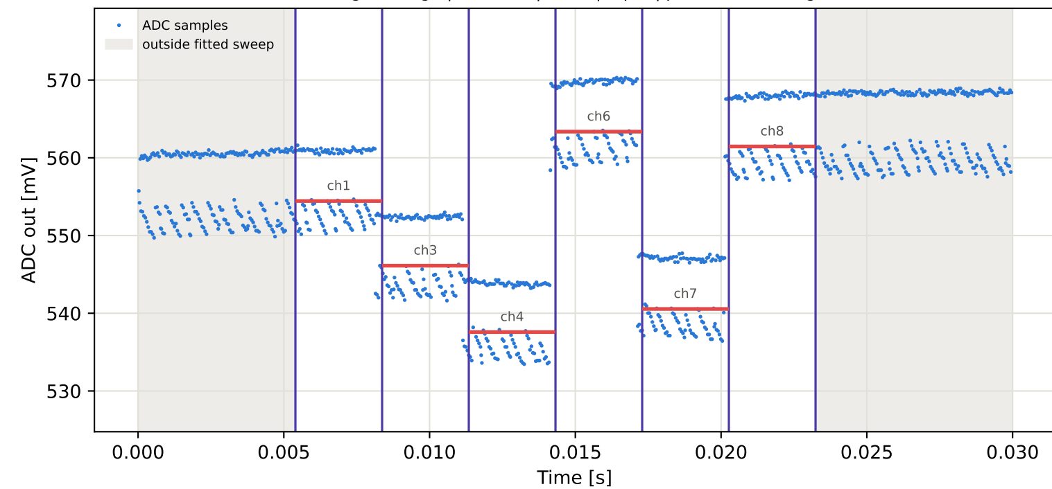
Tag5 &lt;- Tag8 | 975 MHz | run 0 | rep 1 | phase -162.05 deg
