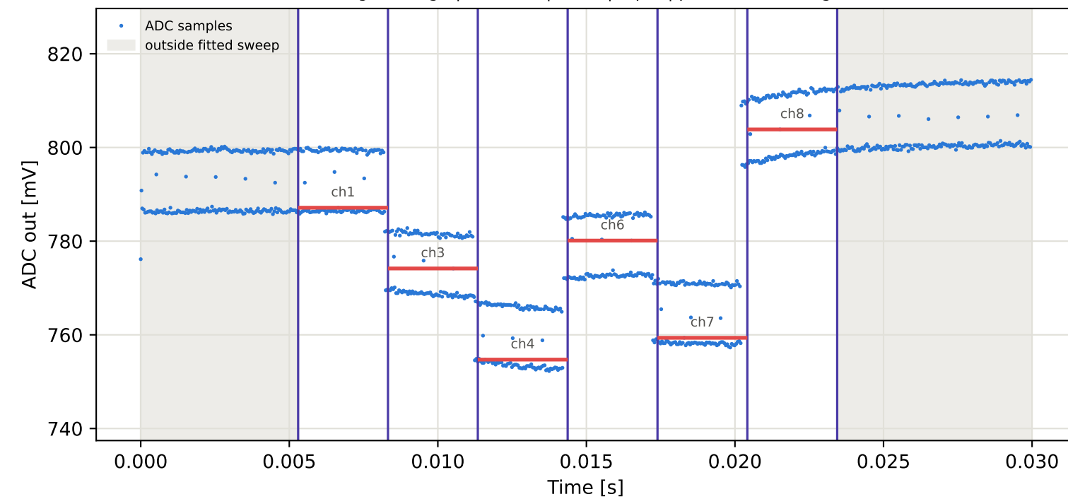
Tag4 &lt;- Tag15 | 905 MHz | run 0 | rep 1 | phase -2.59 deg
