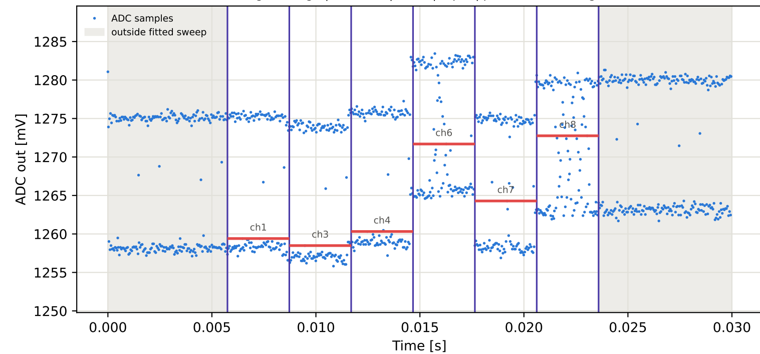
Tag8 &lt;- Tag4 | 885 MHz | run 0 | rep 1 | phase -93.63 deg
