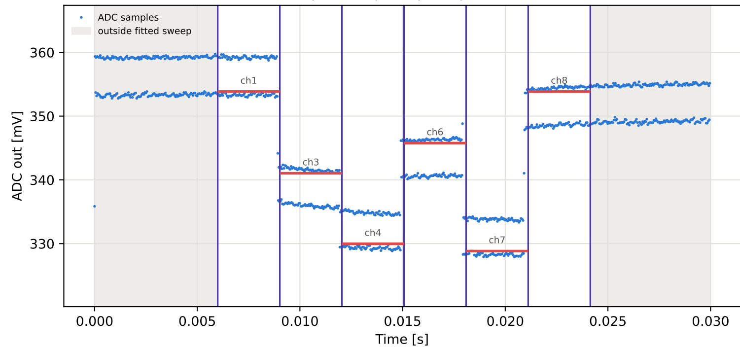
Tag9 &lt;- Tag8 | 835 MHz | run 0 | rep 1 | phase 105.57 deg
