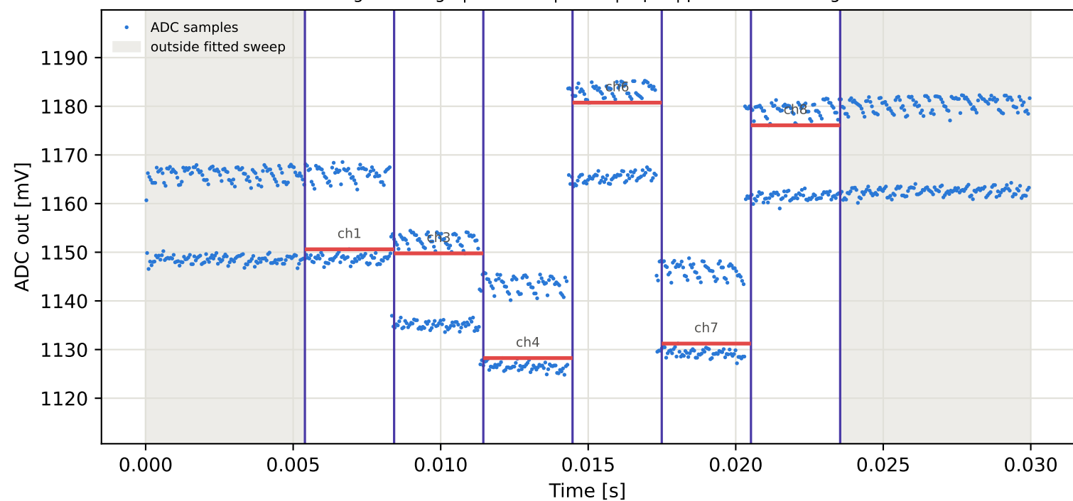
Tag2 &lt;- Tag10 | 955 MHz | run 0 | rep 1 | phase 82.07 deg
