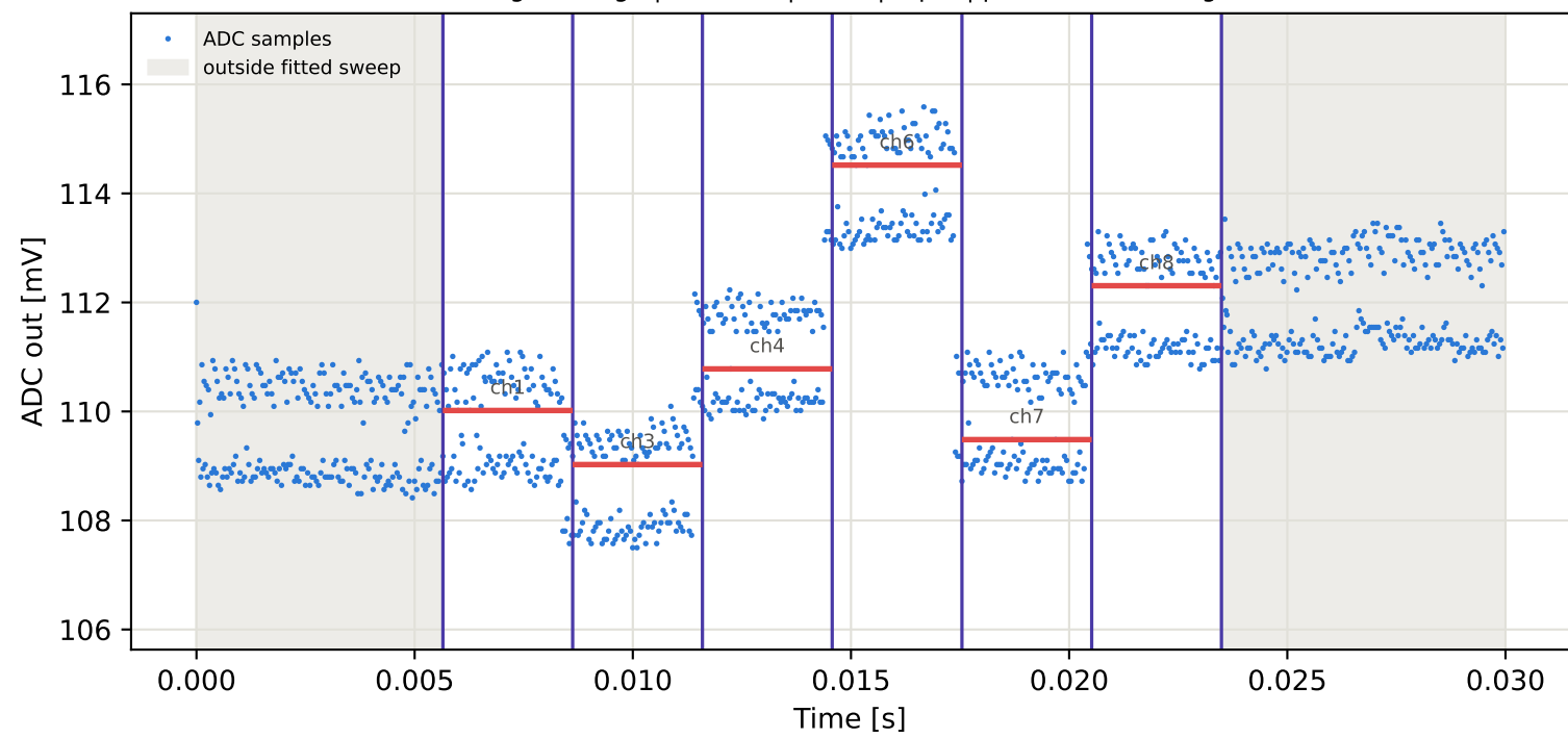
Tag3 &lt;- Tag2 | 775 MHz | run 0 | rep 1 | phase -159.14 deg
