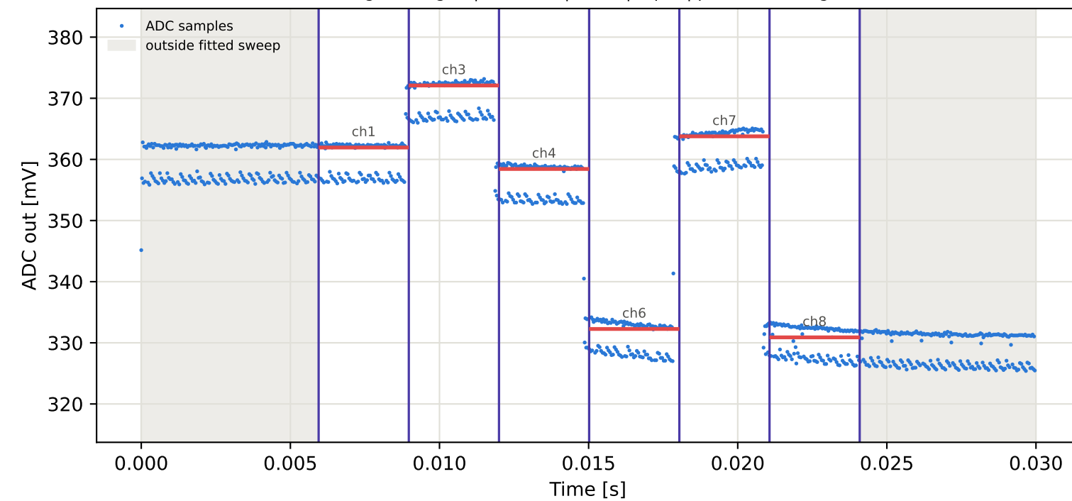
Tag1 &lt;- Tag16 | 865 MHz | run 0 | rep 1 | phase -85.70 deg
