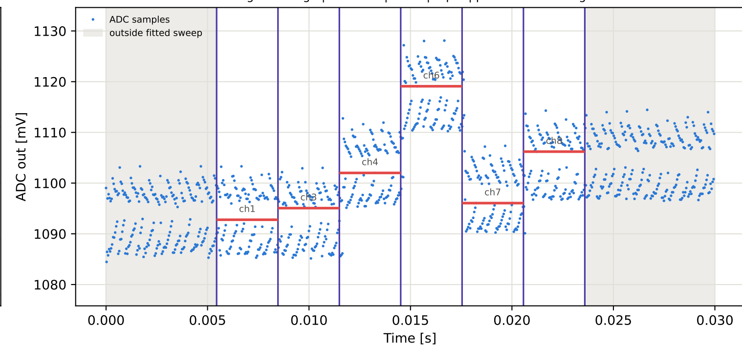
Tag16 &lt;- Tag15 | 945 MHz | run 0 | rep 1 | phase -89.90 deg
