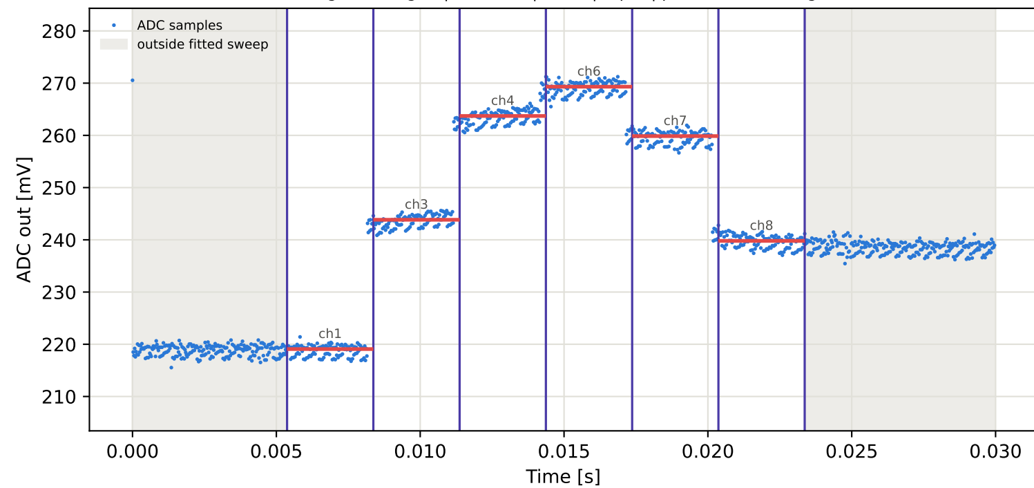
Tag10 &lt;- Tag3 | 885 MHz | run 0 | rep 1 | phase -153.59 deg
