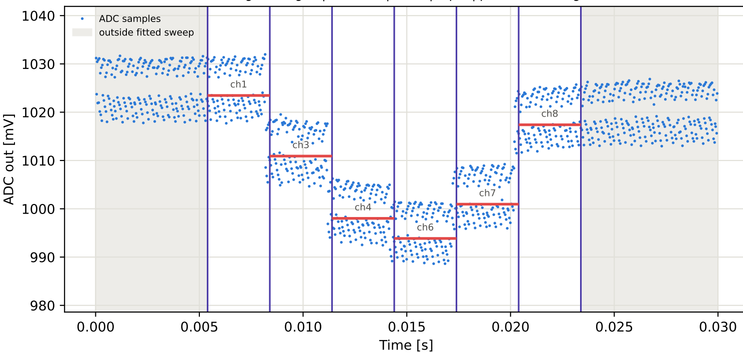
Tag3 &lt;- Tag16 | 895 MHz | run 0 | rep 1 | phase 60.22 deg
