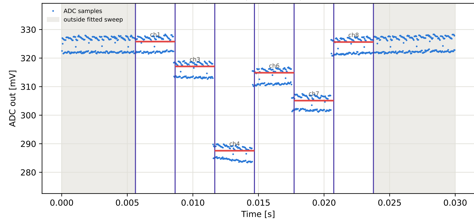
Tag6 &lt;- Tag10 | 985 MHz | run 0 | rep 1 | phase 74.99 deg
