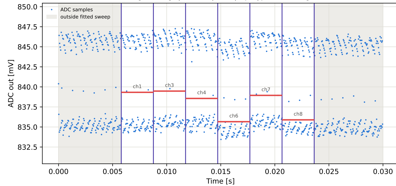
Tag16 &lt;- Tag4 | 865 MHz | run 0 | rep 1 | phase 76.30 deg
