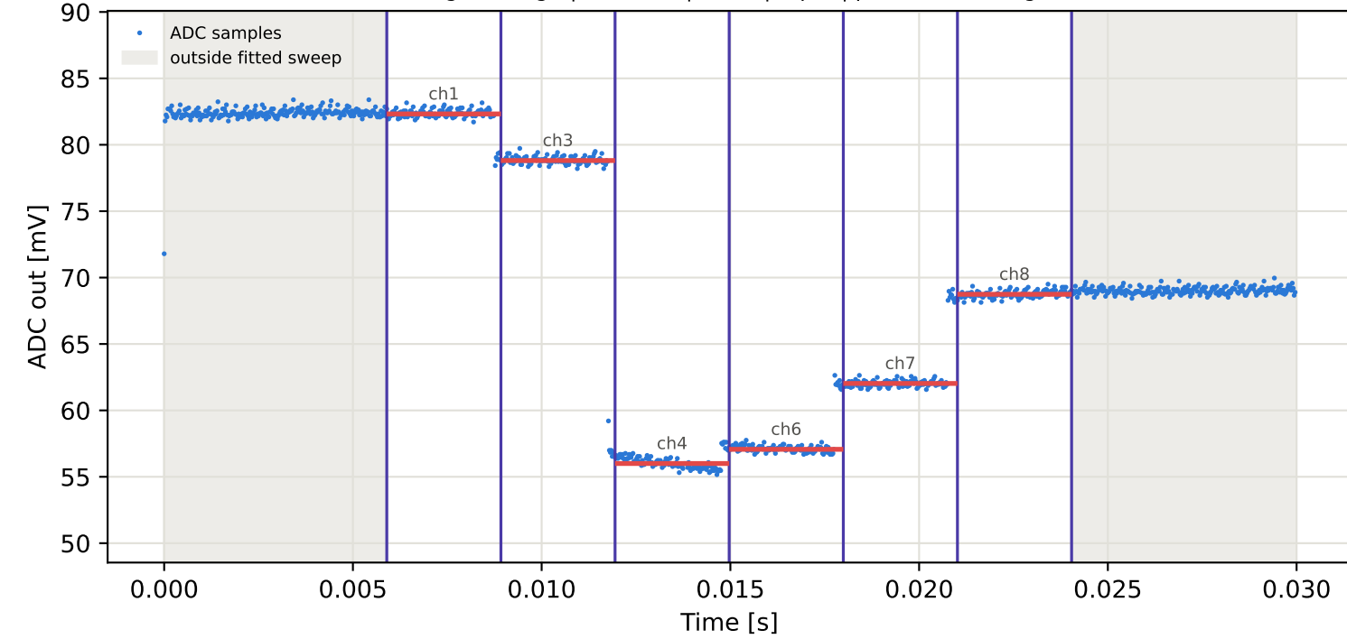
Tag1 &lt;- Tag8 | 835 MHz | run 0 | rep 1 | phase -174.47 deg
