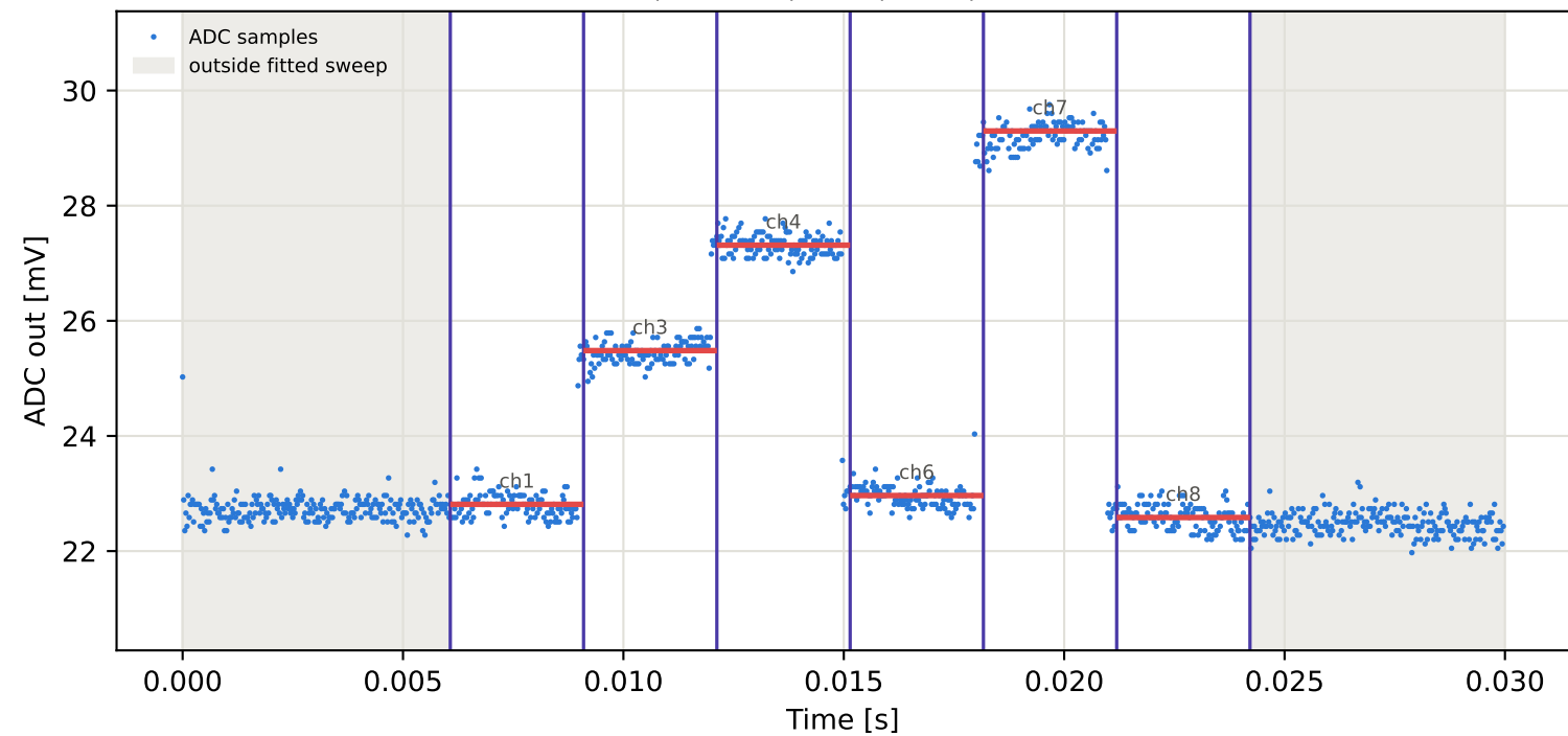
Tag6 &lt;- Tag4 | 775 MHz | run 0 | rep 1 | phase -47.97 deg
