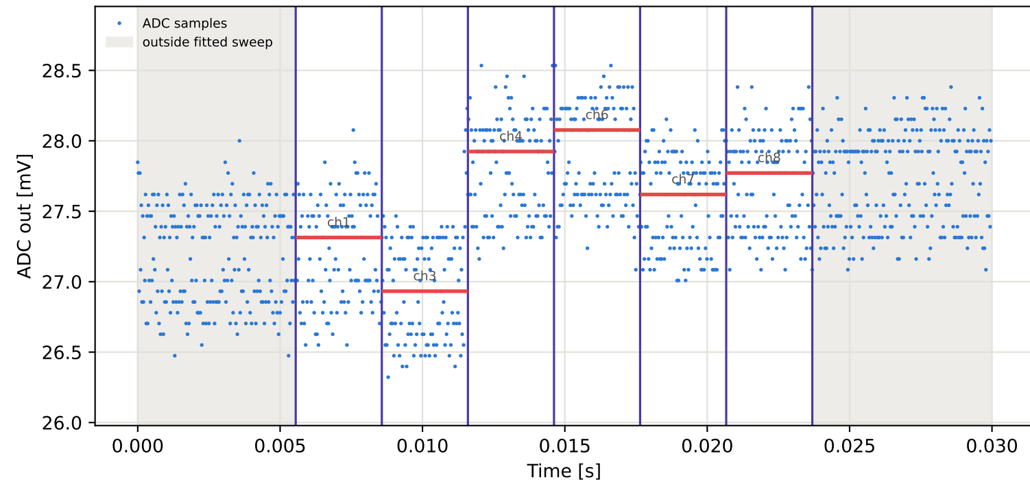
Tag2 &lt;- Tag16 | 825 MHz | run 0 | rep 1 | phase -128.52 deg
