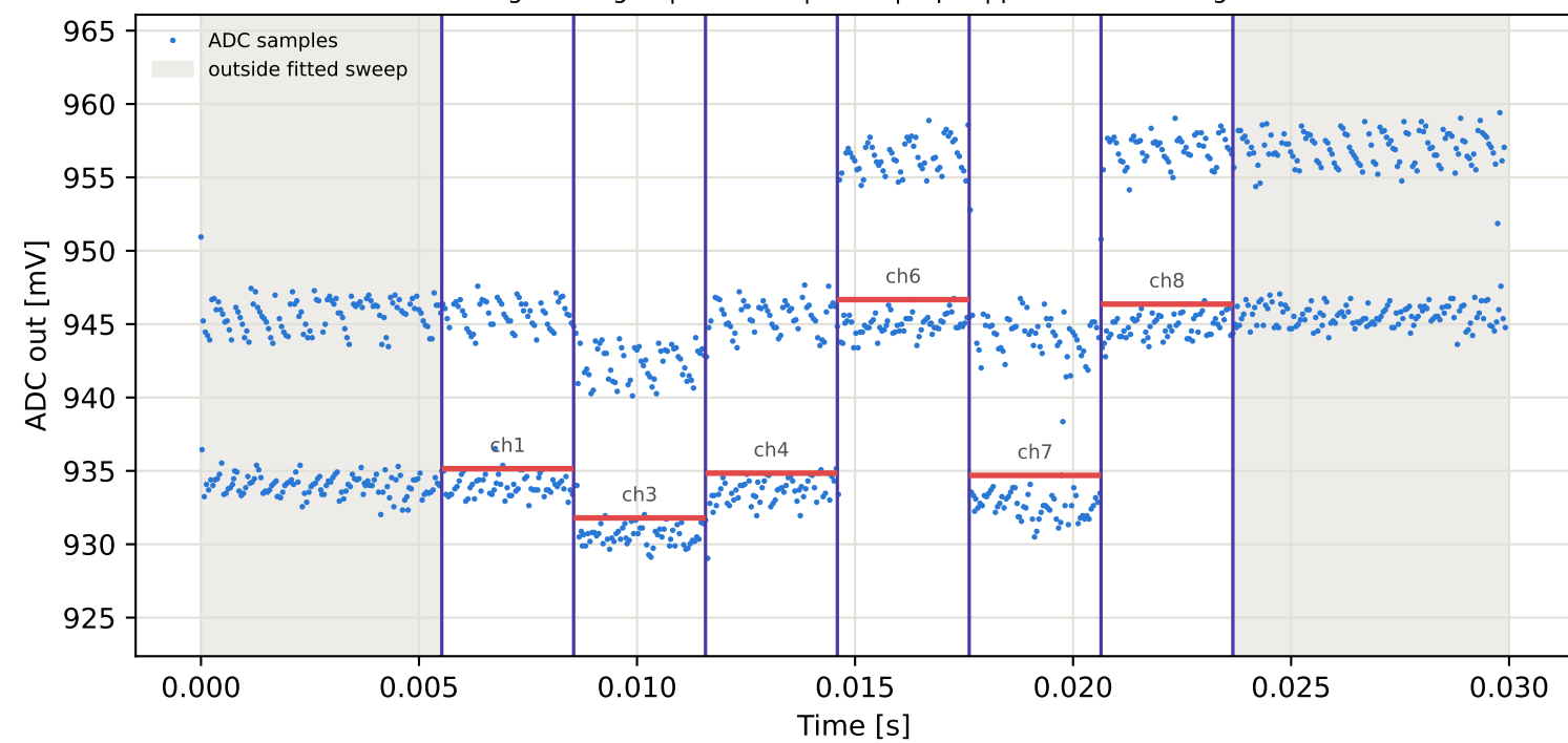
Tag5 &lt;- Tag16 | 885 MHz | run 0 | rep 1 | phase 31.90 deg
