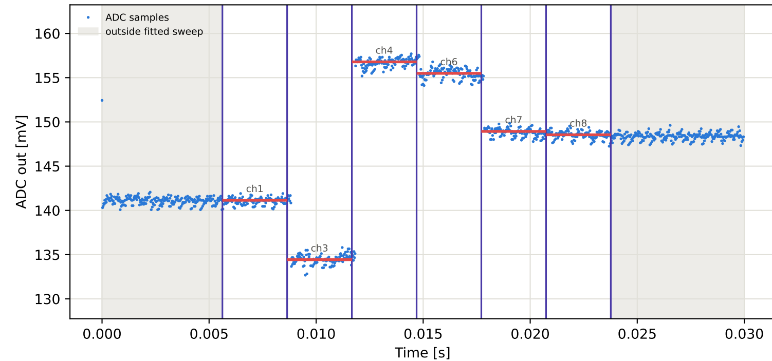
Tag4 &lt;- Tag2 | 785 MHz | run 0 | rep 1 | phase 13.93 deg
