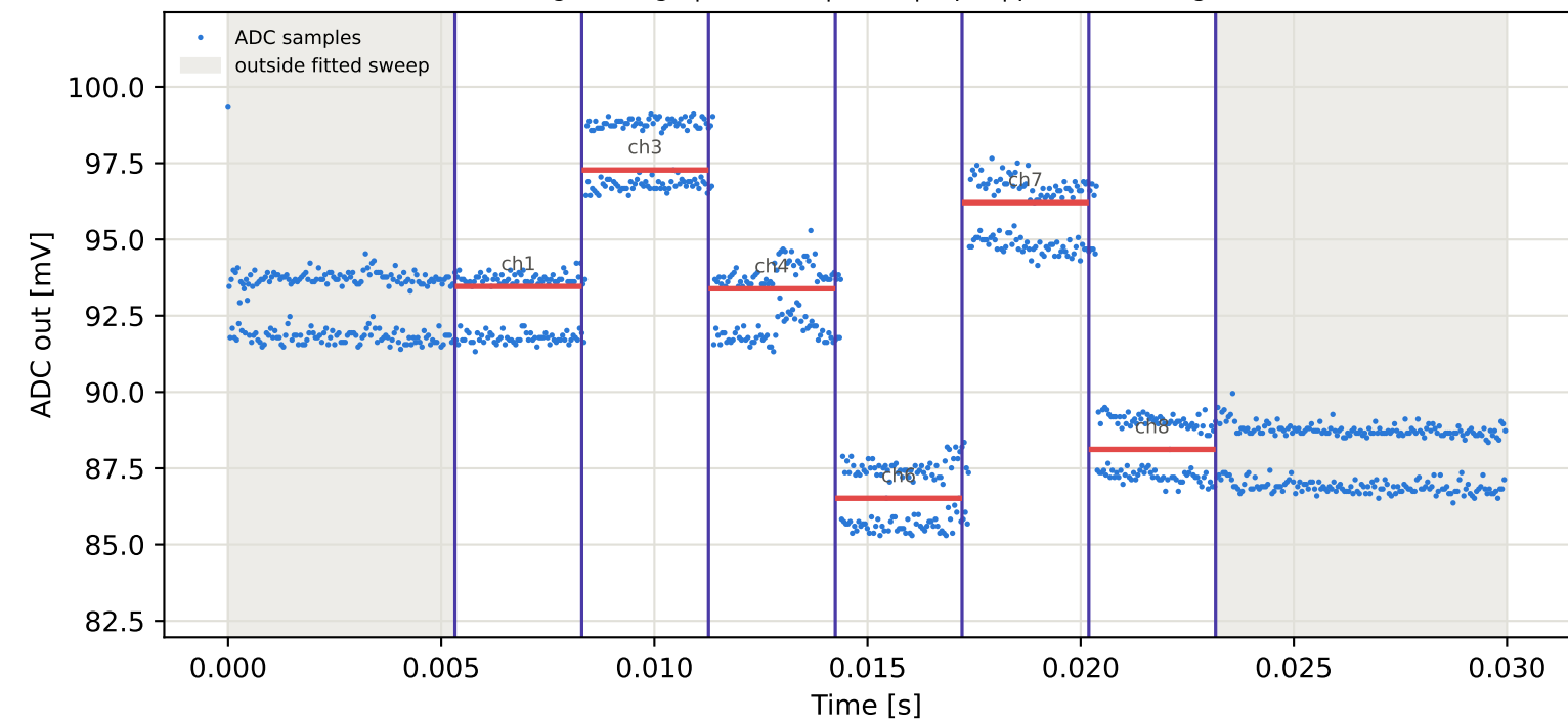
Tag4 &lt;- Tag8 | 805 MHz | run 0 | rep 1 | phase 106.29 deg
