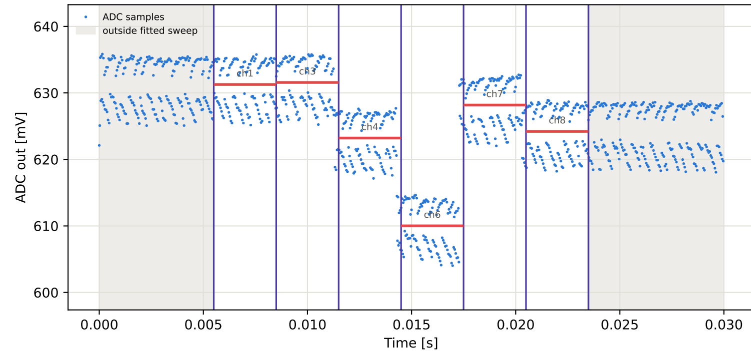
Tag7 &lt;- Tag5 | 955 MHz | run 0 | rep 1 | phase 111.60 deg
