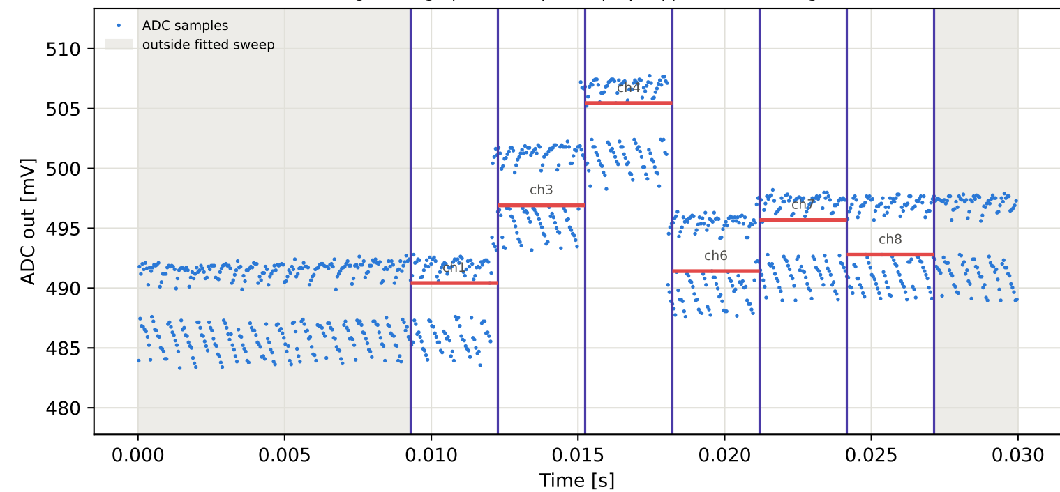
Tag5 &lt;- Tag9 | 955 MHz | run 0 | rep 1 | phase -64.60 deg
