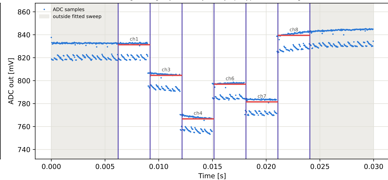
Tag4 &lt;- Tag3 | 925 MHz | run 0 | rep 1 | phase 134.11 deg
