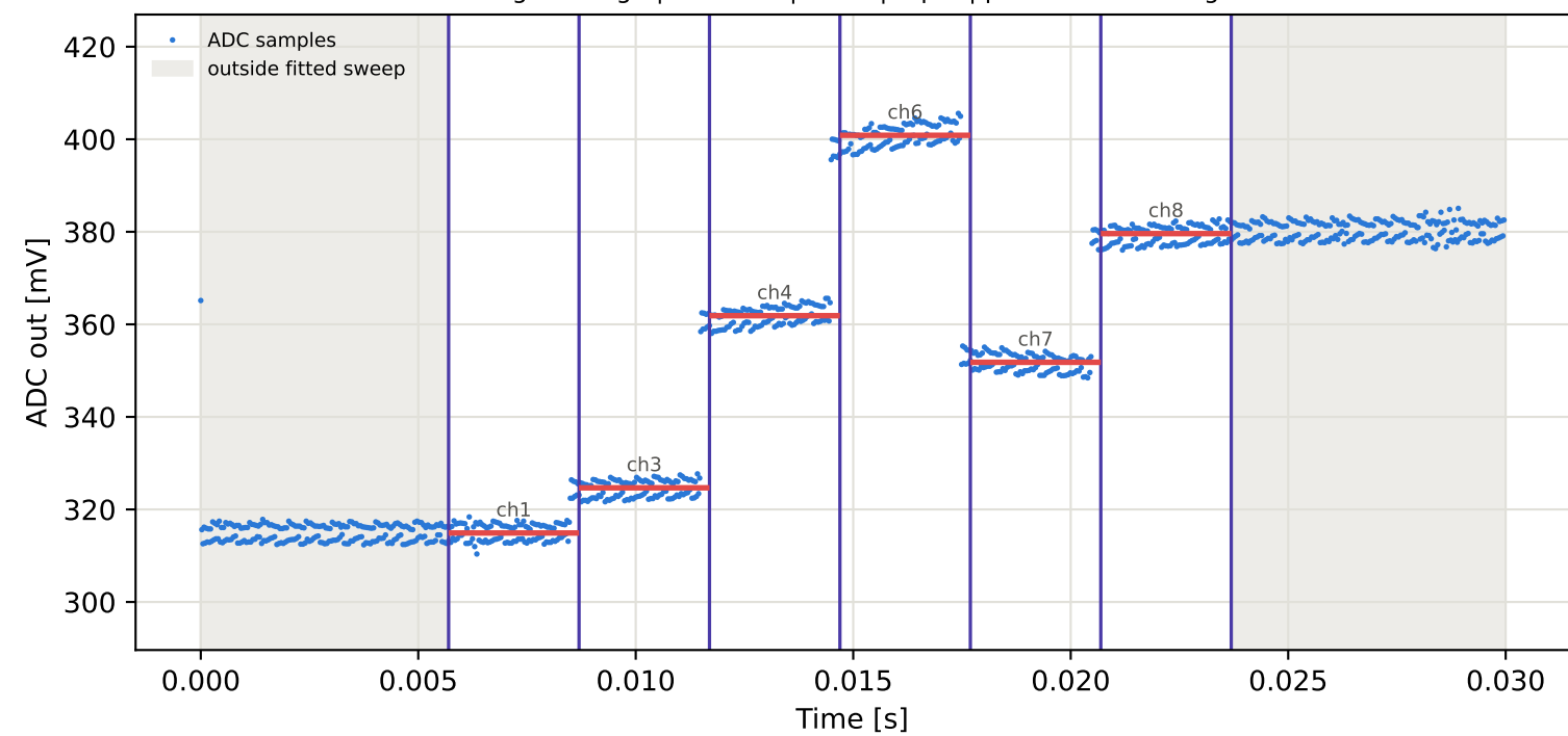
Tag4 &lt;- Tag8 | 875 MHz | run 0 | rep 1 | phase -129.58 deg
