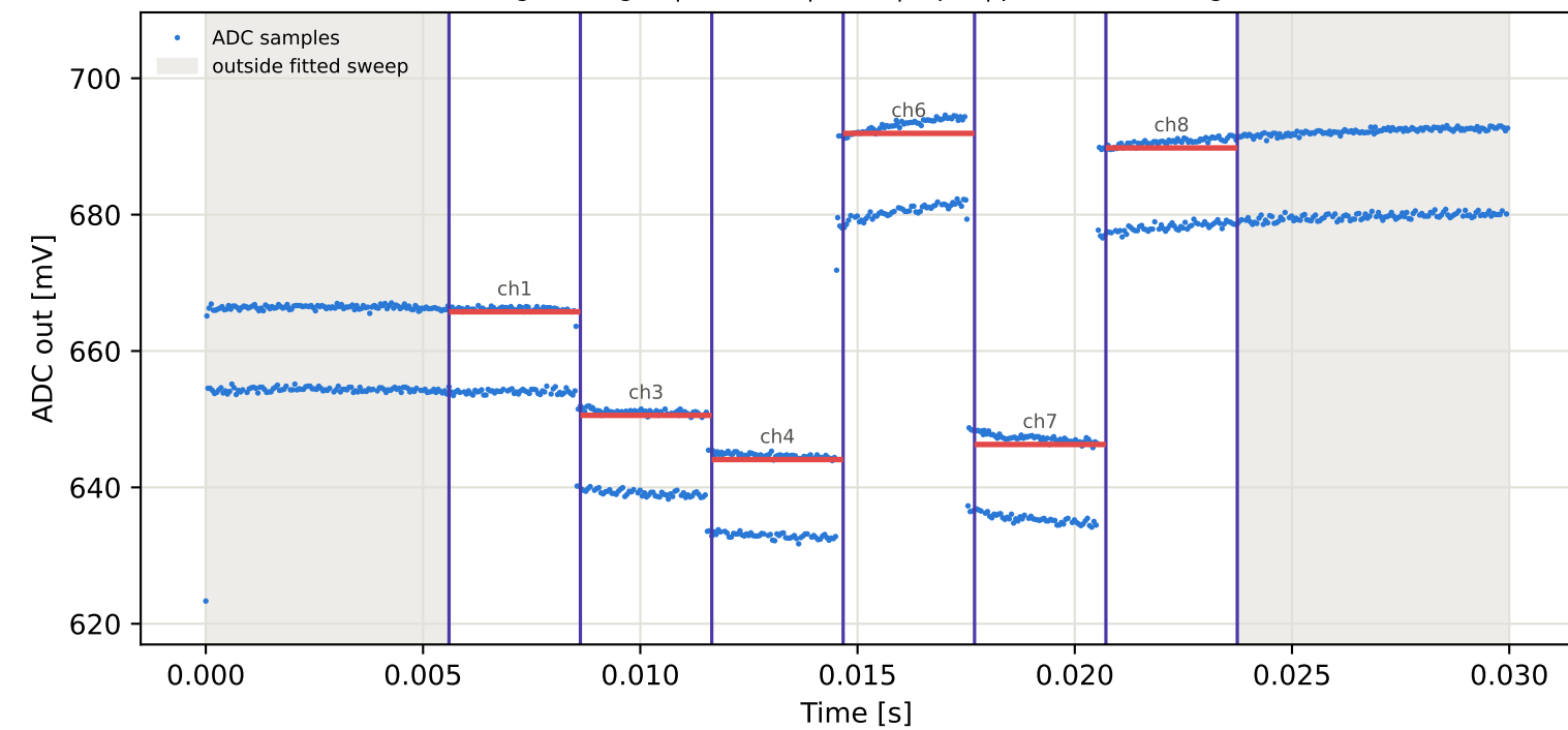
Tag1 &lt;- Tag16 | 925 MHz | run 0 | rep 1 | phase -32.62 deg
