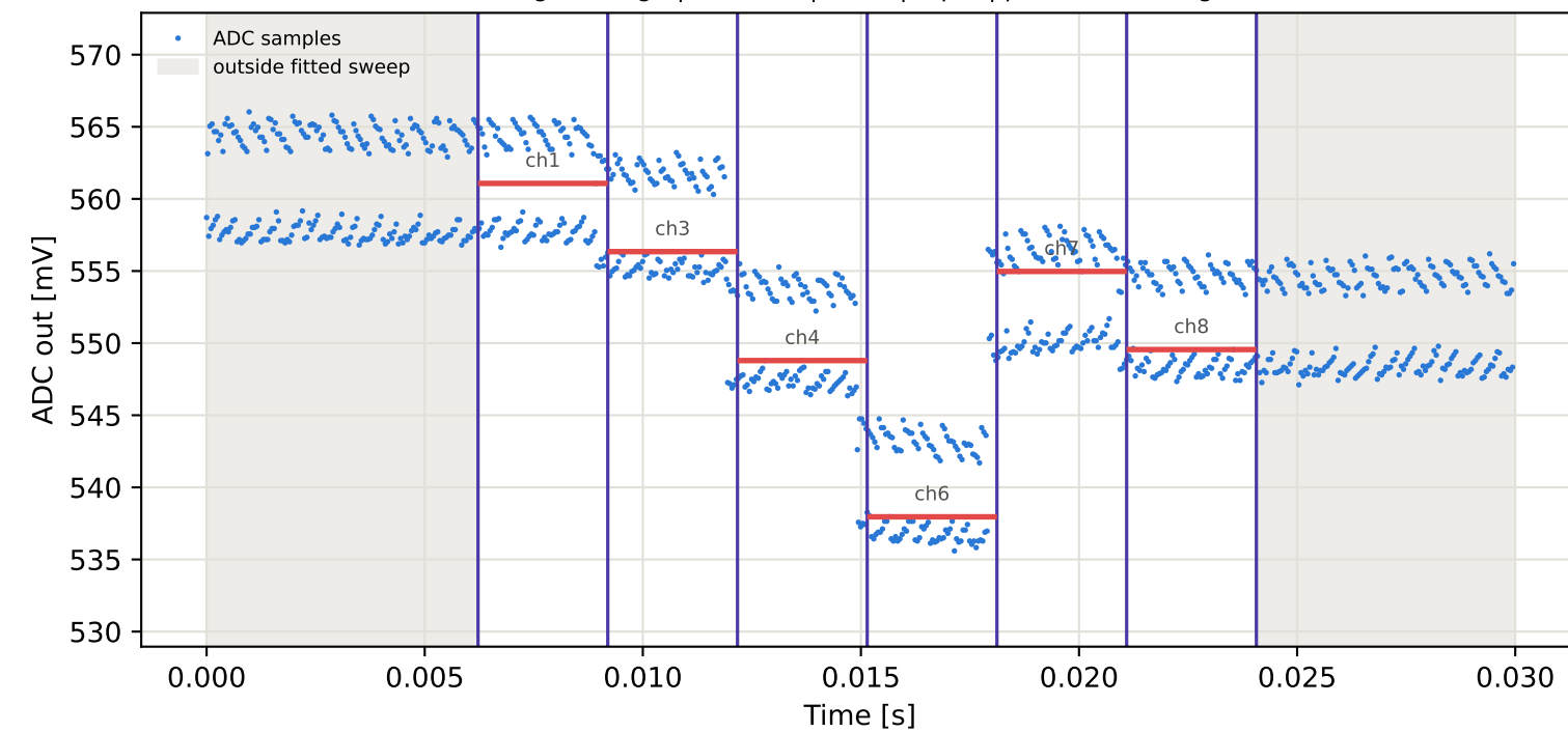
Tag7 &lt;- Tag5 | 895 MHz | run 0 | rep 1 | phase 15.19 deg
