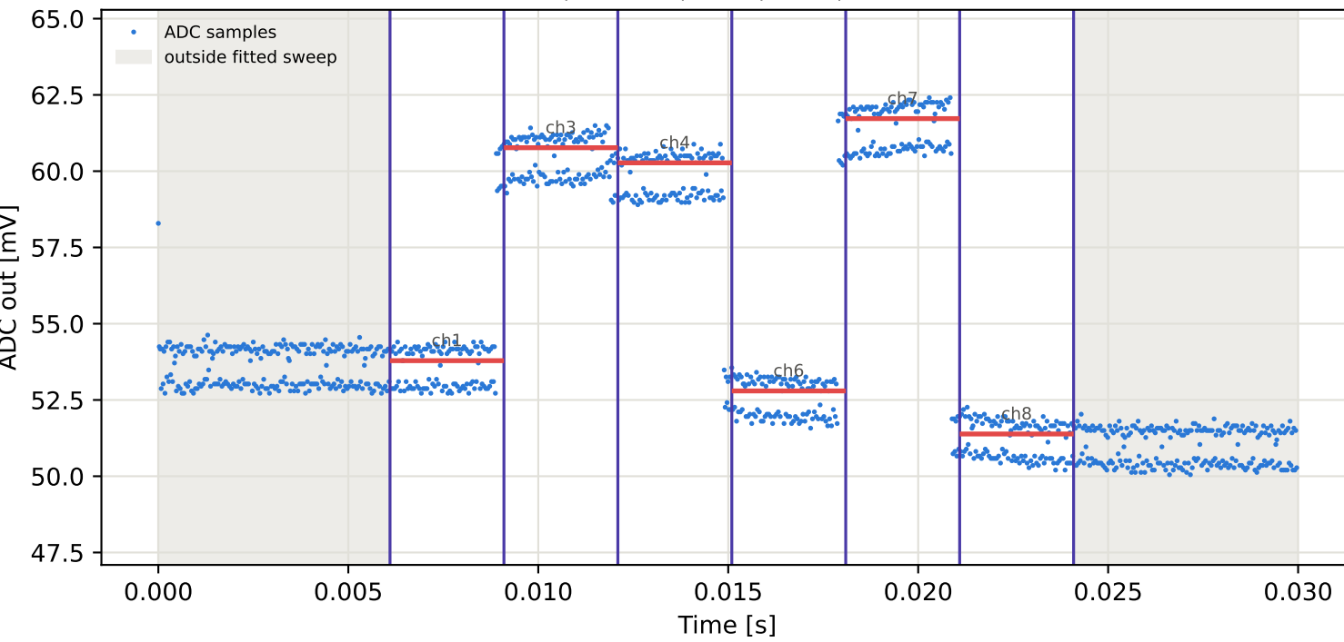
Tag1 &lt;- Tag9 | 835 MHz | run 0 | rep 1 | phase -34.77 deg
