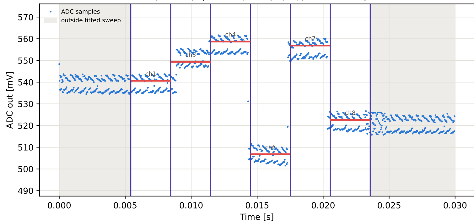
Tag10 &lt;- Tag5 | 955 MHz | run 0 | rep 1 | phase 45.81 deg
