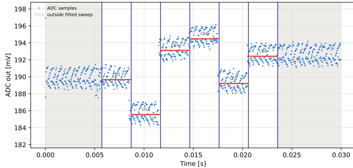
Tag5 &lt;- Tag3 | 785 MHz | run 0 | rep 1 | phase -102.92 deg
