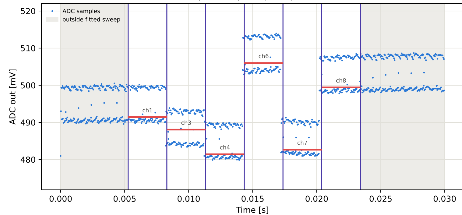
Tag5 &lt;- Tag16 | 955 MHz | run 0 | rep 1 | phase 167.67 deg
