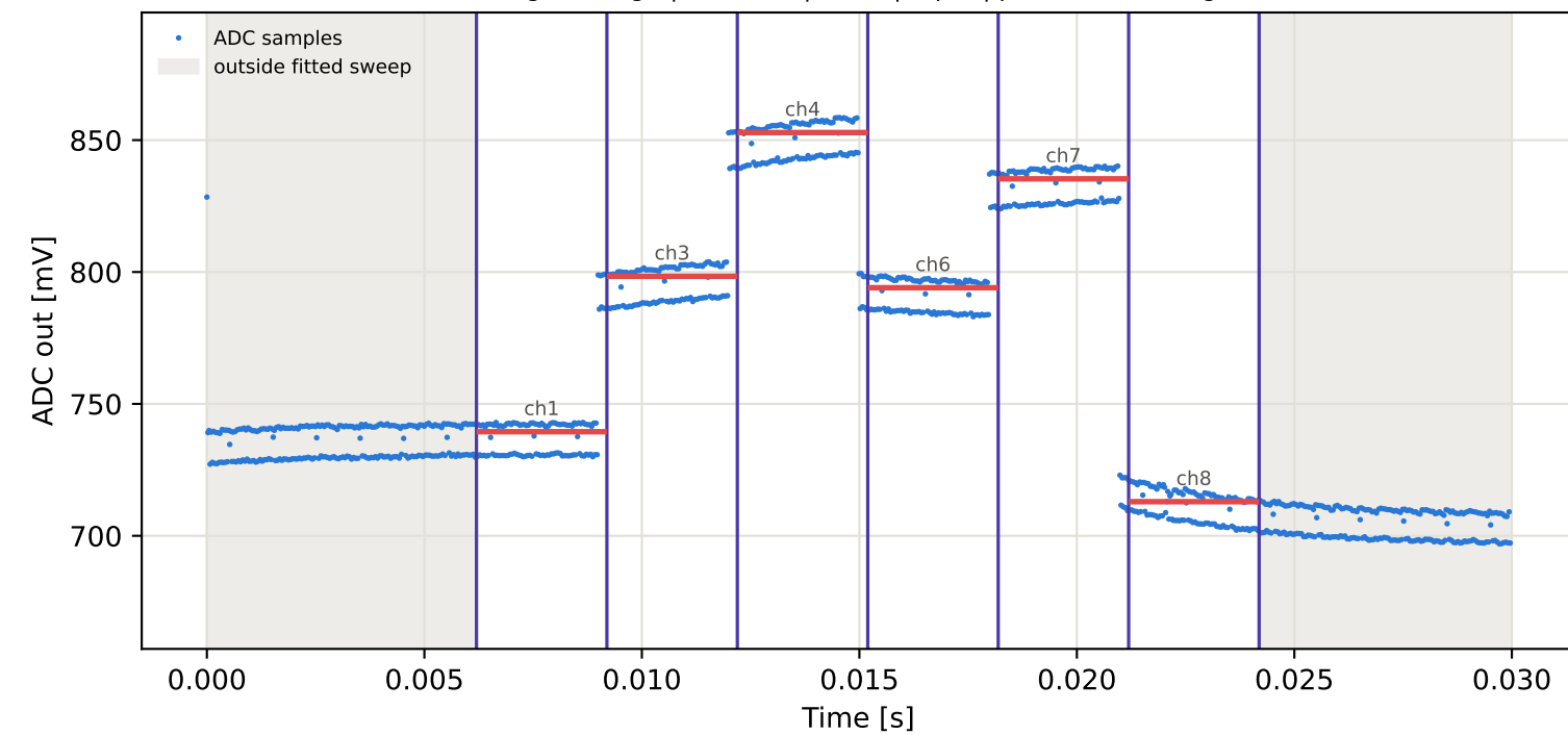
Tag4 &lt;- Tag7 | 905 MHz | run 0 | rep 1 | phase 56.37 deg
