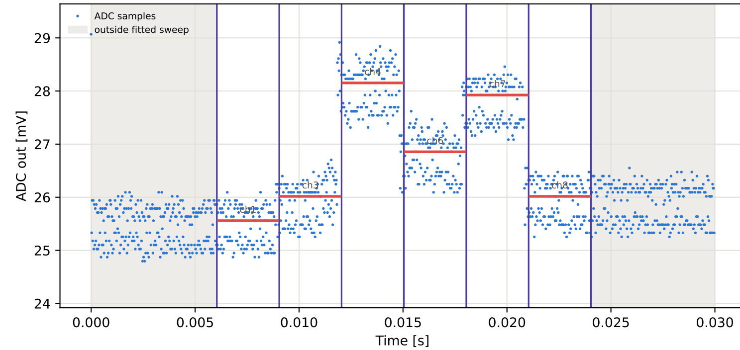
Tag2 &lt;- Tag15 | 785 MHz | run 0 | rep 1 | phase -89.38 deg
