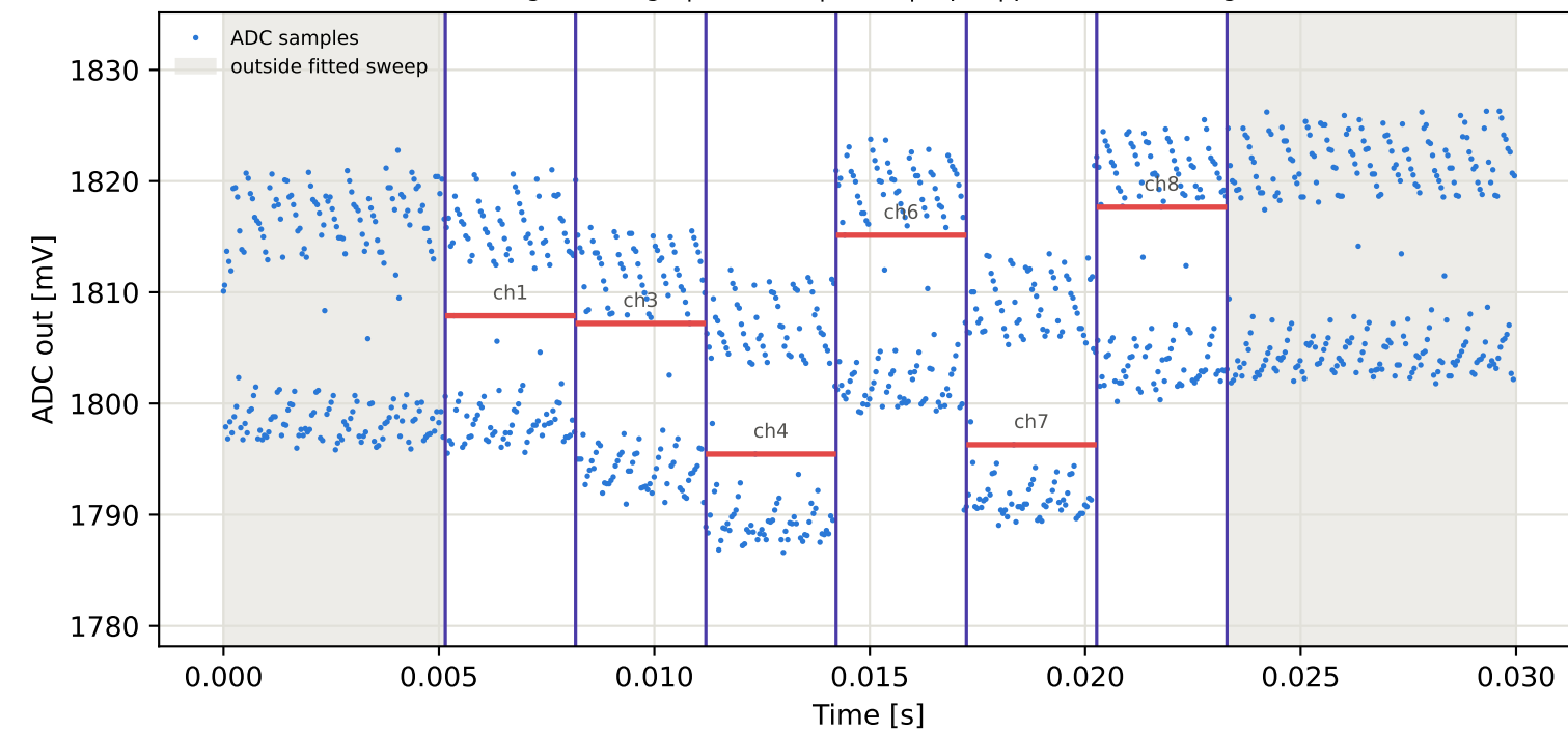
Tag15 &lt;- Tag9 | 925 MHz | run 0 | rep 1 | phase -140.36 deg
