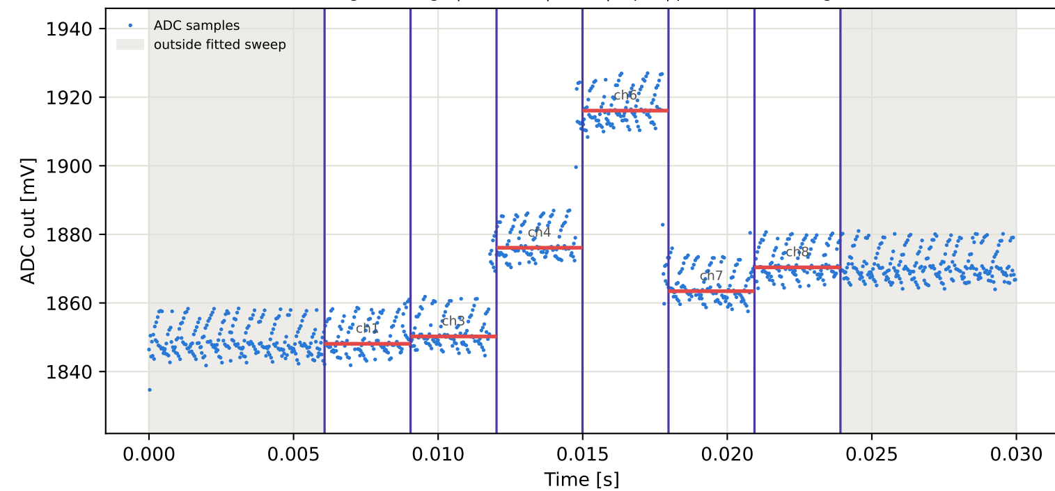
Tag16 &lt;- Tag1 | 935 MHz | run 0 | rep 1 | phase 151.56 deg
