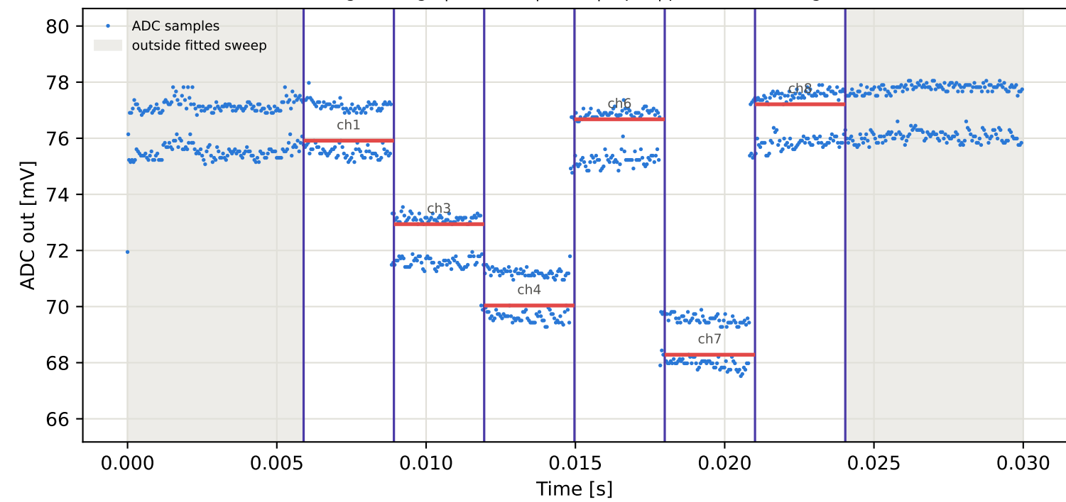
Tag7 &lt;- Tag1 | 785 MHz | run 0 | rep 1 | phase 0.28 deg
