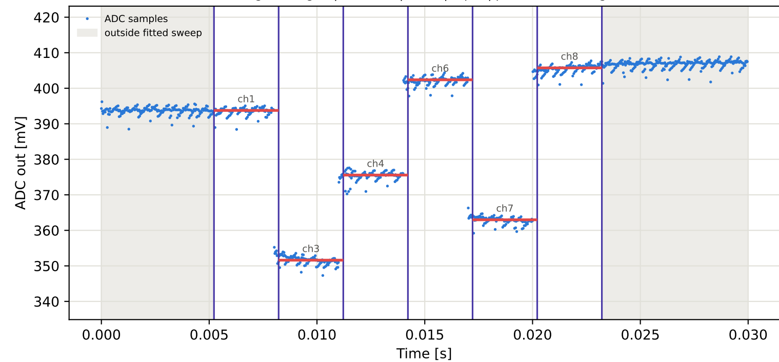
Tag5 &lt;- Tag2 | 845 MHz | run 0 | rep 1 | phase -21.81 deg
