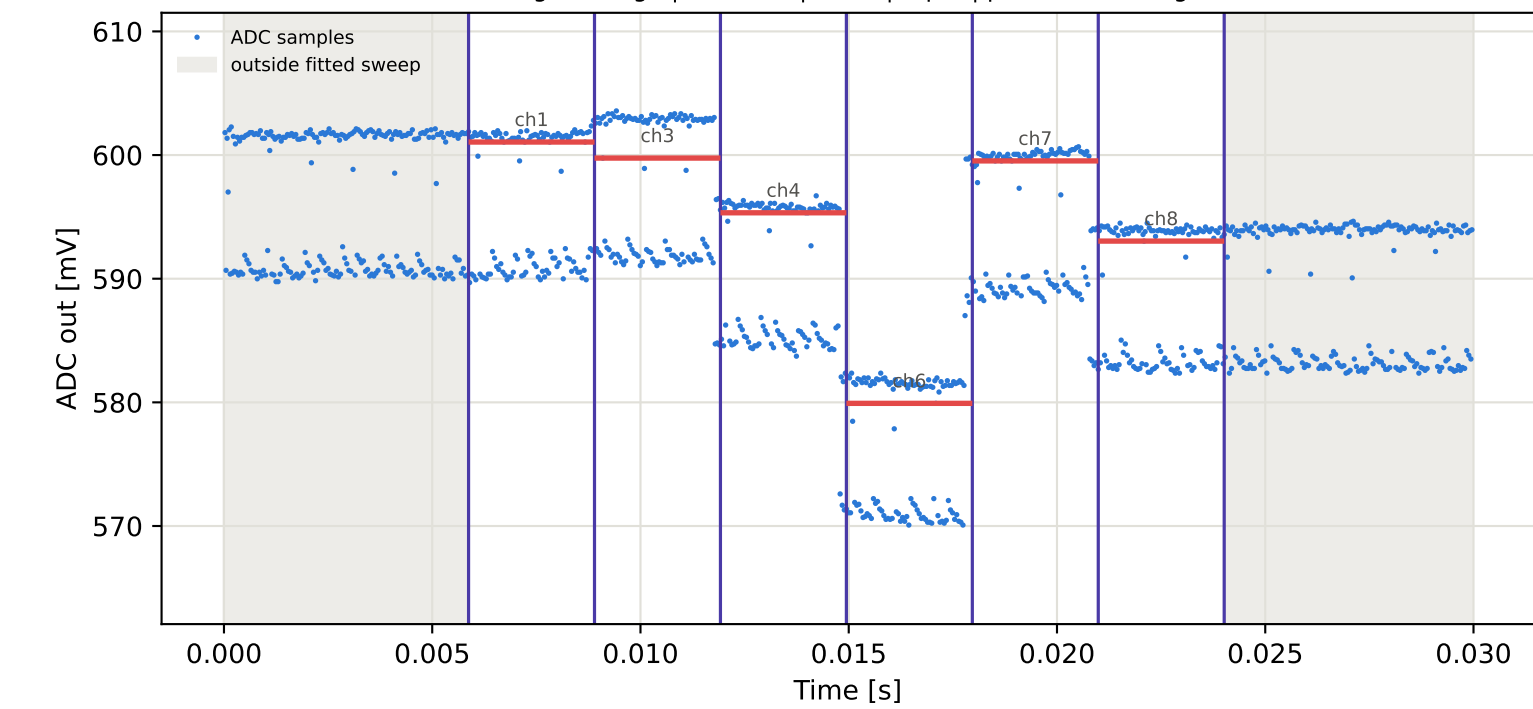
Tag8 &lt;- Tag6 | 945 MHz | run 0 | rep 1 | phase 14.66 deg
