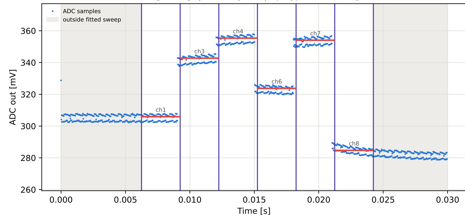
Tag9 &lt;- Tag5 | 875 MHz | run 0 | rep 1 | phase -151.02 deg
