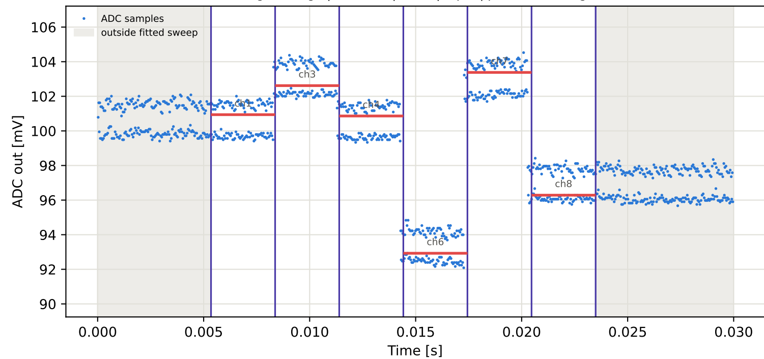
Tag7 &lt;- Tag1 | 995 MHz | run 0 | rep 1 | phase -104.19 deg
