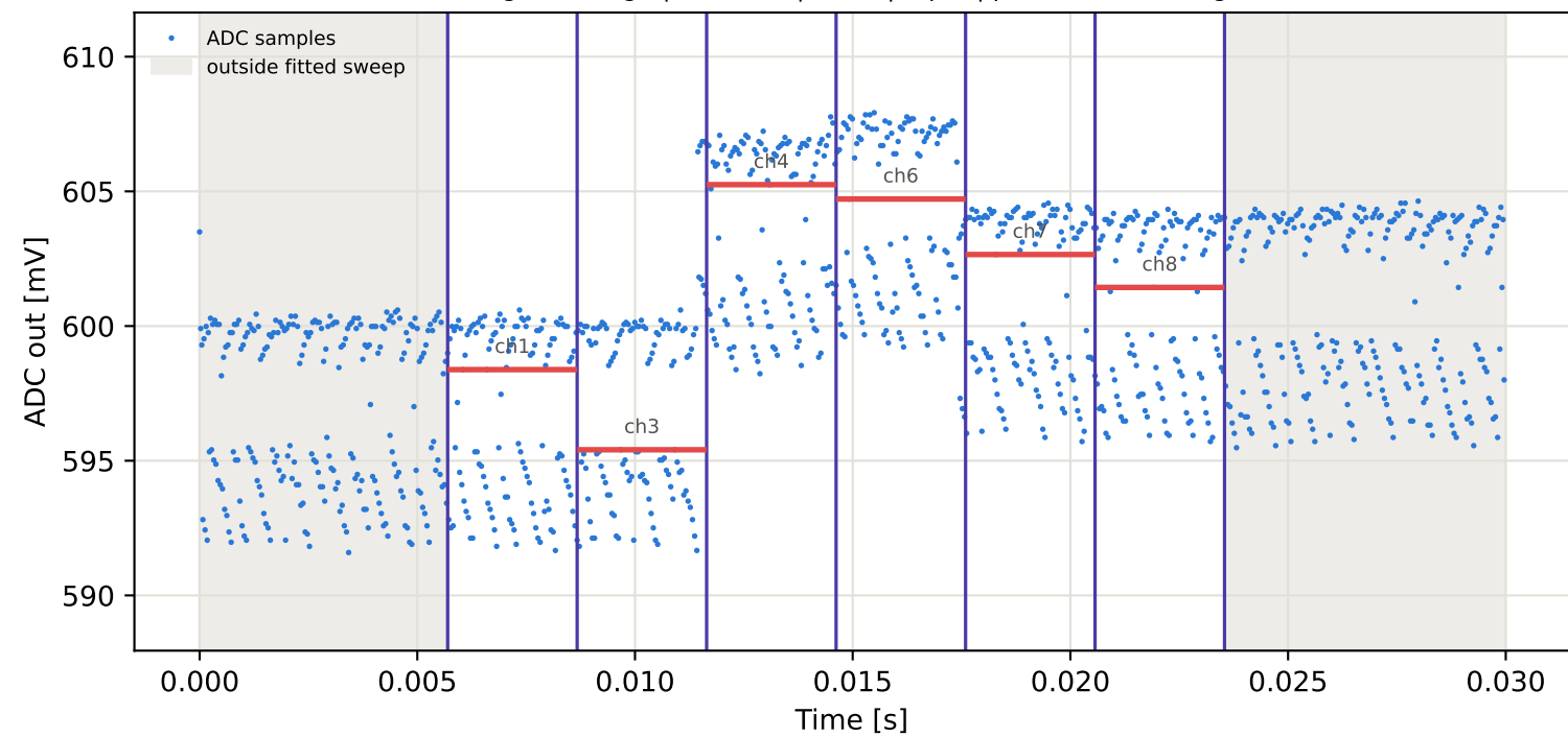
Tag15 &lt;- Tag9 | 835 MHz | run 0 | rep 1 | phase 67.66 deg
