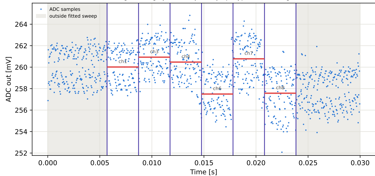
Tag10 &lt;- Tag4 | 885 MHz | run 0 | rep 1 | phase -15.00 deg
