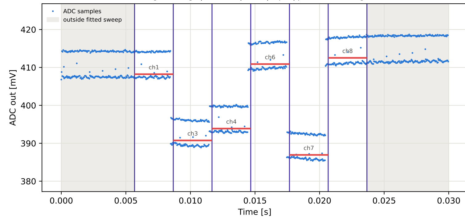
Tag2 &lt;- Tag1 | 805 MHz | run 0 | rep 1 | phase 168.73 deg
