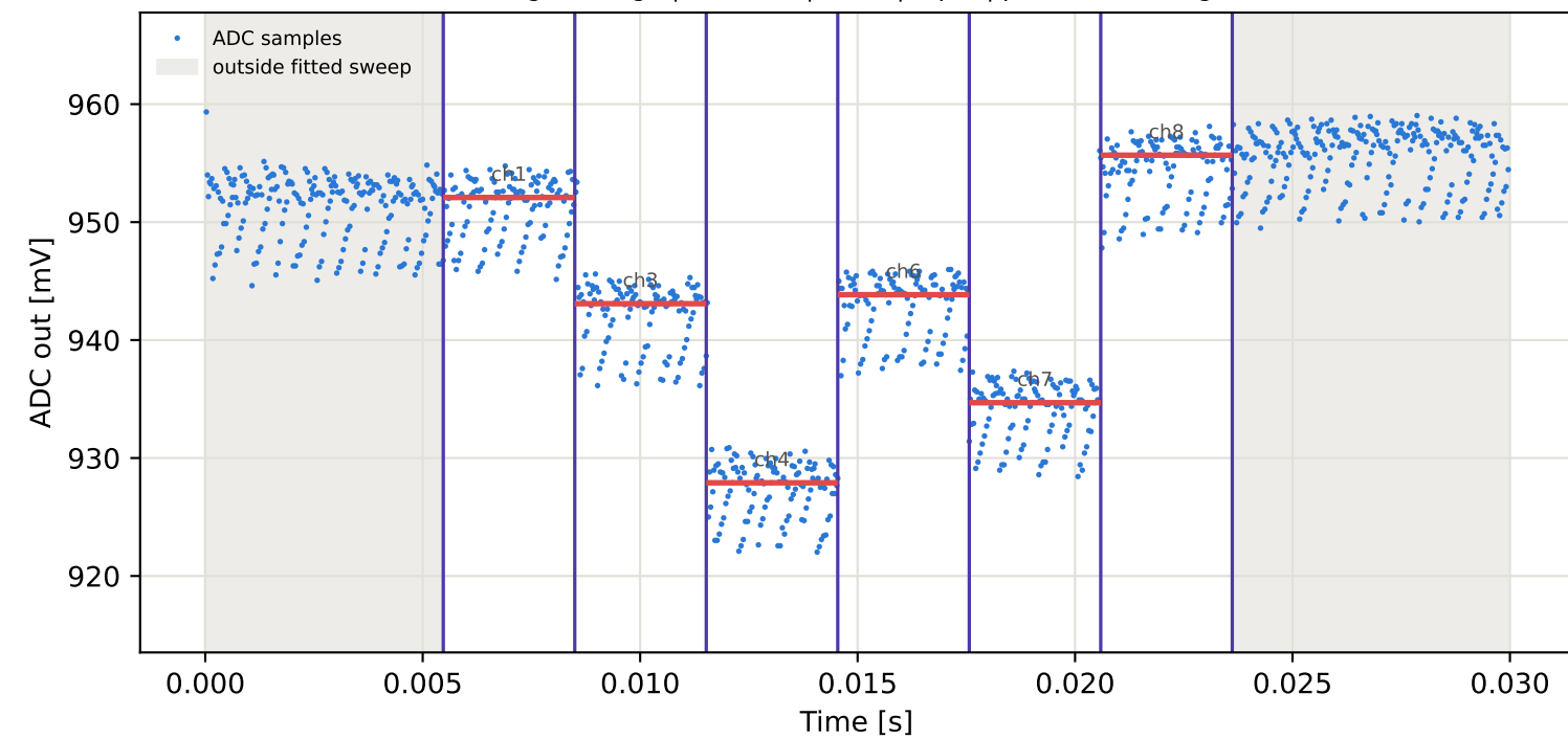
Tag4 &lt;- Tag8 | 935 MHz | run 0 | rep 1 | phase -51.87 deg
