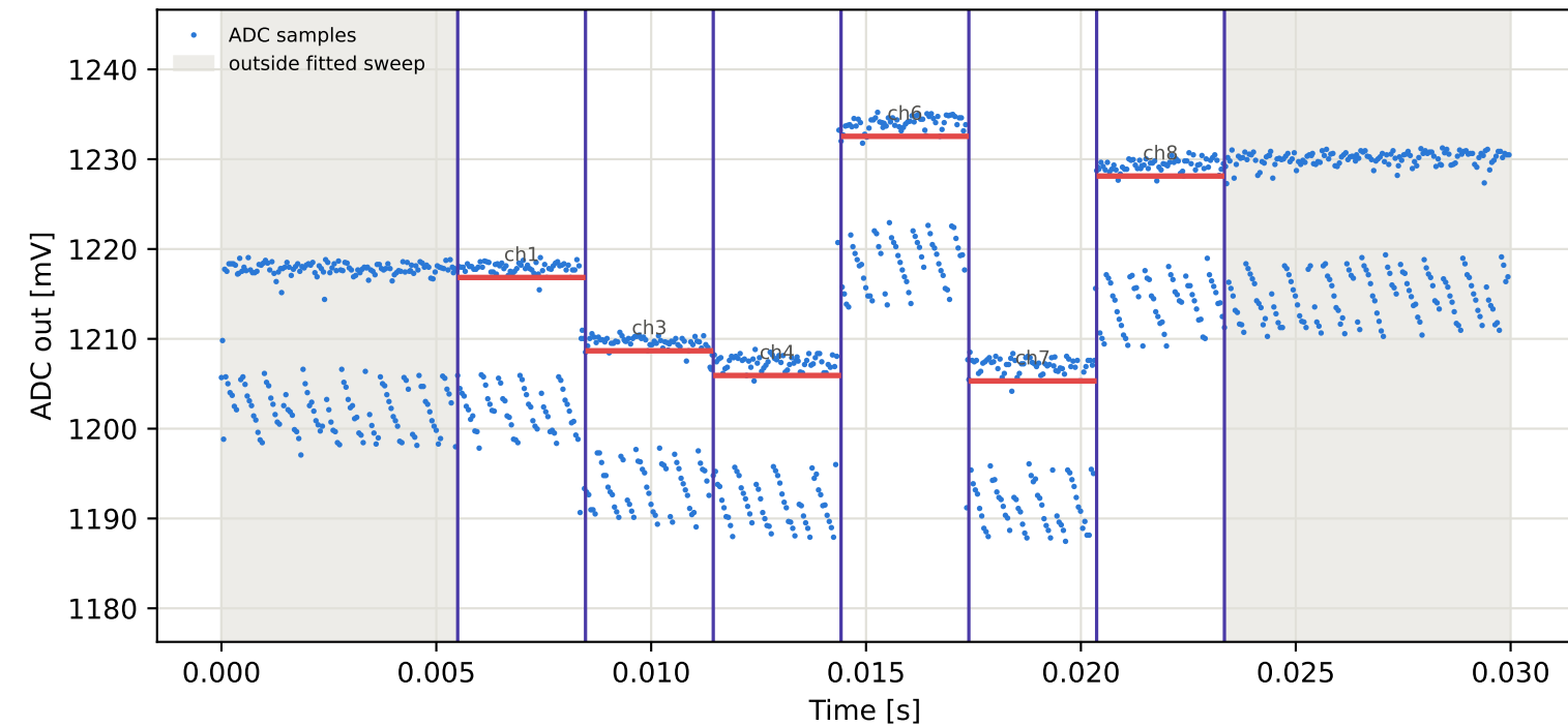
Tag16 &lt;- Tag15 | 935 MHz | run 0 | rep 1 | phase -144.07 deg
