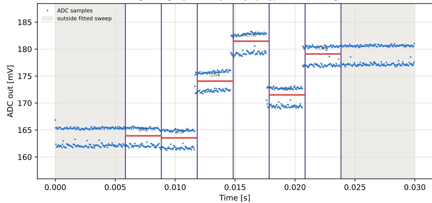
Tag9 &lt;- Tag2 | 865 MHz | run 0 | rep 1 | phase -71.56 deg
