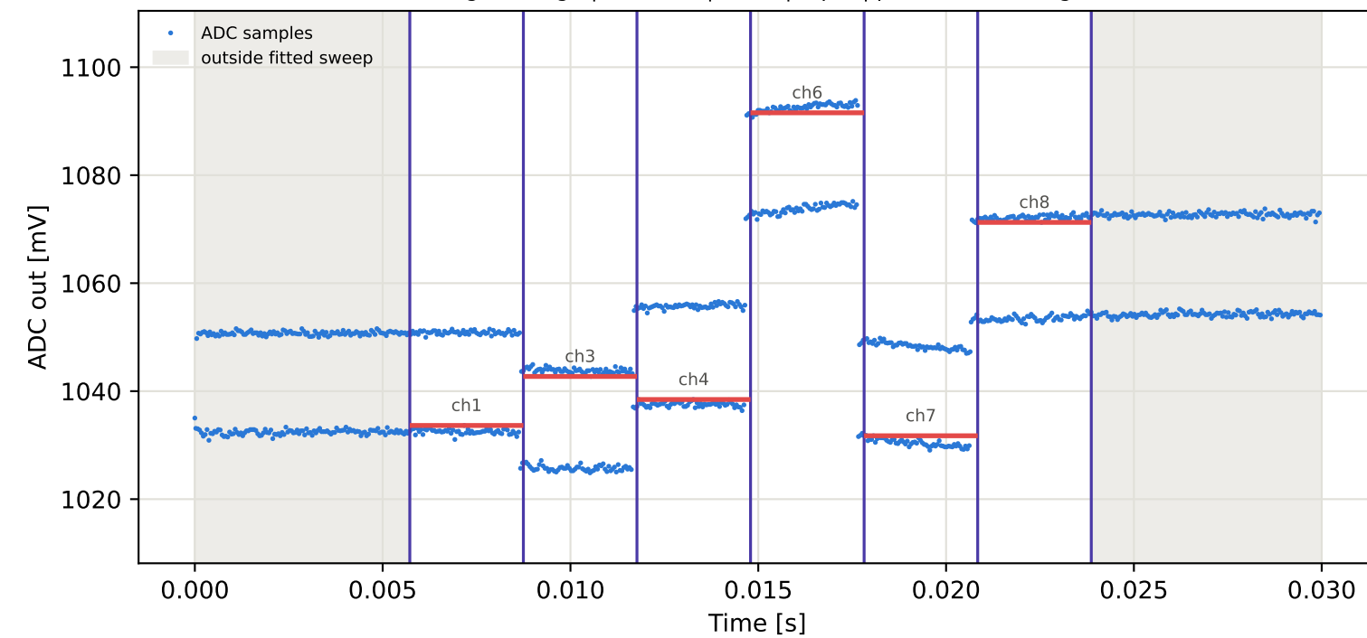
Tag4 &lt;- Tag15 | 945 MHz | run 0 | rep 1 | phase 91.73 deg
