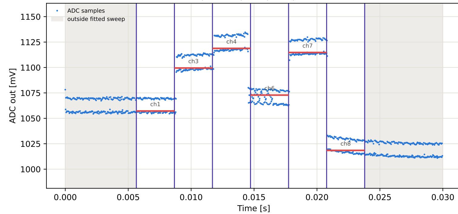
Tag15 &lt;- Tag5 | 885 MHz | run 0 | rep 1 | phase -69.73 deg
