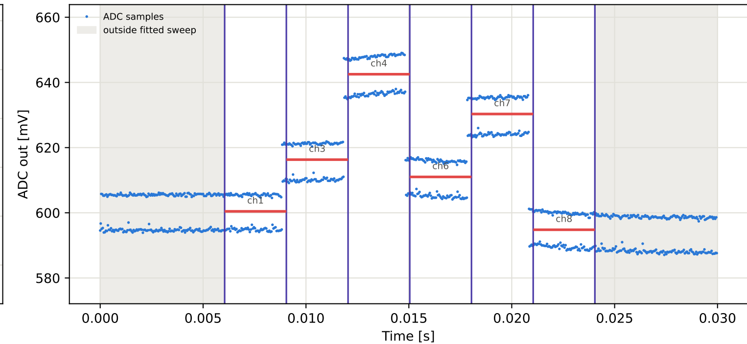
Tag9 &lt;- Tag8 | 945 MHz | run 0 | rep 1 | phase 17.01 deg
