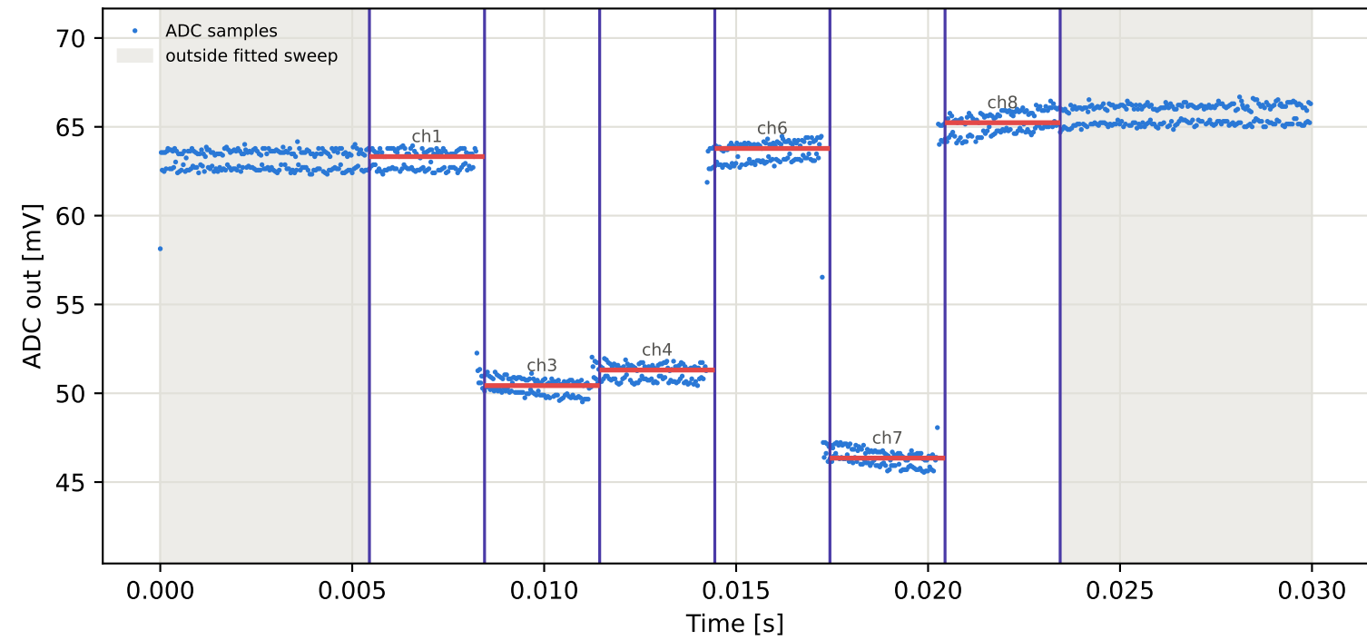
Tag9 &lt;- Tag2 | 825 MHz | run 0 | rep 1 | phase 8.58 deg
