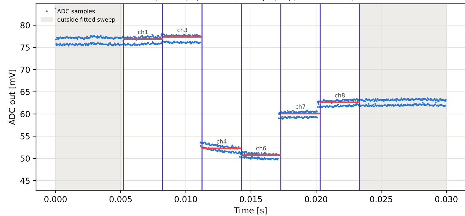
Tag9 &lt;- Tag8 | 825 MHz | run 0 | rep 1 | phase 63.71 deg
