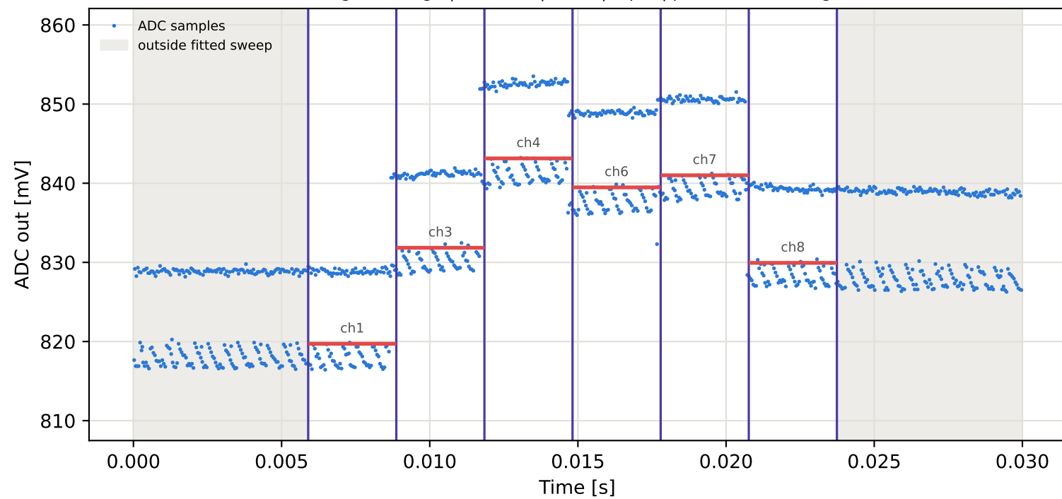
Tag2 &lt;- Tag10 | 865 MHz | run 0 | rep 1 | phase 63.42 deg
