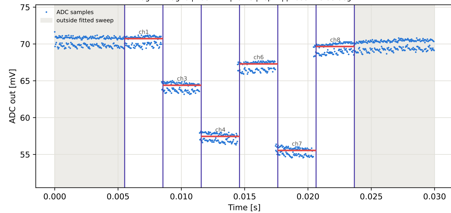
Tag7 &lt;- Tag3 | 795 MHz | run 0 | rep 1 | phase 56.74 deg
