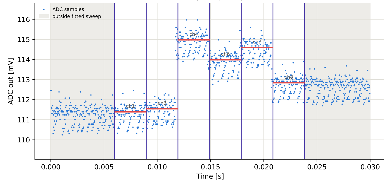
Tag5 &lt;- Tag16 | 805 MHz | run 0 | rep 1 | phase -115.70 deg
