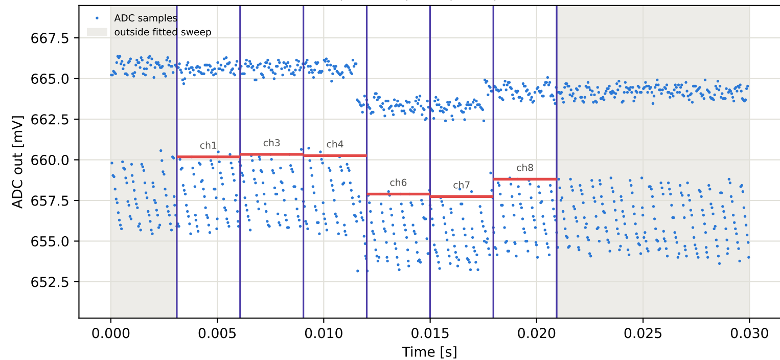
Tag8 &lt;- Tag7 | 845 MHz | run 0 | rep 1 | phase 29.69 deg
