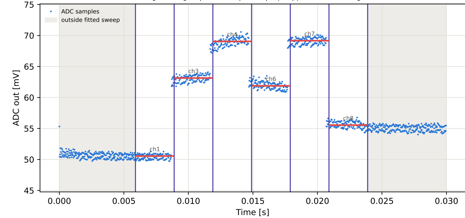
Tag2 &lt;- Tag16 | 845 MHz | run 0 | rep 1 | phase -85.90 deg
