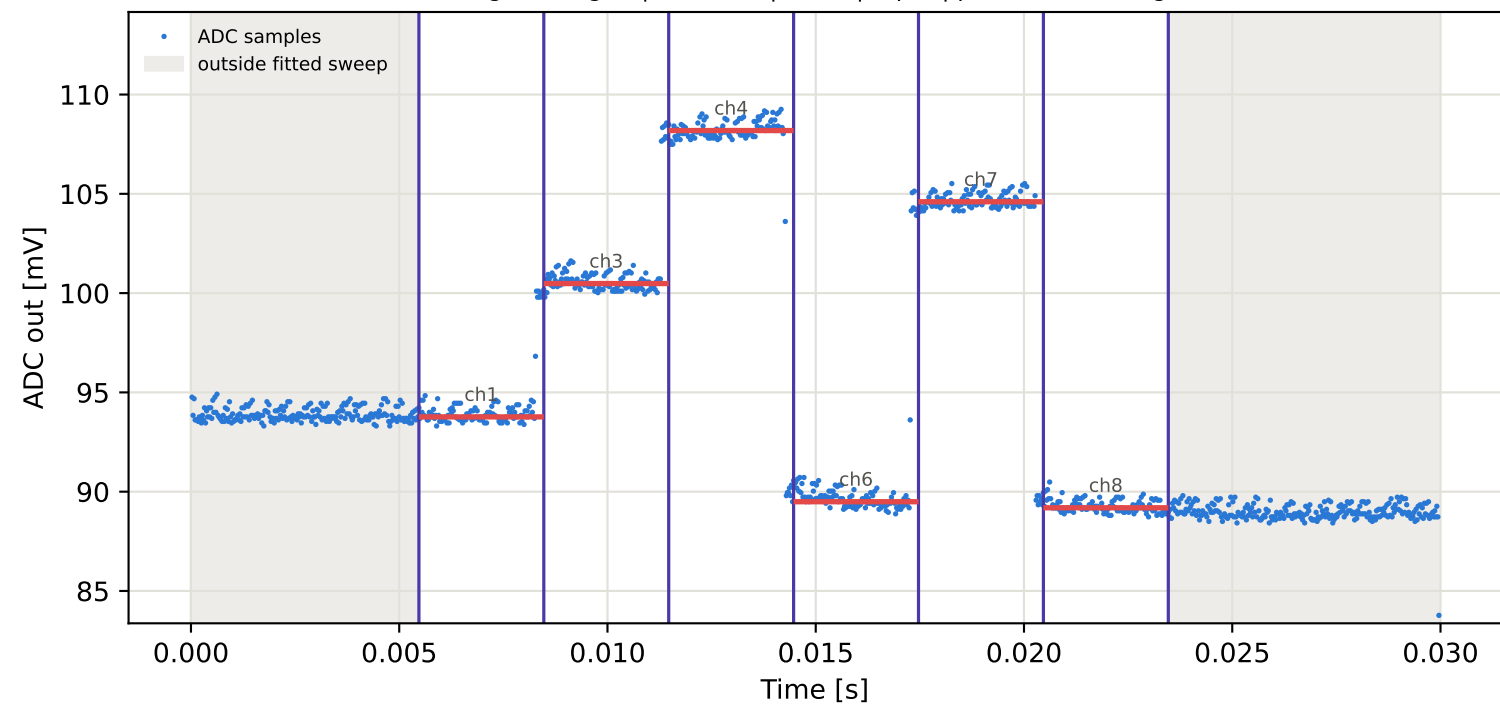
Tag6 &lt;- Tag2 | 995 MHz | run 0 | rep 1 | phase 84.35 deg
