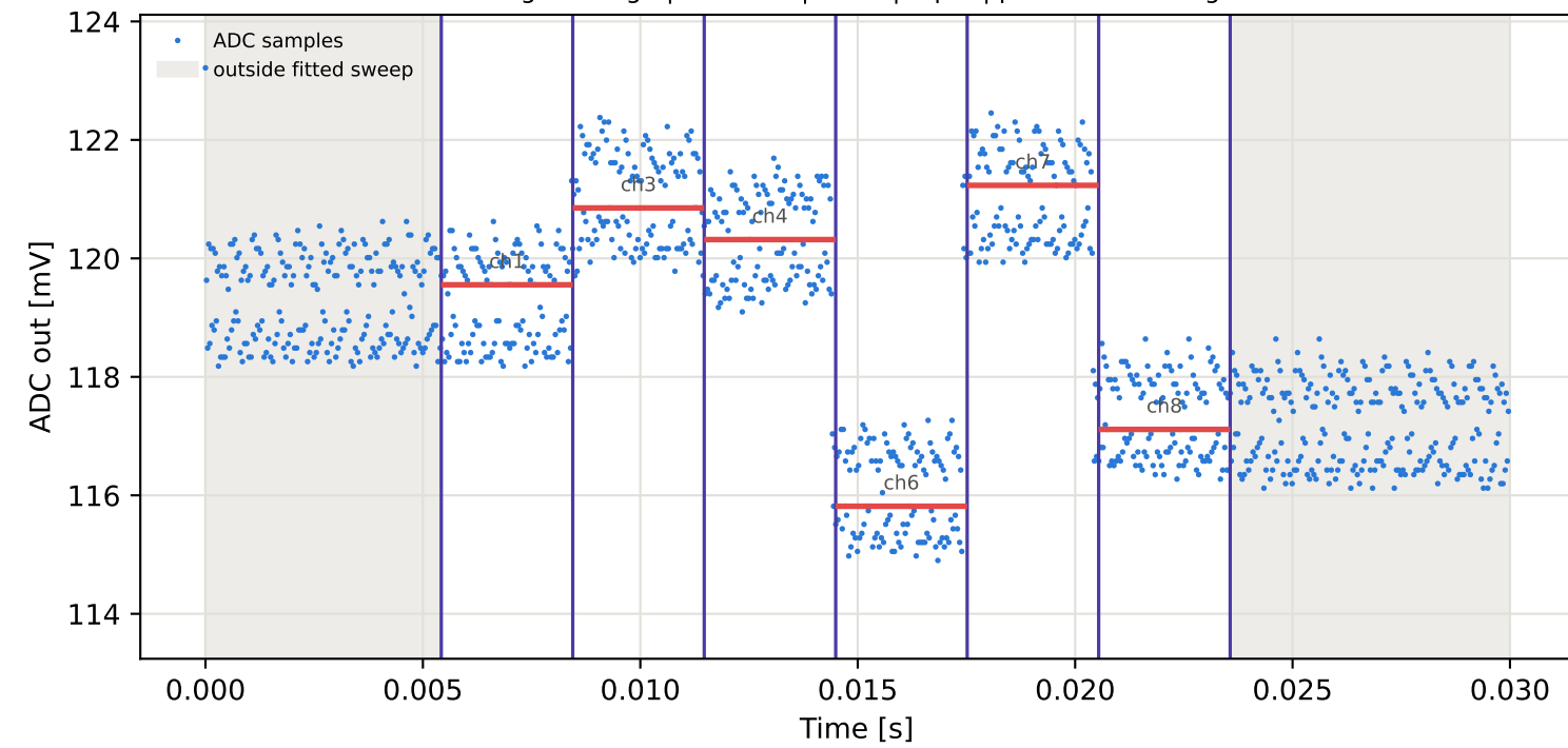
Tag5 &lt;- Tag9 | 995 MHz | run 0 | rep 1 | phase 14.11 deg
