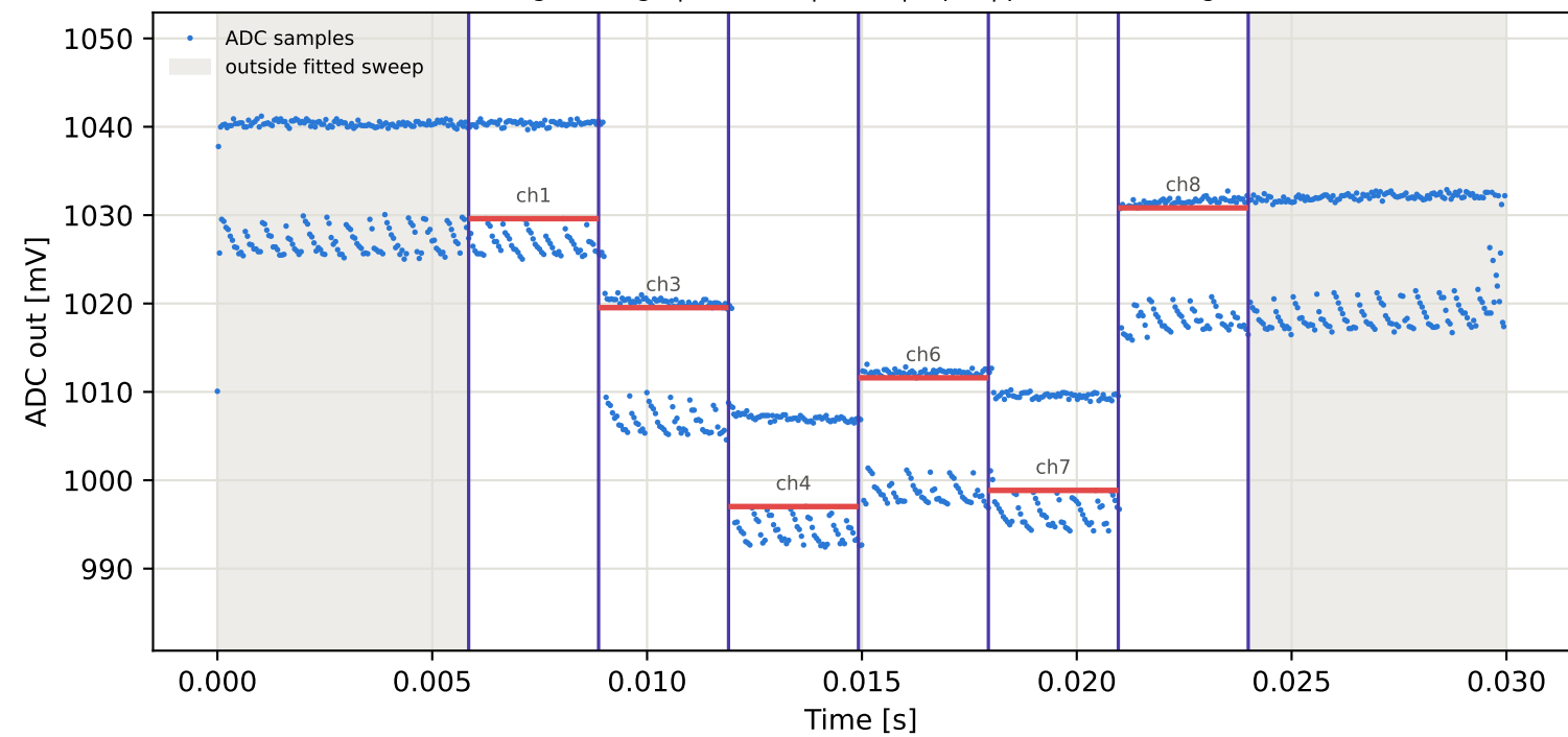
Tag8 &lt;- Tag5 | 865 MHz | run 0 | rep 1 | phase 77.11 deg
