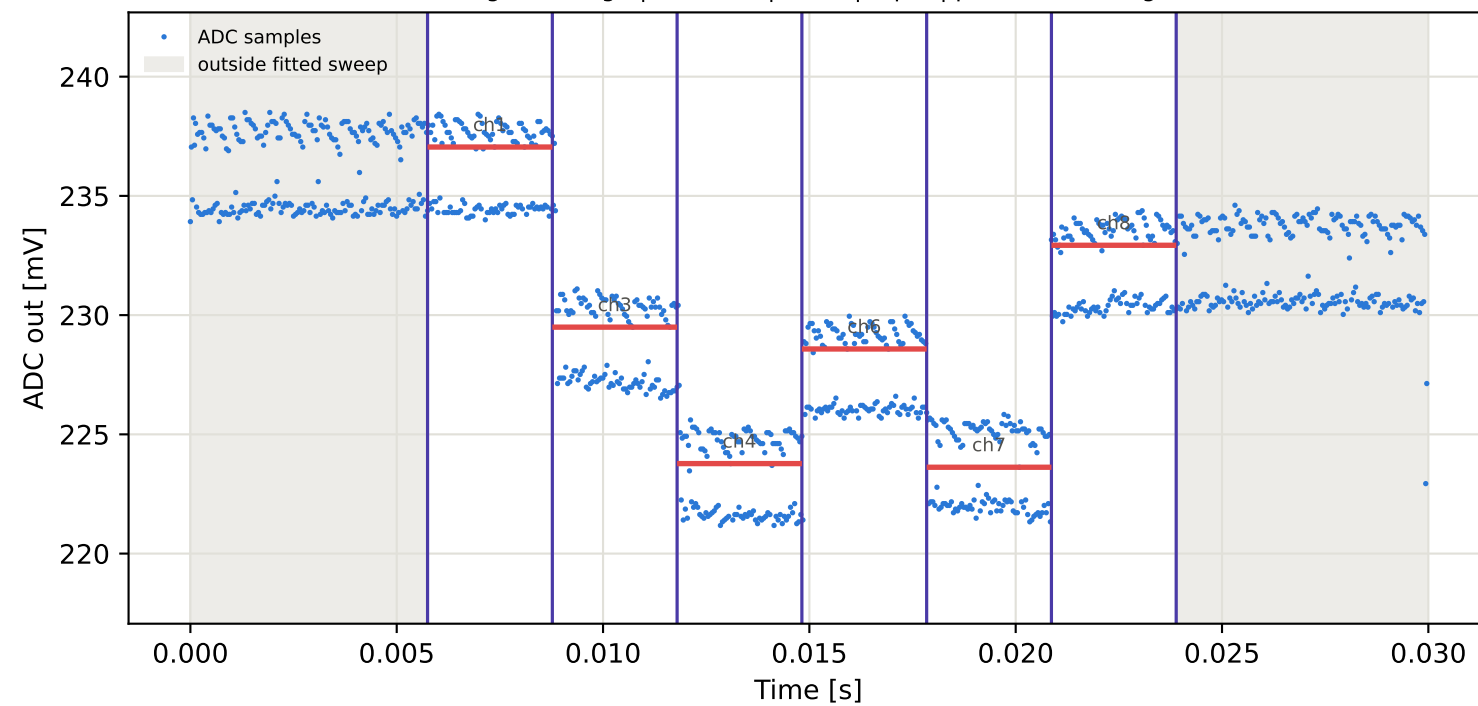
Tag15 &lt;- Tag1 | 835 MHz | run 0 | rep 1 | phase -177.26 deg
