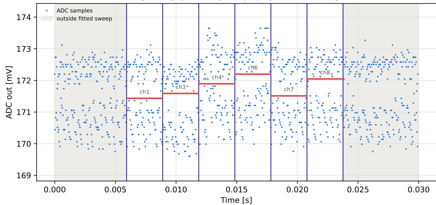
Tag4 &lt;- Tag15 | 825 MHz | run 0 | rep 1 | phase -27.89 deg
