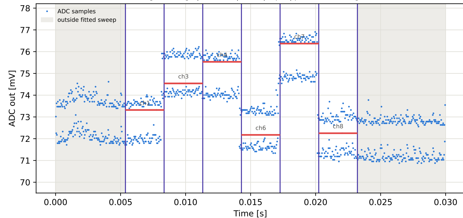
Tag10 &lt;- Tag9 | 795 MHz | run 0 | rep 1 | phase 131.52 deg
