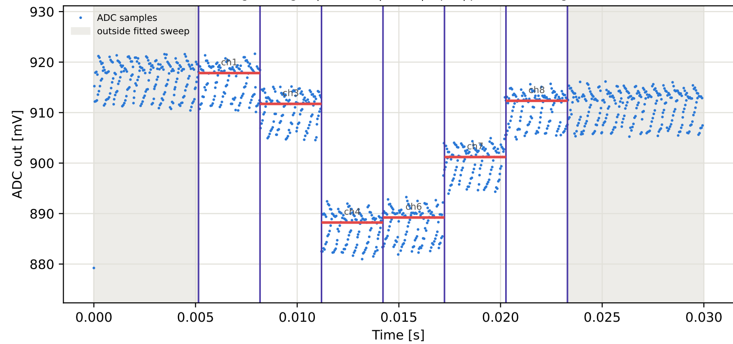
Tag4 &lt;- Tag16 | 955 MHz | run 0 | rep 1 | phase 90.62 deg
