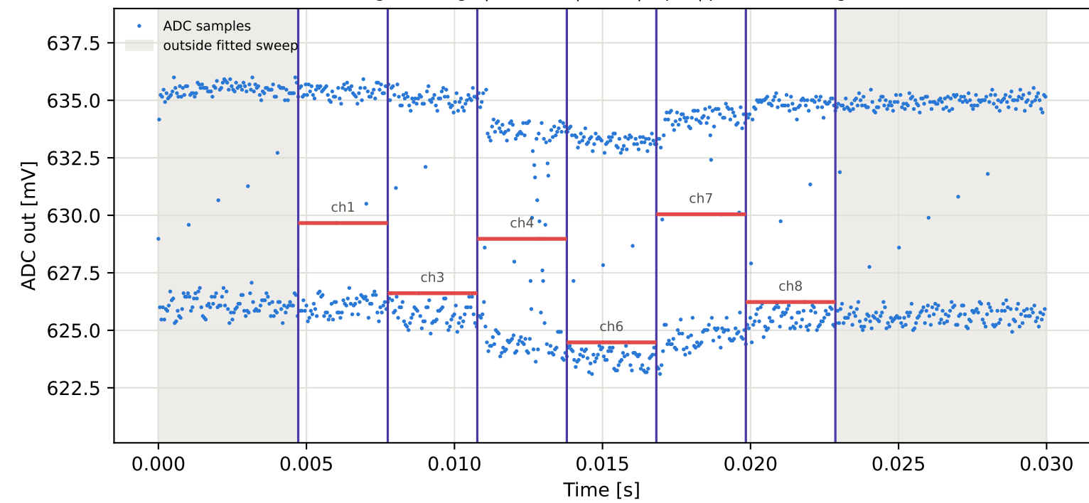
Tag15 &lt;- Tag4 | 855 MHz | run 0 | rep 1 | phase -130.49 deg
