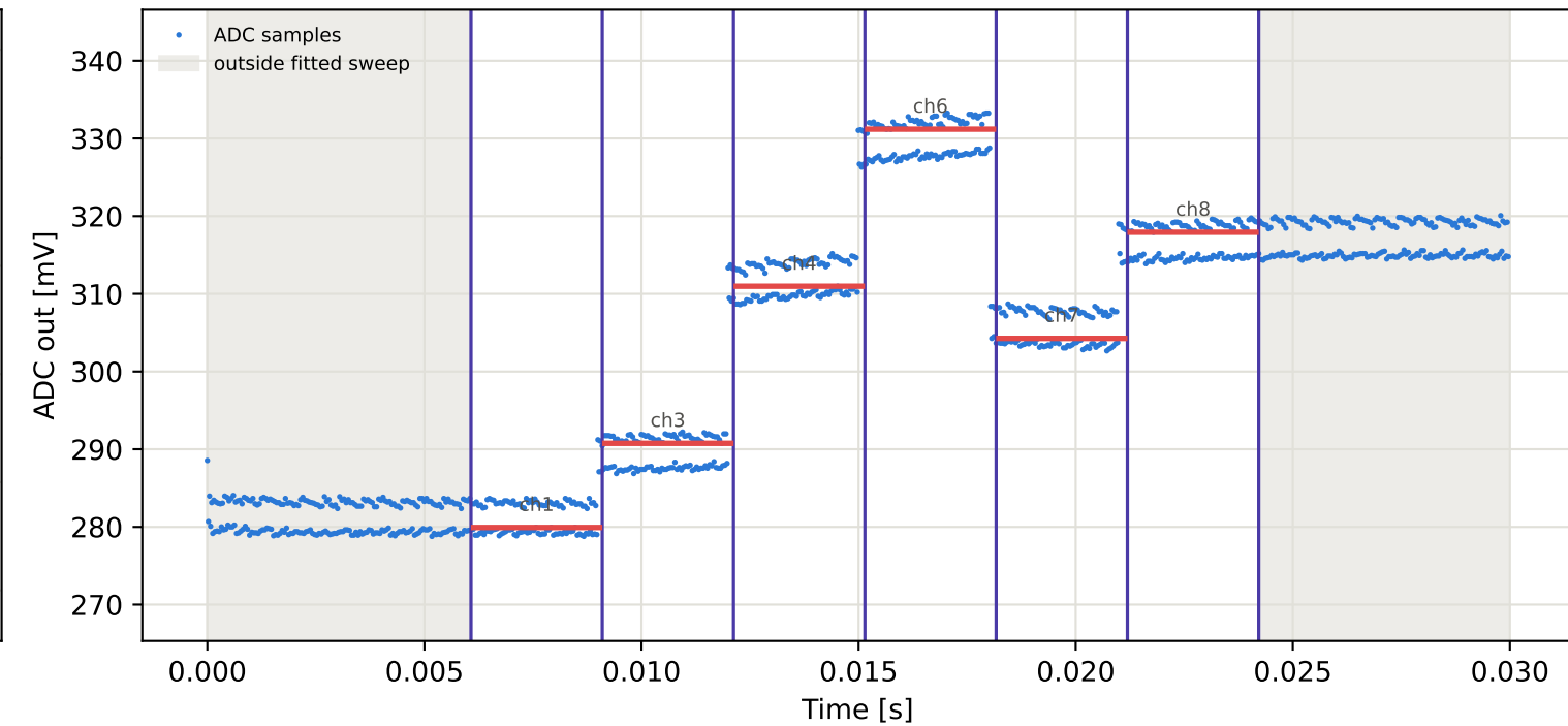
Tag10 &lt;- Tag5 | 865 MHz | run 0 | rep 1 | phase -123.21 deg
