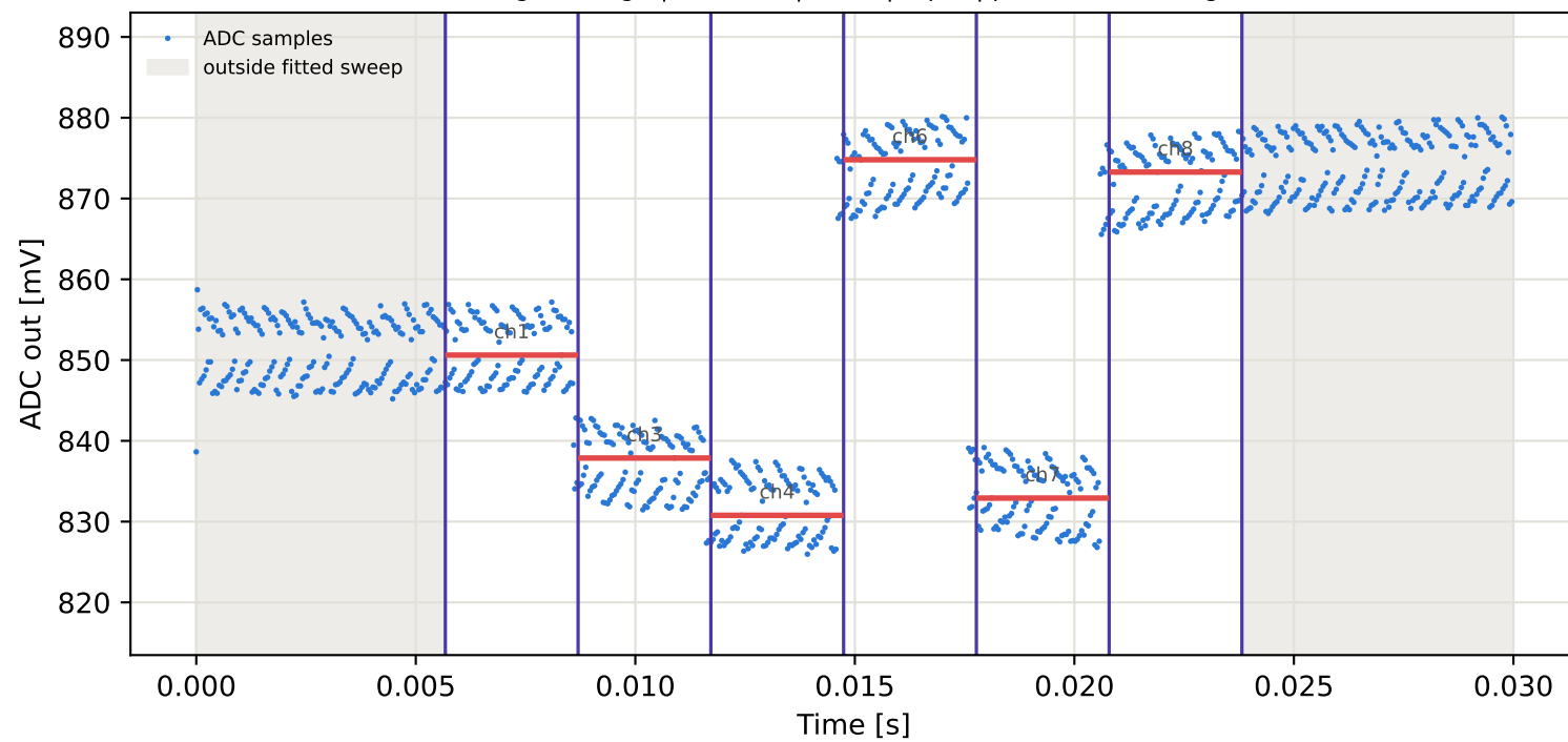
Tag4 &lt;- Tag15 | 915 MHz | run 0 | rep 1 | phase 32.23 deg
