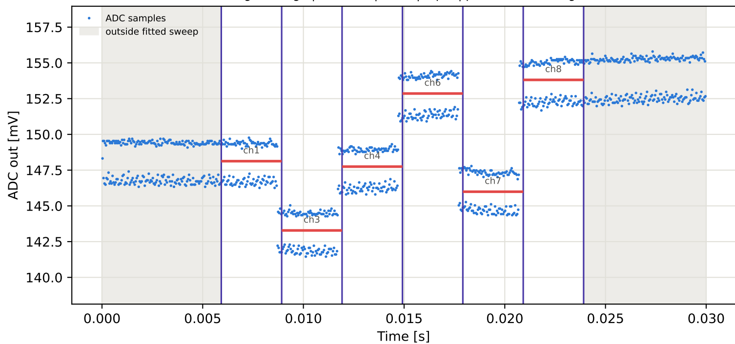
Tag1 &lt;- Tag4 | 845 MHz | run 0 | rep 1 | phase -176.12 deg
