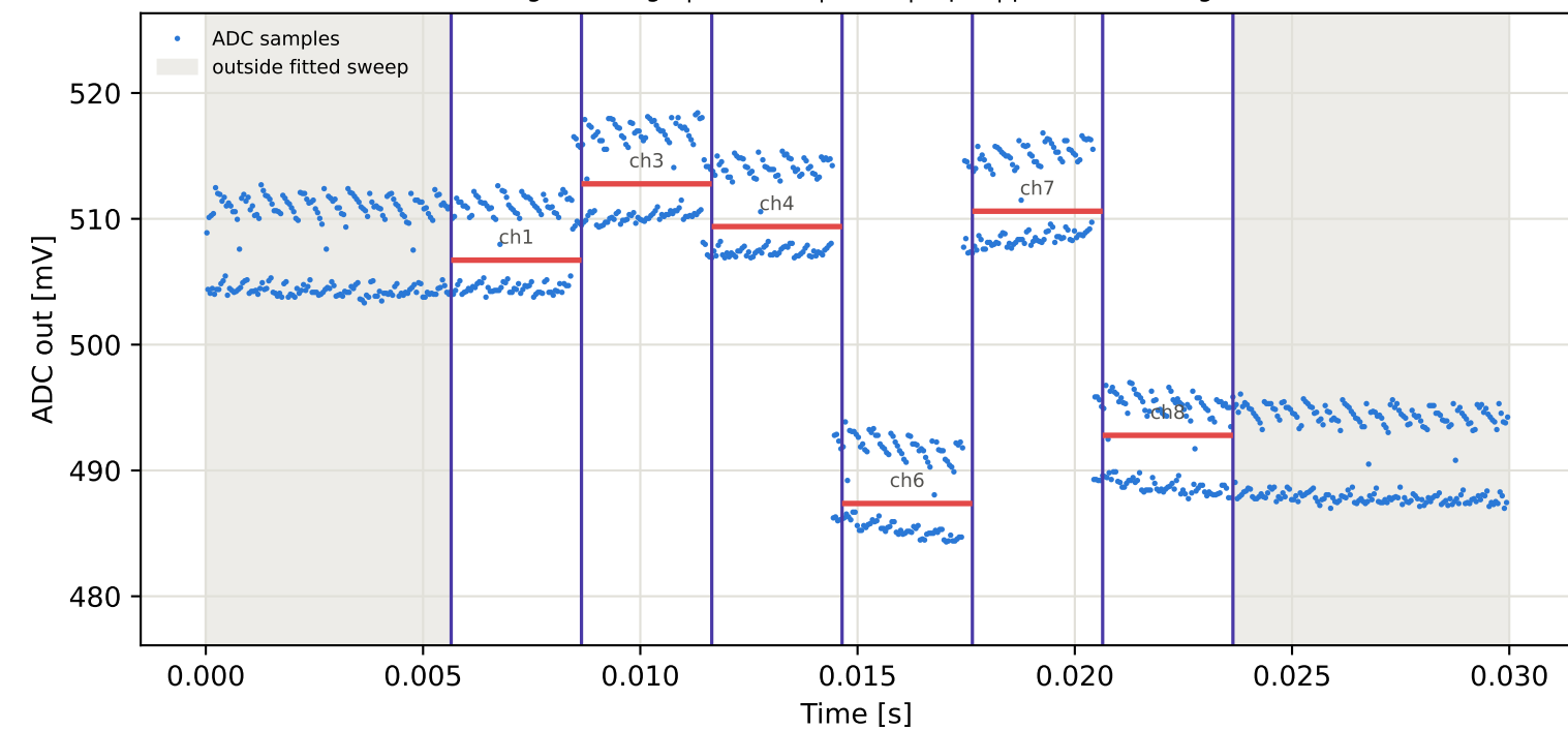
Tag10 &lt;- Tag4 | 895 MHz | run 0 | rep 1 | phase -3.45 deg
