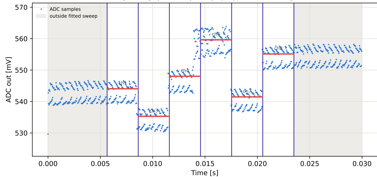
Tag6 &lt;- Tag9 | 835 MHz | run 0 | rep 1 | phase -133.51 deg
