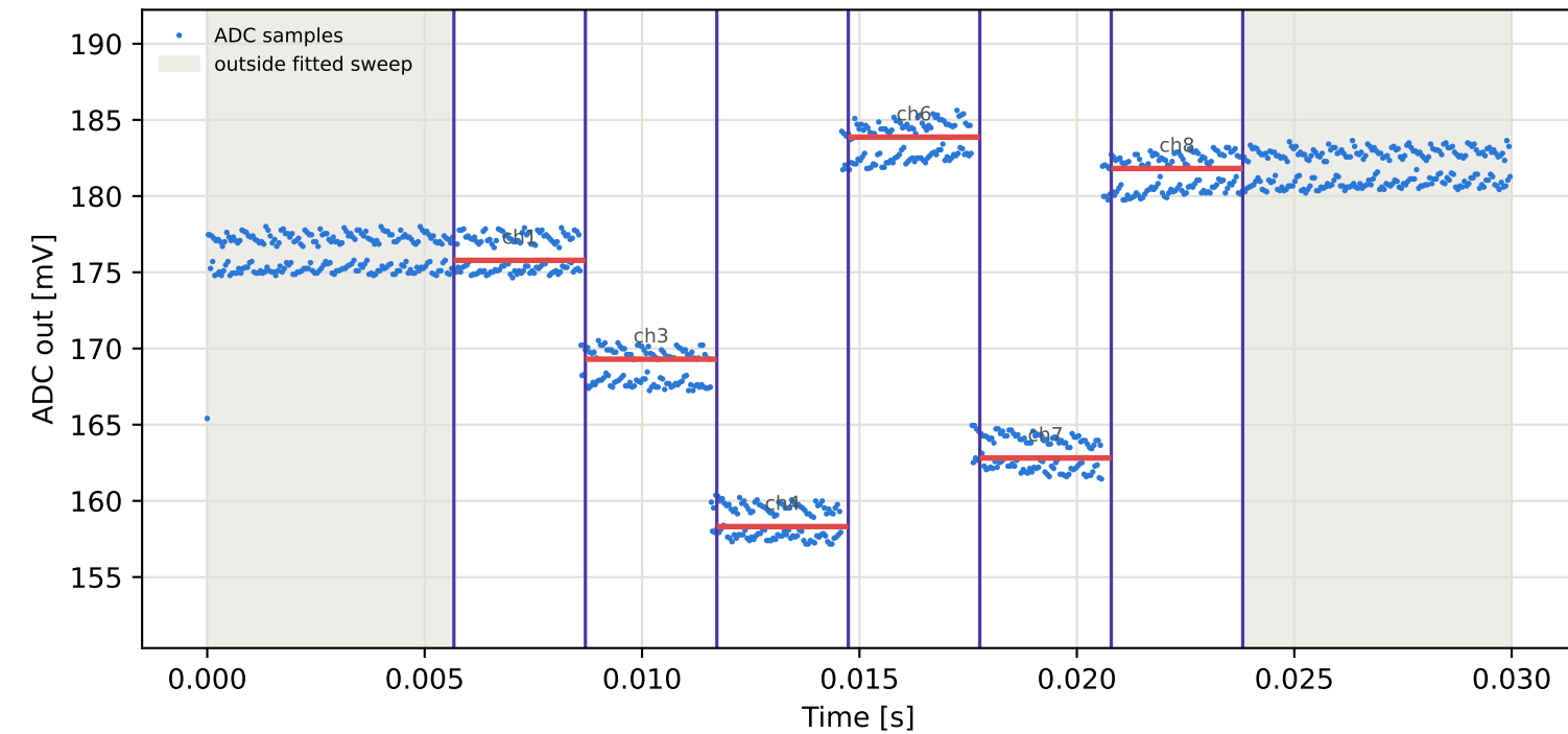
Tag7 &lt;- Tag5 | 995 MHz | run 0 | rep 1 | phase -96.00 deg
