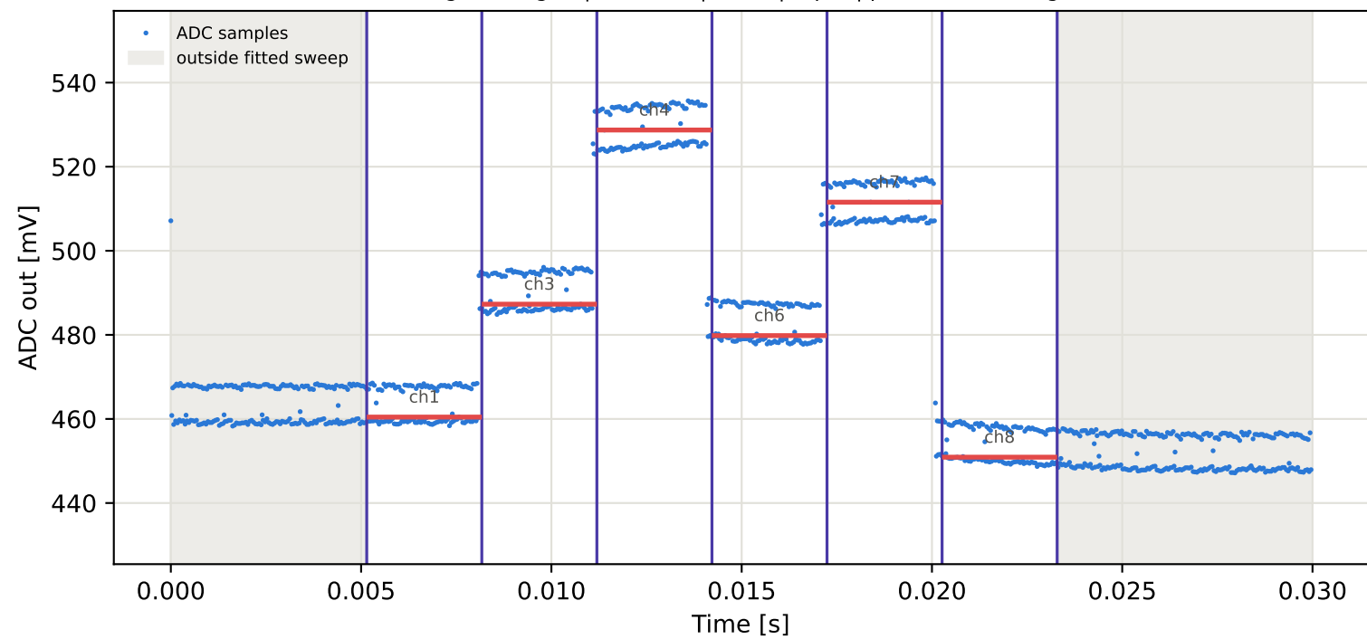
Tag5 &lt;- Tag2 | 955 MHz | run 0 | rep 1 | phase -37.90 deg
