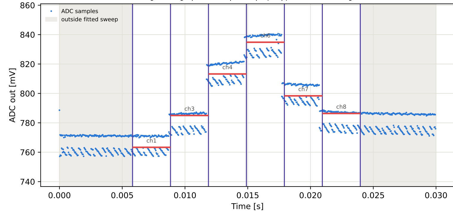
Tag5 &lt;- Tag3 | 925 MHz | run 0 | rep 1 | phase -137.55 deg
