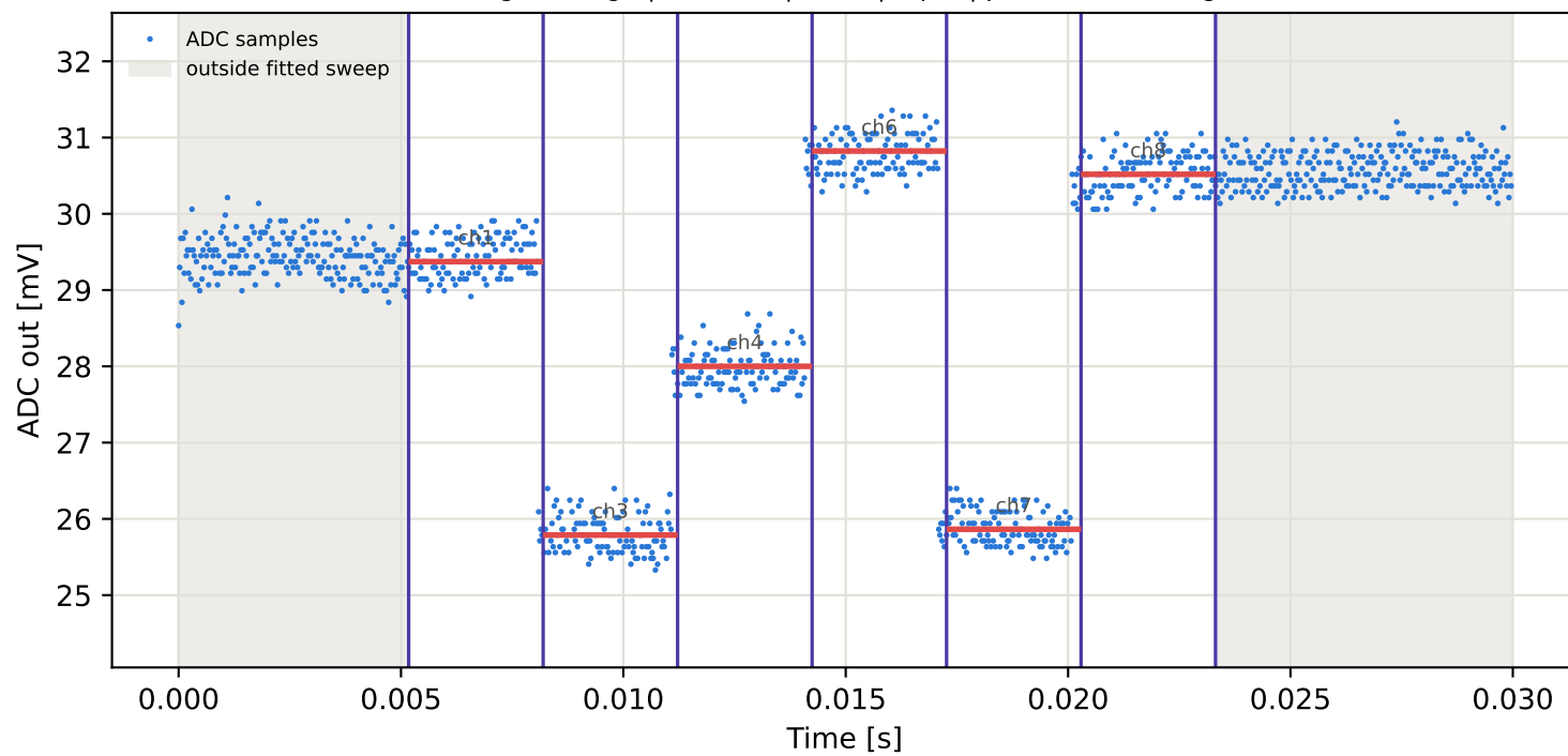
Tag2 &lt;- Tag5 | 795 MHz | run 0 | rep 1 | phase 43.90 deg
