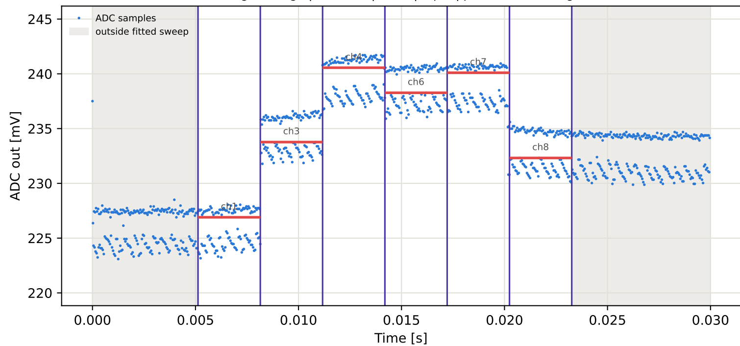
Tag7 &lt;- Tag15 | 865 MHz | run 0 | rep 1 | phase -39.10 deg
