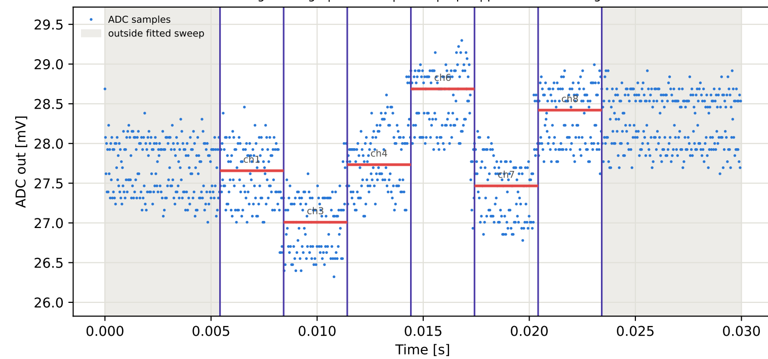
Tag3 &lt;- Tag10 | 825 MHz | run 0 | rep 1 | phase -63.80 deg
