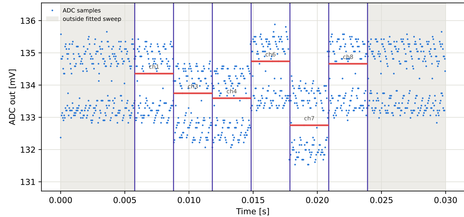
Tag16 &lt;- Tag15 | 775 MHz | run 0 | rep 1 | phase 12.07 deg
