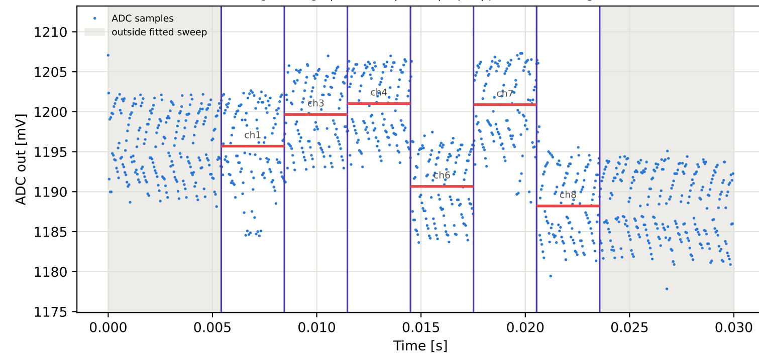
Tag8 &lt;- Tag4 | 895 MHz | run 0 | rep 1 | phase -80.14 deg
