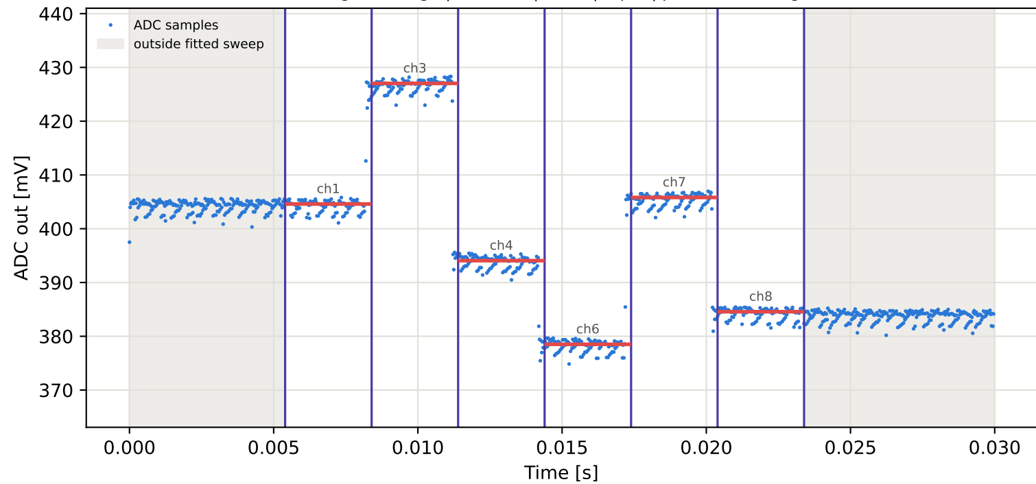
Tag16 &lt;- Tag1 | 825 MHz | run 0 | rep 1 | phase 133.32 deg
