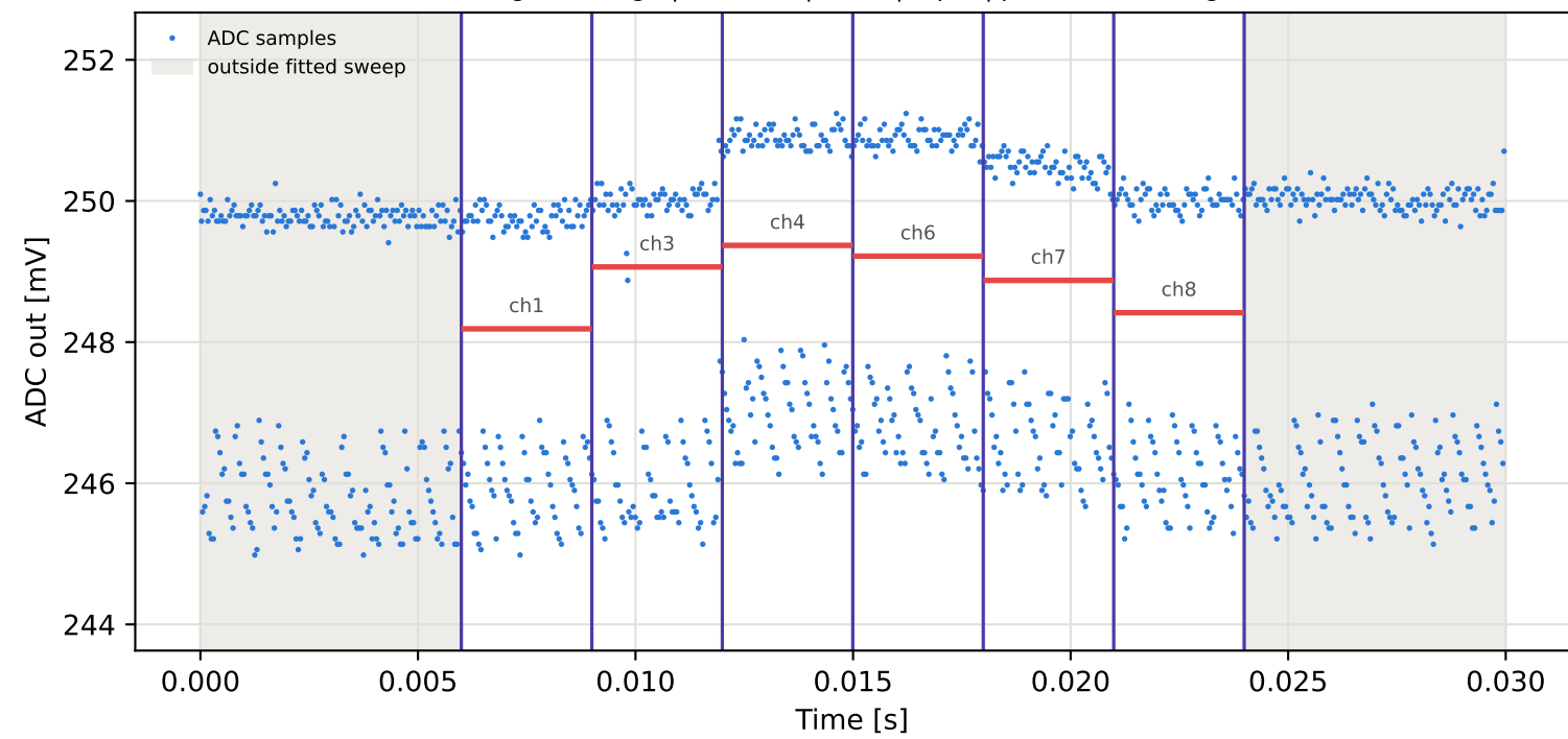
Tag15 &lt;- Tag4 | 785 MHz | run 0 | rep 1 | phase 129.94 deg
