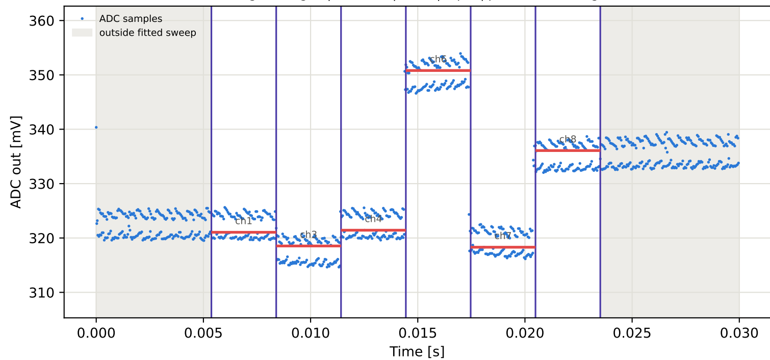
Tag6 &lt;- Tag3 | 935 MHz | run 0 | rep 1 | phase 156.23 deg
