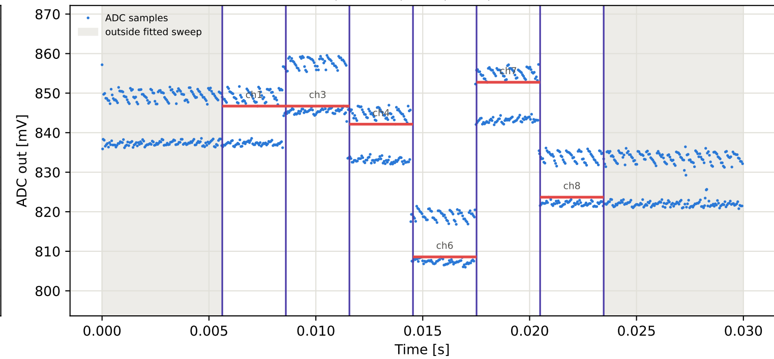
Tag8 &lt;- Tag7 | 975 MHz | run 0 | rep 1 | phase -2.02 deg
