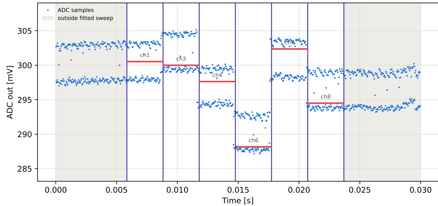
Tag4 &lt;- Tag7 | 995 MHz | run 0 | rep 1 | phase -110.46 deg
