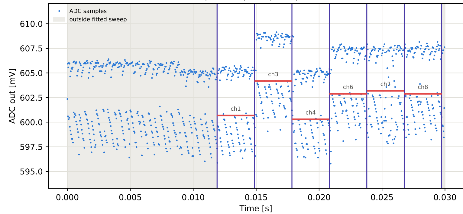
Tag15 &lt;- Tag4 | 835 MHz | run 0 | rep 1 | phase -98.02 deg
