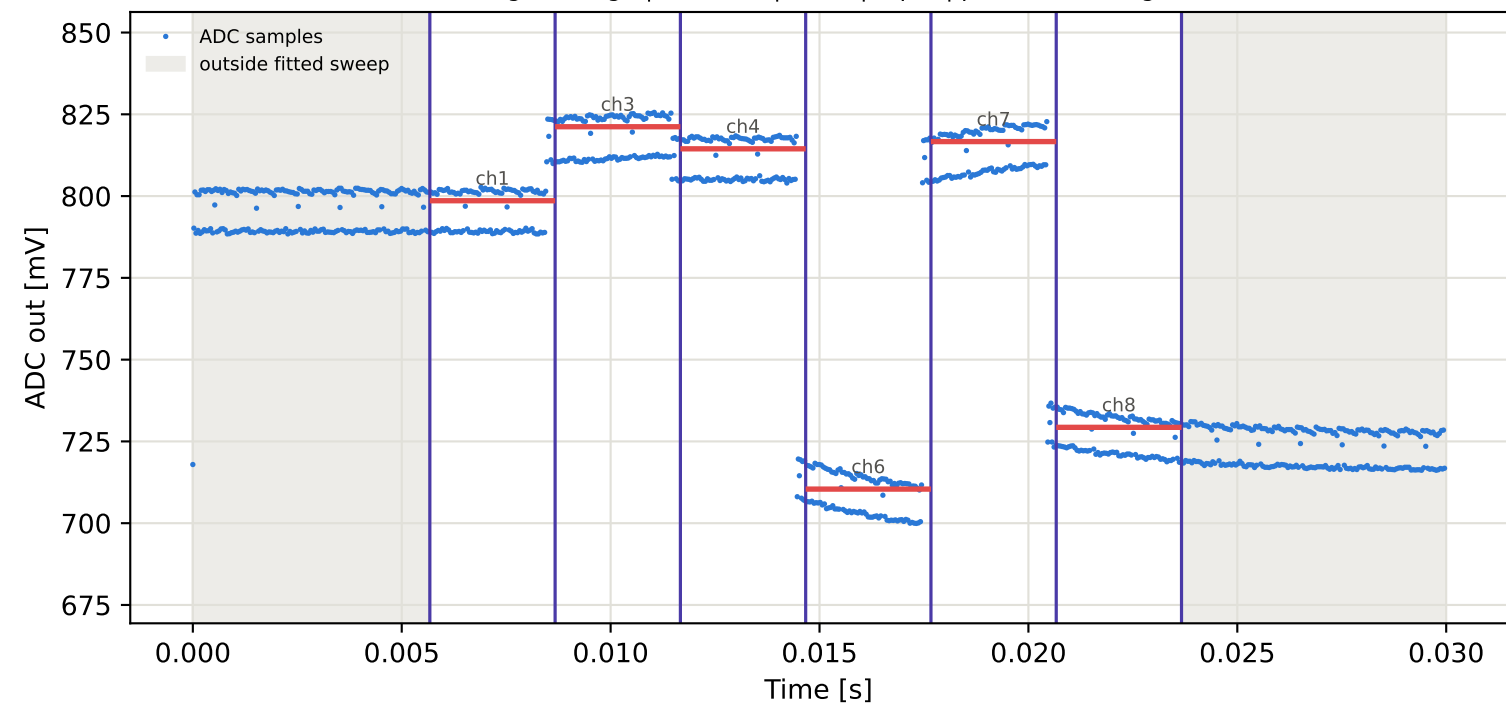
Tag4 &lt;- Tag8 | 905 MHz | run 0 | rep 1 | phase -69.71 deg
