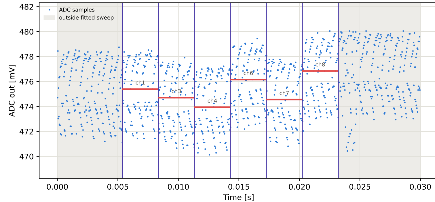
Tag10 &lt;- Tag4 | 925 MHz | run 0 | rep 1 | phase -9.61 deg
