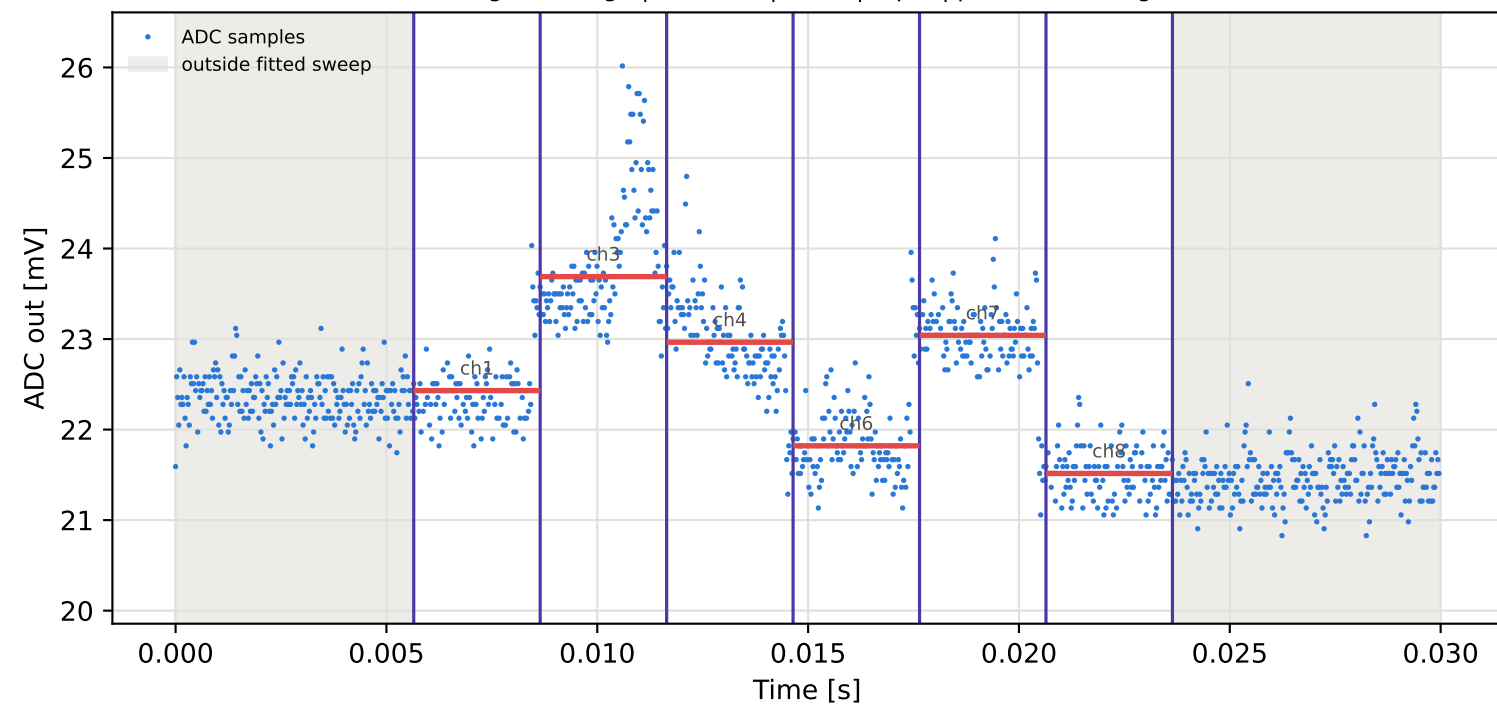
Tag10 &lt;- Tag5 | 845 MHz | run 0 | rep 1 | phase 71.59 deg
