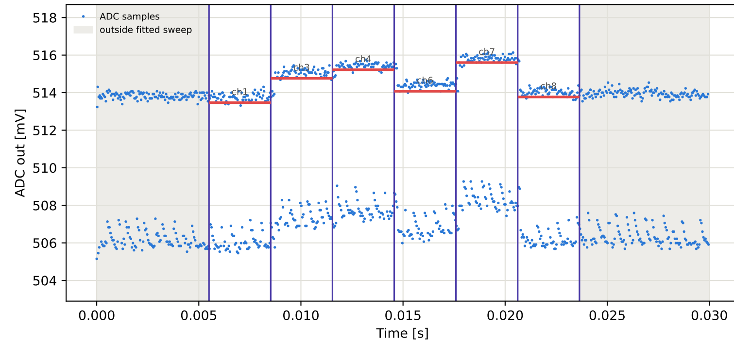
Tag8 &lt;- Tag15 | 825 MHz | run 0 | rep 1 | phase 91.99 deg
