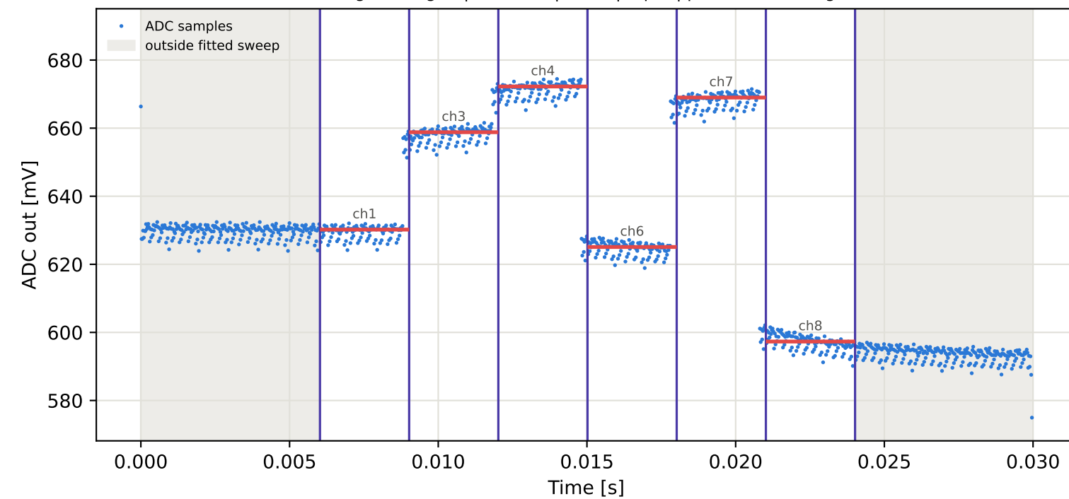
Tag3 &lt;- Tag16 | 905 MHz | run 0 | rep 1 | phase 45.57 deg
