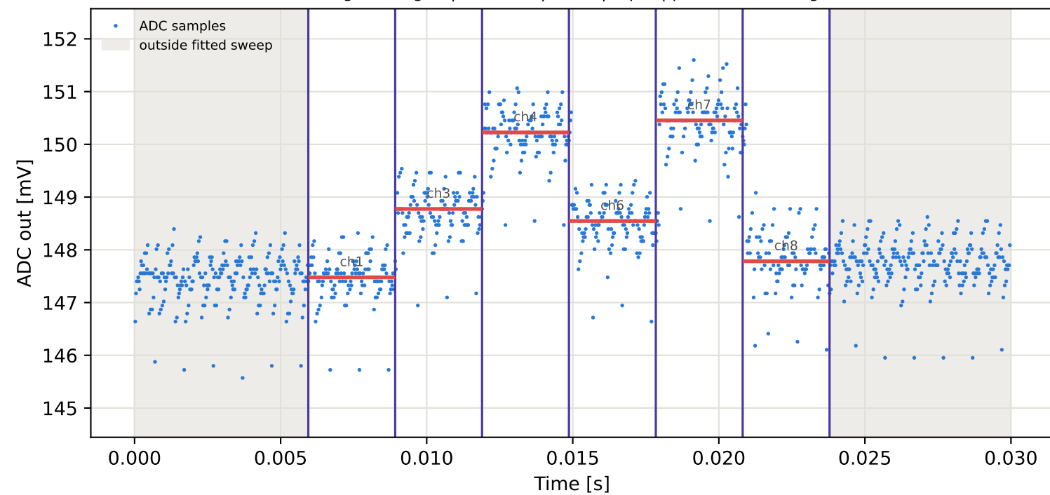
Tag8 &lt;- Tag16 | 795 MHz | run 0 | rep 1 | phase 84.83 deg
