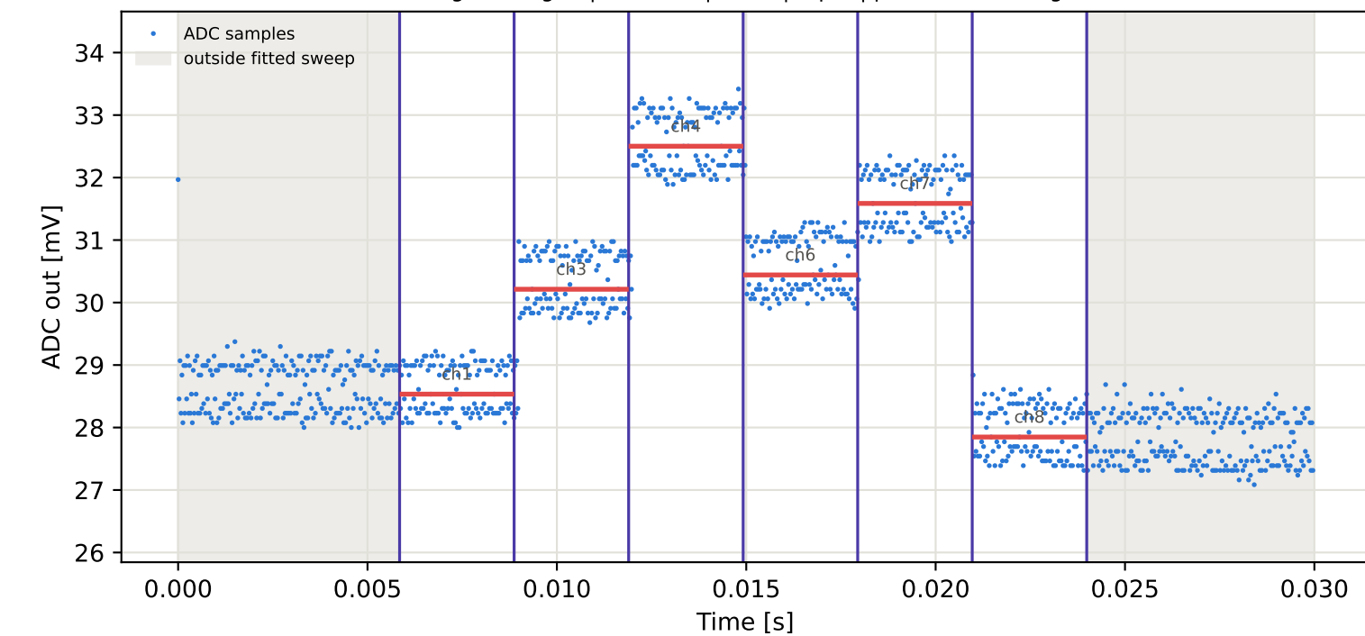
Tag2 &lt;- Tag16 | 925 MHz | run 0 | rep 1 | phase -95.63 deg
