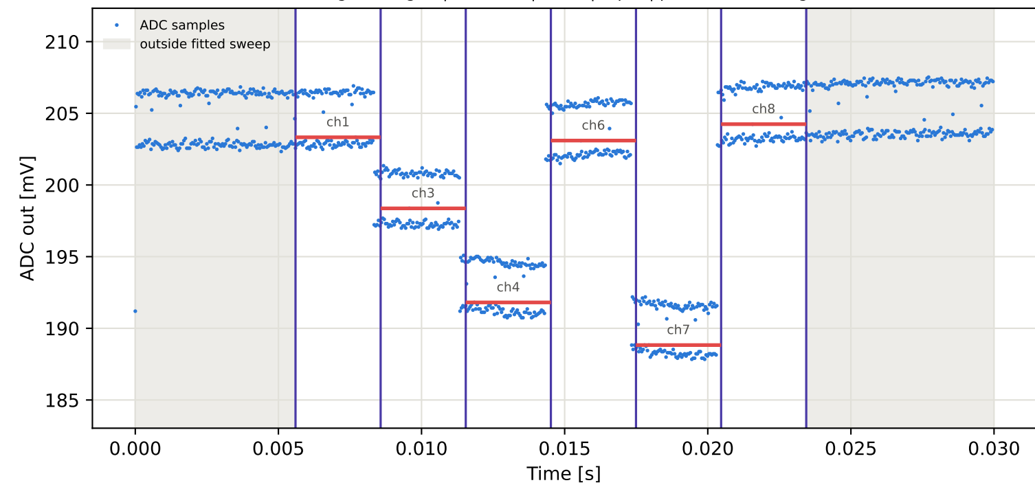
Tag5 &lt;- Tag2 | 775 MHz | run 0 | rep 1 | phase -34.29 deg
