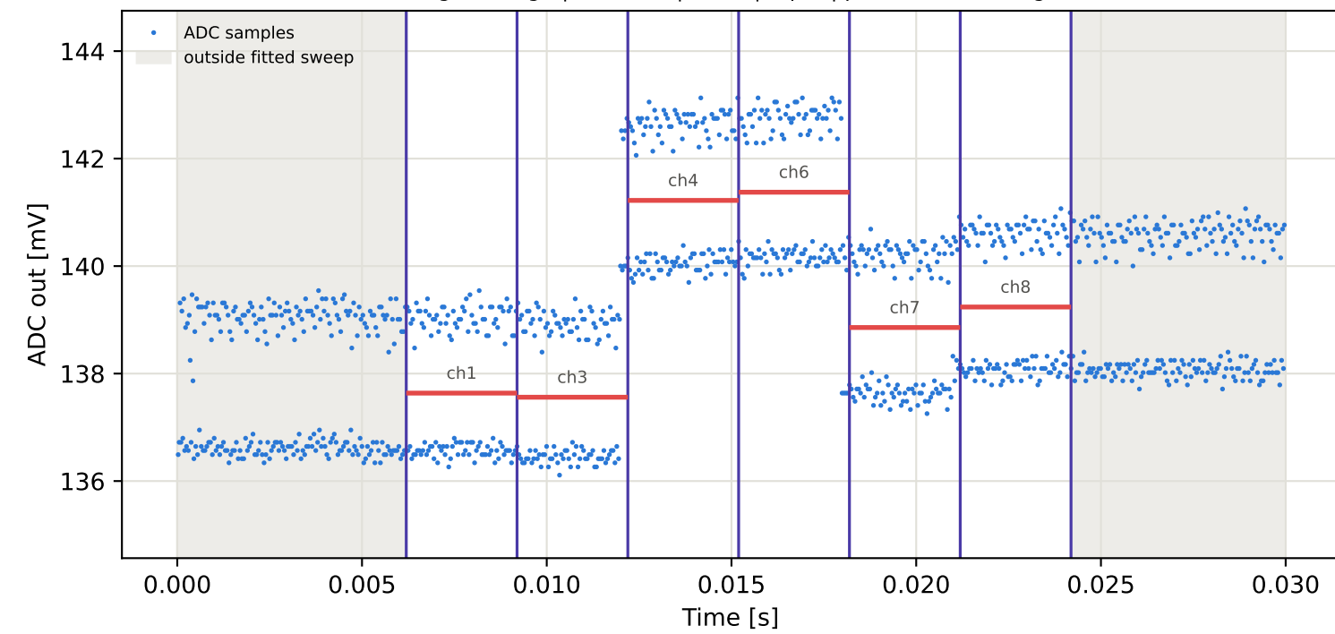
Tag1 &lt;- Tag8 | 995 MHz | run 0 | rep 1 | phase -12.33 deg
