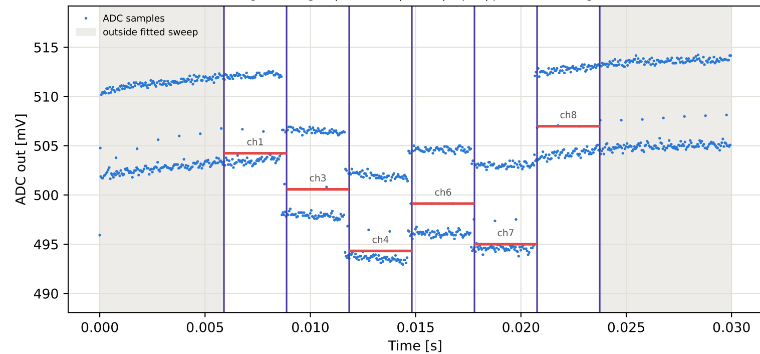
Tag10 &lt;- Tag2 | 895 MHz | run 0 | rep 1 | phase -107.52 deg
