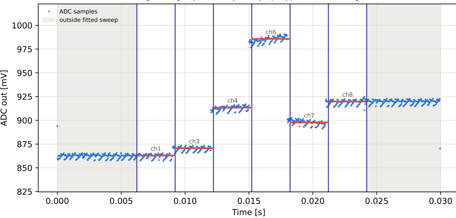
Tag8 &lt;- Tag15 | 915 MHz | run 0 | rep 1 | phase -152.17 deg
