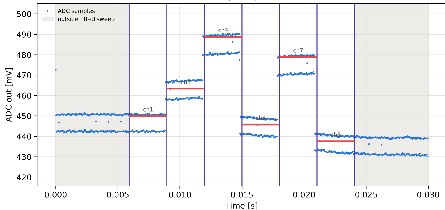
Tag10 &lt;- Tag8 | 945 MHz | run 0 | rep 1 | phase -23.60 deg
