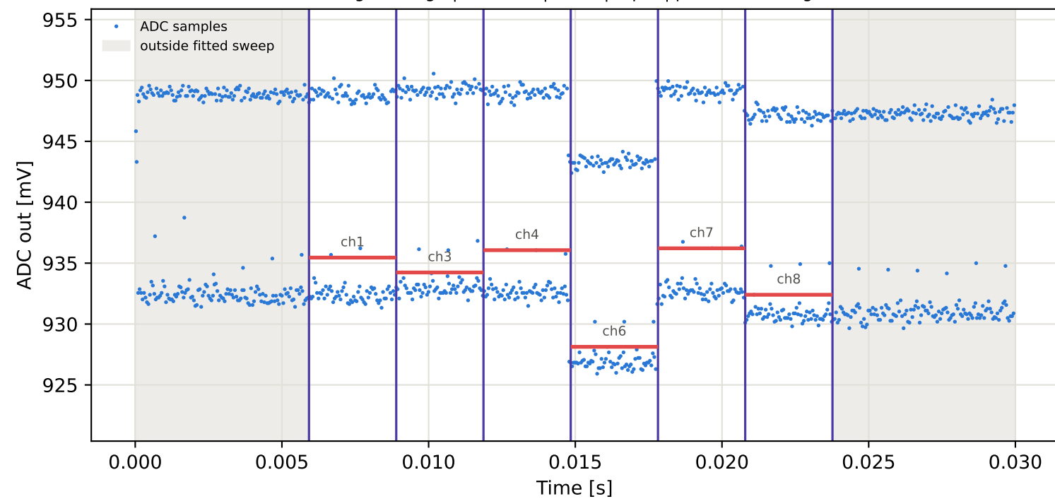
Tag4 &lt;- Tag2 | 935 MHz | run 0 | rep 1 | phase -9.25 deg
