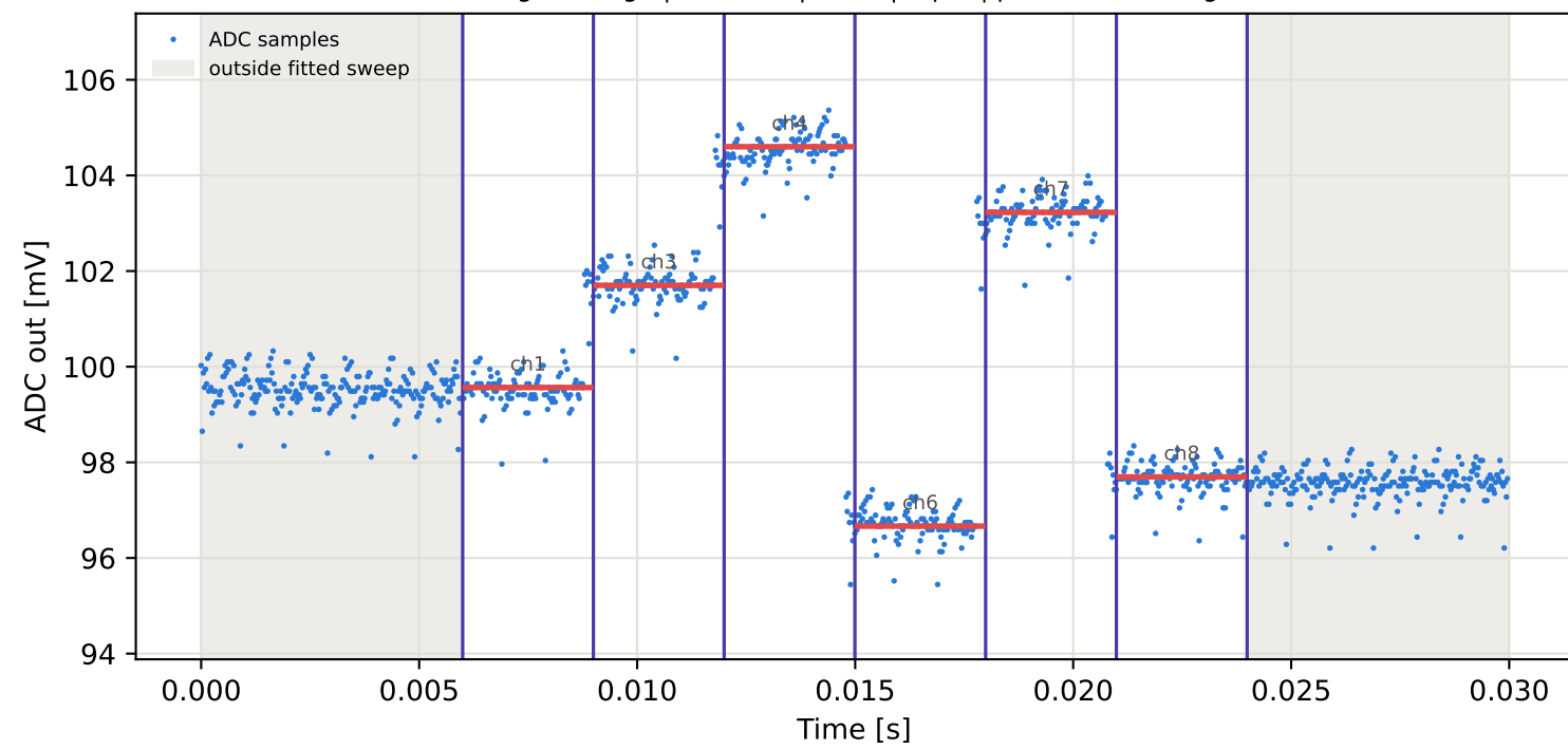
Tag6 &lt;- Tag1 | 995 MHz | run 0 | rep 1 | phase -56.10 deg
