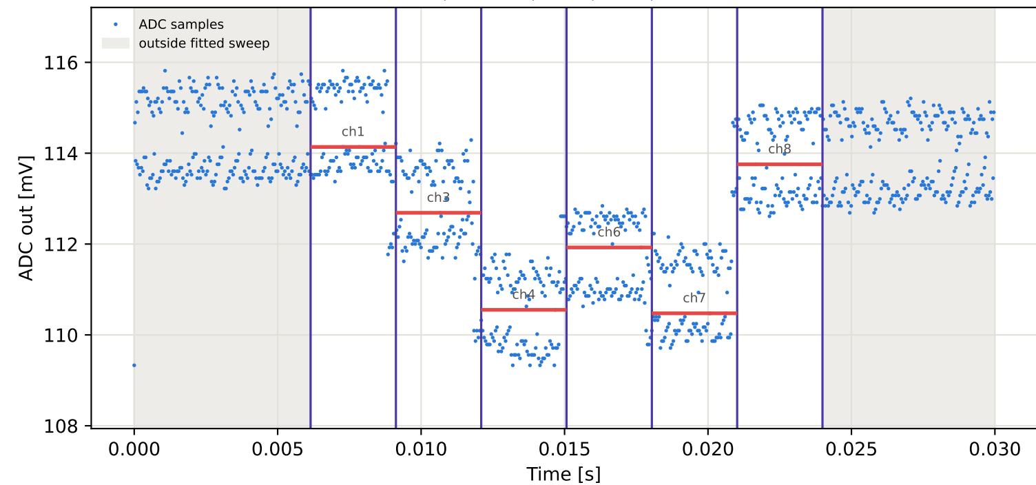
Tag9 &lt;- Tag2 | 795 MHz | run 0 | rep 1 | phase 91.28 deg
