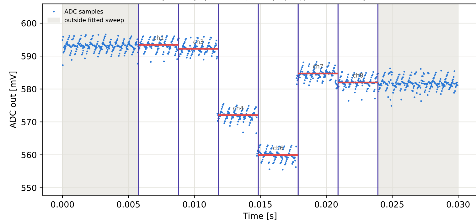
Tag9 &lt;- Tag7 | 975 MHz | run 0 | rep 1 | phase -84.84 deg
