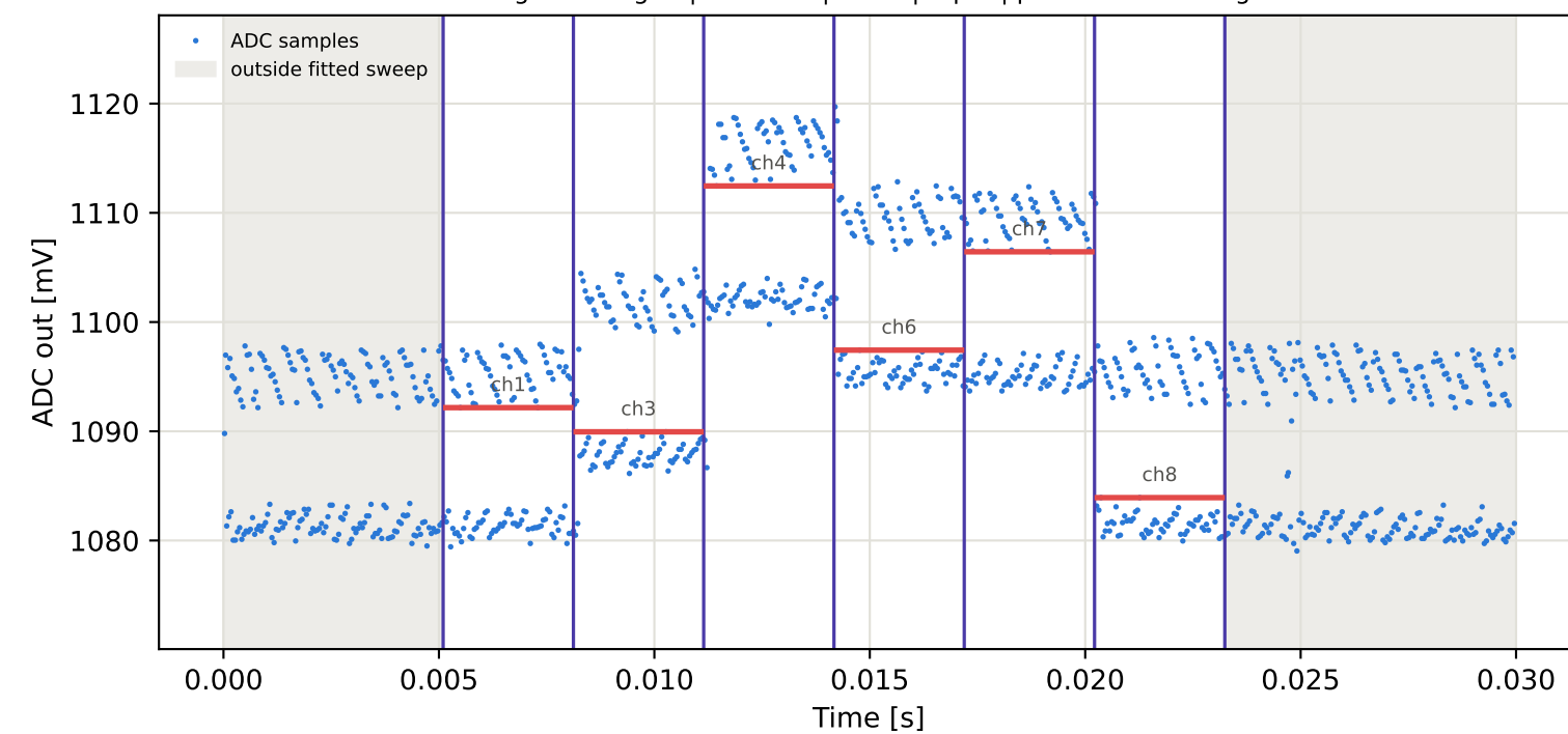
Tag16 &lt;- Tag10 | 945 MHz | run 0 | rep 1 | phase -101.27 deg
