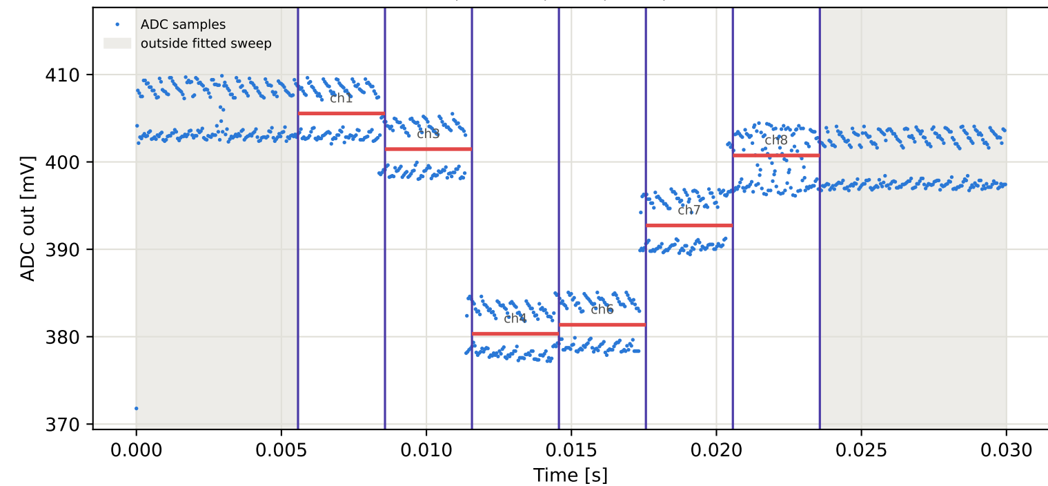
Tag6 &lt;- Tag10 | 965 MHz | run 0 | rep 1 | phase 49.17 deg
