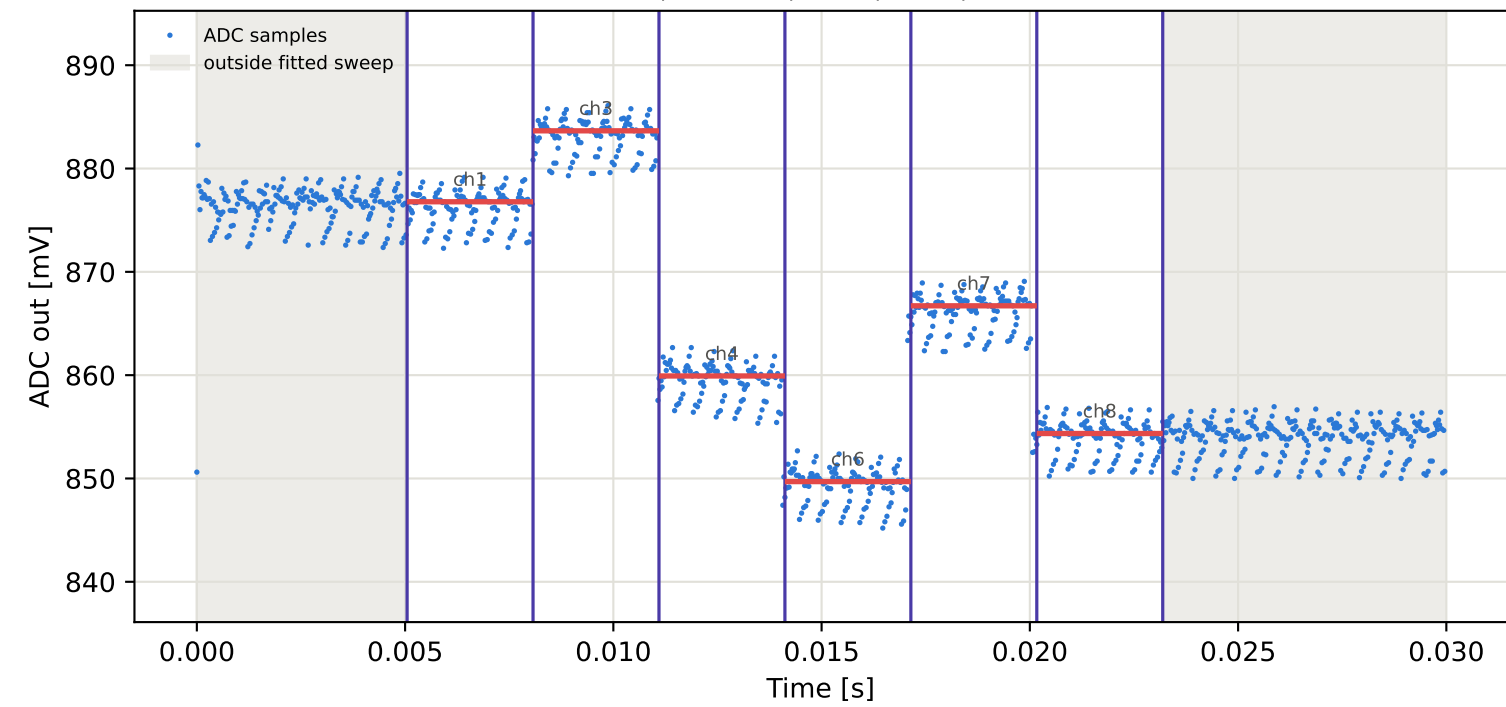
Tag16 &lt;- Tag15 | 855 MHz | run 0 | rep 1 | phase 35.15 deg
