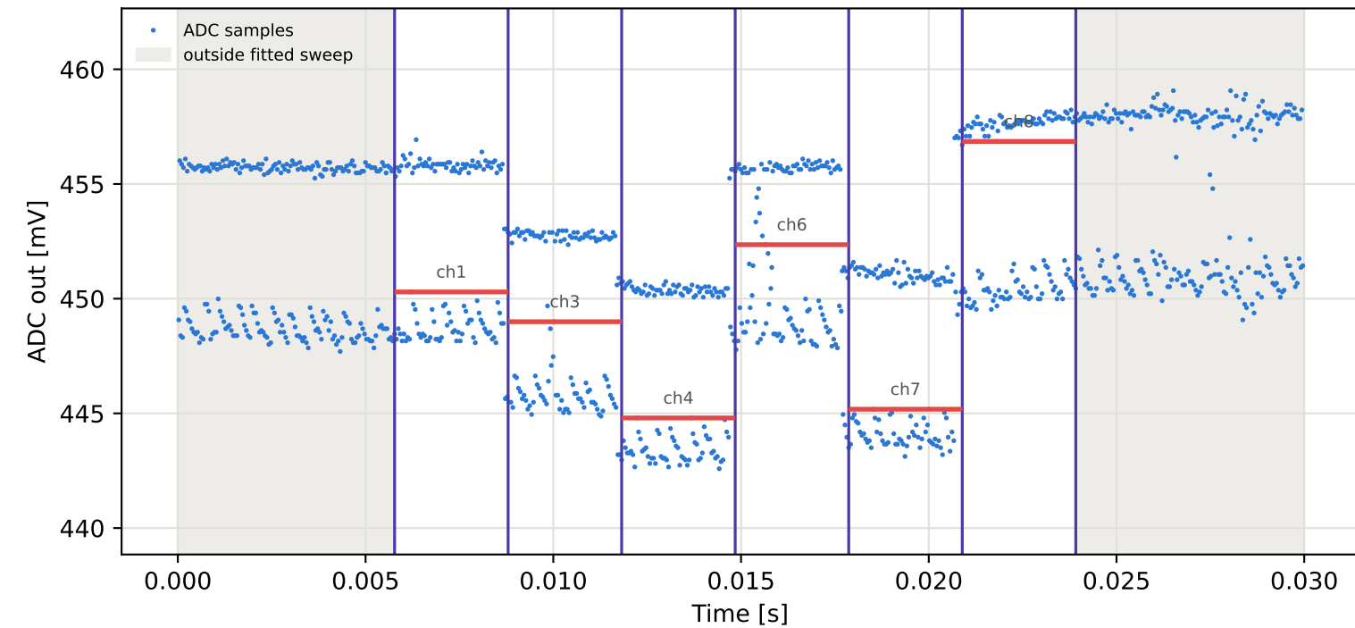
Tag10 &lt;- Tag4 | 875 MHz | run 0 | rep 1 | phase 23.98 deg
