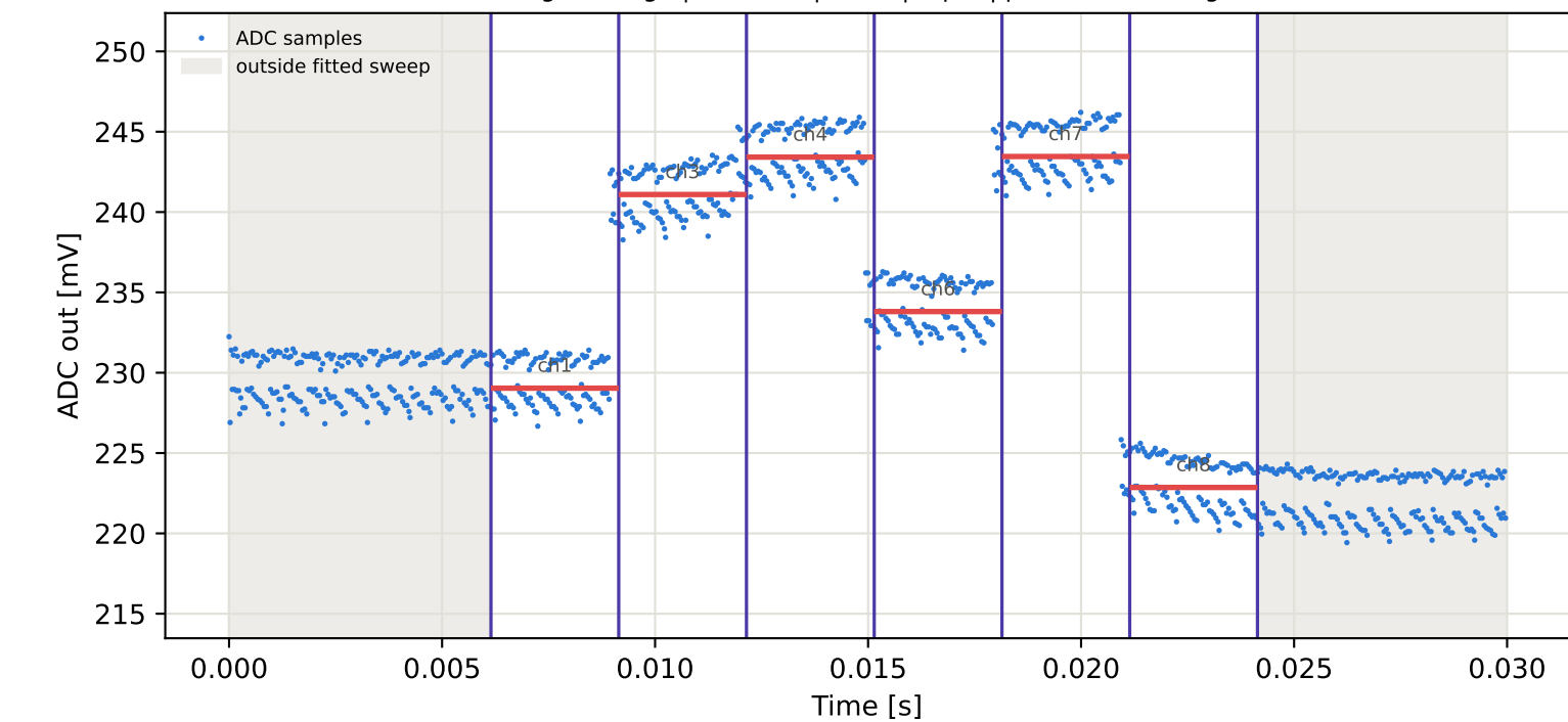
Tag7 &lt;- Tag5 | 865 MHz | run 0 | rep 1 | phase -65.50 deg
