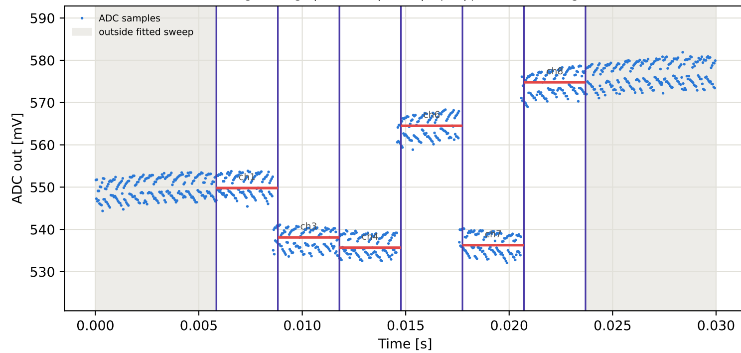
Tag8 &lt;- Tag1 | 895 MHz | run 0 | rep 1 | phase 143.51 deg
