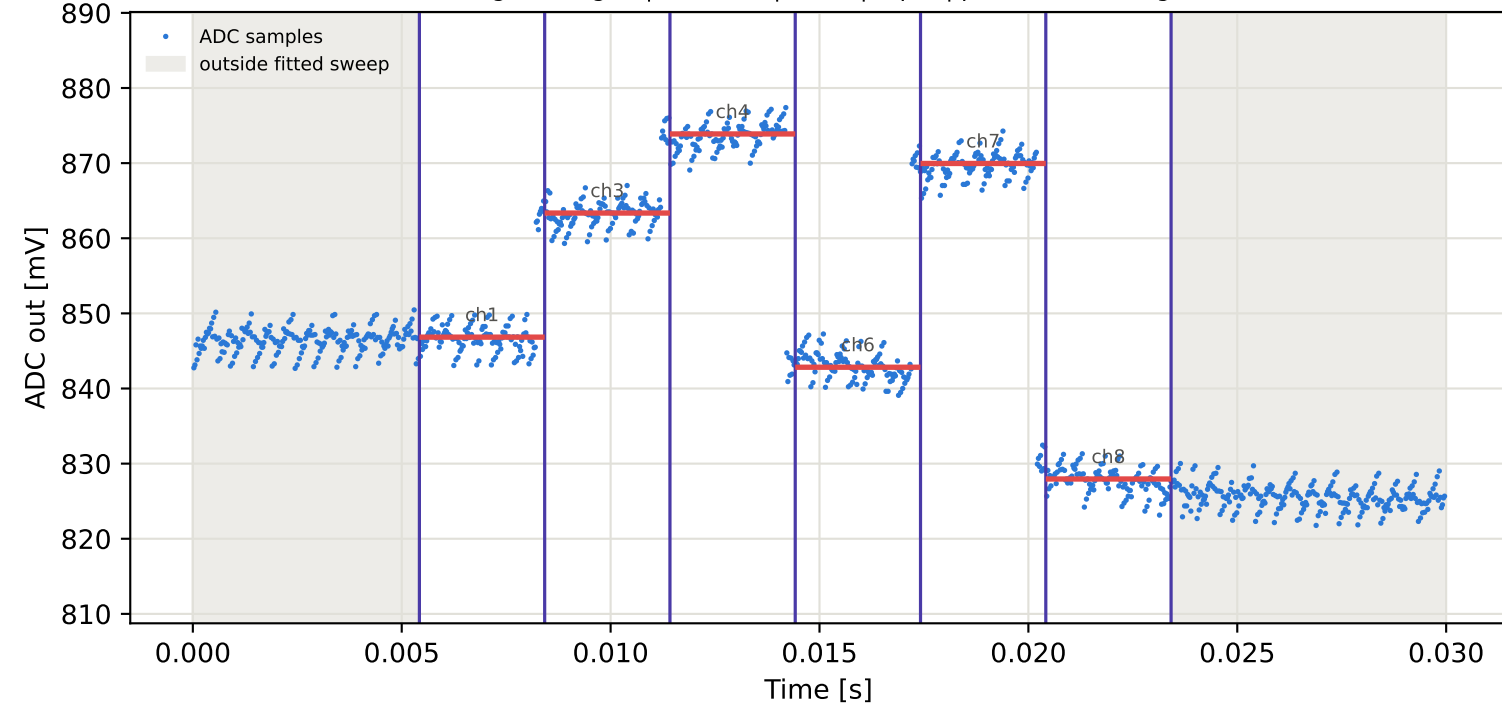
Tag4 &lt;- Tag16 | 915 MHz | run 0 | rep 1 | phase 79.22 deg
