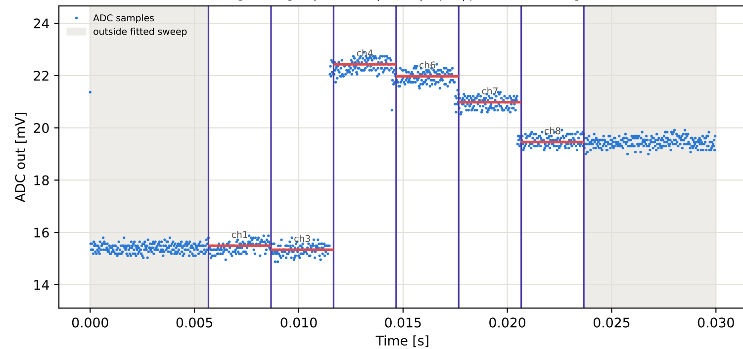
Tag1 &lt;- Tag16 | 825 MHz | run 0 | rep 1 | phase -177.07 deg
