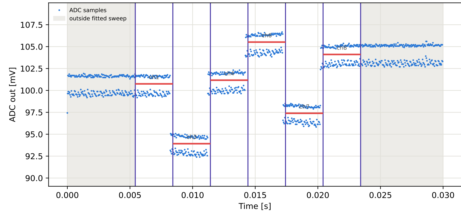
Tag1 &lt;- Tag3 | 805 MHz | run 0 | rep 1 | phase 110.89 deg
