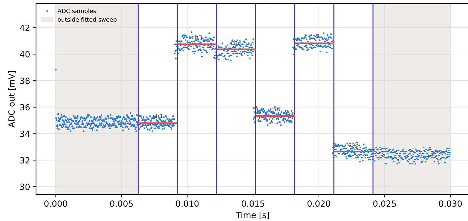
Tag2 &lt;- Tag8 | 855 MHz | run 0 | rep 1 | phase -45.38 deg
