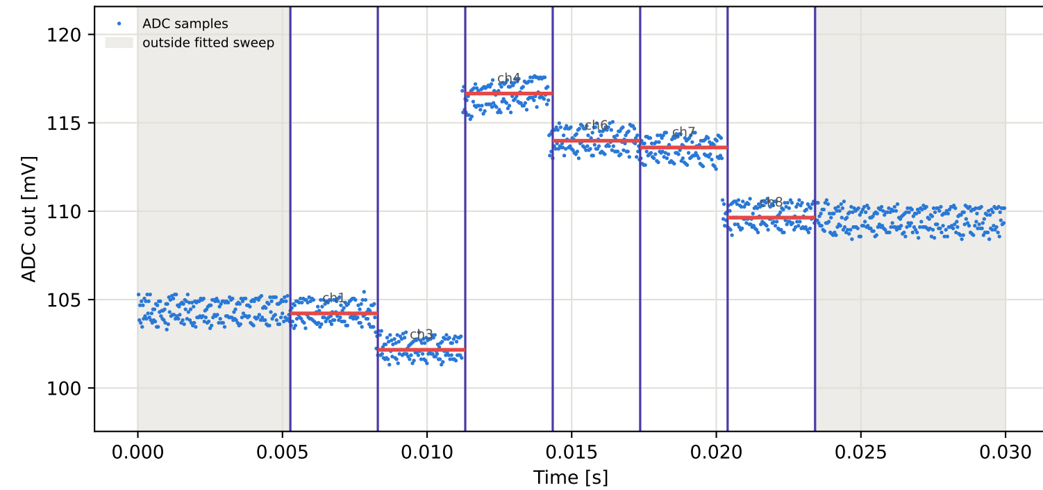
Tag5 &lt;- Tag3 | 805 MHz | run 0 | rep 1 | phase -69.16 deg
