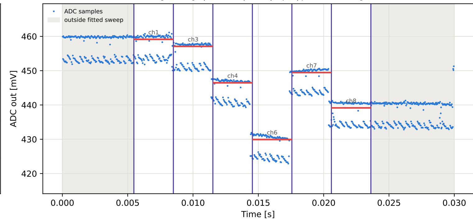
Tag2 &lt;- Tag6 | 875 MHz | run 0 | rep 1 | phase 139.08 deg
