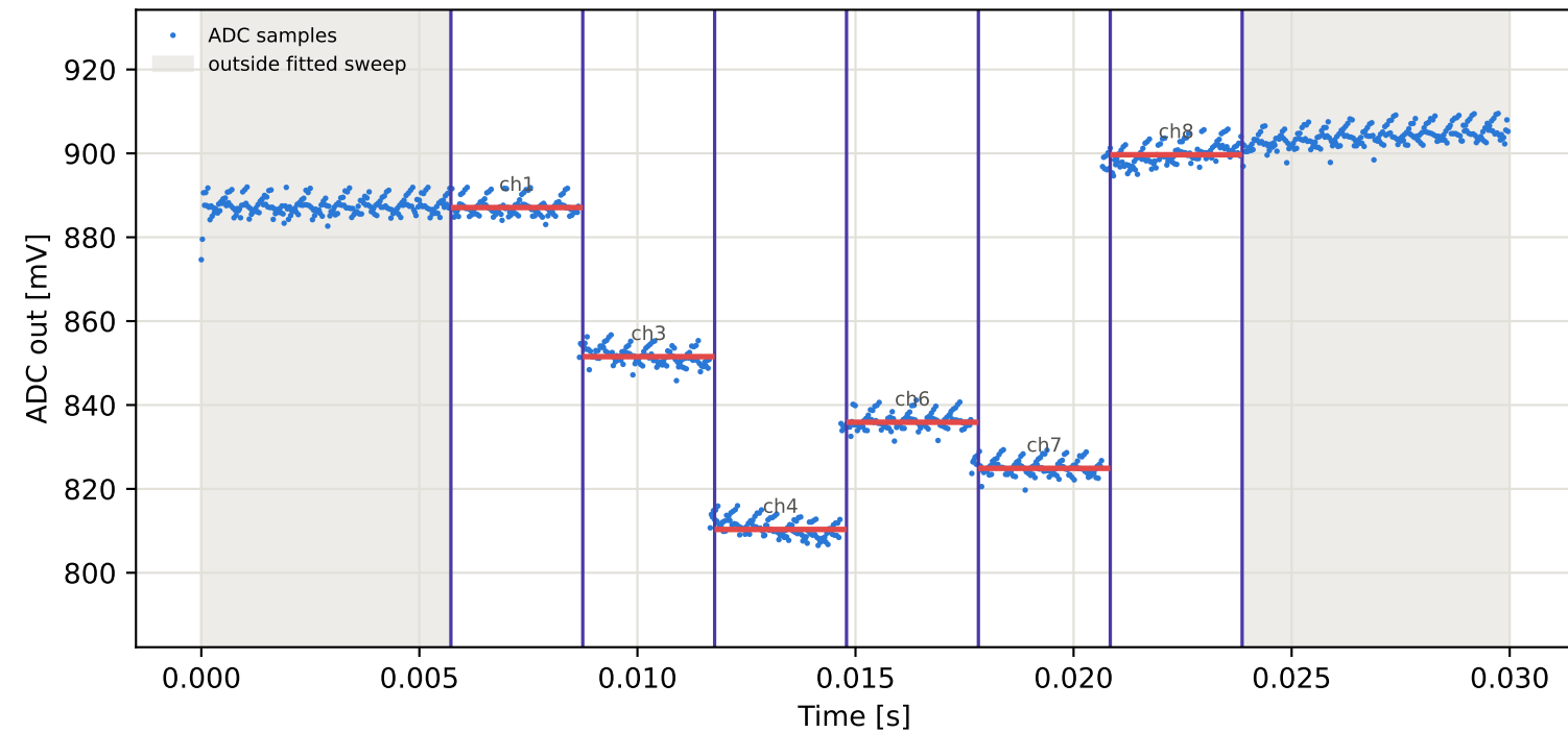
Tag4 &lt;- Tag3 | 915 MHz | run 0 | rep 1 | phase 118.90 deg
