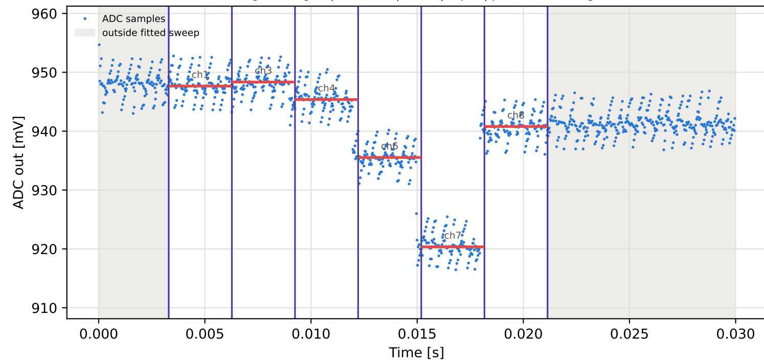
Tag4 &lt;- Tag16 | 935 MHz | run 0 | rep 1 | phase 109.72 deg
