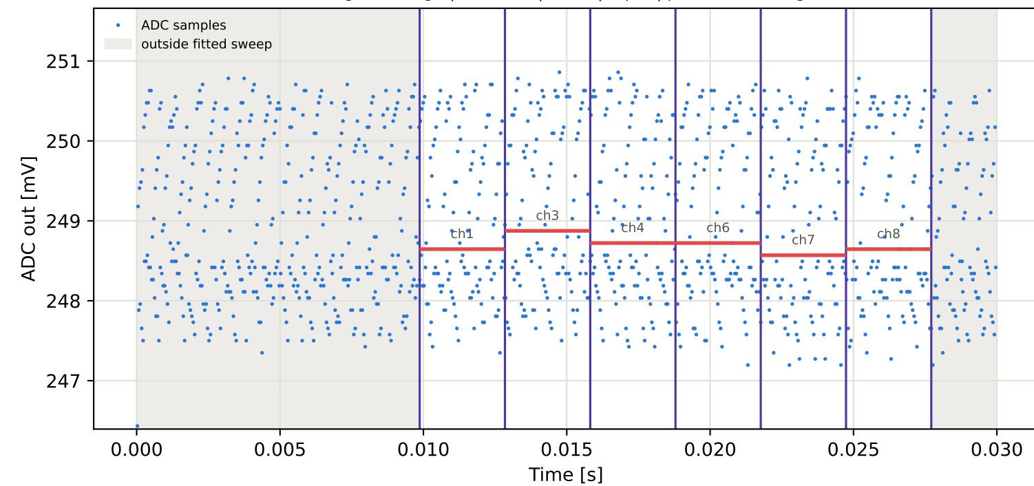
Tag15 &lt;- Tag9 | 785 MHz | run 0 | rep 1 | phase -165.00 deg
