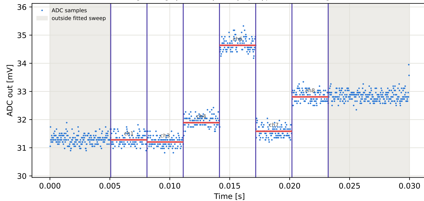
Tag3 &lt;- Tag10 | 915 MHz | run 0 | rep 1 | phase 5.42 deg
