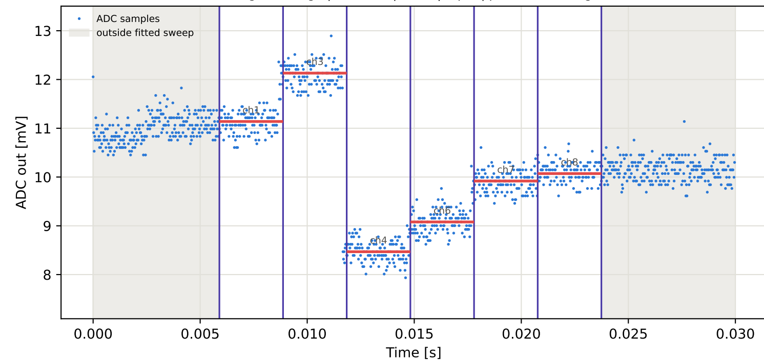
Tag10 &lt;- Tag9 | 775 MHz | run 0 | rep 1 | phase 160.39 deg
