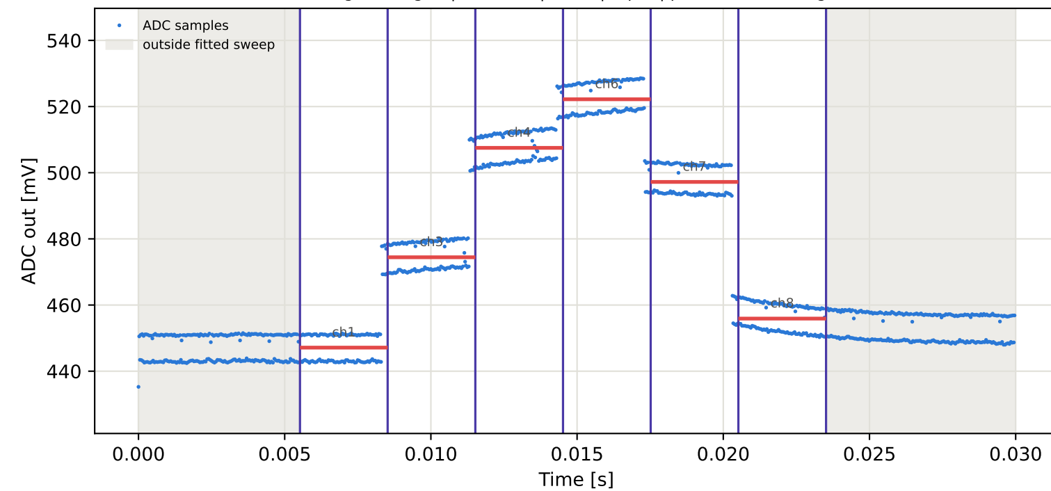
Tag7 &lt;- Tag3 | 905 MHz | run 0 | rep 1 | phase 102.76 deg
