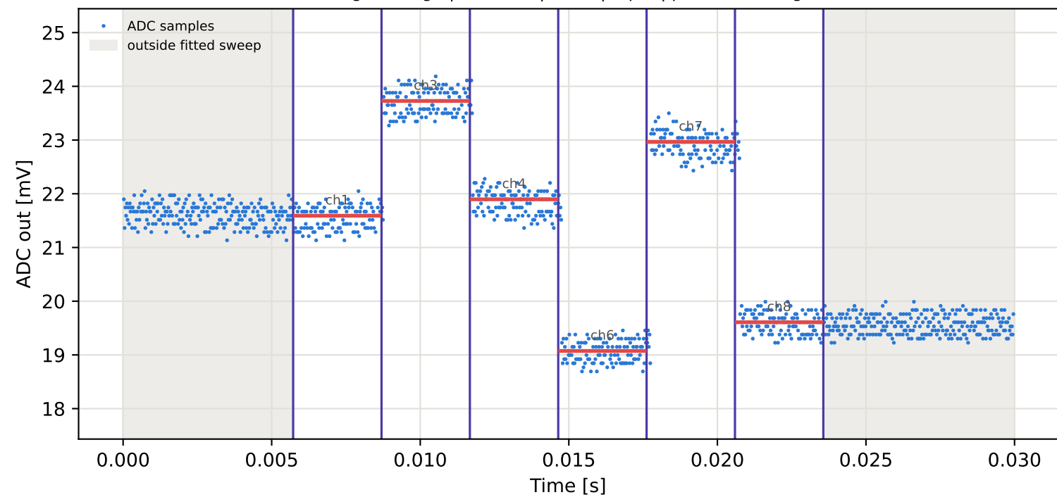
Tag1 &lt;- Tag9 | 825 MHz | run 0 | rep 1 | phase -153.70 deg
