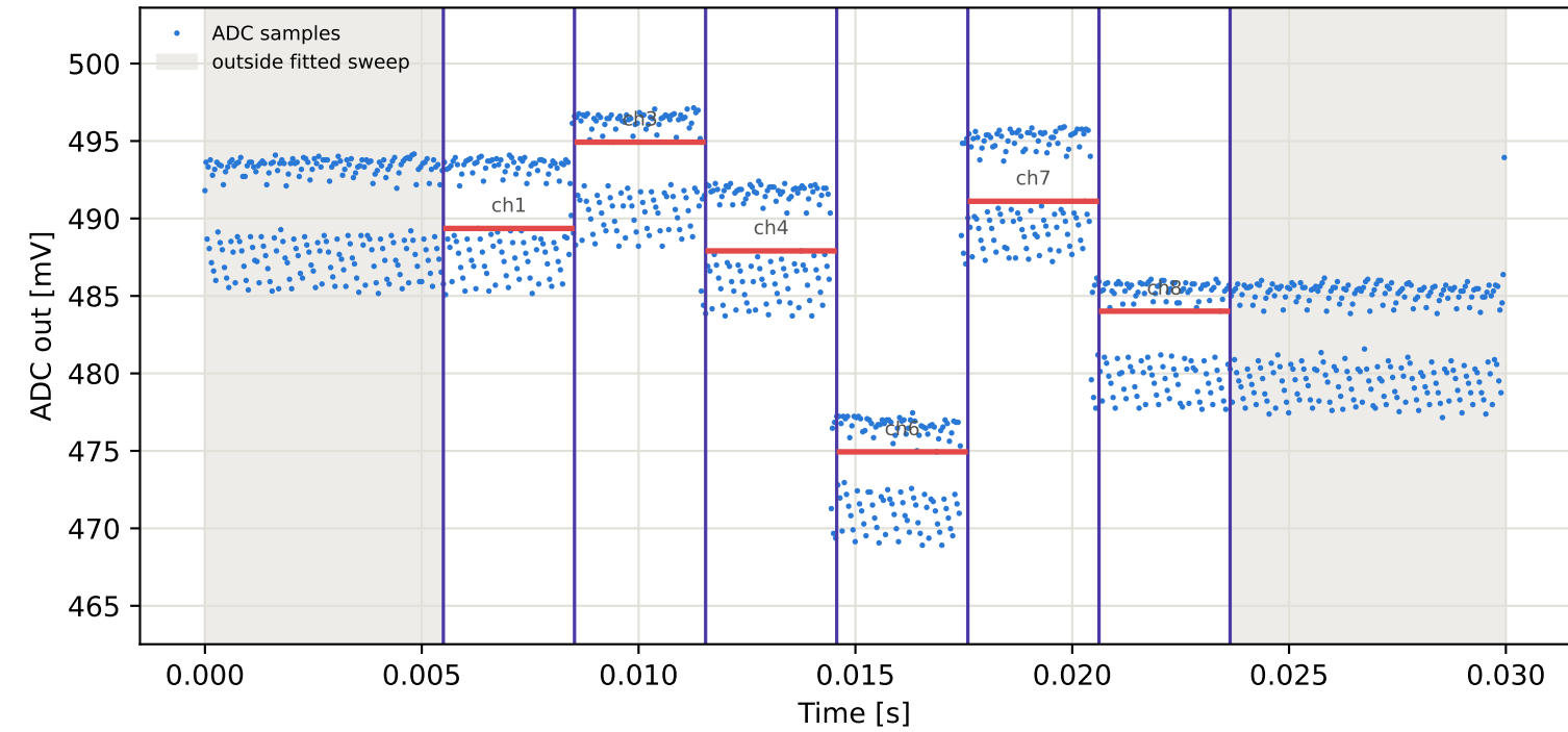
Tag3 &lt;- Tag2 | 975 MHz | run 0 | rep 1 | phase -14.02 deg
