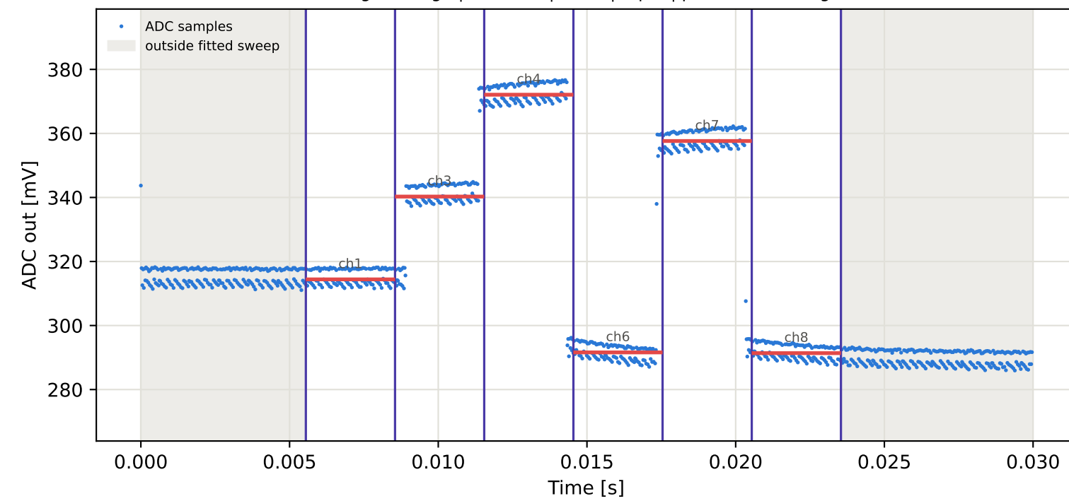
Tag1 &lt;- Tag3 | 955 MHz | run 0 | rep 1 | phase -57.59 deg
