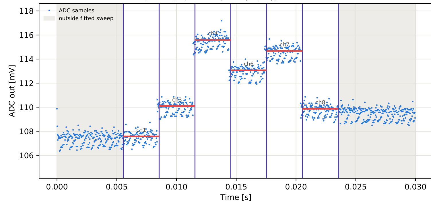
Tag5 &lt;- Tag8 | 805 MHz | run 0 | rep 1 | phase -58.53 deg
