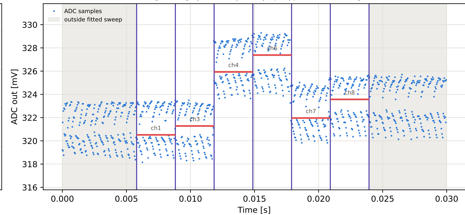
Tag9 &lt;- Tag15 | 995 MHz | run 0 | rep 1 | phase -45.41 deg
