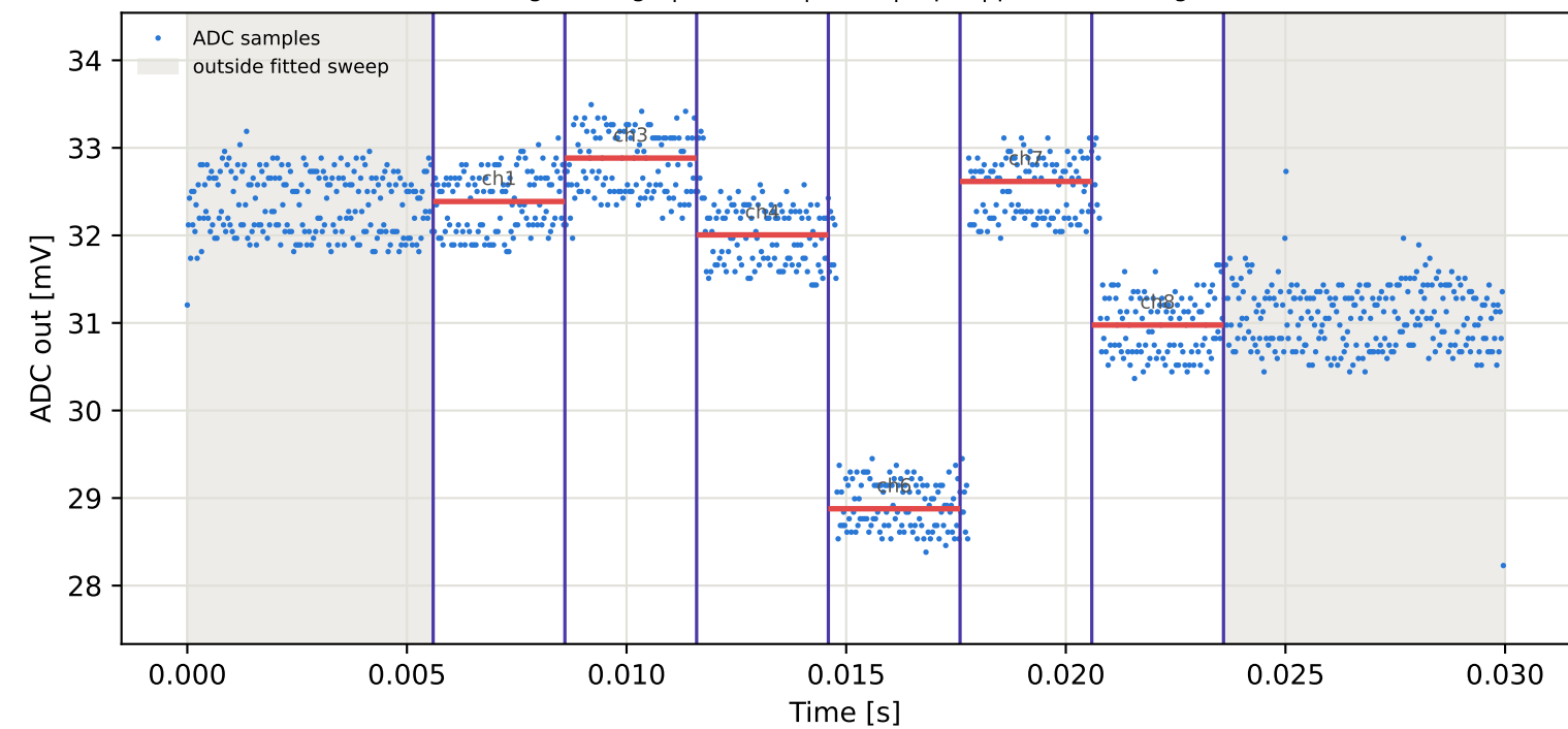
Tag2 &lt;- Tag8 | 945 MHz | run 0 | rep 1 | phase -14.25 deg
