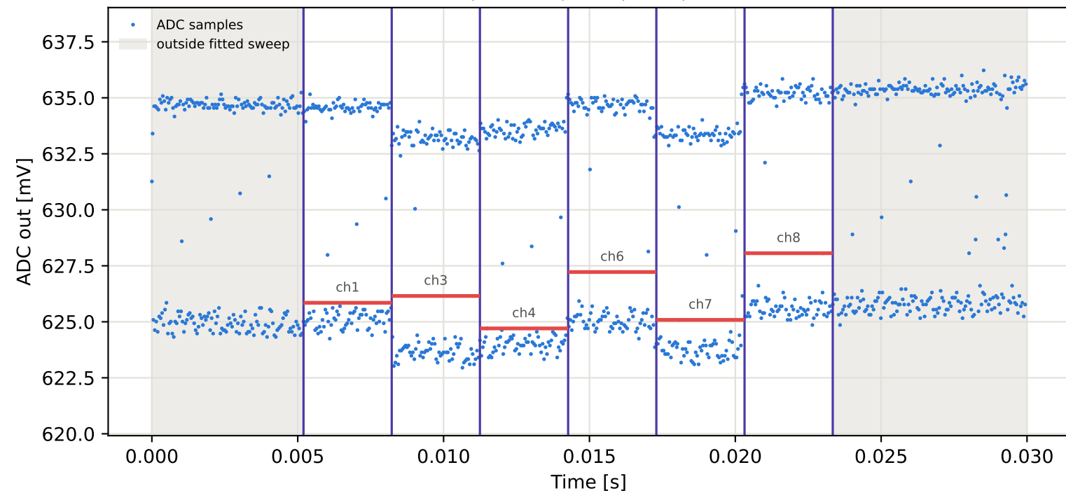
Tag15 &lt;- Tag10 | 855 MHz | run 0 | rep 1 | phase 133.68 deg
