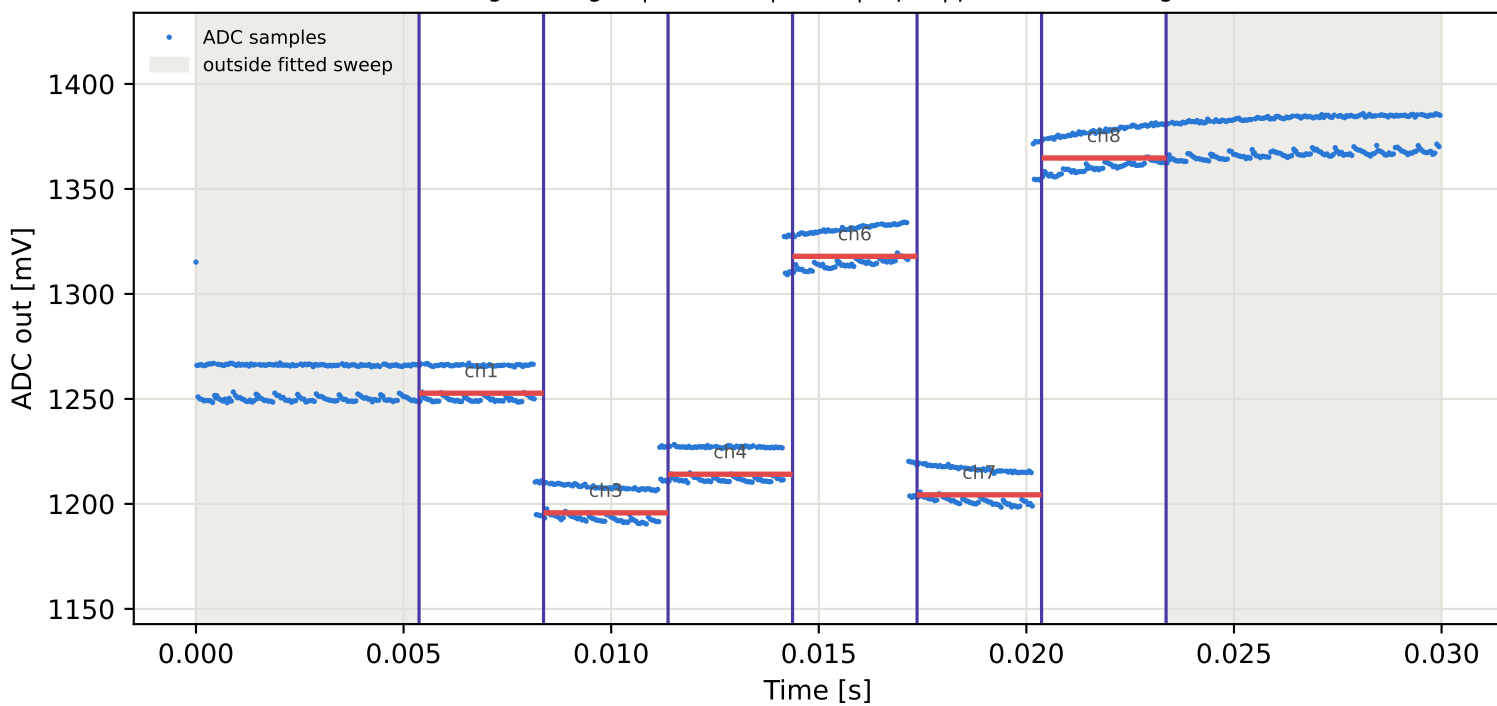
Tag8 &lt;- Tag16 | 885 MHz | run 0 | rep 1 | phase 157.25 deg
