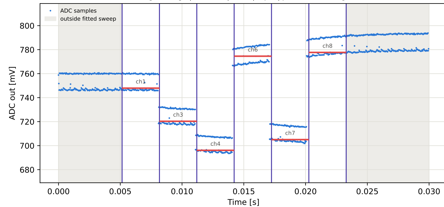
Tag9 &lt;- Tag5 | 935 MHz | run 0 | rep 1 | phase -27.11 deg
