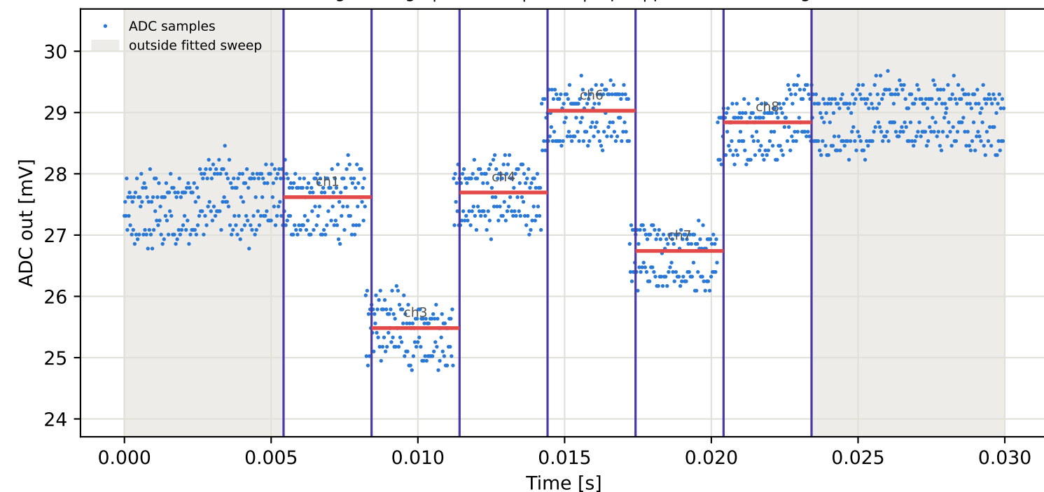
Tag2 &lt;- Tag8 | 825 MHz | run 0 | rep 1 | phase -164.11 deg
