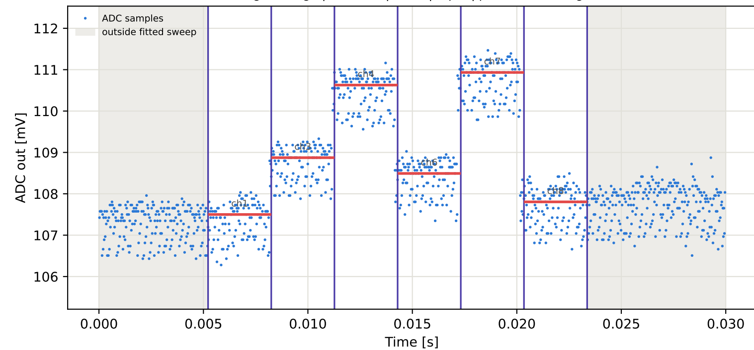
Tag3 &lt;- Tag8 | 775 MHz | run 0 | rep 1 | phase 93.34 deg
