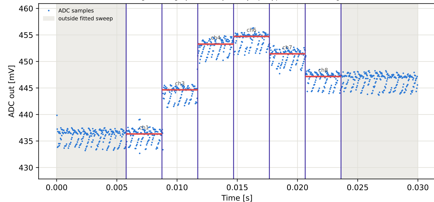
Tag15 &lt;- Tag10 | 875 MHz | run 0 | rep 1 | phase 7.63 deg
