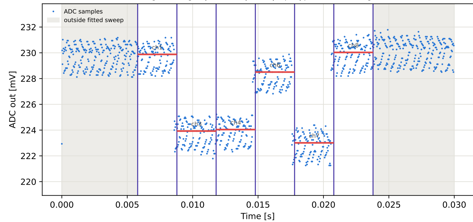
Tag10 &lt;- Tag3 | 835 MHz | run 0 | rep 1 | phase -179.70 deg
