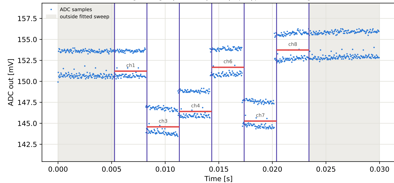
Tag1 &lt;- Tag16 | 845 MHz | run 0 | rep 1 | phase -36.20 deg
