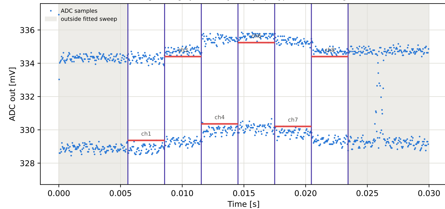
Tag8 &lt;- Tag4 | 805 MHz | run 0 | rep 1 | phase 143.11 deg
