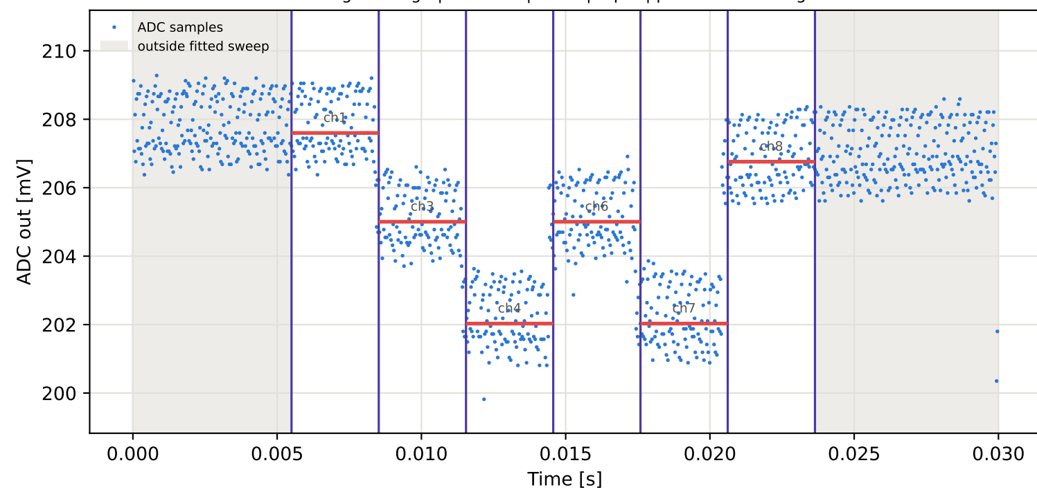
Tag3 &lt;- Tag9 | 805 MHz | run 0 | rep 1 | phase 100.24 deg
