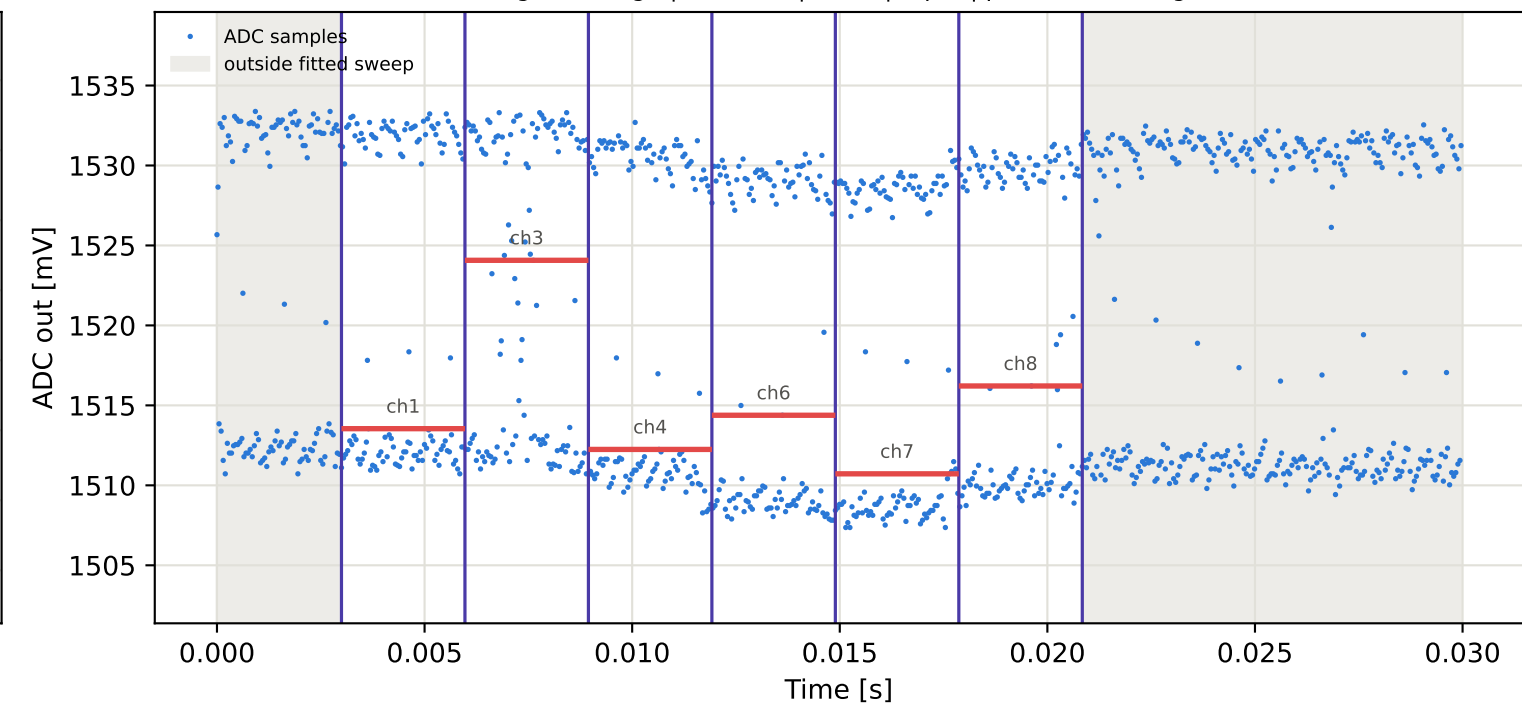
Tag15 &lt;- Tag4 | 895 MHz | run 0 | rep 1 | phase -17.83 deg
