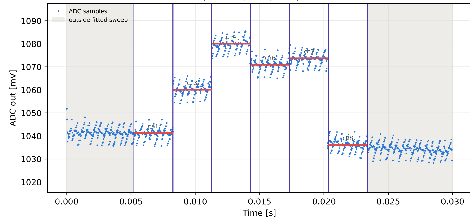
Tag5 &lt;- Tag16 | 915 MHz | run 0 | rep 1 | phase 55.88 deg
