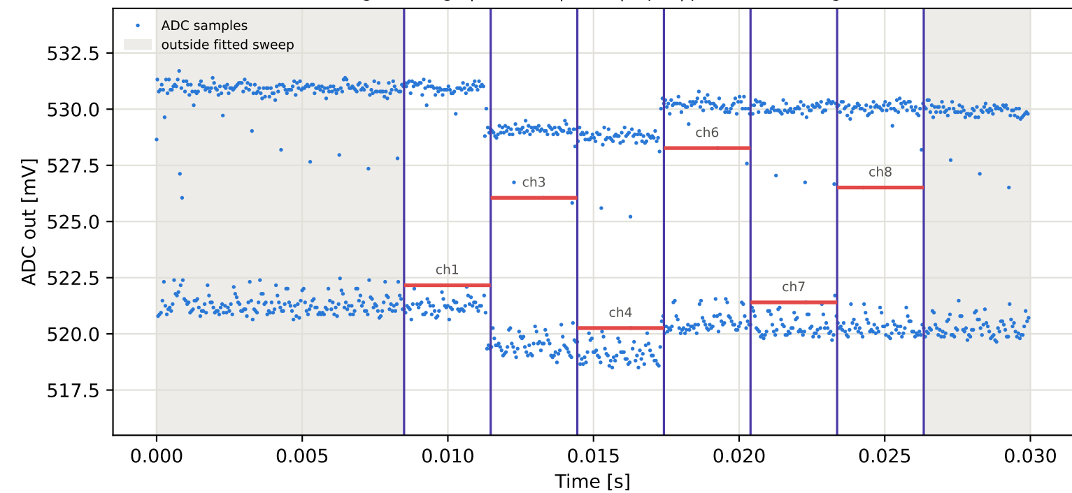
Tag15 &lt;- Tag9 | 995 MHz | run 0 | rep 1 | phase 75.44 deg
