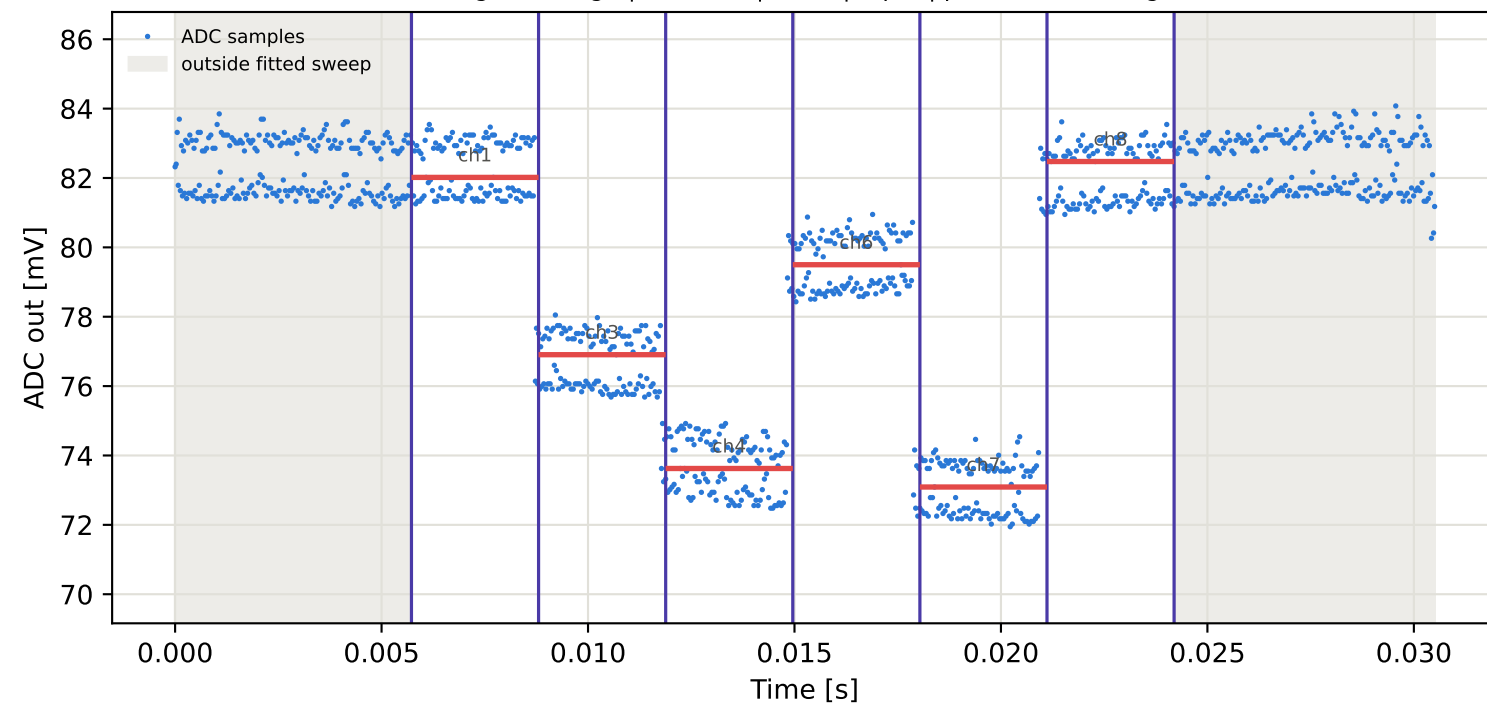
Tag10 &lt;- Tag8 | 795 MHz | run 0 | rep 1 | phase -164.71 deg
