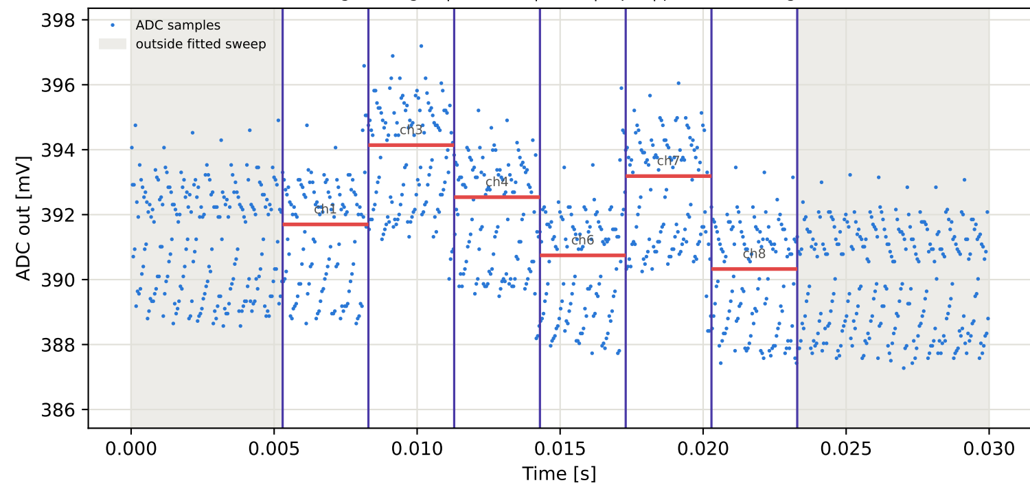
Tag5 &lt;- Tag16 | 835 MHz | run 0 | rep 1 | phase -36.00 deg
