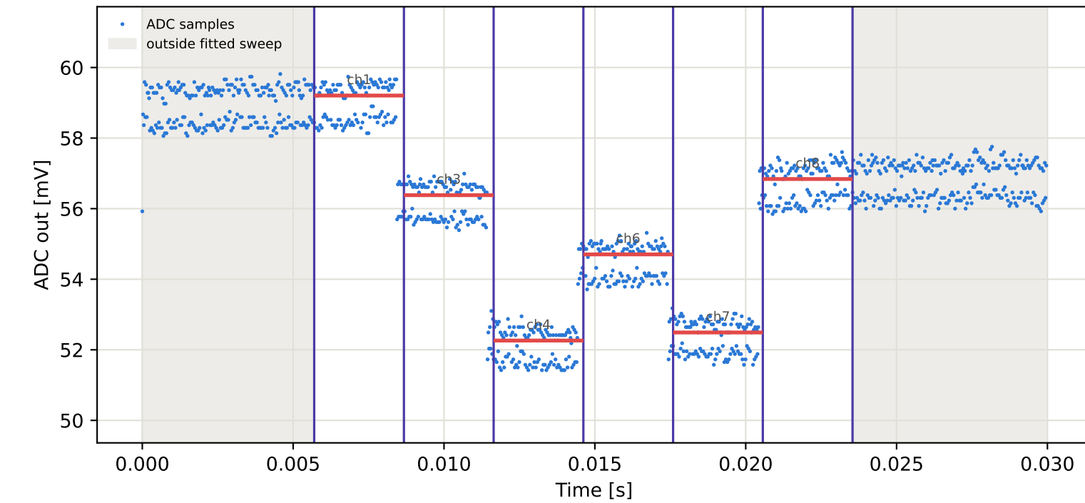
Tag9 &lt;- Tag16 | 825 MHz | run 0 | rep 1 | phase 132.27 deg
