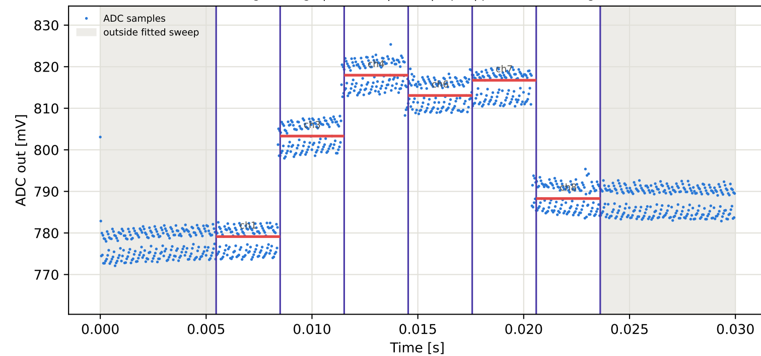
Tag3 &lt;- Tag6 | 865 MHz | run 0 | rep 1 | phase 131.65 deg
