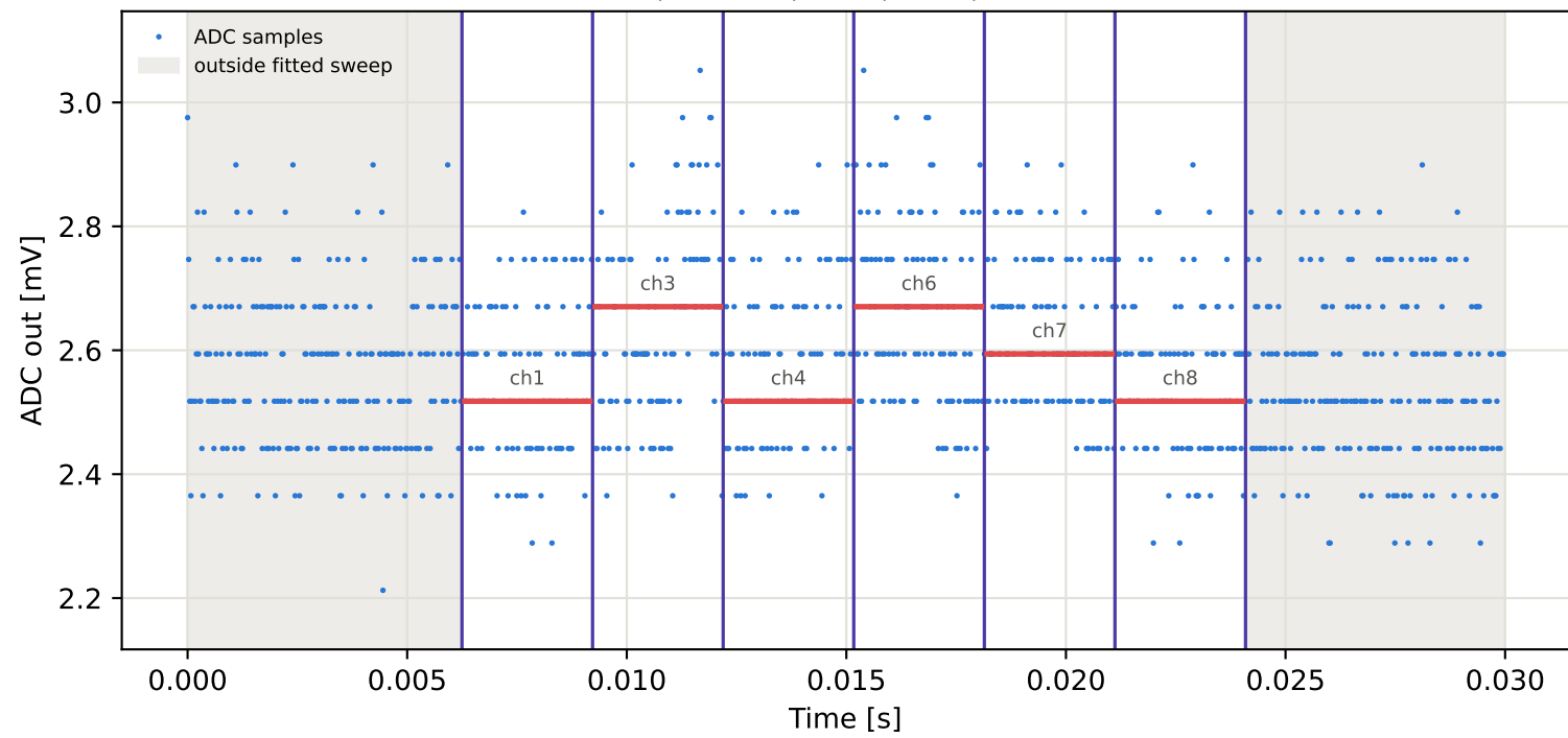
Tag7 &lt;- Tag15 | 785 MHz | run 0 | rep 1 | phase -157.08 deg
