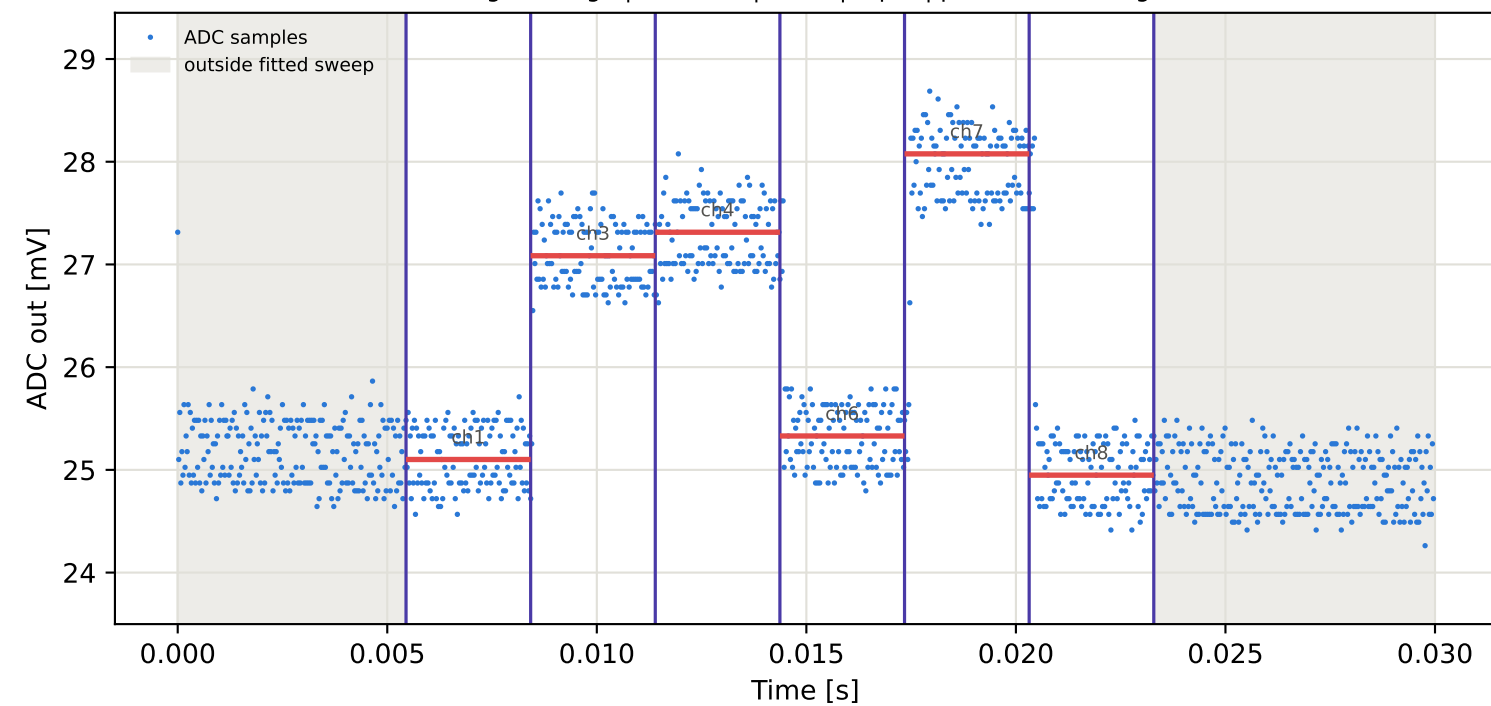
Tag2 &lt;- Tag8 | 805 MHz | run 0 | rep 1 | phase -45.23 deg
