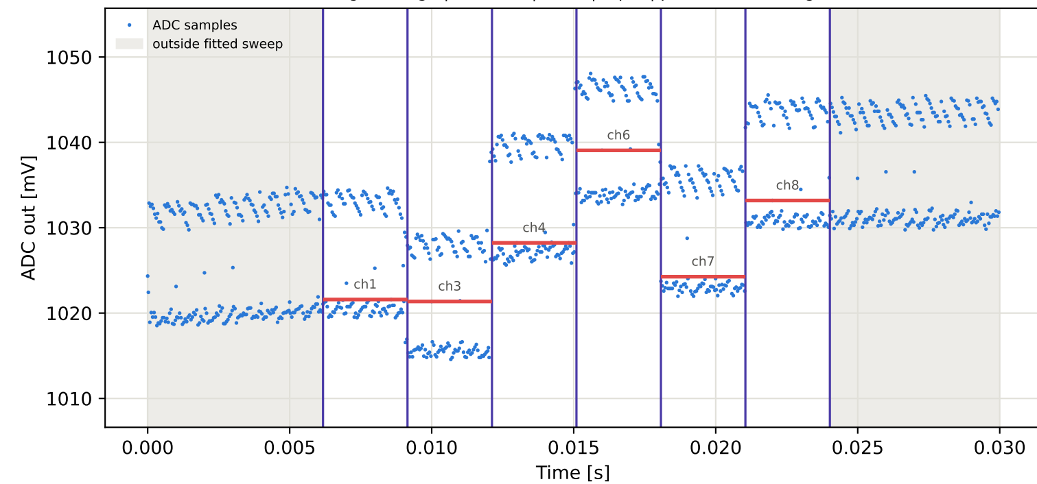
Tag9 &lt;- Tag10 | 855 MHz | run 0 | rep 1 | phase -59.38 deg
