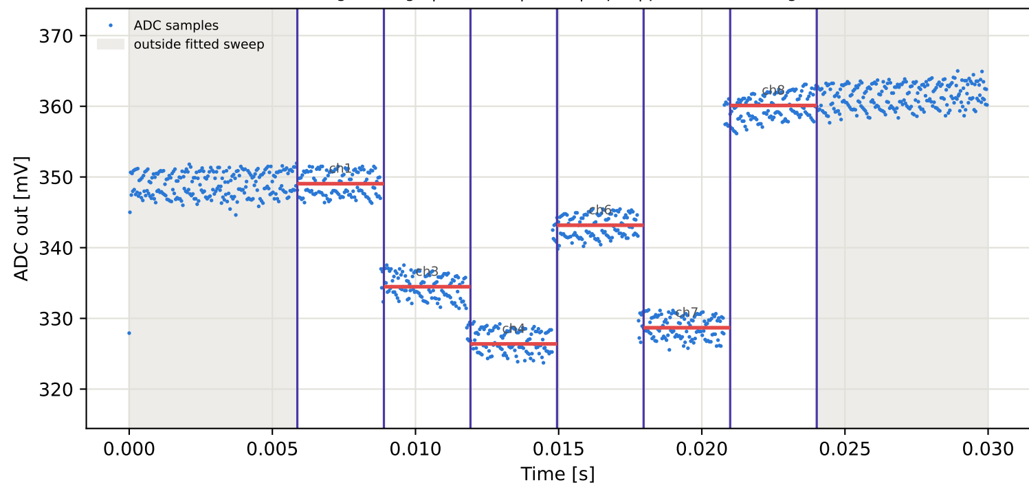
Tag2 &lt;- Tag7 | 885 MHz | run 0 | rep 1 | phase 63.04 deg
