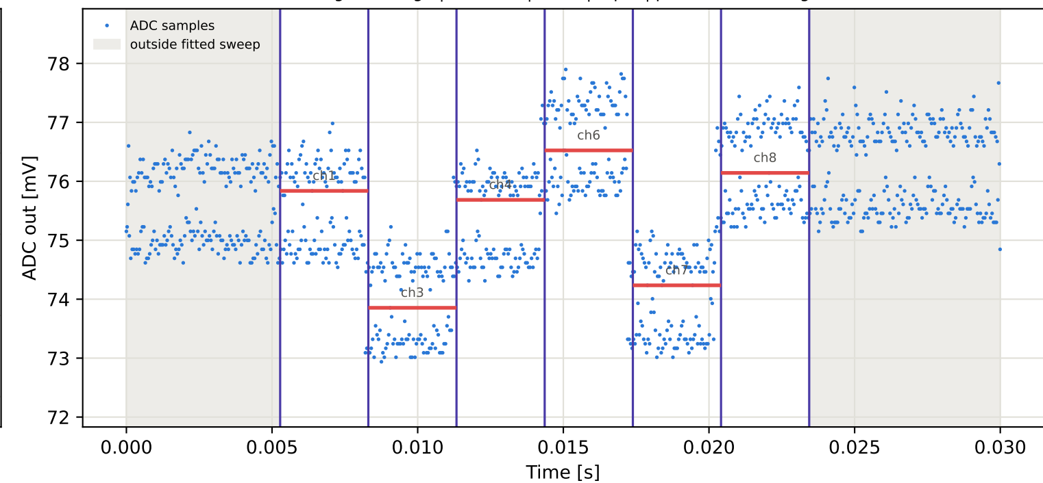
Tag10 &lt;- Tag1 | 795 MHz | run 0 | rep 1 | phase -170.10 deg
