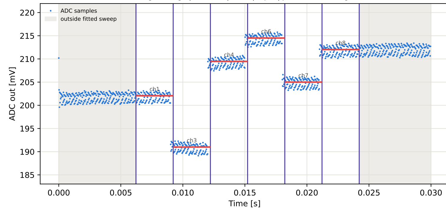
Tag3 &lt;- Tag6 | 825 MHz | run 0 | rep 1 | phase 51.67 deg
