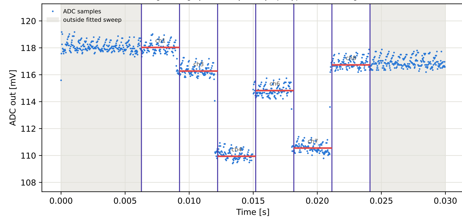
Tag9 &lt;- Tag7 | 795 MHz | run 0 | rep 1 | phase -105.07 deg
