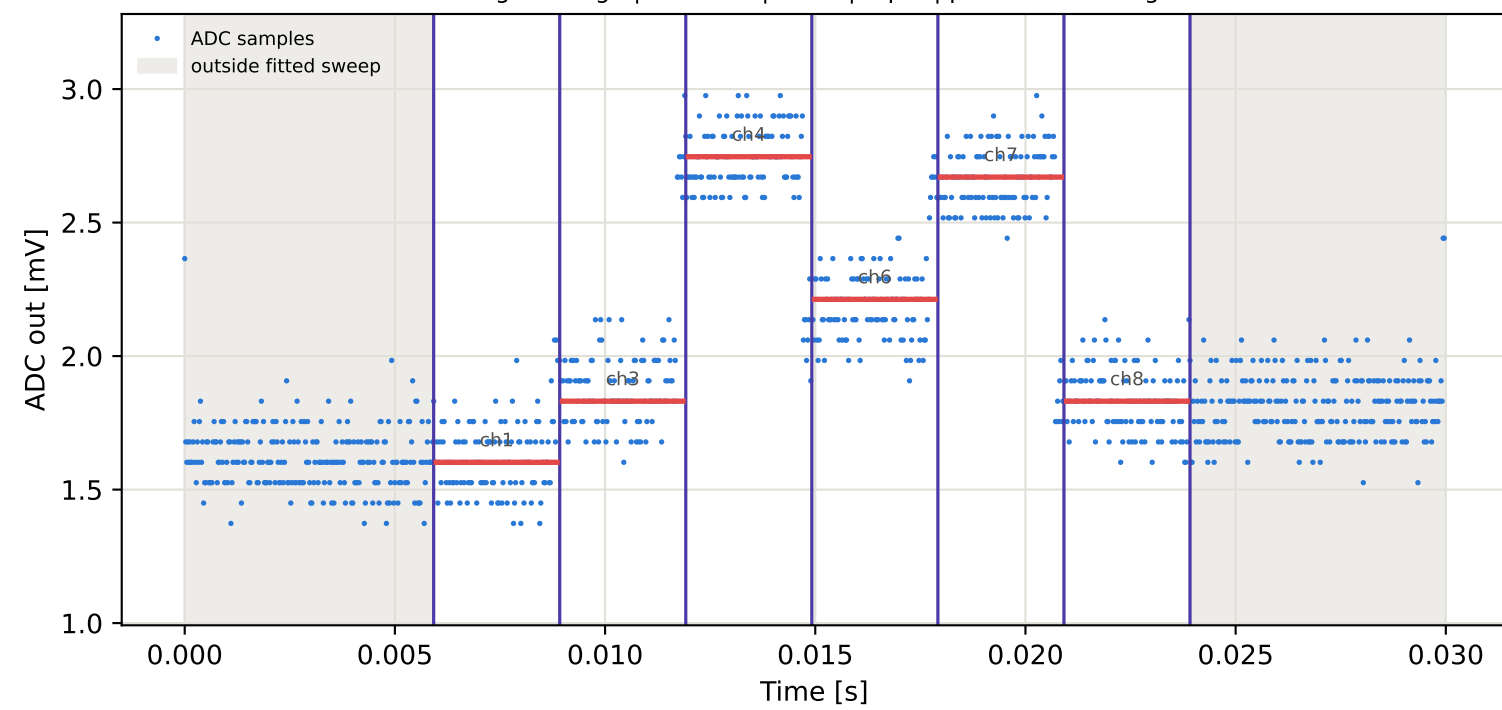
Tag8 &lt;- Tag10 | 785 MHz | run 0 | rep 1 | phase 159.86 deg
