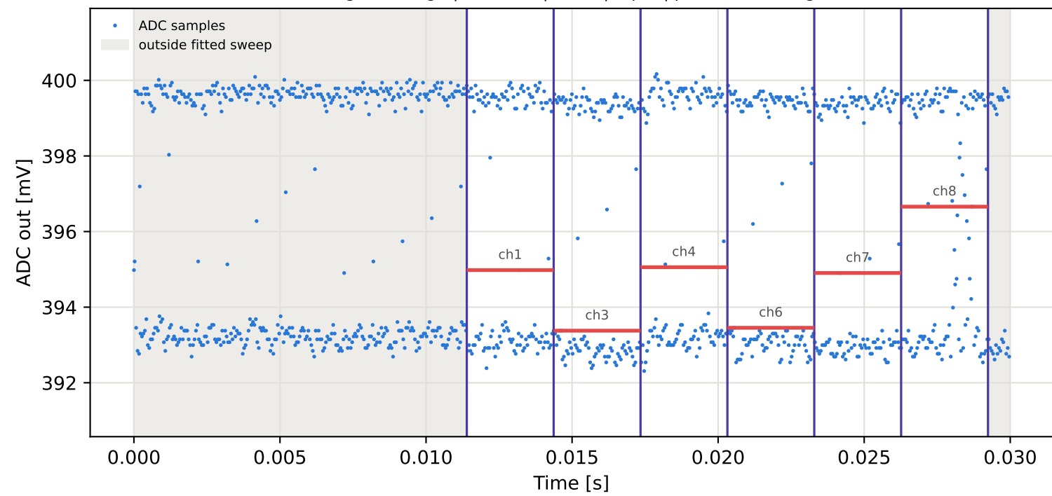
Tag16 &lt;- Tag4 | 805 MHz | run 0 | rep 1 | phase -26.89 deg
