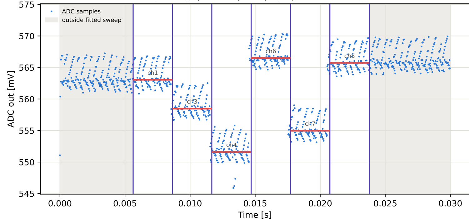
Tag8 &lt;- Tag5 | 995 MHz | run 0 | rep 1 | phase 37.70 deg
