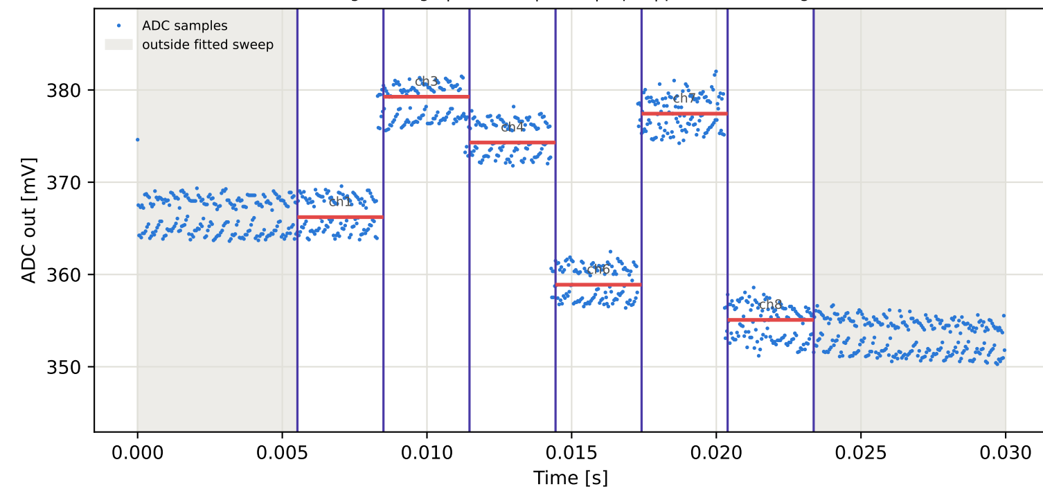
Tag4 &lt;- Tag9 | 875 MHz | run 0 | rep 1 | phase -126.56 deg
