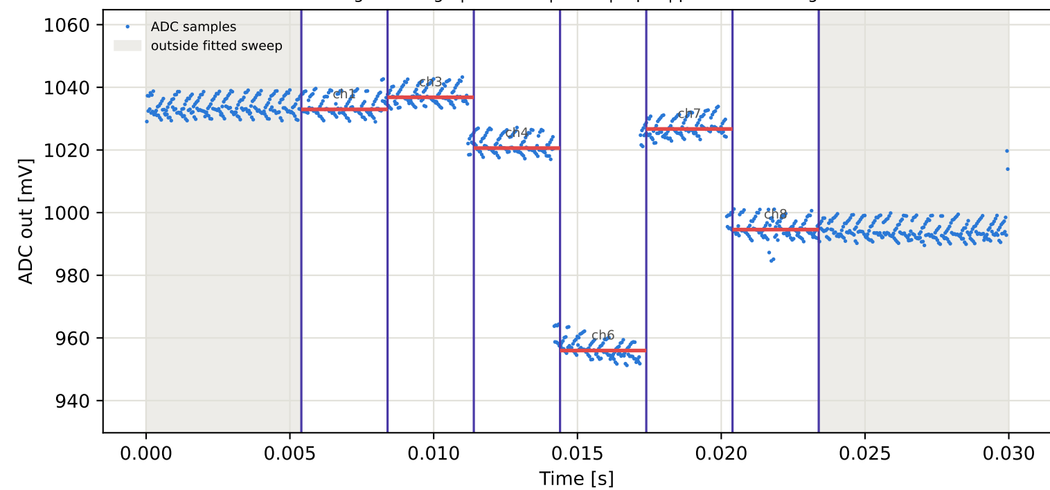
Tag2 &lt;- Tag10 | 915 MHz | run 0 | rep 1 | phase -23.26 deg
