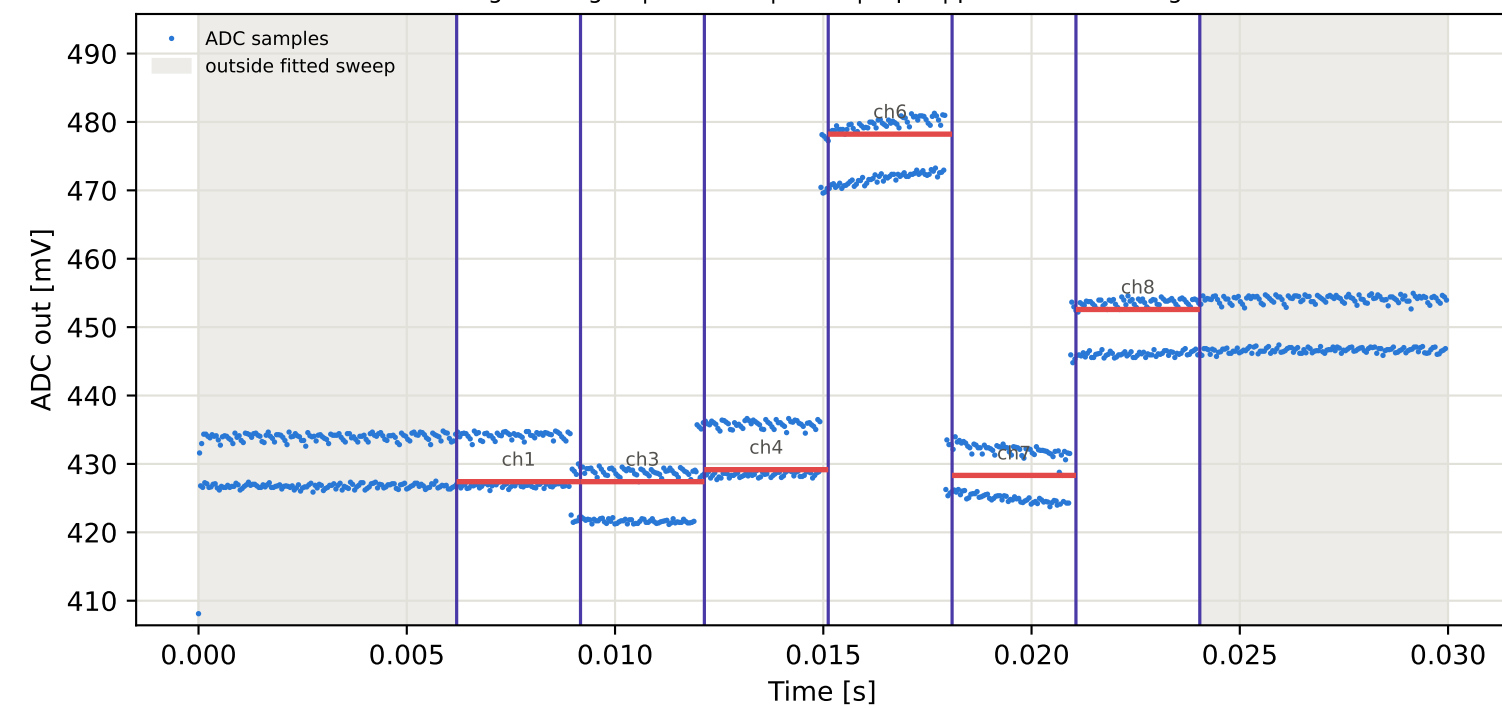
Tag1 &lt;- Tag16 | 935 MHz | run 0 | rep 1 | phase 18.73 deg
