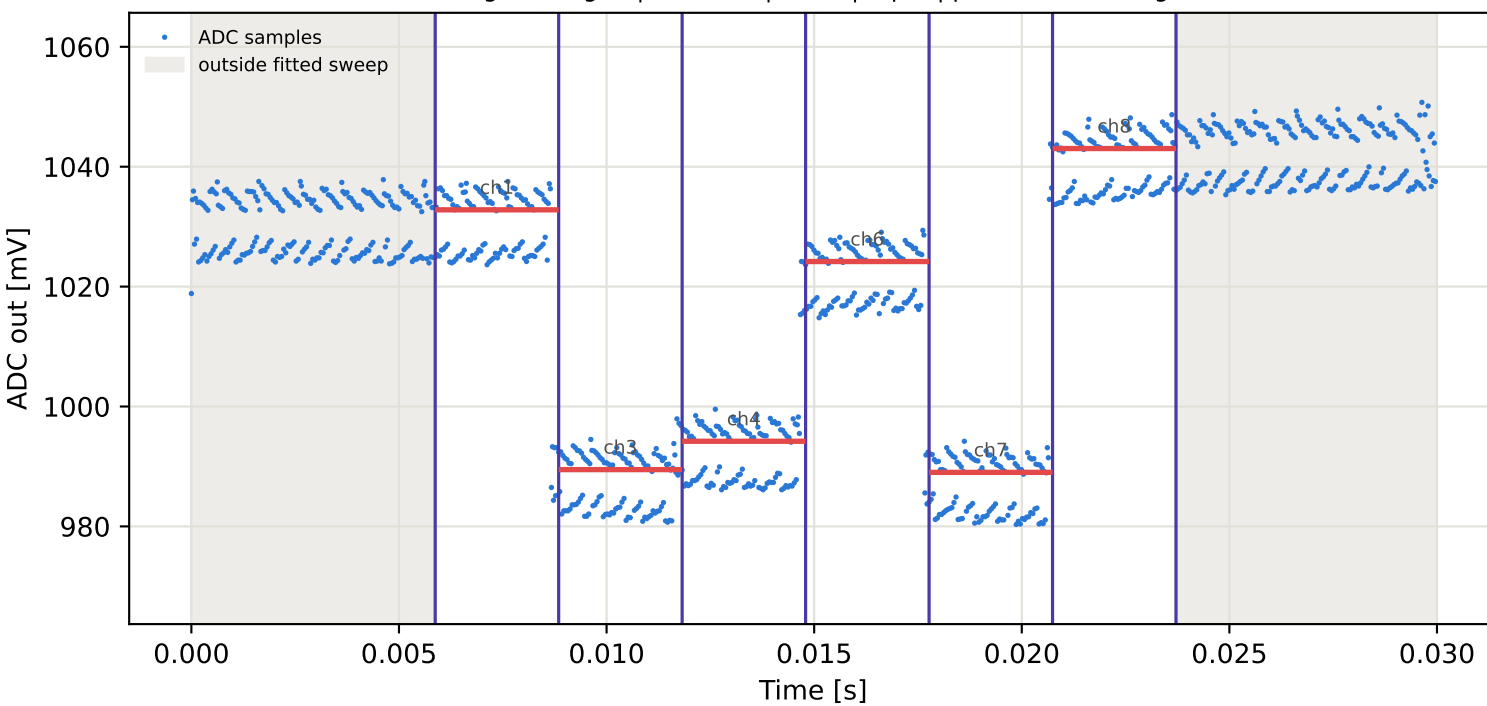
Tag8 &lt;- Tag15 | 865 MHz | run 0 | rep 1 | phase 133.22 deg
