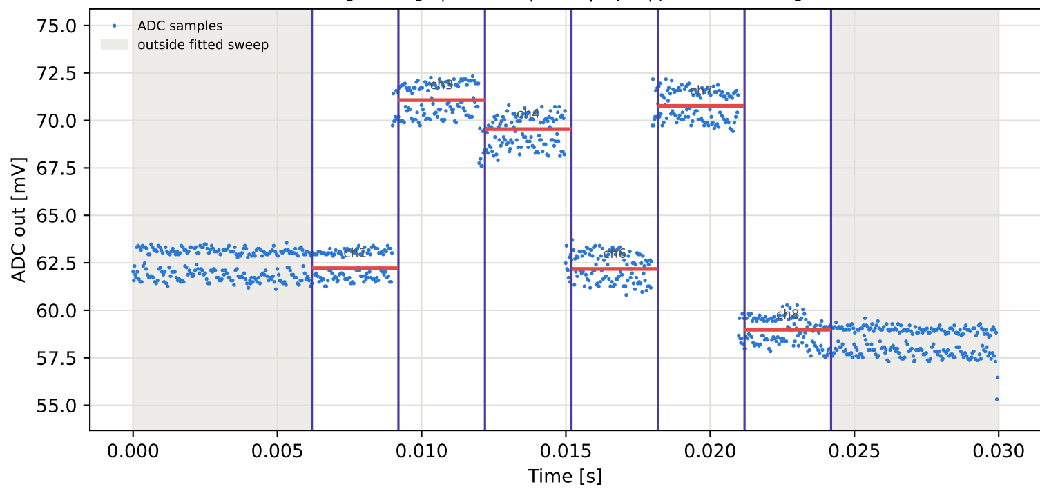
Tag2 &lt;- Tag8 | 845 MHz | run 0 | rep 1 | phase -36.86 deg
