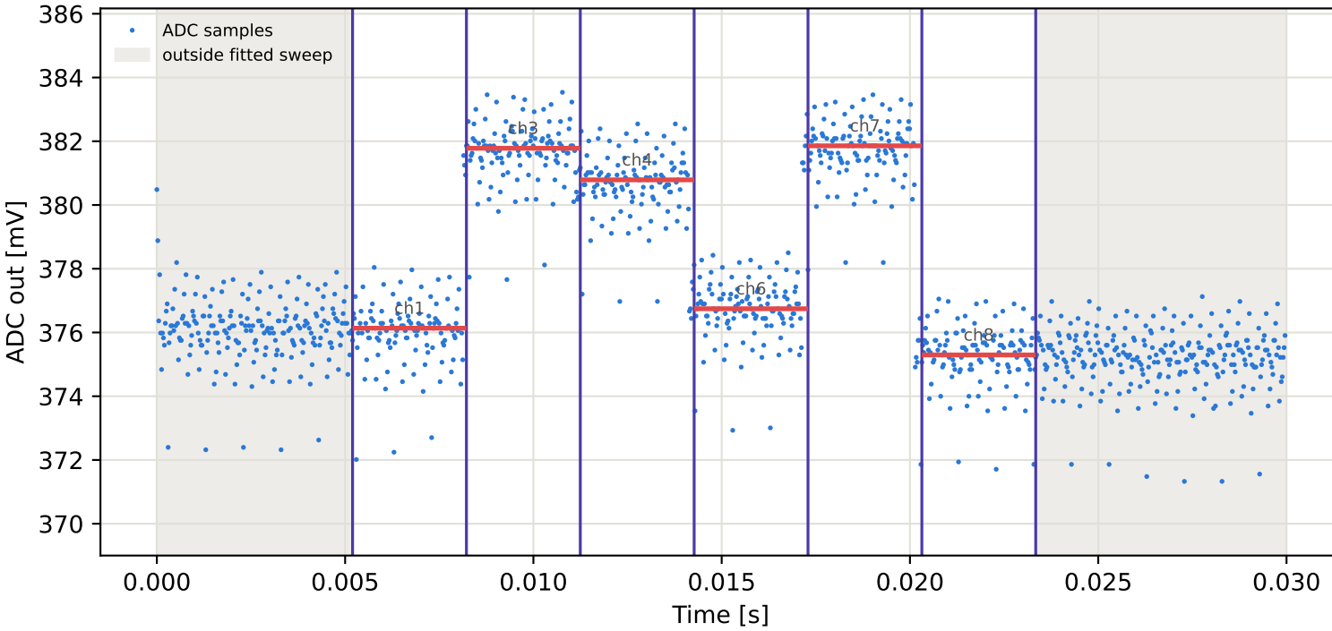
Tag3 &lt;- Tag16 | 835 MHz | run 0 | rep 1 | phase -10.29 deg
