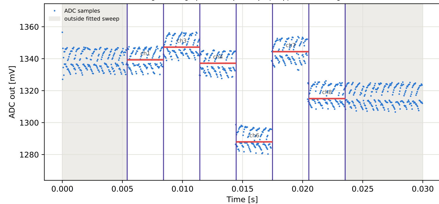
Tag15 &lt;- Tag5 | 955 MHz | run 0 | rep 1 | phase 1.29 deg
