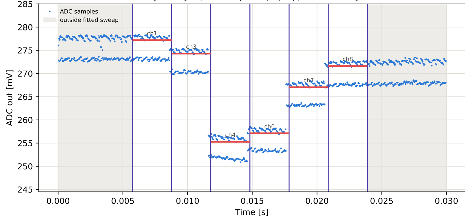
Tag6 &lt;- Tag10 | 975 MHz | run 0 | rep 1 | phase 47.14 deg
