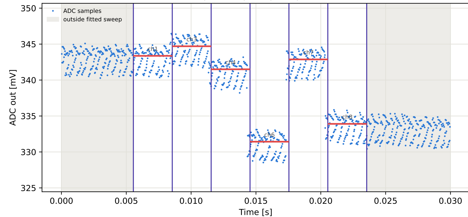
Tag2 &lt;- Tag7 | 895 MHz | run 0 | rep 1 | phase 6.87 deg
