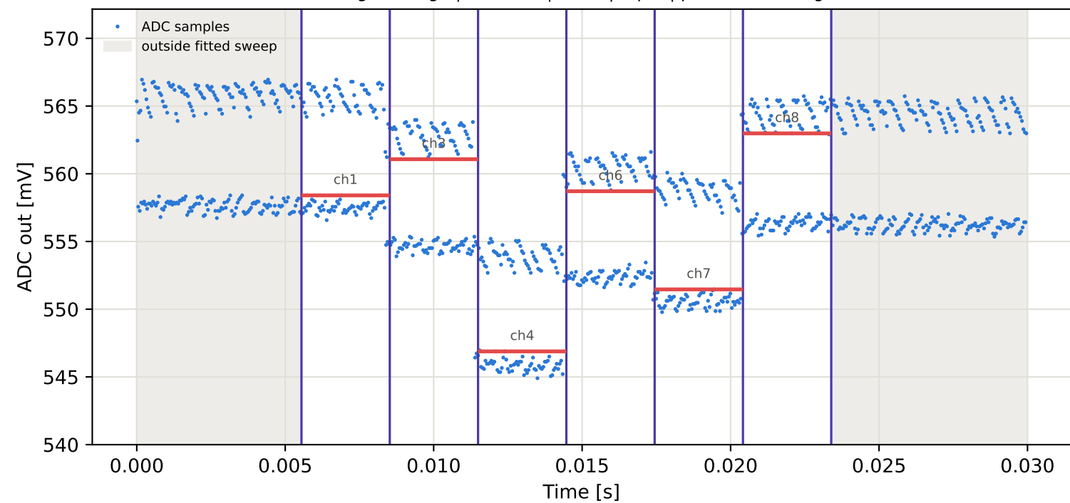
Tag8 &lt;- Tag7 | 995 MHz | run 0 | rep 1 | phase 76.64 deg
