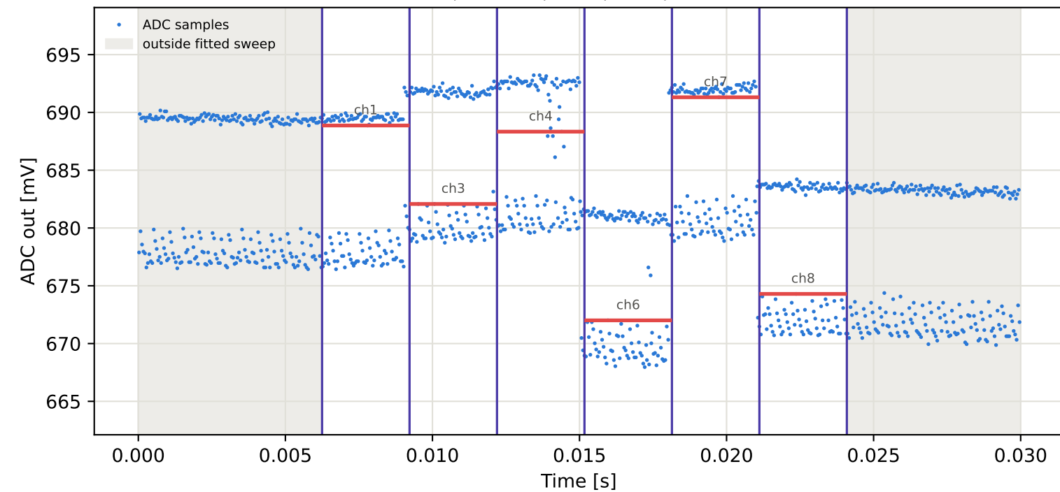
Tag3 &lt;- Tag2 | 915 MHz | run 0 | rep 1 | phase -18.10 deg
