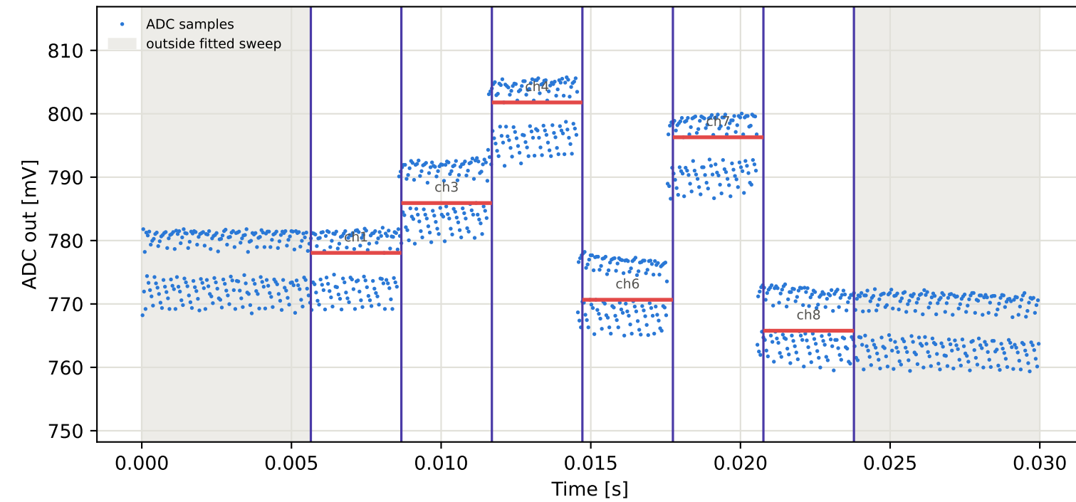
Tag3 &lt;- Tag8 | 935 MHz | run 0 | rep 1 | phase -15.95 deg
