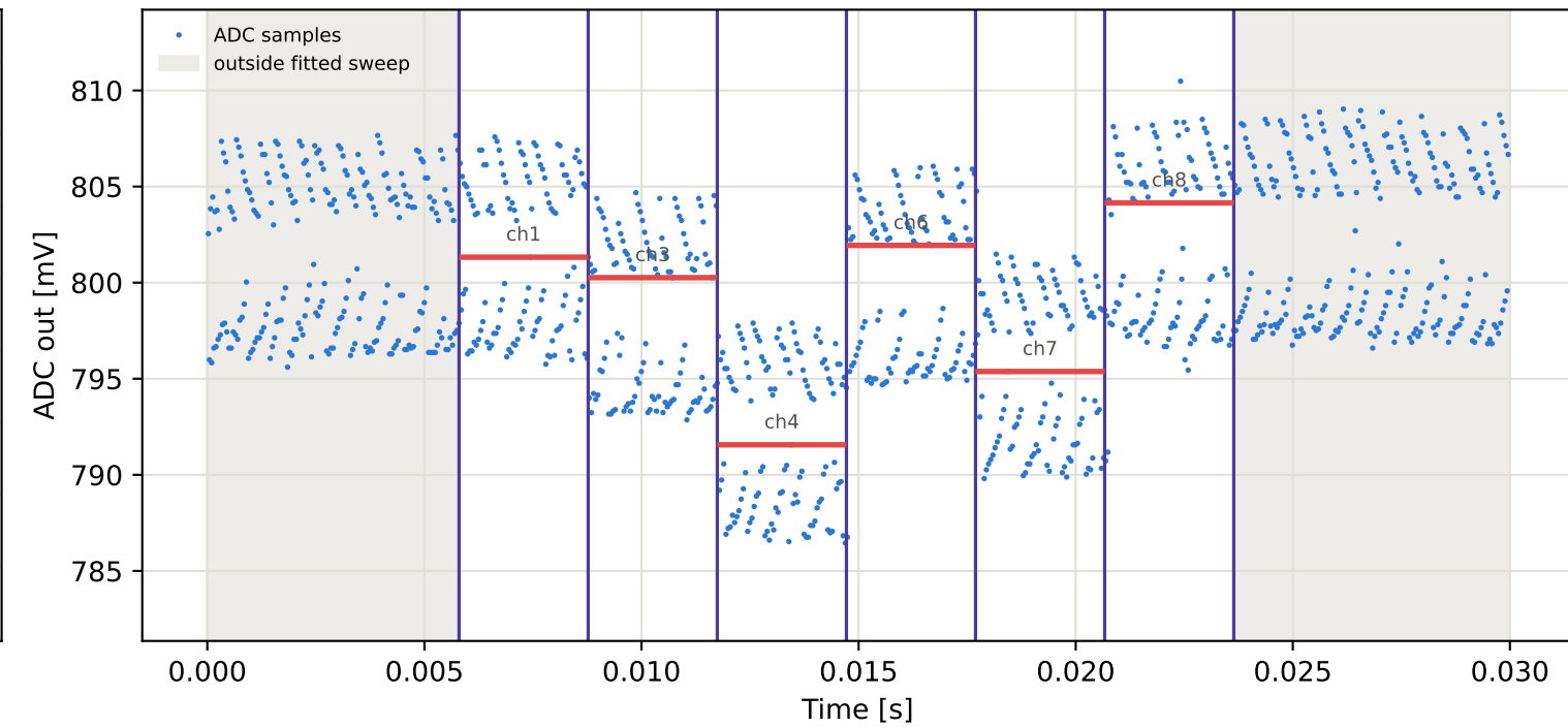
Tag8 &lt;- Tag7 | 985 MHz | run 0 | rep 1 | phase 51.60 deg
