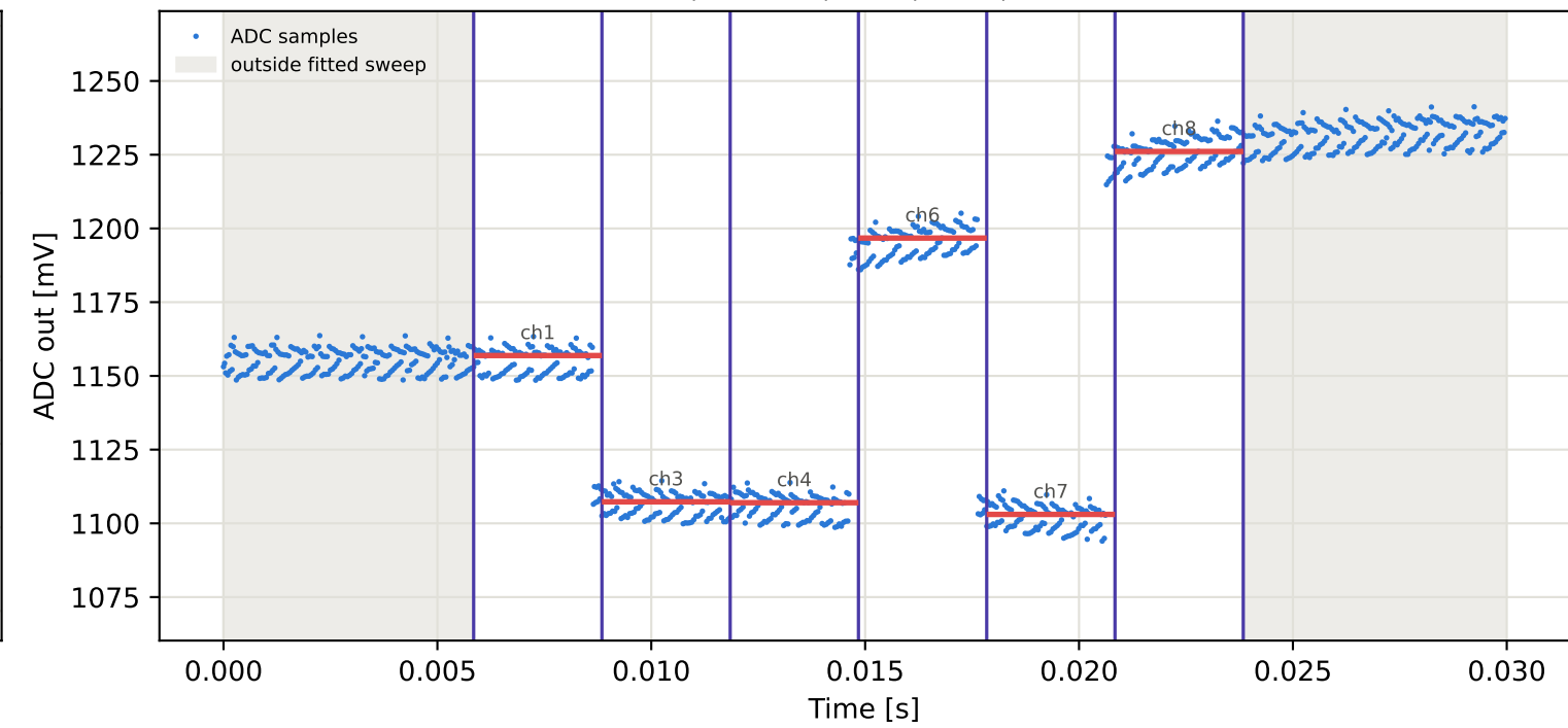
Tag16 &lt;- Tag15 | 895 MHz | run 0 | rep 1 | phase 149.69 deg
