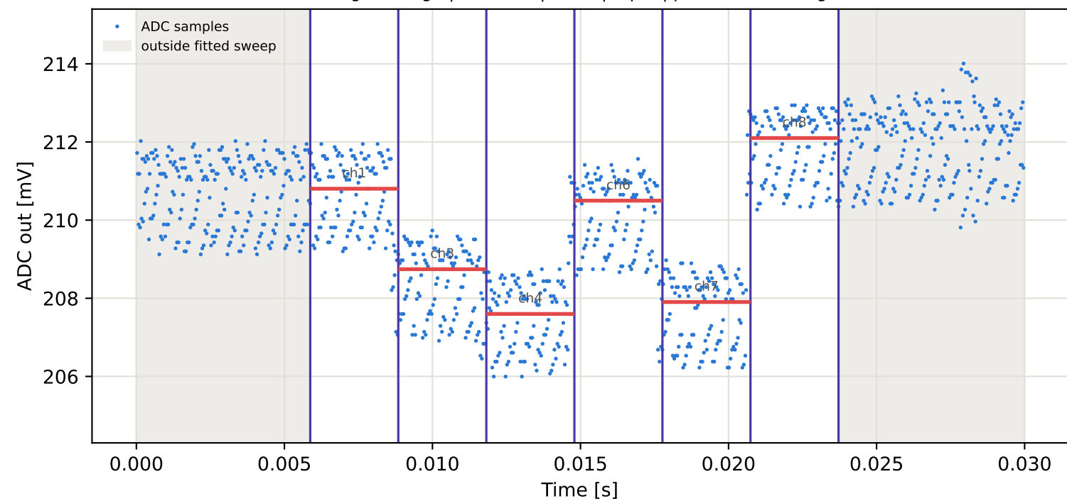
Tag9 &lt;- Tag2 | 805 MHz | run 0 | rep 1 | phase 122.44 deg
