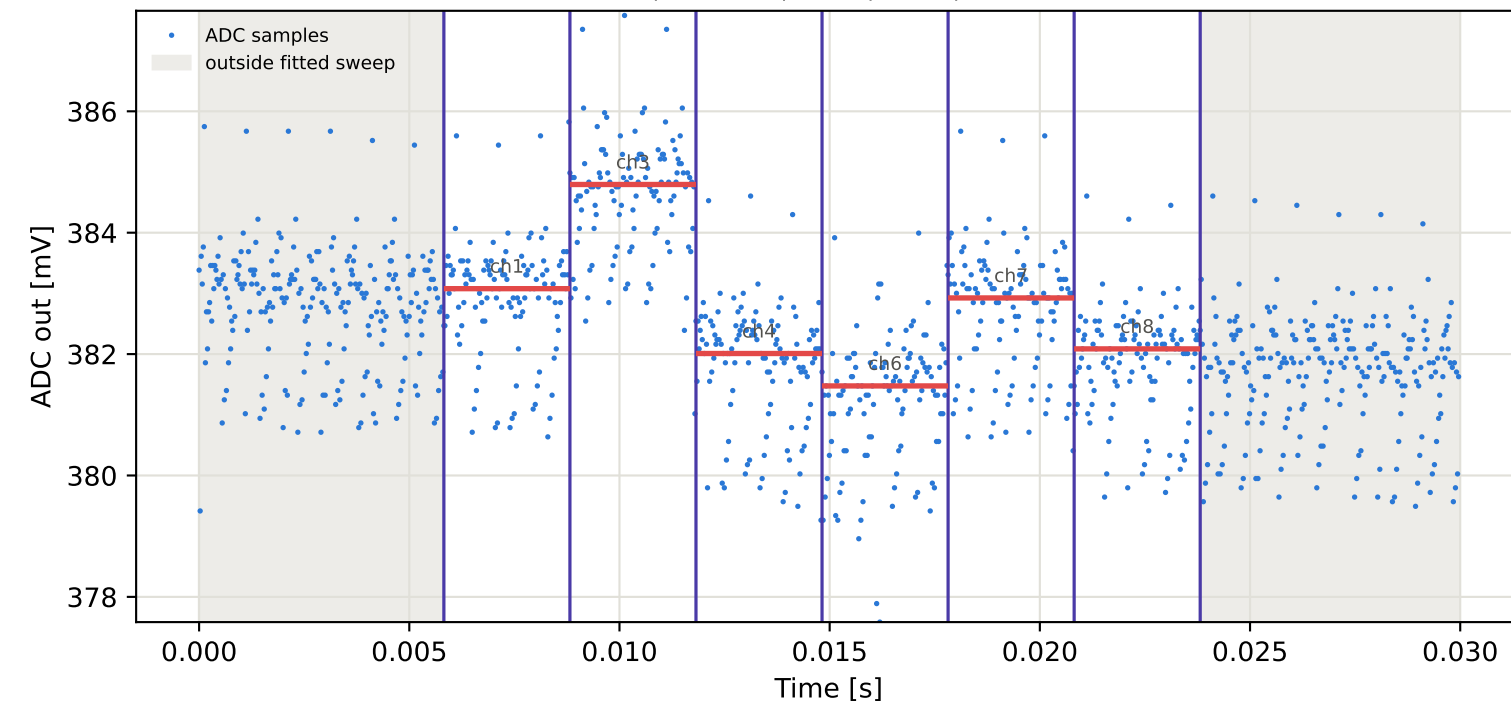
Tag6 &lt;- Tag1 | 825 MHz | run 0 | rep 1 | phase 35.34 deg
