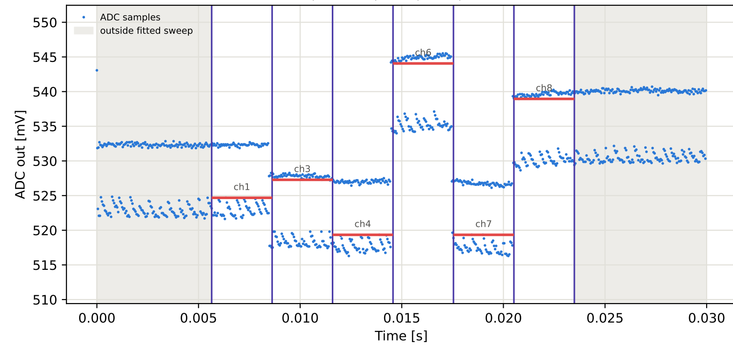
Tag7 &lt;- Tag5 | 945 MHz | run 0 | rep 1 | phase 152.48 deg
