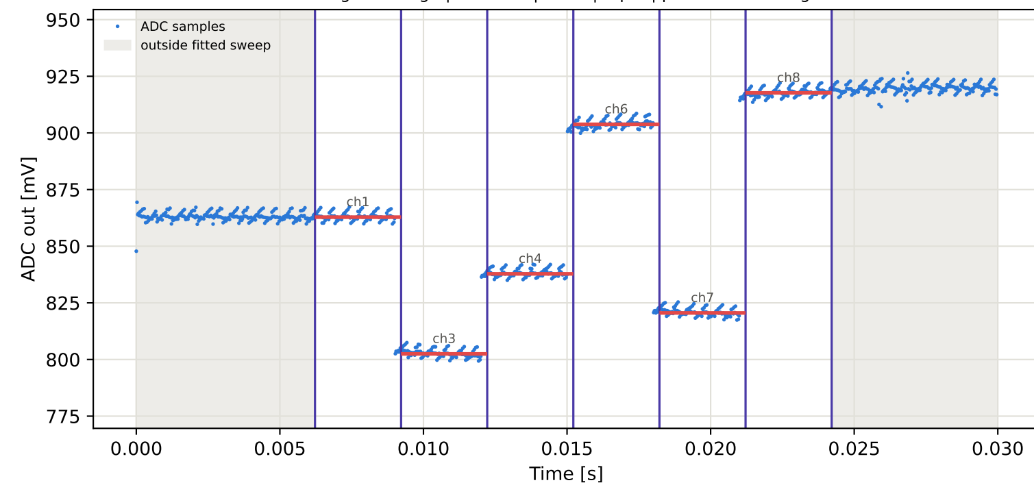
Tag2 &lt;- Tag1 | 855 MHz | run 0 | rep 1 | phase 51.68 deg
