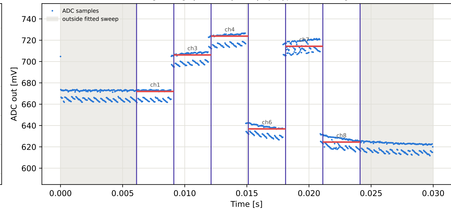
Tag9 &lt;- Tag6 | 915 MHz | run 0 | rep 1 | phase -109.76 deg
