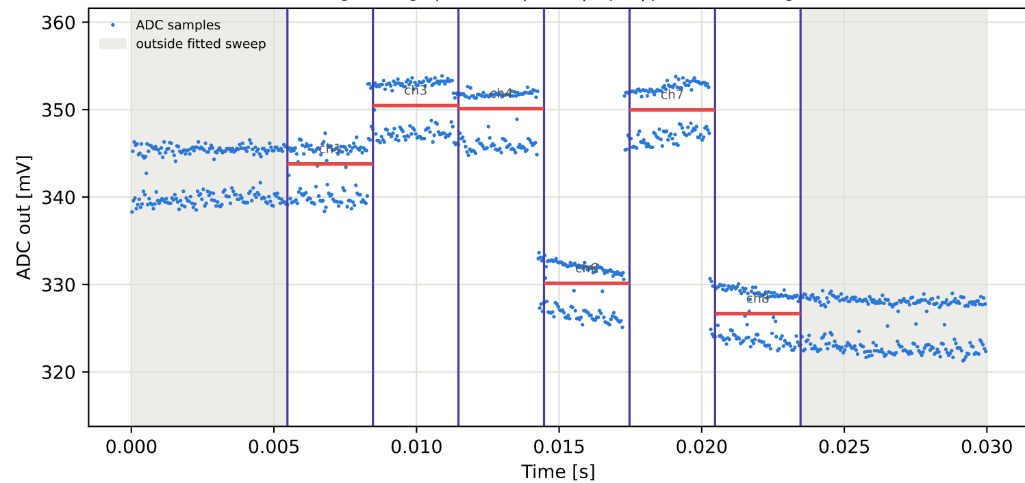
Tag2 &lt;- Tag6 | 885 MHz | run 0 | rep 1 | phase 170.42 deg
