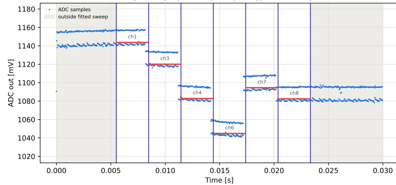
Tag15 &lt;- Tag3 | 885 MHz | run 0 | rep 1 | phase 136.58 deg
