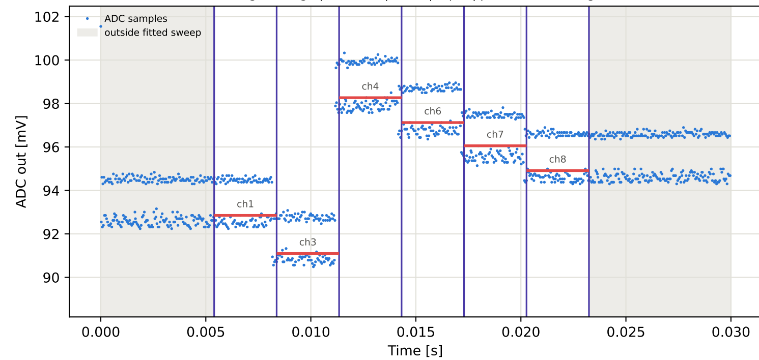
Tag8 &lt;- Tag10 | 775 MHz | run 0 | rep 1 | phase 128.64 deg
