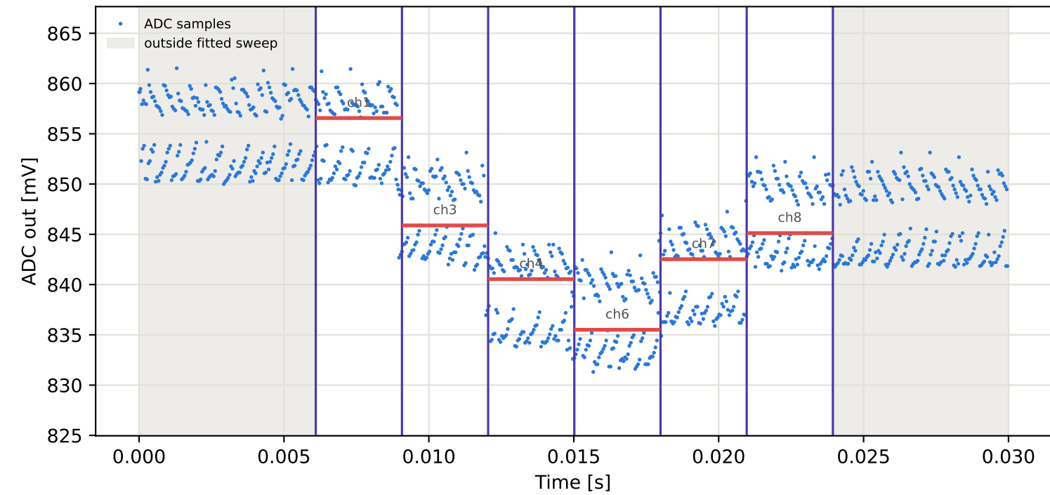
Tag16 &lt;- Tag7 | 865 MHz | run 0 | rep 1 | phase -127.04 deg
