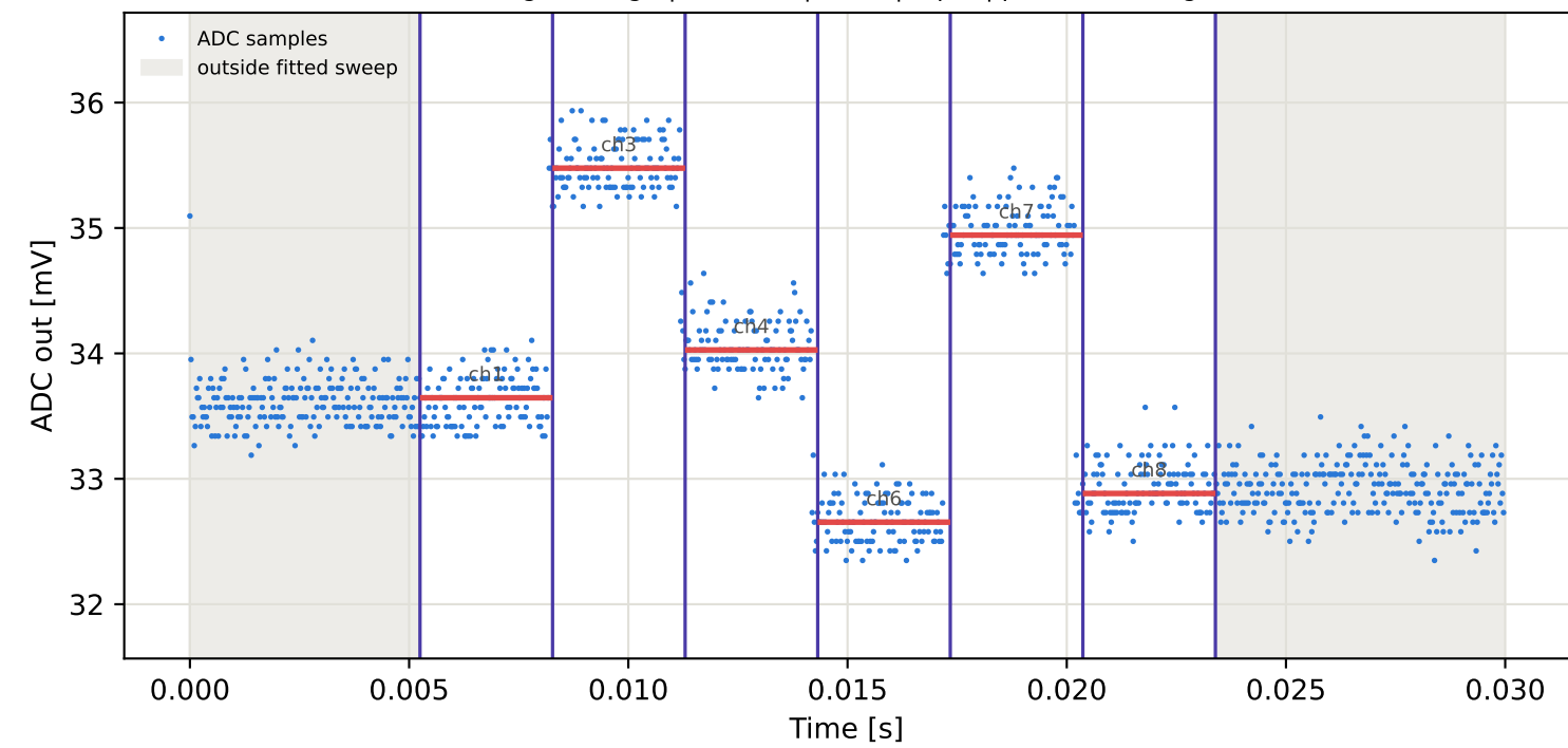
Tag1 &lt;- Tag8 | 775 MHz | run 0 | rep 1 | phase -125.99 deg
