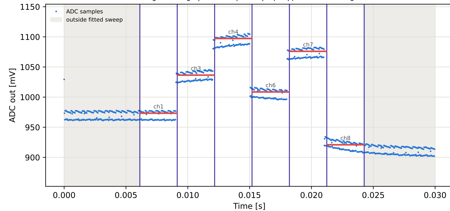
Tag2 &lt;- Tag1 | 915 MHz | run 0 | rep 1 | phase -122.63 deg
