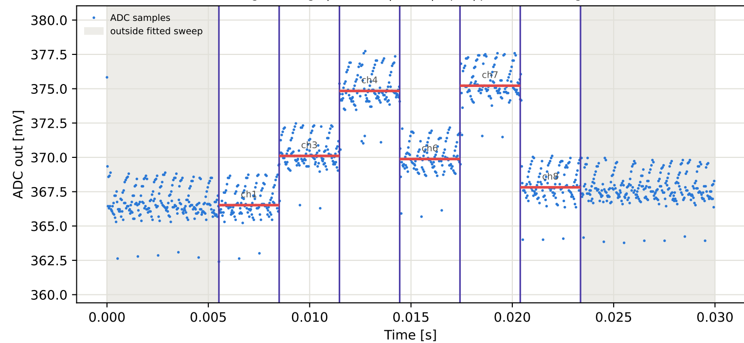
Tag16 &lt;- Tag1 | 805 MHz | run 0 | rep 1 | phase -49.25 deg
