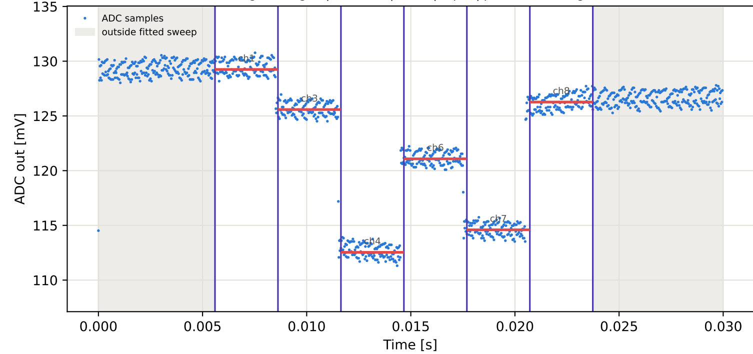
Tag5 &lt;- Tag2 | 805 MHz | run 0 | rep 1 | phase -13.98 deg
