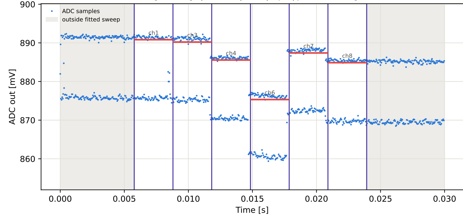
Tag16 &lt;- Tag5 | 925 MHz | run 0 | rep 1 | phase -15.12 deg
