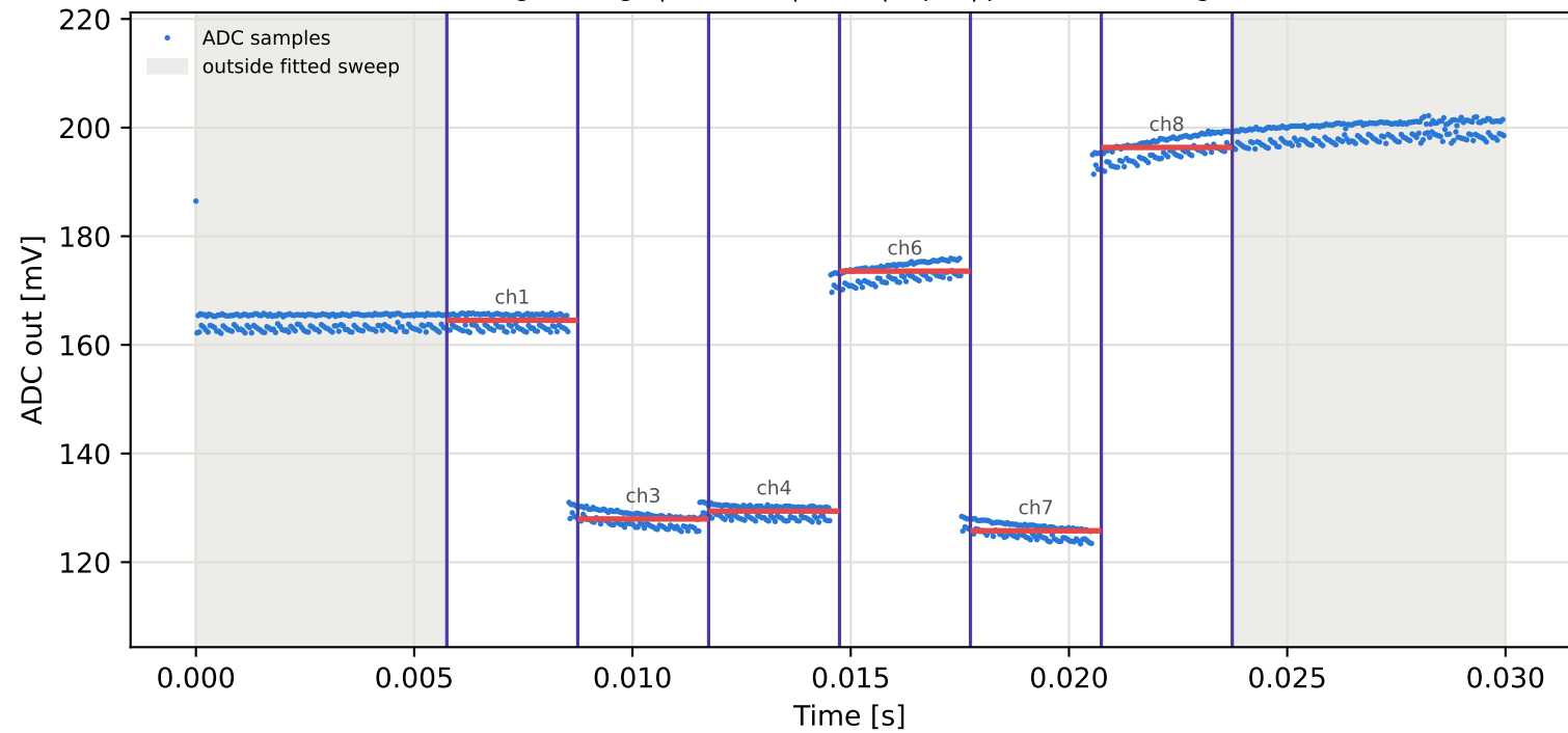
Tag1 &lt;- Tag8 | 875 MHz | run 0 | rep 1 | phase -52.90 deg
