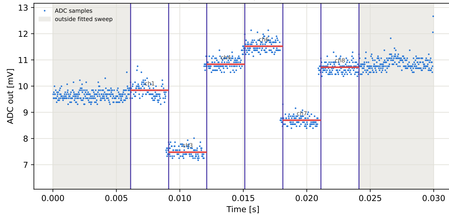
Tag10 &lt;- Tag4 | 775 MHz | run 0 | rep 1 | phase -148.52 deg
