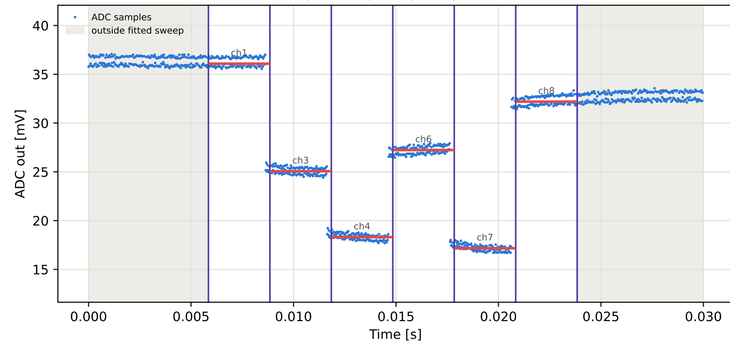
Tag1 &lt;- Tag3 | 825 MHz | run 0 | rep 1 | phase 100.95 deg
