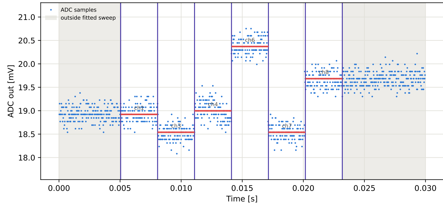
Tag2 &lt;- Tag8 | 975 MHz | run 0 | rep 1 | phase 111.71 deg
