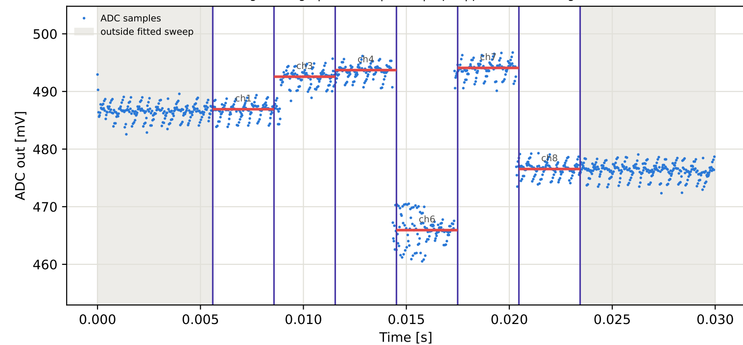
Tag5 &lt;- Tag3 | 955 MHz | run 0 | rep 1 | phase -16.34 deg
