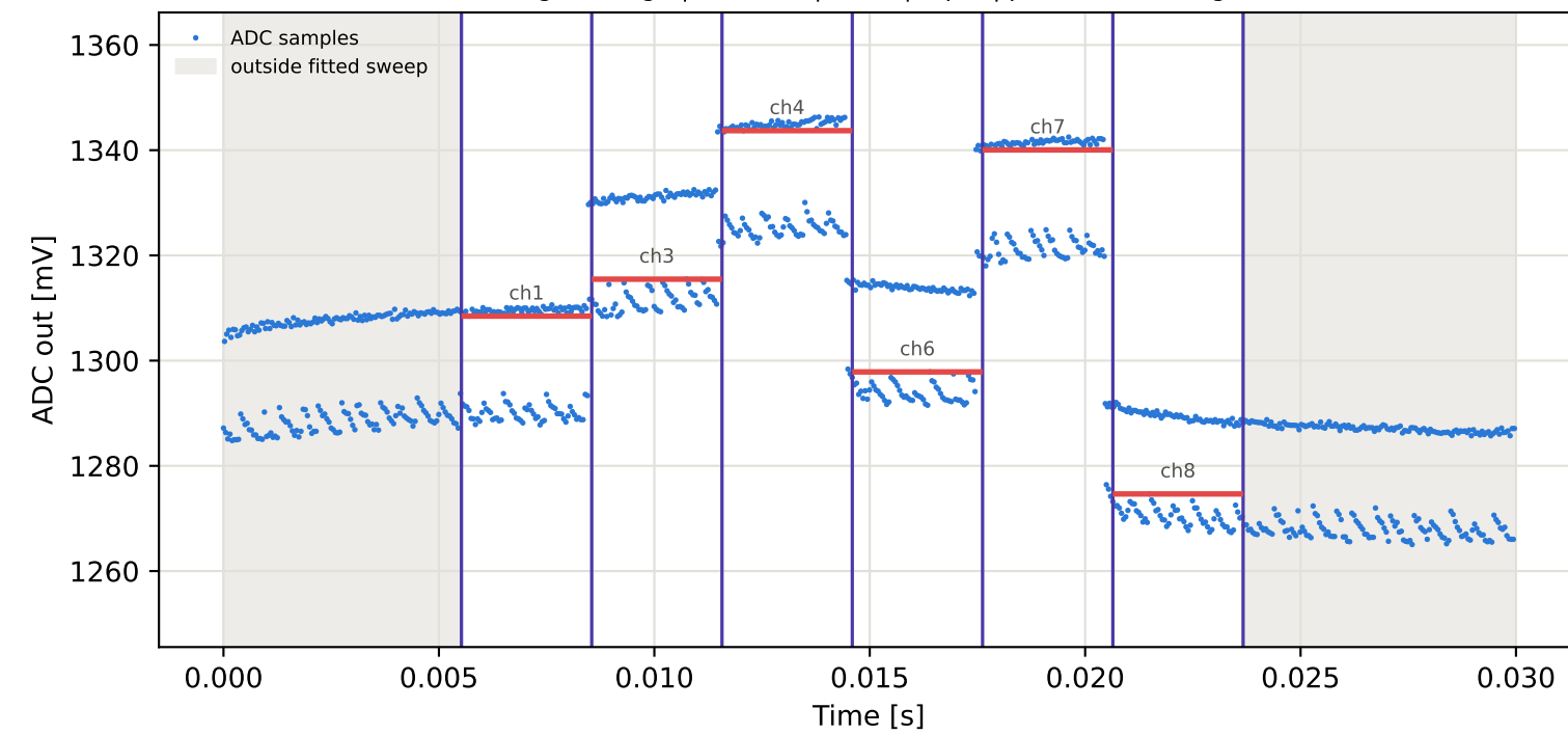
Tag5 &lt;- Tag8 | 905 MHz | run 0 | rep 1 | phase 163.13 deg
