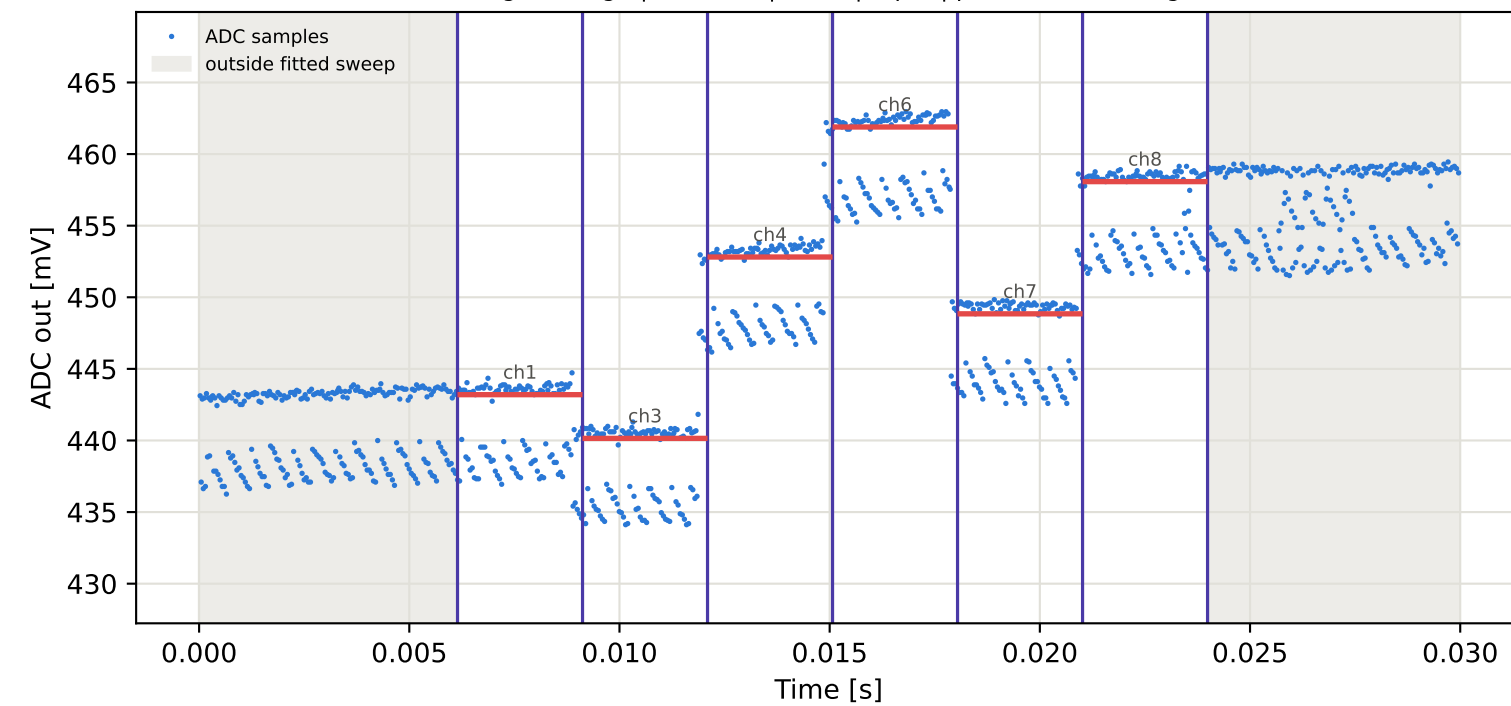
Tag5 &lt;- Tag8 | 855 MHz | run 0 | rep 1 | phase 46.61 deg
