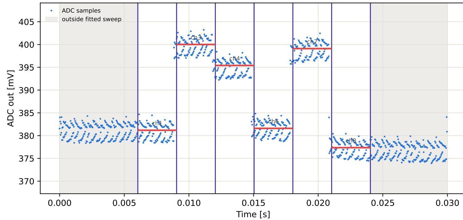
Tag6 &lt;- Tag1 | 835 MHz | run 0 | rep 1 | phase -48.54 deg
