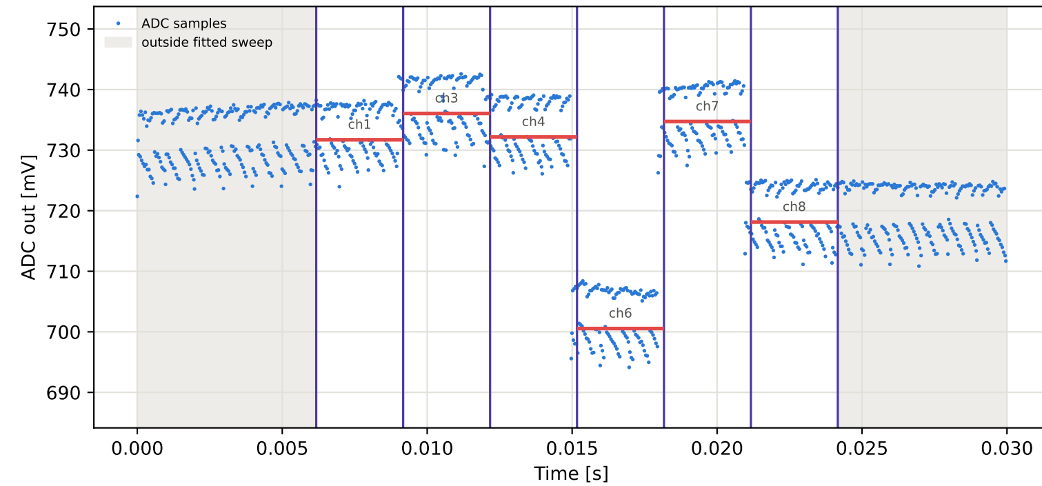
Tag9 &lt;- Tag16 | 935 MHz | run 0 | rep 1 | phase -39.51 deg
