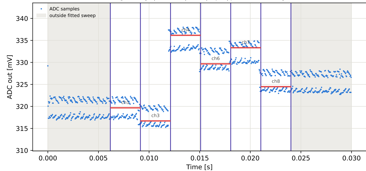
Tag8 &lt;- Tag5 | 805 MHz | run 0 | rep 1 | phase 104.14 deg
