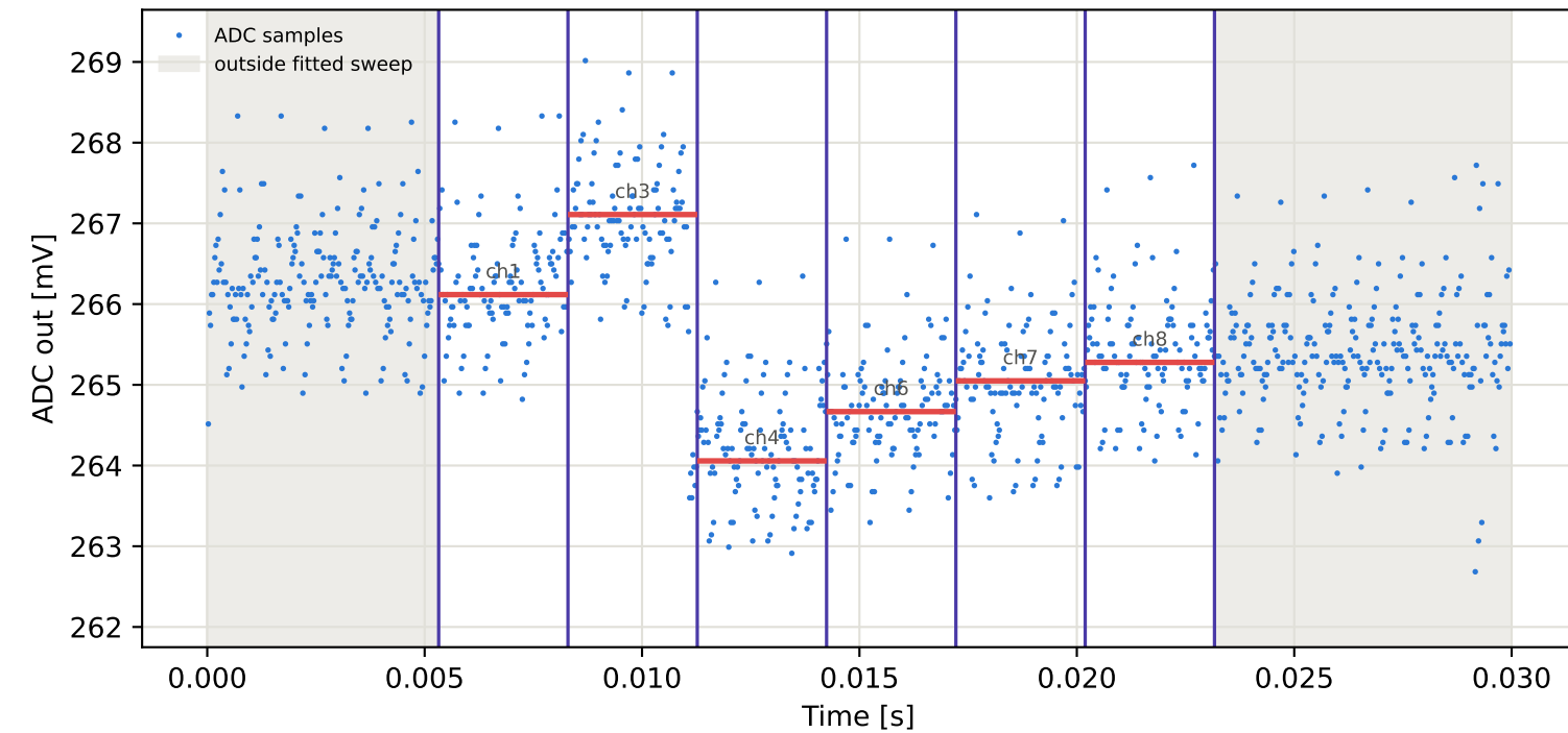
Tag15 &lt;- Tag5 | 795 MHz | run 0 | rep 1 | phase 85.88 deg
