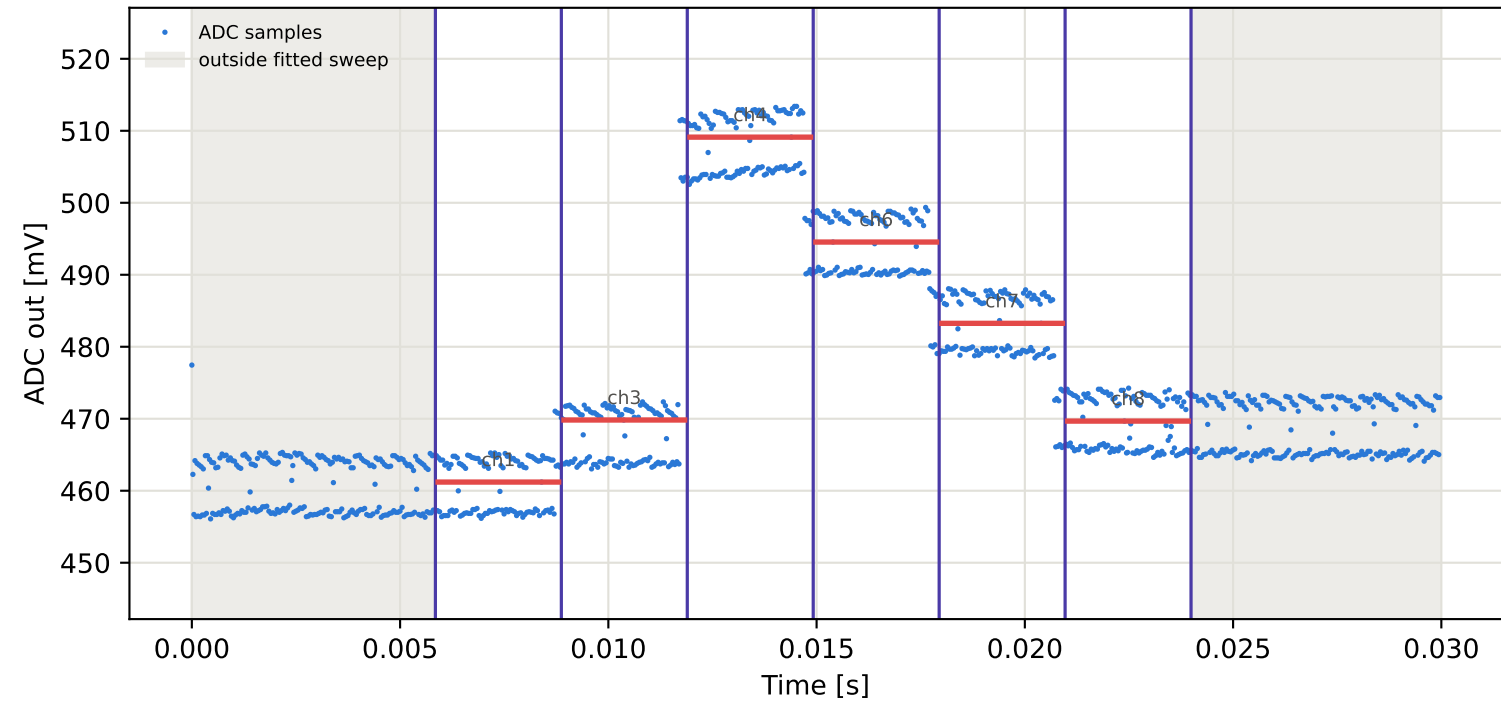
Tag4 &lt;- Tag3 | 975 MHz | run 0 | rep 1 | phase -127.43 deg
