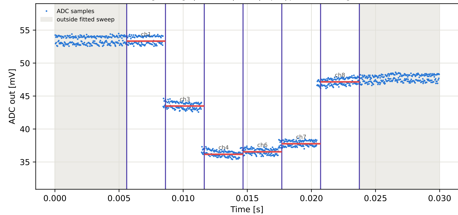
Tag2 &lt;- Tag6 | 865 MHz | run 0 | rep 1 | phase -17.17 deg
