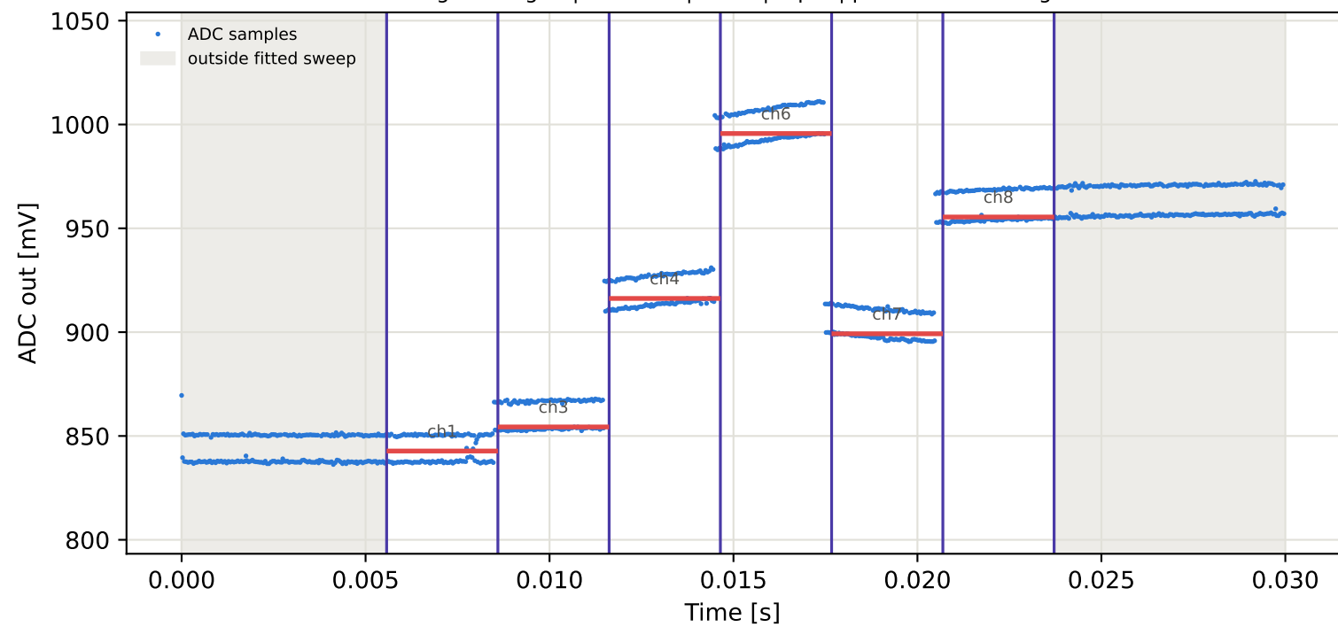
Tag5 &lt;- Tag2 | 885 MHz | run 0 | rep 1 | phase 77.83 deg
