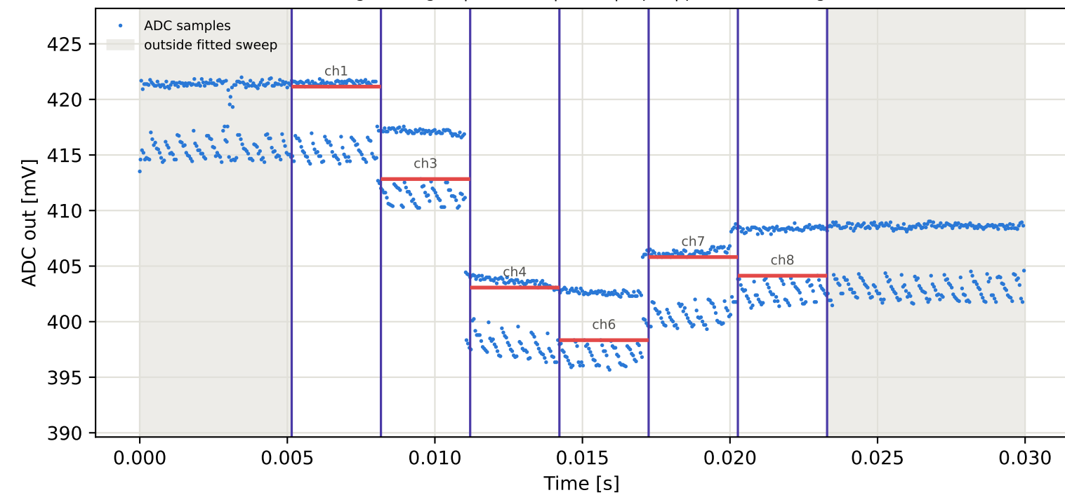
Tag6 &lt;- Tag2 | 855 MHz | run 0 | rep 1 | phase 155.21 deg
