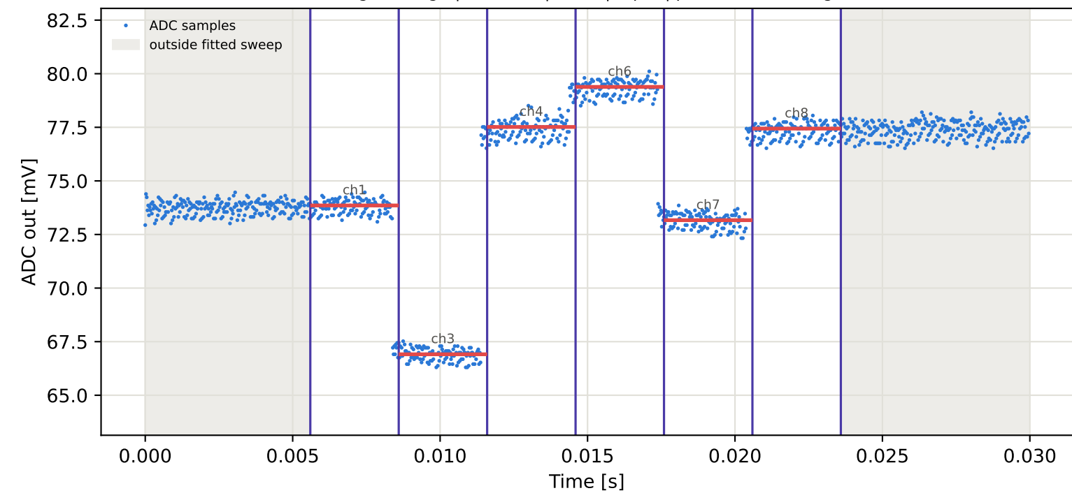
Tag3 &lt;- Tag6 | 795 MHz | run 0 | rep 1 | phase -2.02 deg
