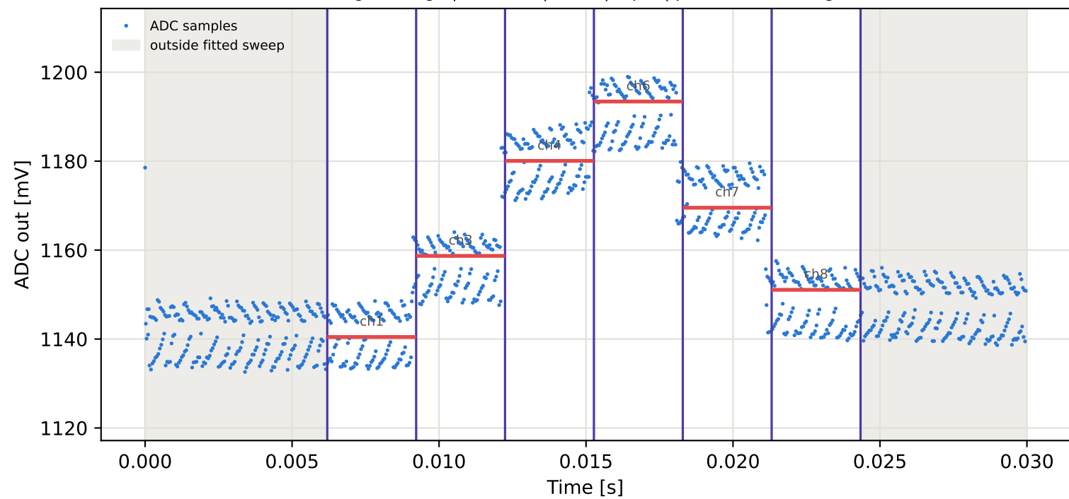
Tag7 &lt;- Tag1 | 915 MHz | run 0 | rep 1 | phase 21.82 deg
