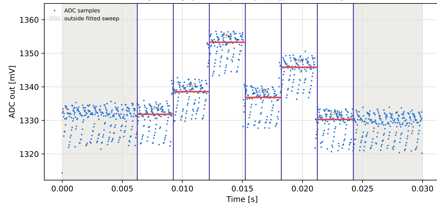
Tag15 &lt;- Tag9 | 955 MHz | run 0 | rep 1 | phase -55.89 deg
