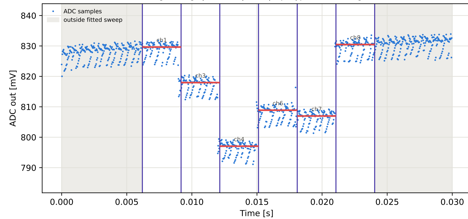
Tag9 &lt;- Tag10 | 935 MHz | run 0 | rep 1 | phase 2.34 deg
