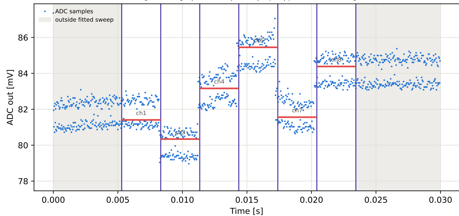
Tag15 &lt;- Tag10 | 825 MHz | run 0 | rep 1 | phase 145.15 deg
