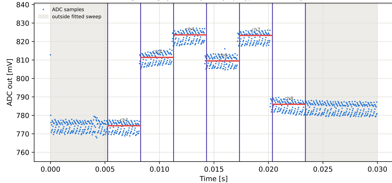
Tag3 &lt;- Tag15 | 865 MHz | run 0 | rep 1 | phase -80.02 deg
