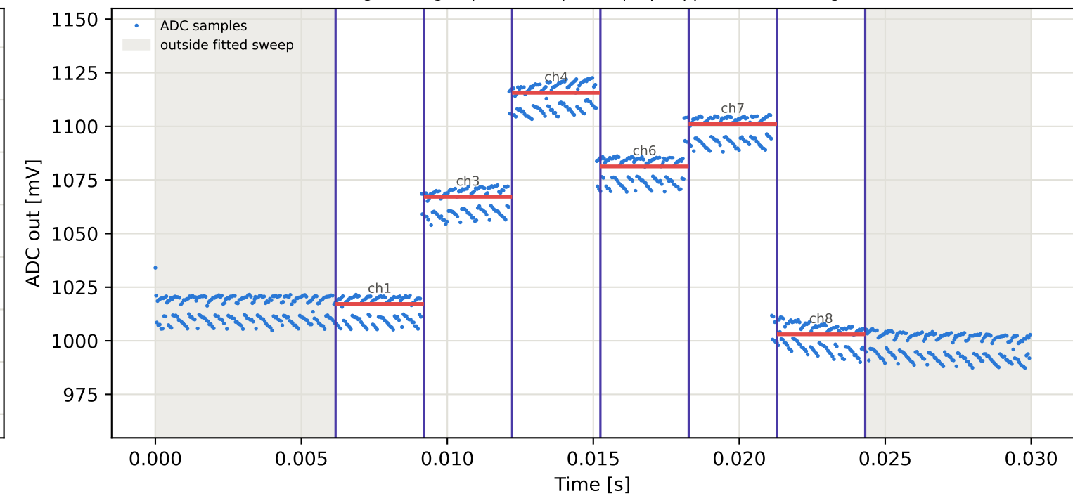
Tag5 &lt;- Tag2 | 915 MHz | run 0 | rep 1 | phase -30.67 deg
