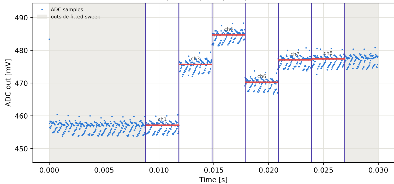
Tag4 &lt;- Tag8 | 855 MHz | run 0 | rep 1 | phase -152.10 deg
