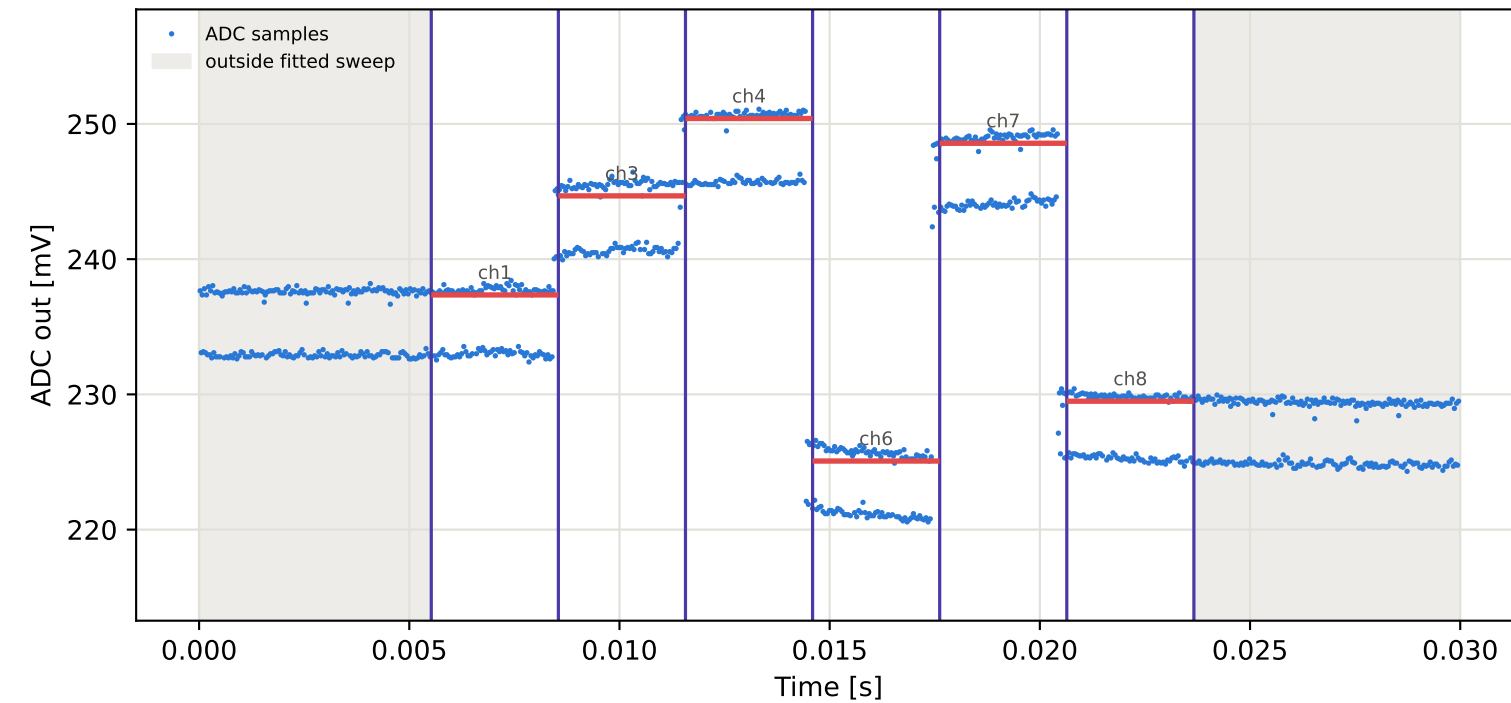
Tag15 &lt;- Tag1 | 975 MHz | run 0 | rep 1 | phase 175.49 deg
