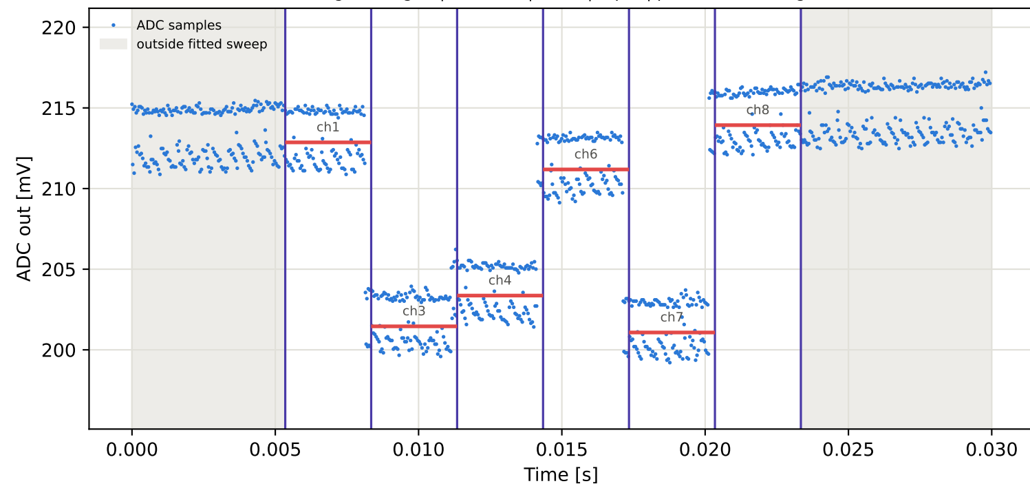
Tag4 &lt;- Tag16 | 835 MHz | run 0 | rep 1 | phase -91.88 deg
