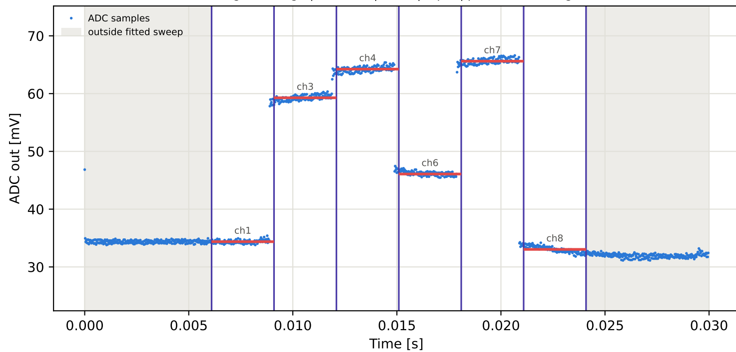
Tag10 &lt;- Tag8 | 855 MHz | run 0 | rep 1 | phase -85.37 deg
