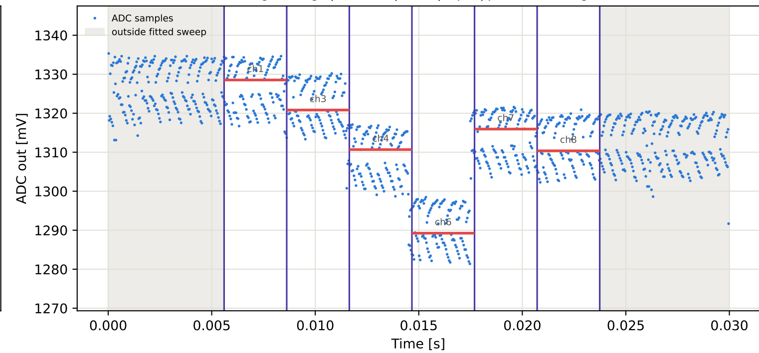
Tag5 &lt;- Tag9 | 905 MHz | run 0 | rep 1 | phase 177.92 deg
