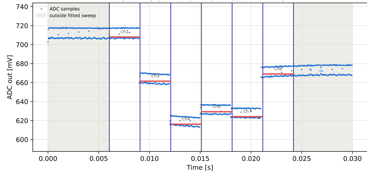
Tag16 &lt;- Tag1 | 855 MHz | run 0 | rep 1 | phase 169.40 deg
