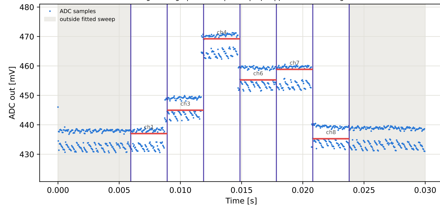
Tag4 &lt;- Tag15 | 965 MHz | run 0 | rep 1 | phase 136.73 deg
