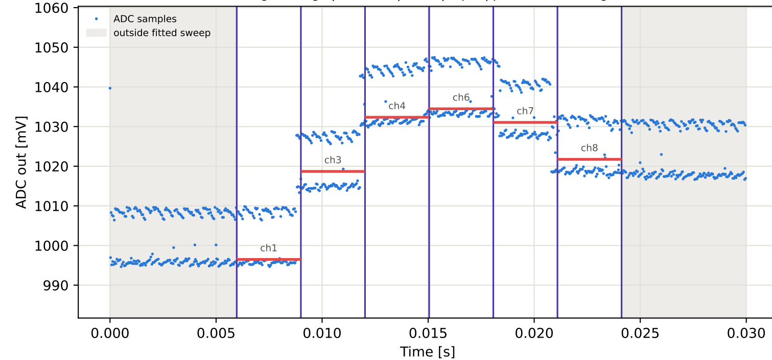
Tag8 &lt;- Tag6 | 855 MHz | run 0 | rep 1 | phase 143.63 deg
