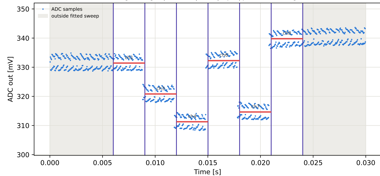
Tag6 &lt;- Tag2 | 935 MHz | run 0 | rep 1 | phase -73.52 deg
