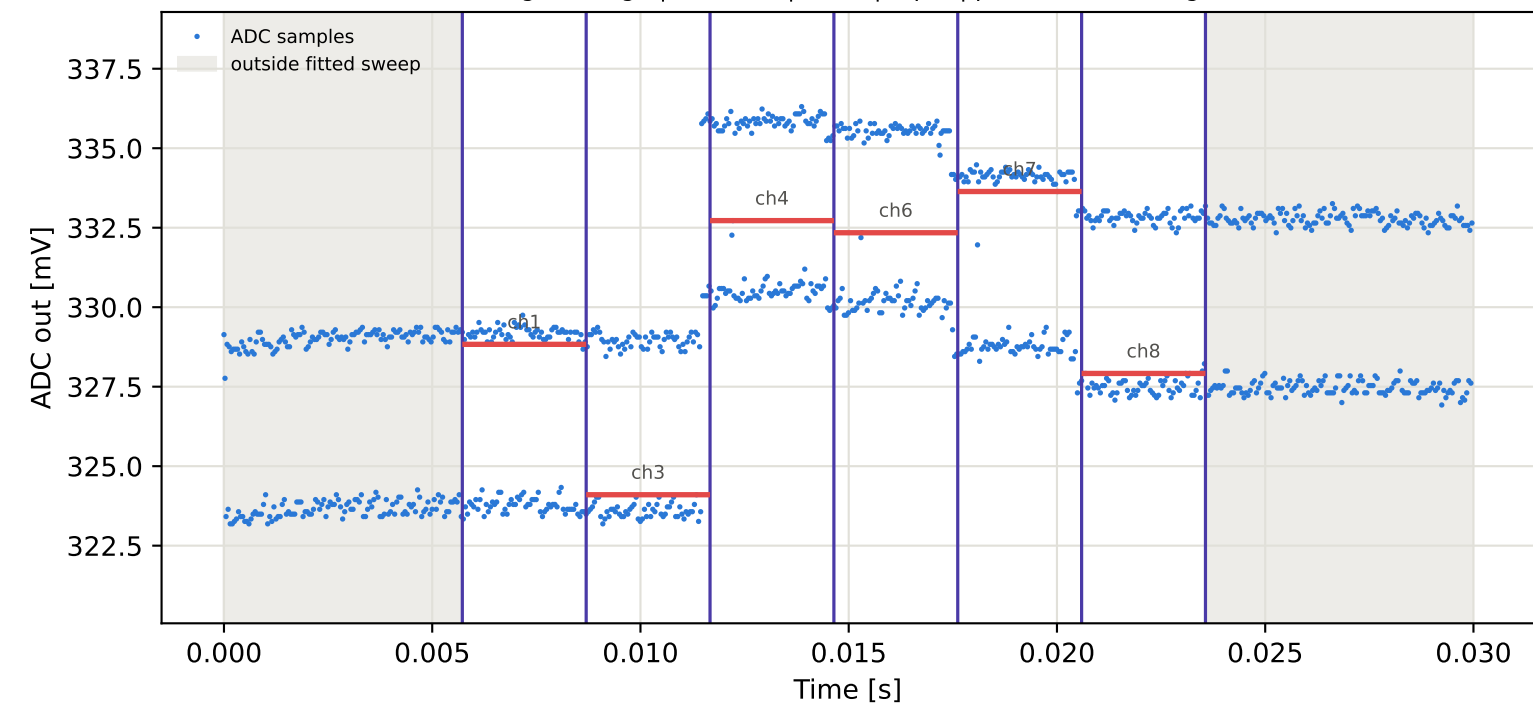
Tag9 &lt;- Tag10 | 805 MHz | run 0 | rep 1 | phase -54.19 deg
