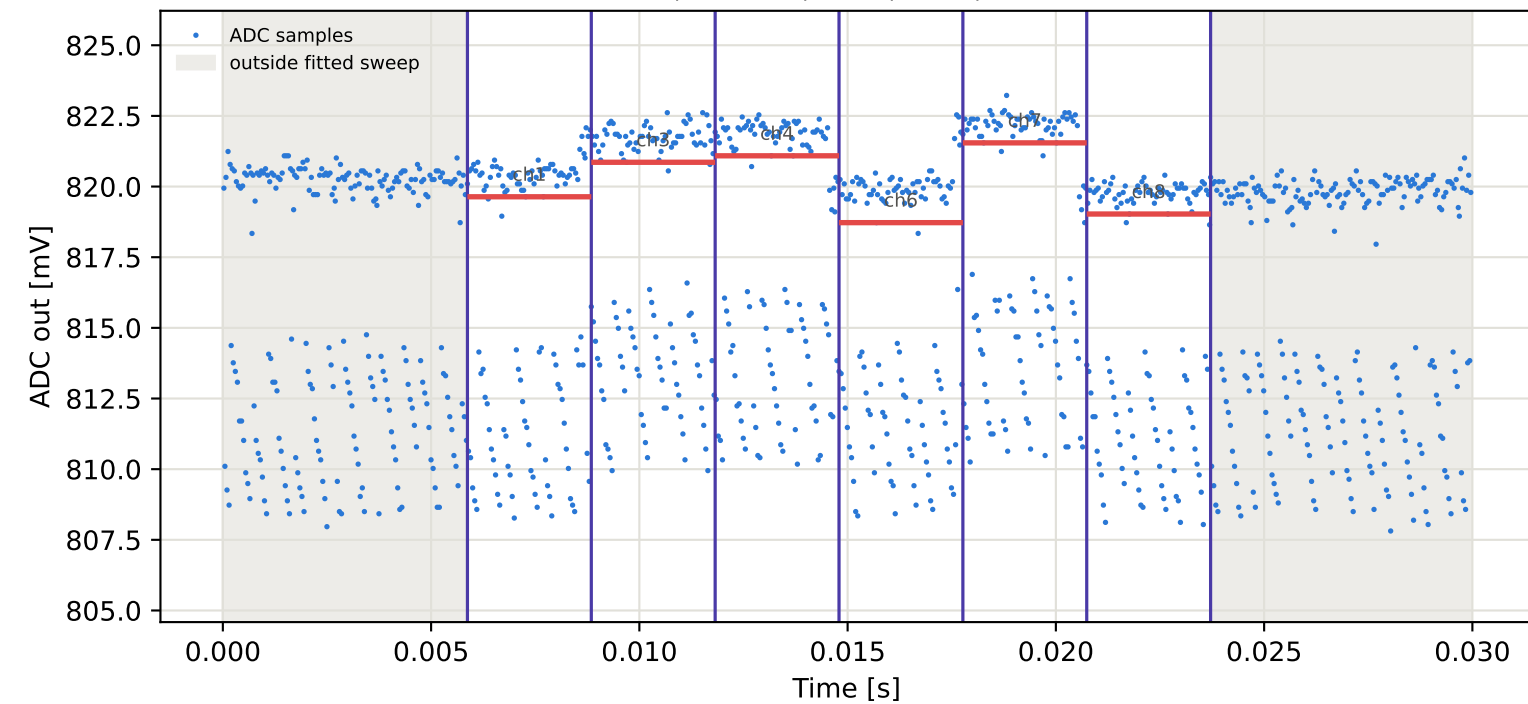
Tag16 &lt;- Tag7 | 845 MHz | run 0 | rep 1 | phase -30.50 deg
