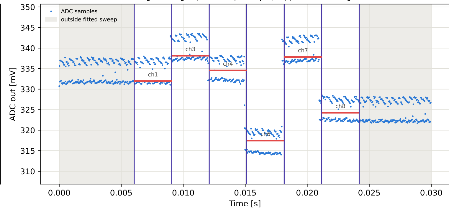
Tag10 &lt;- Tag3 | 985 MHz | run 0 | rep 1 | phase 6.08 deg
