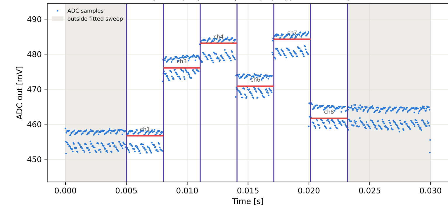
Tag4 &lt;- Tag2 | 855 MHz | run 0 | rep 1 | phase 21.38 deg
