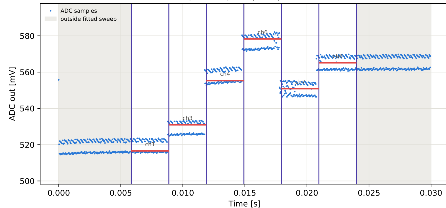
Tag3 &lt;- Tag6 | 855 MHz | run 0 | rep 1 | phase 131.04 deg
