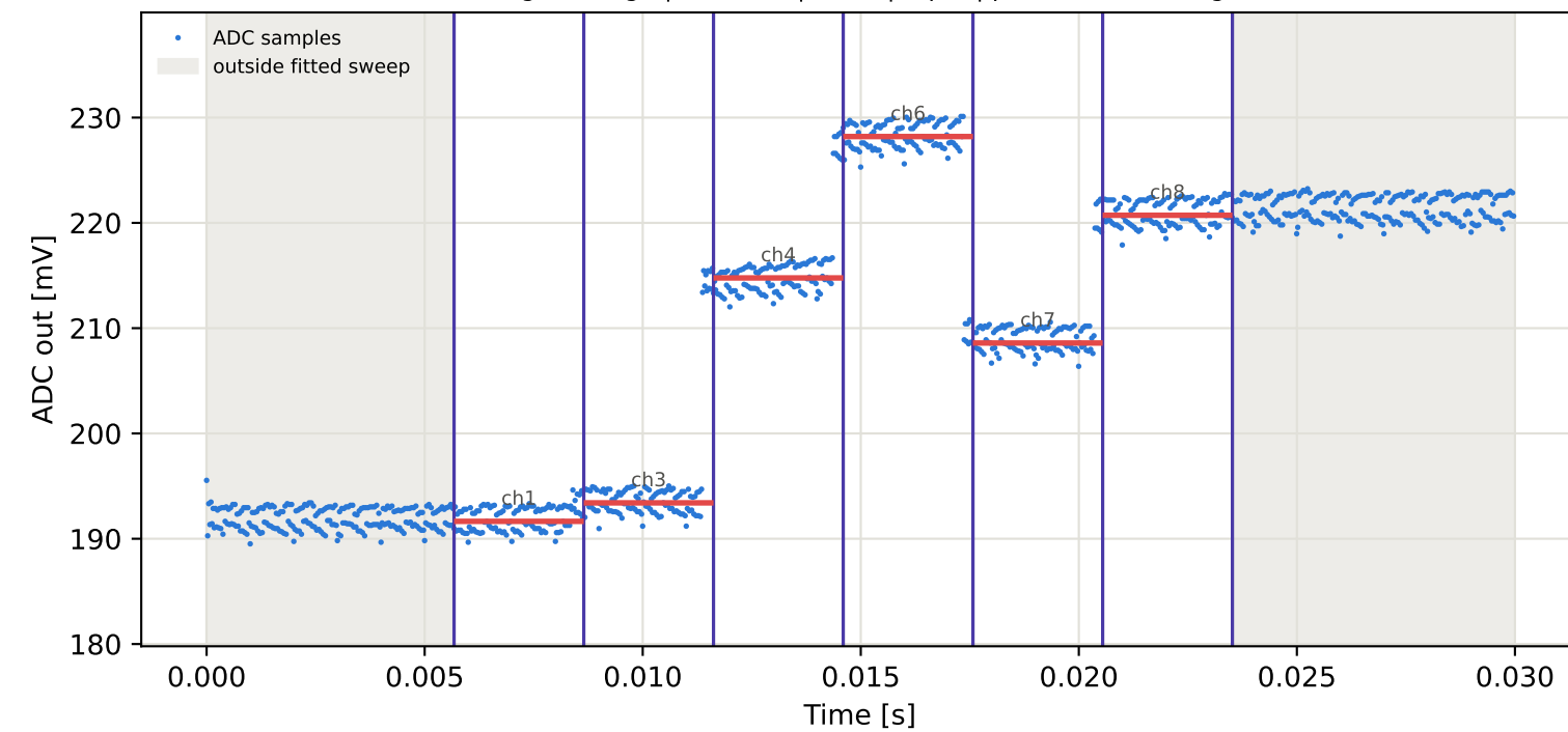
Tag9 &lt;- Tag5 | 855 MHz | run 0 | rep 1 | phase 152.14 deg
