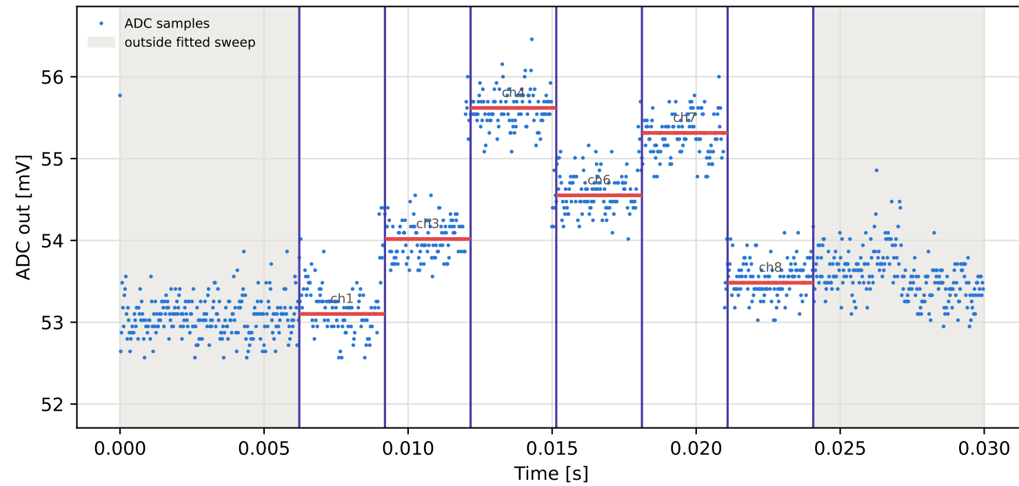
Tag10 &lt;- Tag4 | 785 MHz | run 0 | rep 1 | phase -99.78 deg
