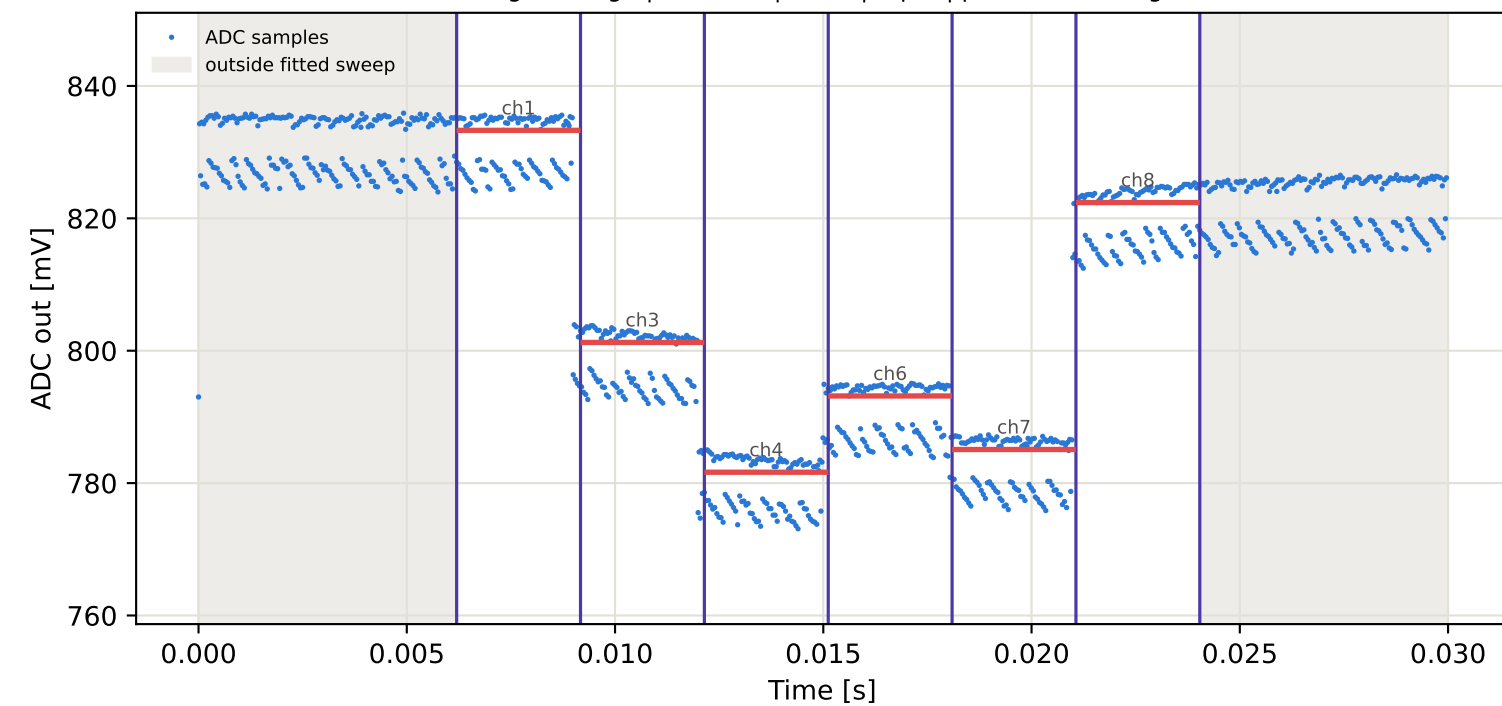
Tag5 &lt;- Tag3 | 865 MHz | run 0 | rep 1 | phase 79.73 deg
