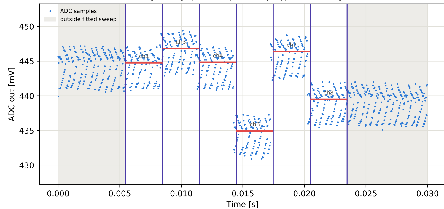
Tag5 &lt;- Tag1 | 935 MHz | run 0 | rep 1 | phase -0.85 deg
