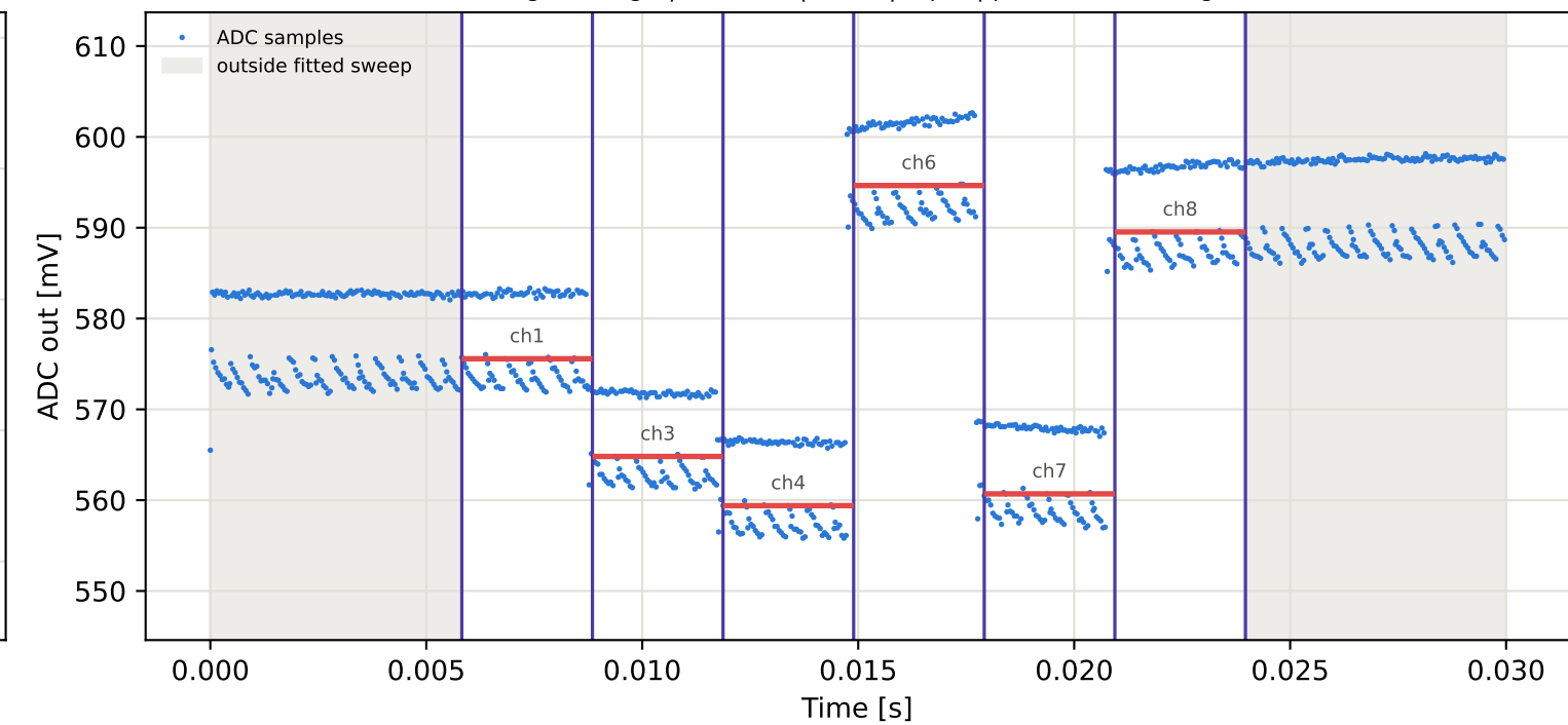
Tag9 &lt;- Tag15 | 965 MHz | run 0 | rep 1 | phase -69.87 deg
