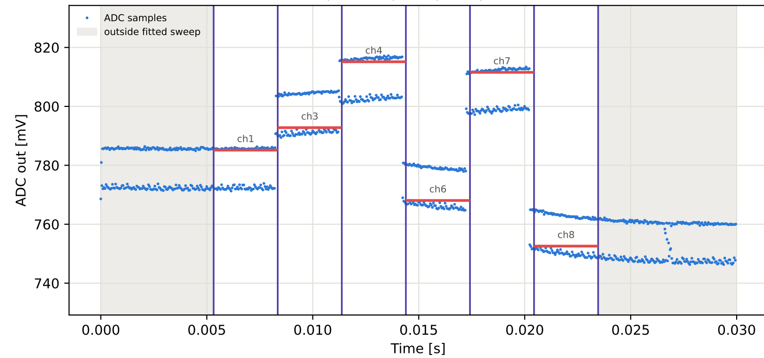
Tag1 &lt;- Tag9 | 915 MHz | run 0 | rep 1 | phase -53.93 deg
