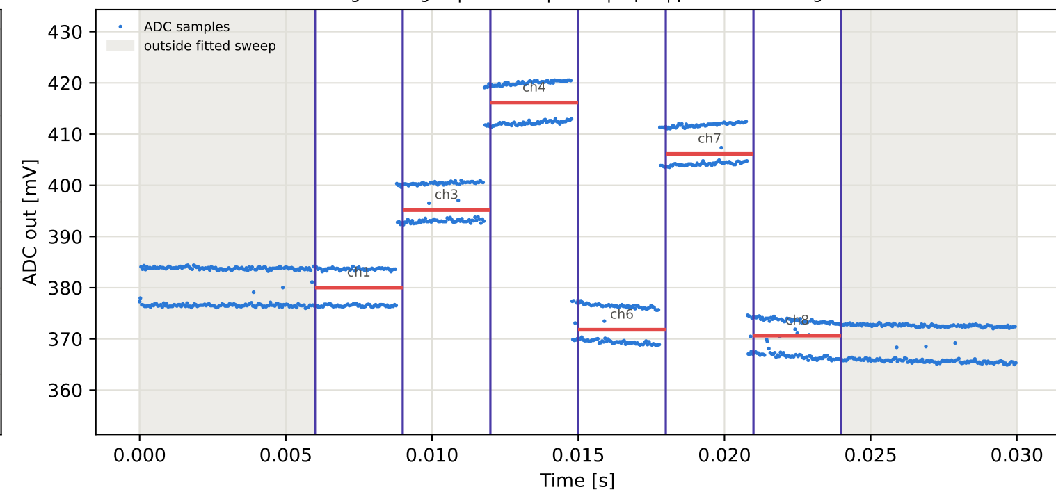
Tag6 &lt;- Tag3 | 965 MHz | run 0 | rep 1 | phase -132.95 deg
