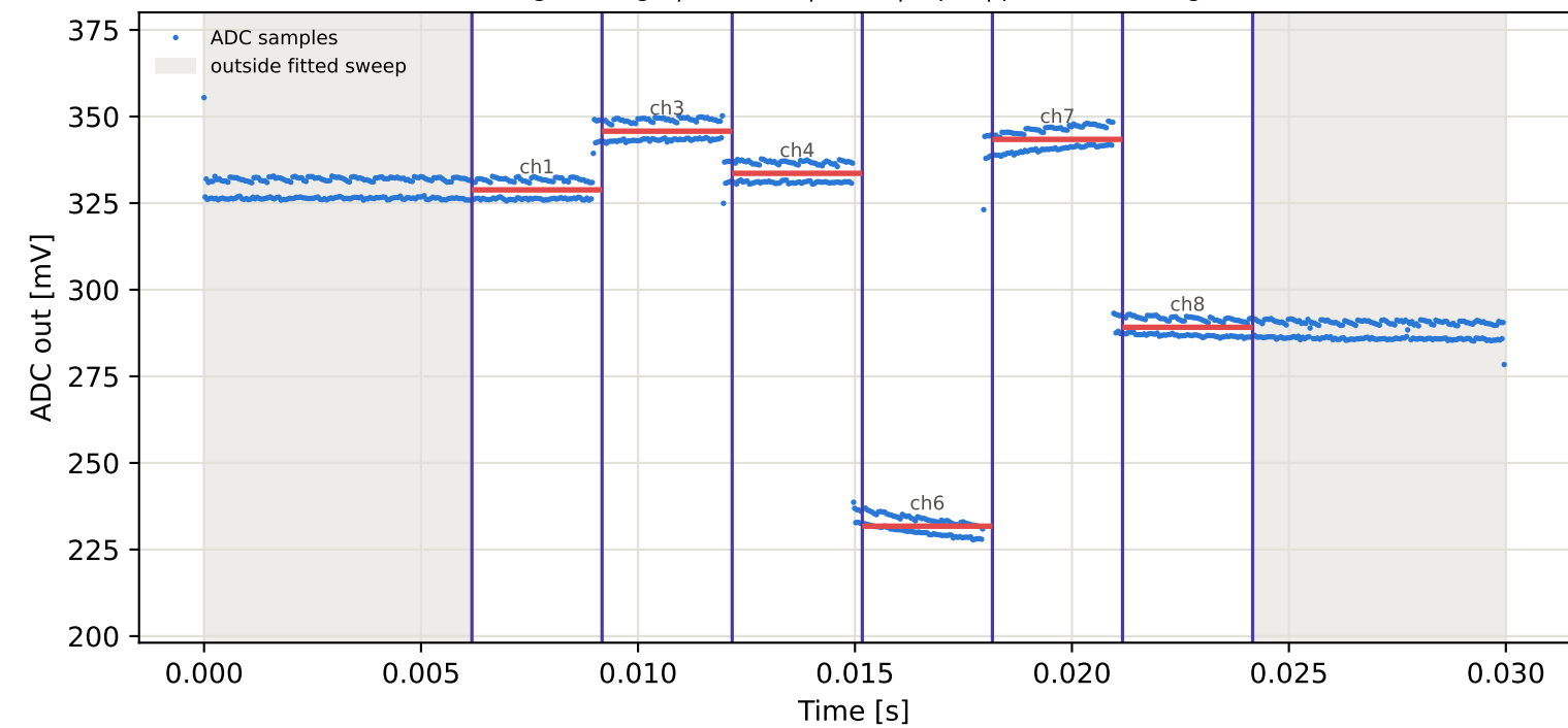
Tag9 &lt;- Tag6 | 955 MHz | run 0 | rep 1 | phase -54.33 deg
