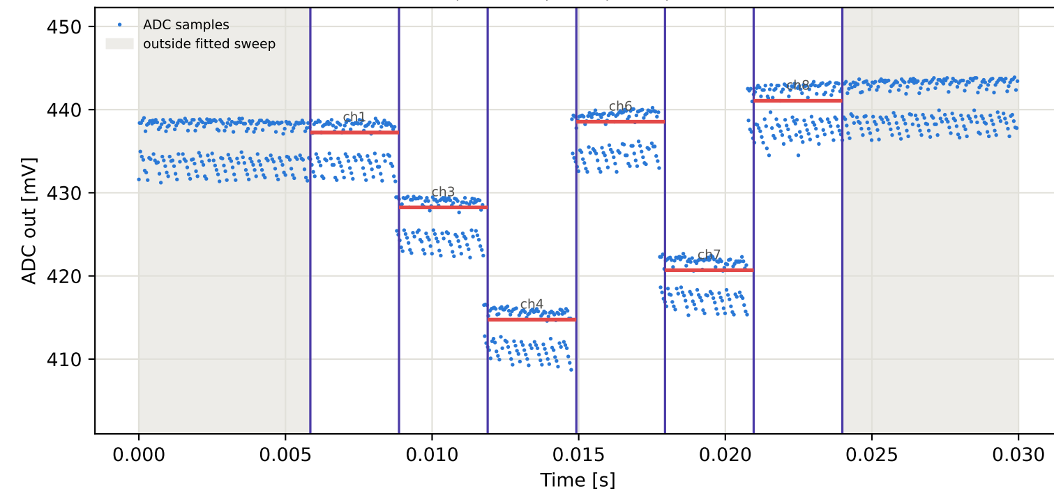
Tag3 &lt;- Tag16 | 965 MHz | run 0 | rep 1 | phase 104.01 deg
