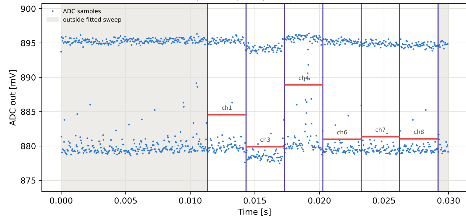
Tag8 &lt;- Tag4 | 965 MHz | run 0 | rep 1 | phase 123.05 deg
