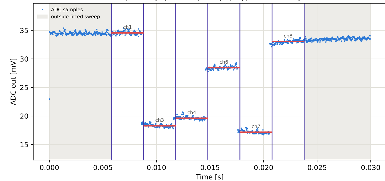
Tag10 &lt;- Tag1 | 845 MHz | run 0 | rep 1 | phase 125.79 deg
