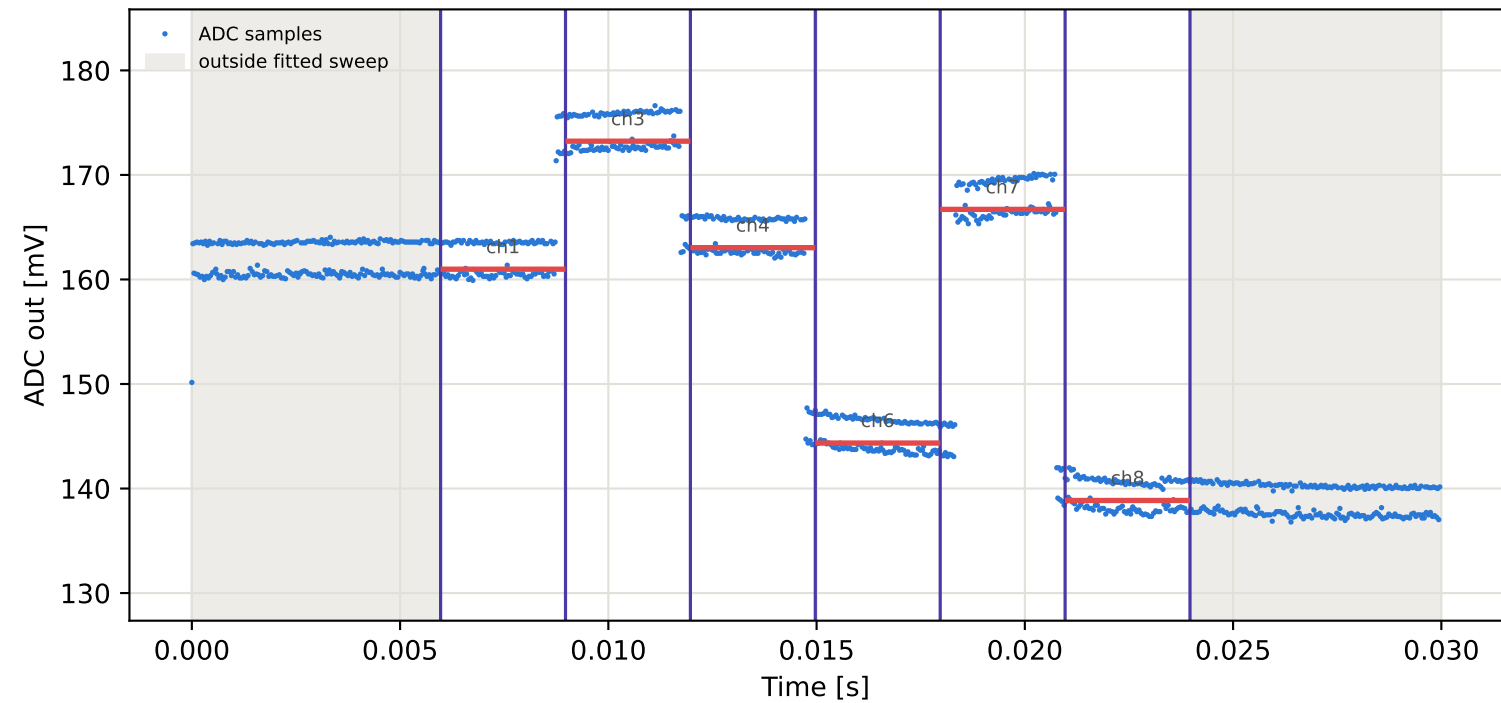
Tag7 &lt;- Tag6 | 855 MHz | run 0 | rep 1 | phase 59.38 deg
