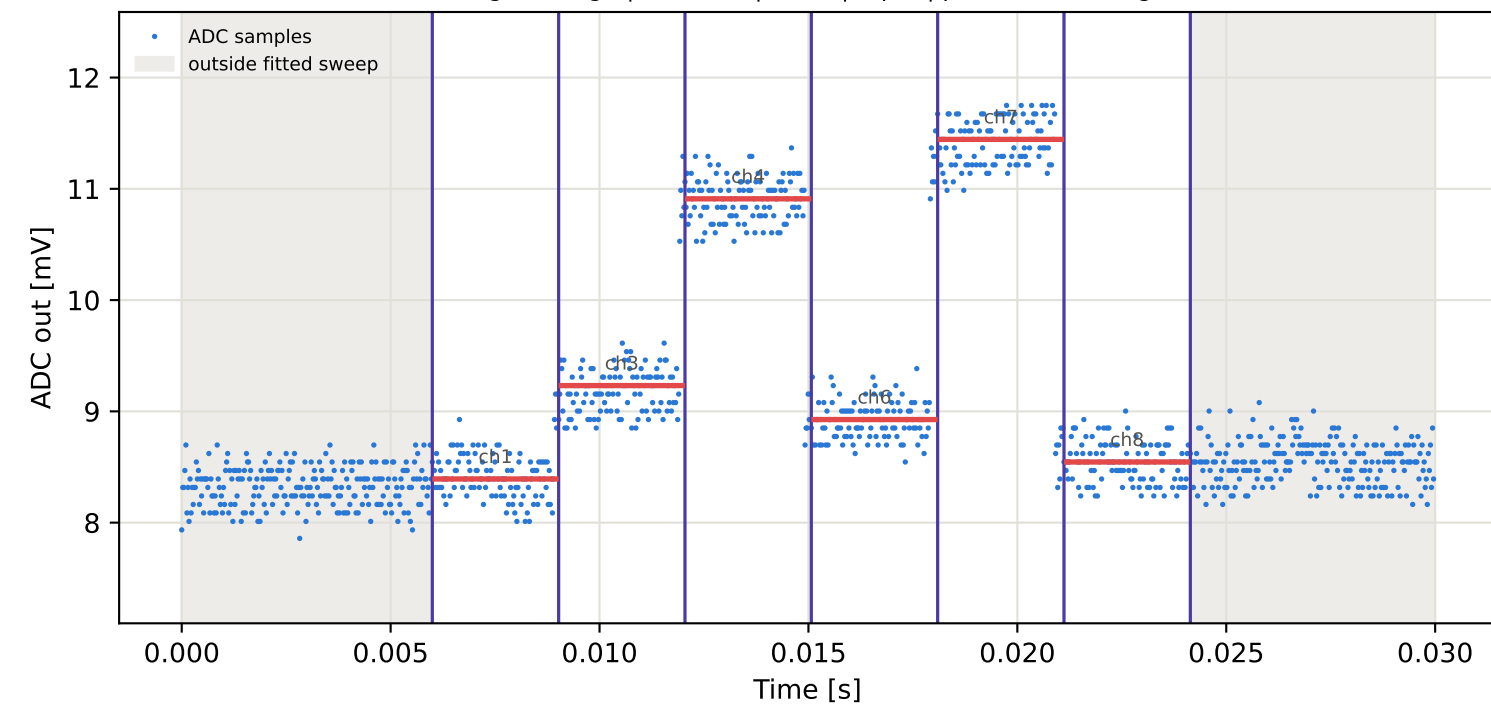
Tag2 &lt;- Tag6 | 775 MHz | run 0 | rep 1 | phase 39.77 deg
