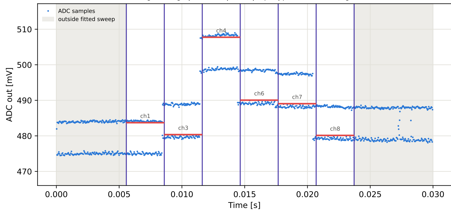
Tag3 &lt;- Tag9 | 975 MHz | run 0 | rep 1 | phase -88.11 deg
