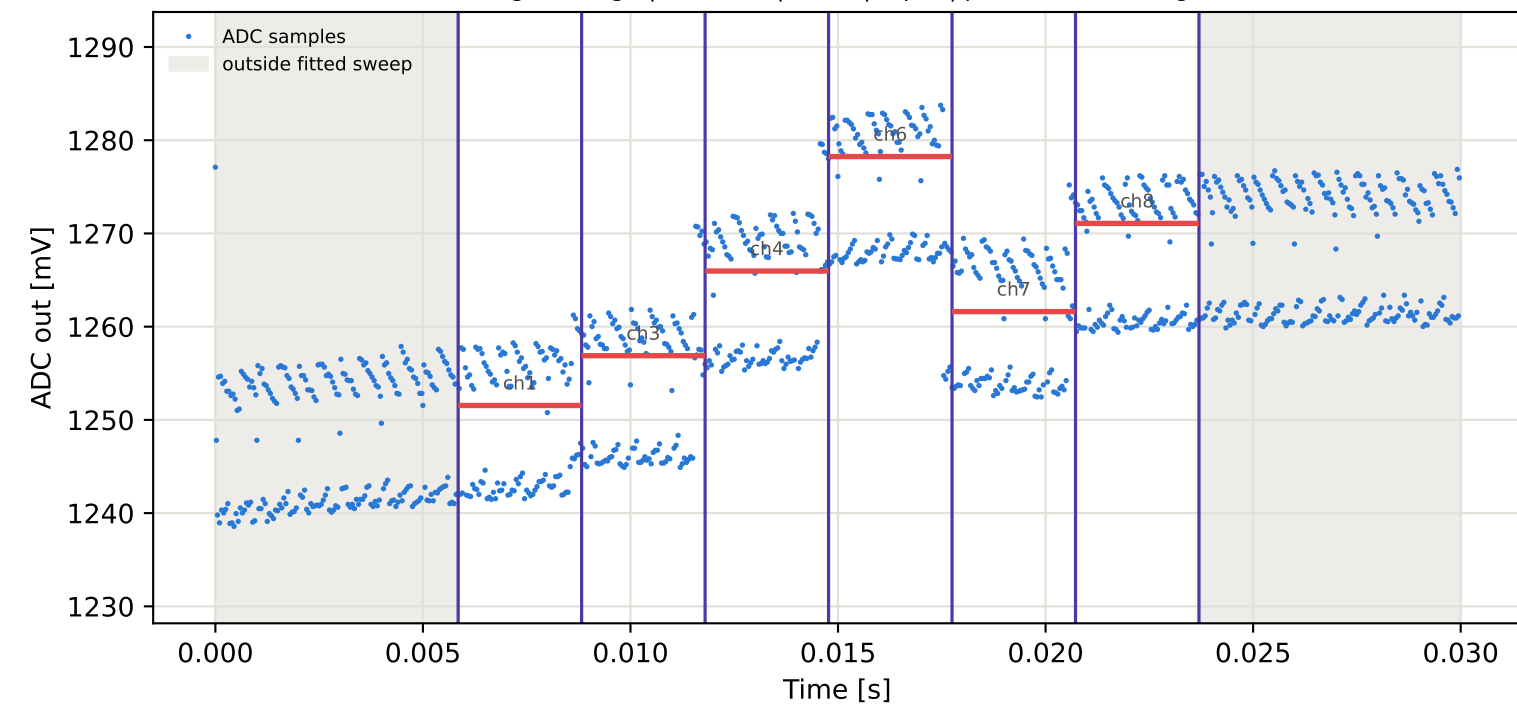
Tag5 &lt;- Tag8 | 875 MHz | run 0 | rep 1 | phase 91.34 deg
