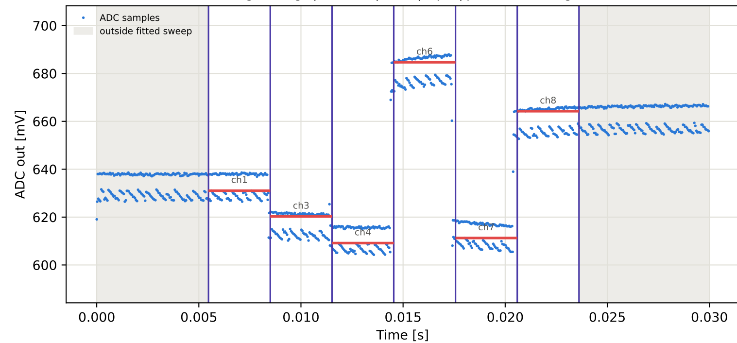
Tag9 &lt;- Tag5 | 945 MHz | run 0 | rep 1 | phase -36.94 deg
