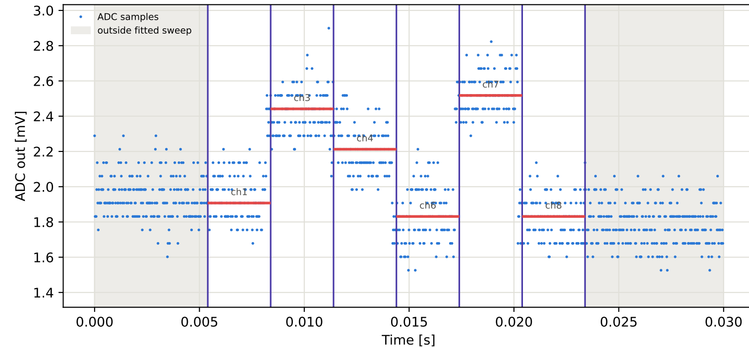
Tag7 &lt;- Tag5 | 785 MHz | run 0 | rep 1 | phase -170.86 deg
