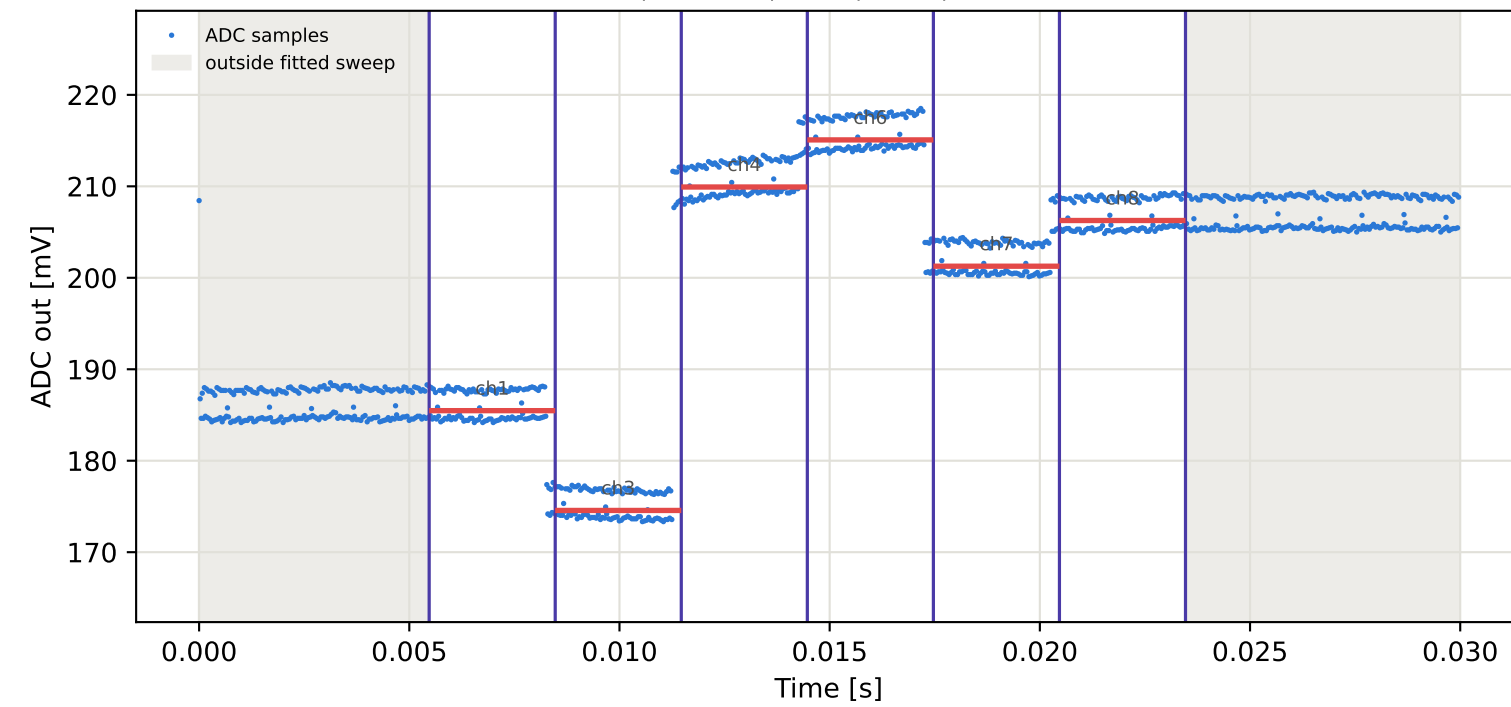
Tag3 &lt;- Tag8 | 825 MHz | run 0 | rep 1 | phase -134.37 deg
