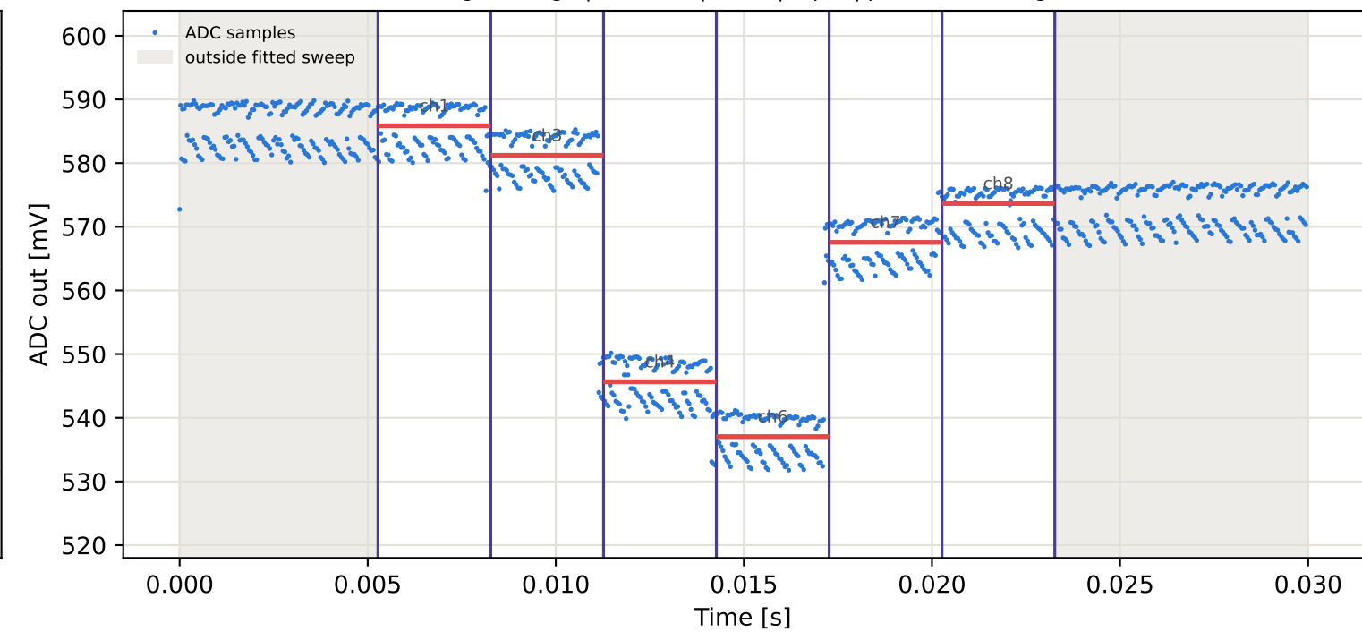
Tag9 &lt;- Tag6 | 965 MHz | run 0 | rep 1 | phase -14.97 deg
