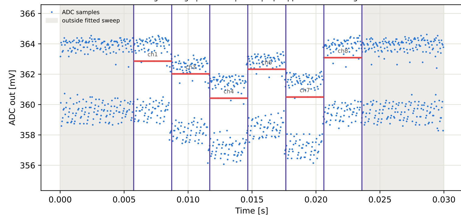
Tag3 &lt;- Tag9 | 845 MHz | run 0 | rep 1 | phase 61.21 deg
