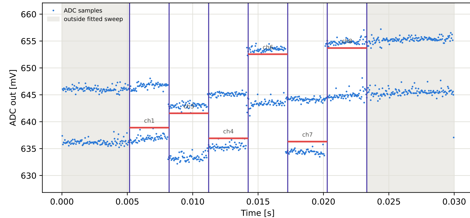
Tag1 &lt;- Tag9 | 885 MHz | run 0 | rep 1 | phase 16.95 deg
