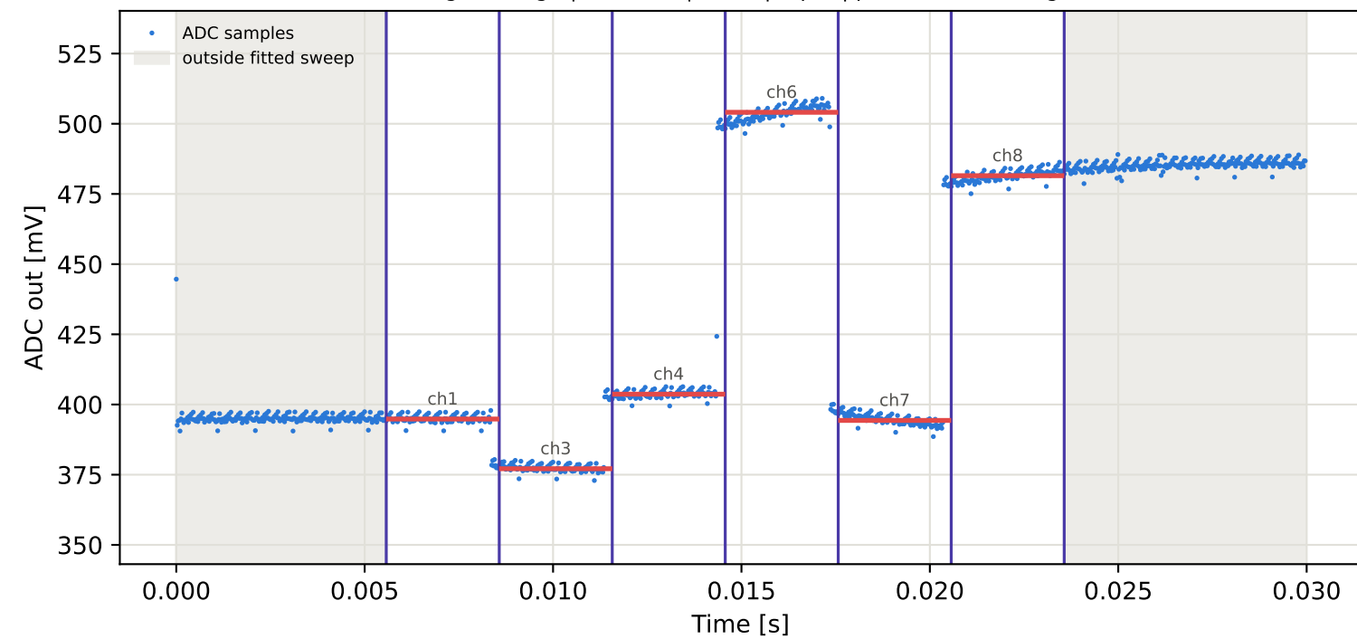
Tag1 &lt;- Tag8 | 895 MHz | run 0 | rep 1 | phase -99.58 deg
