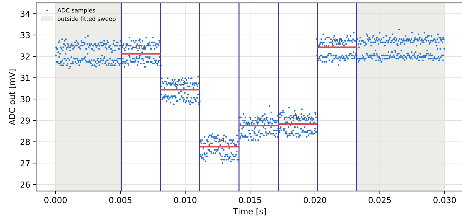
Tag2 &lt;- Tag8 | 925 MHz | run 0 | rep 1 | phase 38.30 deg
