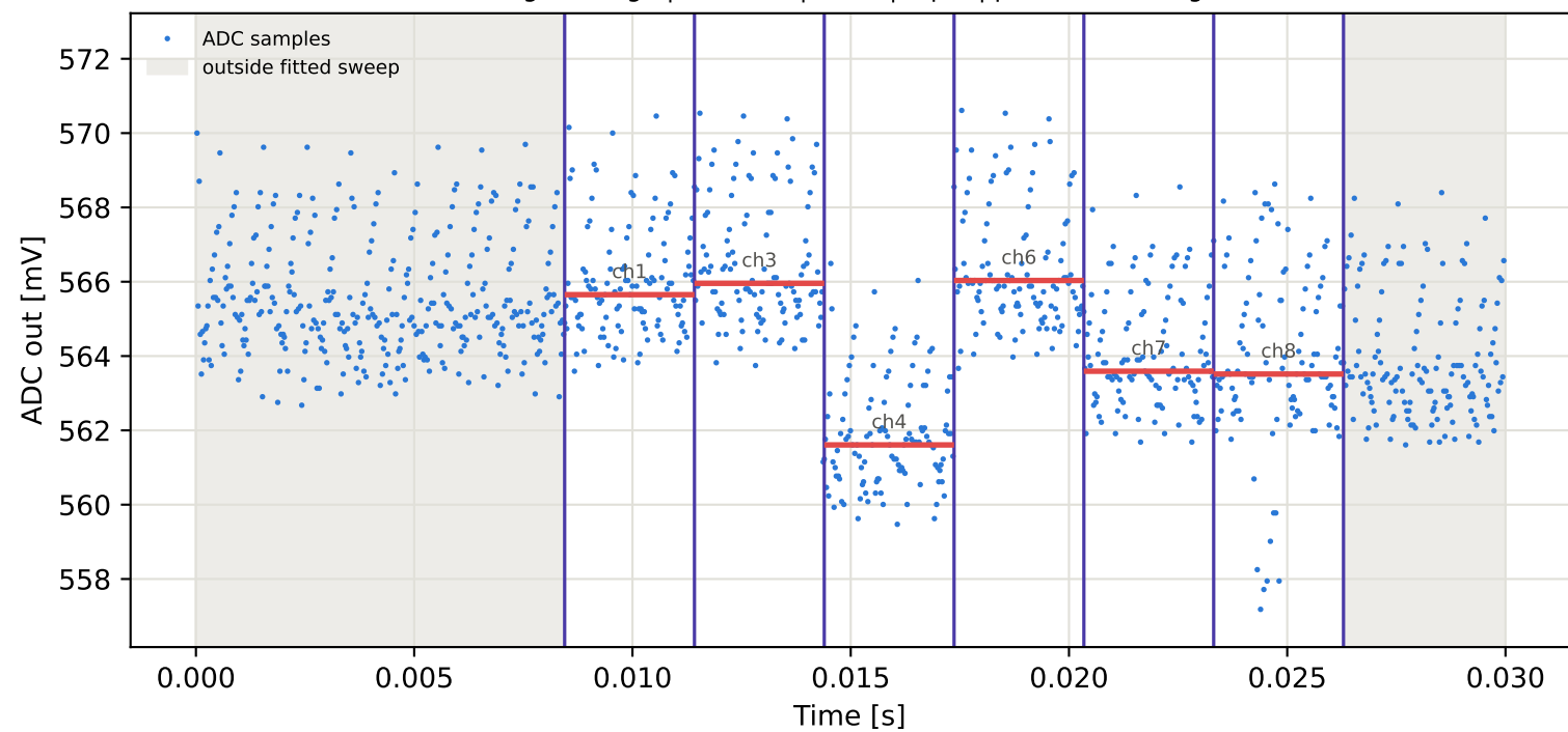
Tag9 &lt;- Tag2 | 925 MHz | run 0 | rep 1 | phase 79.57 deg
