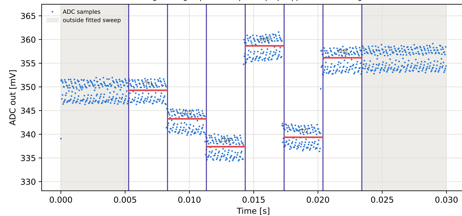
Tag1 &lt;- Tag16 | 955 MHz | run 0 | rep 1 | phase 12.90 deg
