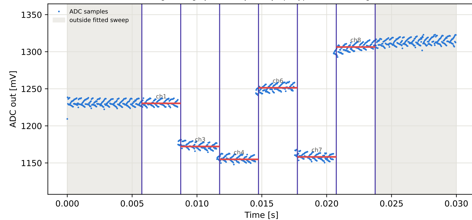
Tag6 &lt;- Tag1 | 895 MHz | run 0 | rep 1 | phase 107.54 deg
