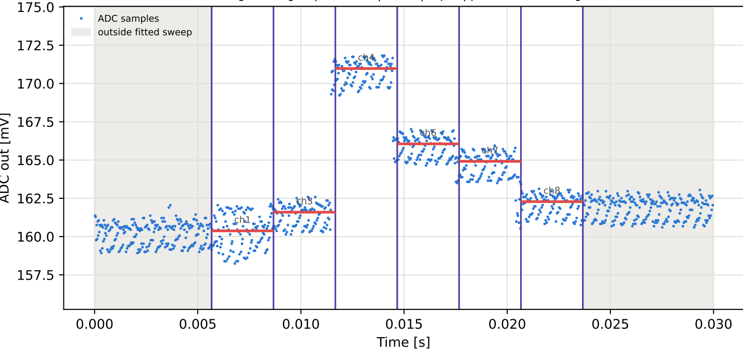
Tag7 &lt;- Tag10 | 995 MHz | run 0 | rep 1 | phase -123.76 deg
