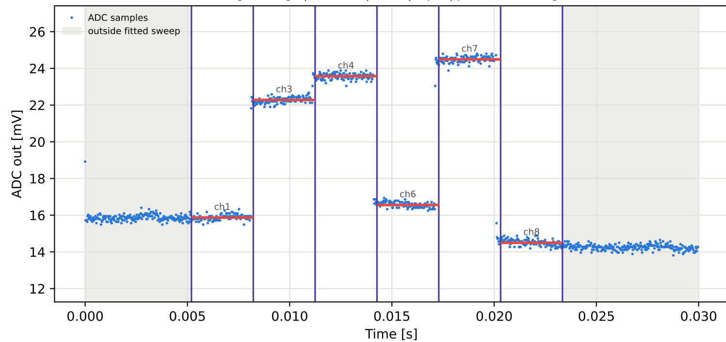
Tag1 &lt;- Tag8 | 825 MHz | run 0 | rep 1 | phase 76.57 deg
