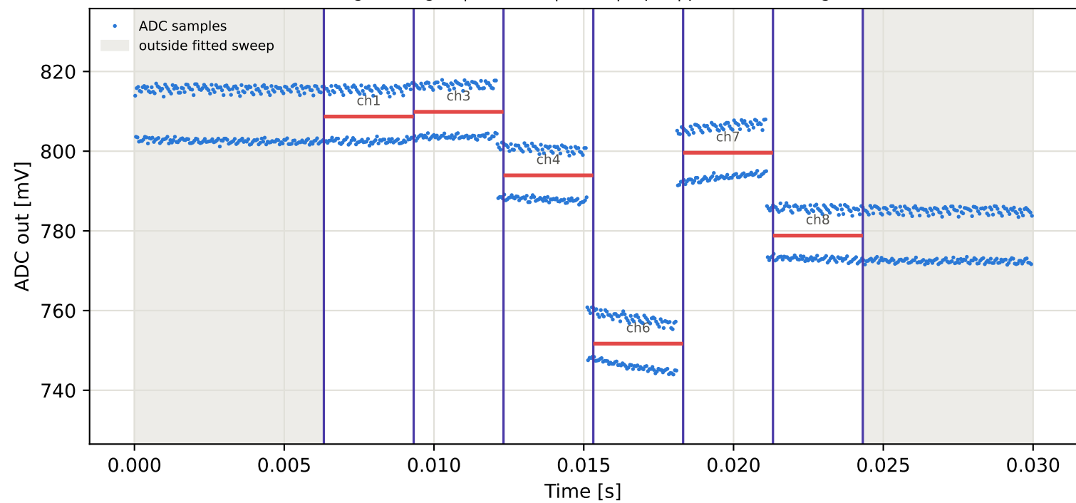
Tag1 &lt;- Tag2 | 915 MHz | run 0 | rep 1 | phase -75.01 deg
