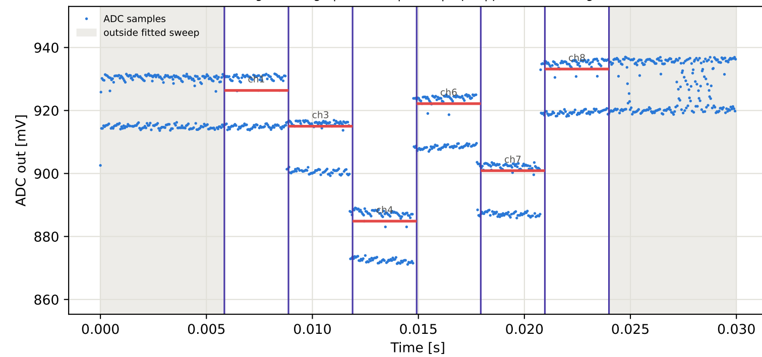
Tag15 &lt;- Tag5 | 975 MHz | run 0 | rep 1 | phase 87.39 deg
