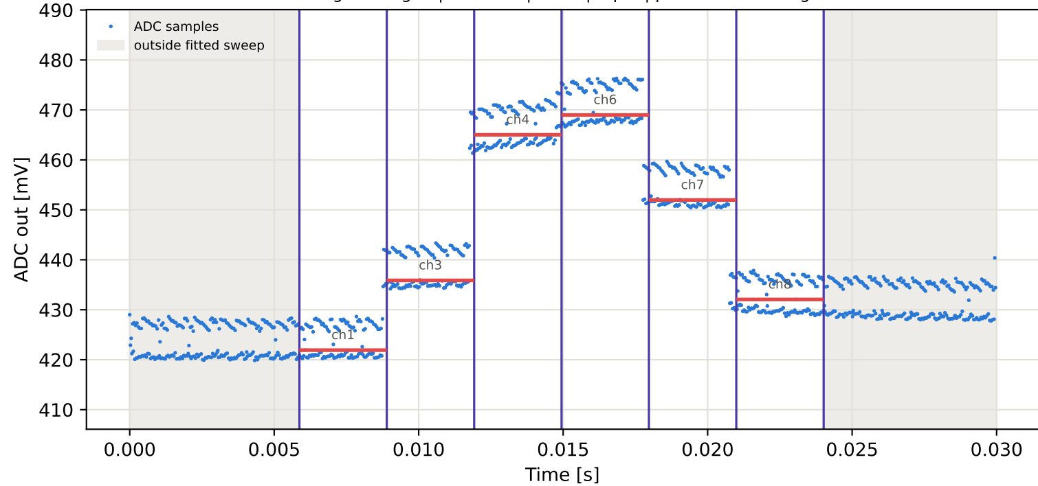
Tag5 &lt;- Tag2 | 935 MHz | run 0 | rep 1 | phase 147.94 deg
