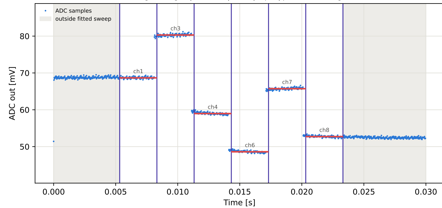
Tag1 &lt;- Tag16 | 835 MHz | run 0 | rep 1 | phase -81.59 deg
