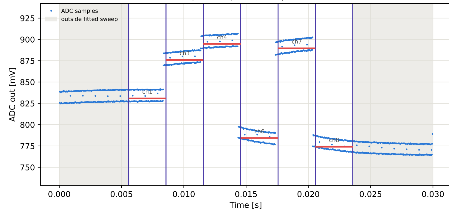
Tag4 &lt;- Tag7 | 915 MHz | run 0 | rep 1 | phase 81.92 deg
