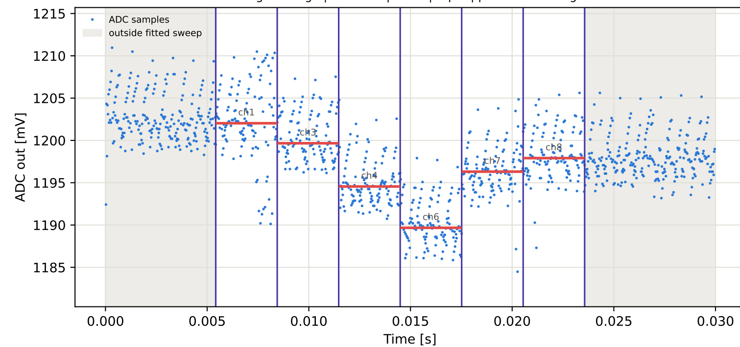
Tag6 &lt;- Tag4 | 895 MHz | run 0 | rep 1 | phase 28.17 deg
