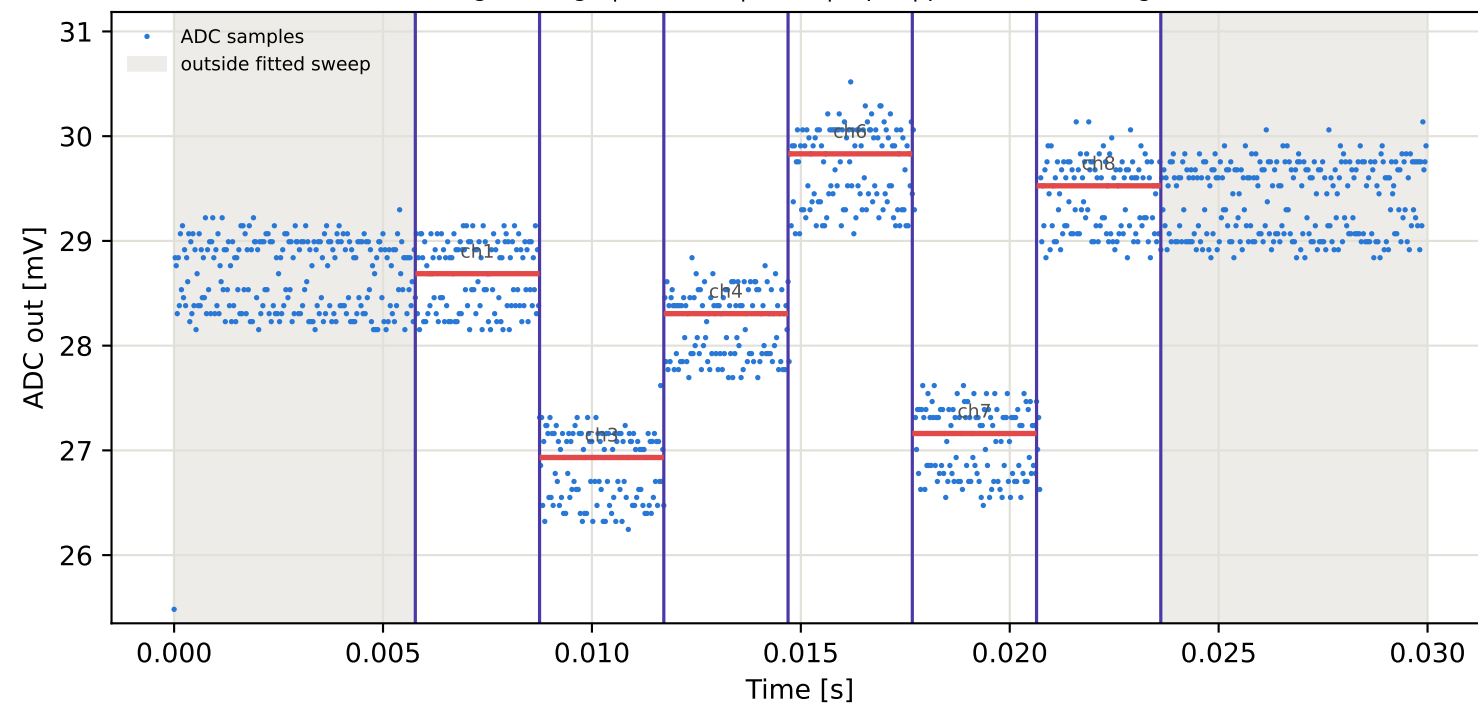
Tag3 &lt;- Tag10 | 785 MHz | run 0 | rep 1 | phase 77.54 deg
