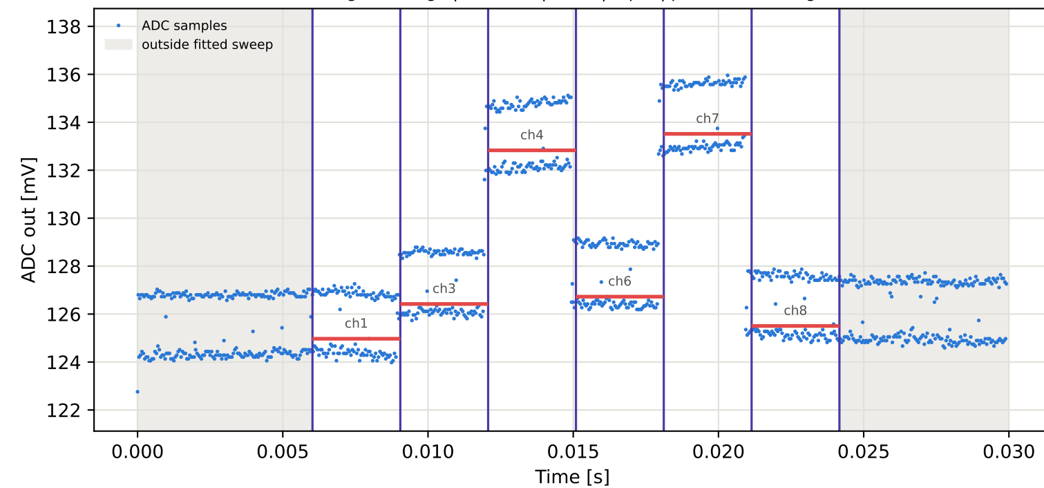
Tag16 &lt;- Tag6 | 775 MHz | run 0 | rep 1 | phase -169.27 deg
