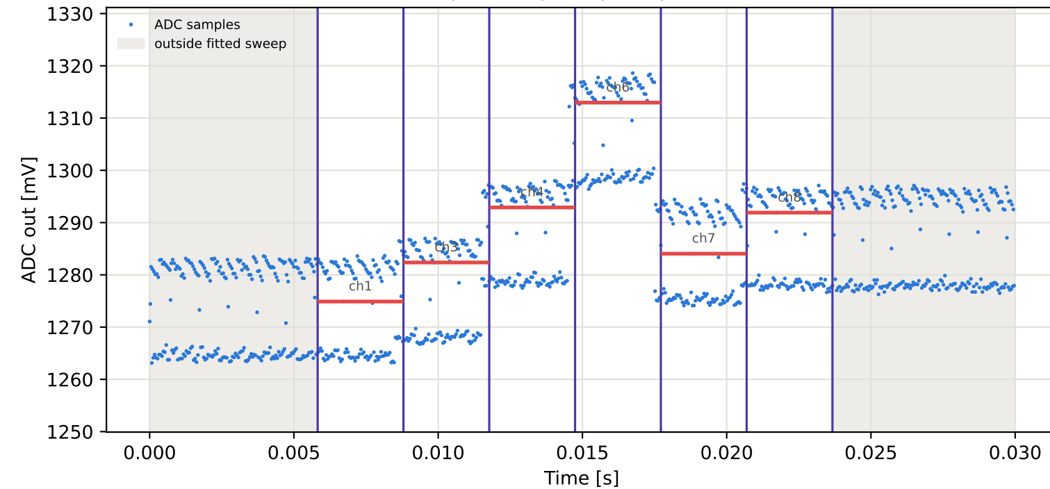
Tag8 &lt;- Tag6 | 905 MHz | run 0 | rep 1 | phase -151.88 deg
