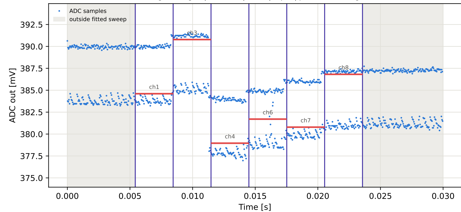
Tag6 &lt;- Tag2 | 825 MHz | run 0 | rep 1 | phase -64.73 deg
