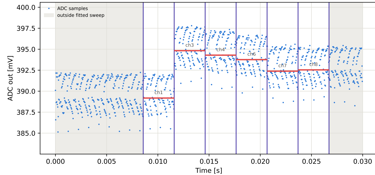
Tag15 &lt;- Tag5 | 825 MHz | run 0 | rep 1 | phase 80.67 deg
