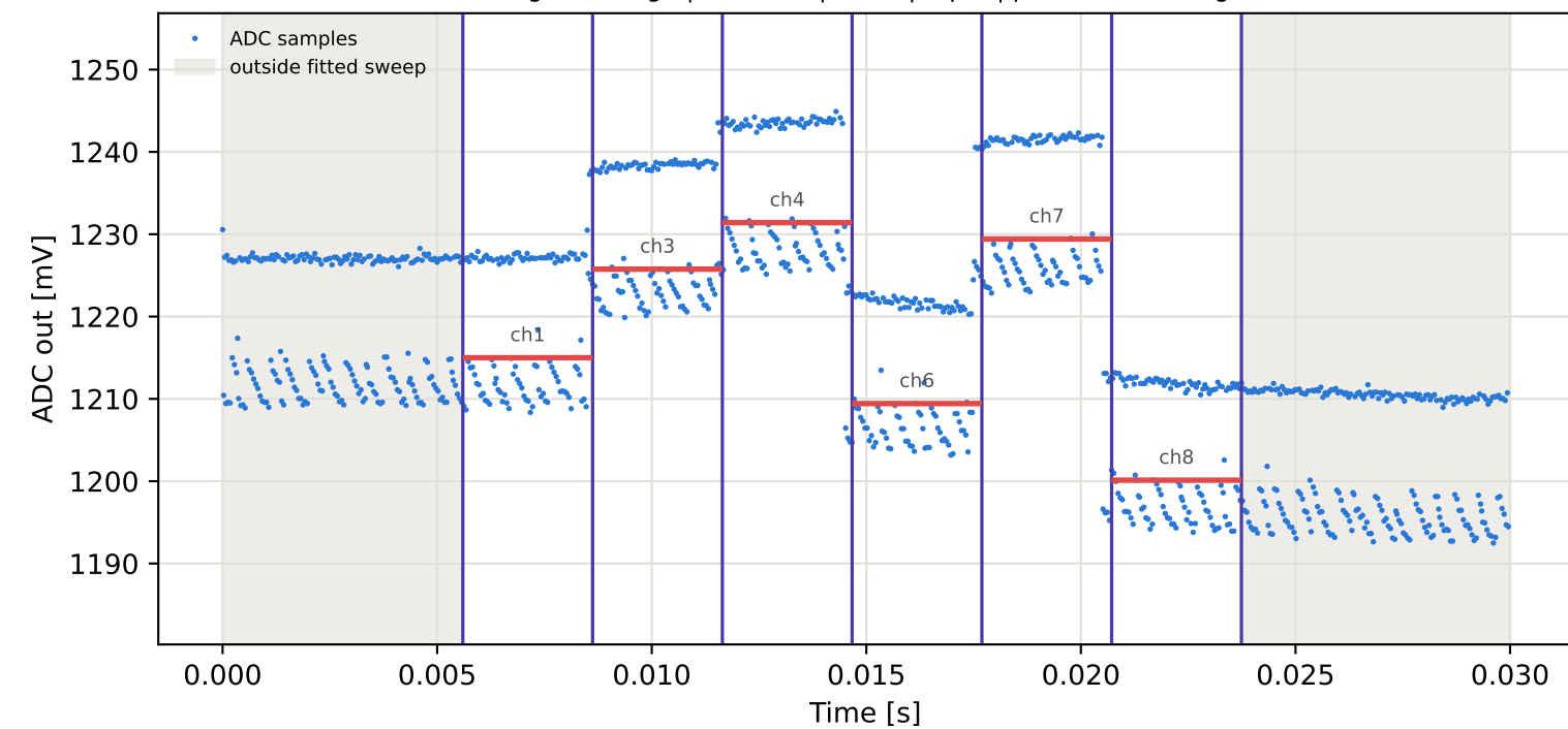
Tag16 &lt;- Tag6 | 905 MHz | run 0 | rep 1 | phase -50.35 deg
