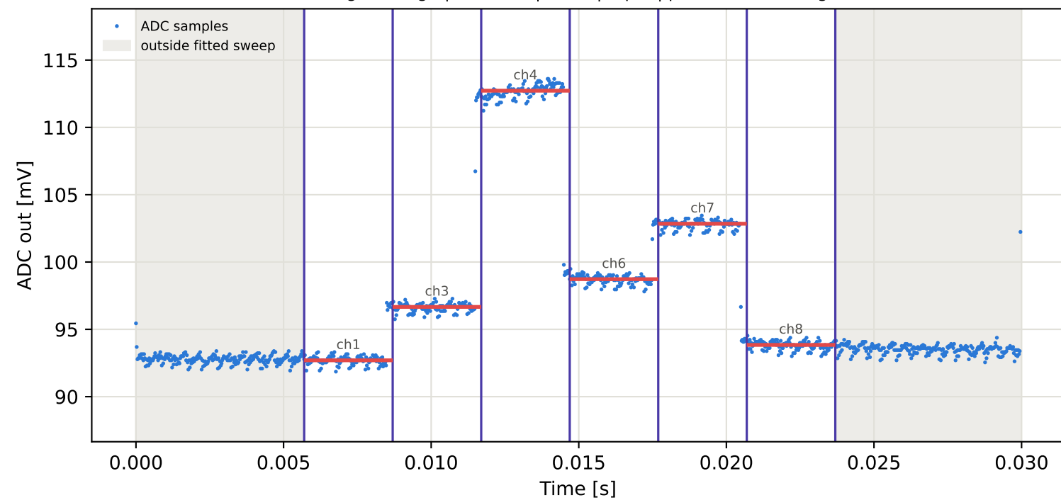
Tag6 &lt;- Tag5 | 995 MHz | run 0 | rep 1 | phase -177.14 deg
