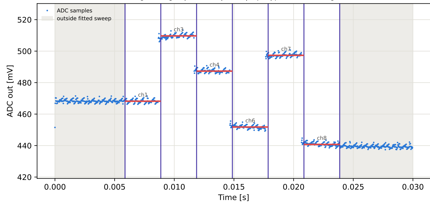
Tag4 &lt;- Tag3 | 855 MHz | run 0 | rep 1 | phase -40.79 deg
