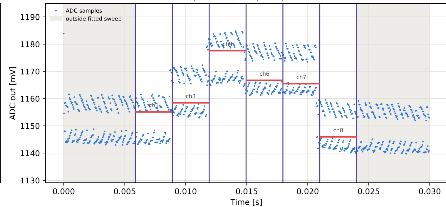
Tag6 &lt;- Tag3 | 915 MHz | run 0 | rep 1 | phase 151.13 deg
