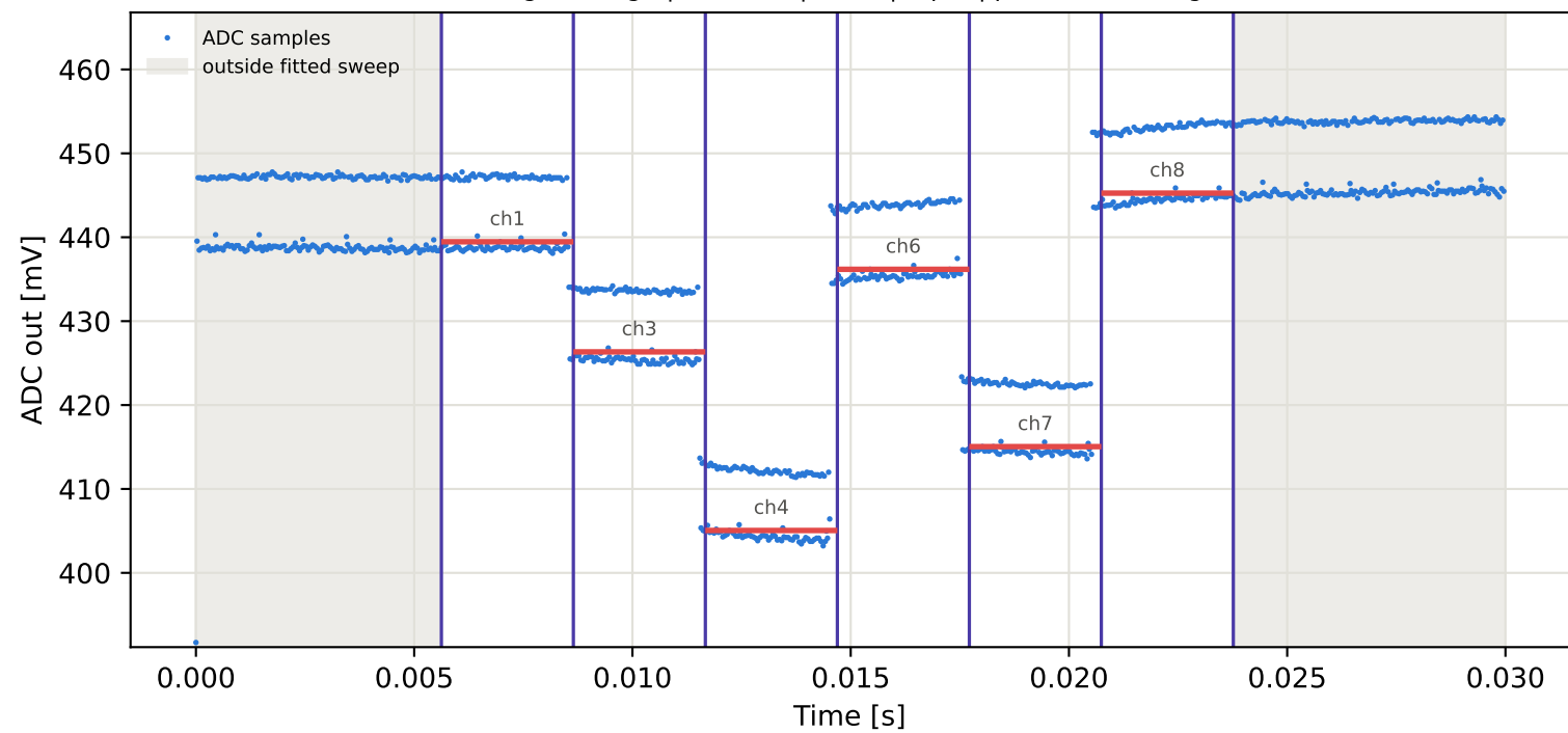
Tag3 &lt;- Tag7 | 965 MHz | run 0 | rep 1 | phase -170.20 deg
