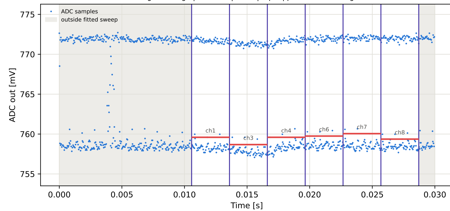
Tag16 &lt;- Tag4 | 995 MHz | run 0 | rep 1 | phase 60.11 deg
