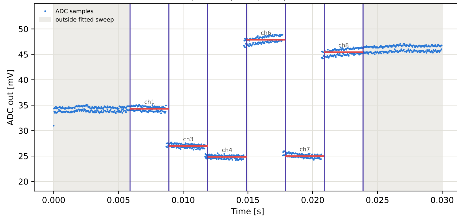
Tag2 &lt;- Tag5 | 925 MHz | run 0 | rep 1 | phase -6.71 deg
