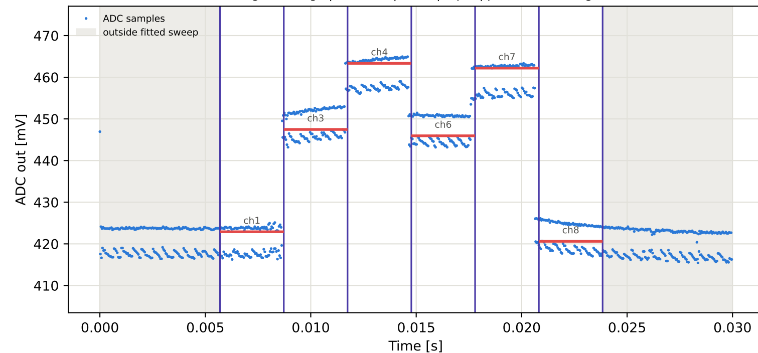
Tag15 &lt;- Tag1 | 875 MHz | run 0 | rep 1 | phase 100.03 deg
