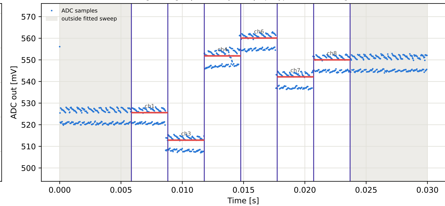
Tag6 &lt;- Tag3 | 835 MHz | run 0 | rep 1 | phase -10.03 deg
