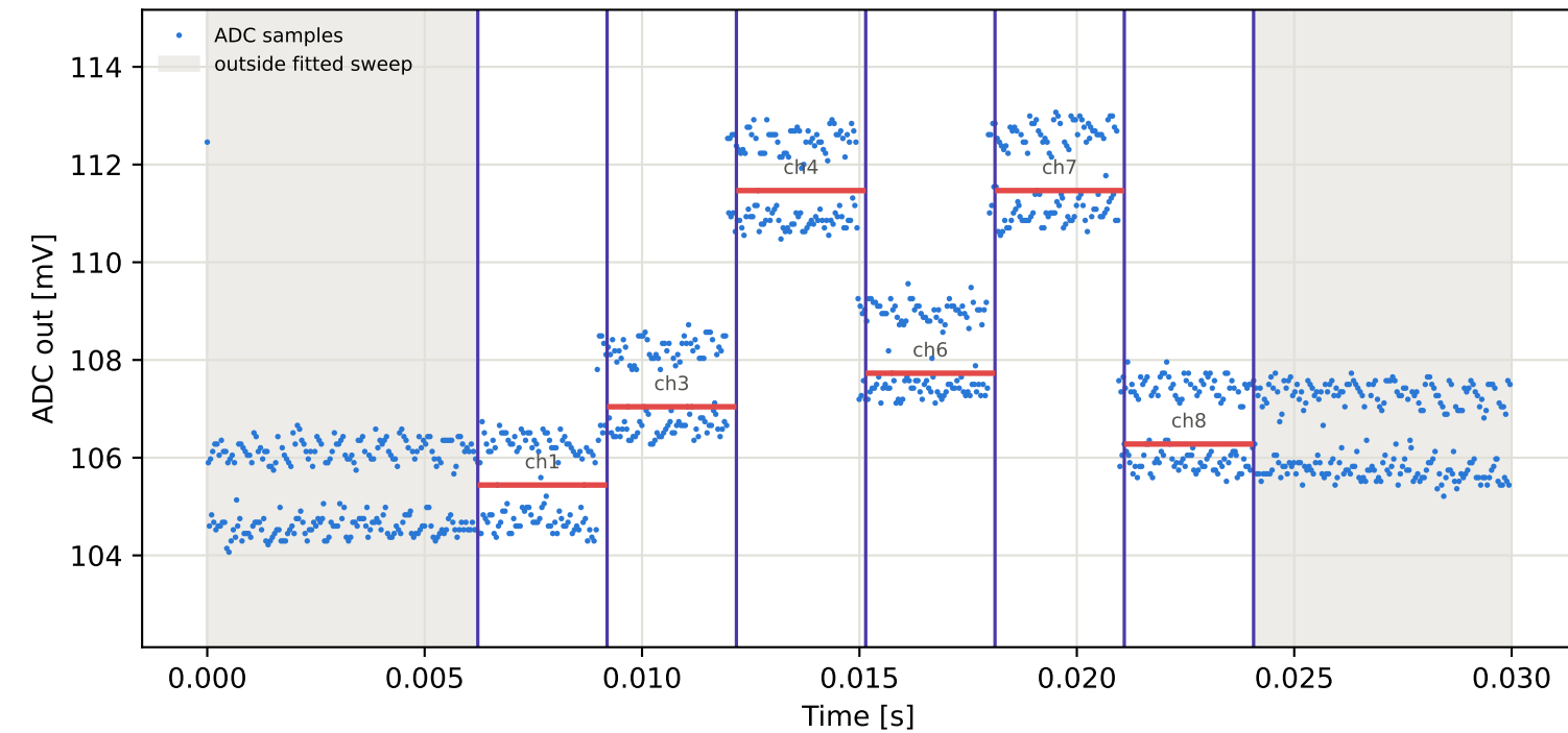
Tag9 &lt;- Tag16 | 795 MHz | run 0 | rep 1 | phase 127.34 deg
