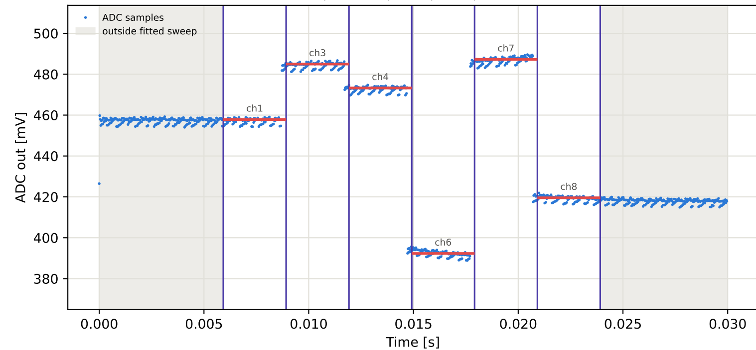
Tag4 &lt;- Tag9 | 985 MHz | run 0 | rep 1 | phase -13.44 deg
