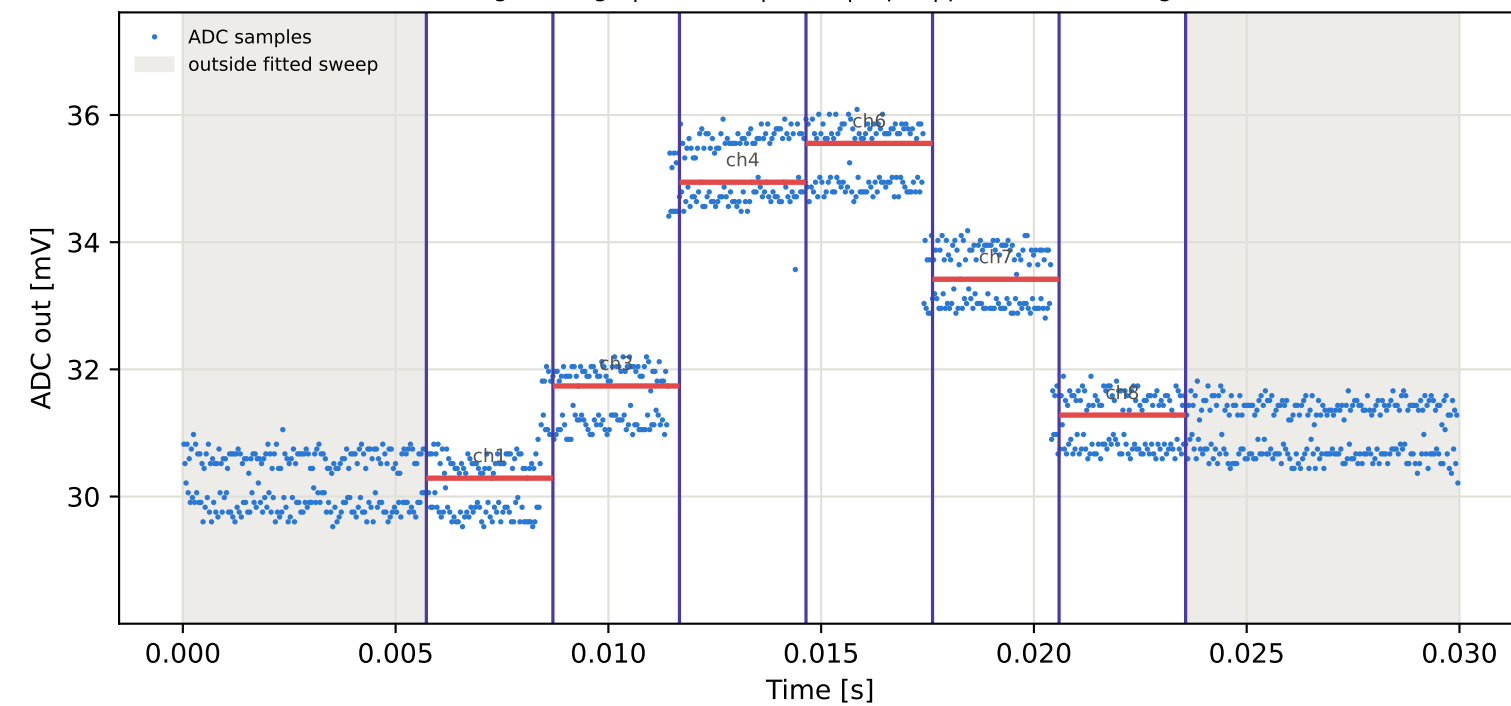
Tag2 &lt;- Tag7 | 945 MHz | run 0 | rep 1 | phase -75.90 deg
