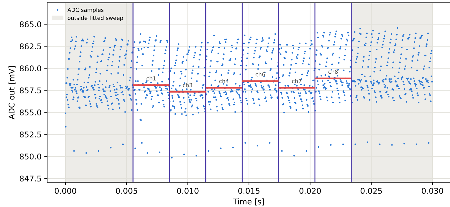
Tag16 &lt;- Tag15 | 855 MHz | run 0 | rep 1 | phase 35.15 deg
