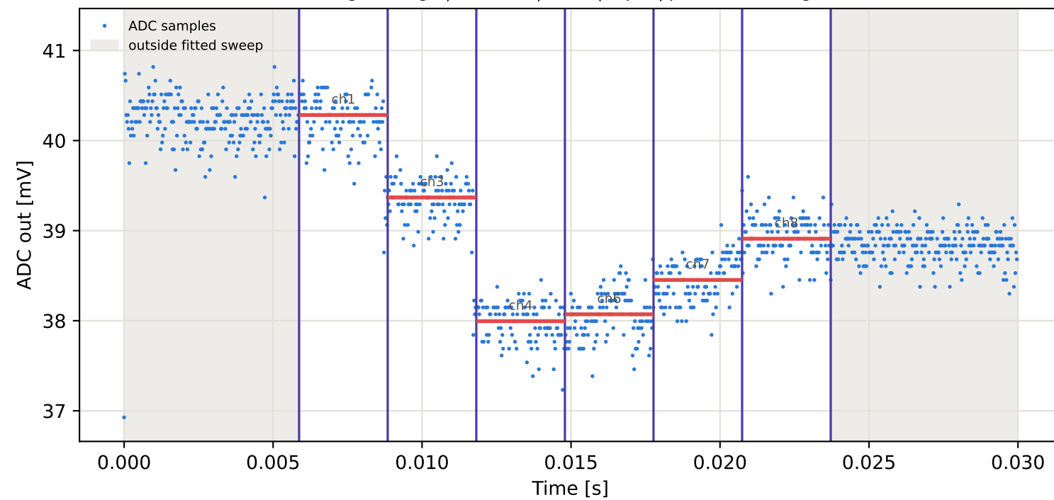
Tag3 &lt;- Tag10 | 865 MHz | run 0 | rep 1 | phase -138.10 deg
