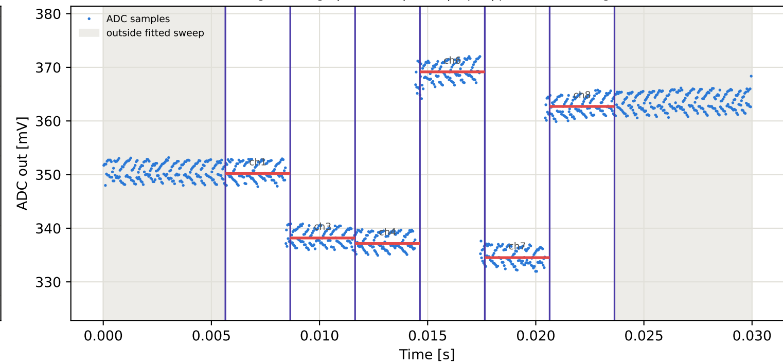
Tag10 &lt;- Tag9 | 985 MHz | run 0 | rep 1 | phase -35.21 deg
