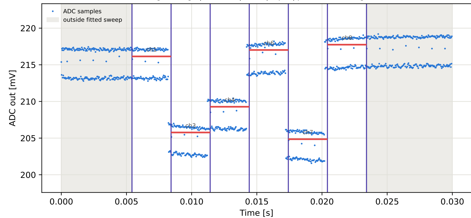
Tag9 &lt;- Tag6 | 805 MHz | run 0 | rep 1 | phase -85.99 deg
