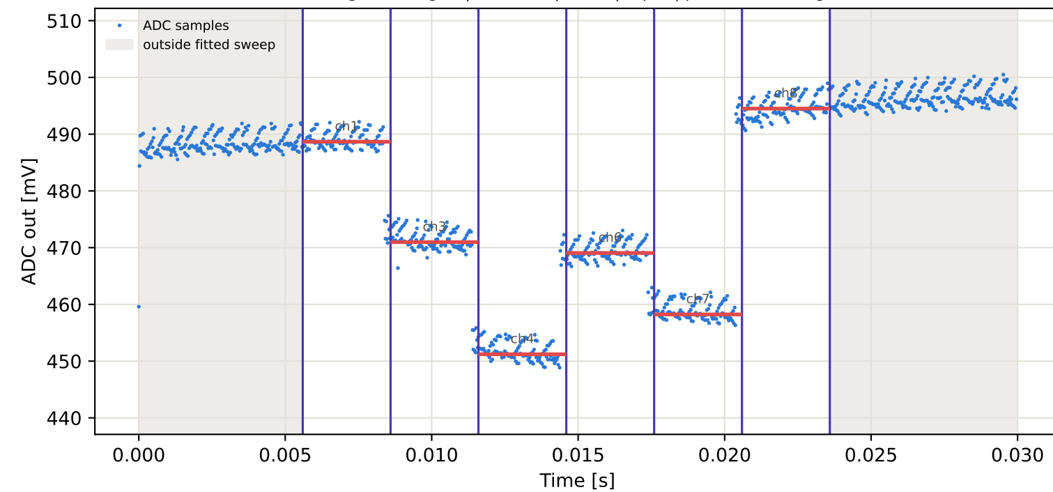
Tag10 &lt;- Tag2 | 925 MHz | run 0 | rep 1 | phase 126.19 deg
