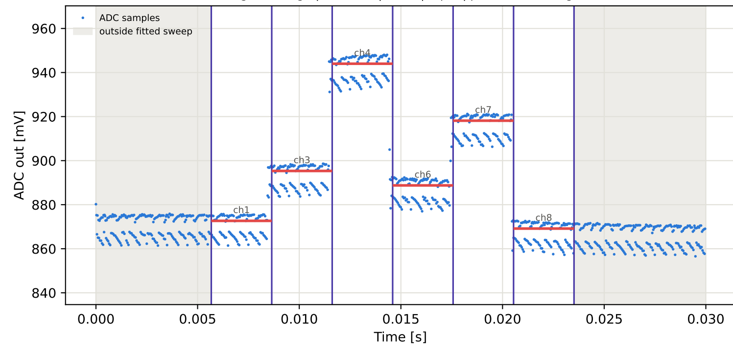
Tag16 &lt;- Tag1 | 975 MHz | run 0 | rep 1 | phase -29.98 deg
