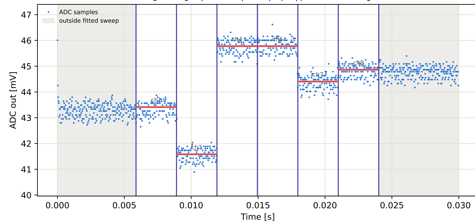
Tag1 &lt;- Tag16 | 795 MHz | run 0 | rep 1 | phase 160.06 deg
