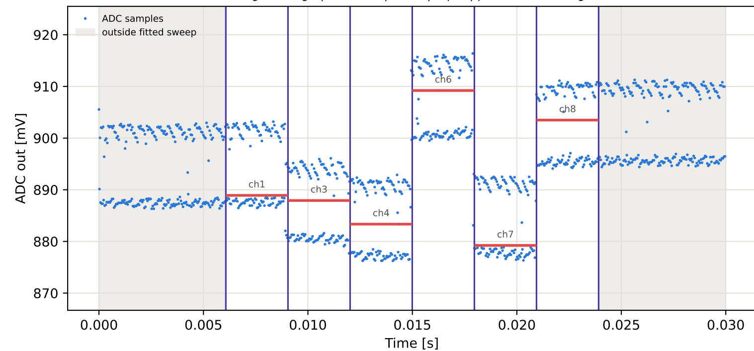
Tag8 &lt;- Tag6 | 965 MHz | run 0 | rep 1 | phase 155.82 deg
