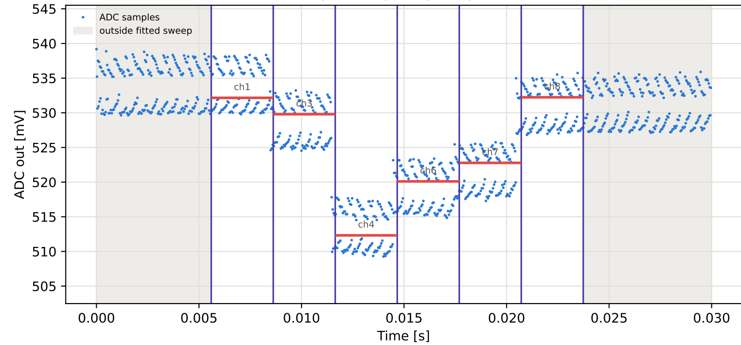
Tag7 &lt;- Tag15 | 975 MHz | run 0 | rep 1 | phase 59.62 deg
