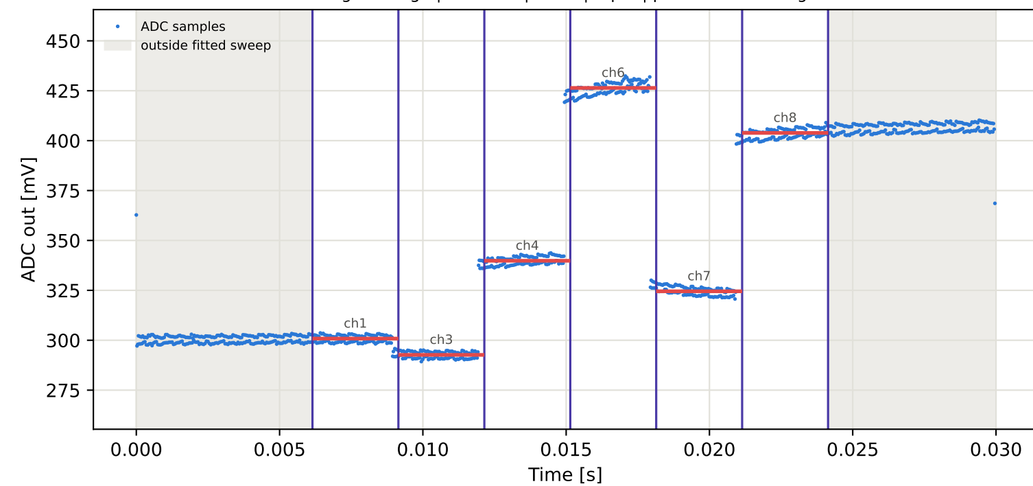
Tag4 &lt;- Tag7 | 875 MHz | run 0 | rep 1 | phase -20.80 deg
