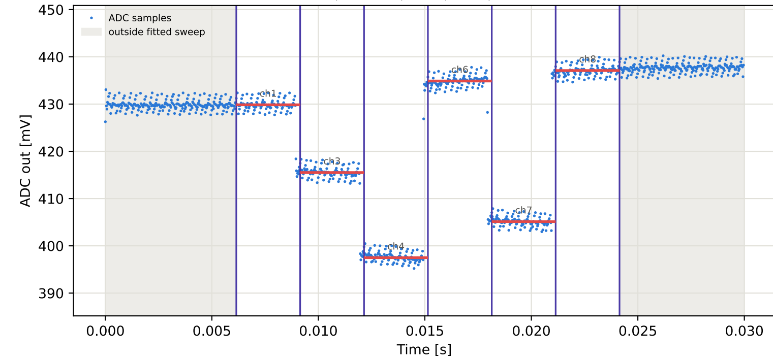
Tag3 &lt;- Tag16 | 985 MHz | run 0 | rep 1 | phase 108.76 deg
