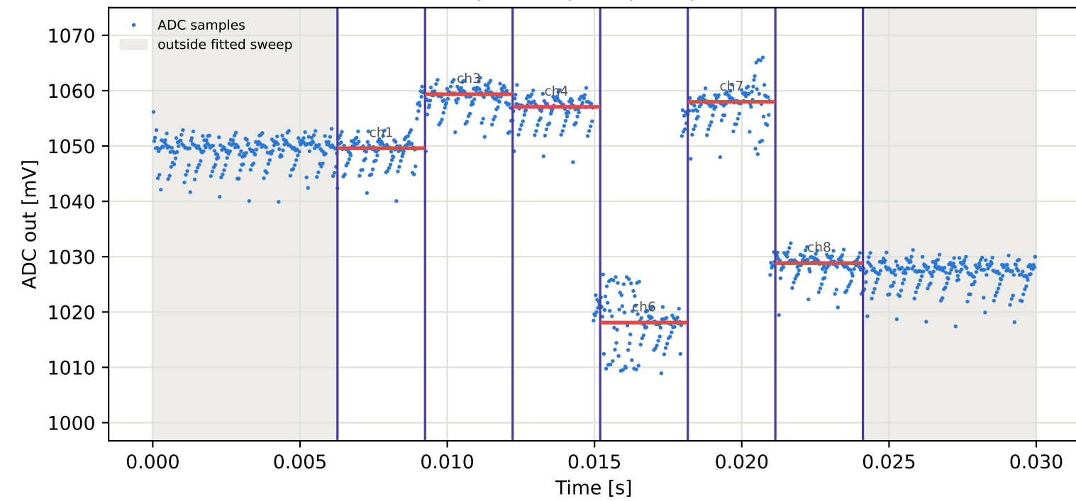
Tag10 &lt;- Tag4 | 915 MHz | run 0 | rep 1 | phase -9.10 deg
