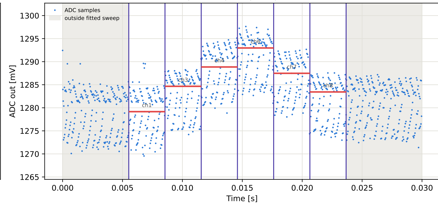
Tag8 &lt;- Tag7 | 905 MHz | run 0 | rep 1 | phase -131.86 deg
