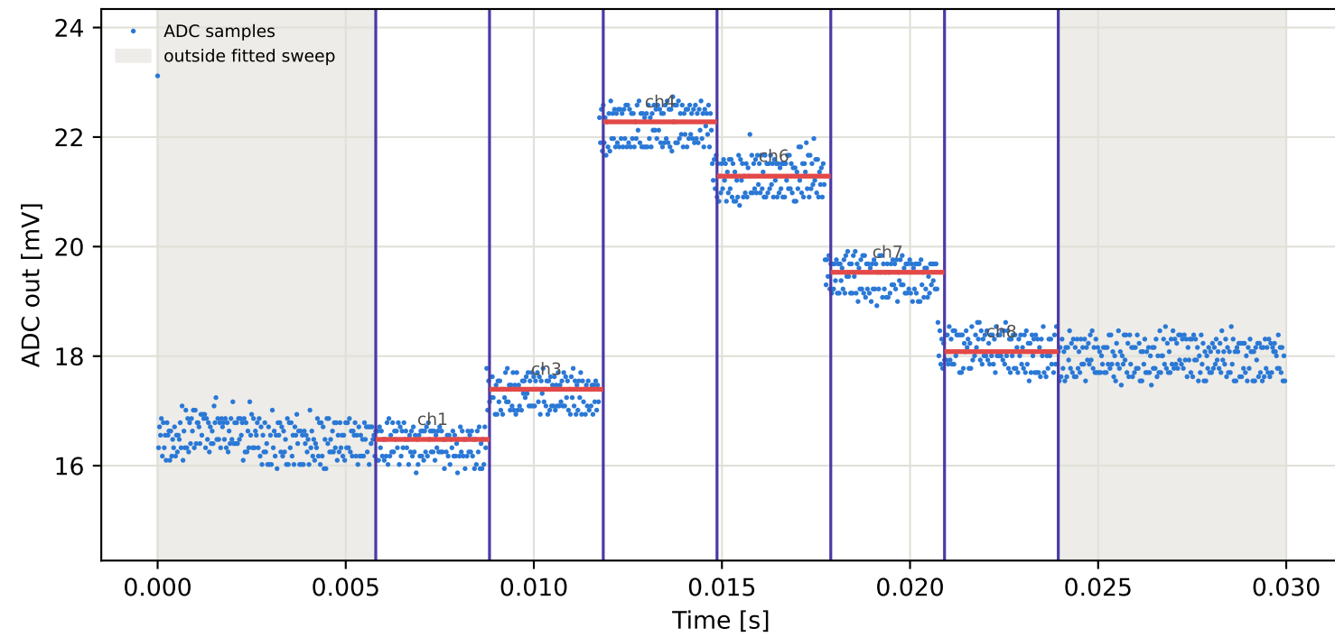
Tag3 &lt;- Tag10 | 975 MHz | run 0 | rep 1 | phase 163.15 deg
