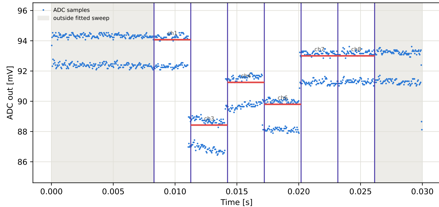
Tag9 &lt;- Tag7 | 785 MHz | run 0 | rep 1 | phase -67.97 deg
