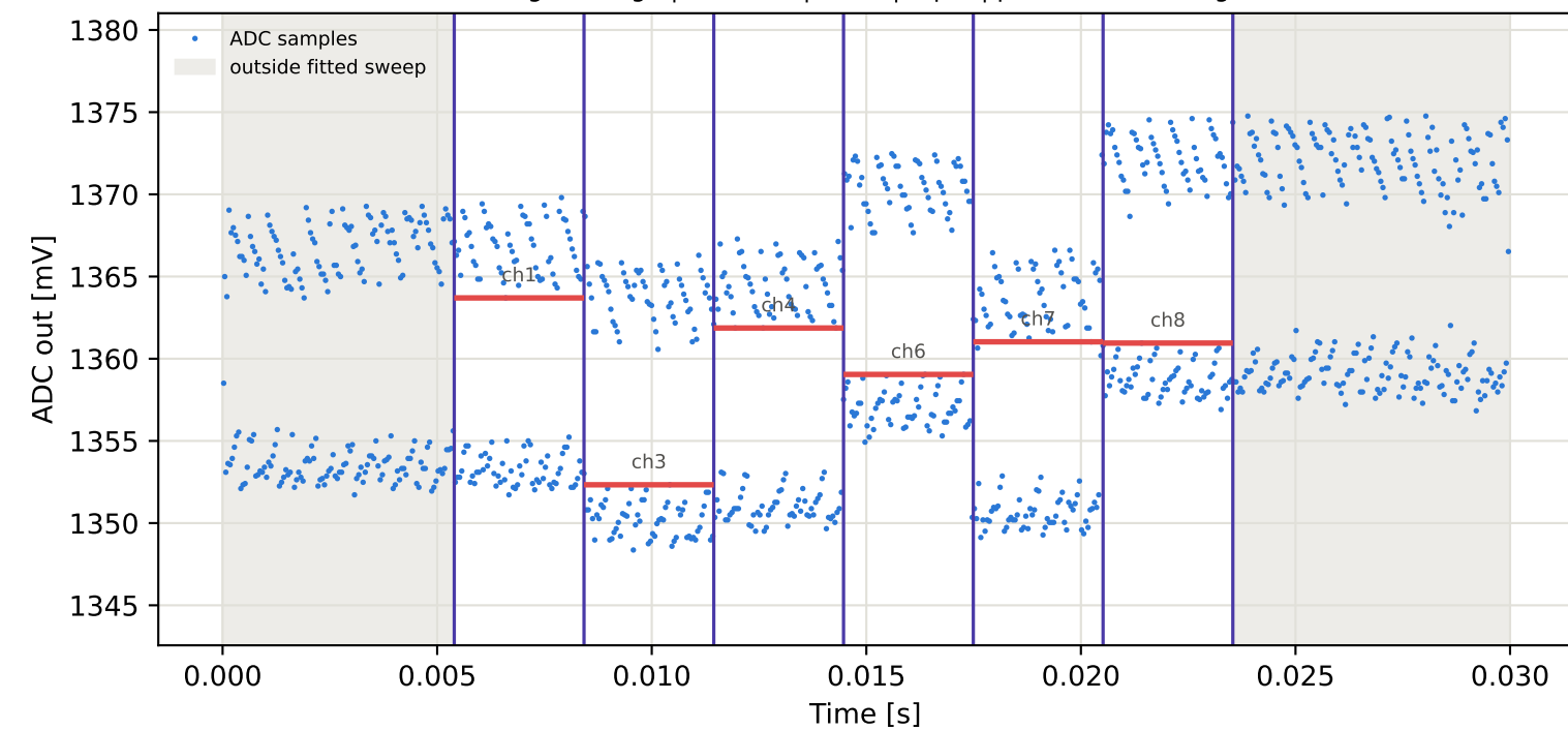
Tag8 &lt;- Tag6 | 875 MHz | run 0 | rep 1 | phase -146.72 deg
