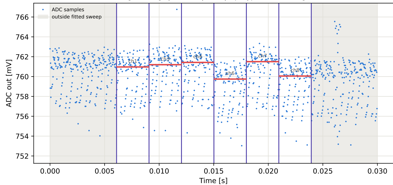
Tag16 &lt;- Tag4 | 835 MHz | run 0 | rep 1 | phase -25.89 deg
