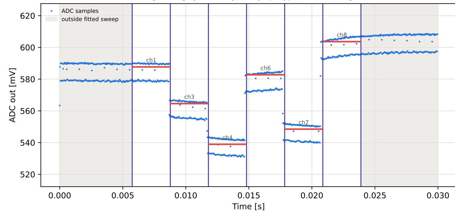
Tag9 &lt;- Tag5 | 925 MHz | run 0 | rep 1 | phase -43.20 deg
