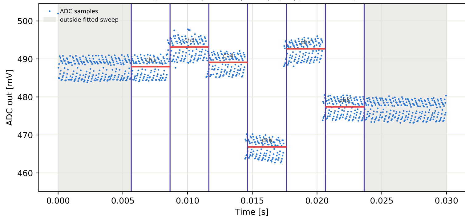
Tag1 &lt;- Tag2 | 975 MHz | run 0 | rep 1 | phase -88.77 deg
