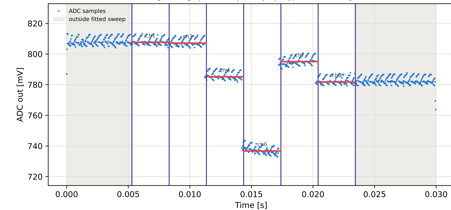
Tag8 &lt;- Tag6 | 925 MHz | run 0 | rep 1 | phase -6.50 deg
