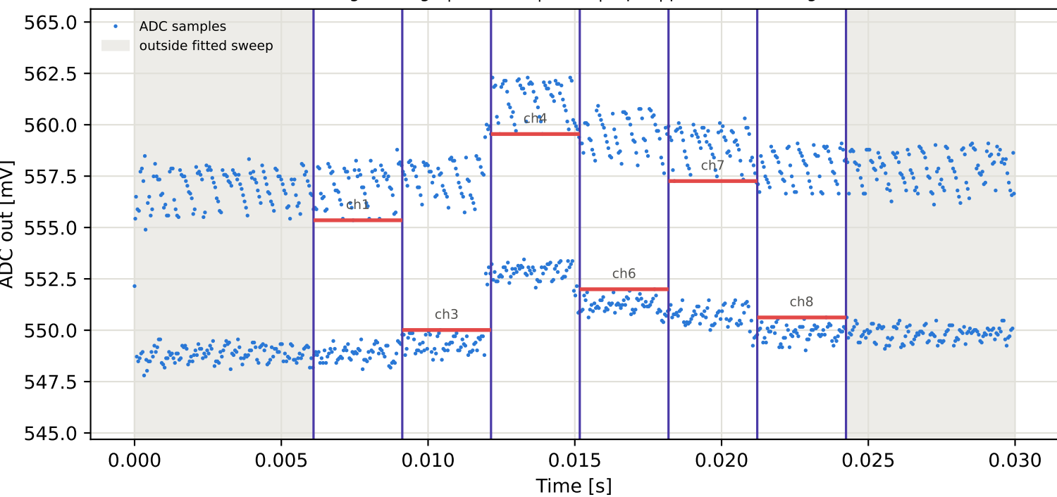
Tag8 &lt;- Tag6 | 995 MHz | run 0 | rep 1 | phase -97.52 deg
