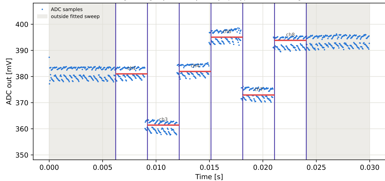
Tag6 &lt;- Tag3 | 825 MHz | run 0 | rep 1 | phase -44.34 deg
