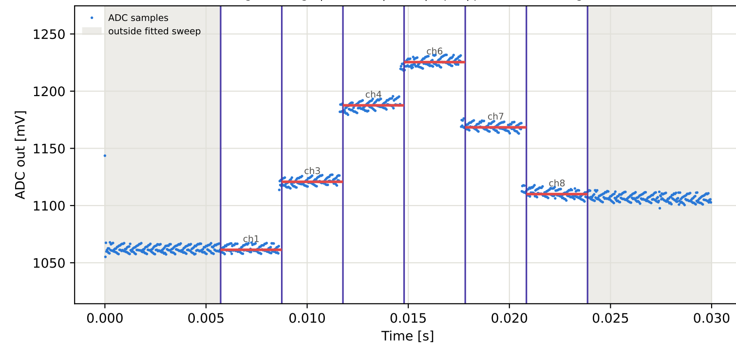
Tag2 &lt;- Tag1 | 895 MHz | run 0 | rep 1 | phase -124.14 deg
