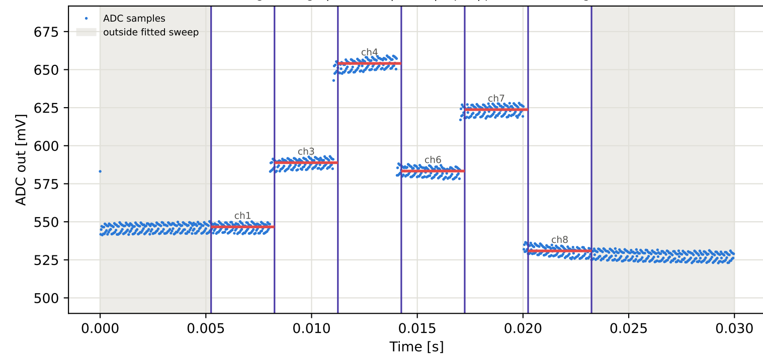
Tag3 &lt;- Tag6 | 945 MHz | run 0 | rep 1 | phase -110.90 deg
