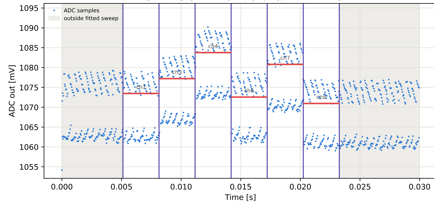
Tag15 &lt;- Tag9 | 965 MHz | run 0 | rep 1 | phase -81.97 deg
