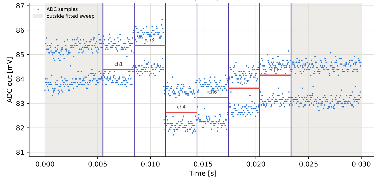
Tag10 &lt;- Tag2 | 825 MHz | run 0 | rep 1 | phase 135.28 deg
