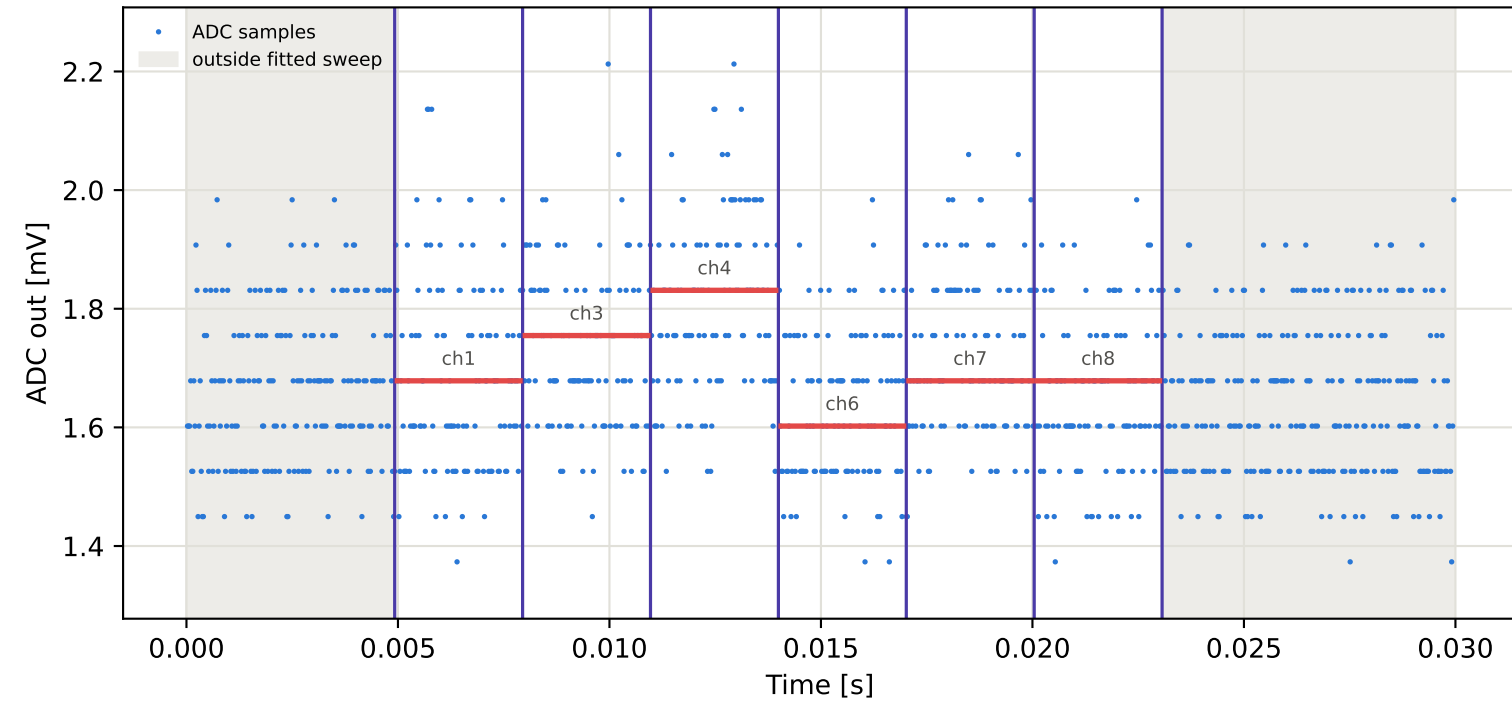
Tag2 &lt;- Tag8 | 985 MHz | run 0 | rep 1 | phase -132.00 deg
