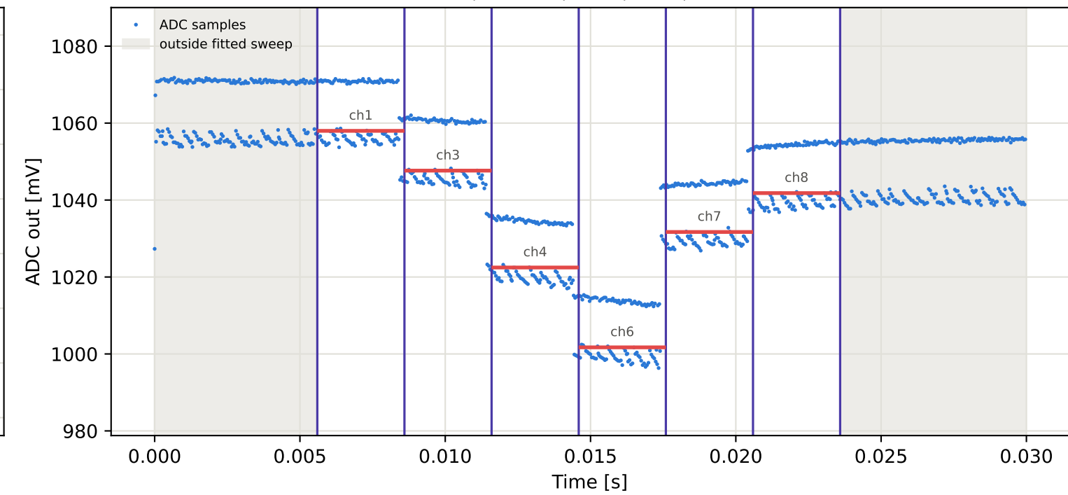
Tag10 &lt;- Tag5 | 915 MHz | run 0 | rep 1 | phase 40.83 deg
