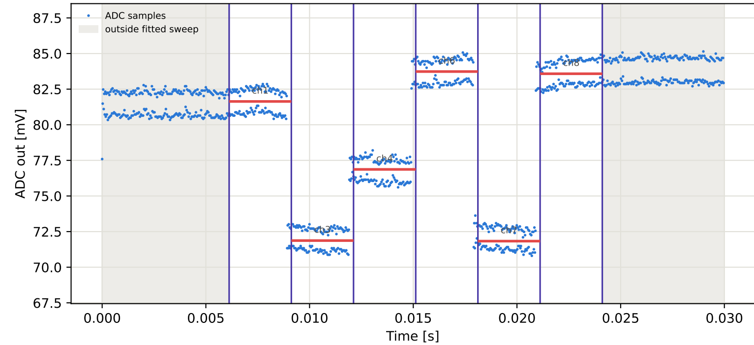
Tag3 &lt;- Tag16 | 795 MHz | run 0 | rep 1 | phase -132.52 deg
