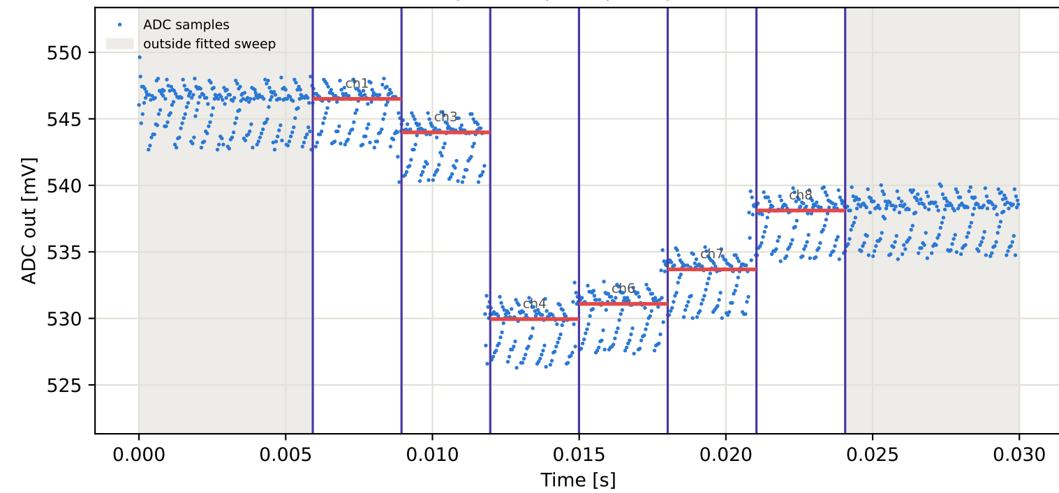
Tag8 &lt;- Tag6 | 835 MHz | run 0 | rep 1 | phase 60.33 deg
