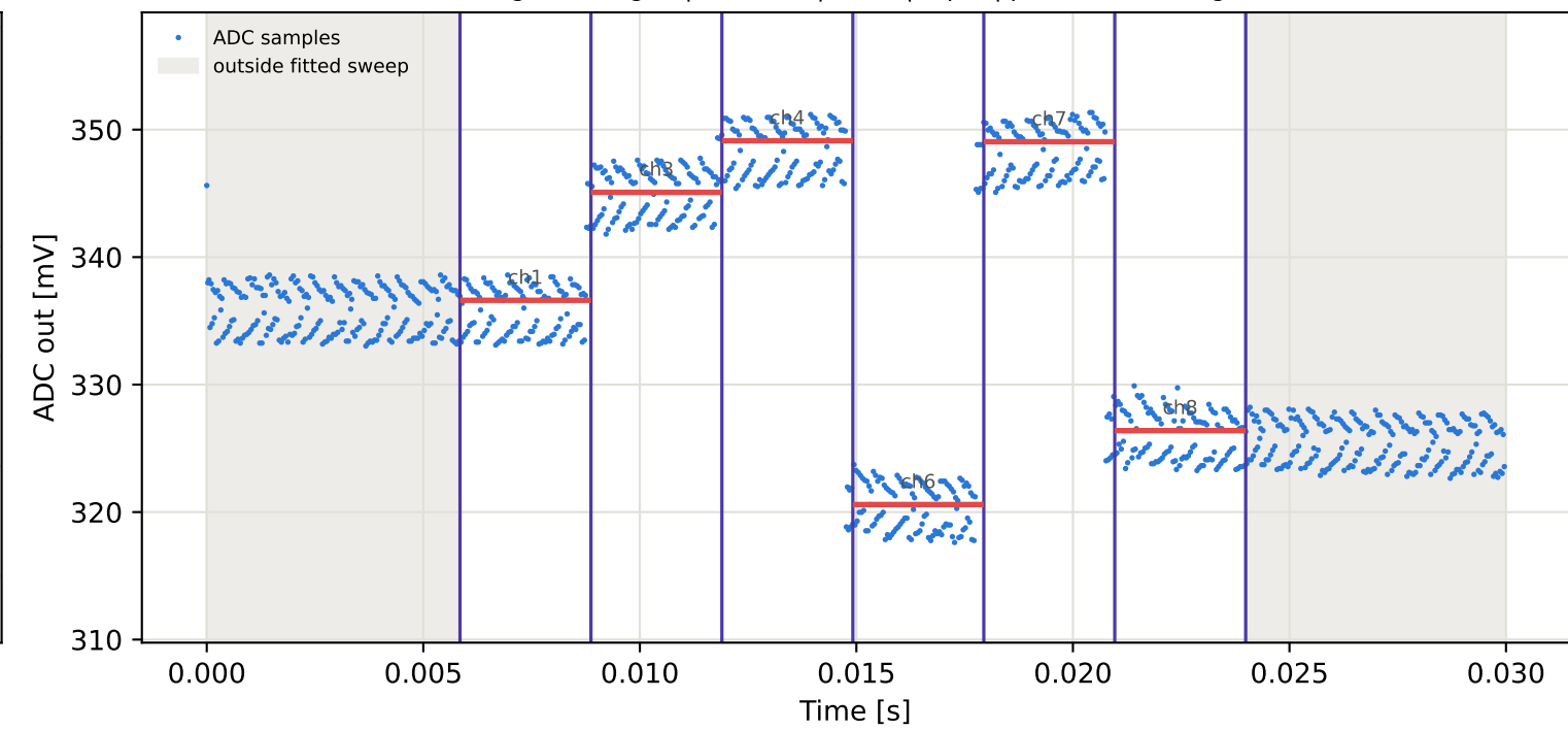
Tag10 &lt;- Tag3 | 965 MHz | run 0 | rep 1 | phase -14.95 deg
