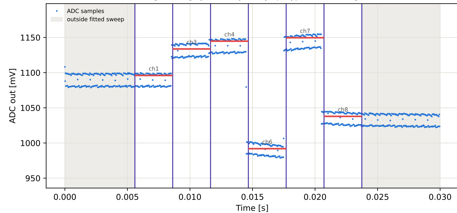
Tag2 &lt;- Tag1 | 975 MHz | run 0 | rep 1 | phase 102.22 deg
