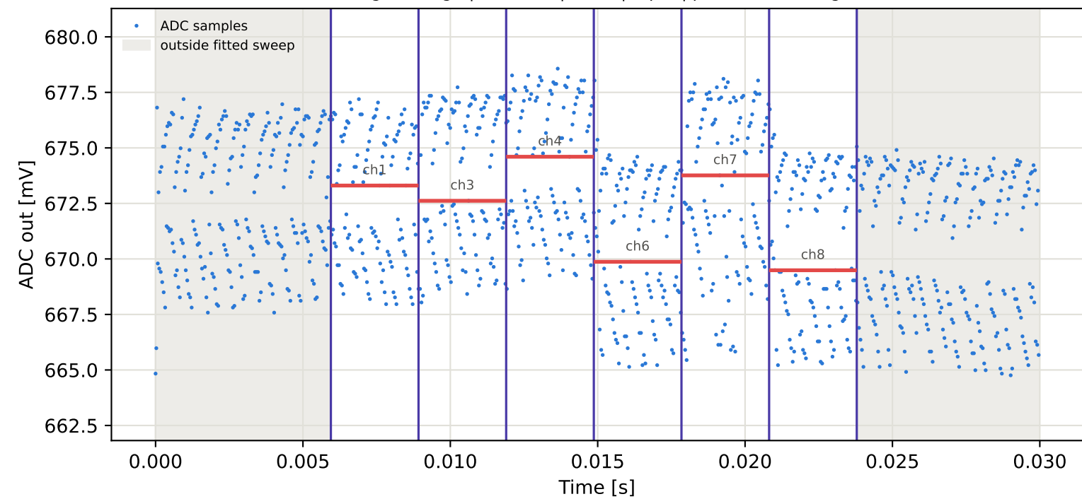
Tag7 &lt;- Tag4 | 915 MHz | run 0 | rep 1 | phase 43.24 deg
