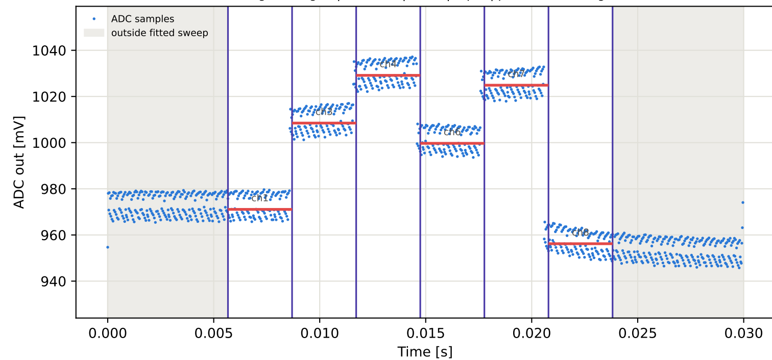
Tag3 &lt;- Tag2 | 895 MHz | run 0 | rep 1 | phase 165.72 deg
