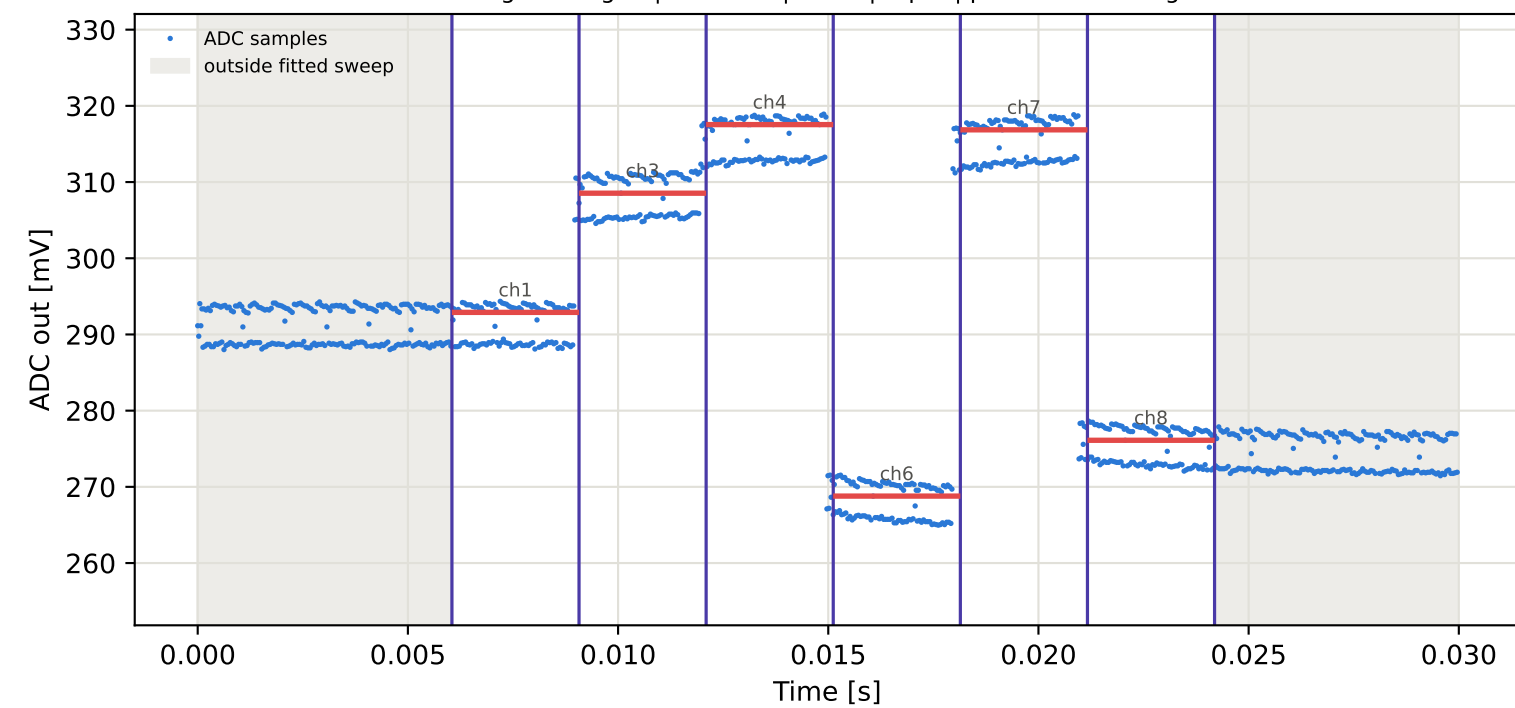
Tag6 &lt;- Tag3 | 985 MHz | run 0 | rep 1 | phase -125.03 deg
