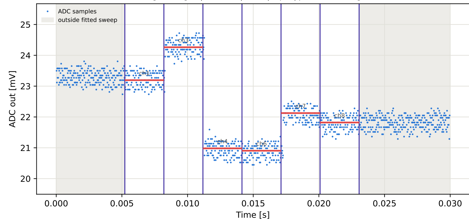
Tag1 &lt;- Tag2 | 825 MHz | run 0 | rep 1 | phase 76.00 deg
