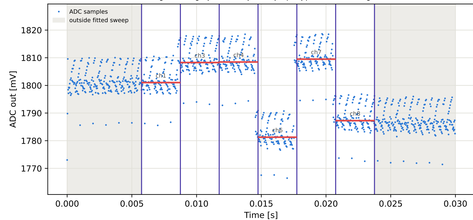
Tag15 &lt;- Tag1 | 915 MHz | run 0 | rep 1 | phase -16.77 deg
