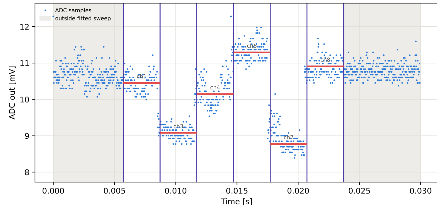
Tag10 &lt;- Tag5 | 775 MHz | run 0 | rep 1 | phase -178.51 deg
