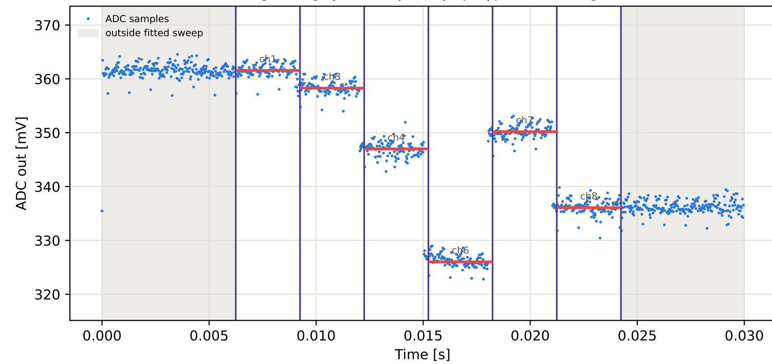
Tag4 &lt;- Tag15 | 885 MHz | run 0 | rep 1 | phase -39.87 deg
