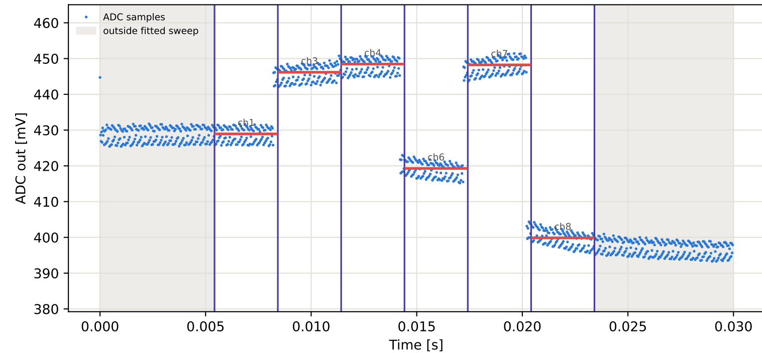
Tag1 &lt;- Tag3 | 895 MHz | run 0 | rep 1 | phase -49.45 deg
