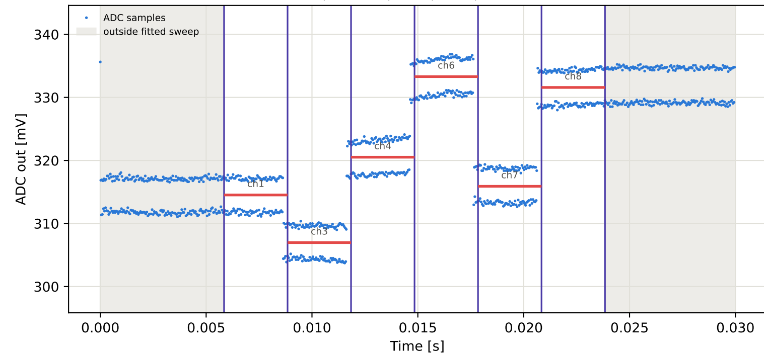
Tag4 &lt;- Tag9 | 865 MHz | run 0 | rep 1 | phase -162.67 deg
