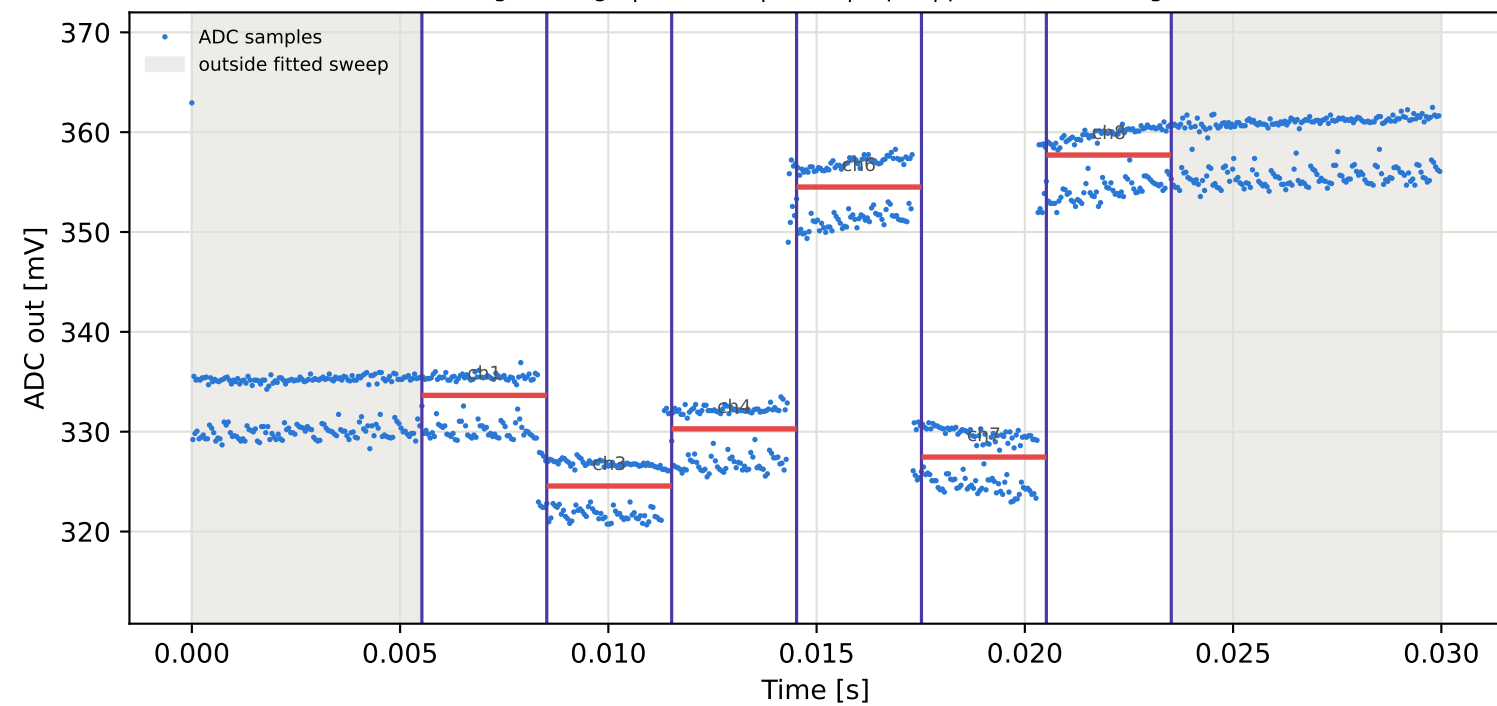
Tag2 &lt;- Tag8 | 885 MHz | run 0 | rep 1 | phase 157.22 deg
