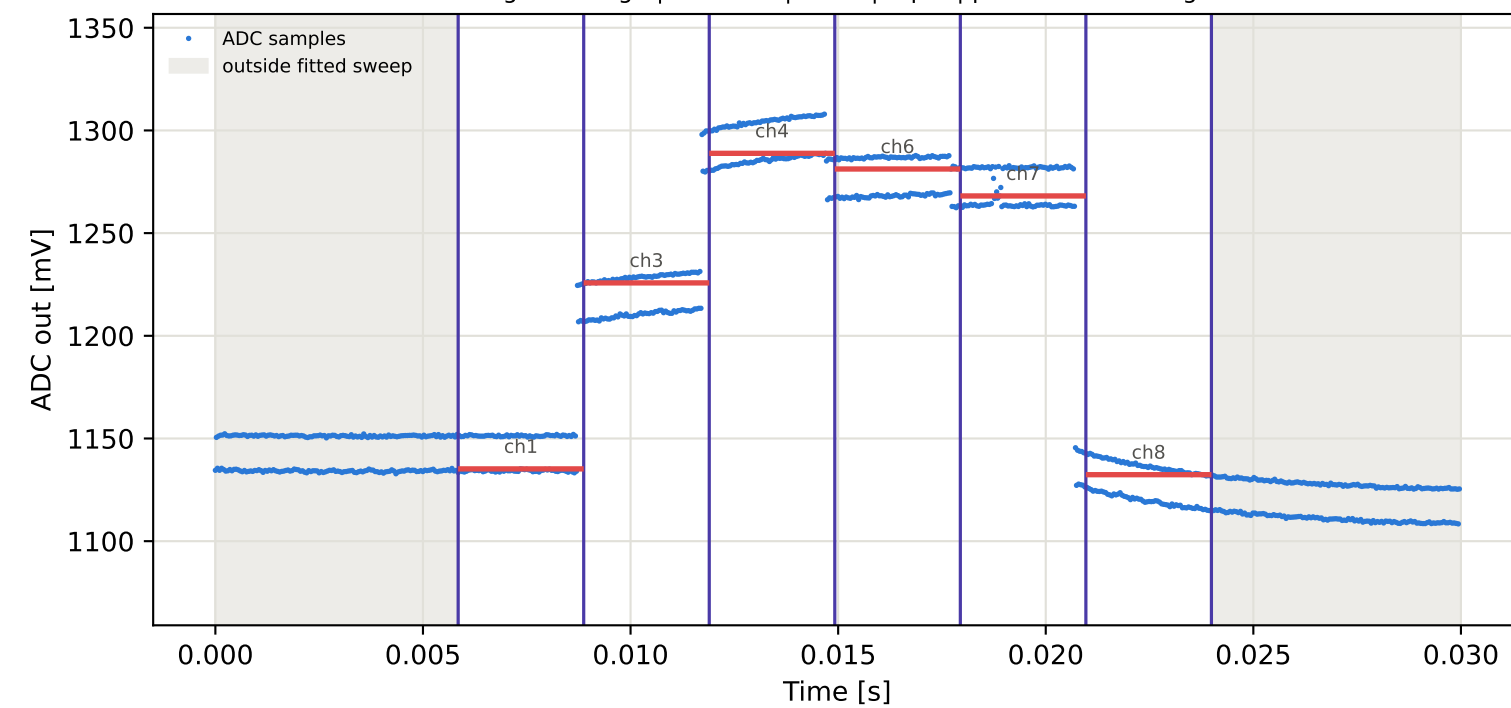
Tag2 &lt;- Tag1 | 905 MHz | run 0 | rep 1 | phase -128.48 deg
