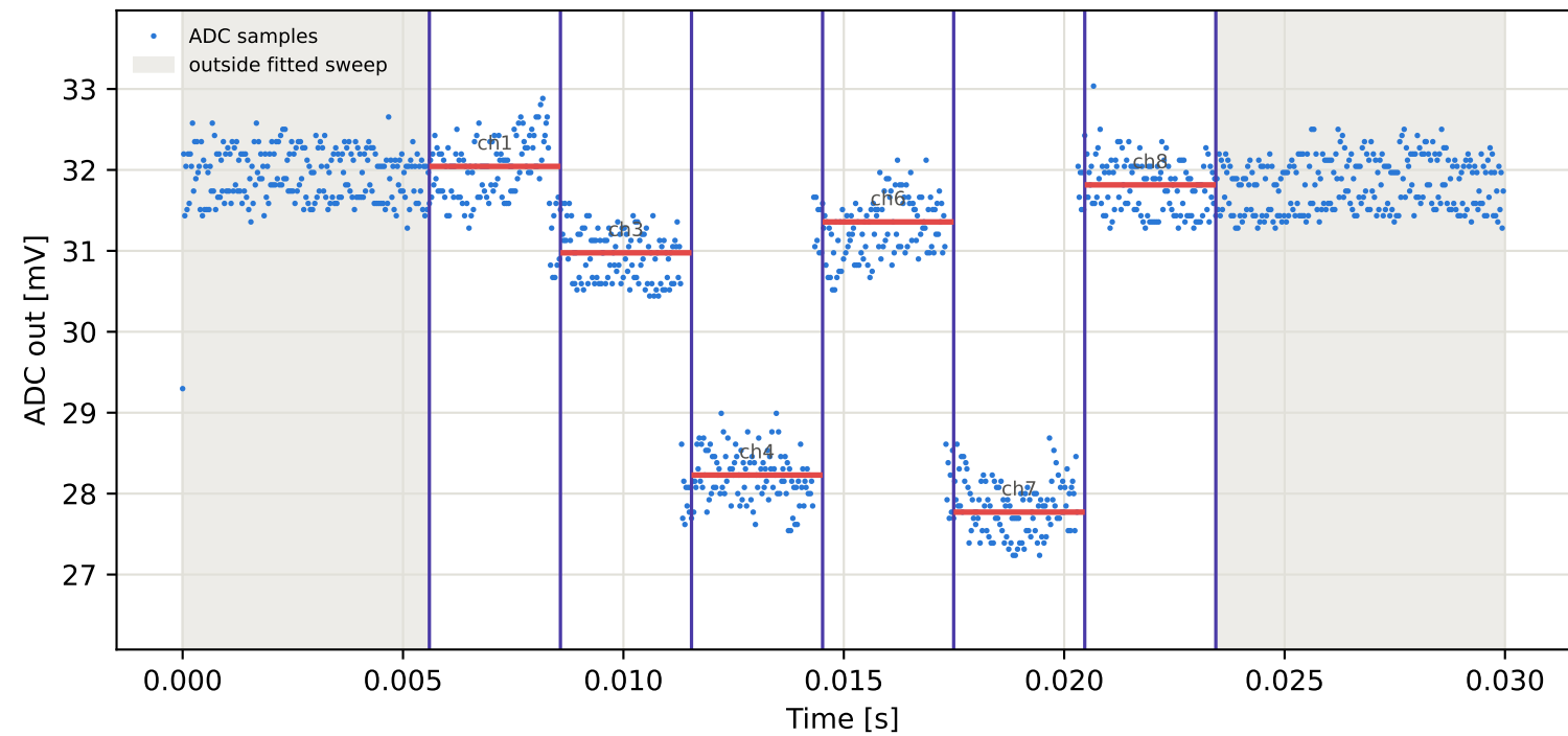
Tag6 &lt;- Tag2 | 775 MHz | run 0 | rep 1 | phase 25.58 deg
