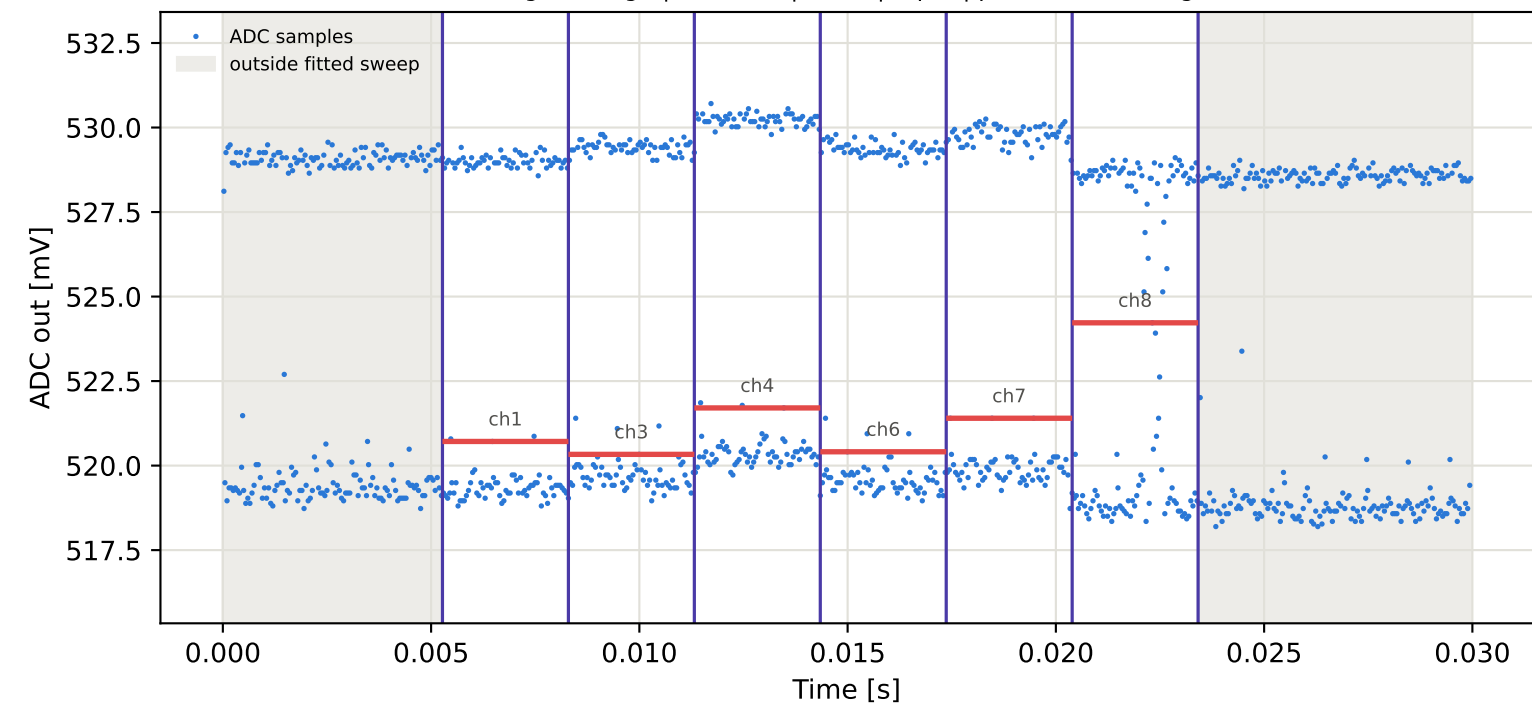
Tag7 &lt;- Tag4 | 975 MHz | run 0 | rep 1 | phase 136.26 deg
