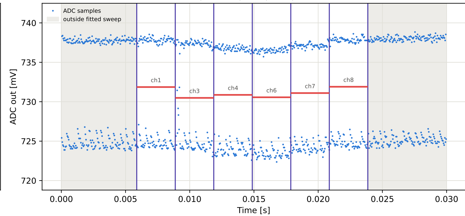
Tag9 &lt;- Tag2 | 935 MHz | run 0 | rep 1 | phase 69.76 deg
