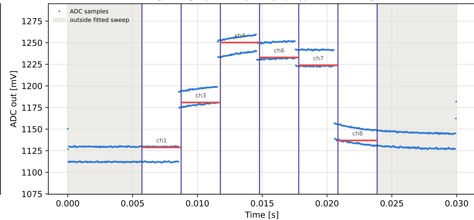
Tag5 &lt;- Tag2 | 895 MHz | run 0 | rep 1 | phase 175.14 deg
