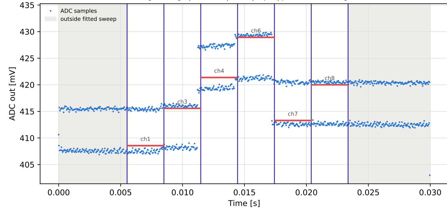
Tag1 &lt;- Tag9 | 965 MHz | run 0 | rep 1 | phase 28.86 deg
