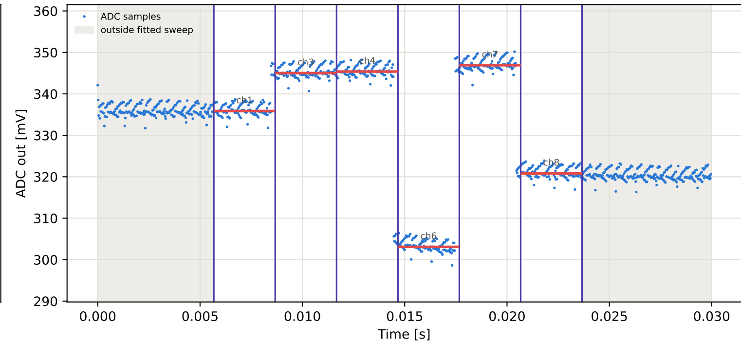
Tag10 &lt;- Tag5 | 965 MHz | run 0 | rep 1 | phase 54.72 deg
