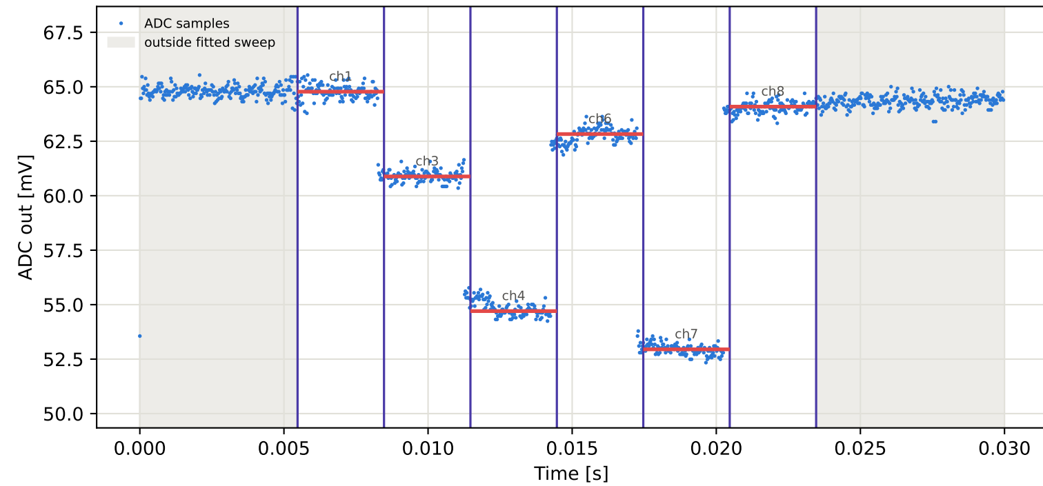
Tag10 &lt;- Tag5 | 785 MHz | run 0 | rep 1 | phase -139.31 deg
