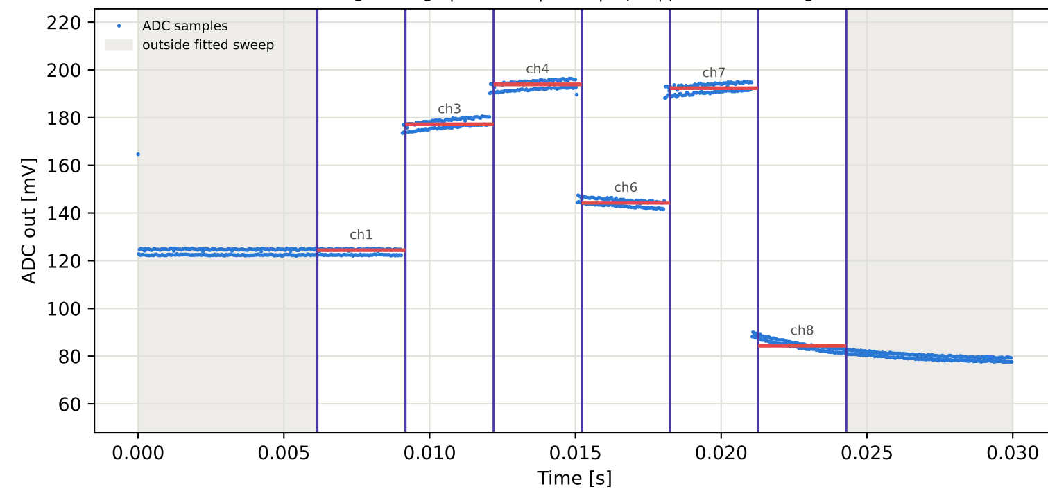
Tag1 &lt;- Tag3 | 875 MHz | run 0 | rep 1 | phase -66.86 deg
