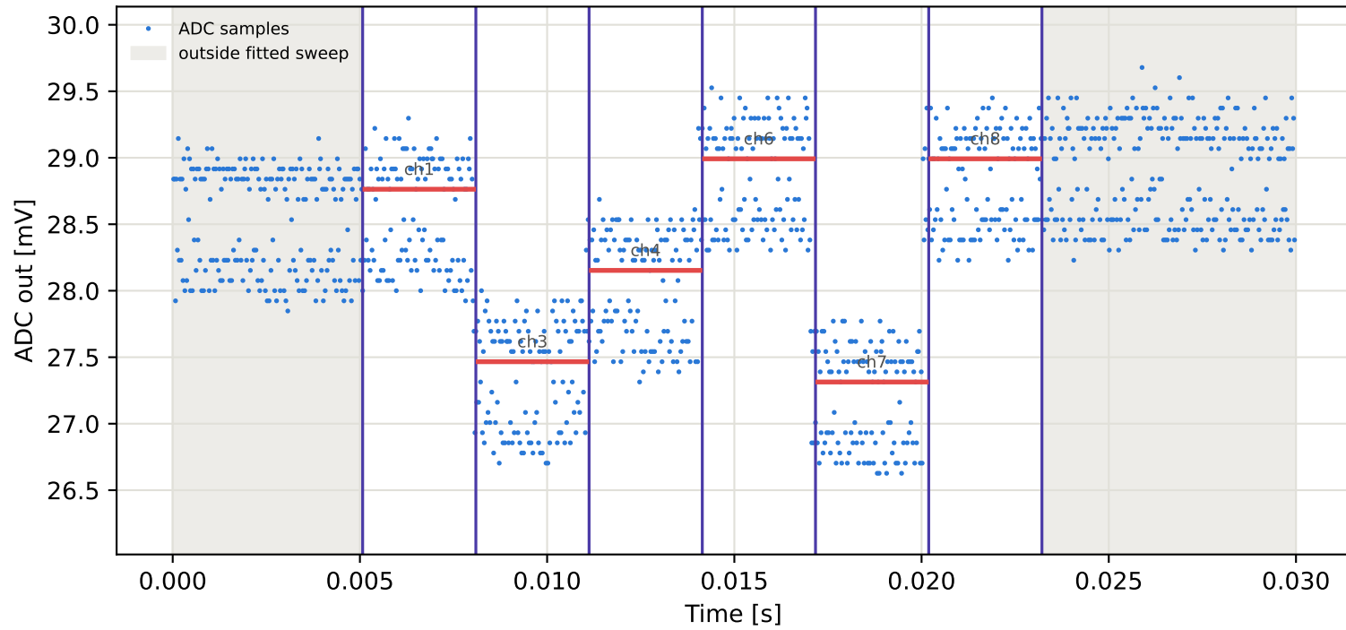
Tag2 &lt;- Tag16 | 785 MHz | run 0 | rep 1 | phase 15.62 deg
