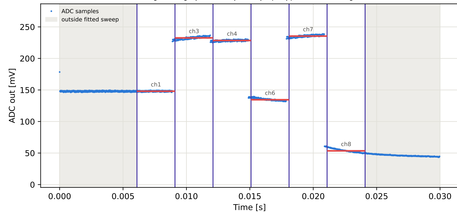
Tag9 &lt;- Tag8 | 875 MHz | run 0 | rep 1 | phase -42.94 deg
