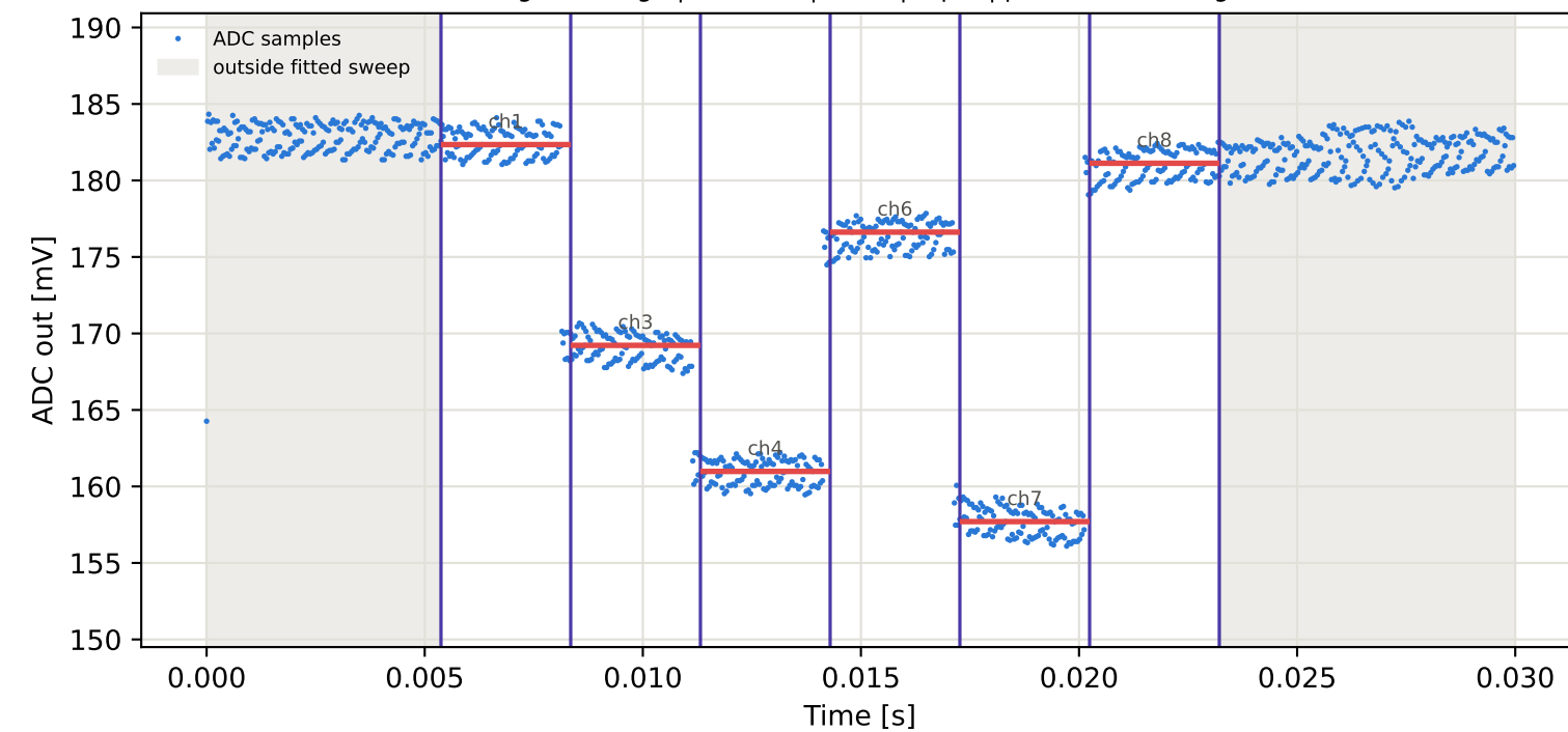
Tag15 &lt;- Tag5 | 785 MHz | run 0 | rep 1 | phase 118.64 deg
