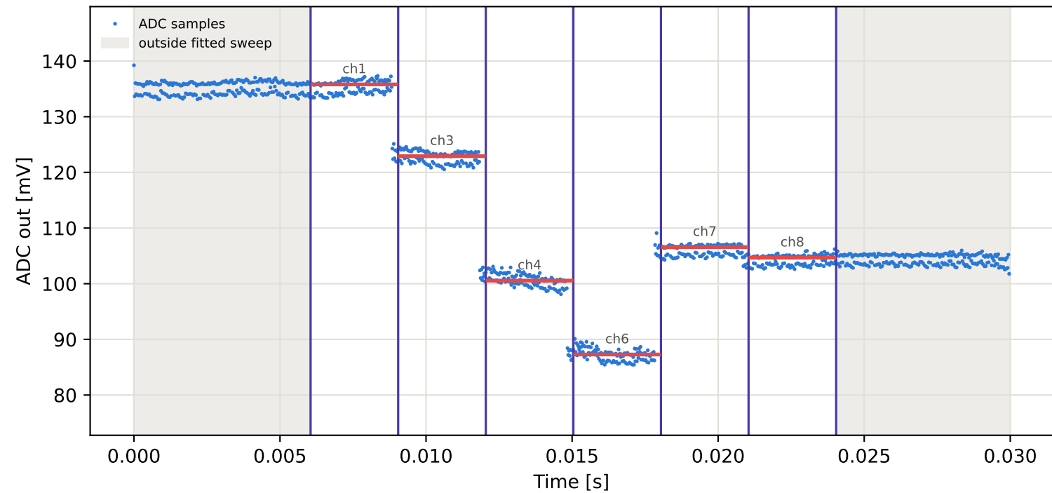
Tag15 &lt;- Tag1 | 875 MHz | run 0 | rep 1 | phase 139.23 deg
