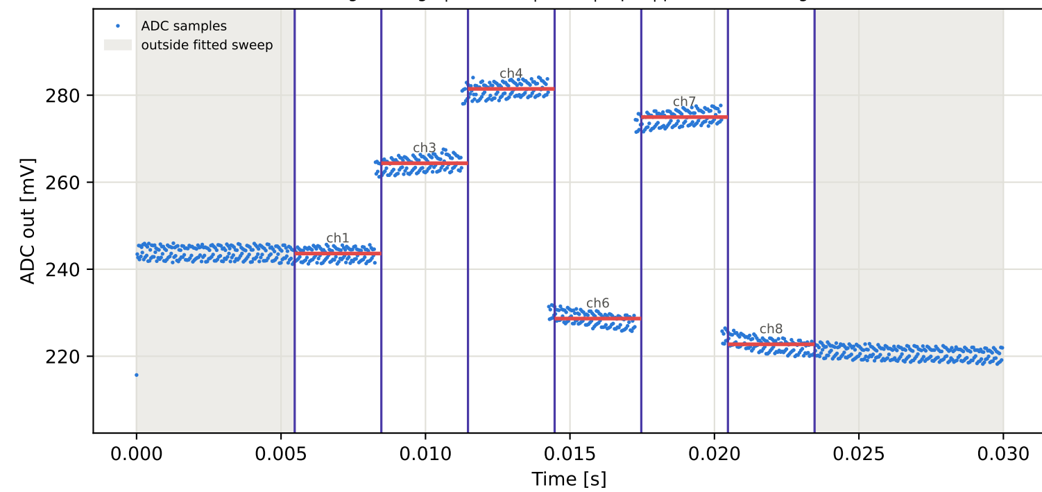
Tag1 &lt;- Tag4 | 925 MHz | run 0 | rep 1 | phase -51.15 deg
