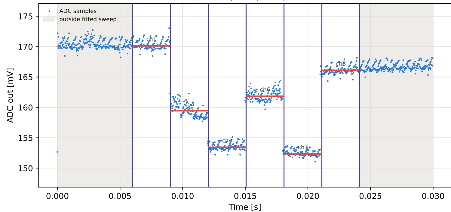
Tag6 &lt;- Tag2 | 845 MHz | run 0 | rep 1 | phase -90.58 deg
