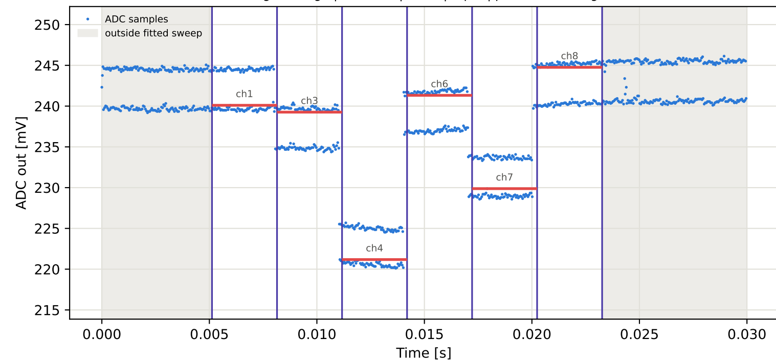
Tag5 &lt;- Tag3 | 995 MHz | run 0 | rep 1 | phase 84.90 deg
