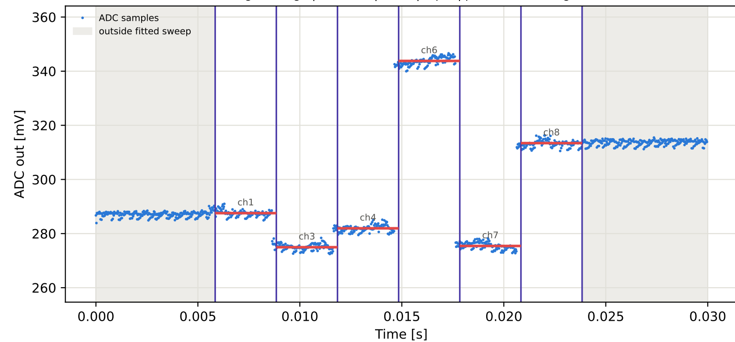
Tag6 &lt;- Tag5 | 955 MHz | run 0 | rep 1 | phase 133.66 deg
