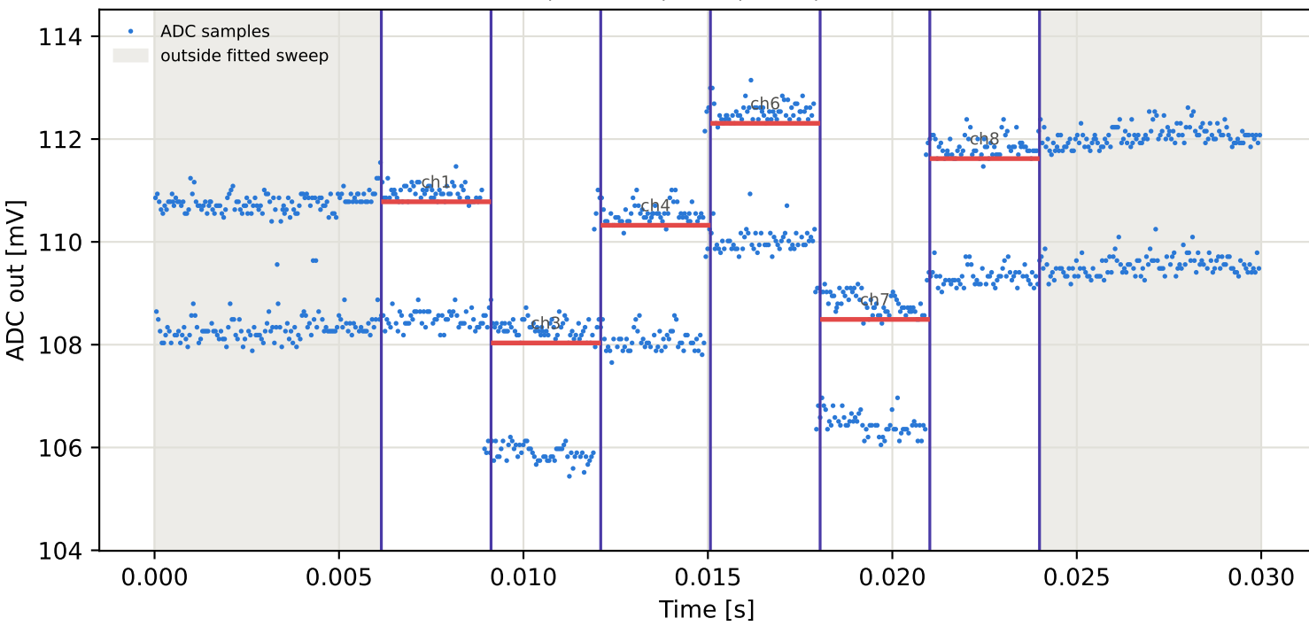
Tag3 &lt;- Tag16 | 795 MHz | run 0 | rep 1 | phase -174.46 deg
