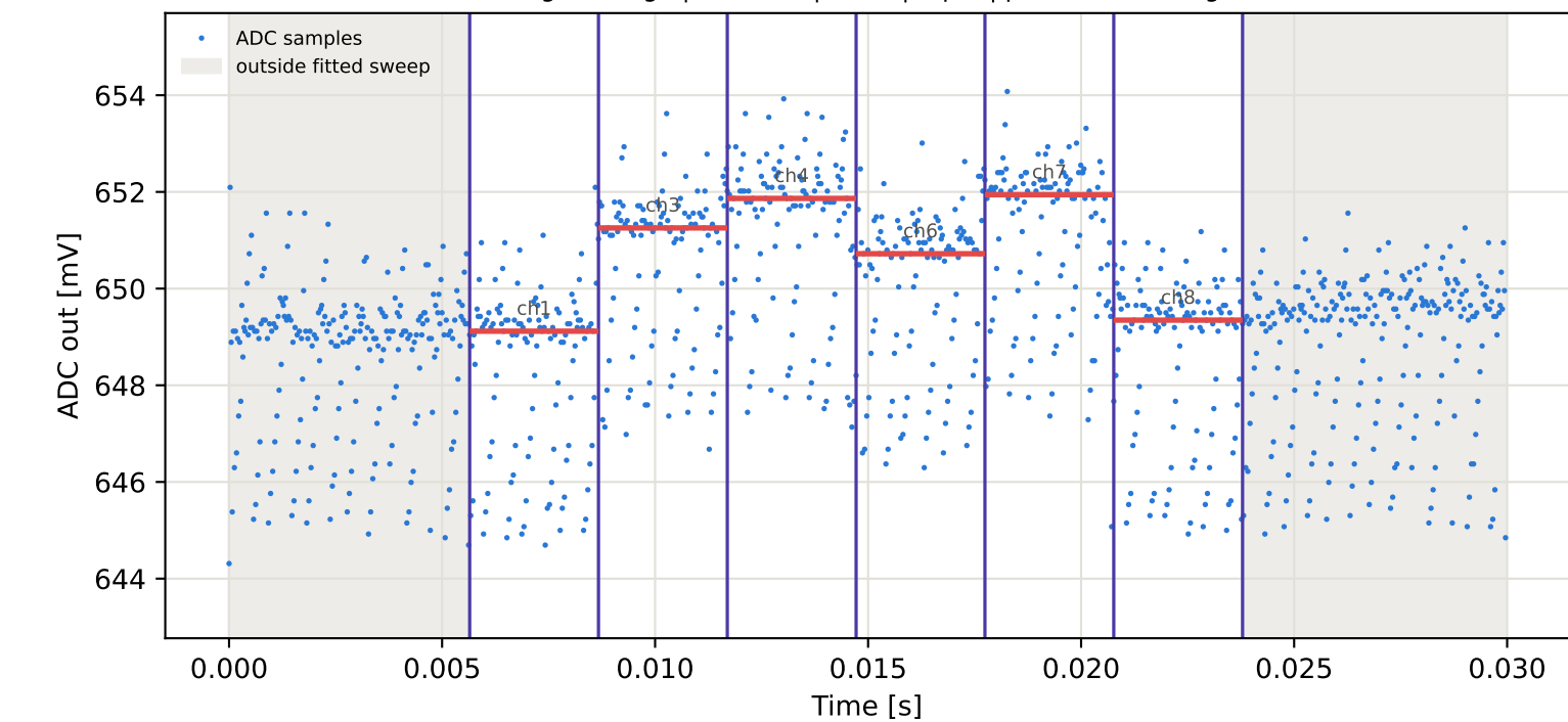
Tag8 &lt;- Tag6 | 845 MHz | run 0 | rep 1 | phase -79.50 deg
