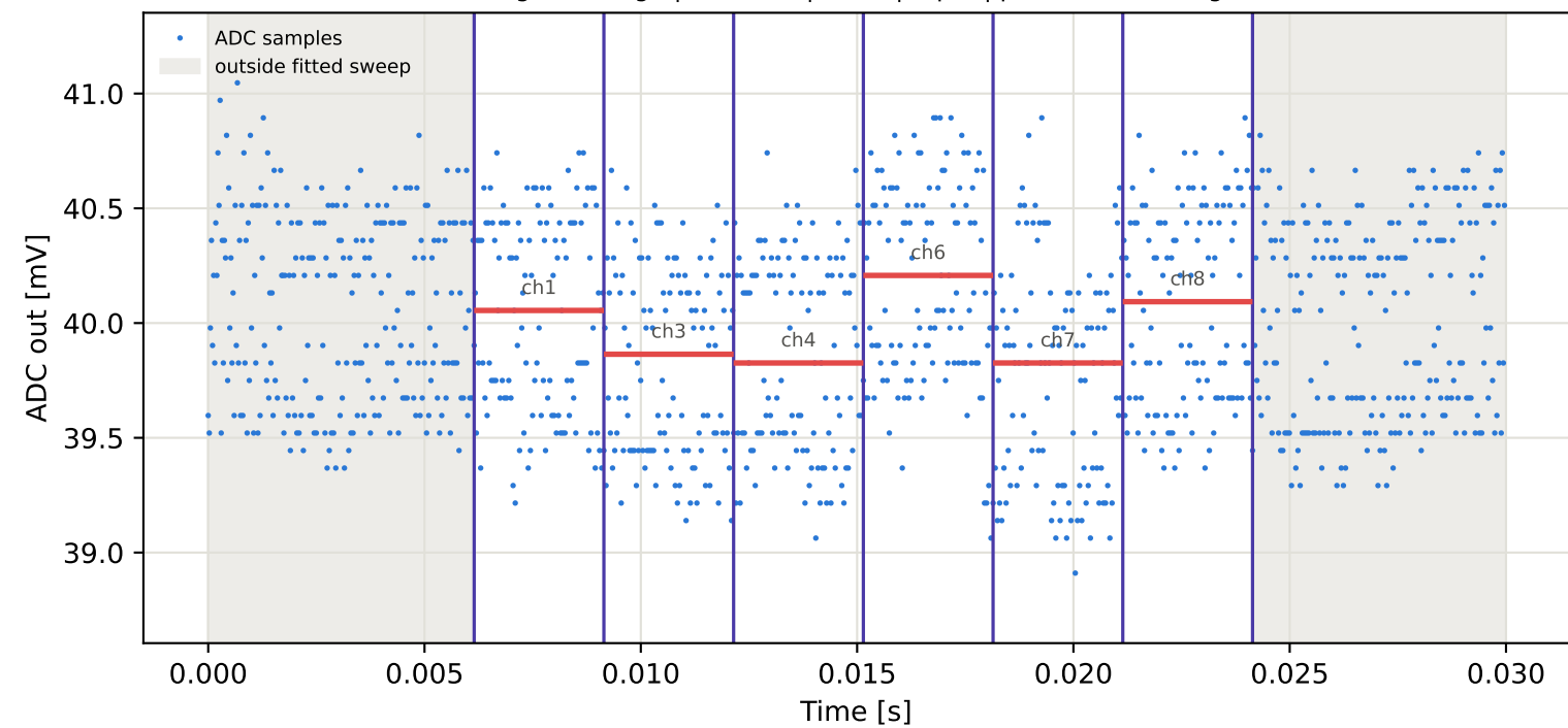
Tag16 &lt;- Tag15 | 785 MHz | run 0 | rep 1 | phase 89.36 deg
