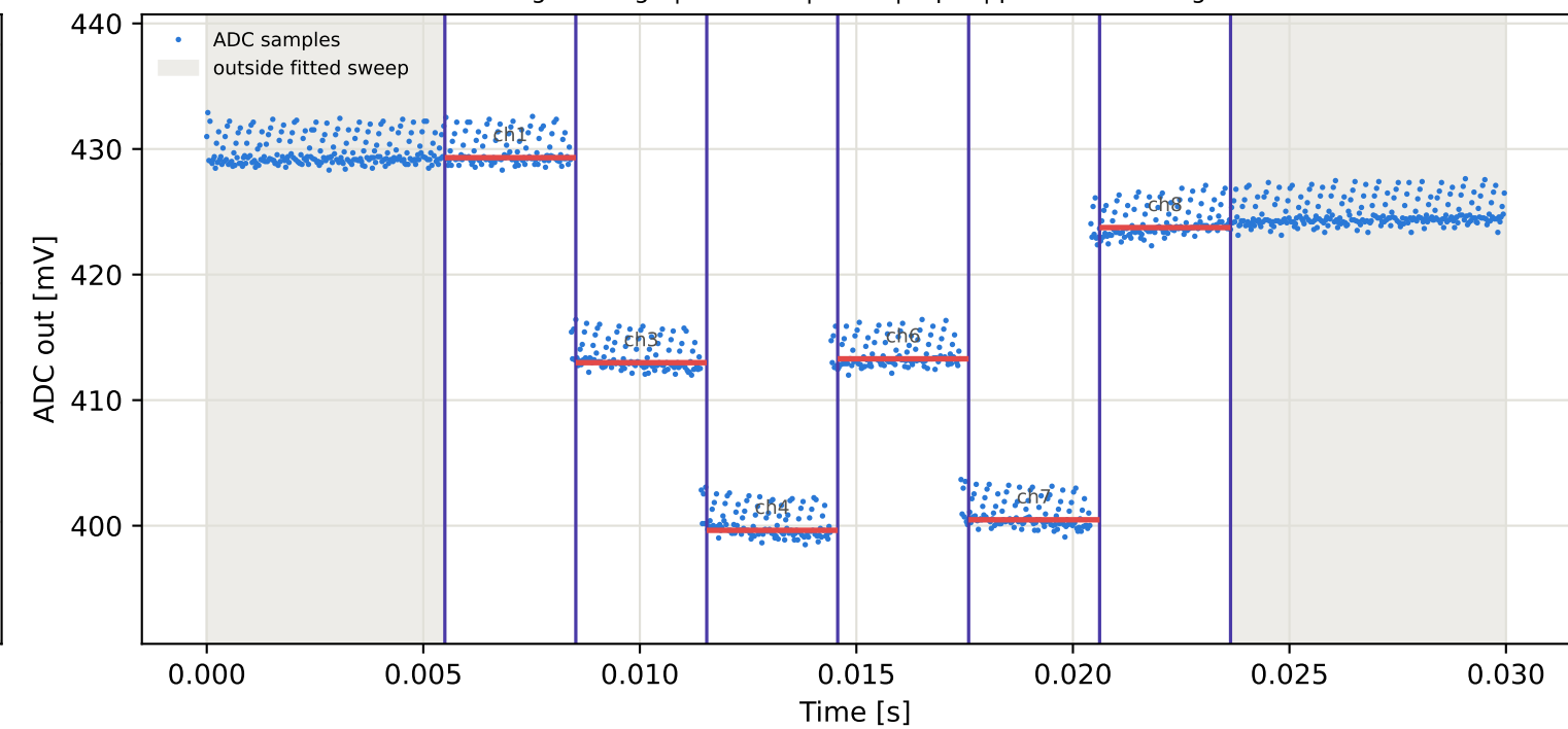
Tag3 &lt;- Tag7 | 845 MHz | run 0 | rep 1 | phase 124.05 deg
