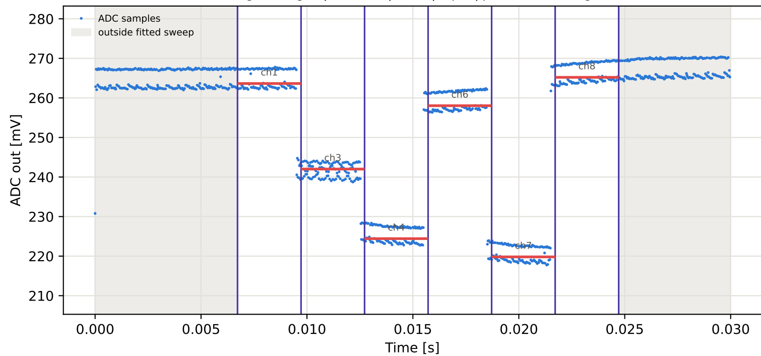
Tag5 &lt;- Tag2 | 805 MHz | run 0 | rep 1 | phase 61.64 deg
