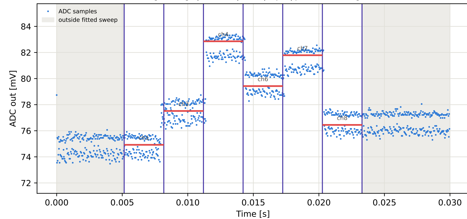
Tag1 &lt;- Tag7 | 805 MHz | run 0 | rep 1 | phase -75.83 deg
