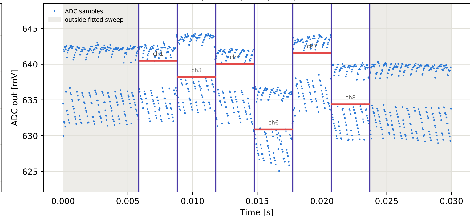
Tag8 &lt;- Tag5 | 985 MHz | run 0 | rep 1 | phase 134.93 deg
