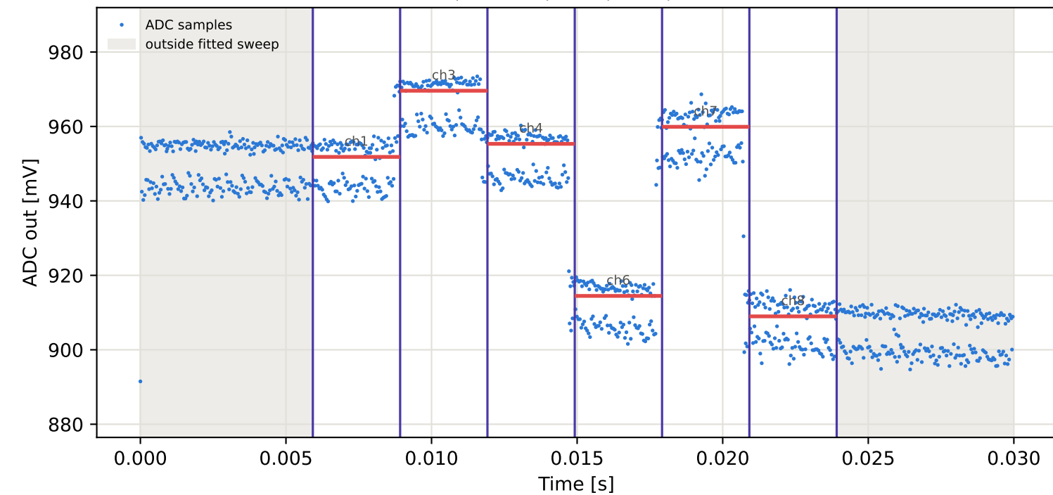
Tag4 &lt;- Tag9 | 885 MHz | run 0 | rep 1 | phase -5.15 deg
