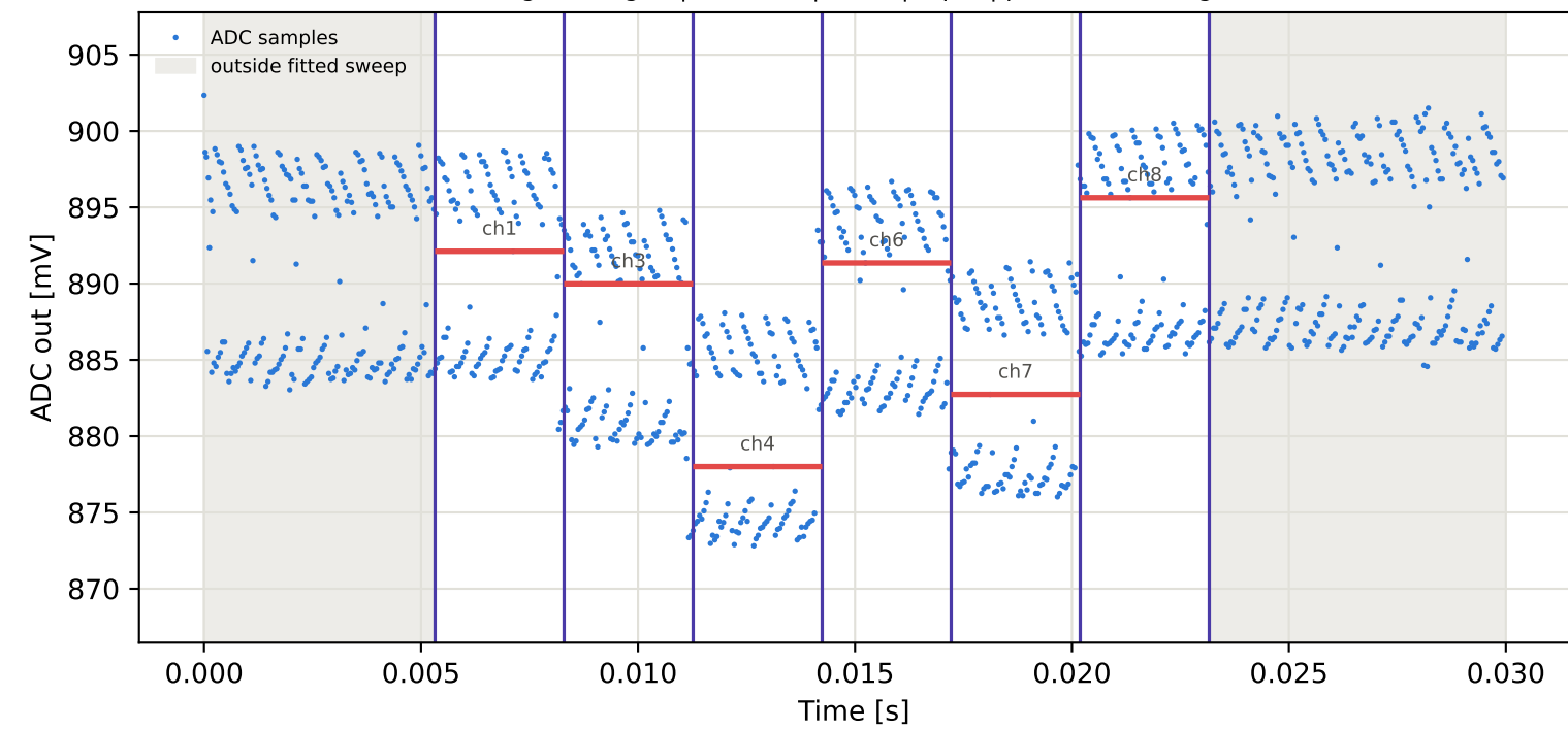
Tag4 &lt;- Tag16 | 945 MHz | run 0 | rep 1 | phase -33.54 deg
