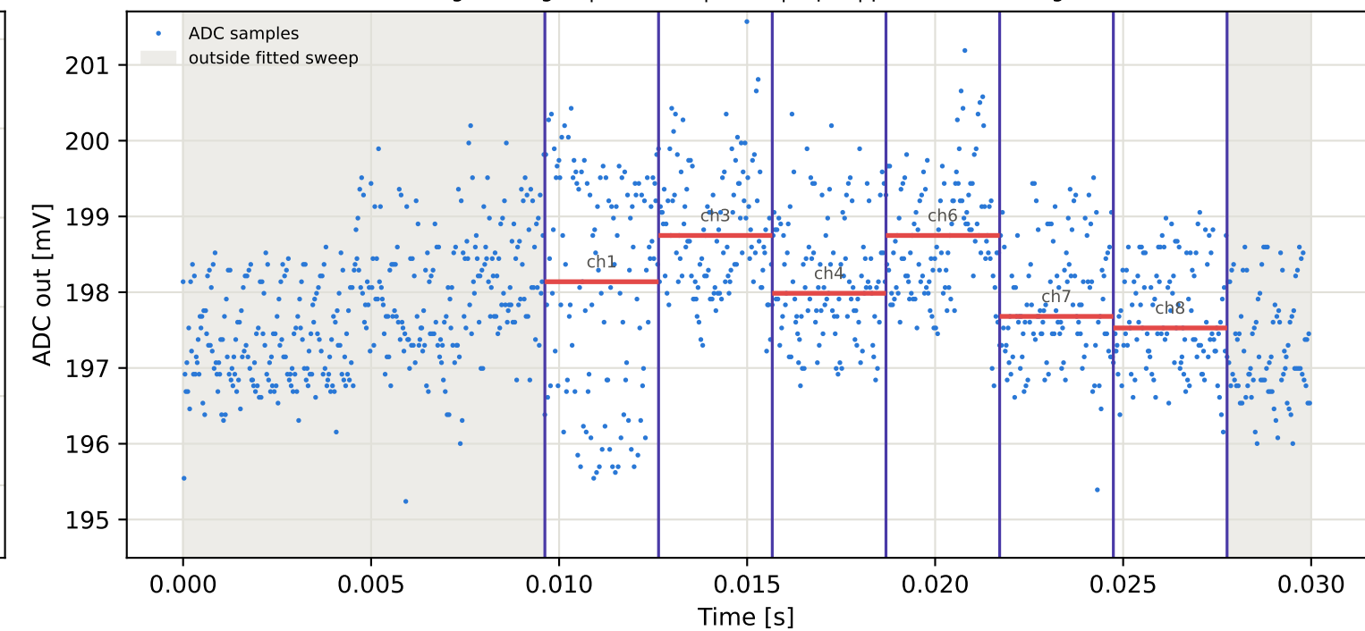
Tag7 &lt;- Tag15 | 805 MHz | run 0 | rep 1 | phase 151.65 deg
