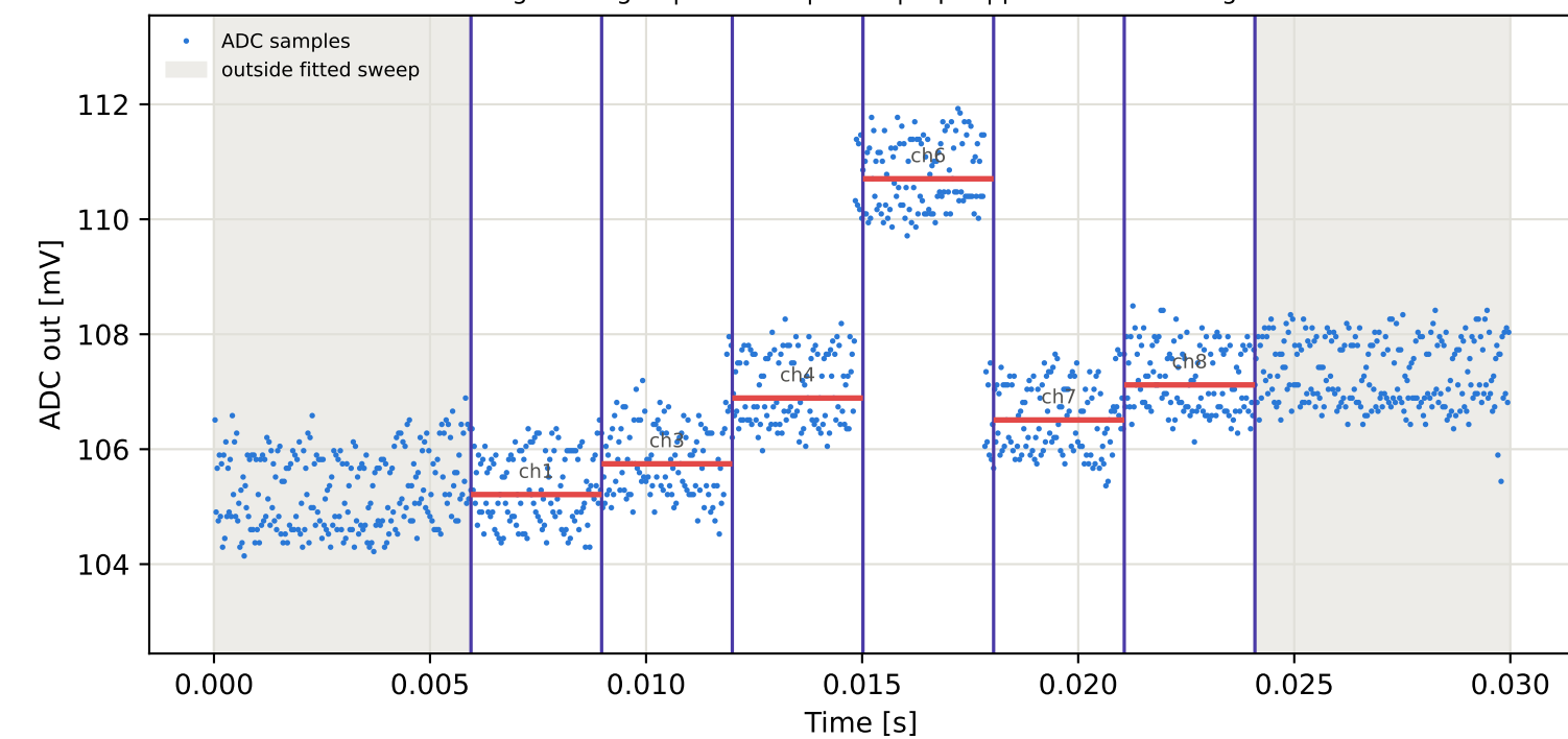
Tag2 &lt;- Tag16 | 915 MHz | run 0 | rep 1 | phase -156.56 deg
