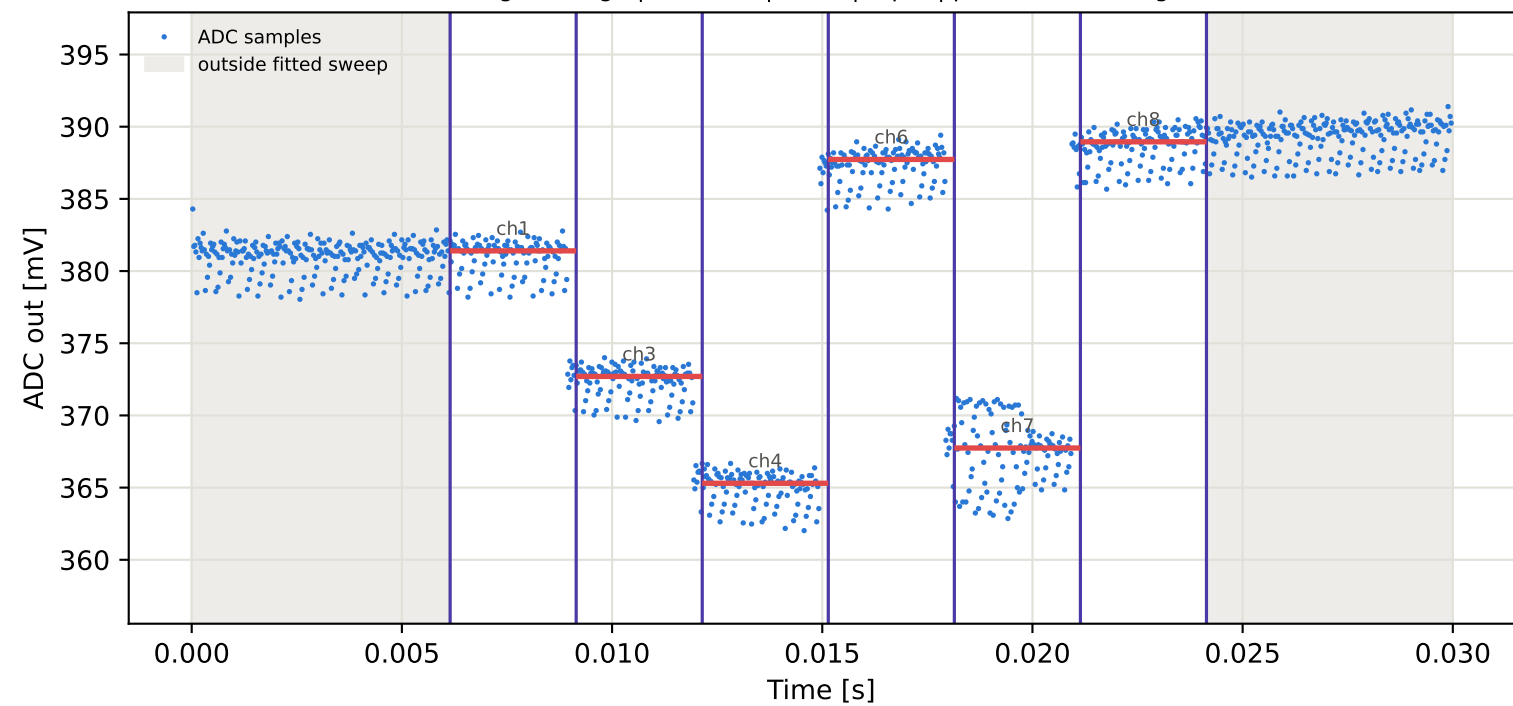
Tag3 &lt;- Tag9 | 935 MHz | run 0 | rep 1 | phase 2.41 deg
