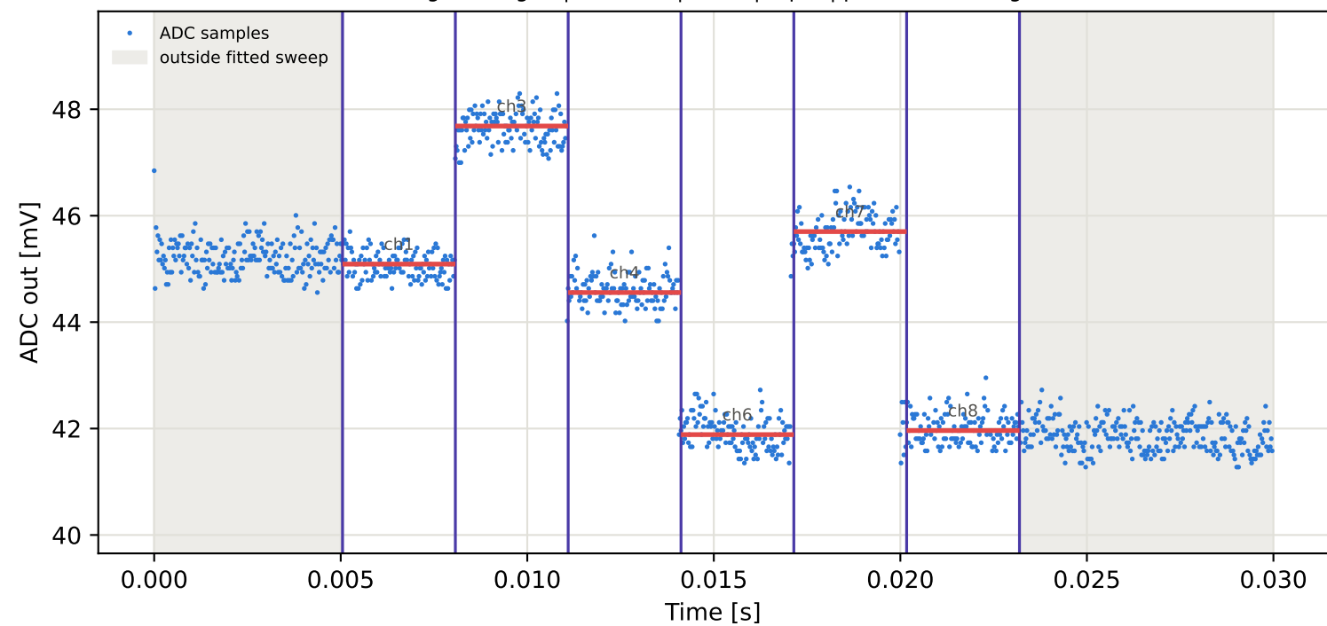
Tag2 &lt;- Tag16 | 855 MHz | run 0 | rep 1 | phase 11.27 deg
