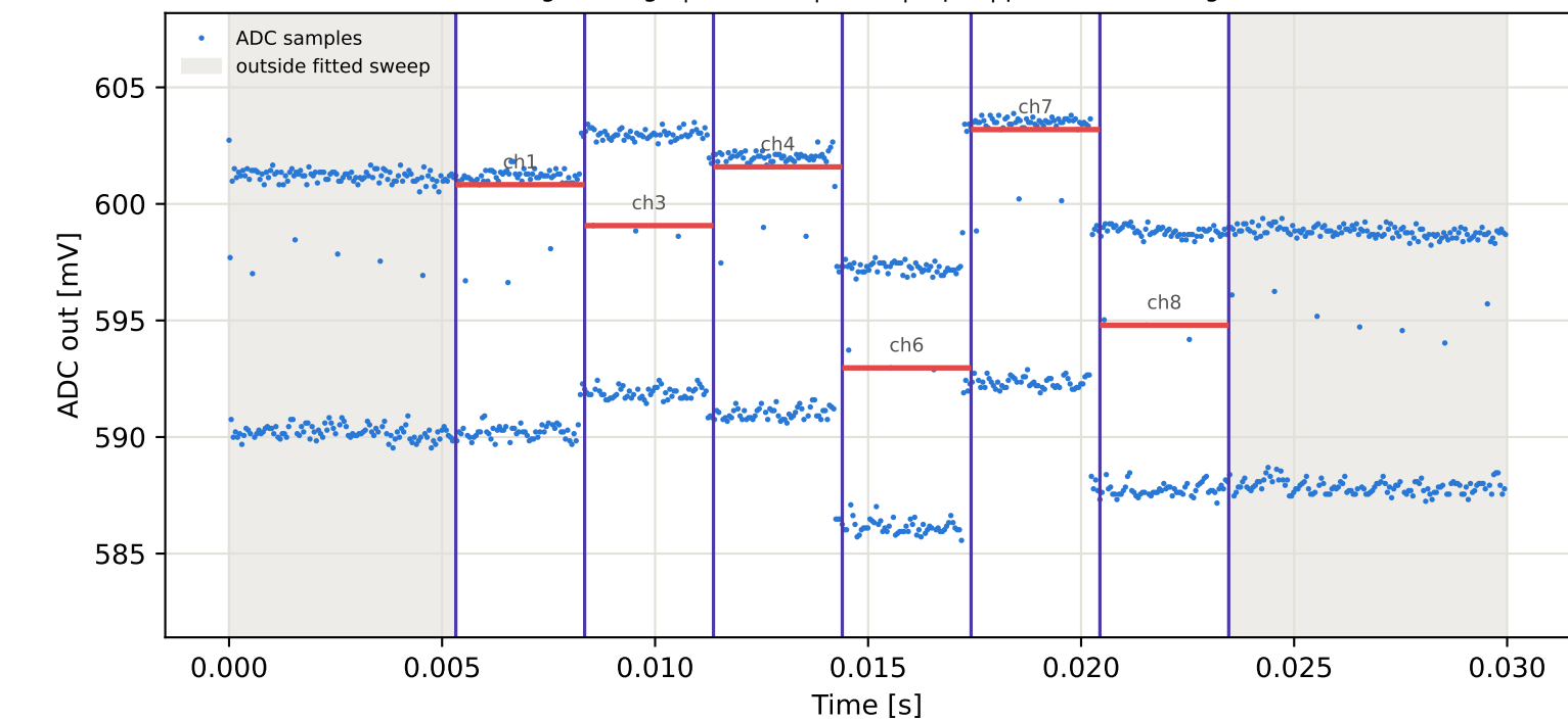
Tag8 &lt;- Tag6 | 995 MHz | run 0 | rep 1 | phase -24.73 deg
