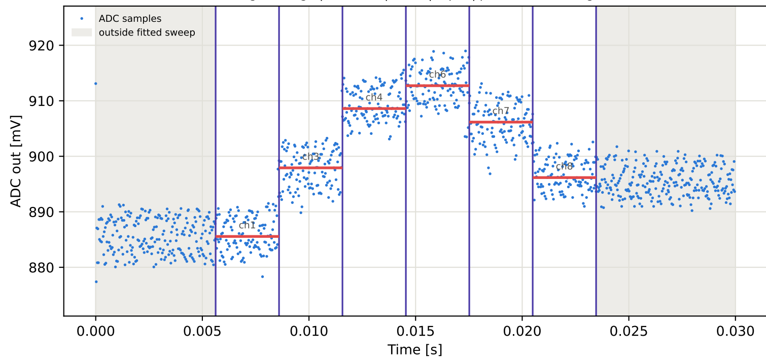
Tag7 &lt;- Tag1 | 885 MHz | run 0 | rep 1 | phase -49.01 deg
