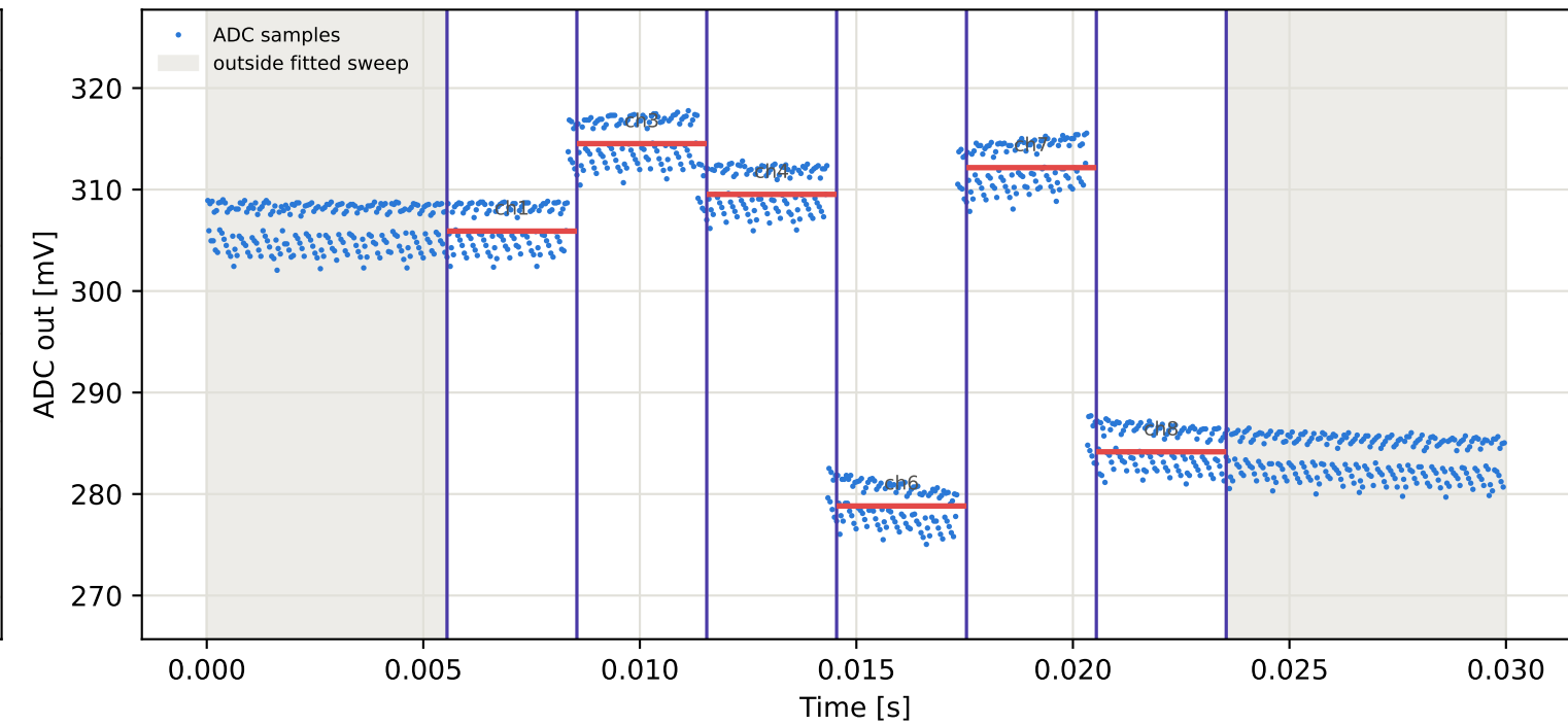
Tag3 &lt;- Tag9 | 905 MHz | run 0 | rep 1 | phase -75.33 deg
