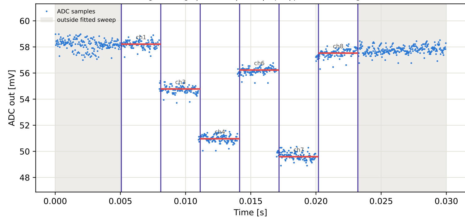
Tag16 &lt;- Tag7 | 775 MHz | run 0 | rep 1 | phase -45.39 deg
