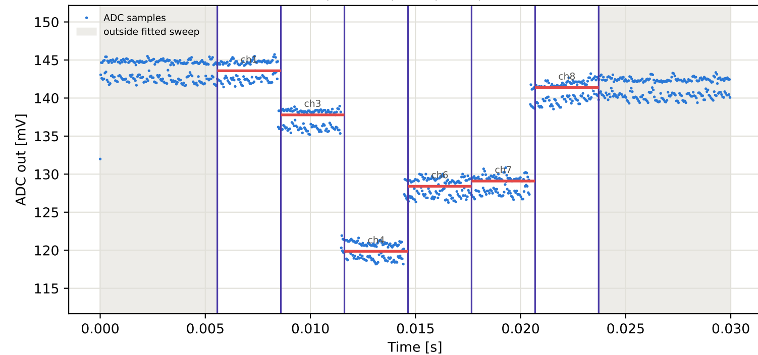
Tag6 &lt;- Tag1 | 965 MHz | run 0 | rep 1 | phase 62.89 deg
