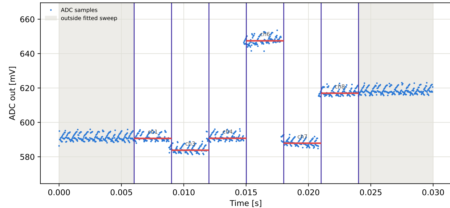
Tag6 &lt;- Tag1 | 925 MHz | run 0 | rep 1 | phase -18.46 deg
