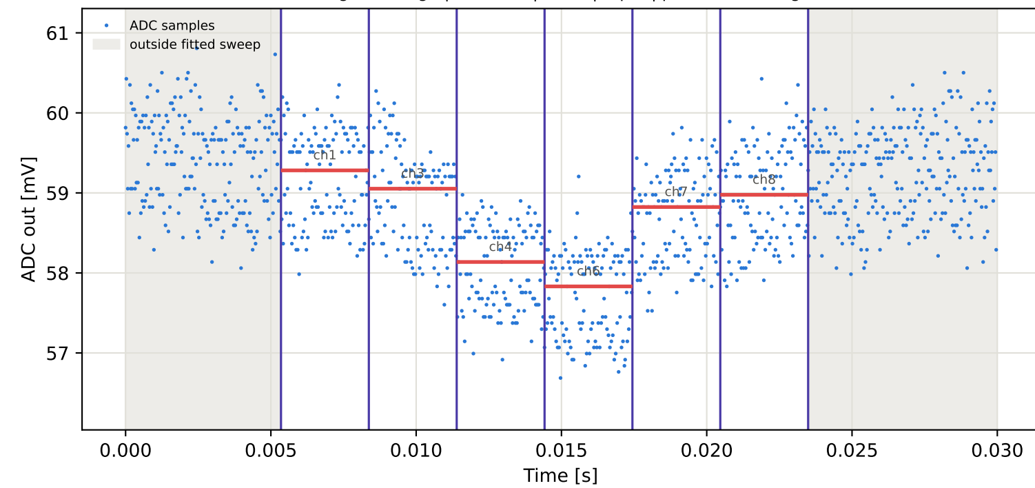
Tag10 &lt;- Tag4 | 785 MHz | run 0 | rep 1 | phase 58.96 deg
