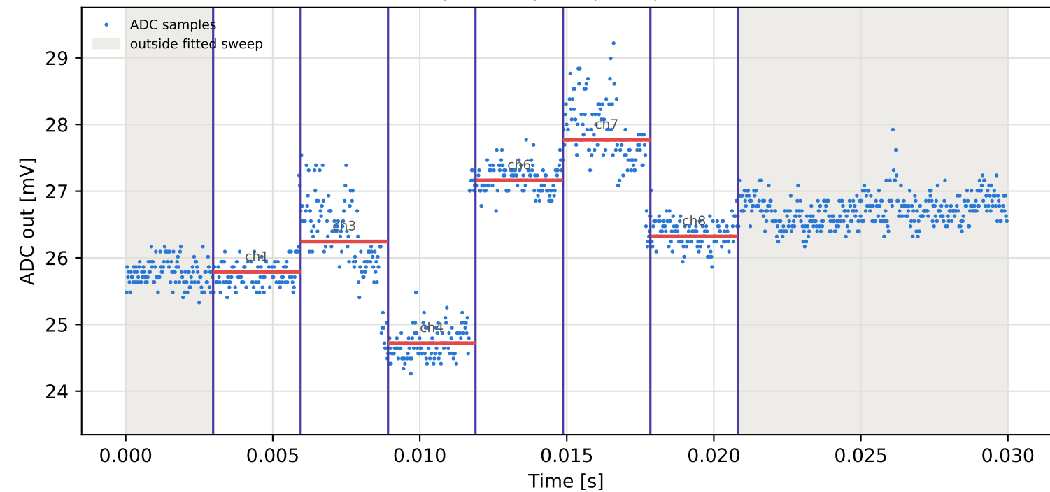
Tag2 &lt;- Tag16 | 805 MHz | run 0 | rep 1 | phase 158.31 deg
