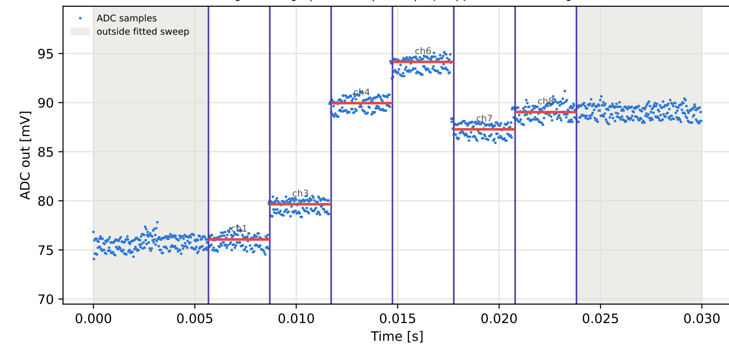
Tag10 &lt;- Tag1 | 865 MHz | run 0 | rep 1 | phase -135.10 deg
