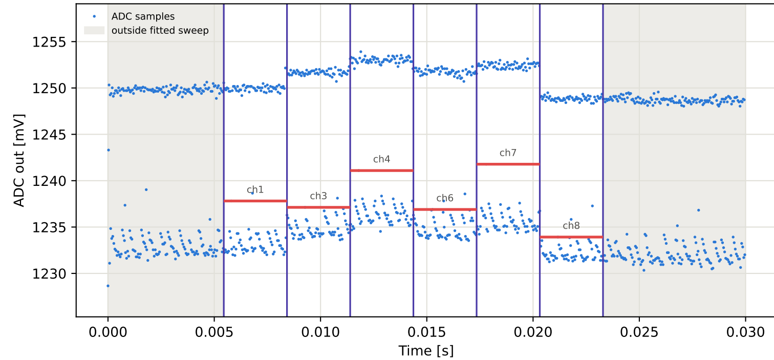
Tag16 &lt;- Tag15 | 895 MHz | run 0 | rep 1 | phase -124.14 deg
