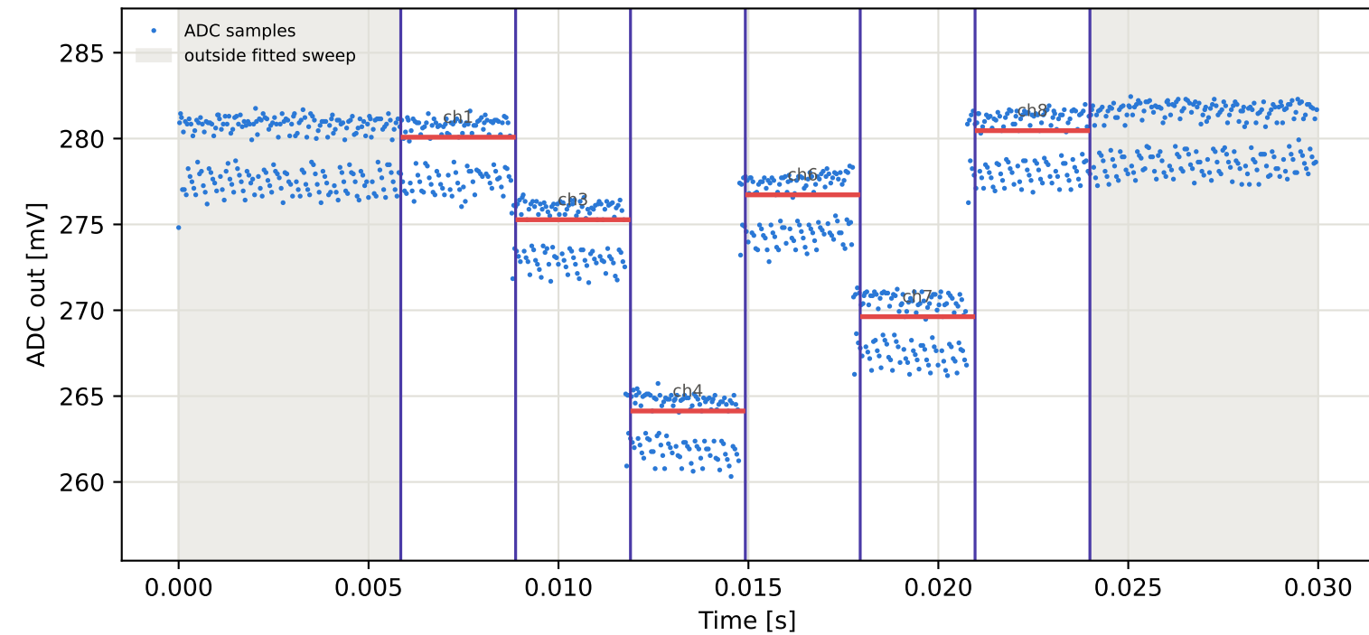
Tag3 &lt;- Tag2 | 995 MHz | run 0 | rep 1 | phase -168.59 deg
