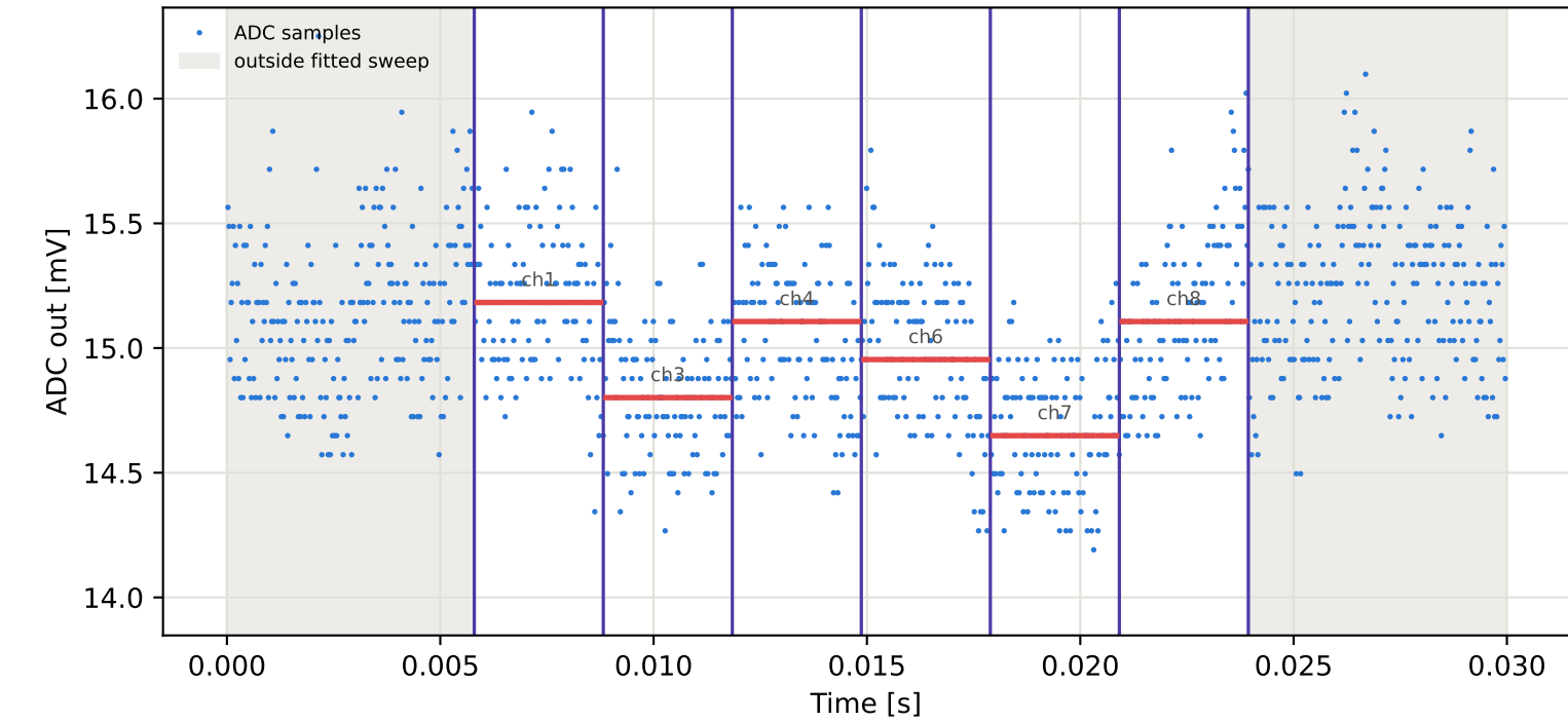
Tag2 &lt;- Tag16 | 795 MHz | run 0 | rep 1 | phase 101.58 deg
