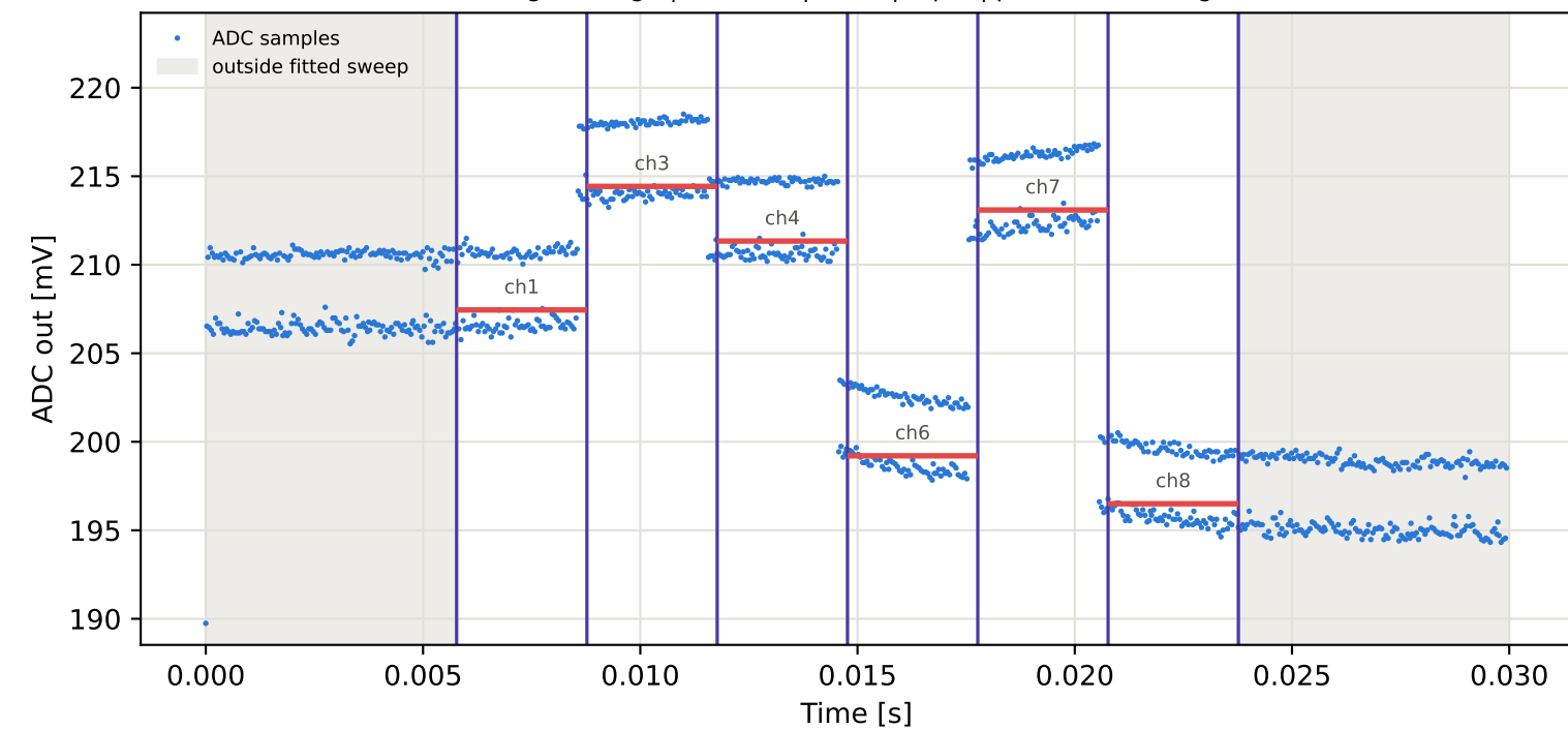
Tag2 &lt;- Tag7 | 875 MHz | run 0 | rep 1 | phase -142.93 deg
