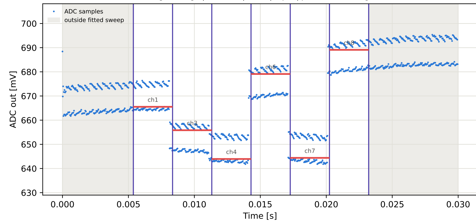
Tag6 &lt;- Tag9 | 895 MHz | run 0 | rep 1 | phase -126.78 deg
