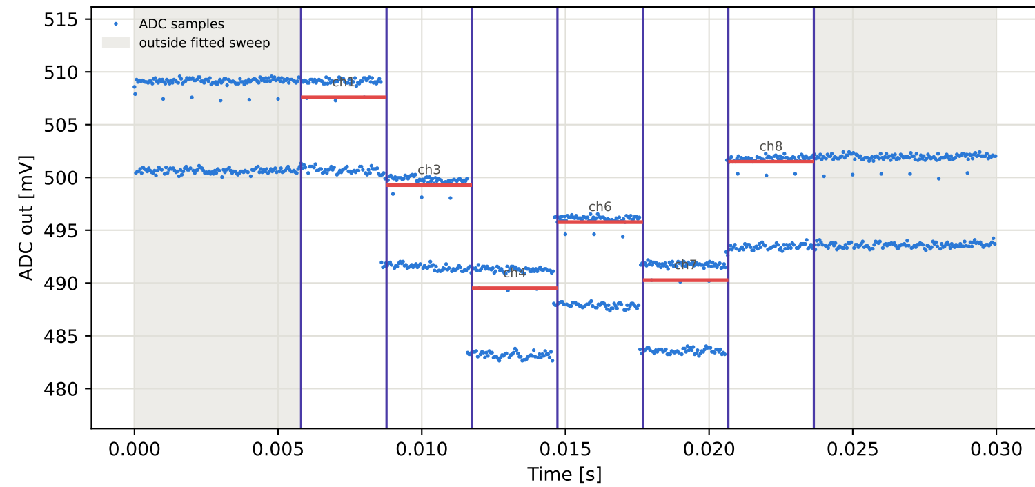
Tag16 &lt;- Tag5 | 835 MHz | run 0 | rep 1 | phase -35.65 deg
