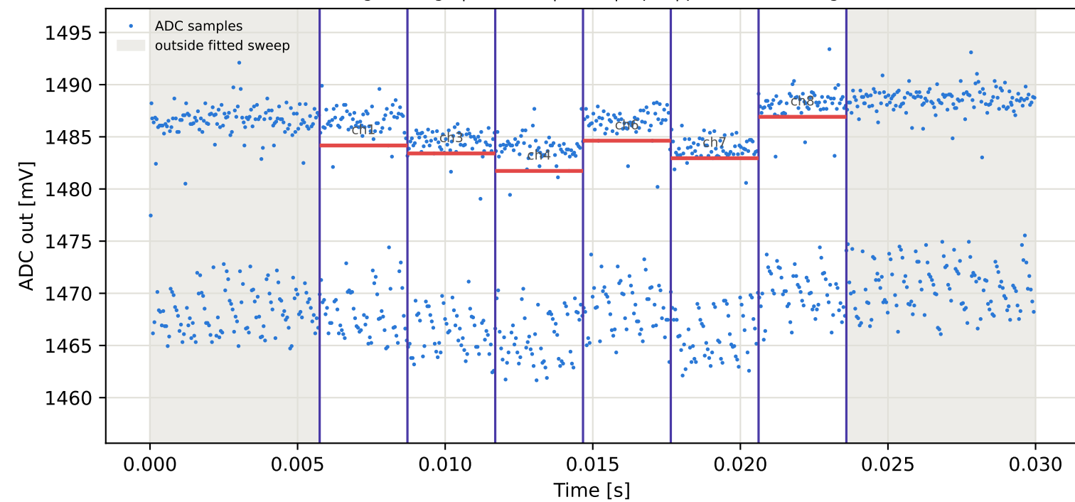
Tag5 &lt;- Tag9 | 885 MHz | run 0 | rep 1 | phase 6.97 deg
