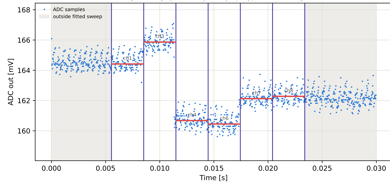
Tag15 &lt;- Tag9 | 785 MHz | run 0 | rep 1 | phase -39.34 deg
