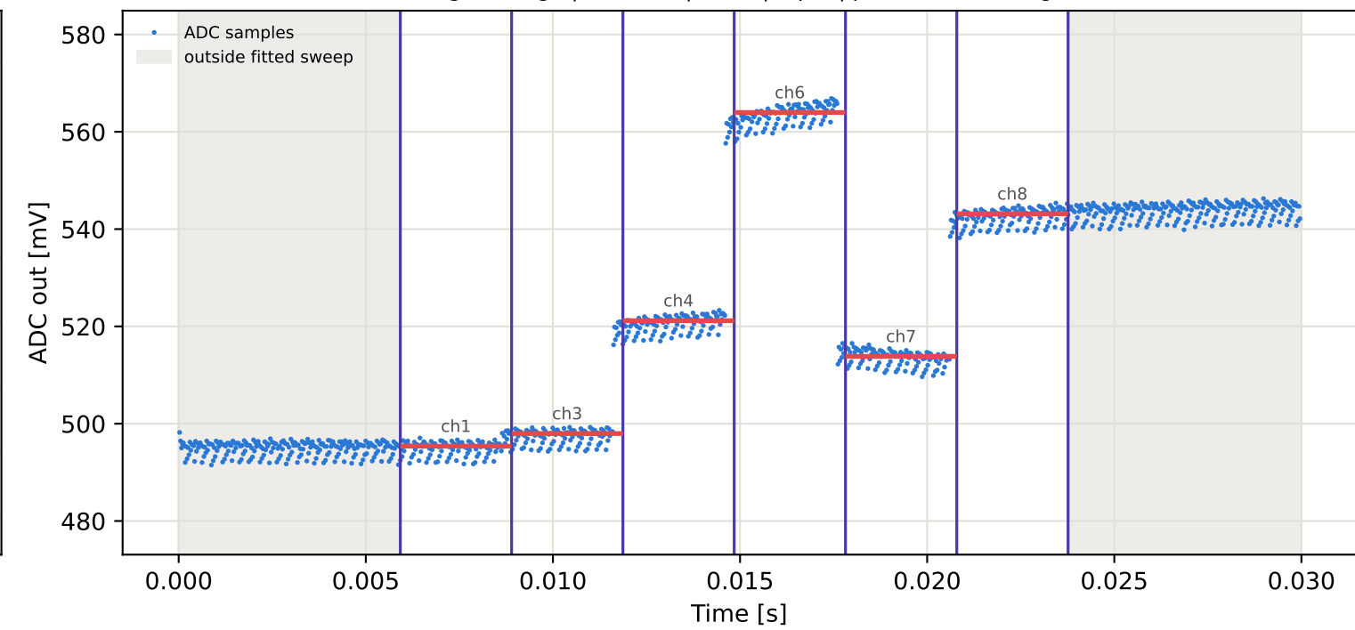
Tag3 &lt;- Tag7 | 895 MHz | run 0 | rep 1 | phase -63.72 deg
