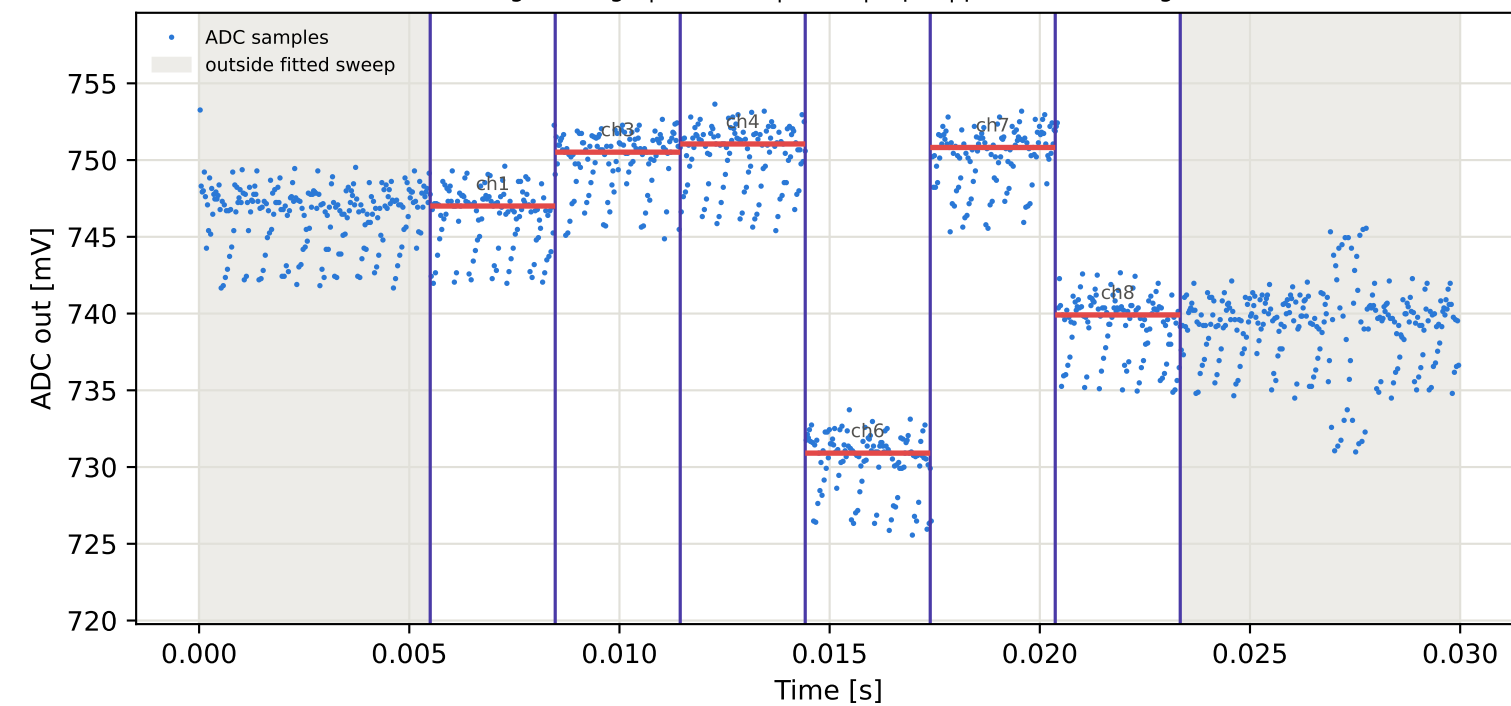
Tag4 &lt;- Tag2 | 975 MHz | run 0 | rep 1 | phase -13.54 deg
