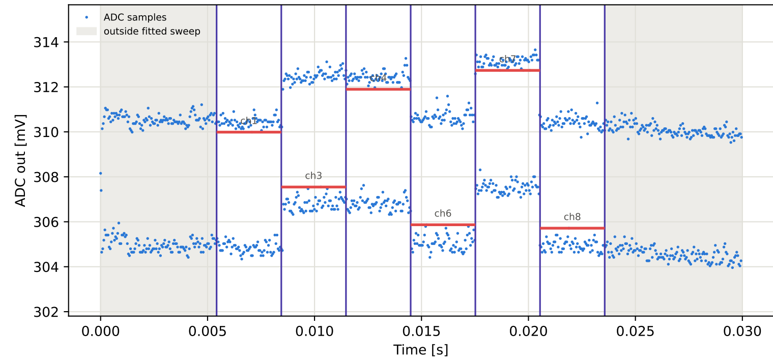
Tag7 &lt;- Tag15 | 835 MHz | run 0 | rep 1 | phase -28.56 deg
