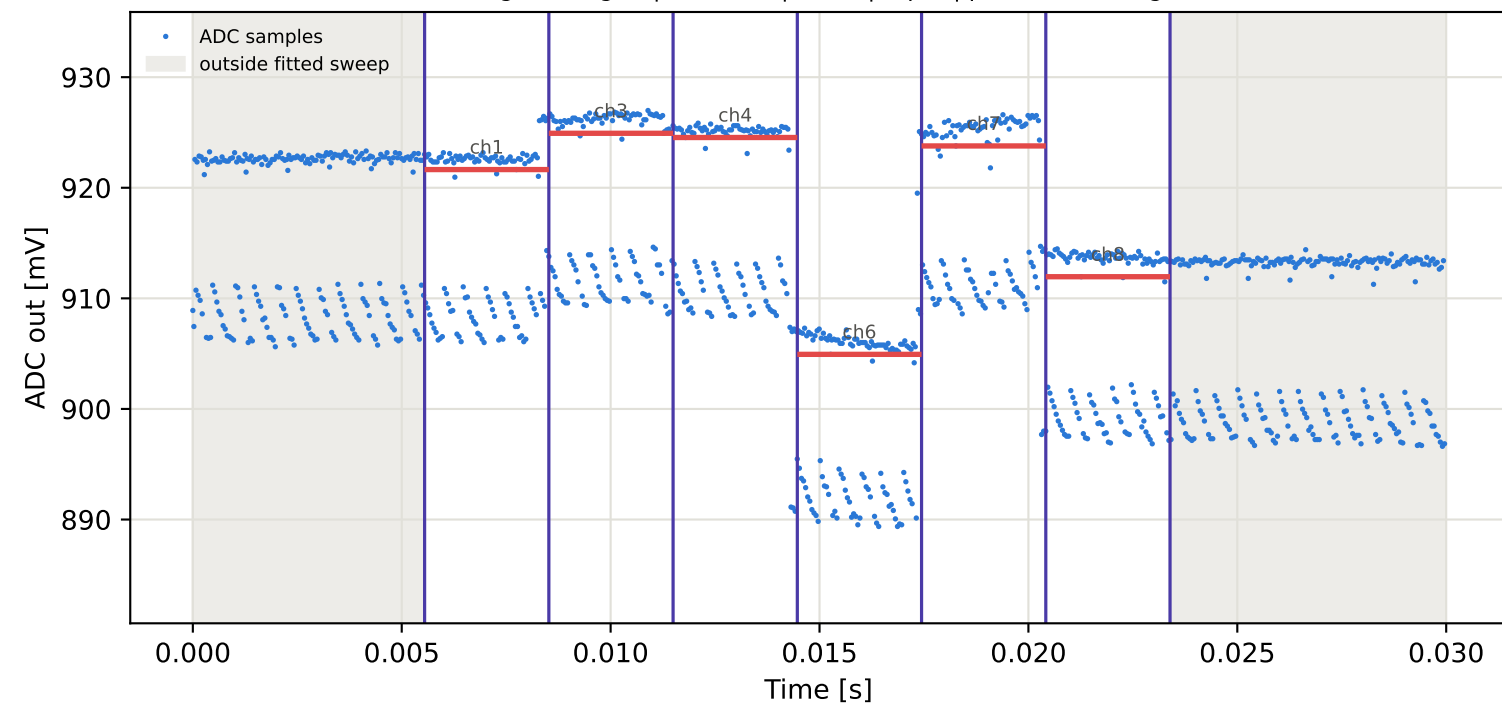
Tag4 &lt;- Tag16 | 925 MHz | run 0 | rep 1 | phase -61.05 deg
