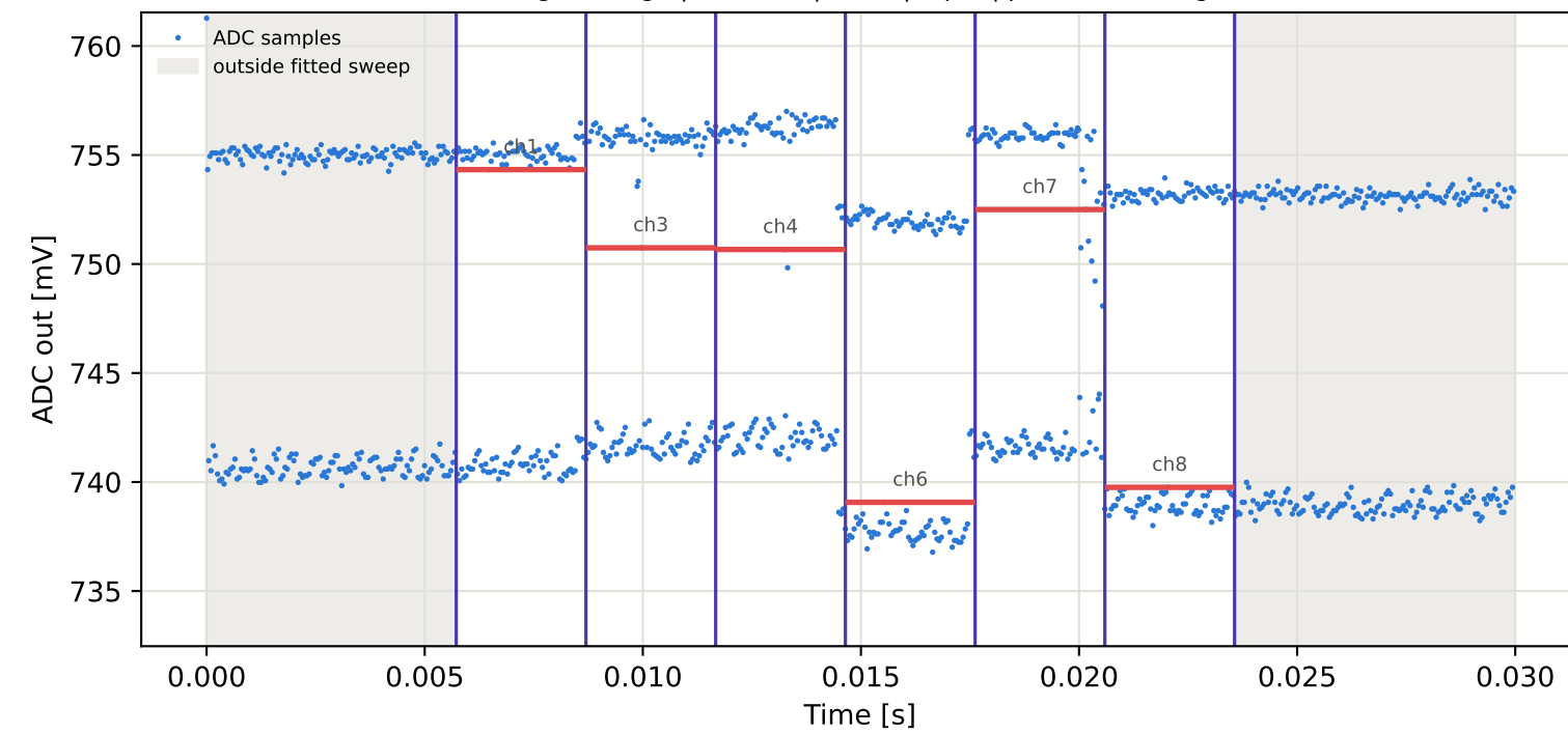
Tag8 &lt;- Tag4 | 935 MHz | run 0 | rep 1 | phase 147.01 deg
