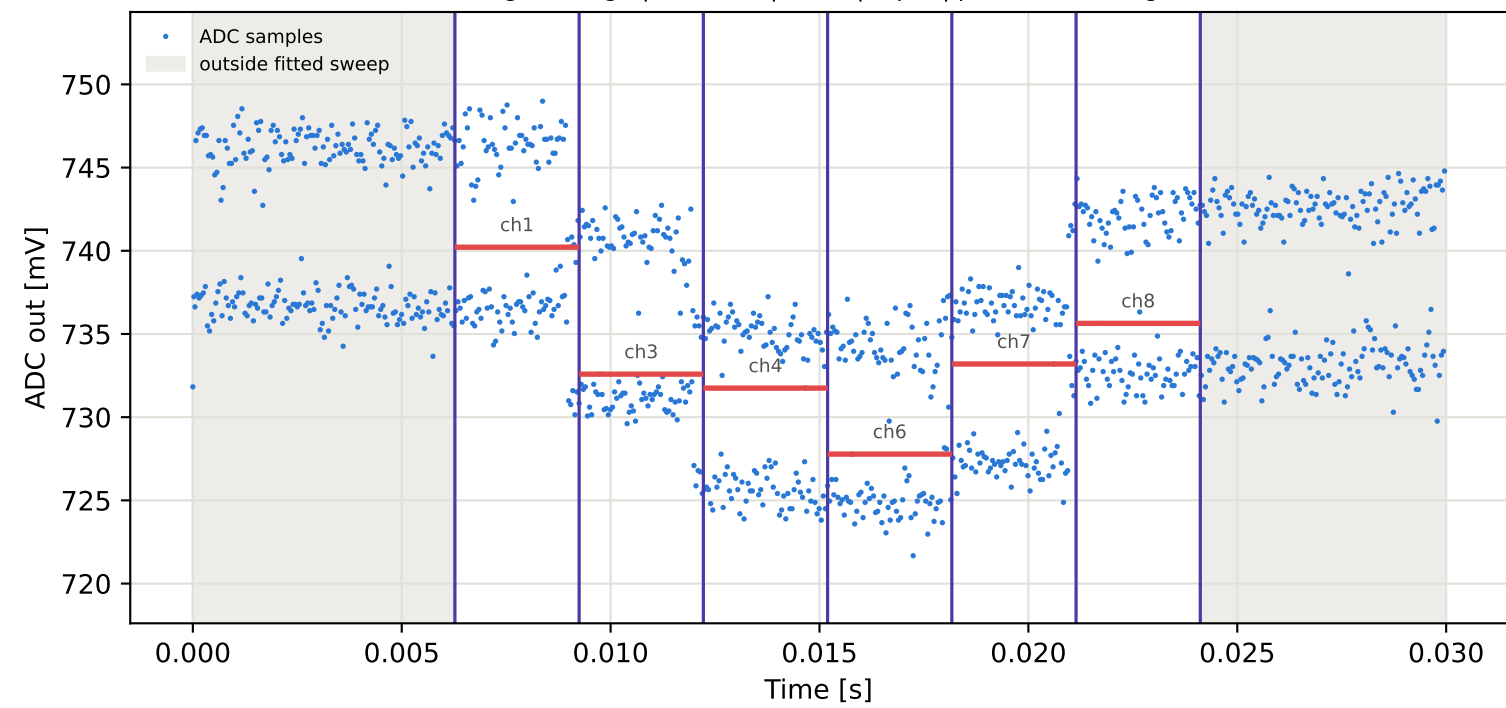
Tag9 &lt;- Tag15 | 885 MHz | run 0 | rep 1 | phase -133.06 deg
