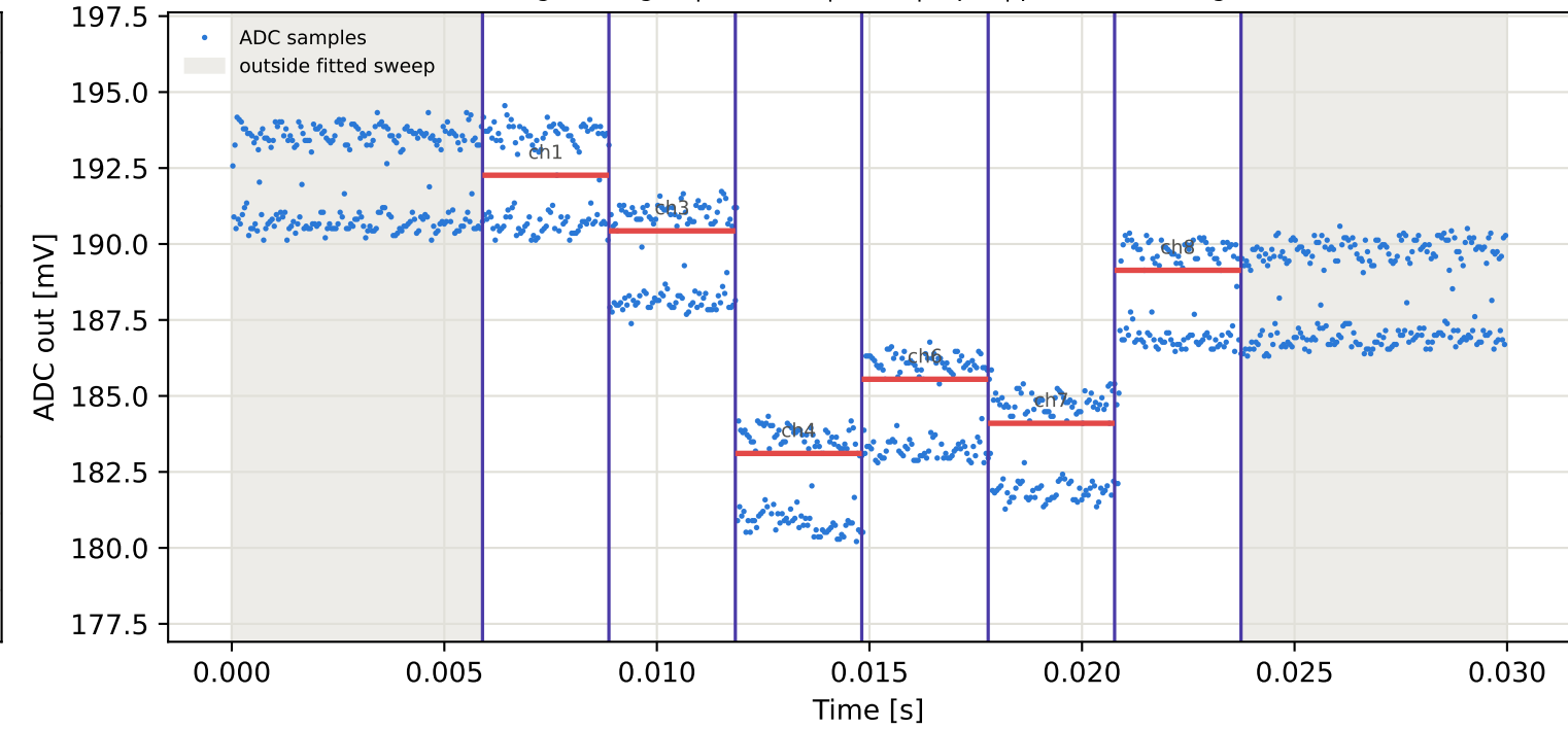
Tag4 &lt;- Tag16 | 825 MHz | run 0 | rep 1 | phase -144.33 deg
