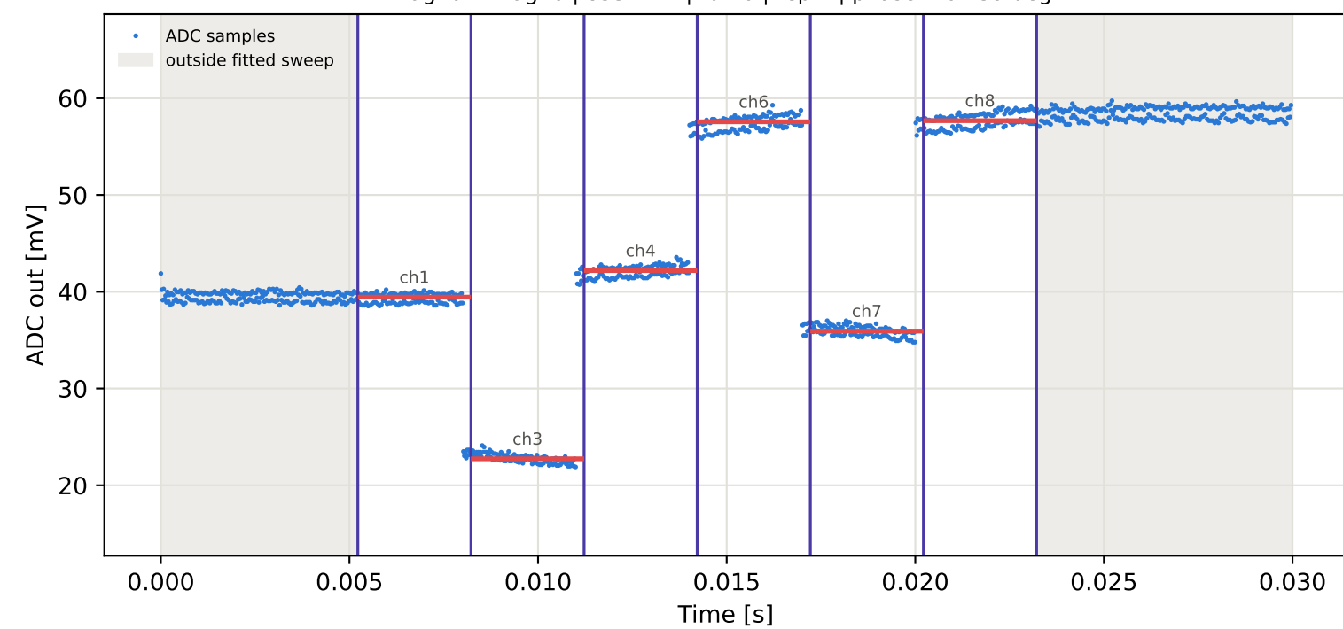
Tag10 &lt;- Tag3 | 855 MHz | run 0 | rep 1 | phase -92.20 deg
