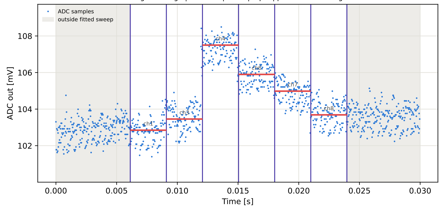
Tag10 &lt;- Tag1 | 995 MHz | run 0 | rep 1 | phase -127.29 deg
