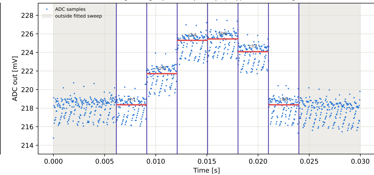
Tag2 &lt;- Tag16 | 905 MHz | run 0 | rep 1 | phase -114.13 deg
