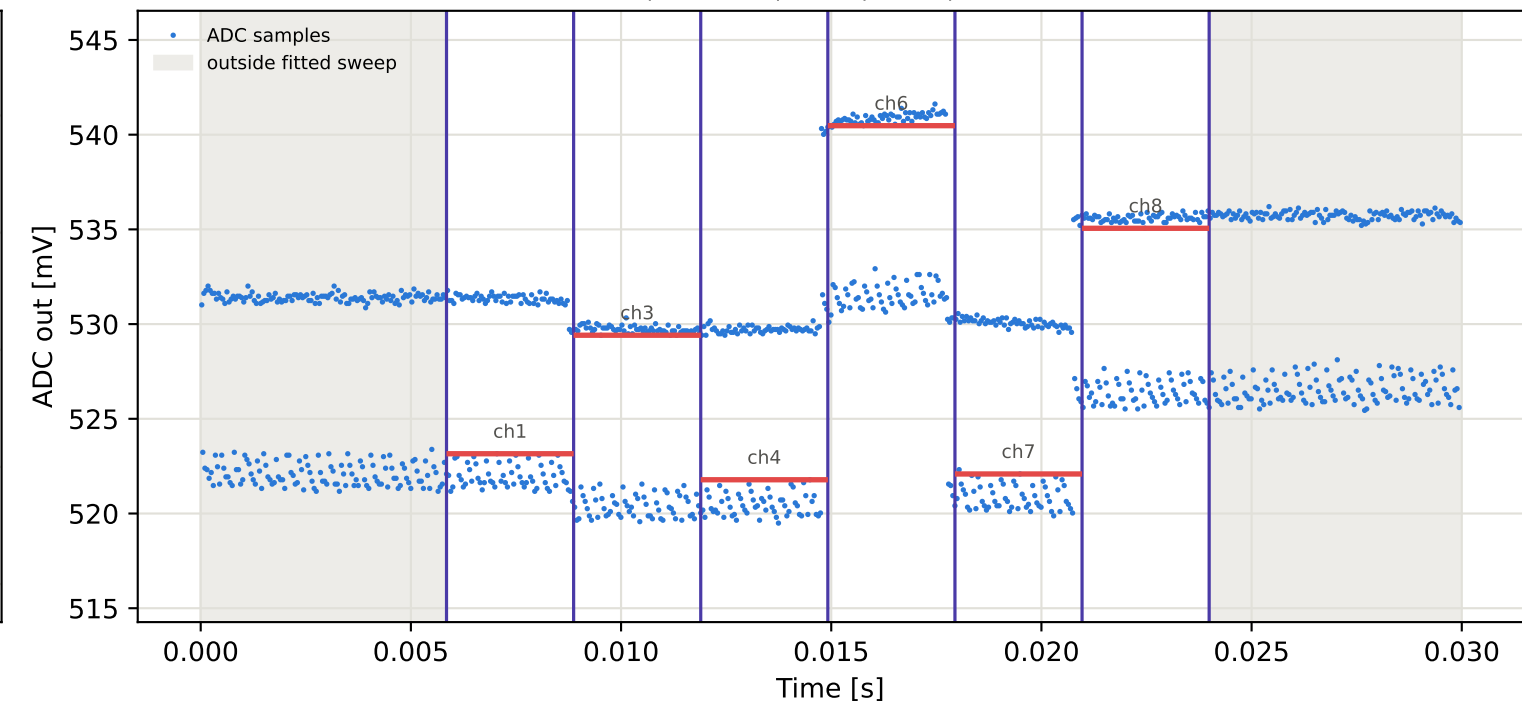
Tag3 &lt;- Tag2 | 895 MHz | run 0 | rep 1 | phase 162.30 deg
