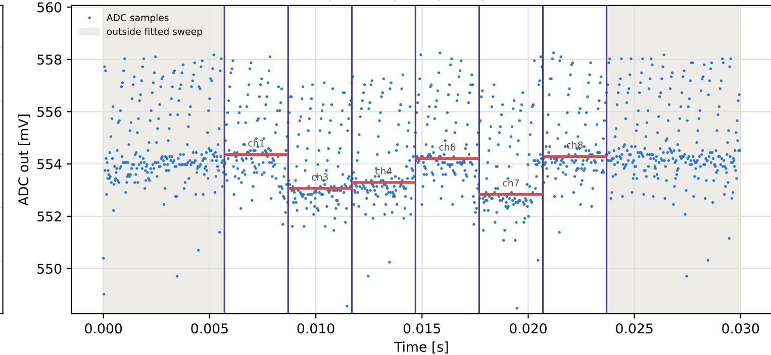
Tag5 &lt;- Tag1 | 845 MHz | run 0 | rep 1 | phase 140.37 deg
