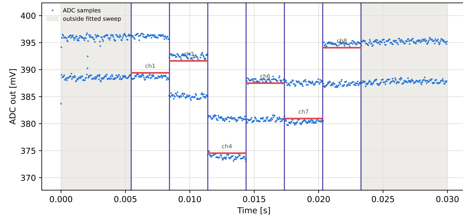
Tag9 &lt;- Tag7 | 975 MHz | run 0 | rep 1 | phase 137.20 deg
