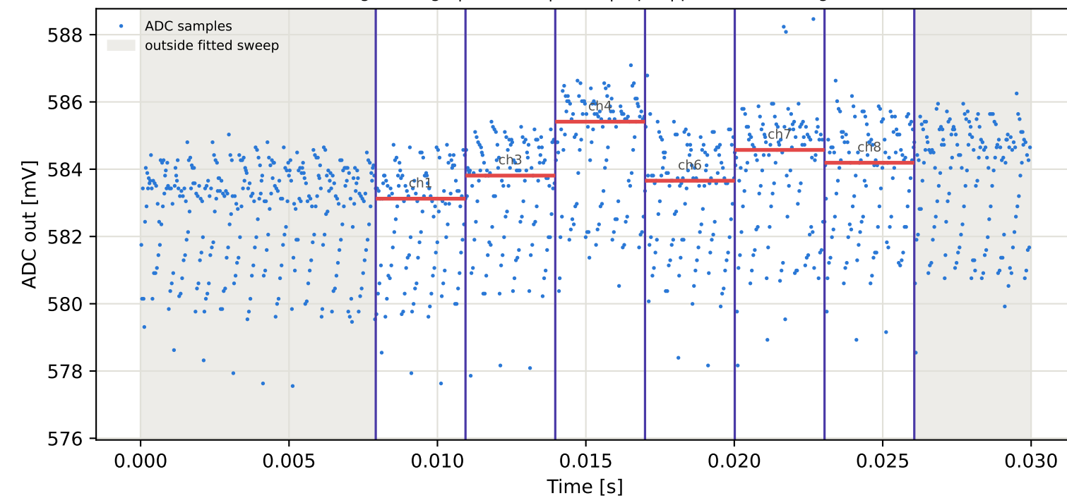
Tag6 &lt;- Tag4 | 865 MHz | run 0 | rep 1 | phase 106.78 deg
