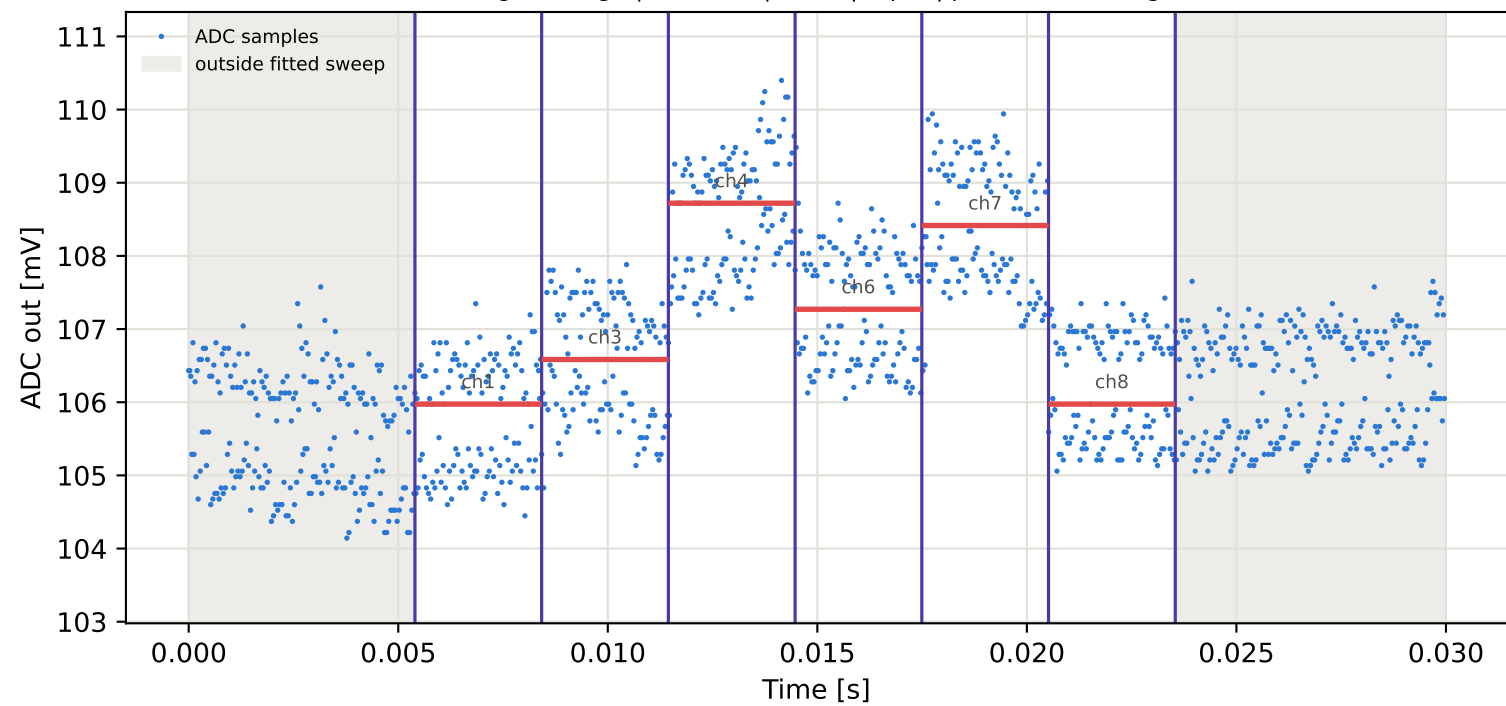
Tag8 &lt;- Tag10 | 785 MHz | run 0 | rep 1 | phase 33.59 deg
