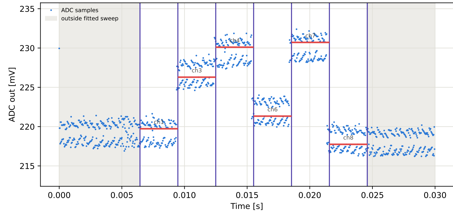
Tag6 &lt;- Tag10 | 805 MHz | run 0 | rep 1 | phase 78.76 deg
