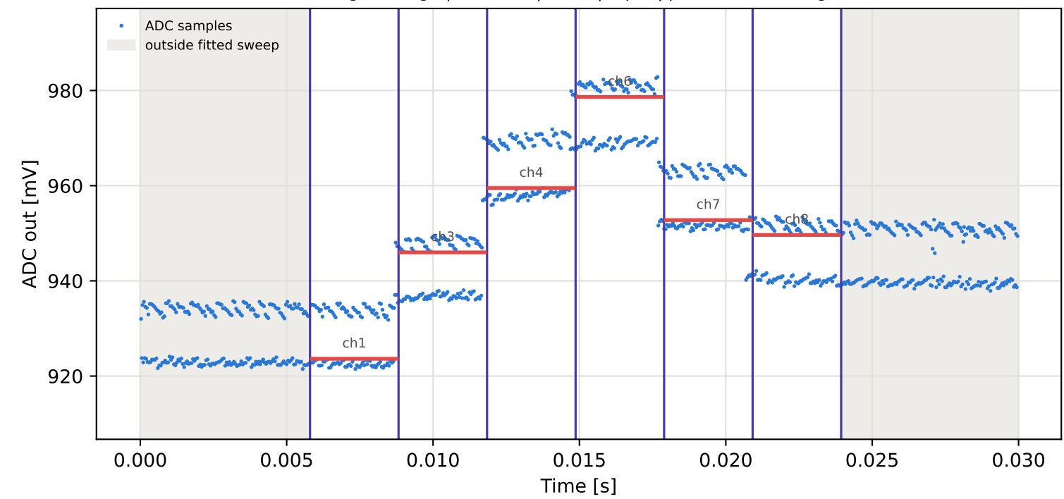
Tag4 &lt;- Tag8 | 875 MHz | run 0 | rep 1 | phase -44.68 deg
