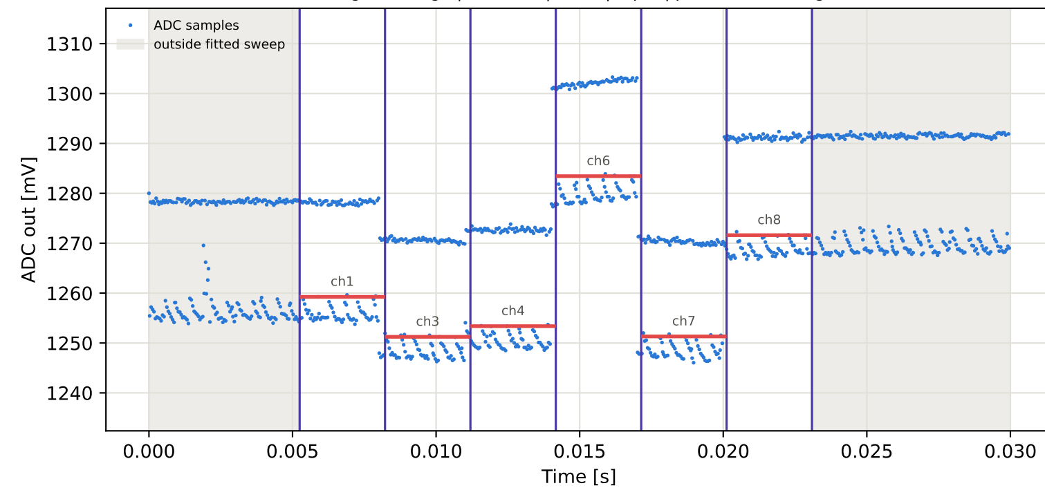
Tag15 &lt;- Tag9 | 945 MHz | run 0 | rep 1 | phase -39.63 deg
