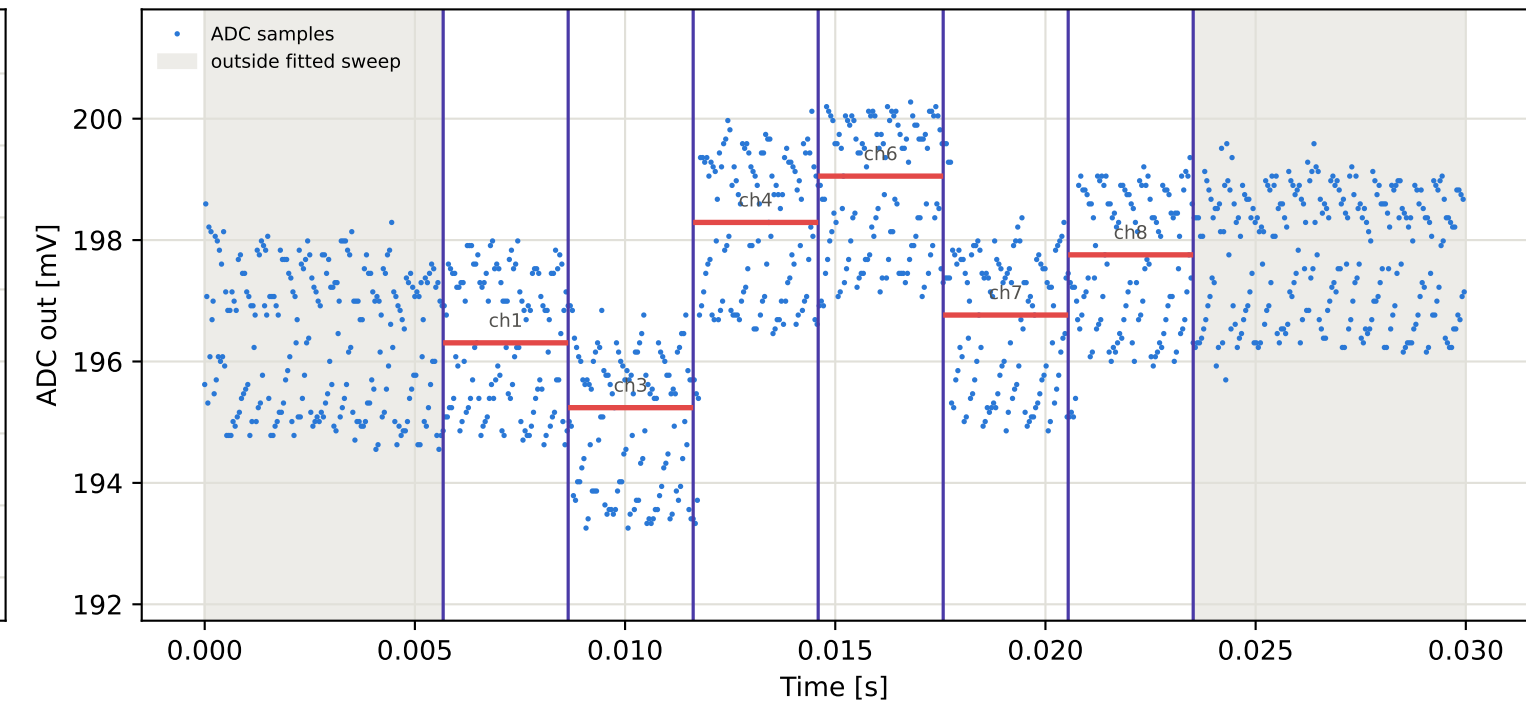
Tag7 &lt;- Tag15 | 805 MHz | run 0 | rep 1 | phase 151.65 deg
