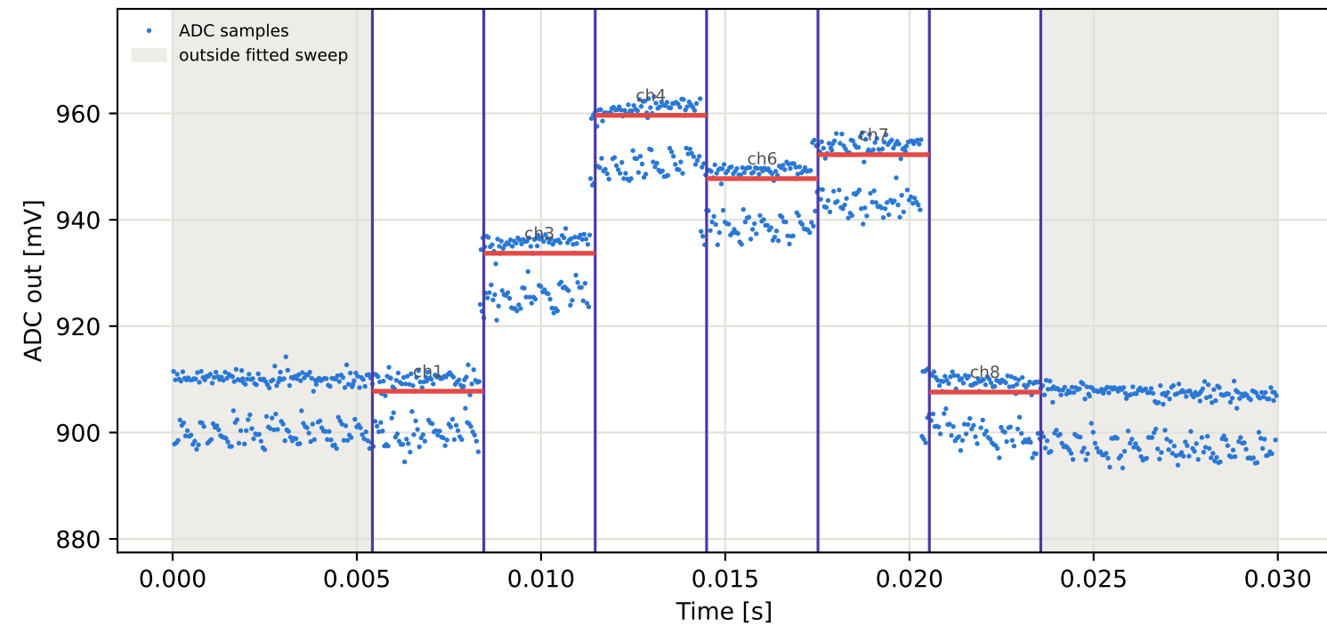
Tag4 &lt;- Tag8 | 885 MHz | run 0 | rep 1 | phase 4.63 deg
