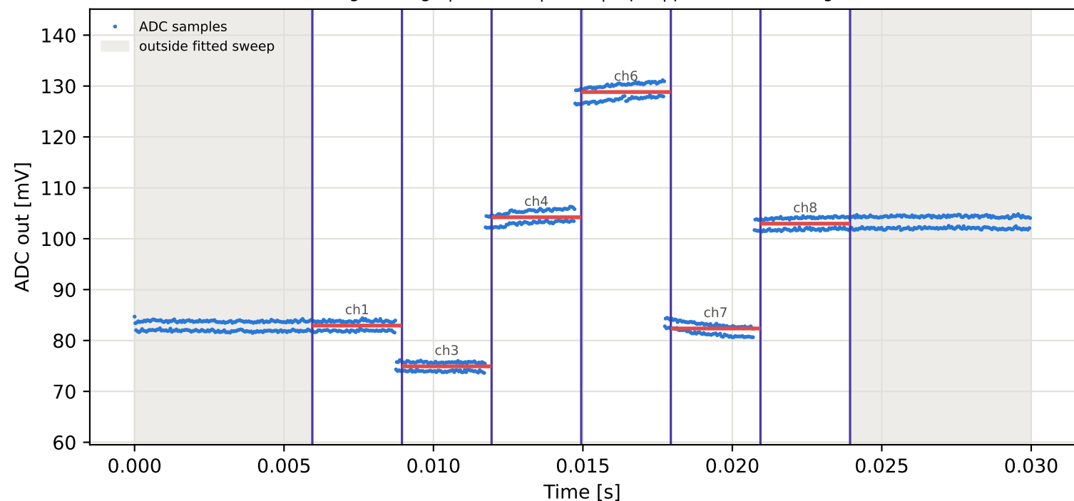
Tag5 &lt;- Tag4 | 985 MHz | run 0 | rep 1 | phase -161.35 deg
