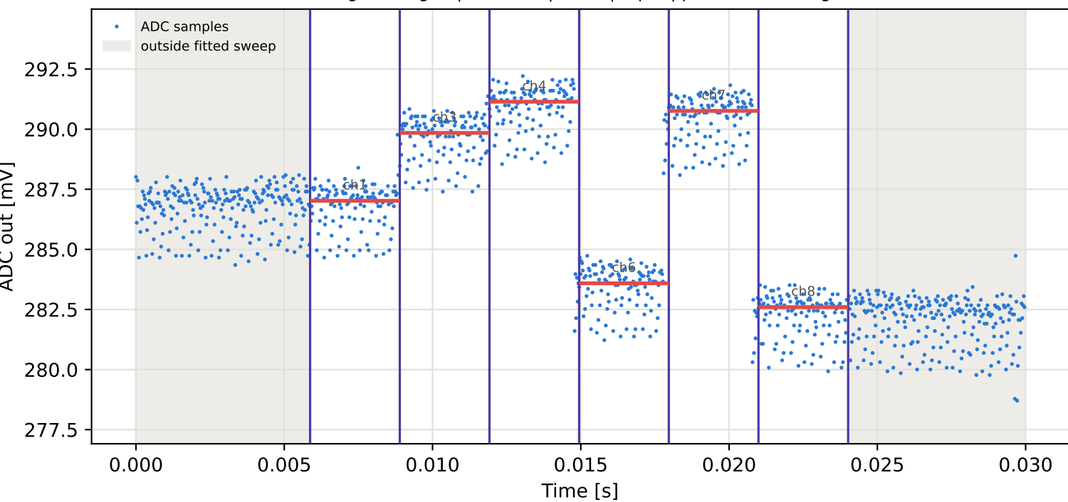
Tag3 &lt;- Tag16 | 915 MHz | run 0 | rep 1 | phase -38.02 deg
