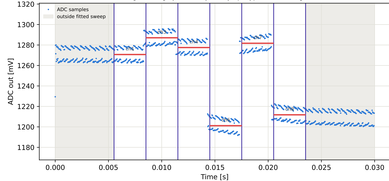
Tag16 &lt;- Tag6 | 895 MHz | run 0 | rep 1 | phase 120.51 deg
