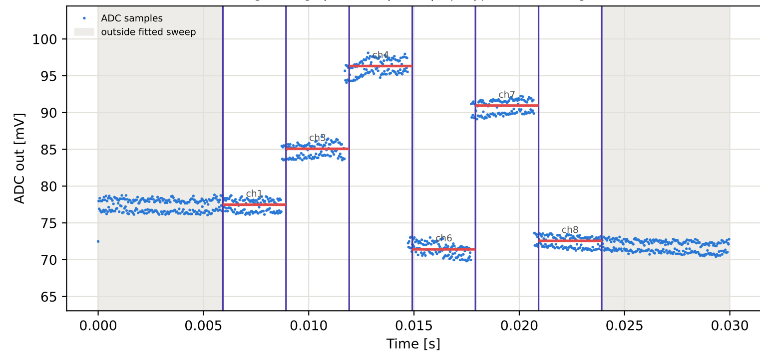
Tag2 &lt;- Tag6 | 985 MHz | run 0 | rep 1 | phase 121.97 deg
