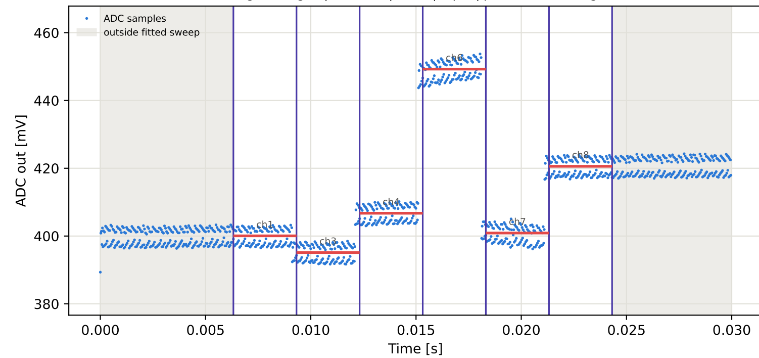
Tag1 &lt;- Tag16 | 935 MHz | run 0 | rep 1 | phase 83.55 deg
