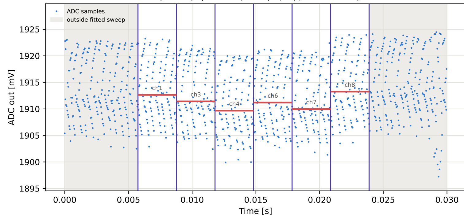
Tag5 &lt;- Tag4 | 895 MHz | run 0 | rep 1 | phase 46.16 deg
