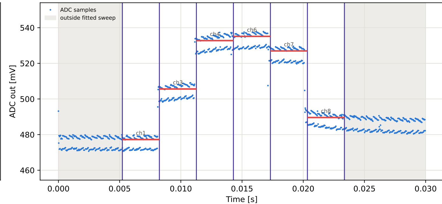
Tag9 &lt;- Tag2 | 895 MHz | run 0 | rep 1 | phase 28.89 deg
