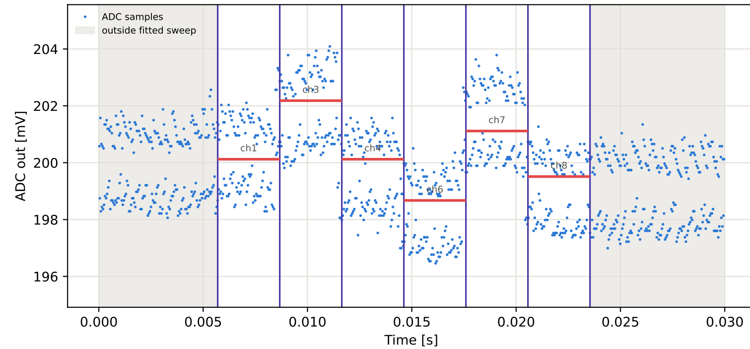
Tag5 &lt;- Tag3 | 775 MHz | run 0 | rep 1 | phase -179.15 deg
