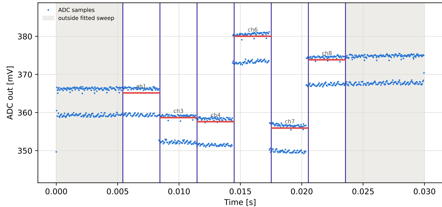
Tag3 &lt;- Tag8 | 975 MHz | run 0 | rep 1 | phase -49.07 deg
