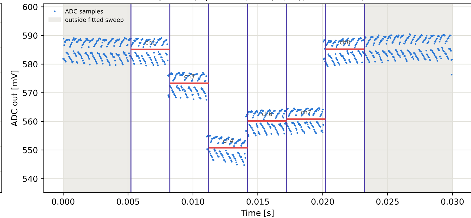
Tag10 &lt;- Tag5 | 935 MHz | run 0 | rep 1 | phase -150.01 deg
