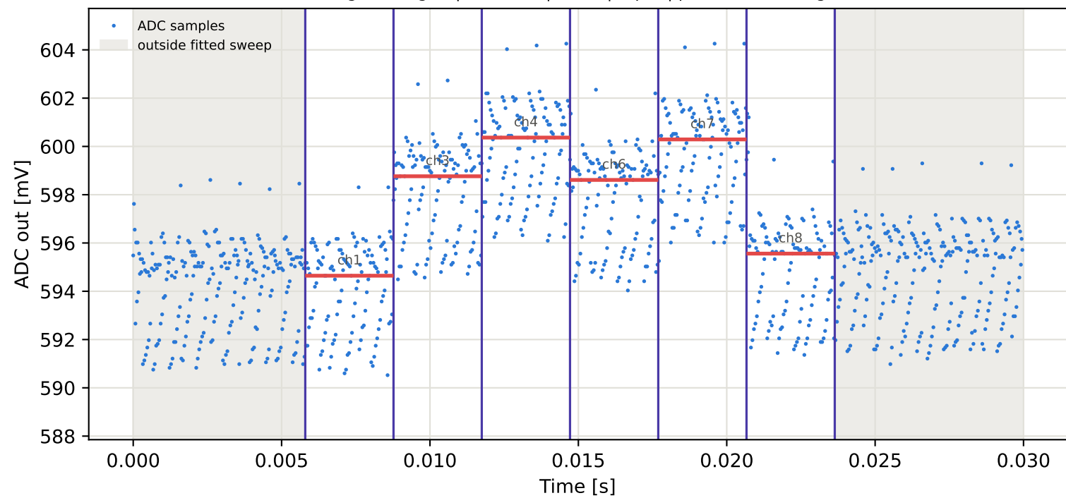
Tag4 &lt;- Tag16 | 865 MHz | run 0 | rep 1 | phase -167.61 deg
