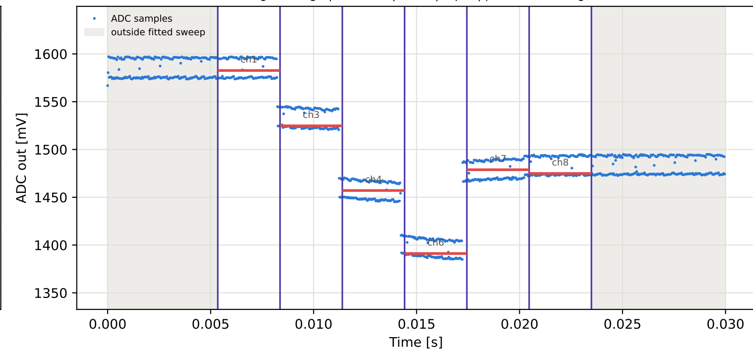
Tag5 &lt;- Tag4 | 875 MHz | run 0 | rep 1 | phase 42.95 deg
