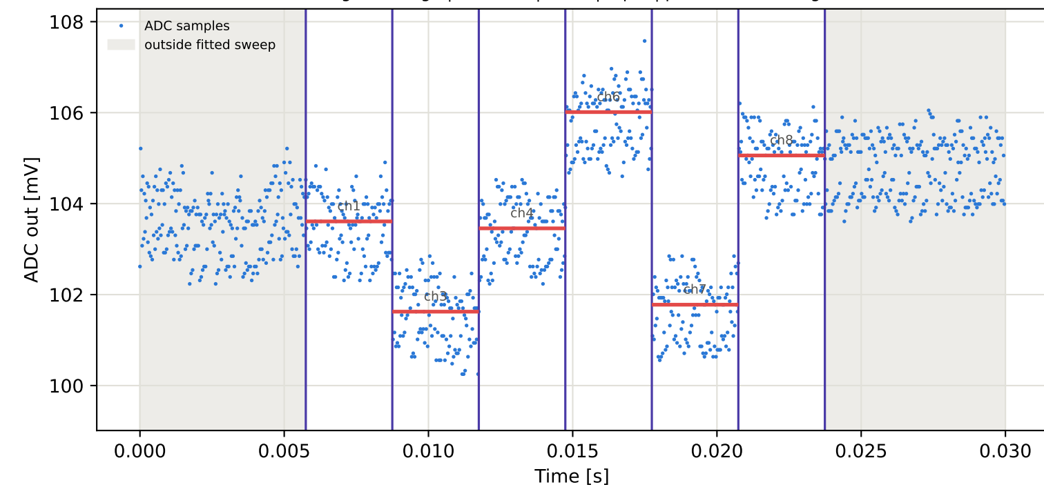
Tag10 &lt;- Tag1 | 775 MHz | run 0 | rep 1 | phase -171.01 deg
