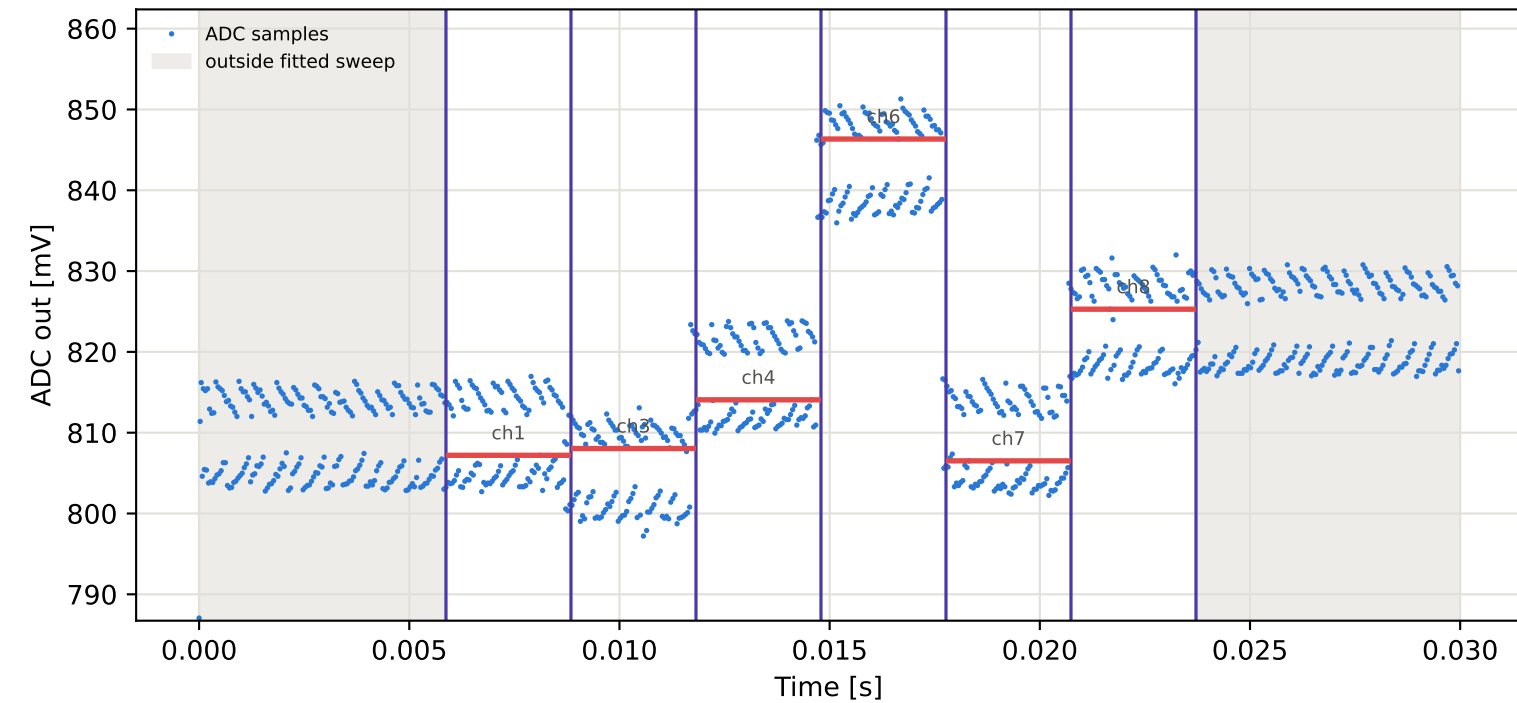
Tag8 &lt;- Tag6 | 955 MHz | run 0 | rep 1 | phase -70.54 deg
