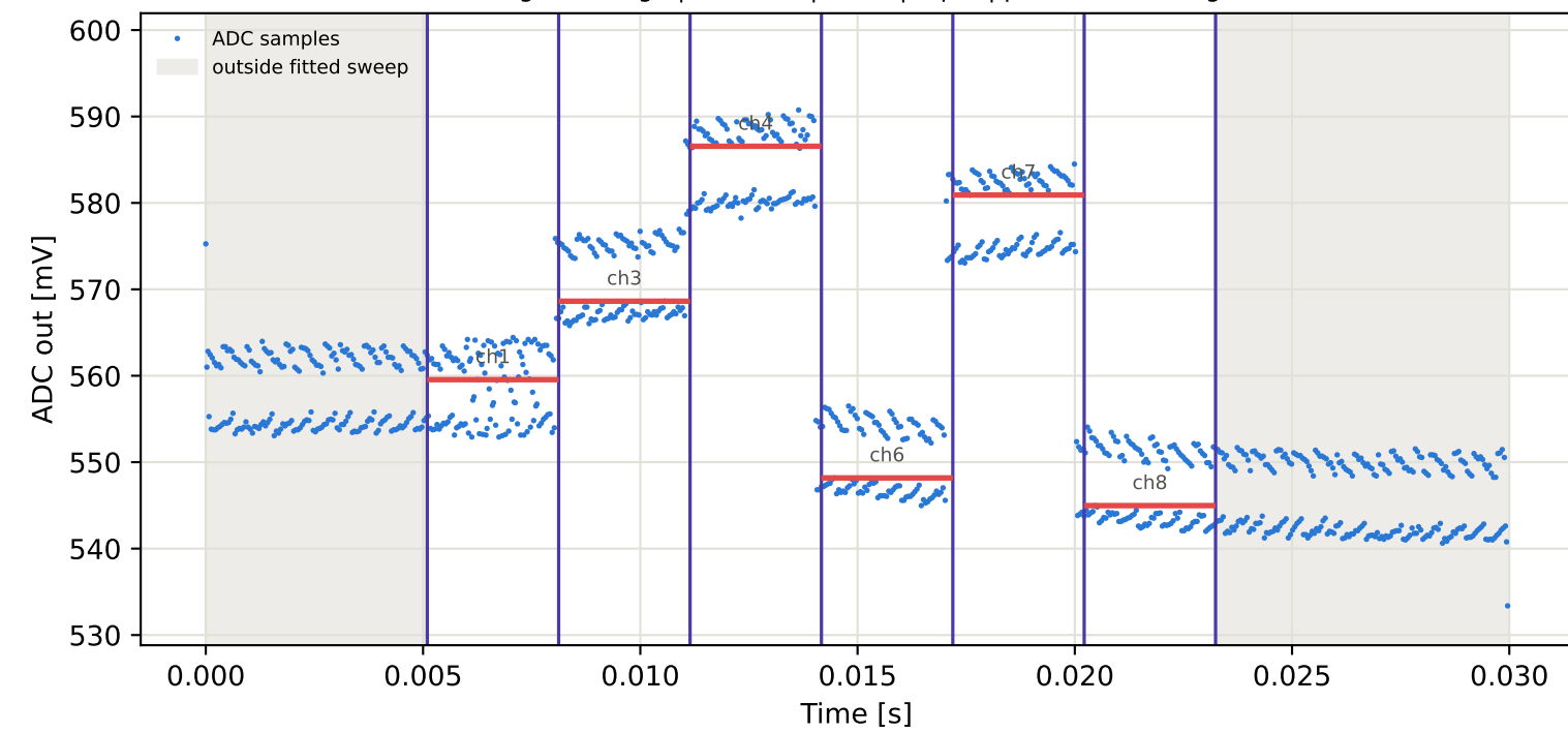
Tag10 &lt;- Tag4 | 935 MHz | run 0 | rep 1 | phase -58.45 deg
