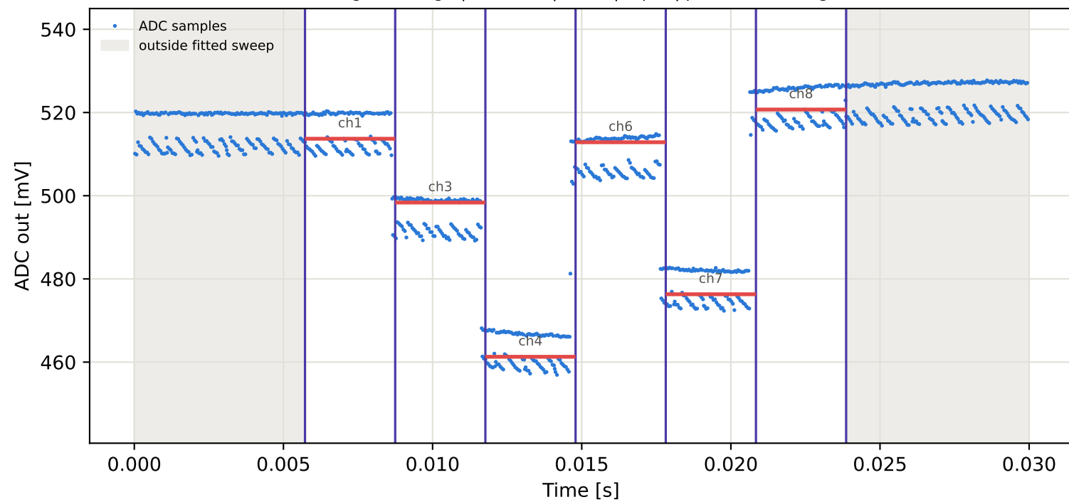
Tag2 &lt;- Tag10 | 985 MHz | run 0 | rep 1 | phase 46.35 deg
