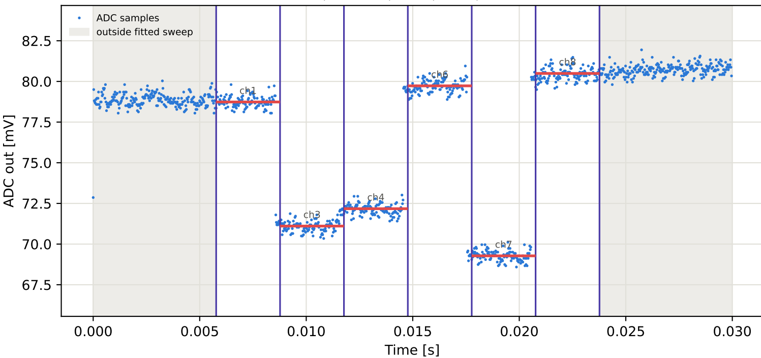
Tag2 &lt;- Tag15 | 825 MHz | run 0 | rep 1 | phase 150.26 deg
