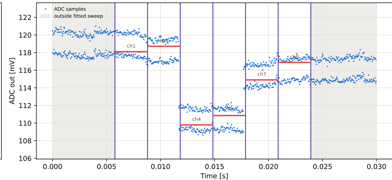
Tag2 &lt;- Tag8 | 975 MHz | run 0 | rep 1 | phase 44.17 deg
