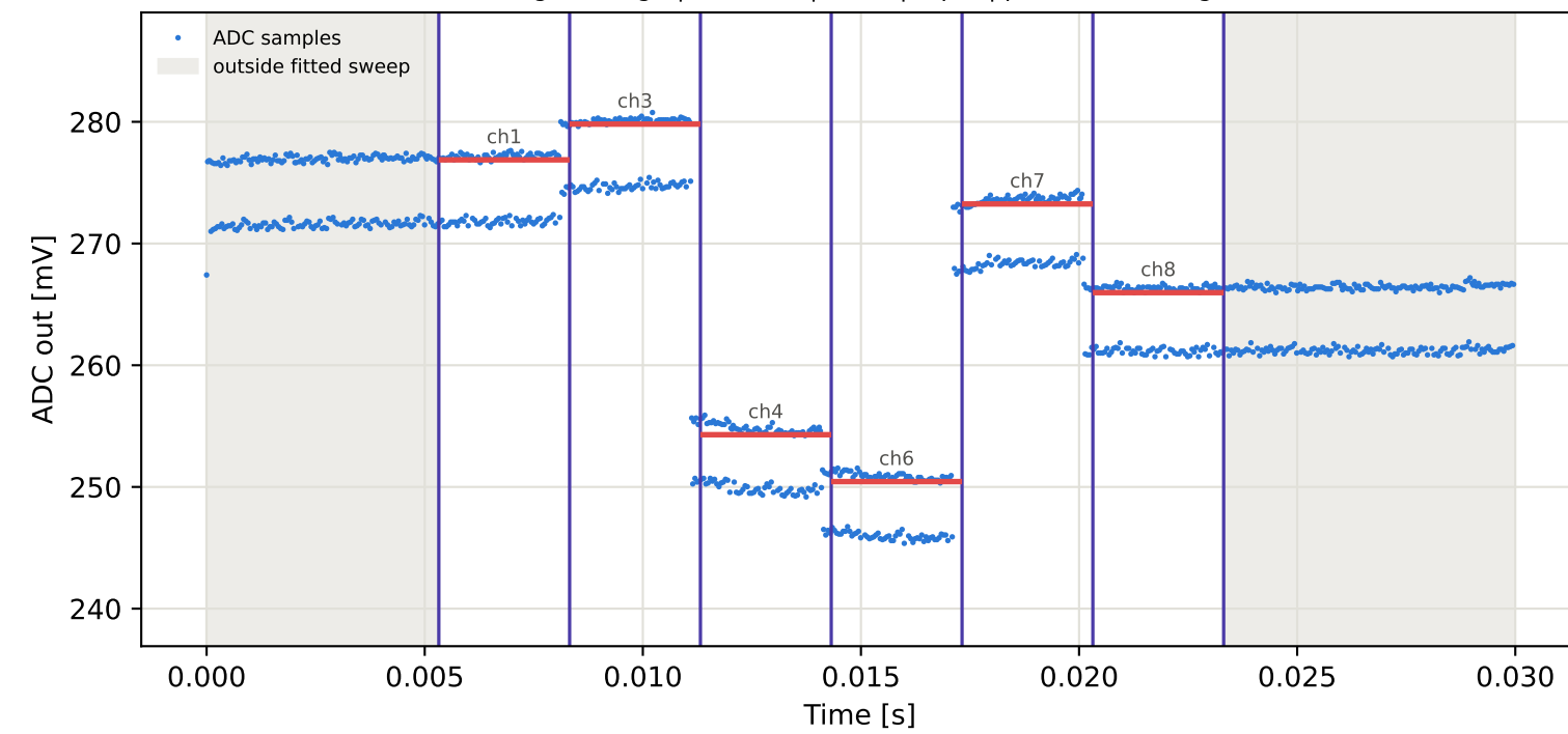
Tag3 &lt;- Tag6 | 995 MHz | run 0 | rep 1 | phase -157.83 deg
