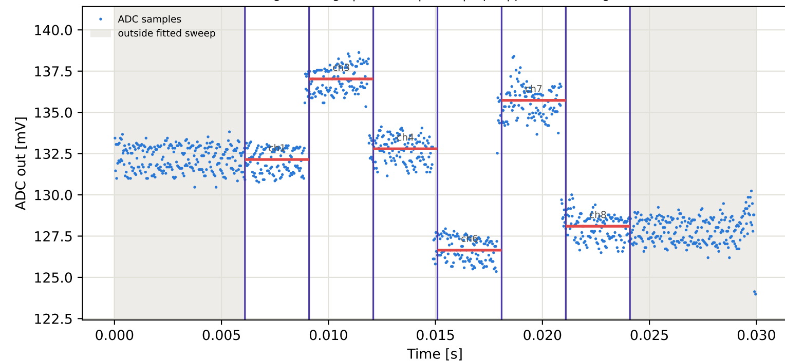
Tag10 &lt;- Tag5 | 825 MHz | run 0 | rep 1 | phase 4.89 deg
