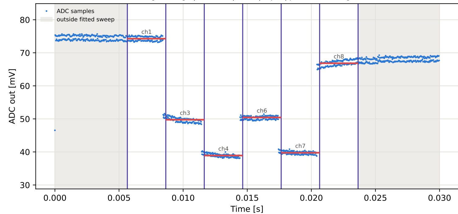
Tag2 &lt;- Tag6 | 855 MHz | run 0 | rep 1 | phase 75.06 deg
