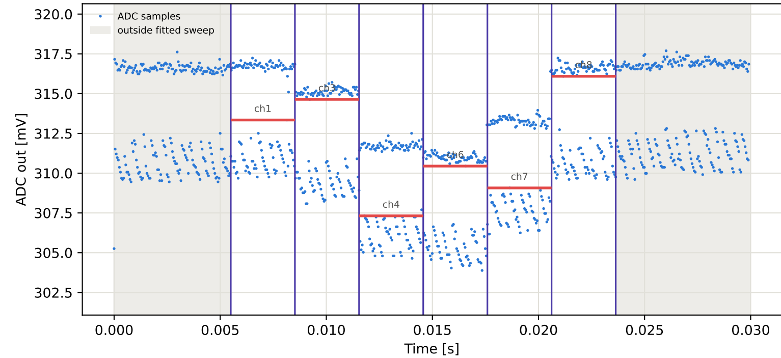
Tag6 &lt;- Tag4 | 925 MHz | run 0 | rep 1 | phase -145.22 deg
