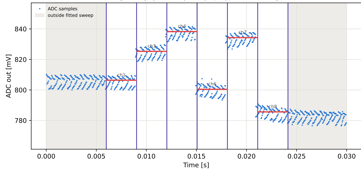
Tag4 &lt;- Tag8 | 905 MHz | run 0 | rep 1 | phase -22.64 deg
