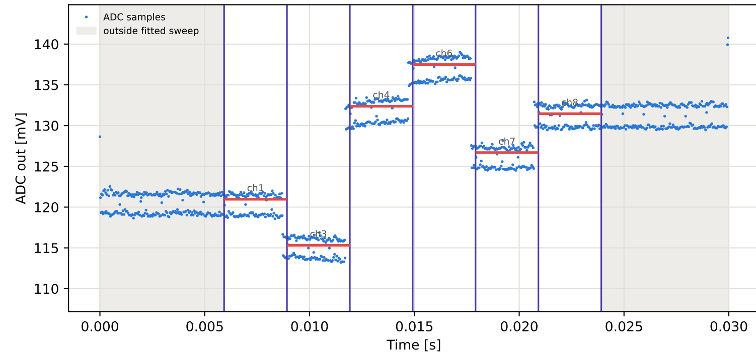
Tag2 &lt;- Tag7 | 835 MHz | run 0 | rep 1 | phase 103.40 deg
