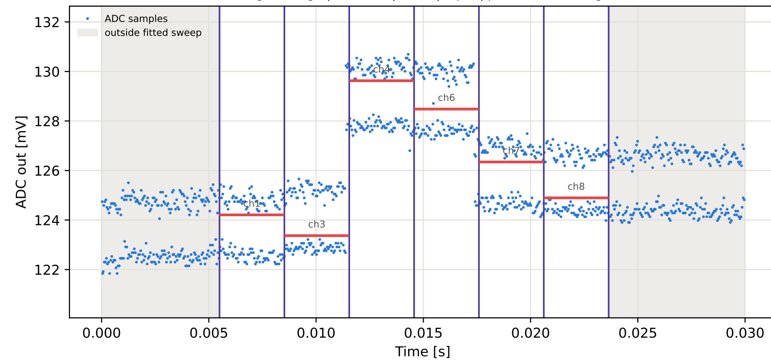
Tag5 &lt;- Tag8 | 975 MHz | run 0 | rep 1 | phase -173.71 deg
