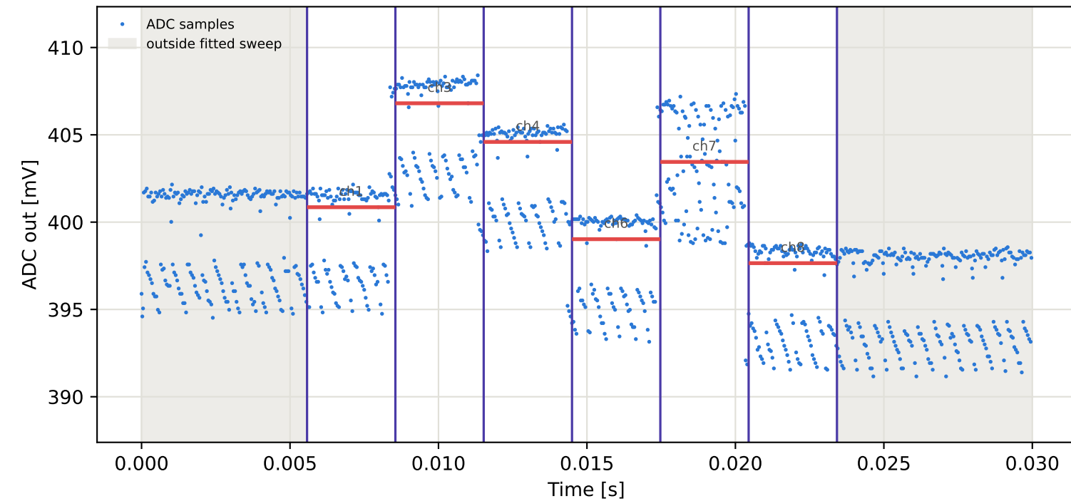
Tag15 &lt;- Tag5 | 845 MHz | run 0 | rep 1 | phase -99.09 deg
