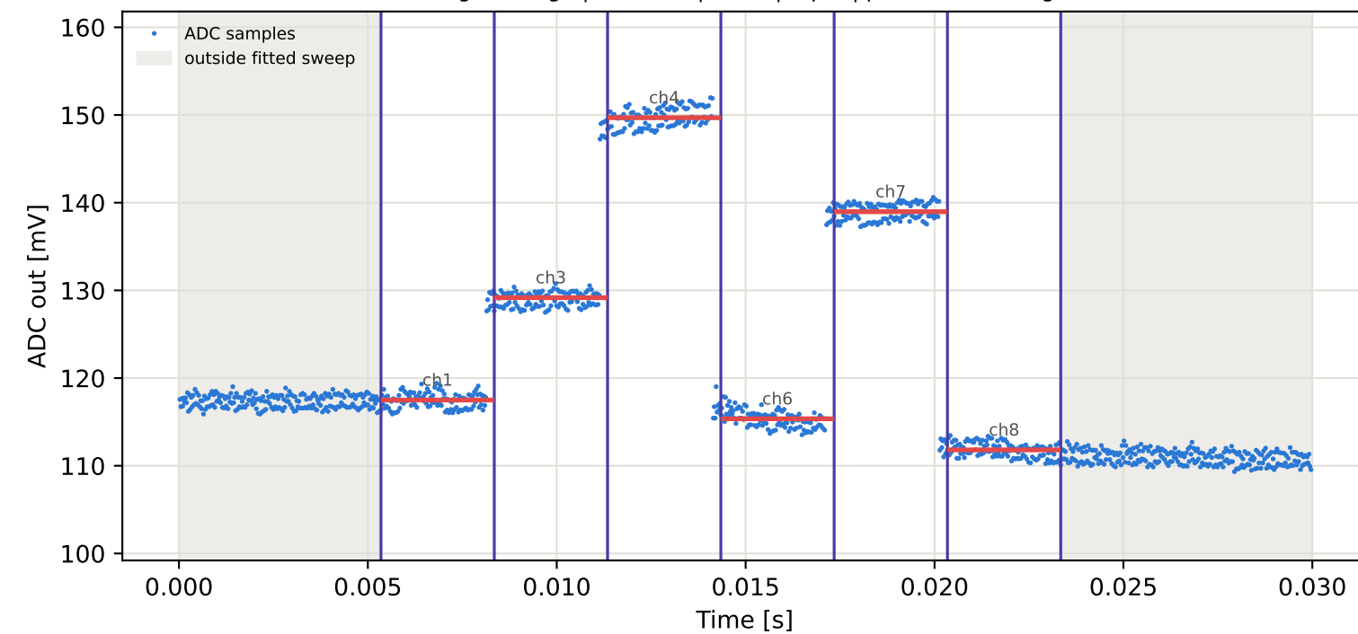
Tag6 &lt;- Tag4 | 975 MHz | run 0 | rep 1 | phase -78.22 deg
