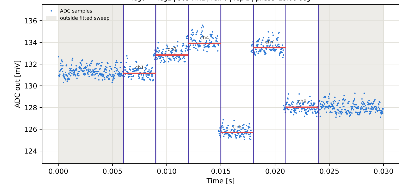
Tag6 &lt;- Tag4 | 965 MHz | run 0 | rep 1 | phase -131.82 deg
