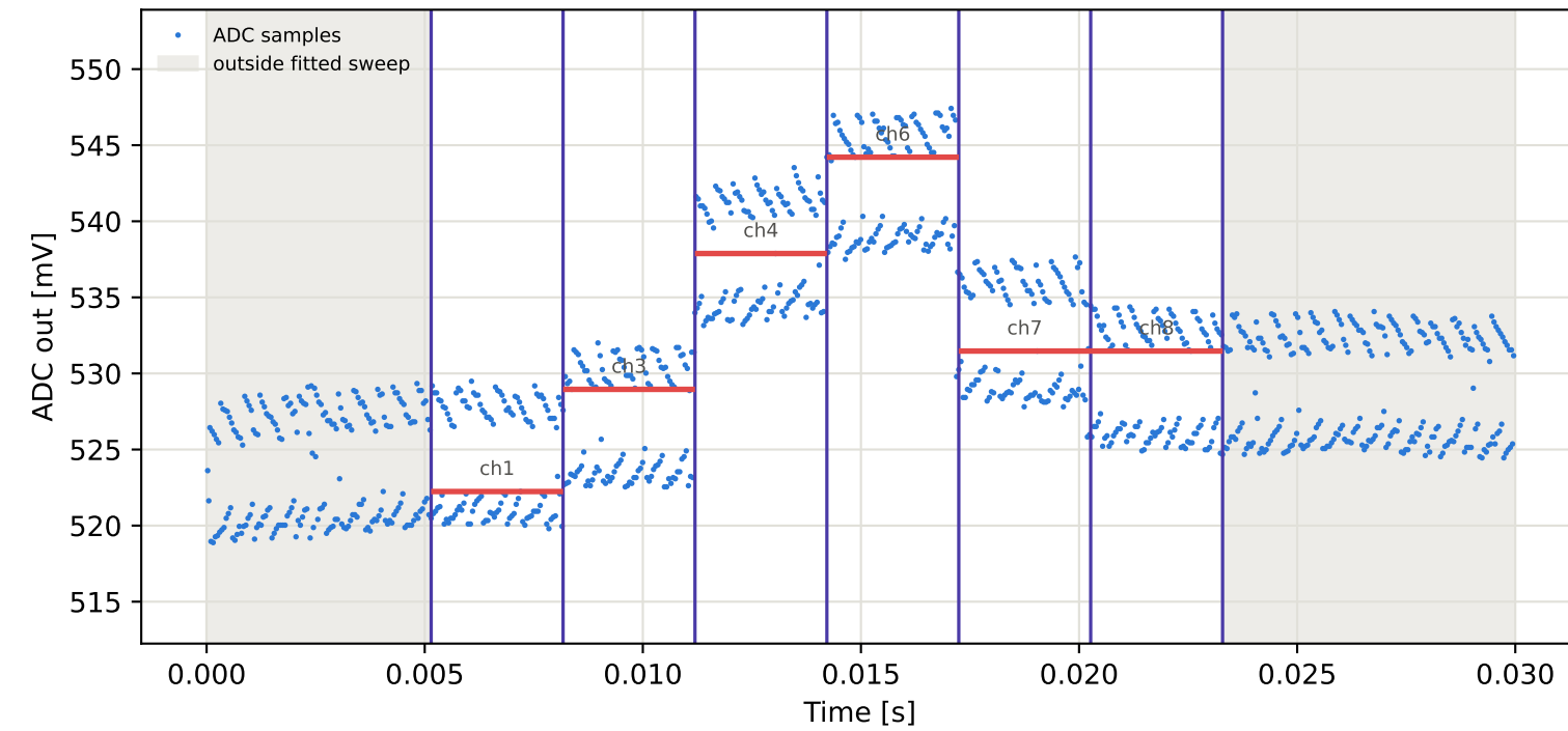
Tag9 &lt;- Tag16 | 945 MHz | run 0 | rep 1 | phase -0.40 deg
