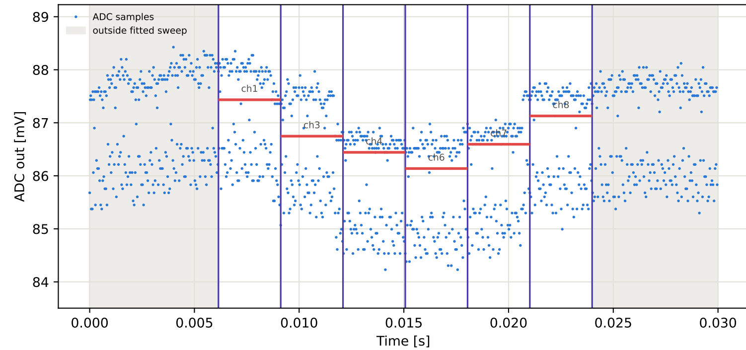
Tag1 &lt;- Tag4 | 845 MHz | run 0 | rep 1 | phase -144.77 deg
