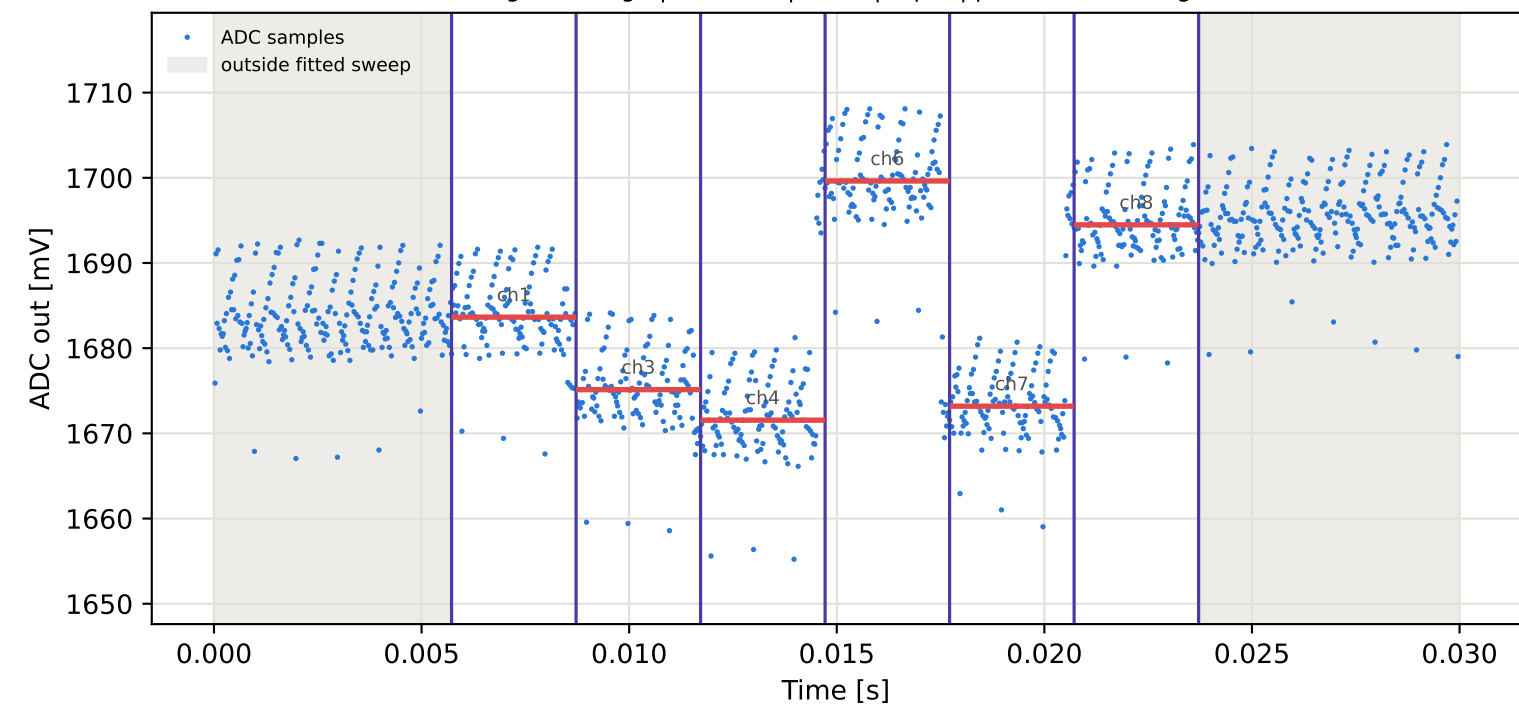
Tag15 &lt;- Tag6 | 925 MHz | run 0 | rep 1 | phase 151.51 deg
