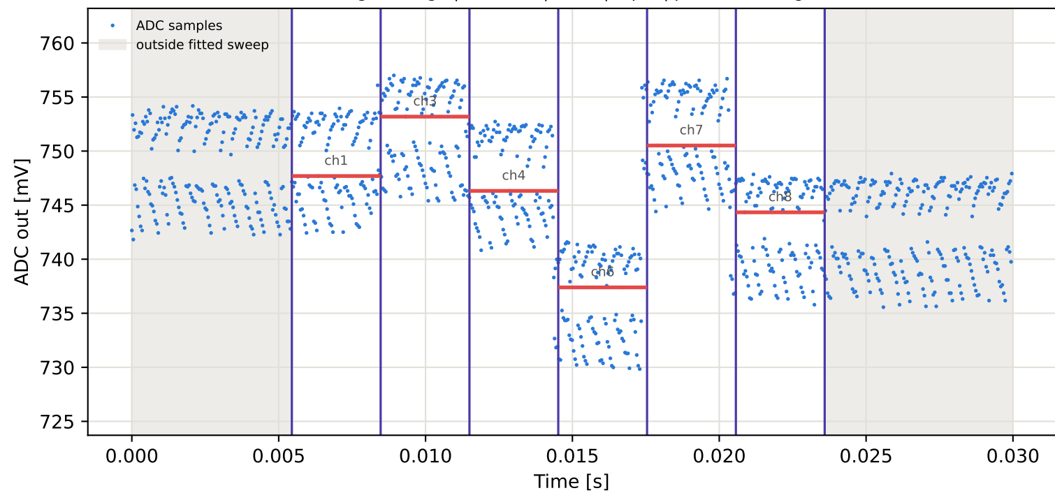
Tag4 &lt;- Tag8 | 975 MHz | run 0 | rep 1 | phase -39.21 deg
