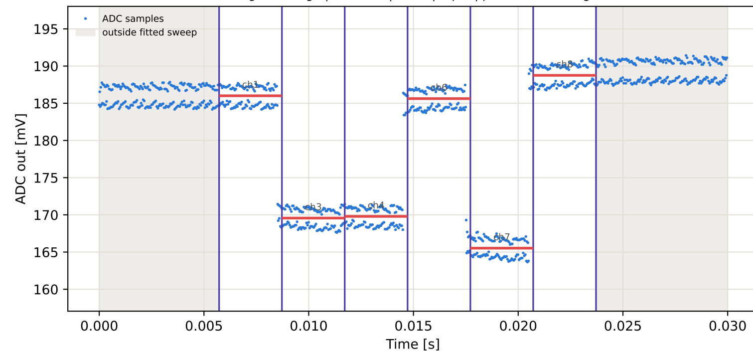
Tag15 &lt;- Tag5 | 795 MHz | run 0 | rep 1 | phase 141.78 deg
