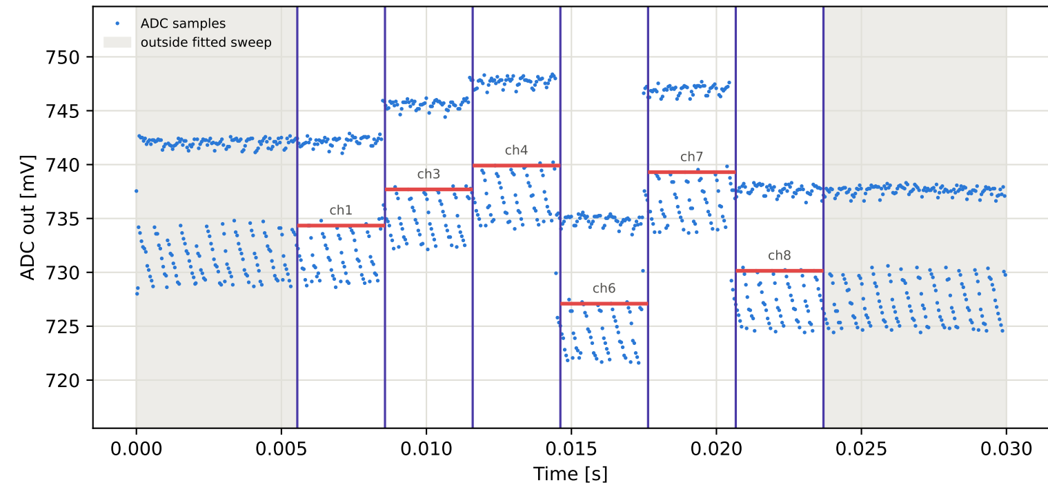
Tag8 &lt;- Tag16 | 965 MHz | run 0 | rep 1 | phase 141.64 deg
