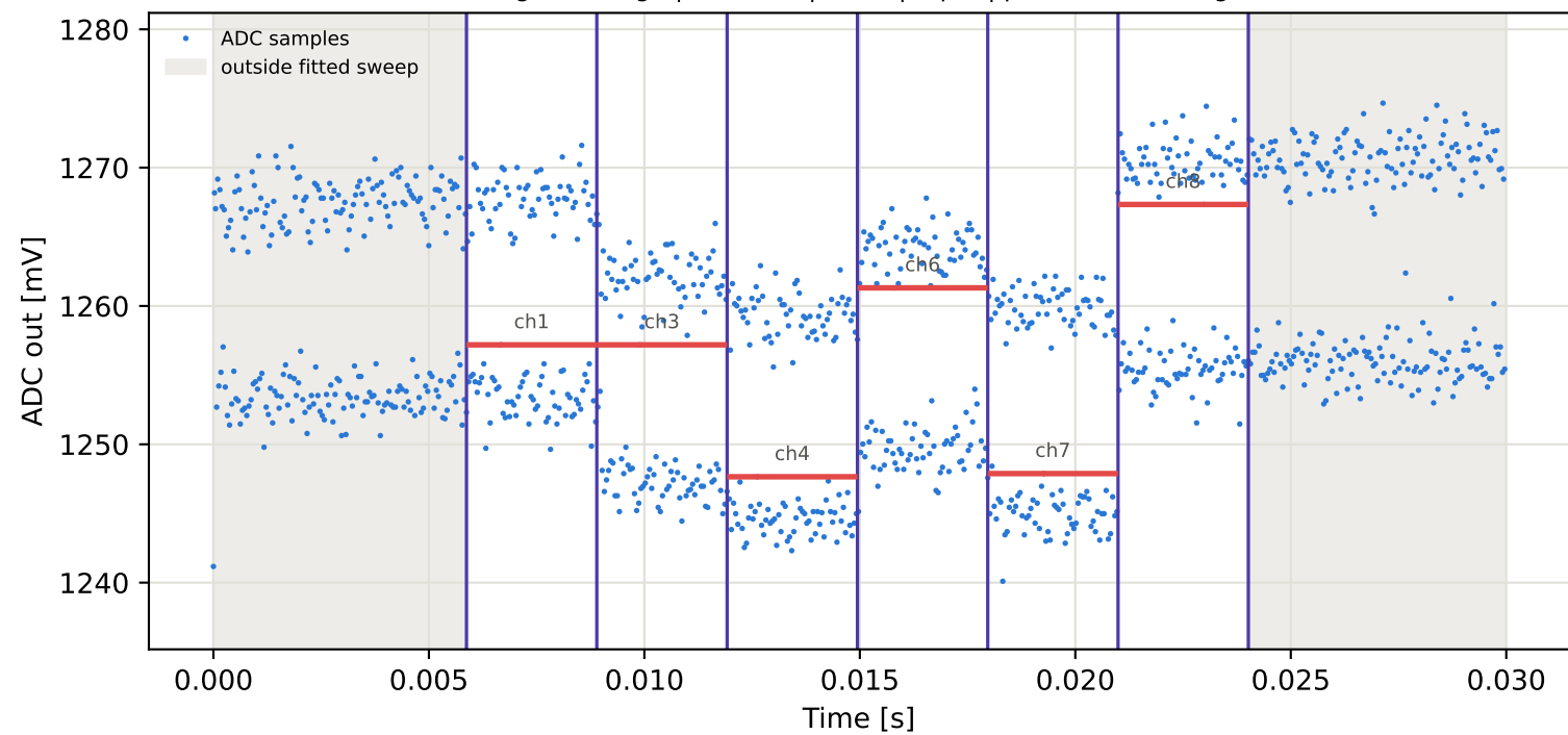
Tag16 &lt;- Tag15 | 885 MHz | run 0 | rep 1 | phase -161.89 deg
