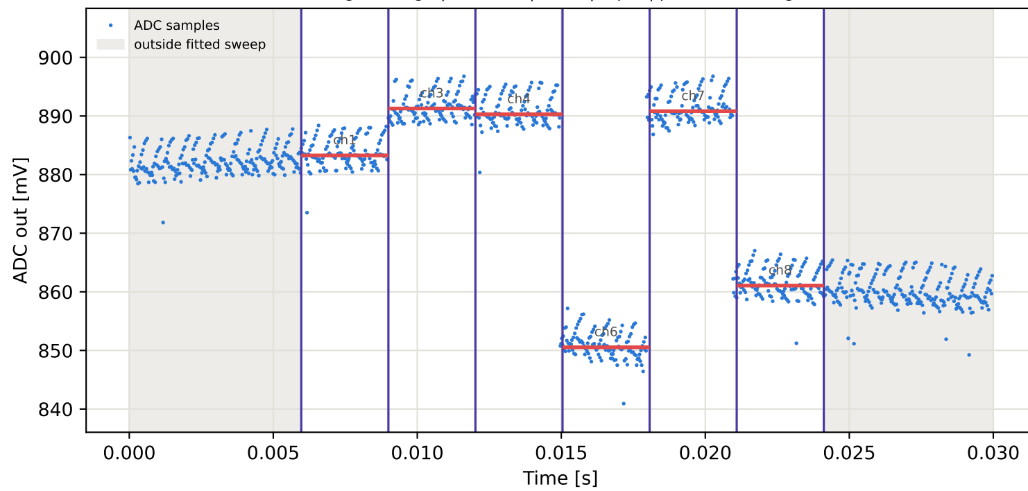
Tag8 &lt;- Tag1 | 915 MHz | run 0 | rep 1 | phase 71.22 deg
