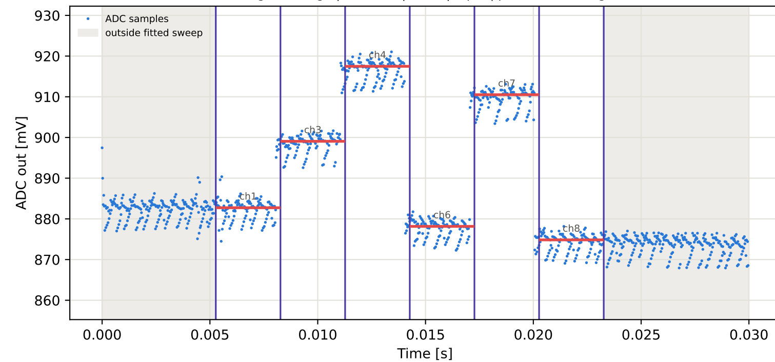
Tag15 &lt;- Tag9 | 975 MHz | run 0 | rep 1 | phase 85.63 deg
