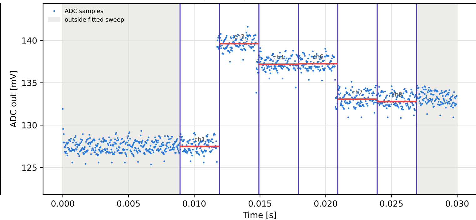
Tag7 &lt;- Tag6 | 795 MHz | run 0 | rep 1 | phase -97.54 deg
