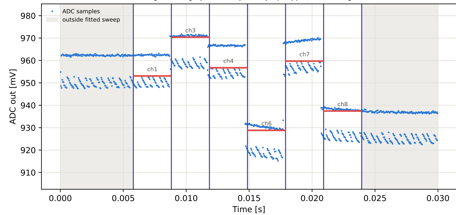
Tag15 &lt;- Tag6 | 895 MHz | run 0 | rep 1 | phase 1.78 deg
