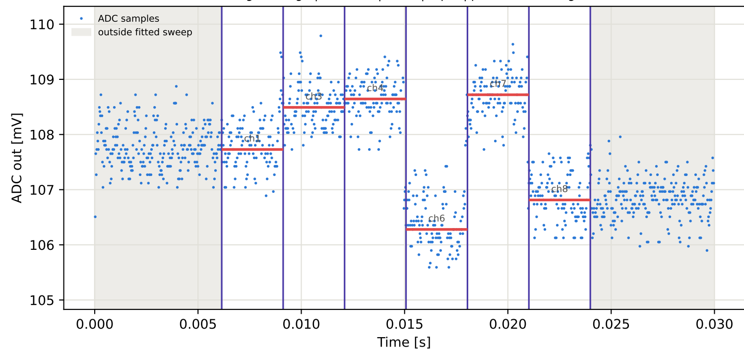
Tag2 &lt;- Tag7 | 935 MHz | run 0 | rep 1 | phase -24.39 deg
