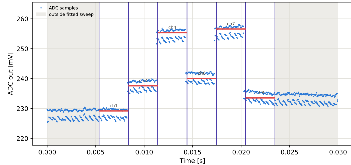
Tag6 &lt;- Tag5 | 805 MHz | run 0 | rep 1 | phase -105.70 deg
