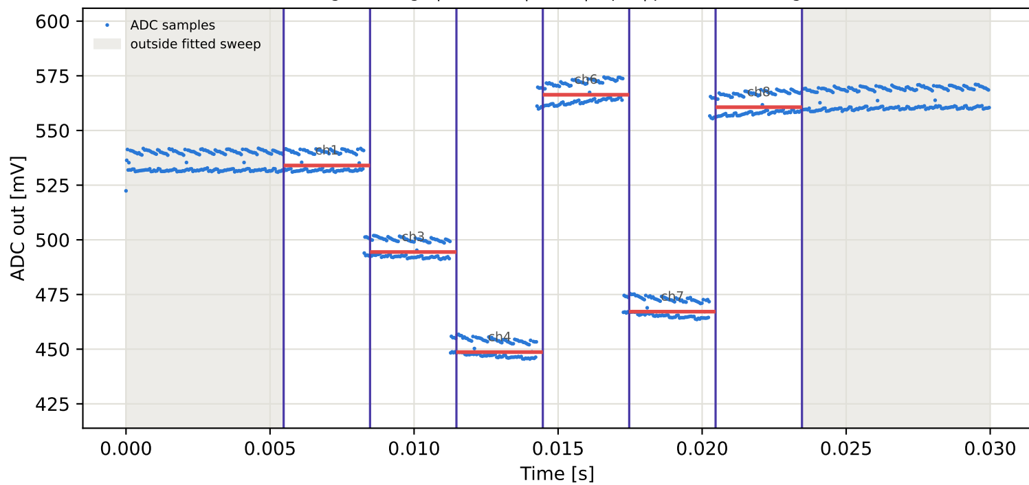
Tag2 &lt;- Tag1 | 985 MHz | run 0 | rep 1 | phase 50.12 deg
