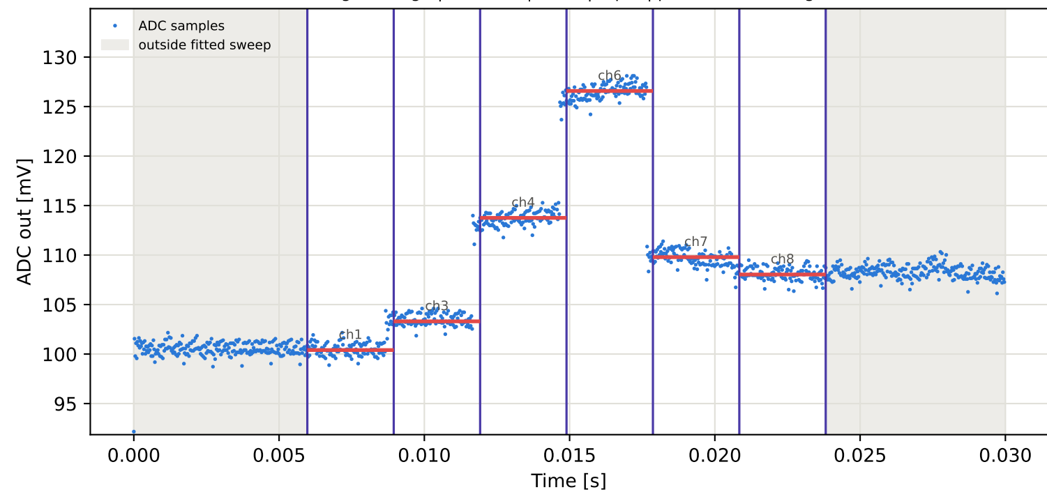
Tag2 &lt;- Tag8 | 915 MHz | run 0 | rep 1 | phase 61.13 deg
