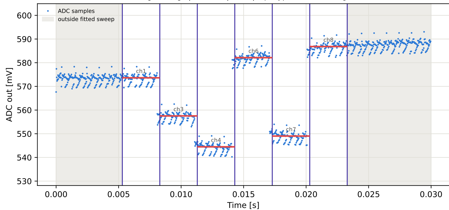
Tag6 &lt;- Tag10 | 945 MHz | run 0 | rep 1 | phase -28.20 deg
