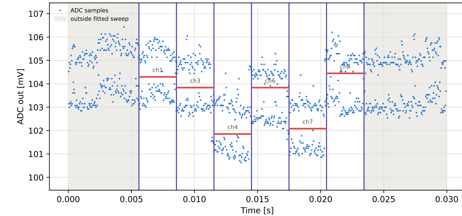
Tag15 &lt;- Tag1 | 775 MHz | run 0 | rep 1 | phase 19.77 deg
