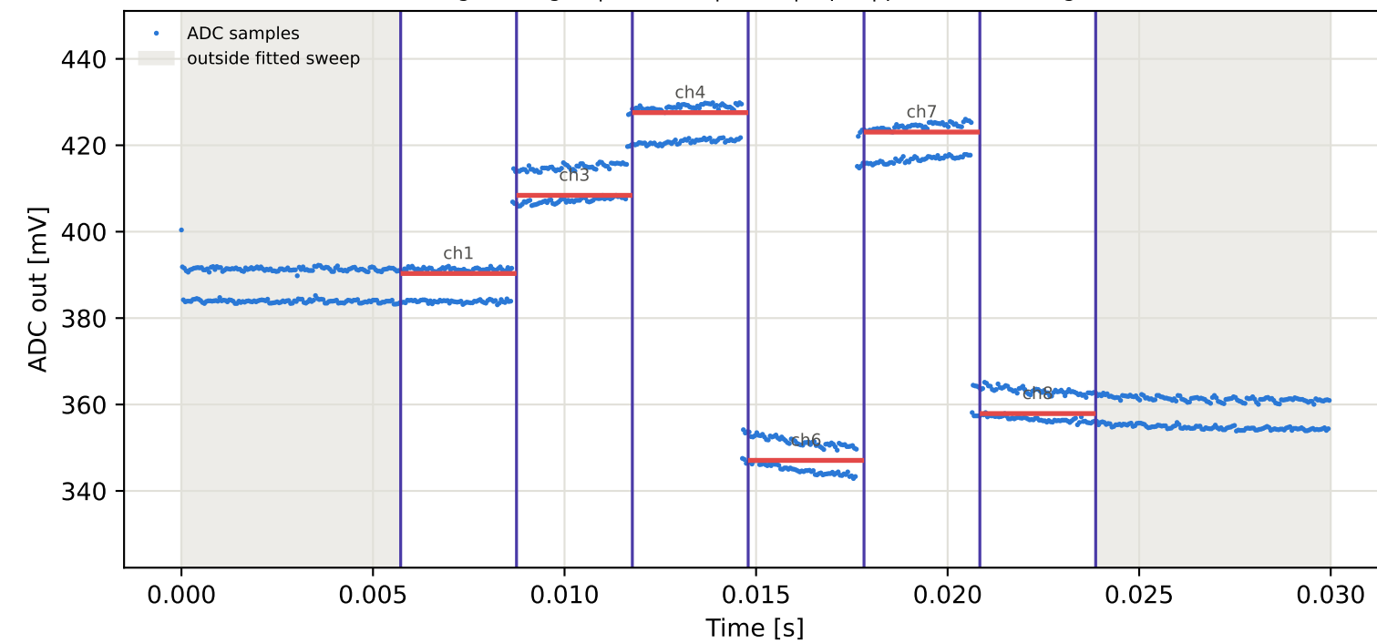
Tag7 &lt;- Tag3 | 945 MHz | run 0 | rep 1 | phase 60.07 deg
