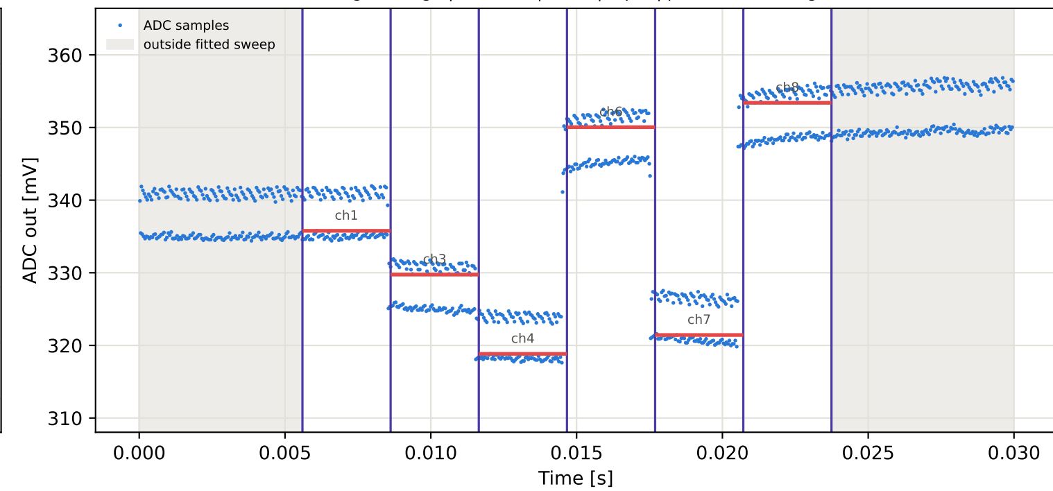
Tag3 &lt;- Tag7 | 925 MHz | run 0 | rep 1 | phase 93.94 deg
