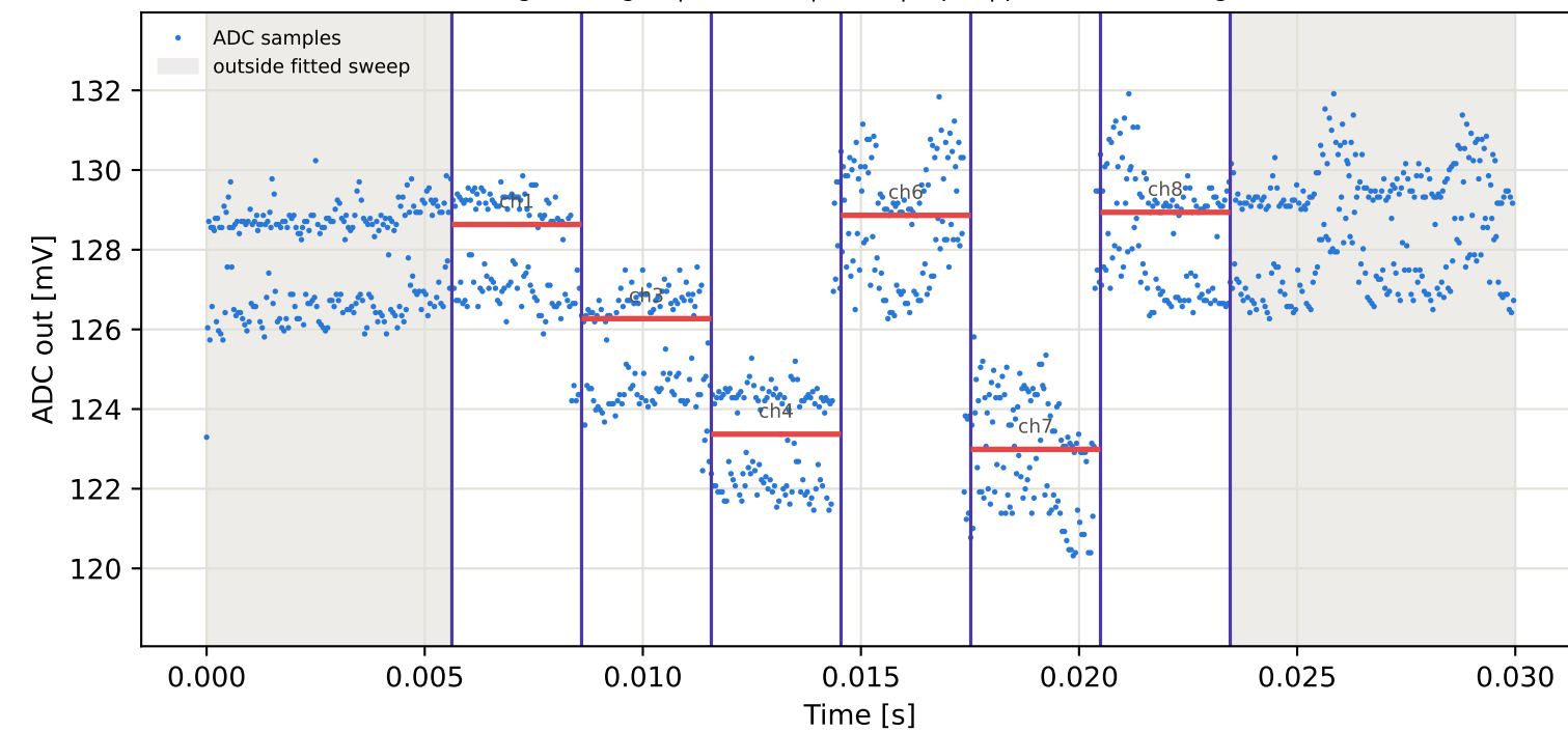
Tag7 &lt;- Tag3 | 775 MHz | run 0 | rep 1 | phase 69.84 deg
