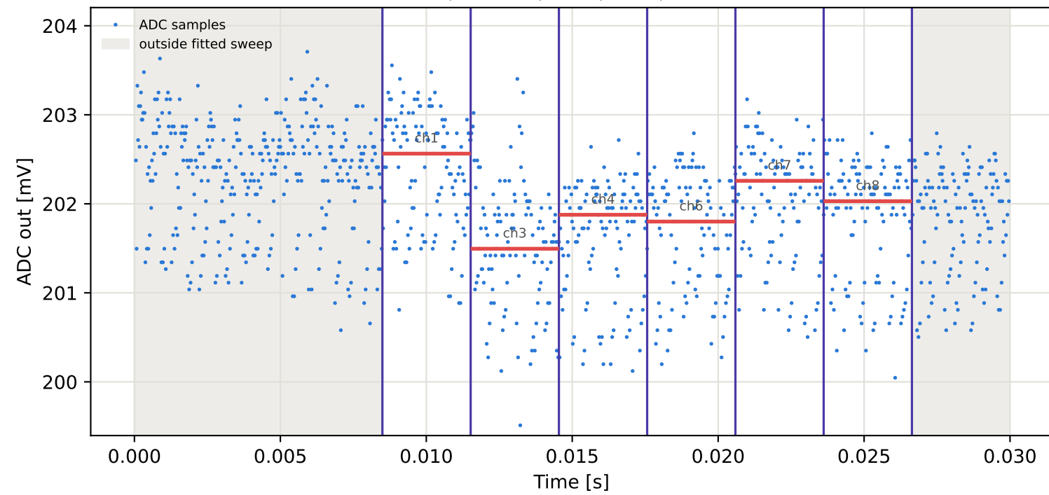
Tag5 &lt;- Tag1 | 775 MHz | run 0 | rep 1 | phase 80.05 deg
