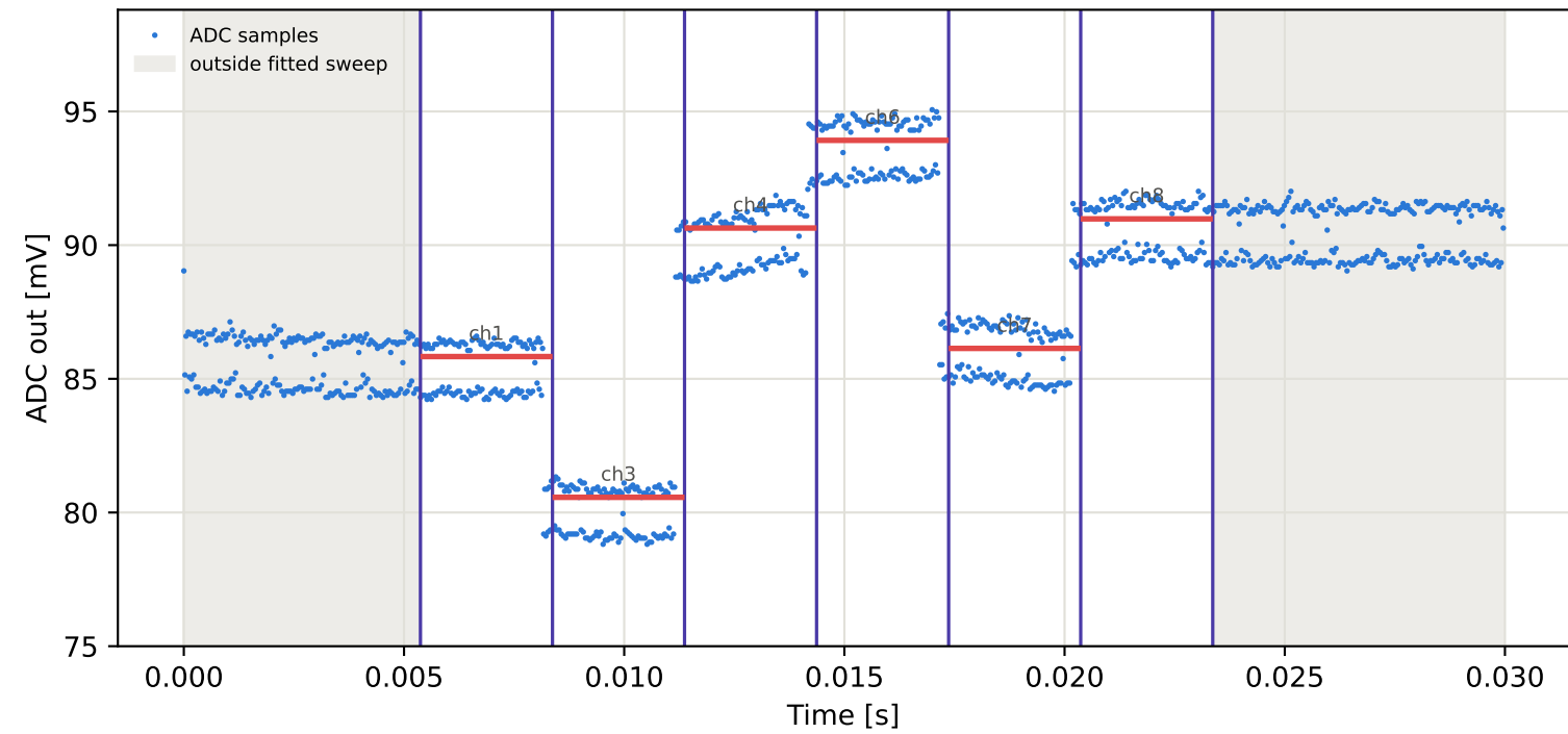
Tag9 &lt;- Tag2 | 795 MHz | run 0 | rep 1 | phase -82.06 deg
