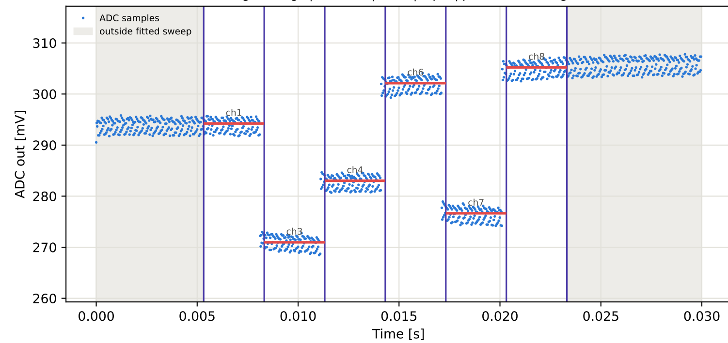
Tag3 &lt;- Tag8 | 835 MHz | run 0 | rep 1 | phase 168.91 deg
