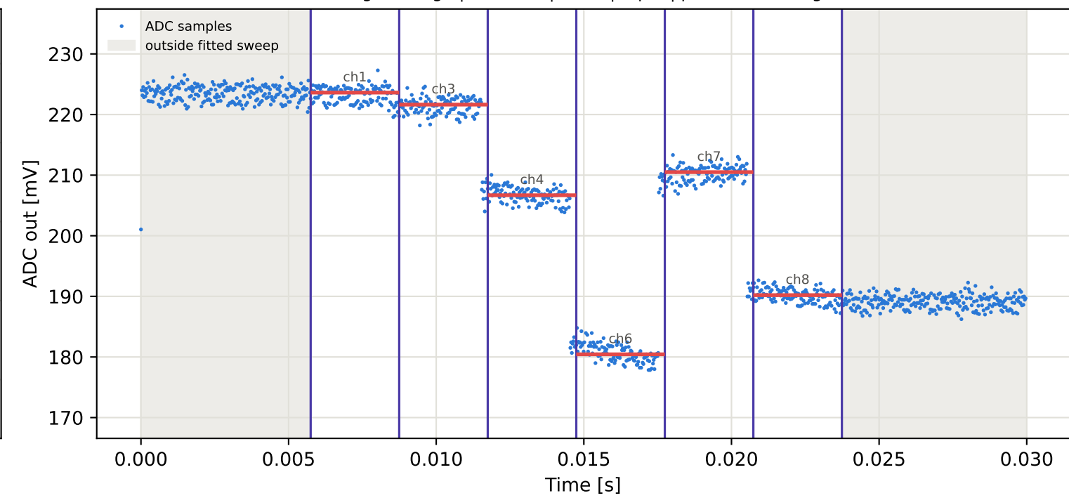
Tag2 &lt;- Tag8 | 885 MHz | run 0 | rep 1 | phase 21.44 deg
