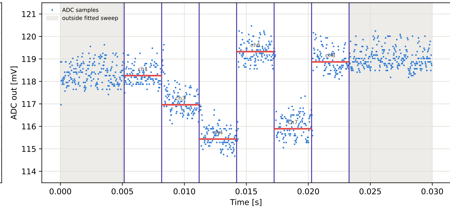
Tag2 &lt;- Tag8 | 975 MHz | run 0 | rep 1 | phase 44.17 deg
