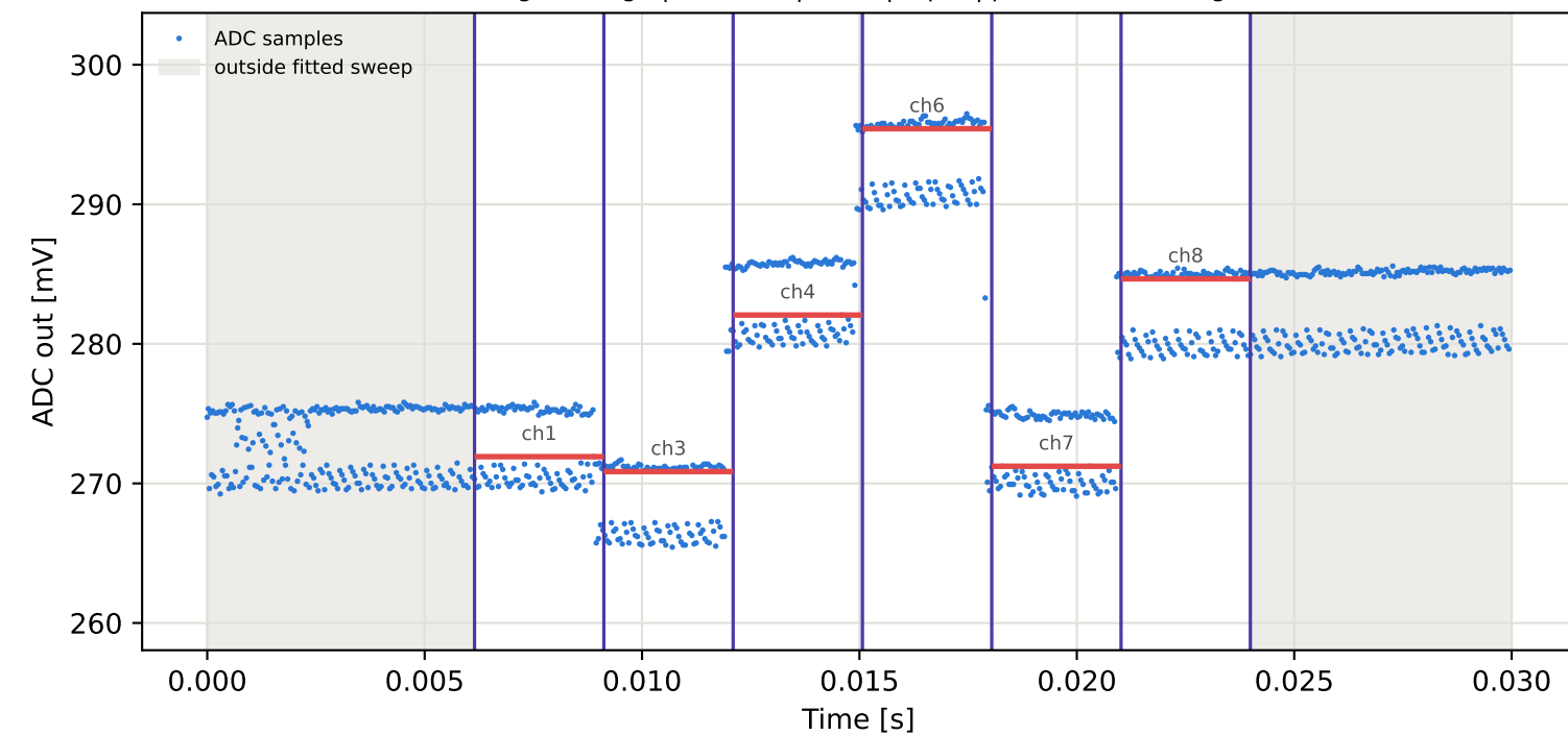
Tag3 &lt;- Tag8 | 985 MHz | run 0 | rep 1 | phase -98.22 deg
