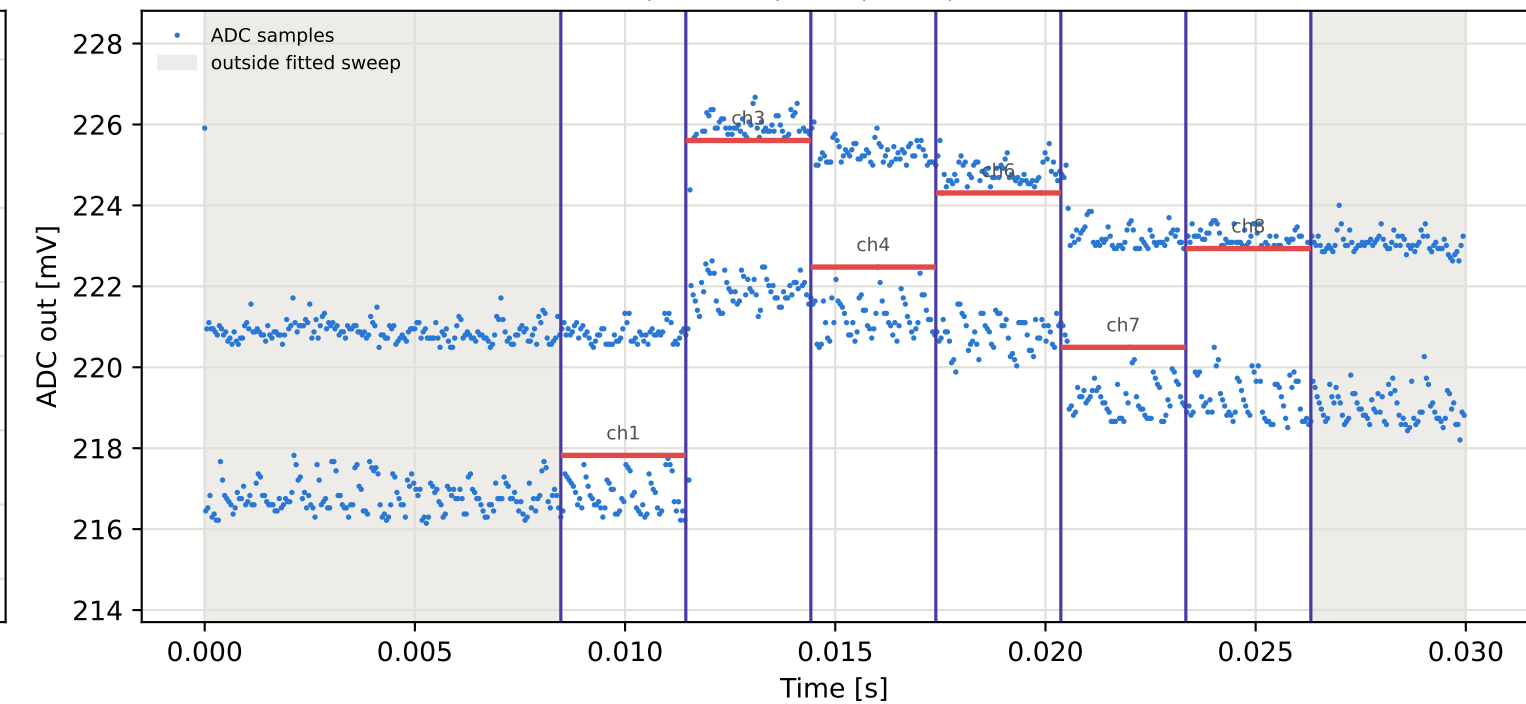
Tag6 &lt;- Tag5 | 795 MHz | run 0 | rep 1 | phase -132.38 deg
