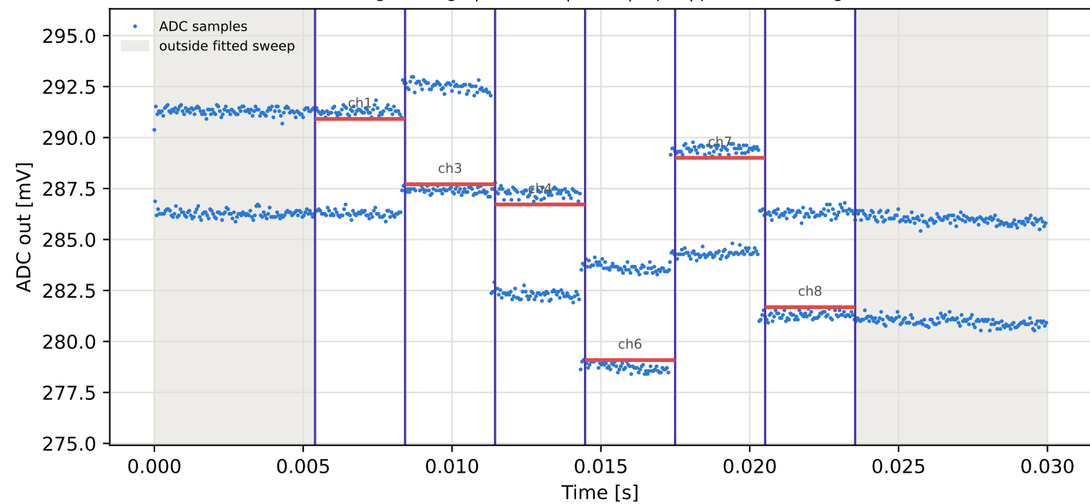
Tag1 &lt;- Tag9 | 865 MHz | run 0 | rep 1 | phase 19.26 deg
