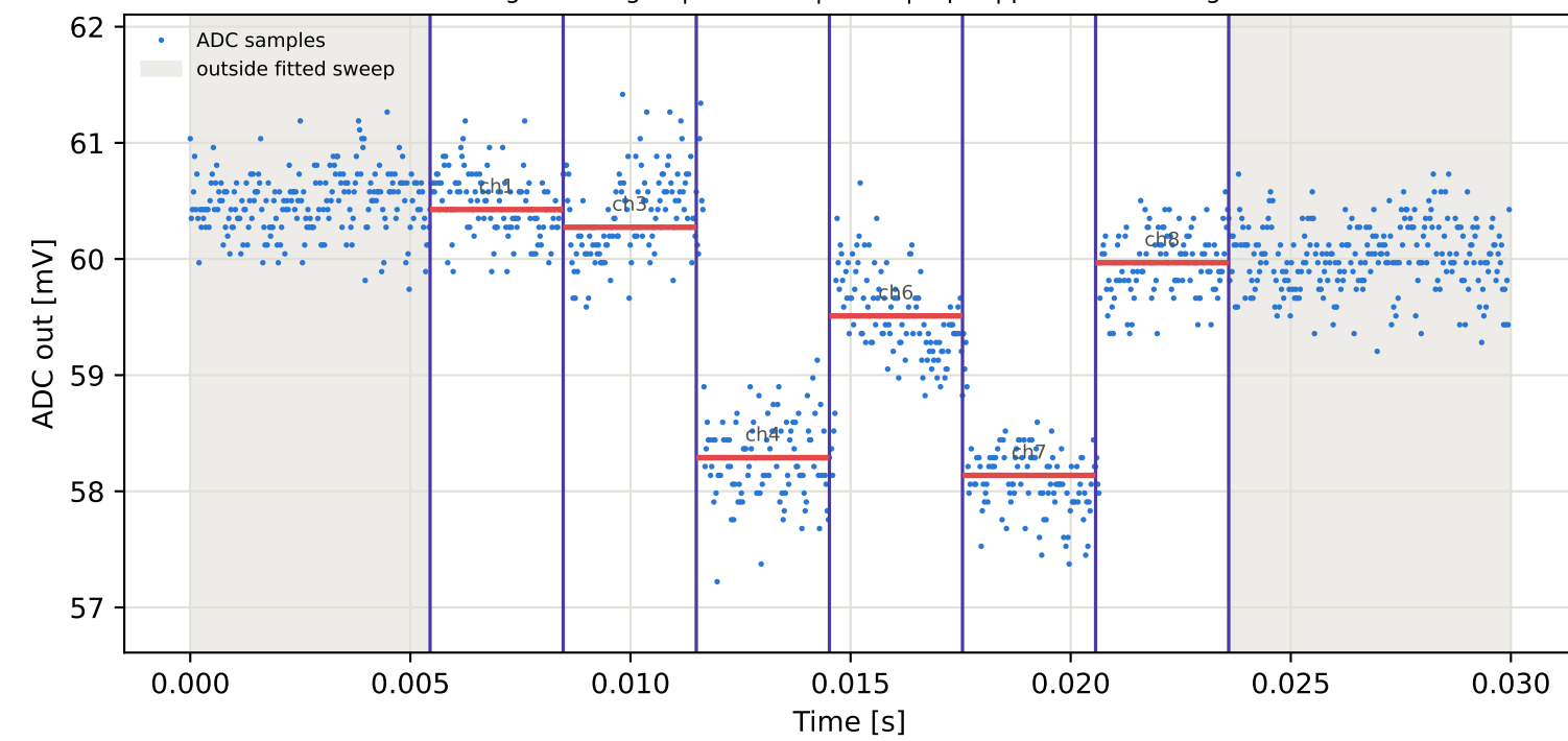
Tag10 &lt;- Tag2 | 785 MHz | run 0 | rep 1 | phase 55.46 deg
