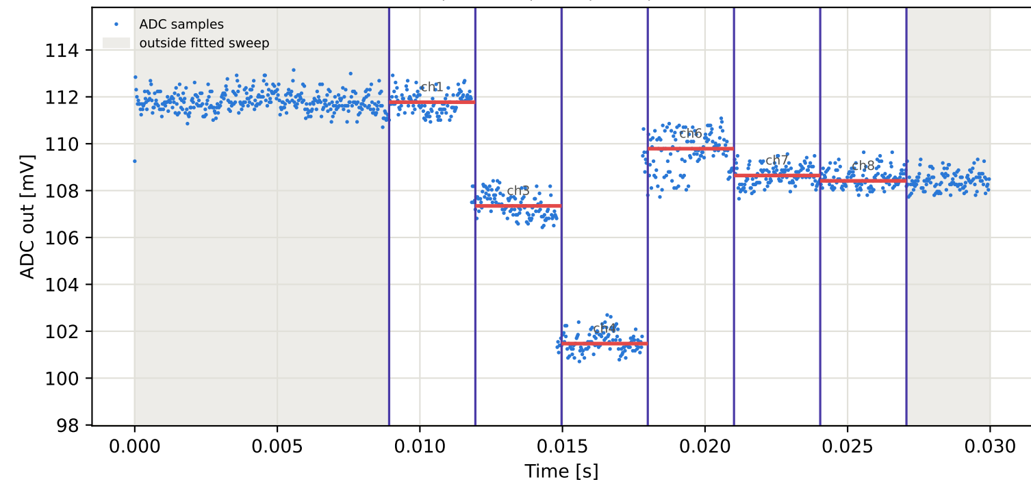
Tag2 &lt;- Tag8 | 945 MHz | run 0 | rep 1 | phase 77.93 deg
