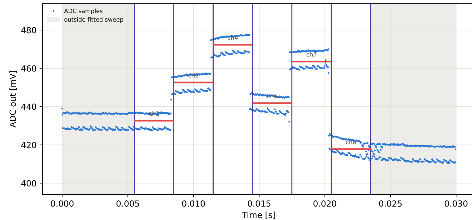
Tag10 &lt;- Tag4 | 915 MHz | run 0 | rep 1 | phase -78.94 deg
