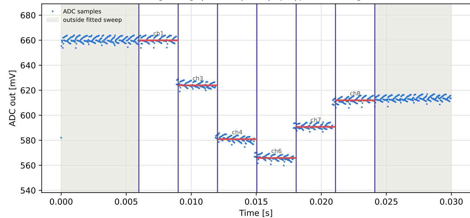
Tag6 &lt;- Tag5 | 865 MHz | run 0 | rep 1 | phase -13.46 deg
