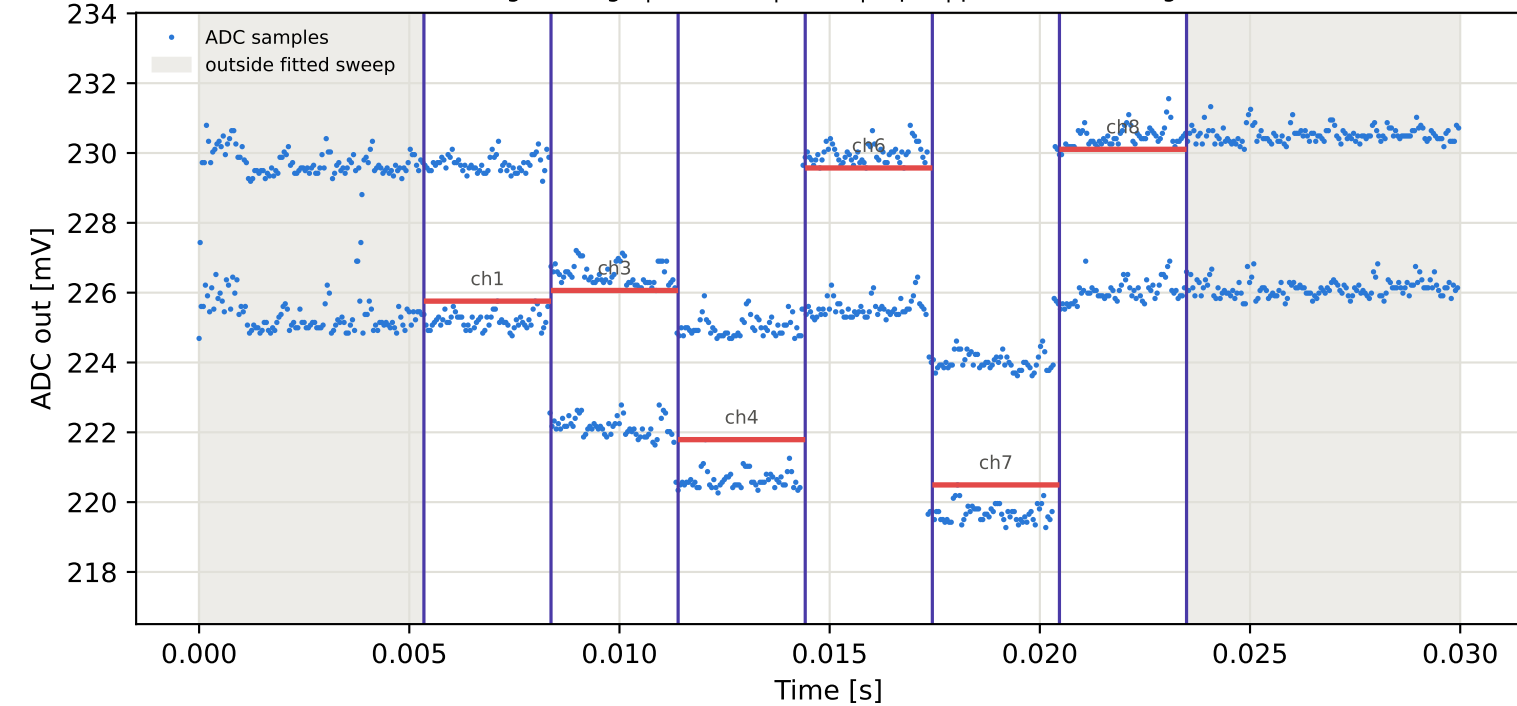
Tag6 &lt;- Tag1 | 795 MHz | run 0 | rep 1 | phase 140.27 deg
