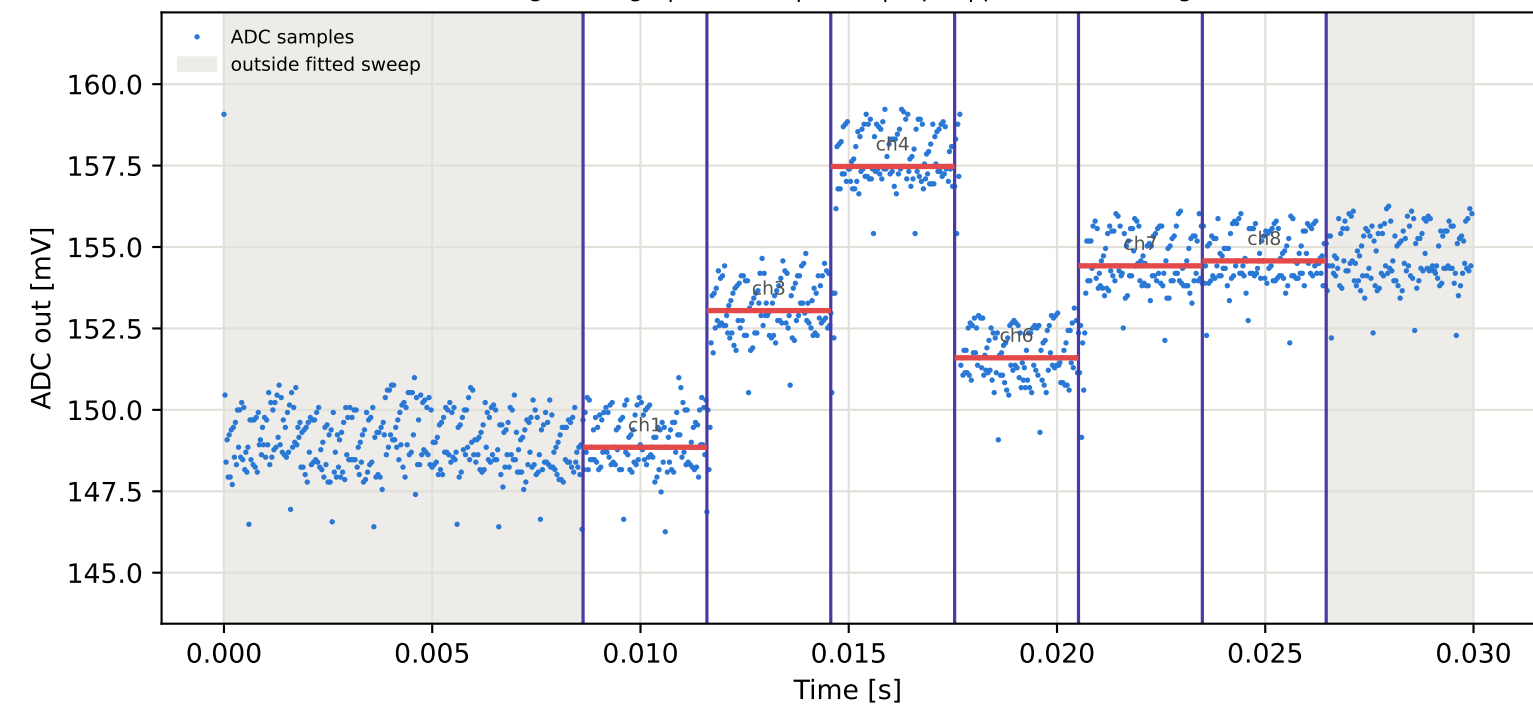
Tag6 &lt;- Tag4 | 845 MHz | run 0 | rep 1 | phase 82.62 deg
