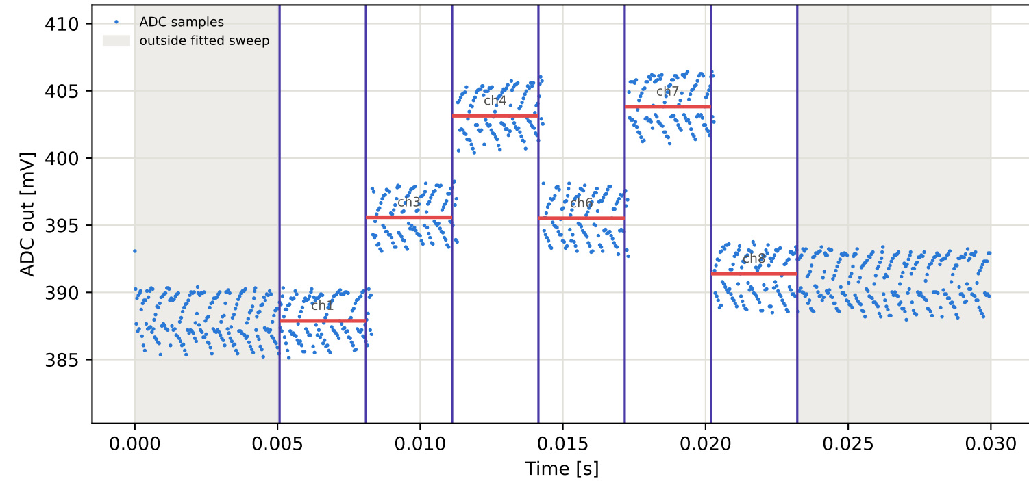
Tag9 &lt;- Tag2 | 835 MHz | run 0 | rep 1 | phase 92.38 deg
