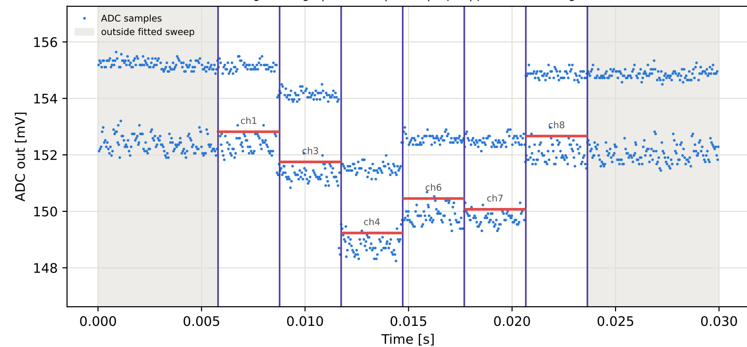
Tag4 &lt;- Tag2 | 805 MHz | run 0 | rep 1 | phase 81.75 deg
