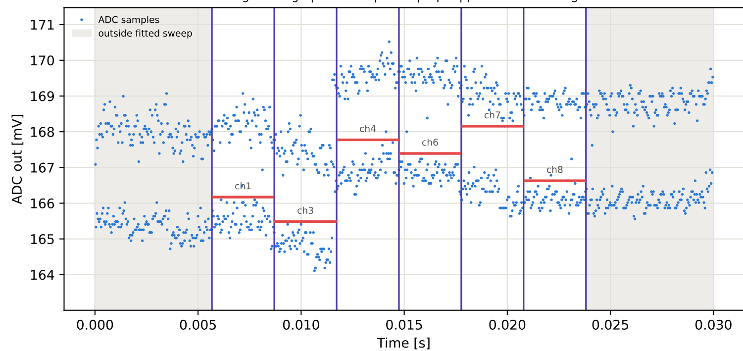
Tag6 &lt;- Tag10 | 785 MHz | run 0 | rep 1 | phase 104.62 deg
