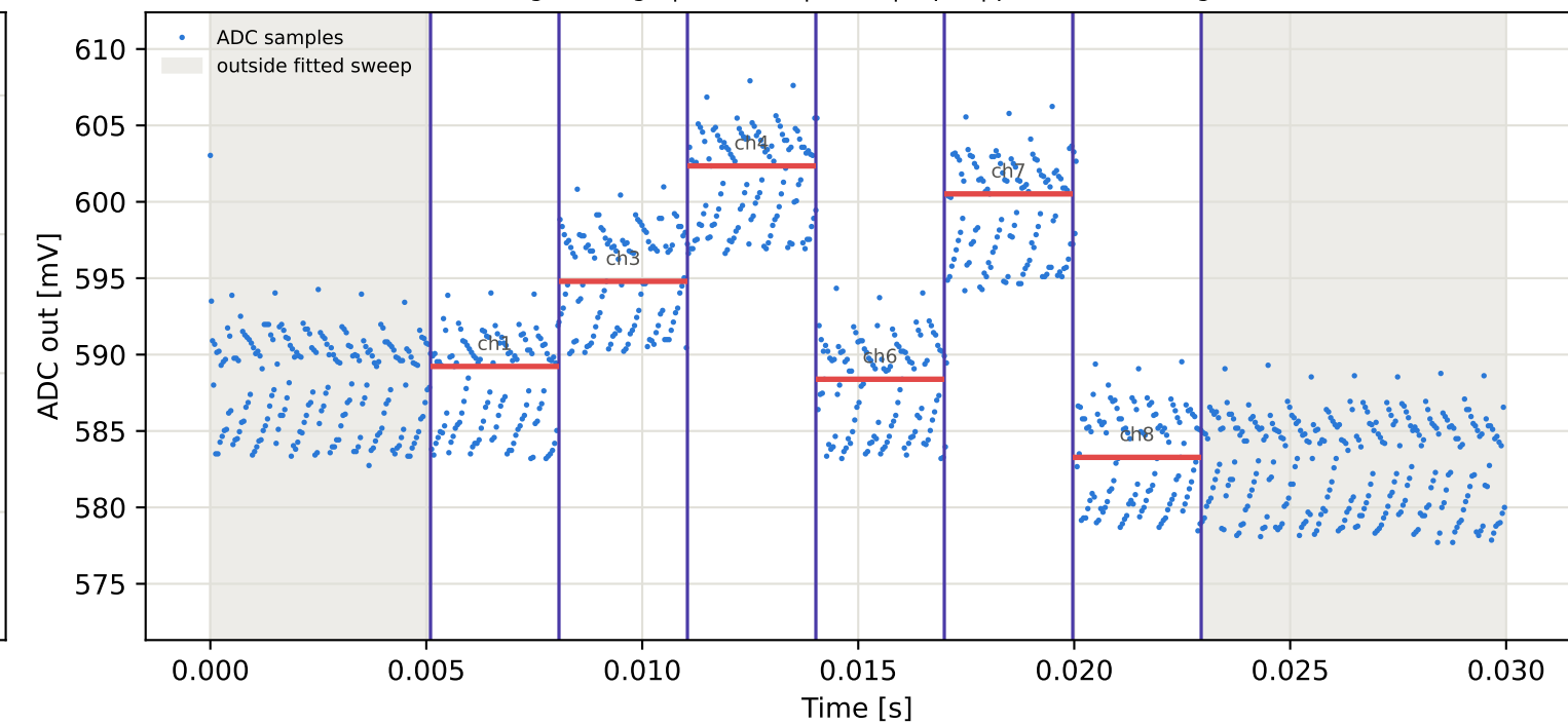
Tag5 &lt;- Tag9 | 925 MHz | run 0 | rep 1 | phase 87.46 deg
