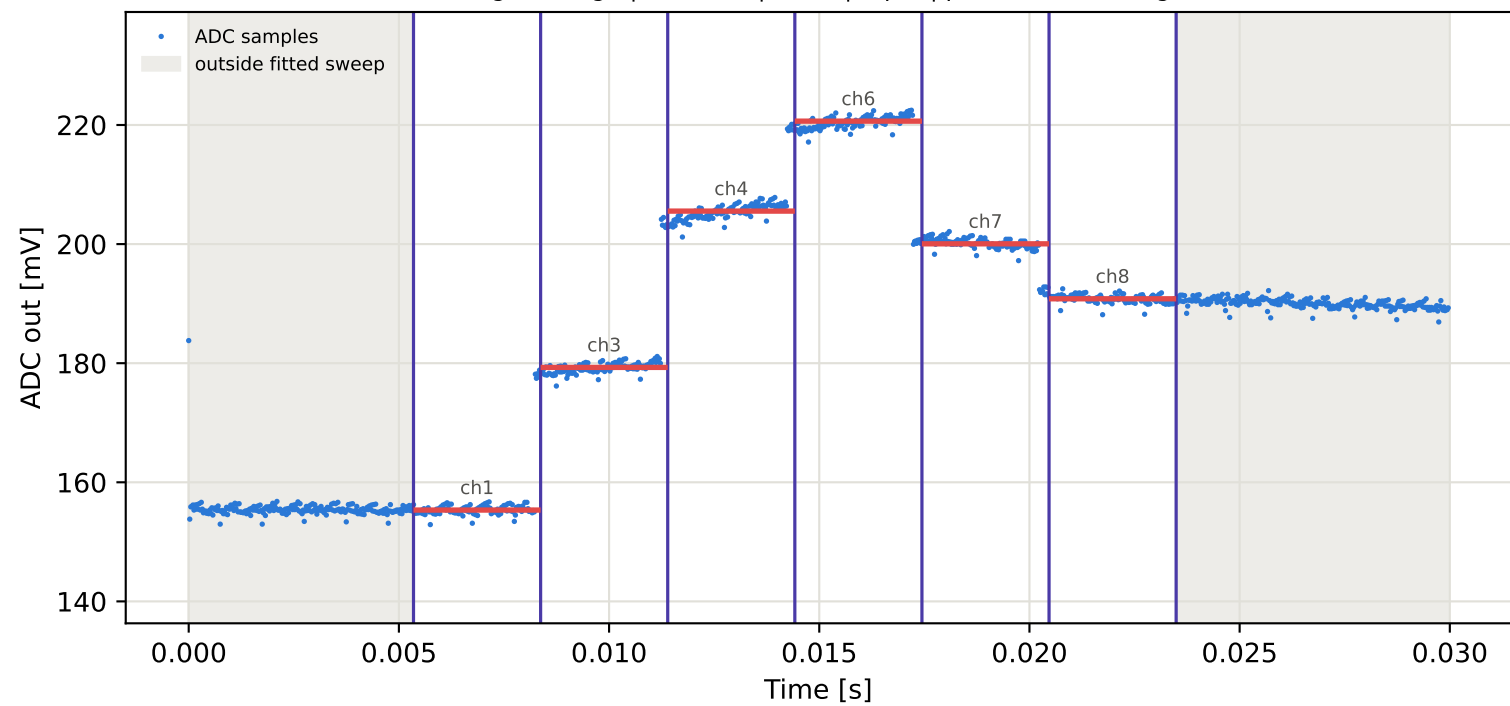
Tag2 &lt;- Tag6 | 875 MHz | run 0 | rep 1 | phase -137.37 deg
