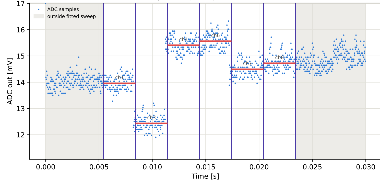
Tag2 &lt;- Tag6 | 795 MHz | run 0 | rep 1 | phase -15.76 deg
