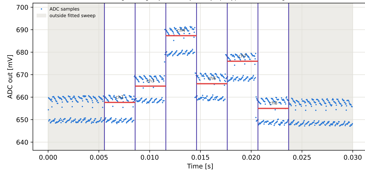
Tag7 &lt;- Tag10 | 965 MHz | run 0 | rep 1 | phase -99.37 deg
