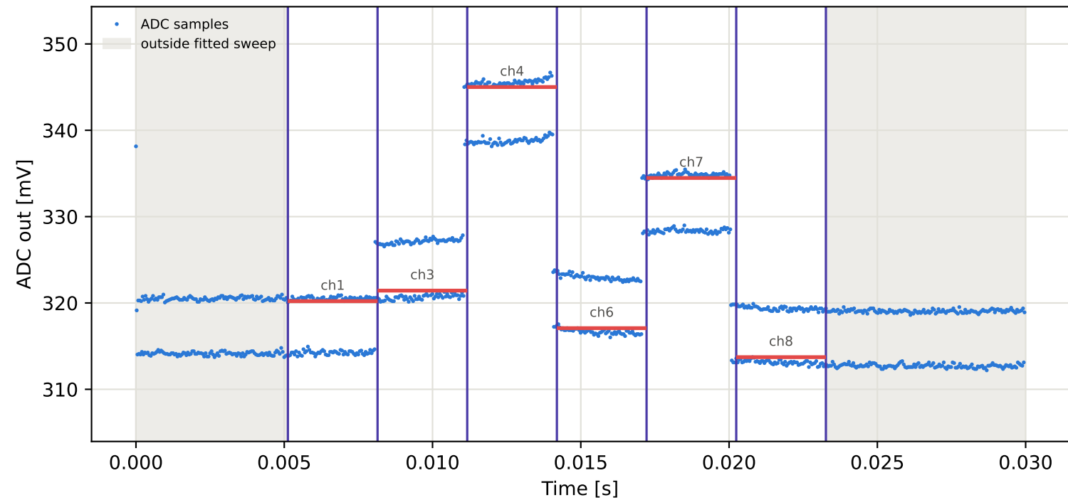
Tag16 &lt;- Tag6 | 995 MHz | run 0 | rep 1 | phase 27.57 deg
