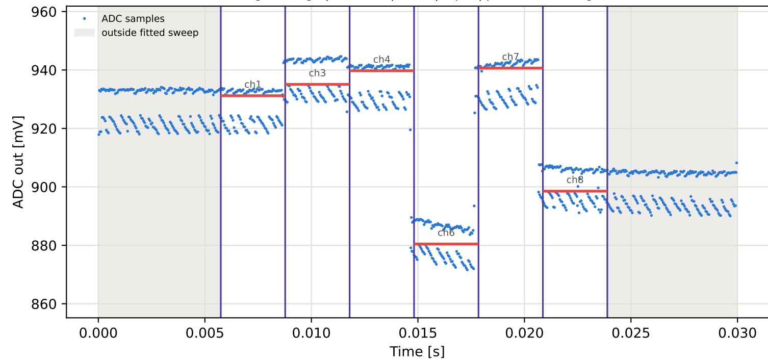
Tag4 &lt;- Tag8 | 915 MHz | run 0 | rep 1 | phase 7.33 deg
