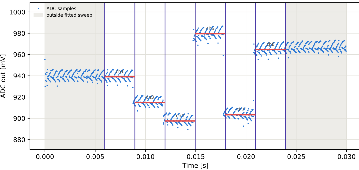
Tag15 &lt;- Tag5 | 965 MHz | run 0 | rep 1 | phase 140.43 deg
