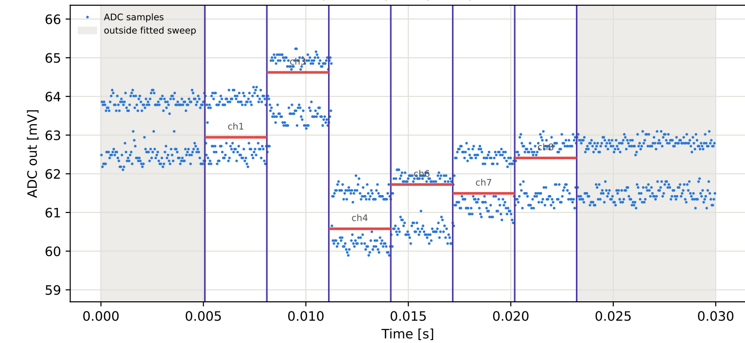
Tag8 &lt;- Tag6 | 775 MHz | run 0 | rep 1 | phase 67.55 deg
