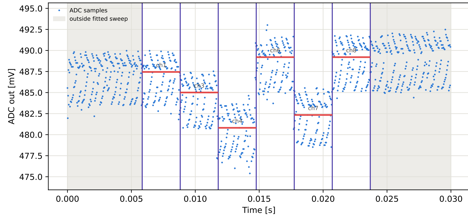
Tag16 &lt;- Tag15 | 985 MHz | run 0 | rep 1 | phase 15.40 deg
