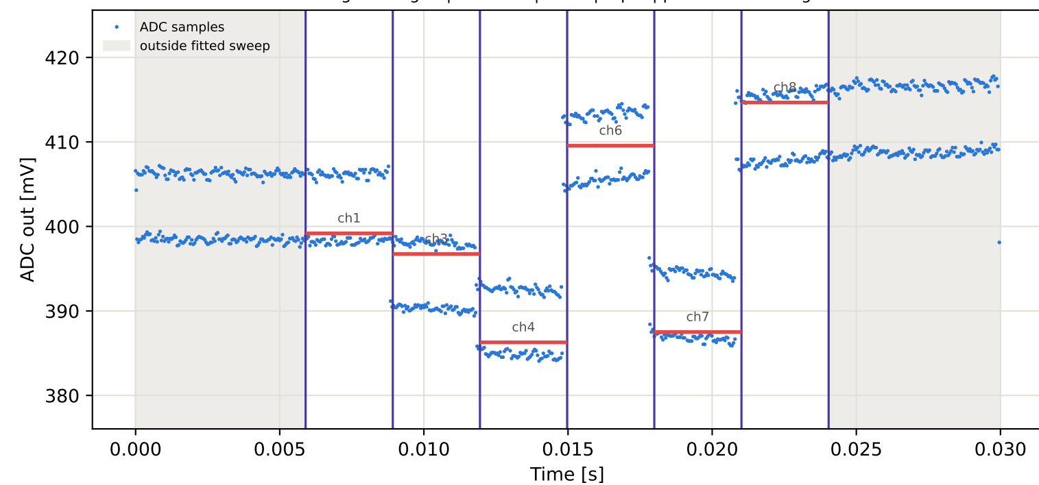
Tag7 &lt;- Tag15 | 935 MHz | run 0 | rep 1 | phase 129.99 deg
