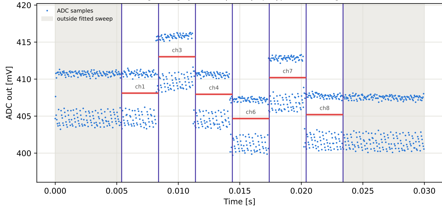
Tag3 &lt;- Tag15 | 845 MHz | run 0 | rep 1 | phase 15.09 deg
