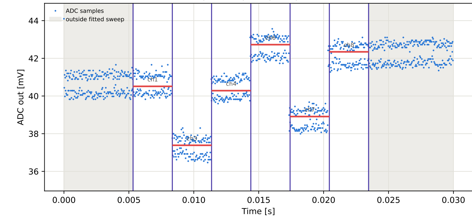
Tag16 &lt;- Tag6 | 785 MHz | run 0 | rep 1 | phase -168.03 deg
