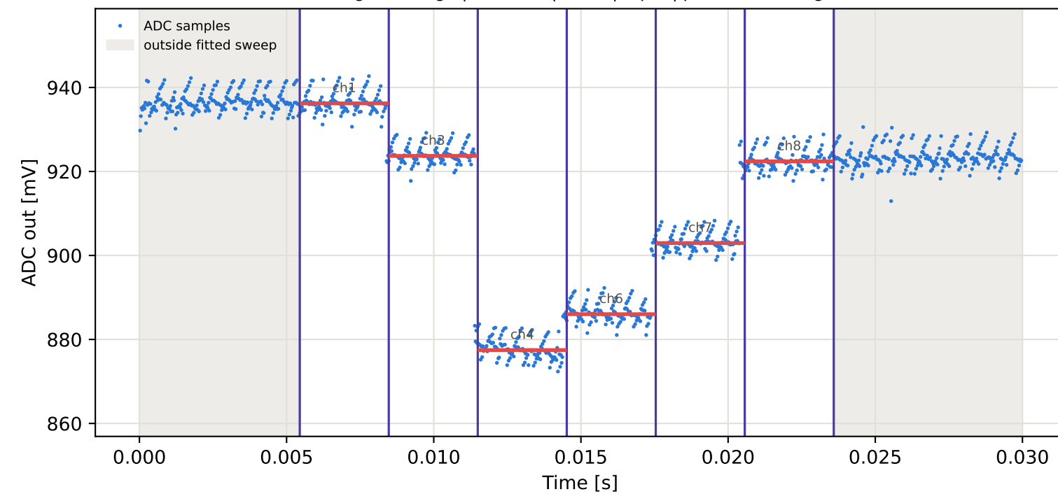
Tag16 &lt;- Tag10 | 965 MHz | run 0 | rep 1 | phase -124.51 deg
