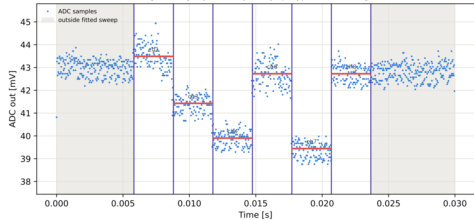
Tag10 &lt;- Tag3 | 805 MHz | run 0 | rep 1 | phase -67.26 deg
