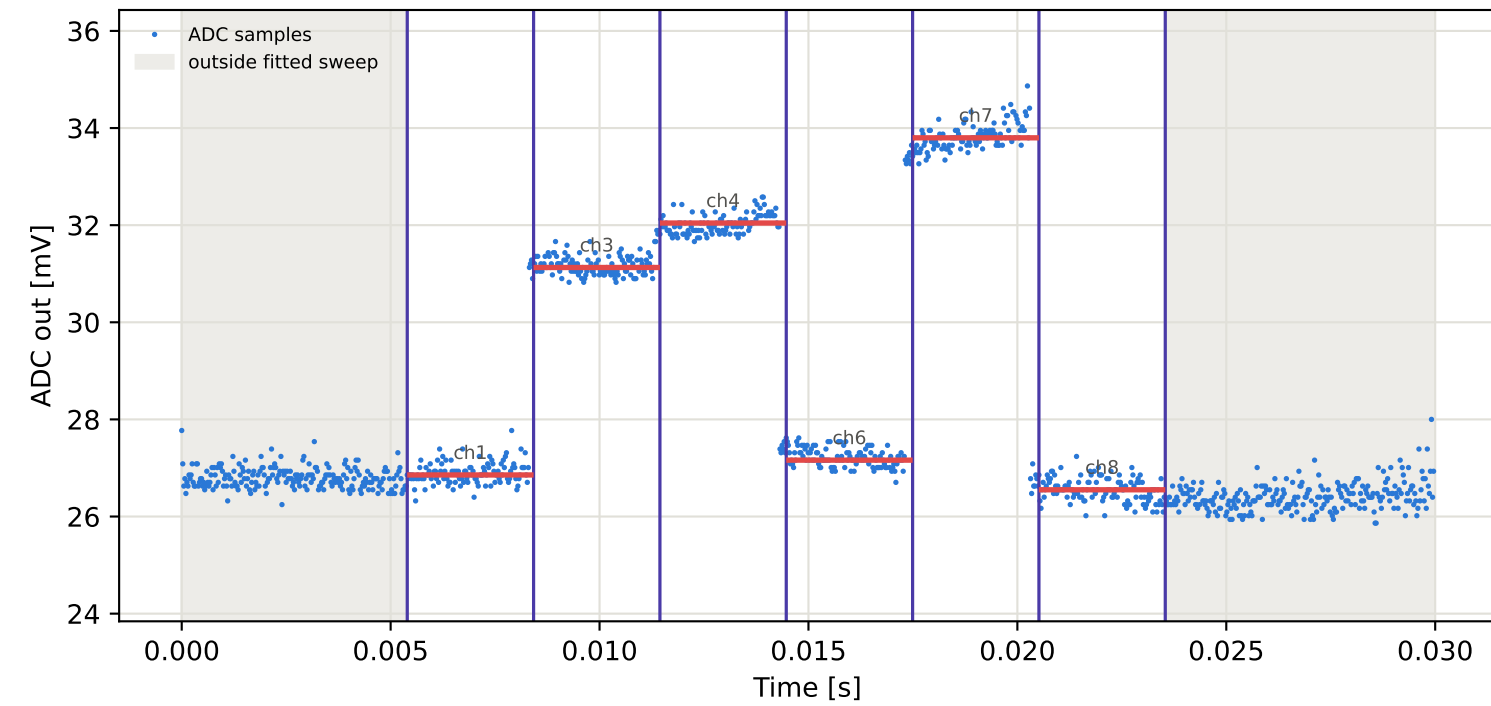
Tag1 &lt;- Tag8 | 785 MHz | run 0 | rep 1 | phase -106.79 deg
