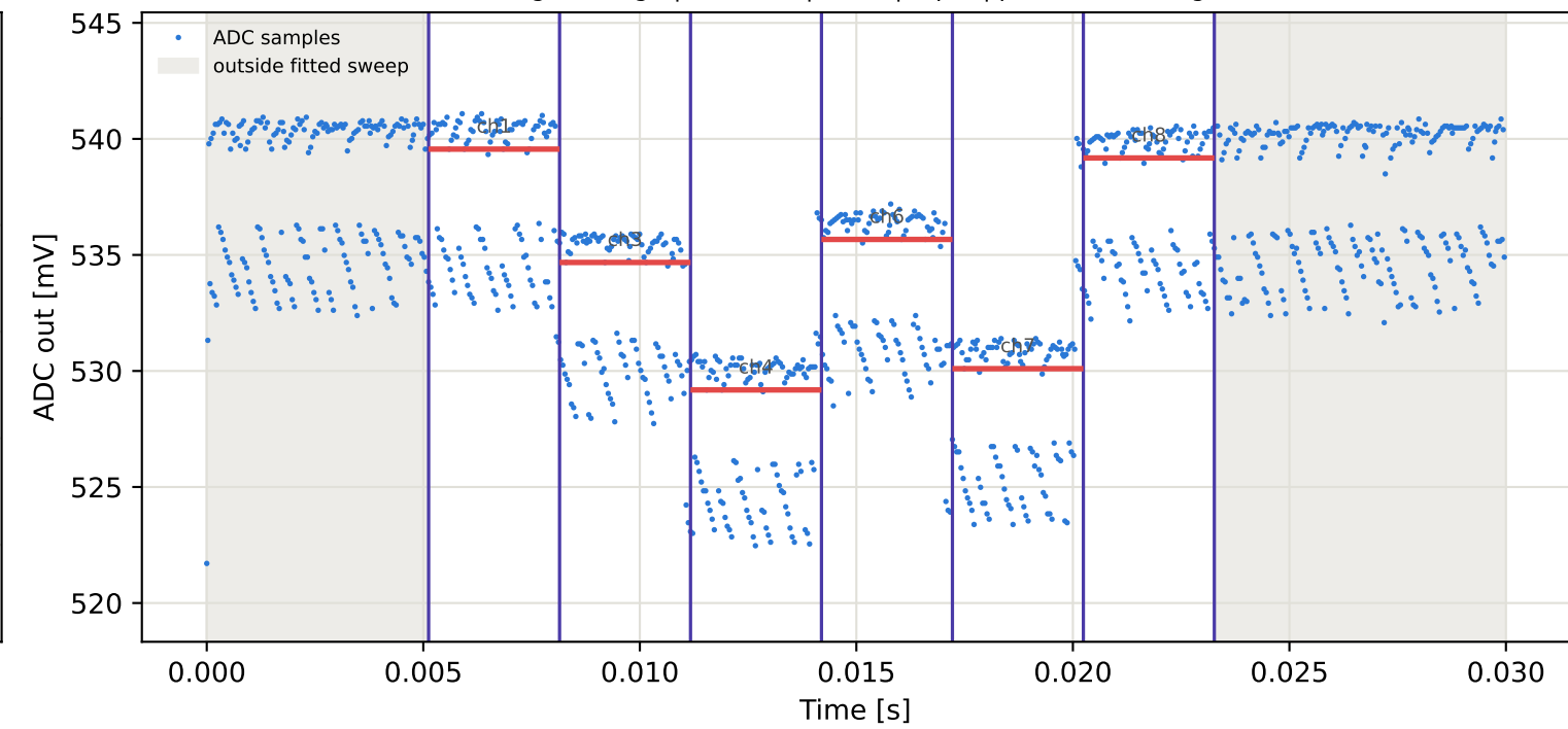
Tag5 &lt;- Tag9 | 835 MHz | run 0 | rep 1 | phase 3.68 deg
