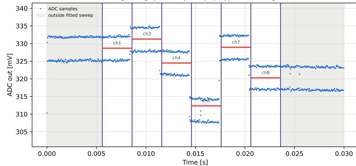
Tag1 &lt;- Tag9 | 965 MHz | run 0 | rep 1 | phase 10.79 deg
