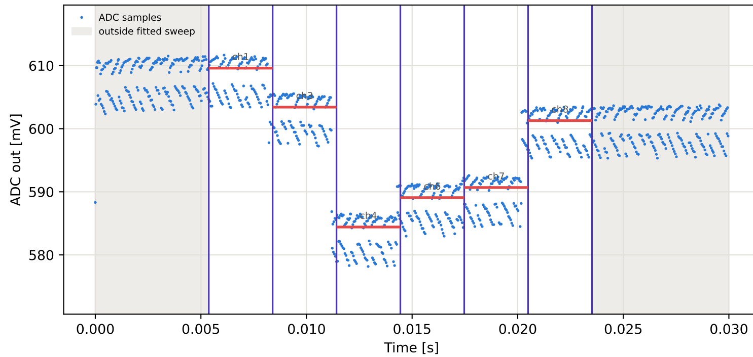
Tag9 &lt;- Tag10 | 835 MHz | run 0 | rep 1 | phase -30.16 deg
