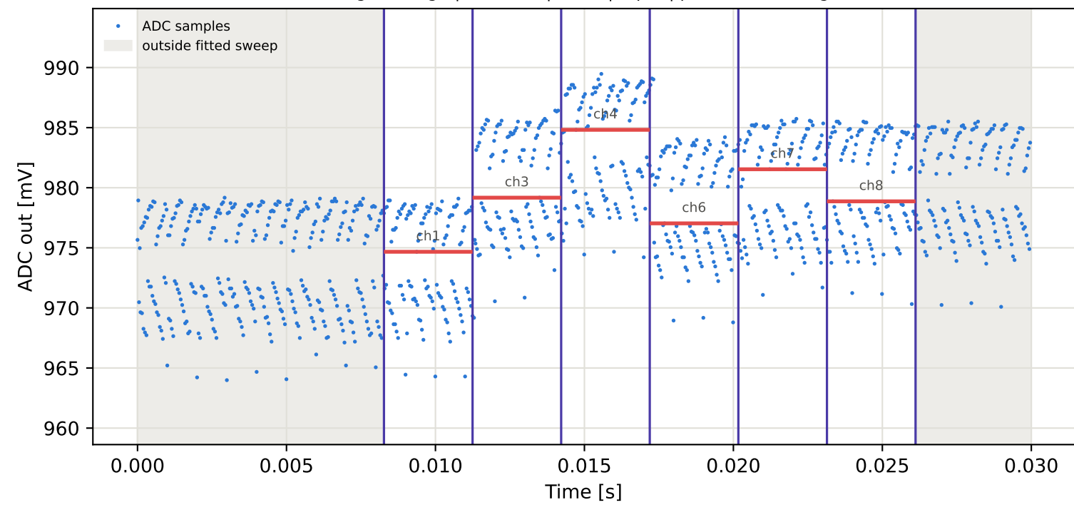
Tag5 &lt;- Tag9 | 865 MHz | run 0 | rep 1 | phase 120.25 deg
