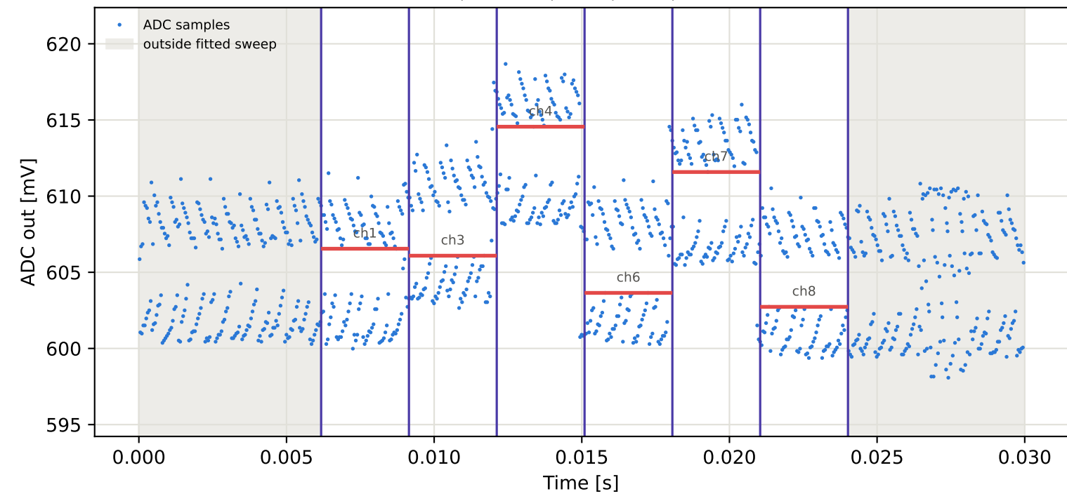
Tag15 &lt;- Tag6 | 985 MHz | run 0 | rep 1 | phase -81.32 deg
