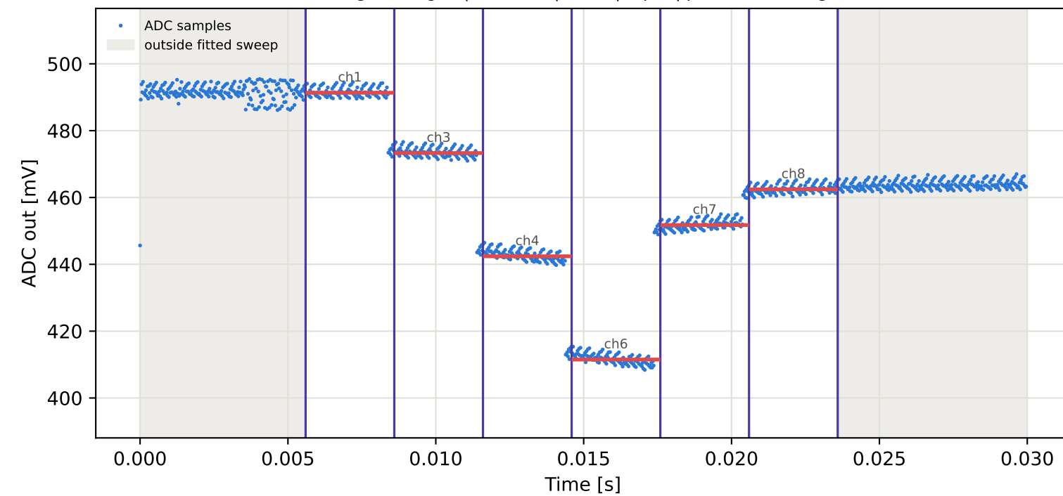
Tag1 &lt;- Tag16 | 895 MHz | run 0 | rep 1 | phase 157.52 deg
