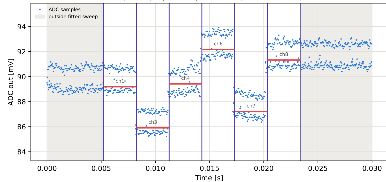
Tag4 &lt;- Tag2 | 795 MHz | run 0 | rep 1 | phase 87.29 deg
