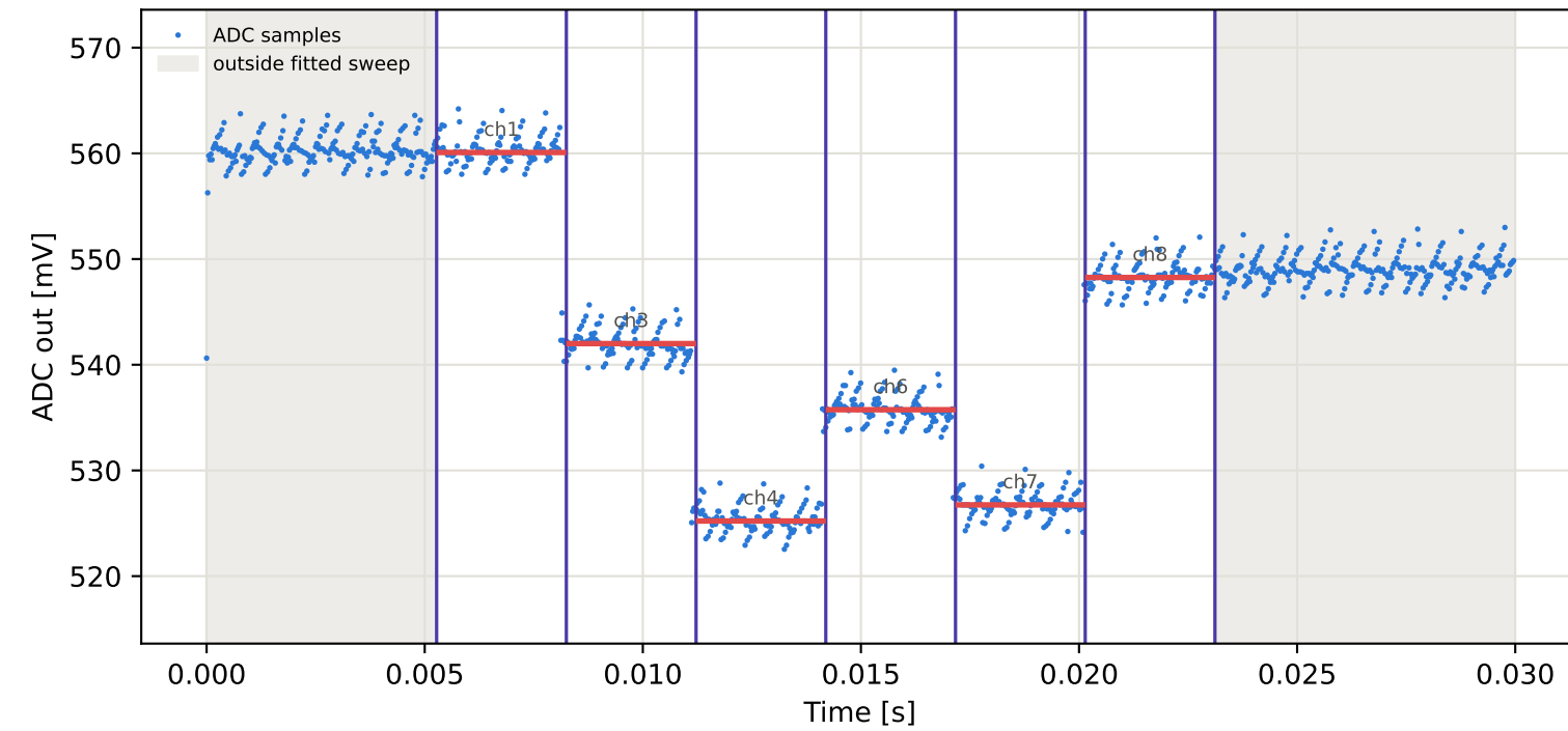
Tag6 &lt;- Tag1 | 835 MHz | run 0 | rep 1 | phase 127.35 deg
