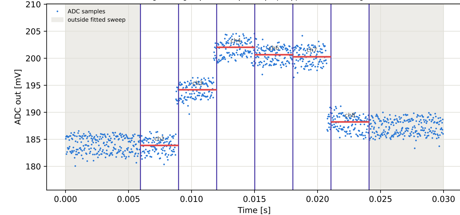
Tag2 &lt;- Tag15 | 885 MHz | run 0 | rep 1 | phase -108.64 deg
