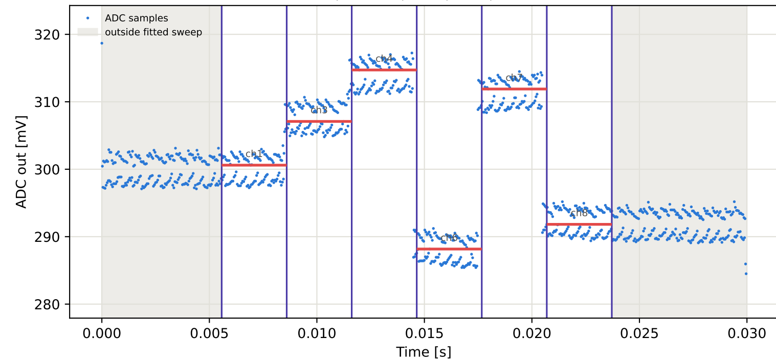
Tag10 &lt;- Tag4 | 965 MHz | run 0 | rep 1 | phase -43.31 deg
