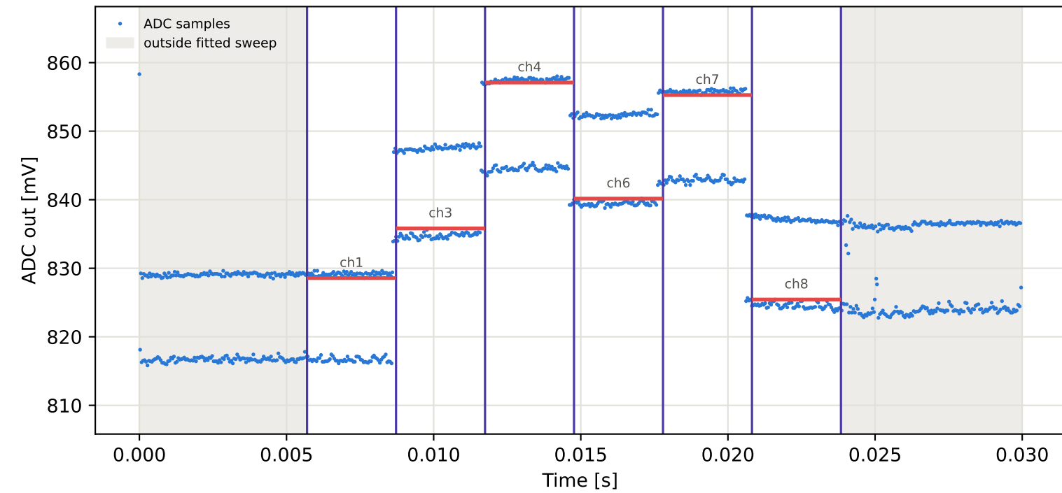
Tag16 &lt;- Tag6 | 865 MHz | run 0 | rep 1 | phase 24.33 deg
