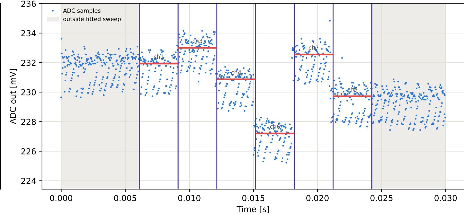
Tag5 &lt;- Tag1 | 995 MHz | run 0 | rep 1 | phase 6.05 deg
