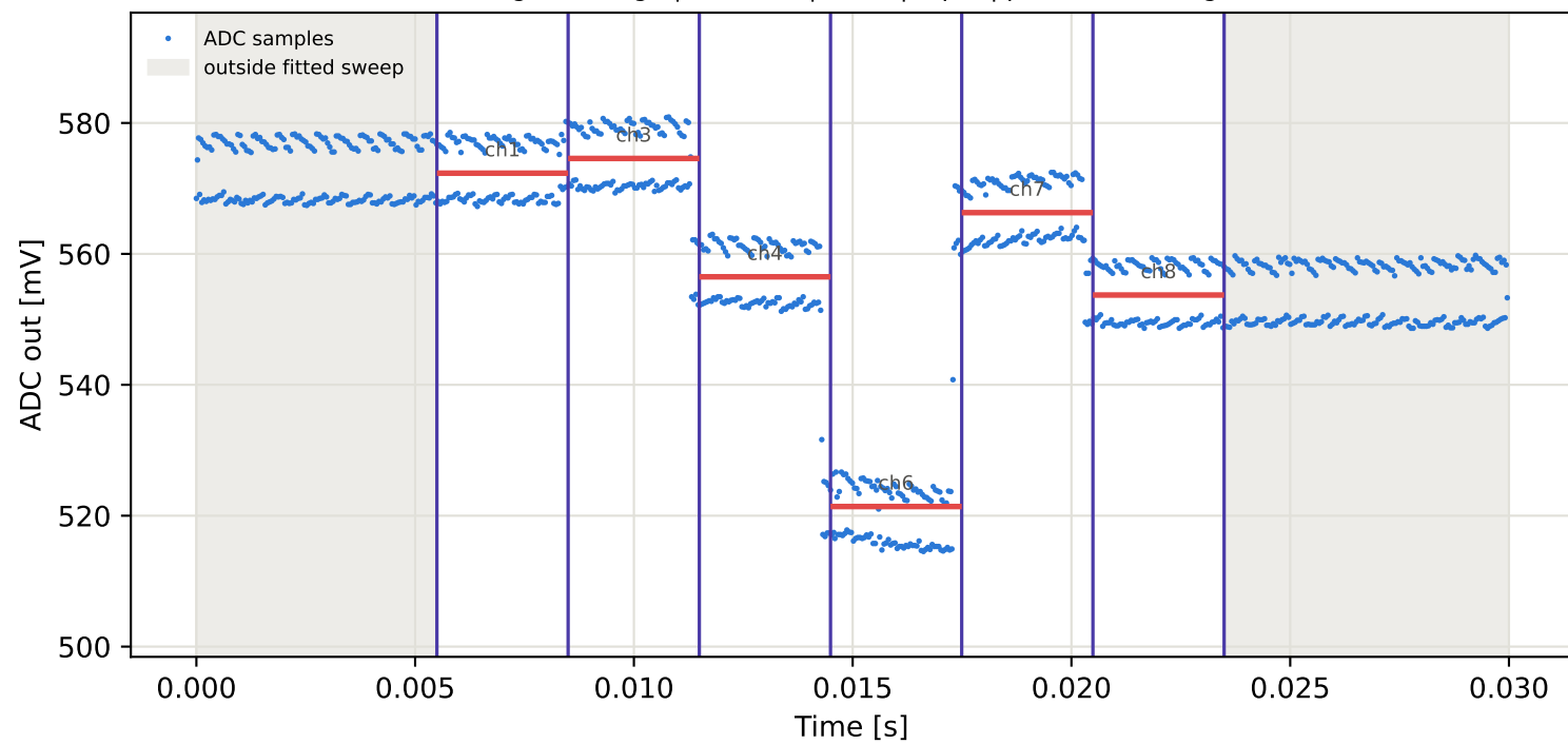
Tag10 &lt;- Tag8 | 935 MHz | run 0 | rep 1 | phase -25.46 deg
