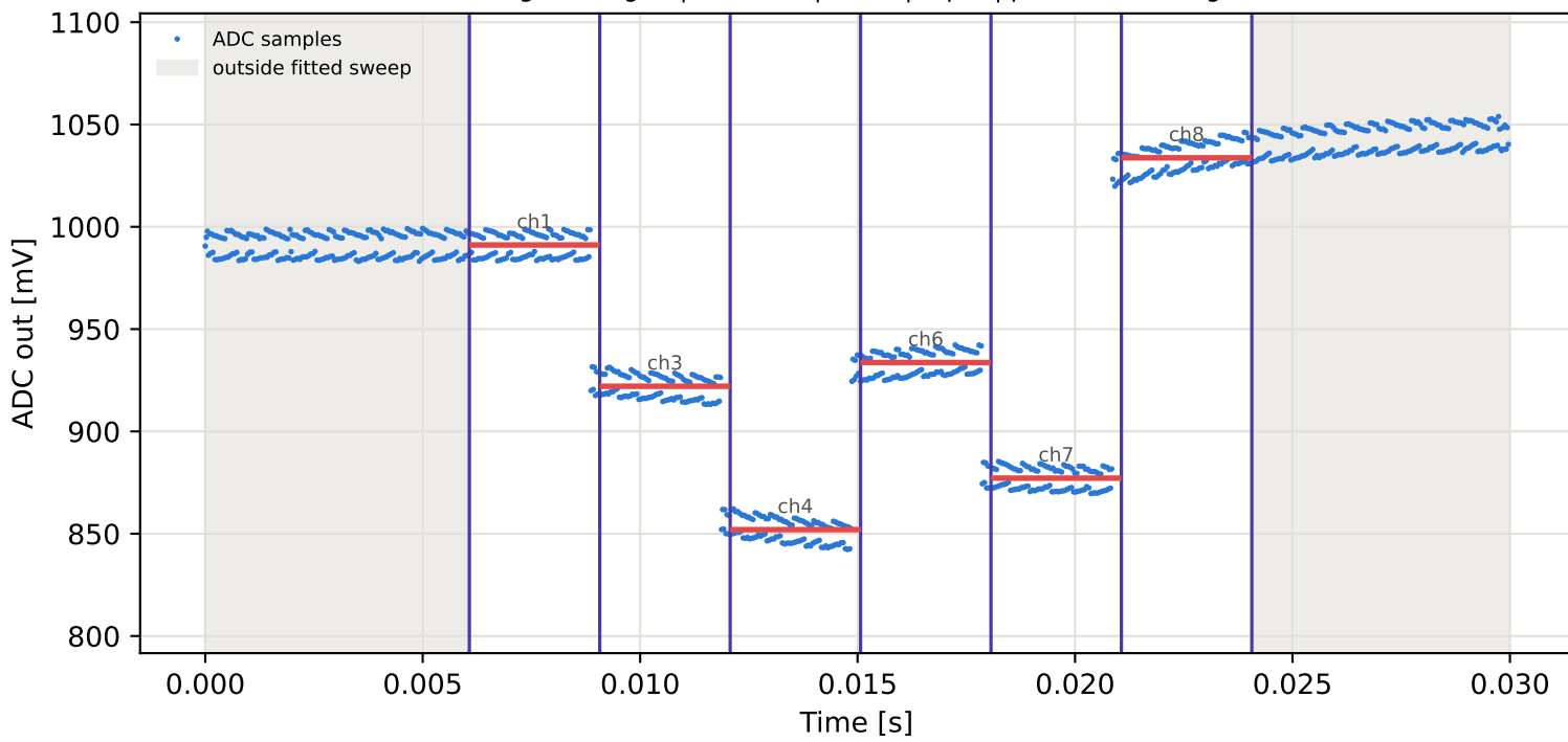
Tag8 &lt;- Tag16 | 915 MHz | run 0 | rep 1 | phase 92.76 deg
