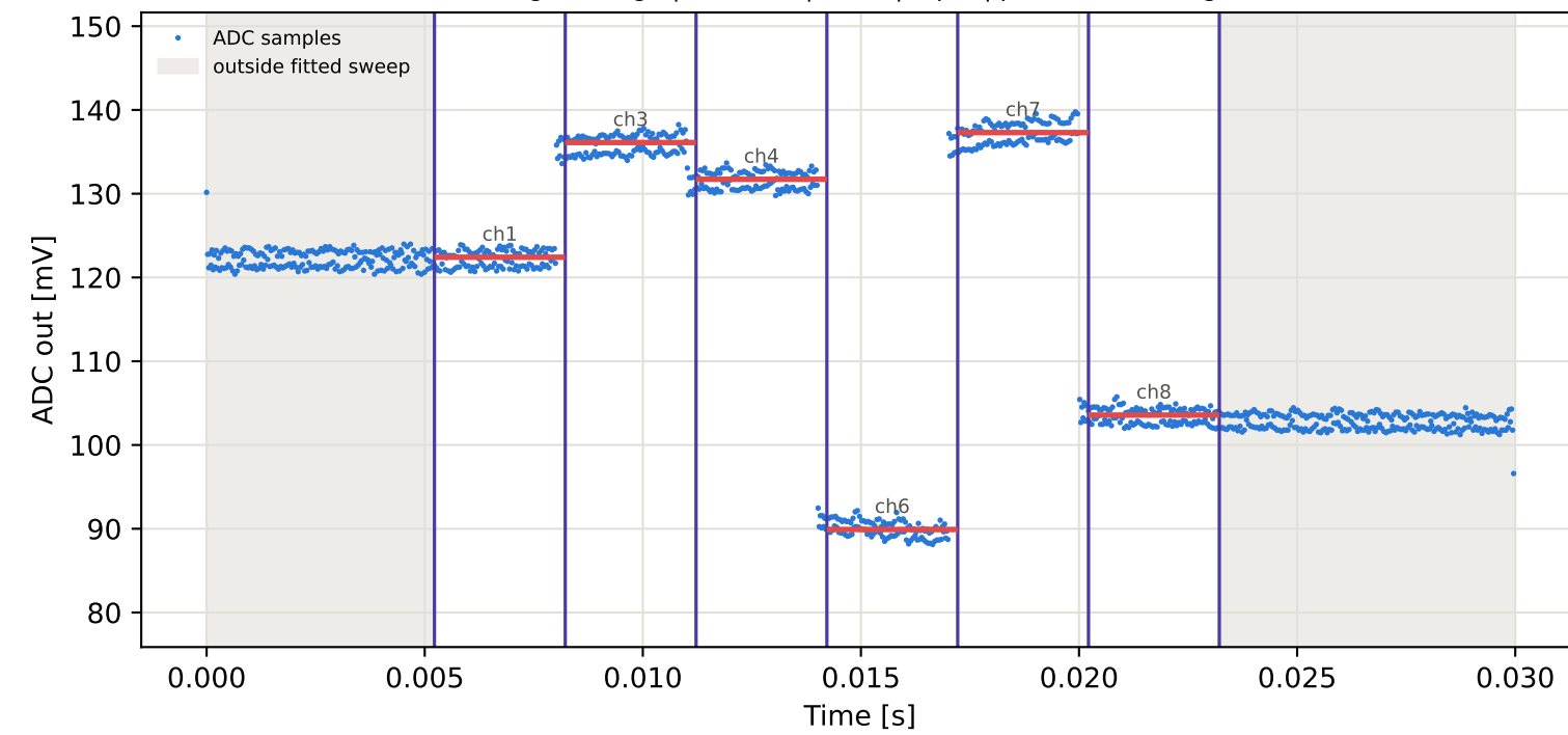
Tag6 &lt;- Tag9 | 975 MHz | run 0 | rep 1 | phase -32.33 deg
