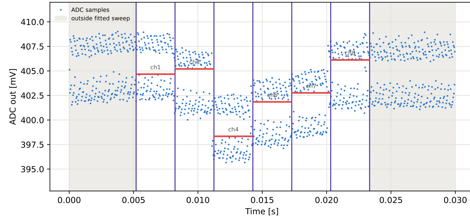
Tag1 &lt;- Tag3 | 955 MHz | run 0 | rep 1 | phase -106.26 deg
