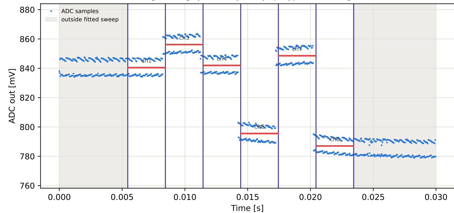
Tag15 &lt;- Tag6 | 875 MHz | run 0 | rep 1 | phase -82.53 deg
