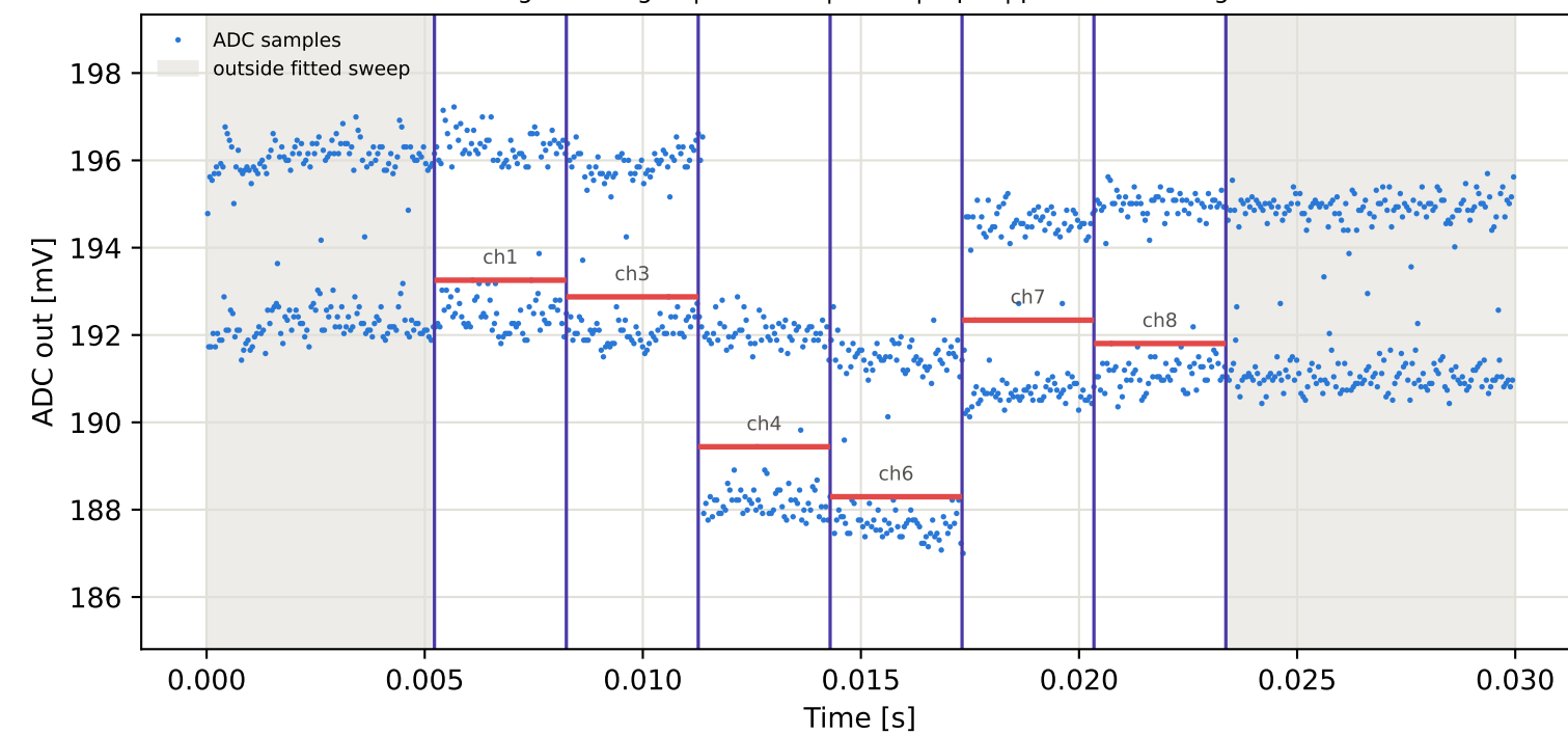
Tag10 &lt;- Tag2 | 985 MHz | run 0 | rep 1 | phase -128.71 deg
