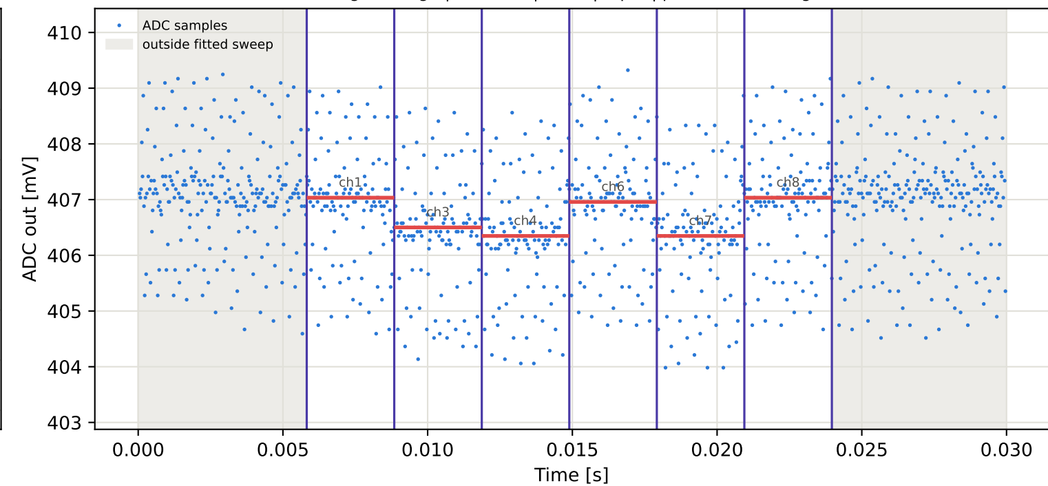
Tag3 &lt;- Tag9 | 845 MHz | run 0 | rep 1 | phase -95.87 deg
