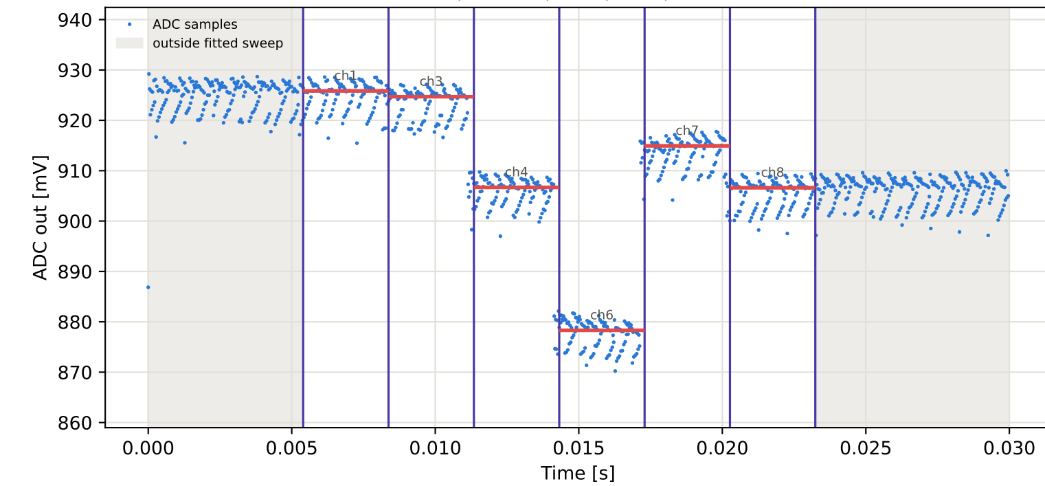
Tag4 &lt;- Tag9 | 925 MHz | run 0 | rep 1 | phase 25.50 deg
