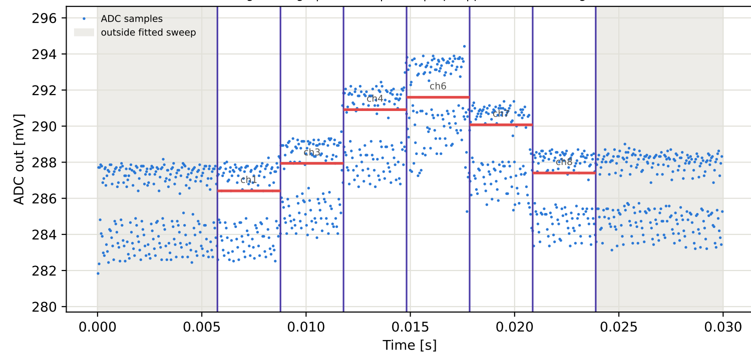
Tag3 &lt;- Tag2 | 915 MHz | run 0 | rep 1 | phase -126.17 deg
