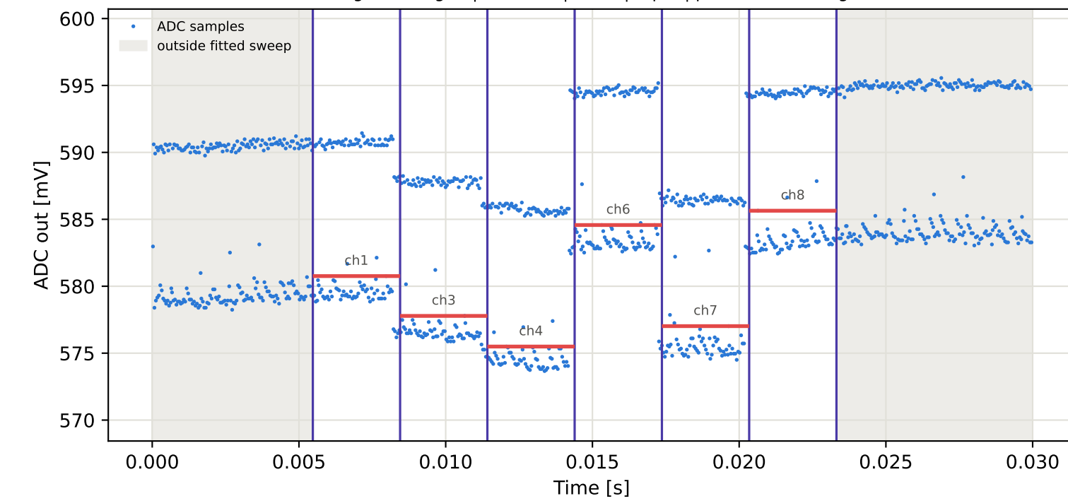
Tag16 &lt;- Tag10 | 925 MHz | run 0 | rep 1 | phase 137.98 deg
