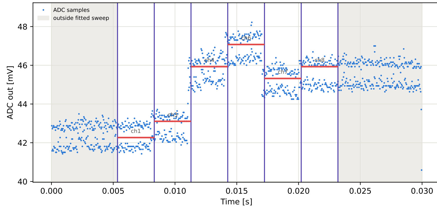
Tag15 &lt;- Tag1 | 855 MHz | run 0 | rep 1 | phase -116.51 deg
