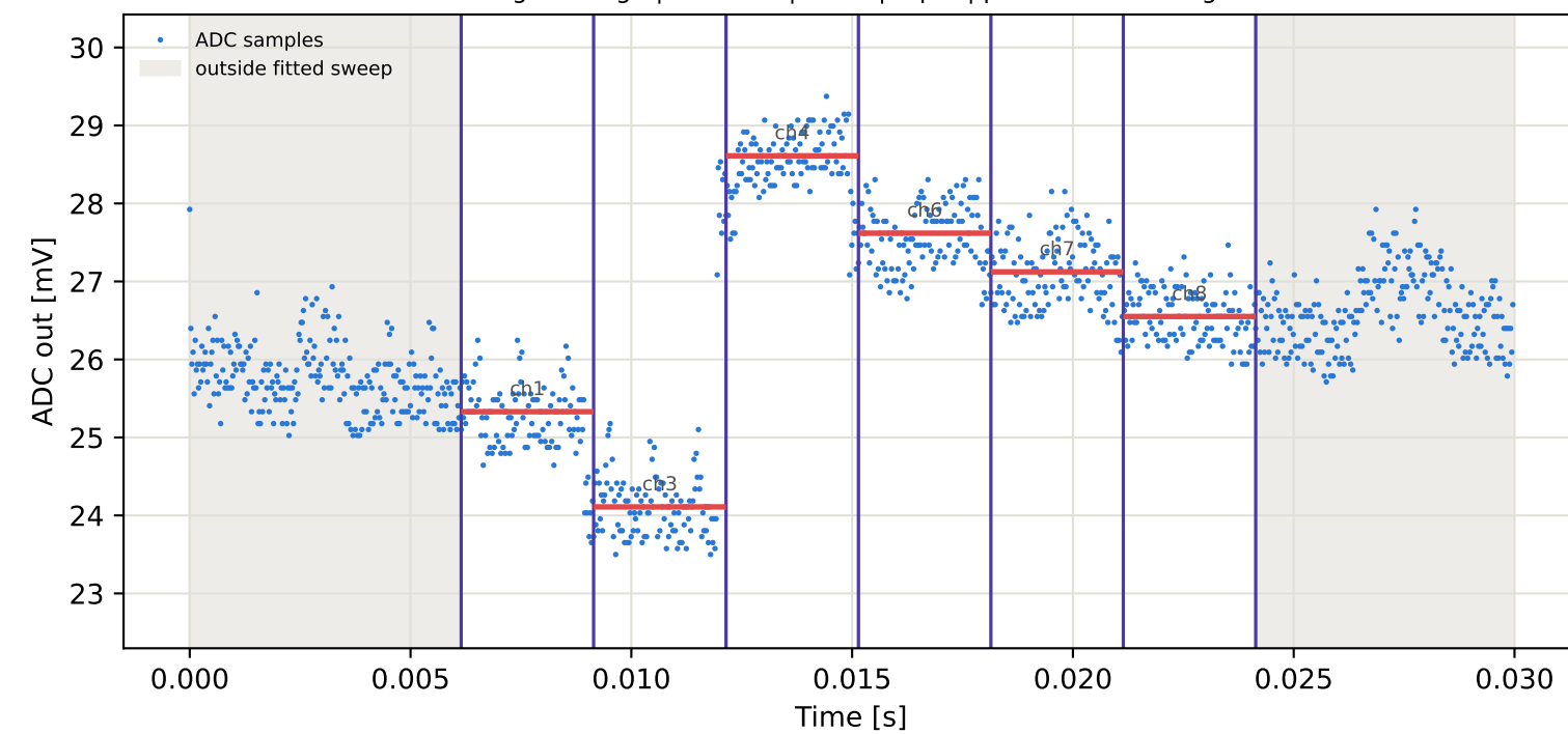
Tag9 &lt;- Tag5 | 775 MHz | run 0 | rep 1 | phase 63.91 deg
