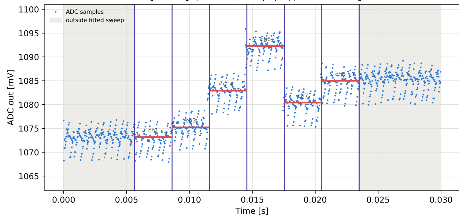
Tag16 &lt;- Tag5 | 875 MHz | run 0 | rep 1 | phase 12.13 deg
