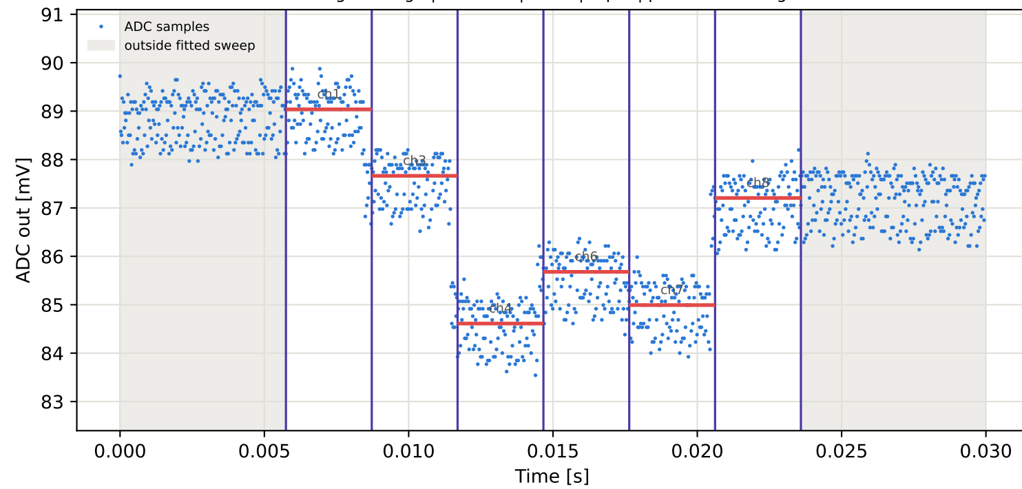
Tag1 &lt;- Tag7 | 845 MHz | run 0 | rep 1 | phase 111.83 deg
