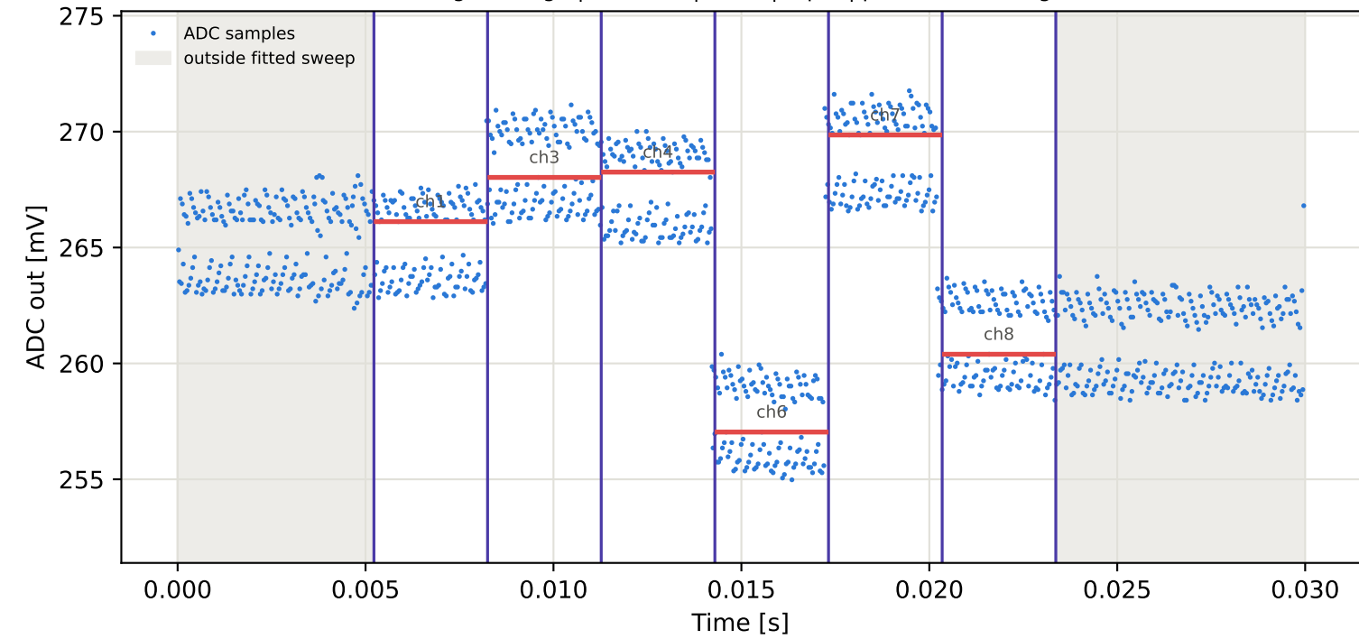
Tag10 &lt;- Tag1 | 985 MHz | run 0 | rep 1 | phase -156.89 deg
