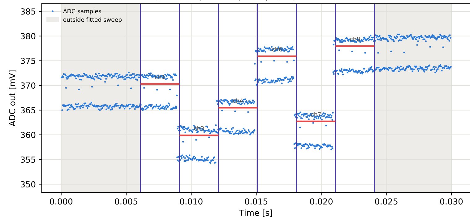
Tag4 &lt;- Tag8 | 835 MHz | run 0 | rep 1 | phase -109.86 deg
