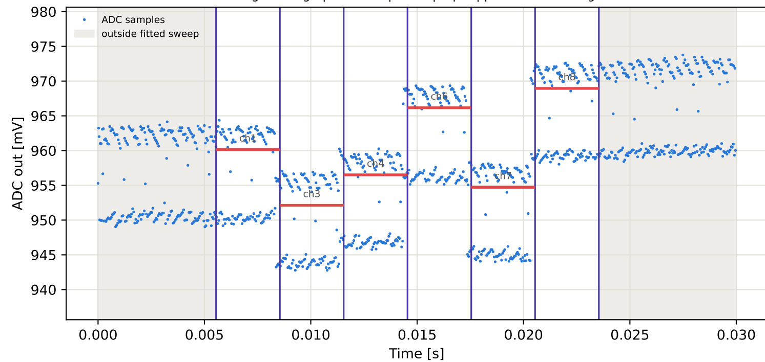
Tag4 &lt;- Tag15 | 875 MHz | run 0 | rep 1 | phase -73.07 deg
