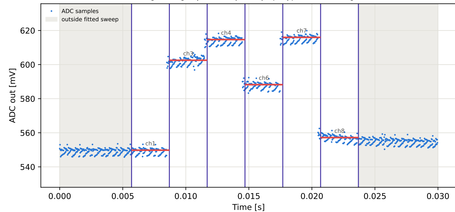
Tag4 &lt;- Tag2 | 865 MHz | run 0 | rep 1 | phase -45.51 deg
