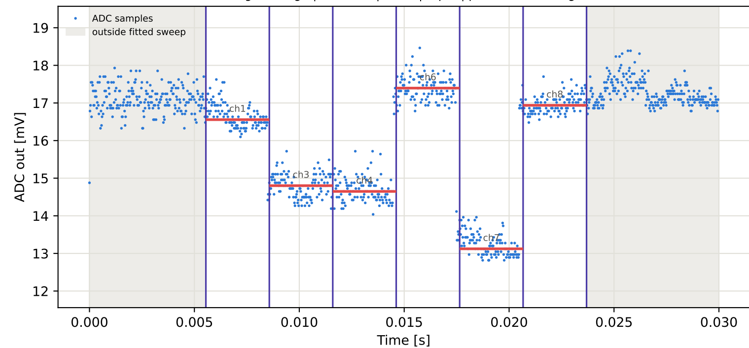
Tag9 &lt;- Tag8 | 785 MHz | run 0 | rep 1 | phase 152.84 deg
