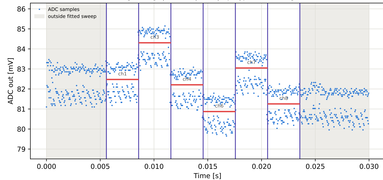
Tag9 &lt;- Tag10 | 785 MHz | run 0 | rep 1 | phase 163.88 deg
