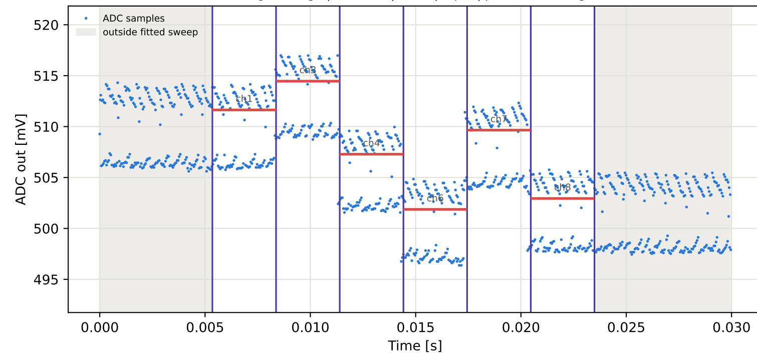
Tag9 &lt;- Tag5 | 845 MHz | run 0 | rep 1 | phase -168.48 deg
