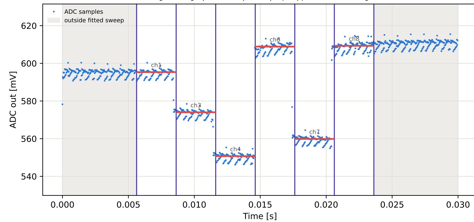
Tag9 &lt;- Tag7 | 965 MHz | run 0 | rep 1 | phase 117.85 deg
