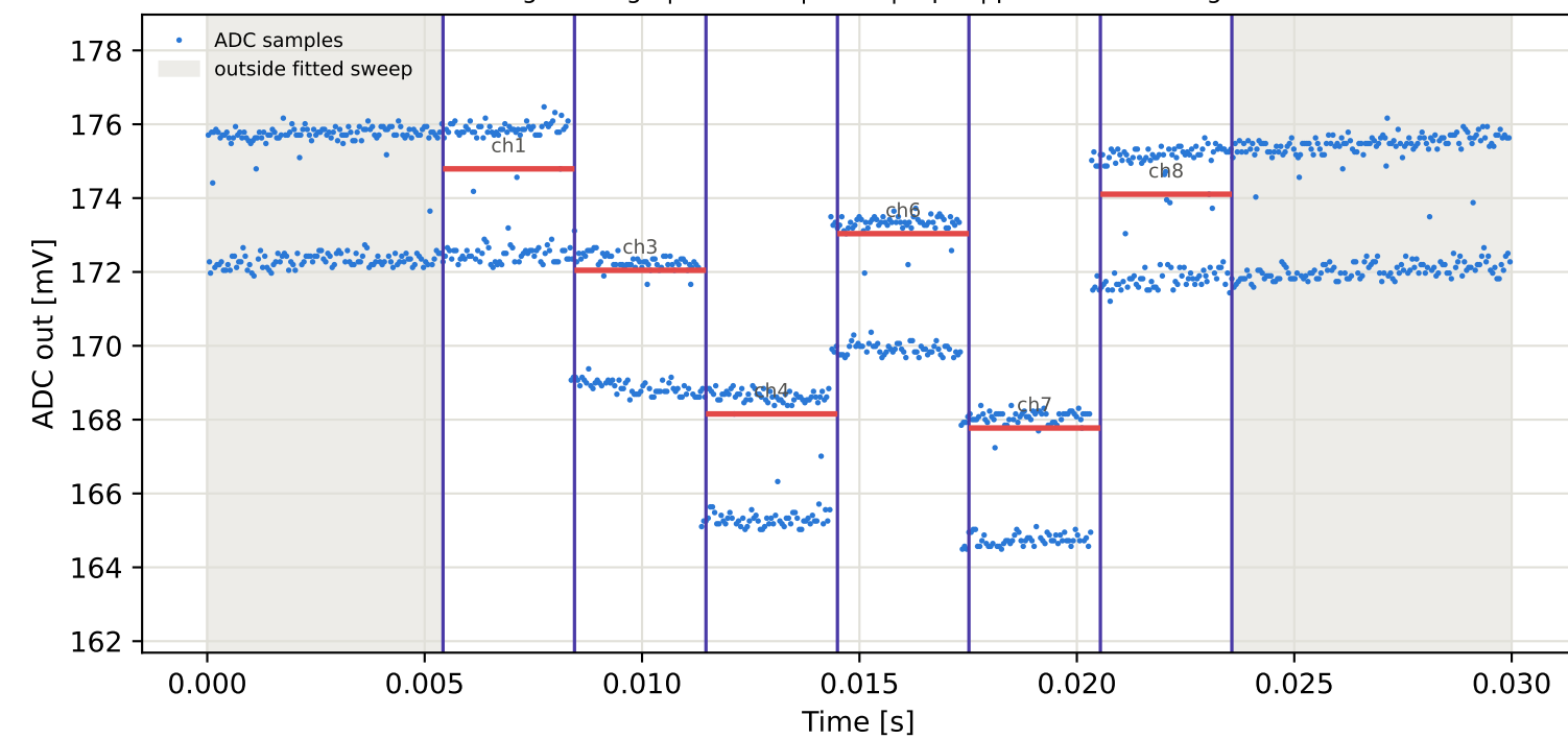
Tag5 &lt;- Tag8 | 785 MHz | run 0 | rep 1 | phase 28.67 deg
