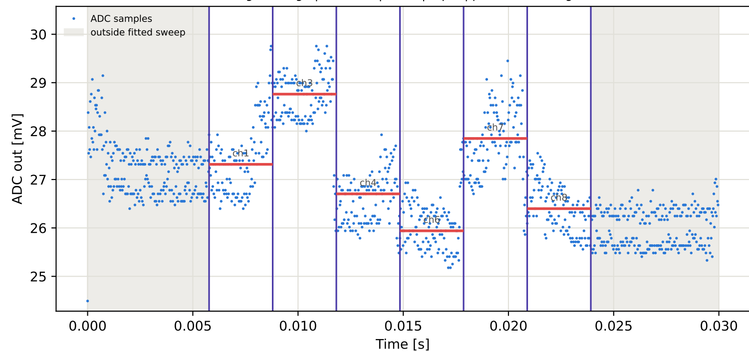
Tag2 &lt;- Tag8 | 805 MHz | run 0 | rep 1 | phase 27.31 deg
