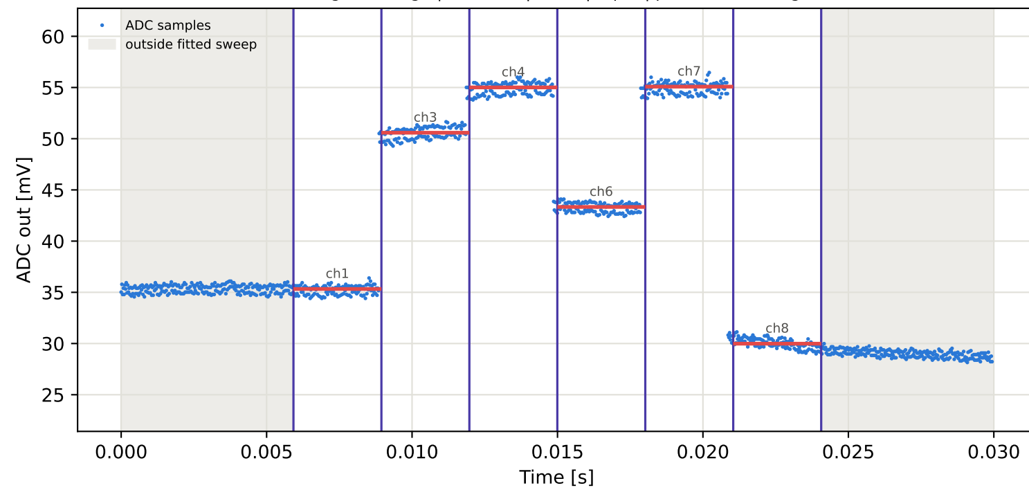
Tag10 &lt;- Tag8 | 855 MHz | run 0 | rep 1 | phase -135.49 deg
