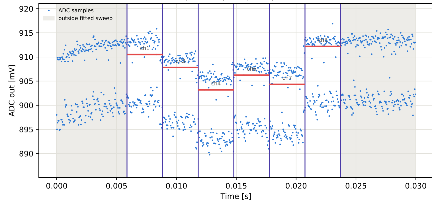
Tag6 &lt;- Tag9 | 885 MHz | run 0 | rep 1 | phase -145.30 deg
