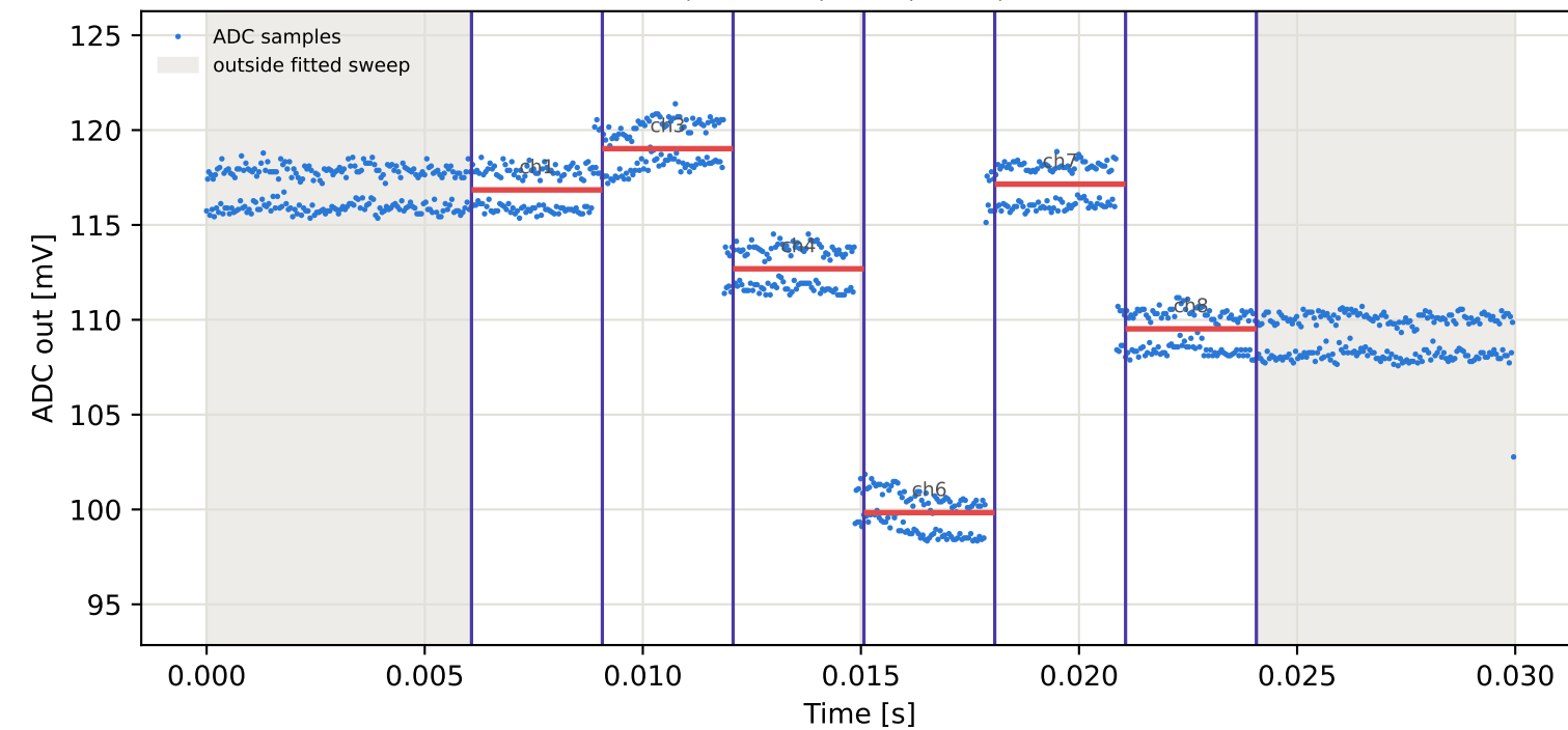
Tag2 &lt;- Tag15 | 975 MHz | run 0 | rep 1 | phase 12.23 deg
