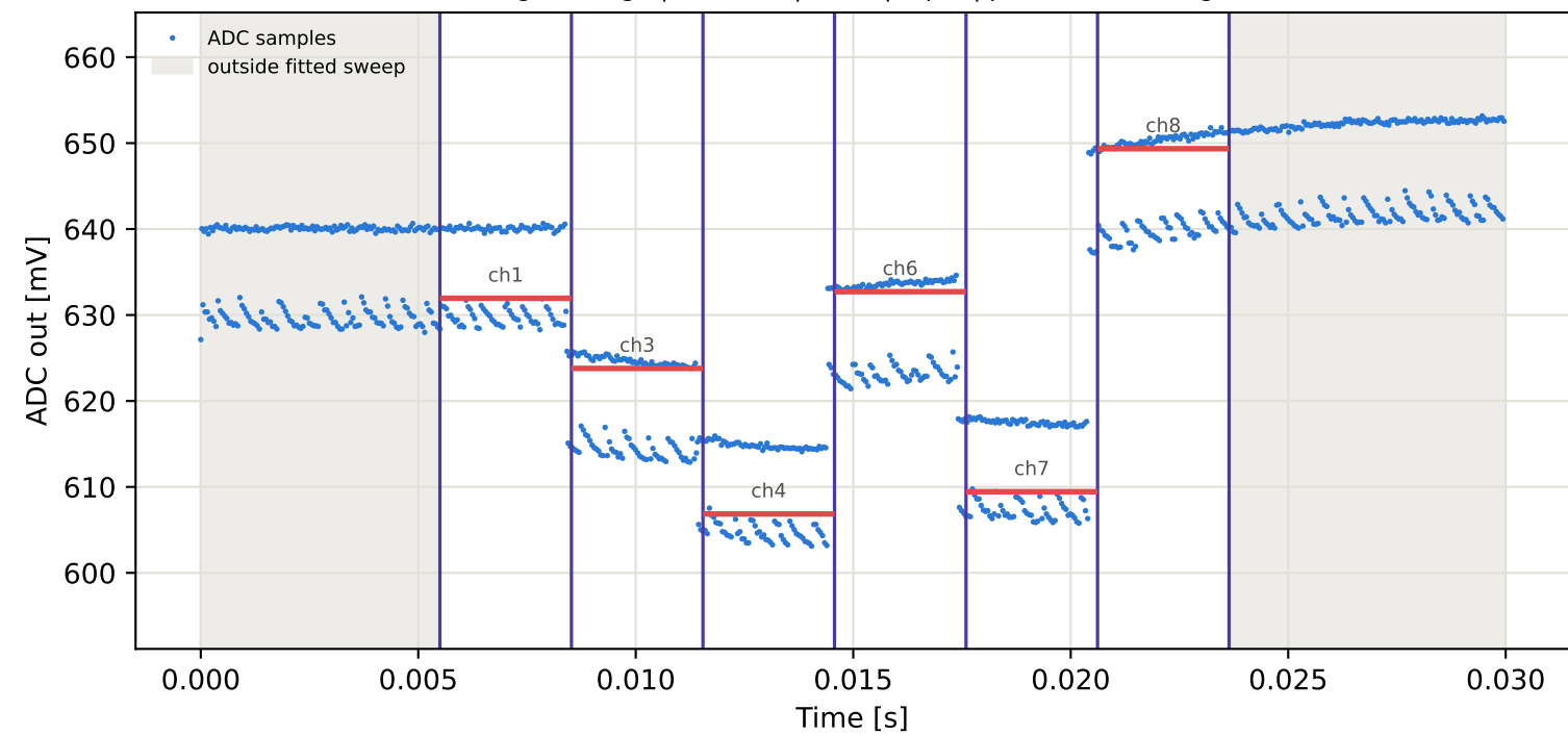
Tag8 &lt;- Tag10 | 905 MHz | run 0 | rep 1 | phase 93.17 deg
