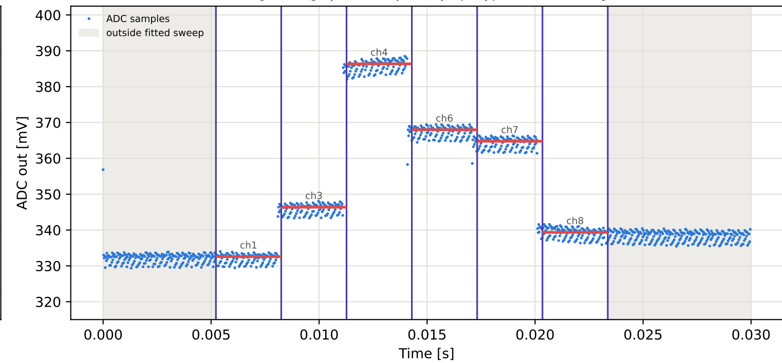
Tag3 &lt;- Tag15 | 975 MHz | run 0 | rep 1 | phase 67.66 deg
