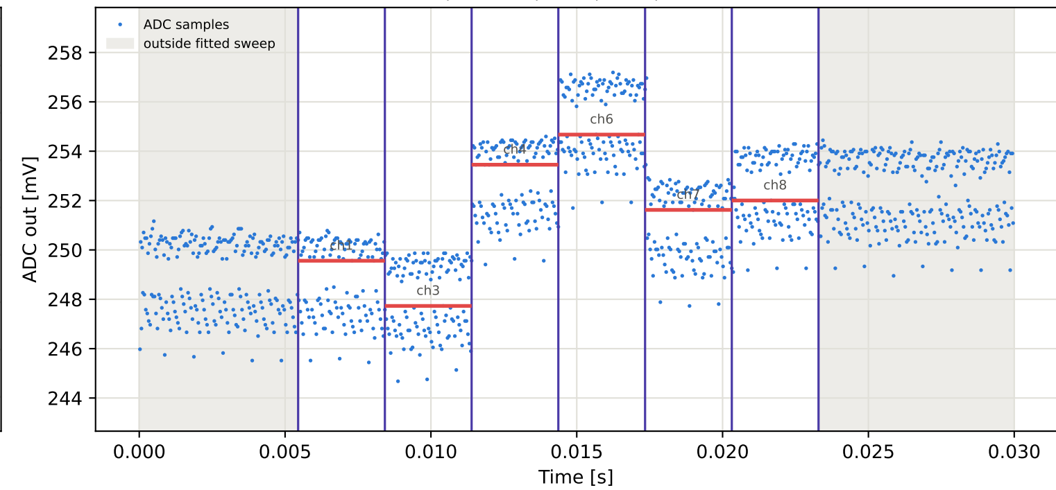
Tag3 &lt;- Tag9 | 825 MHz | run 0 | rep 1 | phase -134.42 deg
