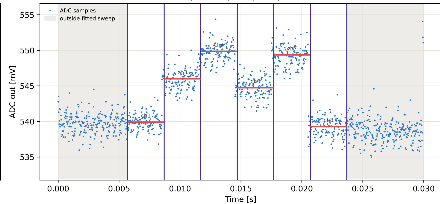
Tag10 &lt;- Tag9 | 885 MHz | run 0 | rep 1 | phase -102.52 deg
