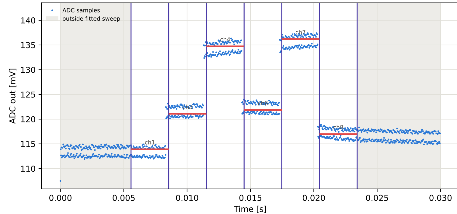
Tag3 &lt;- Tag8 | 785 MHz | run 0 | rep 1 | phase 72.24 deg
