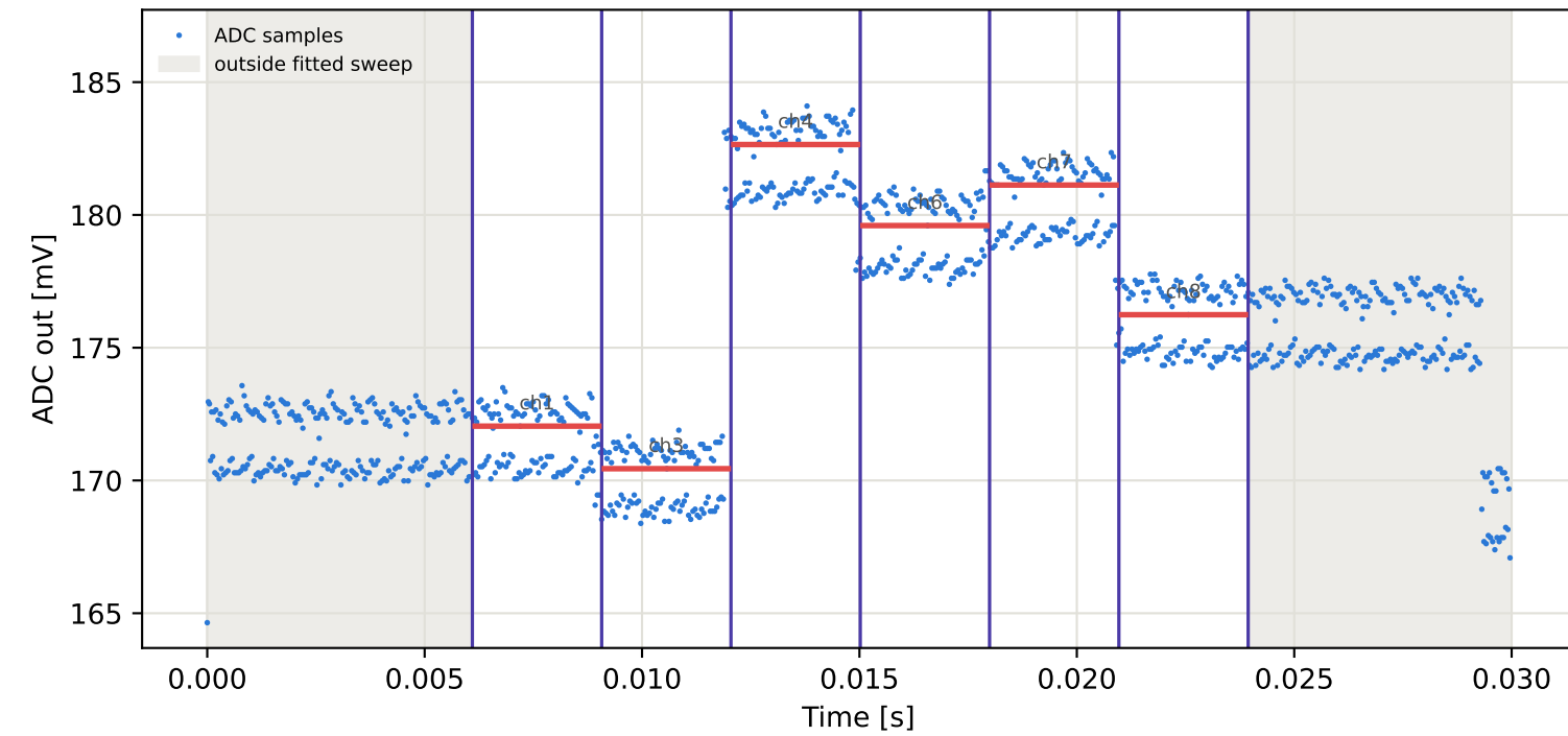
Tag16 &lt;- Tag6 | 805 MHz | run 0 | rep 1 | phase -97.62 deg
