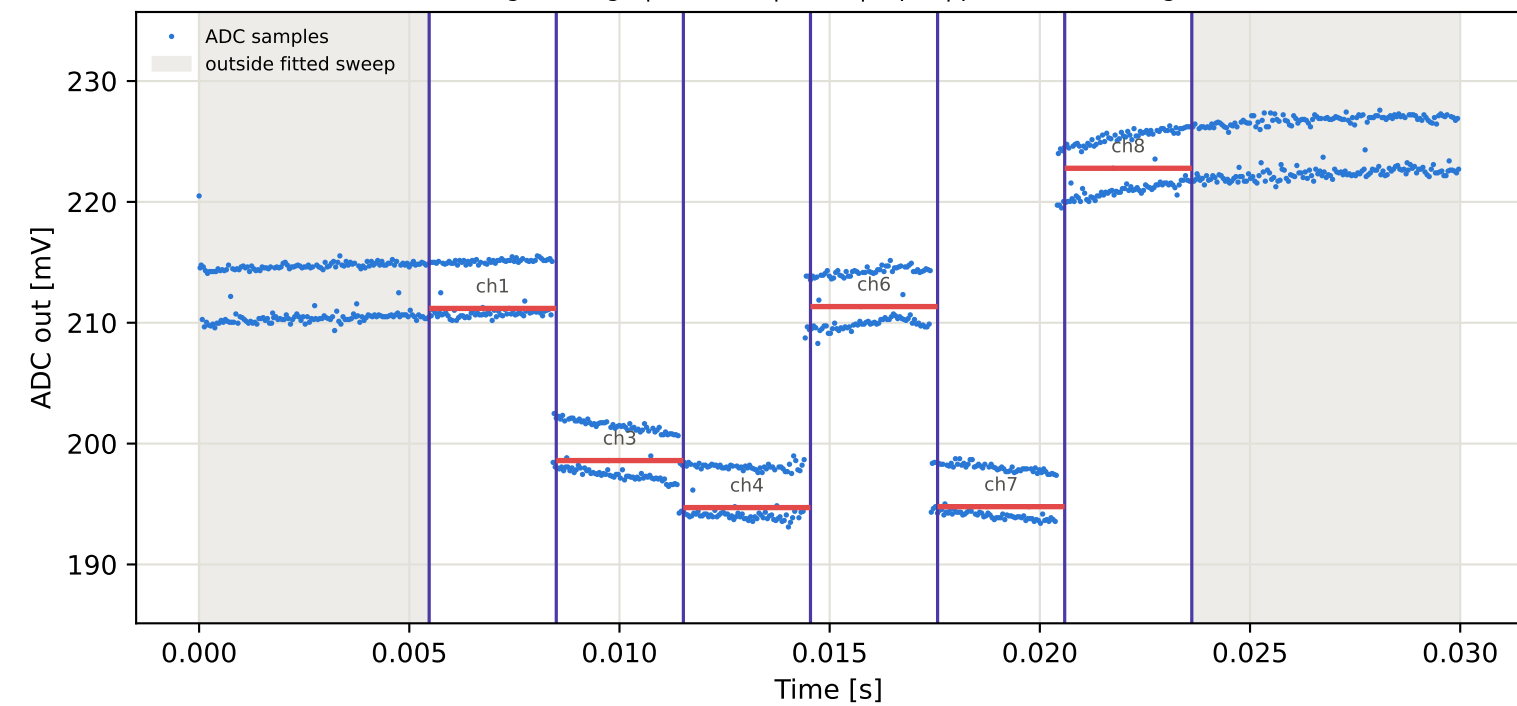
Tag2 &lt;- Tag5 | 875 MHz | run 0 | rep 1 | phase -15.66 deg
