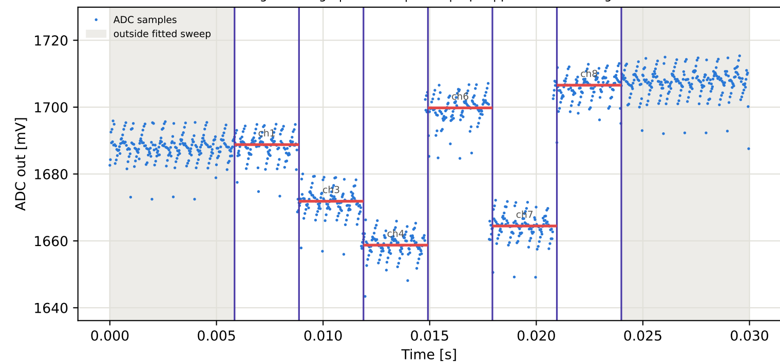
Tag16 &lt;- Tag1 | 925 MHz | run 0 | rep 1 | phase -154.62 deg
