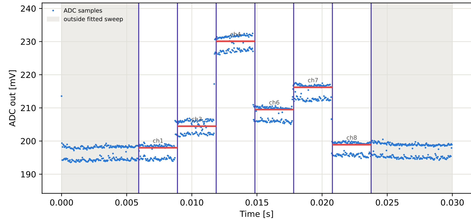
Tag6 &lt;- Tag5 | 985 MHz | run 0 | rep 1 | phase 172.43 deg
