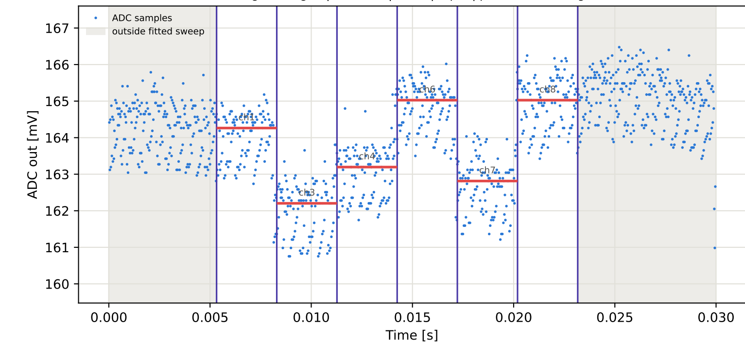
Tag9 &lt;- Tag16 | 805 MHz | run 0 | rep 1 | phase 167.76 deg
