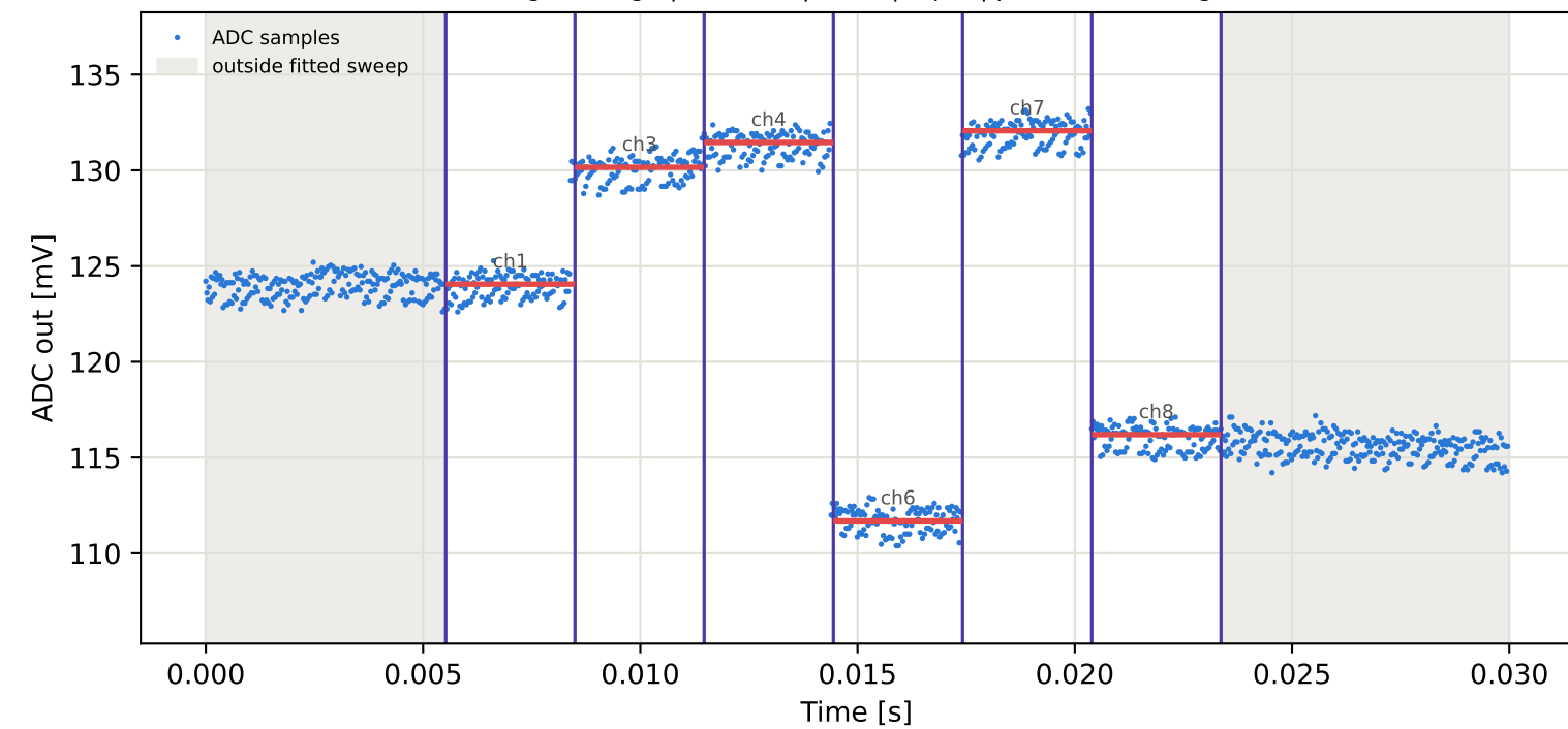
Tag3 &lt;- Tag10 | 965 MHz | run 0 | rep 1 | phase 83.26 deg
