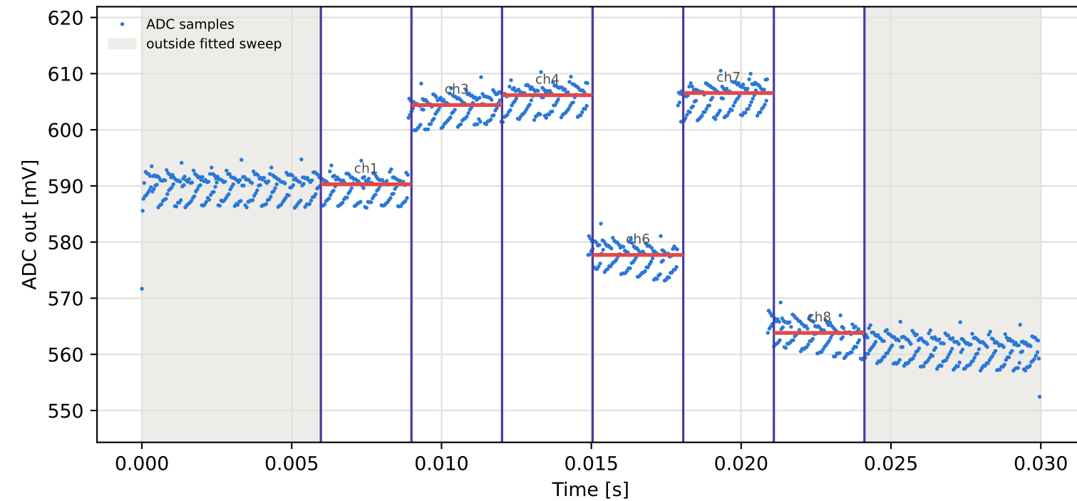
Tag15 &lt;- Tag1 | 895 MHz | run 0 | rep 1 | phase -80.50 deg
