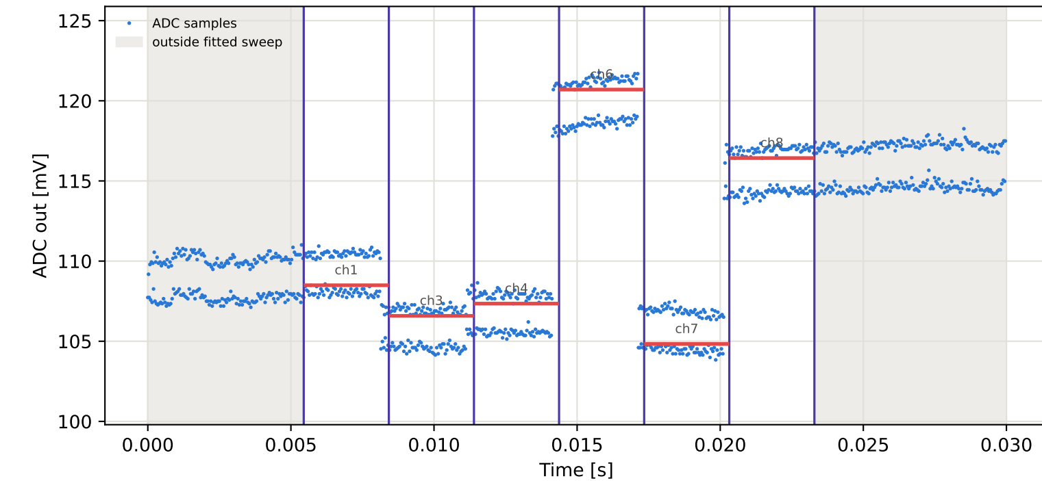
Tag2 &lt;- Tag15 | 935 MHz | run 0 | rep 1 | phase -6.95 deg
