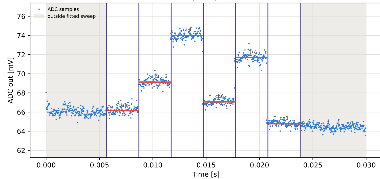
Tag2 &lt;- Tag5 | 955 MHz | run 0 | rep 1 | phase -54.66 deg
