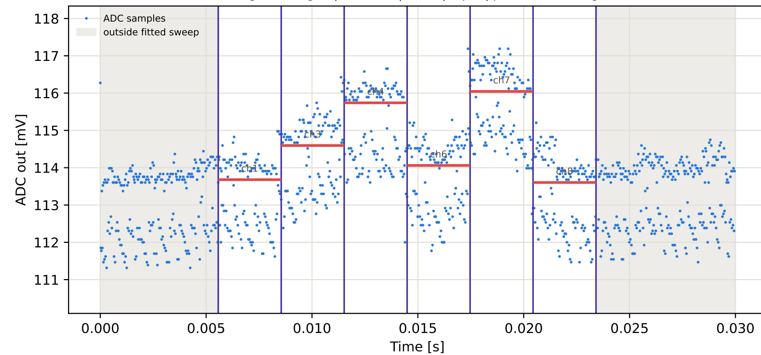
Tag15 &lt;- Tag3 | 775 MHz | run 0 | rep 1 | phase 73.61 deg
