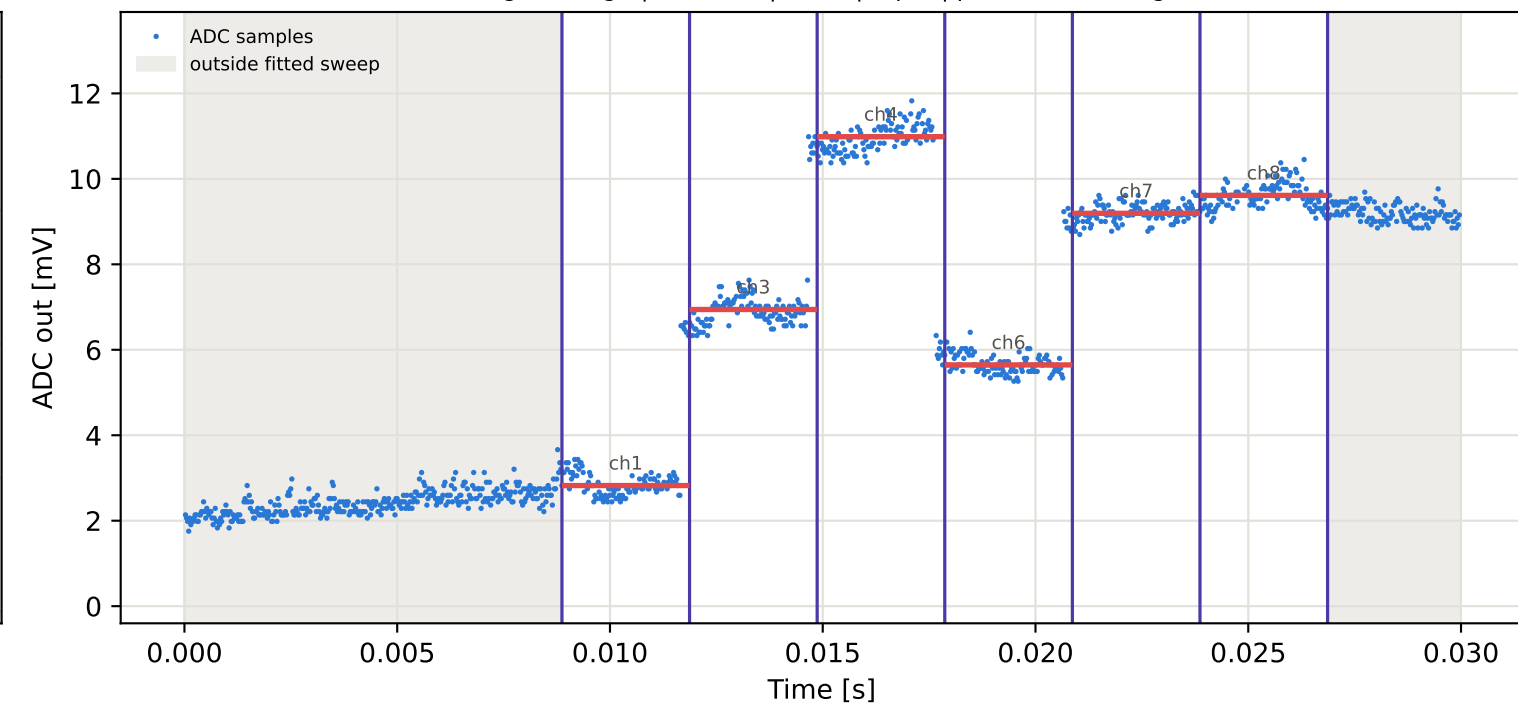
Tag2 &lt;- Tag6 | 865 MHz | run 0 | rep 1 | phase -141.47 deg
