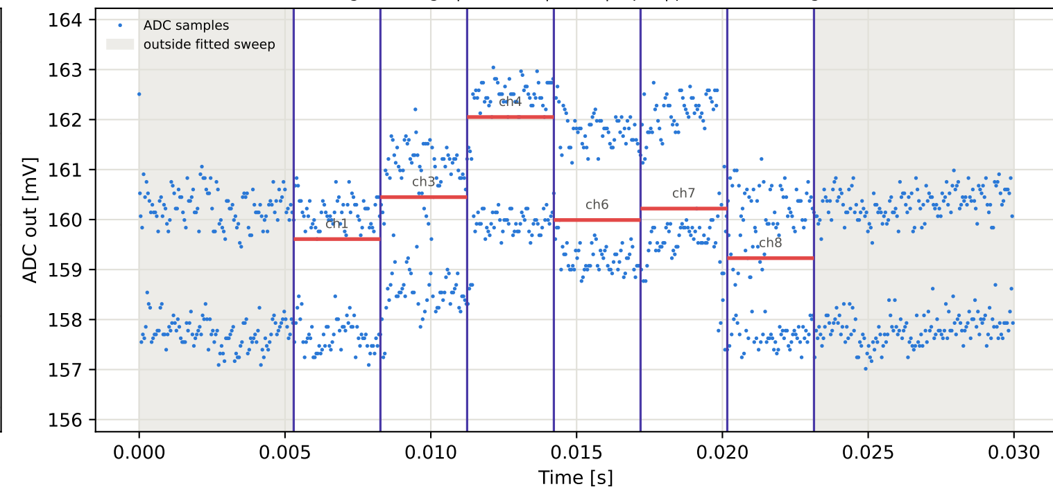
Tag15 &lt;- Tag4 | 785 MHz | run 0 | rep 1 | phase 131.28 deg
