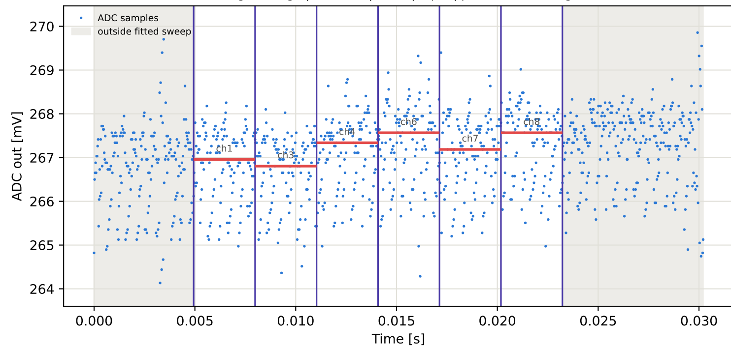
Tag7 &lt;- Tag4 | 825 MHz | run 0 | rep 1 | phase 79.08 deg
