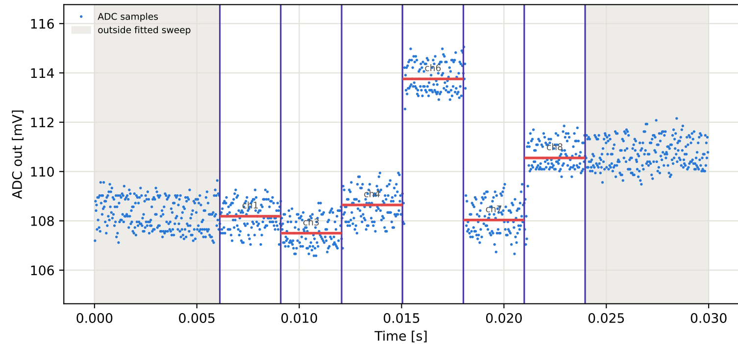
Tag2 &lt;- Tag16 | 935 MHz | run 0 | rep 1 | phase -105.82 deg
