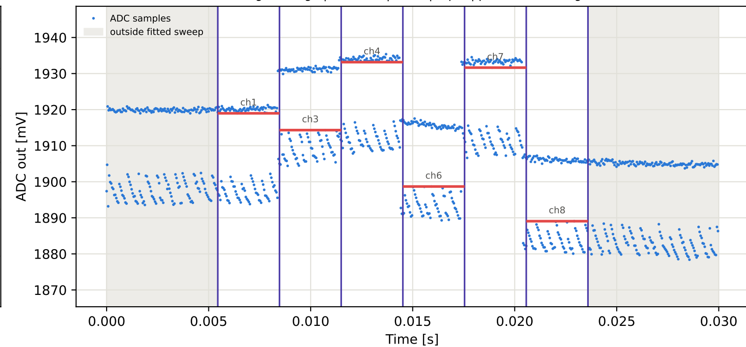
Tag5 &lt;- Tag1 | 895 MHz | run 0 | rep 1 | phase -46.95 deg
