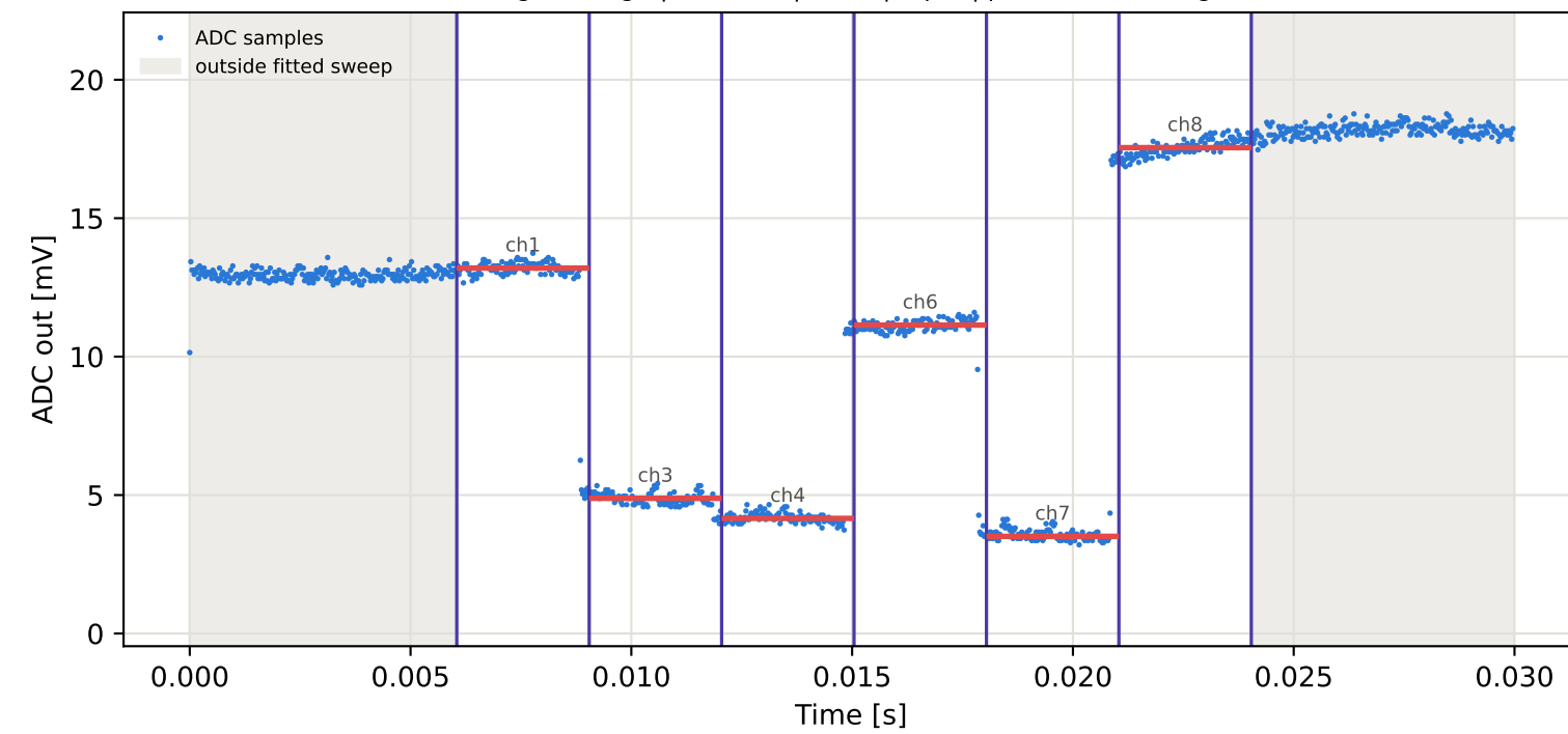
Tag2 &lt;- Tag5 | 865 MHz | run 0 | rep 1 | phase -10.79 deg
