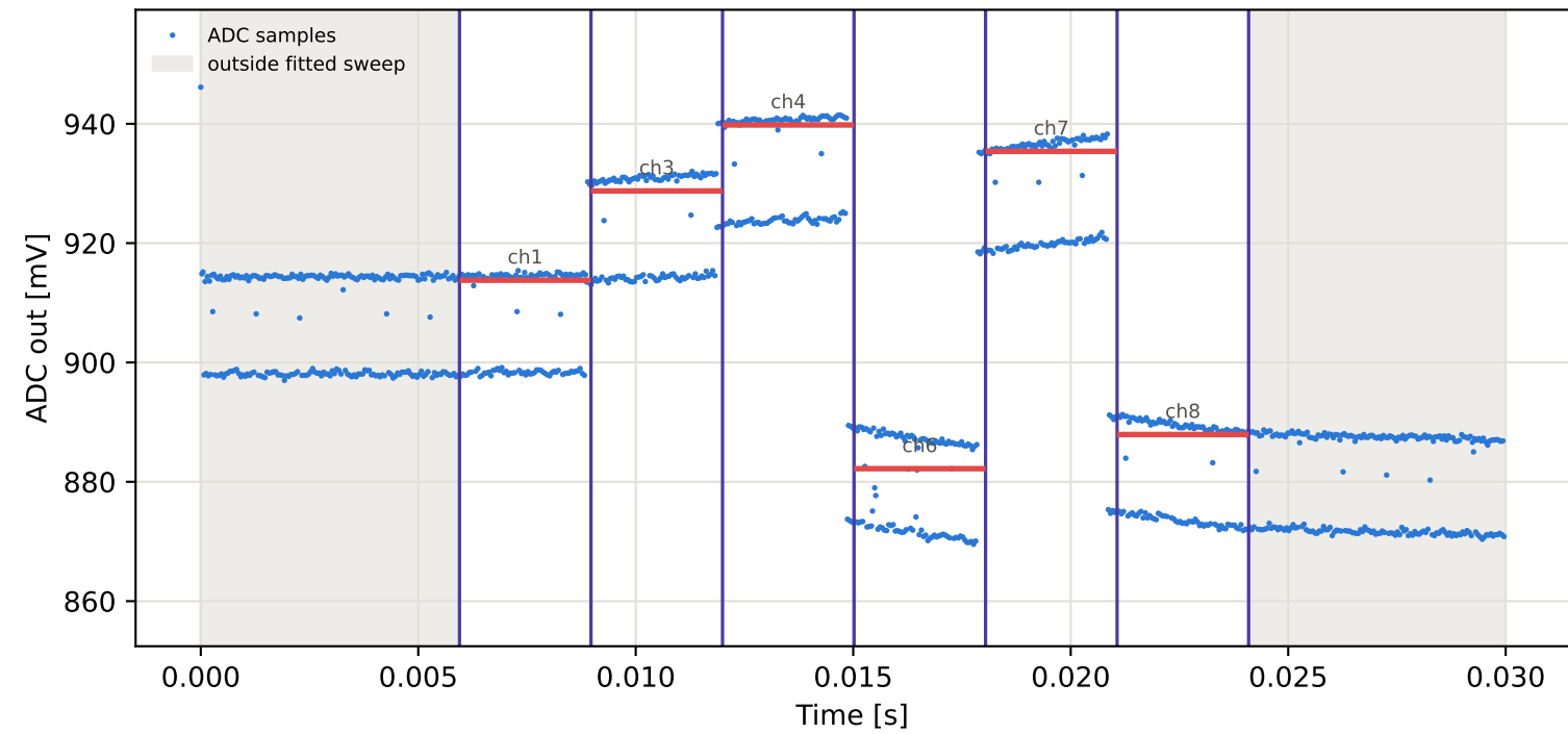
Tag5 &lt;- Tag1 | 925 MHz | run 0 | rep 1 | phase 70.32 deg
