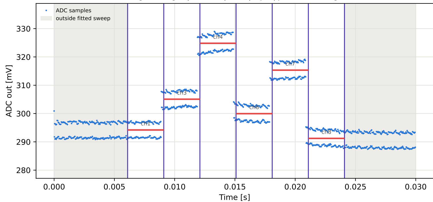
Tag10 &lt;- Tag3 | 965 MHz | run 0 | rep 1 | phase 126.91 deg
