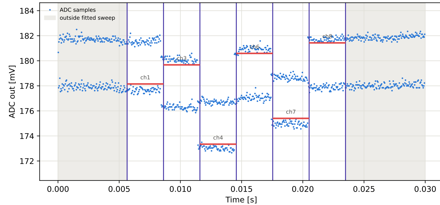
Tag1 &lt;- Tag3 | 995 MHz | run 0 | rep 1 | phase -62.32 deg
