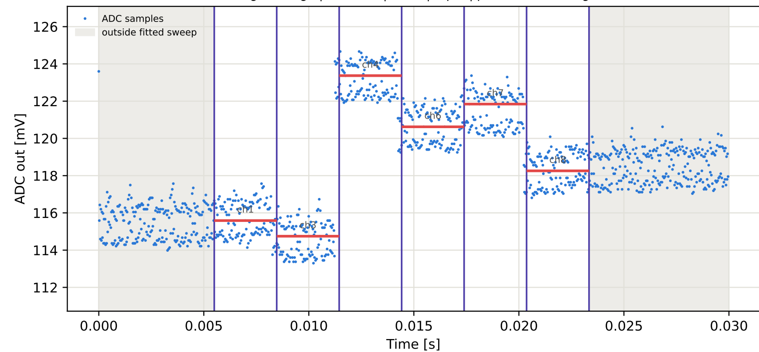
Tag7 &lt;- Tag6 | 775 MHz | run 0 | rep 1 | phase -105.82 deg
