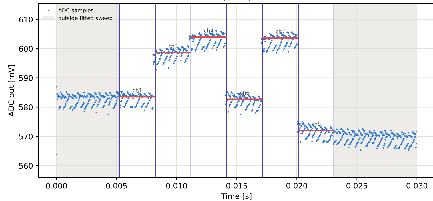
Tag10 &lt;- Tag9 | 895 MHz | run 0 | rep 1 | phase -88.33 deg
