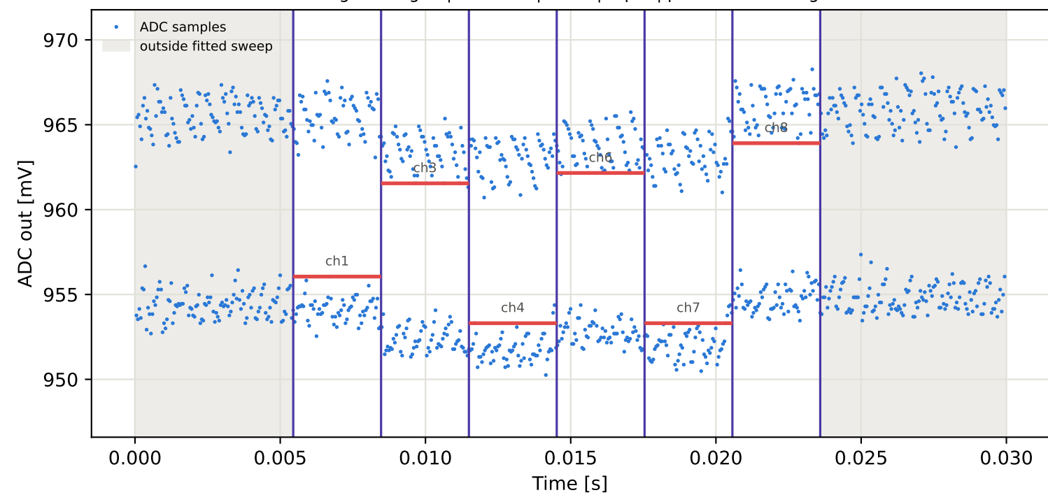
Tag4 &lt;- Tag16 | 875 MHz | run 0 | rep 1 | phase -153.21 deg
