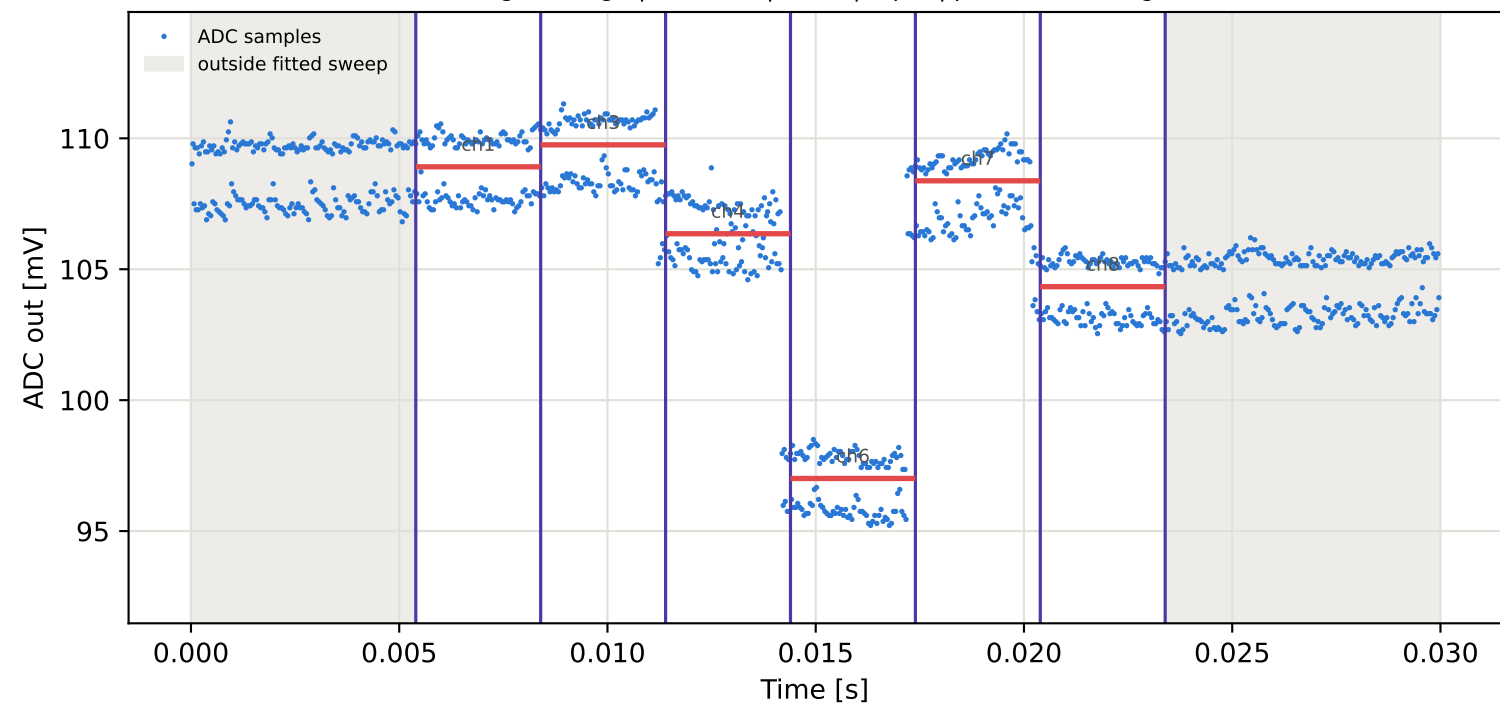
Tag2 &lt;- Tag5 | 935 MHz | run 0 | rep 1 | phase -1.61 deg
