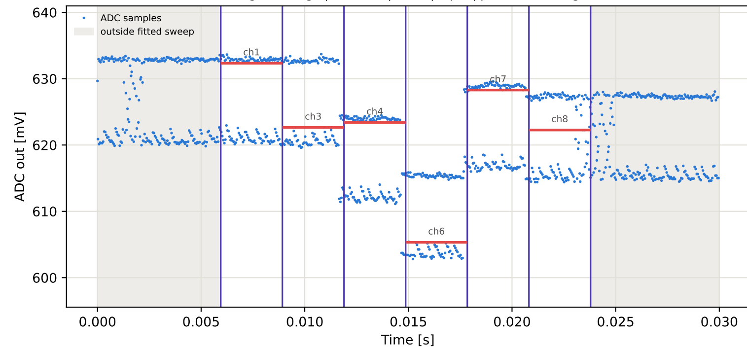
Tag16 &lt;- Tag5 | 955 MHz | run 0 | rep 1 | phase 179.43 deg
