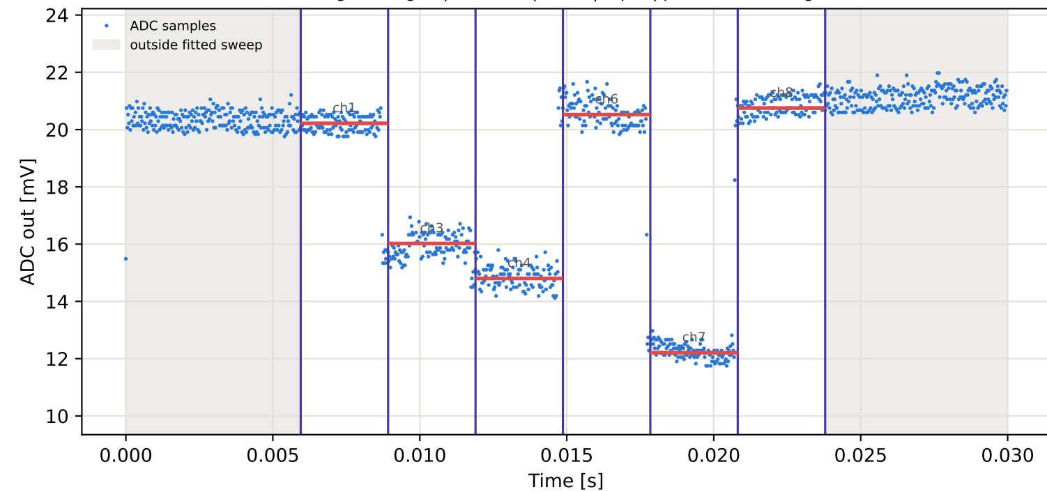
Tag9 &lt;- Tag2 | 785 MHz | run 0 | rep 1 | phase 142.42 deg
