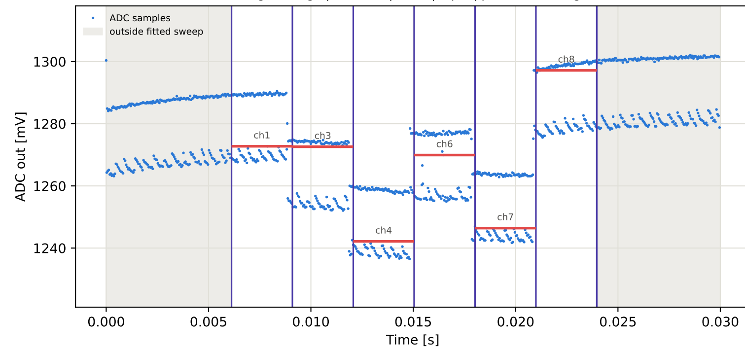
Tag5 &lt;- Tag8 | 905 MHz | run 0 | rep 1 | phase 155.88 deg
