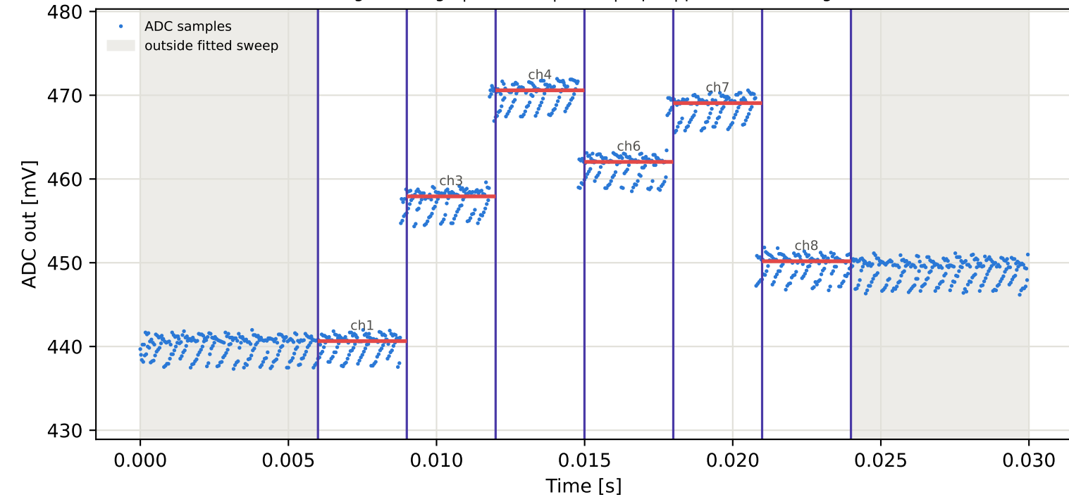
Tag15 &lt;- Tag5 | 855 MHz | run 0 | rep 1 | phase -98.78 deg
