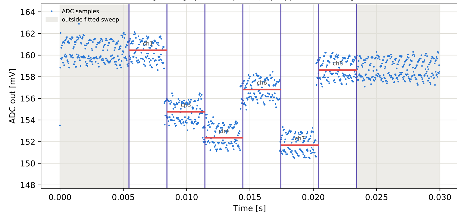
Tag6 &lt;- Tag1 | 845 MHz | run 0 | rep 1 | phase 105.92 deg
