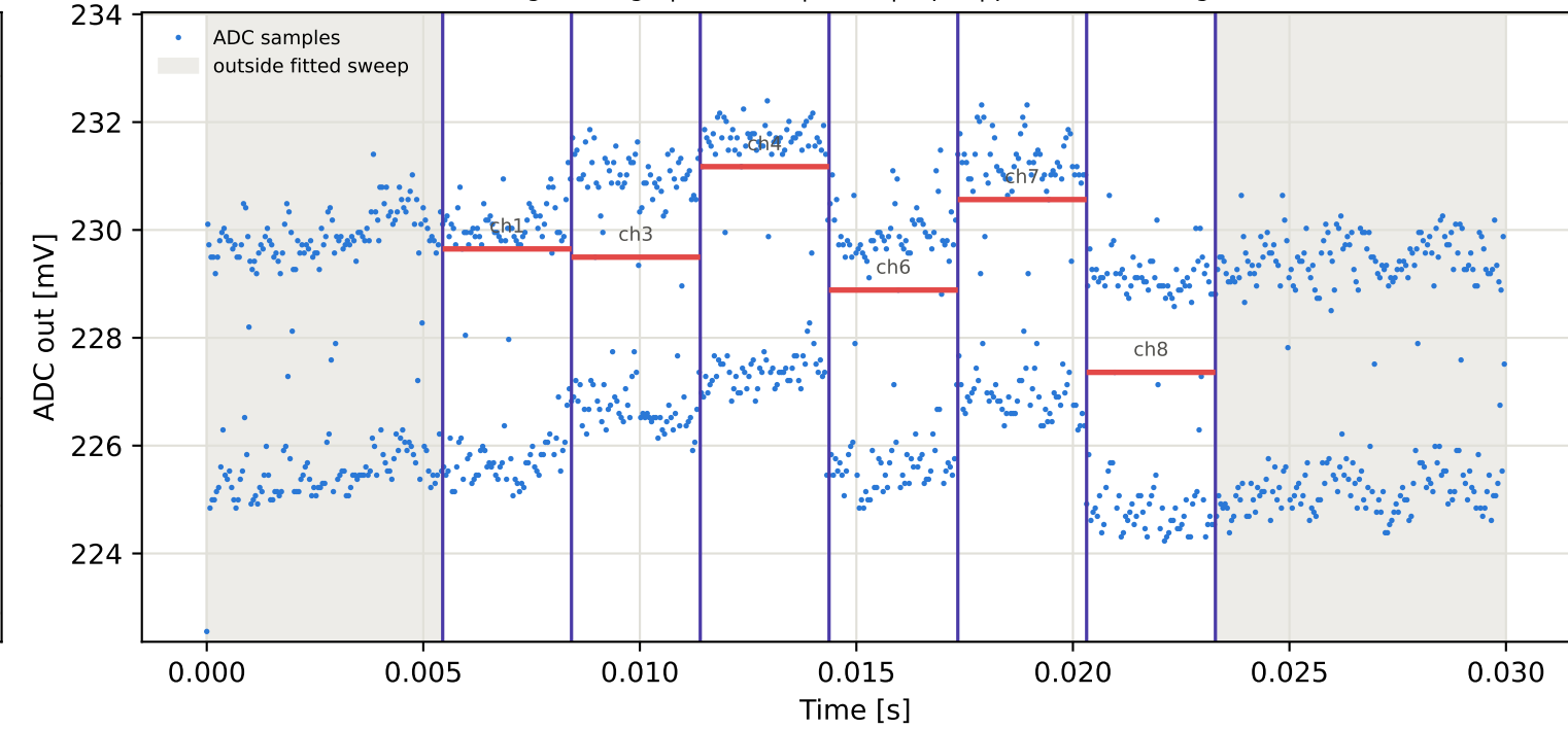
Tag7 &lt;- Tag4 | 995 MHz | run 0 | rep 1 | phase -14.29 deg
