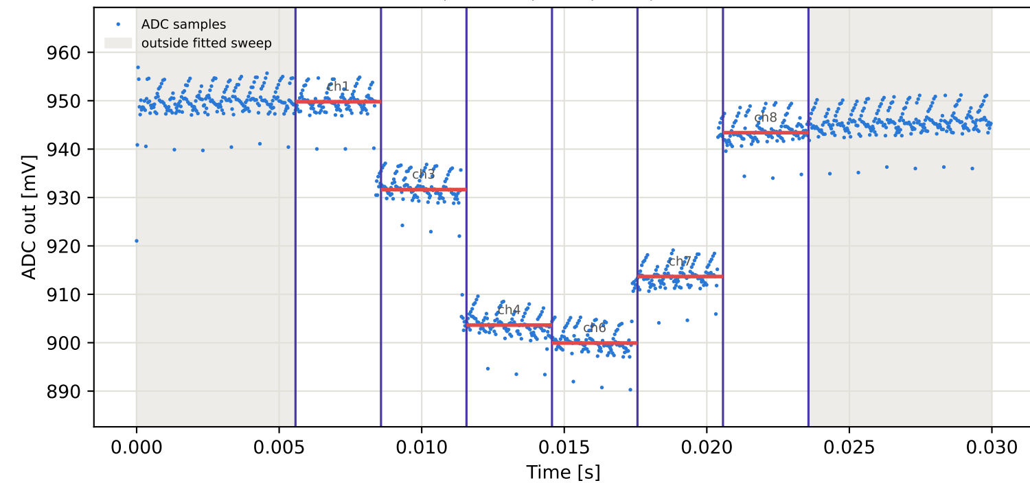
Tag4 &lt;- Tag3 | 915 MHz | run 0 | rep 1 | phase 57.06 deg
