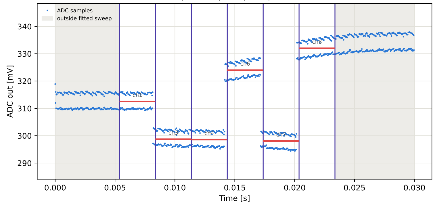
Tag8 &lt;- Tag10 | 895 MHz | run 0 | rep 1 | phase -7.99 deg
