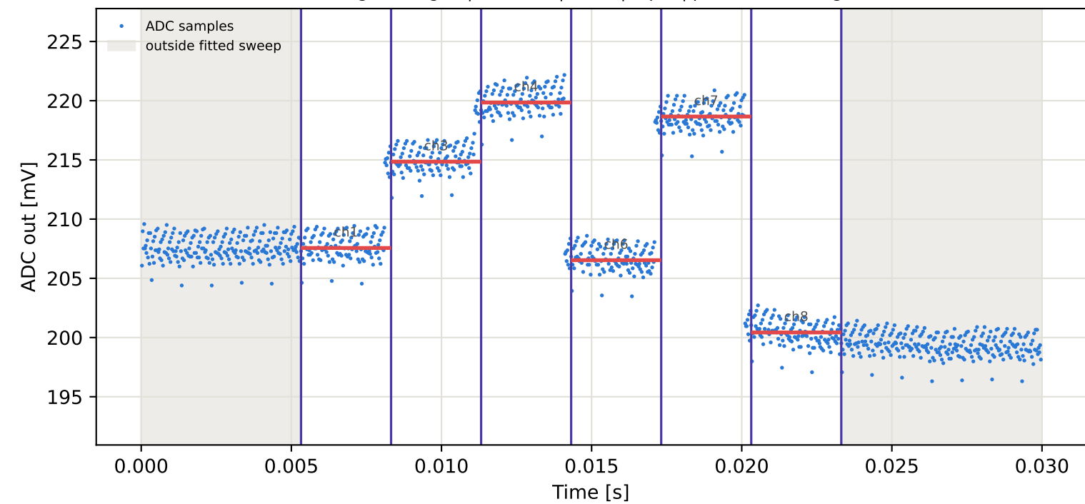
Tag1 &lt;- Tag2 | 915 MHz | run 0 | rep 1 | phase 103.66 deg
