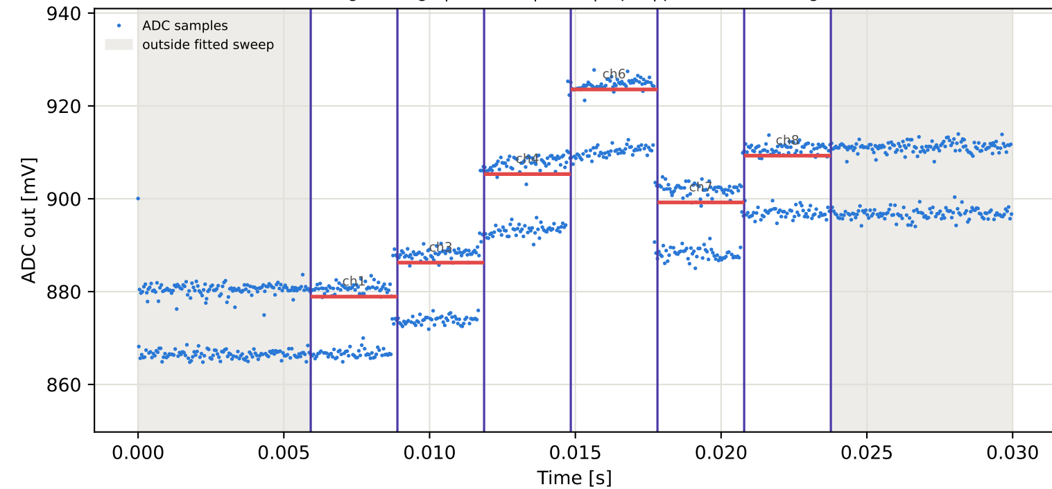
Tag7 &lt;- Tag10 | 885 MHz | run 0 | rep 1 | phase 171.81 deg
