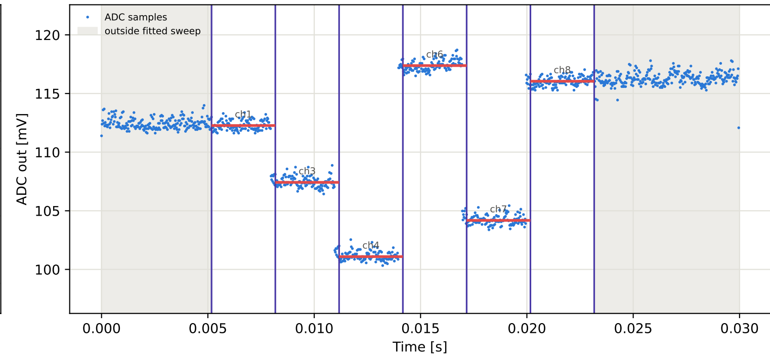
Tag10 &lt;- Tag5 | 995 MHz | run 0 | rep 1 | phase -119.99 deg
