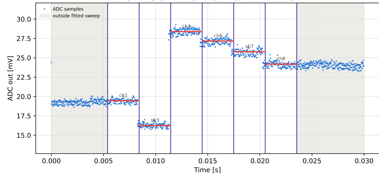
Tag2 &lt;- Tag5 | 805 MHz | run 0 | rep 1 | phase -8.32 deg
