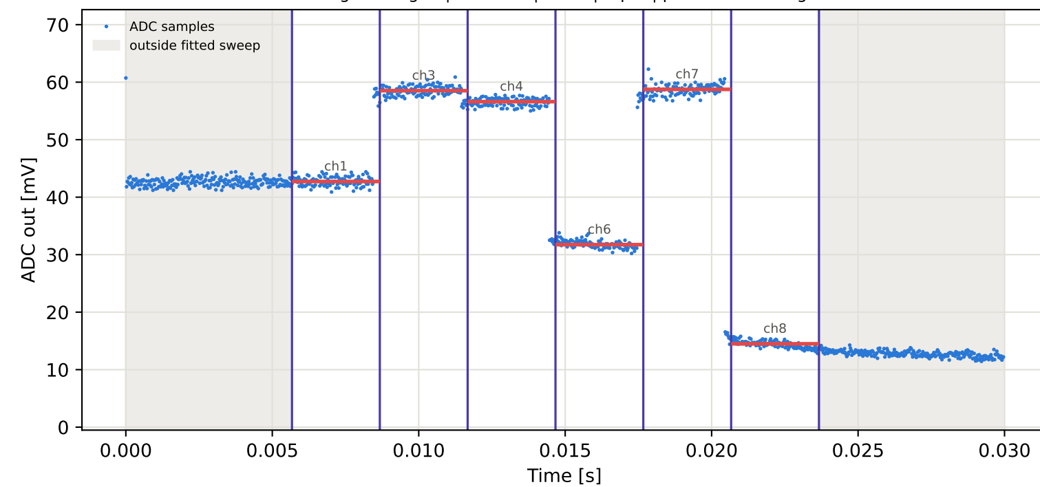
Tag7 &lt;- Tag3 | 885 MHz | run 0 | rep 1 | phase 82.78 deg
