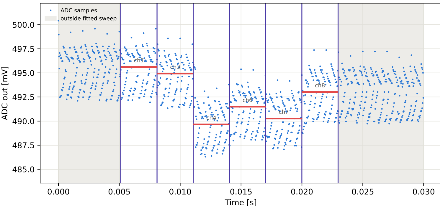
Tag16 &lt;- Tag15 | 835 MHz | run 0 | rep 1 | phase 72.45 deg
