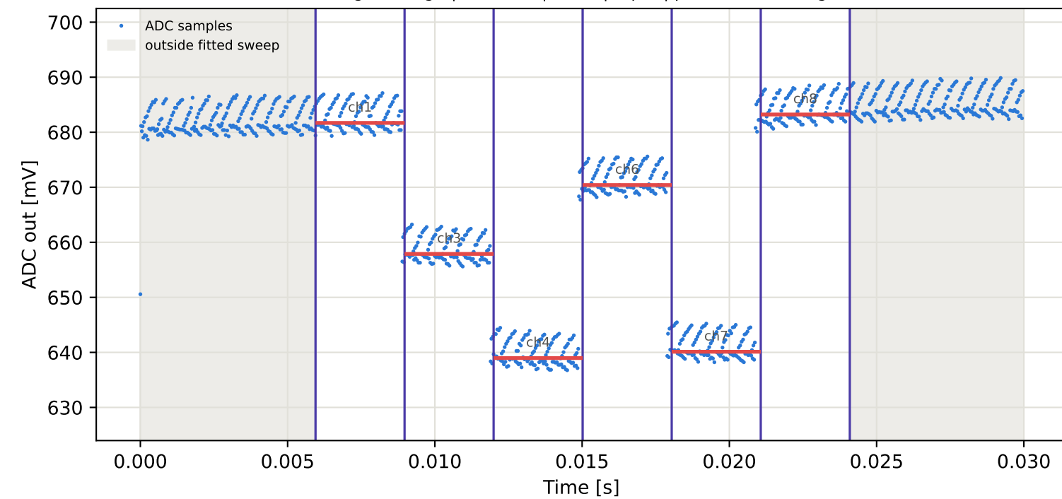
Tag9 &lt;- Tag10 | 845 MHz | run 0 | rep 1 | phase -72.28 deg
