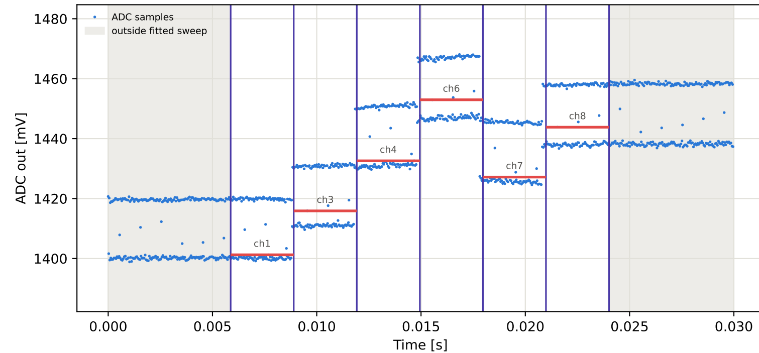
Tag5 &lt;- Tag3 | 875 MHz | run 0 | rep 1 | phase -154.81 deg
