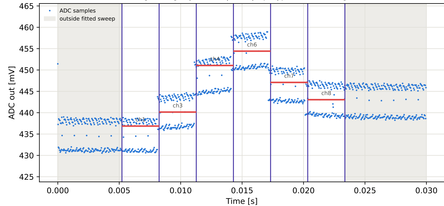
Tag1 &lt;- Tag2 | 895 MHz | run 0 | rep 1 | phase 92.43 deg
