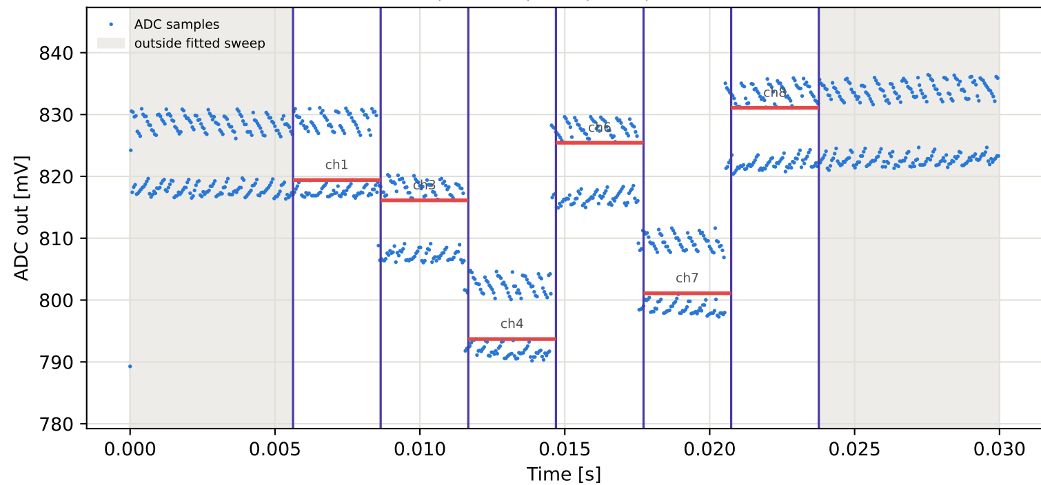
Tag8 &lt;- Tag7 | 955 MHz | run 0 | rep 1 | phase 102.50 deg
