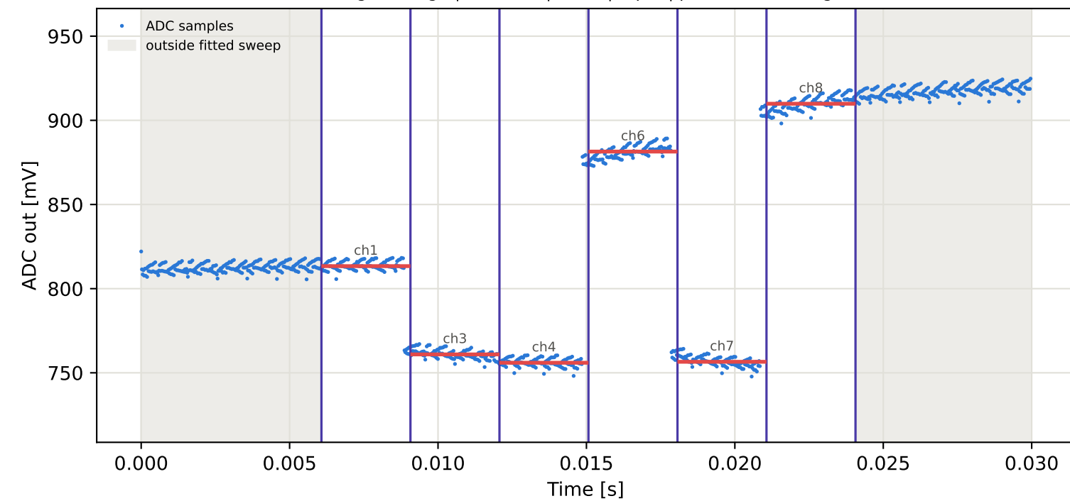
Tag4 &lt;- Tag7 | 905 MHz | run 0 | rep 1 | phase -35.69 deg
