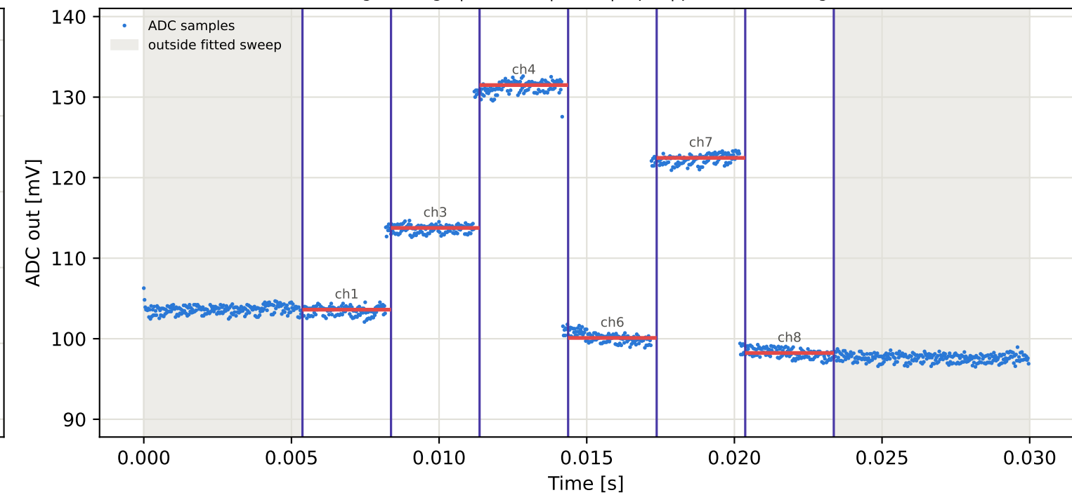
Tag2 &lt;- Tag6 | 975 MHz | run 0 | rep 1 | phase 119.77 deg
