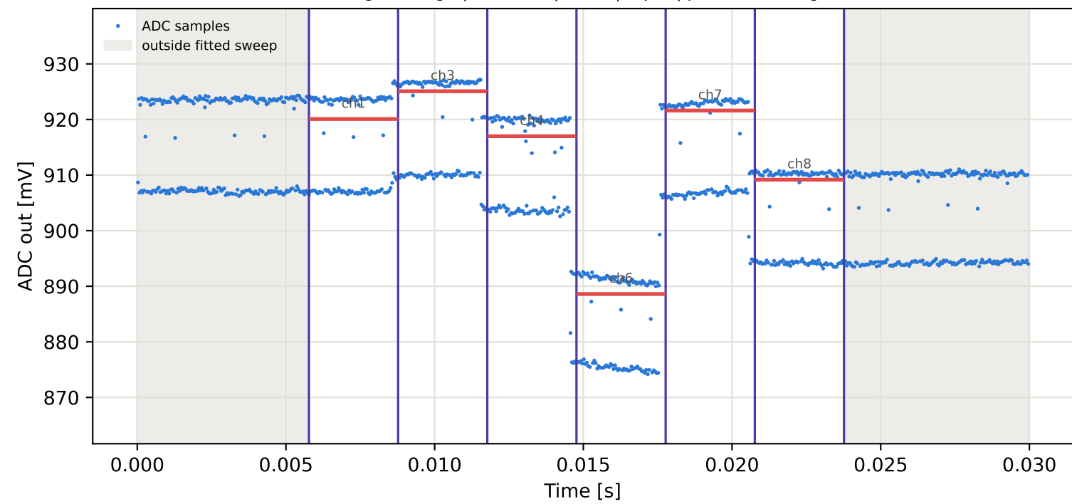
Tag4 &lt;- Tag8 | 925 MHz | run 0 | rep 1 | phase -32.40 deg
