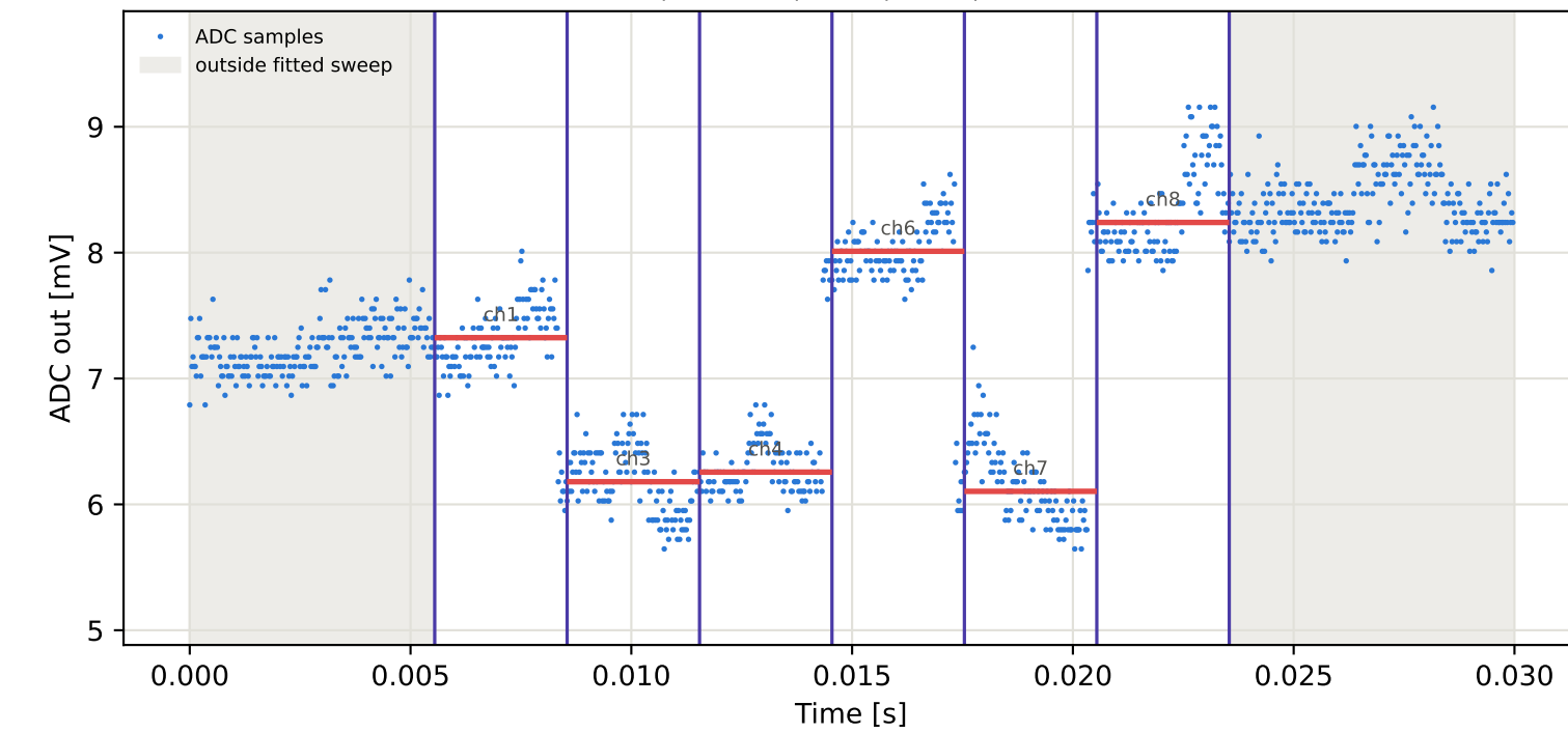
Tag2 &lt;- Tag7 | 865 MHz | run 0 | rep 1 | phase 150.13 deg
