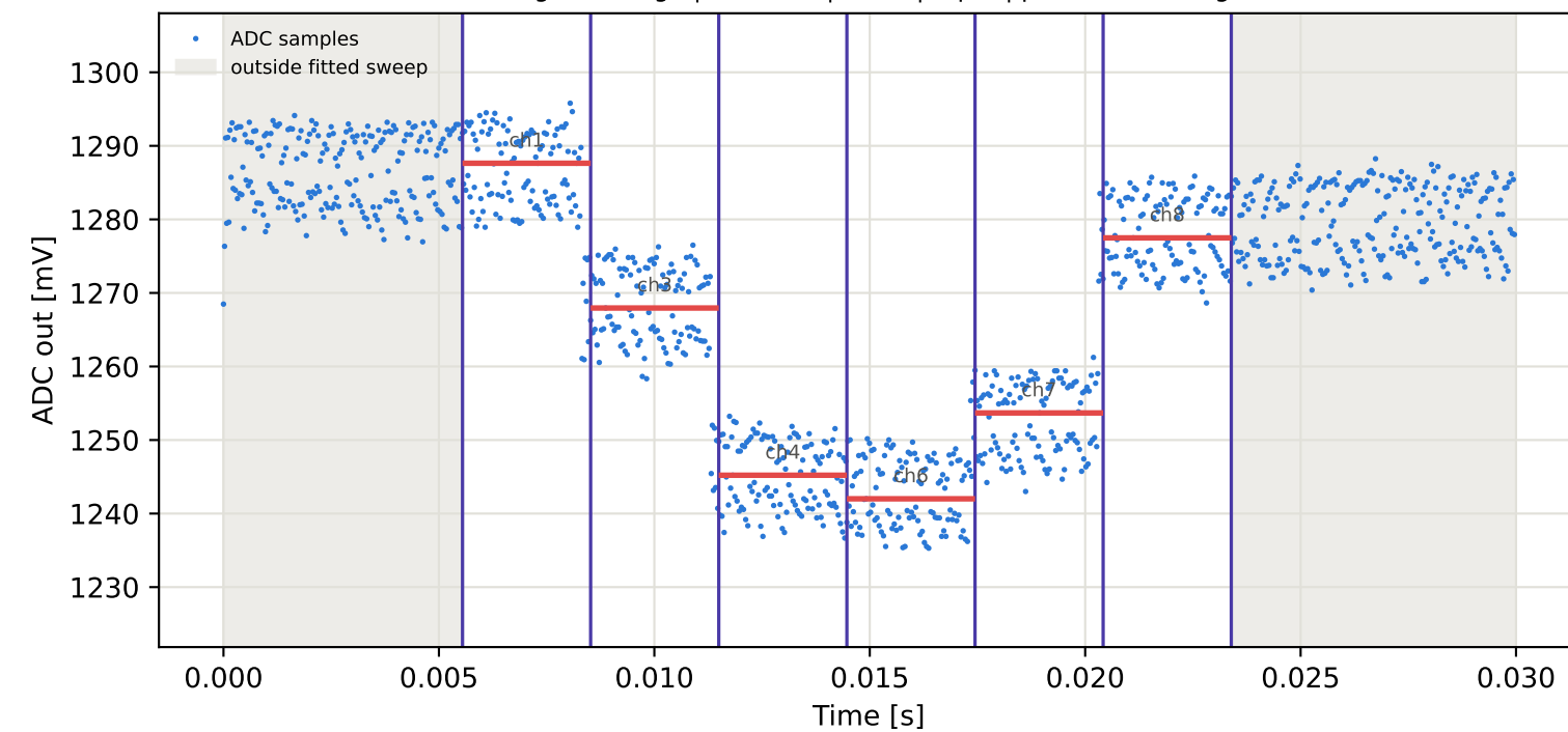
Tag16 &lt;- Tag6 | 885 MHz | run 0 | rep 1 | phase 60.59 deg
