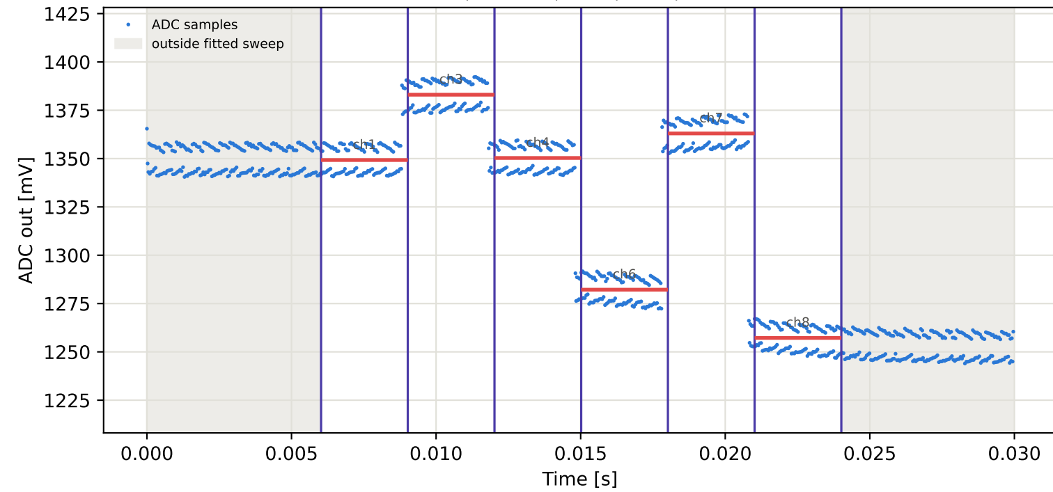
Tag8 &lt;- Tag16 | 875 MHz | run 0 | rep 1 | phase -4.94 deg
