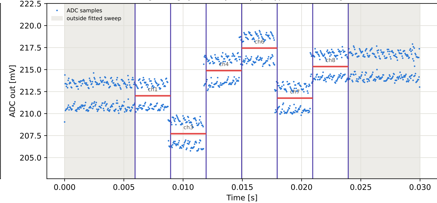
Tag9 &lt;- Tag15 | 825 MHz | run 0 | rep 1 | phase -110.04 deg
