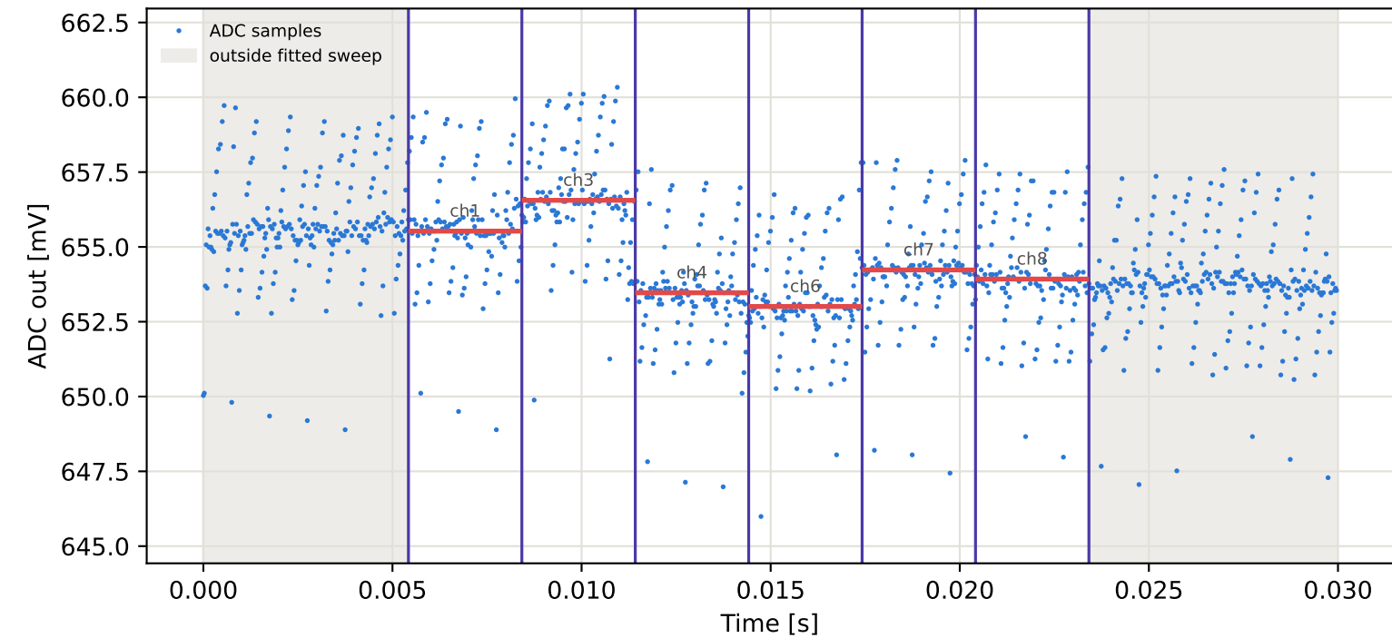
Tag8 &lt;- Tag15 | 845 MHz | run 0 | rep 1 | phase 36.22 deg
