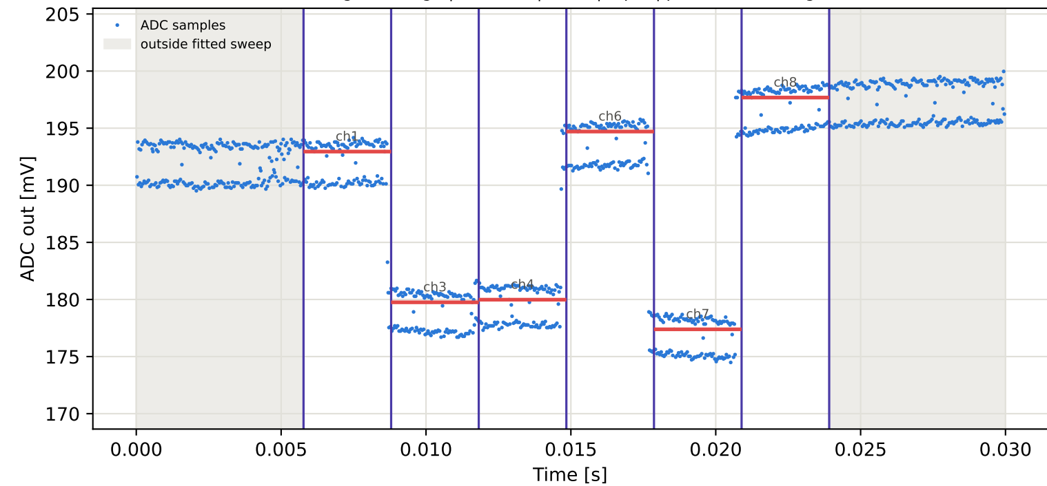
Tag2 &lt;- Tag10 | 805 MHz | run 0 | rep 1 | phase -143.01 deg
