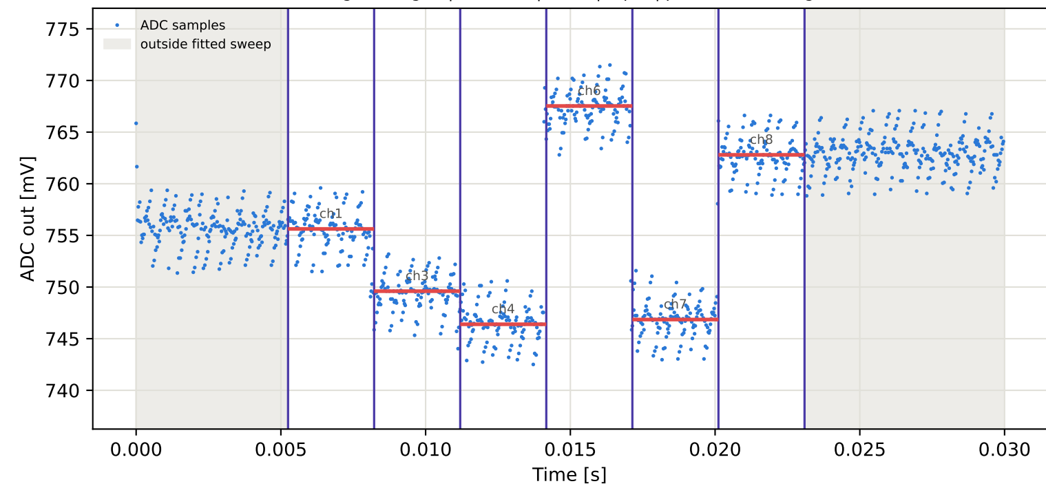
Tag4 &lt;- Tag16 | 975 MHz | run 0 | rep 1 | phase 87.89 deg
