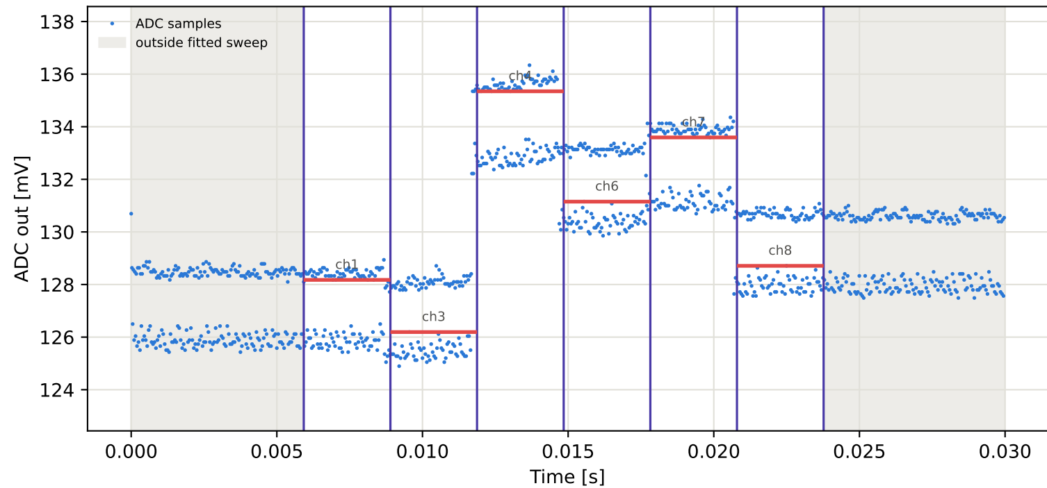
Tag3 &lt;- Tag2 | 785 MHz | run 0 | rep 1 | phase 25.28 deg
