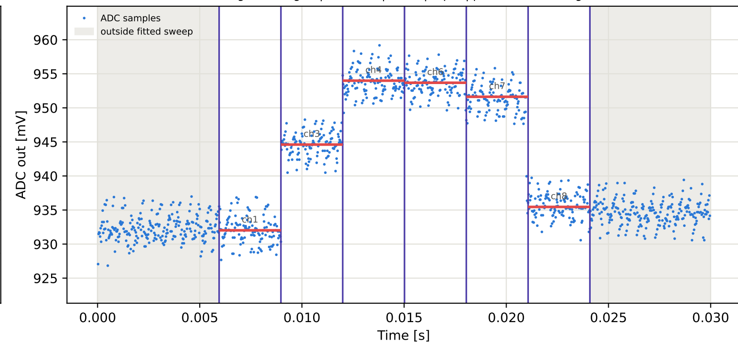
Tag15 &lt;- Tag10 | 885 MHz | run 0 | rep 1 | phase -109.71 deg
