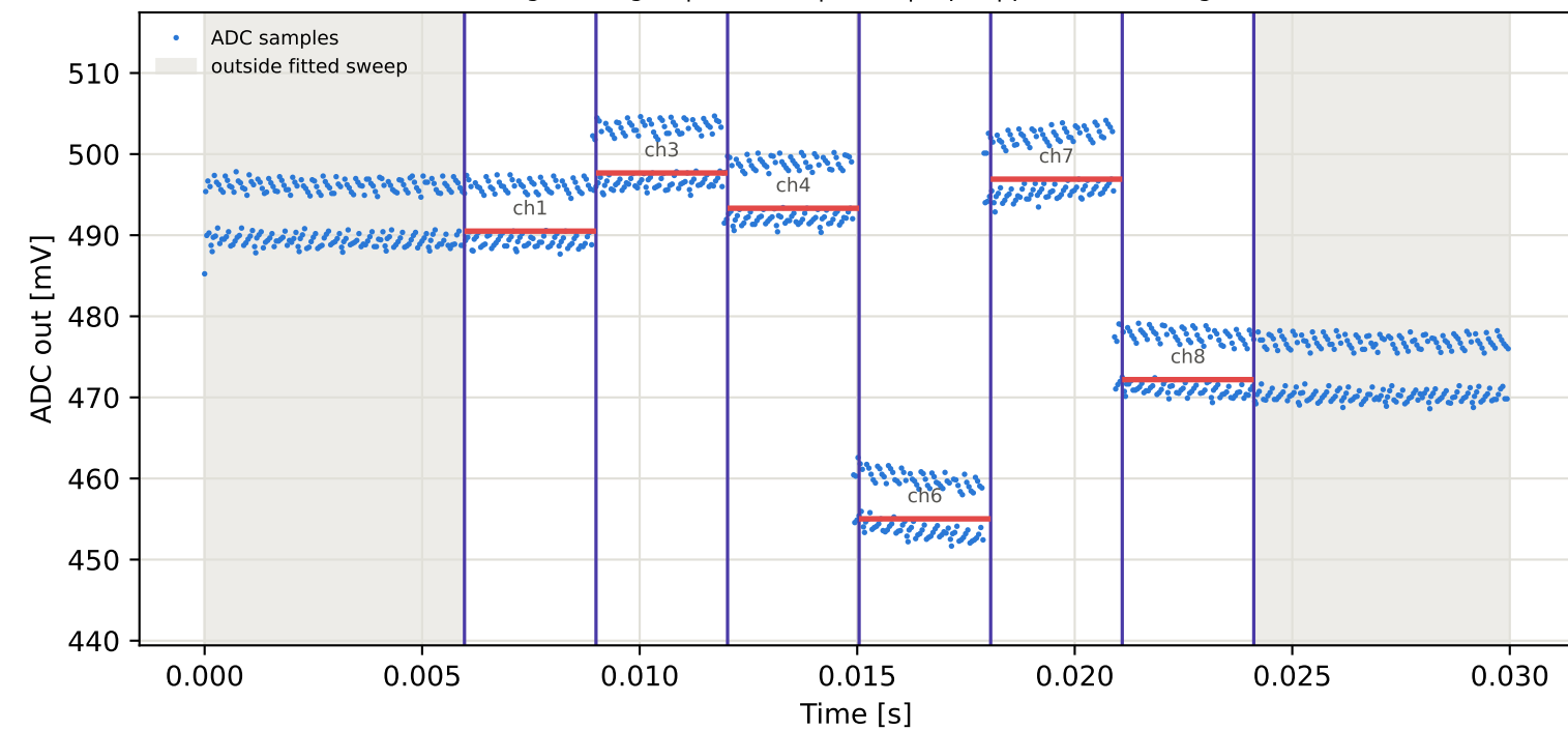
Tag1 &lt;- Tag2 | 945 MHz | run 0 | rep 1 | phase -6.79 deg
