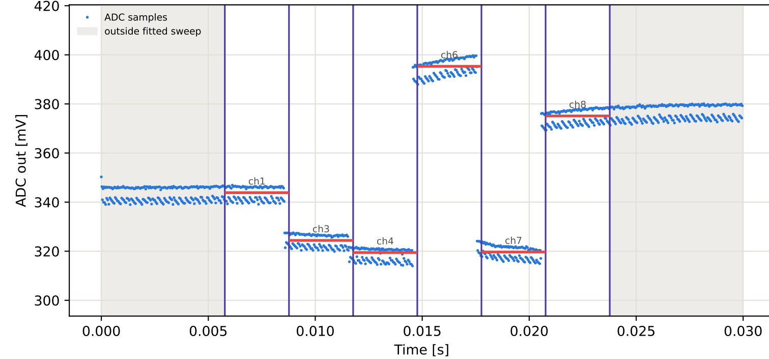
Tag3 &lt;- Tag8 | 925 MHz | run 0 | rep 1 | phase -128.04 deg
