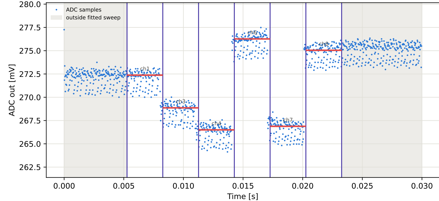
Tag1 &lt;- Tag3 | 985 MHz | run 0 | rep 1 | phase -53.05 deg
