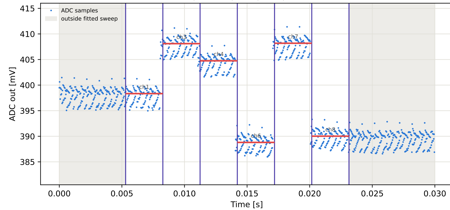
Tag9 &lt;- Tag7 | 835 MHz | run 0 | rep 1 | phase -12.73 deg
