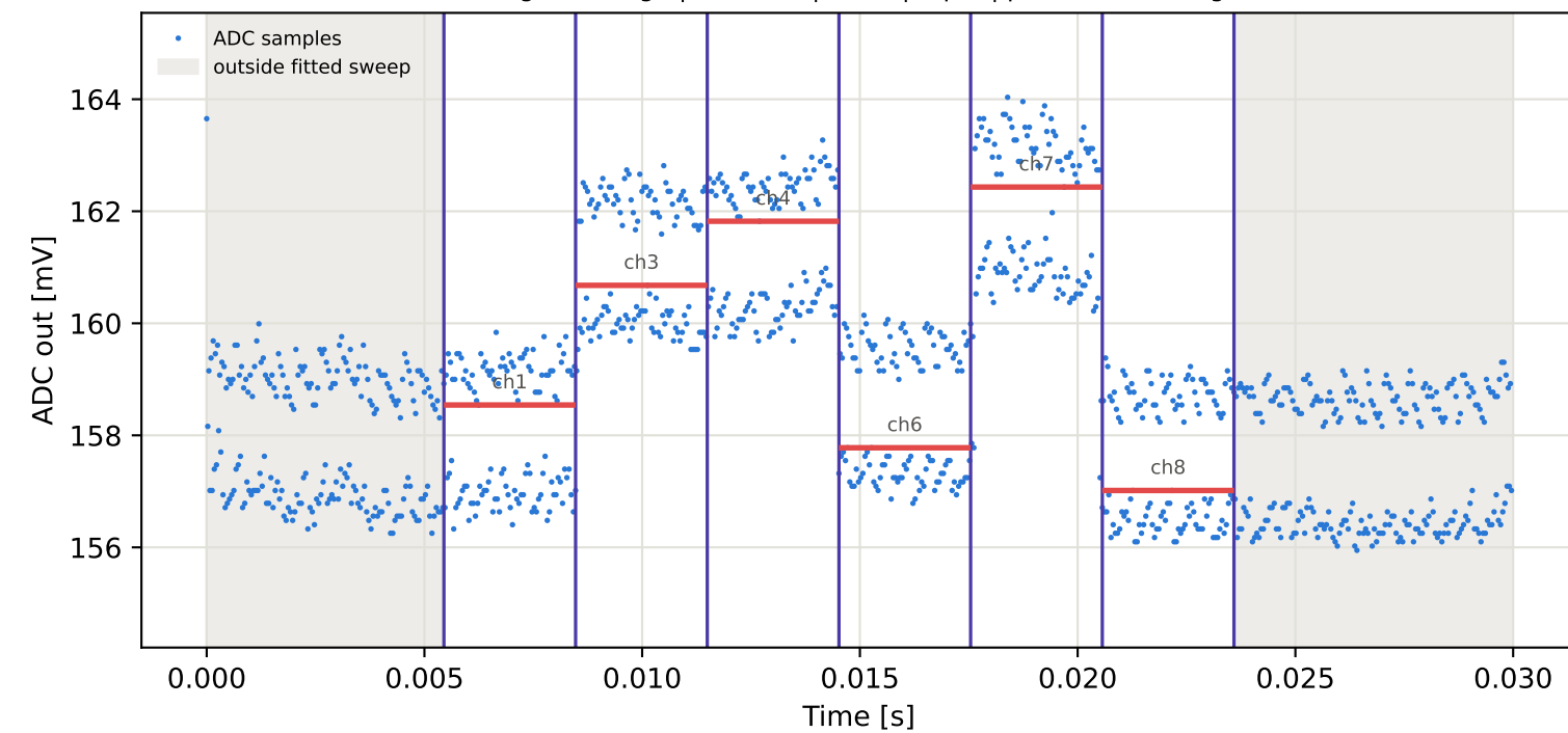
Tag16 &lt;- Tag10 | 785 MHz | run 0 | rep 1 | phase 75.96 deg
