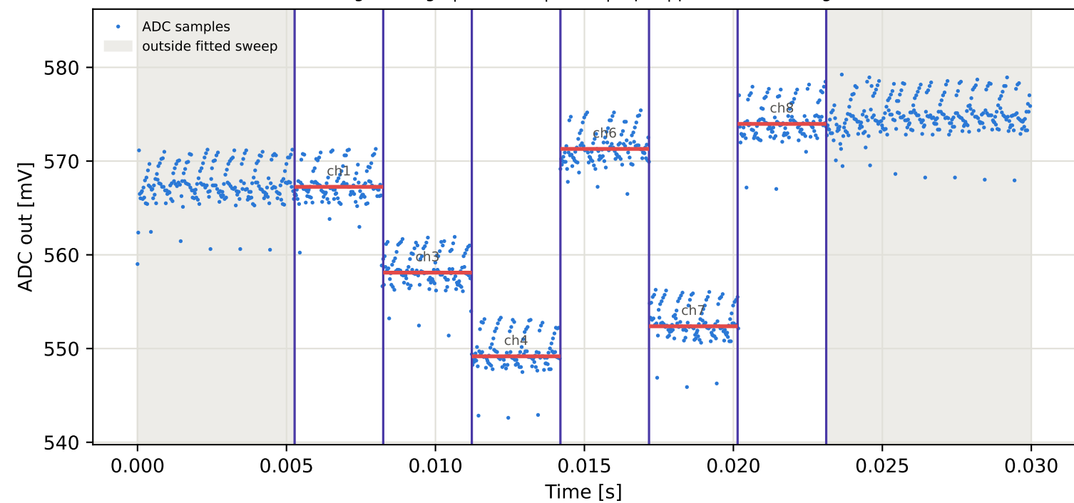
Tag5 &lt;- Tag1 | 945 MHz | run 0 | rep 1 | phase 118.72 deg
