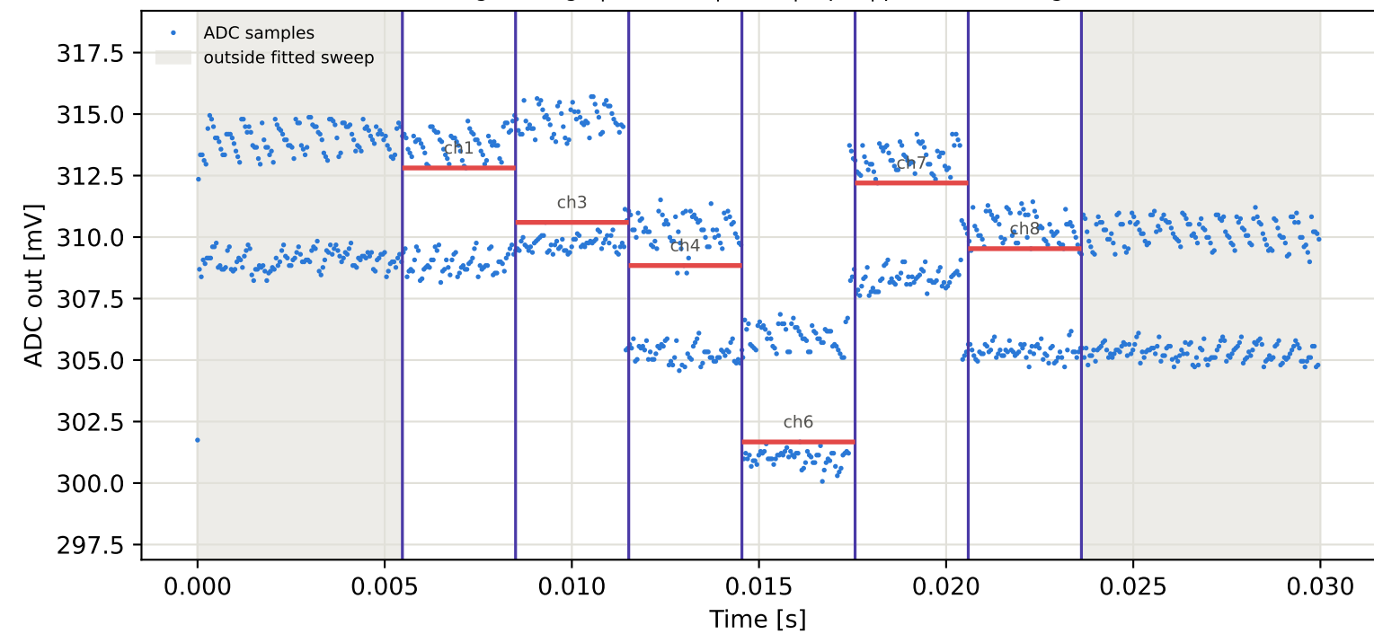
Tag5 &lt;- Tag9 | 965 MHz | run 0 | rep 1 | phase -173.26 deg
