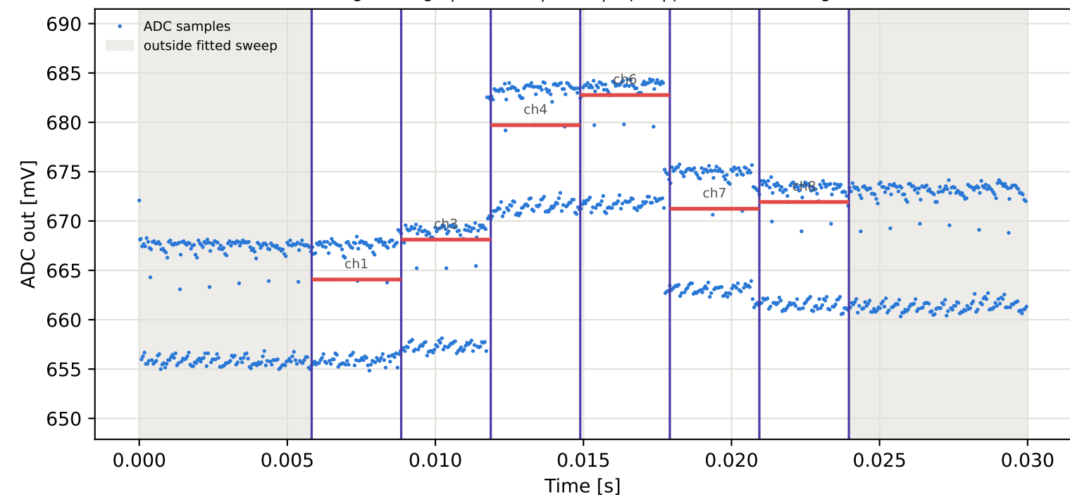
Tag7 &lt;- Tag6 | 965 MHz | run 0 | rep 1 | phase -142.03 deg
