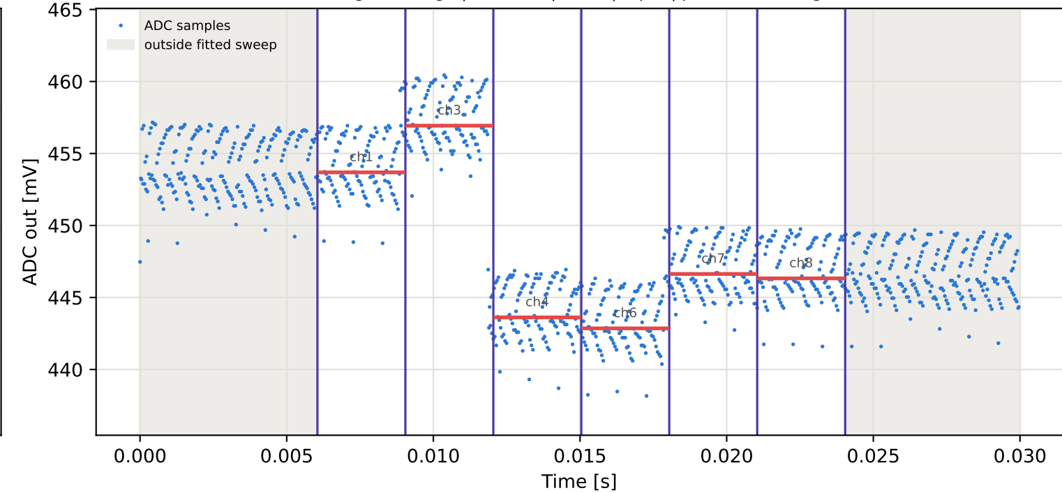
Tag16 &lt;- Tag5 | 825 MHz | run 0 | rep 1 | phase -87.68 deg
