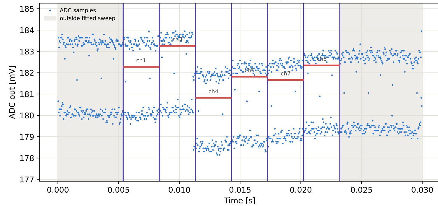
Tag16 &lt;- Tag10 | 805 MHz | run 0 | rep 1 | phase 71.73 deg
