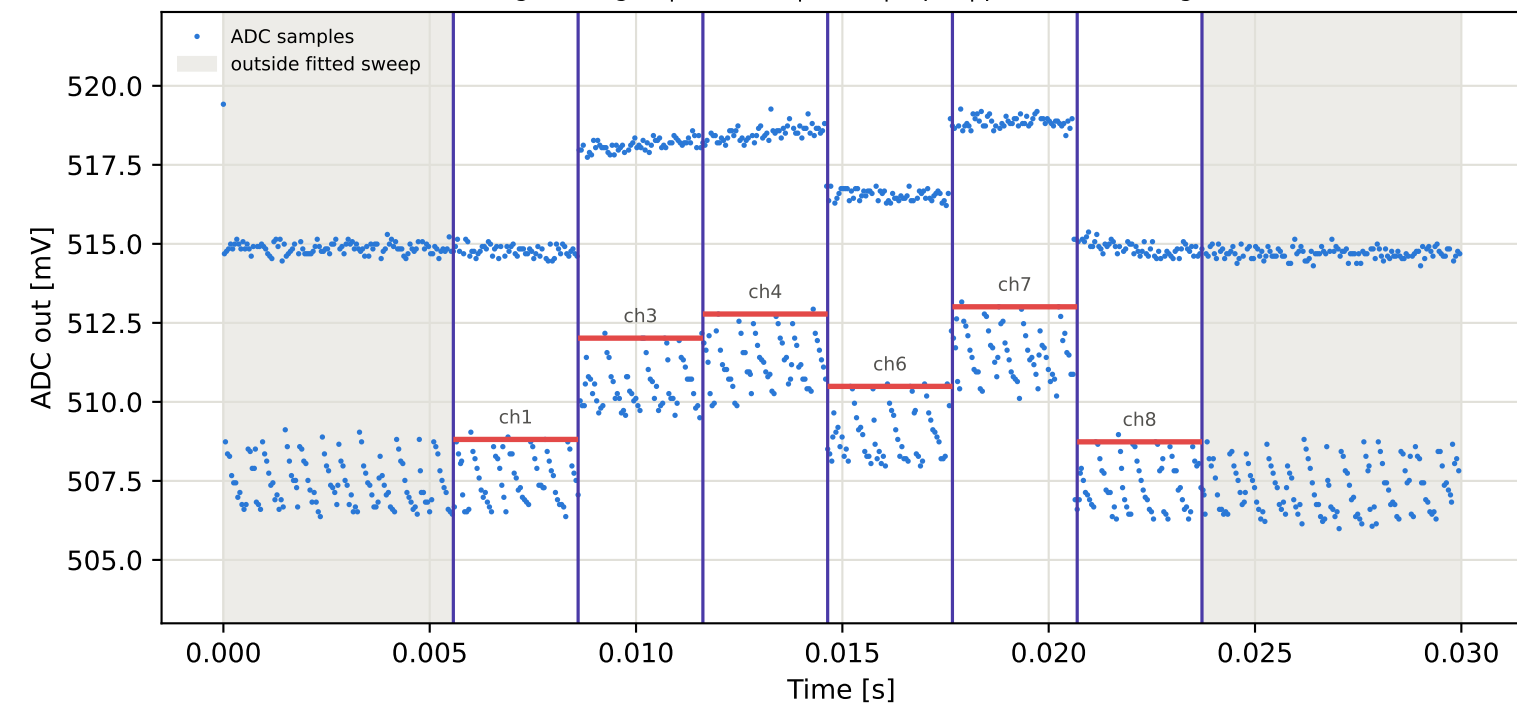
Tag5 &lt;- Tag16 | 855 MHz | run 0 | rep 1 | phase -149.05 deg
