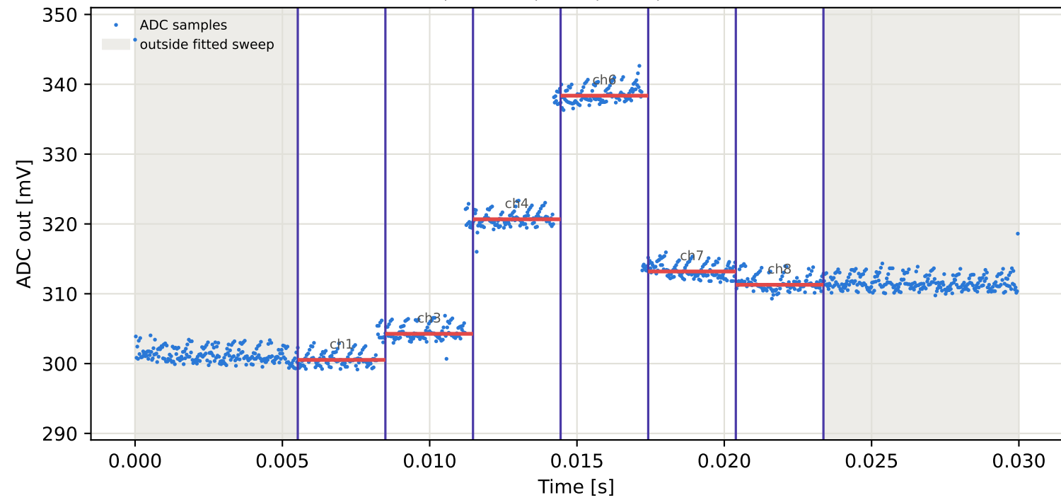
Tag6 &lt;- Tag4 | 925 MHz | run 0 | rep 1 | phase -145.22 deg
