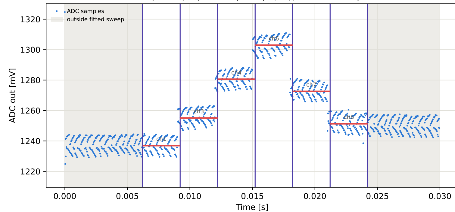
Tag5 &lt;- Tag3 | 905 MHz | run 0 | rep 1 | phase -12.92 deg
