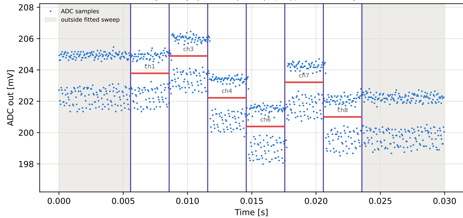
Tag1 &lt;- Tag7 | 855 MHz | run 0 | rep 1 | phase -75.22 deg
