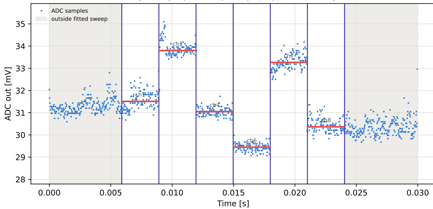
Tag1 &lt;- Tag16 | 785 MHz | run 0 | rep 1 | phase 6.52 deg
