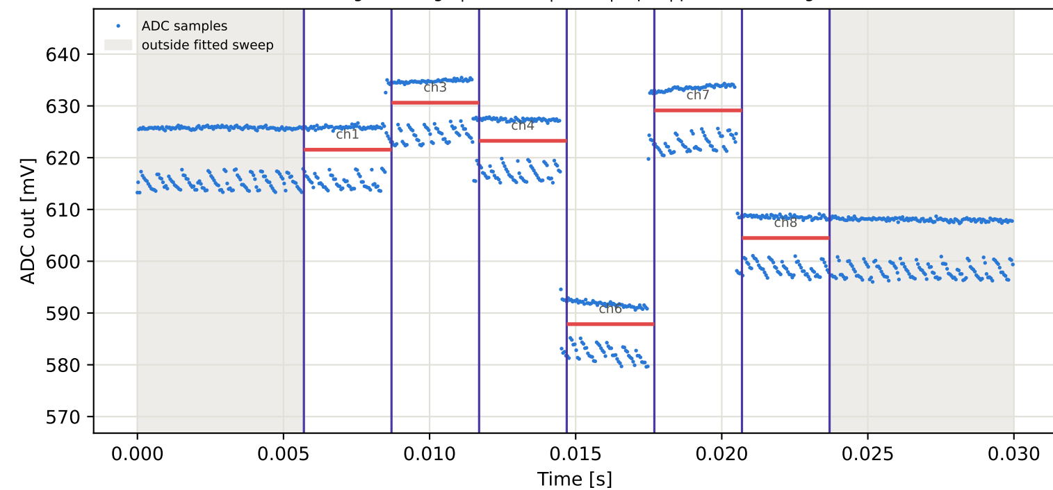
Tag16 &lt;- Tag7 | 955 MHz | run 0 | rep 1 | phase -2.83 deg
