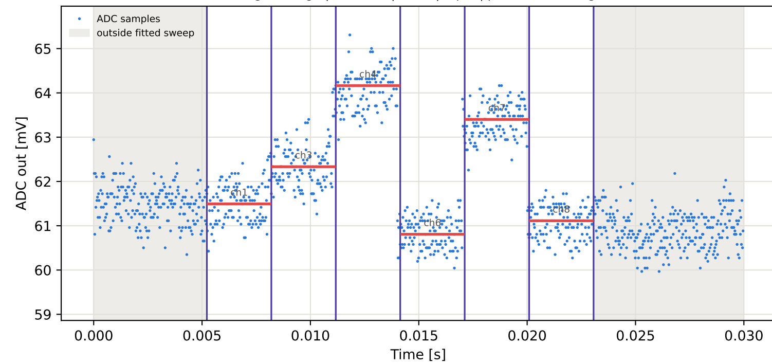
Tag2 &lt;- Tag5 | 995 MHz | run 0 | rep 1 | phase 7.26 deg
