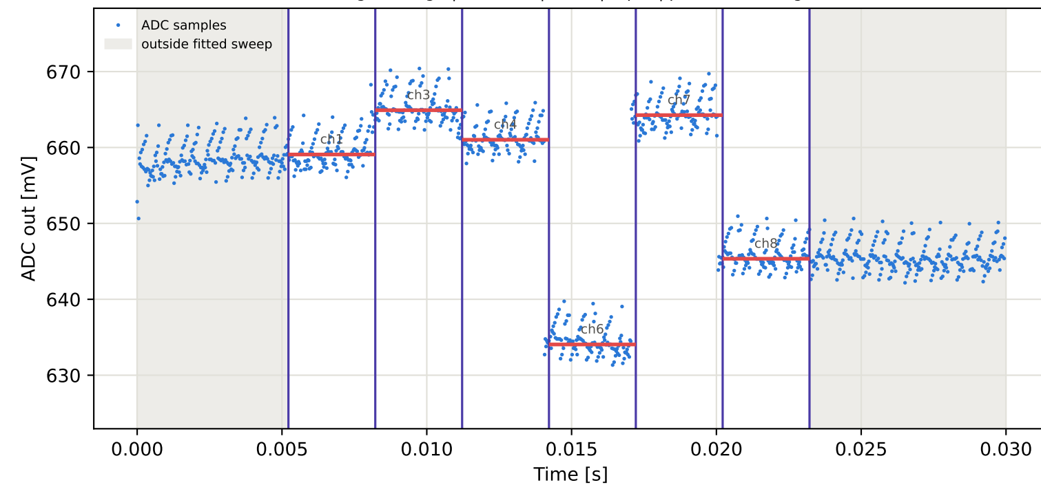
Tag9 &lt;- Tag10 | 945 MHz | run 0 | rep 1 | phase -140.33 deg
