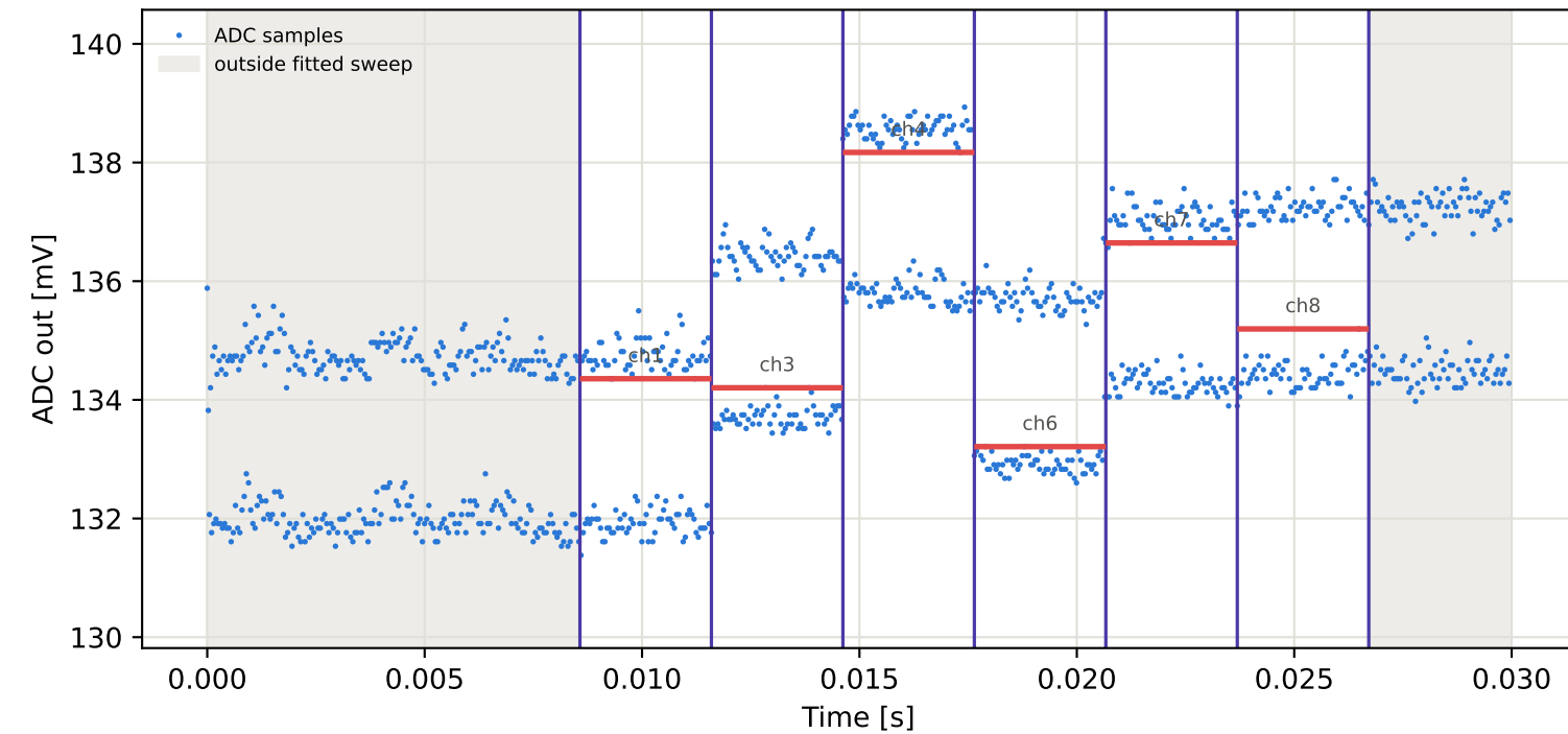
Tag10 &lt;- Tag4 | 845 MHz | run 0 | rep 1 | phase 153.99 deg
