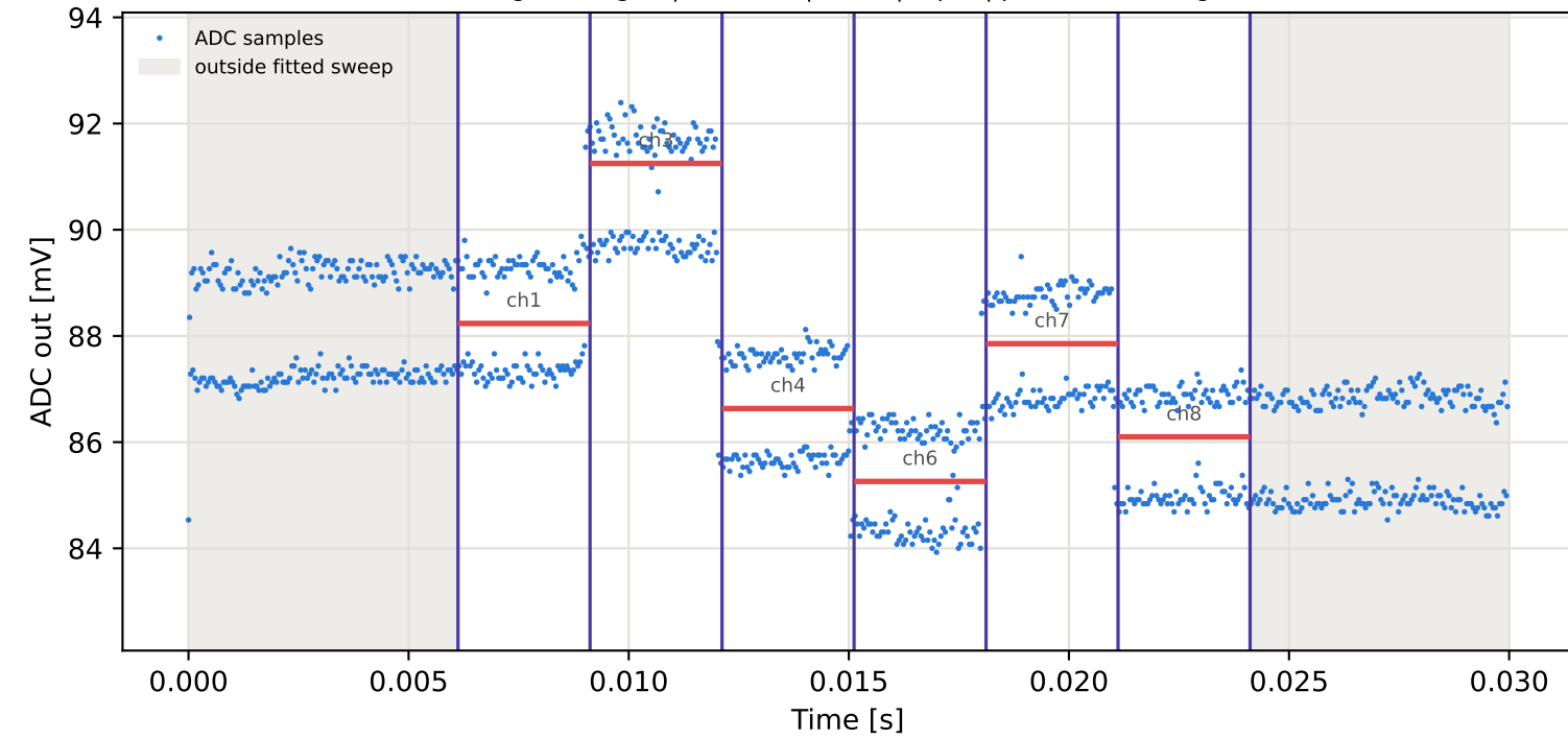
Tag1 &lt;- Tag2 | 845 MHz | run 0 | rep 1 | phase 60.48 deg
