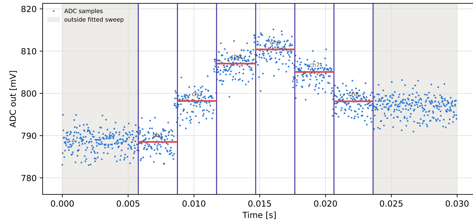
Tag3 &lt;- Tag8 | 885 MHz | run 0 | rep 1 | phase -124.65 deg
