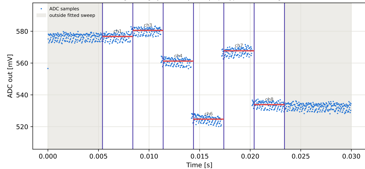
Tag1 &lt;- Tag7 | 885 MHz | run 0 | rep 1 | phase 139.75 deg
