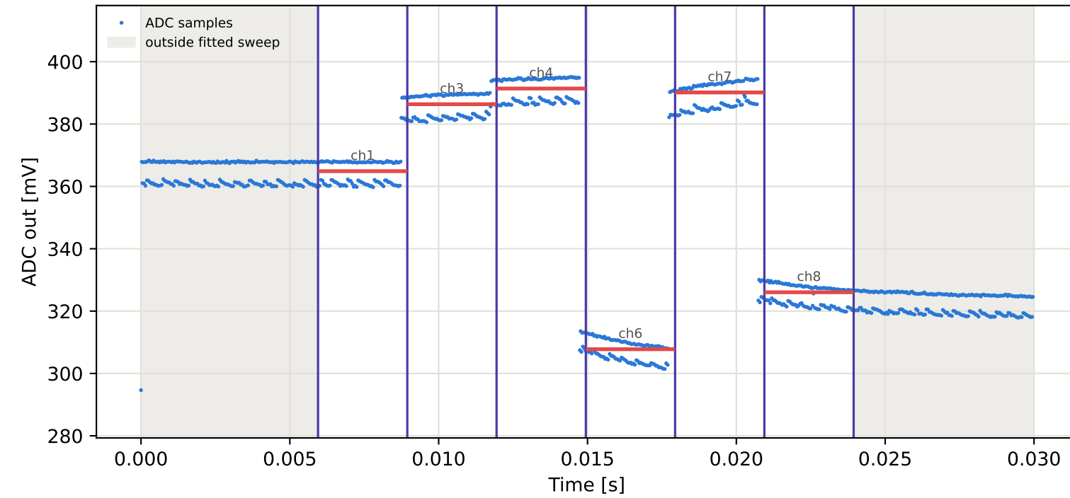
Tag9 &lt;- Tag16 | 925 MHz | run 0 | rep 1 | phase -20.10 deg
