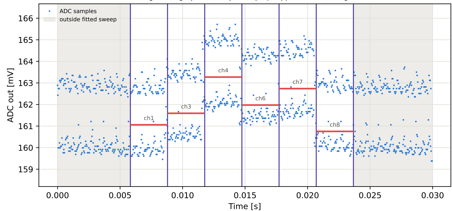
Tag9 &lt;- Tag2 | 805 MHz | run 0 | rep 1 | phase -87.68 deg
