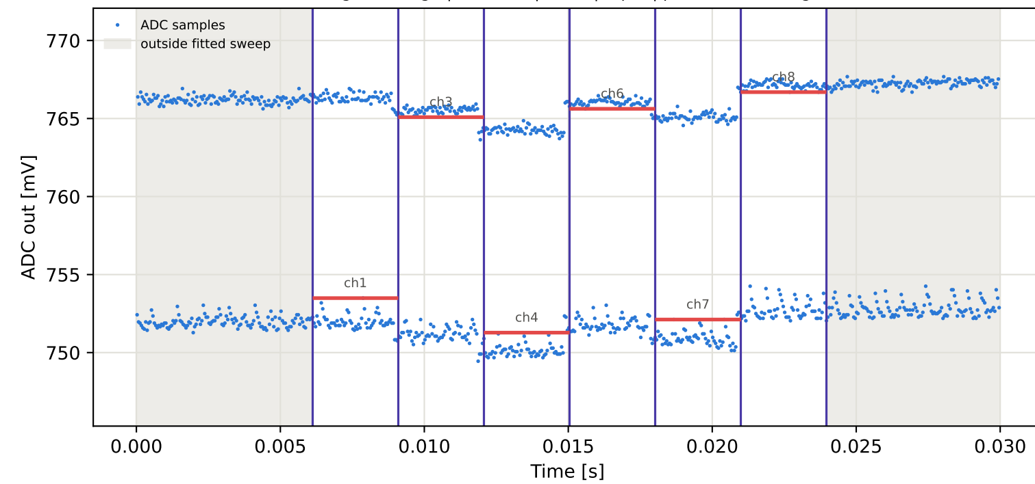
Tag16 &lt;- Tag4 | 965 MHz | run 0 | rep 1 | phase -172.29 deg
