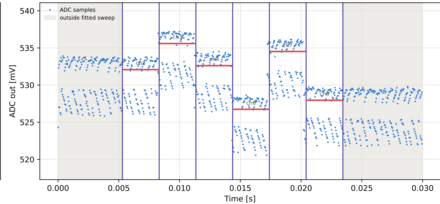
Tag6 &lt;- Tag10 | 835 MHz | run 0 | rep 1 | phase 158.39 deg
