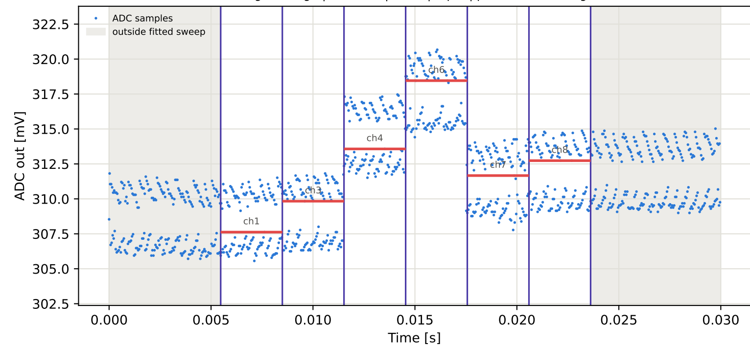
Tag5 &lt;- Tag1 | 965 MHz | run 0 | rep 1 | phase -151.07 deg
