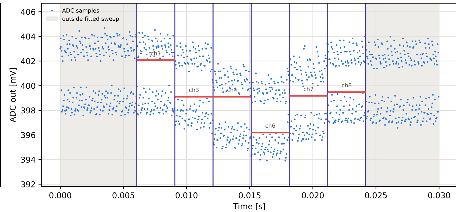
Tag3 &lt;- Tag2 | 955 MHz | run 0 | rep 1 | phase 32.00 deg
