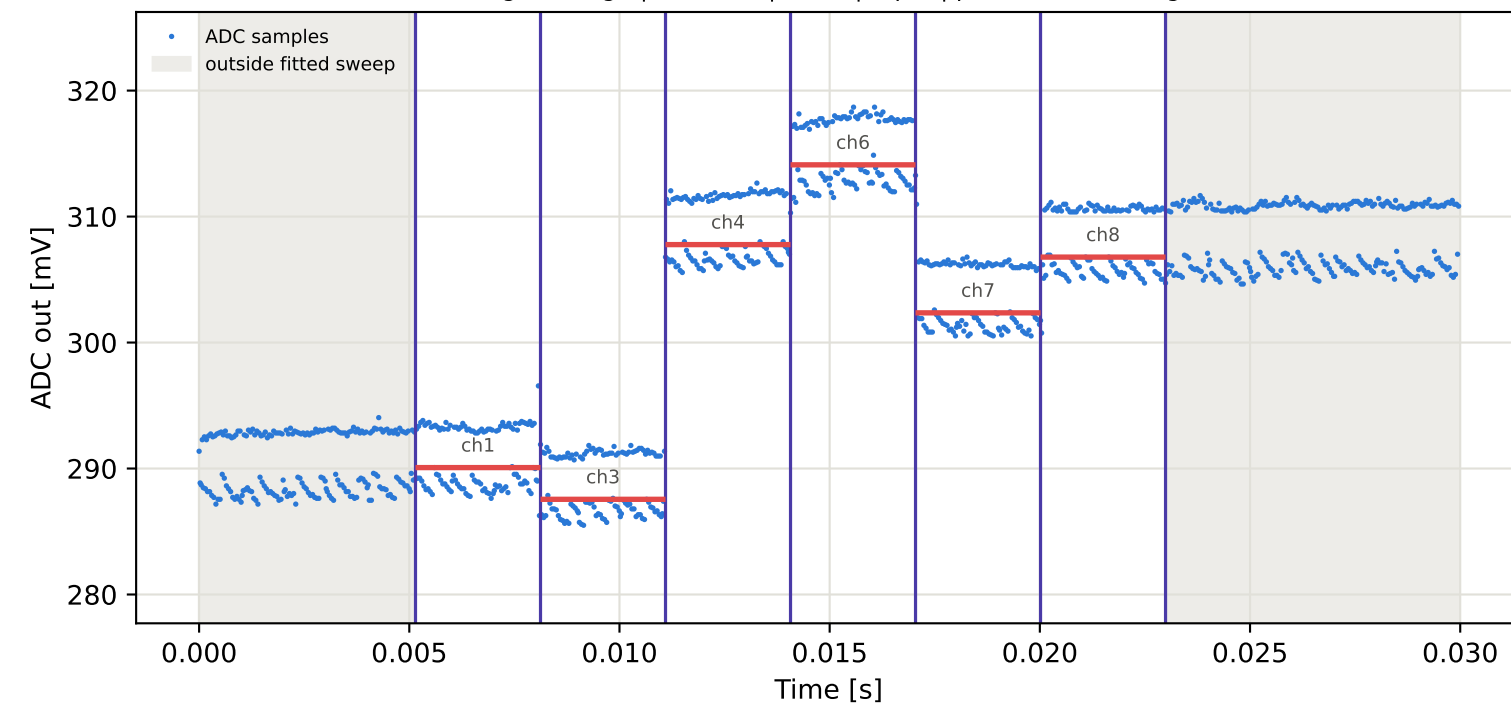
Tag8 &lt;- Tag1 | 835 MHz | run 0 | rep 1 | phase 80.79 deg
