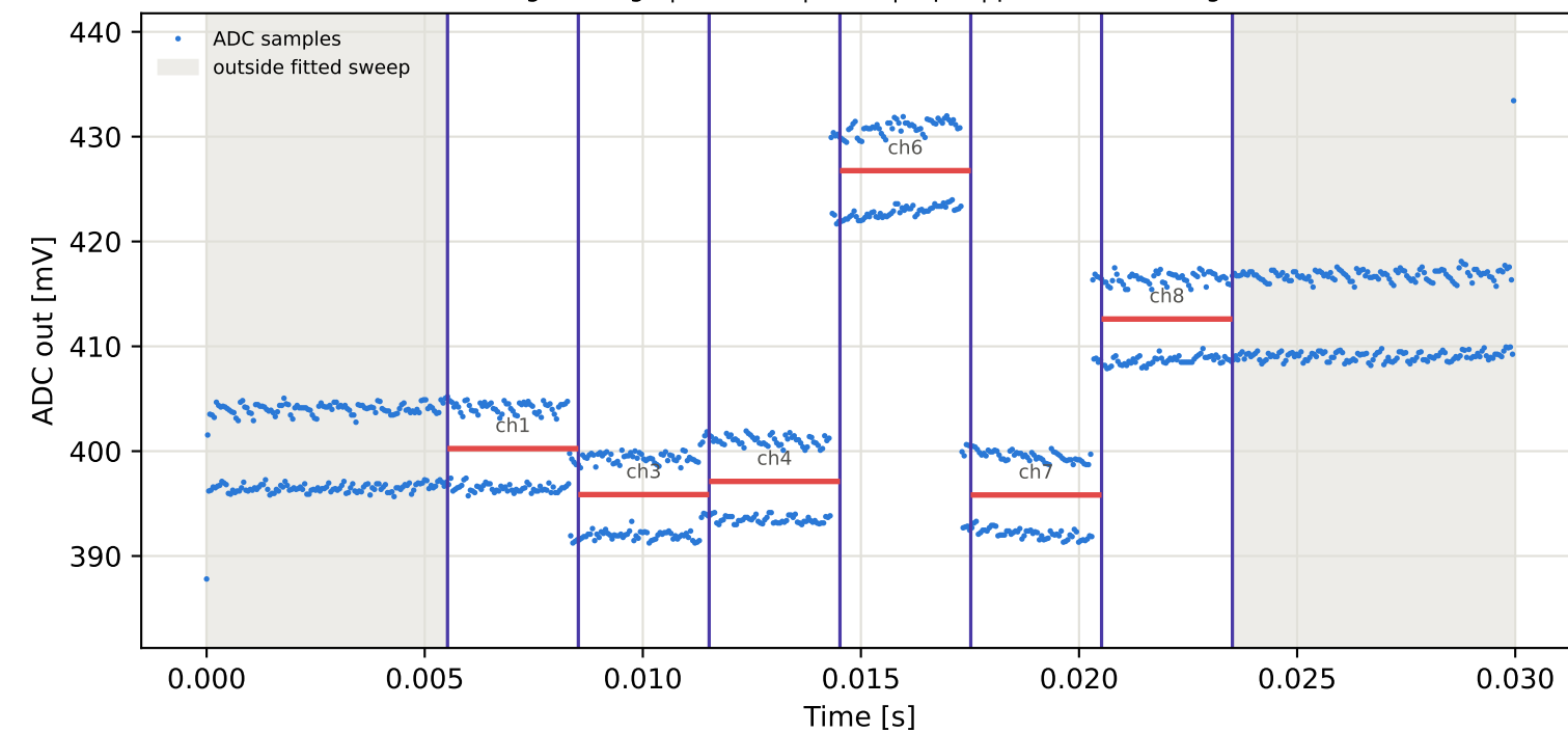
Tag7 &lt;- Tag5 | 935 MHz | run 0 | rep 1 | phase 174.72 deg
