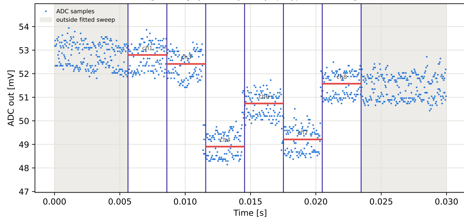
Tag2 &lt;- Tag10 | 775 MHz | run 0 | rep 1 | phase 96.82 deg
