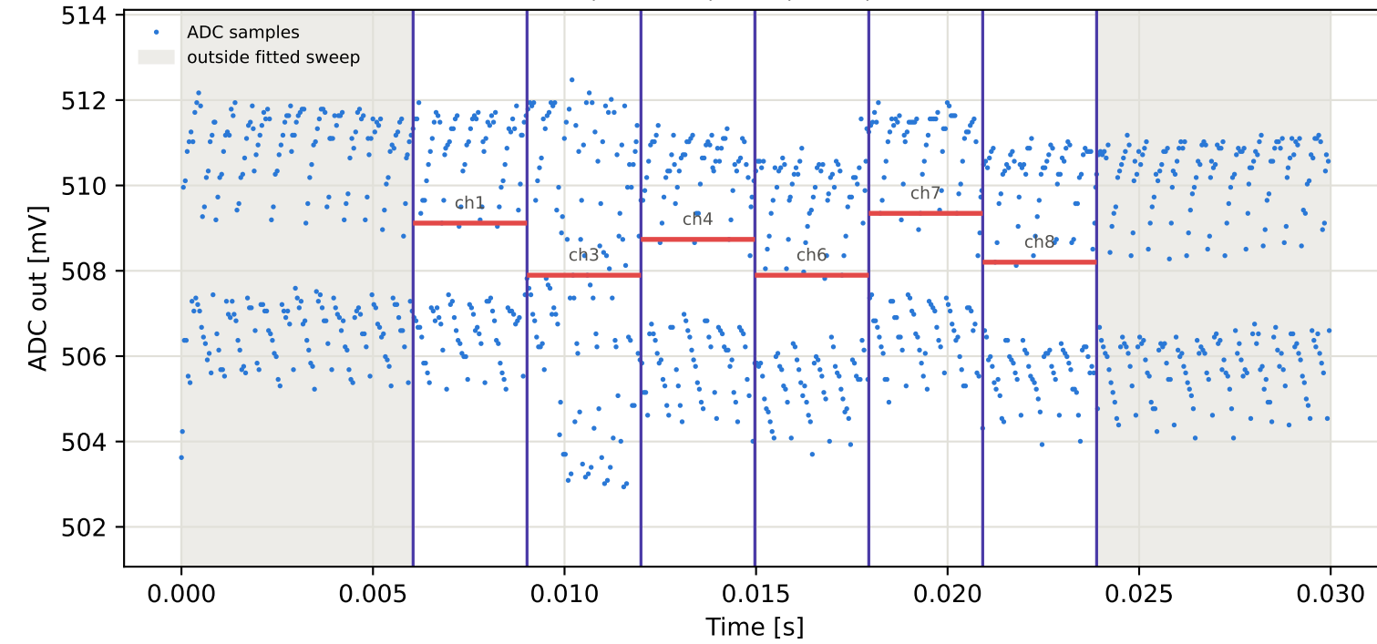
Tag9 &lt;- Tag7 | 845 MHz | run 0 | rep 1 | phase -20.15 deg
