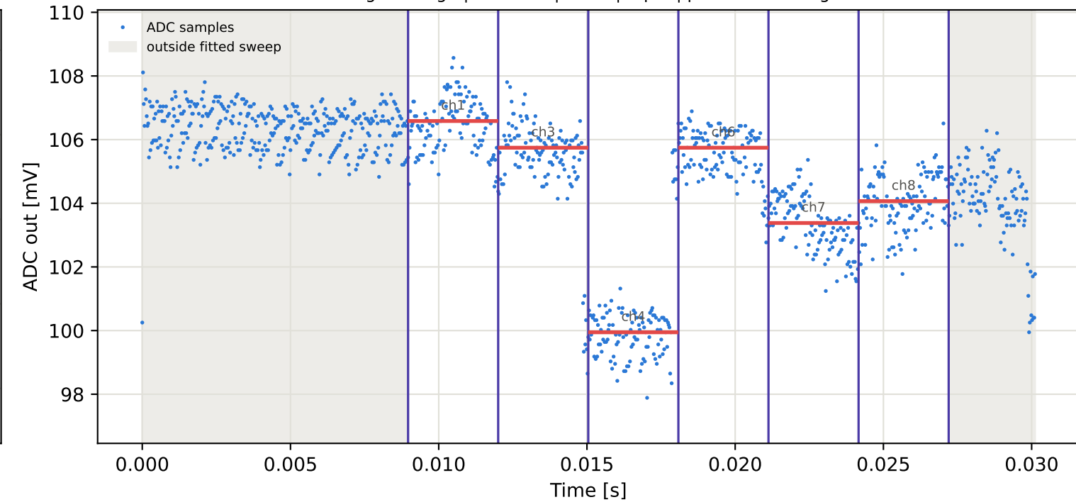
Tag7 &lt;- Tag4 | 875 MHz | run 0 | rep 1 | phase 144.28 deg
