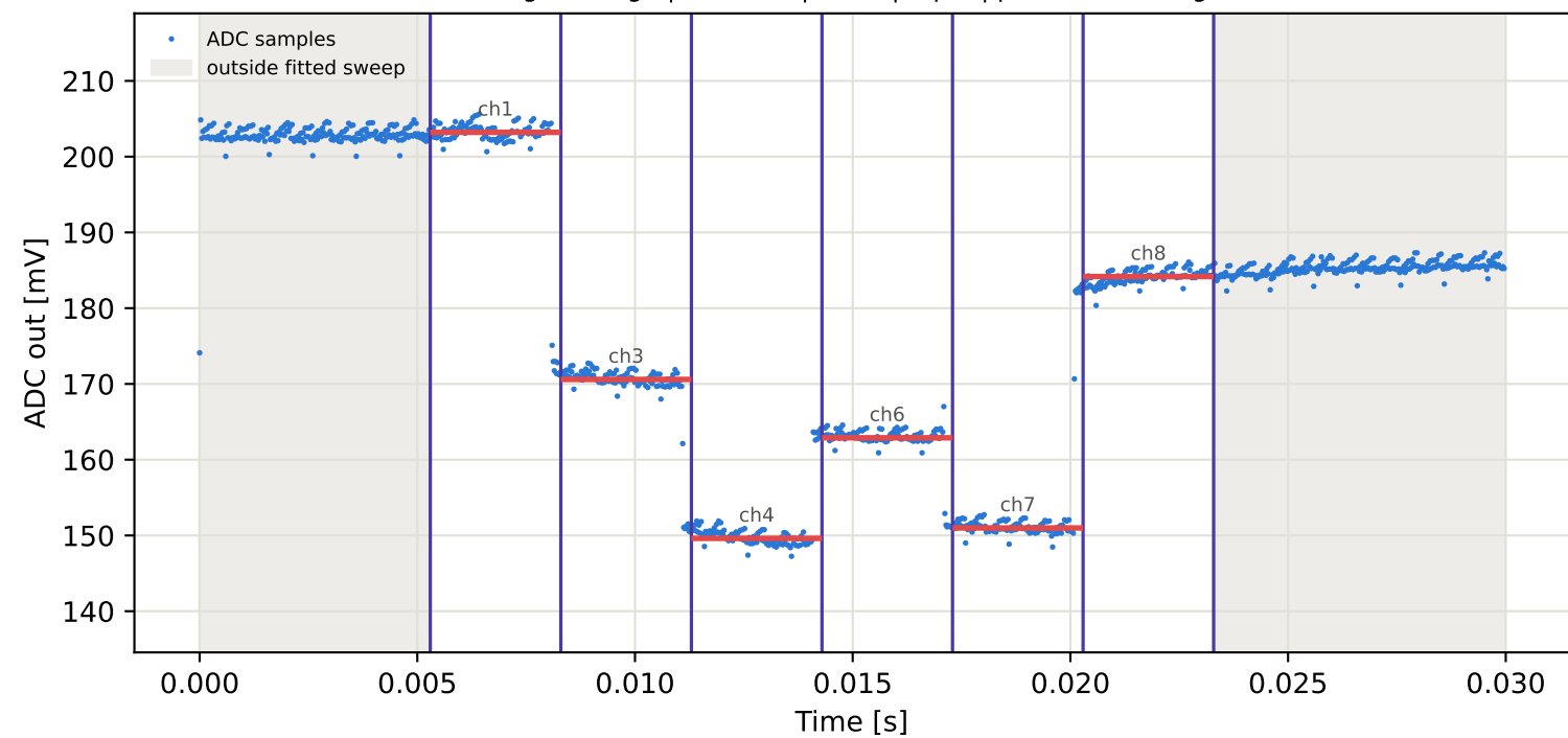
Tag6 &lt;- Tag4 | 845 MHz | run 0 | rep 1 | phase 82.62 deg
