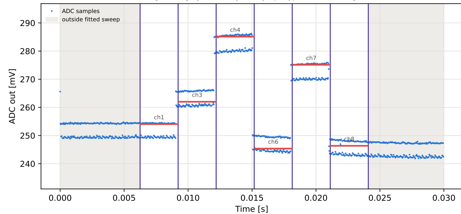
Tag3 &lt;- Tag15 | 995 MHz | run 0 | rep 1 | phase 83.00 deg
