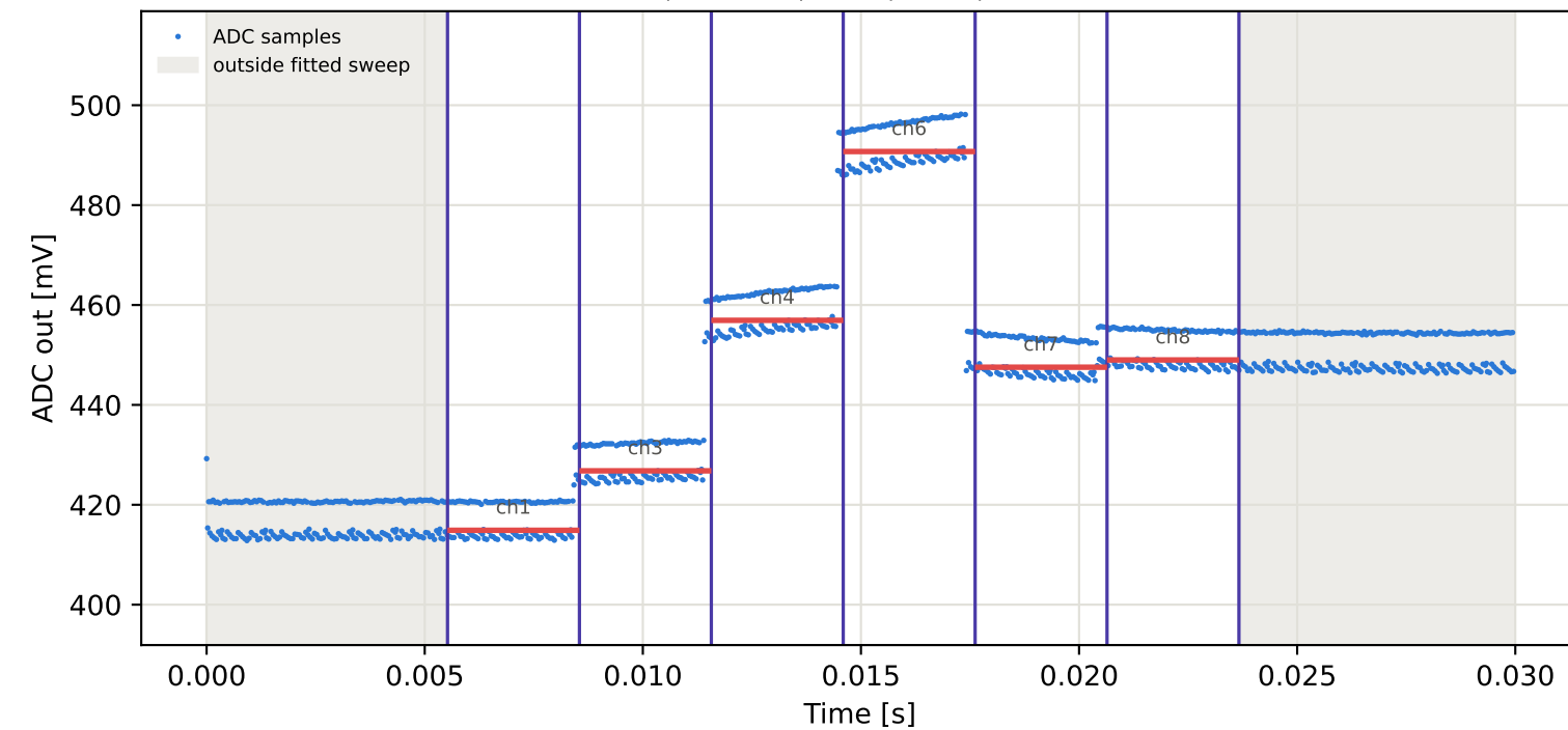
Tag1 &lt;- Tag3 | 895 MHz | run 0 | rep 1 | phase -144.13 deg
