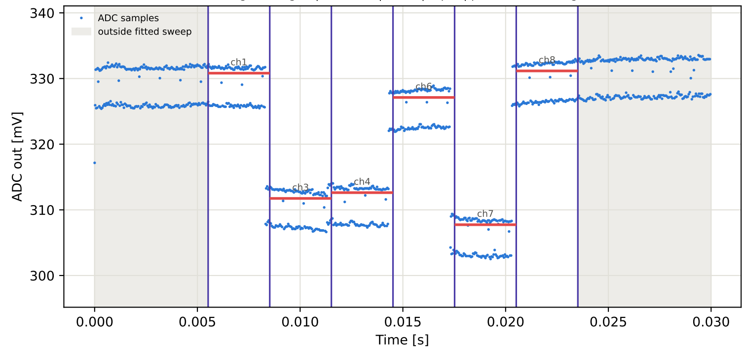
Tag6 &lt;- Tag3 | 825 MHz | run 0 | rep 1 | phase -34.38 deg
