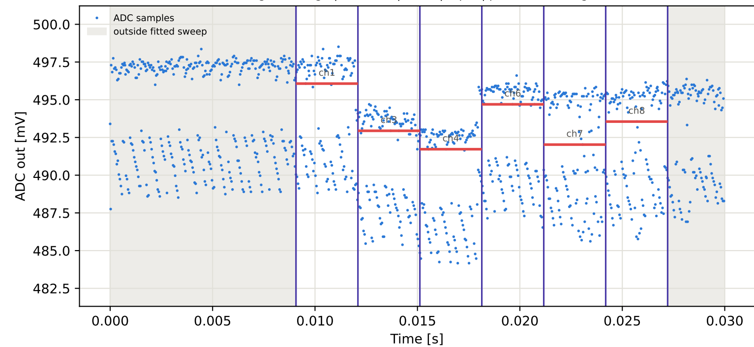
Tag15 &lt;- Tag9 | 995 MHz | run 0 | rep 1 | phase 159.96 deg
