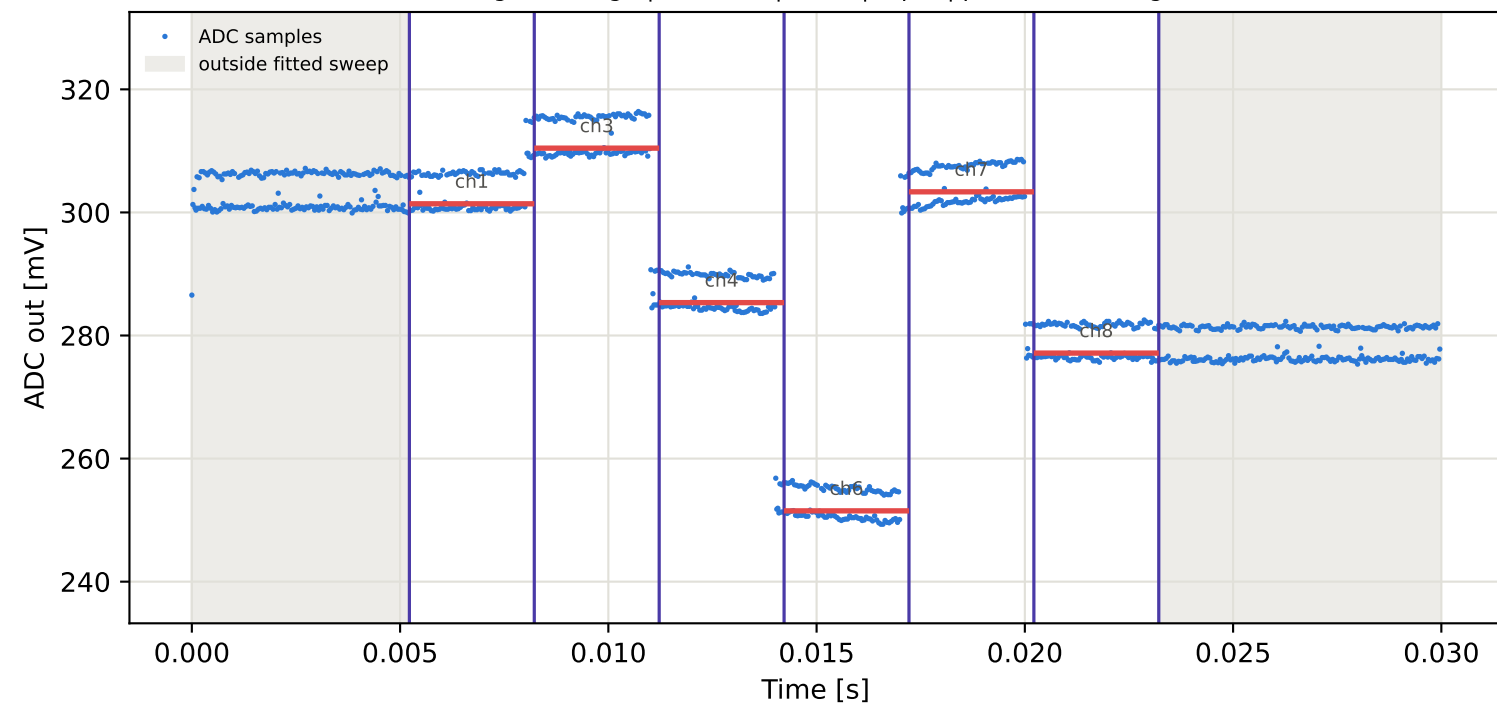
Tag10 &lt;- Tag9 | 975 MHz | run 0 | rep 1 | phase -4.59 deg
