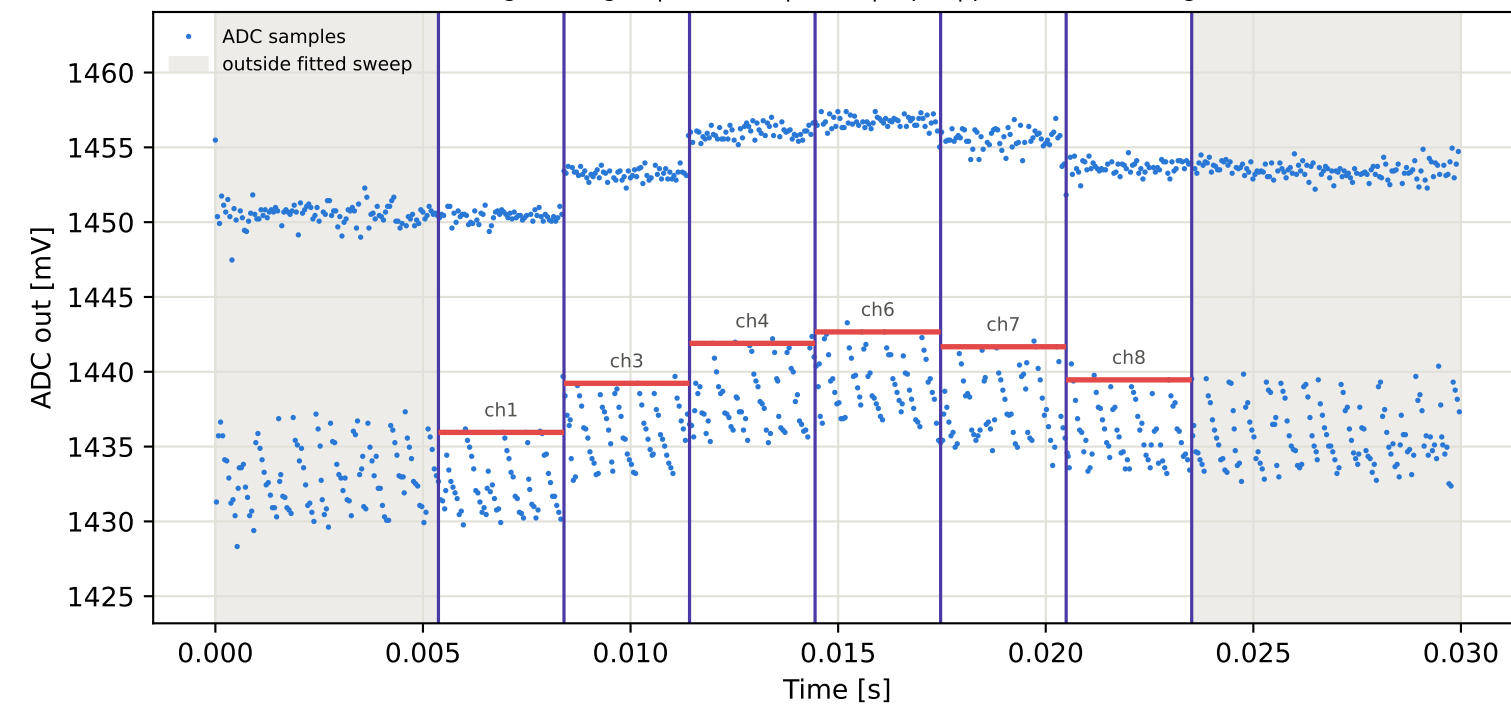
Tag5 &lt;- Tag16 | 875 MHz | run 0 | rep 1 | phase -146.36 deg
