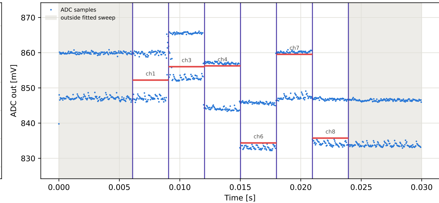
Tag16 &lt;- Tag7 | 865 MHz | run 0 | rep 1 | phase -170.52 deg
