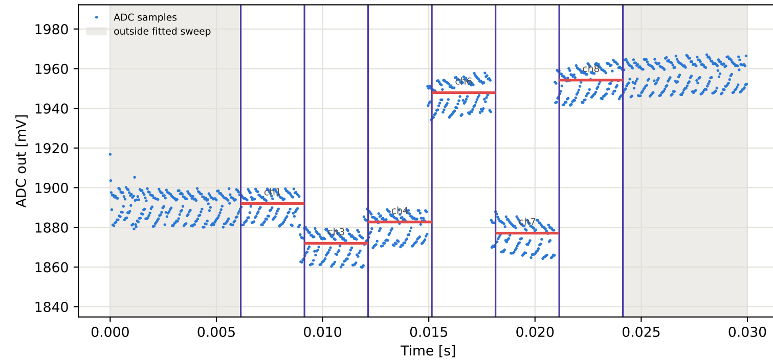
Tag6 &lt;- Tag1 | 895 MHz | run 0 | rep 1 | phase -62.27 deg
