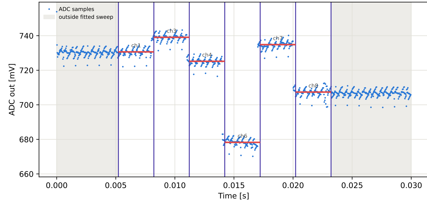
Tag4 &lt;- Tag3 | 955 MHz | run 0 | rep 1 | phase 150.42 deg
