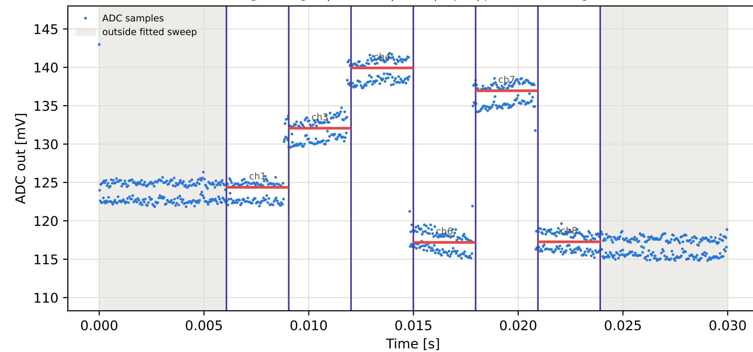
Tag6 &lt;- Tag2 | 975 MHz | run 0 | rep 1 | phase 104.49 deg
