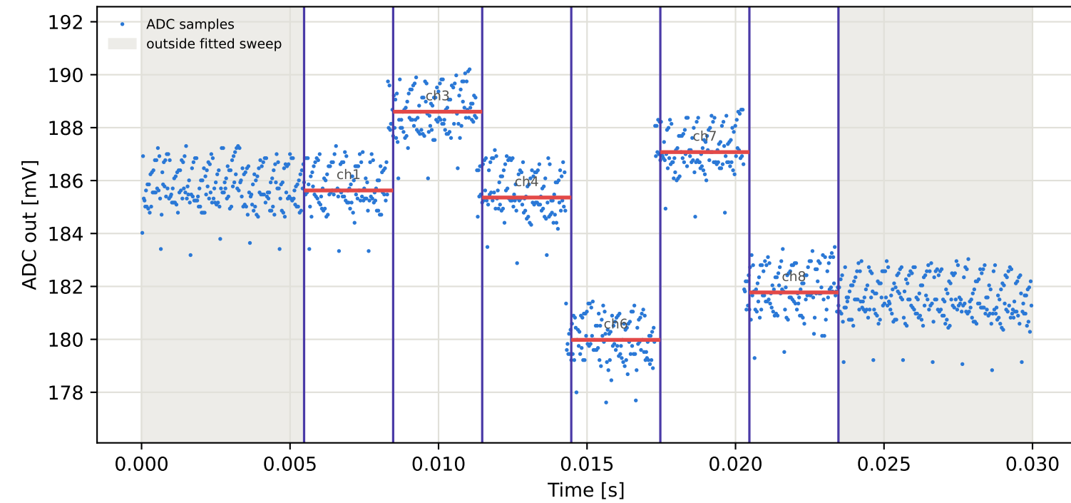
Tag4 &lt;- Tag9 | 825 MHz | run 0 | rep 1 | phase -75.24 deg
