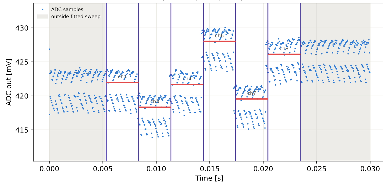
Tag15 &lt;- Tag9 | 825 MHz | run 0 | rep 1 | phase 115.89 deg
