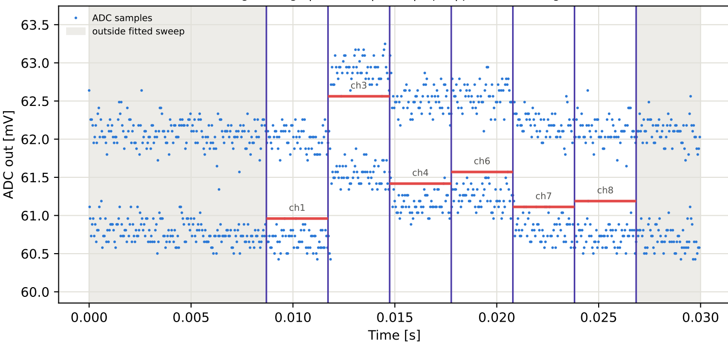
Tag8 &lt;- Tag15 | 775 MHz | run 0 | rep 1 | phase -102.67 deg
