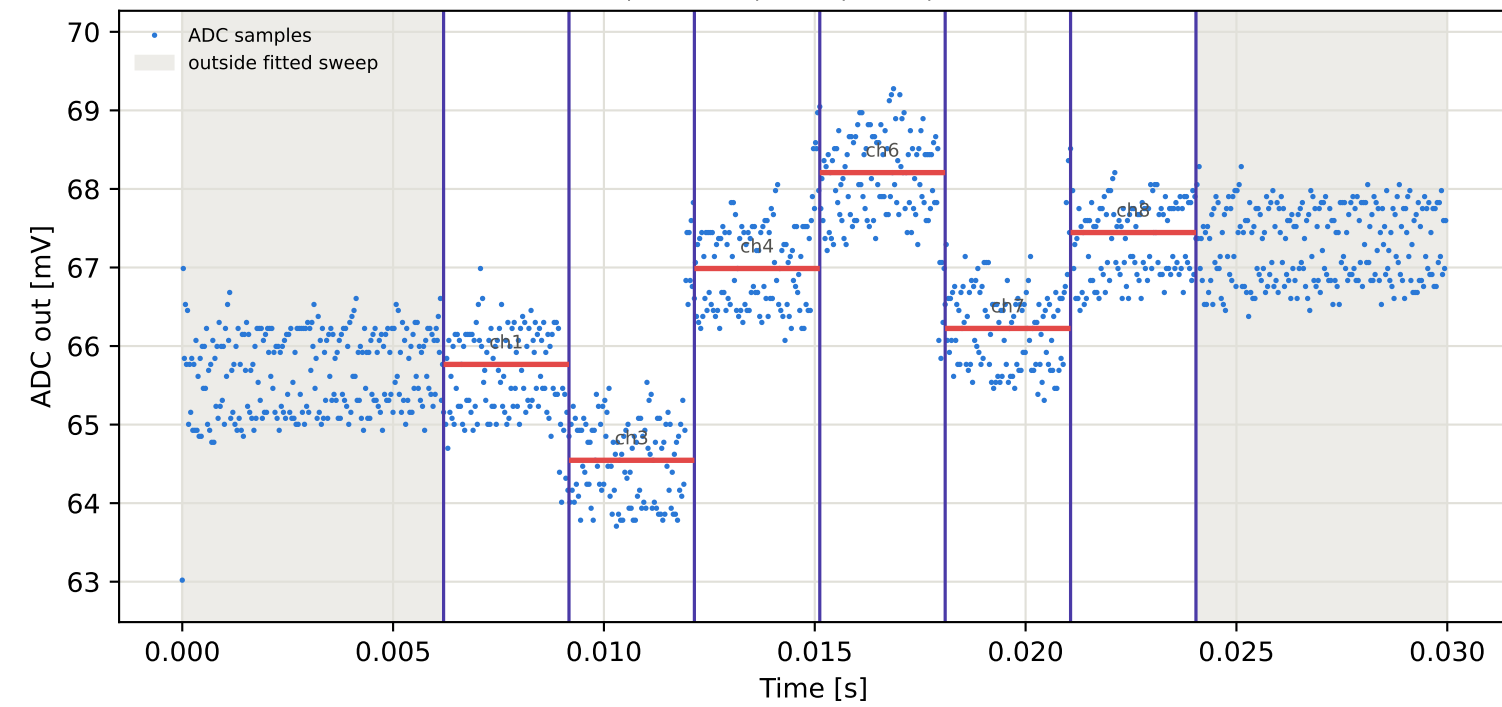
Tag1 &lt;- Tag9 | 795 MHz | run 0 | rep 1 | phase -145.67 deg
