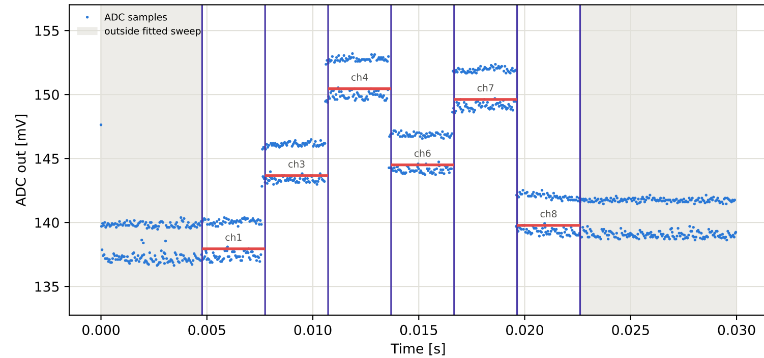
Tag4 &lt;- Tag9 | 805 MHz | run 0 | rep 1 | phase -132.93 deg
