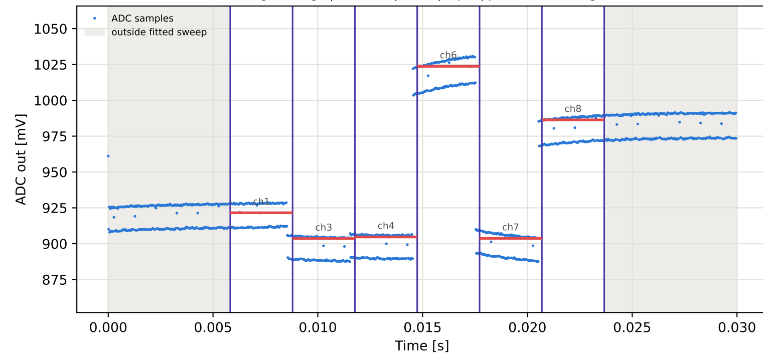
Tag4 &lt;- Tag7 | 925 MHz | run 0 | rep 1 | phase 112.45 deg
