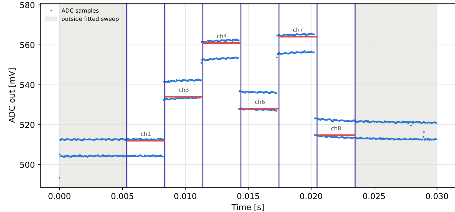
Tag8 &lt;- Tag16 | 825 MHz | run 0 | rep 1 | phase -74.64 deg
