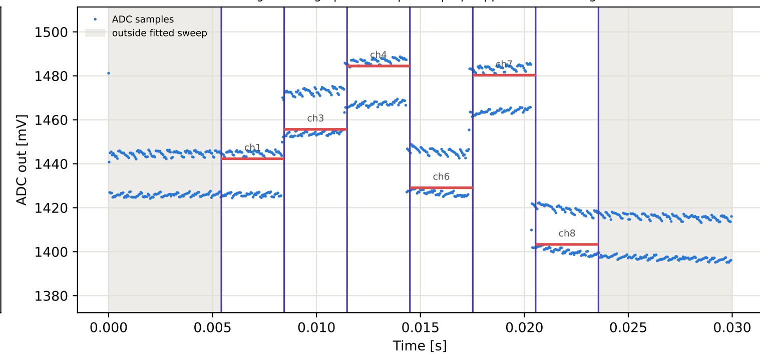
Tag2 &lt;- Tag10 | 905 MHz | run 0 | rep 1 | phase -27.39 deg
