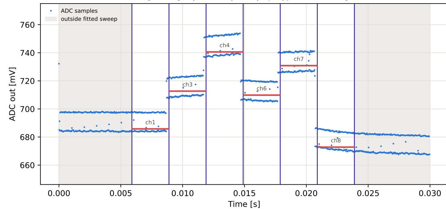
Tag7 &lt;- Tag3 | 925 MHz | run 0 | rep 1 | phase 10.61 deg
