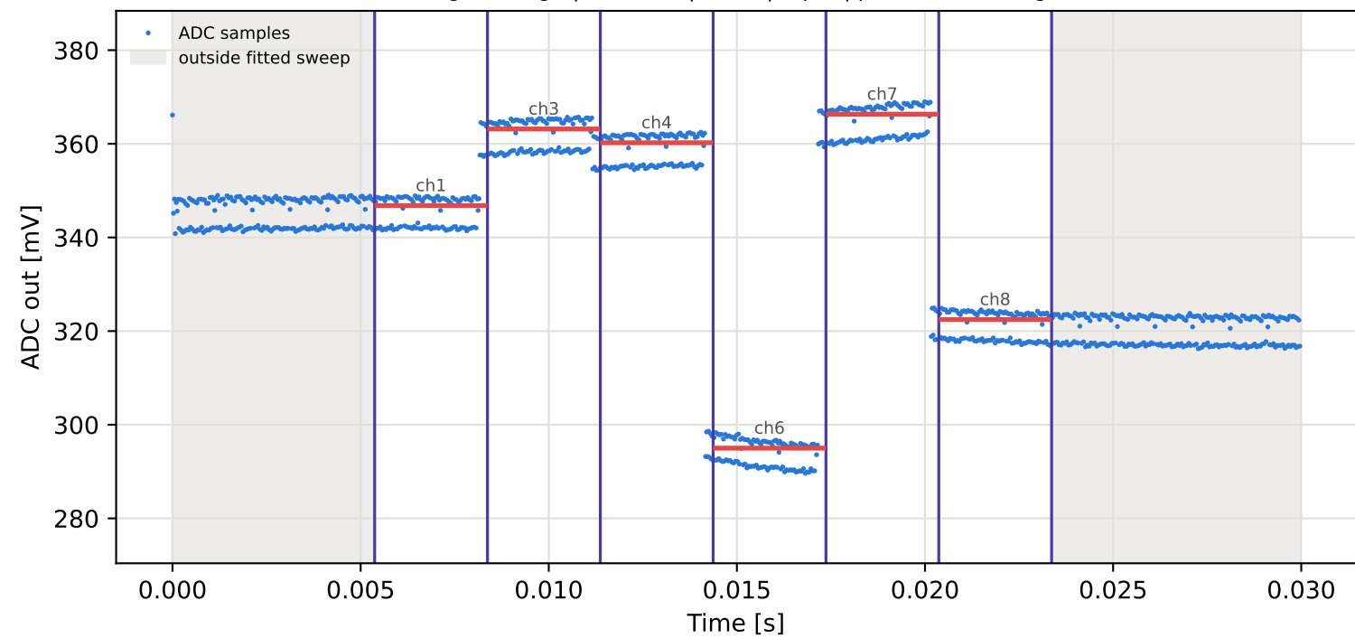
Tag3 &lt;- Tag6 | 975 MHz | run 0 | rep 1 | phase 155.19 deg
