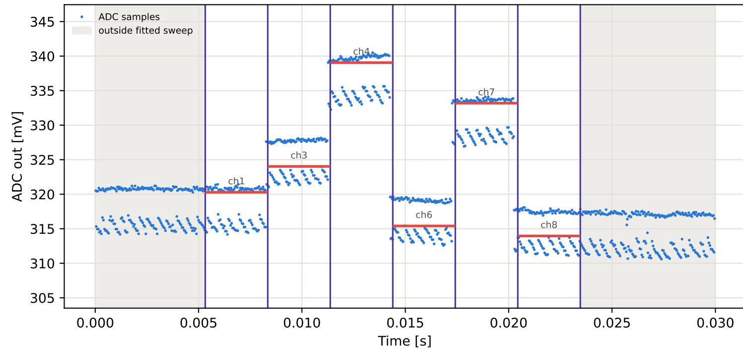
Tag16 &lt;- Tag7 | 995 MHz | run 0 | rep 1 | phase -168.29 deg
