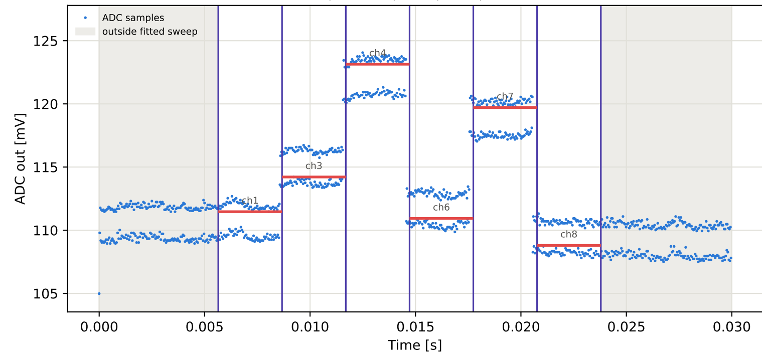
Tag2 &lt;- Tag16 | 975 MHz | run 0 | rep 1 | phase -83.32 deg
