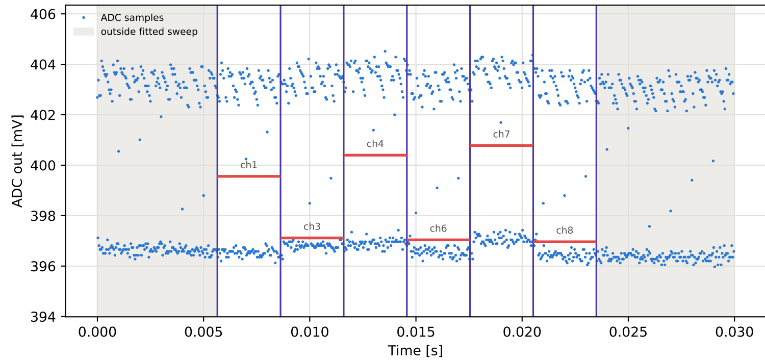
Tag15 &lt;- Tag9 | 845 MHz | run 0 | rep 1 | phase 167.27 deg
