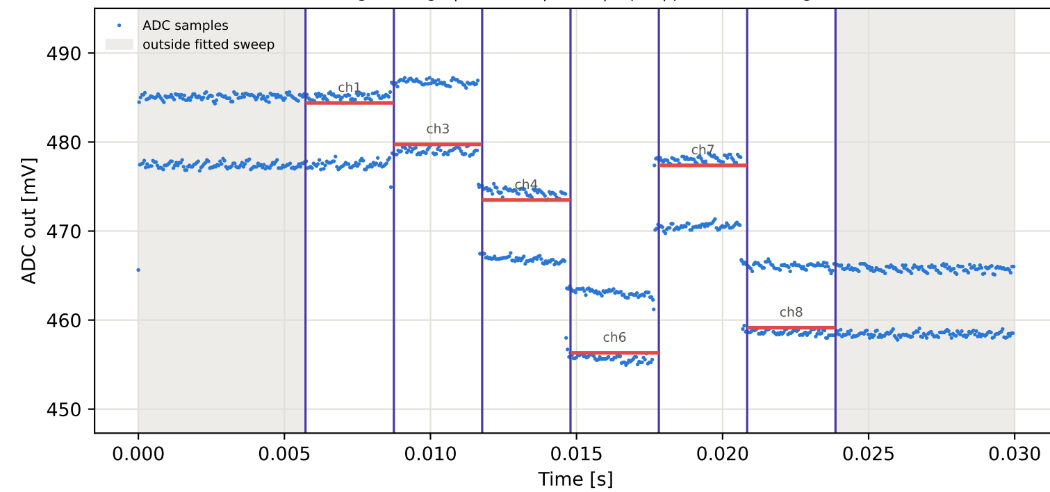
Tag9 &lt;- Tag5 | 855 MHz | run 0 | rep 1 | phase 179.24 deg
