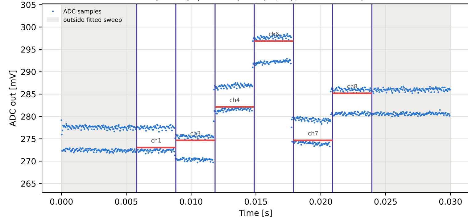
Tag3 &lt;- Tag8 | 965 MHz | run 0 | rep 1 | phase -42.99 deg
