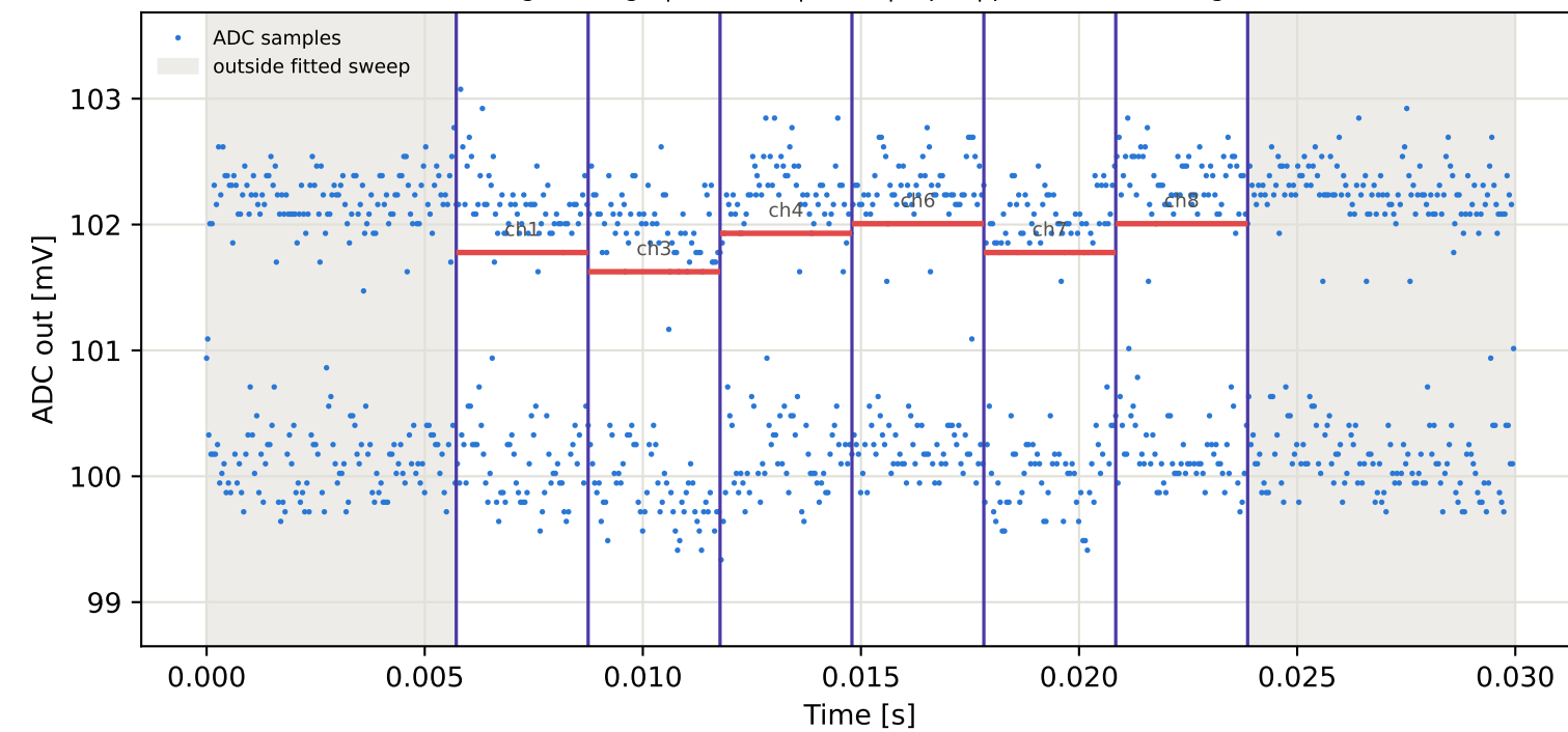
Tag4 &lt;- Tag15 | 775 MHz | run 0 | rep 1 | phase -155.29 deg
