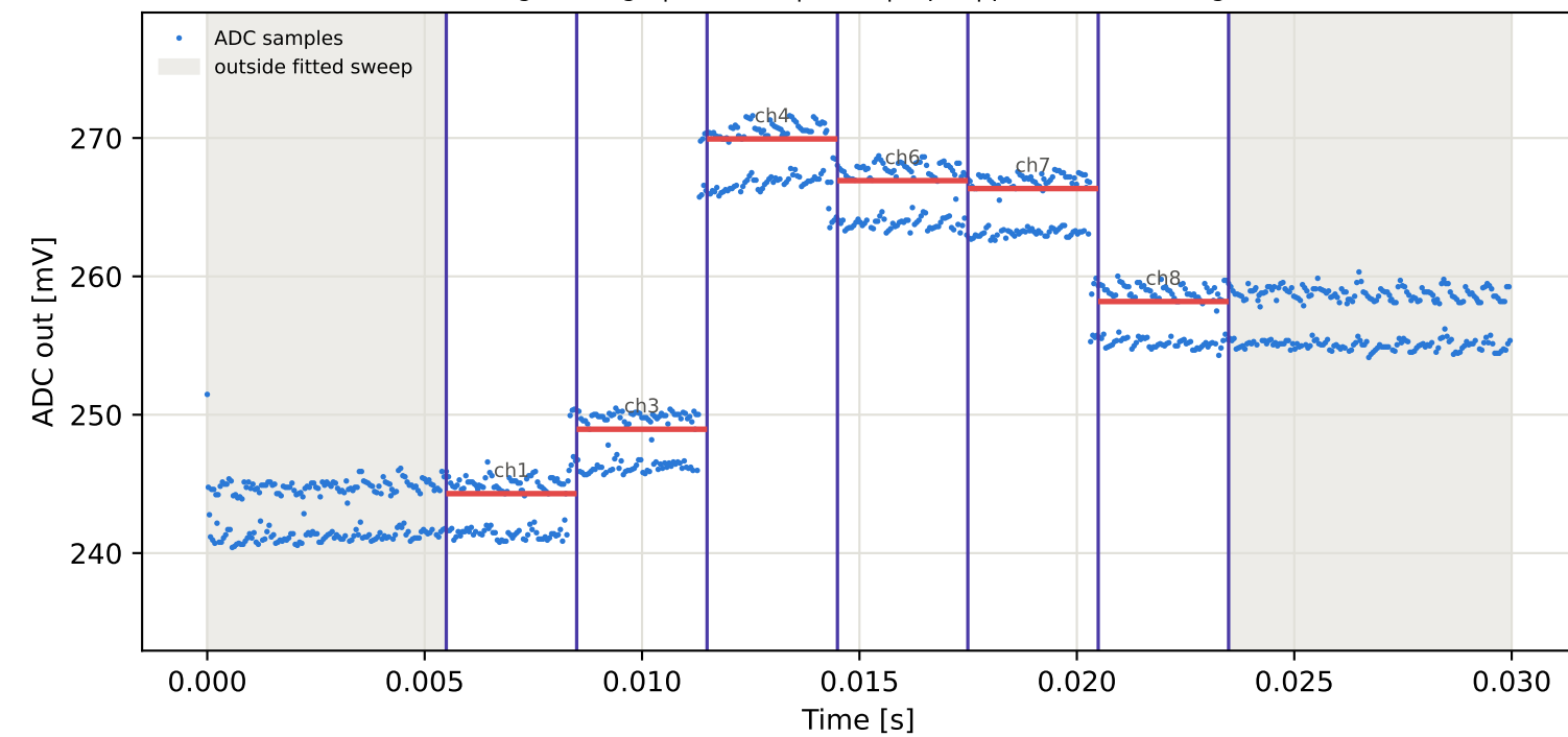
Tag8 &lt;- Tag1 | 825 MHz | run 0 | rep 1 | phase 79.60 deg
