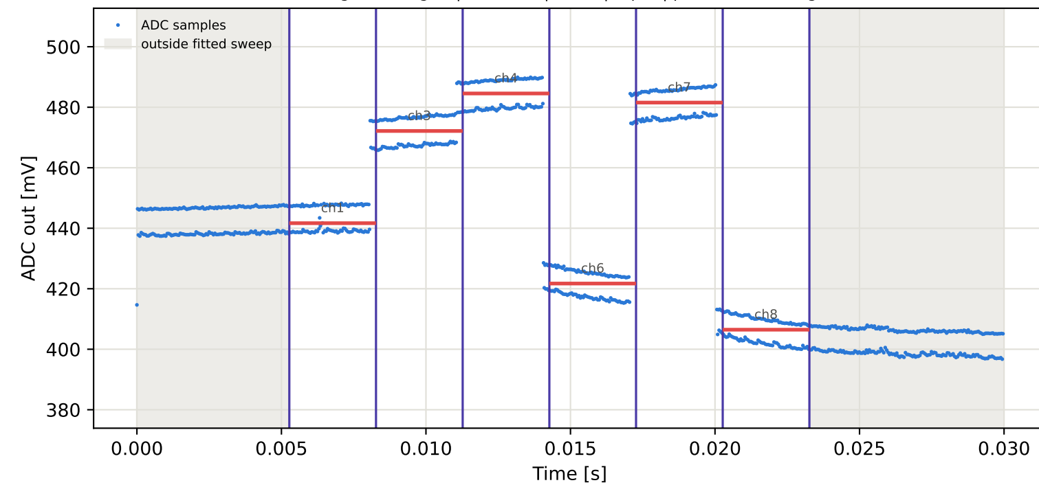
Tag10 &lt;- Tag2 | 915 MHz | run 0 | rep 1 | phase 118.89 deg
