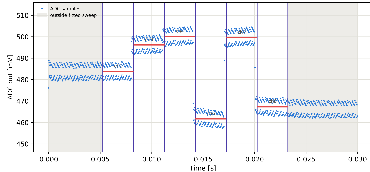
Tag1 &lt;- Tag9 | 945 MHz | run 0 | rep 1 | phase -28.82 deg
