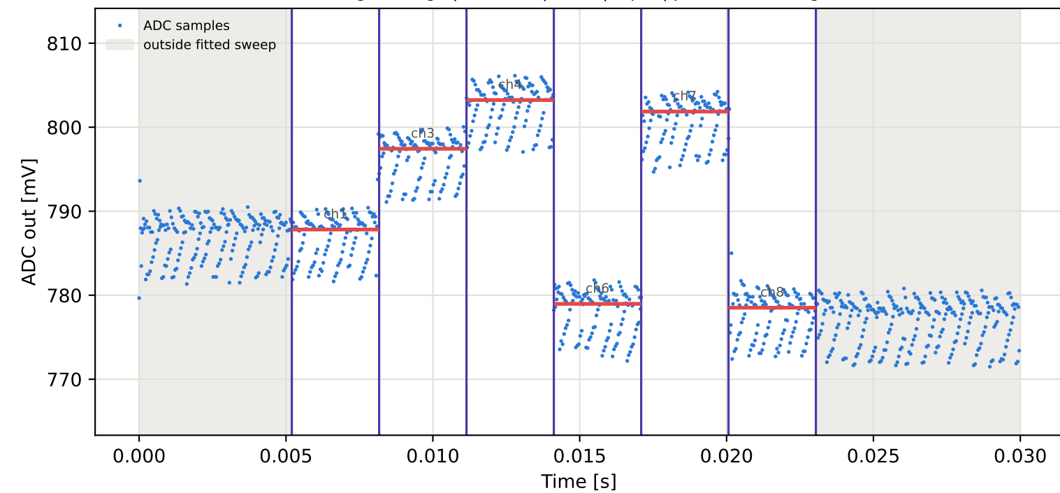
Tag4 &lt;- Tag15 | 935 MHz | run 0 | rep 1 | phase 15.45 deg
