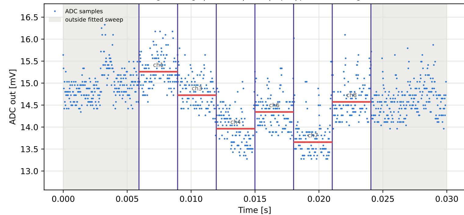
Tag15 &lt;- Tag1 | 795 MHz | run 0 | rep 1 | phase -114.72 deg
