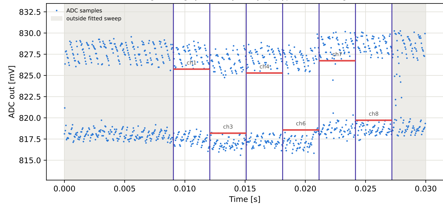
Tag15 &lt;- Tag4 | 875 MHz | run 0 | rep 1 | phase -3.81 deg
