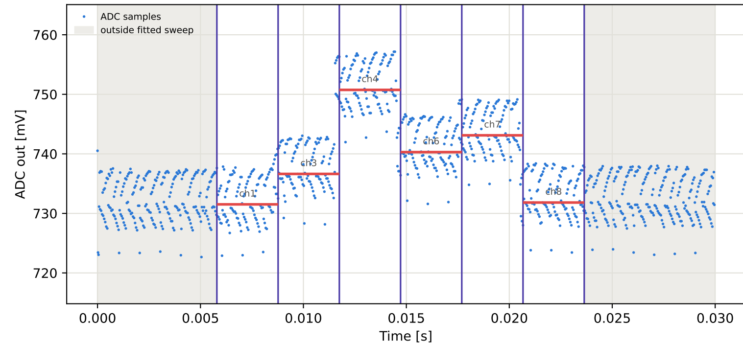
Tag8 &lt;- Tag6 | 965 MHz | run 0 | rep 1 | phase -40.81 deg
