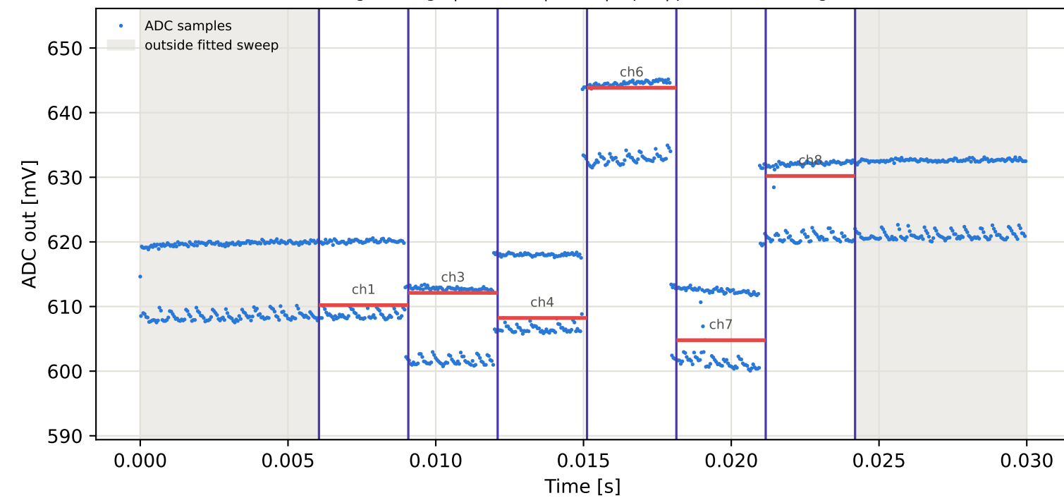
Tag4 &lt;- Tag7 | 985 MHz | run 0 | rep 1 | phase -52.99 deg
