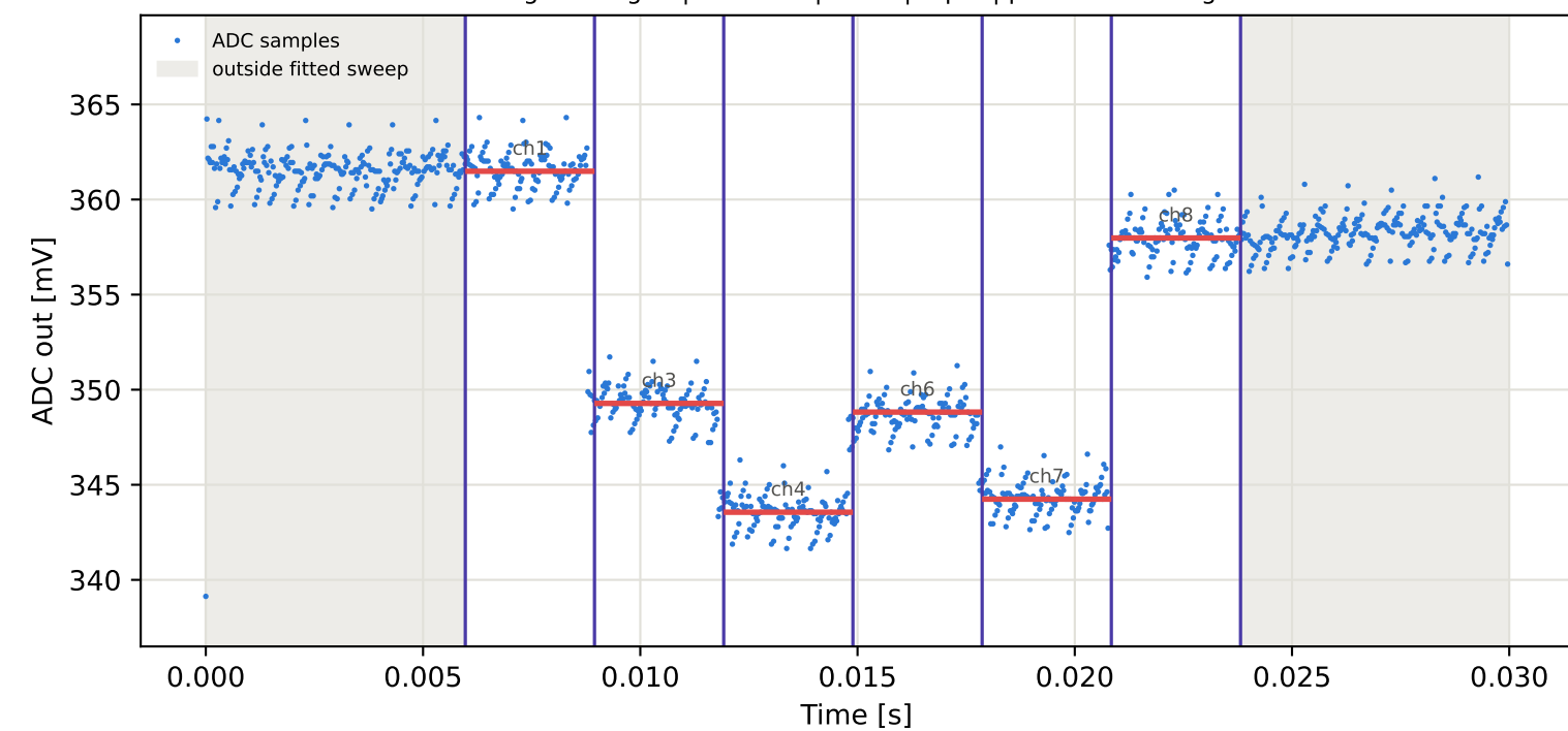
Tag7 &lt;- Tag10 | 865 MHz | run 0 | rep 1 | phase 87.93 deg
