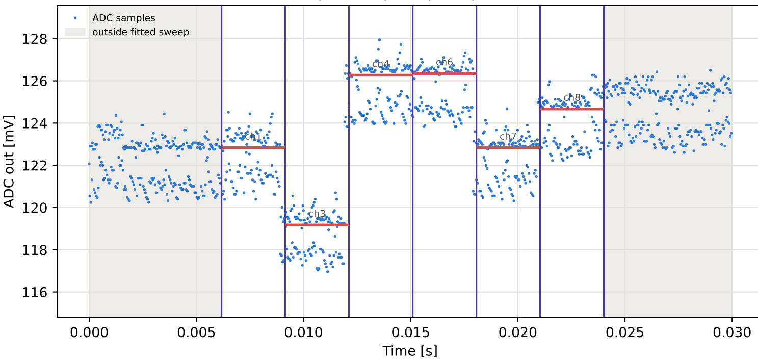
Tag7 &lt;- Tag10 | 775 MHz | run 0 | rep 1 | phase -133.14 deg
