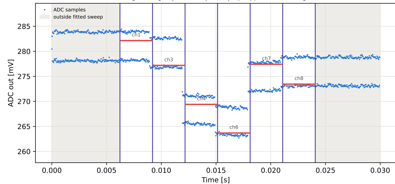
Tag3 &lt;- Tag16 | 965 MHz | run 0 | rep 1 | phase 31.23 deg
