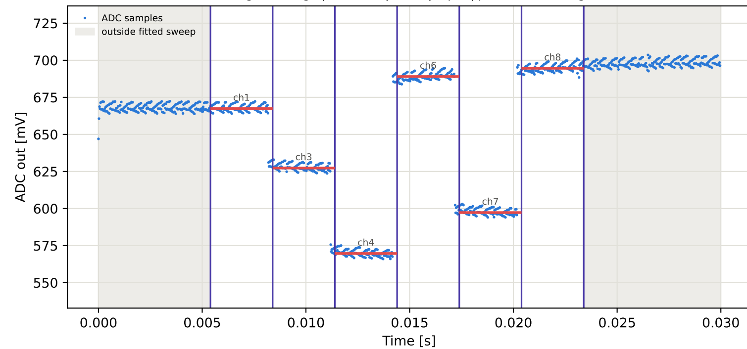
Tag2 &lt;- Tag1 | 955 MHz | run 0 | rep 1 | phase -132.63 deg
