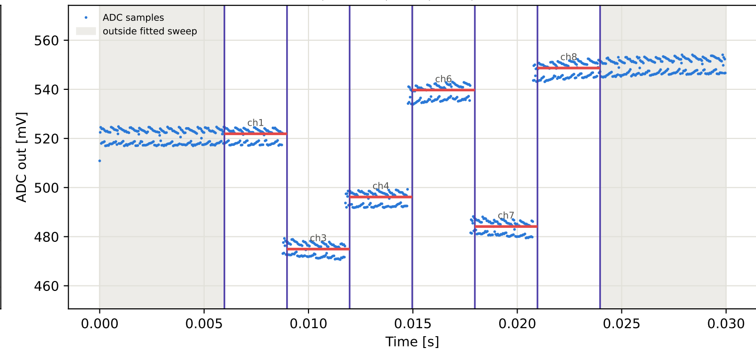
Tag9 &lt;- Tag8 | 845 MHz | run 0 | rep 1 | phase 164.57 deg
