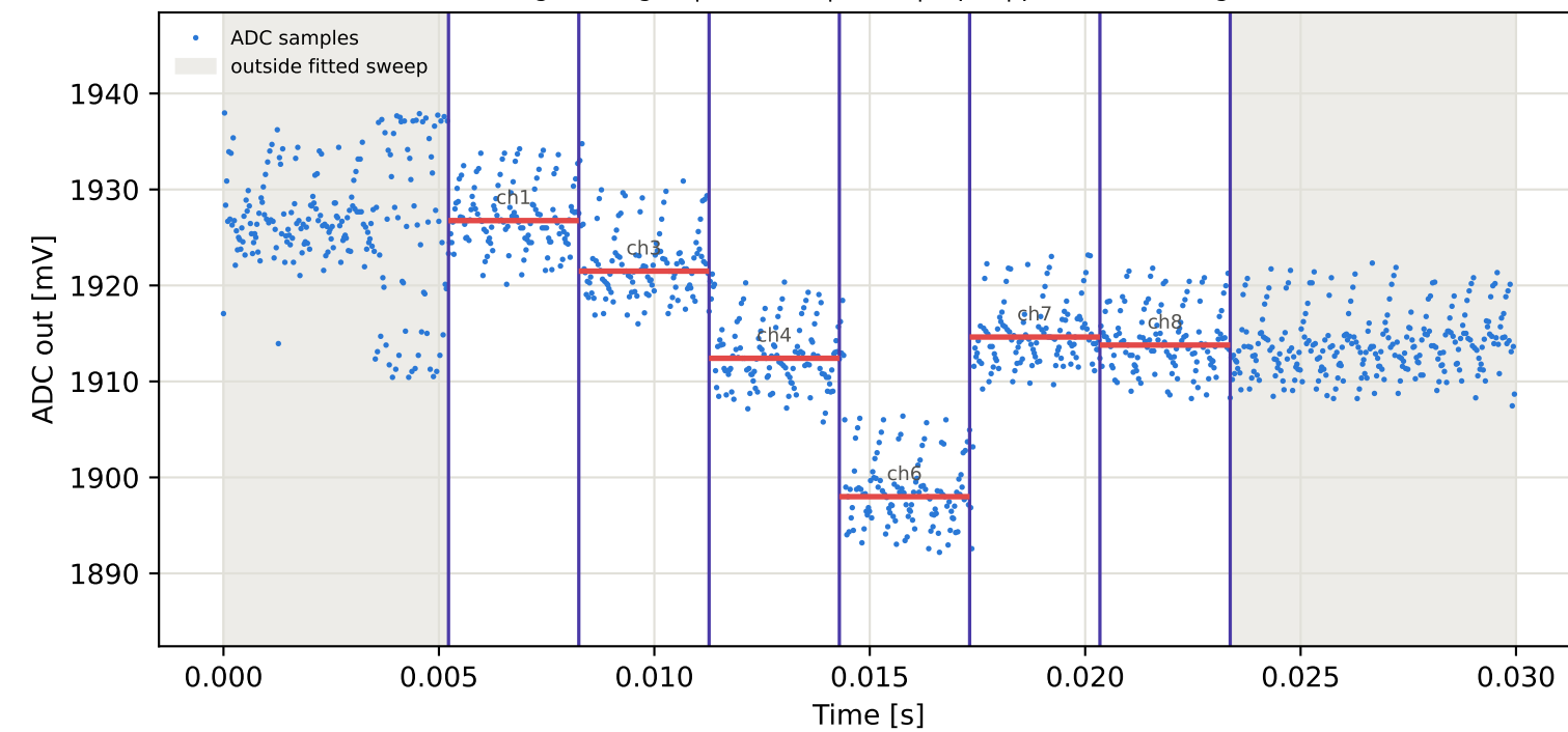
Tag5 &lt;- Tag16 | 895 MHz | run 0 | rep 1 | phase -95.12 deg
