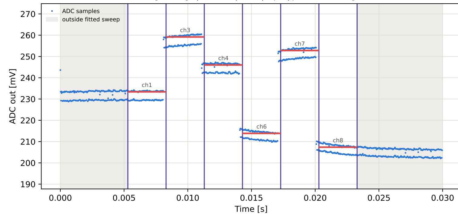
Tag8 &lt;- Tag1 | 855 MHz | run 0 | rep 1 | phase 103.69 deg
