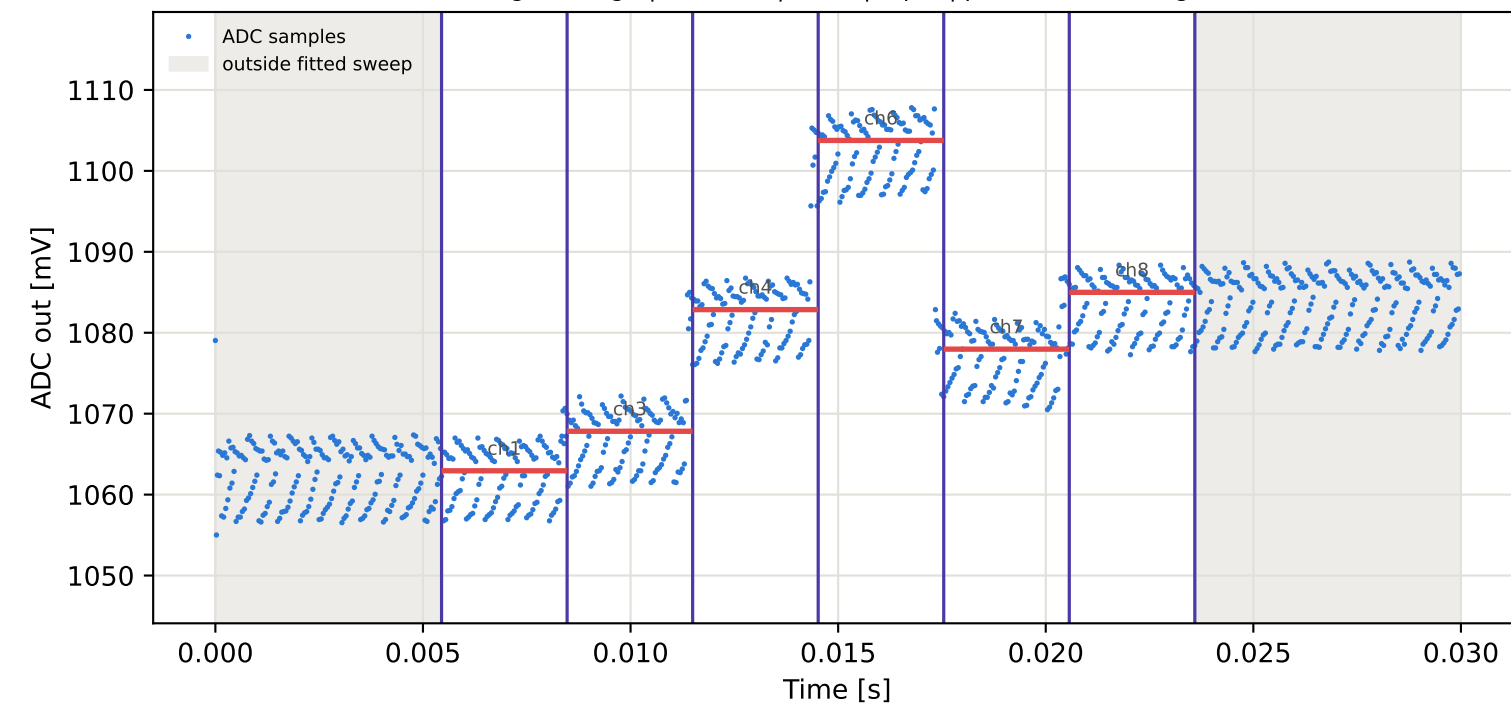
Tag4 &lt;- Tag15 | 895 MHz | run 0 | rep 1 | phase -38.28 deg
