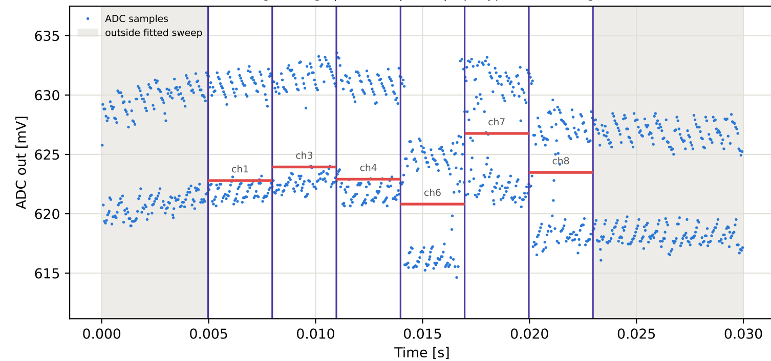
Tag8 &lt;- Tag1 | 905 MHz | run 0 | rep 1 | phase 23.66 deg
