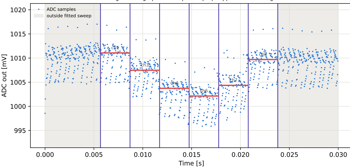
Tag15 &lt;- Tag1 | 905 MHz | run 0 | rep 1 | phase 59.21 deg
