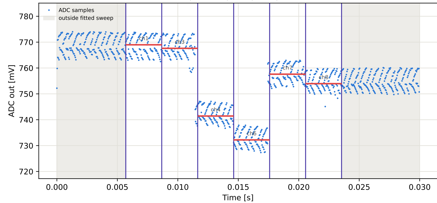
Tag16 &lt;- Tag7 | 965 MHz | run 0 | rep 1 | phase 33.11 deg
