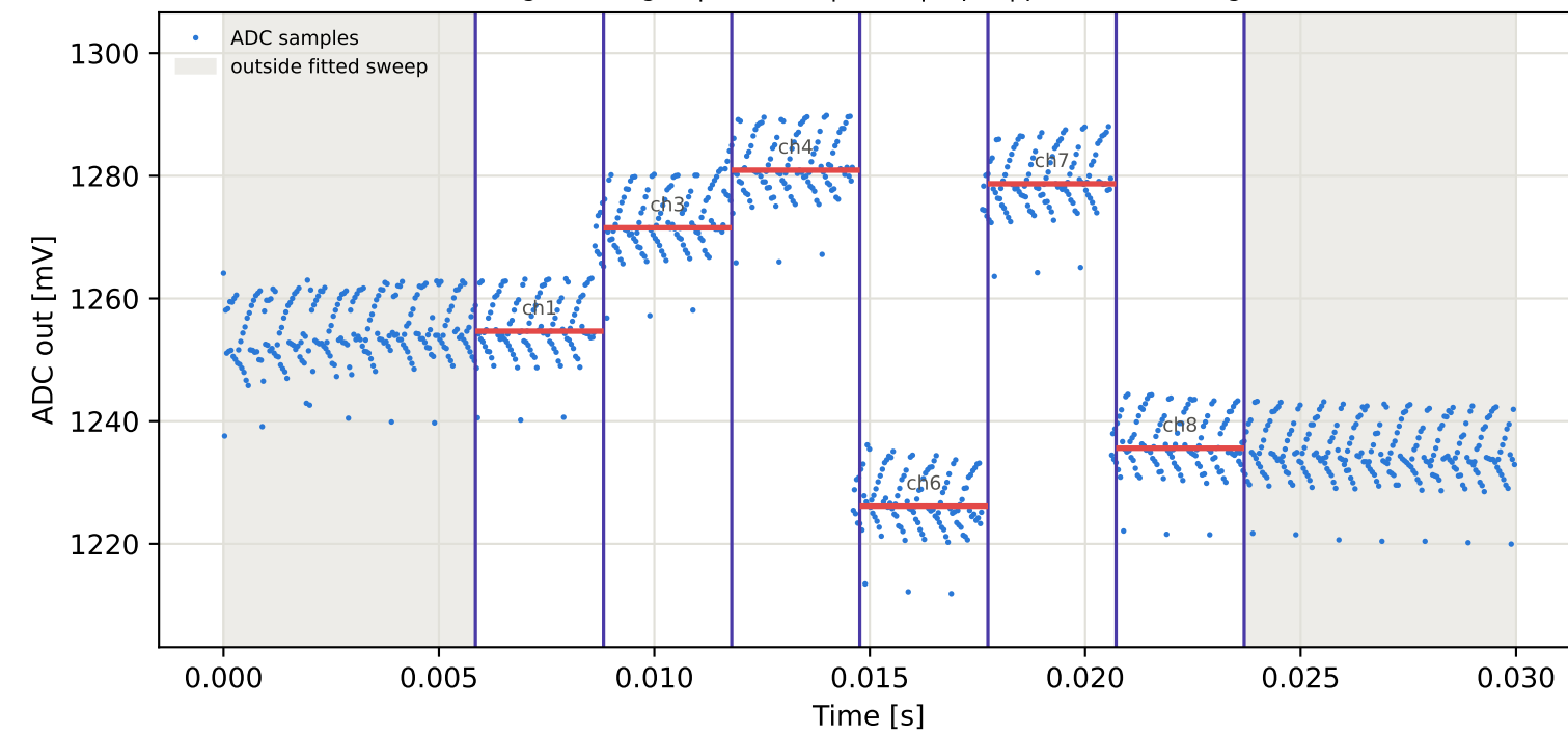
Tag15 &lt;- Tag3 | 945 MHz | run 0 | rep 1 | phase -43.39 deg
