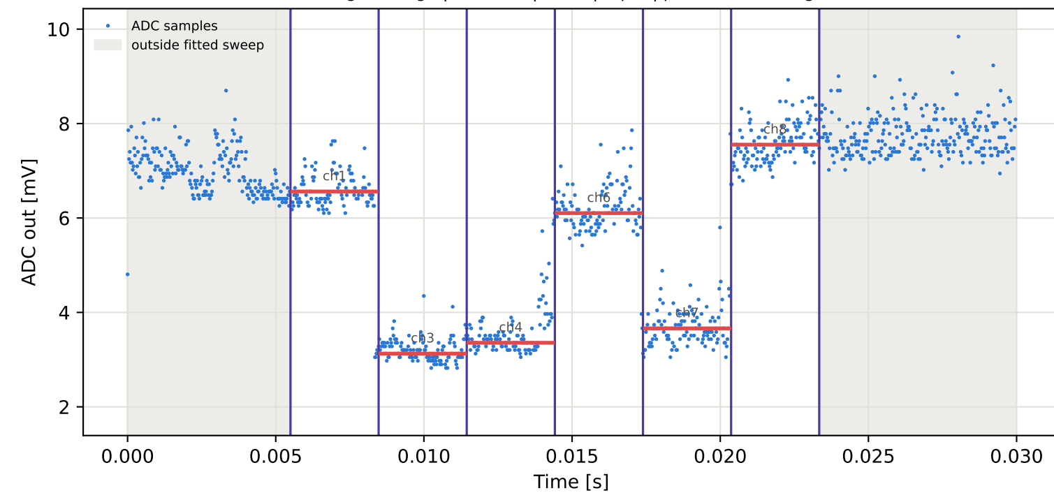
Tag7 &lt;- Tag5 | 845 MHz | run 0 | rep 1 | phase -128.34 deg
