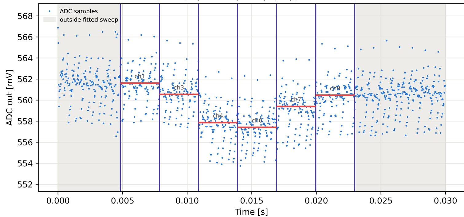
Tag5 &lt;- Tag9 | 945 MHz | run 0 | rep 1 | phase 123.29 deg
