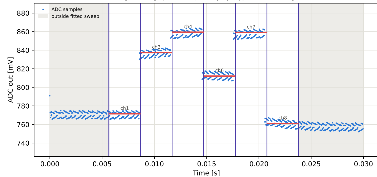
Tag15 &lt;- Tag5 | 875 MHz | run 0 | rep 1 | phase -77.10 deg
