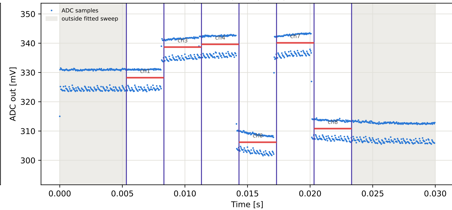
Tag3 &lt;- Tag9 | 925 MHz | run 0 | rep 1 | phase -21.21 deg
