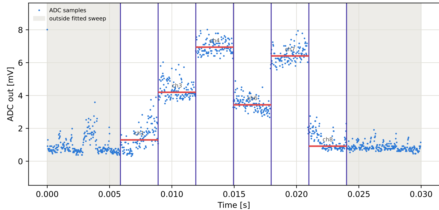
Tag8 &lt;- Tag10 | 845 MHz | run 0 | rep 1 | phase -113.16 deg
