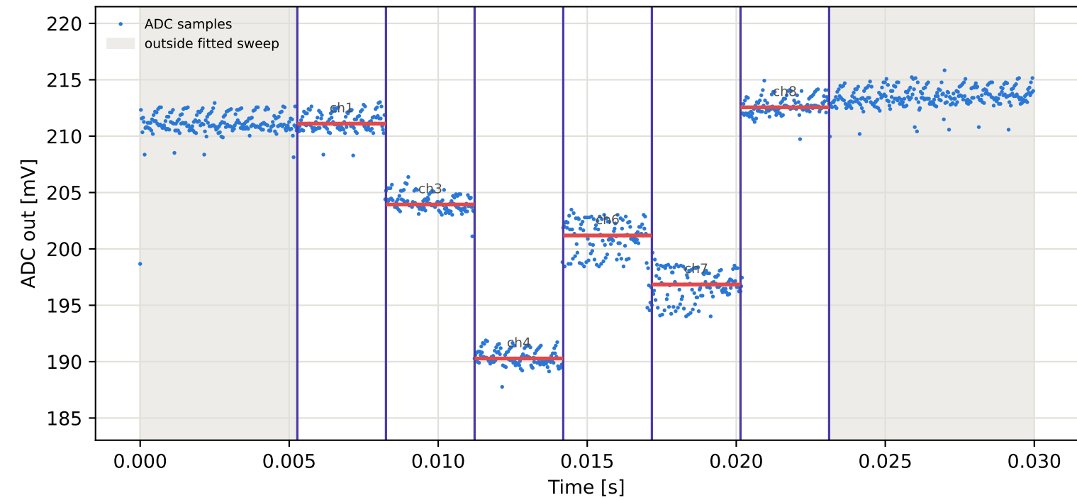
Tag10 &lt;- Tag5 | 945 MHz | run 0 | rep 1 | phase -120.27 deg
