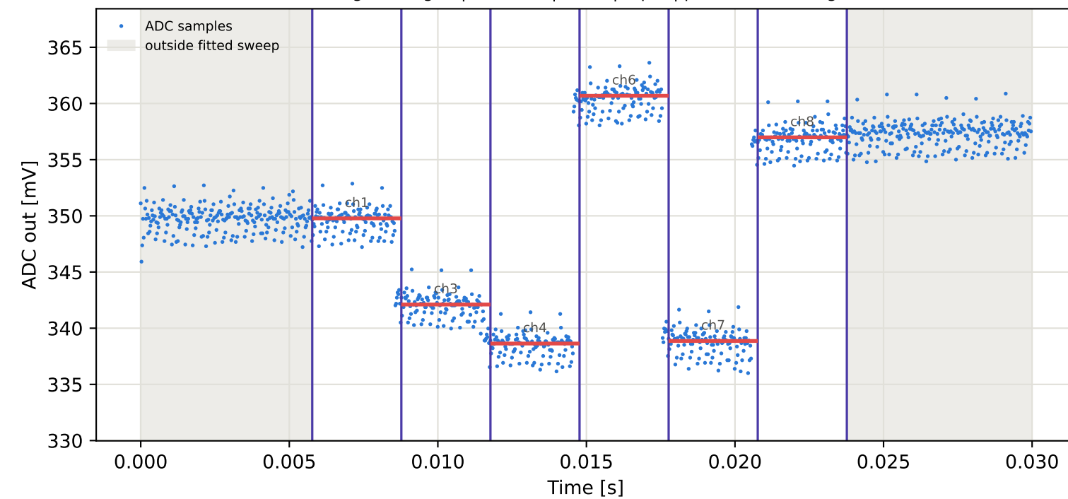
Tag1 &lt;- Tag3 | 975 MHz | run 0 | rep 1 | phase -69.23 deg
