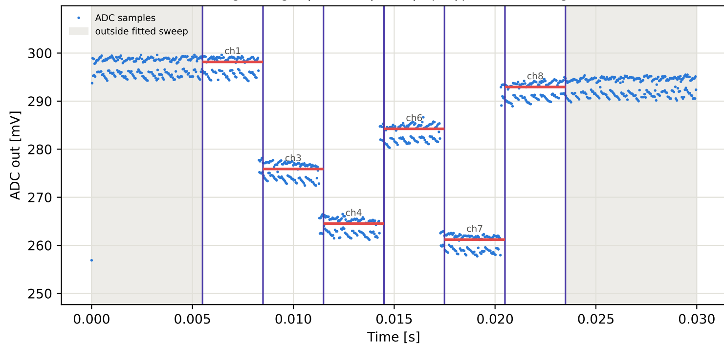
Tag7 &lt;- Tag3 | 825 MHz | run 0 | rep 1 | phase -173.88 deg
