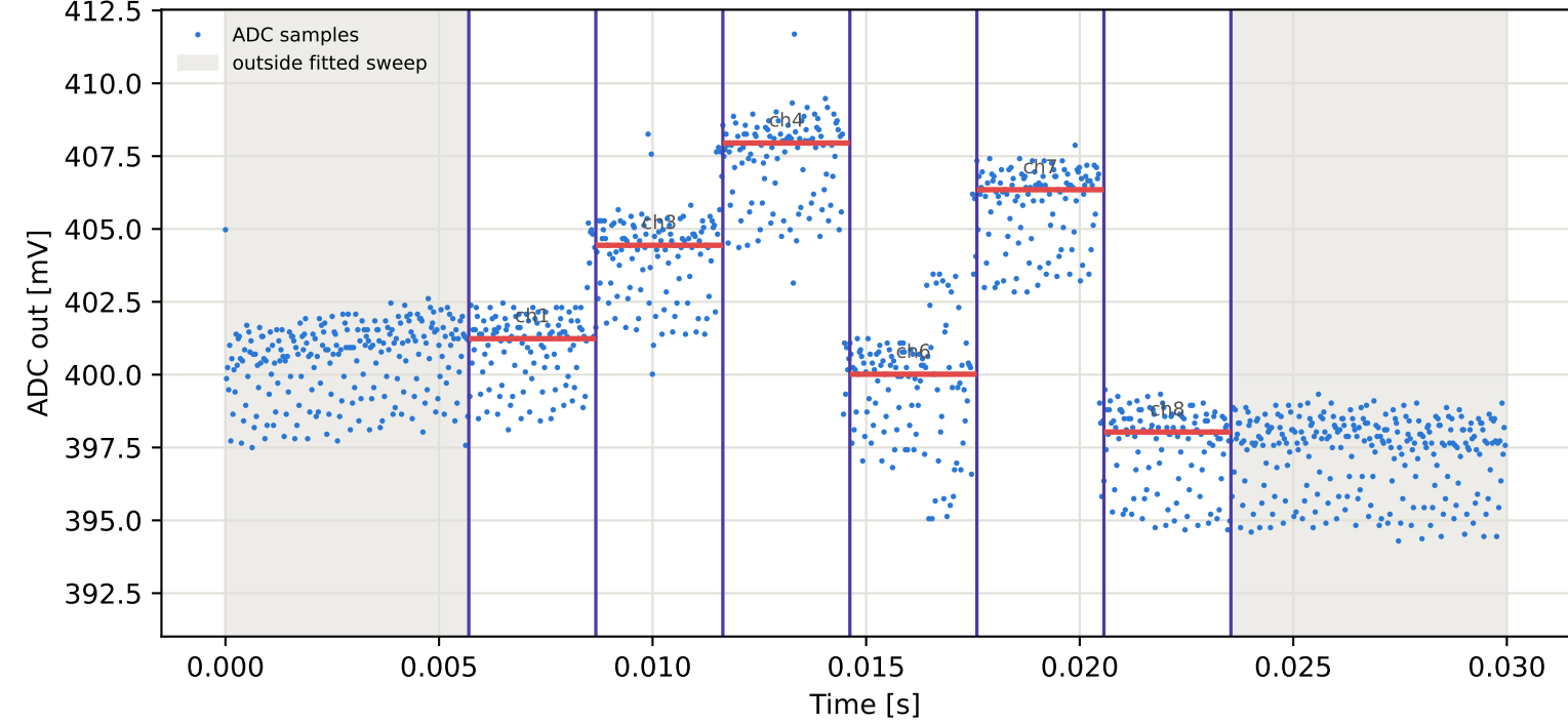
Tag1 &lt;- Tag4 | 935 MHz | run 0 | rep 1 | phase -77.93 deg
