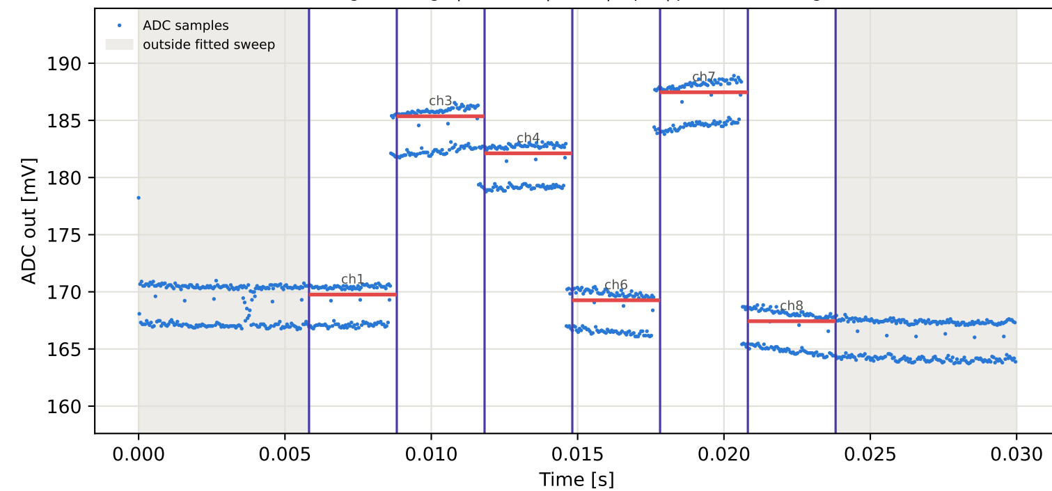
Tag2 &lt;- Tag1 | 805 MHz | run 0 | rep 1 | phase -71.81 deg
