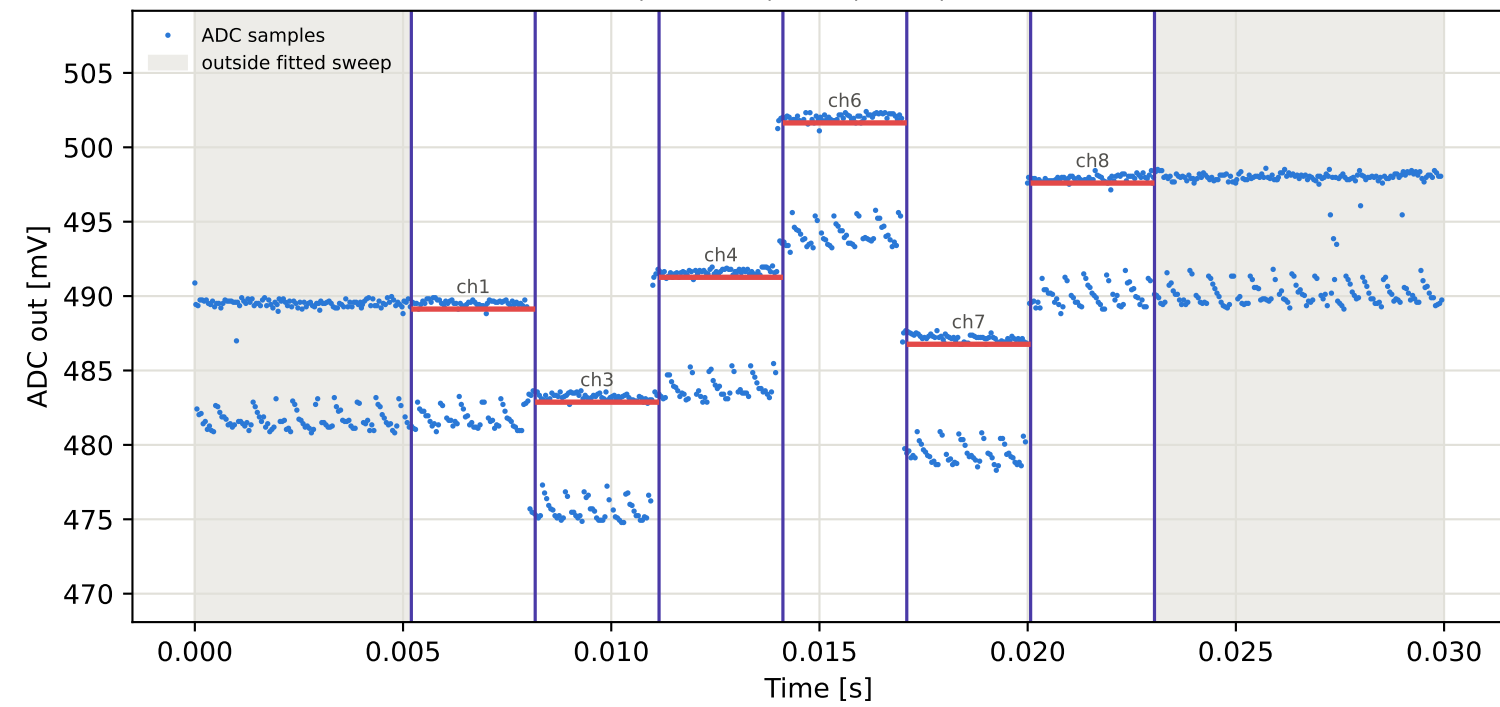
Tag16 &lt;- Tag7 | 835 MHz | run 0 | rep 1 | phase -164.47 deg
