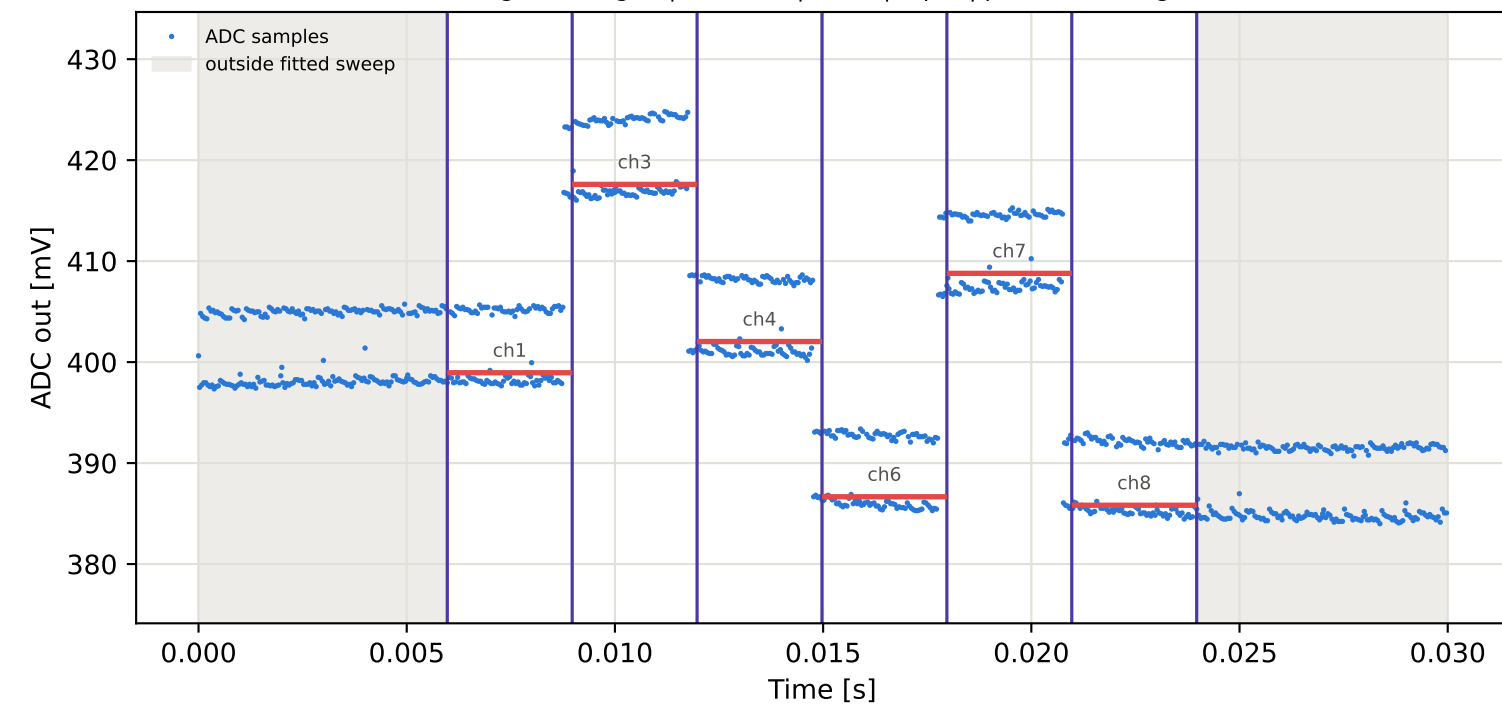
Tag15 &lt;- Tag3 | 845 MHz | run 0 | rep 1 | phase -18.22 deg
