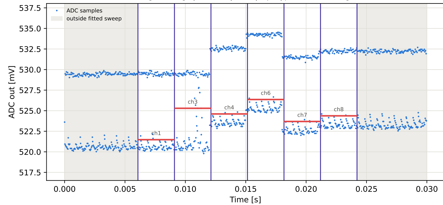
Tag15 &lt;- Tag4 | 835 MHz | run 0 | rep 1 | phase -174.76 deg
