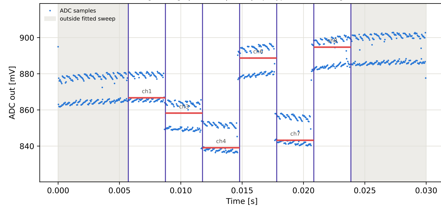
Tag5 &lt;- Tag8 | 915 MHz | run 0 | rep 1 | phase -173.75 deg
