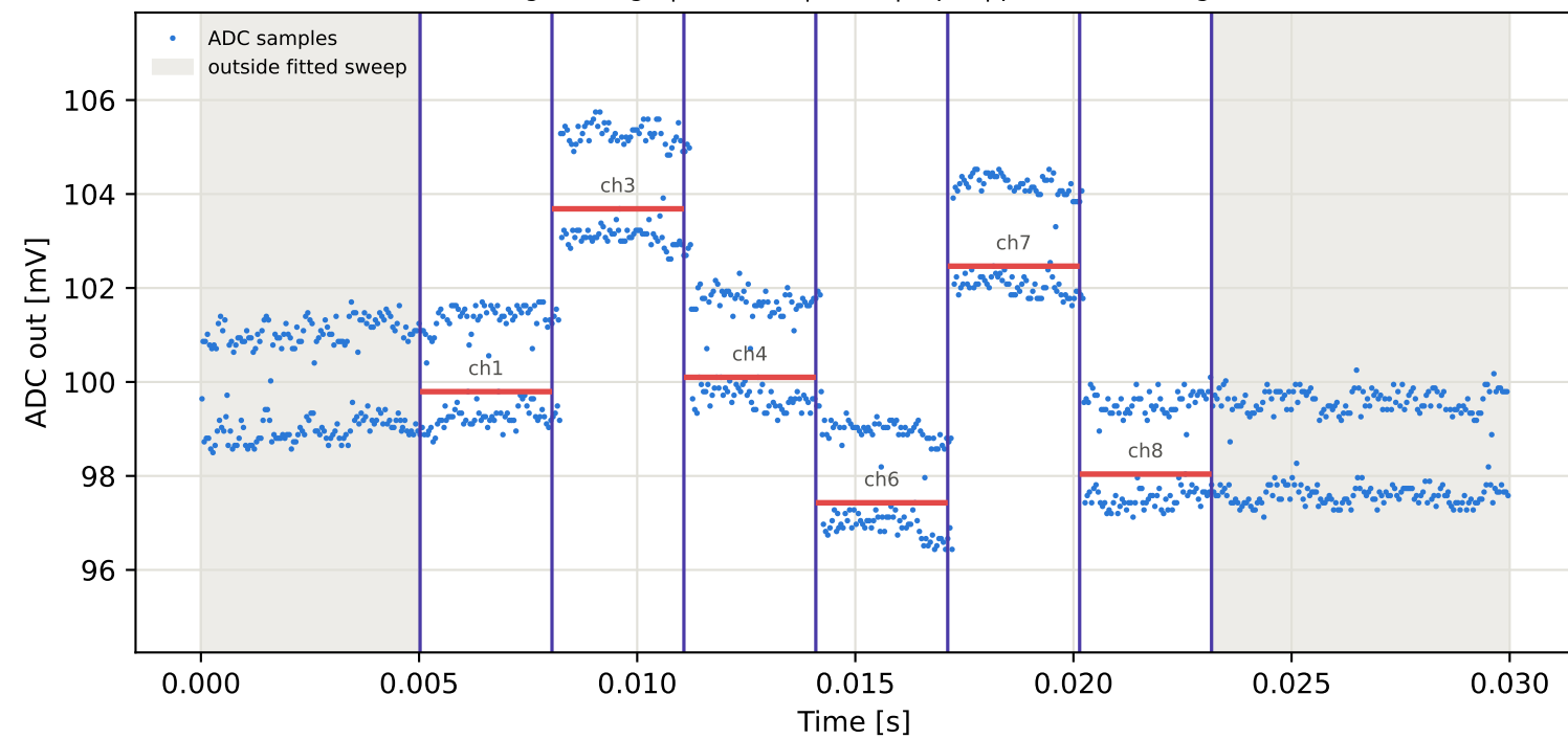
Tag4 &lt;- Tag8 | 775 MHz | run 0 | rep 1 | phase -100.38 deg
