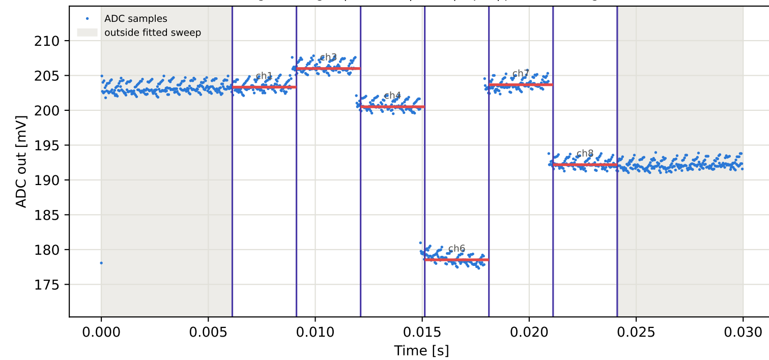
Tag10 &lt;- Tag2 | 945 MHz | run 0 | rep 1 | phase -51.34 deg
