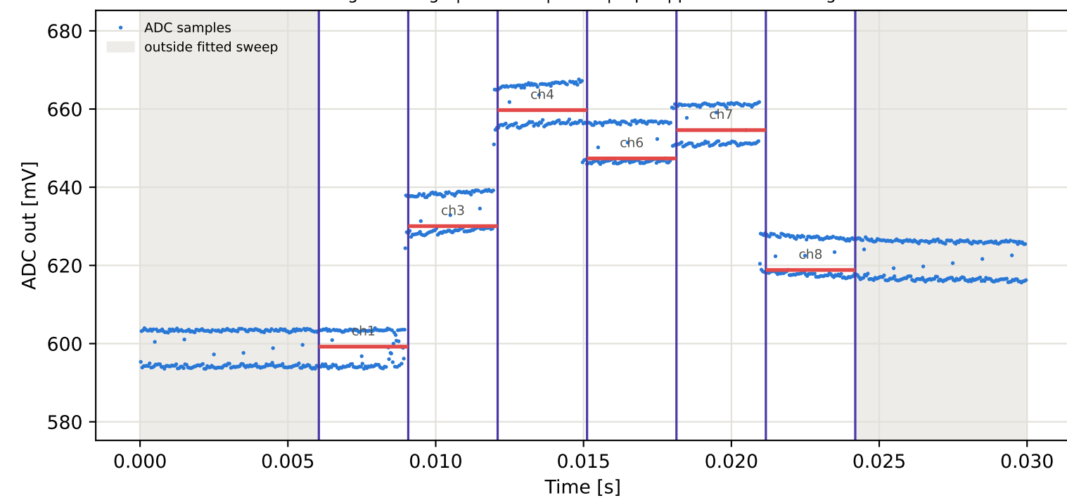
Tag15 &lt;- Tag5 | 865 MHz | run 0 | rep 1 | phase -106.17 deg
