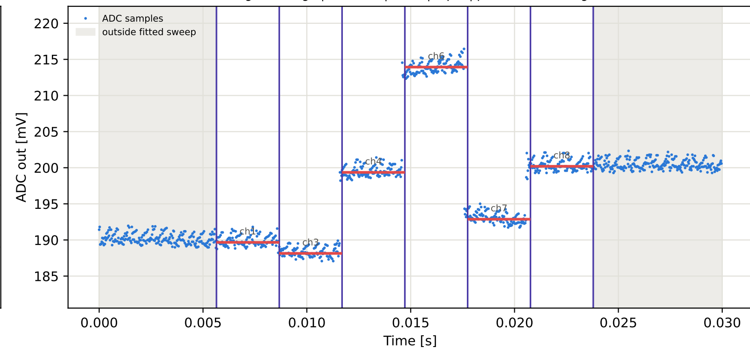
Tag10 &lt;- Tag1 | 955 MHz | run 0 | rep 1 | phase -159.80 deg
