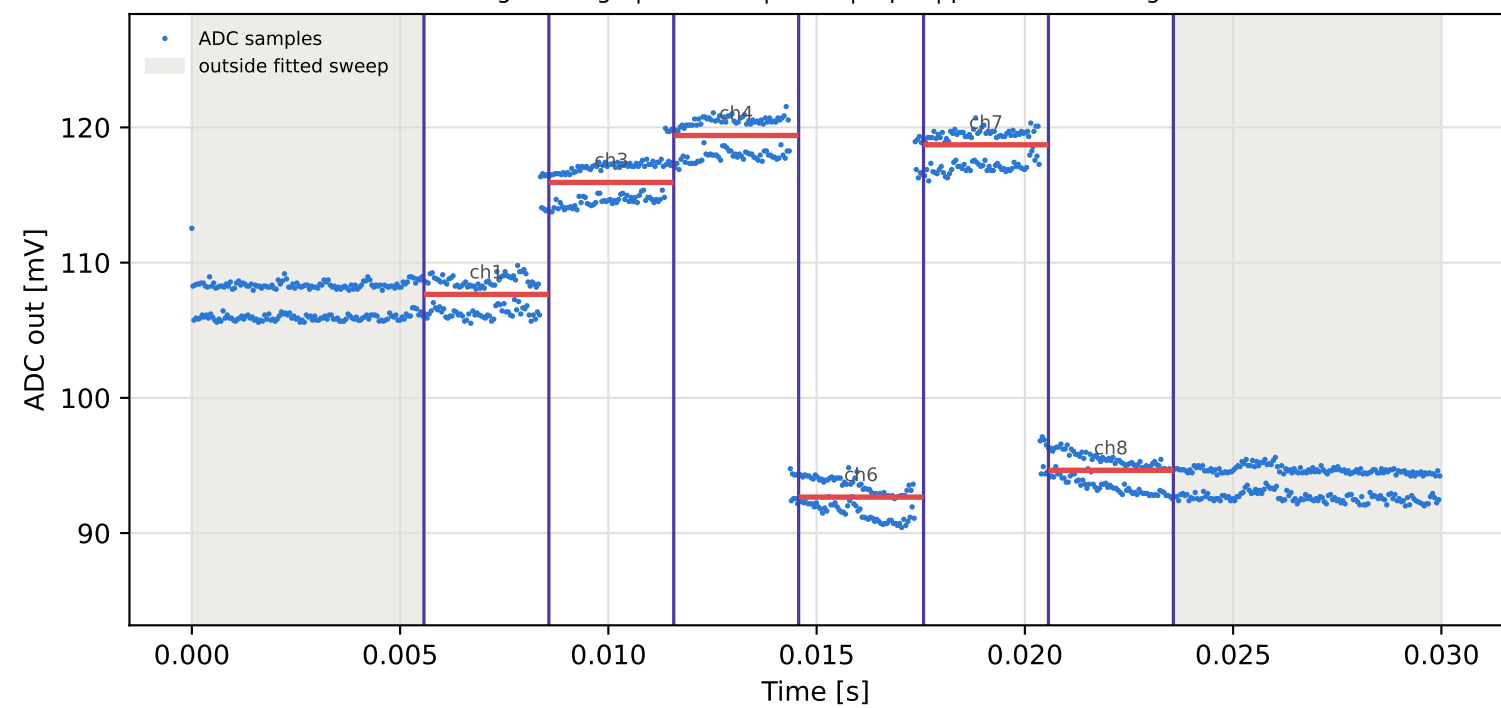
Tag2 &lt;- Tag6 | 915 MHz | run 0 | rep 1 | phase -145.03 deg
