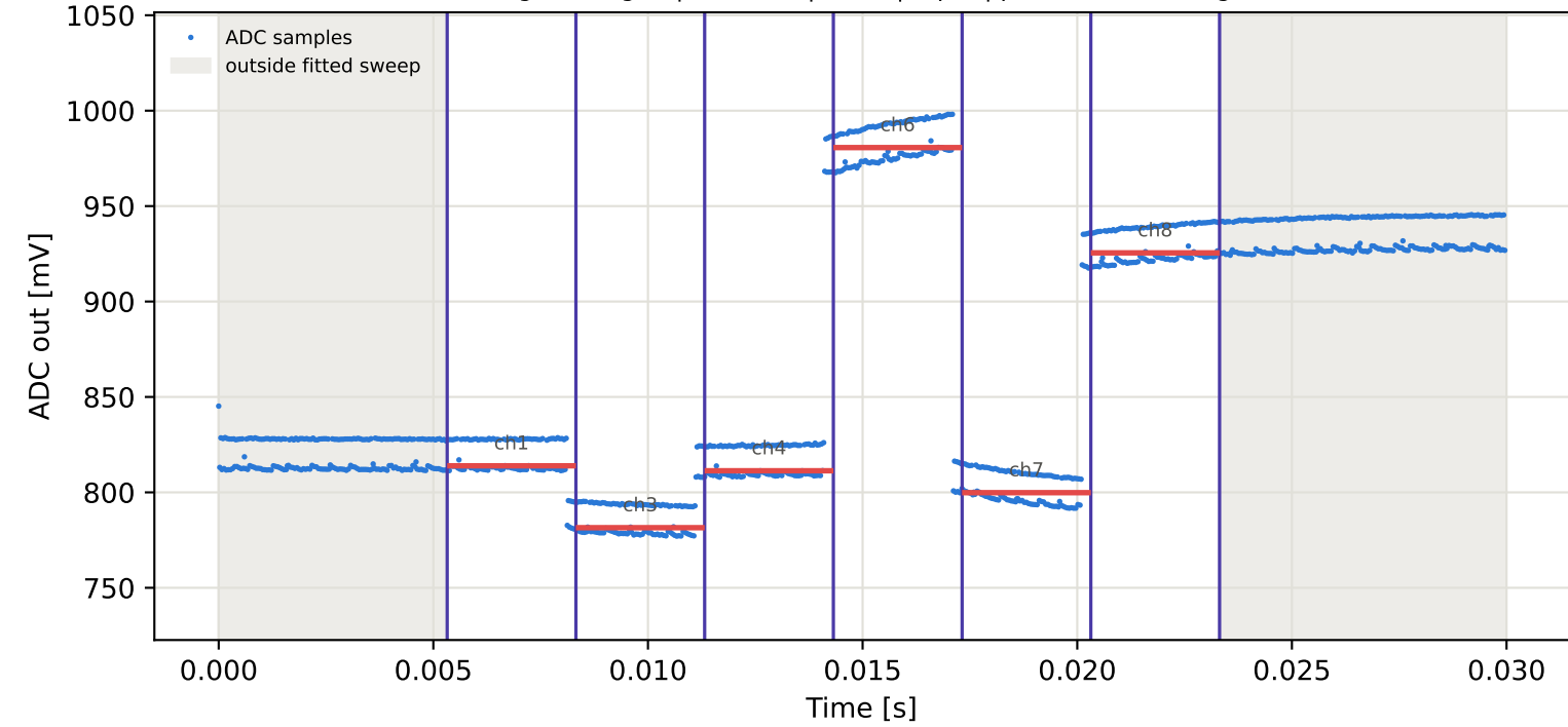
Tag5 &lt;- Tag2 | 915 MHz | run 0 | rep 1 | phase 174.58 deg
