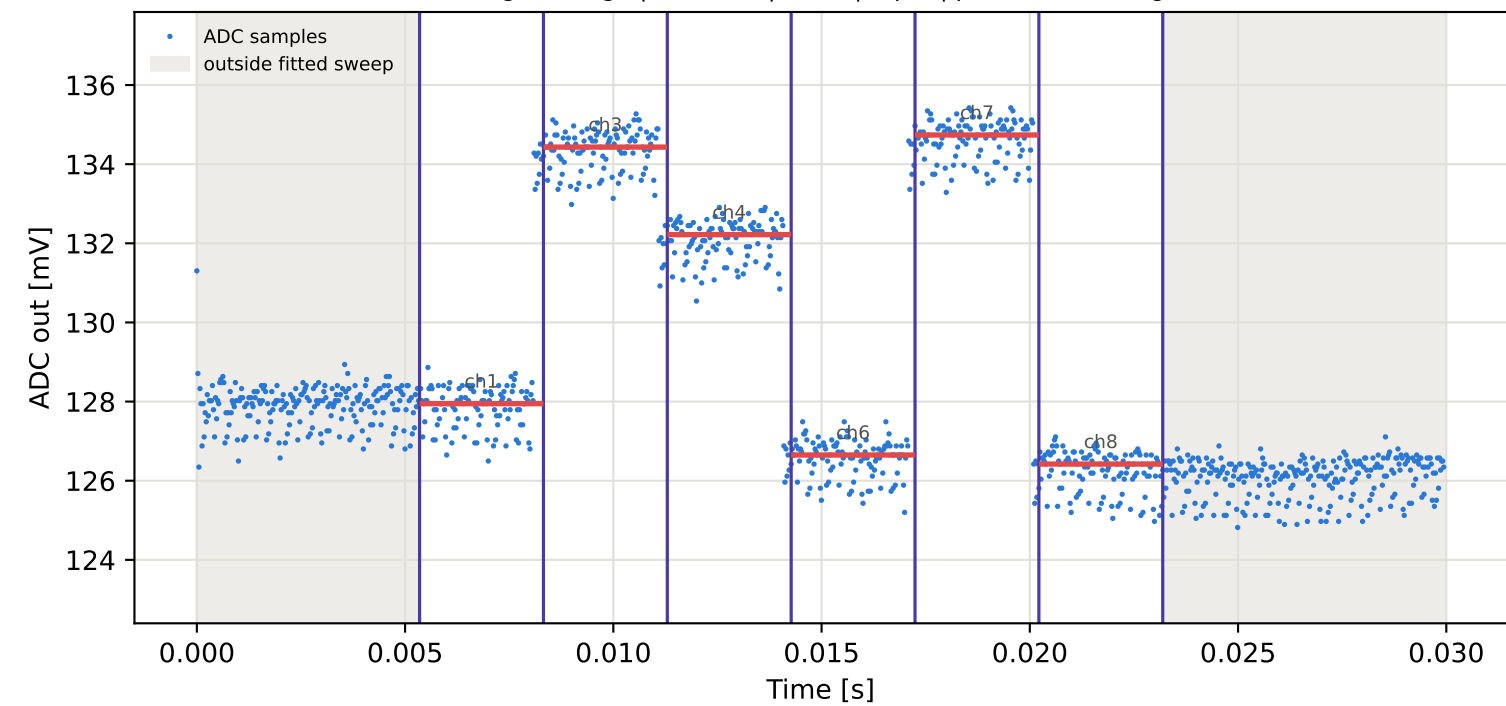
Tag3 &lt;- Tag7 | 785 MHz | run 0 | rep 1 | phase -52.72 deg
