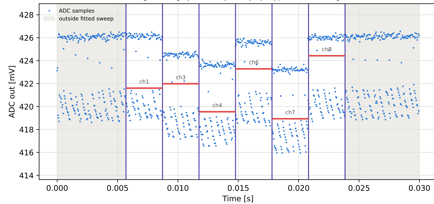
Tag15 &lt;- Tag1 | 825 MHz | run 0 | rep 1 | phase 130.42 deg
