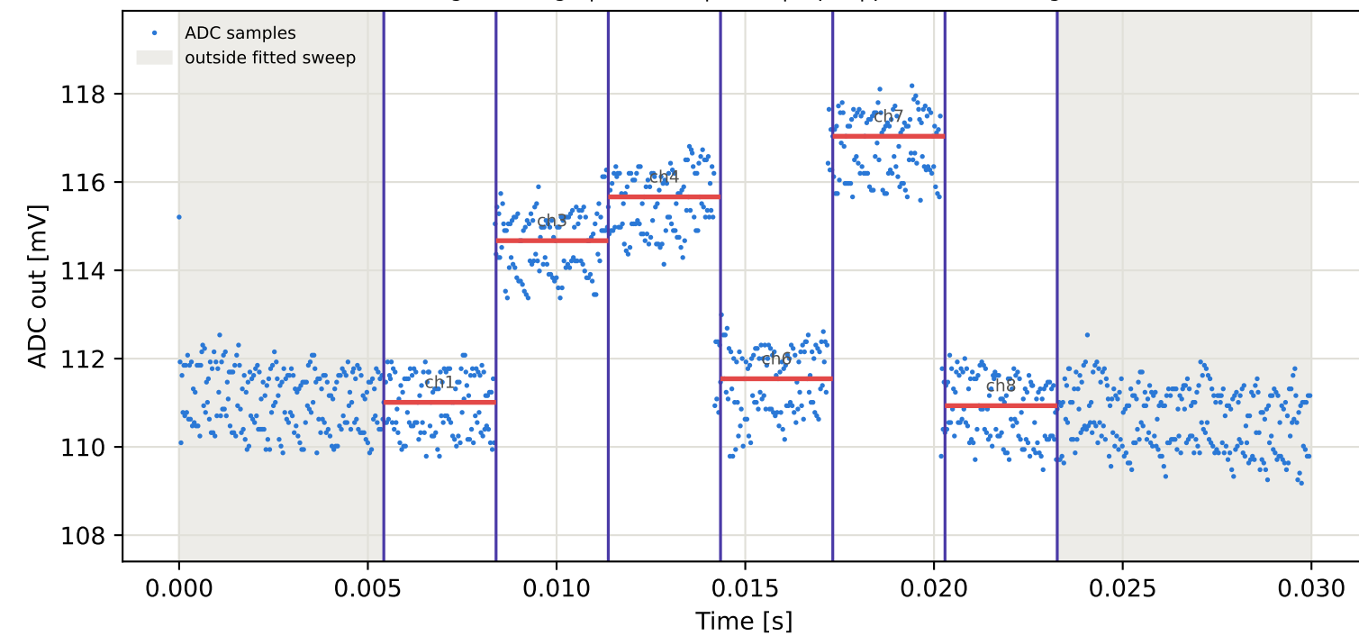
Tag15 &lt;- Tag9 | 775 MHz | run 0 | rep 1 | phase -76.88 deg
