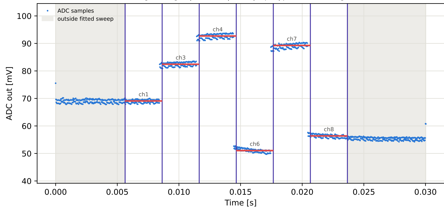
Tag5 &lt;- Tag2 | 985 MHz | run 0 | rep 1 | phase 84.52 deg
