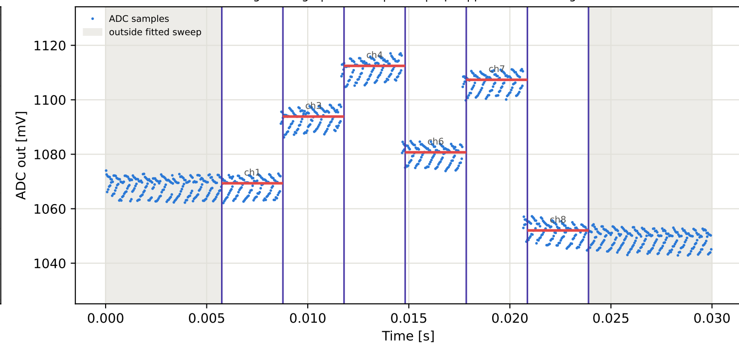
Tag4 &lt;- Tag8 | 895 MHz | run 0 | rep 1 | phase -11.23 deg
