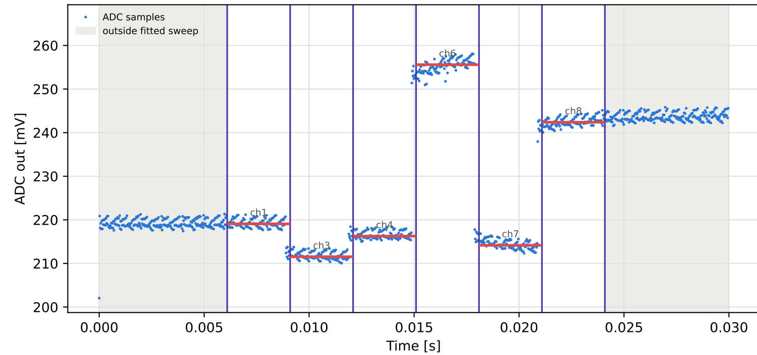
Tag2 &lt;- Tag8 | 905 MHz | run 0 | rep 1 | phase 17.63 deg
