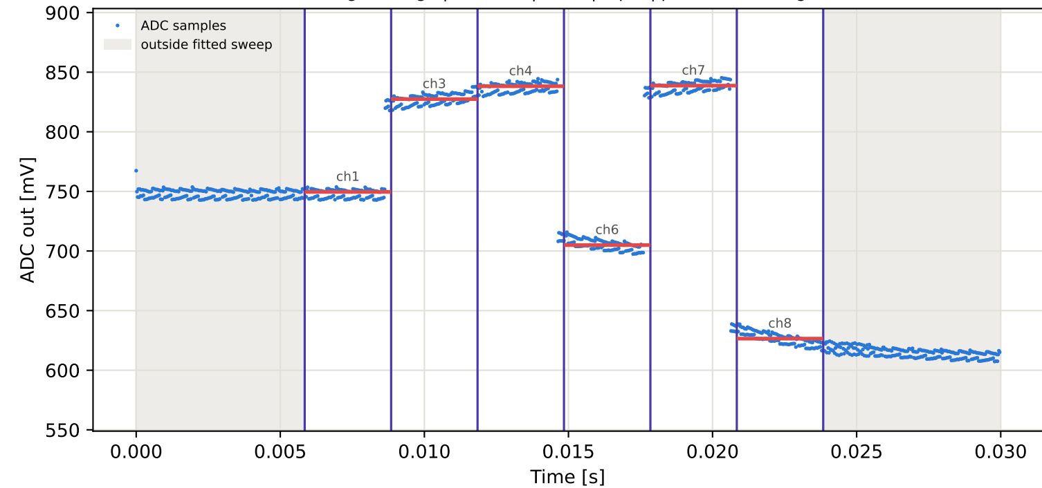
Tag8 &lt;- Tag7 | 895 MHz | run 0 | rep 1 | phase -105.90 deg
