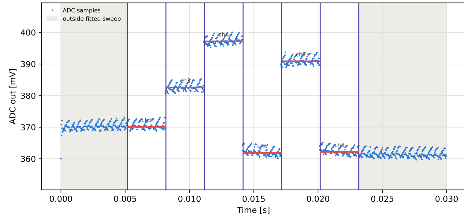
Tag9 &lt;- Tag16 | 975 MHz | run 0 | rep 1 | phase 12.20 deg
