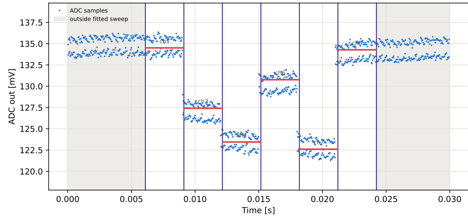
Tag2 &lt;- Tag10 | 795 MHz | run 0 | rep 1 | phase 152.30 deg
