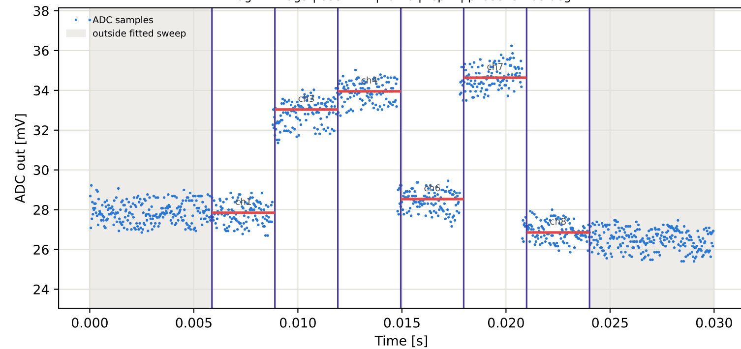
Tag1 &lt;- Tag7 | 835 MHz | run 0 | rep 1 | phase -90.83 deg
