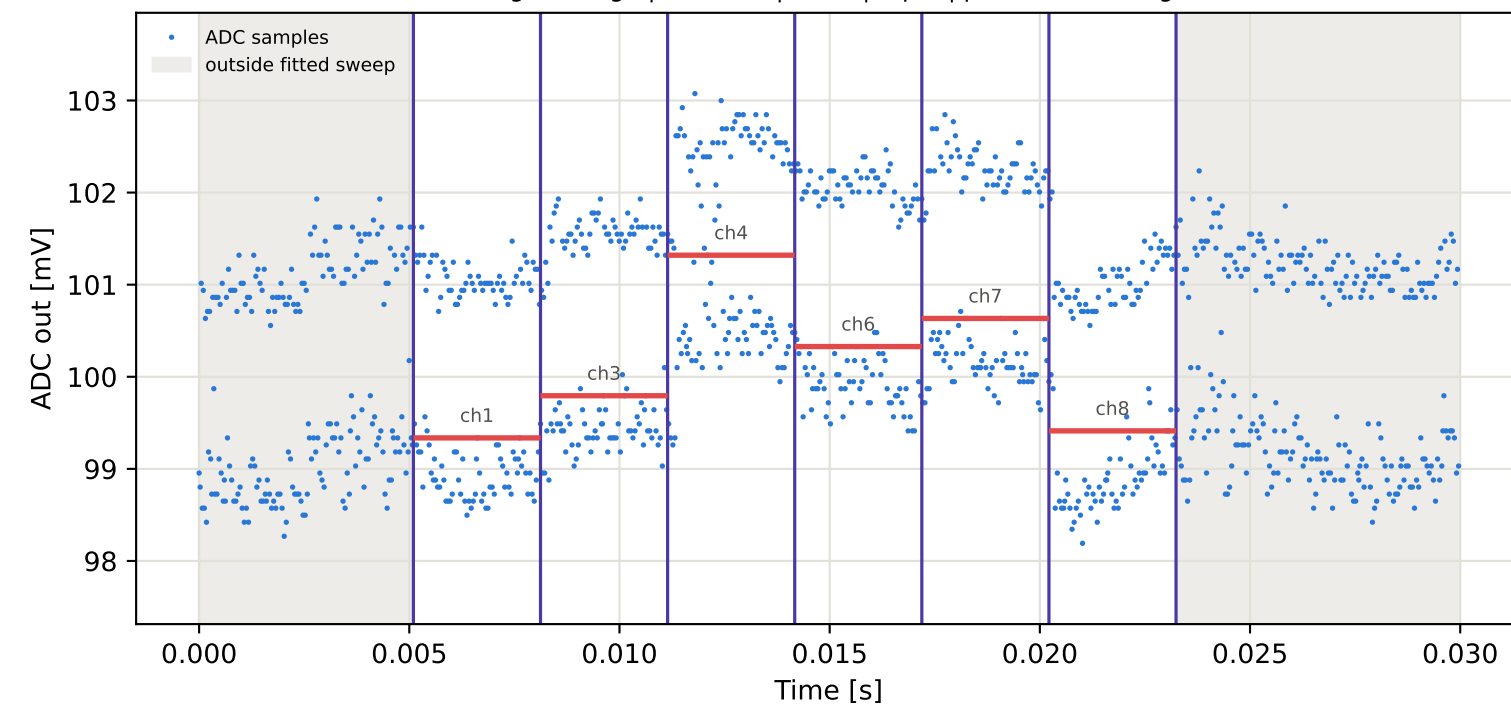
Tag4 &lt;- Tag2 | 775 MHz | run 0 | rep 1 | phase -91.50 deg
