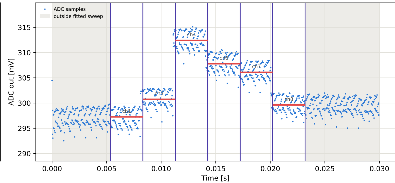
Tag10 &lt;- Tag1 | 975 MHz | run 0 | rep 1 | phase -121.83 deg
