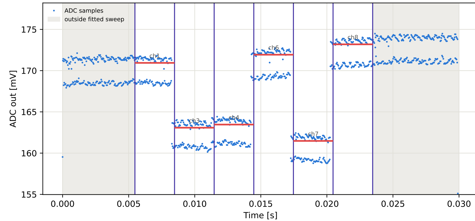
Tag9 &lt;- Tag7 | 805 MHz | run 0 | rep 1 | phase -92.77 deg
