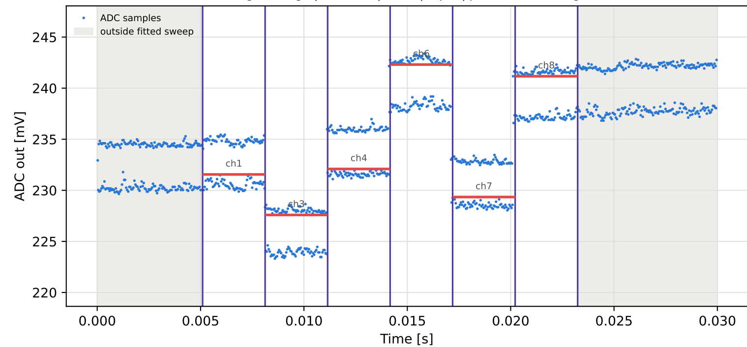
Tag7 &lt;- Tag1 | 835 MHz | run 0 | rep 1 | phase -43.42 deg
