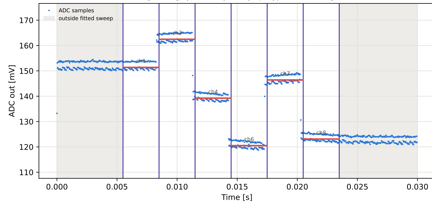
Tag2 &lt;- Tag5 | 845 MHz | run 0 | rep 1 | phase -126.97 deg
