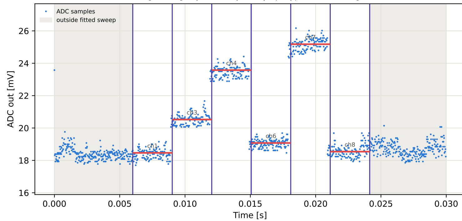
Tag1 &lt;- Tag16 | 775 MHz | run 0 | rep 1 | phase -18.73 deg
