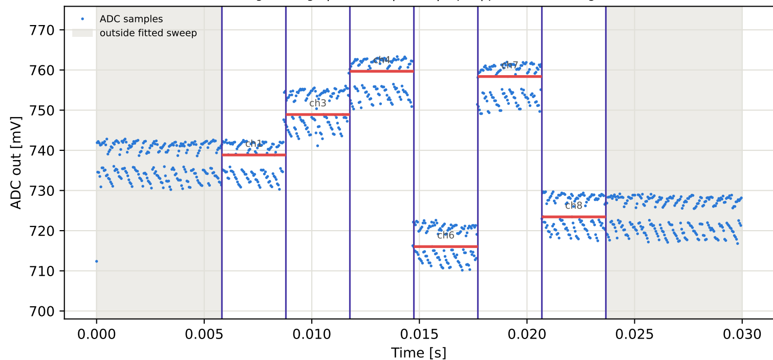
Tag5 &lt;- Tag1 | 975 MHz | run 0 | rep 1 | phase -113.75 deg
