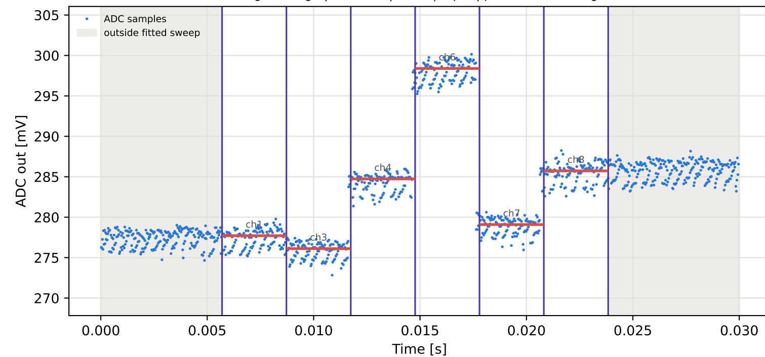
Tag6 &lt;- Tag4 | 955 MHz | run 0 | rep 1 | phase -161.80 deg
