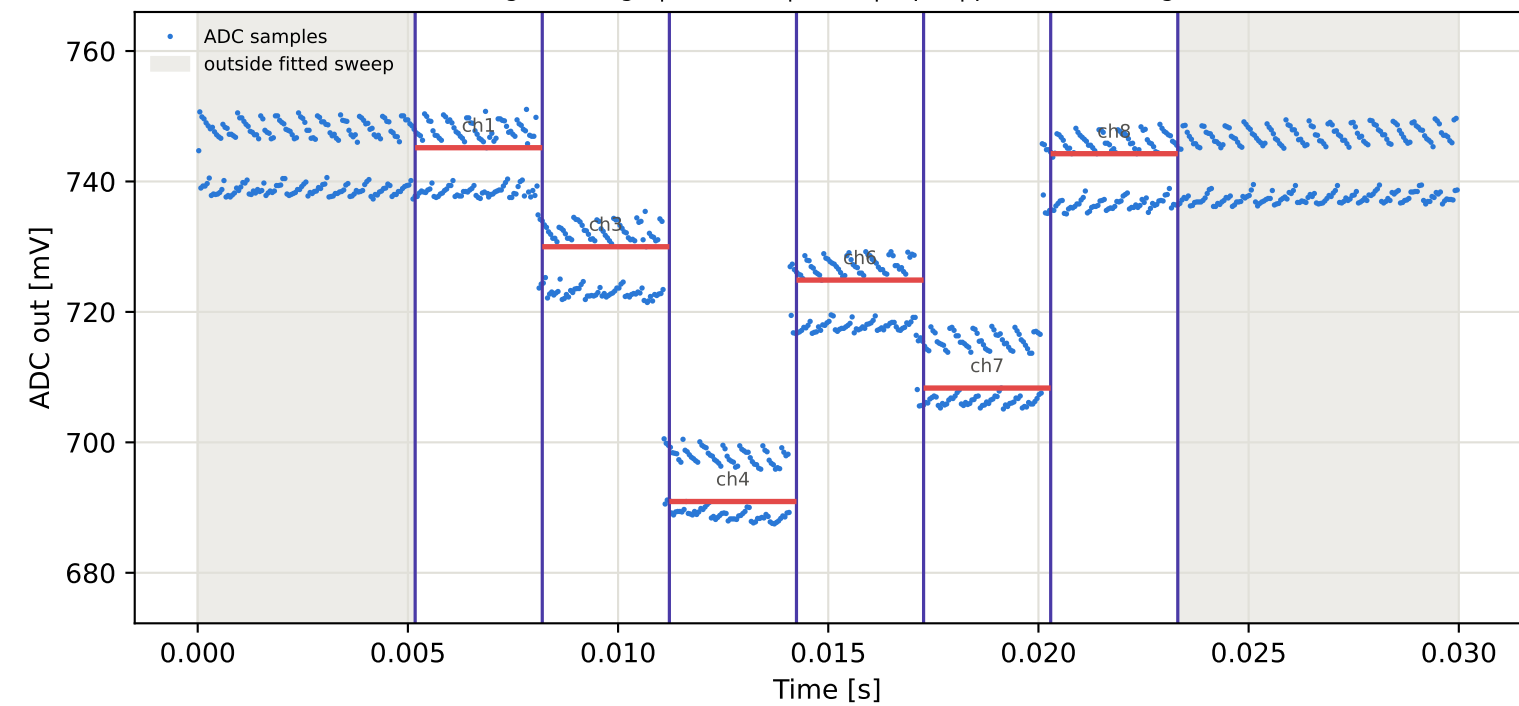
Tag2 &lt;- Tag10 | 975 MHz | run 0 | rep 1 | phase -48.99 deg
