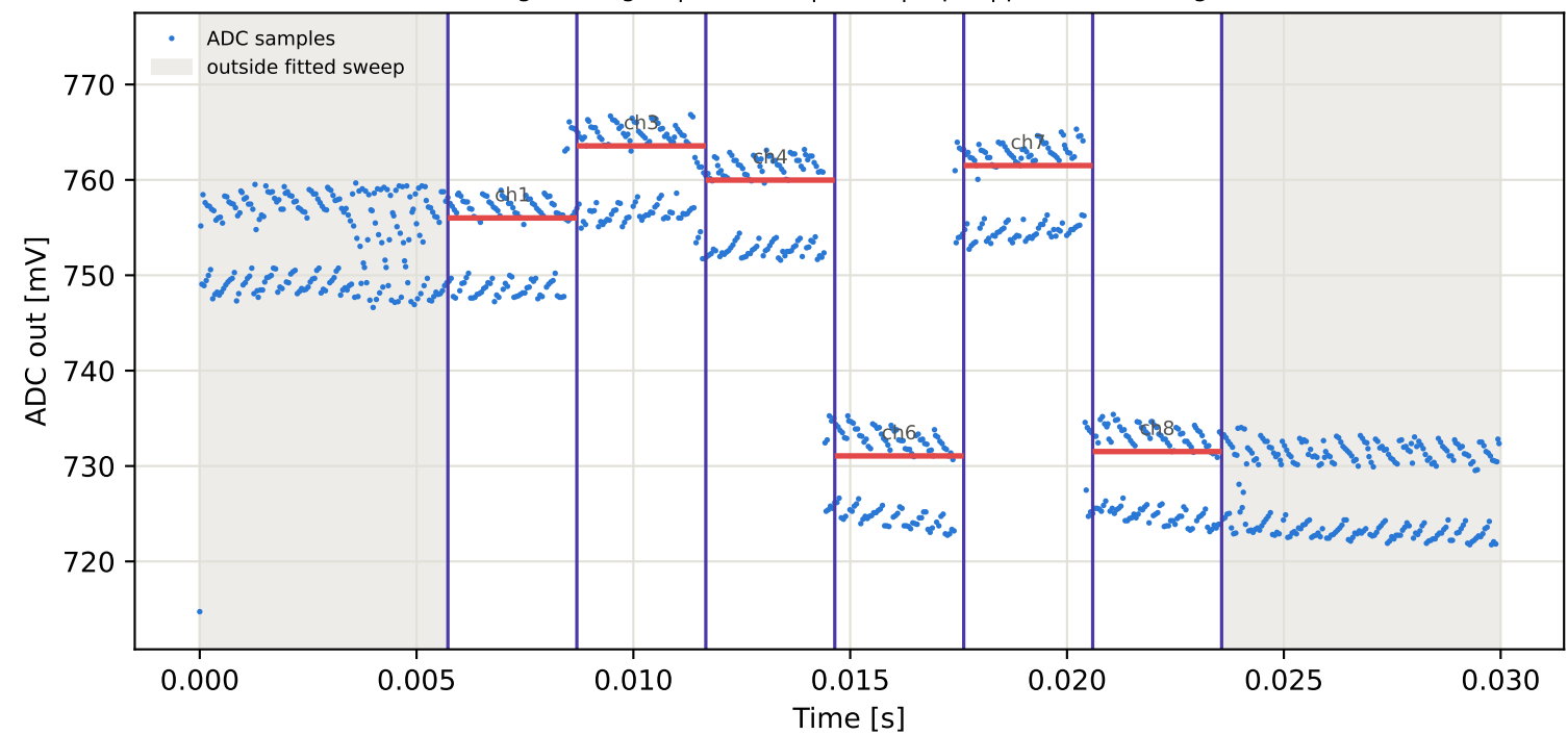
Tag8 &lt;- Tag16 | 895 MHz | run 0 | rep 1 | phase 33.47 deg
