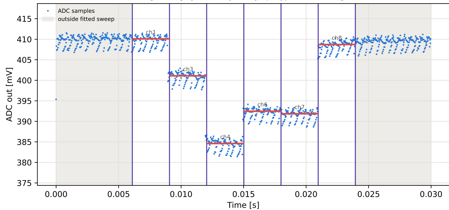
Tag8 &lt;- Tag10 | 935 MHz | run 0 | rep 1 | phase -156.76 deg
