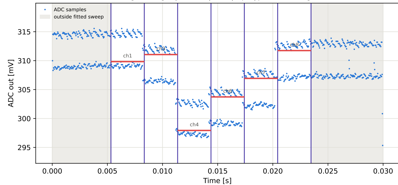
Tag10 &lt;- Tag2 | 965 MHz | run 0 | rep 1 | phase 128.41 deg
