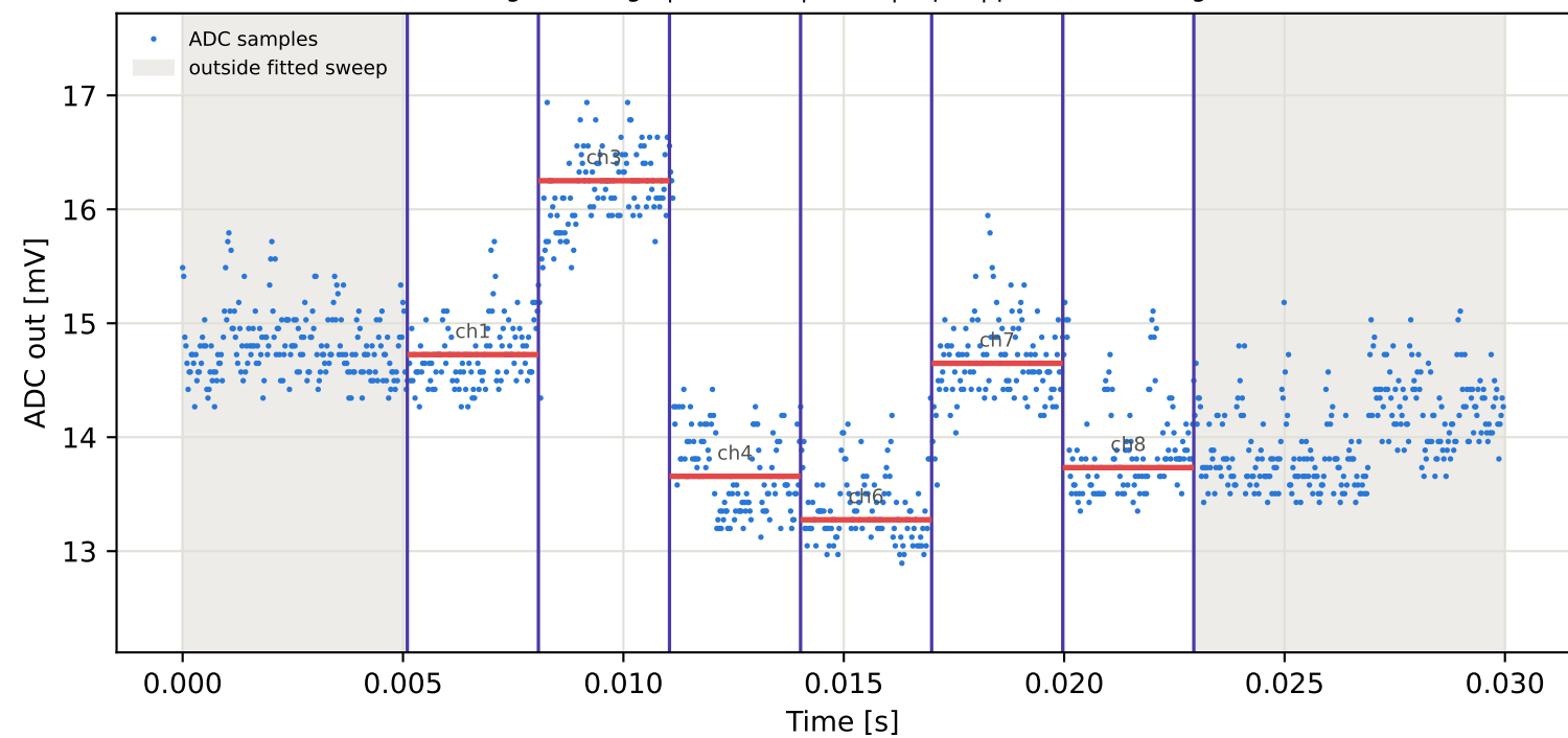
Tag10 &lt;- Tag4 | 795 MHz | run 0 | rep 1 | phase 38.80 deg
