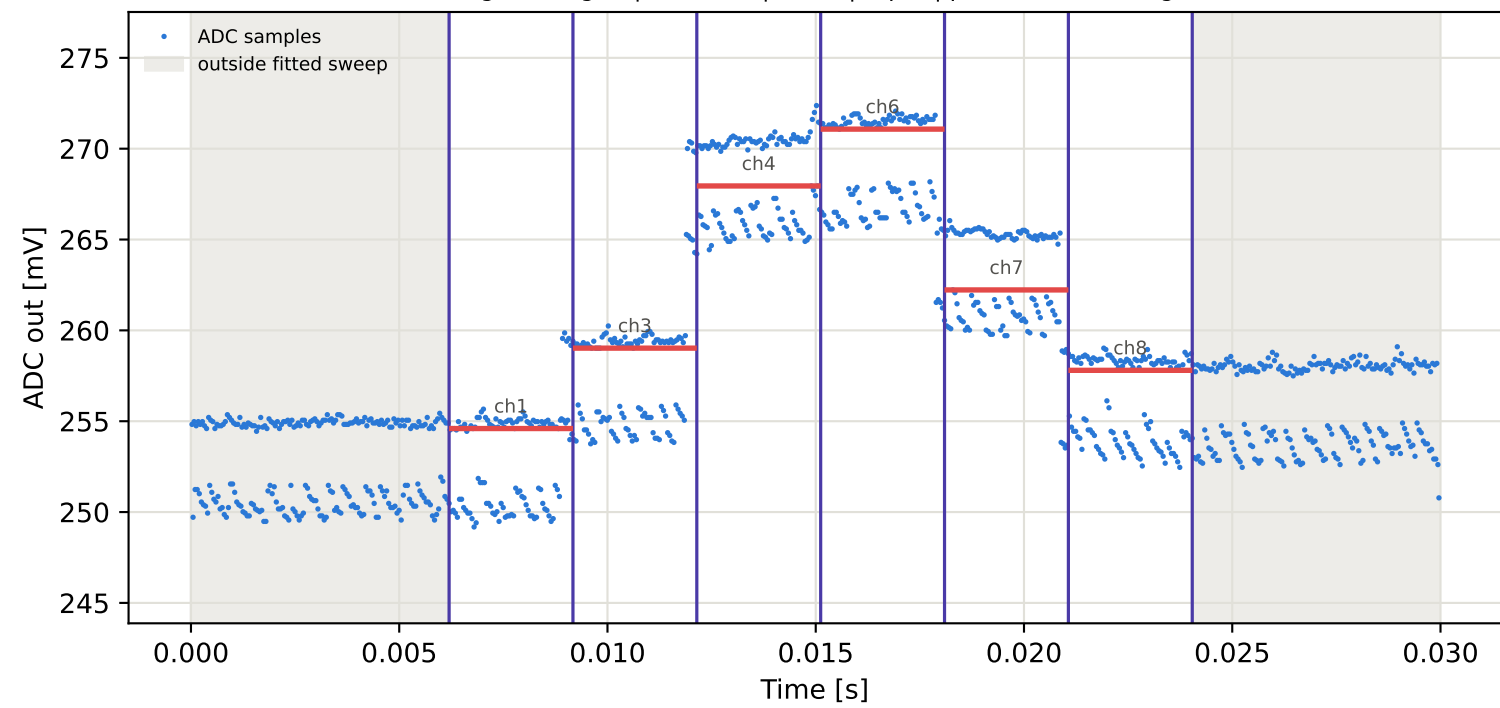
Tag6 &lt;- Tag2 | 945 MHz | run 0 | rep 1 | phase -168.49 deg
