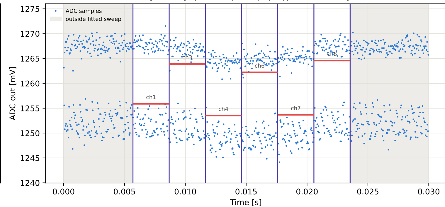
Tag16 &lt;- Tag7 | 885 MHz | run 0 | rep 1 | phase 107.71 deg
