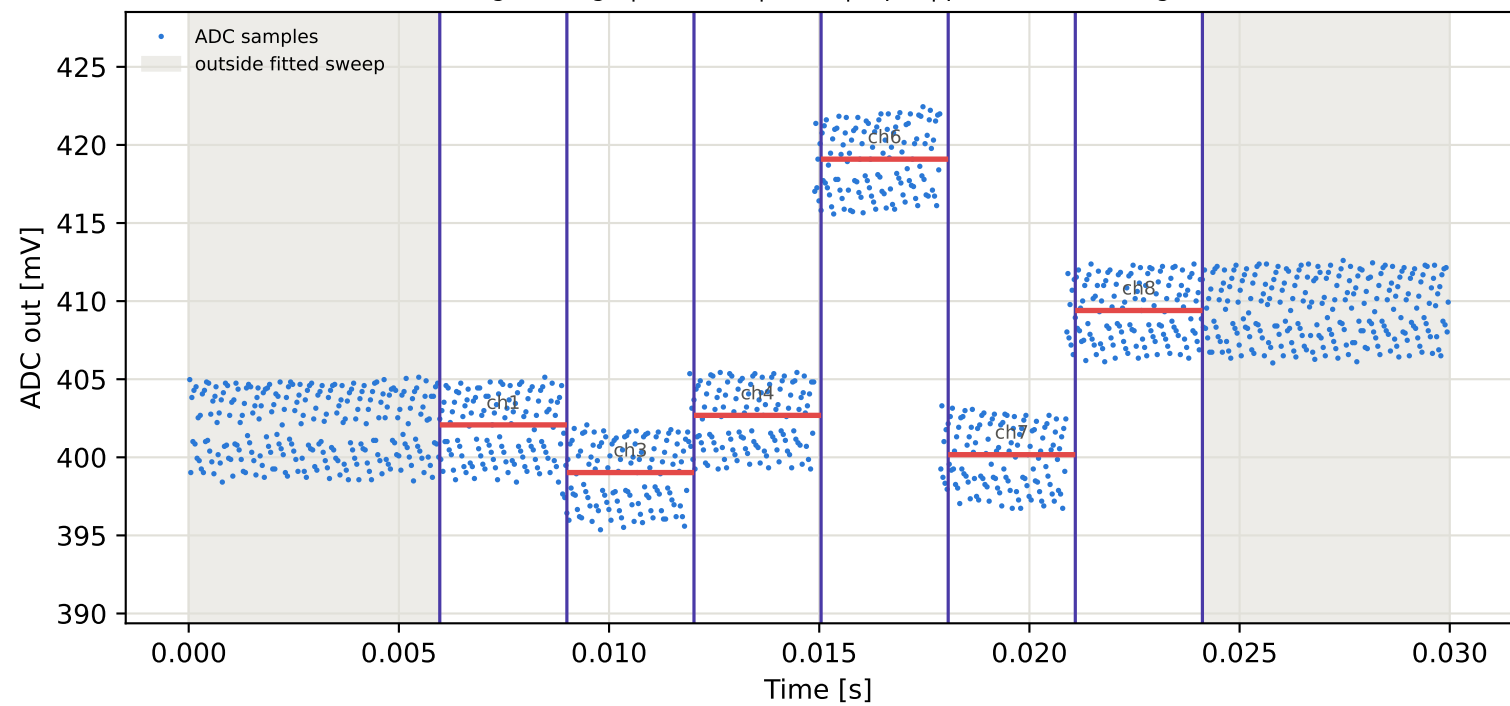
Tag3 &lt;- Tag7 | 955 MHz | run 0 | rep 1 | phase 152.68 deg
