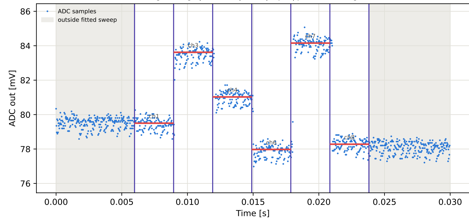
Tag8 &lt;- Tag5 | 785 MHz | run 0 | rep 1 | phase 94.02 deg
