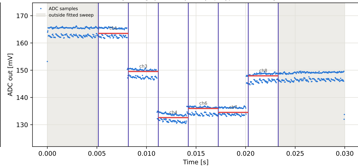
Tag2 &lt;- Tag6 | 845 MHz | run 0 | rep 1 | phase 75.05 deg
