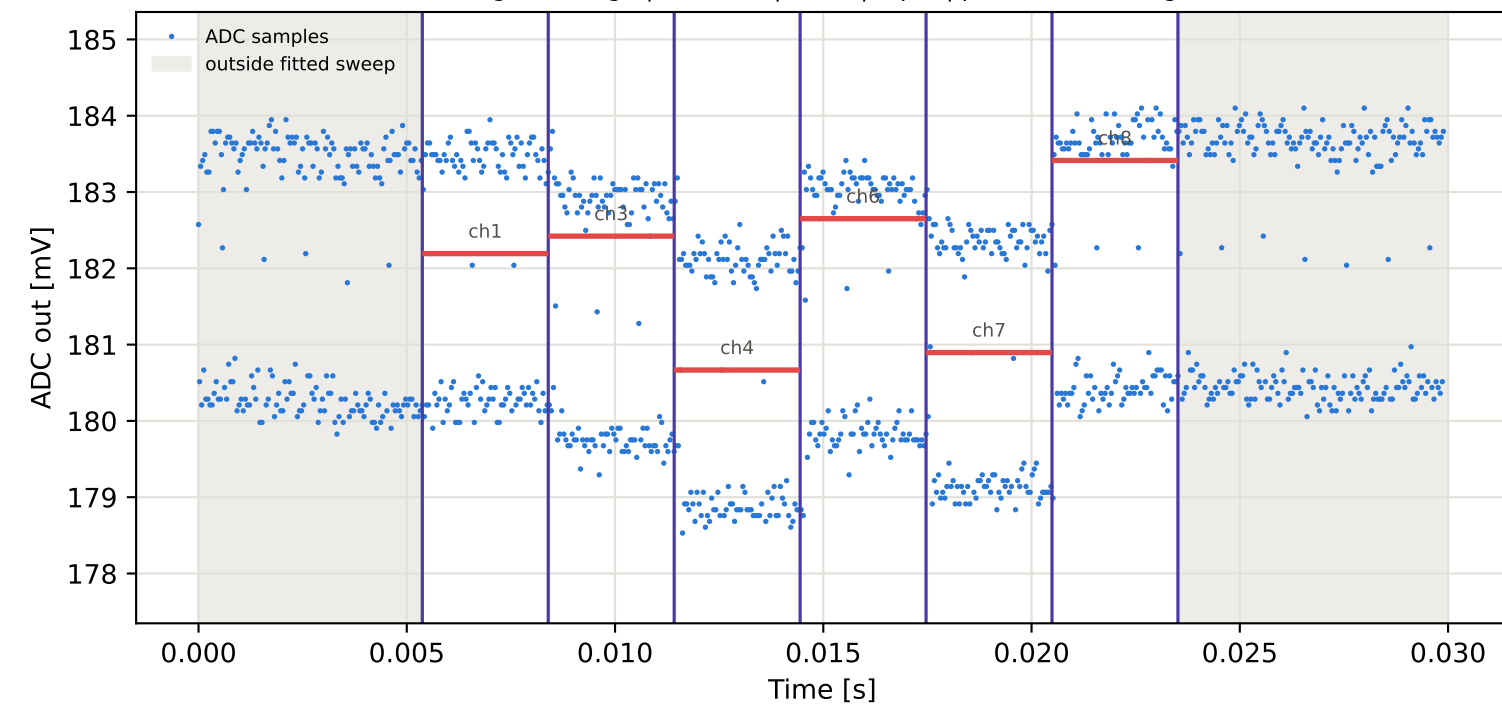
Tag16 &lt;- Tag4 | 805 MHz | run 0 | rep 1 | phase -111.11 deg
