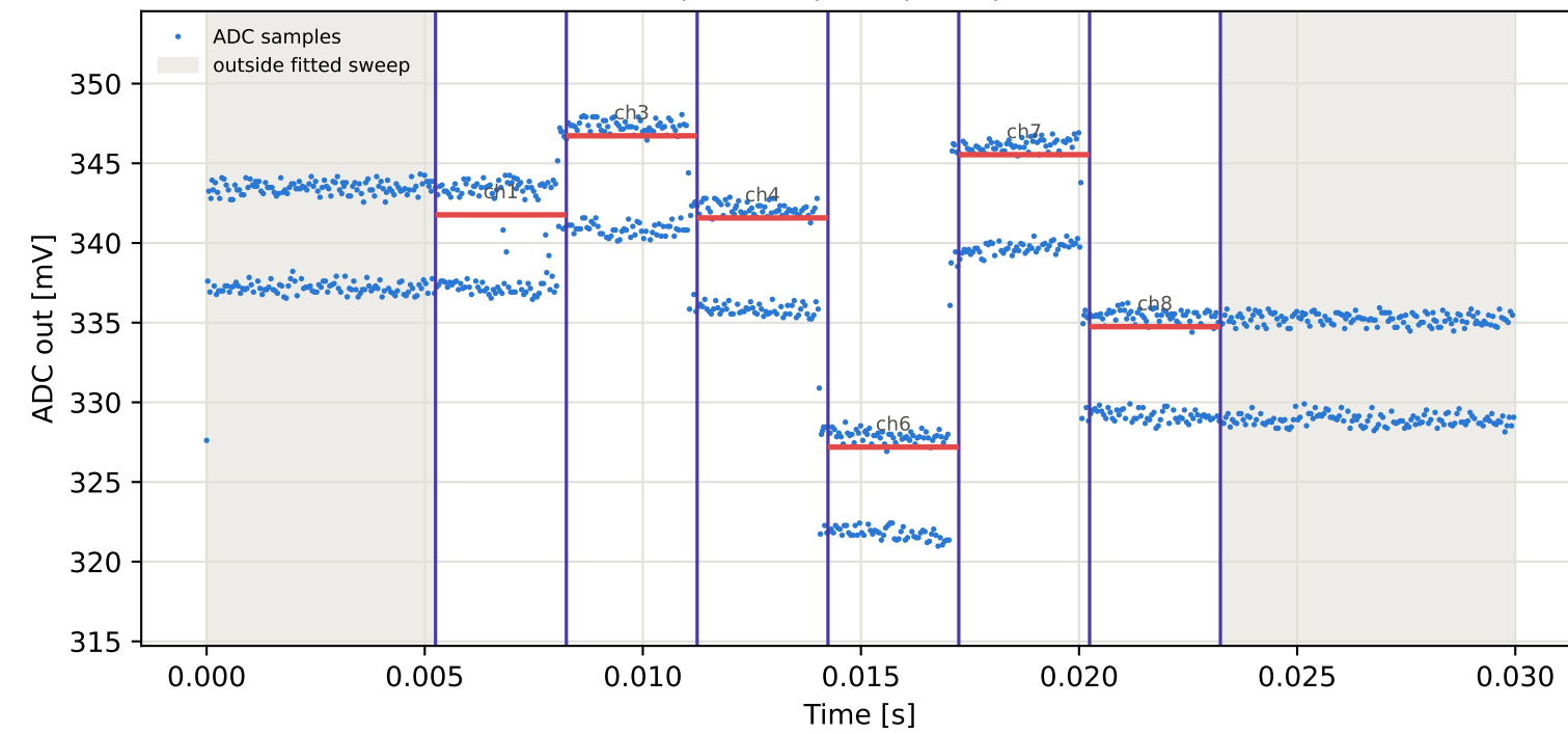
Tag1 &lt;- Tag9 | 975 MHz | run 0 | rep 1 | phase -0.55 deg
