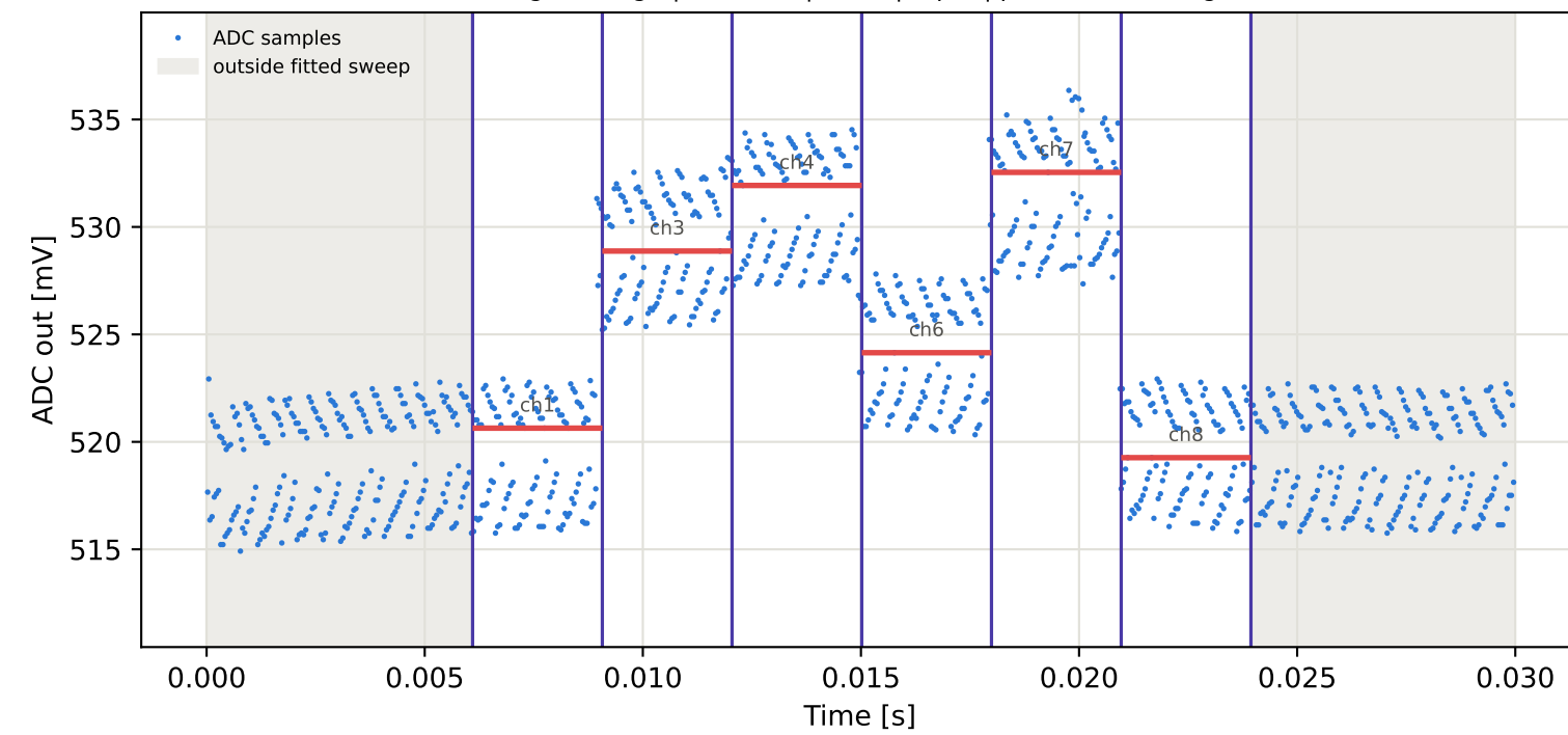
Tag5 &lt;- Tag8 | 835 MHz | run 0 | rep 1 | phase 82.30 deg
