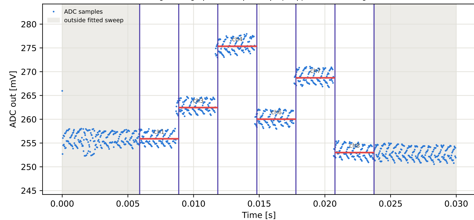
Tag5 &lt;- Tag3 | 955 MHz | run 0 | rep 1 | phase -92.44 deg
