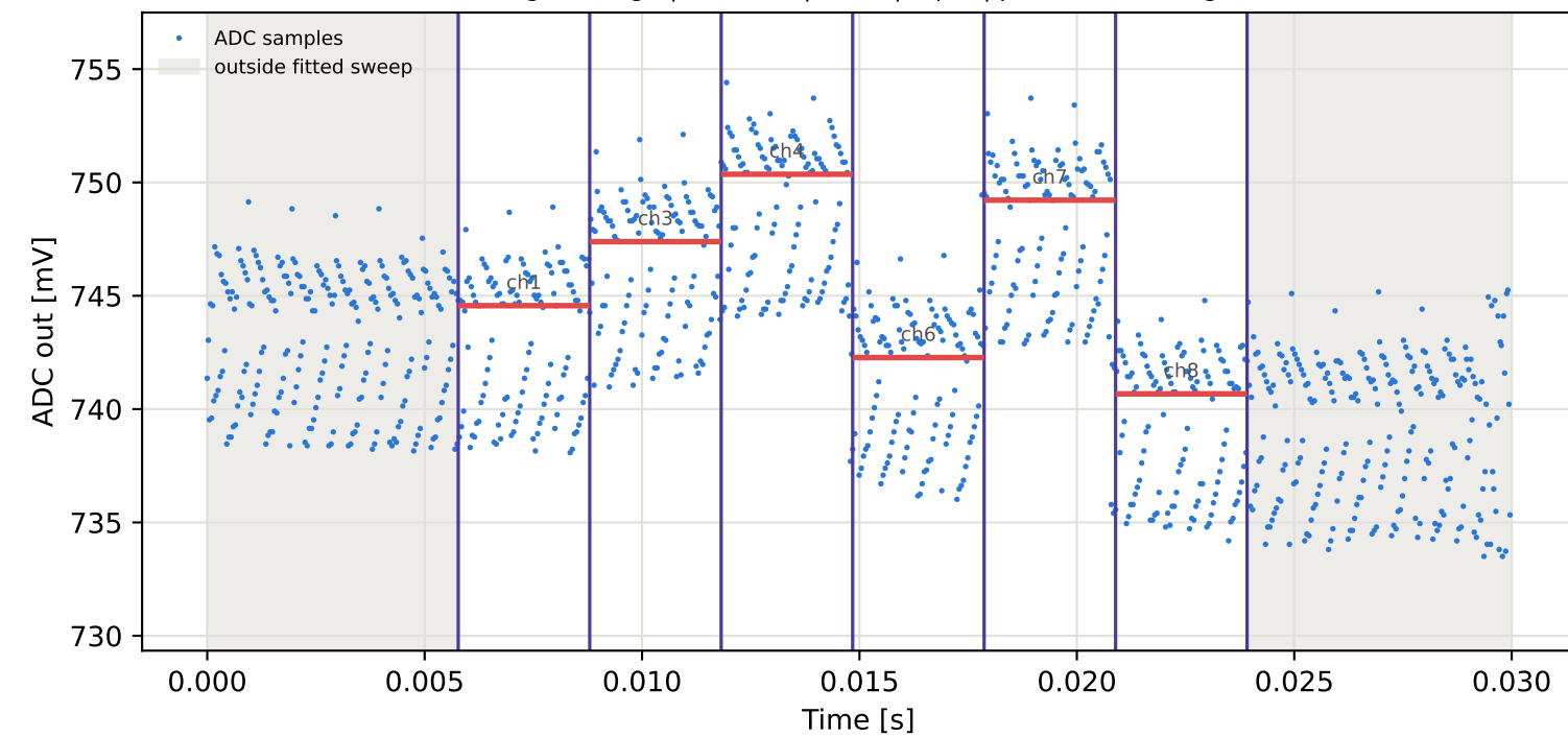
Tag8 &lt;- Tag4 | 895 MHz | run 0 | rep 1 | phase 44.28 deg
