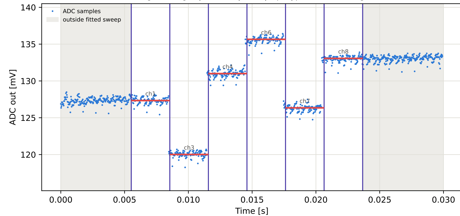
Tag10 &lt;- Tag2 | 825 MHz | run 0 | rep 1 | phase 60.90 deg
