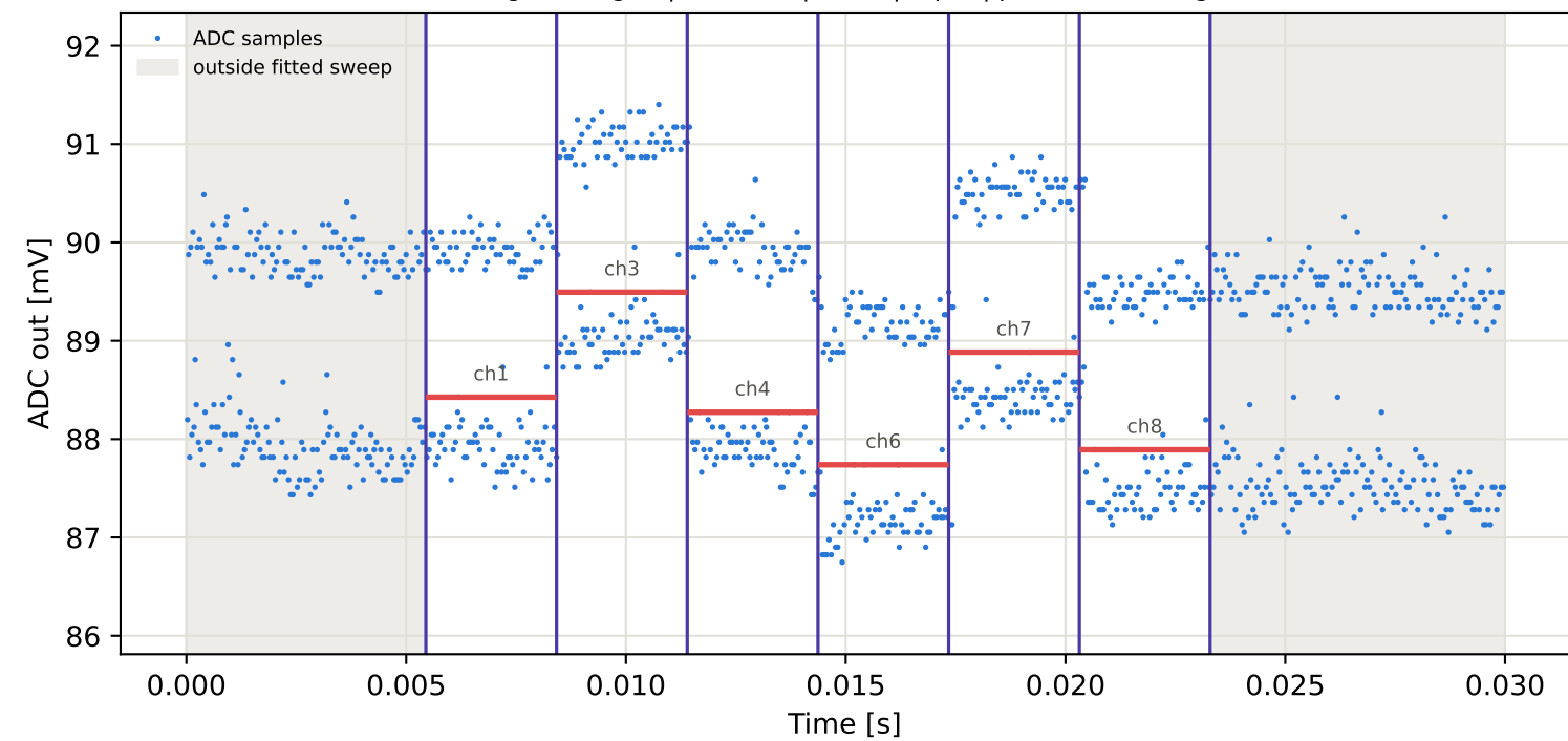
Tag4 &lt;- Tag16 | 795 MHz | run 0 | rep 1 | phase 108.82 deg
