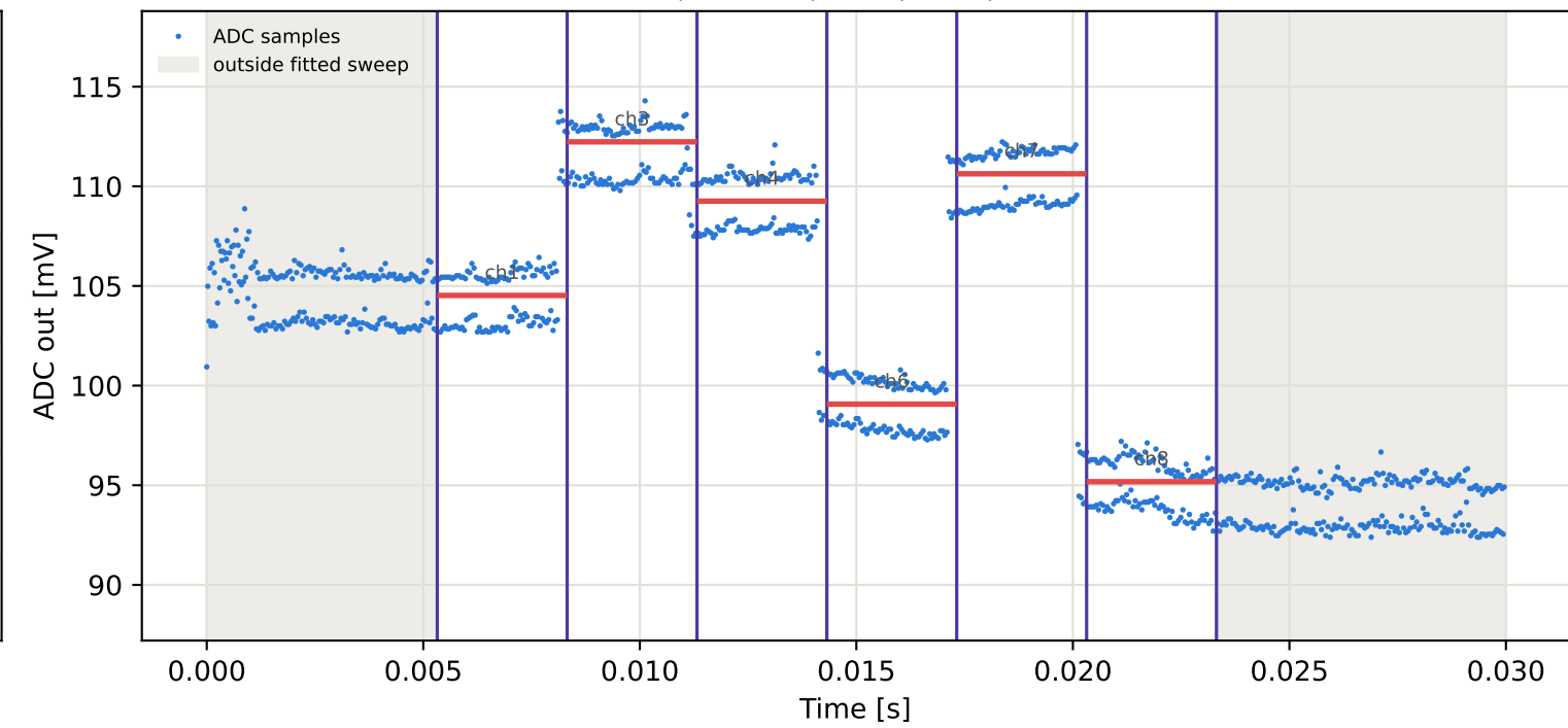
Tag7 &lt;- Tag15 | 875 MHz | run 0 | rep 1 | phase -18.35 deg
