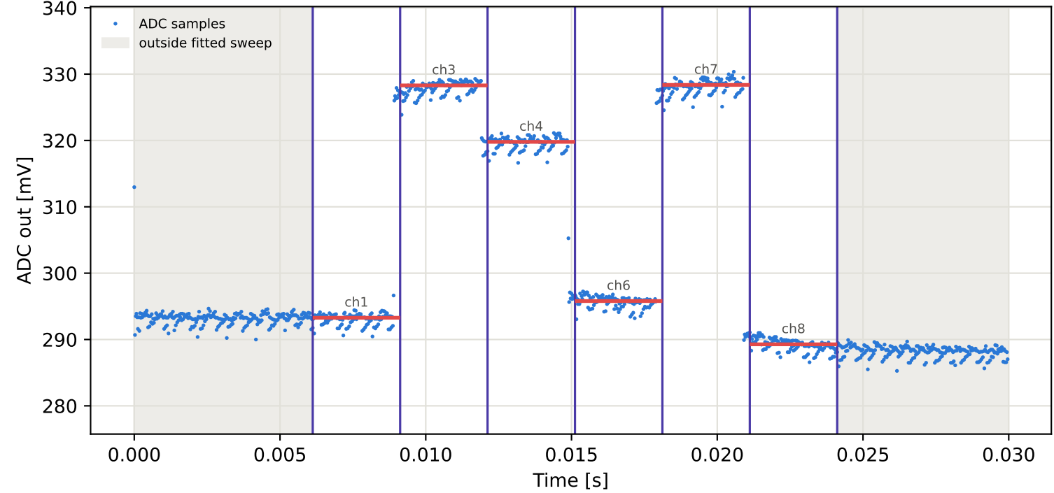
Tag6 &lt;- Tag5 | 825 MHz | run 0 | rep 1 | phase -109.97 deg
