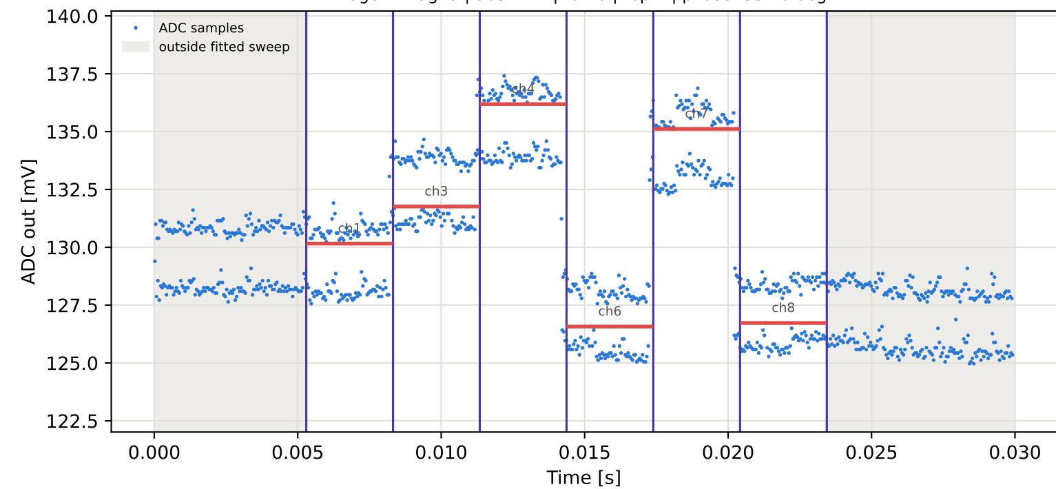
Tag6 &lt;- Tag2 | 965 MHz | run 0 | rep 1 | phase -25.08 deg
