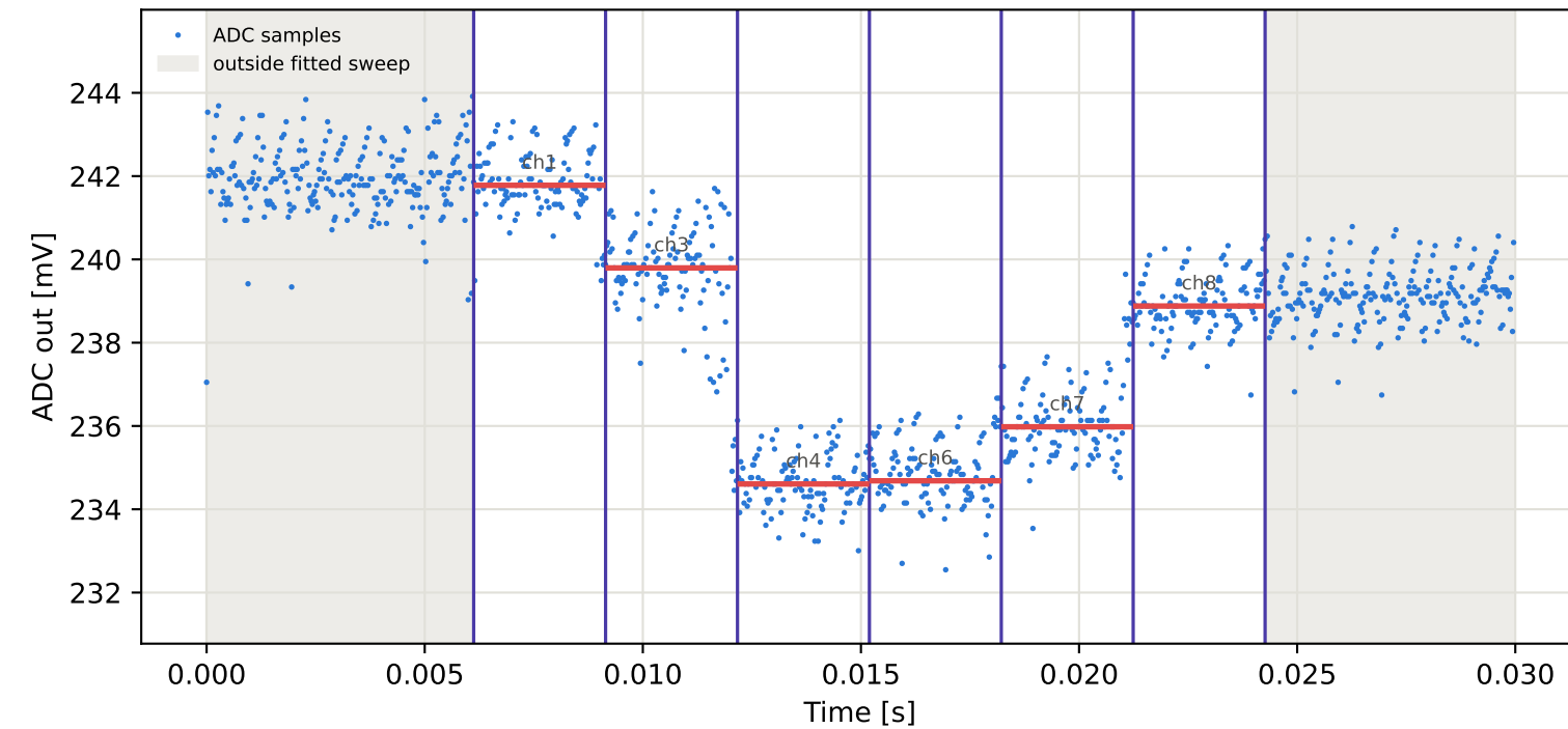
Tag6 &lt;- Tag4 | 835 MHz | run 0 | rep 1 | phase 17.21 deg
