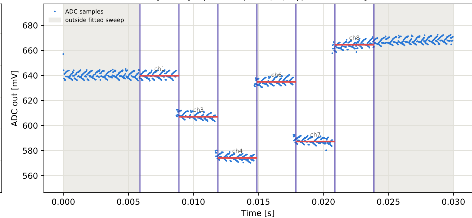
Tag8 &lt;- Tag16 | 925 MHz | run 0 | rep 1 | phase 107.17 deg
