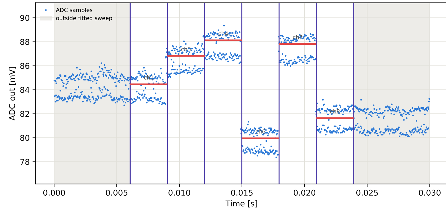
Tag2 &lt;- Tag7 | 985 MHz | run 0 | rep 1 | phase 107.23 deg
