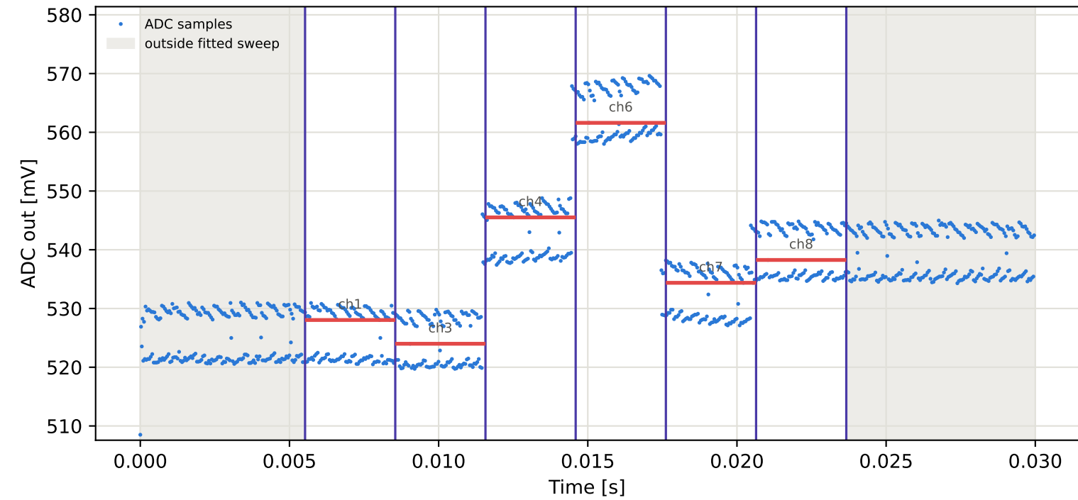
Tag9 &lt;- Tag8 | 945 MHz | run 0 | rep 1 | phase -22.10 deg
