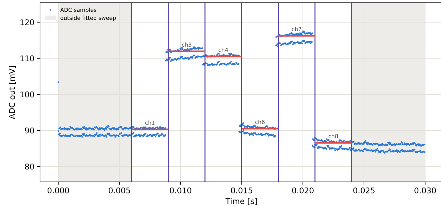
Tag3 &lt;- Tag8 | 795 MHz | run 0 | rep 1 | phase 71.10 deg
