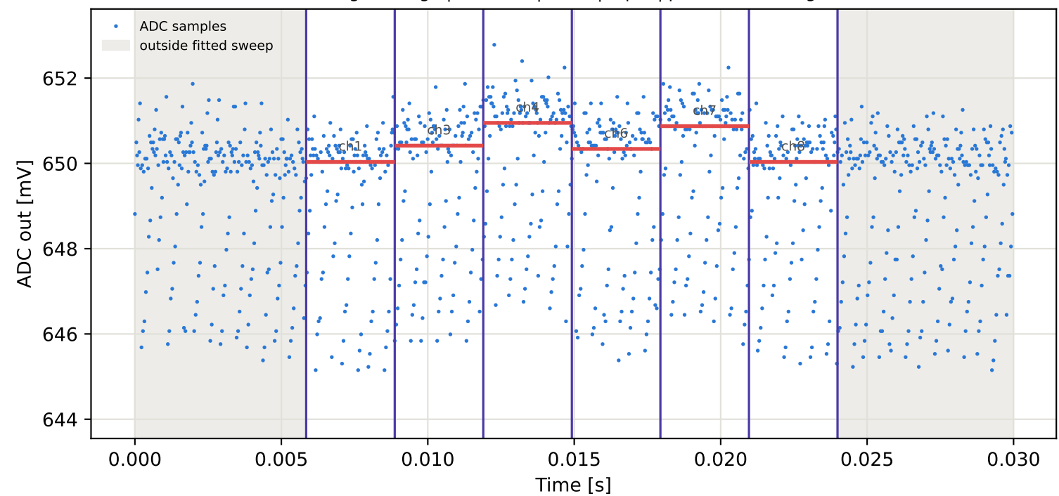
Tag8 &lt;- Tag7 | 845 MHz | run 0 | rep 1 | phase -82.12 deg
