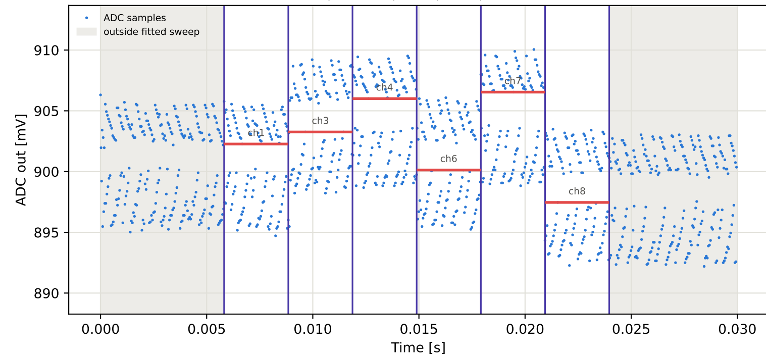
Tag8 &lt;- Tag6 | 855 MHz | run 0 | rep 1 | phase -49.77 deg
