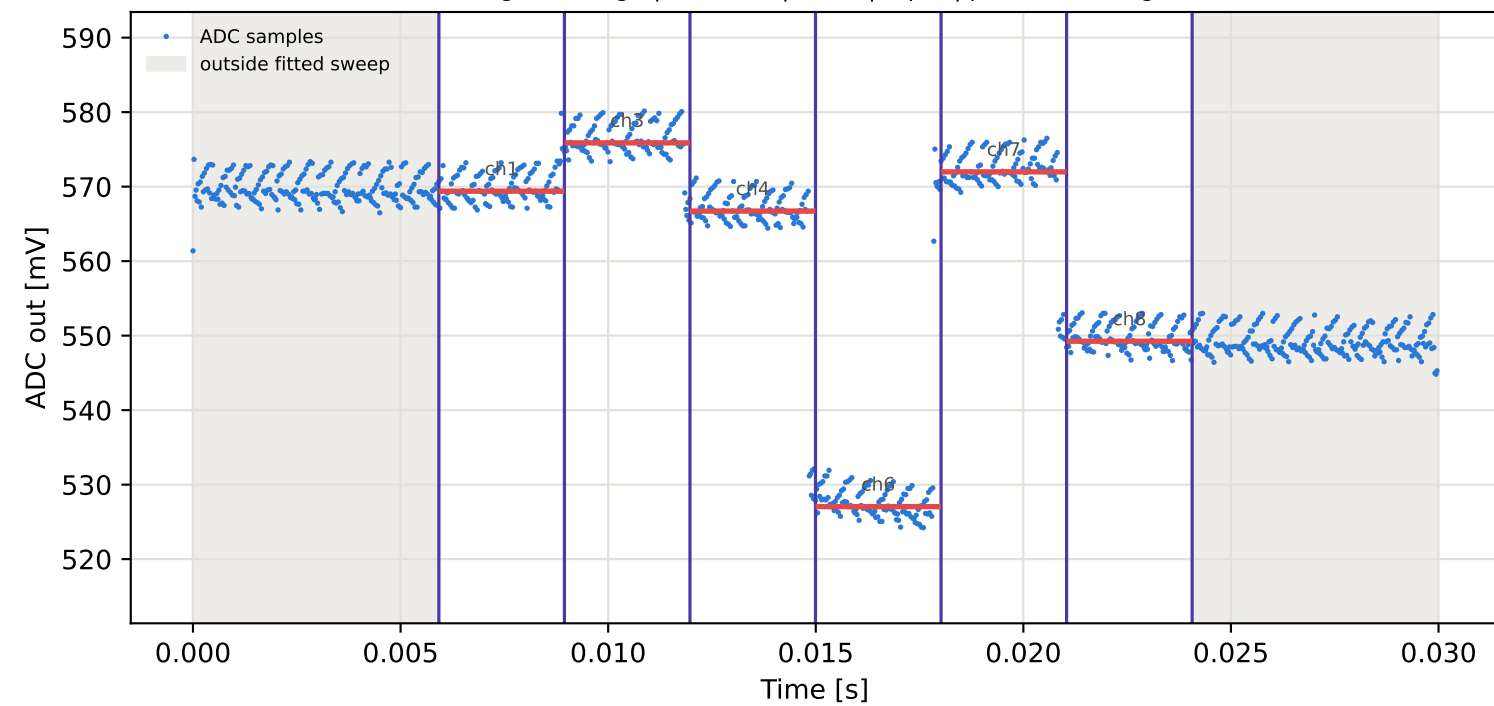
Tag10 &lt;- Tag9 | 935 MHz | run 0 | rep 1 | phase -68.95 deg
