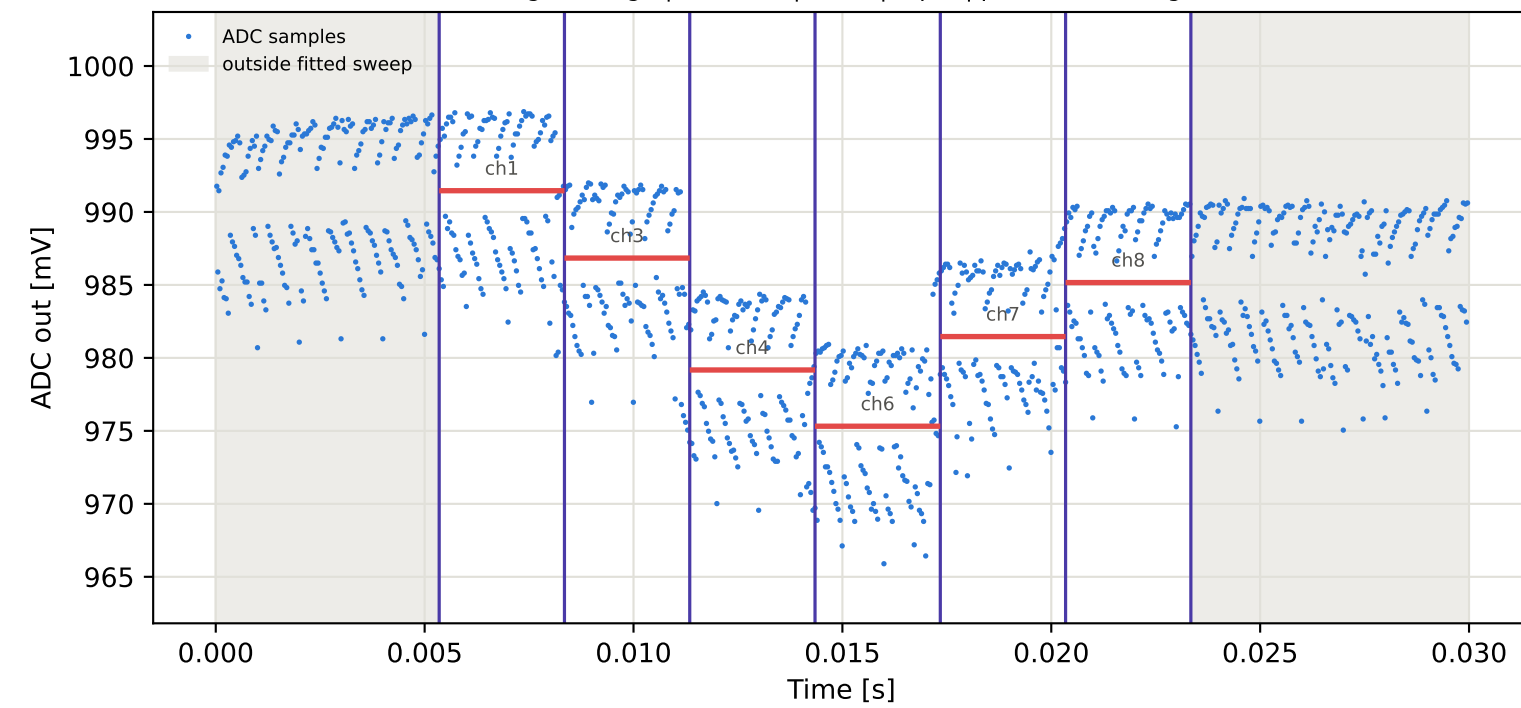
Tag5 &lt;- Tag8 | 865 MHz | run 0 | rep 1 | phase 124.48 deg
