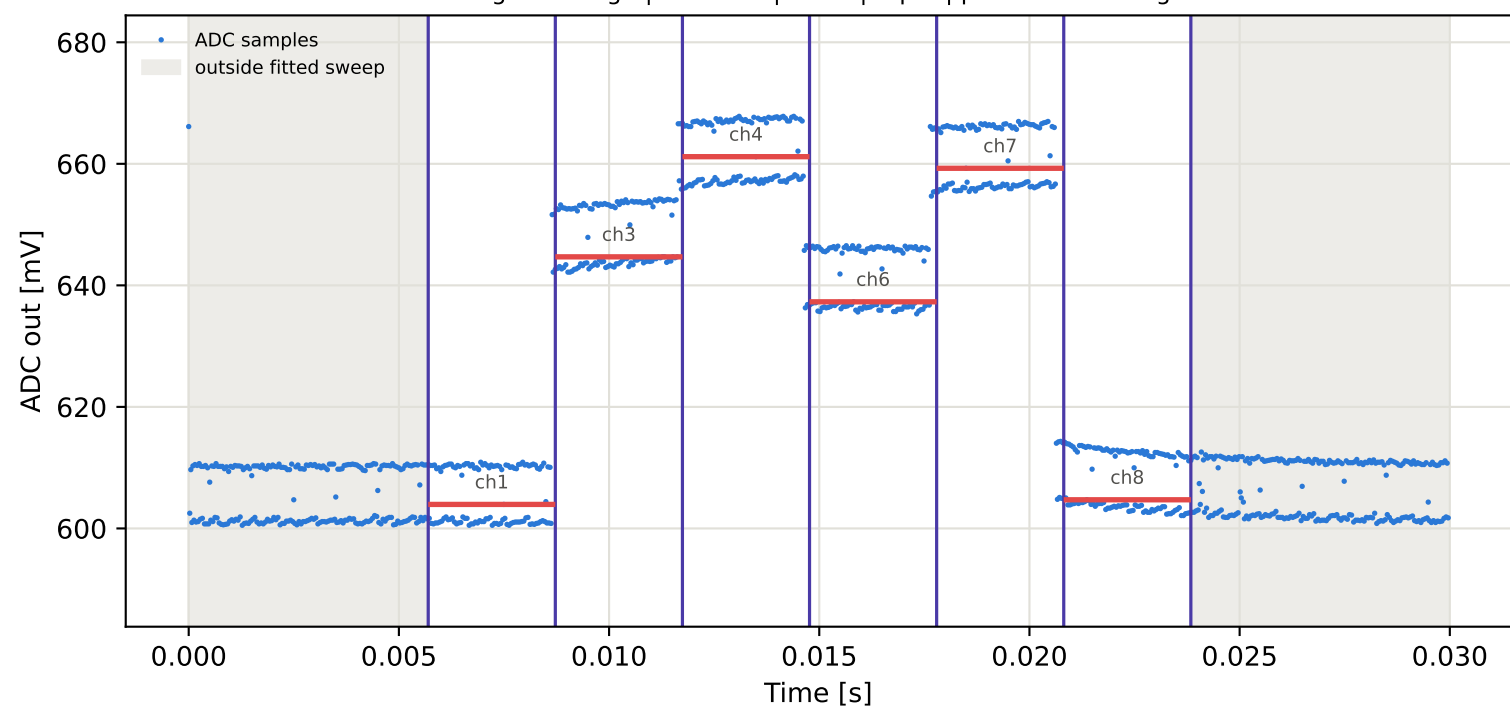
Tag15 &lt;- Tag6 | 865 MHz | run 0 | rep 1 | phase -128.73 deg
