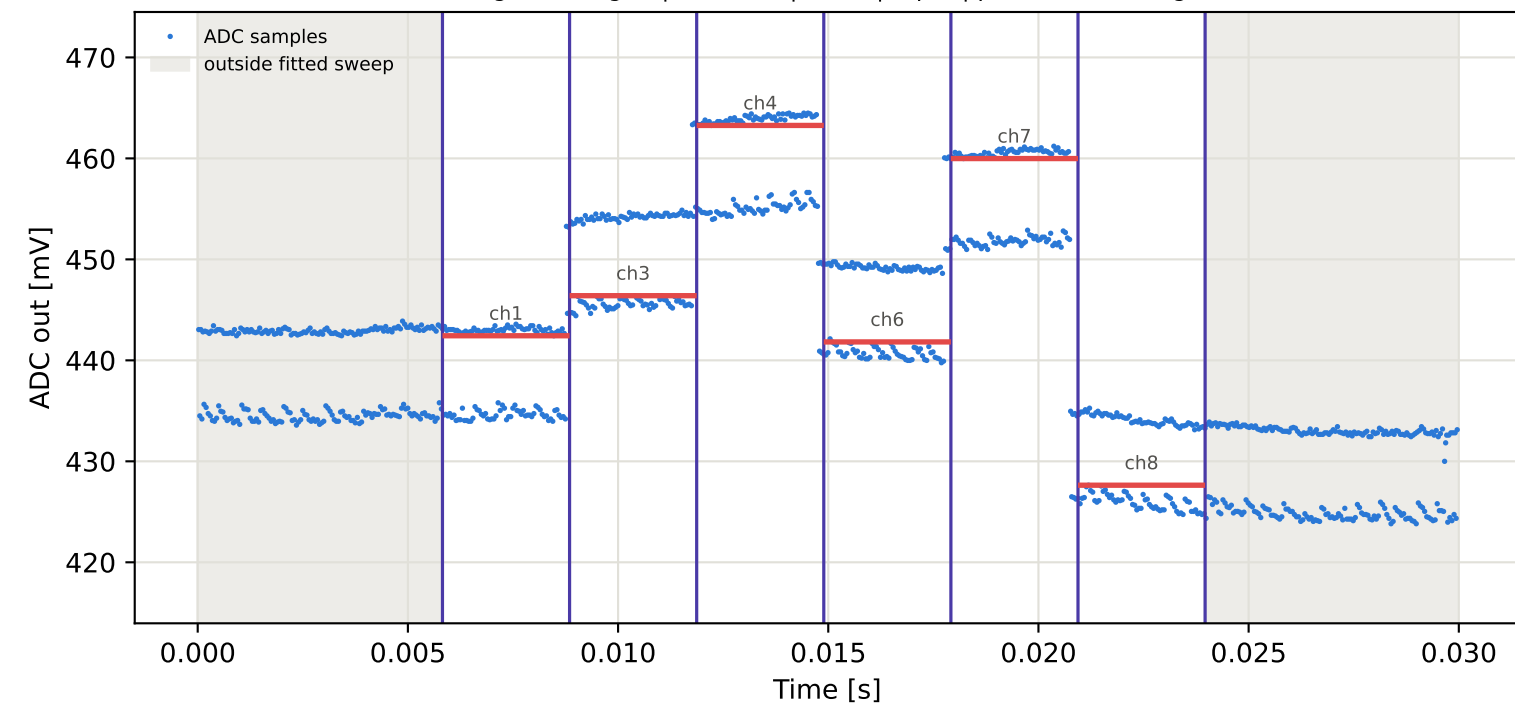
Tag10 &lt;- Tag3 | 915 MHz | run 0 | rep 1 | phase 56.38 deg
