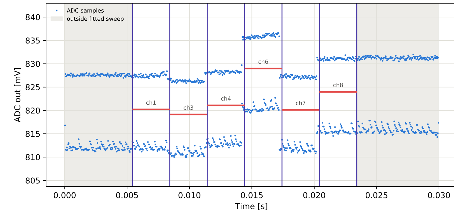
Tag16 &lt;- Tag10 | 945 MHz | run 0 | rep 1 | phase -171.87 deg
