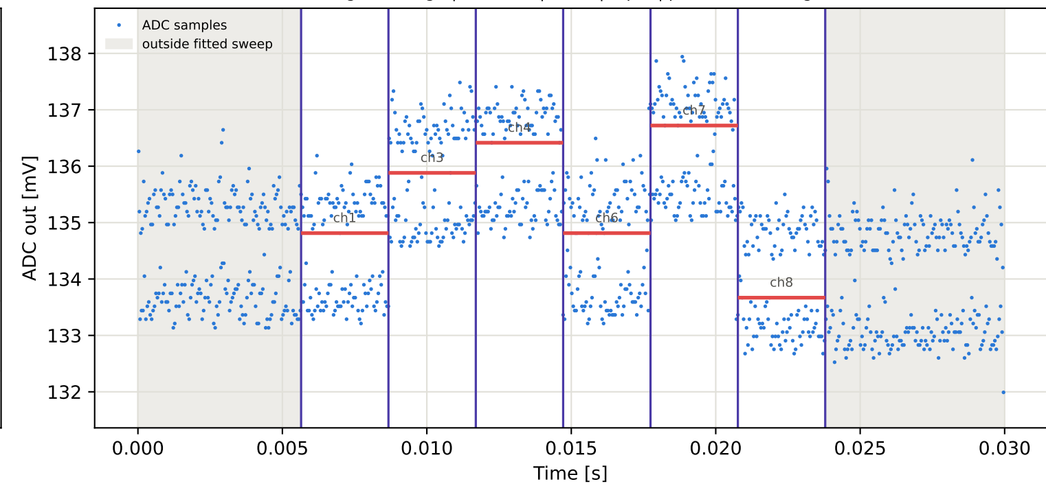
Tag10 &lt;- Tag9 | 845 MHz | run 0 | rep 1 | phase -163.07 deg
