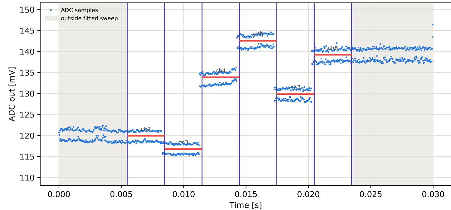
Tag10 &lt;- Tag5 | 845 MHz | run 0 | rep 1 | phase -25.74 deg
