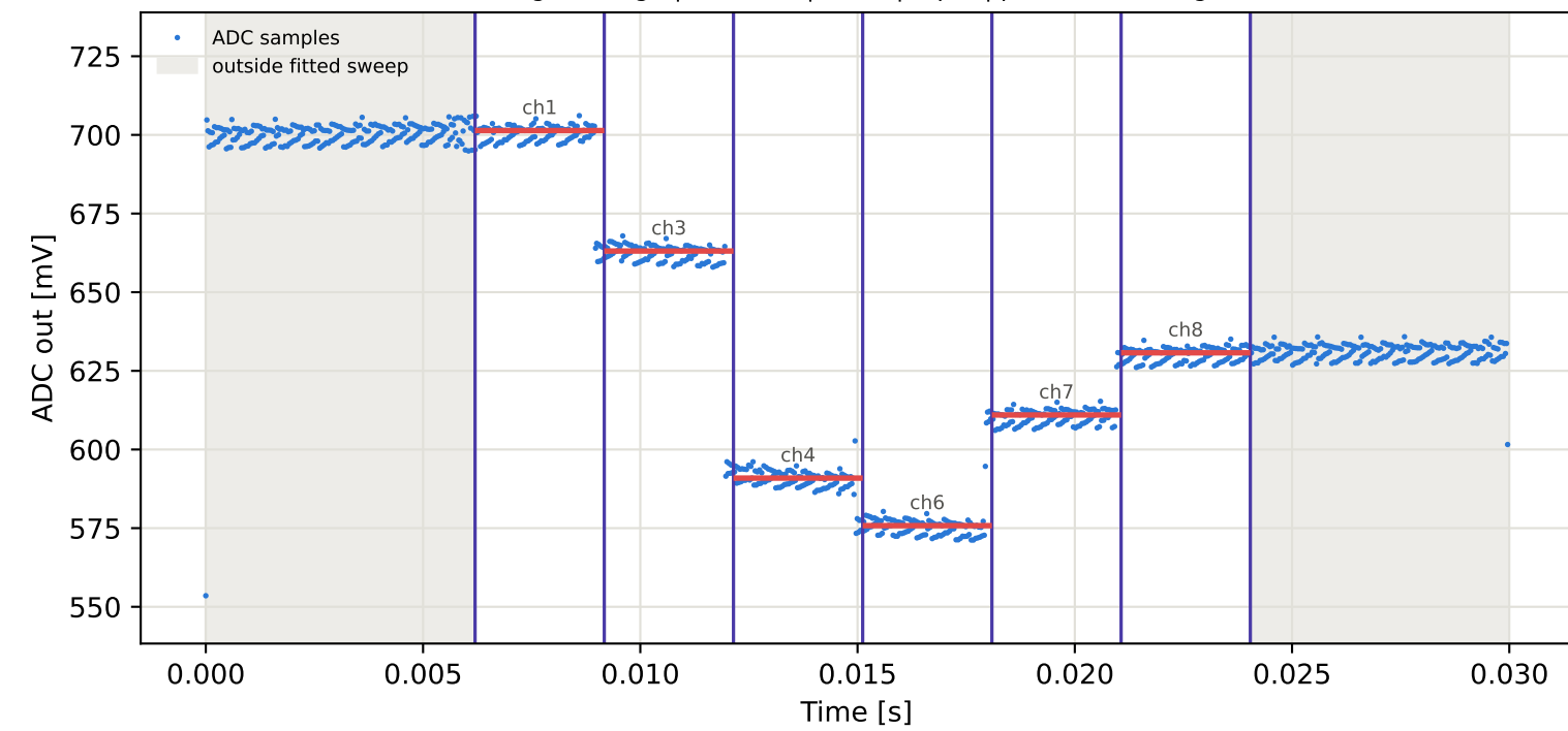
Tag4 &lt;- Tag7 | 865 MHz | run 0 | rep 1 | phase 85.08 deg
