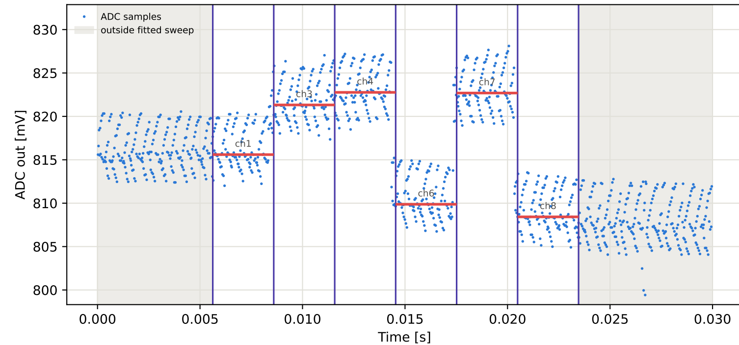
Tag4 &lt;- Tag9 | 905 MHz | run 0 | rep 1 | phase 0.28 deg
