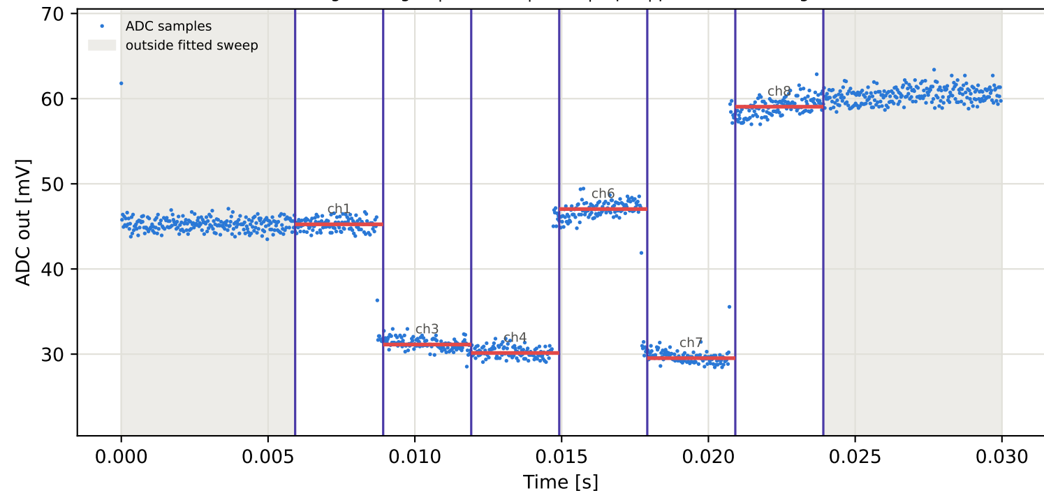
Tag7 &lt;- Tag15 | 885 MHz | run 0 | rep 1 | phase 135.06 deg
