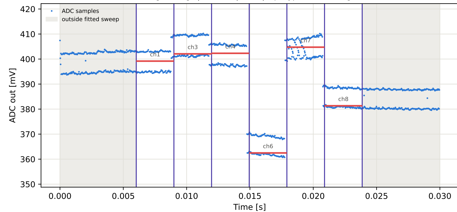
Tag8 &lt;- Tag1 | 945 MHz | run 0 | rep 1 | phase 174.09 deg
