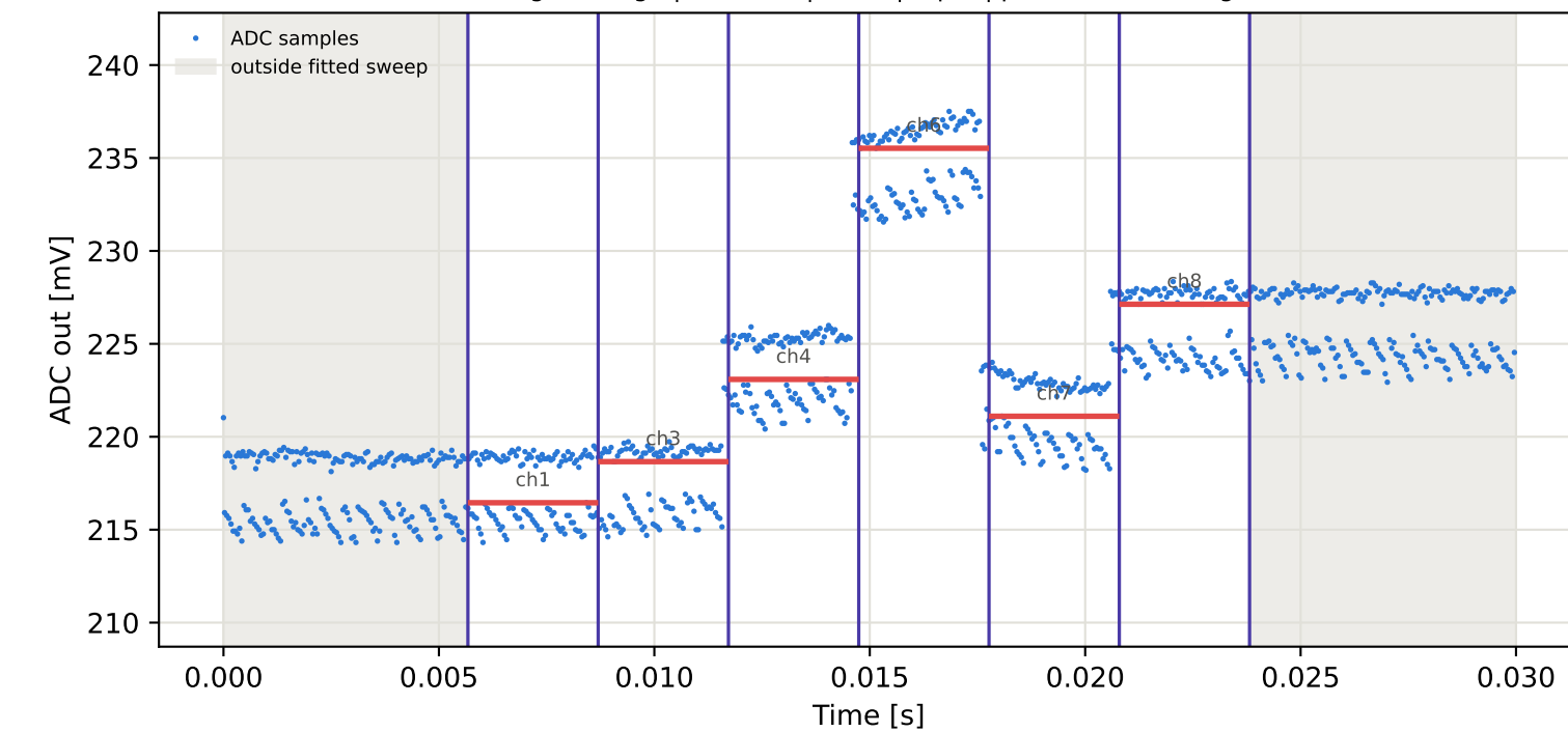
Tag2 &lt;- Tag15 | 905 MHz | run 0 | rep 1 | phase -55.59 deg
