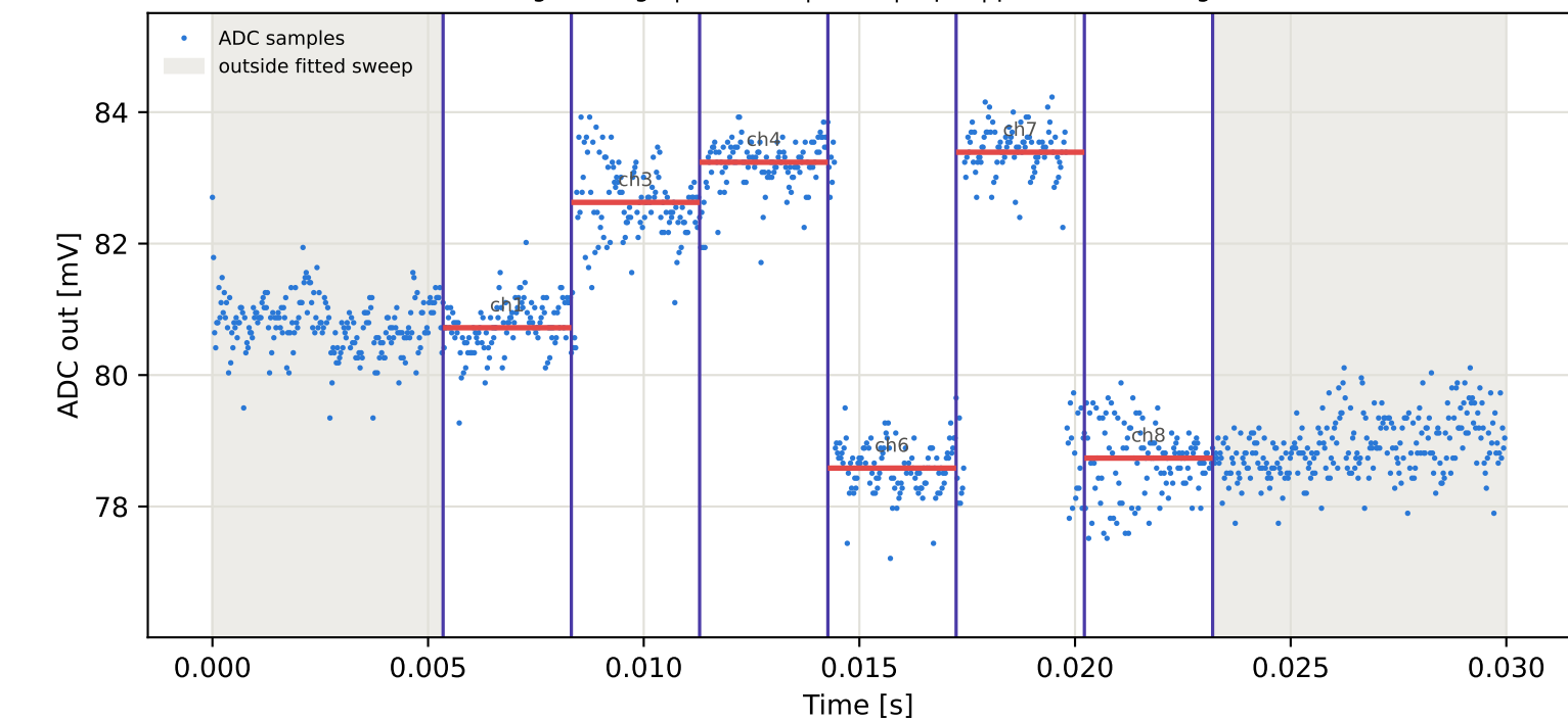
Tag4 &lt;- Tag2 | 785 MHz | run 0 | rep 1 | phase -23.94 deg
