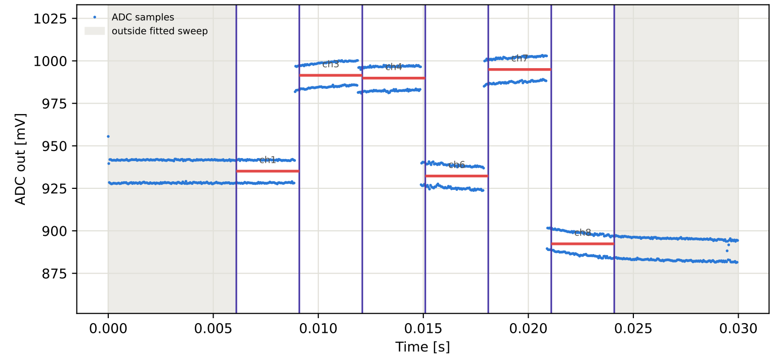
Tag5 &lt;- Tag1 | 875 MHz | run 0 | rep 1 | phase -143.91 deg
