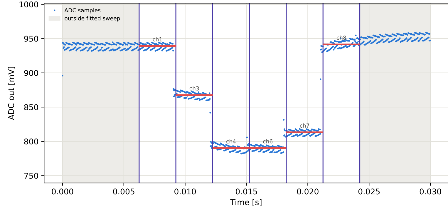
Tag8 &lt;- Tag16 | 905 MHz | run 0 | rep 1 | phase 67.03 deg
