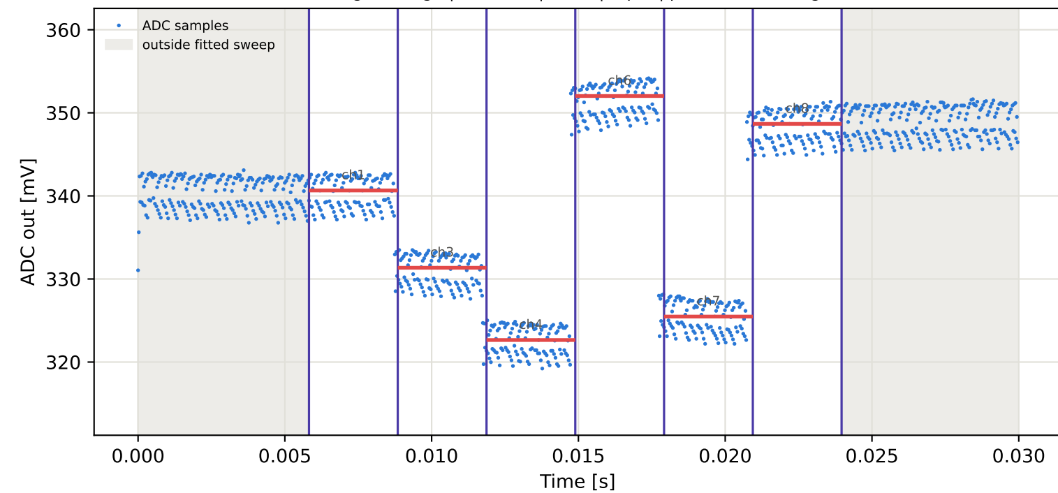
Tag1 &lt;- Tag8 | 965 MHz | run 0 | rep 1 | phase -58.15 deg
