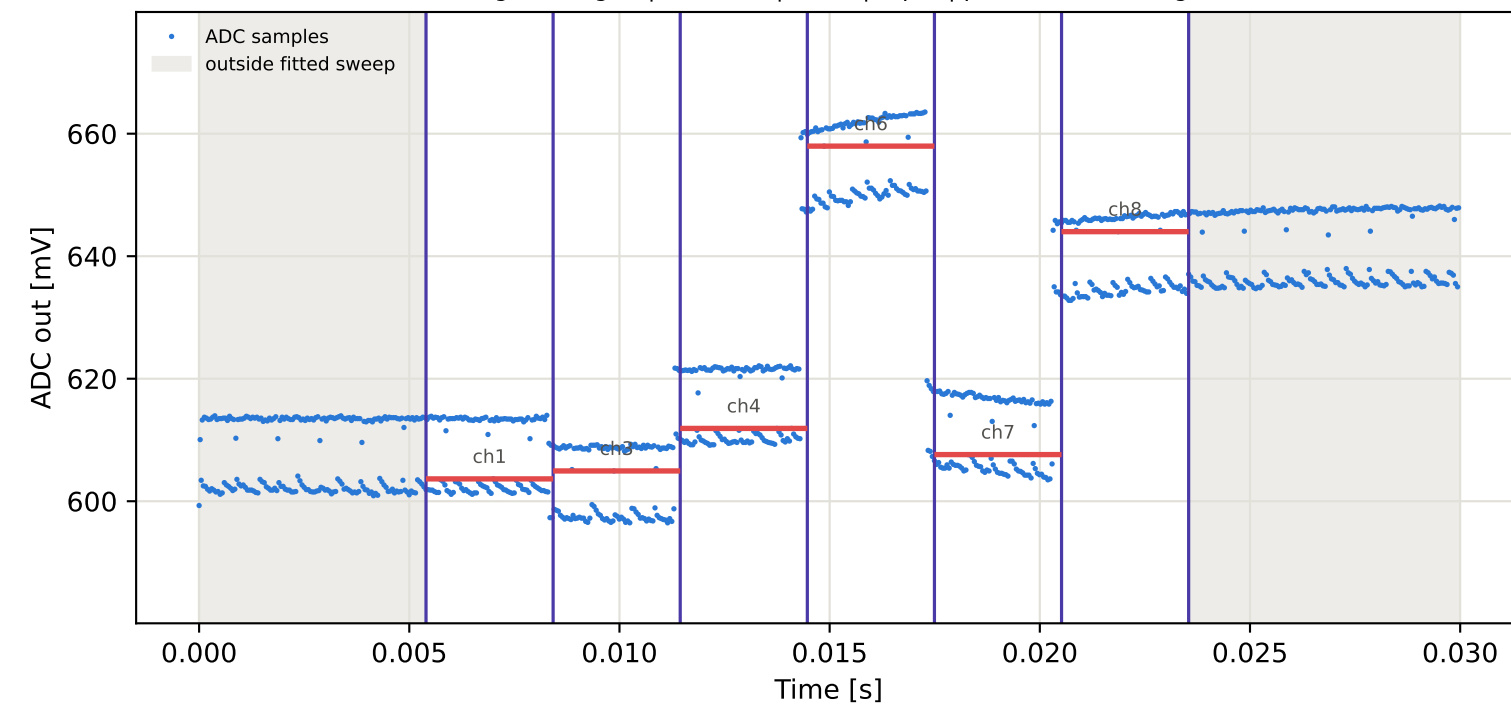
Tag6 &lt;- Tag2 | 905 MHz | run 0 | rep 1 | phase -45.72 deg
