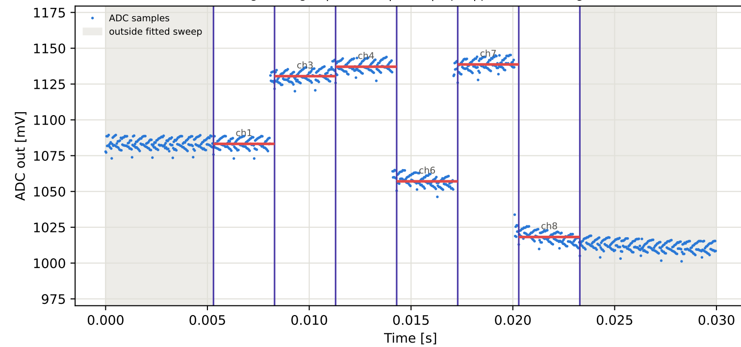
Tag4 &lt;- Tag2 | 895 MHz | run 0 | rep 1 | phase 148.44 deg
