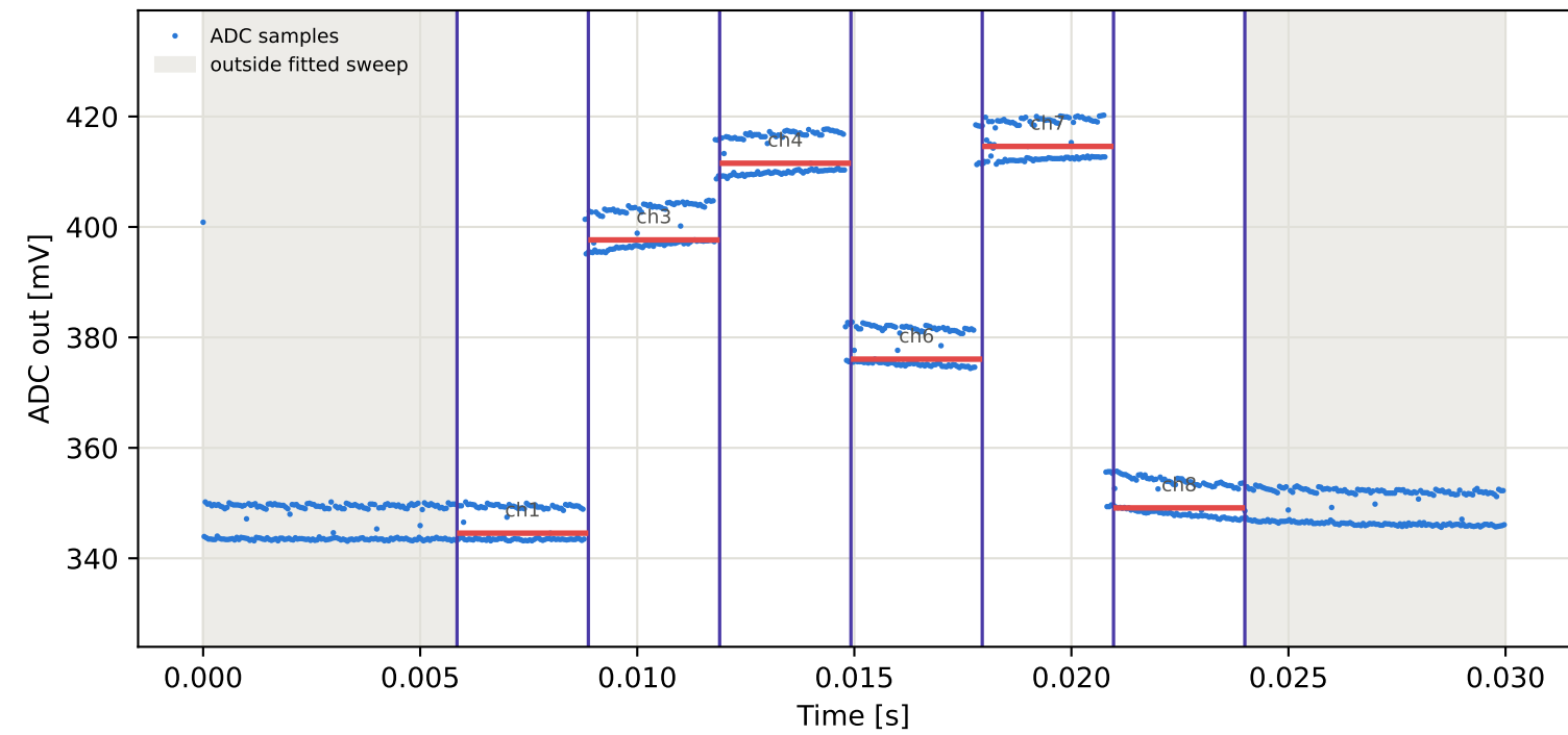
Tag16 &lt;- Tag1 | 845 MHz | run 0 | rep 1 | phase -76.86 deg
