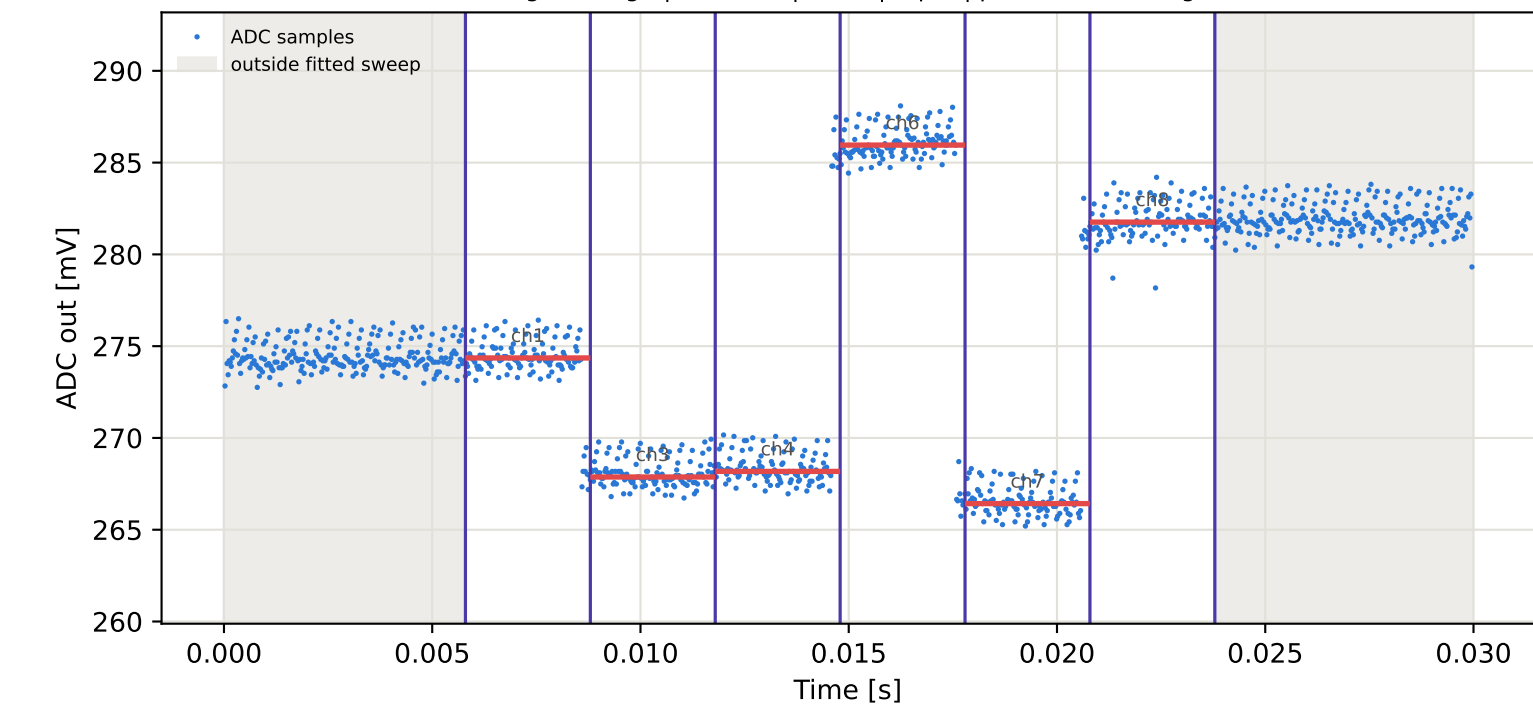
Tag1 &lt;- Tag9 | 985 MHz | run 0 | rep 1 | phase 46.00 deg
