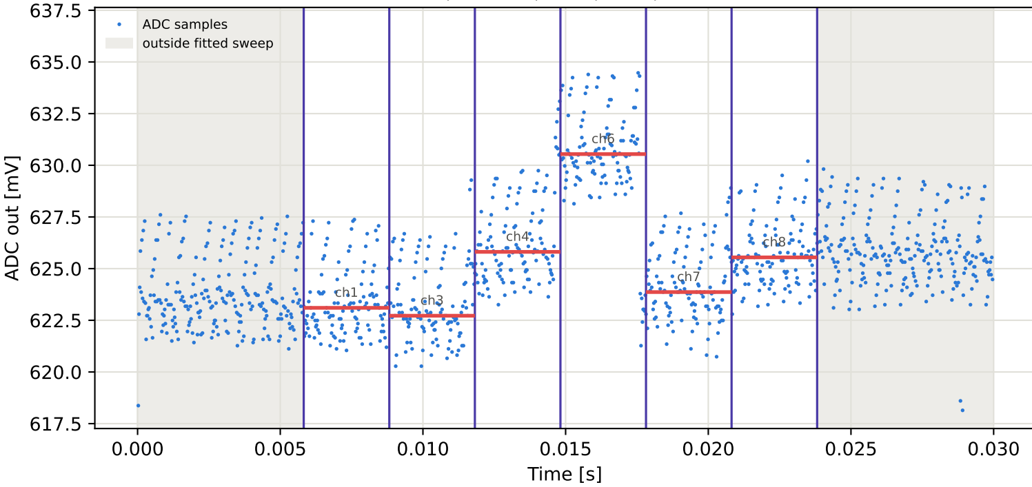
Tag16 &lt;- Tag10 | 955 MHz | run 0 | rep 1 | phase -158.18 deg
