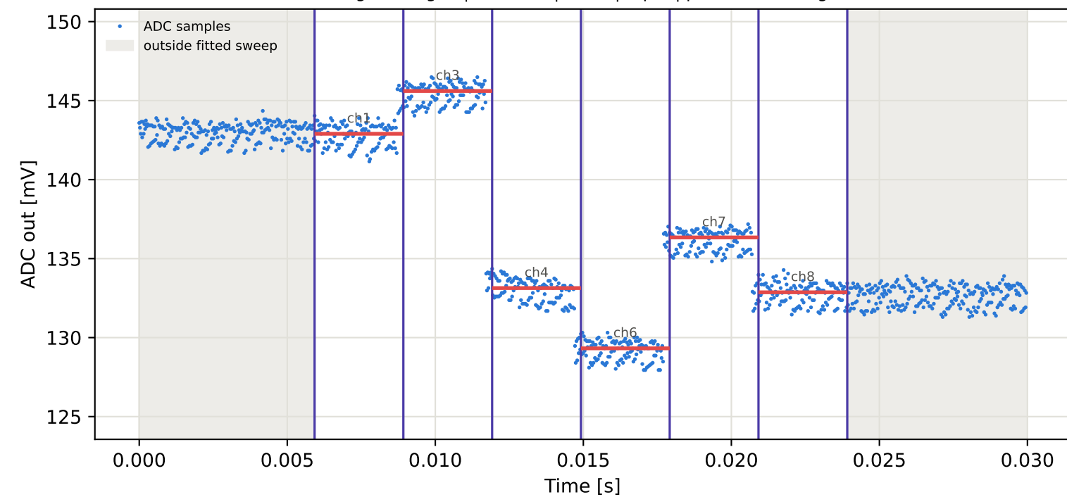
Tag2 &lt;- Tag16 | 845 MHz | run 0 | rep 1 | phase 39.90 deg
