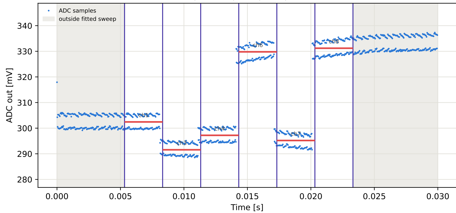
Tag7 &lt;- Tag15 | 895 MHz | run 0 | rep 1 | phase 172.41 deg
