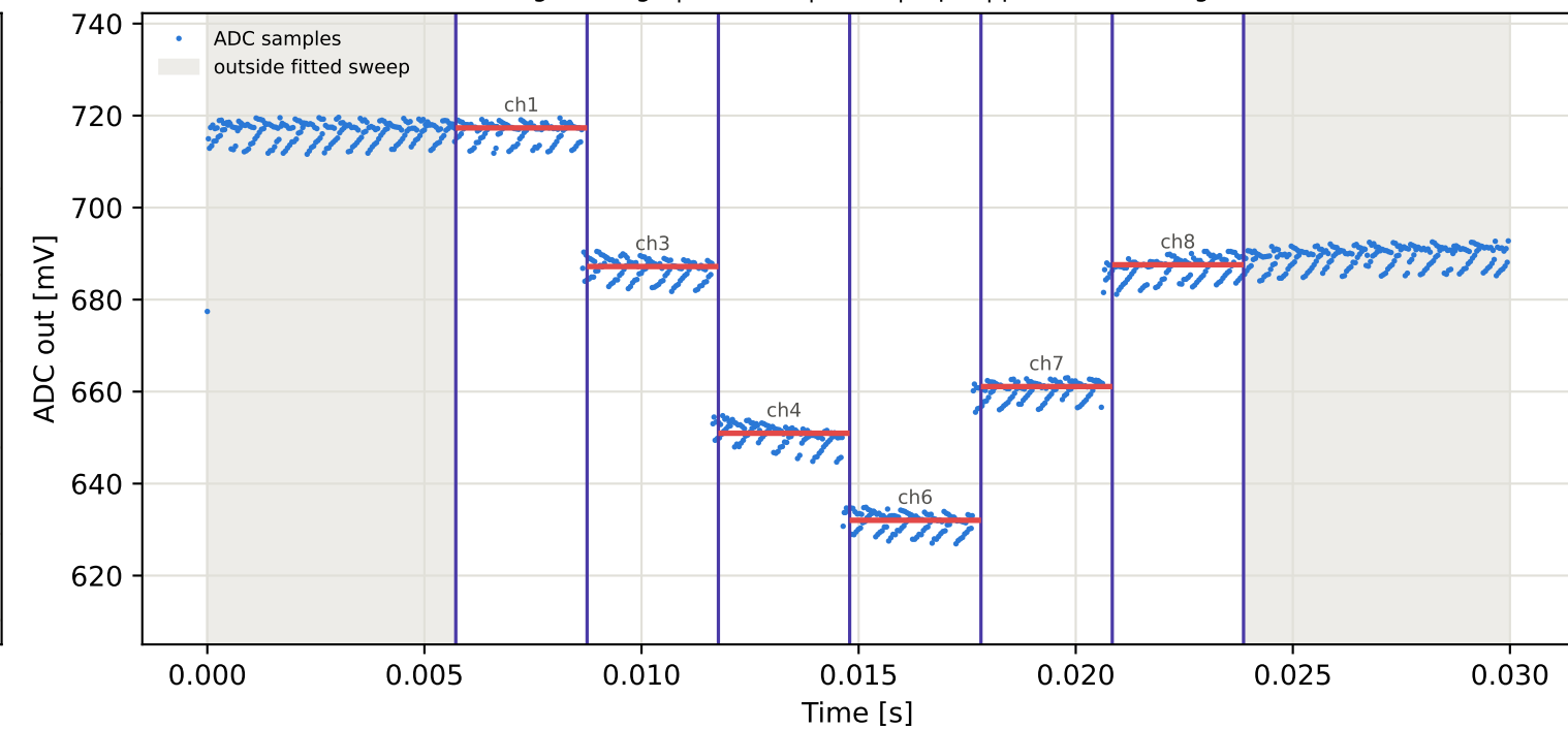
Tag6 &lt;- Tag5 | 895 MHz | run 0 | rep 1 | phase 51.08 deg
