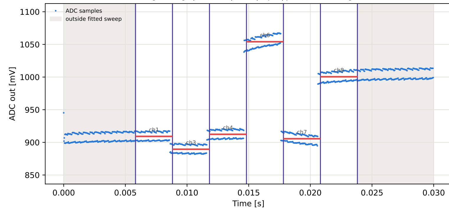
Tag4 &lt;- Tag7 | 915 MHz | run 0 | rep 1 | phase 45.70 deg
