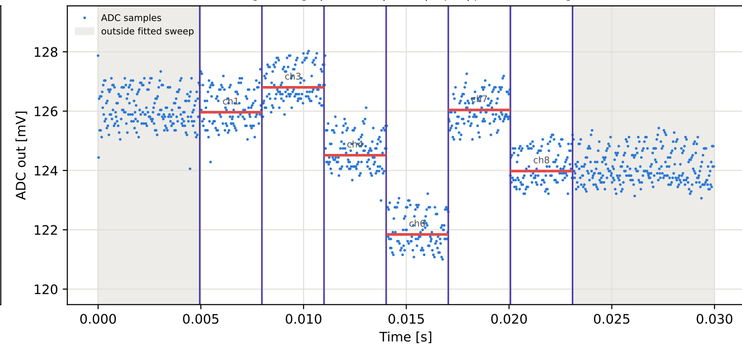
Tag5 &lt;- Tag9 | 975 MHz | run 0 | rep 1 | phase -154.45 deg
