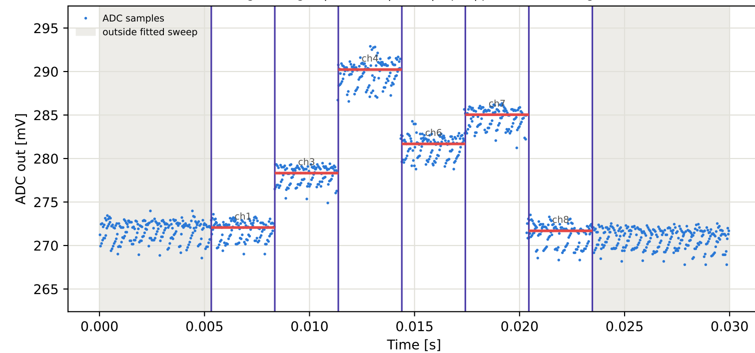
Tag6 &lt;- Tag2 | 955 MHz | run 0 | rep 1 | phase -116.73 deg
