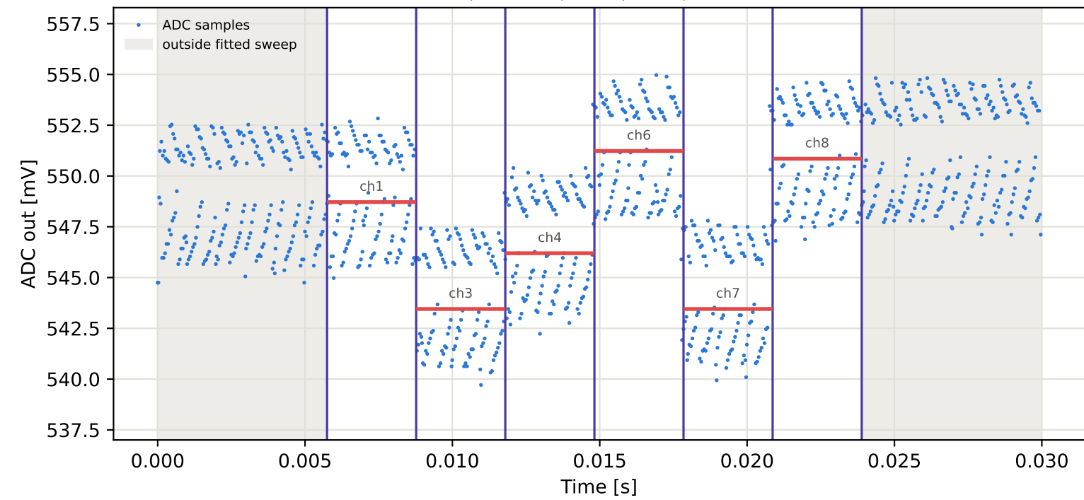
Tag5 &lt;- Tag1 | 825 MHz | run 0 | rep 1 | phase 168.52 deg
