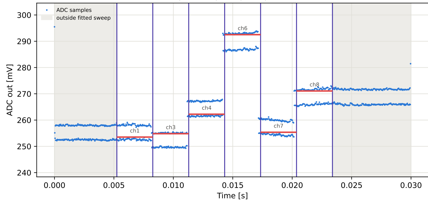
Tag6 &lt;- Tag4 | 945 MHz | run 0 | rep 1 | phase -168.50 deg
