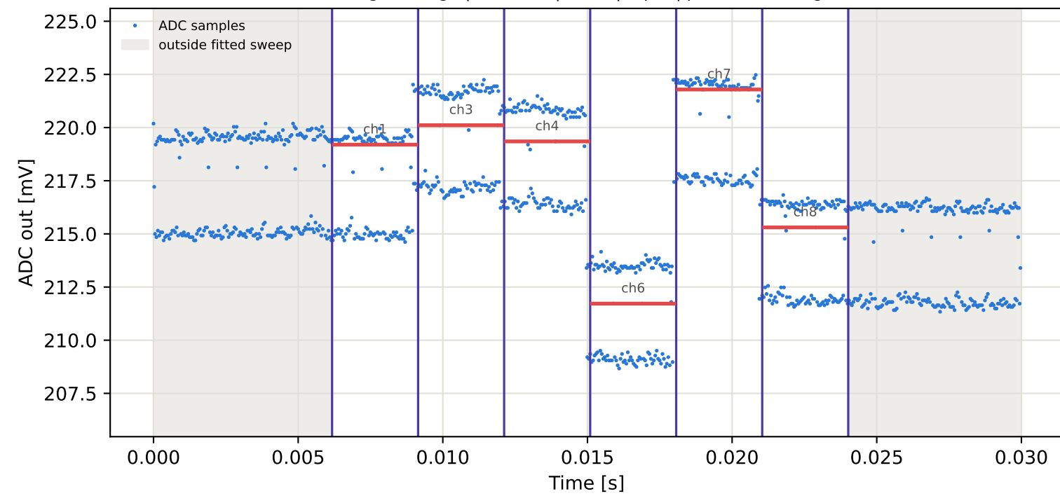
Tag9 &lt;- Tag15 | 995 MHz | run 0 | rep 1 | phase 97.45 deg
