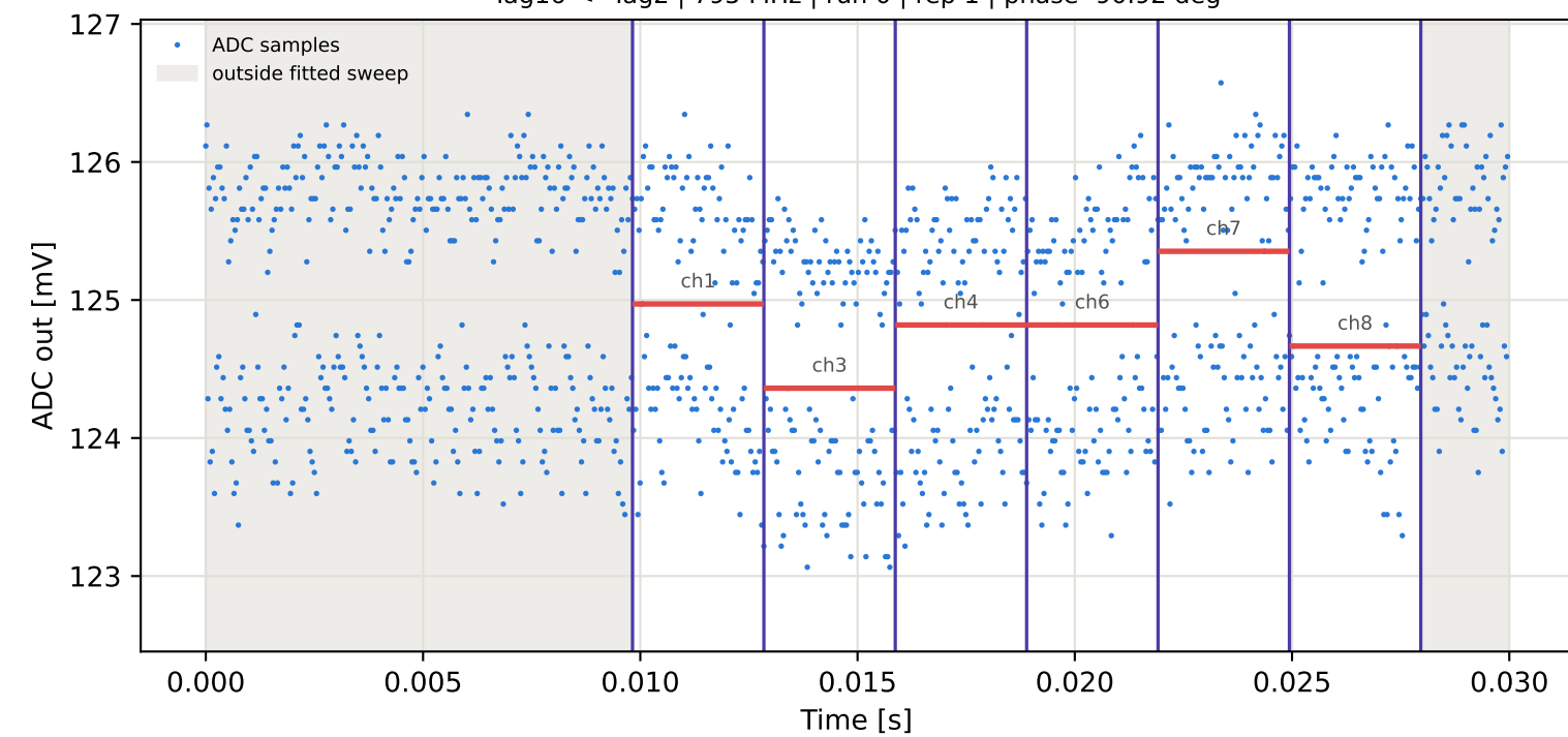
Tag16 &lt;- Tag4 | 795 MHz | run 0 | rep 1 | phase -159.09 deg
