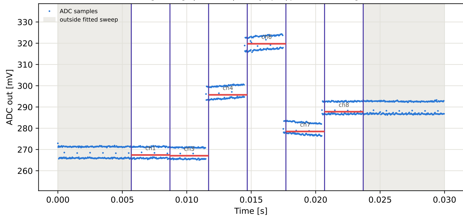
Tag3 &lt;- Tag15 | 965 MHz | run 0 | rep 1 | phase 39.37 deg
