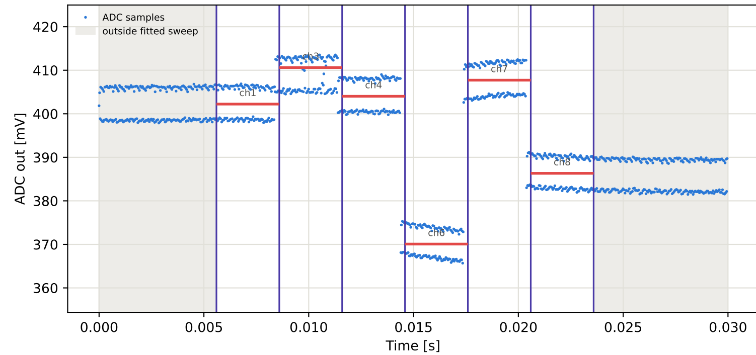
Tag1 &lt;- Tag2 | 955 MHz | run 0 | rep 1 | phase 36.35 deg
