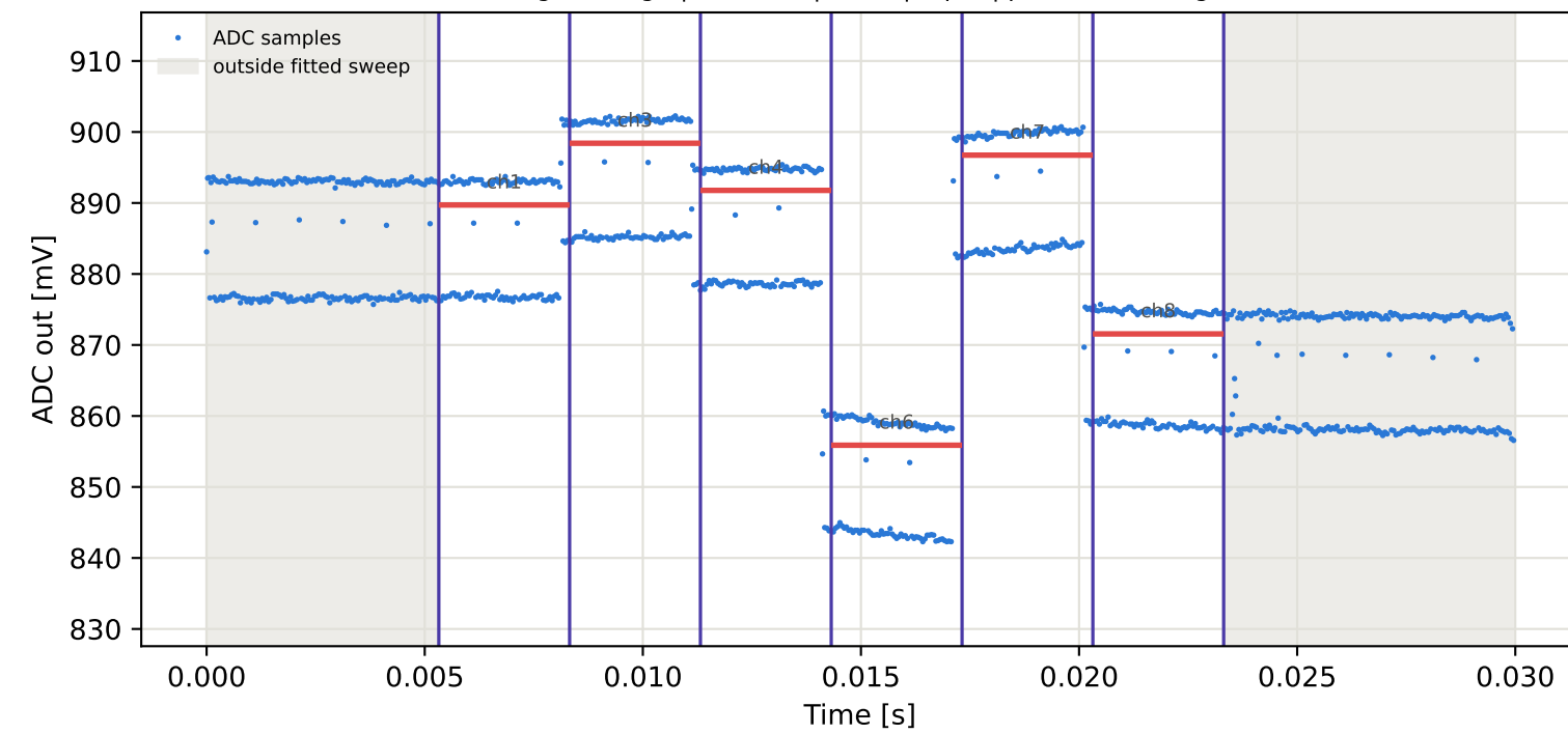
Tag4 &lt;- Tag15 | 945 MHz | run 0 | rep 1 | phase 25.48 deg
