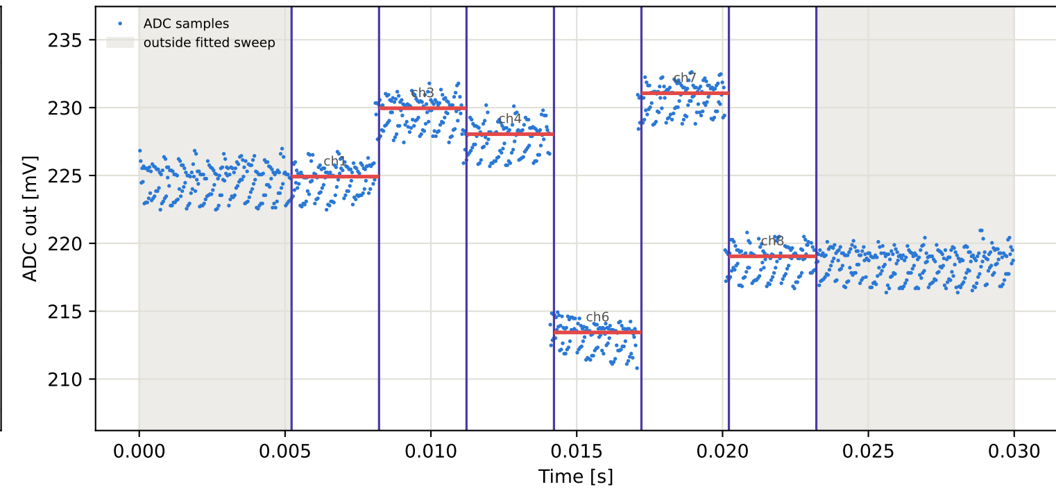
Tag7 &lt;- Tag6 | 995 MHz | run 0 | rep 1 | phase 158.63 deg
