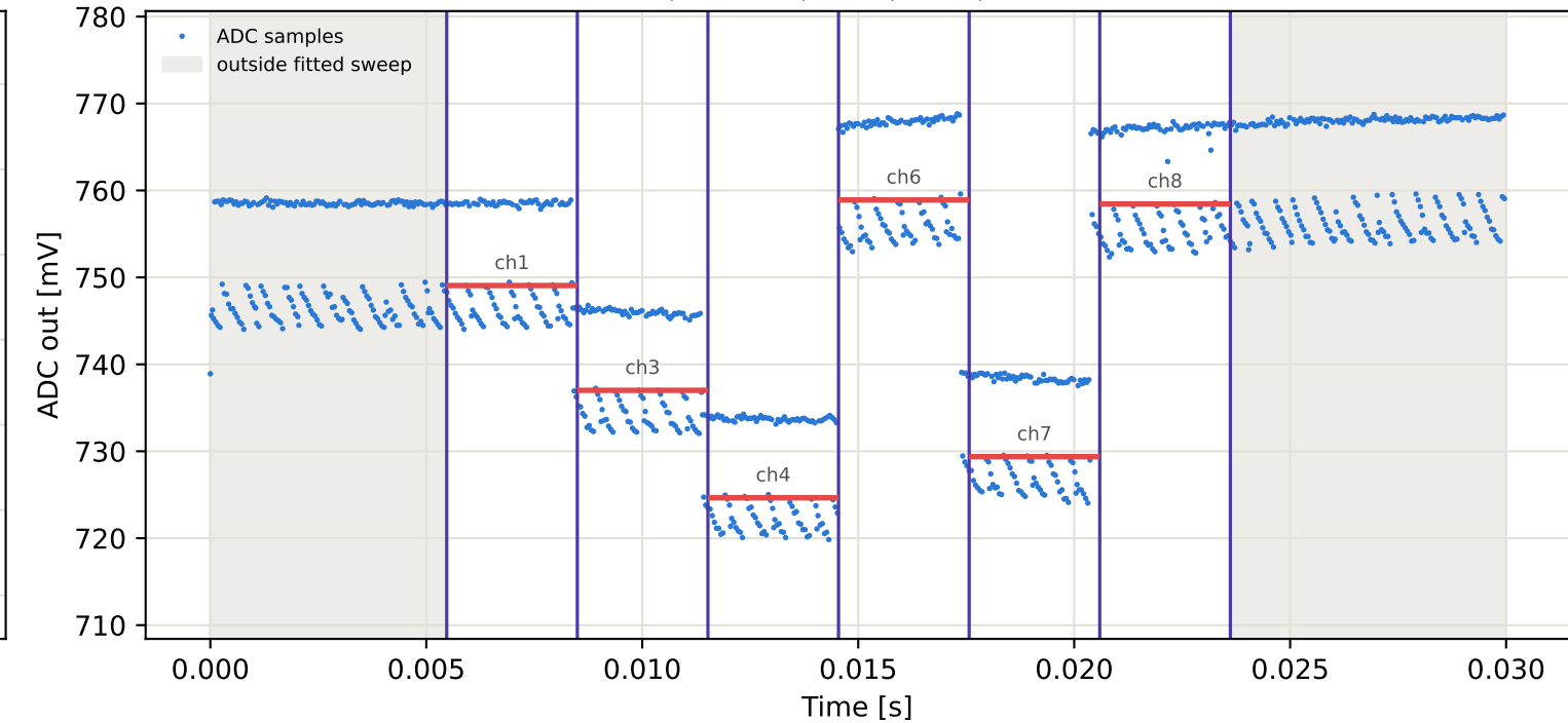
Tag8 &lt;- Tag7 | 965 MHz | run 0 | rep 1 | phase 122.50 deg
