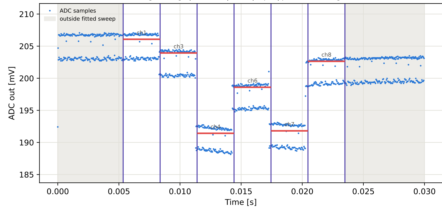
Tag8 &lt;- Tag5 | 805 MHz | run 0 | rep 1 | phase 164.22 deg
