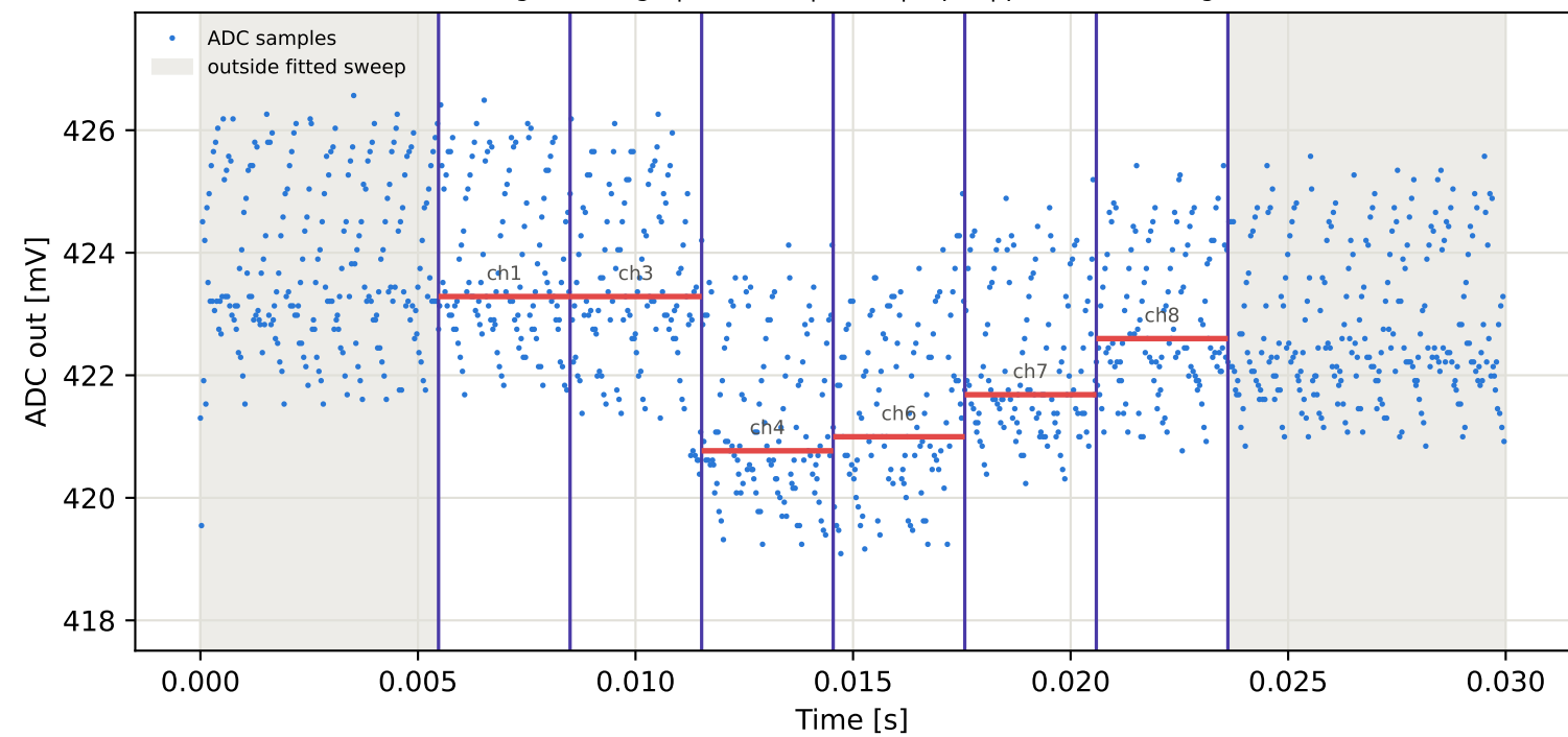
Tag15 &lt;- Tag4 | 825 MHz | run 0 | rep 1 | phase -160.39 deg
