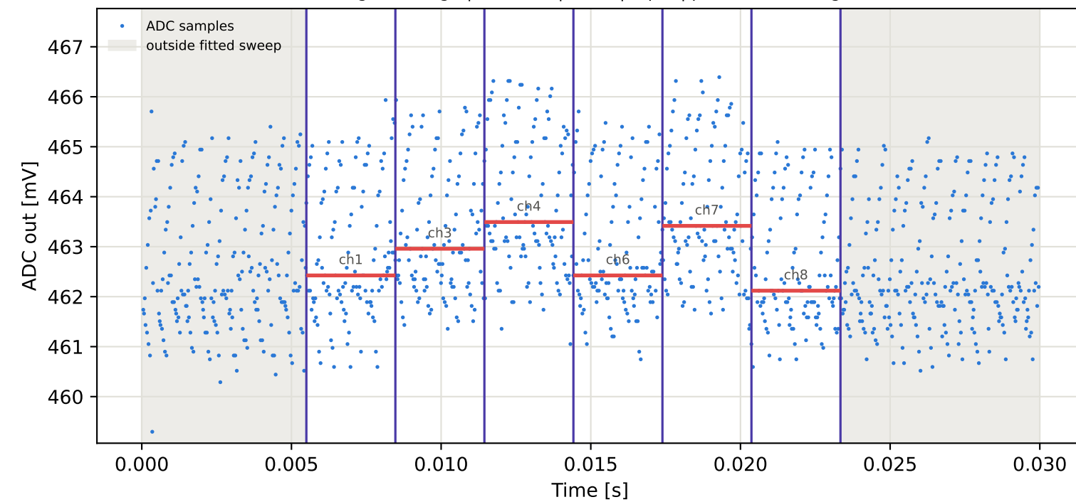
Tag15 &lt;- Tag9 | 855 MHz | run 0 | rep 1 | phase -151.59 deg
