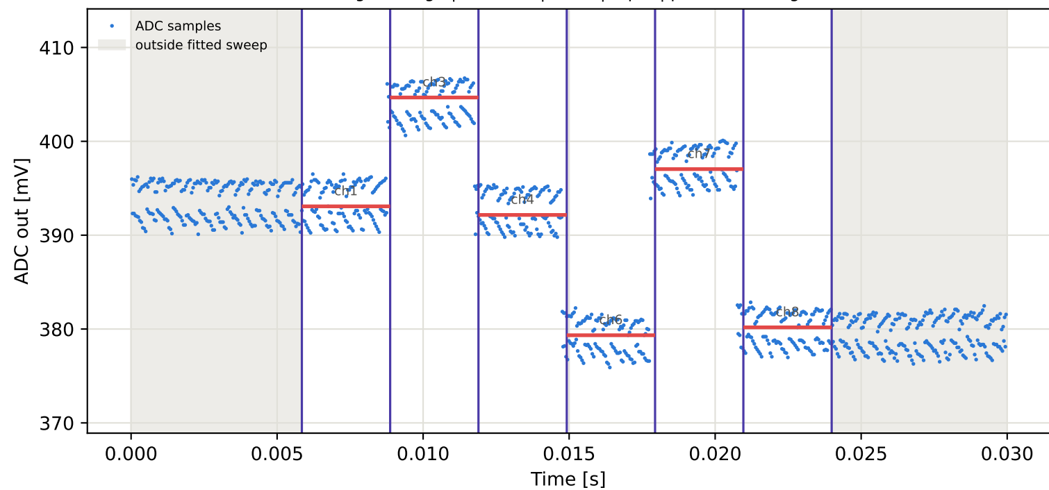
Tag6 &lt;- Tag5 | 855 MHz | run 0 | rep 1 | phase 8.86 deg
