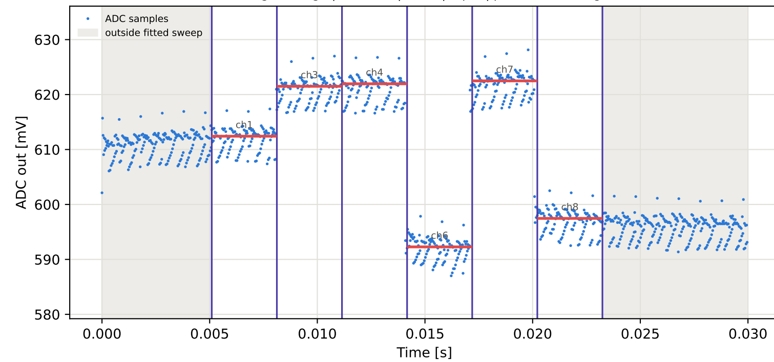
Tag9 &lt;- Tag10 | 925 MHz | run 0 | rep 1 | phase 119.64 deg
