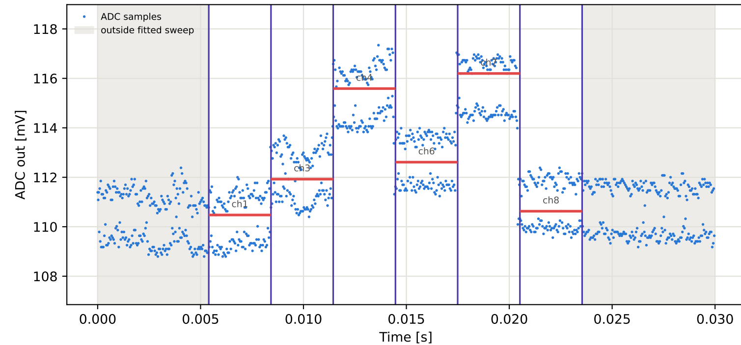
Tag16 &lt;- Tag10 | 775 MHz | run 0 | rep 1 | phase -52.54 deg
