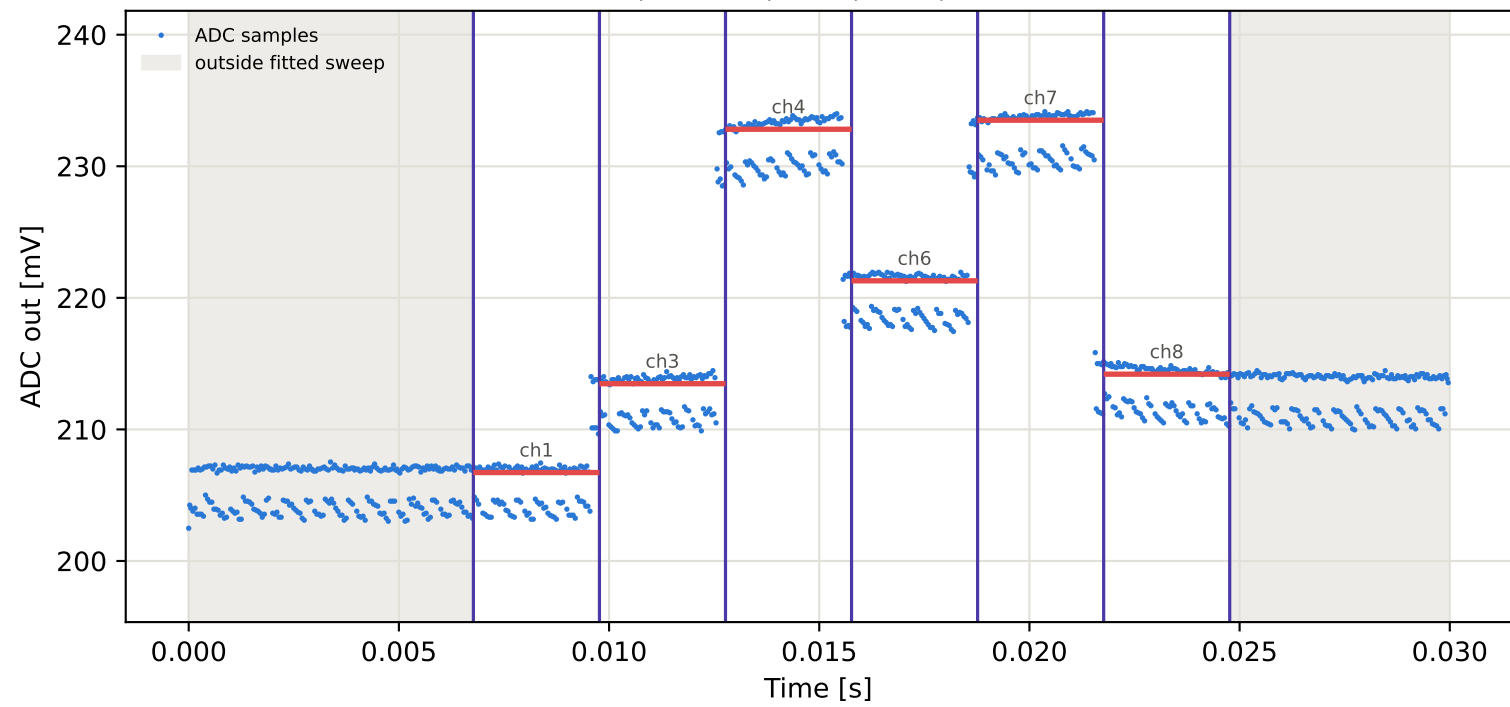
Tag5 &lt;- Tag4 | 805 MHz | run 0 | rep 1 | phase -92.49 deg
