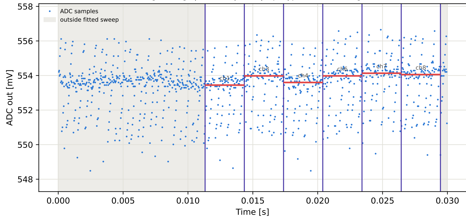
Tag5 &lt;- Tag9 | 845 MHz | run 0 | rep 1 | phase 15.93 deg
