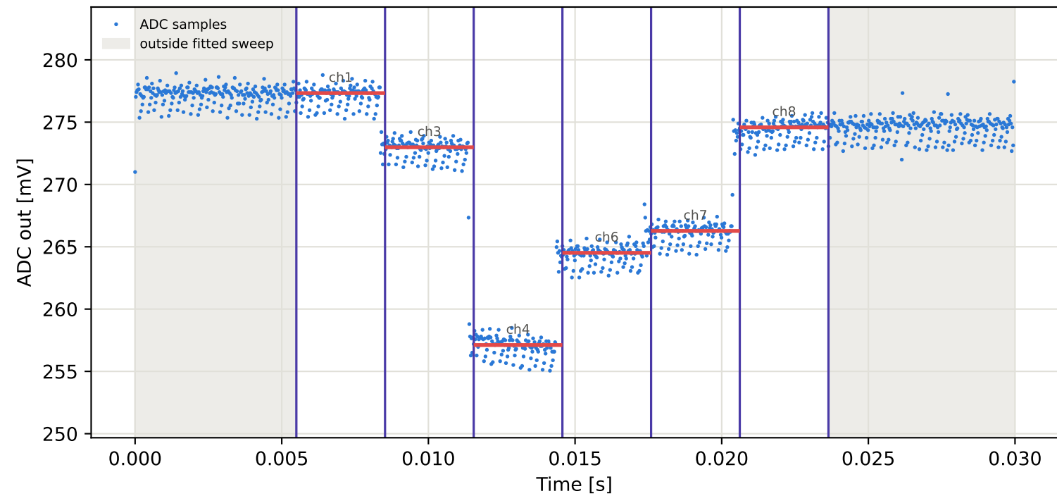
Tag1 &lt;- Tag2 | 985 MHz | run 0 | rep 1 | phase -67.94 deg
