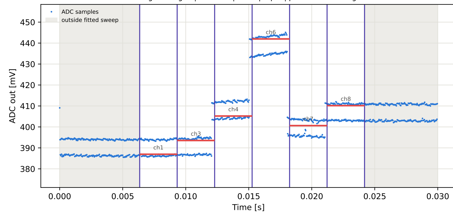
Tag7 &lt;- Tag10 | 935 MHz | run 0 | rep 1 | phase -157.56 deg
