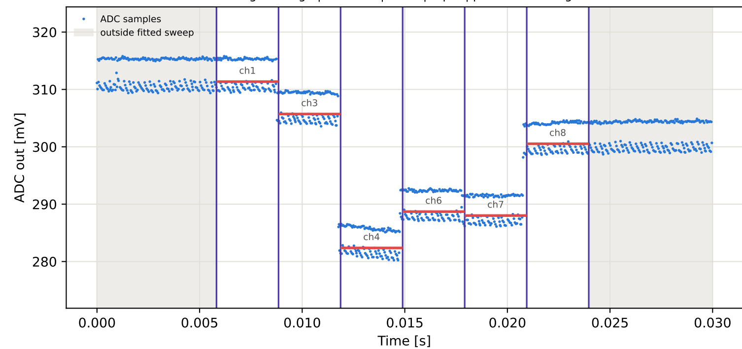
Tag3 &lt;- Tag7 | 835 MHz | run 0 | rep 1 | phase 86.67 deg
