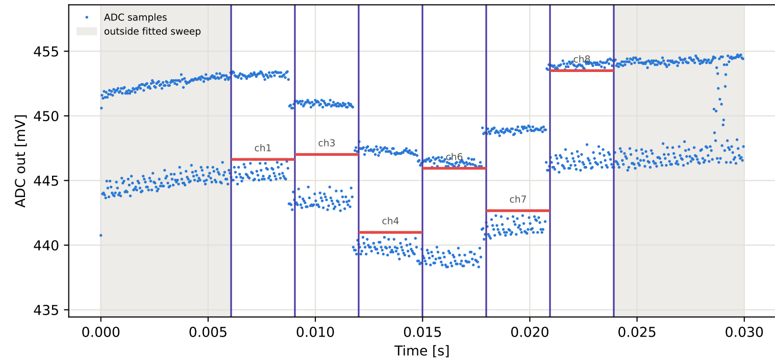
Tag1 &lt;- Tag4 | 895 MHz | run 0 | rep 1 | phase -141.32 deg
