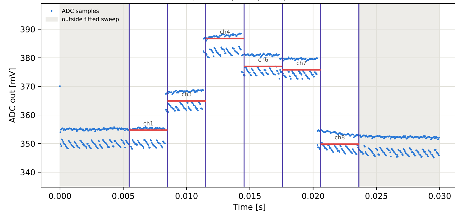
Tag9 &lt;- Tag5 | 925 MHz | run 0 | rep 1 | phase -51.40 deg
