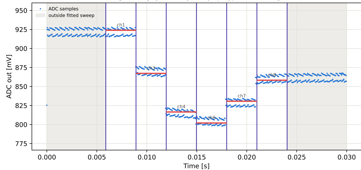
Tag16 &lt;- Tag1 | 875 MHz | run 0 | rep 1 | phase 32.57 deg
