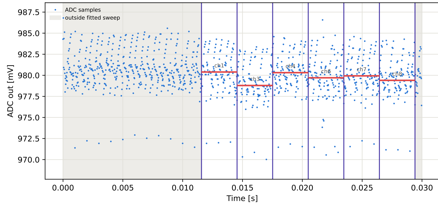
Tag5 &lt;- Tag4 | 865 MHz | run 0 | rep 1 | phase 22.85 deg
