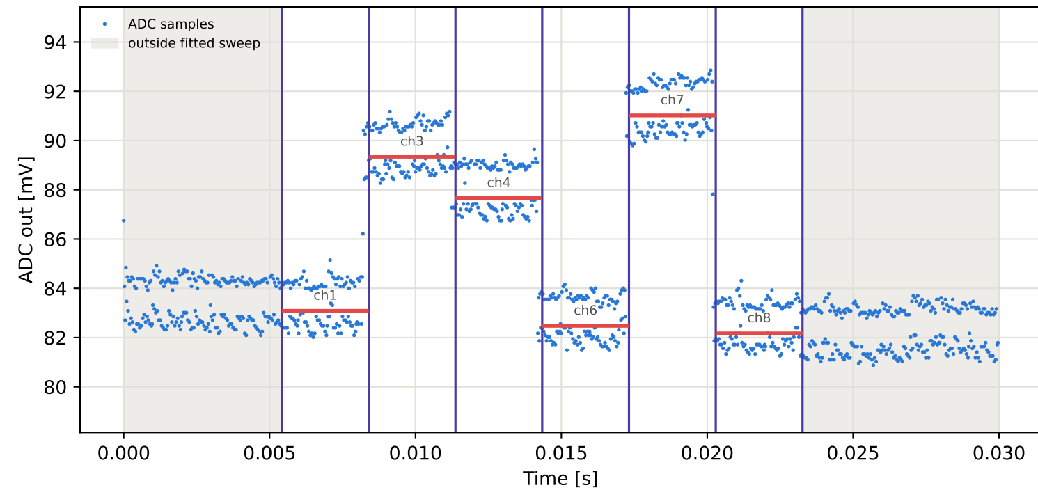
Tag9 &lt;- Tag6 | 795 MHz | run 0 | rep 1 | phase -81.16 deg
