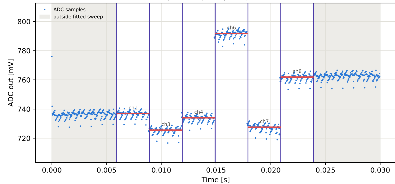
Tag4 &lt;- Tag7 | 955 MHz | run 0 | rep 1 | phase -168.53 deg
