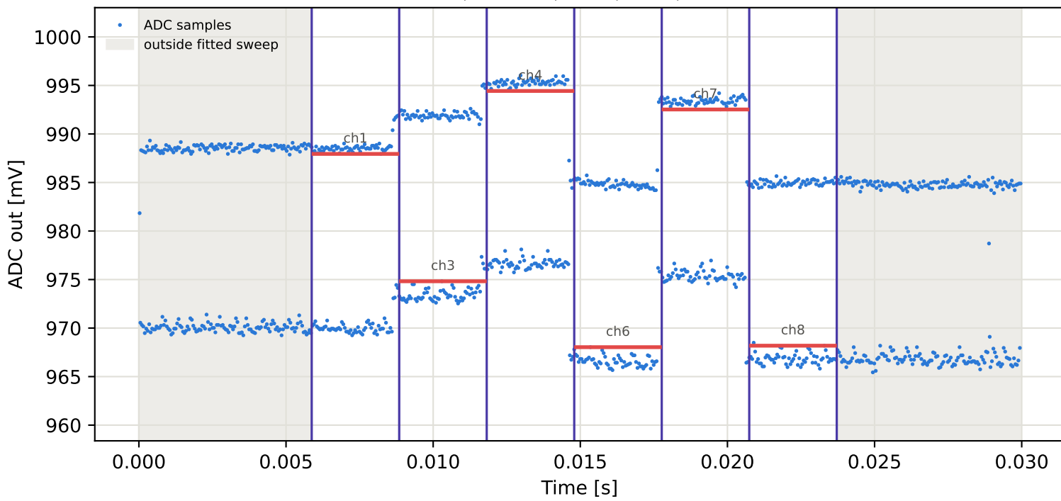
Tag15 &lt;- Tag10 | 955 MHz | run 0 | rep 1 | phase -51.59 deg
