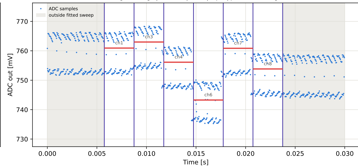
Tag16 &lt;- Tag15 | 965 MHz | run 0 | rep 1 | phase 17.49 deg
