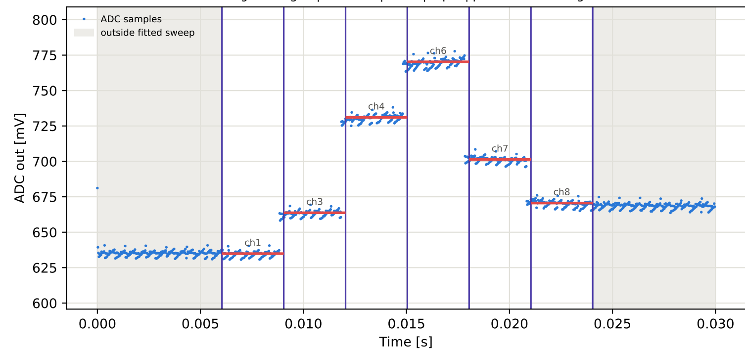
Tag5 &lt;- Tag2 | 935 MHz | run 0 | rep 1 | phase 46.87 deg
