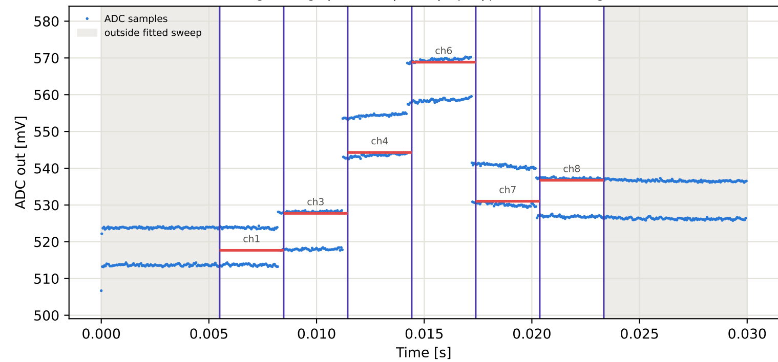
Tag9 &lt;- Tag6 | 945 MHz | run 0 | rep 1 | phase -151.79 deg
