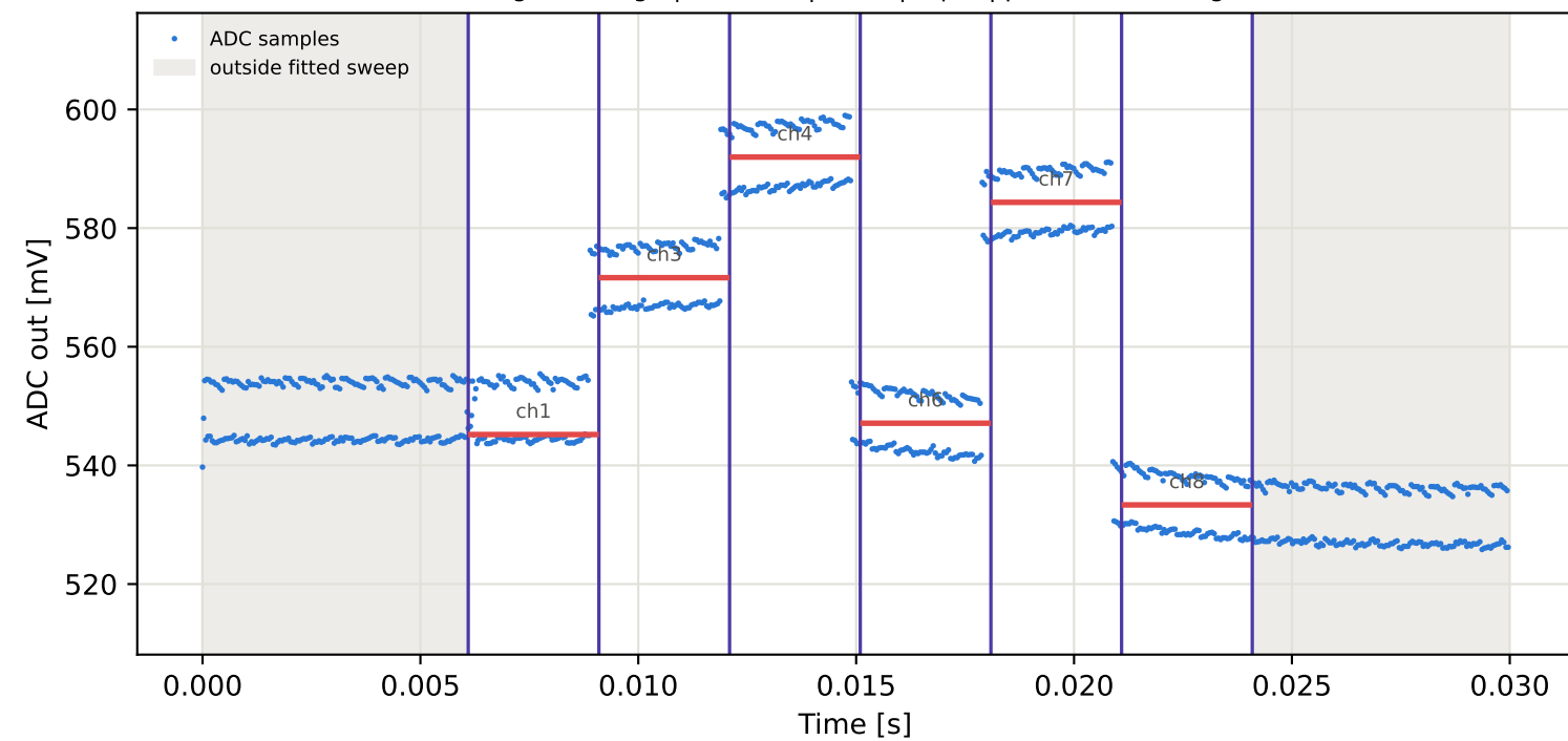
Tag15 &lt;- Tag10 | 935 MHz | run 0 | rep 1 | phase -137.28 deg
