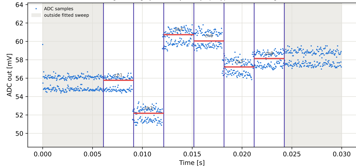
Tag10 &lt;- Tag5 | 785 MHz | run 0 | rep 1 | phase -100.84 deg
