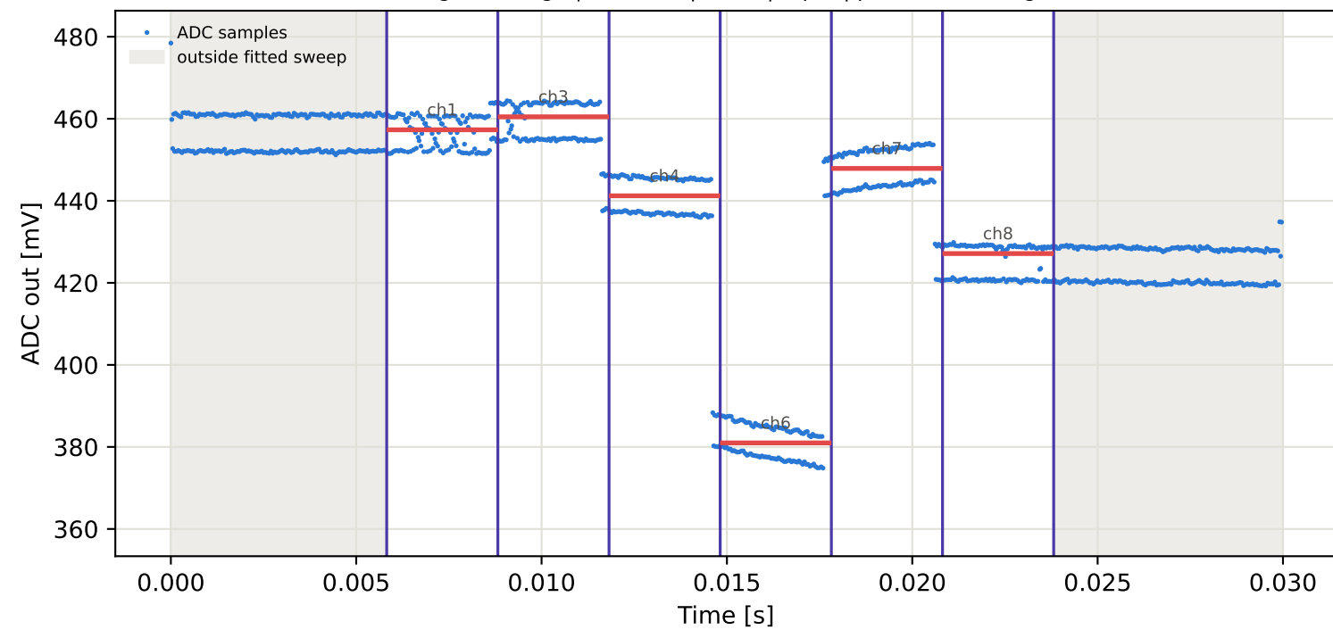
Tag10 &lt;- Tag8 | 915 MHz | run 0 | rep 1 | phase -4.05 deg
