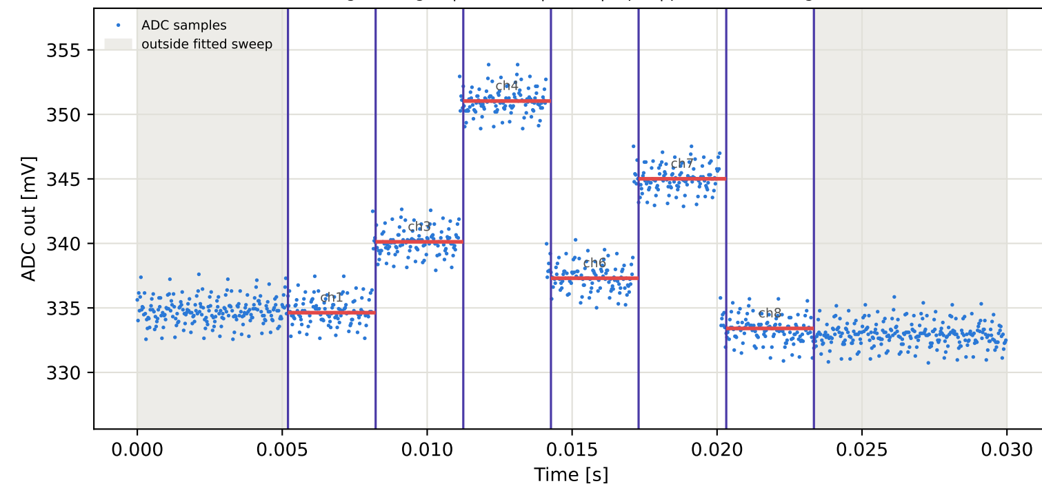
Tag1 &lt;- Tag16 | 975 MHz | run 0 | rep 1 | phase 141.82 deg
