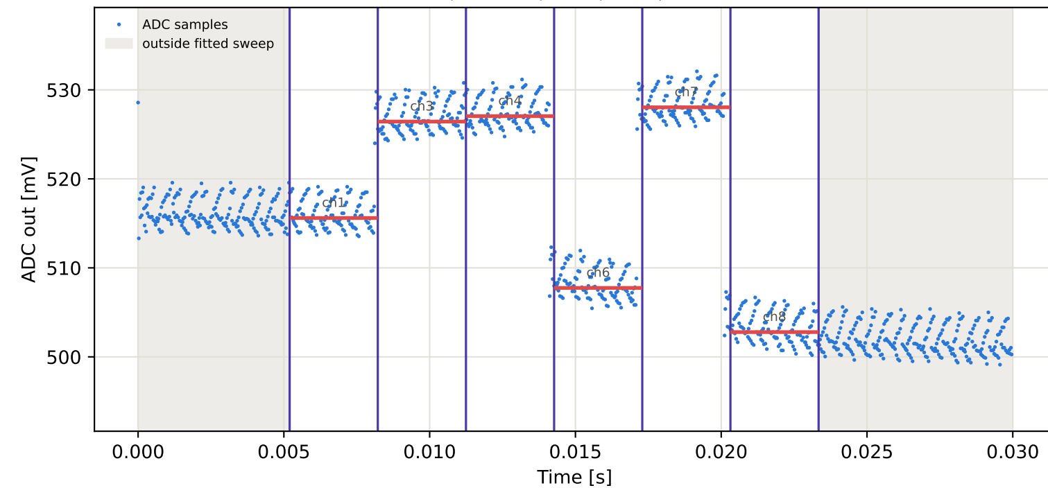
Tag9 &lt;- Tag7 | 895 MHz | run 0 | rep 1 | phase -34.81 deg
