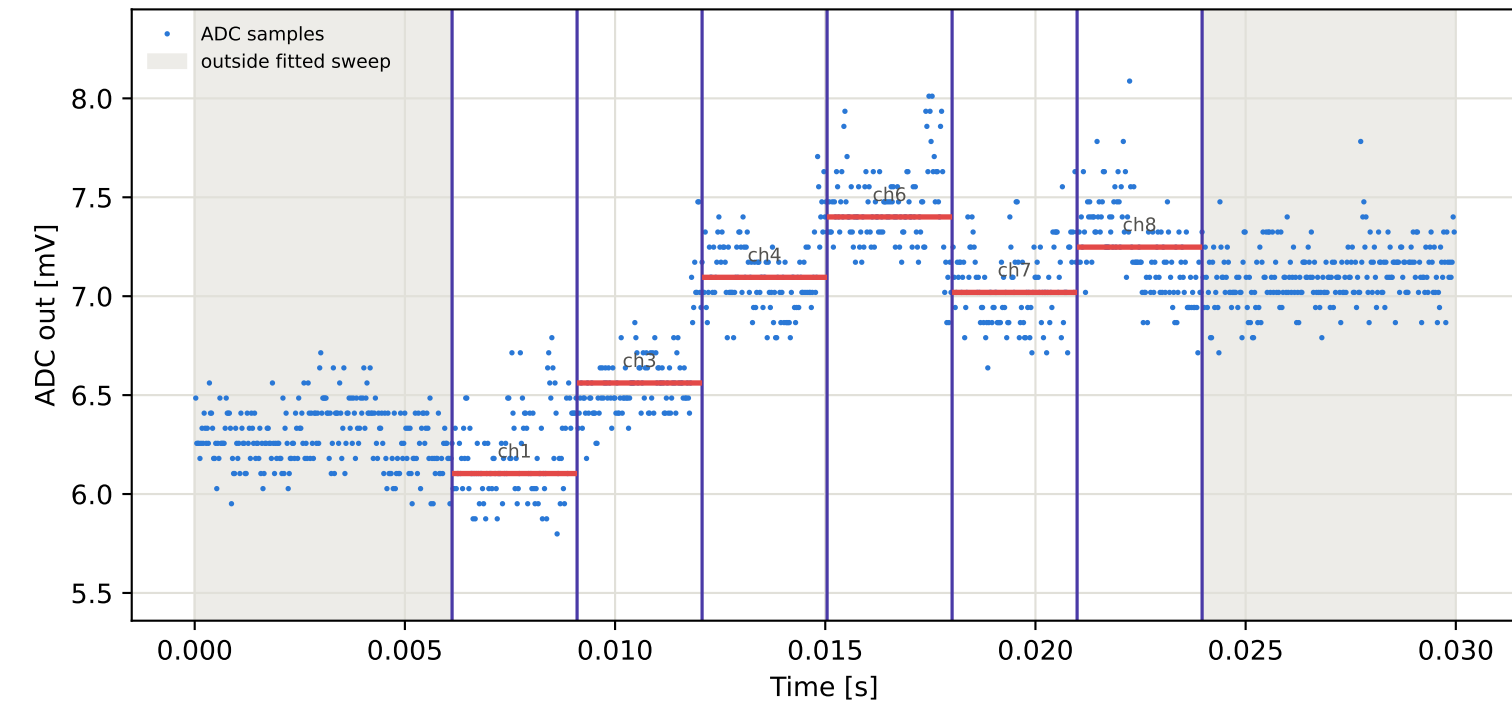
Tag2 &lt;- Tag16 | 865 MHz | run 0 | rep 1 | phase 133.73 deg
