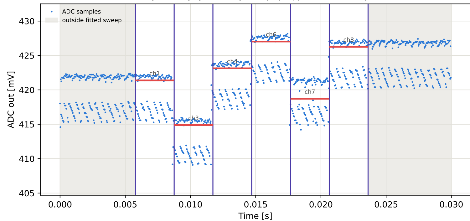
Tag15 &lt;- Tag6 | 825 MHz | run 0 | rep 1 | phase 124.04 deg
