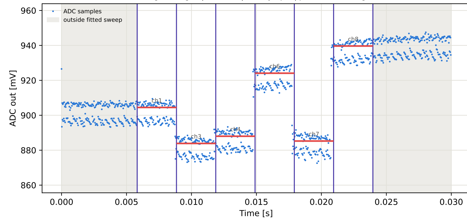
Tag6 &lt;- Tag2 | 885 MHz | run 0 | rep 1 | phase 125.94 deg
