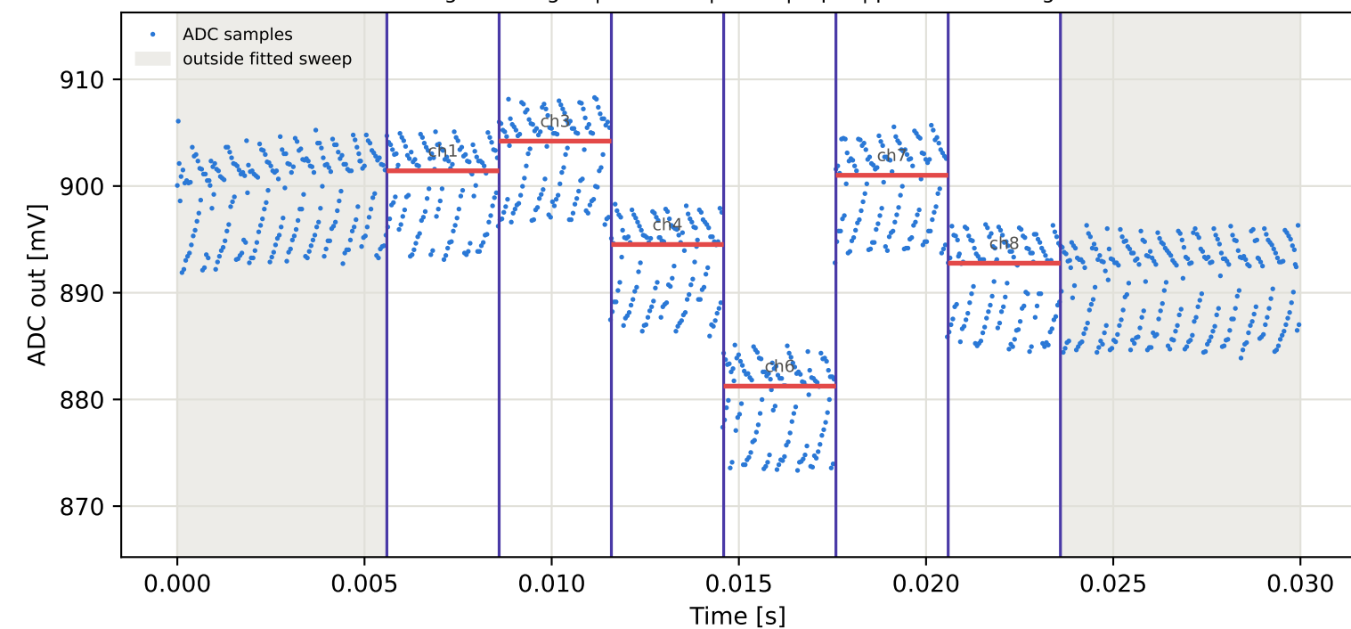
Tag15 &lt;- Tag3 | 975 MHz | run 0 | rep 1 | phase 72.21 deg
