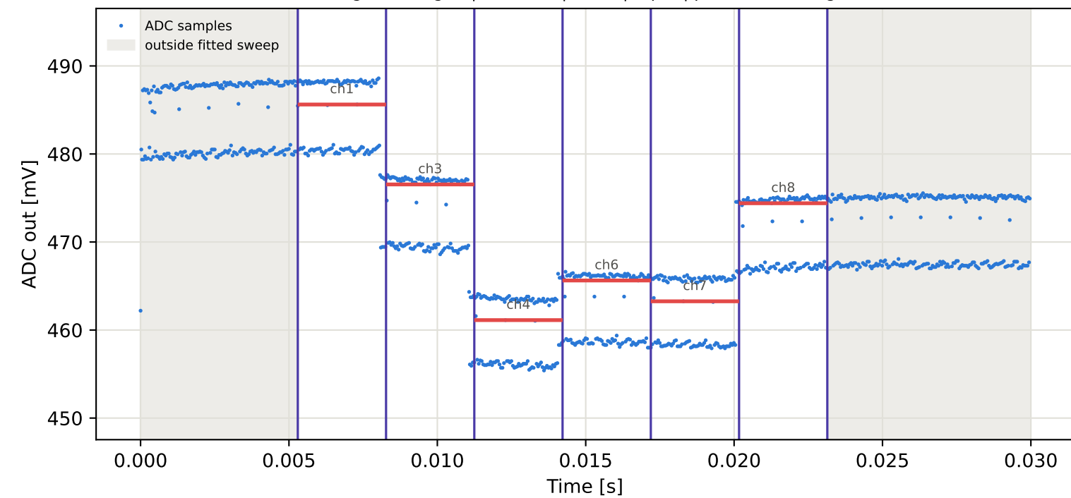
Tag15 &lt;- Tag3 | 855 MHz | run 0 | rep 1 | phase 31.67 deg
