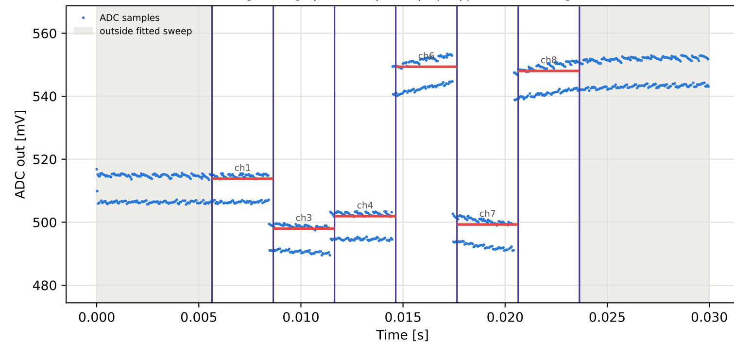
Tag9 &lt;- Tag5 | 895 MHz | run 0 | rep 1 | phase -108.15 deg
