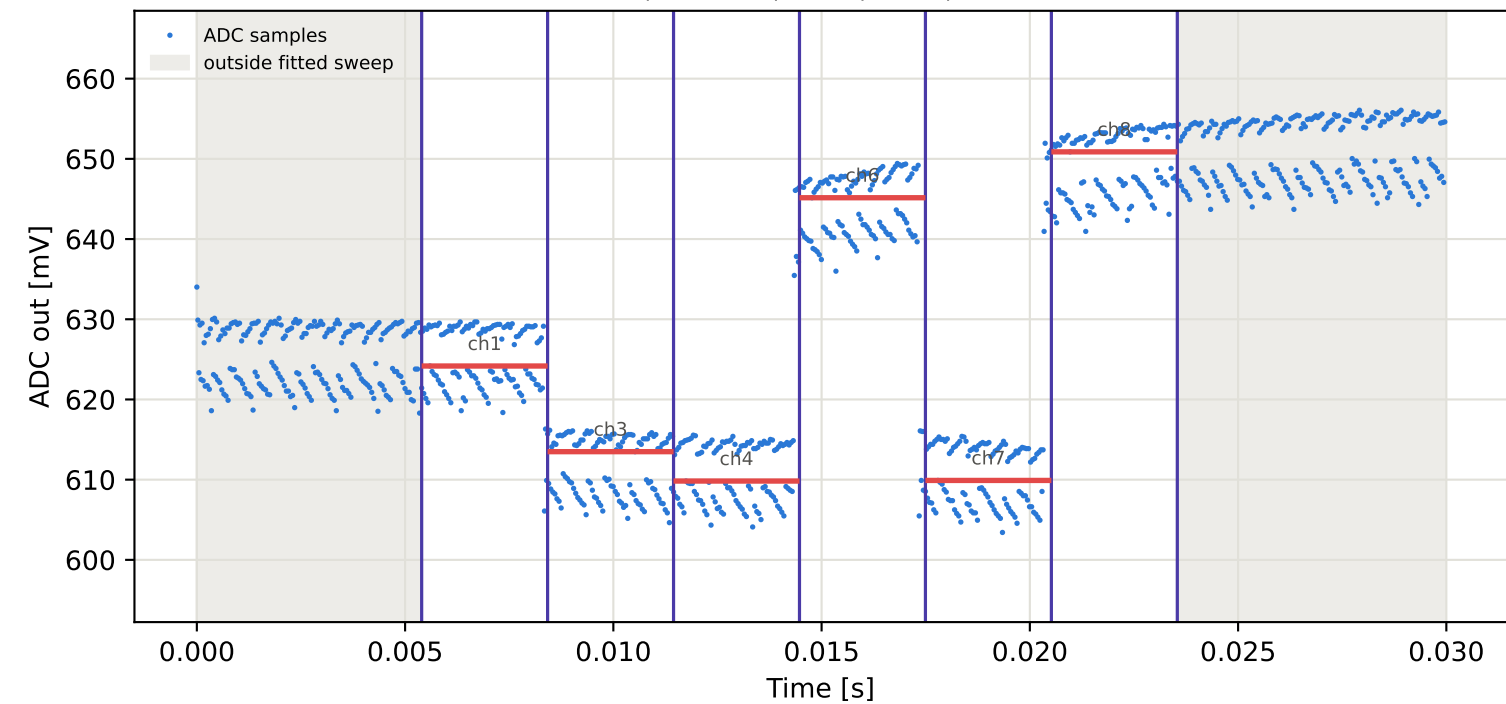
Tag7 &lt;- Tag15 | 905 MHz | run 0 | rep 1 | phase 152.86 deg
