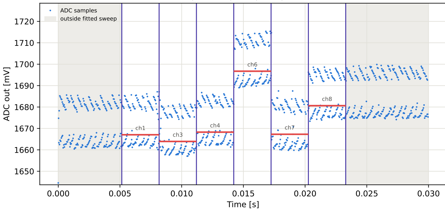
Tag15 &lt;- Tag10 | 925 MHz | run 0 | rep 1 | phase -173.44 deg
