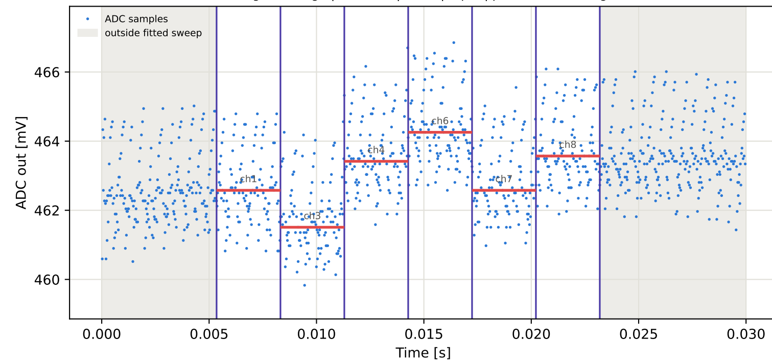
Tag16 &lt;- Tag10 | 855 MHz | run 0 | rep 1 | phase -99.33 deg
