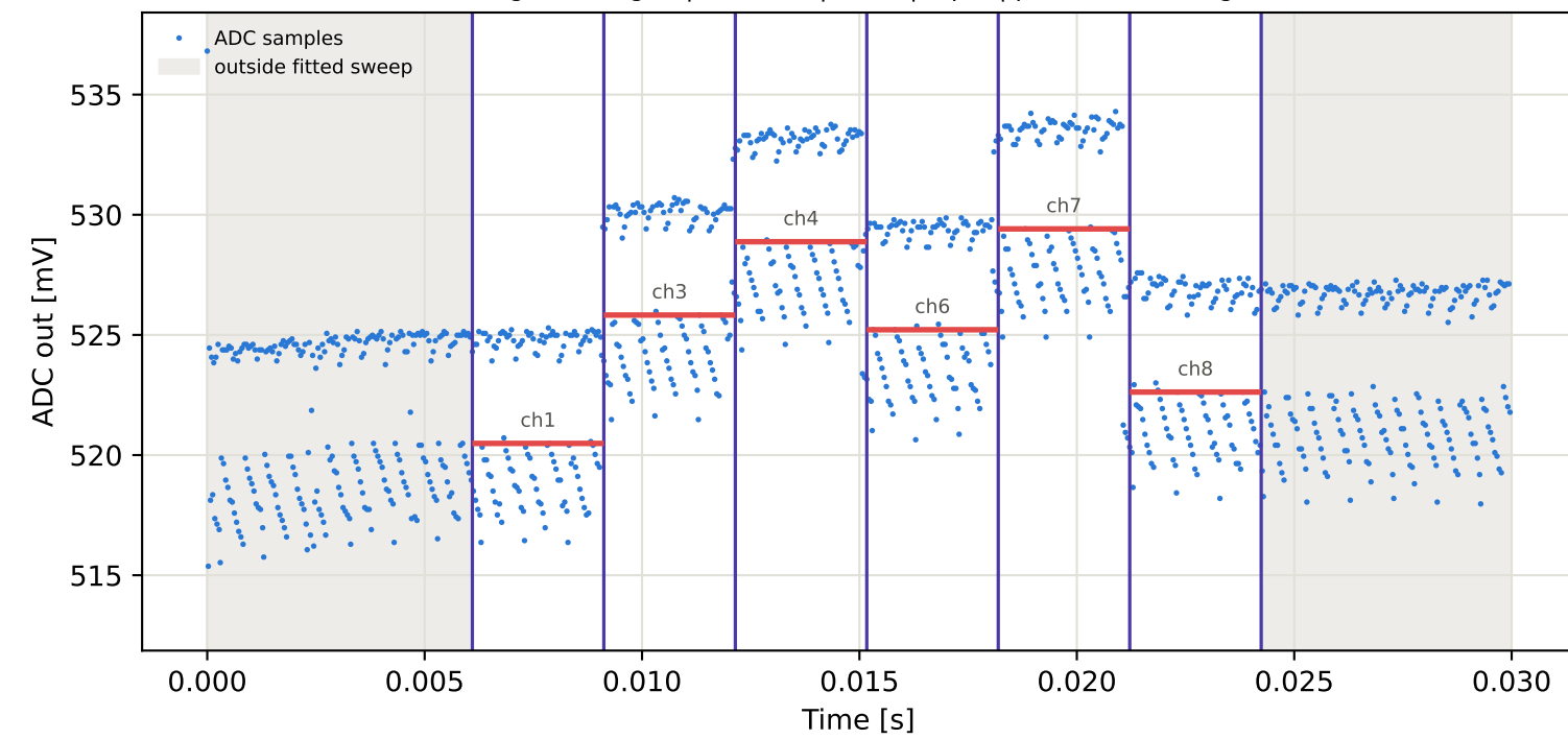
Tag15 &lt;- Tag3 | 835 MHz | run 0 | rep 1 | phase -35.39 deg
