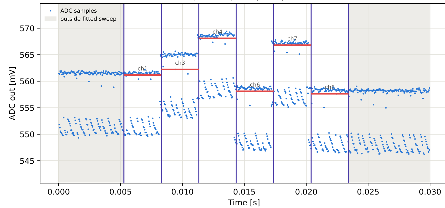
Tag5 &lt;- Tag16 | 945 MHz | run 0 | rep 1 | phase -91.26 deg
