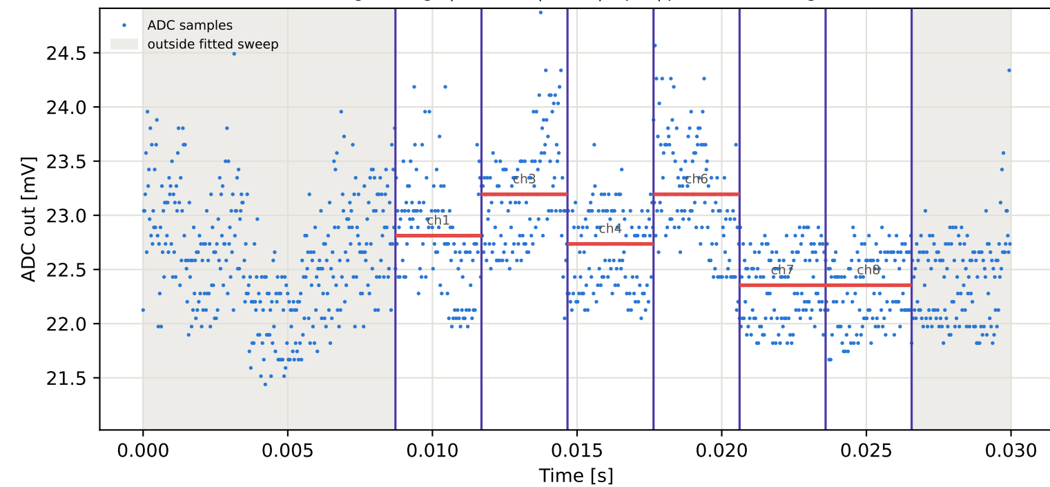
Tag3 &lt;- Tag10 | 785 MHz | run 0 | rep 1 | phase 178.37 deg
