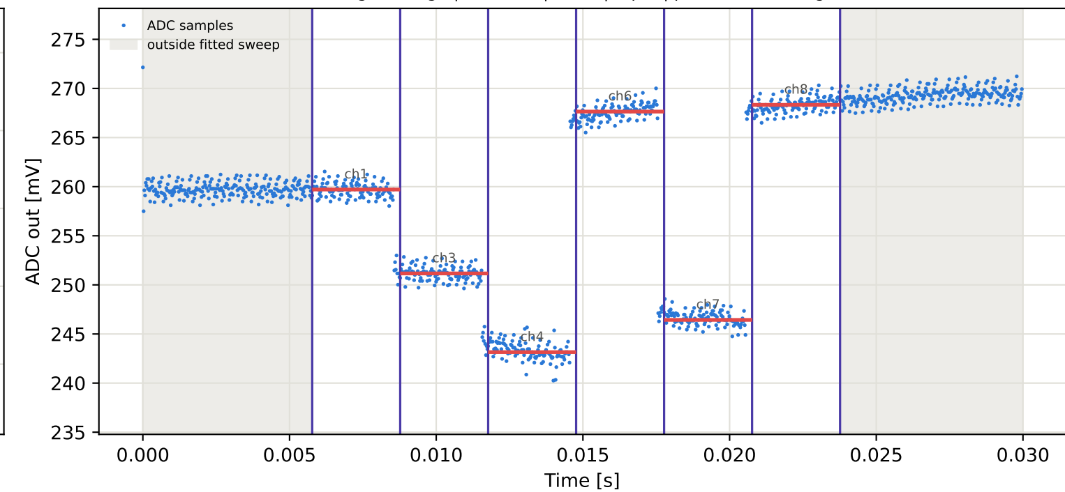
Tag1 &lt;- Tag8 | 925 MHz | run 0 | rep 1 | phase -63.55 deg
