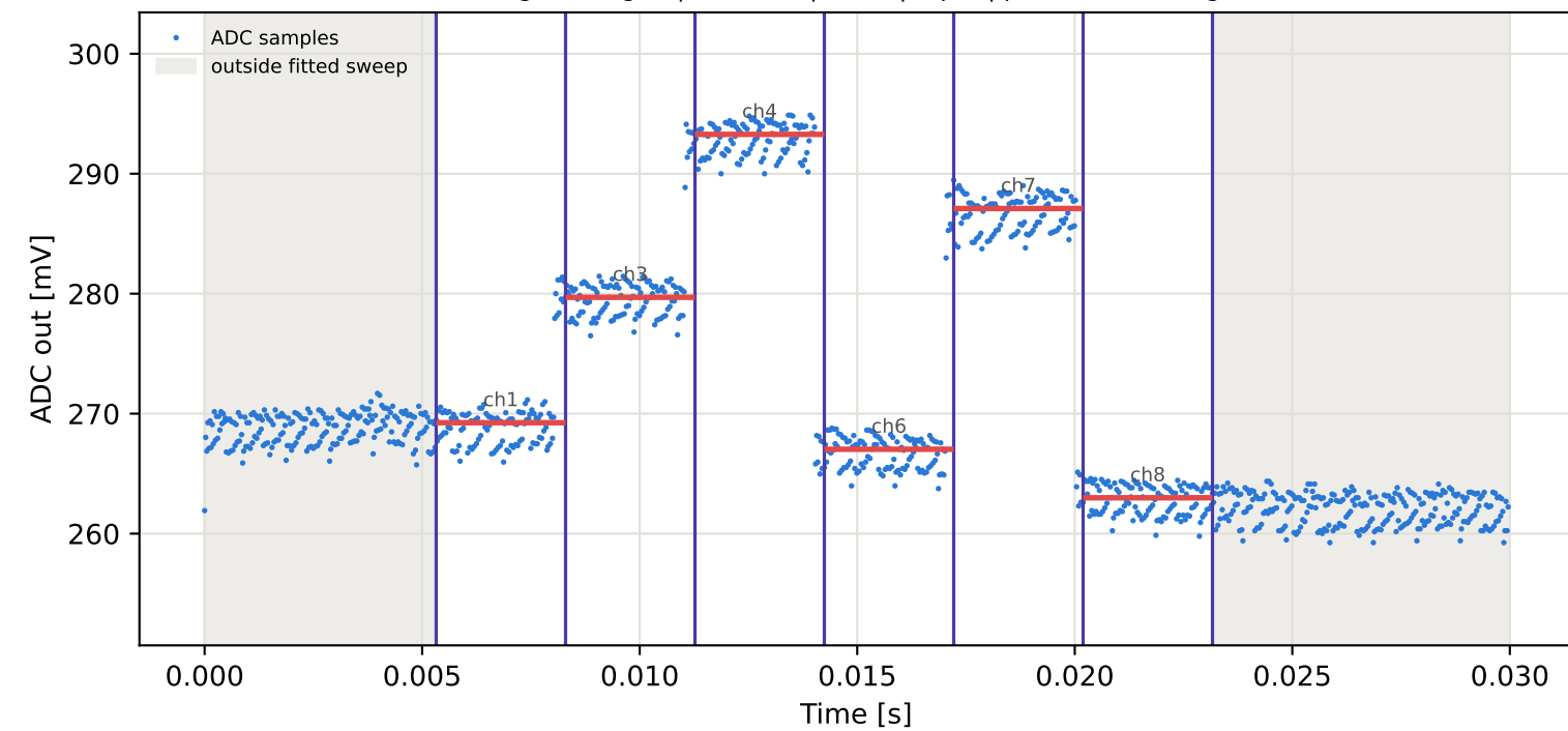
Tag6 &lt;- Tag3 | 955 MHz | run 0 | rep 1 | phase 174.38 deg
