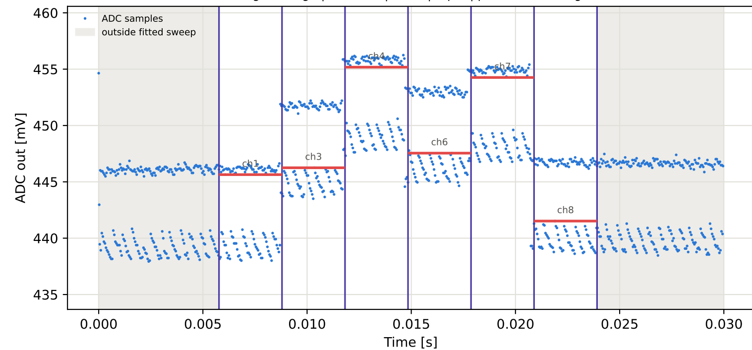
Tag4 &lt;- Tag2 | 845 MHz | run 0 | rep 1 | phase -84.14 deg
