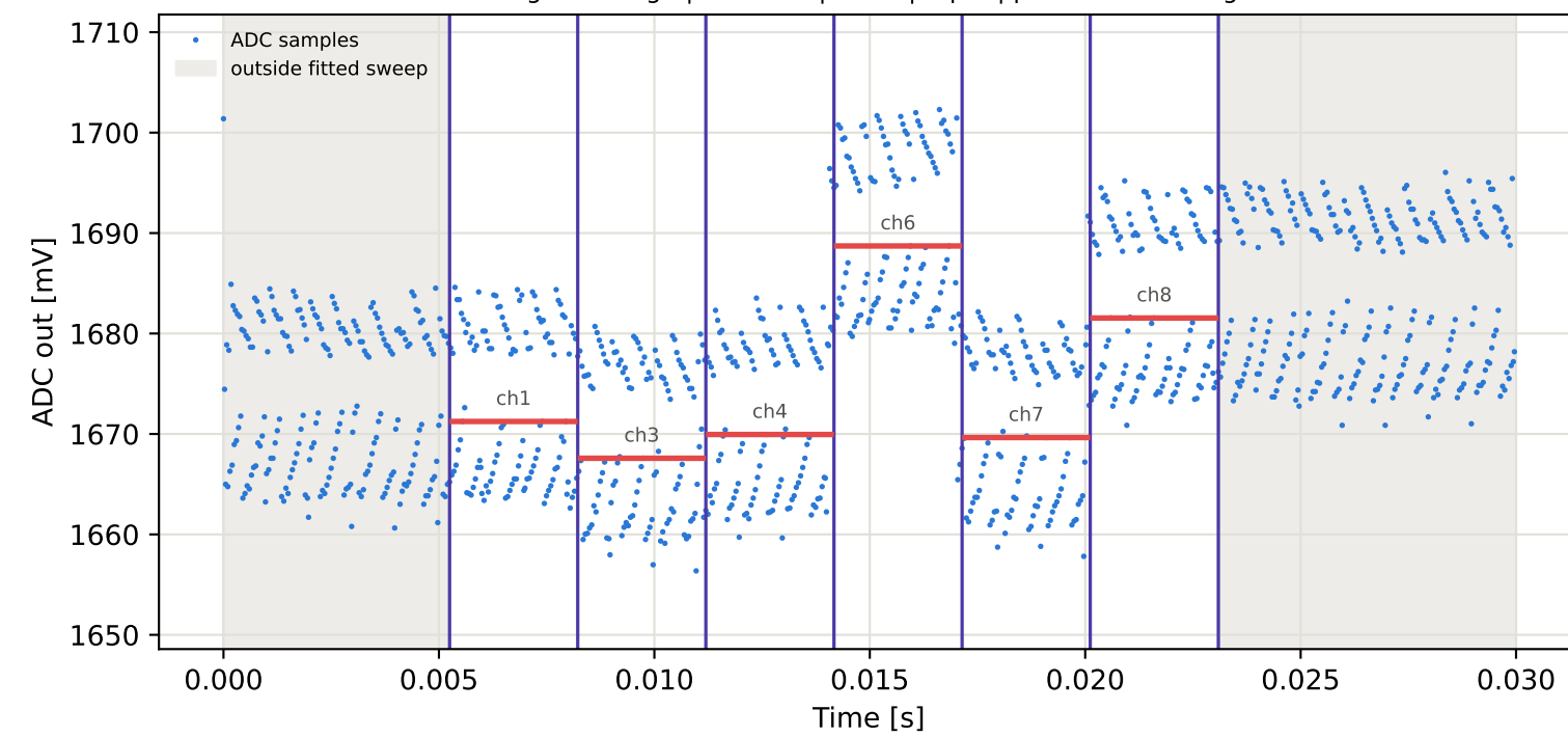
Tag15 &lt;- Tag9 | 925 MHz | run 0 | rep 1 | phase -65.48 deg
