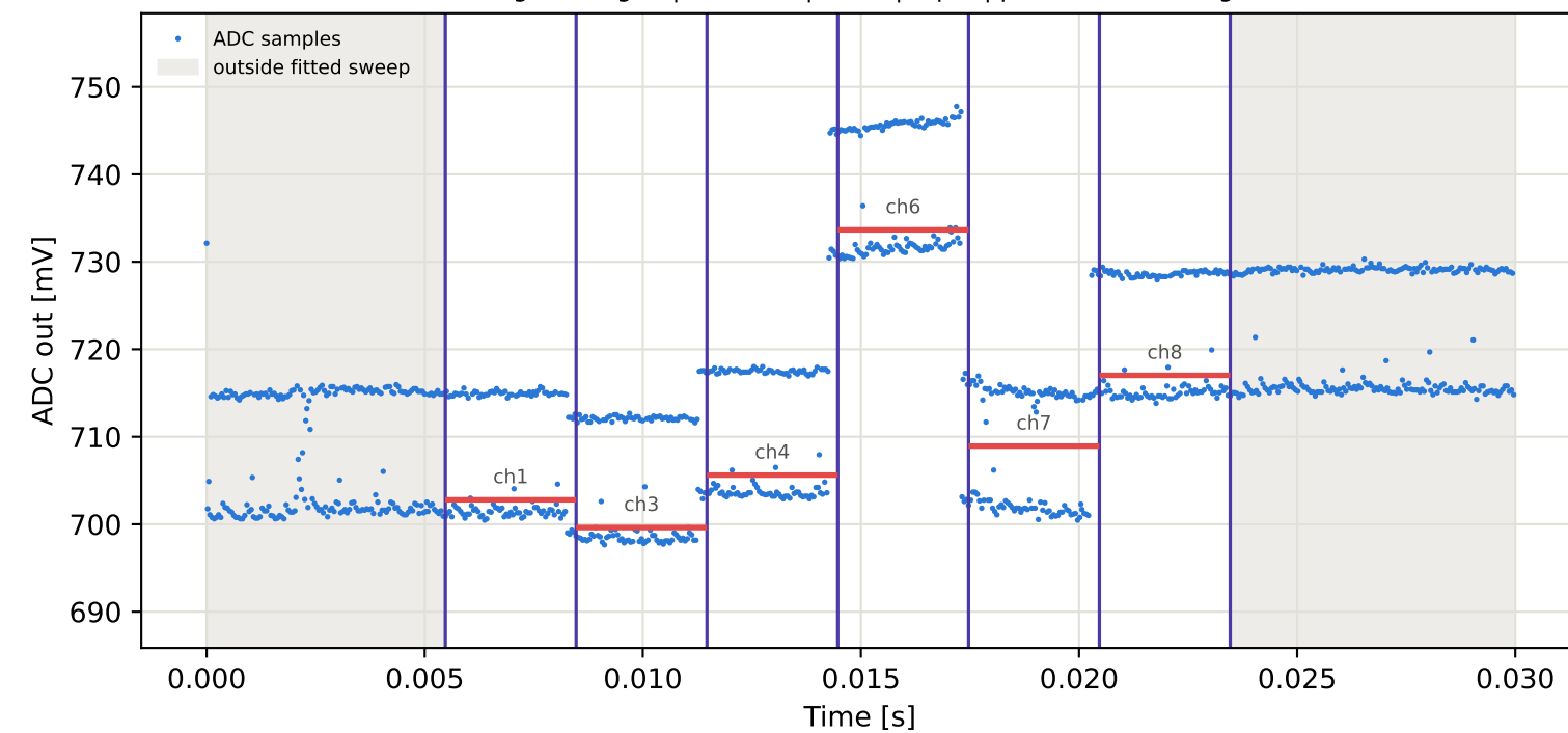
Tag7 &lt;- Tag10 | 925 MHz | run 0 | rep 1 | phase -167.76 deg
