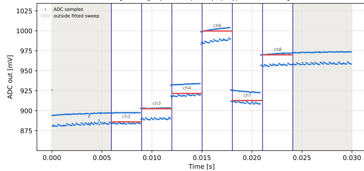
Tag15 &lt;- Tag3 | 895 MHz | run 0 | rep 1 | phase -119.69 deg
