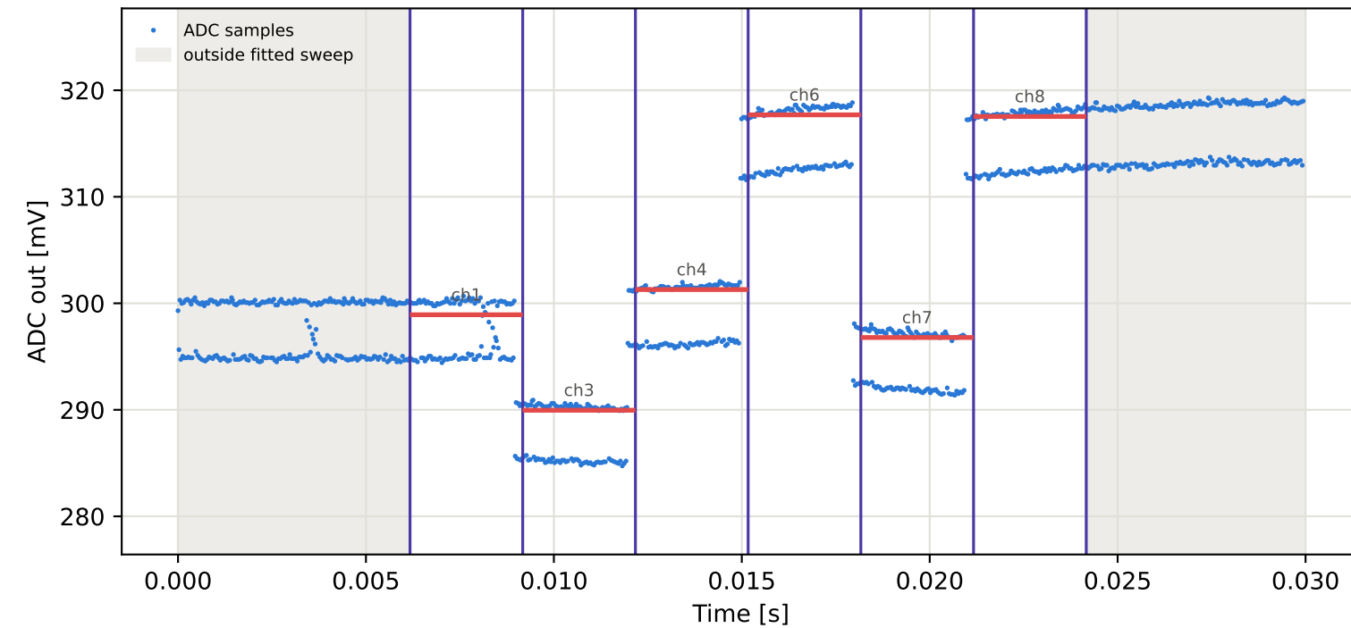
Tag9 &lt;- Tag7 | 865 MHz | run 0 | rep 1 | phase -34.10 deg
