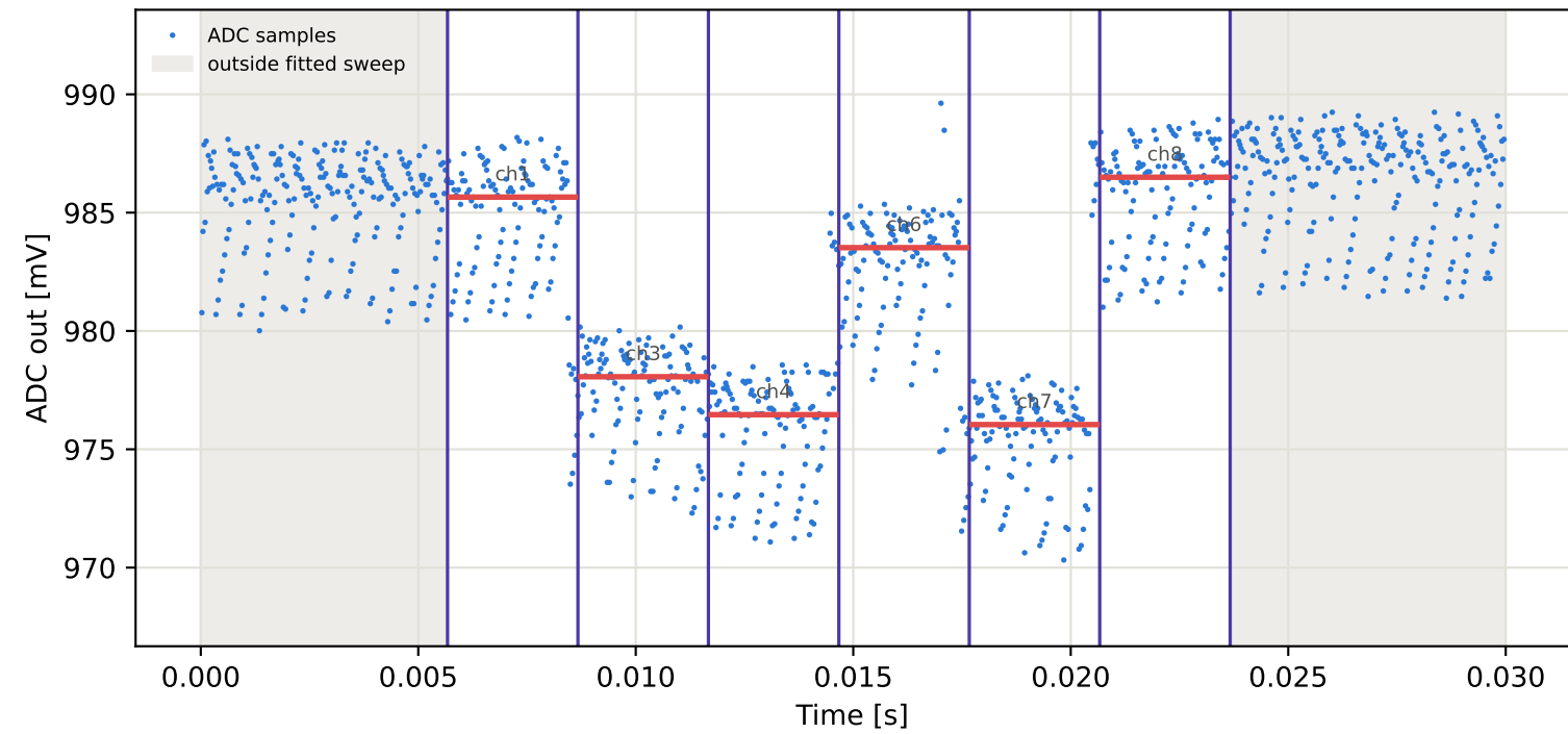
Tag6 &lt;- Tag10 | 865 MHz | run 0 | rep 1 | phase -78.16 deg
