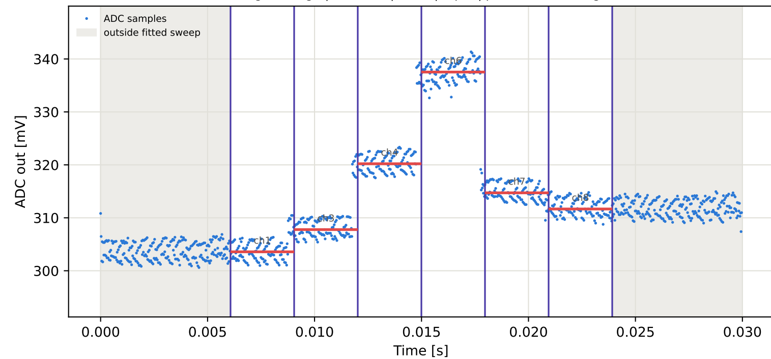
Tag7 &lt;- Tag1 | 925 MHz | run 0 | rep 1 | phase 173.78 deg
