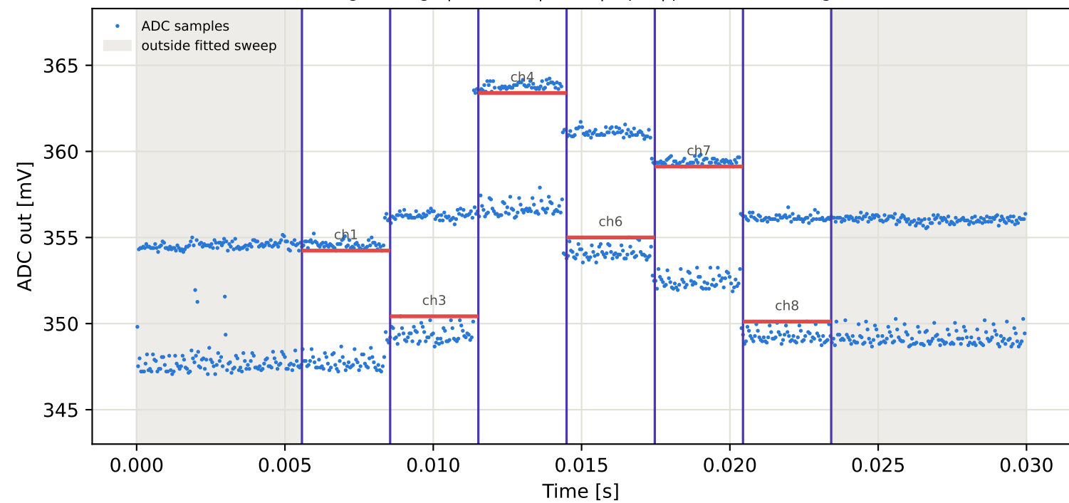
Tag3 &lt;- Tag7 | 975 MHz | run 0 | rep 1 | phase -164.44 deg
