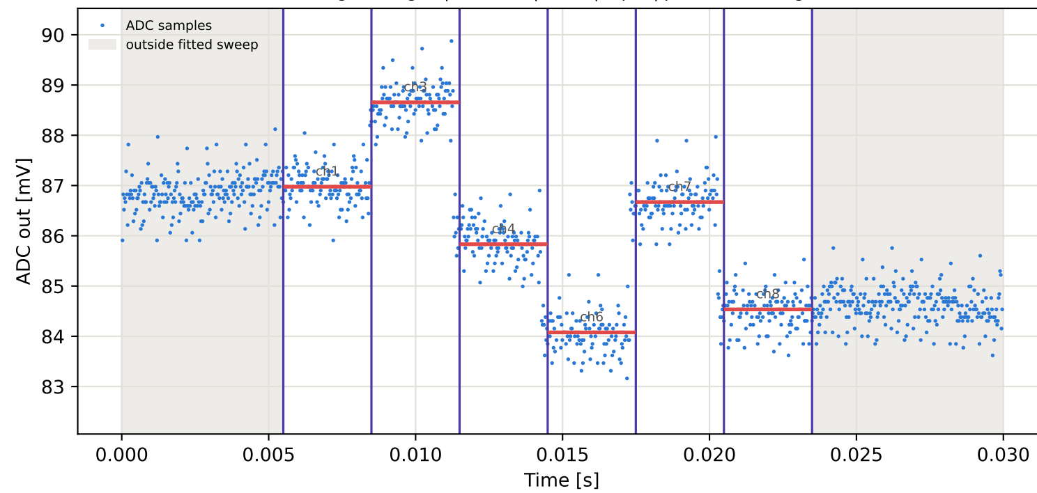
Tag1 &lt;- Tag16 | 845 MHz | run 0 | rep 1 | phase -5.37 deg
