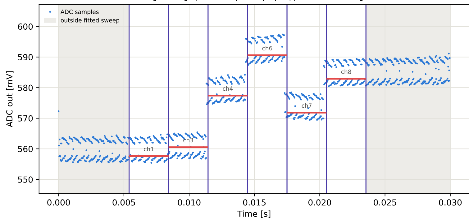
Tag7 &lt;- Tag1 | 865 MHz | run 0 | rep 1 | phase 16.79 deg
