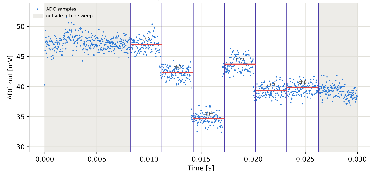
Tag7 &lt;- Tag5 | 885 MHz | run 0 | rep 1 | phase 176.93 deg
