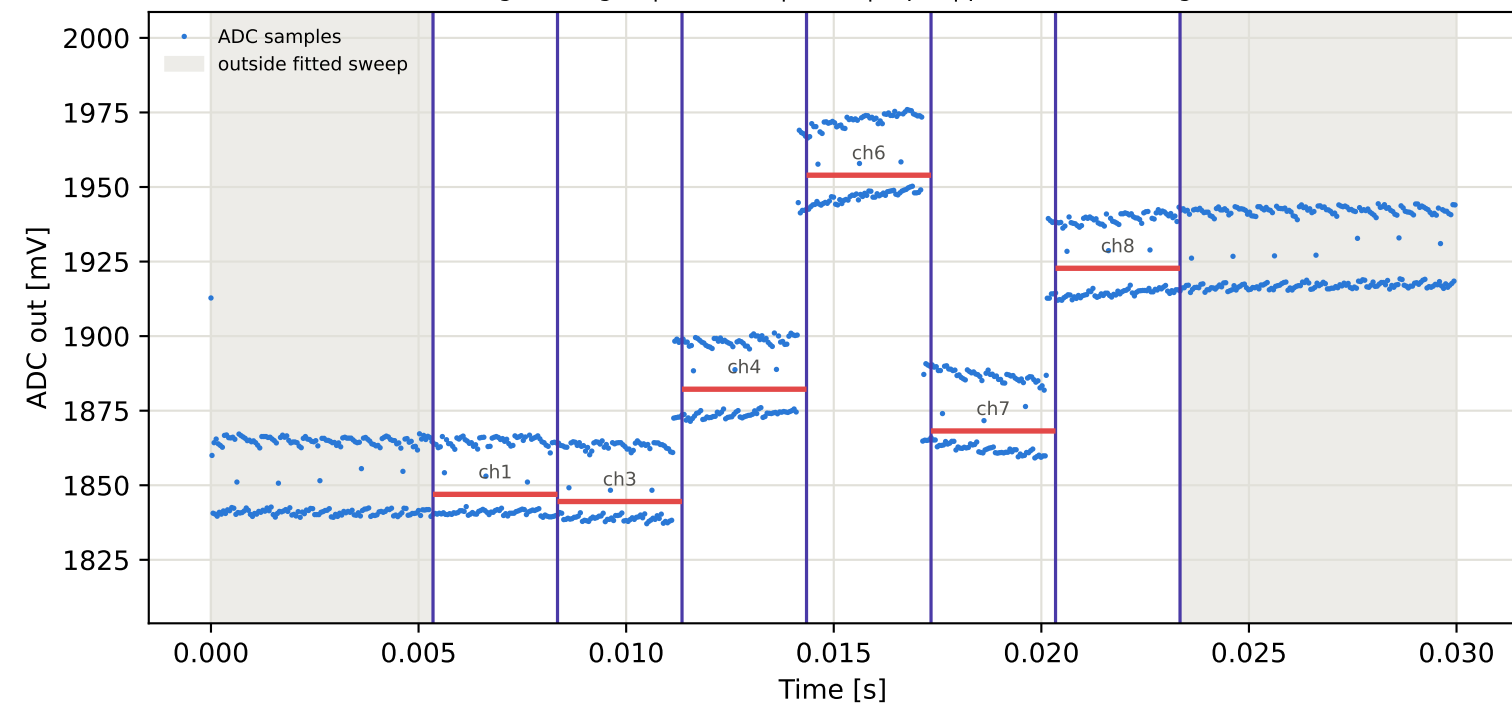
Tag5 &lt;- Tag2 | 895 MHz | run 0 | rep 1 | phase 86.71 deg
