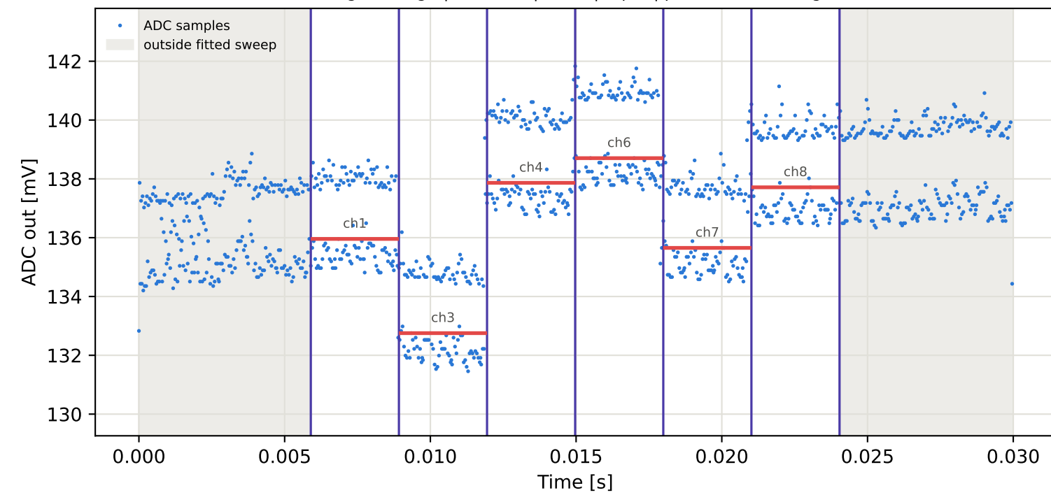
Tag8 &lt;- Tag1 | 795 MHz | run 0 | rep 1 | phase 107.07 deg
