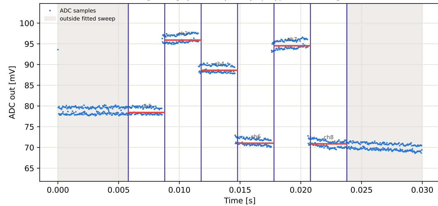
Tag4 &lt;- Tag7 | 795 MHz | run 0 | rep 1 | phase -117.24 deg
