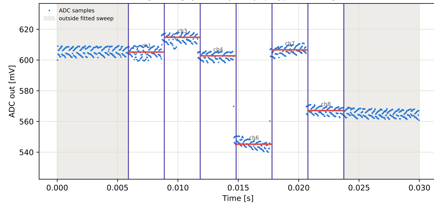
Tag10 &lt;- Tag8 | 895 MHz | run 0 | rep 1 | phase -35.46 deg
