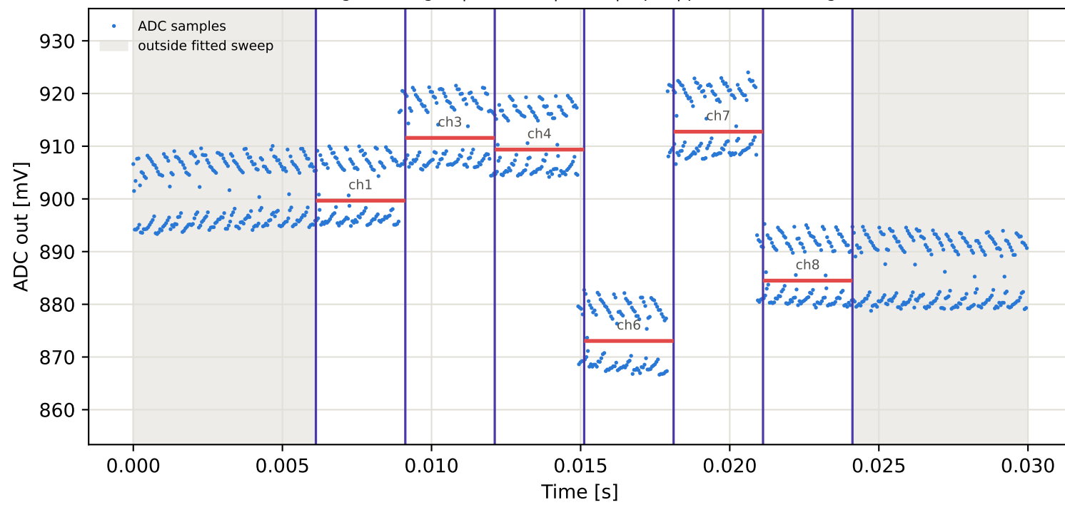
Tag15 &lt;- Tag3 | 965 MHz | run 0 | rep 1 | phase 15.22 deg
