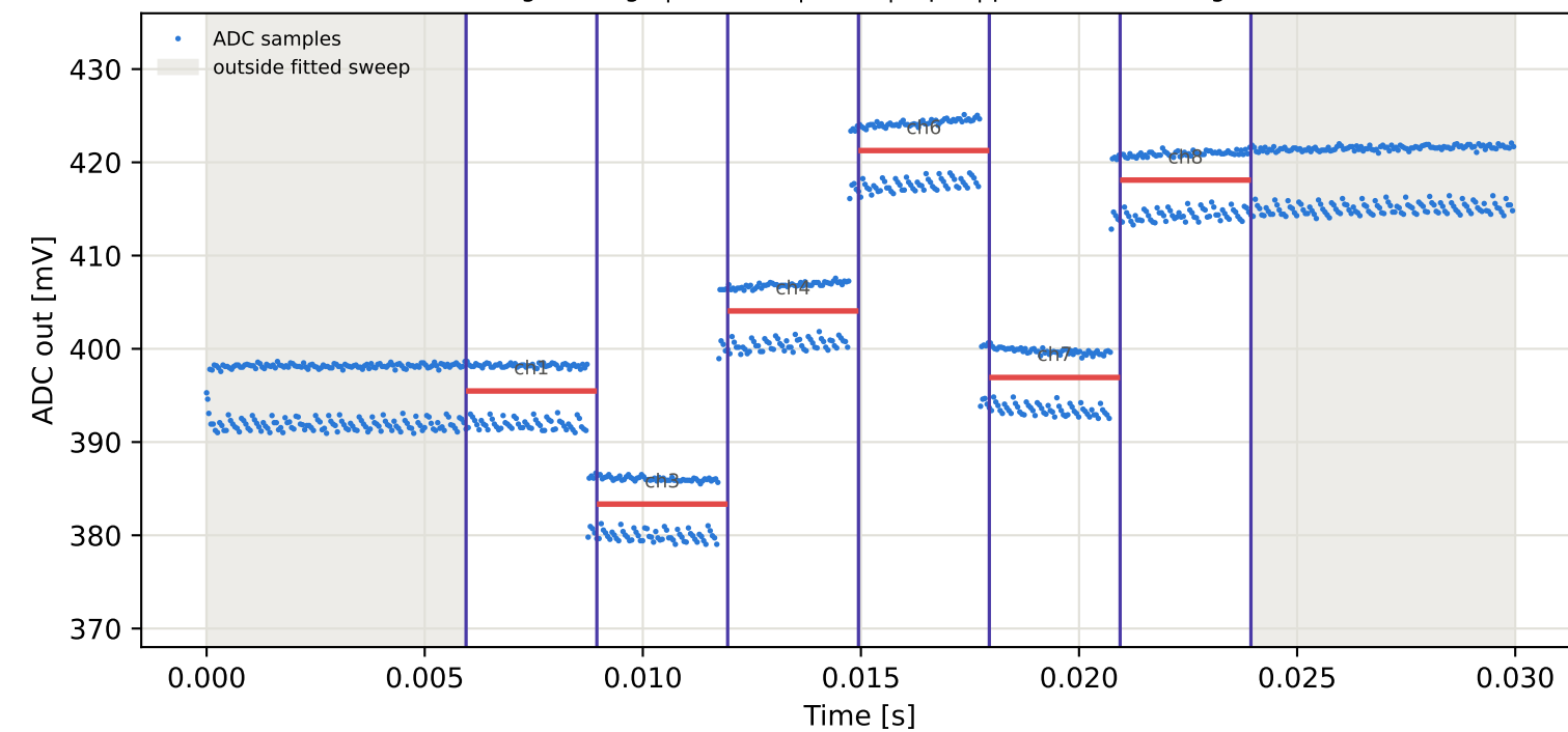
Tag3 &lt;- Tag8 | 845 MHz | run 0 | rep 1 | phase -159.16 deg
