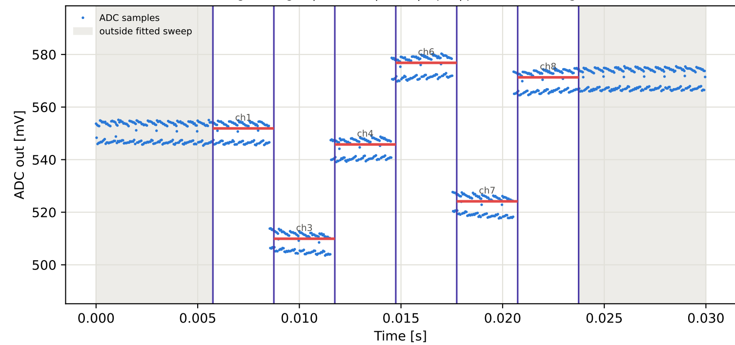
Tag5 &lt;- Tag2 | 825 MHz | run 0 | rep 1 | phase 108.99 deg
