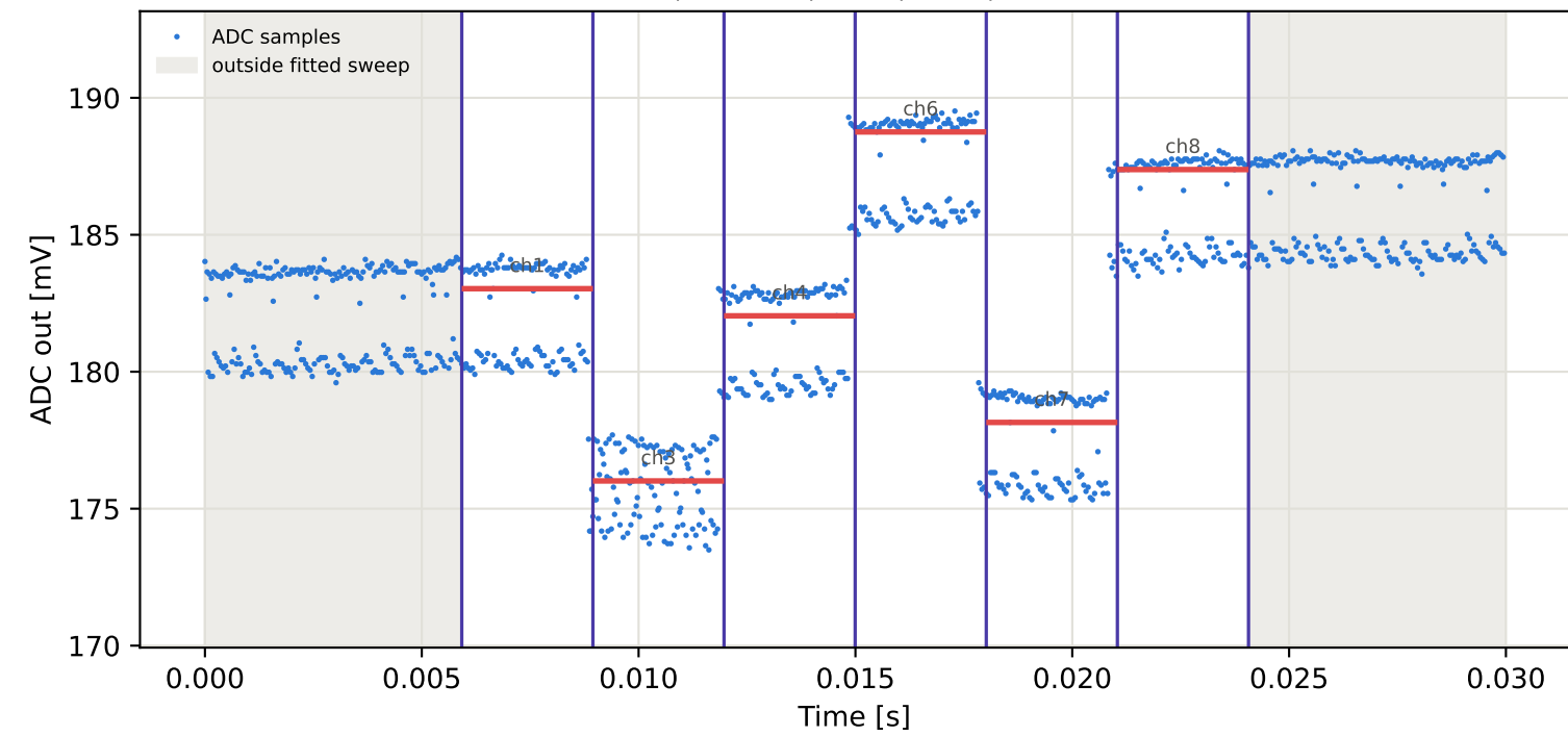
Tag16 &lt;- Tag15 | 805 MHz | run 0 | rep 1 | phase -170.77 deg
