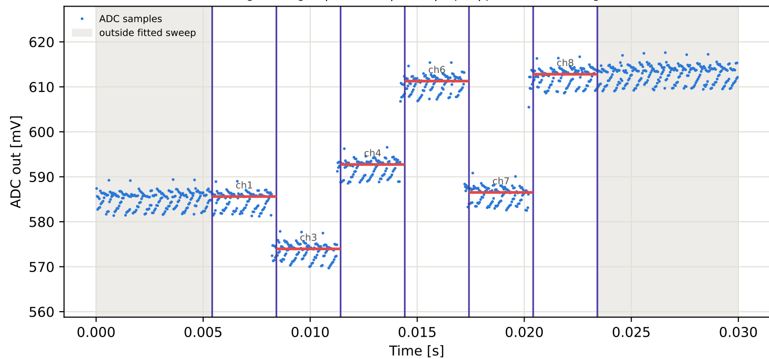
Tag4 &lt;- Tag3 | 865 MHz | run 0 | rep 1 | phase -7.98 deg
