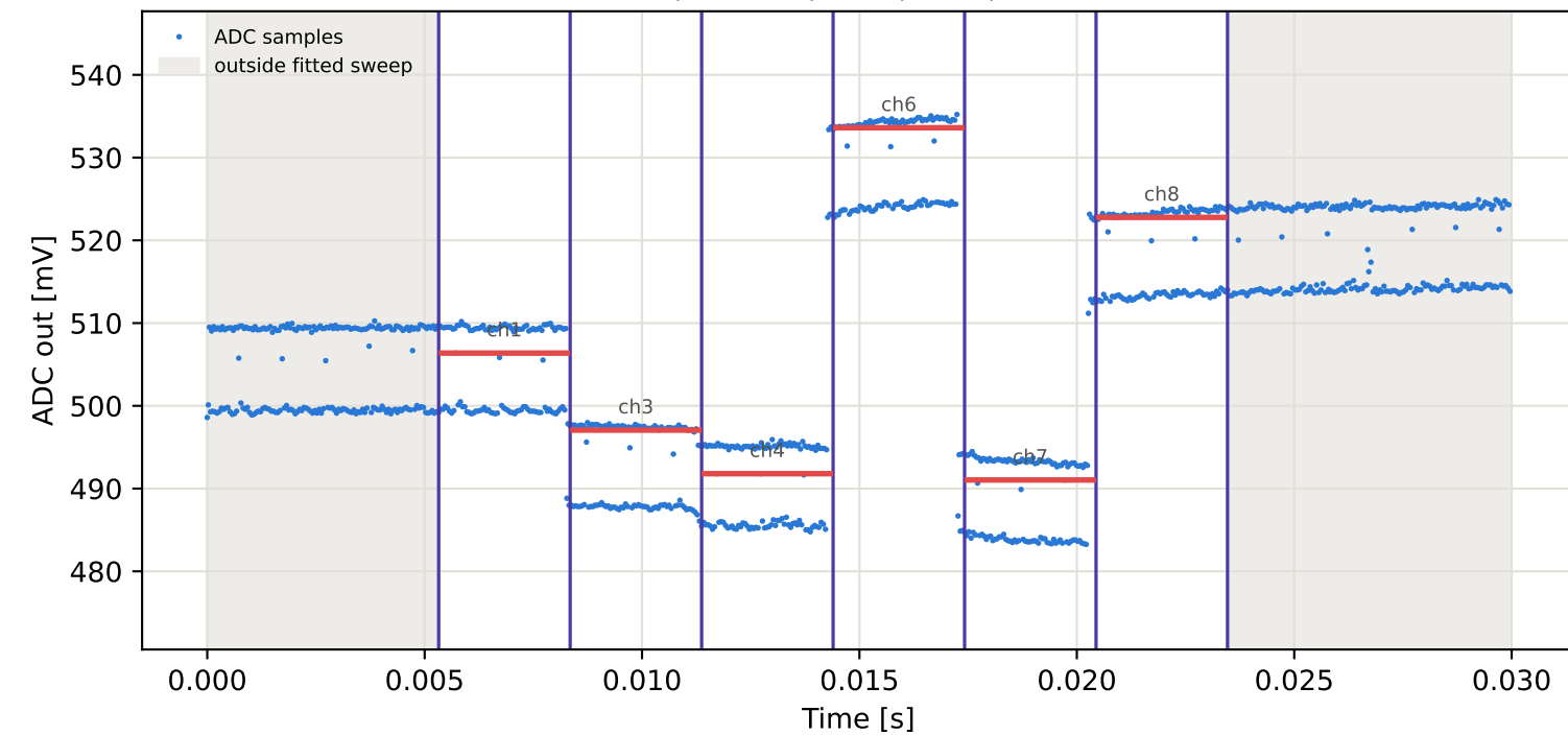
Tag15 &lt;- Tag5 | 995 MHz | run 0 | rep 1 | phase 150.37 deg
