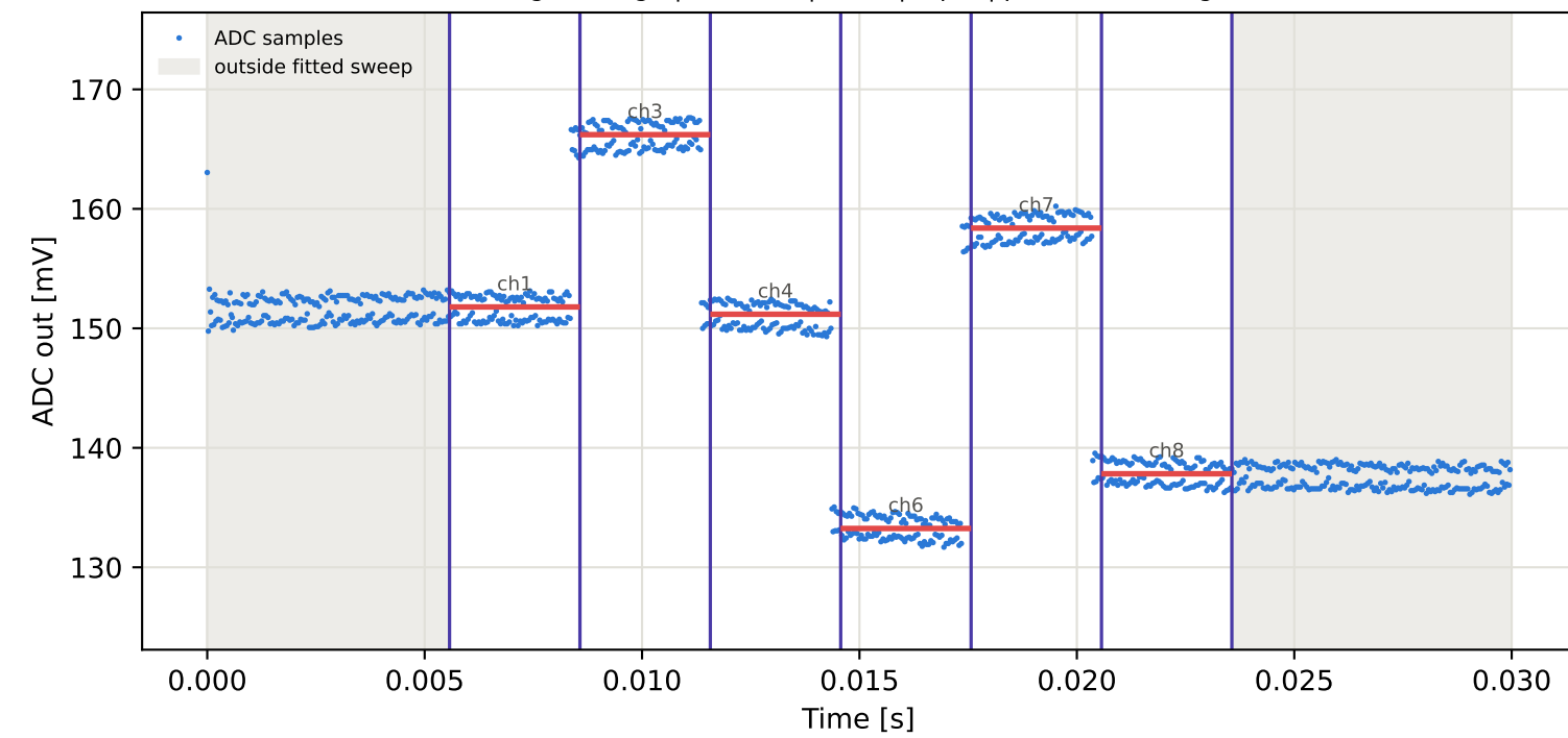
Tag4 &lt;- Tag7 | 805 MHz | run 0 | rep 1 | phase -86.32 deg
