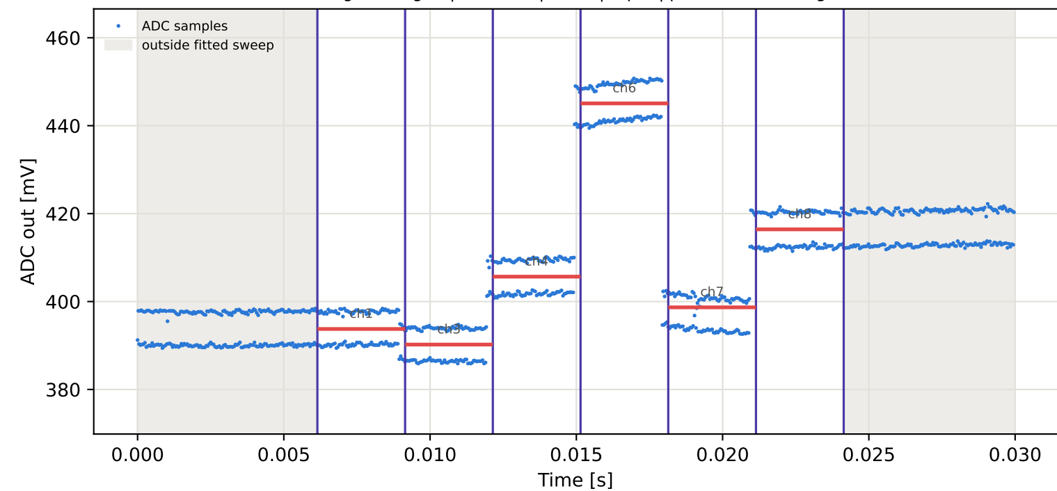
Tag7 &lt;- Tag15 | 945 MHz | run 0 | rep 1 | phase -164.47 deg
