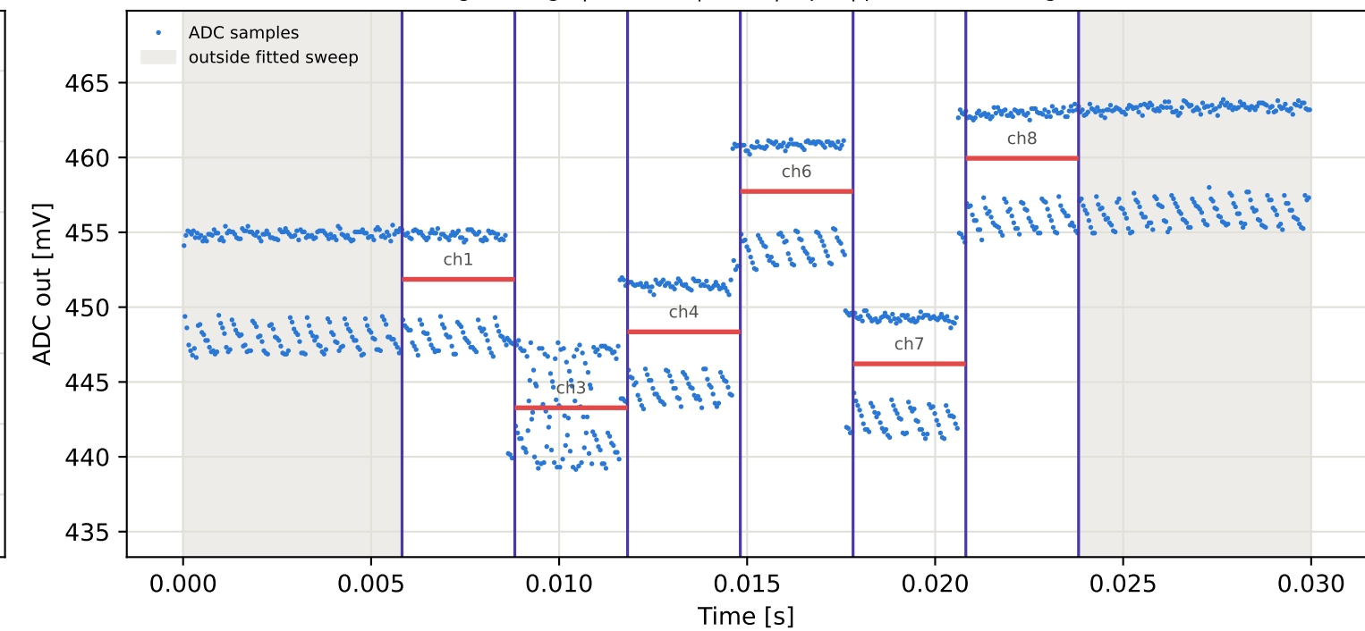
Tag4 &lt;- Tag8 | 845 MHz | run 0 | rep 1 | phase -126.37 deg
