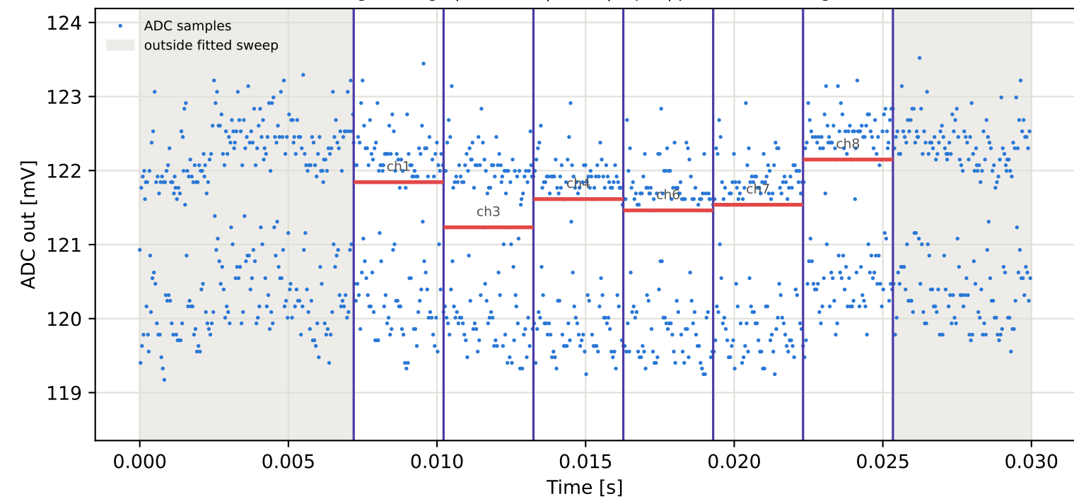
Tag7 &lt;- Tag4 | 775 MHz | run 0 | rep 1 | phase 43.06 deg
