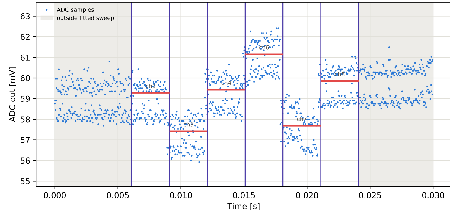
Tag10 &lt;- Tag1 | 785 MHz | run 0 | rep 1 | phase -163.42 deg
