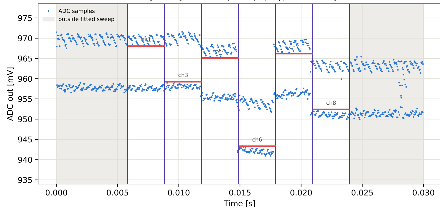
Tag4 &lt;- Tag2 | 875 MHz | run 0 | rep 1 | phase 0.77 deg
