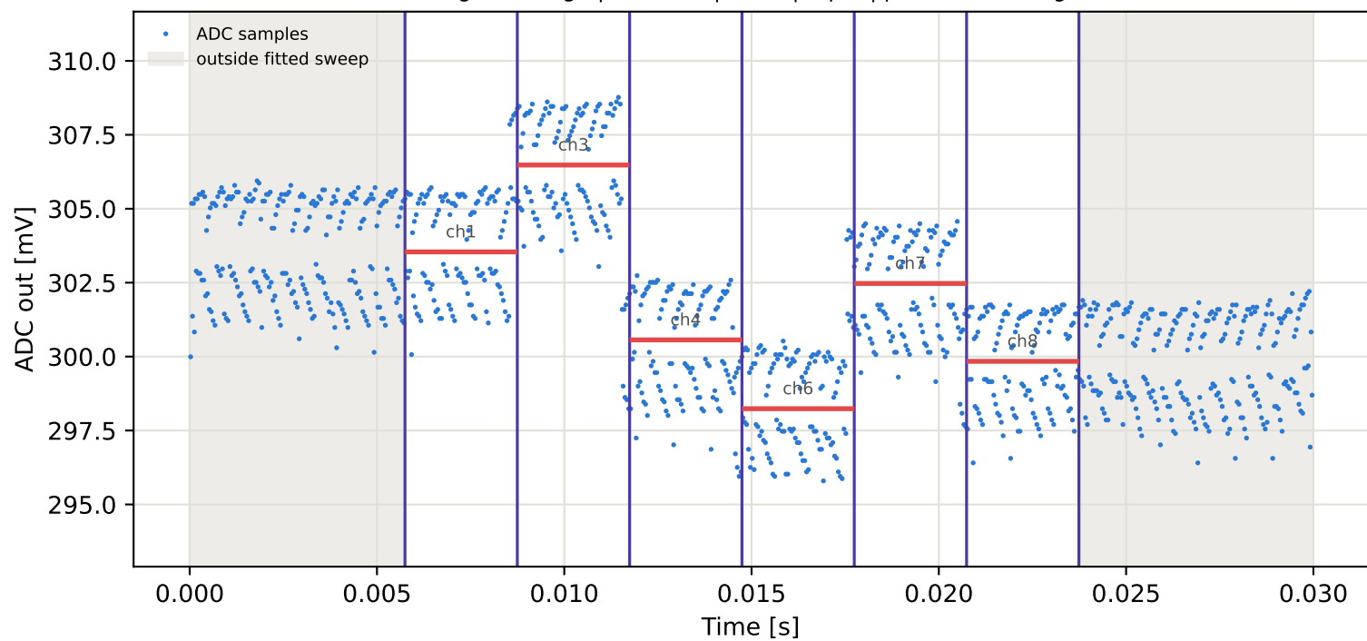
Tag15 &lt;- Tag6 | 805 MHz | run 0 | rep 1 | phase 34.74 deg
