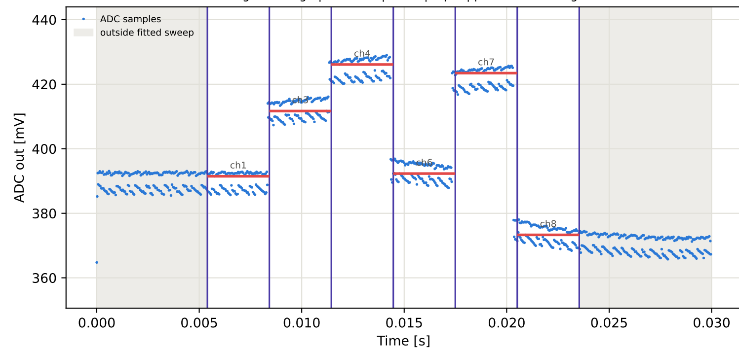
Tag10 &lt;- Tag9 | 905 MHz | run 0 | rep 1 | phase -109.51 deg
