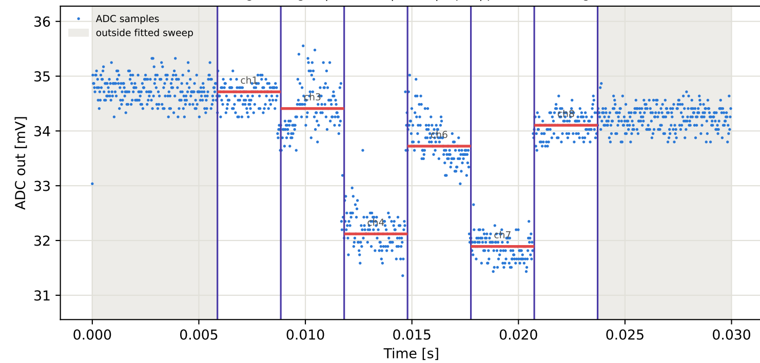
Tag1 &lt;- Tag2 | 785 MHz | run 0 | rep 1 | phase 80.75 deg
