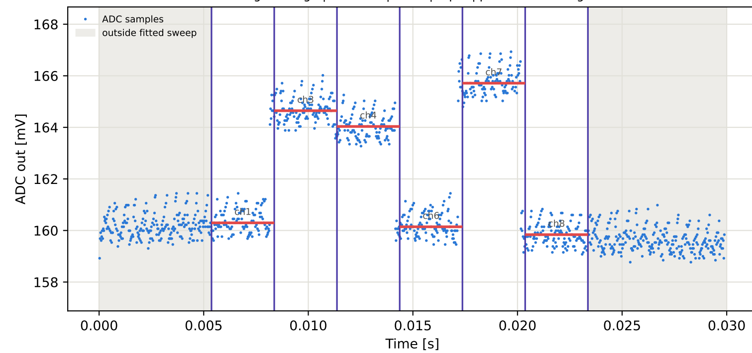
Tag9 &lt;- Tag5 | 805 MHz | run 0 | rep 1 | phase 145.89 deg
