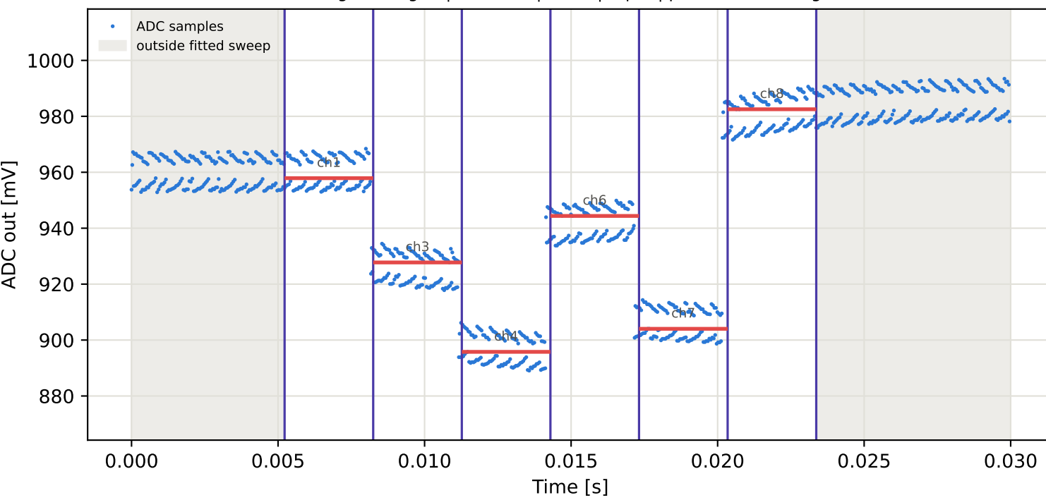
Tag8 &lt;- Tag15 | 915 MHz | run 0 | rep 1 | phase 103.62 deg
