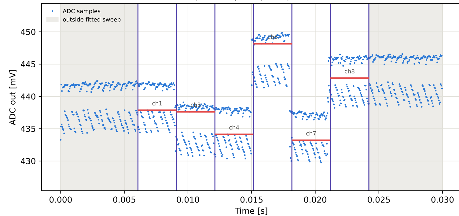
Tag4 &lt;- Tag15 | 995 MHz | run 0 | rep 1 | phase 39.41 deg
