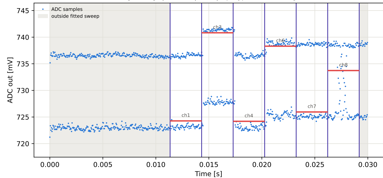
Tag7 &lt;- Tag4 | 975 MHz | run 0 | rep 1 | phase -16.87 deg
