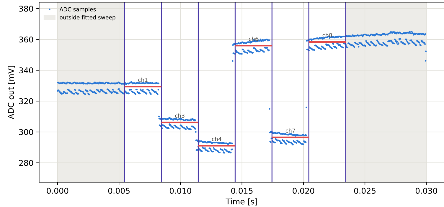
Tag6 &lt;- Tag5 | 925 MHz | run 0 | rep 1 | phase 84.40 deg
