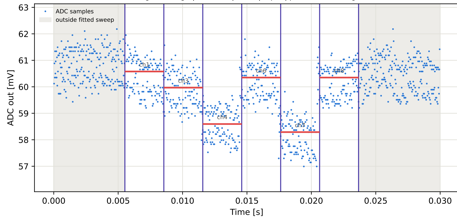
Tag15 &lt;- Tag1 | 785 MHz | run 0 | rep 1 | phase 124.11 deg
