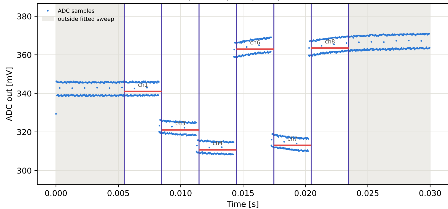
Tag3 &lt;- Tag15 | 925 MHz | run 0 | rep 1 | phase 104.20 deg
