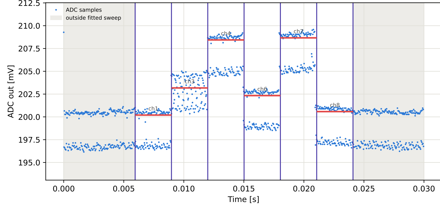
Tag3 &lt;- Tag2 | 805 MHz | run 0 | rep 1 | phase 86.80 deg
