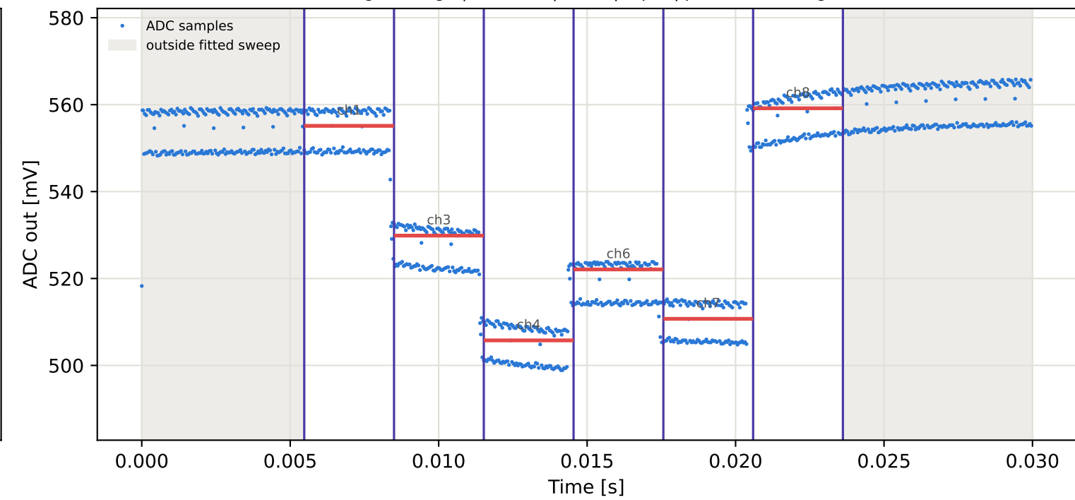
Tag3 &lt;- Tag15 | 895 MHz | run 0 | rep 1 | phase 49.18 deg
