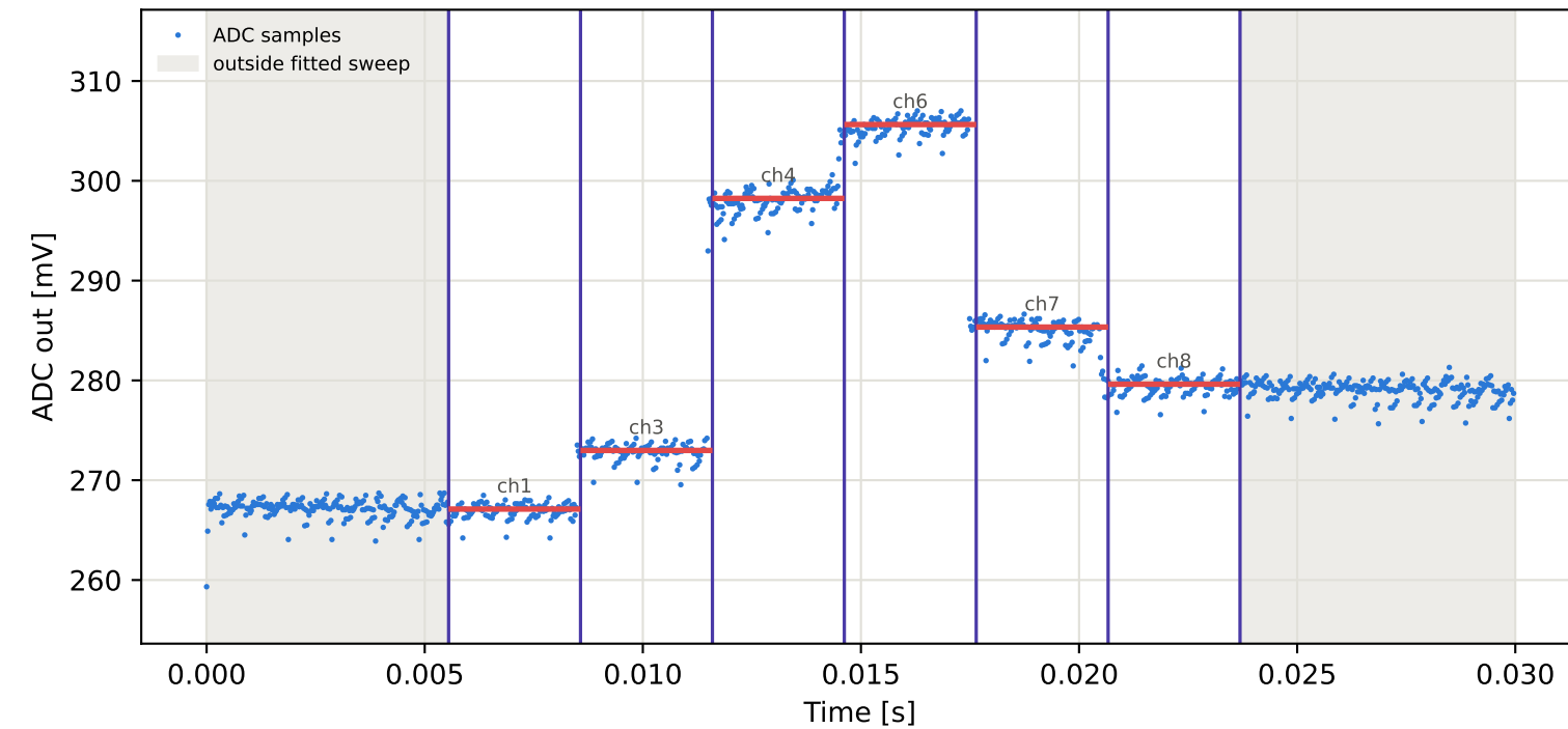
Tag7 &lt;- Tag10 | 955 MHz | run 0 | rep 1 | phase -105.03 deg
