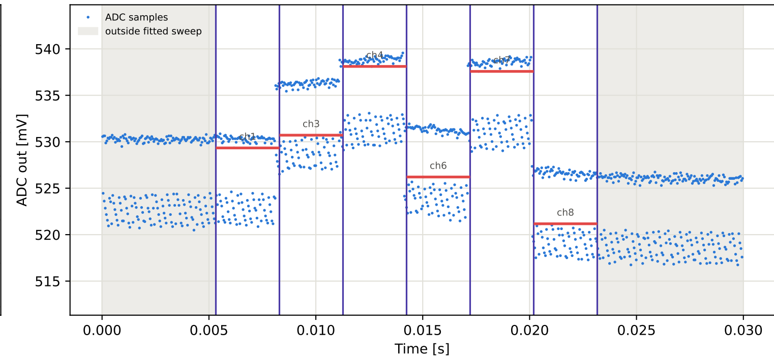
Tag3 &lt;- Tag9 | 895 MHz | run 0 | rep 1 | phase -76.78 deg
