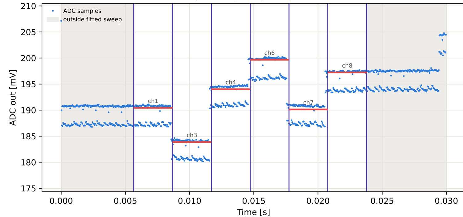
Tag8 &lt;- Tag6 | 805 MHz | run 0 | rep 1 | phase -153.47 deg
