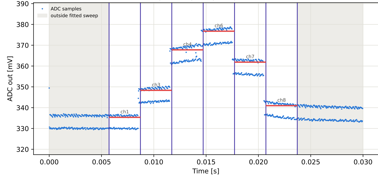
Tag1 &lt;- Tag4 | 905 MHz | run 0 | rep 1 | phase -125.64 deg
