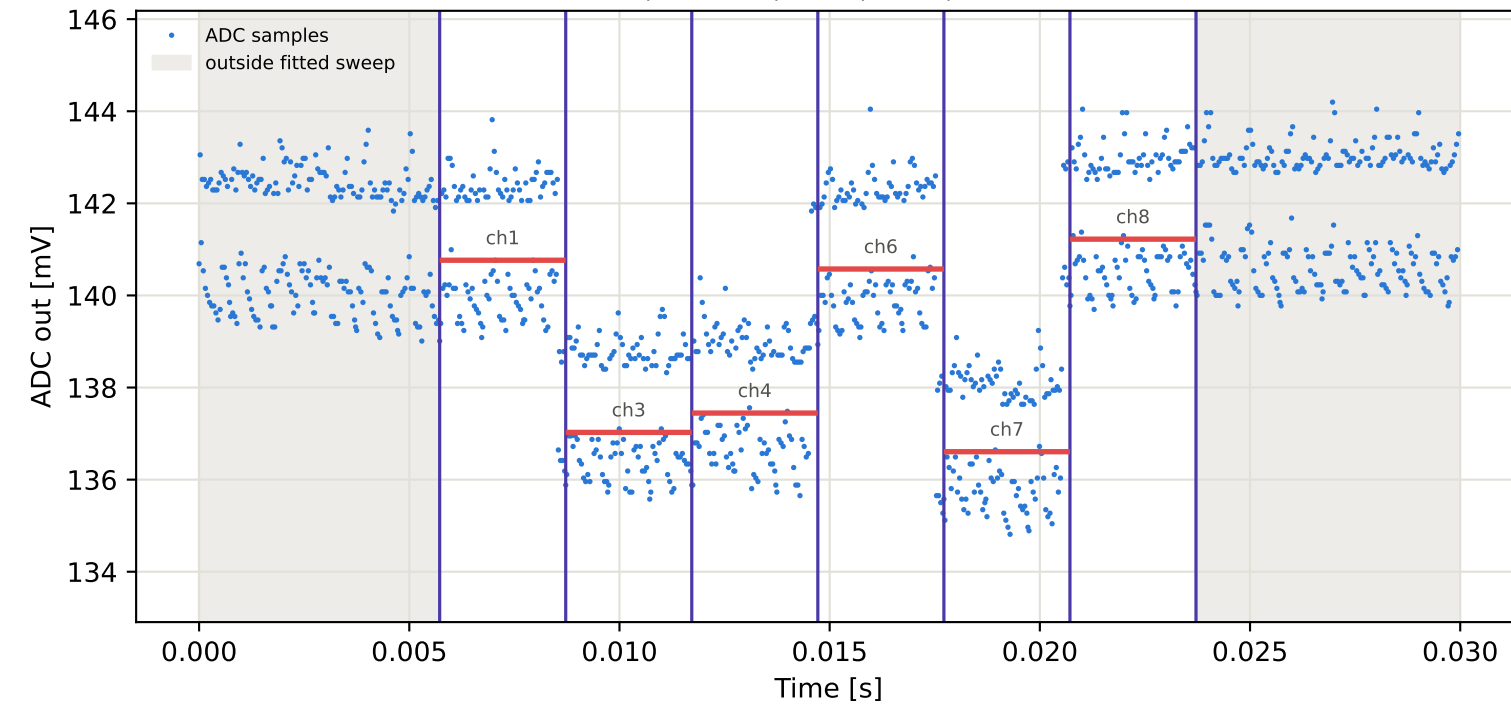
Tag7 &lt;- Tag5 | 795 MHz | run 0 | rep 1 | phase 144.29 deg
