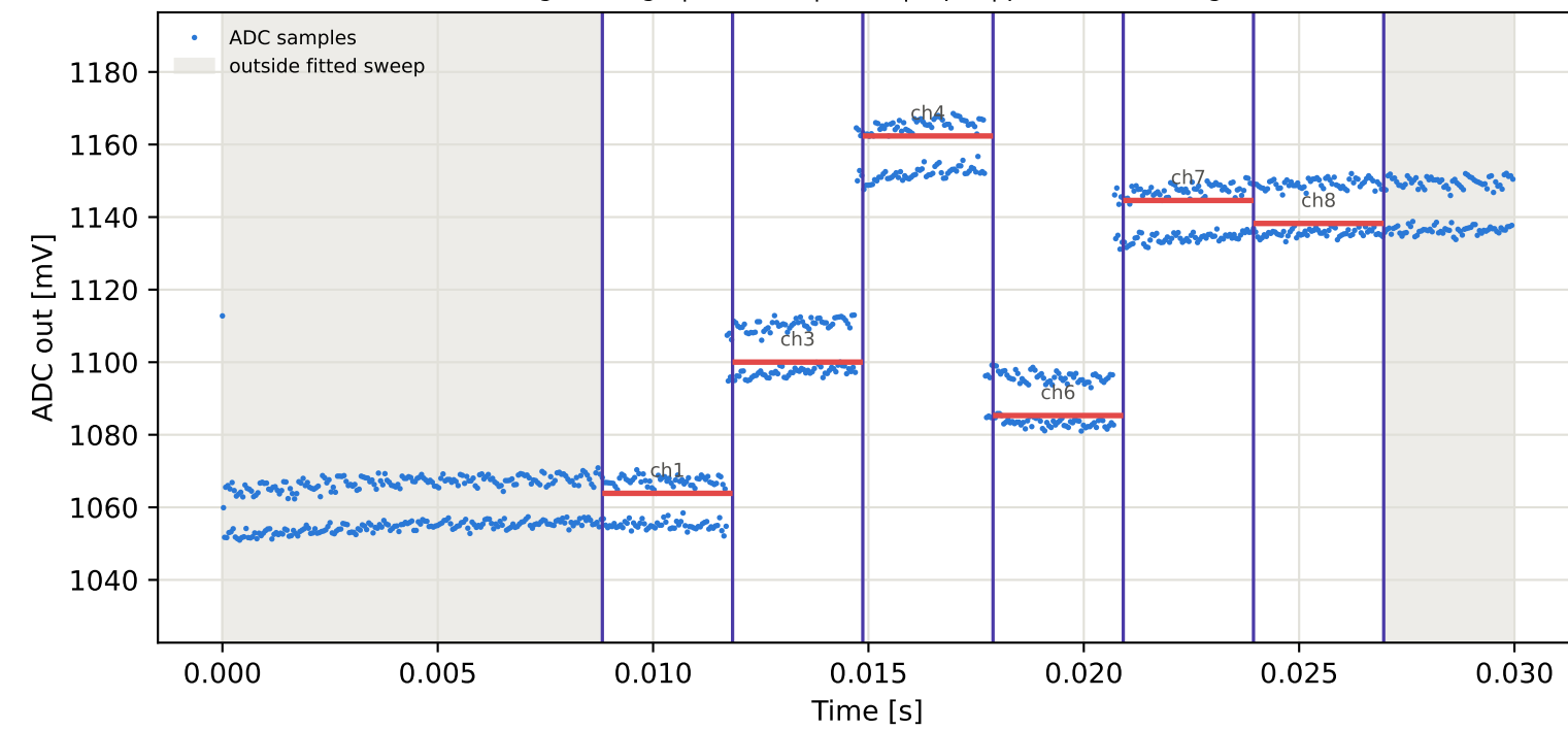
Tag9 &lt;- Tag10 | 885 MHz | run 0 | rep 1 | phase -67.66 deg
