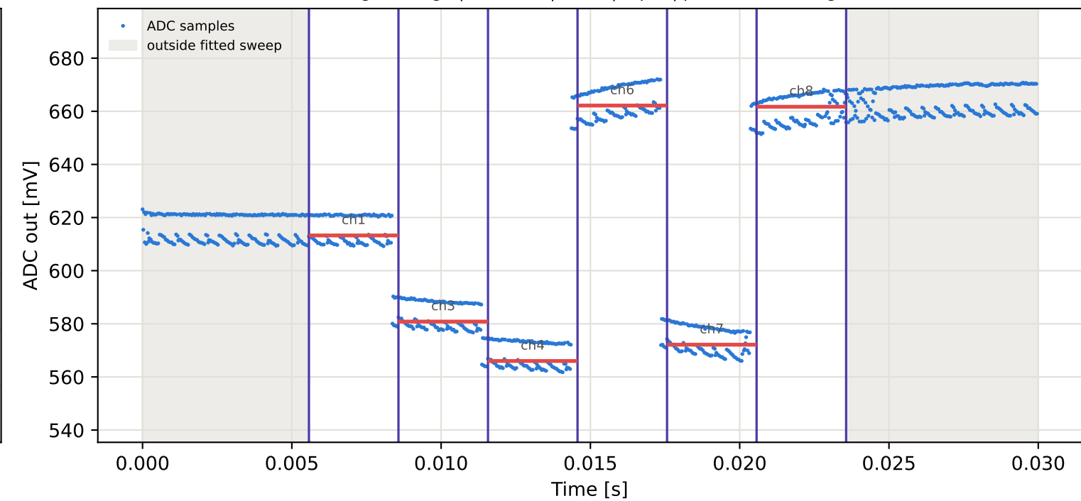
Tag9 &lt;- Tag6 | 915 MHz | run 0 | rep 1 | phase 107.17 deg
