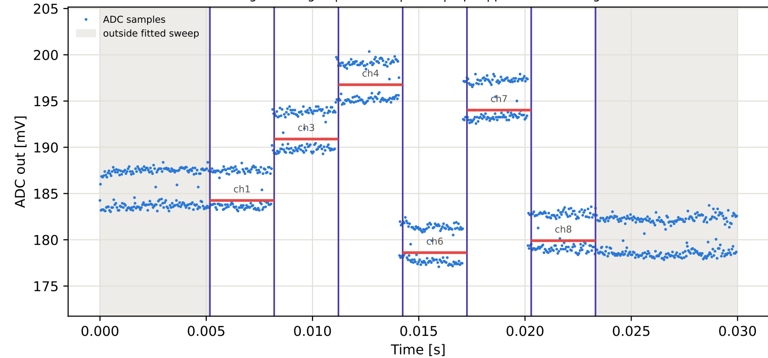
Tag10 &lt;- Tag3 | 985 MHz | run 0 | rep 1 | phase 105.05 deg
