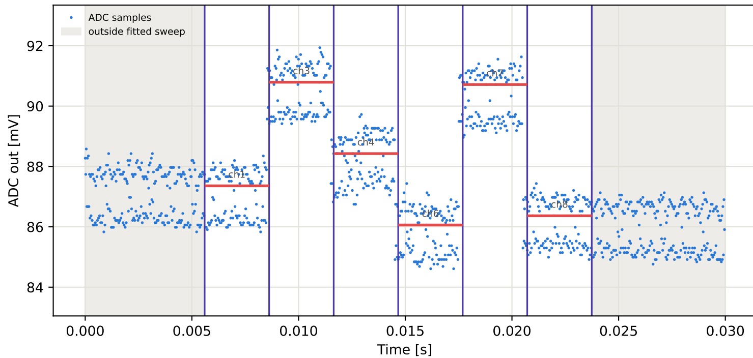
Tag9 &lt;- Tag5 | 795 MHz | run 0 | rep 1 | phase 120.46 deg
