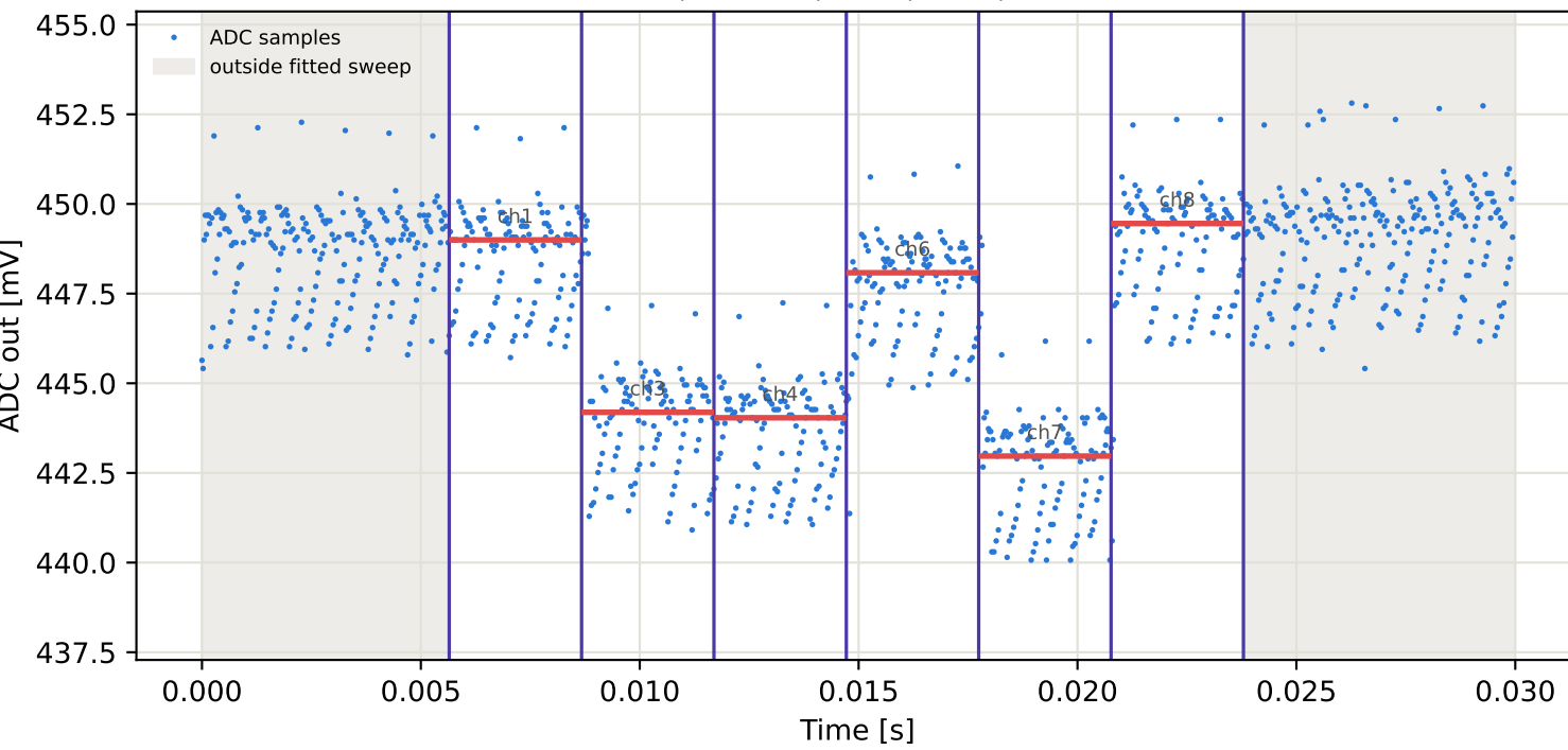
Tag16 &lt;- Tag10 | 825 MHz | run 0 | rep 1 | phase 132.92 deg
