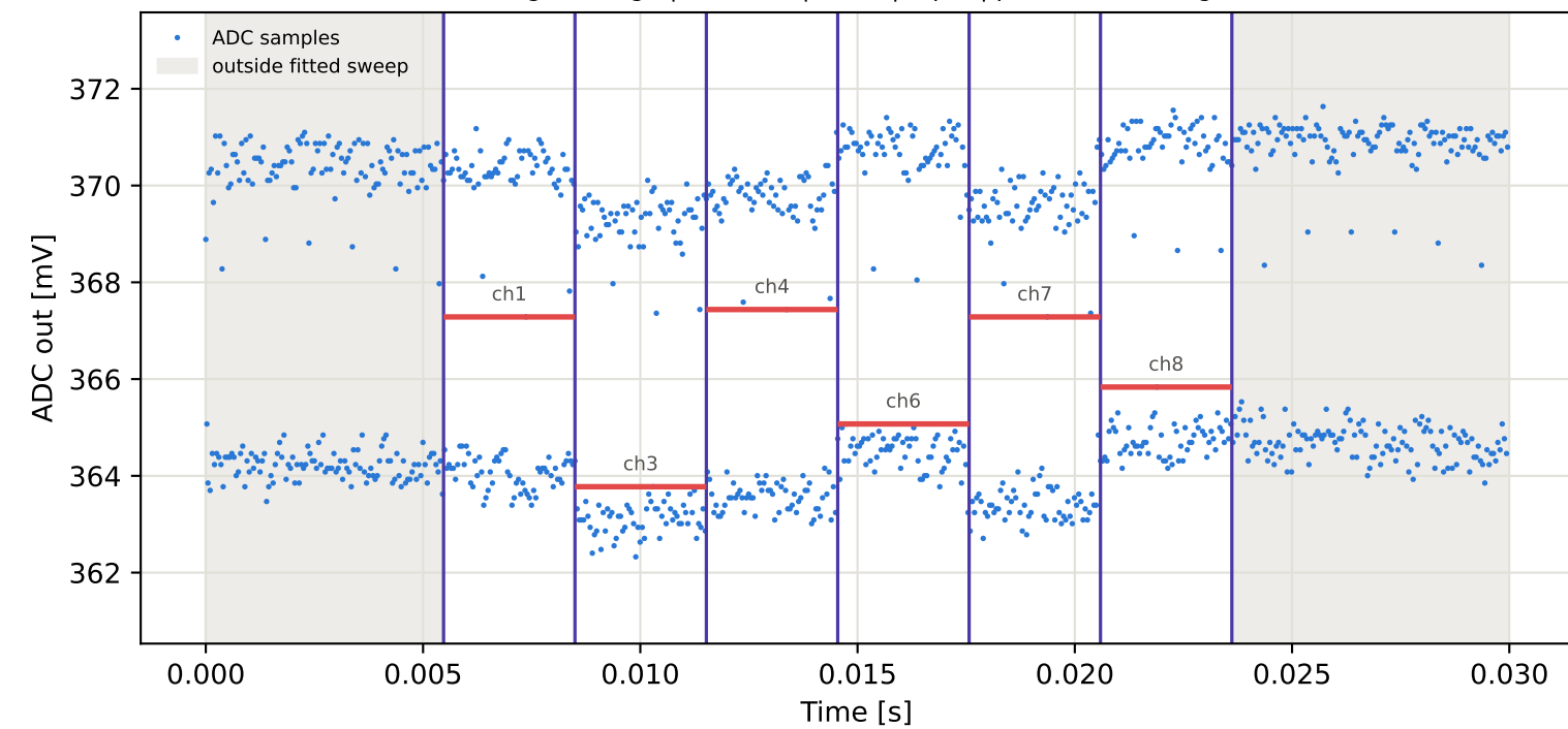
Tag4 &lt;- Tag15 | 835 MHz | run 0 | rep 1 | phase -105.66 deg
