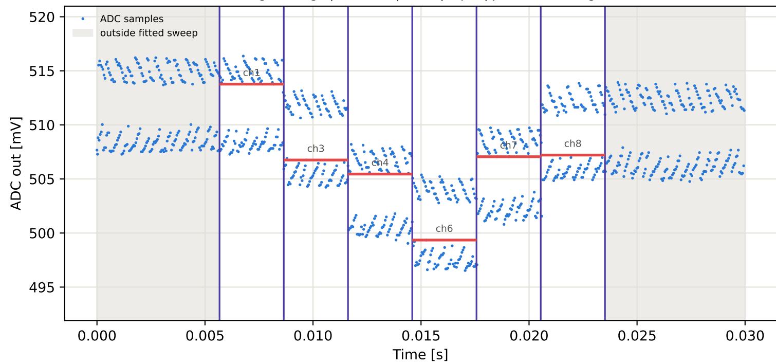
Tag9 &lt;- Tag15 | 905 MHz | run 0 | rep 1 | phase -92.59 deg
