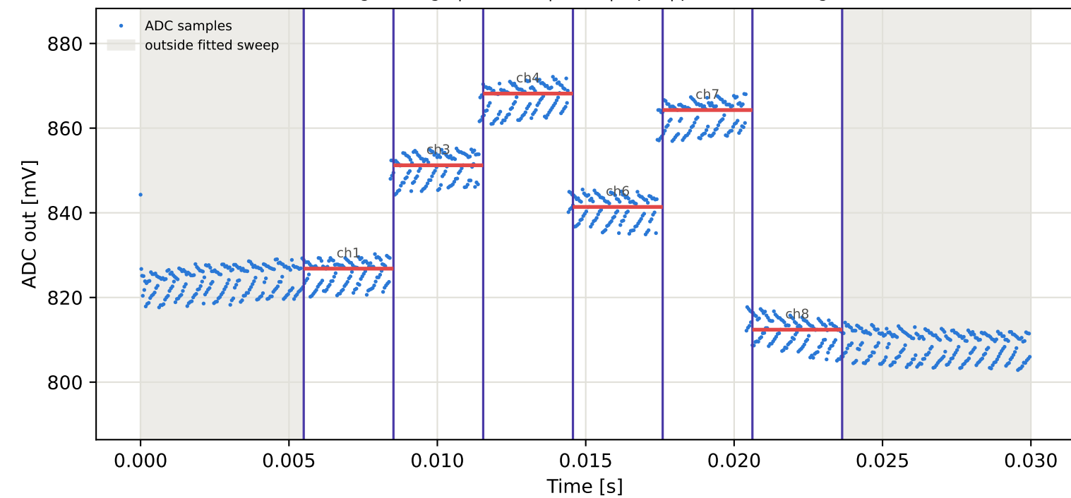
Tag9 &lt;- Tag10 | 905 MHz | run 0 | rep 1 | phase 47.81 deg
