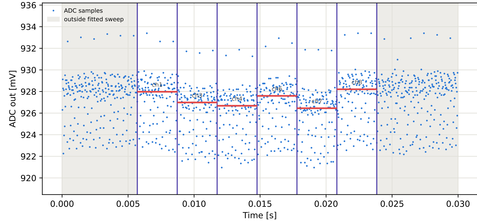
Tag3 &lt;- Tag9 | 875 MHz | run 0 | rep 1 | phase -150.93 deg
