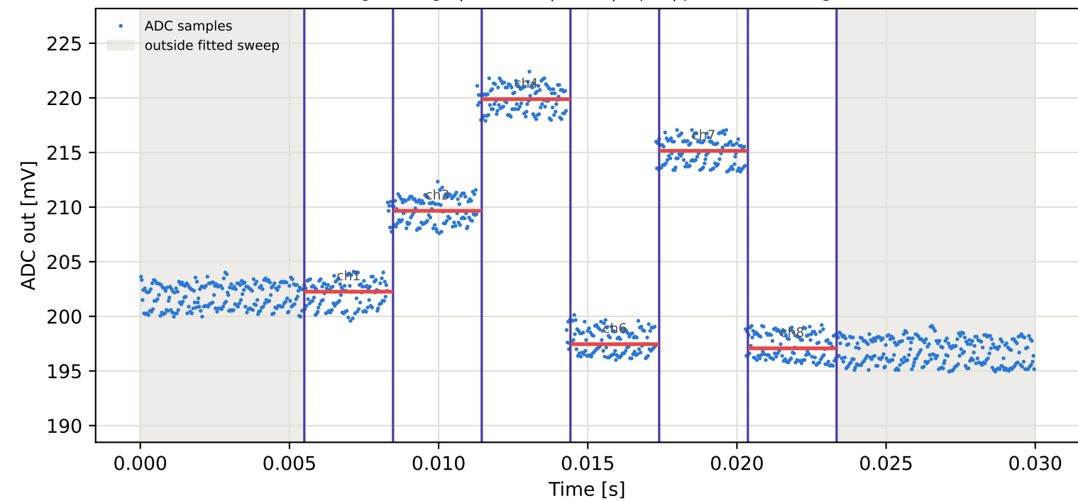
Tag7 &lt;- Tag1 | 985 MHz | run 0 | rep 1 | phase -7.58 deg
