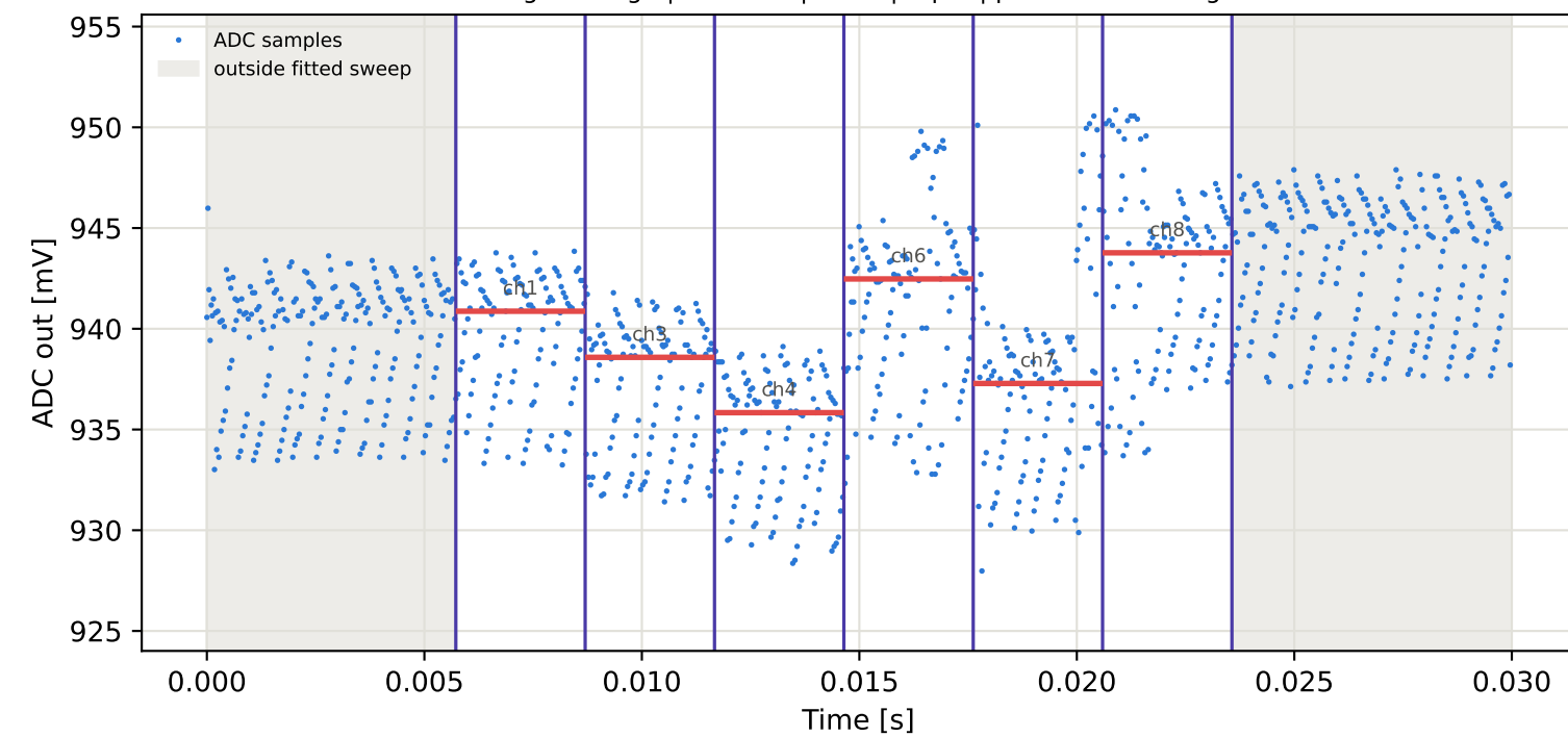
Tag8 &lt;- Tag4 | 915 MHz | run 0 | rep 1 | phase 110.07 deg
