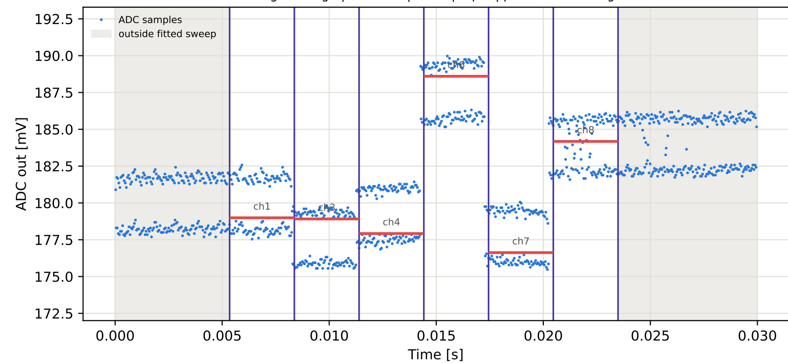
Tag1 &lt;- Tag7 | 995 MHz | run 0 | rep 1 | phase 146.55 deg
