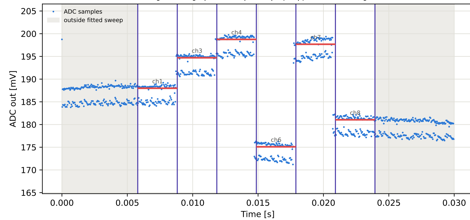
Tag10 &lt;- Tag4 | 985 MHz | run 0 | rep 1 | phase -34.31 deg
