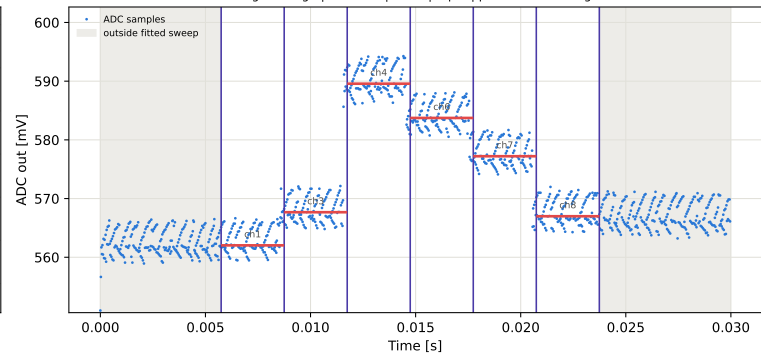
Tag9 &lt;- Tag6 | 965 MHz | run 0 | rep 1 | phase -157.57 deg
