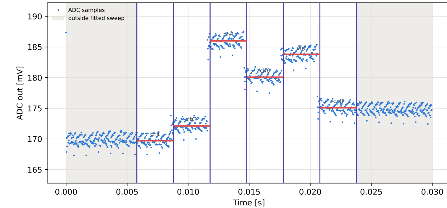
Tag4 &lt;- Tag2 | 825 MHz | run 0 | rep 1 | phase 75.35 deg
