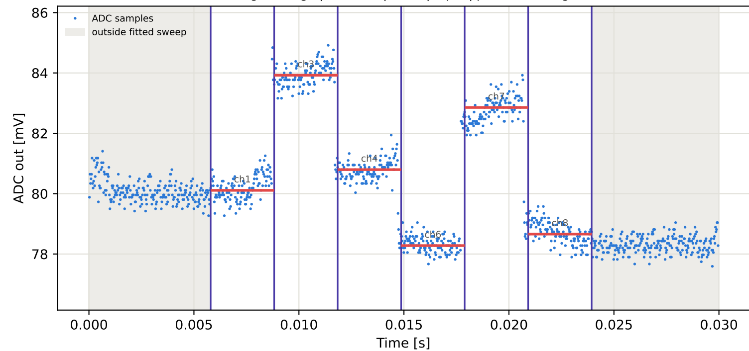
Tag10 &lt;- Tag1 | 805 MHz | run 0 | rep 1 | phase -42.06 deg
