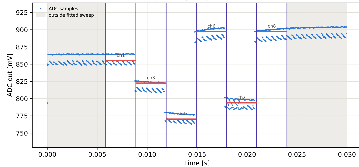
Tag2 &lt;- Tag1 | 945 MHz | run 0 | rep 1 | phase -176.40 deg
