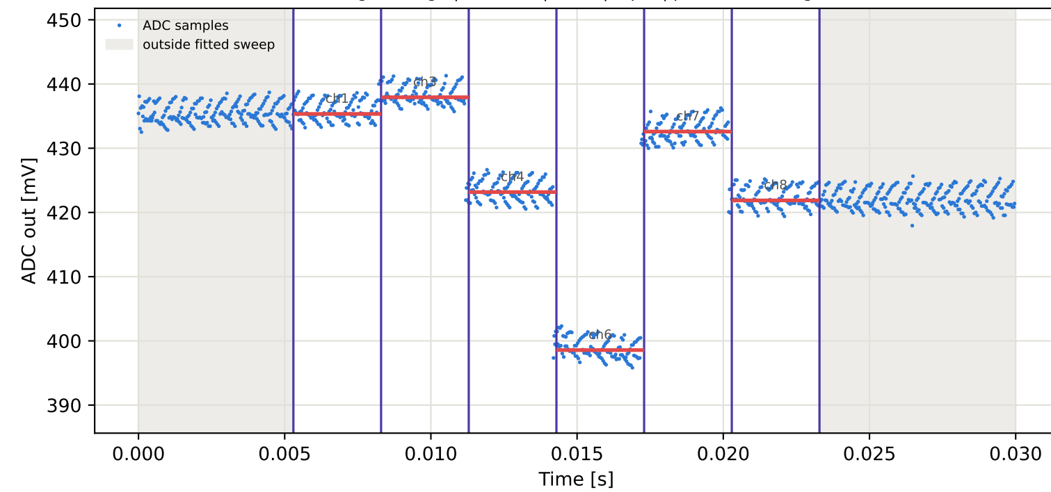
Tag8 &lt;- Tag1 | 955 MHz | run 0 | rep 1 | phase -67.13 deg
