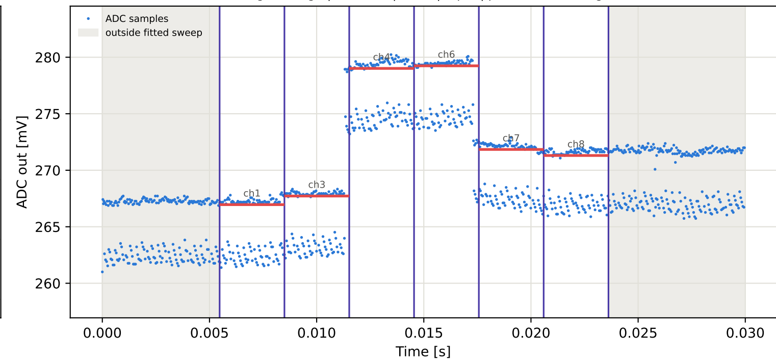
Tag3 &lt;- Tag7 | 995 MHz | run 0 | rep 1 | phase -71.70 deg
