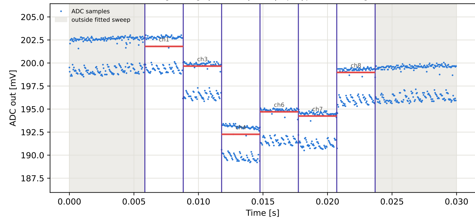
Tag9 &lt;- Tag10 | 805 MHz | run 0 | rep 1 | phase 172.23 deg
