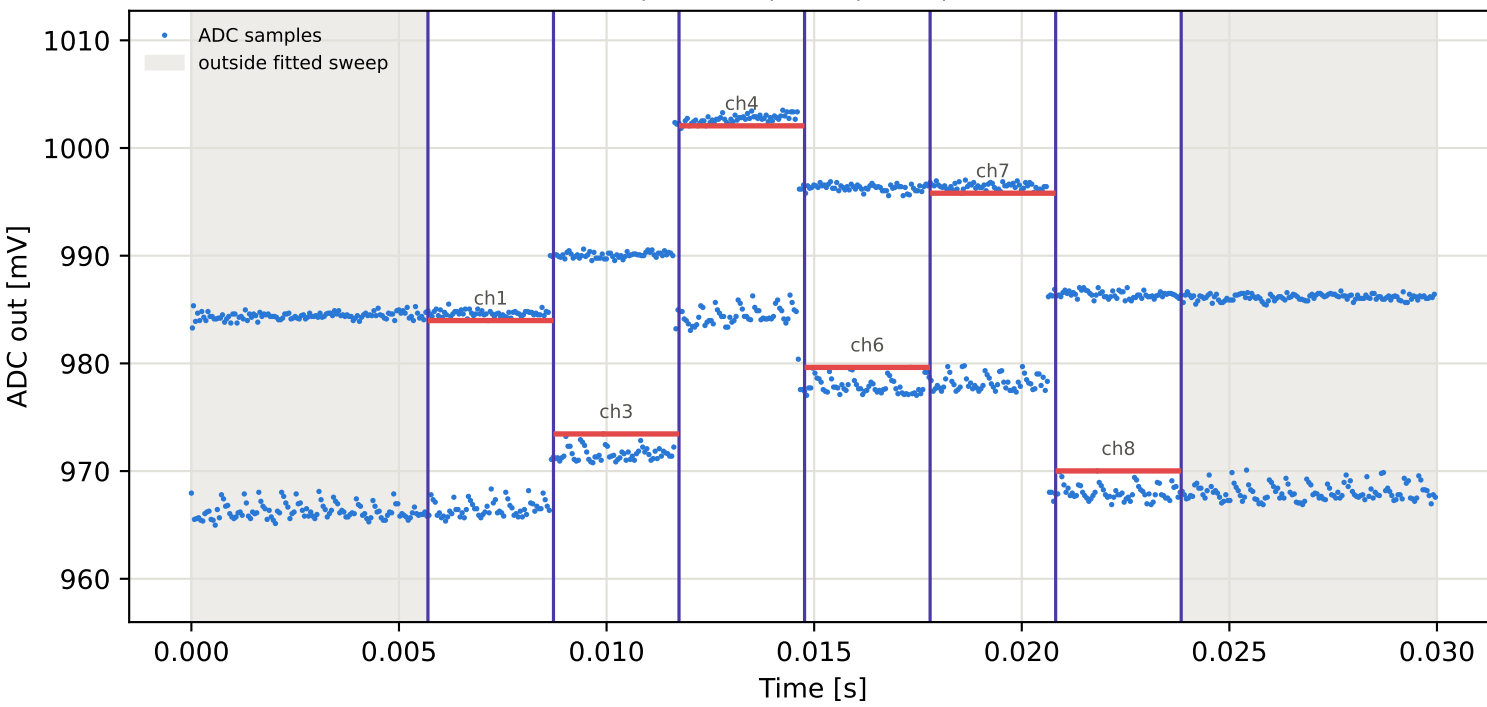
Tag15 &lt;- Tag1 | 955 MHz | run 0 | rep 1 | phase -93.91 deg
