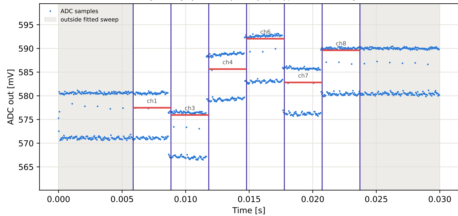
Tag8 &lt;- Tag5 | 835 MHz | run 0 | rep 1 | phase -149.89 deg
