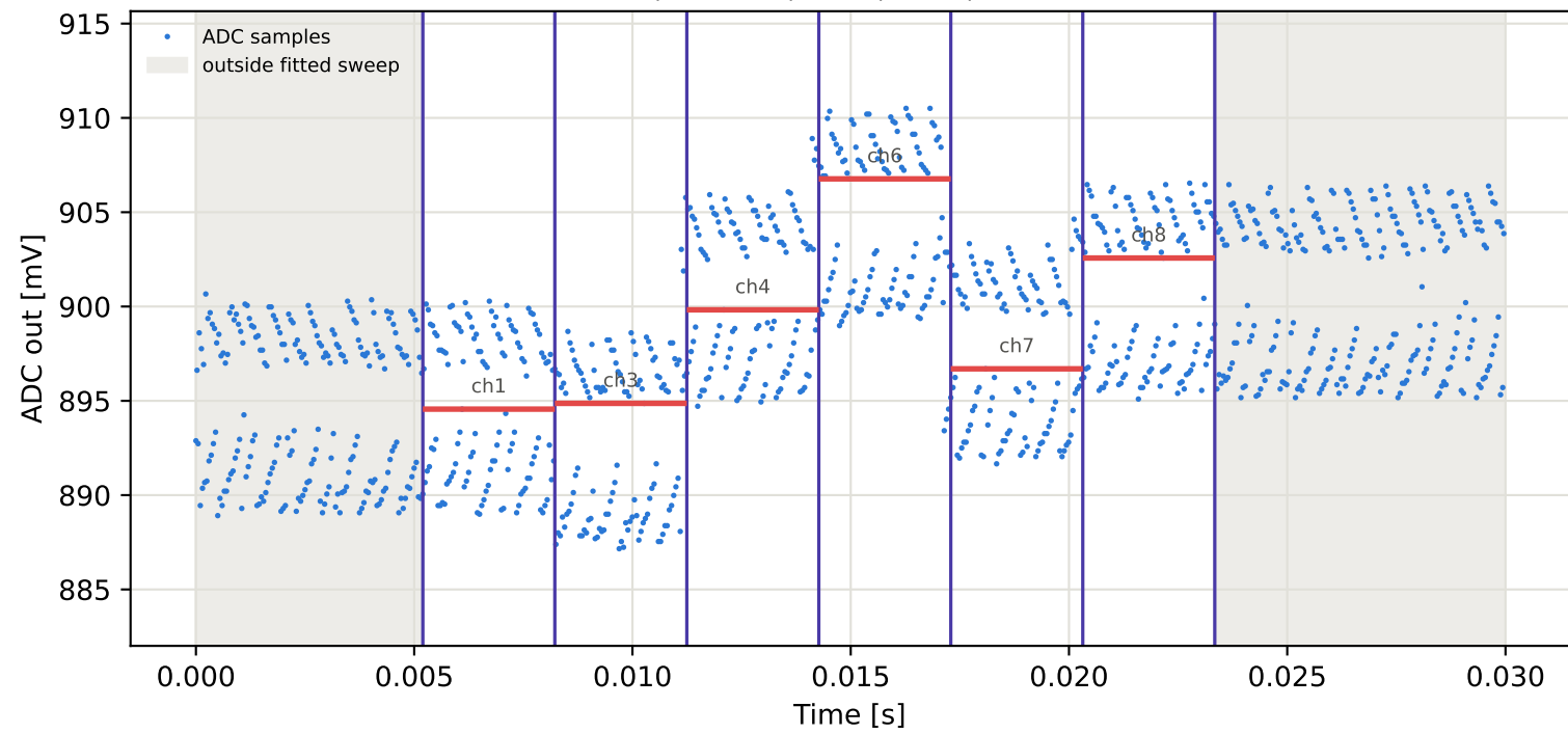
Tag8 &lt;- Tag7 | 855 MHz | run 0 | rep 1 | phase -154.83 deg
