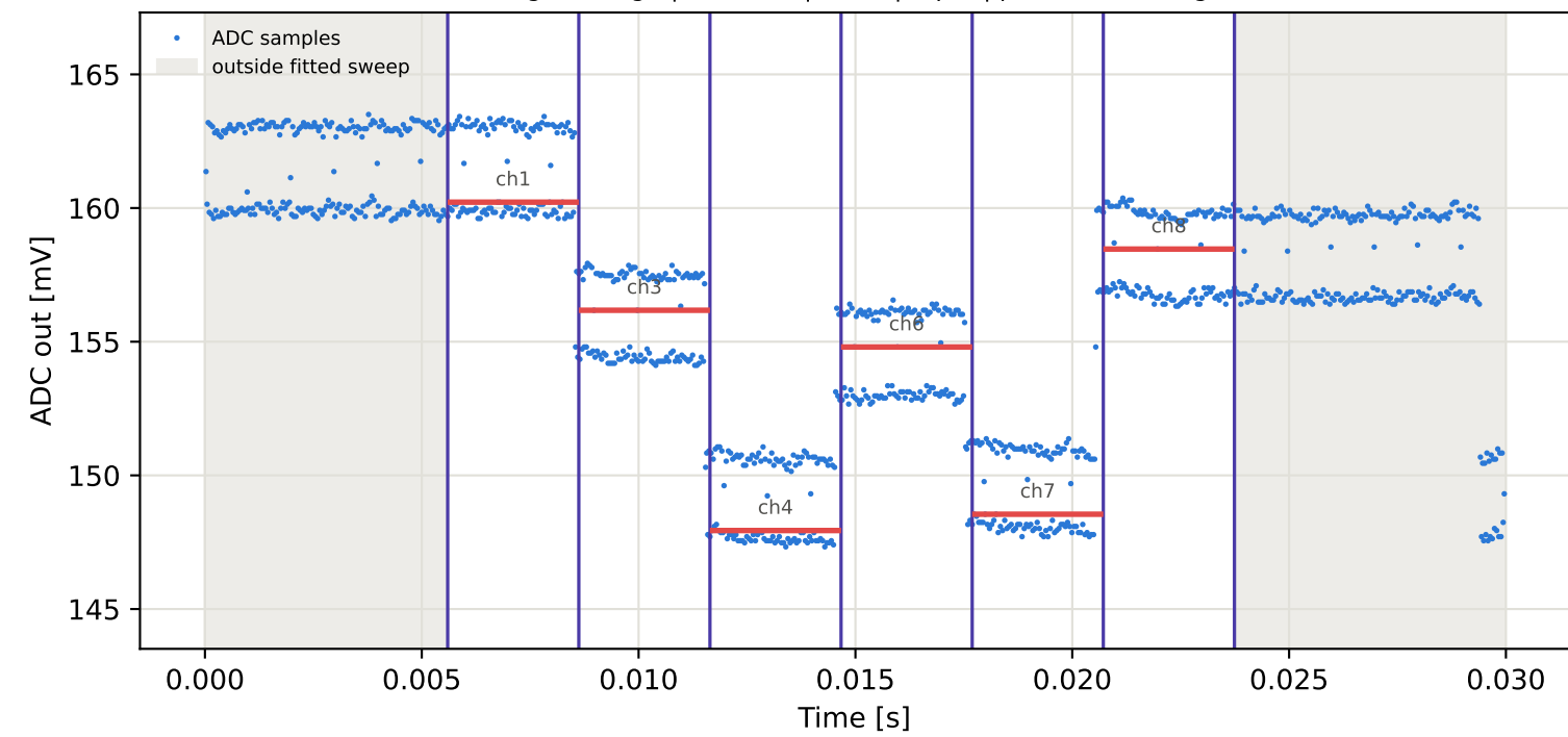
Tag4 &lt;- Tag8 | 805 MHz | run 0 | rep 1 | phase 128.19 deg
