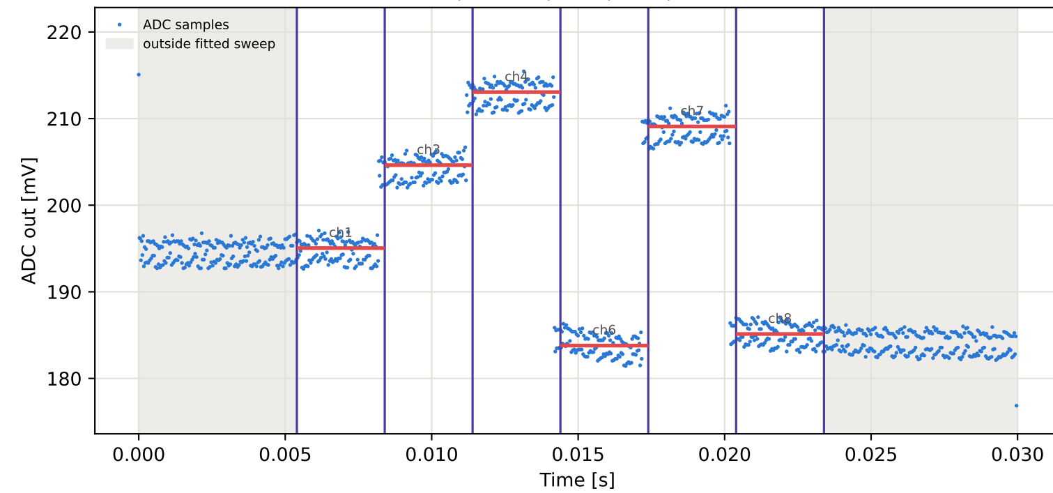
Tag10 &lt;- Tag4 | 945 MHz | run 0 | rep 1 | phase -46.12 deg
