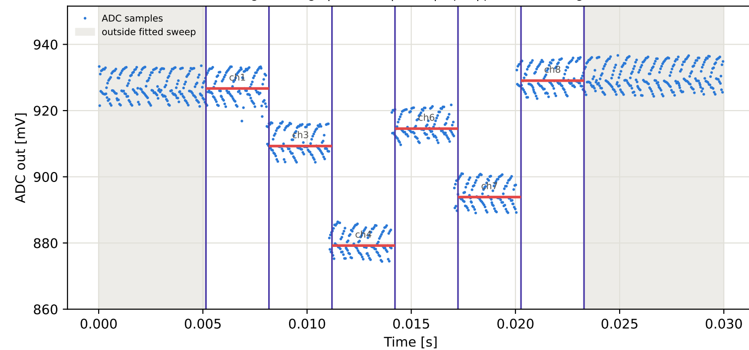
Tag16 &lt;- Tag10 | 975 MHz | run 0 | rep 1 | phase -54.68 deg
