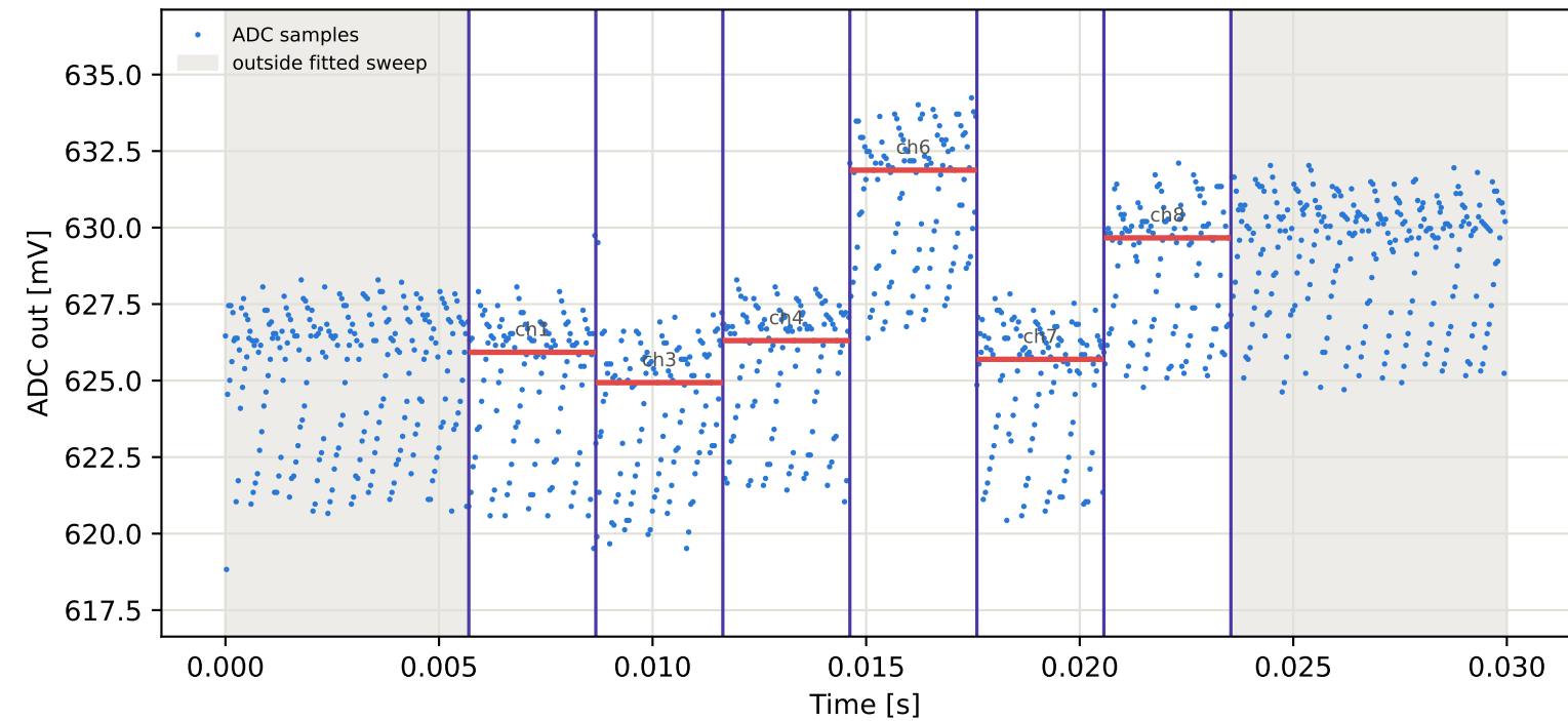
Tag7 &lt;- Tag15 | 905 MHz | run 0 | rep 1 | phase 152.86 deg
