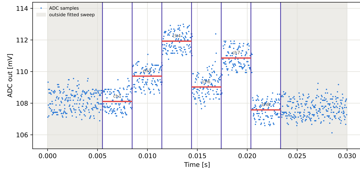
Tag2 &lt;- Tag7 | 945 MHz | run 0 | rep 1 | phase -44.88 deg
