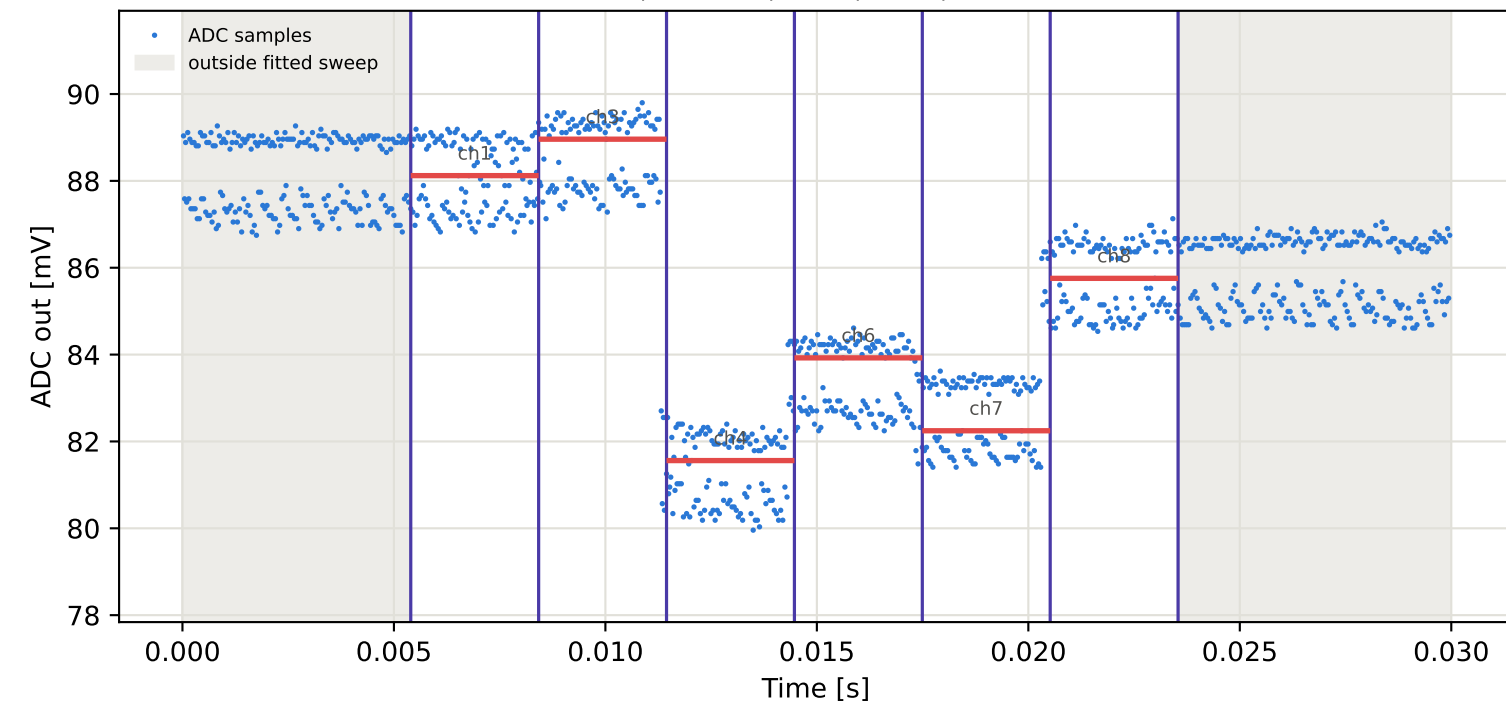
Tag8 &lt;- Tag6 | 785 MHz | run 0 | rep 1 | phase 74.32 deg
