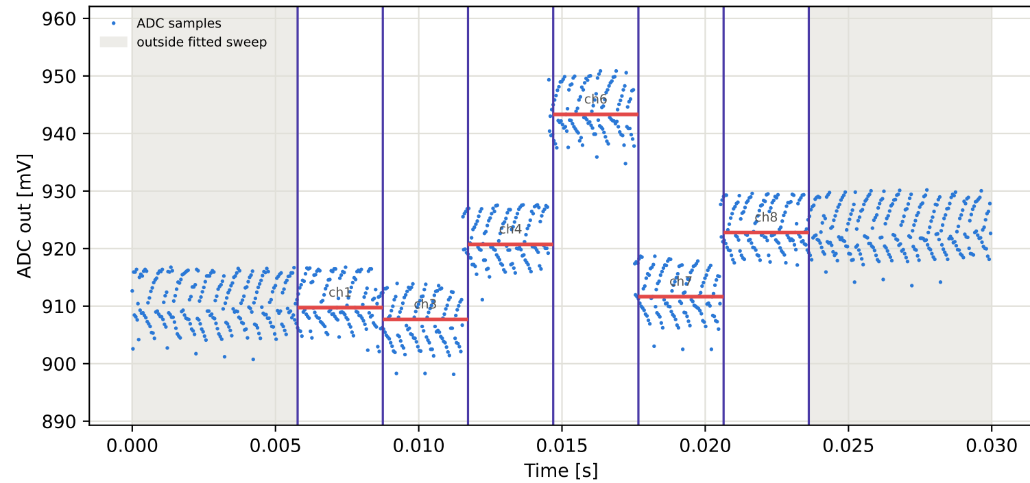
Tag15 &lt;- Tag6 | 965 MHz | run 0 | rep 1 | phase -79.87 deg
