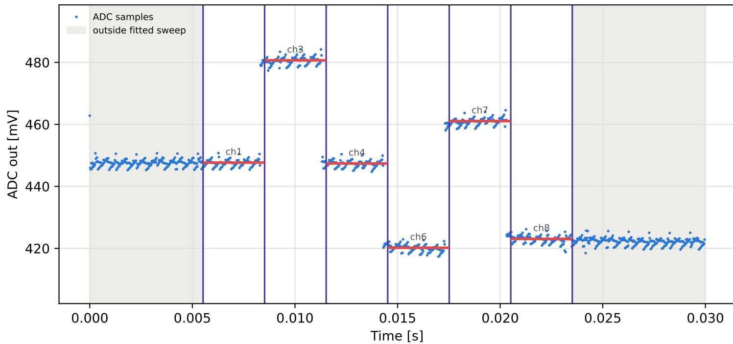
Tag2 &lt;- Tag1 | 825 MHz | run 0 | rep 1 | phase -154.65 deg
