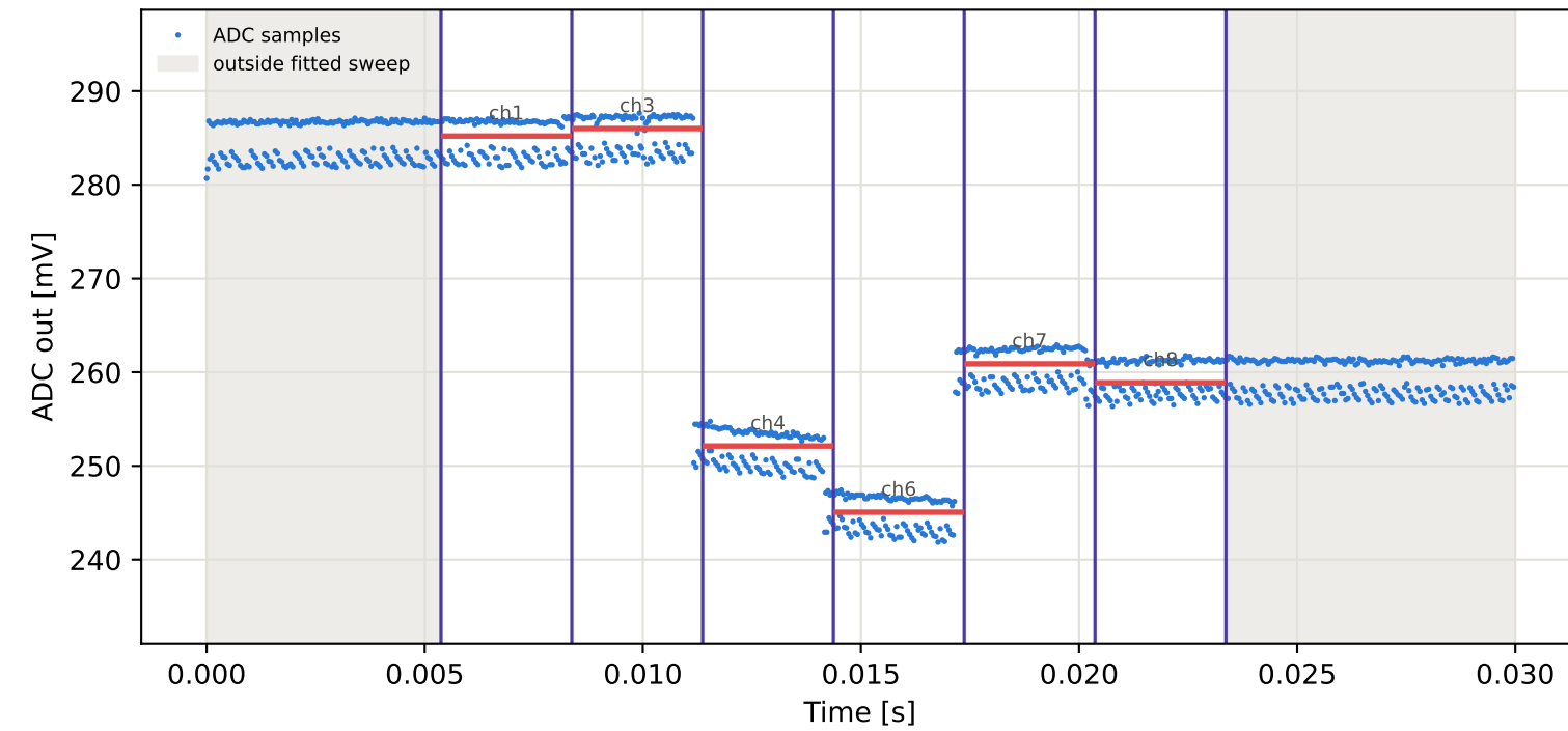
Tag3 &lt;- Tag8 | 825 MHz | run 0 | rep 1 | phase 122.88 deg
