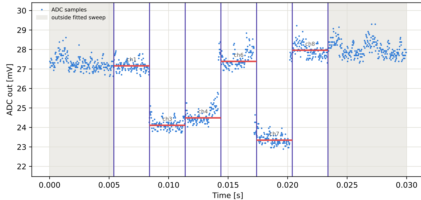
Tag1 &lt;- Tag9 | 775 MHz | run 0 | rep 1 | phase -123.76 deg
