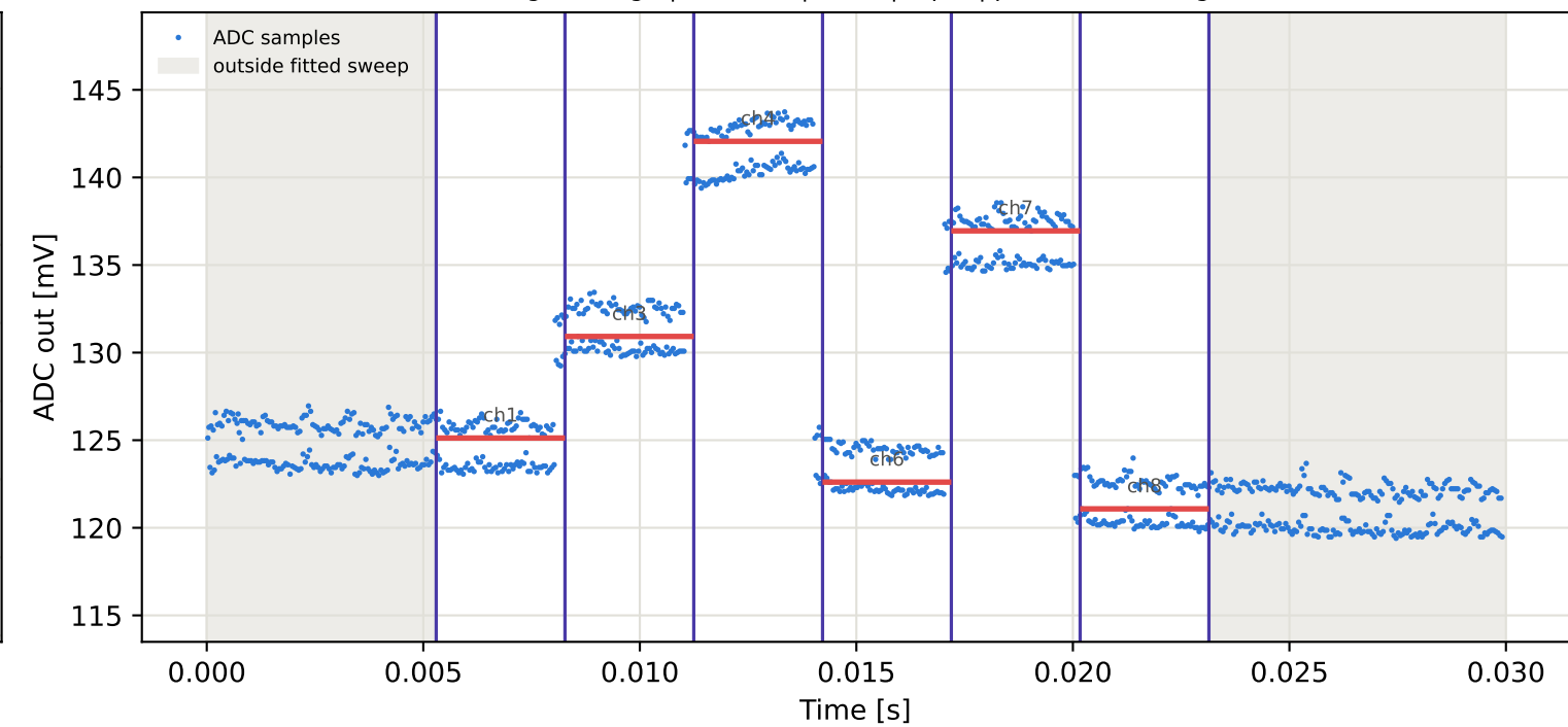
Tag7 &lt;- Tag1 | 965 MHz | run 0 | rep 1 | phase -50.83 deg
