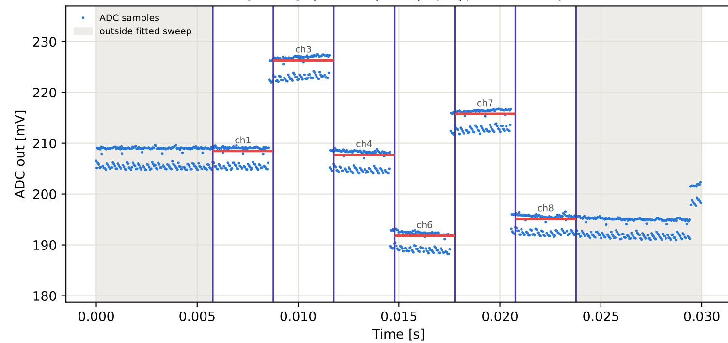
Tag3 &lt;- Tag8 | 805 MHz | run 0 | rep 1 | phase 102.03 deg
