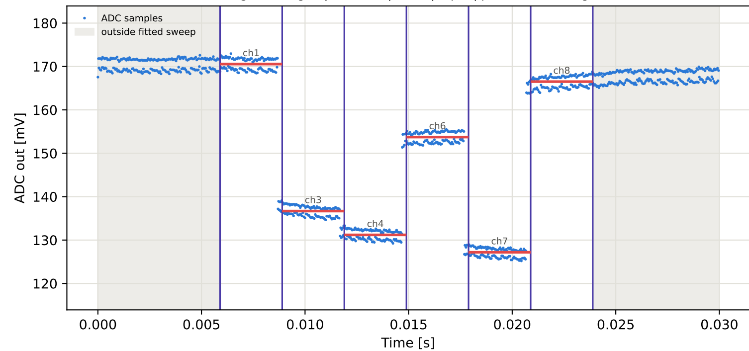
Tag10 &lt;- Tag3 | 845 MHz | run 0 | rep 1 | phase -146.03 deg
