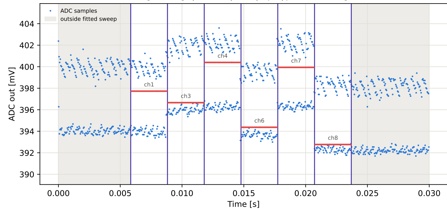
Tag15 &lt;- Tag4 | 845 MHz | run 0 | rep 1 | phase -154.88 deg
