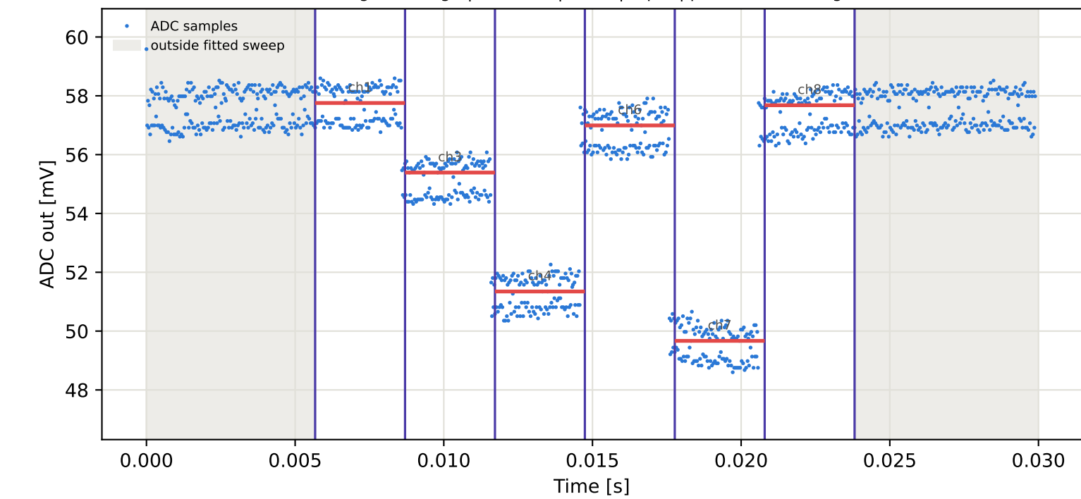
Tag16 &lt;- Tag6 | 775 MHz | run 0 | rep 1 | phase 161.51 deg
