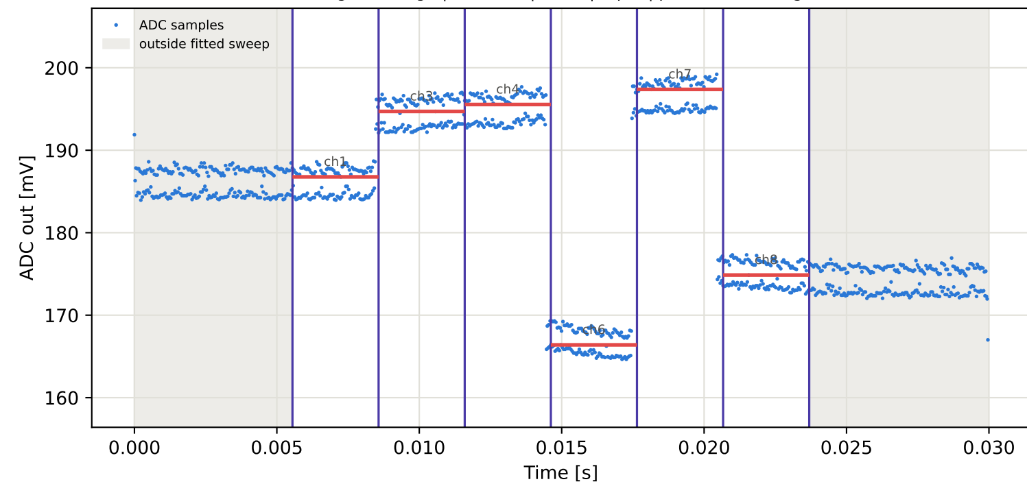
Tag10 &lt;- Tag9 | 955 MHz | run 0 | rep 1 | phase -61.05 deg
