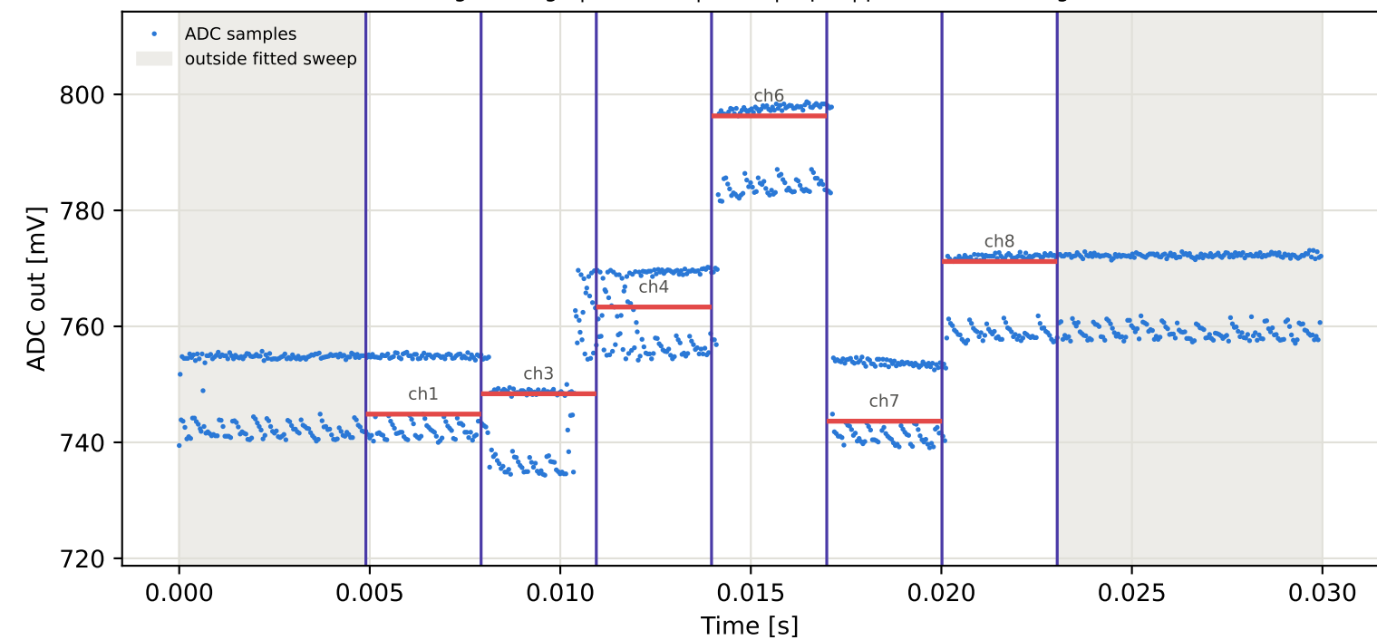
Tag4 &lt;- Tag3 | 975 MHz | run 0 | rep 1 | phase -168.76 deg
