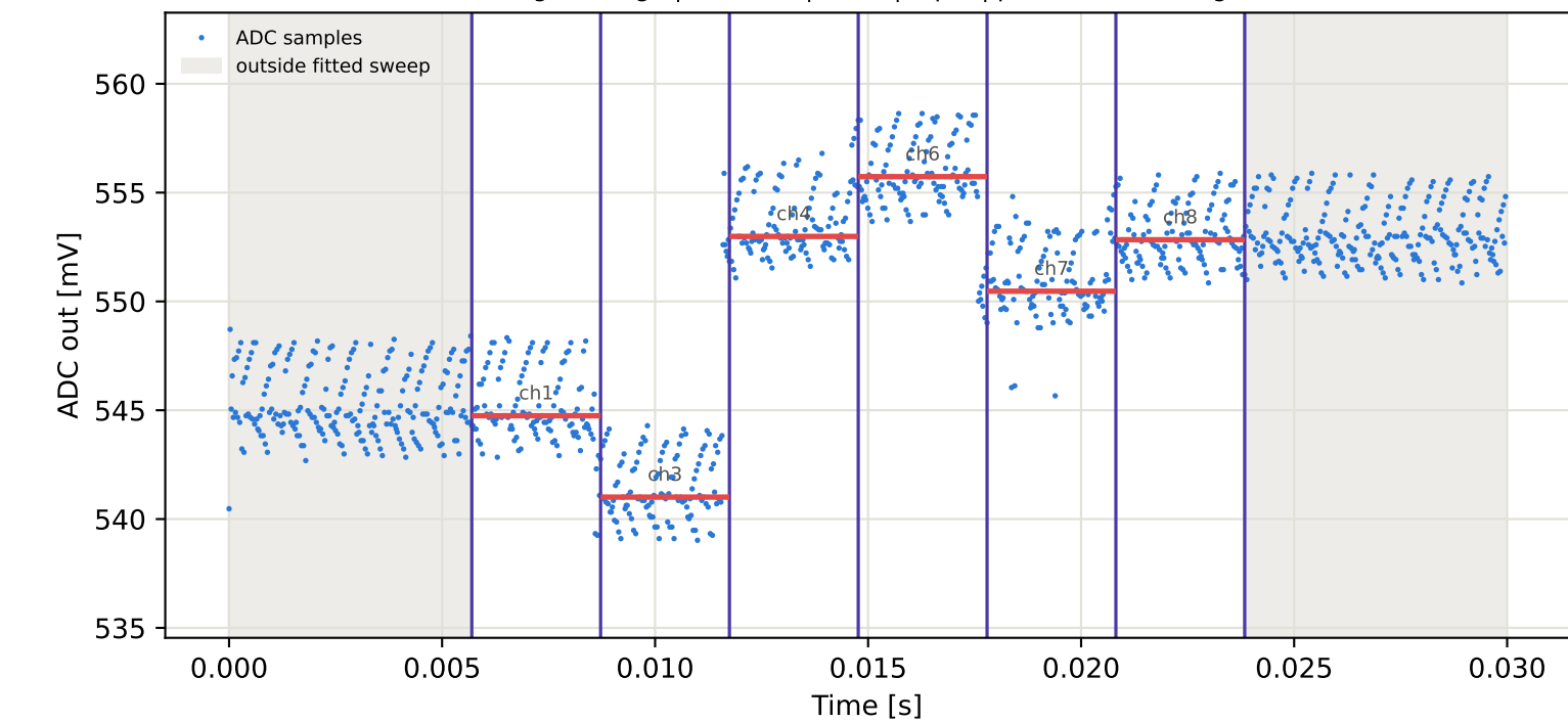
Tag8 &lt;- Tag6 | 825 MHz | run 0 | rep 1 | phase -27.83 deg
