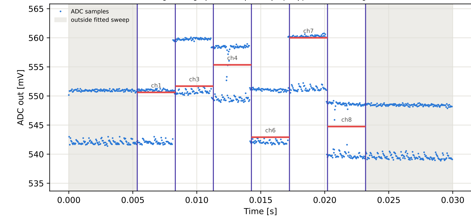
Tag8 &lt;- Tag6 | 825 MHz | run 0 | rep 1 | phase -27.83 deg
