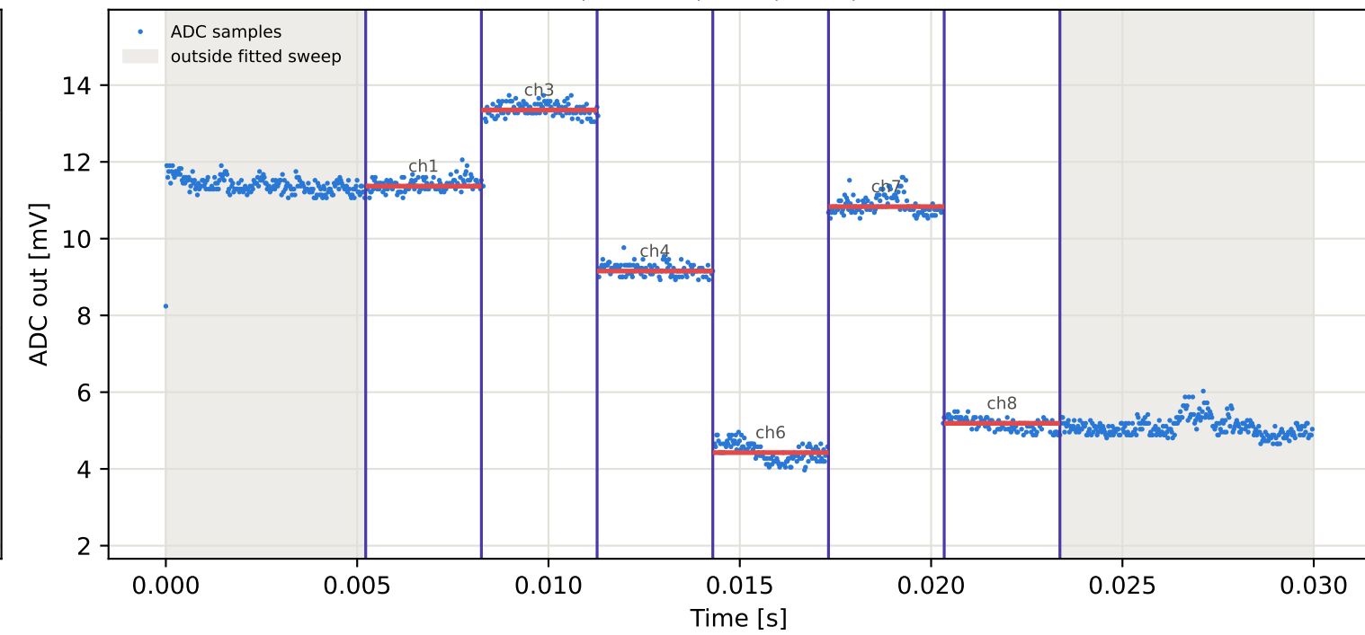
Tag2 &lt;- Tag8 | 865 MHz | run 0 | rep 1 | phase 16.03 deg
