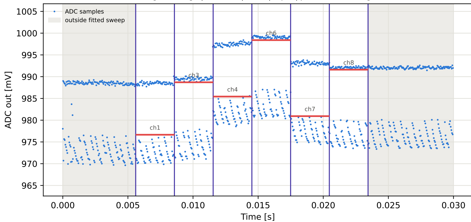
Tag15 &lt;- Tag9 | 955 MHz | run 0 | rep 1 | phase -10.55 deg
