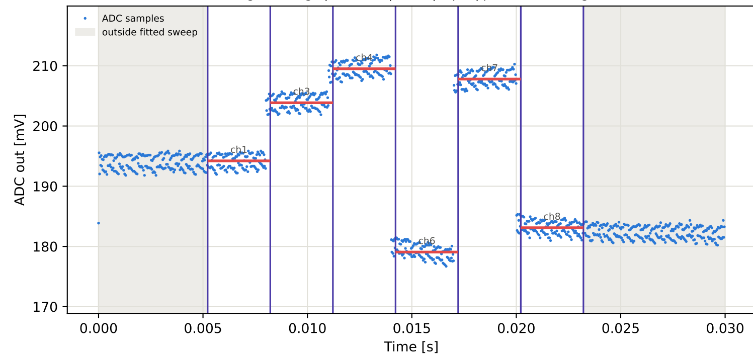
Tag10 &lt;- Tag9 | 945 MHz | run 0 | rep 1 | phase -83.26 deg
