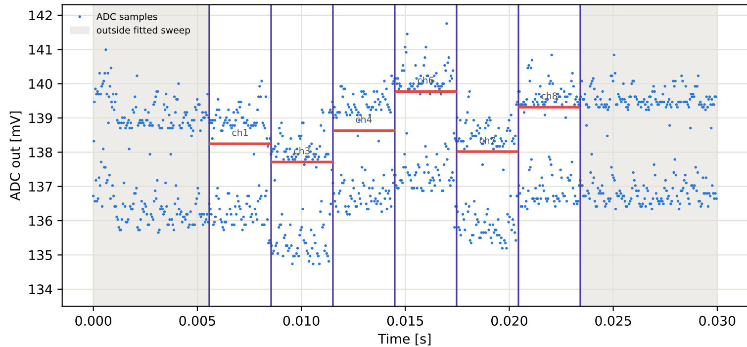
Tag7 &lt;- Tag15 | 795 MHz | run 0 | rep 1 | phase -56.78 deg
