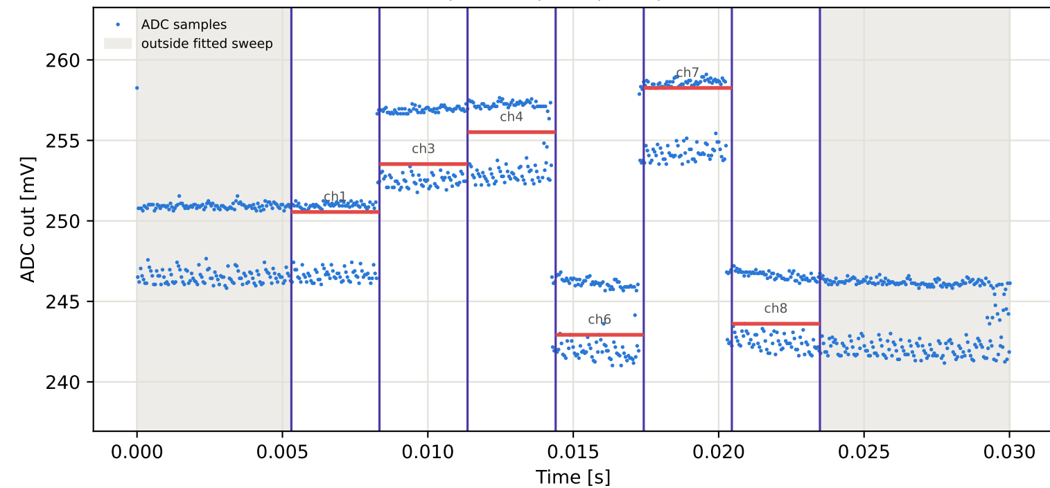
Tag3 &lt;- Tag2 | 825 MHz | run 0 | rep 1 | phase -23.81 deg
