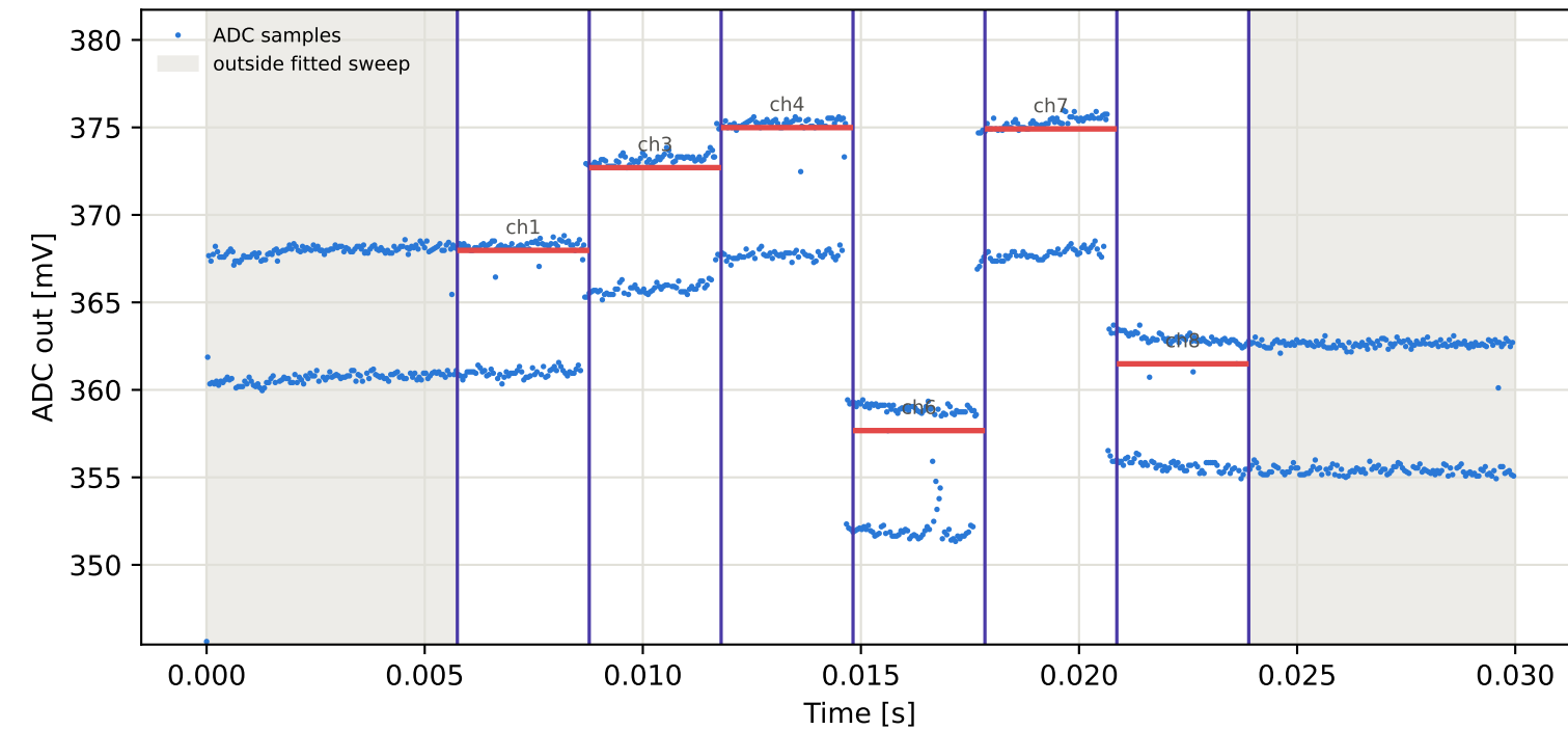
Tag9 &lt;- Tag16 | 985 MHz | run 0 | rep 1 | phase 20.38 deg
