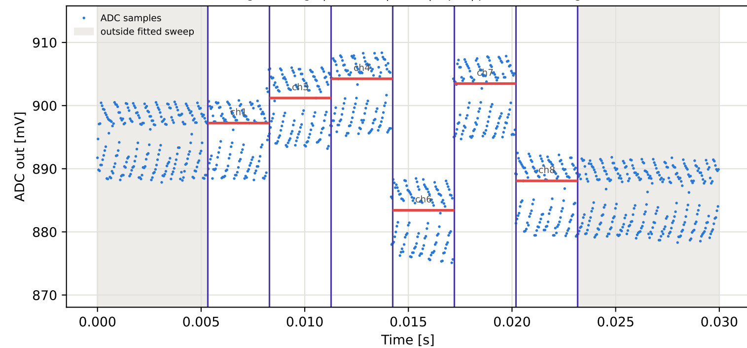
Tag16 &lt;- Tag5 | 935 MHz | run 0 | rep 1 | phase 153.10 deg
