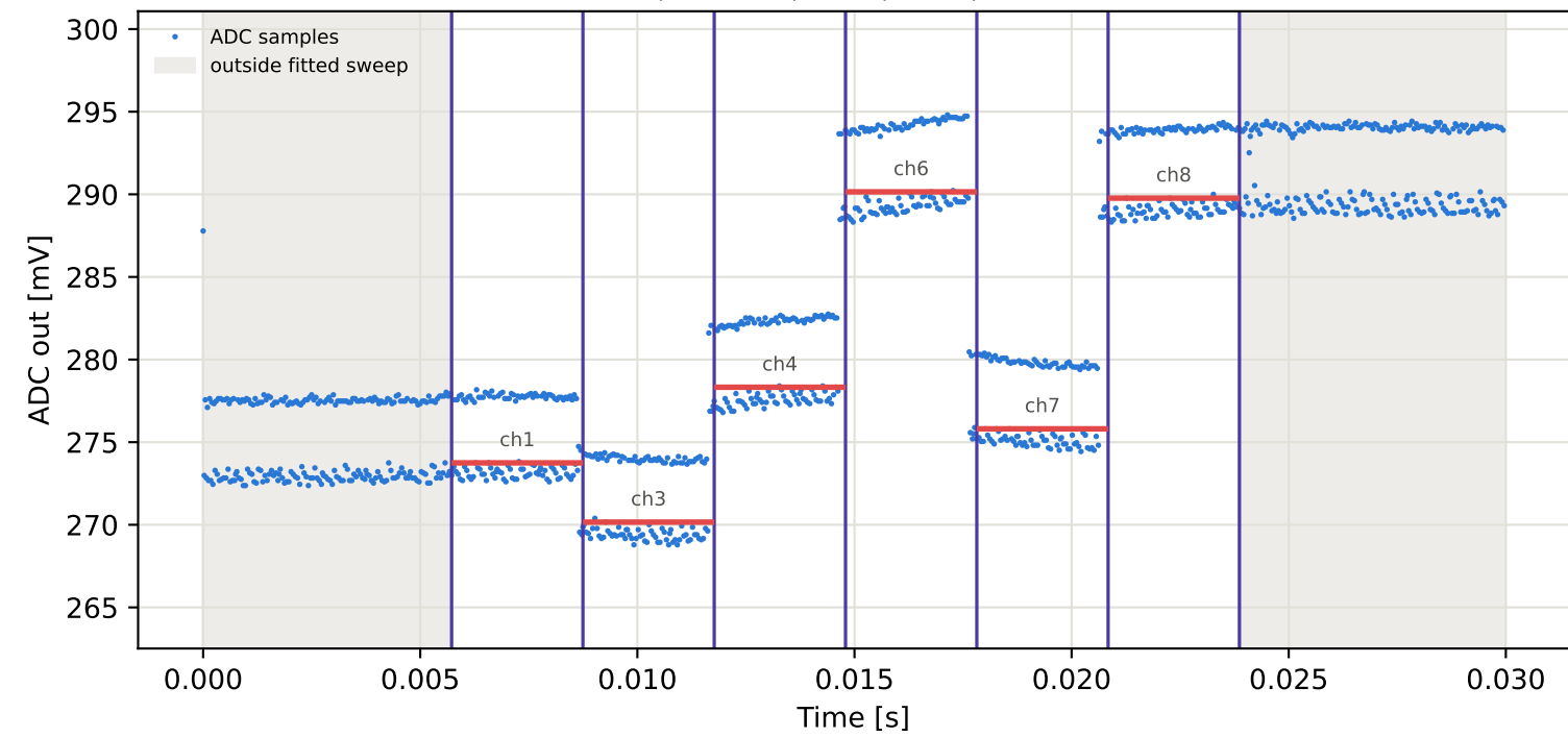
Tag1 &lt;- Tag4 | 865 MHz | run 0 | rep 1 | phase -165.81 deg
