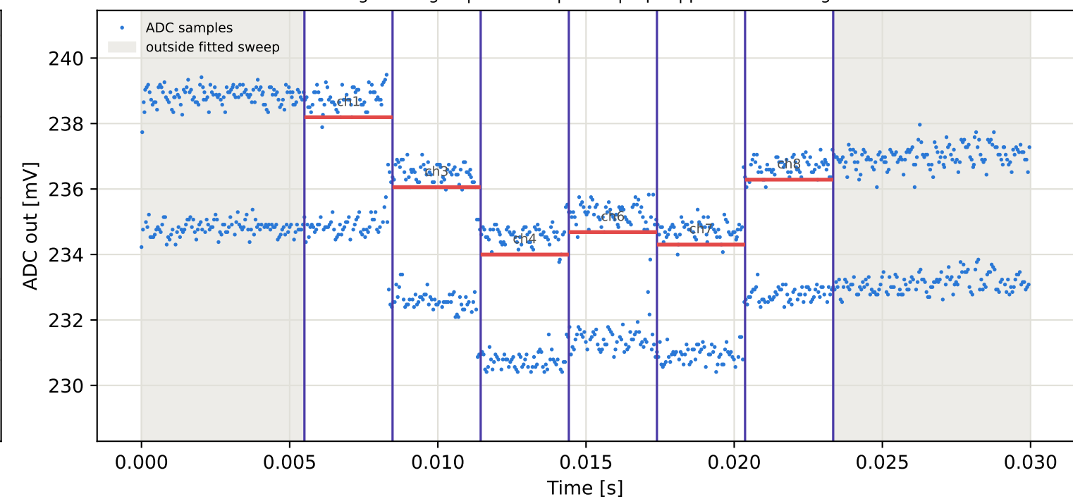
Tag7 &lt;- Tag15 | 855 MHz | run 0 | rep 1 | phase 73.61 deg
