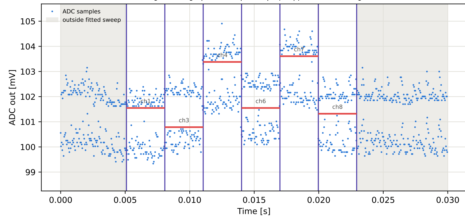
Tag10 &lt;- Tag5 | 775 MHz | run 0 | rep 1 | phase -79.70 deg
