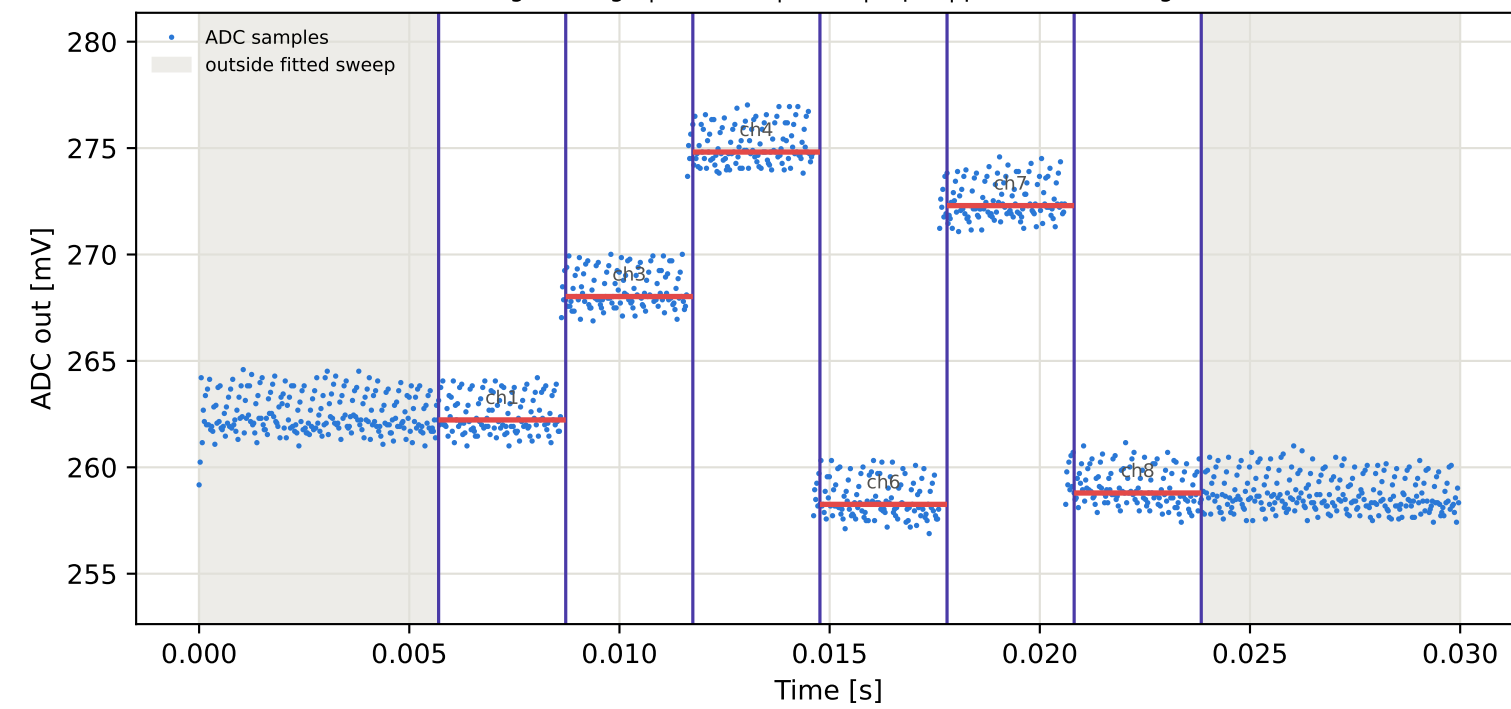
Tag3 &lt;- Tag8 | 995 MHz | run 0 | rep 1 | phase -63.63 deg
