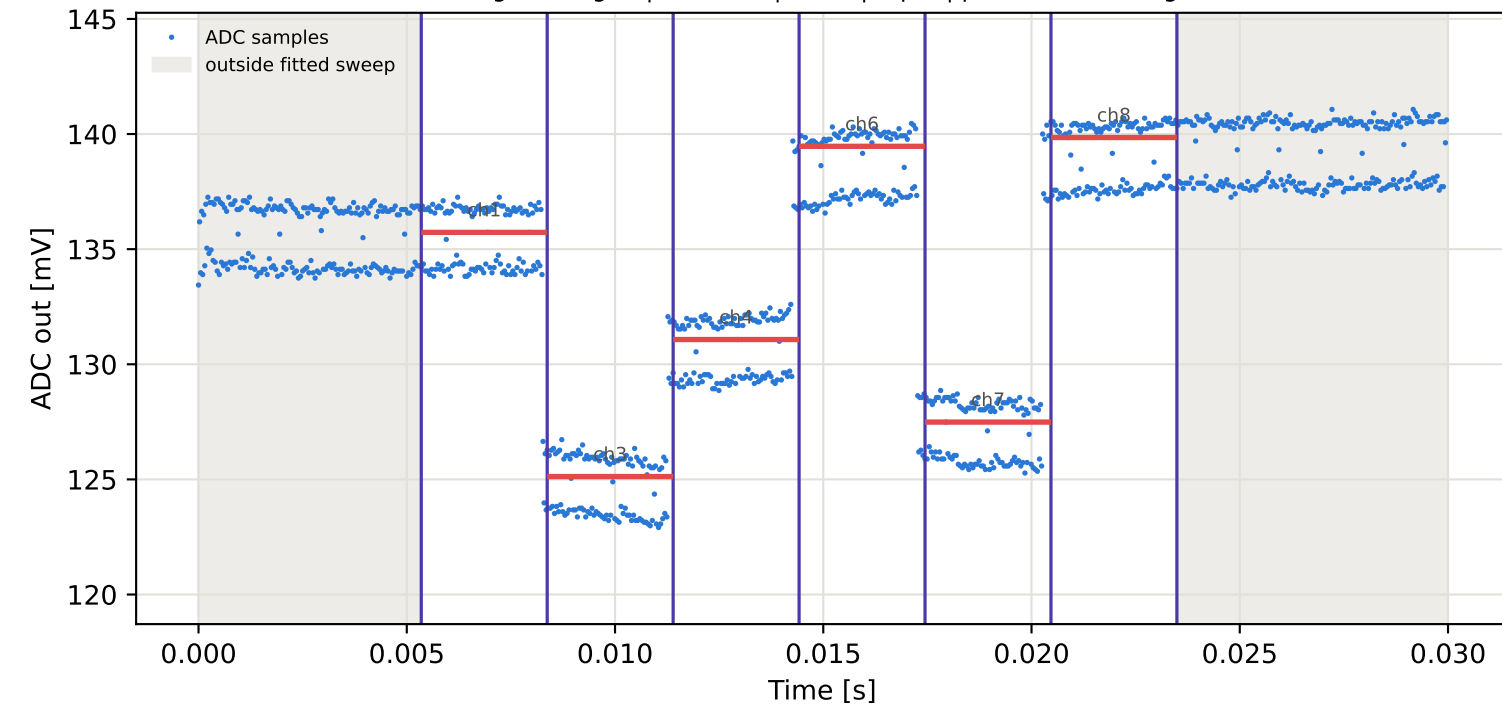
Tag2 &lt;- Tag15 | 835 MHz | run 0 | rep 1 | phase 173.10 deg
