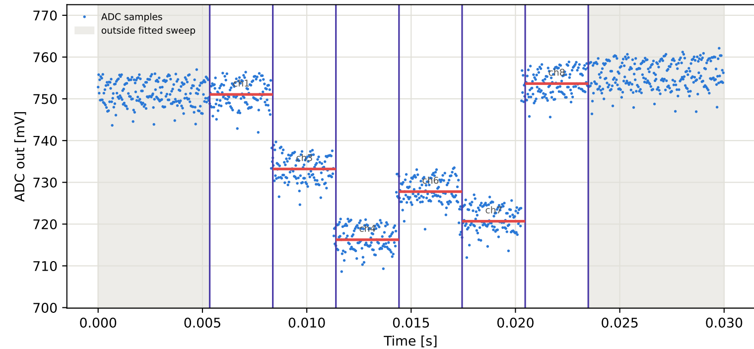
Tag9 &lt;- Tag8 | 885 MHz | run 0 | rep 1 | phase -38.19 deg
