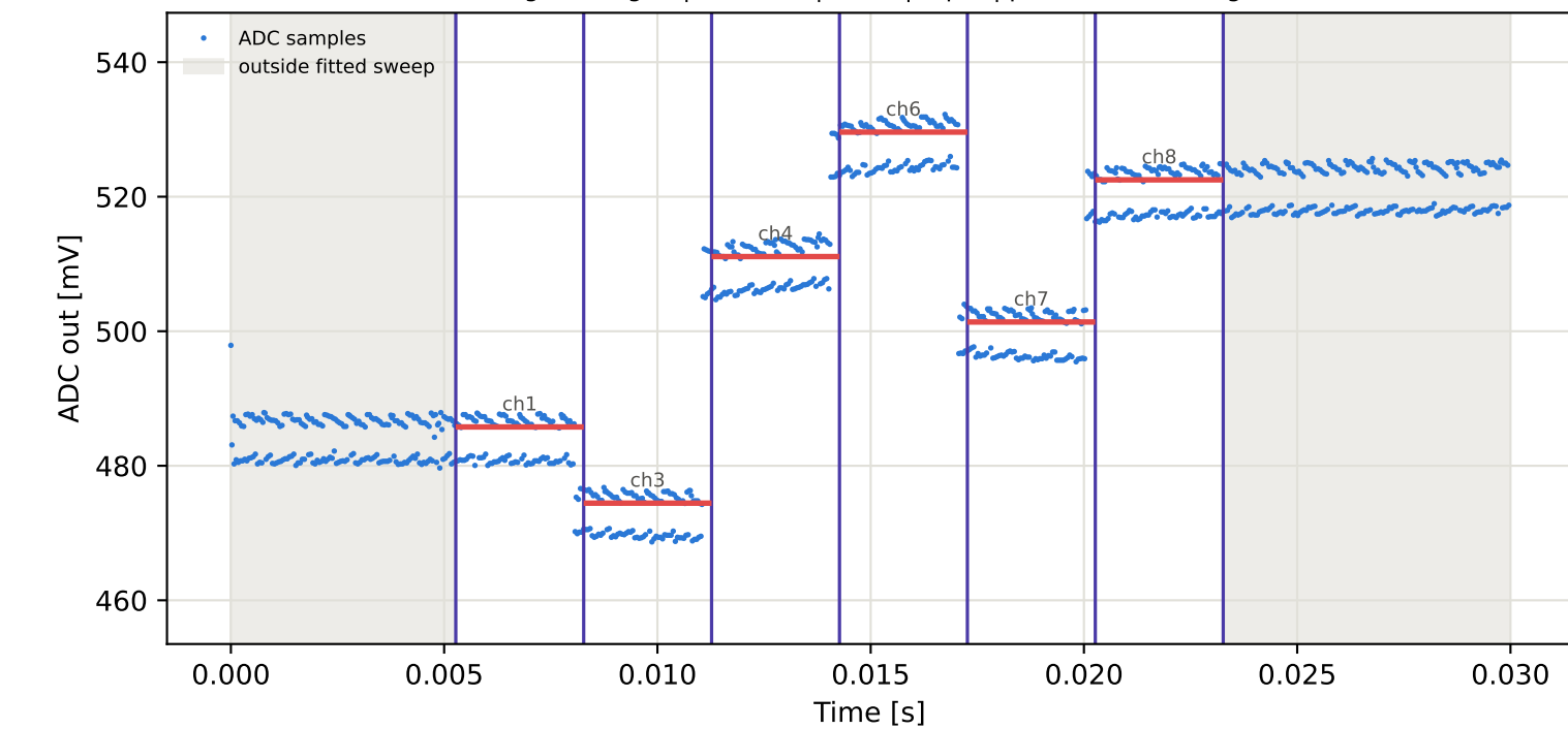
Tag5 &lt;- Tag3 | 855 MHz | run 0 | rep 1 | phase 80.13 deg
