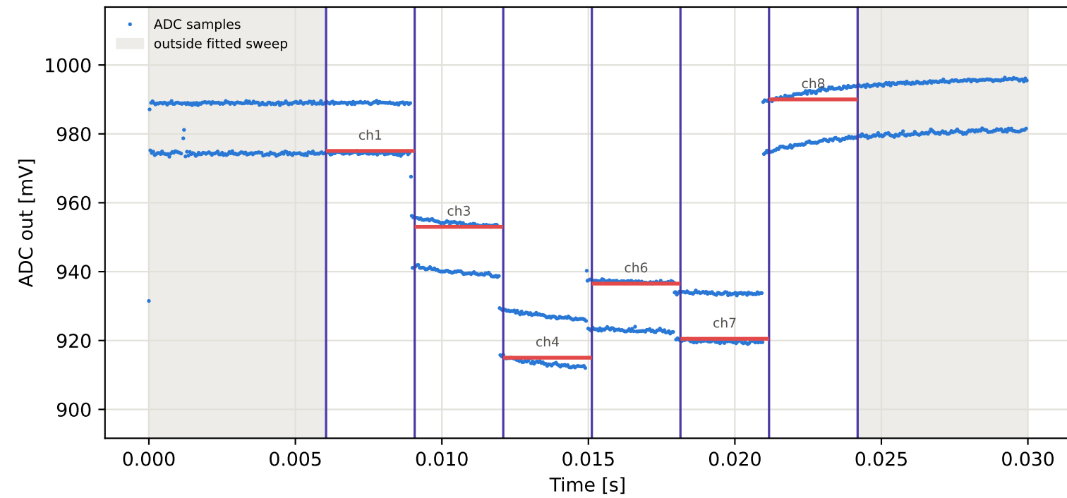
Tag16 &lt;- Tag1 | 895 MHz | run 0 | rep 1 | phase -71.02 deg
