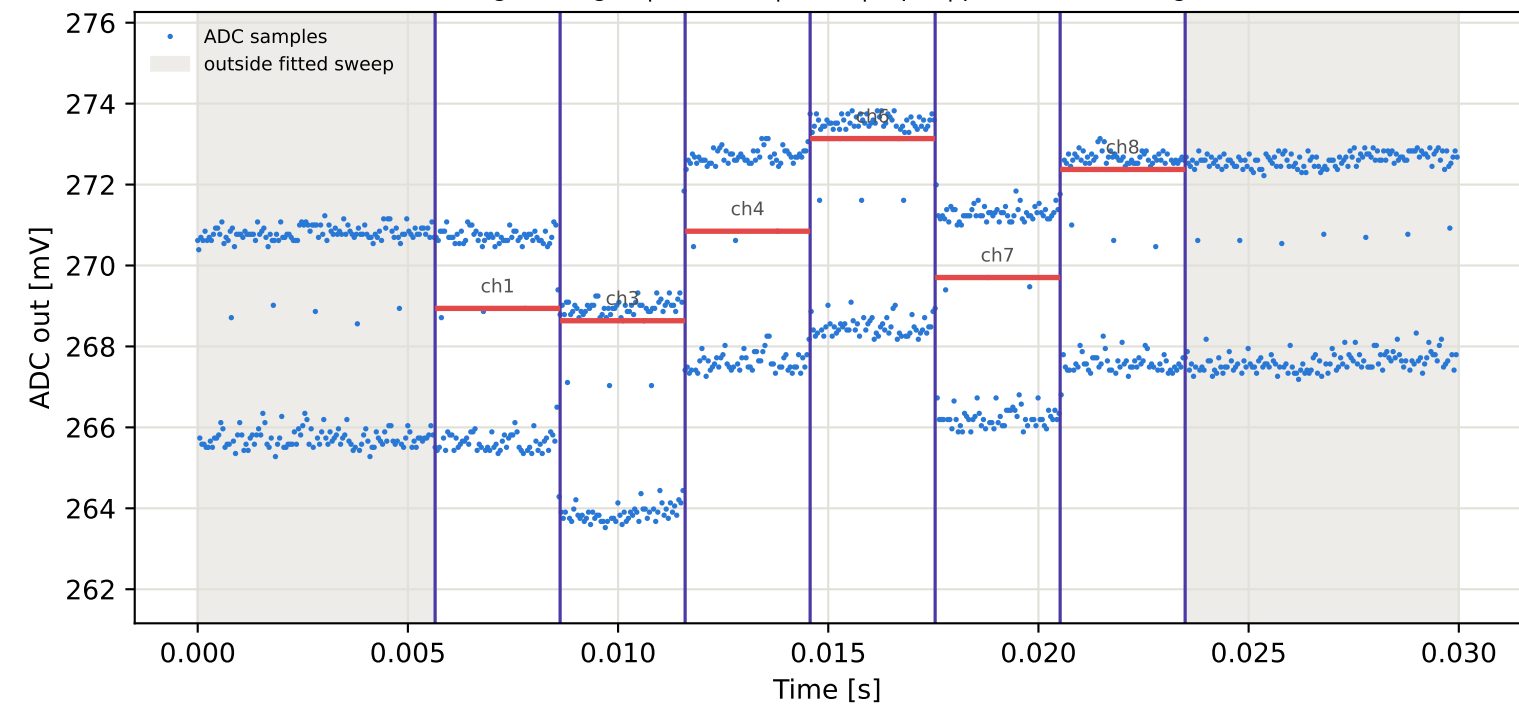
Tag1 &lt;- Tag2 | 825 MHz | run 0 | rep 1 | phase 177.61 deg
