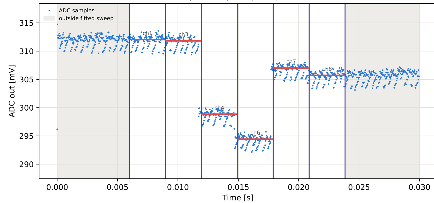
Tag10 &lt;- Tag8 | 965 MHz | run 0 | rep 1 | phase -25.00 deg
