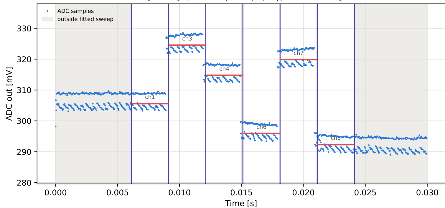
Tag7 &lt;- Tag6 | 835 MHz | run 0 | rep 1 | phase -12.39 deg
