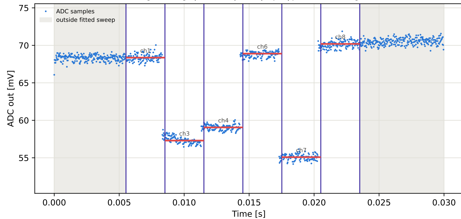
Tag10 &lt;- Tag8 | 785 MHz | run 0 | rep 1 | phase 114.76 deg
