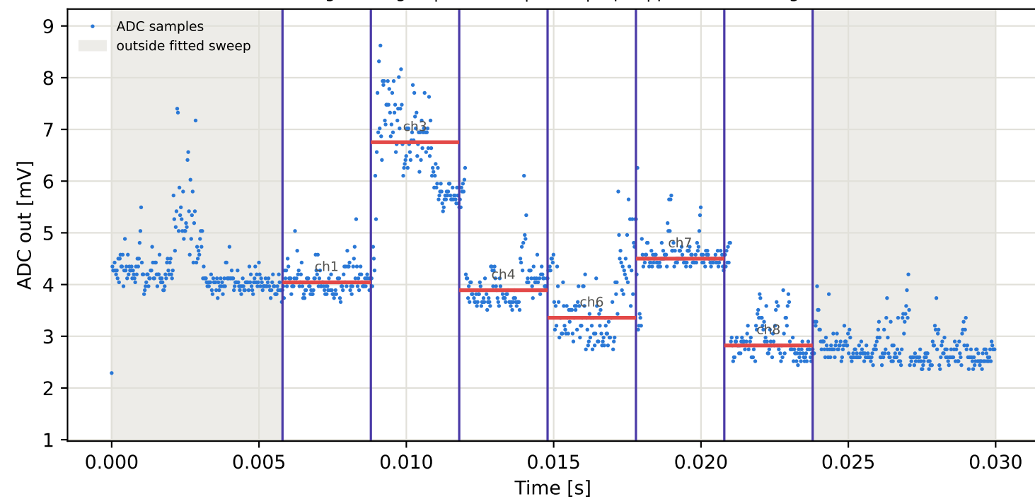
Tag7 &lt;- Tag15 | 845 MHz | run 0 | rep 1 | phase 21.23 deg
