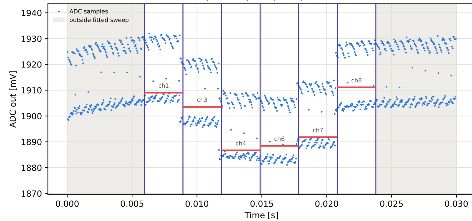
Tag5 &lt;- Tag8 | 895 MHz | run 0 | rep 1 | phase 170.26 deg
