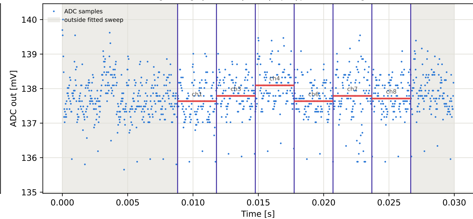
Tag7 &lt;- Tag4 | 795 MHz | run 0 | rep 1 | phase 30.45 deg
