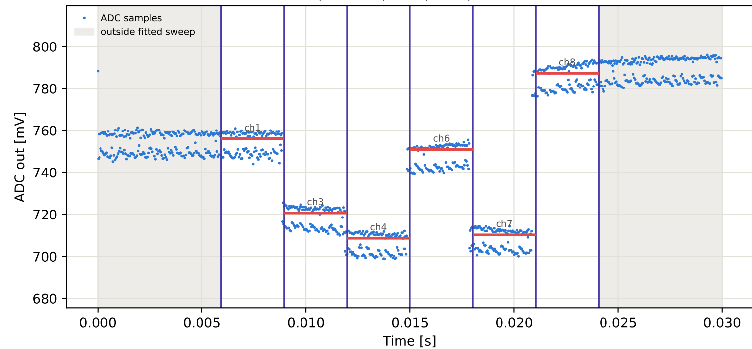
Tag9 &lt;- Tag6 | 885 MHz | run 0 | rep 1 | phase 82.39 deg
