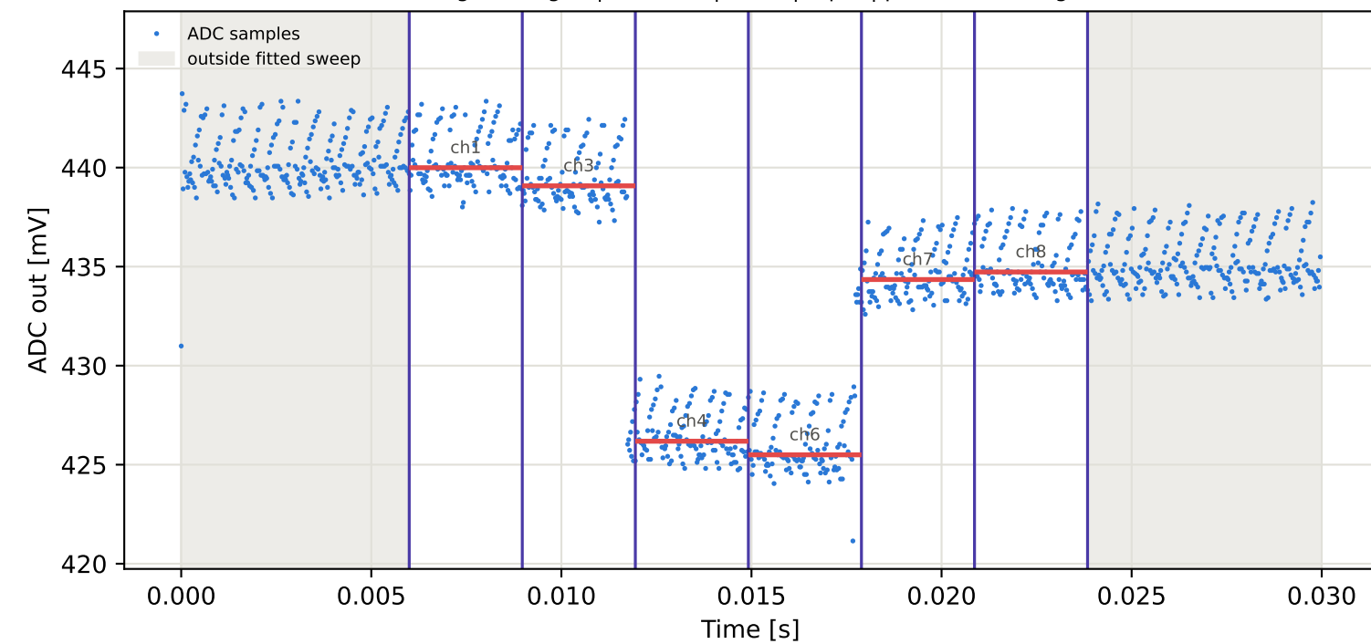
Tag4 &lt;- Tag2 | 995 MHz | run 0 | rep 1 | phase 77.05 deg
