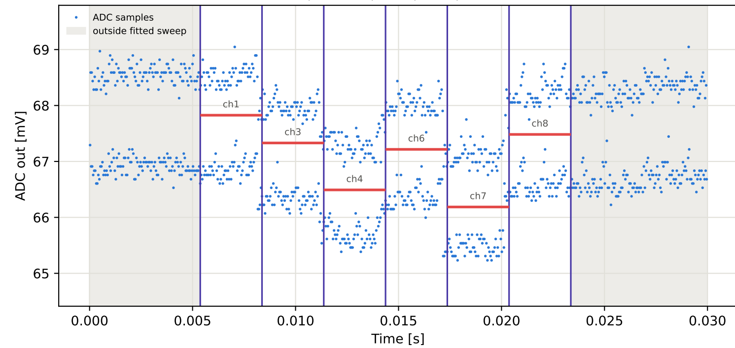
Tag1 &lt;- Tag4 | 795 MHz | run 0 | rep 1 | phase 100.53 deg
