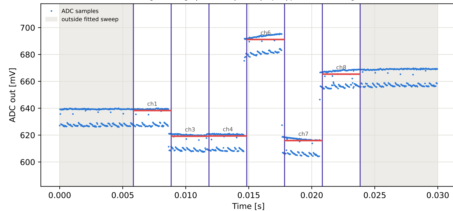
Tag16 &lt;- Tag6 | 955 MHz | run 0 | rep 1 | phase -76.36 deg
