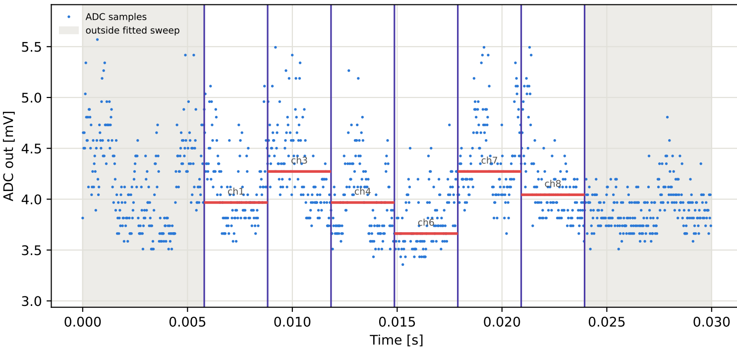
Tag2 &lt;- Tag15 | 775 MHz | run 0 | rep 1 | phase -161.25 deg
