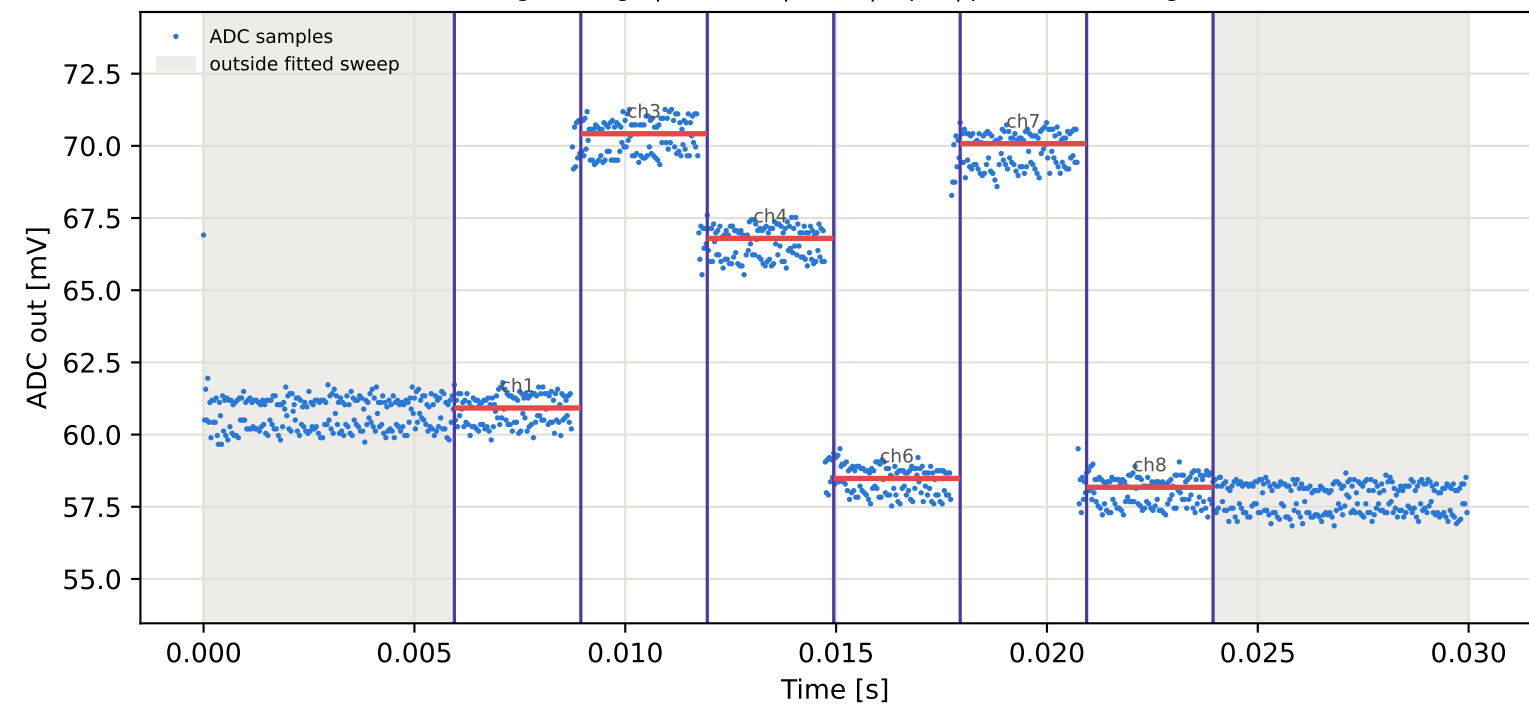
Tag1 &lt;- Tag8 | 795 MHz | run 0 | rep 1 | phase -81.28 deg
