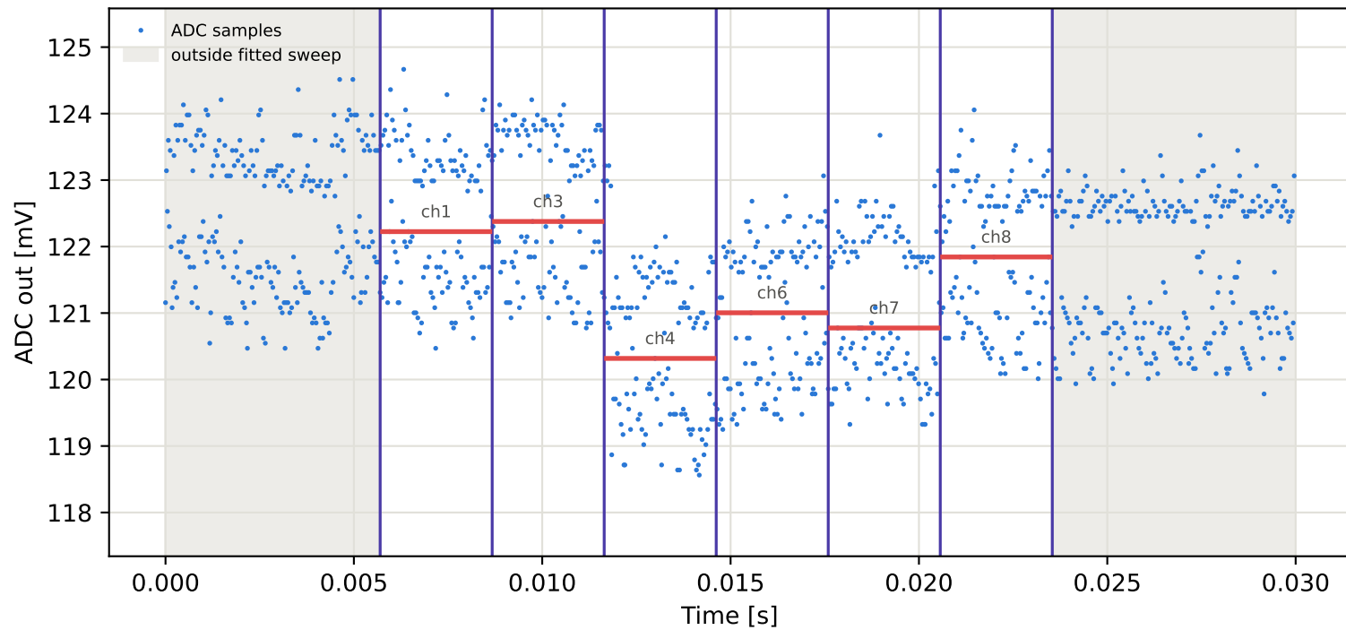
Tag7 &lt;- Tag15 | 775 MHz | run 0 | rep 1 | phase -106.78 deg
