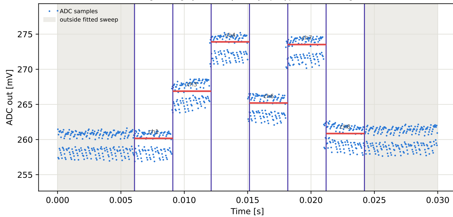
Tag1 &lt;- Tag7 | 825 MHz | run 0 | rep 1 | phase -84.62 deg
