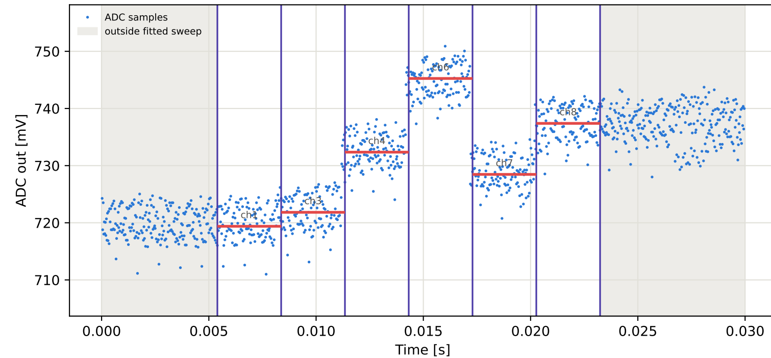
Tag9 &lt;- Tag7 | 885 MHz | run 0 | rep 1 | phase -73.84 deg
