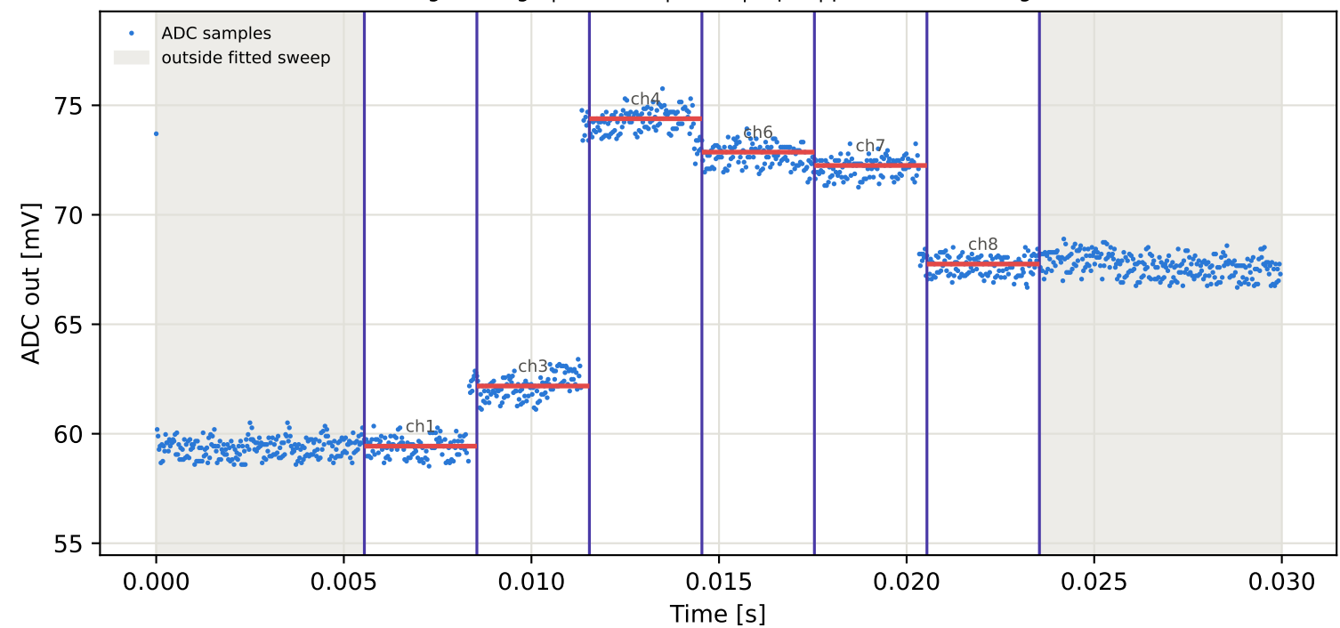
Tag2 &lt;- Tag8 | 825 MHz | run 0 | rep 1 | phase -116.58 deg
