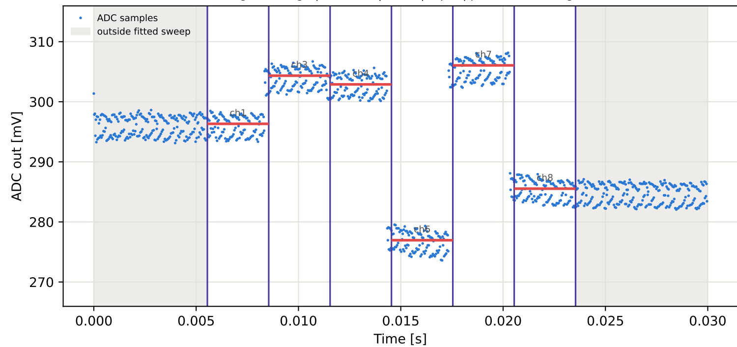
Tag10 &lt;- Tag8 | 975 MHz | run 0 | rep 1 | phase -56.99 deg
