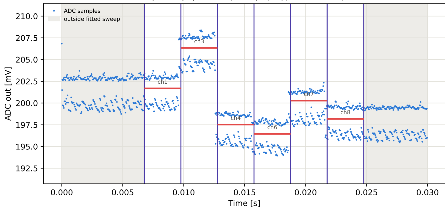
Tag7 &lt;- Tag6 | 805 MHz | run 0 | rep 1 | phase -97.05 deg
