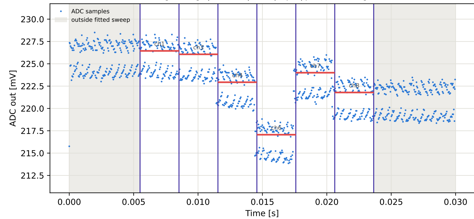
Tag3 &lt;- Tag10 | 905 MHz | run 0 | rep 1 | phase -58.12 deg
