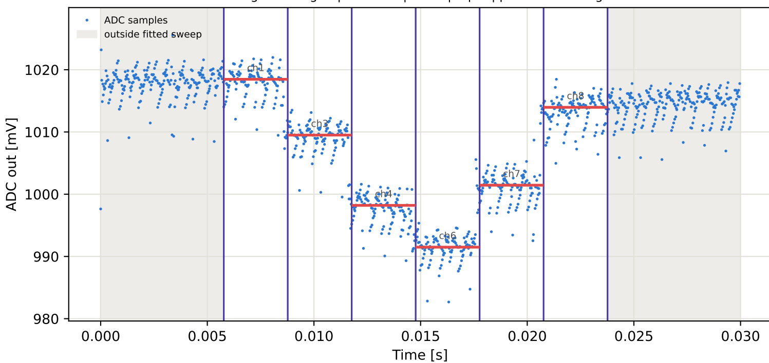
Tag15 &lt;- Tag10 | 905 MHz | run 0 | rep 1 | phase 54.36 deg
