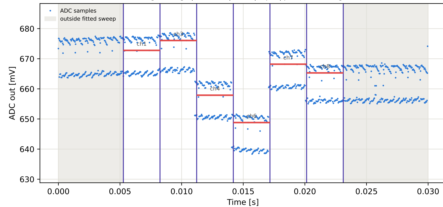
Tag8 &lt;- Tag1 | 965 MHz | run 0 | rep 1 | phase -87.85 deg
