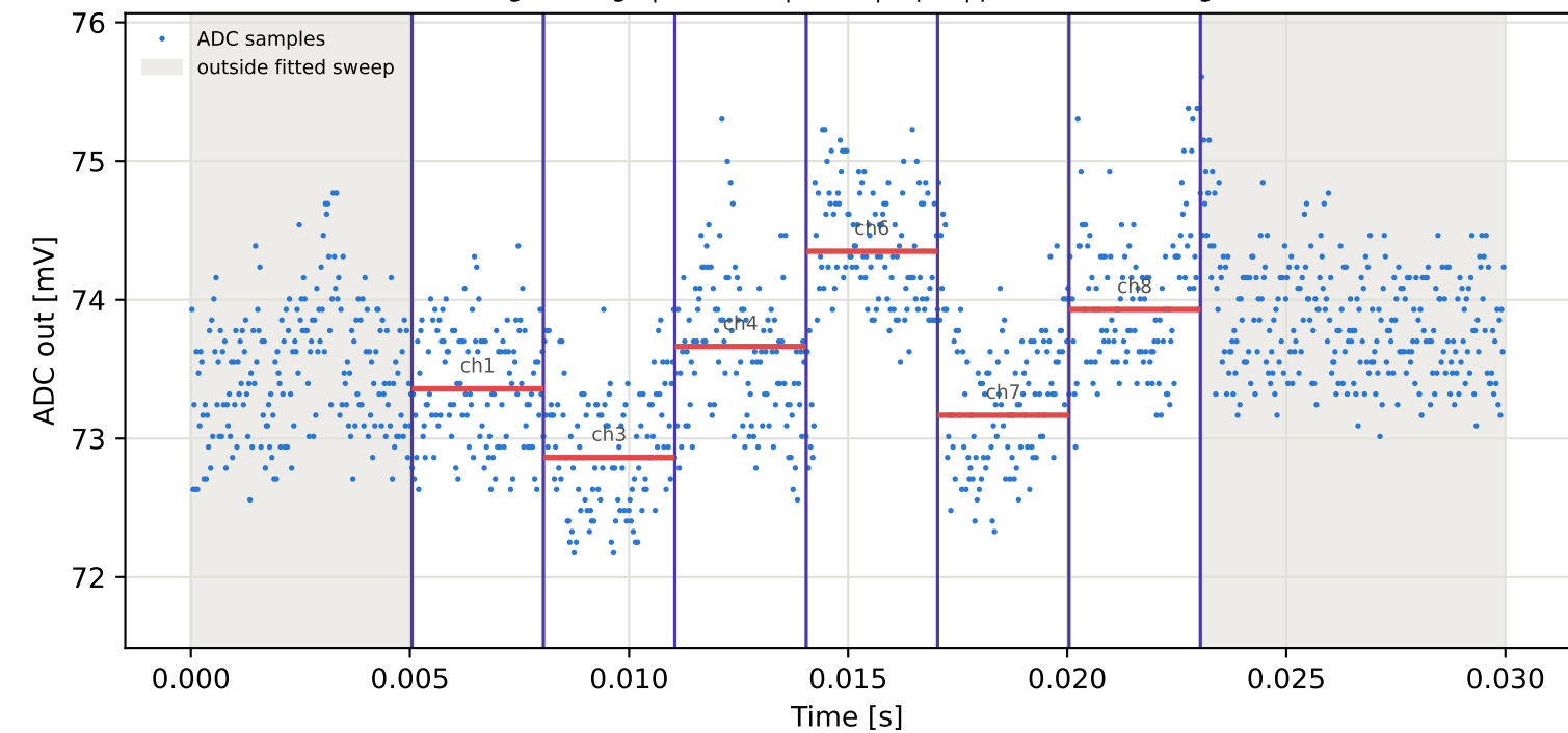
Tag2 &lt;- Tag7 | 825 MHz | run 0 | rep 1 | phase -157.96 deg
