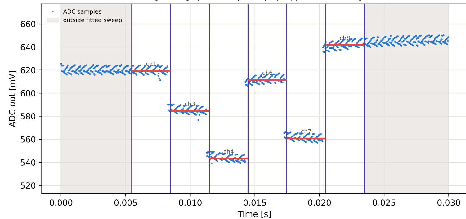
Tag5 &lt;- Tag4 | 925 MHz | run 0 | rep 1 | phase 103.56 deg
