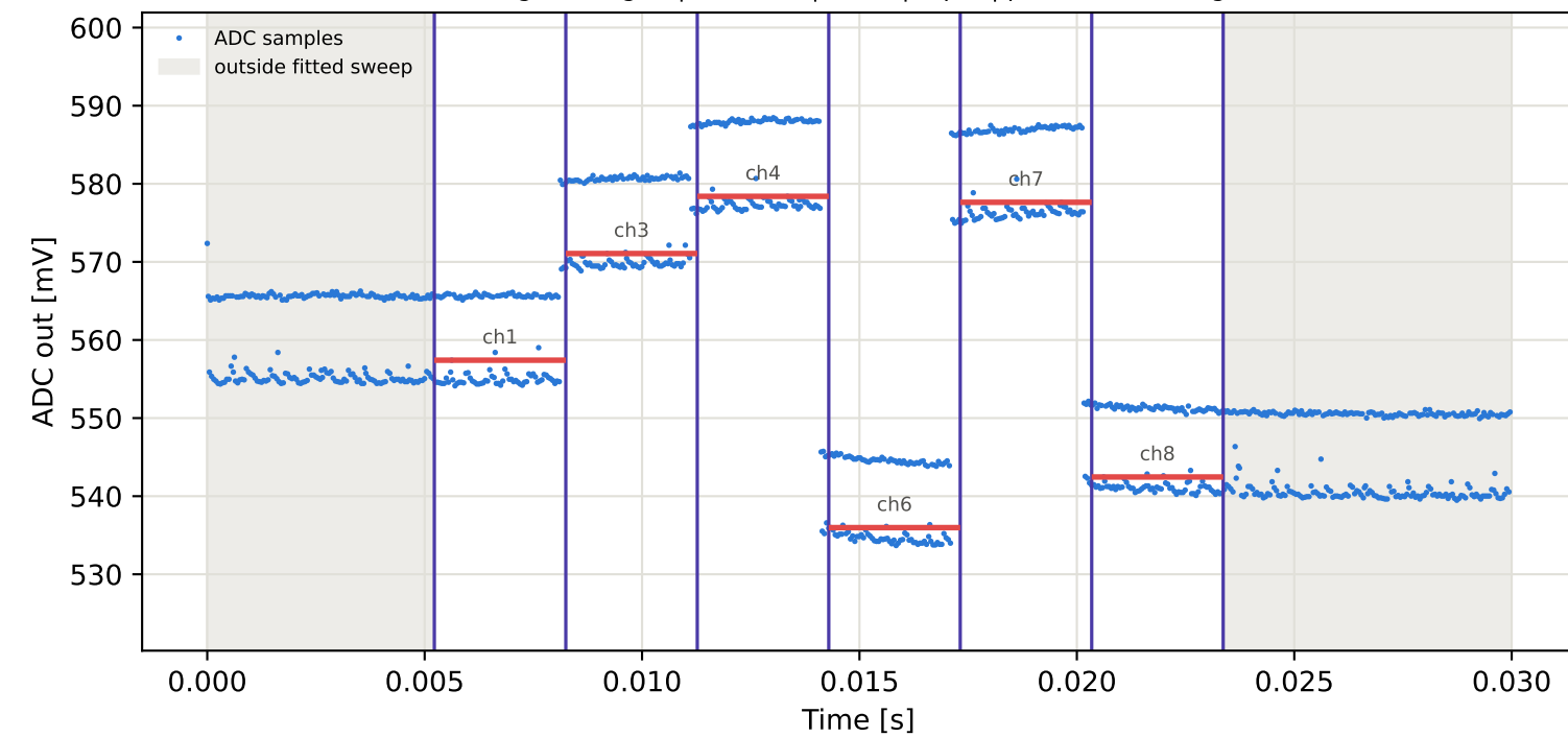
Tag7 &lt;- Tag3 | 985 MHz | run 0 | rep 1 | phase 138.60 deg
