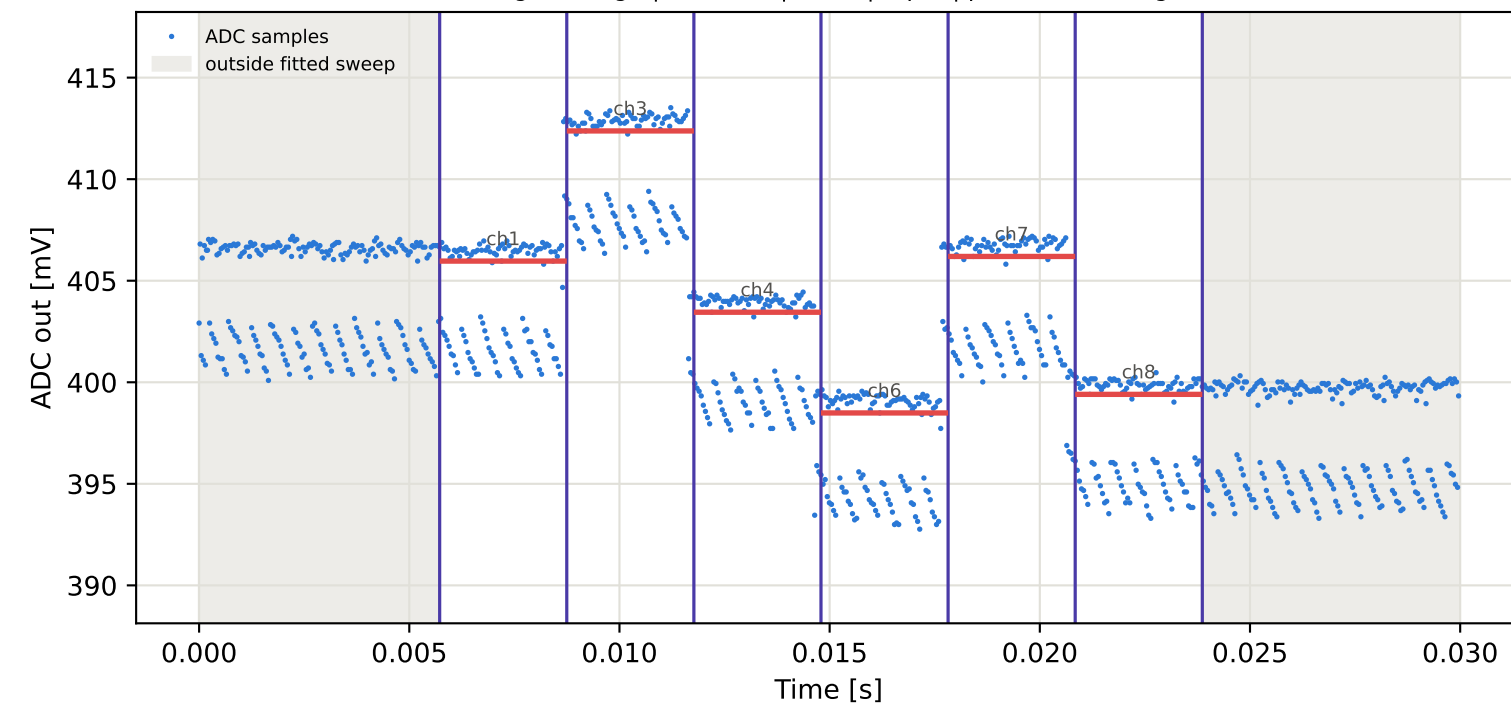
Tag9 &lt;- Tag5 | 835 MHz | run 0 | rep 1 | phase -145.79 deg
