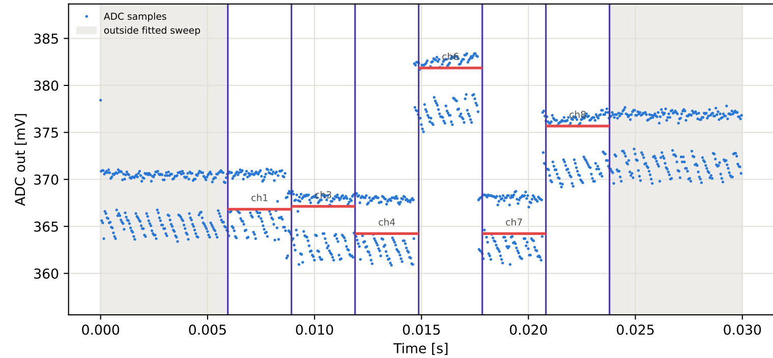
Tag9 &lt;- Tag2 | 925 MHz | run 0 | rep 1 | phase 166.48 deg
