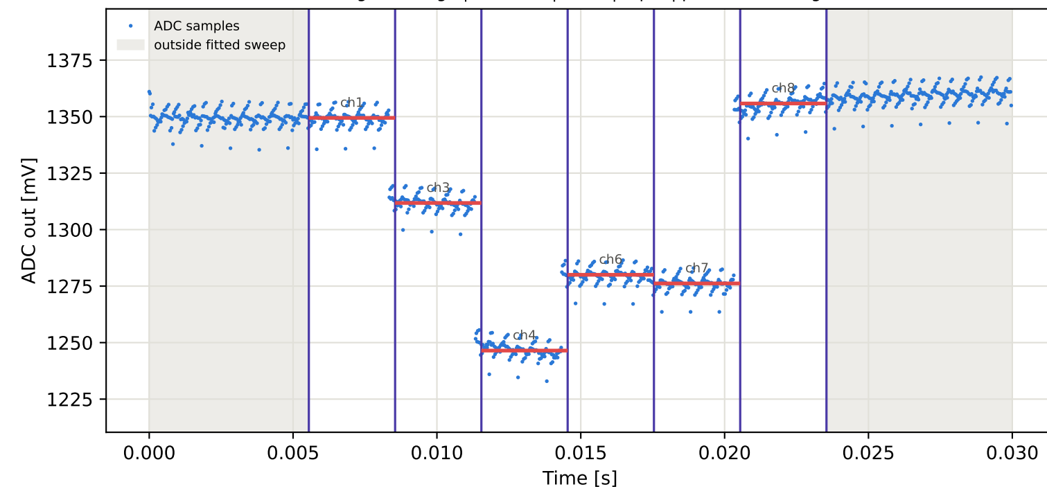
Tag15 &lt;- Tag5 | 935 MHz | run 0 | rep 1 | phase 69.46 deg
