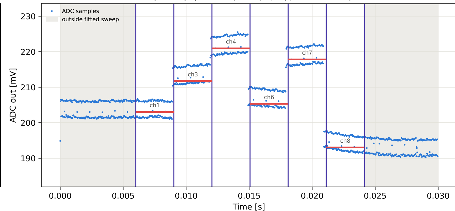
Tag10 &lt;- Tag1 | 915 MHz | run 0 | rep 1 | phase 101.15 deg
