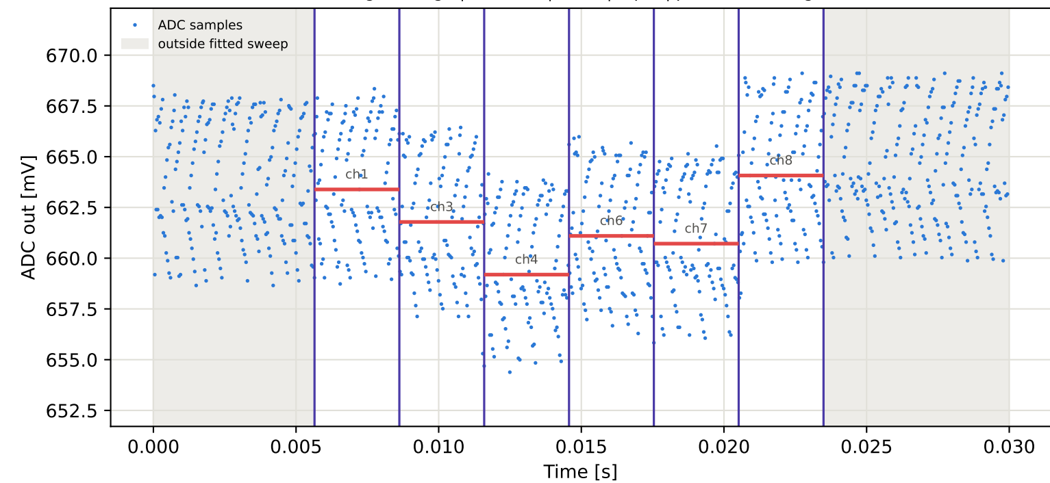
Tag8 &lt;- Tag4 | 945 MHz | run 0 | rep 1 | phase -177.13 deg
