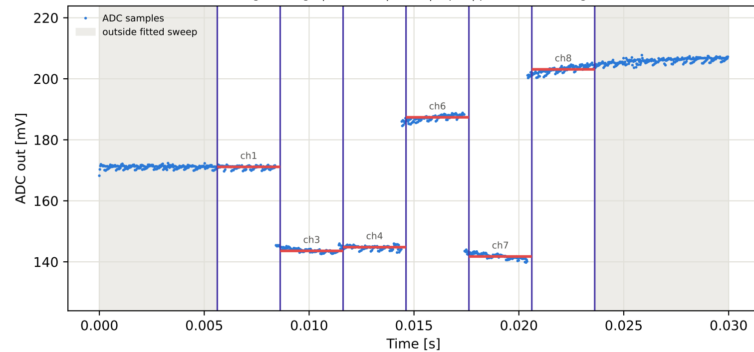
Tag9 &lt;- Tag5 | 875 MHz | run 0 | rep 1 | phase -82.30 deg
