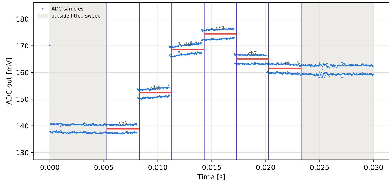
Tag9 &lt;- Tag2 | 875 MHz | run 0 | rep 1 | phase -15.96 deg
