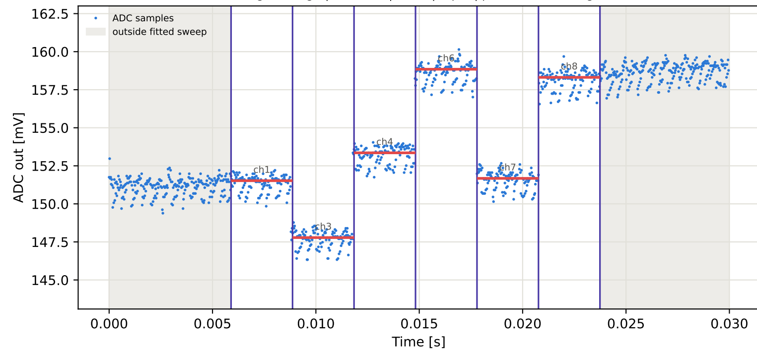
Tag7 &lt;- Tag1 | 845 MHz | run 0 | rep 1 | phase -120.41 deg
