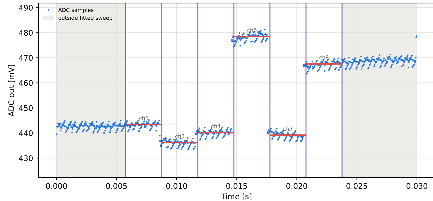
Tag10 &lt;- Tag5 | 915 MHz | run 0 | rep 1 | phase 175.21 deg
