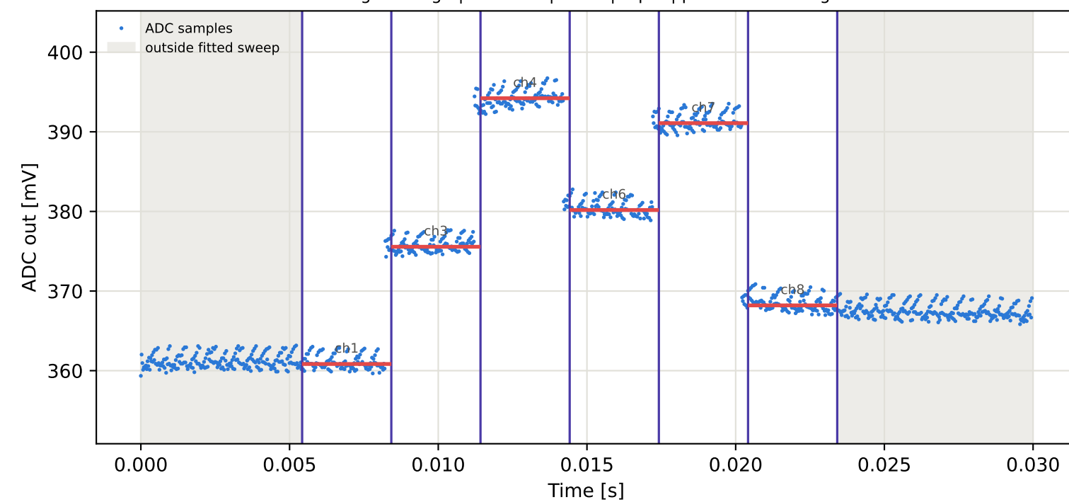
Tag7 &lt;- Tag10 | 855 MHz | run 0 | rep 1 | phase 58.87 deg
