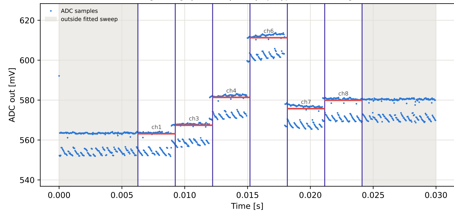
Tag7 &lt;- Tag1 | 915 MHz | run 0 | rep 1 | phase 126.54 deg
