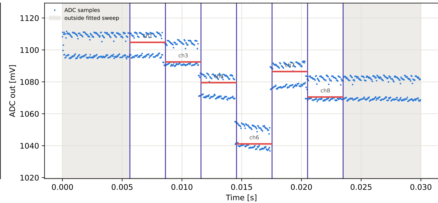
Tag4 &lt;- Tag3 | 895 MHz | run 0 | rep 1 | phase 24.21 deg
