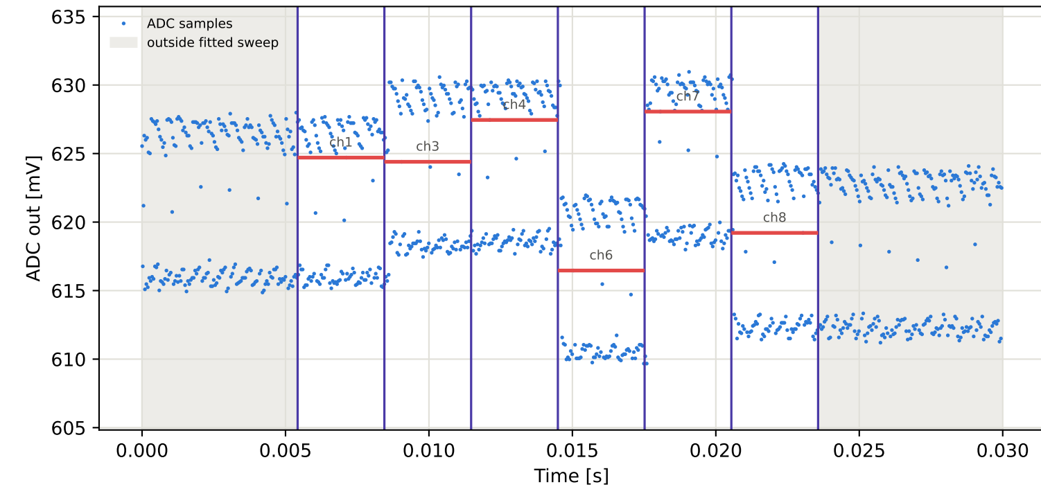
Tag16 &lt;- Tag15 | 955 MHz | run 0 | rep 1 | phase 16.68 deg
