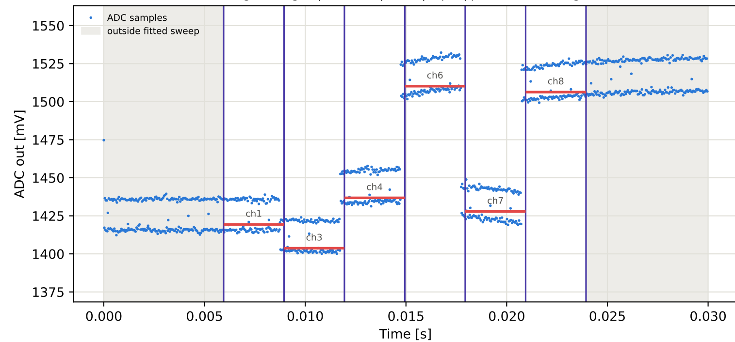
Tag5 &lt;- Tag2 | 885 MHz | run 0 | rep 1 | phase 6.54 deg
