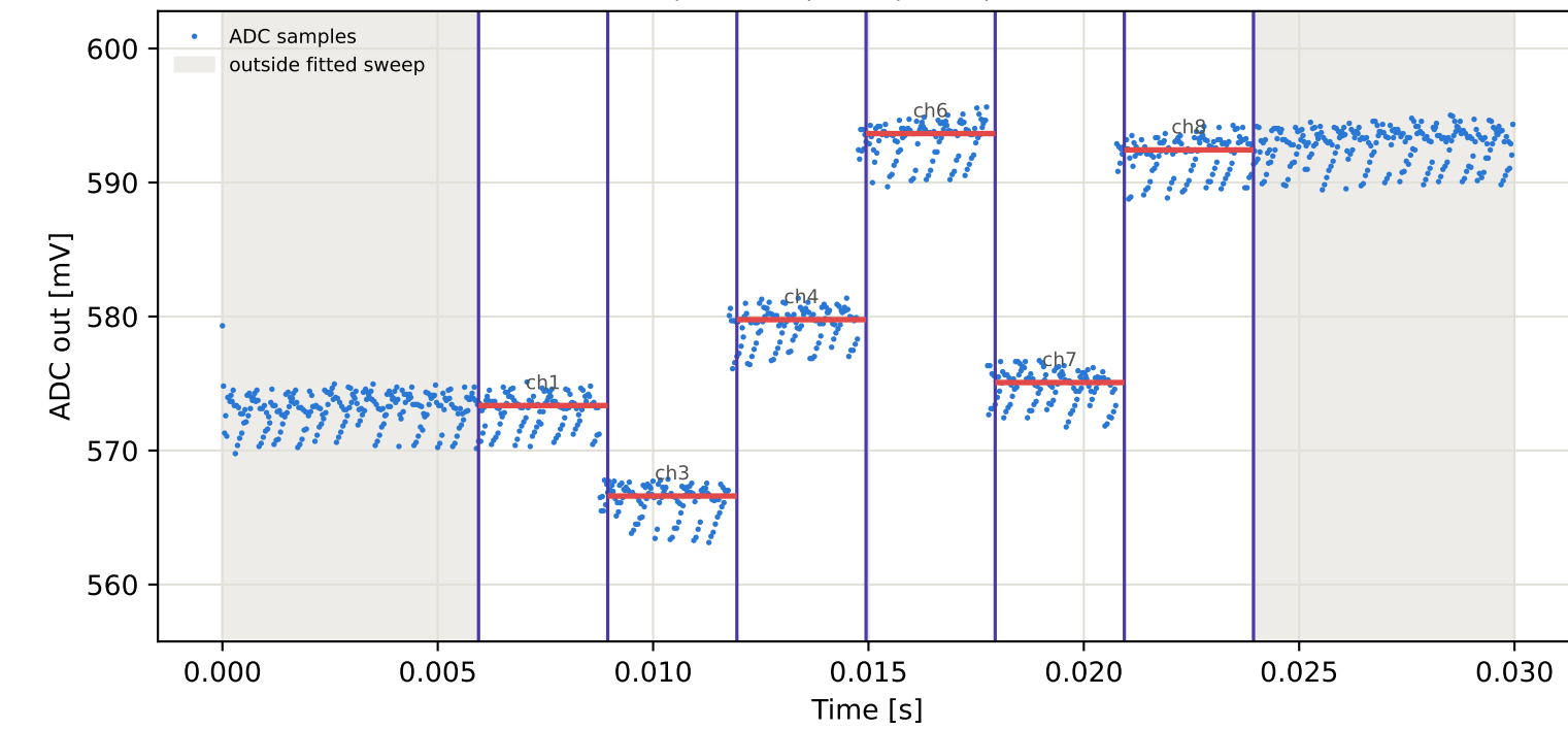
Tag6 &lt;- Tag1 | 865 MHz | run 0 | rep 1 | phase -164.75 deg
