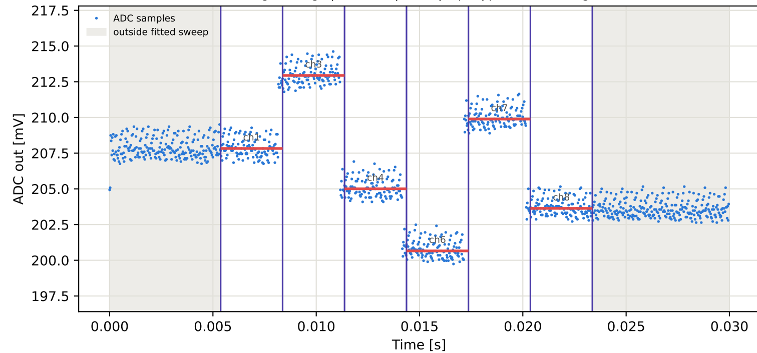
Tag3 &lt;- Tag15 | 805 MHz | run 0 | rep 1 | phase -71.78 deg
