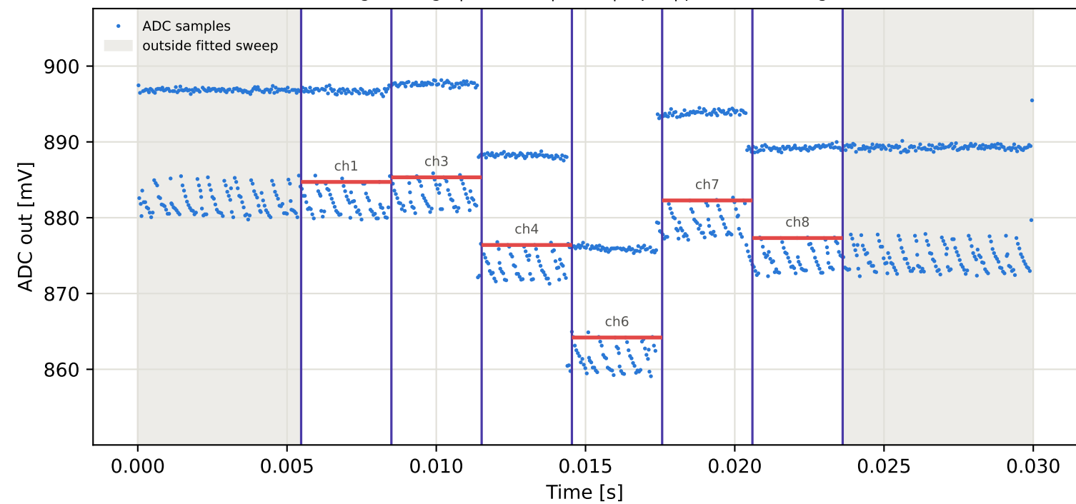
Tag4 &lt;- Tag8 | 945 MHz | run 0 | rep 1 | phase 2.76 deg
