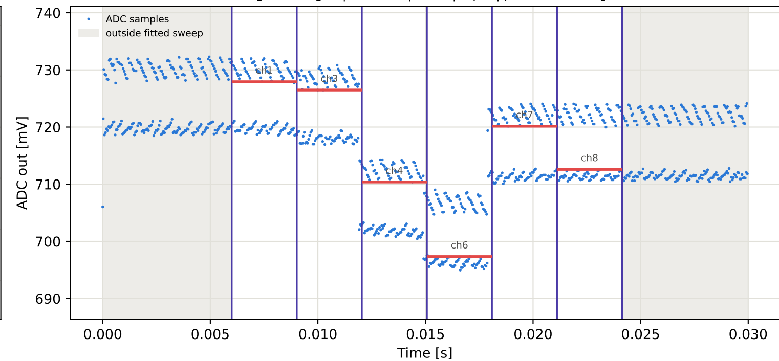
Tag16 &lt;- Tag15 | 975 MHz | run 0 | rep 1 | phase 26.99 deg
