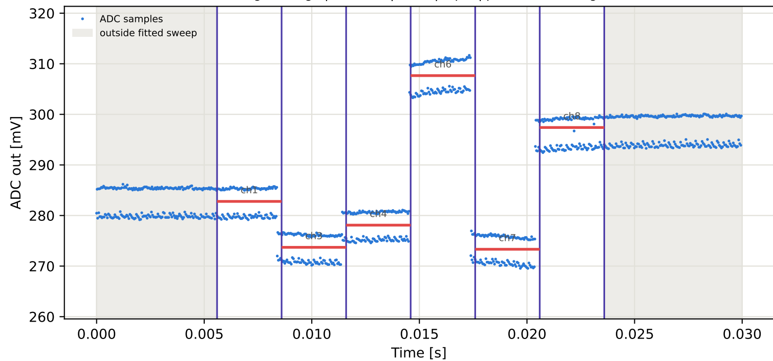
Tag3 &lt;- Tag9 | 965 MHz | run 0 | rep 1 | phase 20.71 deg
