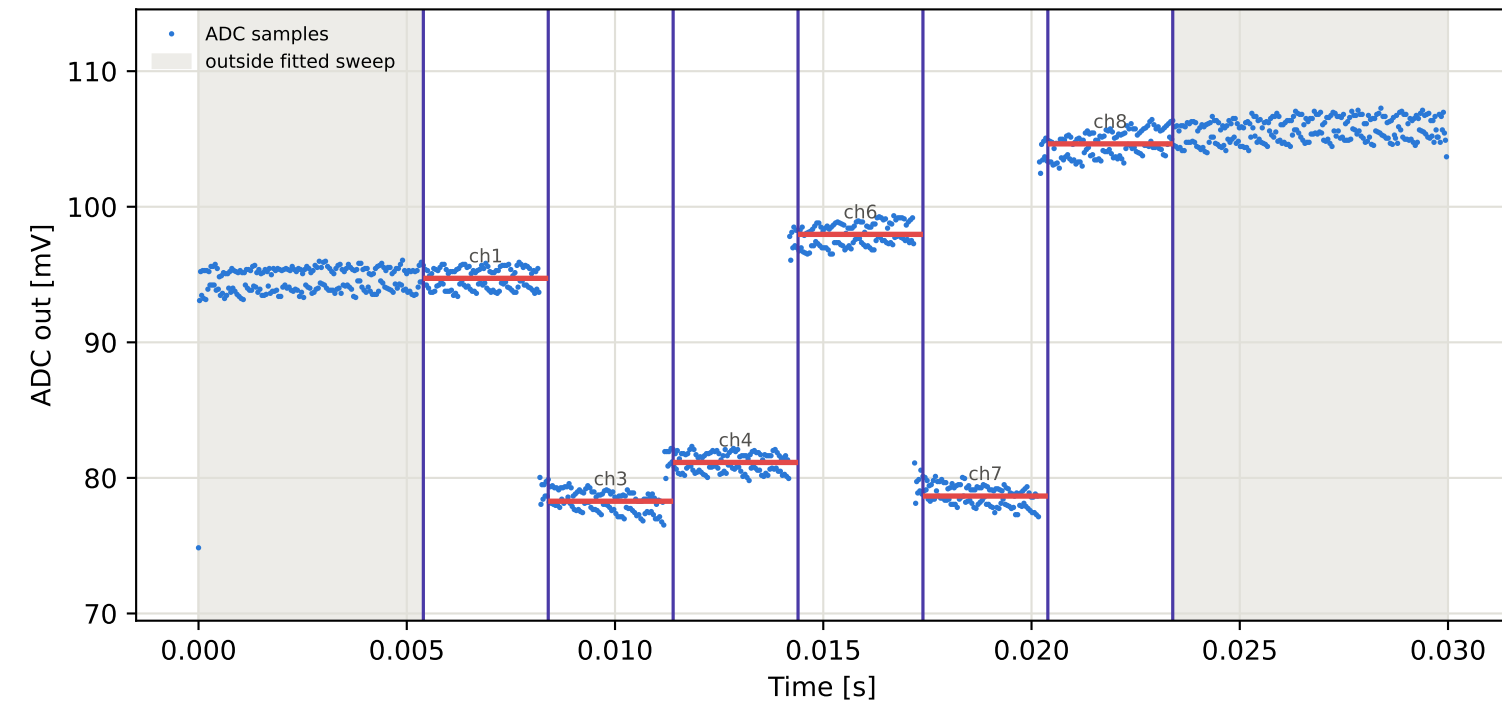
Tag15 &lt;- Tag1 | 865 MHz | run 0 | rep 1 | phase -26.85 deg
