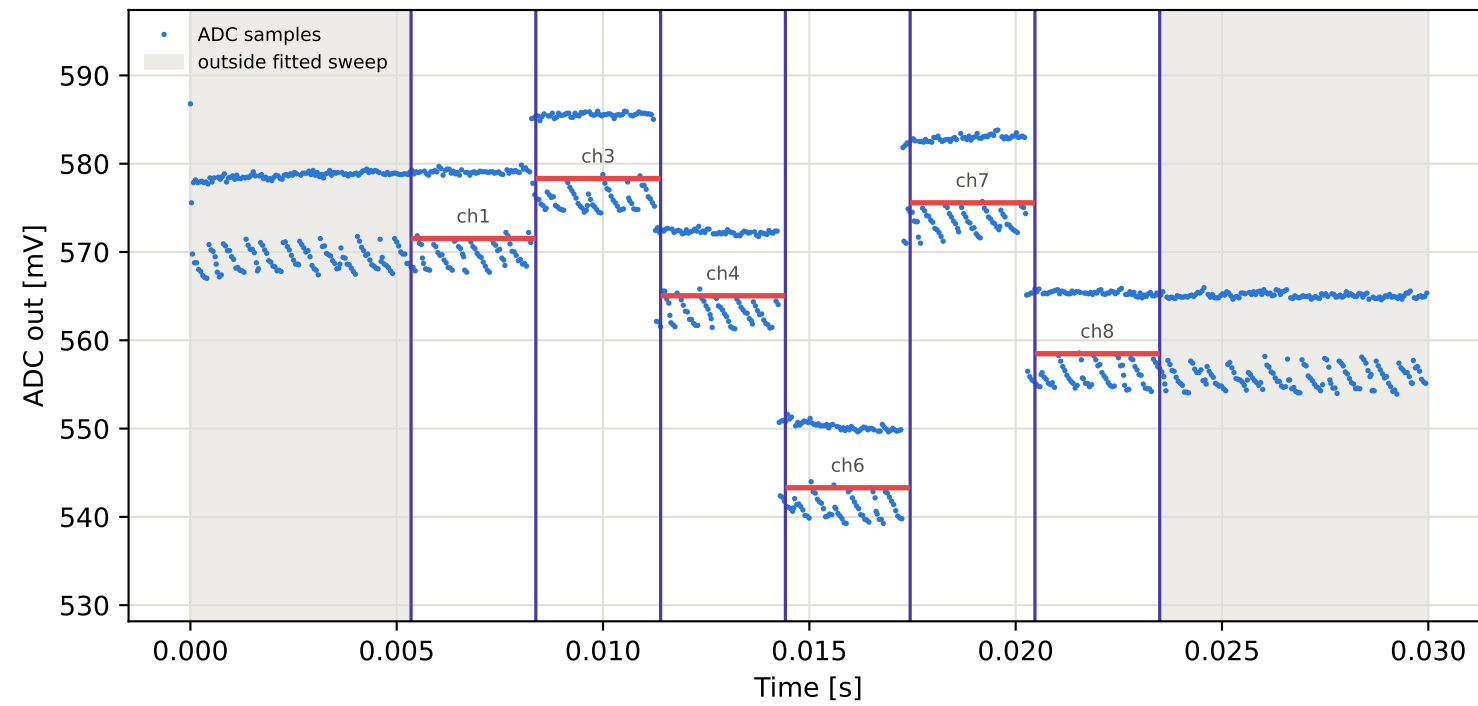
Tag8 &lt;- Tag1 | 985 MHz | run 0 | rep 1 | phase 46.72 deg
