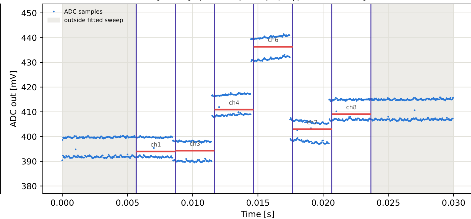
Tag7 &lt;- Tag6 | 945 MHz | run 0 | rep 1 | phase -156.33 deg
