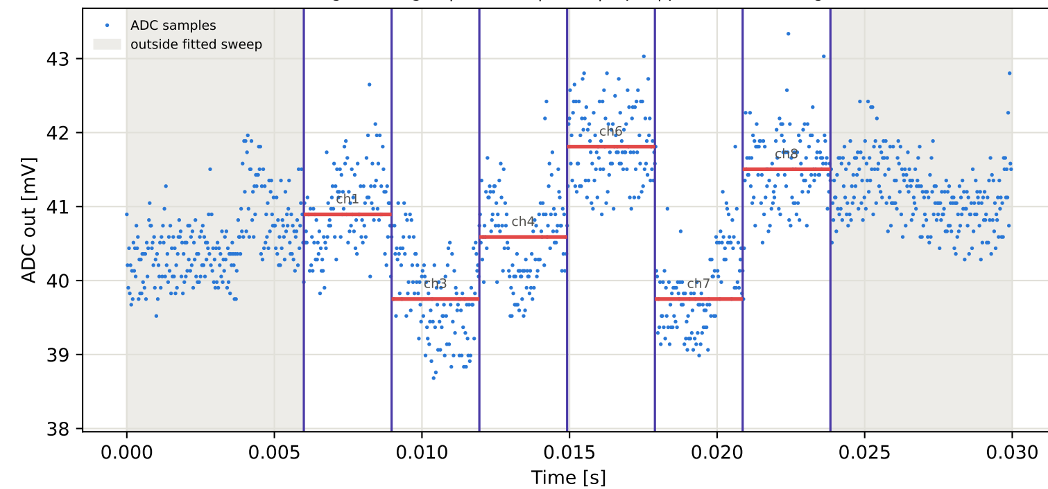
Tag10 &lt;- Tag2 | 805 MHz | run 0 | rep 1 | phase 174.48 deg
