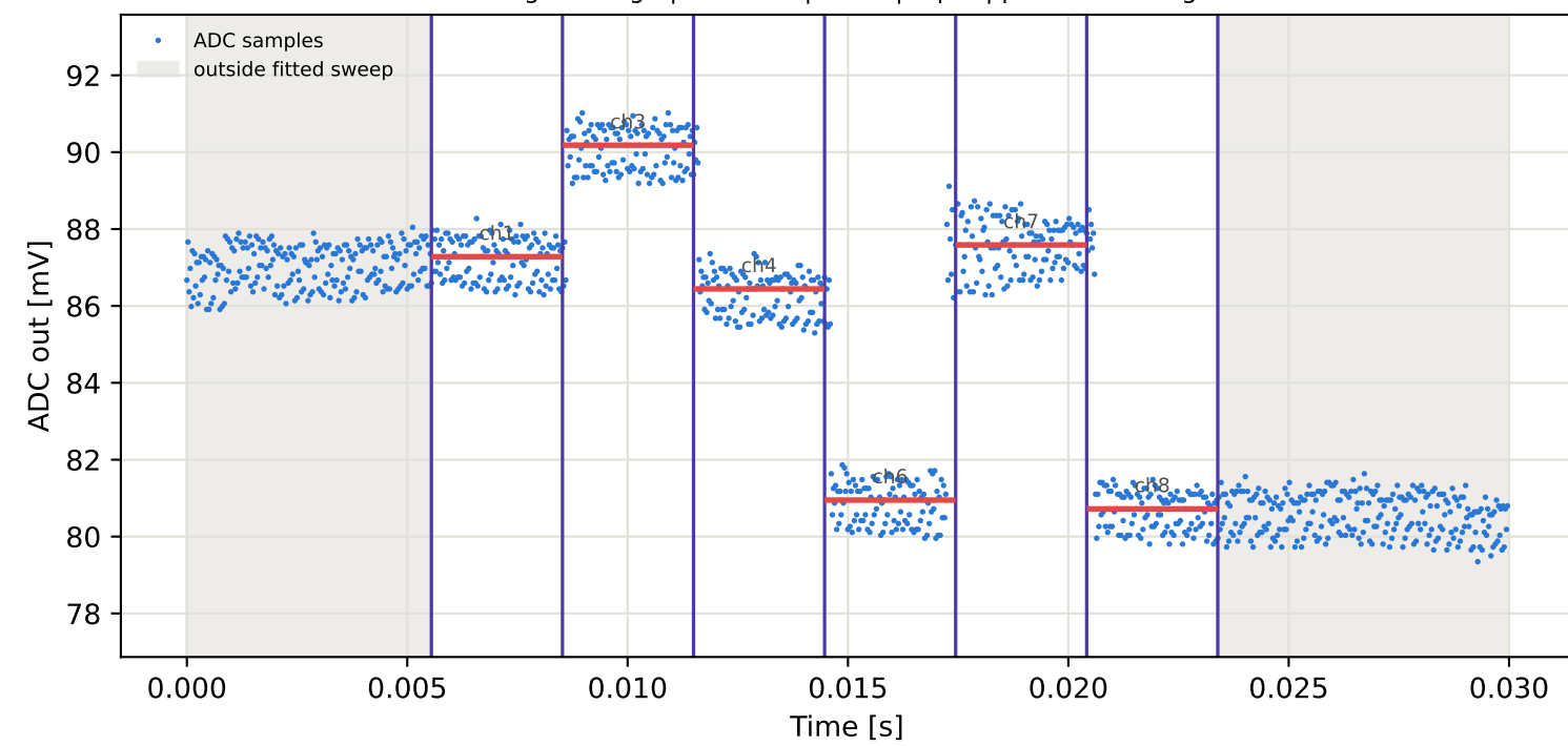
Tag1 &lt;- Tag8 | 845 MHz | run 0 | rep 1 | phase -160.96 deg
