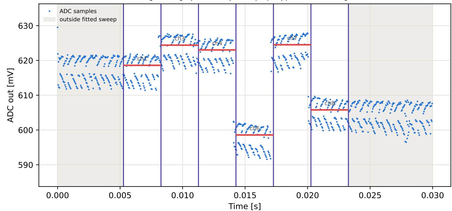
Tag8 &lt;- Tag7 | 925 MHz | run 0 | rep 1 | phase -10.37 deg
