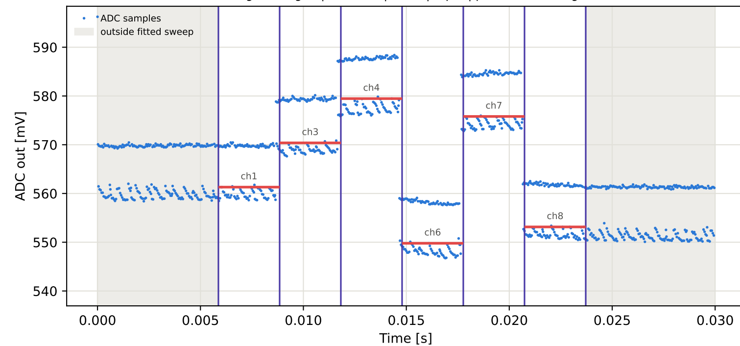
Tag7 &lt;- Tag10 | 985 MHz | run 0 | rep 1 | phase -49.16 deg
