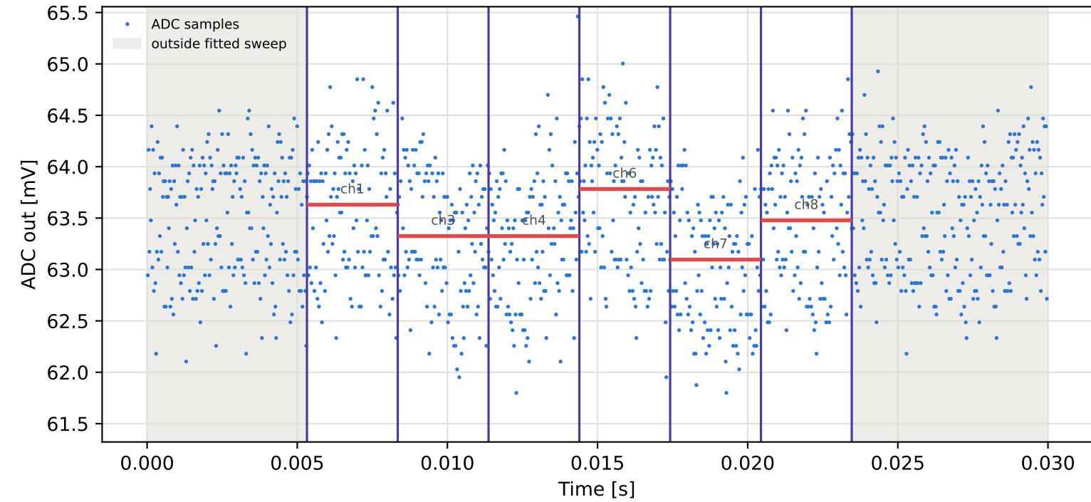
Tag2 &lt;- Tag8 | 995 MHz | run 0 | rep 1 | phase 58.71 deg
