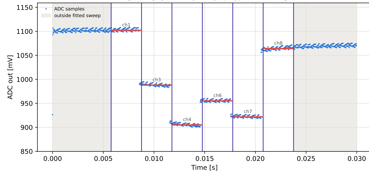
Tag4 &lt;- Tag7 | 875 MHz | run 0 | rep 1 | phase 133.41 deg
