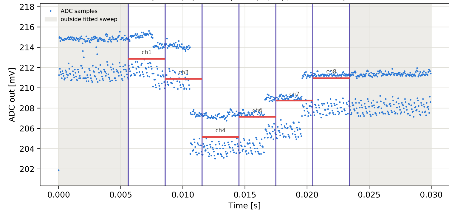
Tag3 &lt;- Tag9 | 805 MHz | run 0 | rep 1 | phase -92.52 deg
