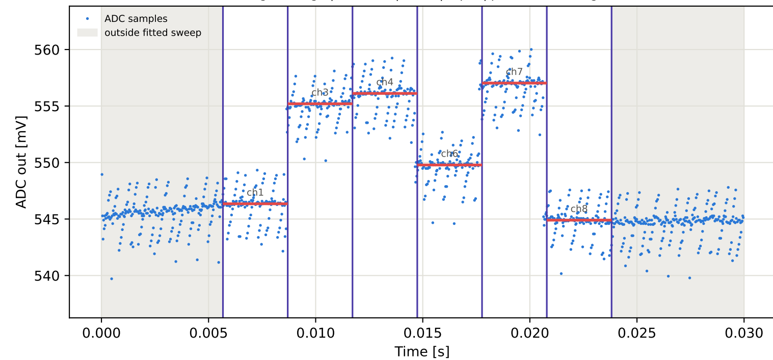
Tag5 &lt;- Tag8 | 845 MHz | run 0 | rep 1 | phase 87.38 deg
