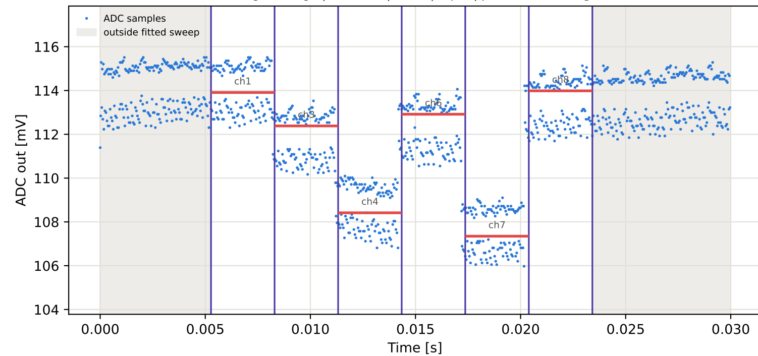
Tag3 &lt;- Tag6 | 795 MHz | run 0 | rep 1 | phase -36.02 deg
