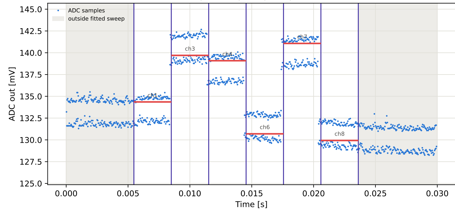
Tag10 &lt;- Tag5 | 845 MHz | run 0 | rep 1 | phase -25.74 deg
