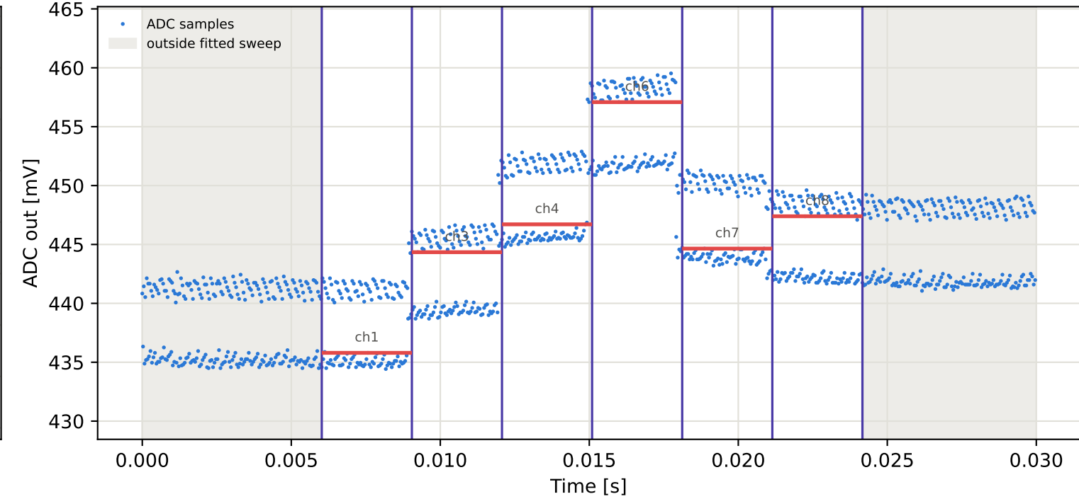
Tag10 &lt;- Tag1 | 895 MHz | run 0 | rep 1 | phase 73.67 deg
