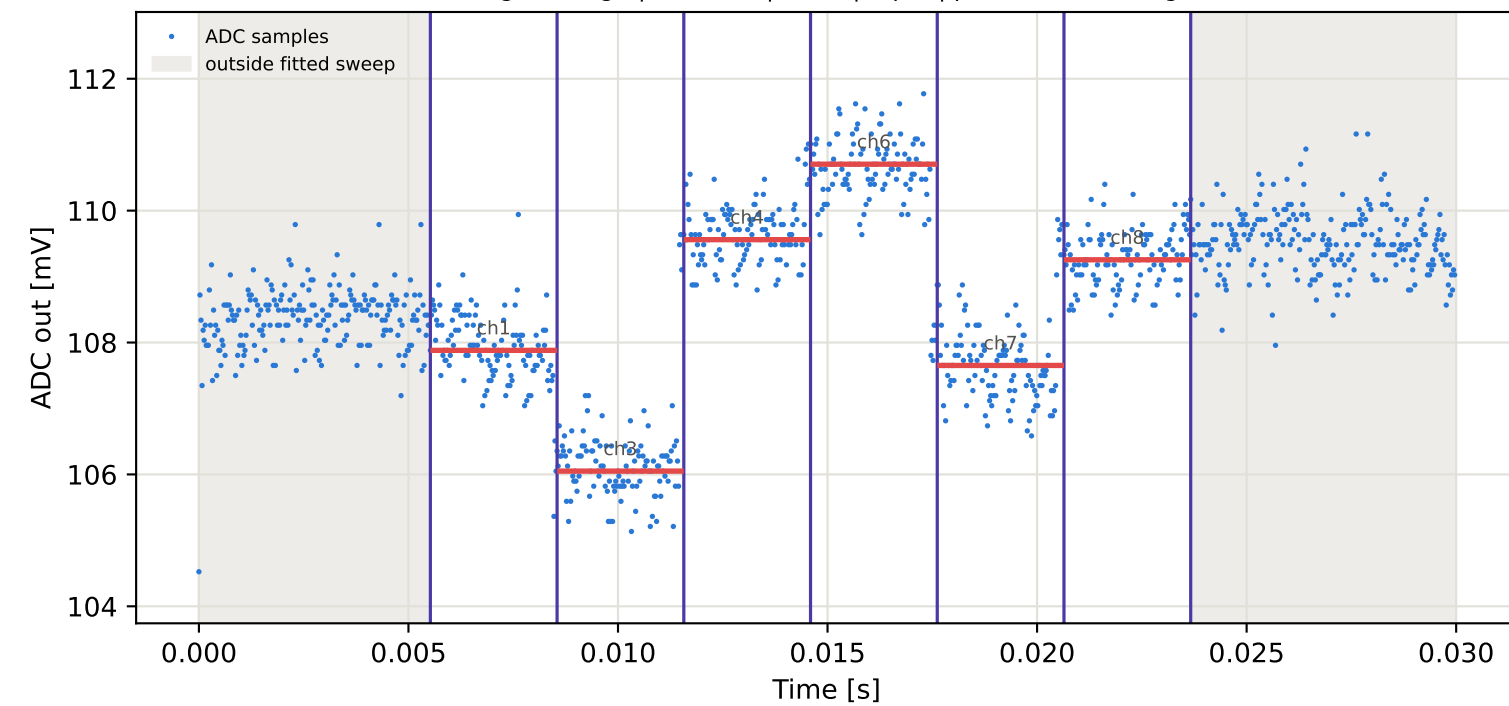
Tag8 &lt;- Tag1 | 785 MHz | run 0 | rep 1 | phase -20.57 deg
