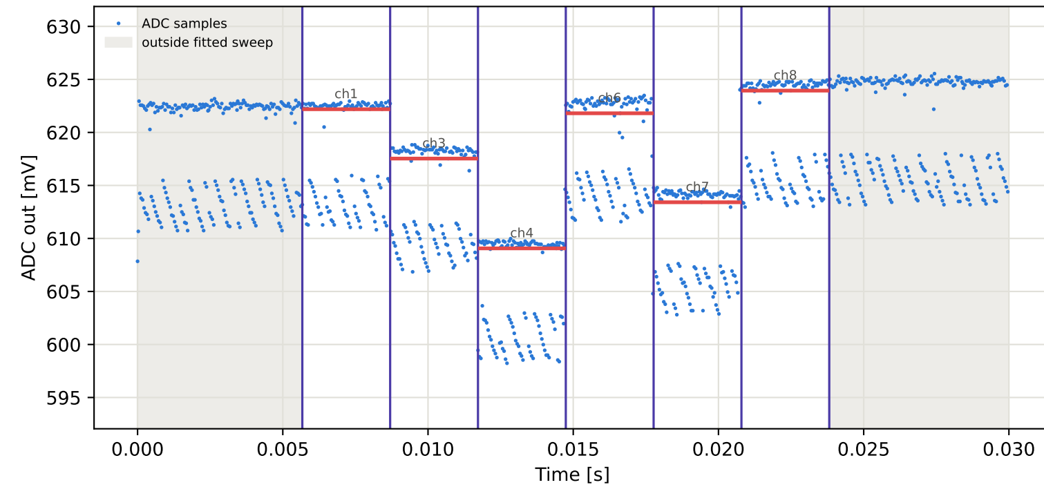
Tag15 &lt;- Tag5 | 985 MHz | run 0 | rep 1 | phase 126.45 deg
