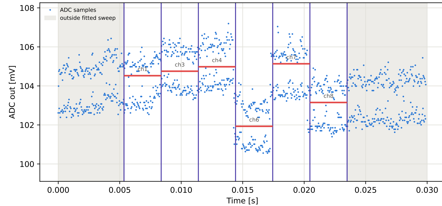
Tag10 &lt;- Tag4 | 995 MHz | run 0 | rep 1 | phase -43.63 deg
