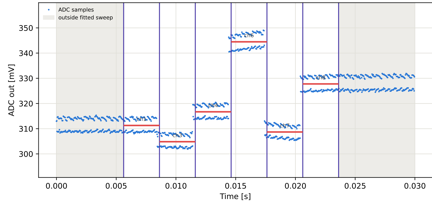
Tag6 &lt;- Tag10 | 965 MHz | run 0 | rep 1 | phase -5.09 deg
