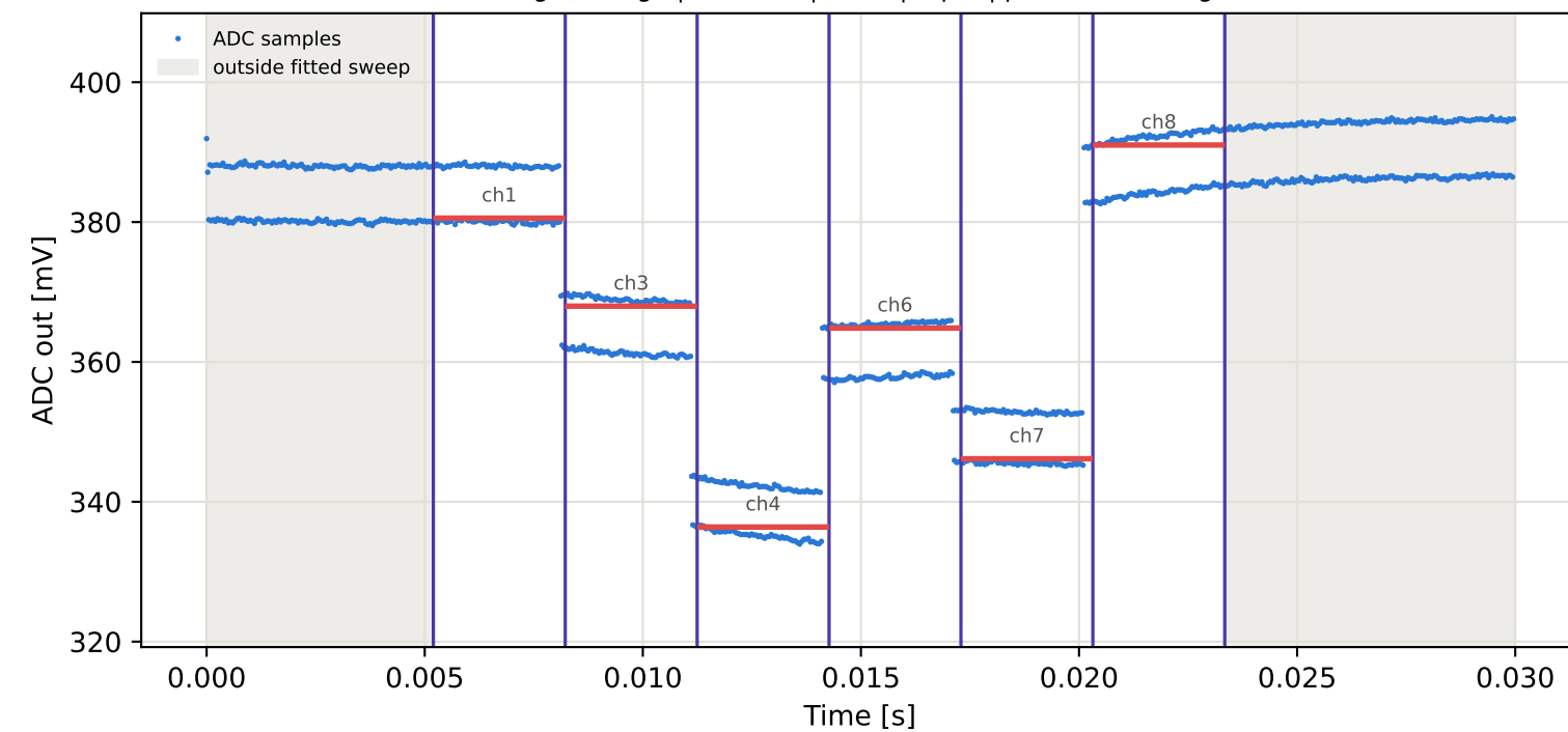
Tag9 &lt;- Tag7 | 925 MHz | run 0 | rep 1 | phase 83.96 deg
