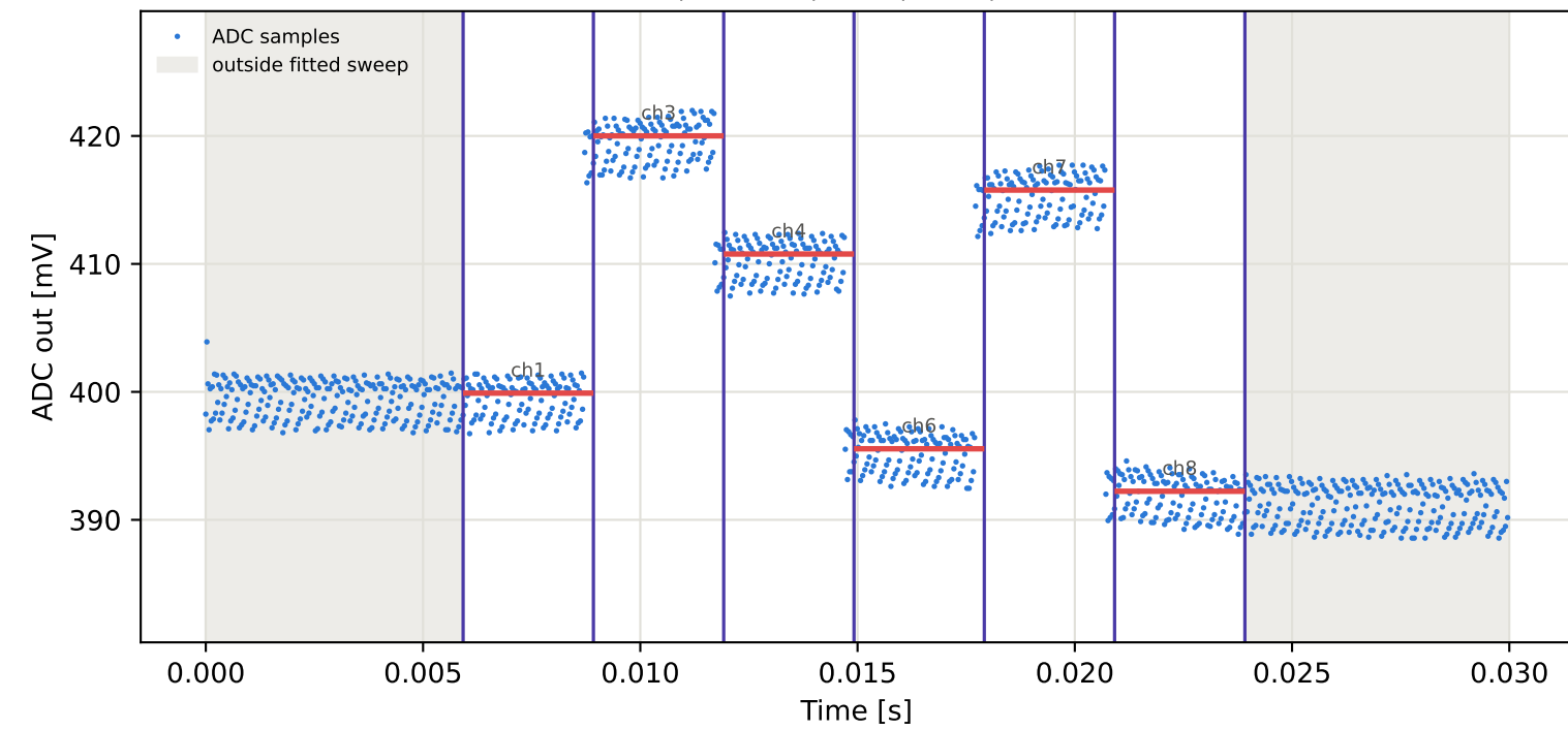
Tag3 &lt;- Tag16 | 845 MHz | run 0 | rep 1 | phase -19.18 deg
