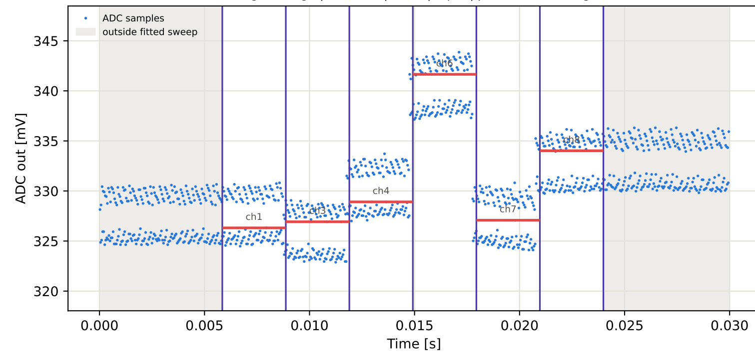
Tag1 &lt;- Tag7 | 965 MHz | run 0 | rep 1 | phase 86.48 deg
