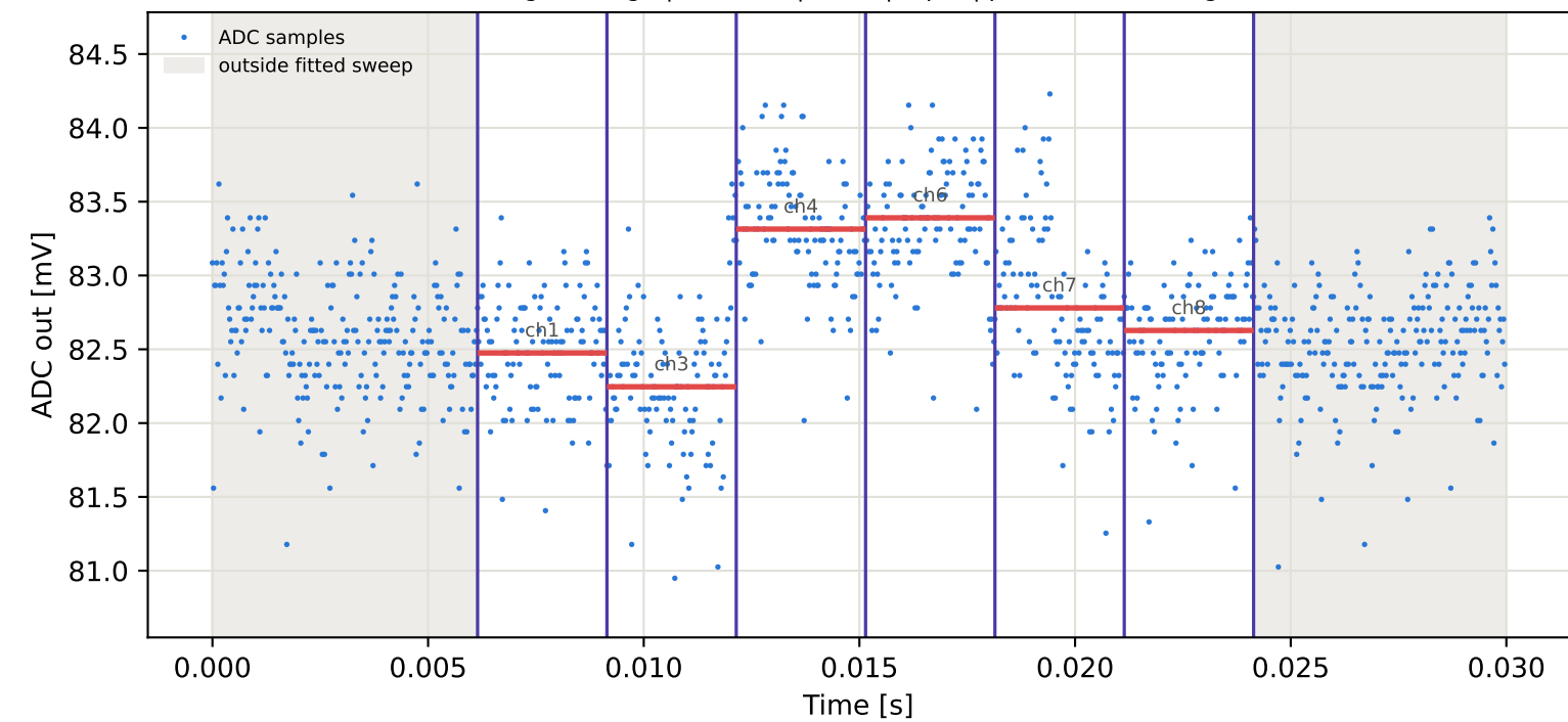
Tag4 &lt;- Tag15 | 785 MHz | run 0 | rep 1 | phase 170.72 deg
