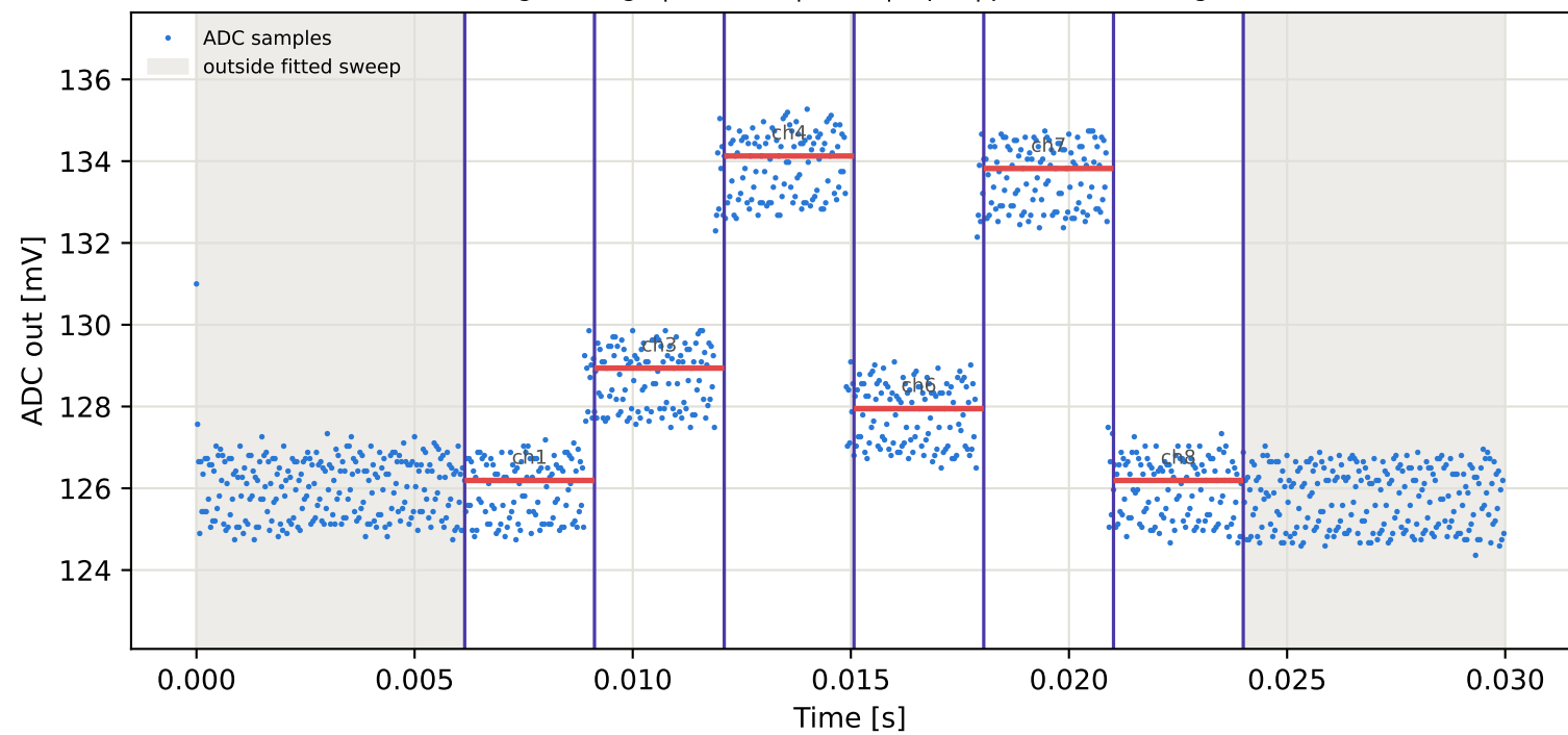
Tag3 &lt;- Tag15 | 785 MHz | run 0 | rep 1 | phase -98.05 deg
