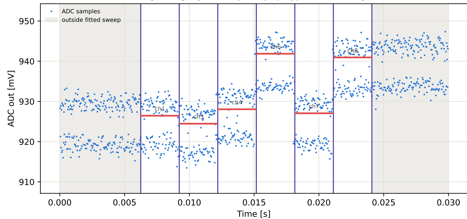
Tag4 &lt;- Tag16 | 885 MHz | run 0 | rep 1 | phase -149.82 deg
