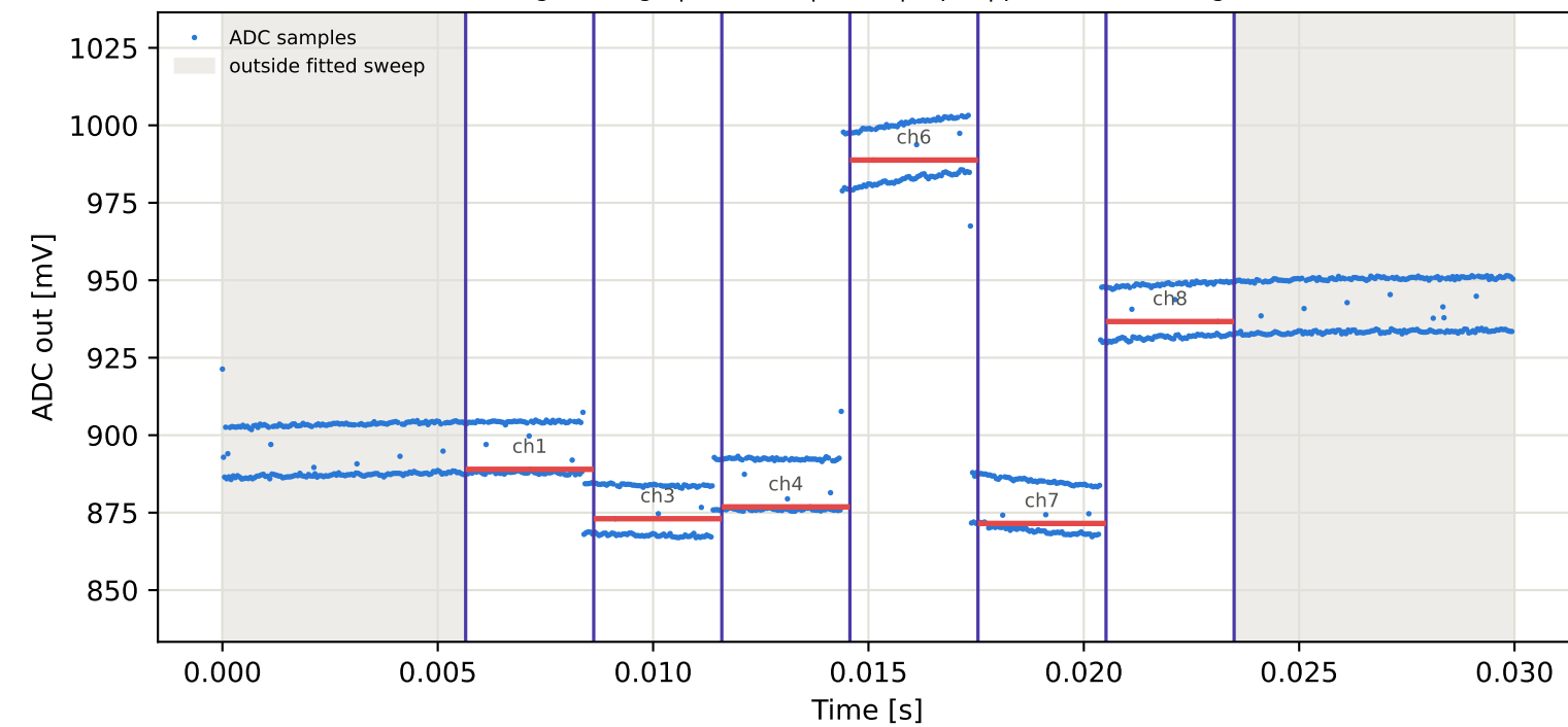
Tag4 &lt;- Tag7 | 945 MHz | run 0 | rep 1 | phase 156.01 deg
