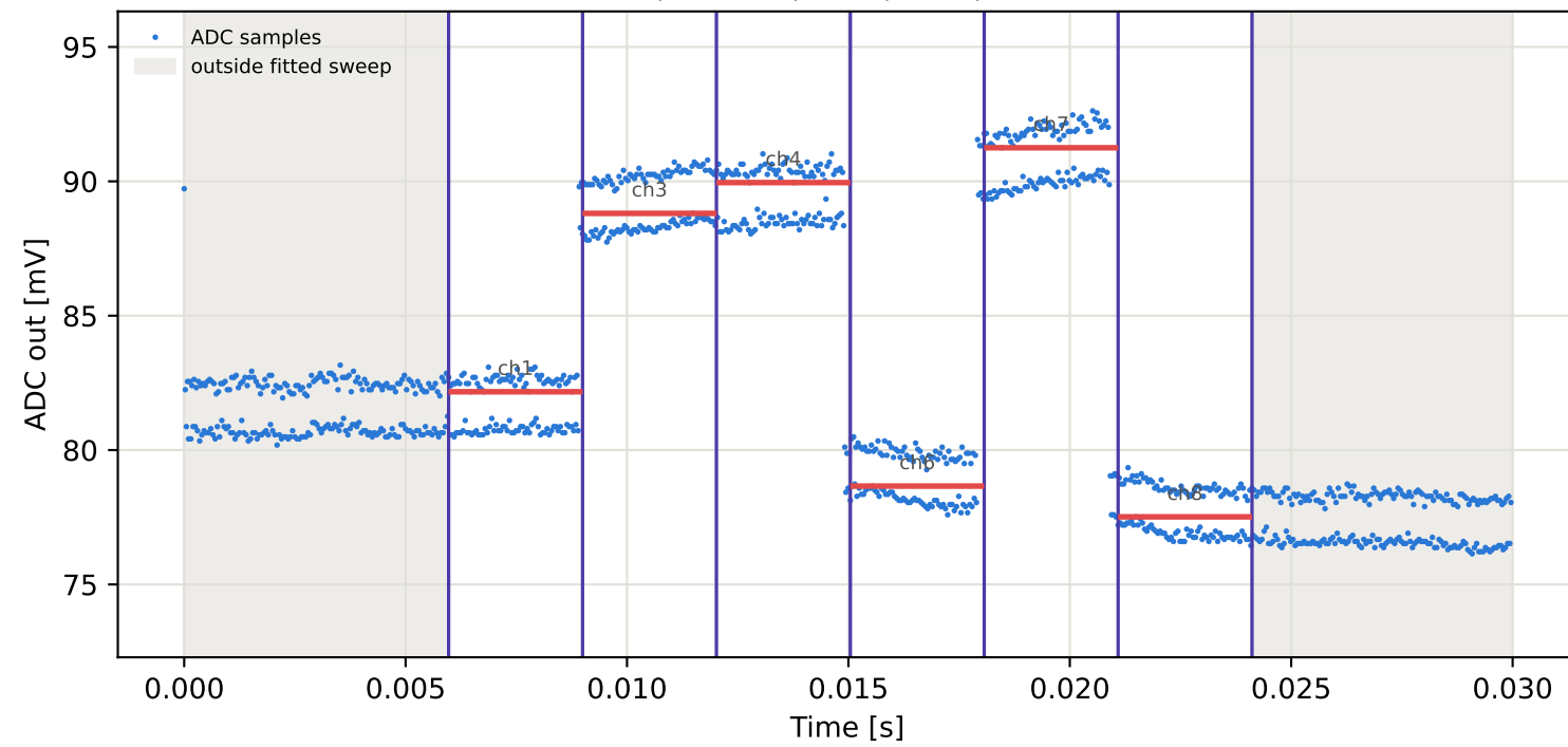
Tag1 &lt;- Tag9 | 845 MHz | run 0 | rep 1 | phase -34.45 deg
