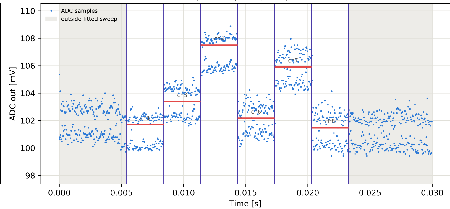
Tag10 &lt;- Tag3 | 995 MHz | run 0 | rep 1 | phase 119.05 deg
