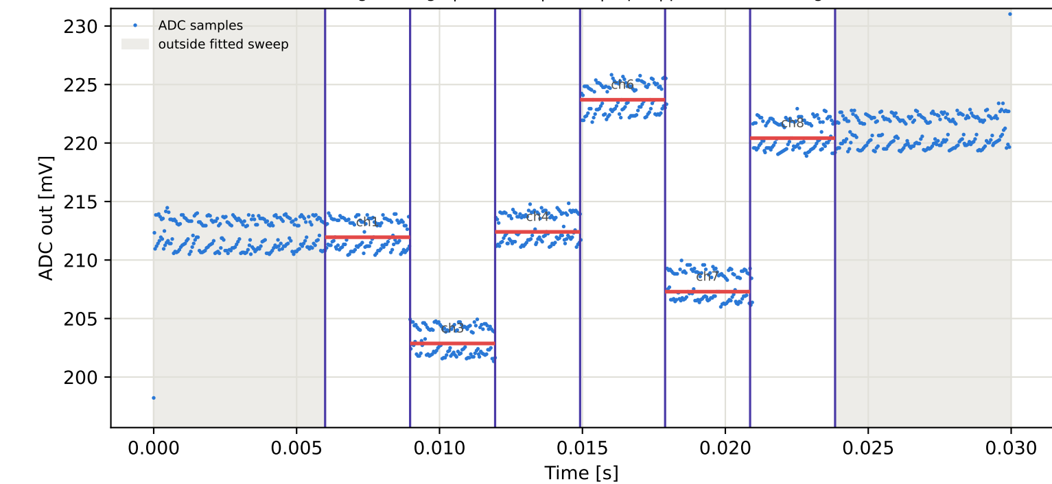
Tag9 &lt;- Tag7 | 825 MHz | run 0 | rep 1 | phase -76.55 deg
