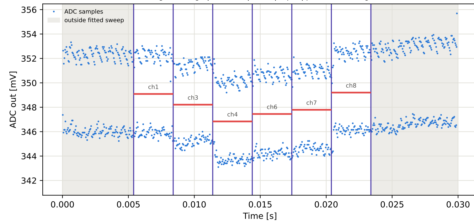
Tag10 &lt;- Tag4 | 925 MHz | run 0 | rep 1 | phase -52.80 deg
