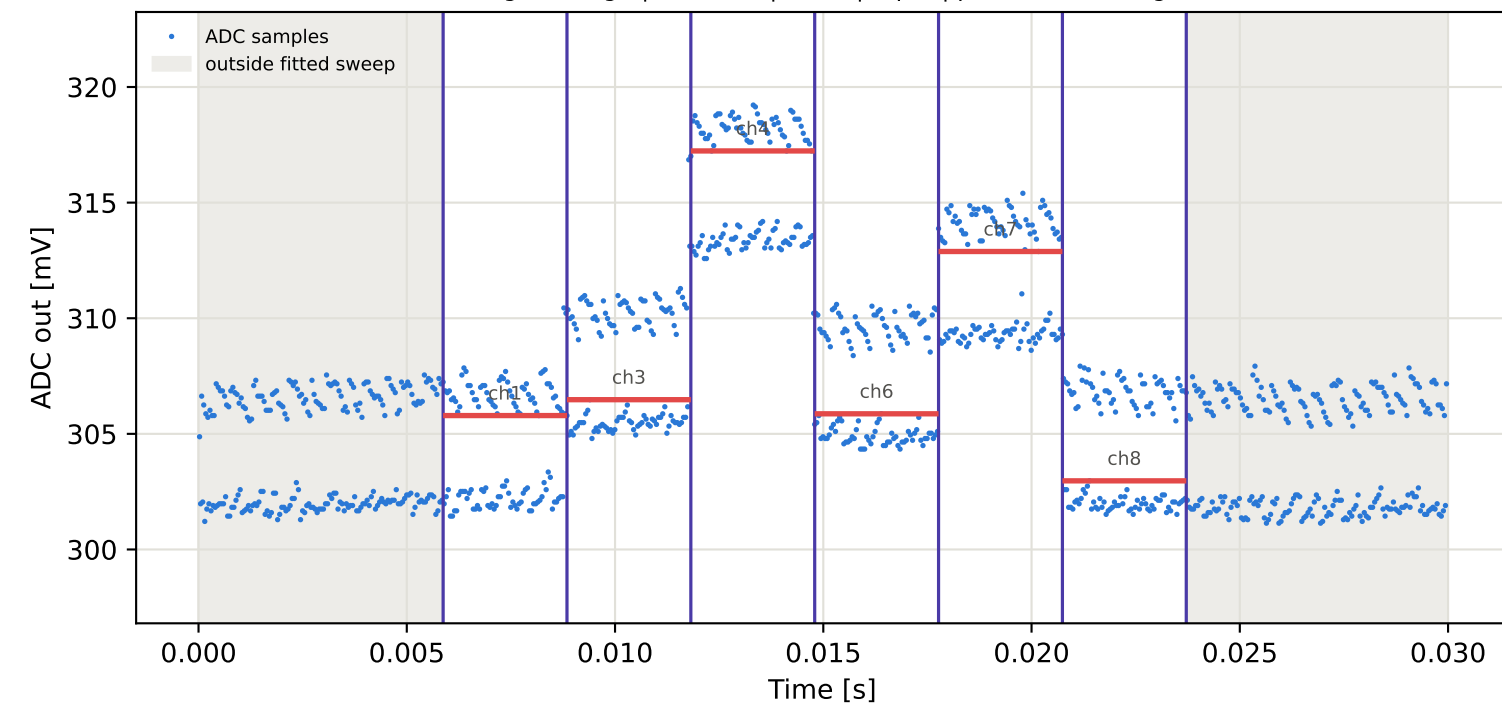
Tag5 &lt;- Tag8 | 965 MHz | run 0 | rep 1 | phase -150.91 deg
