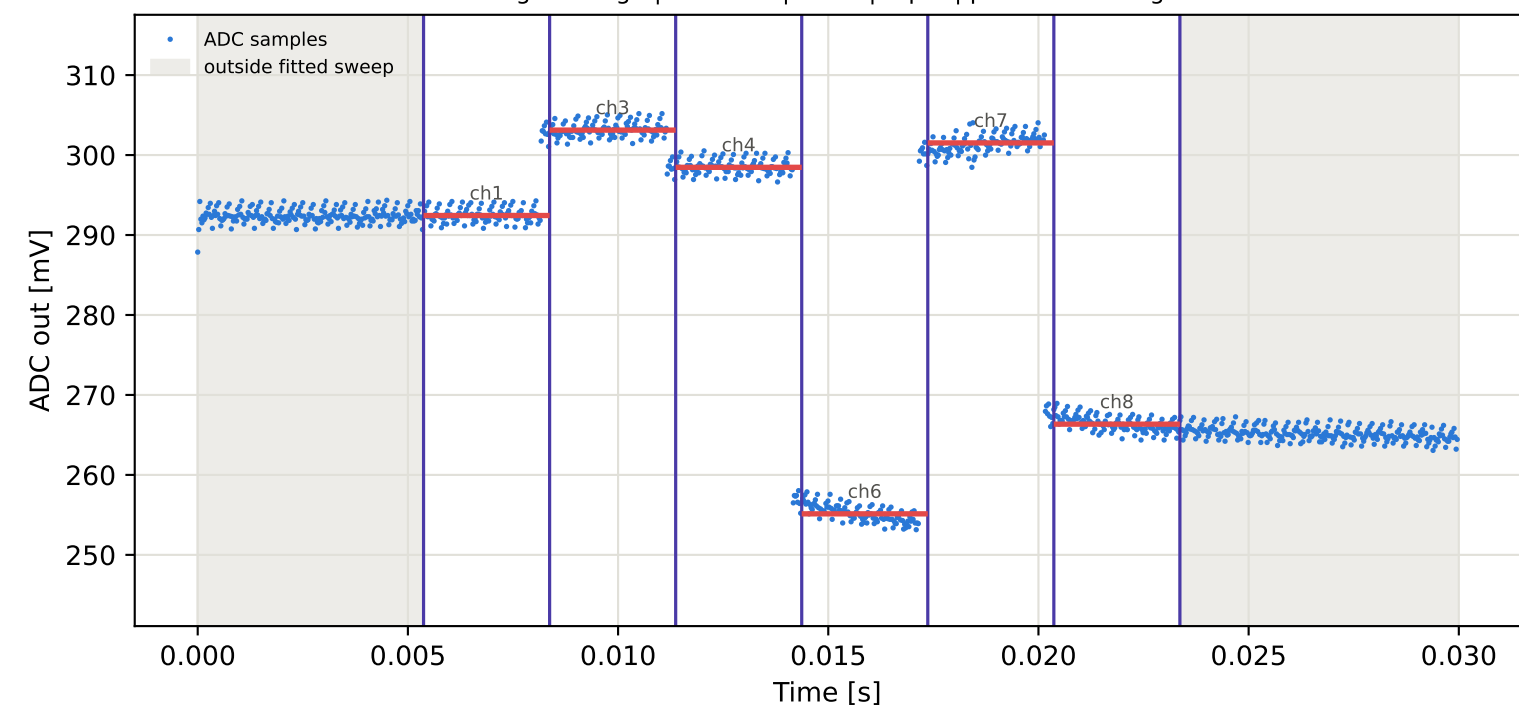
Tag3 &lt;- Tag9 | 915 MHz | run 0 | rep 1 | phase -7.11 deg
