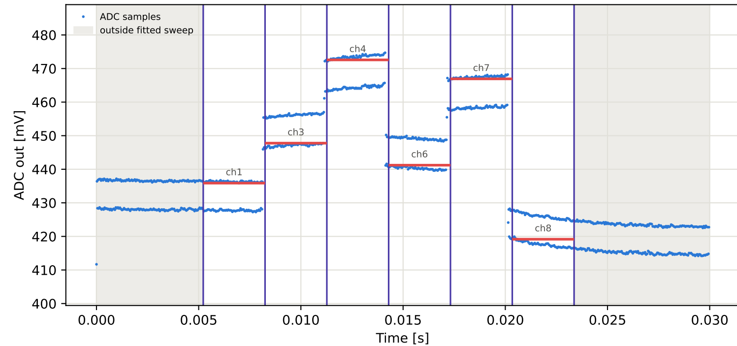
Tag15 &lt;- Tag10 | 915 MHz | run 0 | rep 1 | phase 123.85 deg
