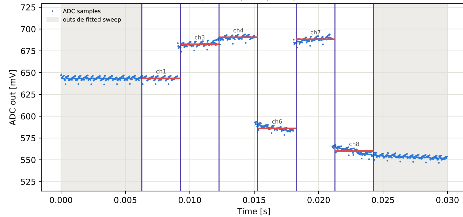
Tag7 &lt;- Tag3 | 905 MHz | run 0 | rep 1 | phase 30.97 deg
