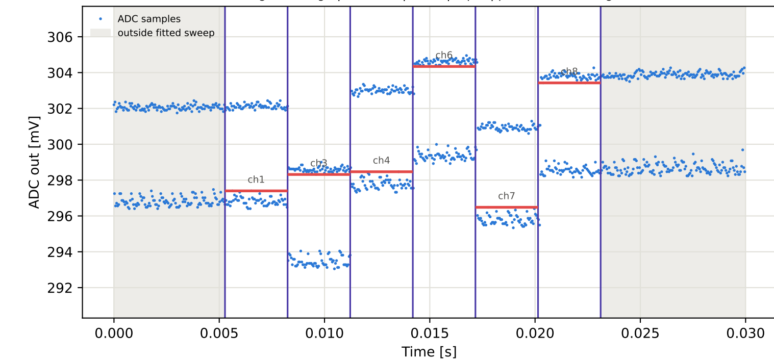
Tag15 &lt;- Tag5 | 805 MHz | run 0 | rep 1 | phase 170.08 deg
