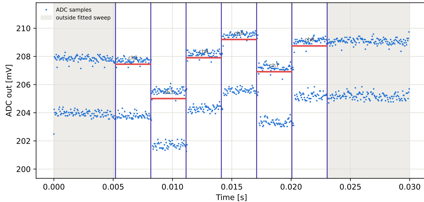
Tag3 &lt;- Tag16 | 805 MHz | run 0 | rep 1 | phase -110.85 deg
