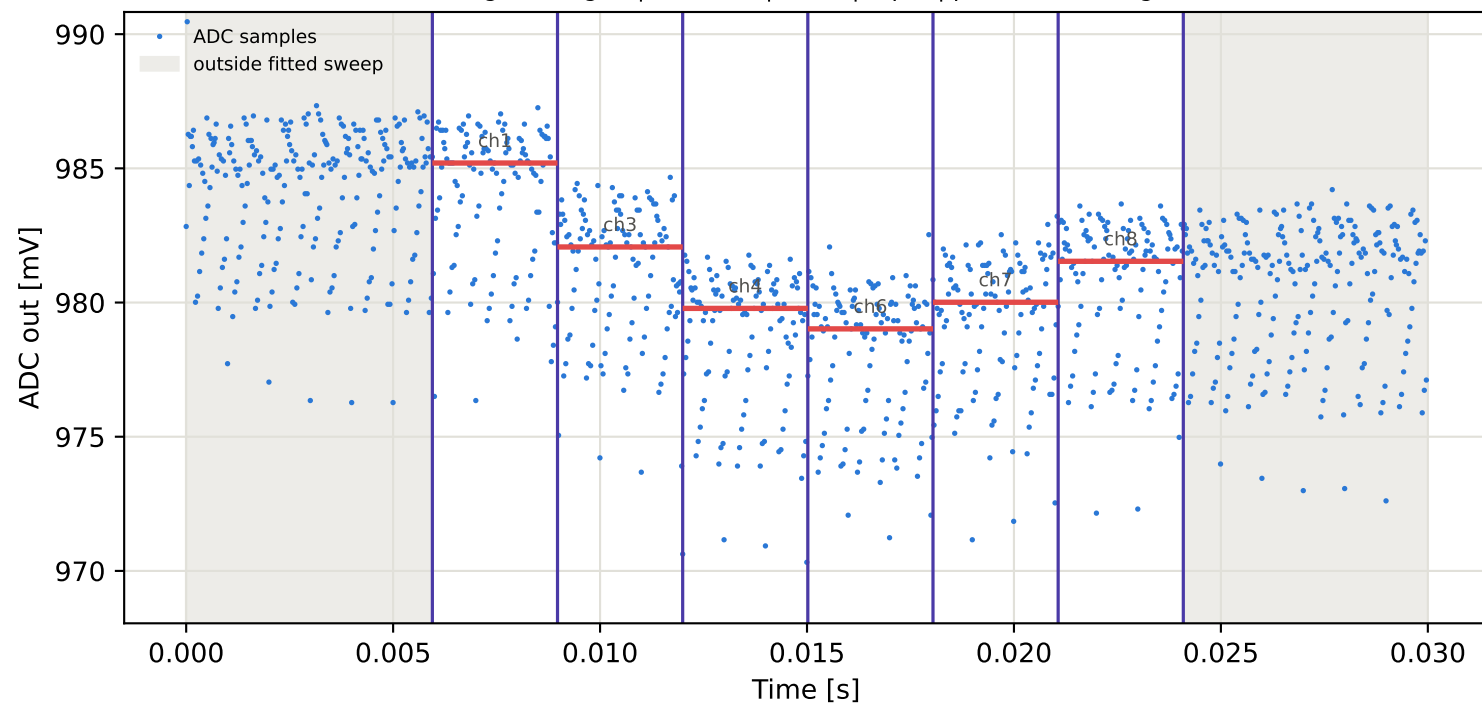
Tag5 &lt;- Tag16 | 865 MHz | run 0 | rep 1 | phase -108.67 deg
