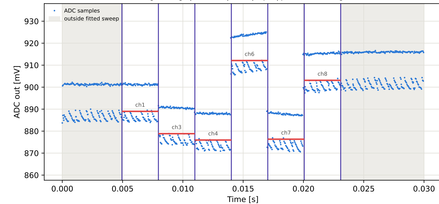
Tag4 &lt;- Tag9 | 945 MHz | run 0 | rep 1 | phase 55.24 deg
