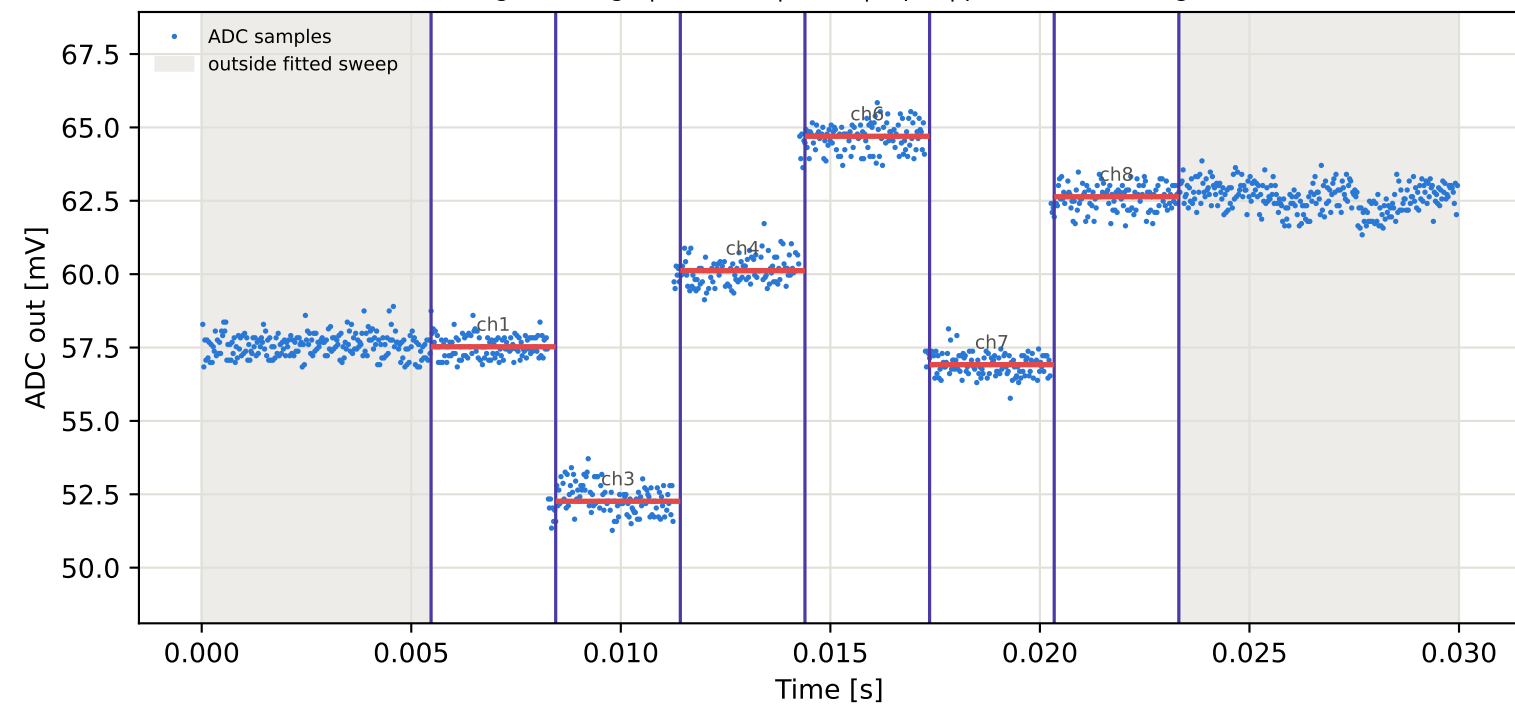
Tag10 &lt;- Tag9 | 785 MHz | run 0 | rep 1 | phase 127.21 deg
