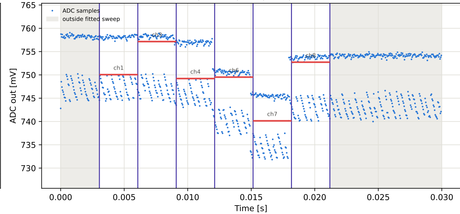
Tag8 &lt;- Tag7 | 935 MHz | run 0 | rep 1 | phase 75.80 deg
