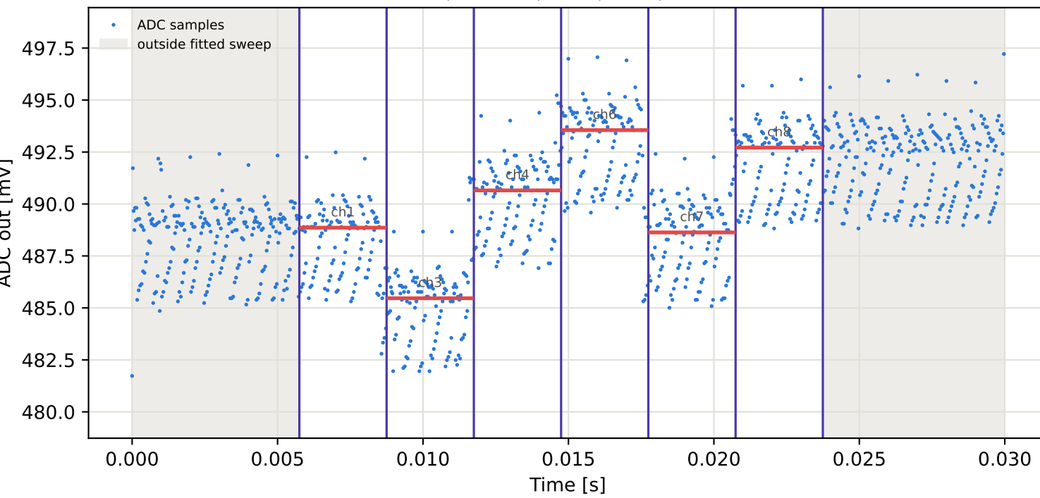
Tag16 &lt;- Tag10 | 835 MHz | run 0 | rep 1 | phase -155.58 deg
