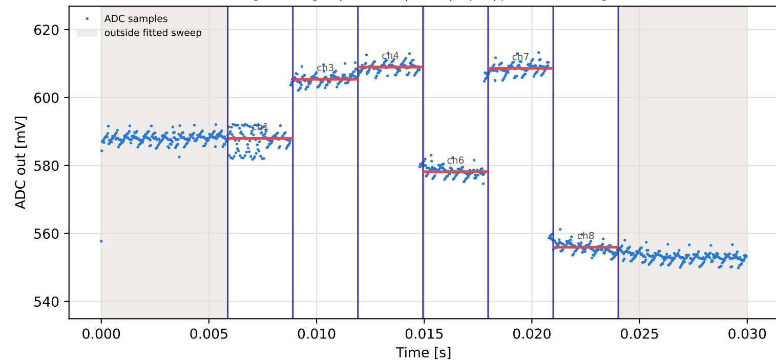
Tag10 &lt;- Tag3 | 895 MHz | run 0 | rep 1 | phase 70.68 deg
