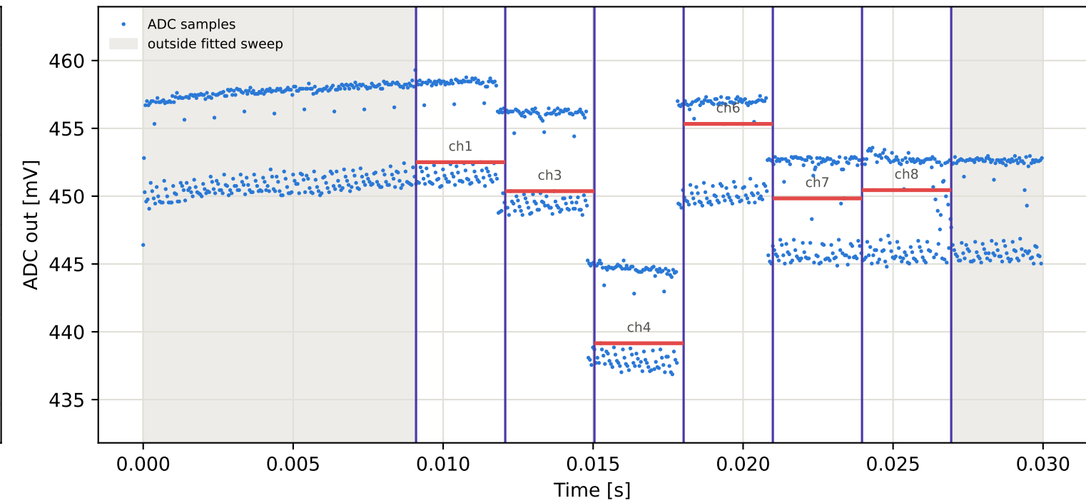
Tag1 &lt;- Tag4 | 875 MHz | run 0 | rep 1 | phase -135.01 deg
