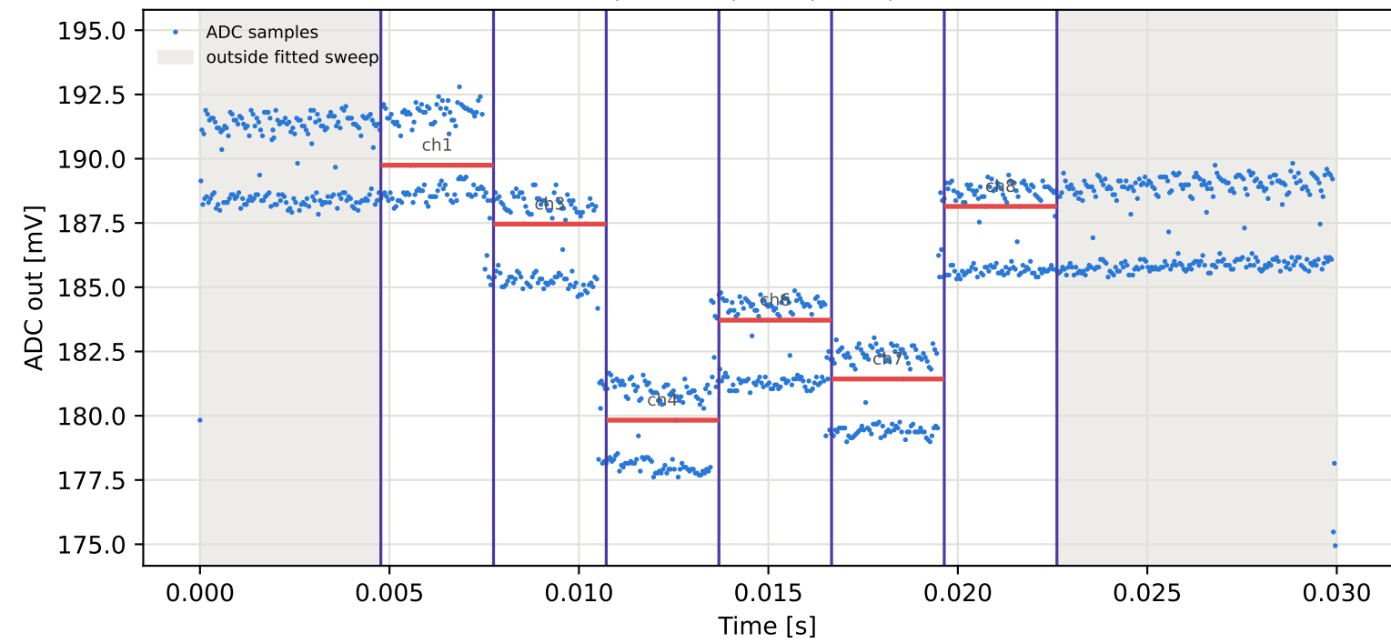
Tag16 &lt;- Tag7 | 805 MHz | run 0 | rep 1 | phase 81.79 deg
