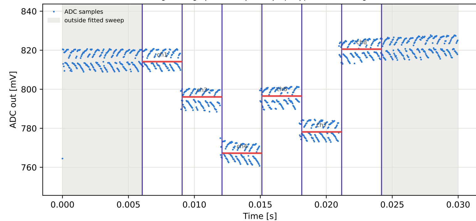
Tag4 &lt;- Tag9 | 935 MHz | run 0 | rep 1 | phase 86.86 deg
