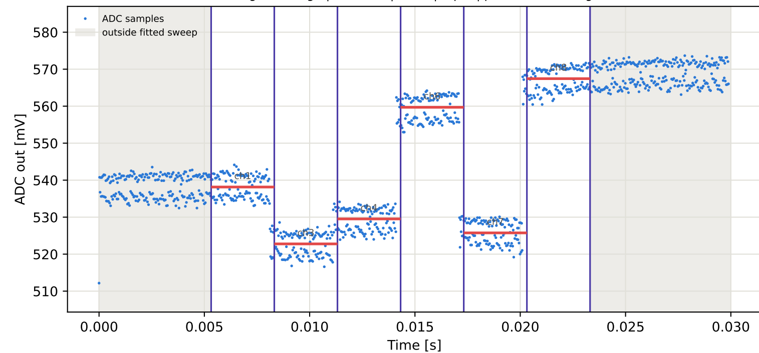
Tag10 &lt;- Tag5 | 885 MHz | run 0 | rep 1 | phase 163.56 deg
