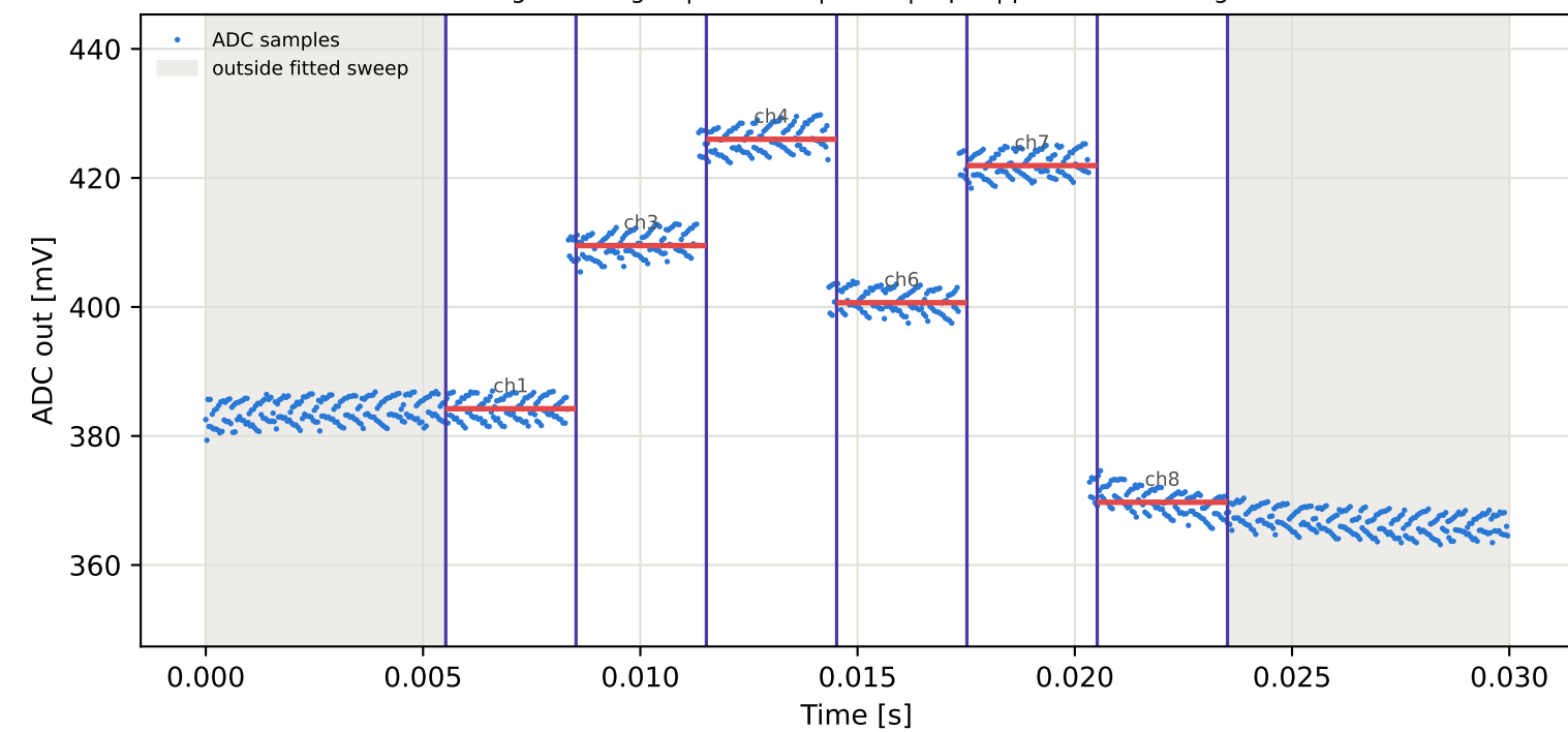
Tag10 &lt;- Tag2 | 905 MHz | run 0 | rep 1 | phase 159.46 deg
