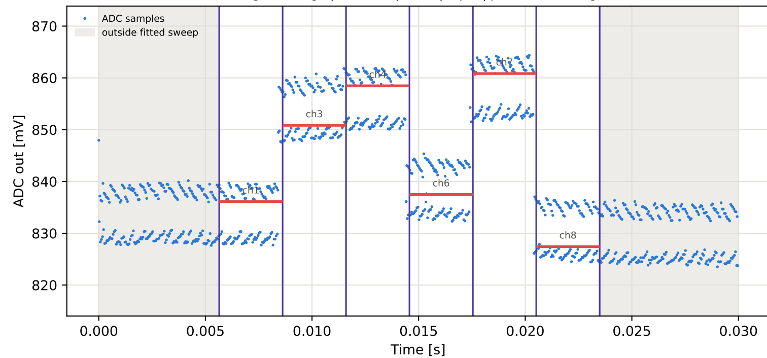
Tag2 &lt;- Tag10 | 865 MHz | run 0 | rep 1 | phase -134.32 deg
