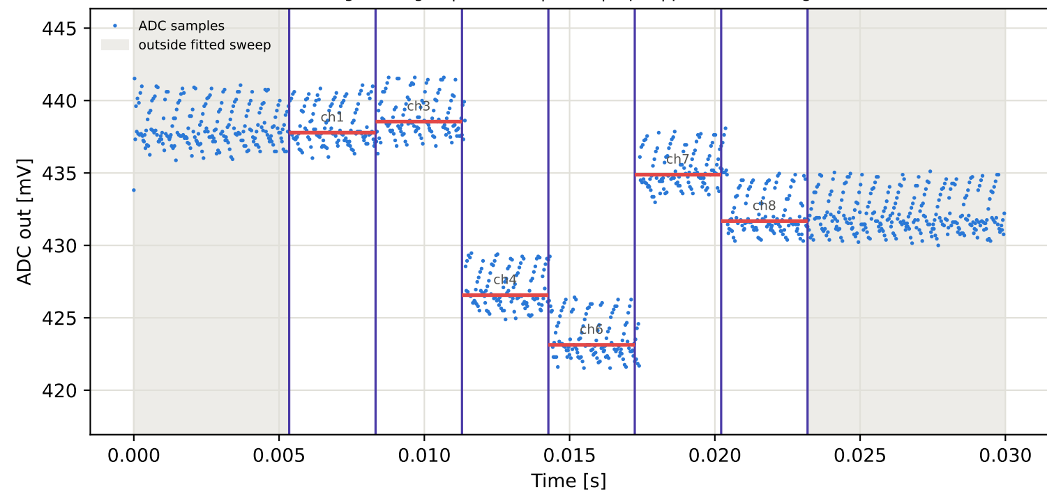
Tag4 &lt;- Tag3 | 995 MHz | run 0 | rep 1 | phase -118.59 deg
