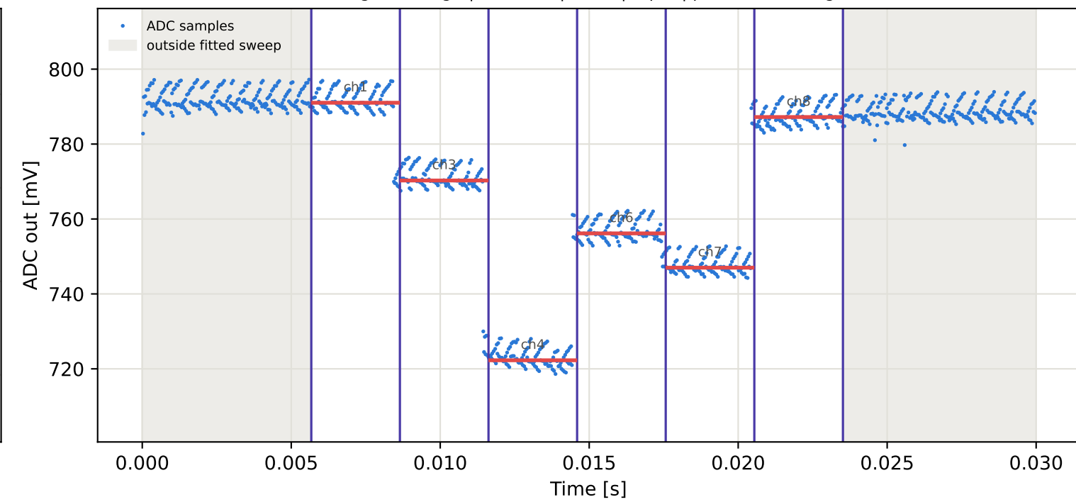
Tag2 &lt;- Tag10 | 965 MHz | run 0 | rep 1 | phase -110.99 deg
