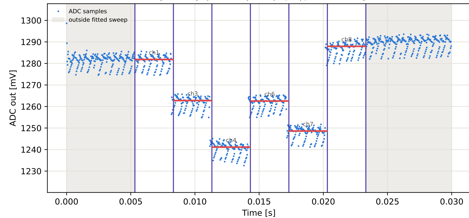
Tag15 &lt;- Tag9 | 915 MHz | run 0 | rep 1 | phase -72.95 deg
