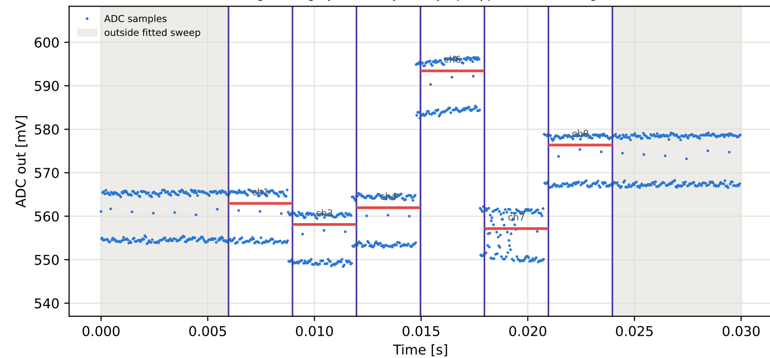
Tag6 &lt;- Tag1 | 945 MHz | run 0 | rep 1 | phase 1.38 deg
