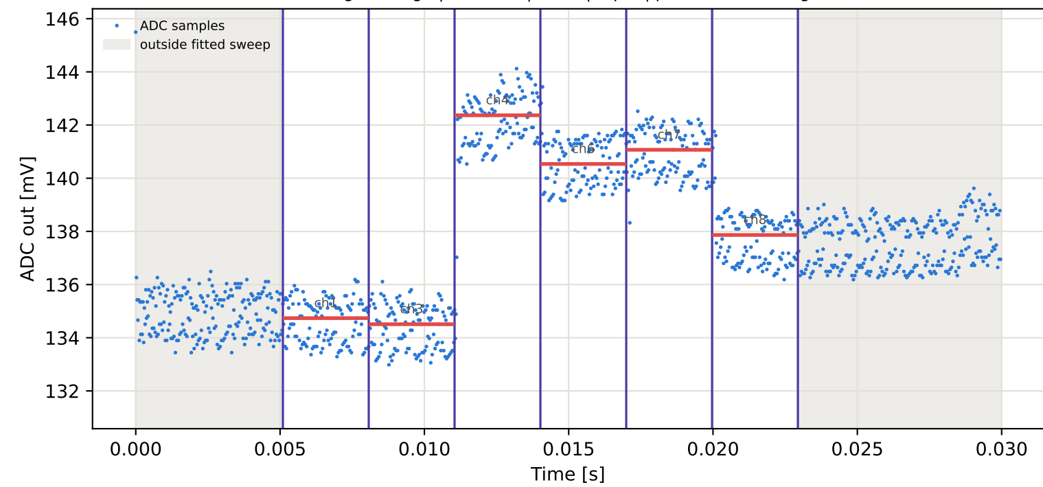
Tag6 &lt;- Tag5 | 785 MHz | run 0 | rep 1 | phase -109.77 deg
