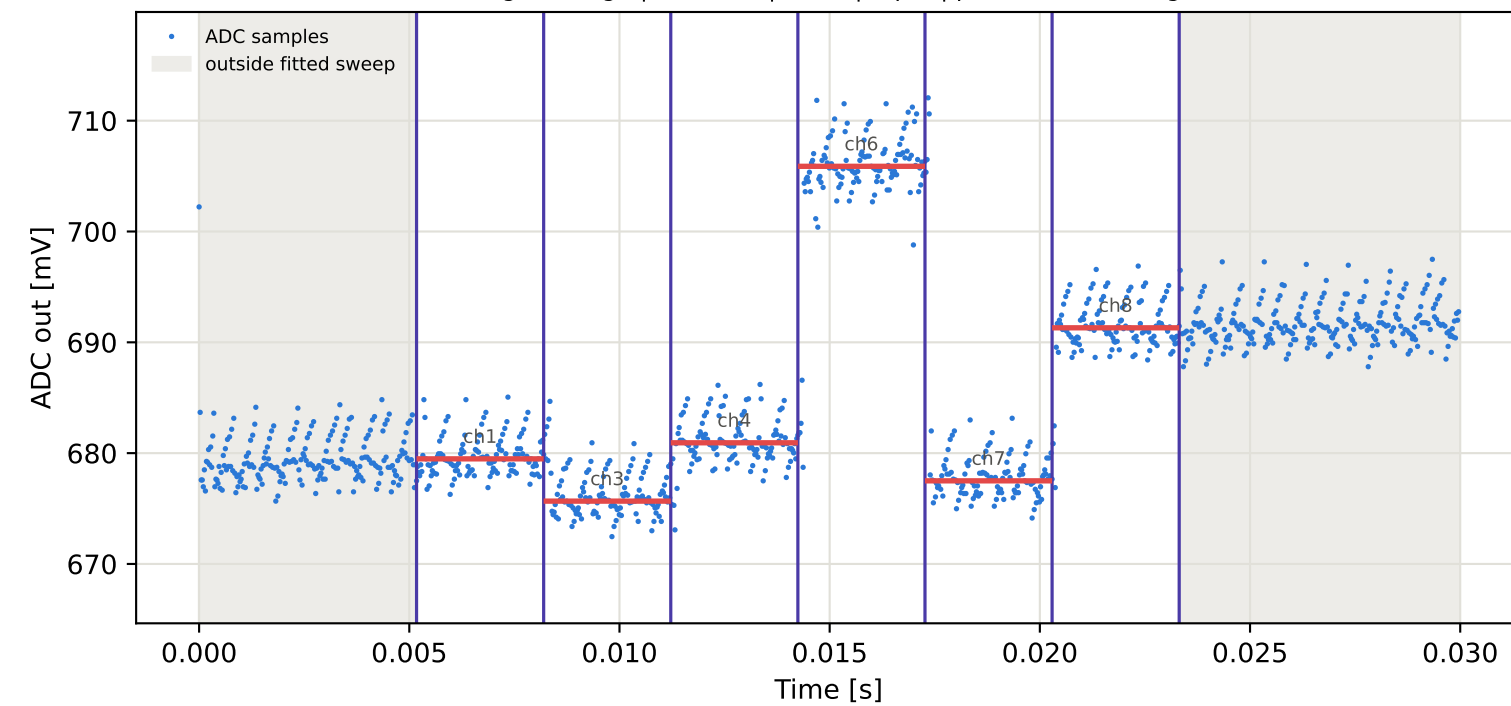
Tag5 &lt;- Tag8 | 935 MHz | run 0 | rep 1 | phase -166.08 deg
