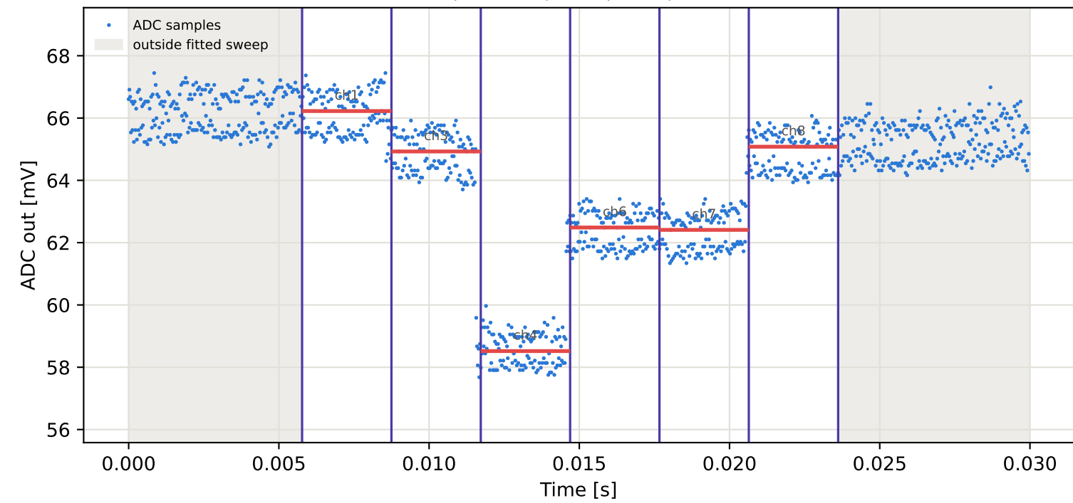
Tag2 &lt;- Tag8 | 995 MHz | run 0 | rep 1 | phase 58.71 deg
