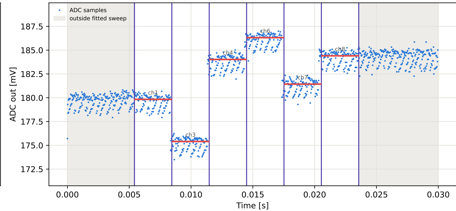
Tag4 &lt;- Tag3 | 825 MHz | run 0 | rep 1 | phase -129.33 deg
