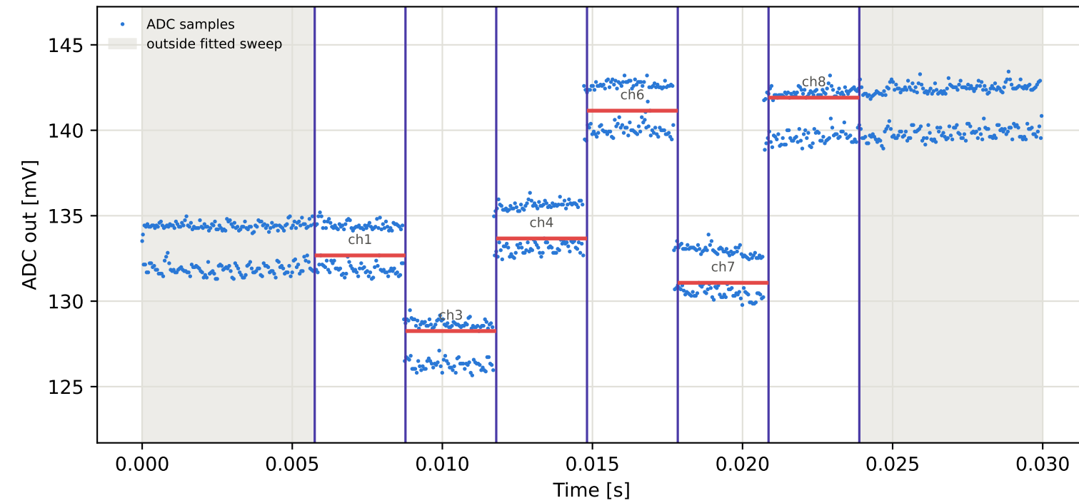
Tag15 &lt;- Tag1 | 845 MHz | run 0 | rep 1 | phase 130.16 deg
