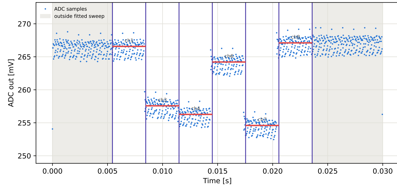
Tag3 &lt;- Tag8 | 825 MHz | run 0 | rep 1 | phase -152.10 deg
