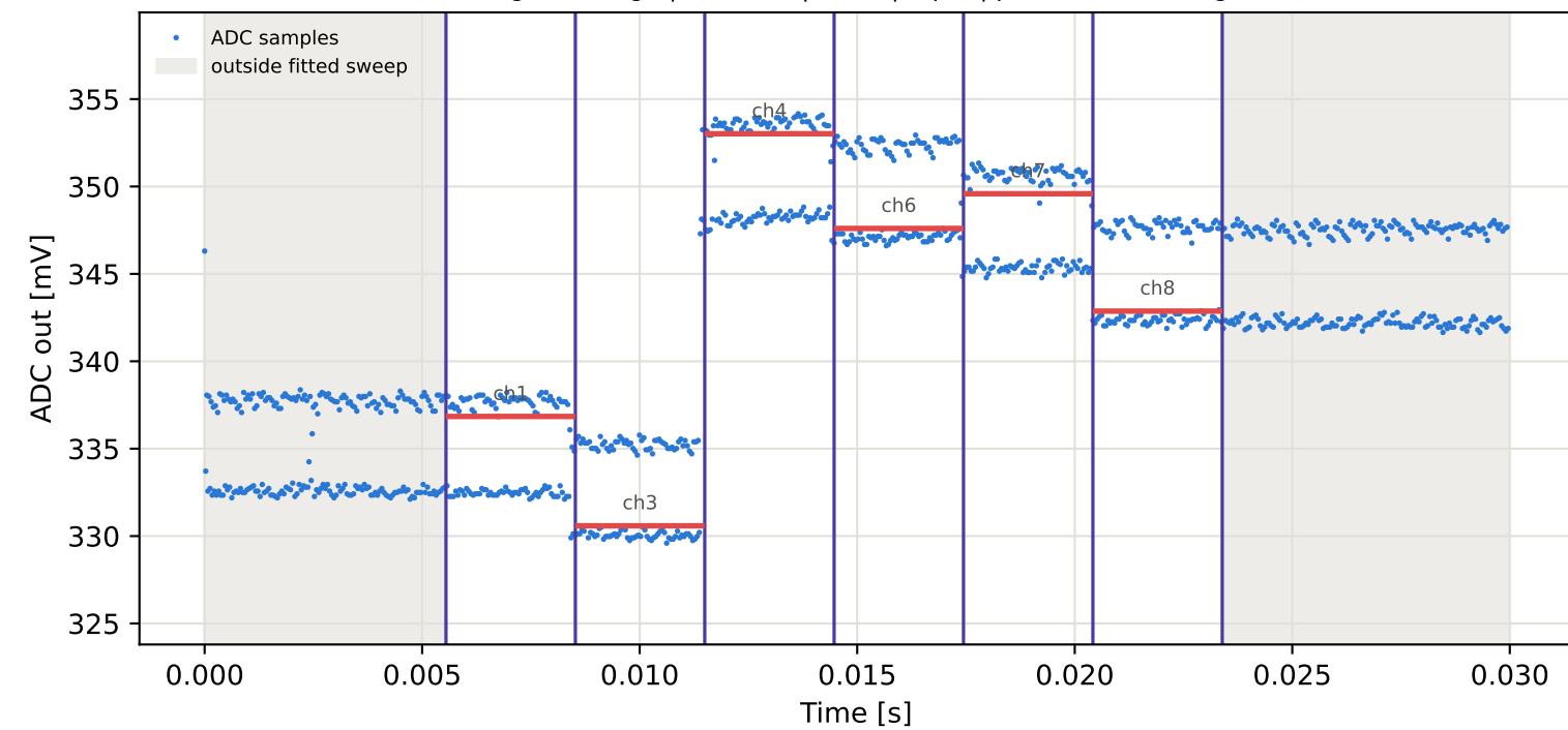
Tag16 &lt;- Tag5 | 825 MHz | run 0 | rep 1 | phase -4.32 deg
