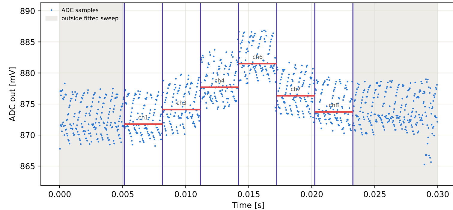
Tag6 &lt;- Tag4 | 875 MHz | run 0 | rep 1 | phase 164.06 deg
