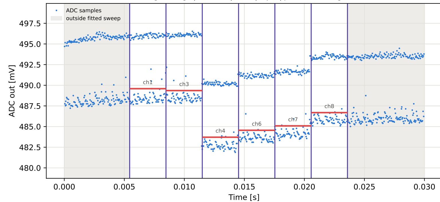
Tag9 &lt;- Tag10 | 825 MHz | run 0 | rep 1 | phase -157.34 deg
