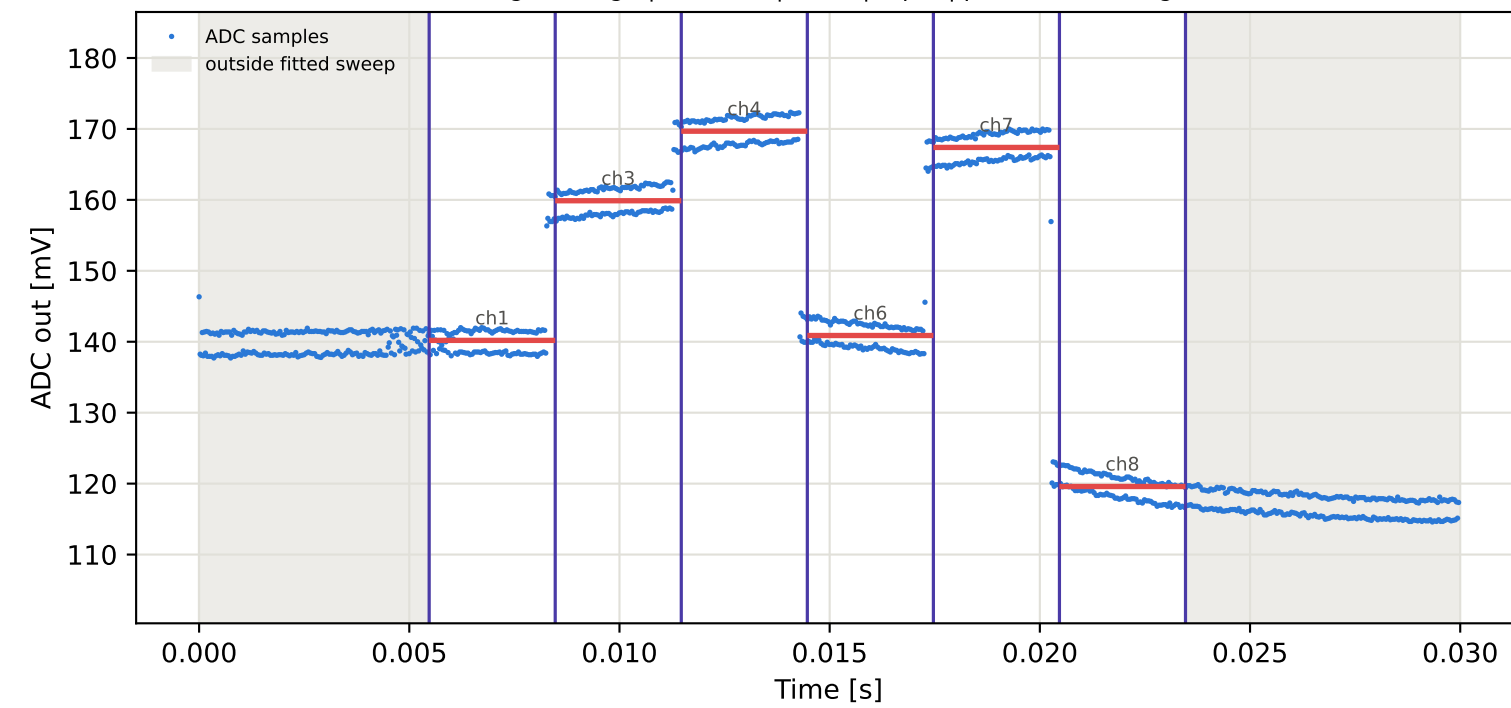
Tag9 &lt;- Tag5 | 895 MHz | run 0 | rep 1 | phase -130.51 deg
