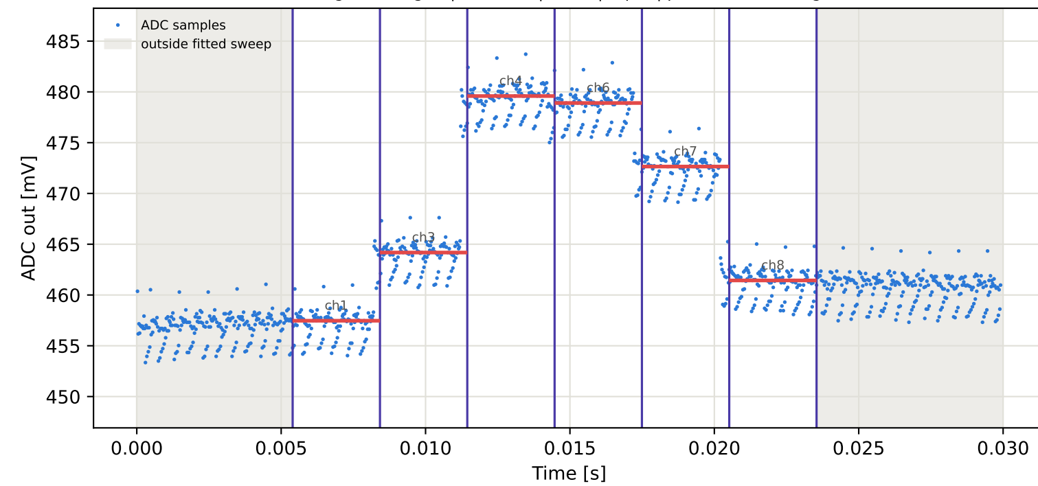
Tag10 &lt;- Tag2 | 945 MHz | run 0 | rep 1 | phase 158.30 deg
