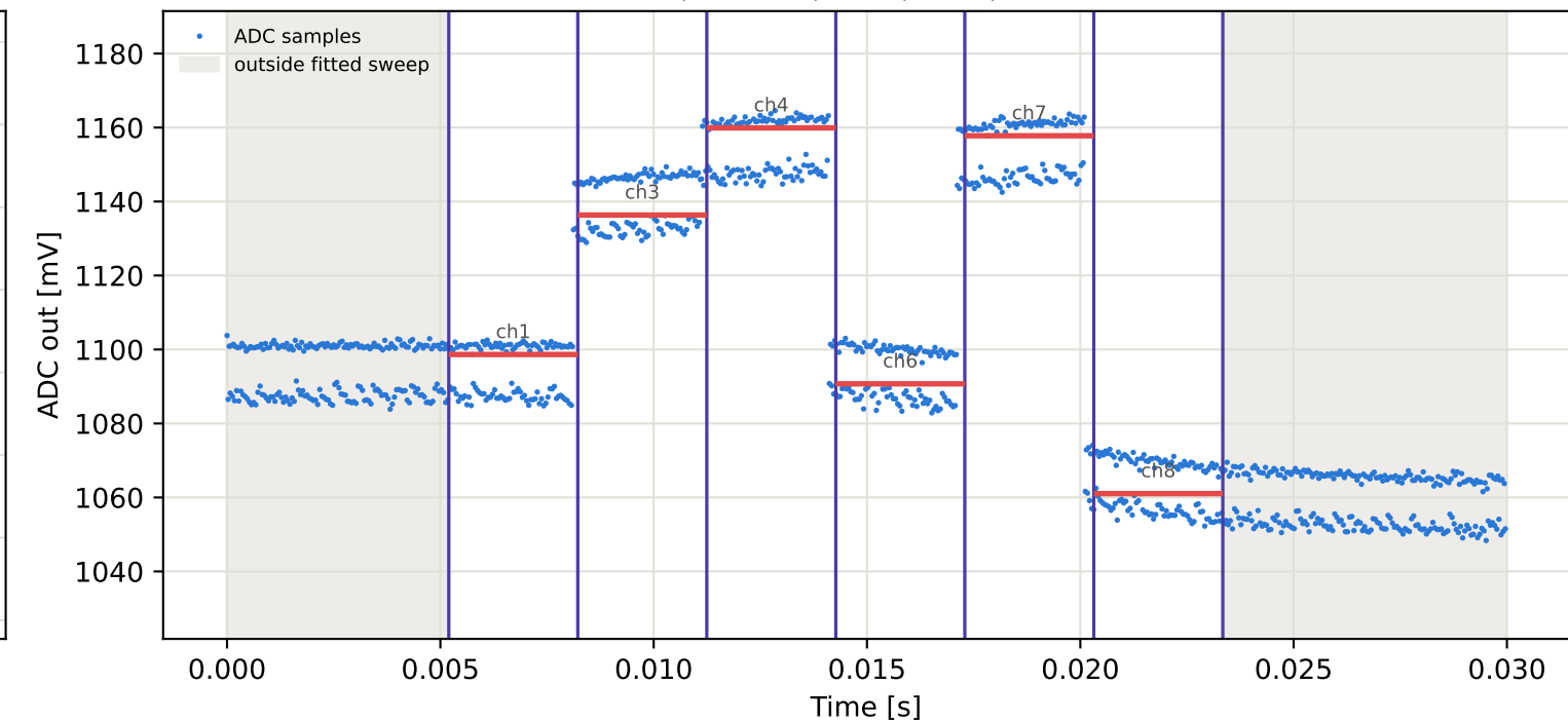
Tag8 &lt;- Tag7 | 885 MHz | run 0 | rep 1 | phase -56.96 deg
