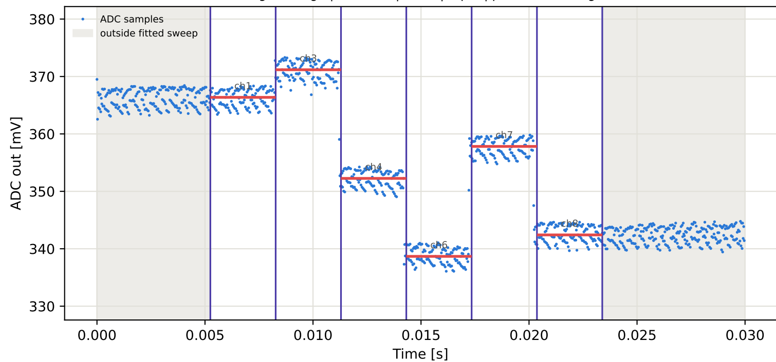
Tag5 &lt;- Tag4 | 845 MHz | run 0 | rep 1 | phase 28.87 deg
