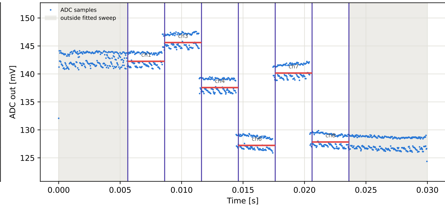
Tag7 &lt;- Tag6 | 855 MHz | run 0 | rep 1 | phase 76.37 deg
