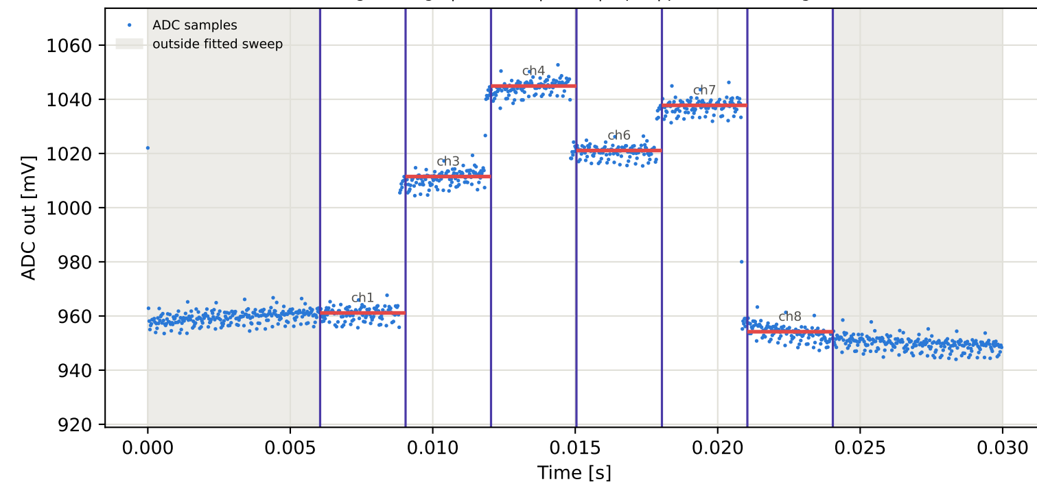
Tag3 &lt;- Tag6 | 885 MHz | run 0 | rep 1 | phase -117.07 deg
