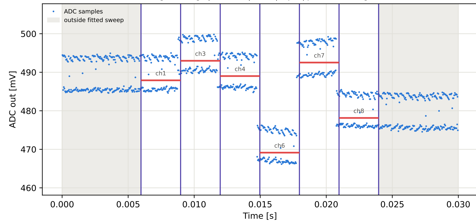
Tag10 &lt;- Tag9 | 955 MHz | run 0 | rep 1 | phase -69.17 deg
