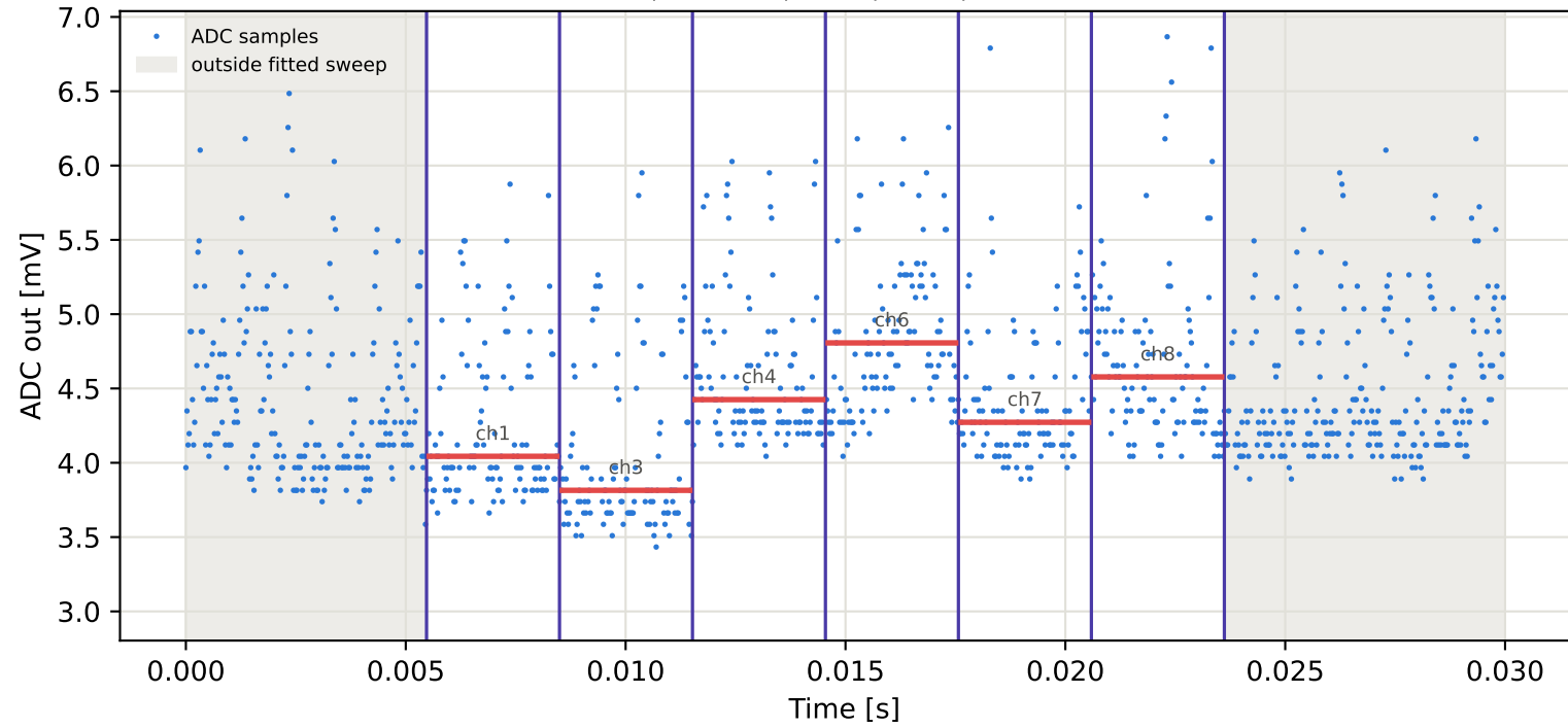
Tag2 &lt;- Tag7 | 785 MHz | run 0 | rep 1 | phase -143.23 deg
