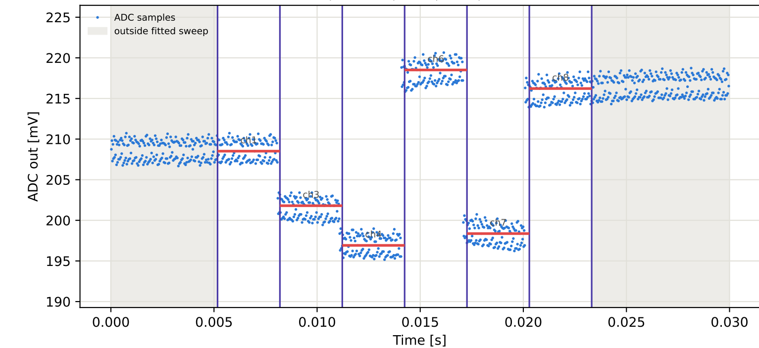
Tag1 &lt;- Tag9 | 965 MHz | run 0 | rep 1 | phase 138.44 deg
