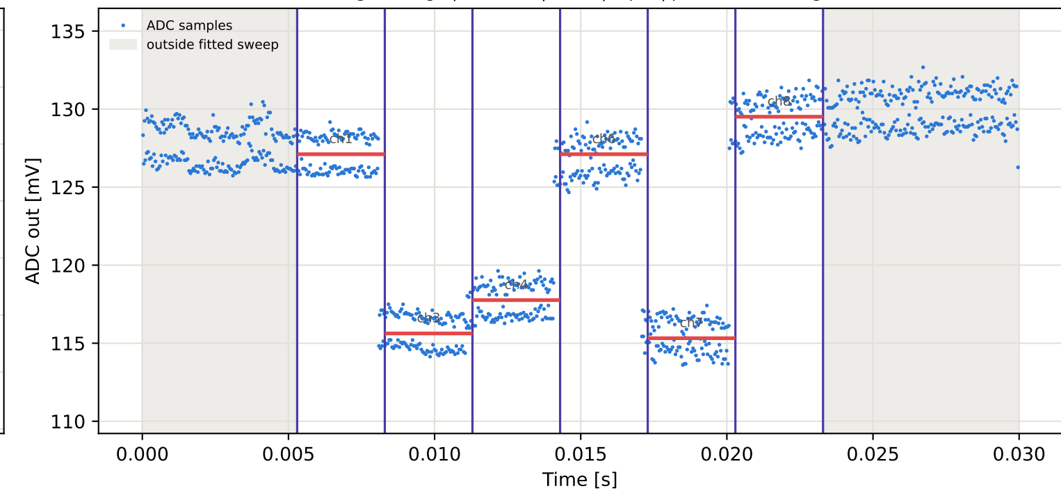
Tag7 &lt;- Tag1 | 825 MHz | run 0 | rep 1 | phase 24.17 deg
