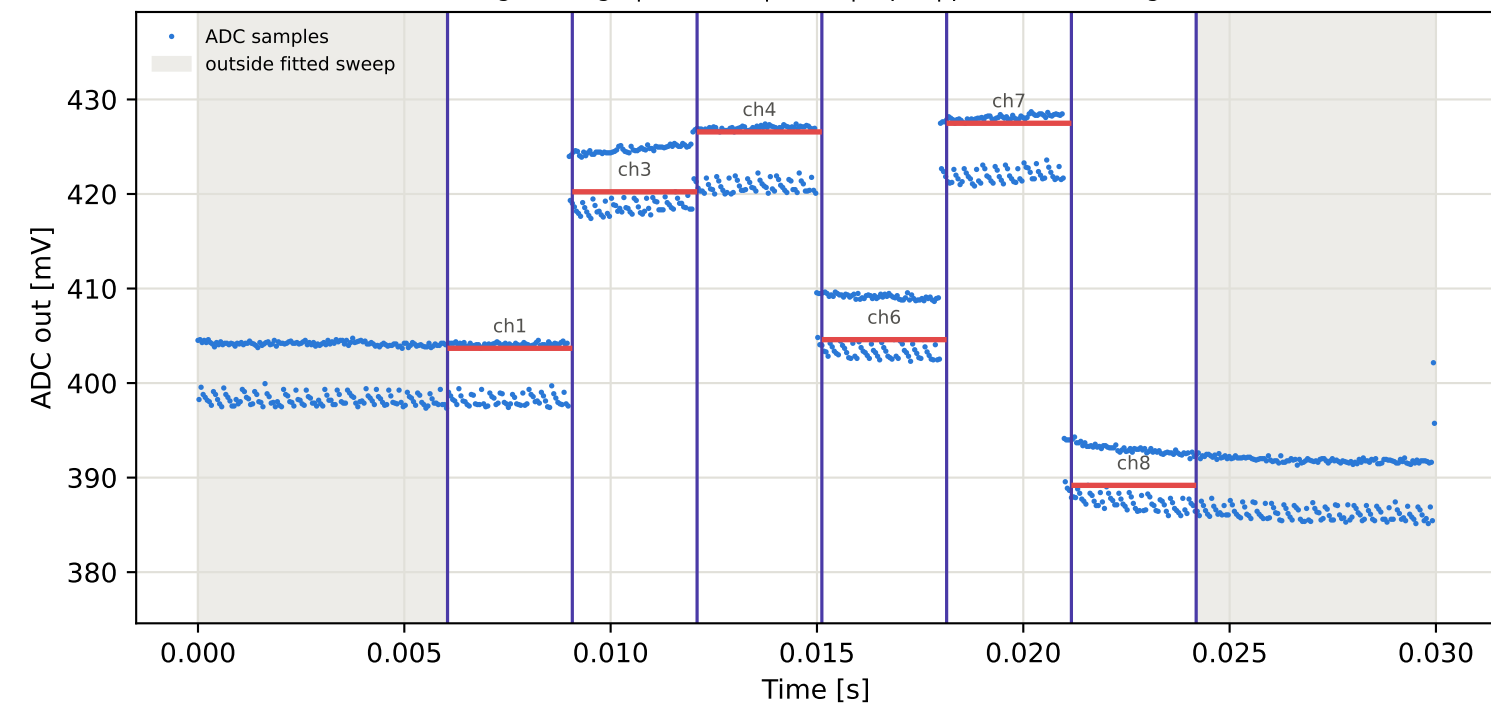
Tag1 &lt;- Tag8 | 865 MHz | run 0 | rep 1 | phase -171.34 deg
