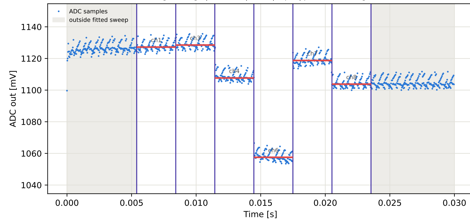
Tag8 &lt;- Tag1 | 935 MHz | run 0 | rep 1 | phase 179.26 deg
