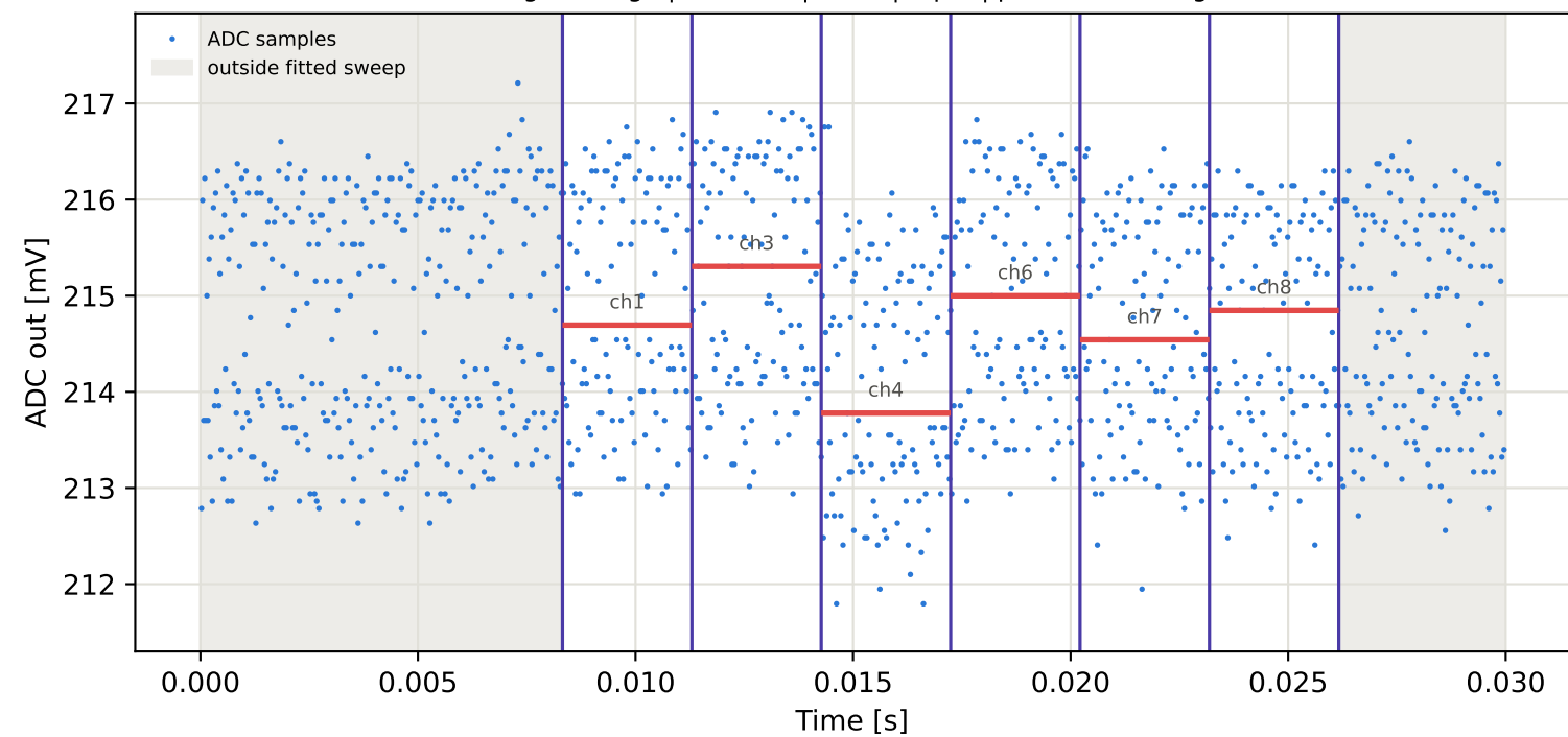
Tag3 &lt;- Tag2 | 995 MHz | run 0 | rep 1 | phase 66.76 deg
