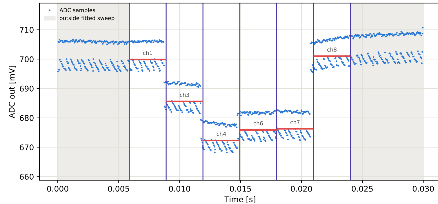
Tag10 &lt;- Tag4 | 895 MHz | run 0 | rep 1 | phase 73.39 deg
