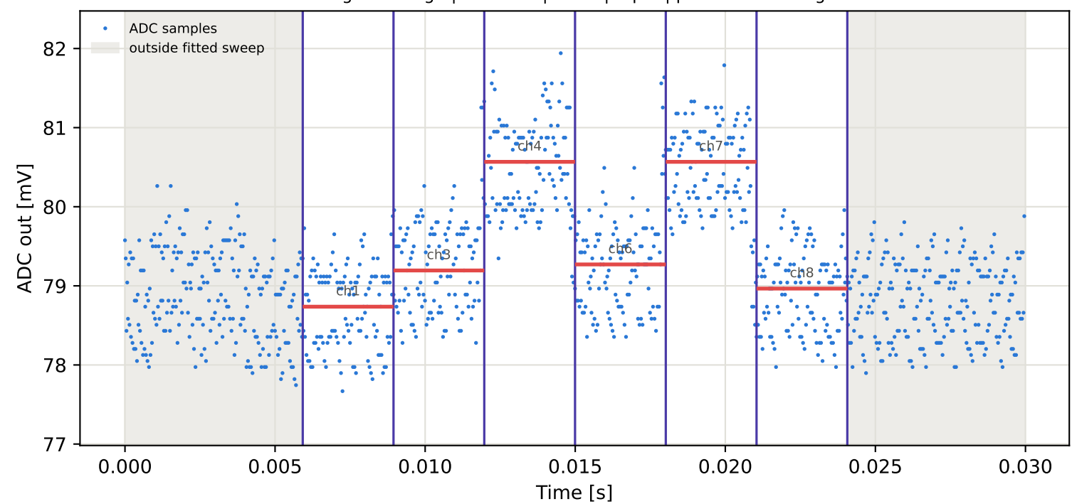
Tag10 &lt;- Tag5 | 795 MHz | run 0 | rep 1 | phase -81.06 deg
