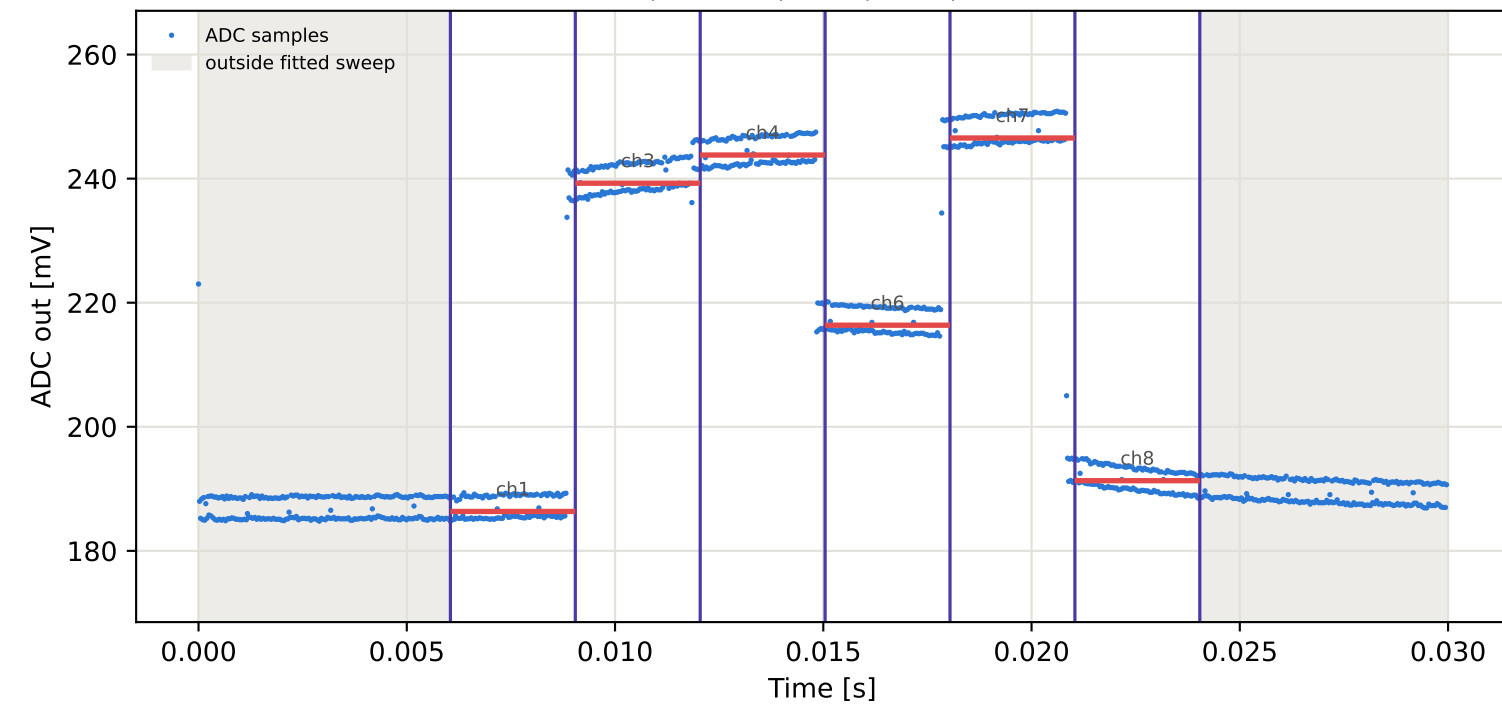
Tag9 &lt;- Tag16 | 855 MHz | run 0 | rep 1 | phase -70.82 deg
