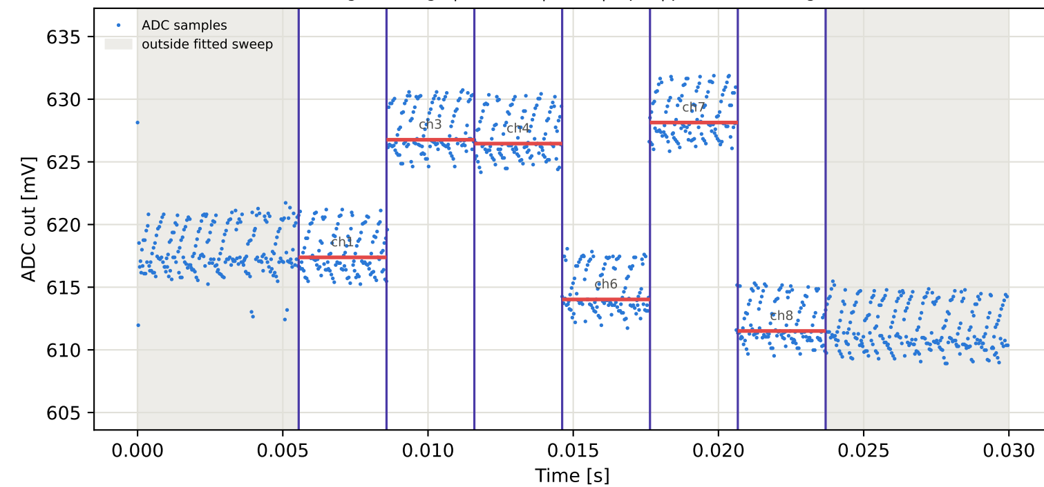
Tag15 &lt;- Tag9 | 865 MHz | run 0 | rep 1 | phase -68.92 deg
