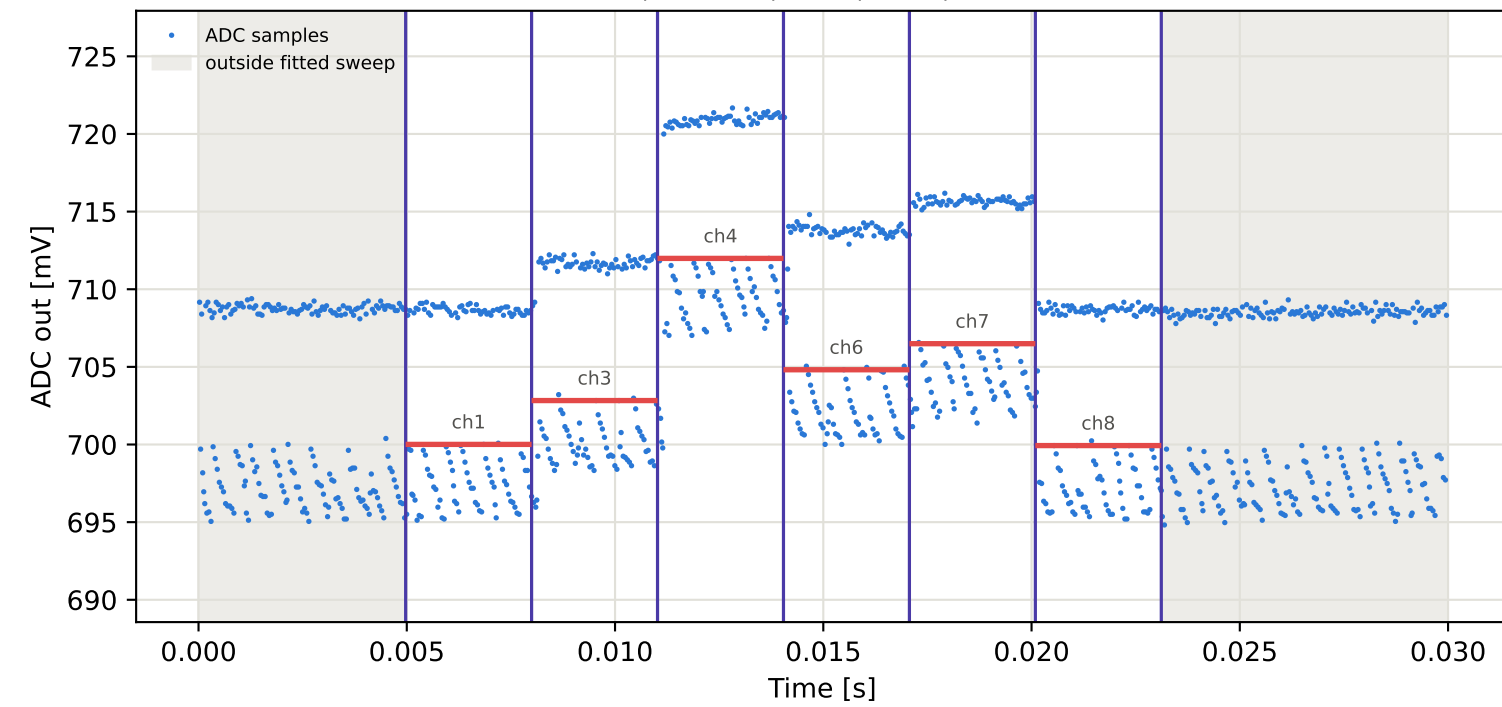
Tag15 &lt;- Tag5 | 975 MHz | run 0 | rep 1 | phase -111.03 deg
