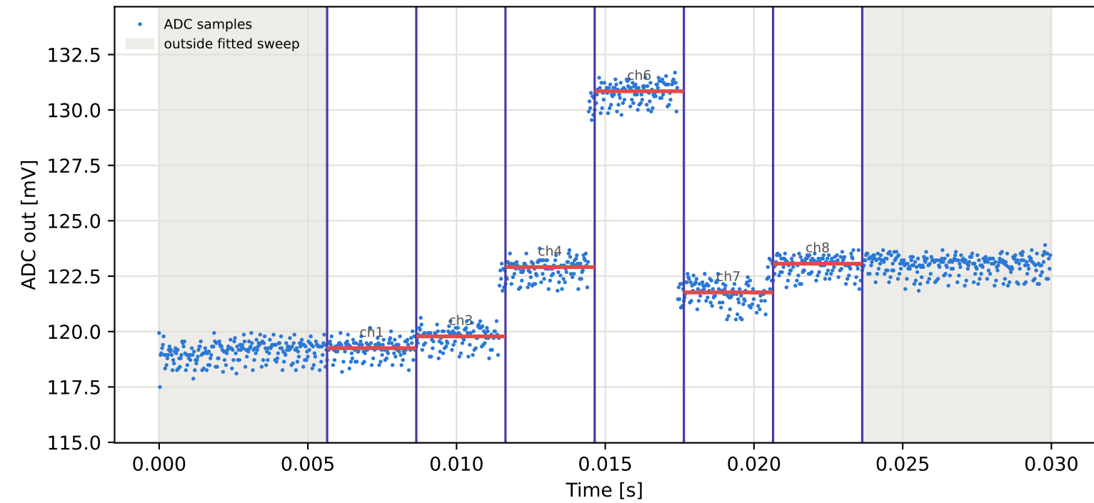
Tag1 &lt;- Tag4 | 925 MHz | run 0 | rep 1 | phase -27.90 deg
