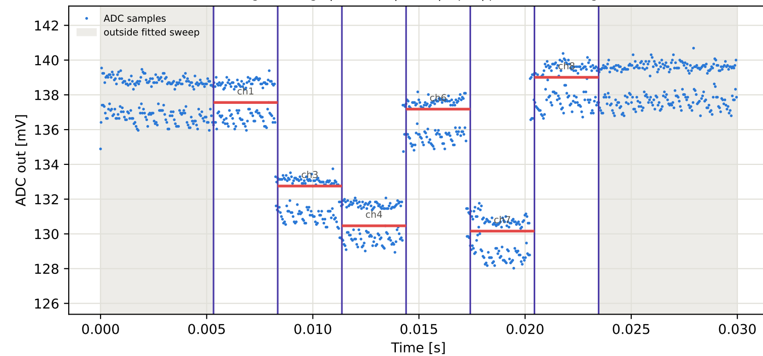
Tag15 &lt;- Tag9 | 795 MHz | run 0 | rep 1 | phase 132.12 deg
