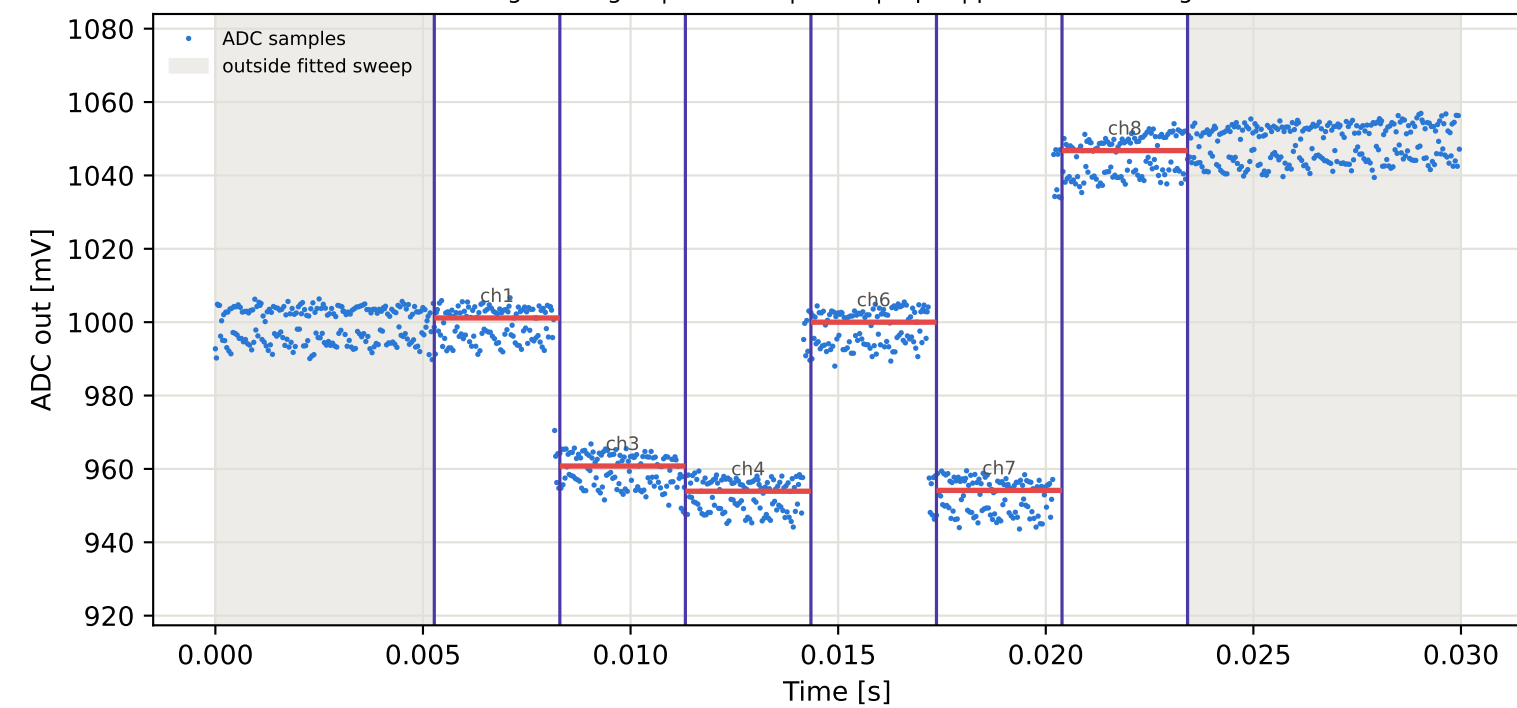
Tag7 &lt;- Tag3 | 885 MHz | run 0 | rep 1 | phase 47.55 deg
