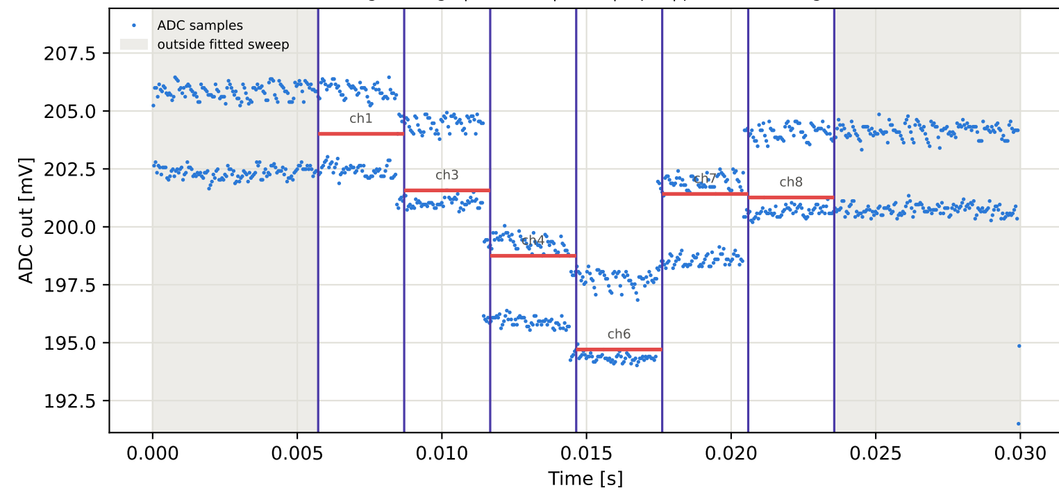
Tag9 &lt;- Tag6 | 945 MHz | run 0 | rep 1 | phase -42.67 deg
