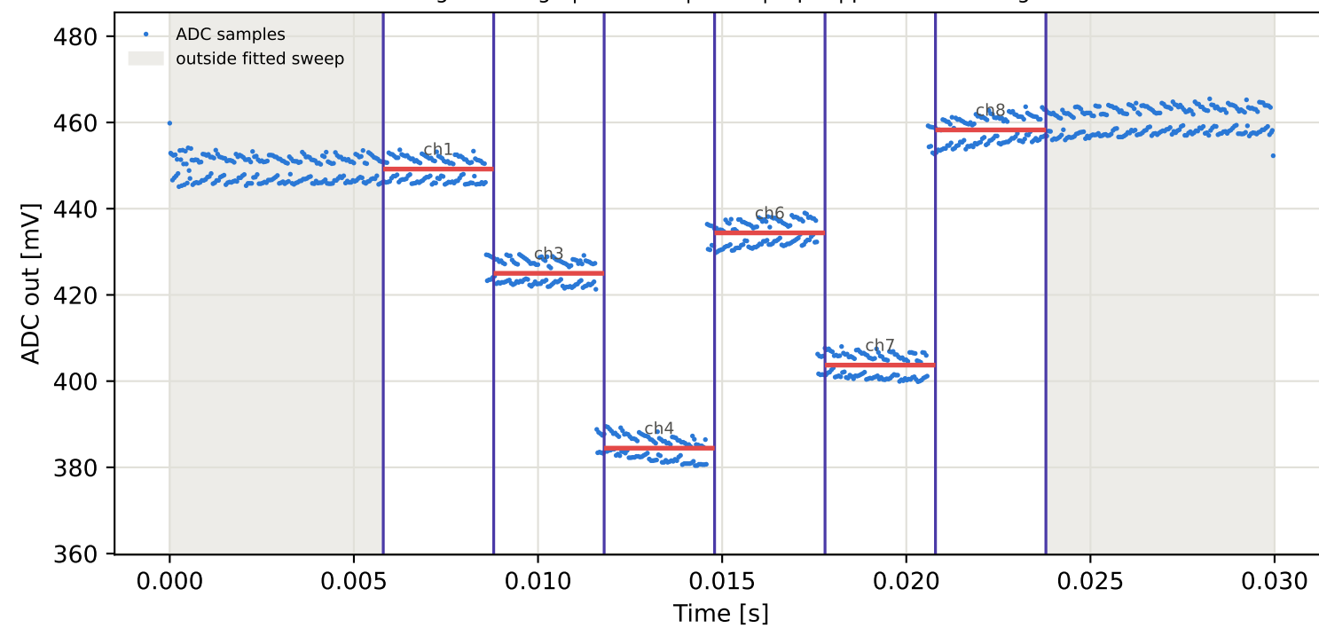
Tag10 &lt;- Tag8 | 935 MHz | run 0 | rep 1 | phase -73.05 deg
