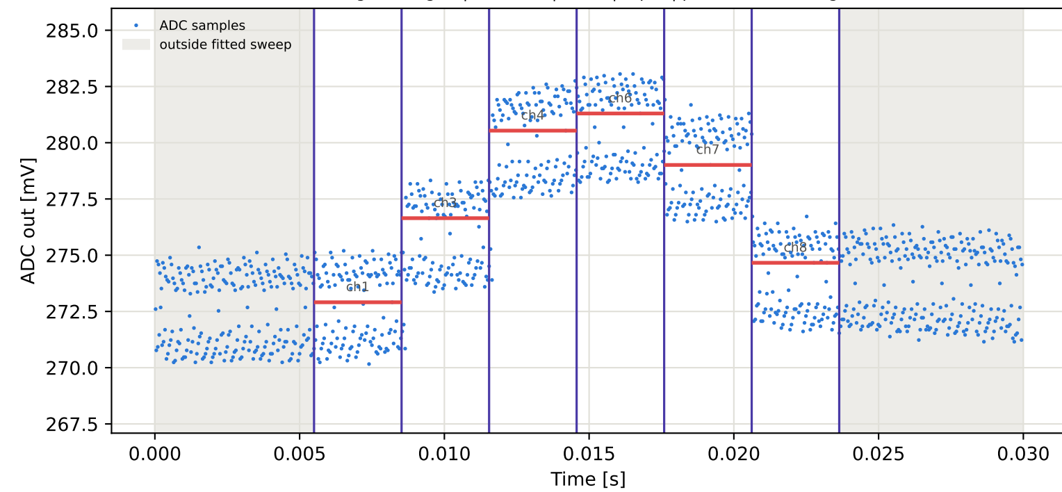
Tag1 &lt;- Tag2 | 905 MHz | run 0 | rep 1 | phase 35.93 deg
