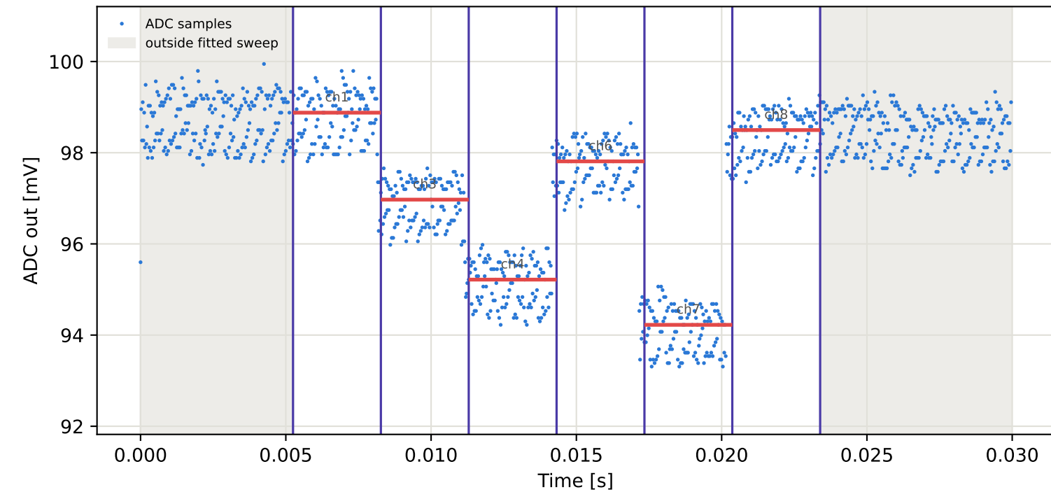
Tag7 &lt;- Tag6 | 795 MHz | run 0 | rep 1 | phase -75.52 deg
