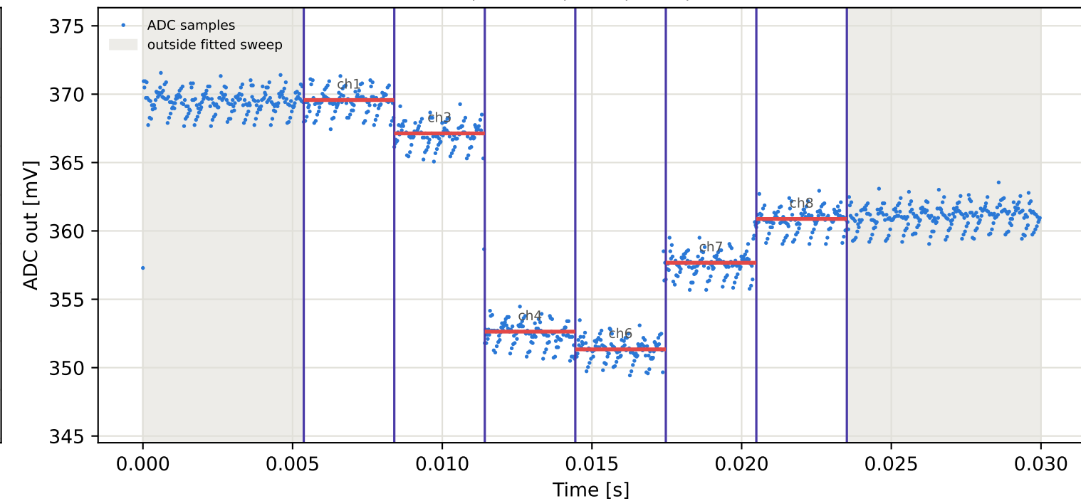
Tag16 &lt;- Tag7 | 845 MHz | run 0 | rep 1 | phase 54.06 deg
