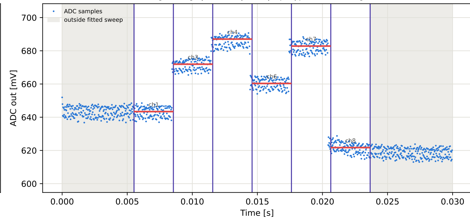
Tag1 &lt;- Tag8 | 885 MHz | run 0 | rep 1 | phase 124.42 deg
