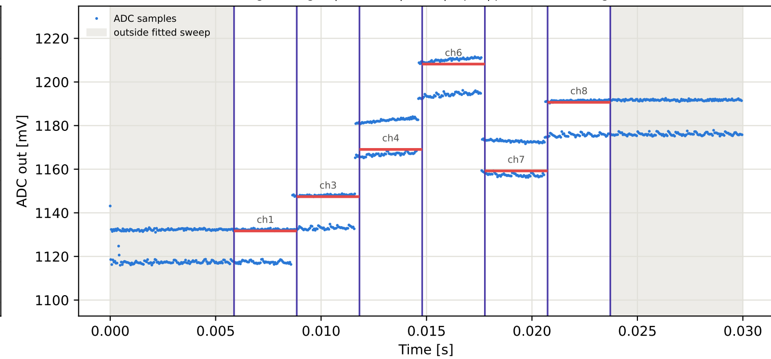
Tag5 &lt;- Tag2 | 875 MHz | run 0 | rep 1 | phase -116.12 deg
