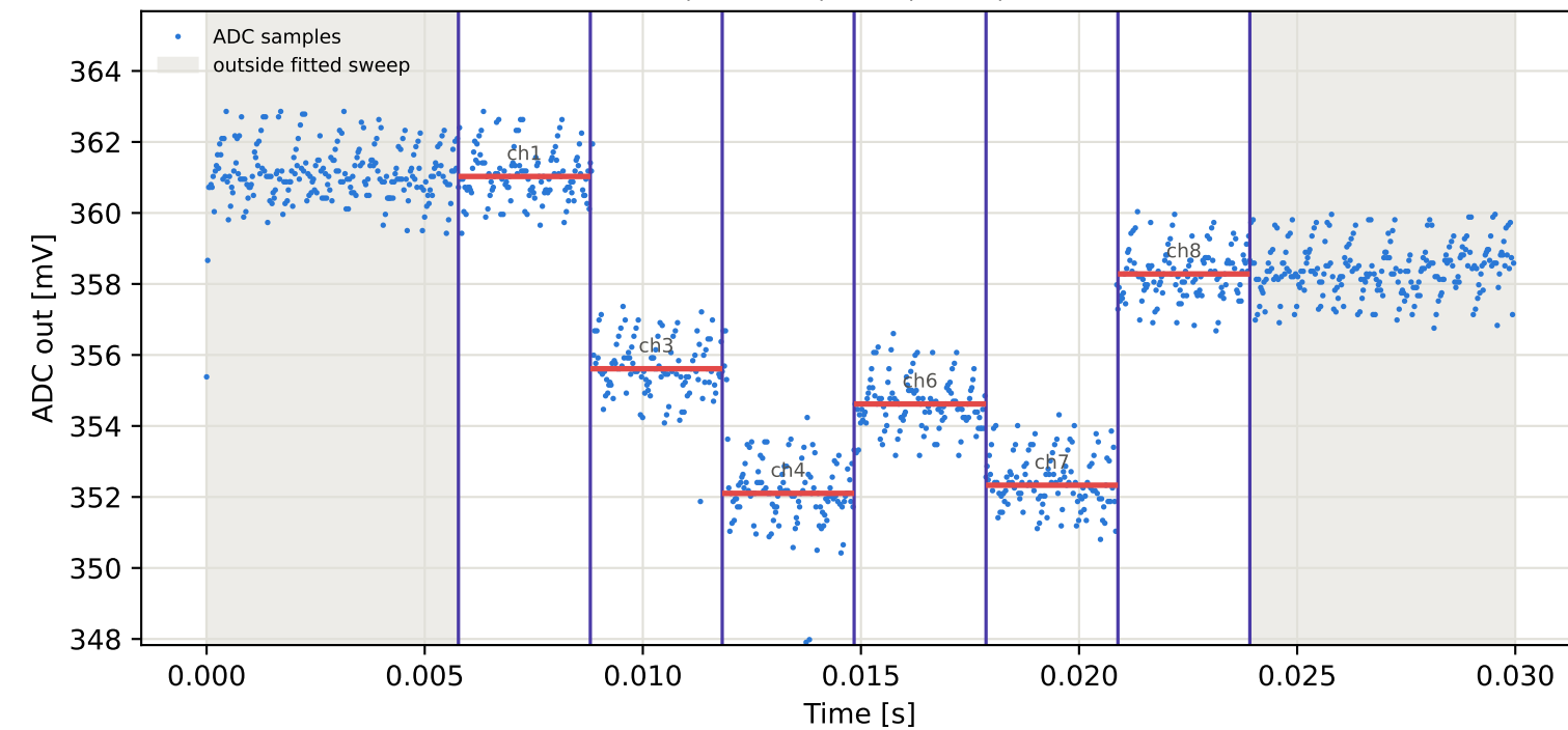
Tag16 &lt;- Tag6 | 845 MHz | run 0 | rep 1 | phase 84.20 deg
