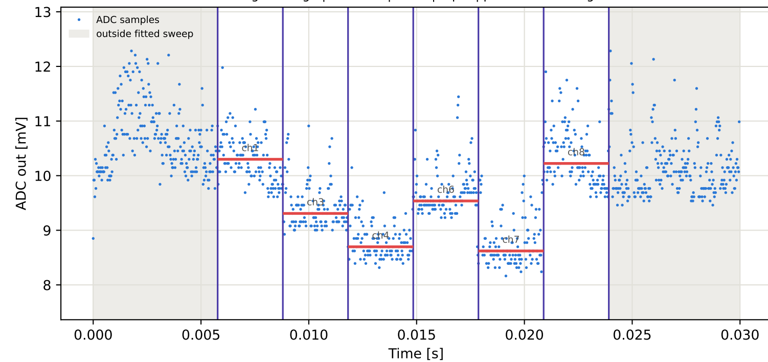
Tag3 &lt;- Tag10 | 795 MHz | run 0 | rep 1 | phase 139.93 deg
