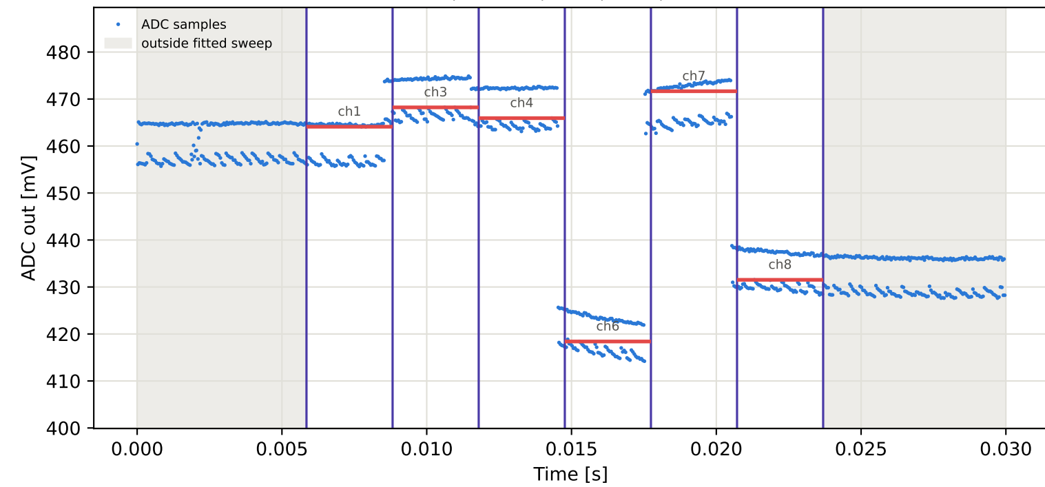
Tag7 &lt;- Tag5 | 915 MHz | run 0 | rep 1 | phase -5.74 deg
