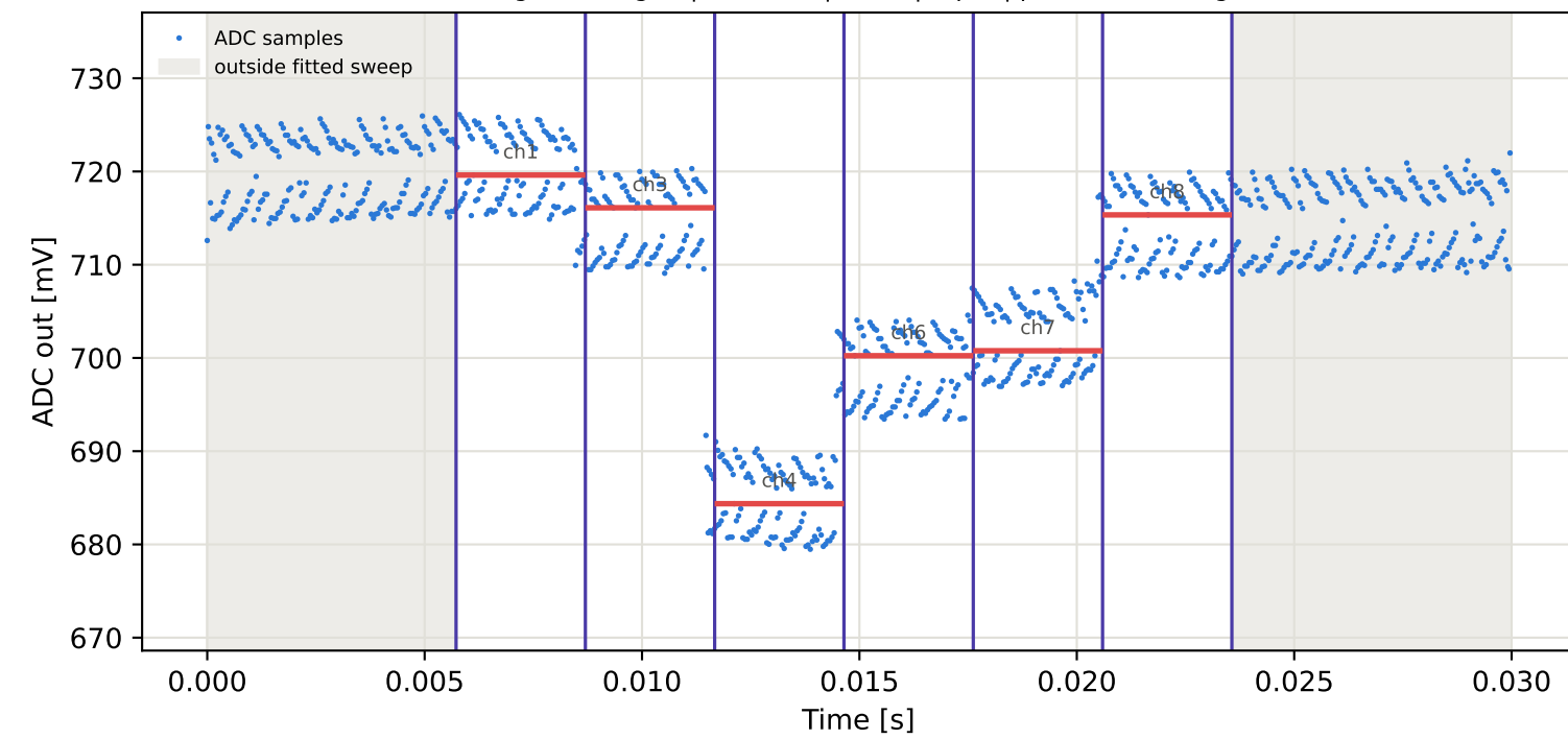
Tag15 &lt;- Tag3 | 975 MHz | run 0 | rep 1 | phase -4.73 deg
