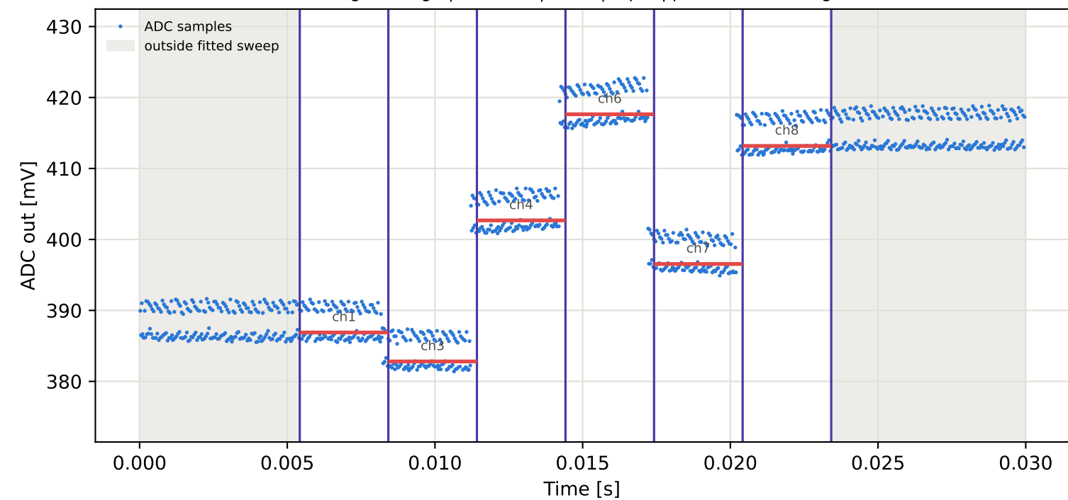
Tag3 &lt;- Tag9 | 855 MHz | run 0 | rep 1 | phase -151.91 deg
