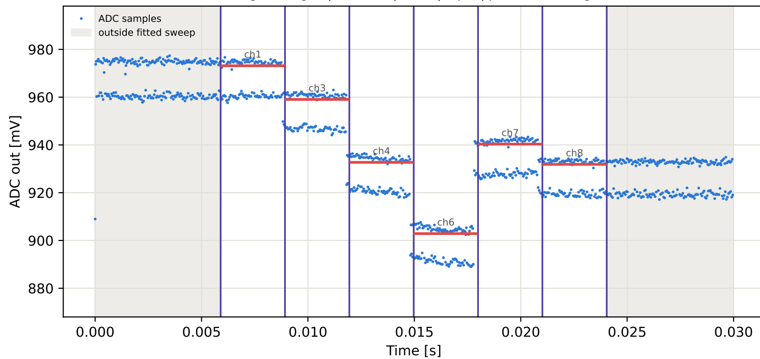
Tag6 &lt;- Tag2 | 885 MHz | run 0 | rep 1 | phase -56.93 deg
