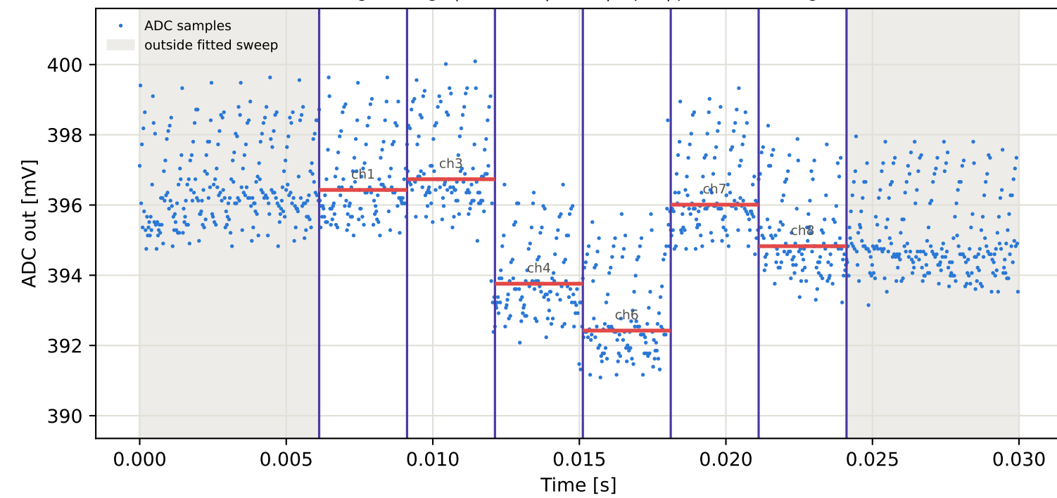
Tag9 &lt;- Tag10 | 995 MHz | run 0 | rep 1 | phase -77.64 deg
