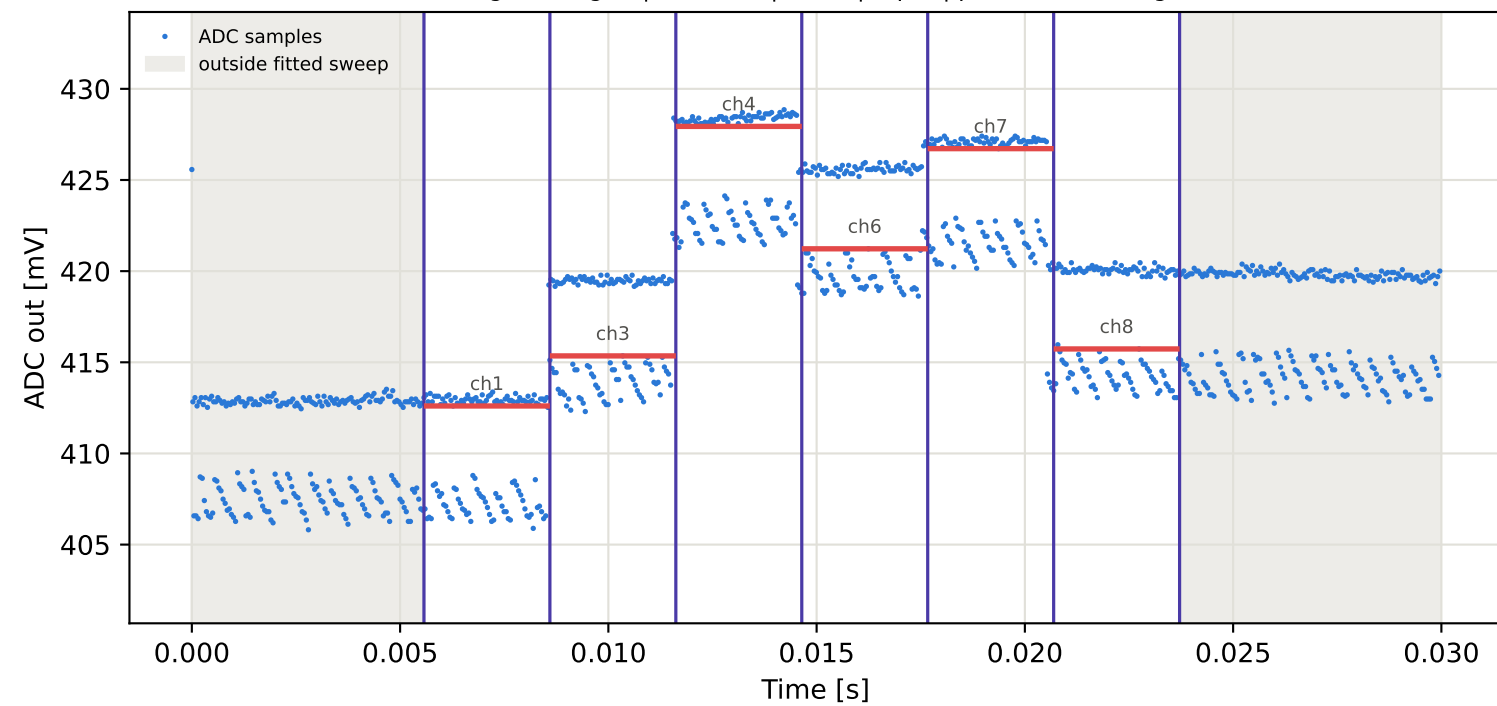
Tag4 &lt;- Tag16 | 835 MHz | run 0 | rep 1 | phase 6.46 deg
