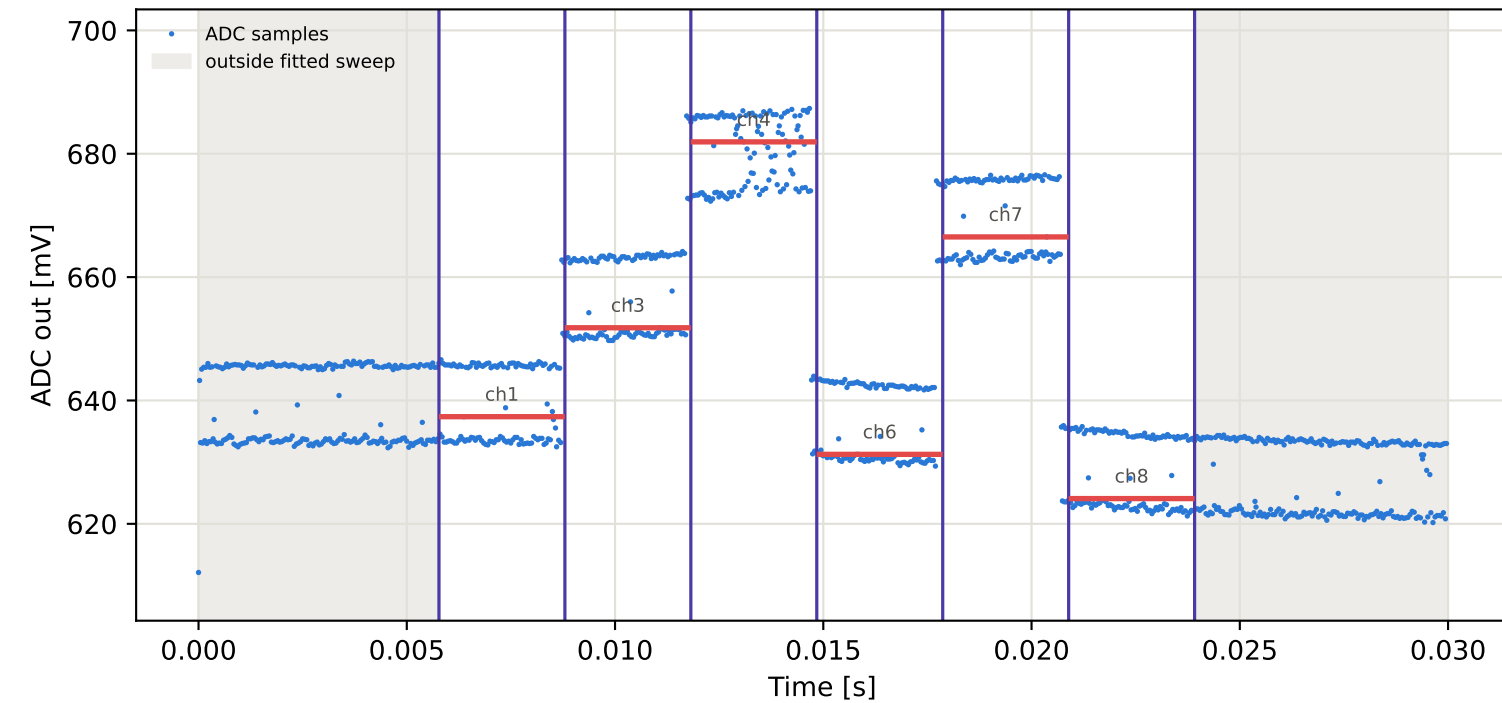
Tag5 &lt;- Tag3 | 945 MHz | run 0 | rep 1 | phase -132.86 deg
