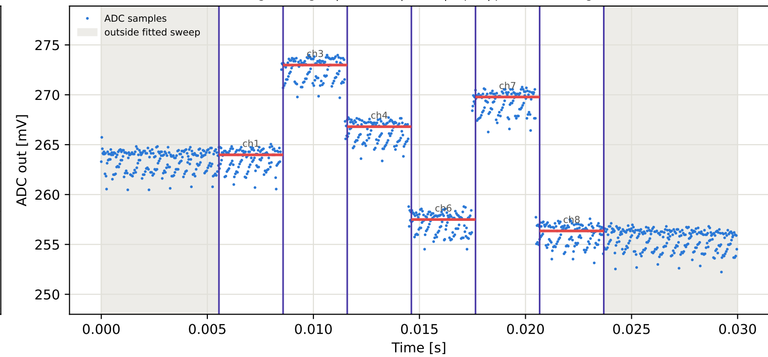
Tag4 &lt;- Tag16 | 845 MHz | run 0 | rep 1 | phase 98.68 deg
