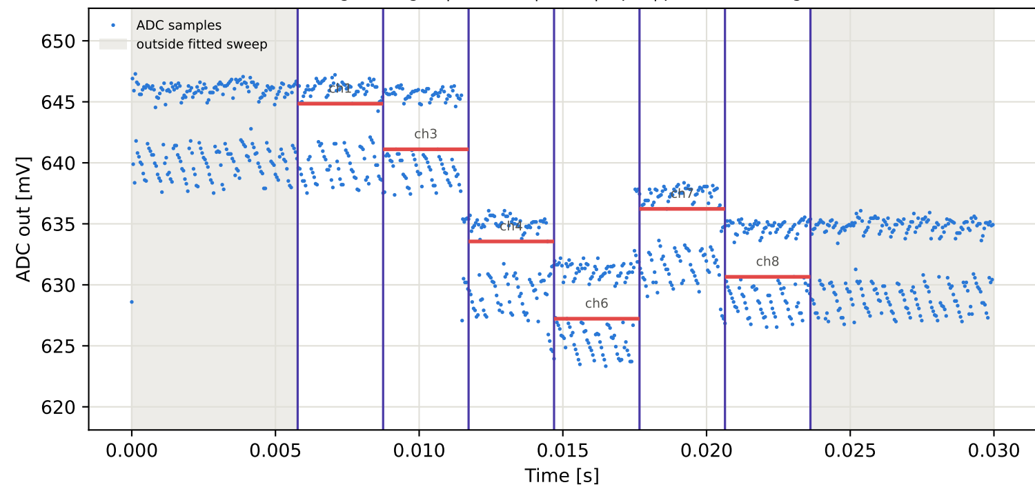
Tag6 &lt;- Tag2 | 855 MHz | run 0 | rep 1 | phase 179.95 deg
