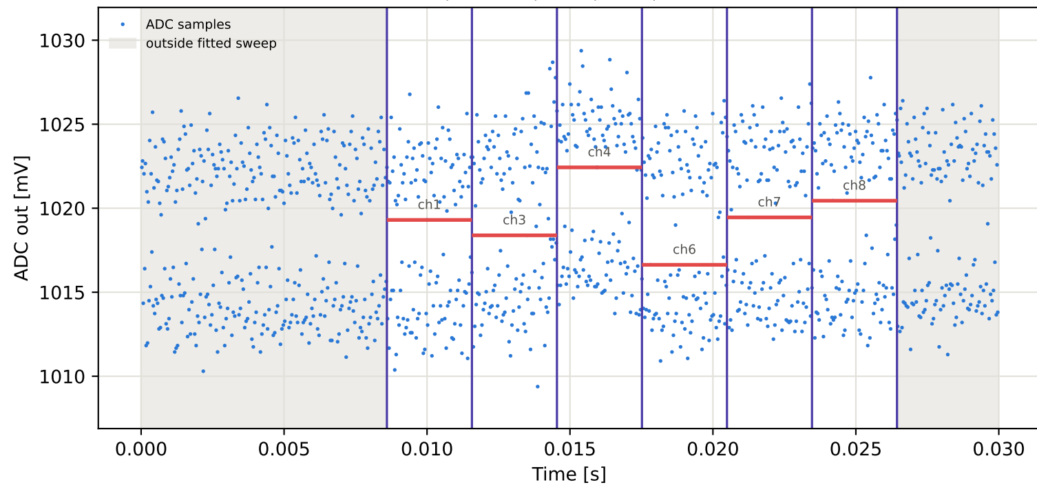
Tag3 &lt;- Tag2 | 885 MHz | run 0 | rep 1 | phase -62.50 deg
