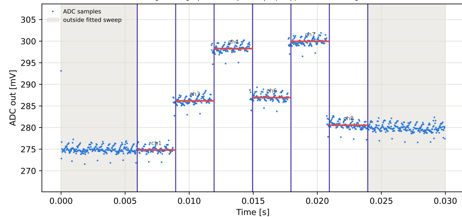
Tag6 &lt;- Tag1 | 835 MHz | run 0 | rep 1 | phase -84.84 deg
