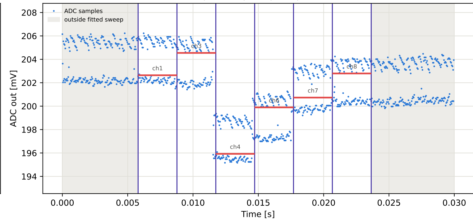
Tag7 &lt;- Tag6 | 995 MHz | run 0 | rep 1 | phase 51.77 deg
