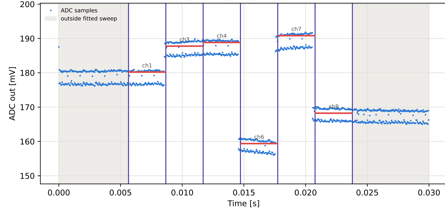
Tag3 &lt;- Tag8 | 975 MHz | run 0 | rep 1 | phase -20.56 deg
