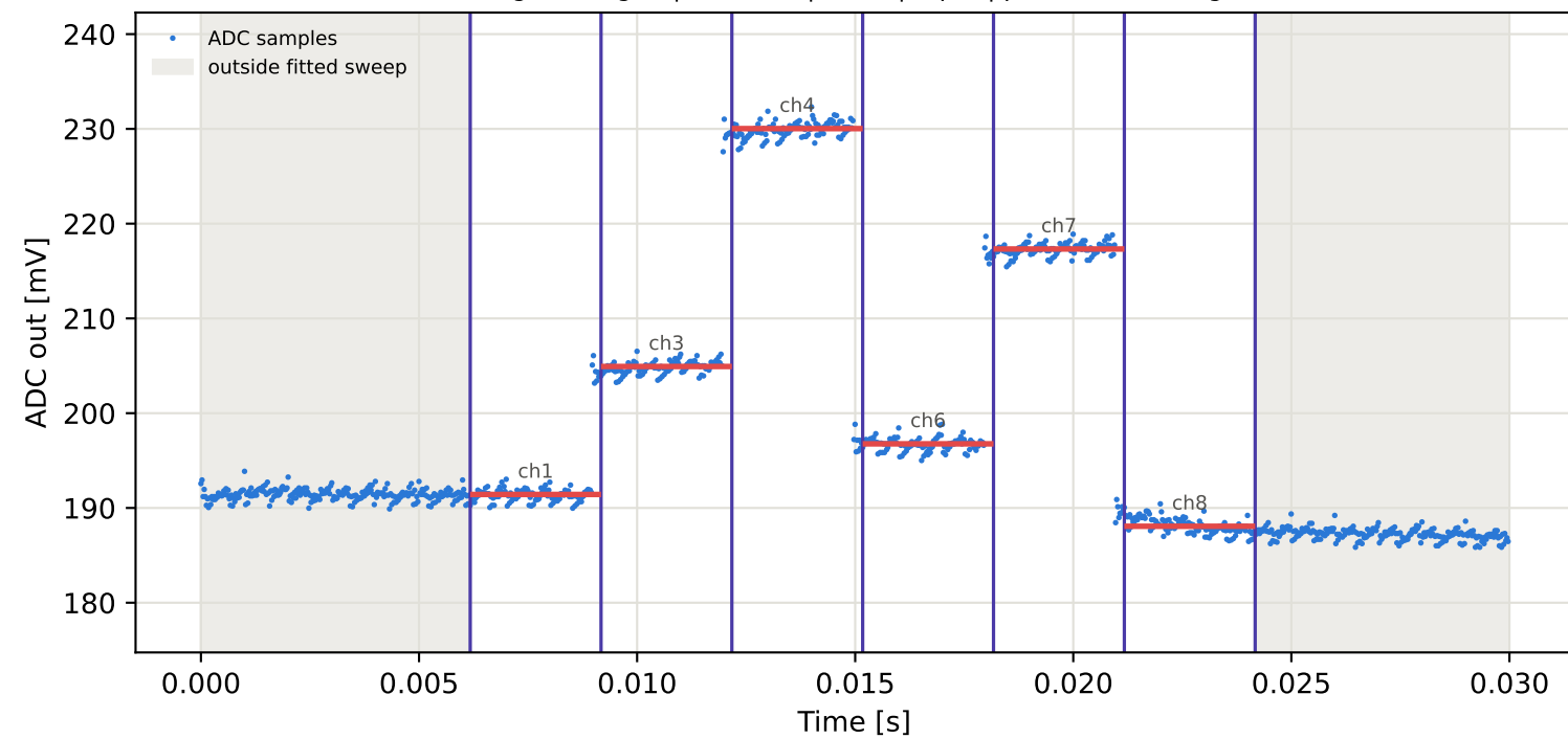
Tag5 &lt;- Tag2 | 995 MHz | run 0 | rep 1 | phase -8.25 deg
