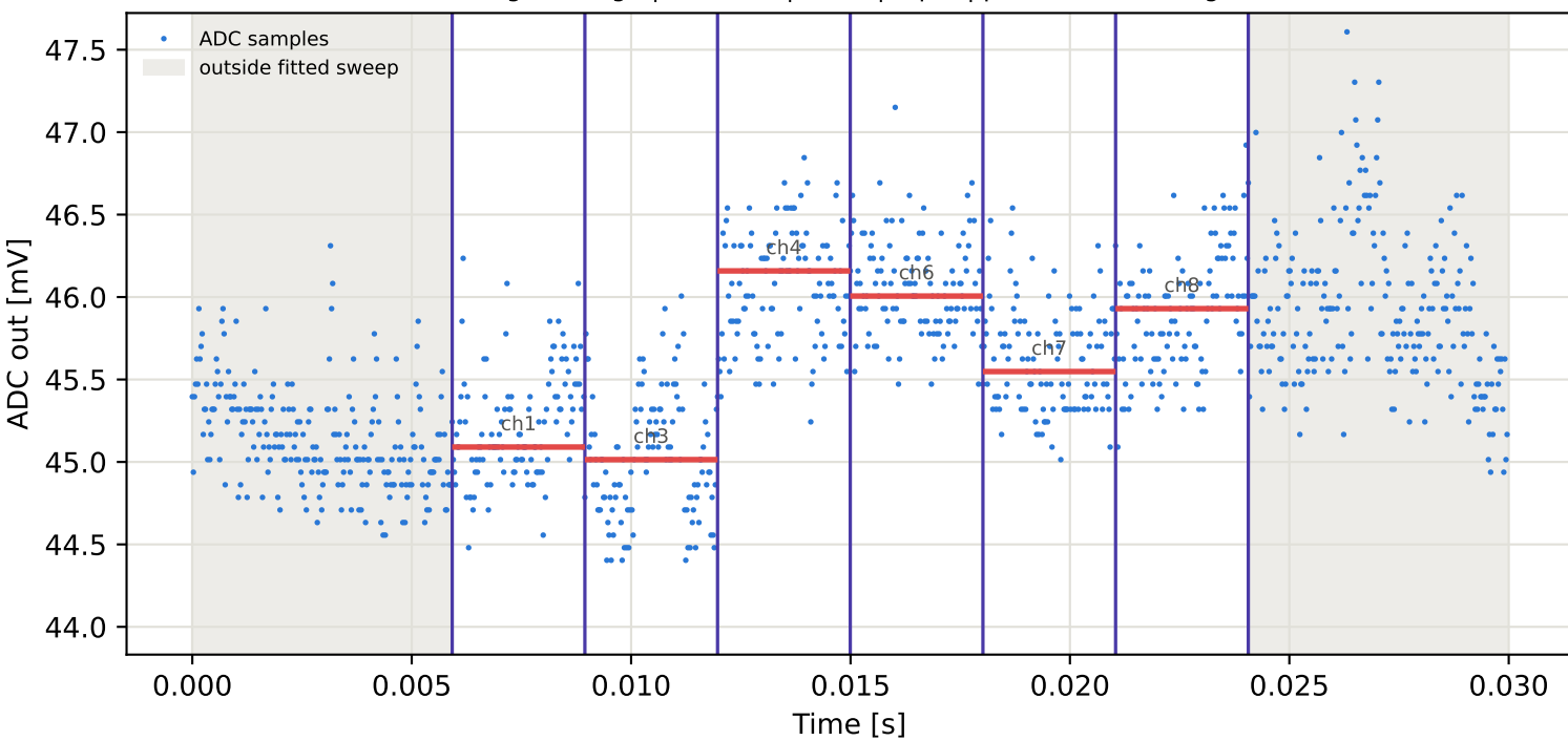
Tag8 &lt;- Tag15 | 775 MHz | run 0 | rep 1 | phase -165.19 deg
