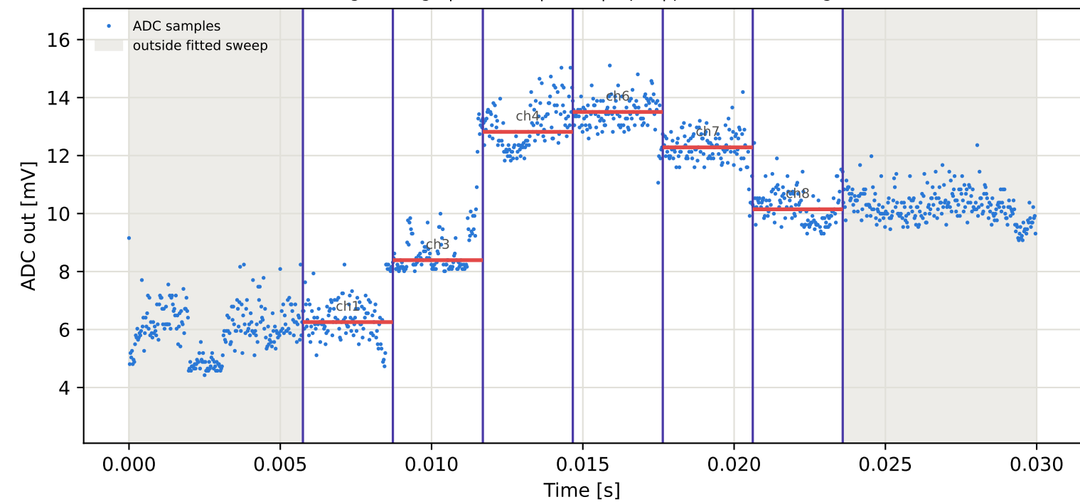
Tag2 &lt;- Tag6 | 855 MHz | run 0 | rep 1 | phase 49.61 deg
