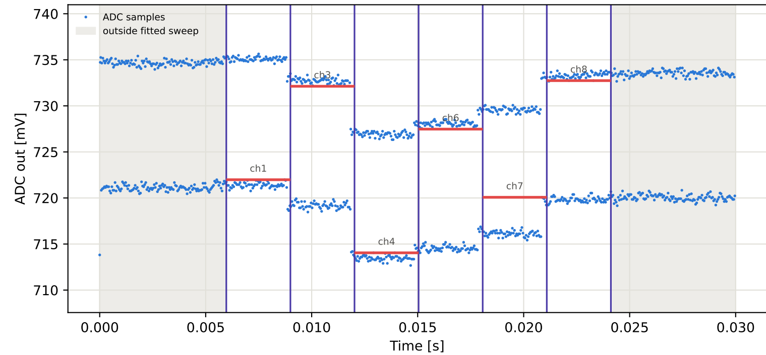
Tag7 &lt;- Tag15 | 945 MHz | run 0 | rep 1 | phase 116.18 deg
