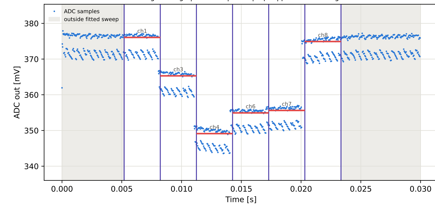
Tag6 &lt;- Tag1 | 915 MHz | run 0 | rep 1 | phase 69.65 deg
