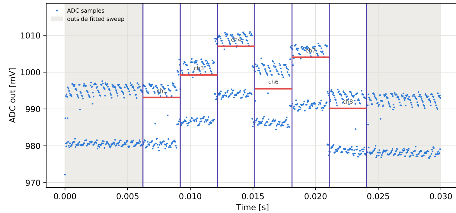
Tag4 &lt;- Tag9 | 935 MHz | run 0 | rep 1 | phase -80.63 deg
