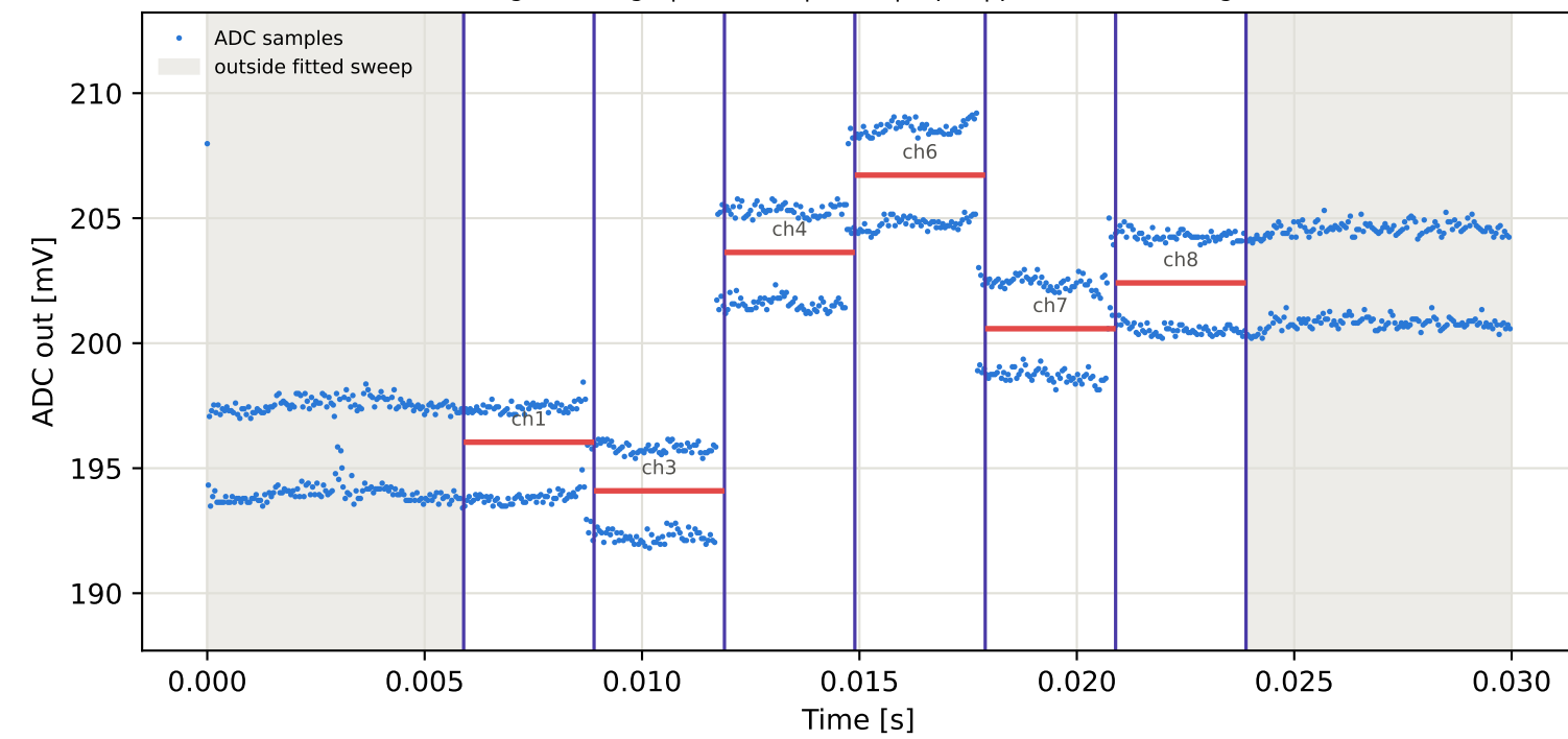
Tag15 &lt;- Tag9 | 805 MHz | run 0 | rep 1 | phase -172.69 deg
