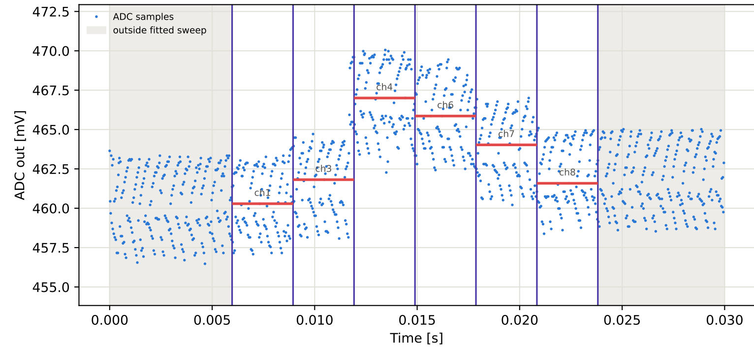
Tag16 &lt;- Tag15 | 975 MHz | run 0 | rep 1 | phase -68.46 deg
