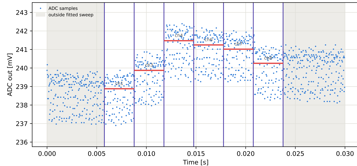
Tag1 &lt;- Tag9 | 845 MHz | run 0 | rep 1 | phase -114.68 deg
