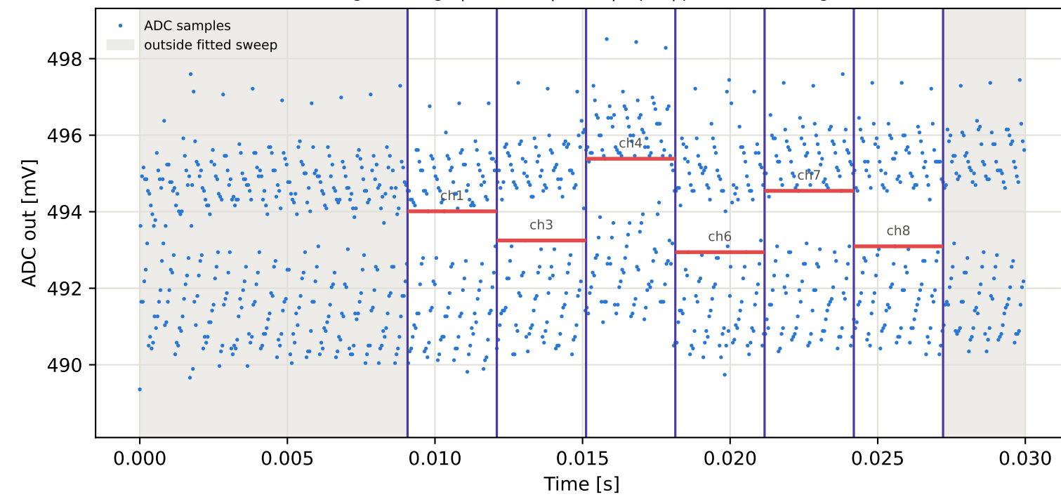
Tag16 &lt;- Tag4 | 855 MHz | run 0 | rep 1 | phase 86.25 deg
