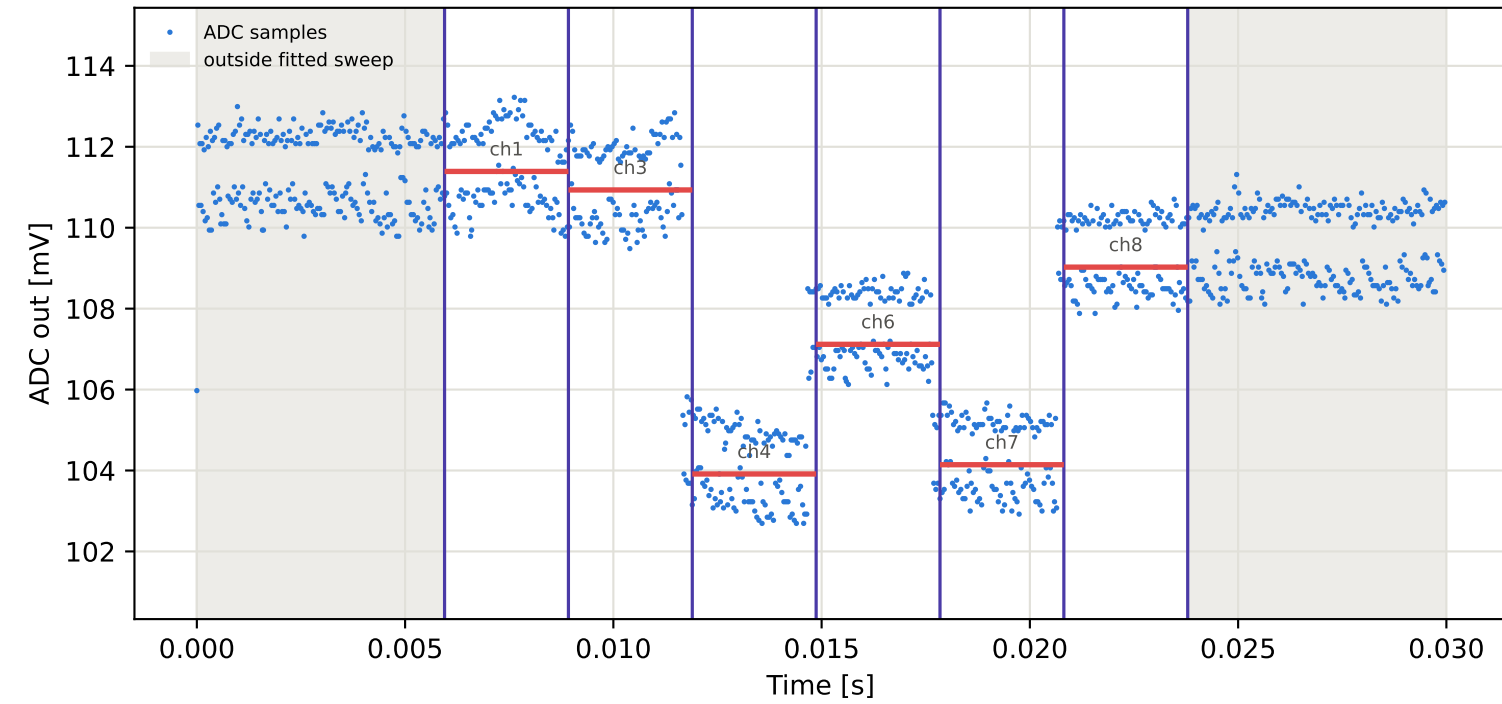
Tag8 &lt;- Tag16 | 795 MHz | run 0 | rep 1 | phase 82.40 deg
