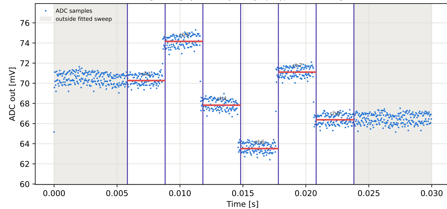
Tag1 &lt;- Tag7 | 805 MHz | run 0 | rep 1 | phase 89.16 deg
