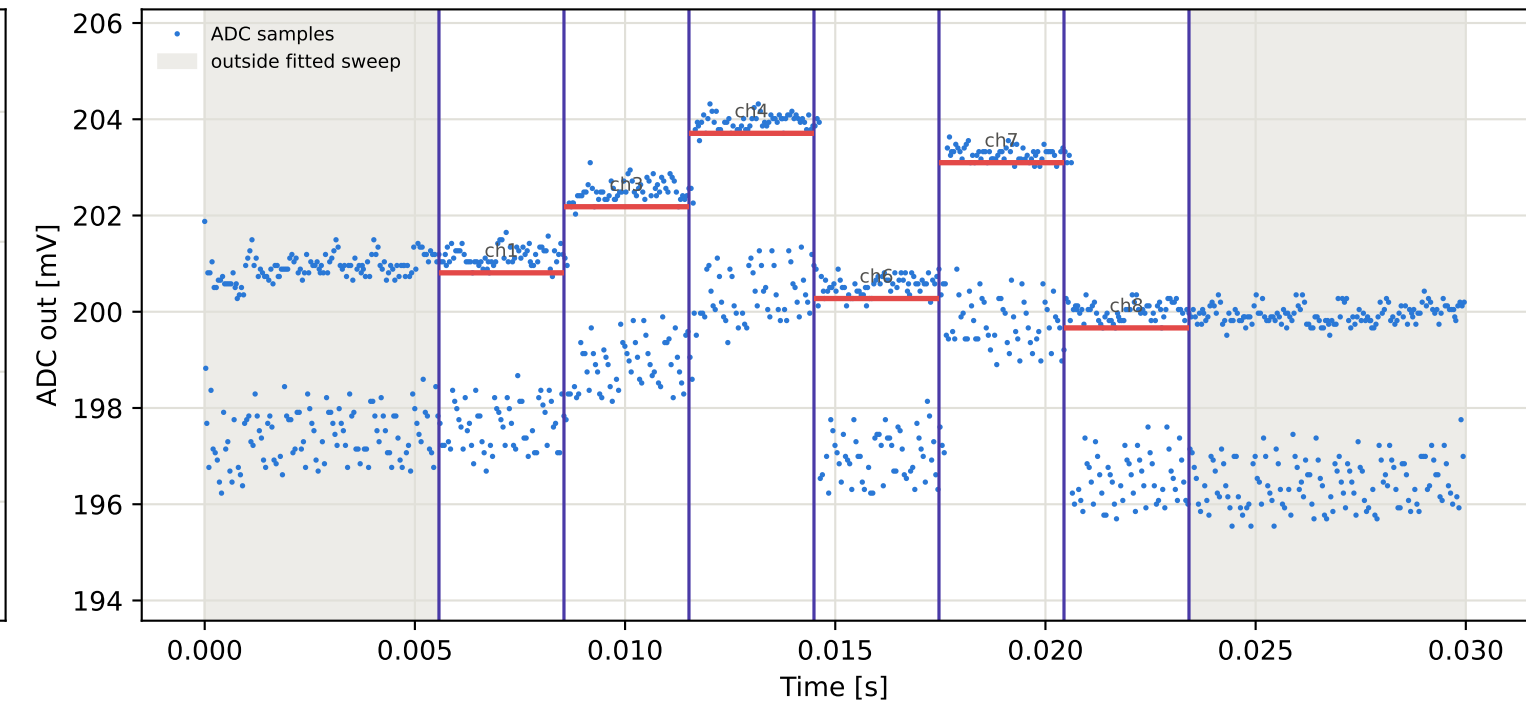
Tag1 &lt;- Tag4 | 965 MHz | run 0 | rep 1 | phase 105.94 deg
