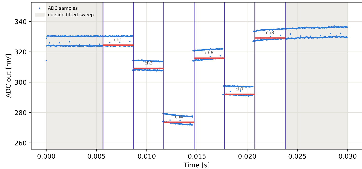
Tag5 &lt;- Tag1 | 965 MHz | run 0 | rep 1 | phase -120.16 deg
