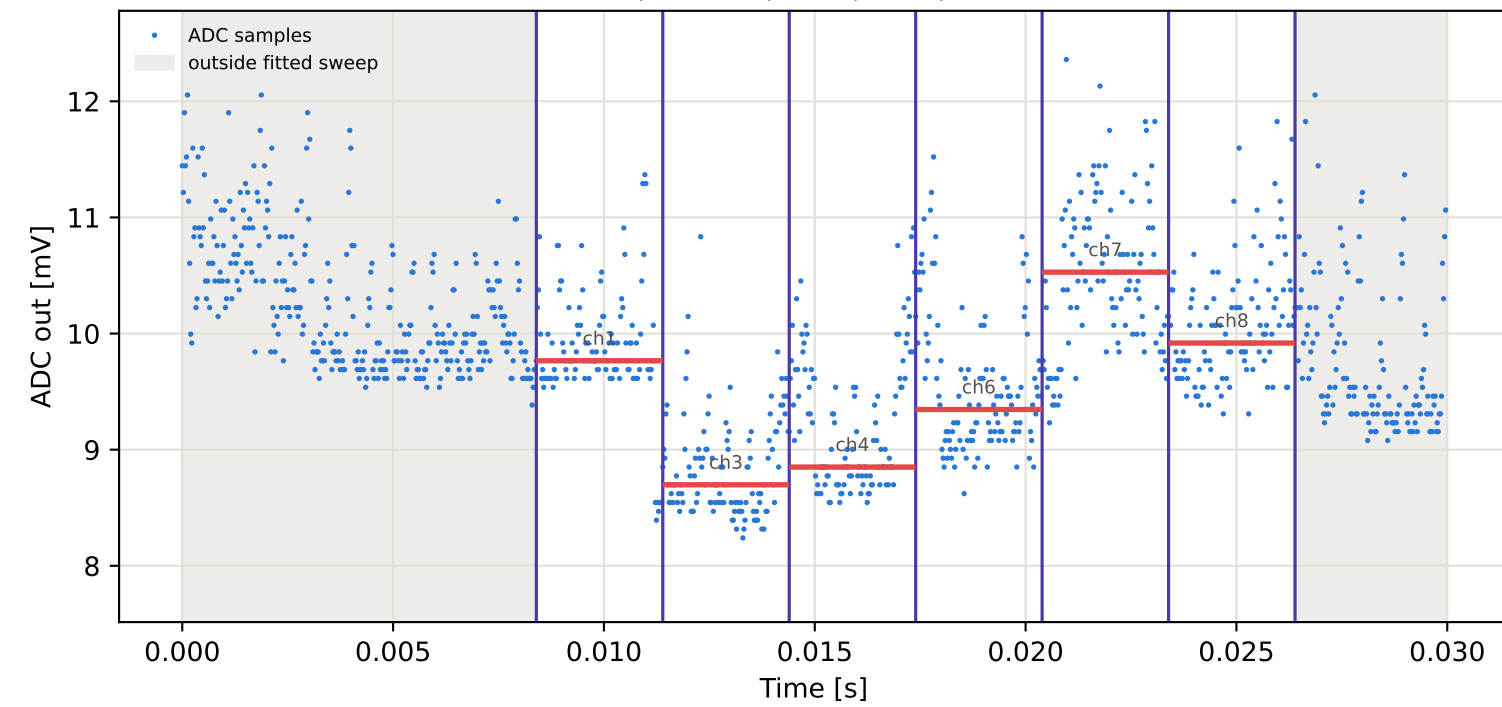
Tag2 &lt;- Tag7 | 795 MHz | run 0 | rep 1 | phase 90.75 deg
