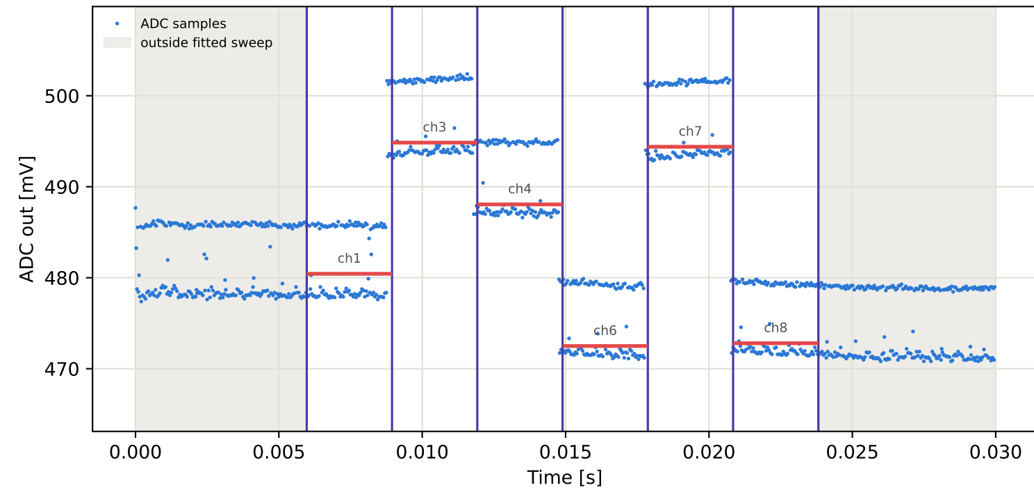
Tag8 &lt;- Tag7 | 825 MHz | run 0 | rep 1 | phase -81.41 deg
