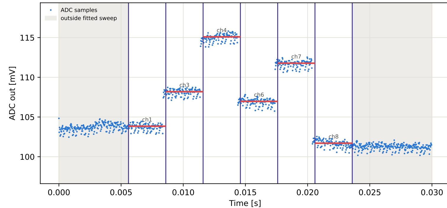
Tag1 &lt;- Tag3 | 935 MHz | run 0 | rep 1 | phase -88.49 deg
