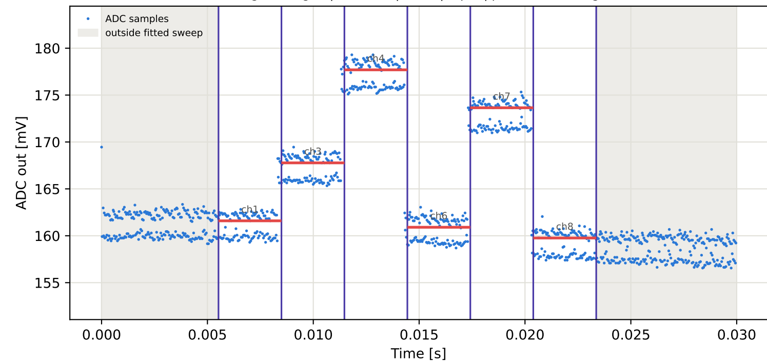
Tag6 &lt;- Tag3 | 995 MHz | run 0 | rep 1 | phase -39.00 deg
