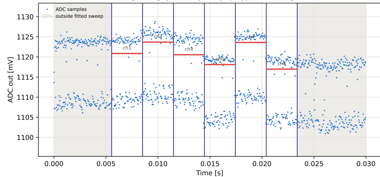
Tag8 &lt;- Tag15 | 885 MHz | run 0 | rep 1 | phase -31.41 deg
