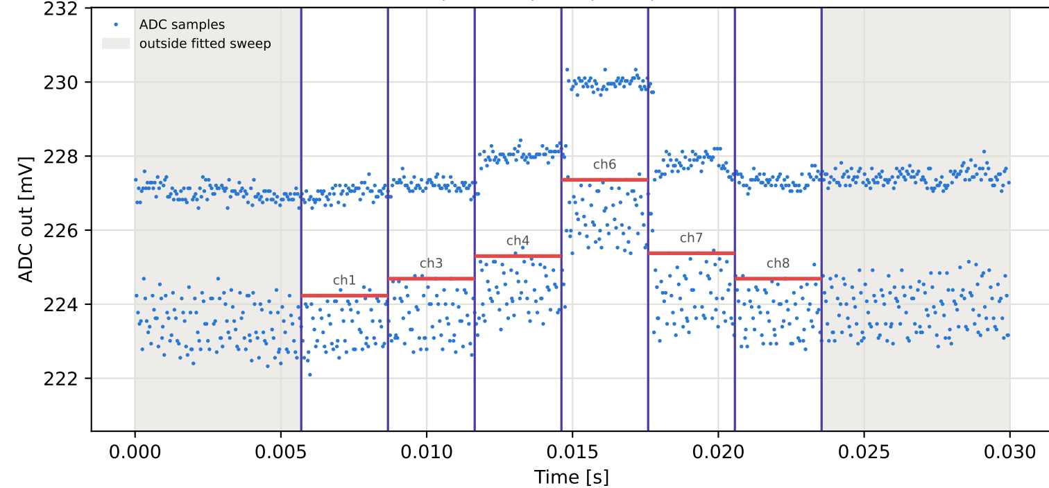
Tag3 &lt;- Tag2 | 955 MHz | run 0 | rep 1 | phase -151.63 deg
