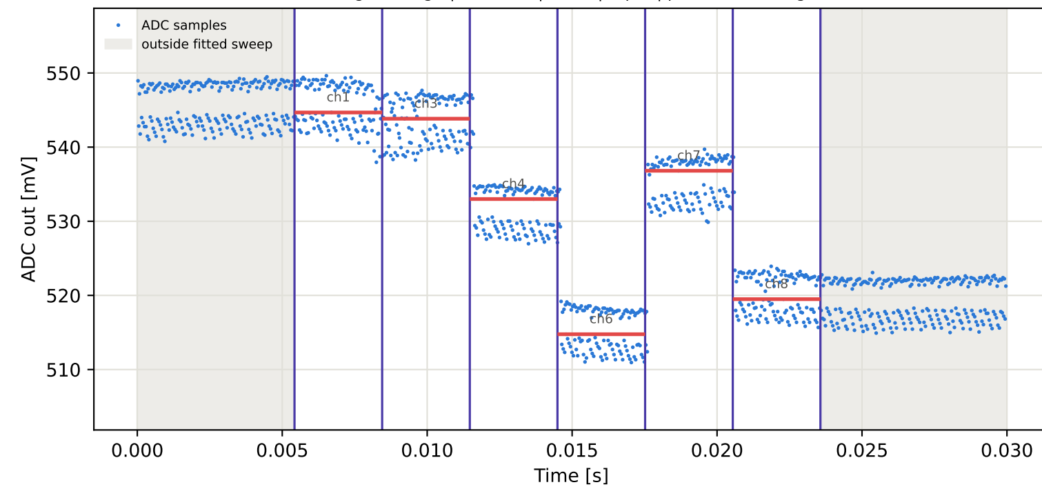
Tag1 &lt;- Tag7 | 875 MHz | run 0 | rep 1 | phase 99.95 deg
