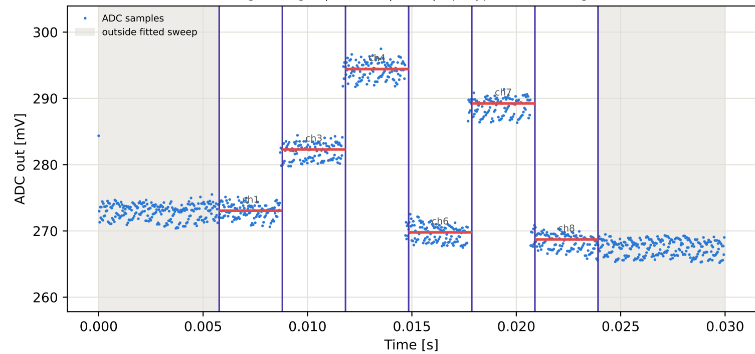
Tag6 &lt;- Tag3 | 985 MHz | run 0 | rep 1 | phase -39.39 deg
