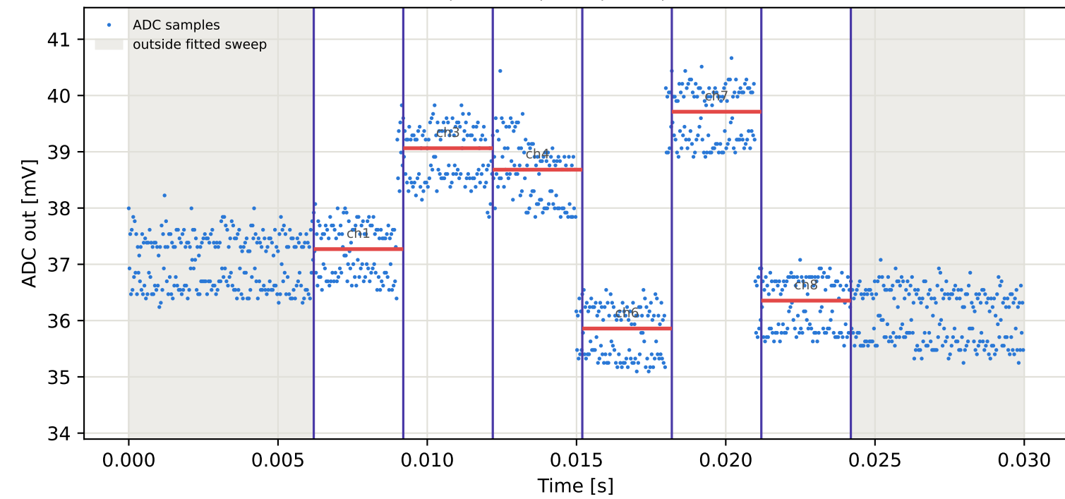
Tag4 &lt;- Tag9 | 775 MHz | run 0 | rep 1 | phase -12.73 deg
