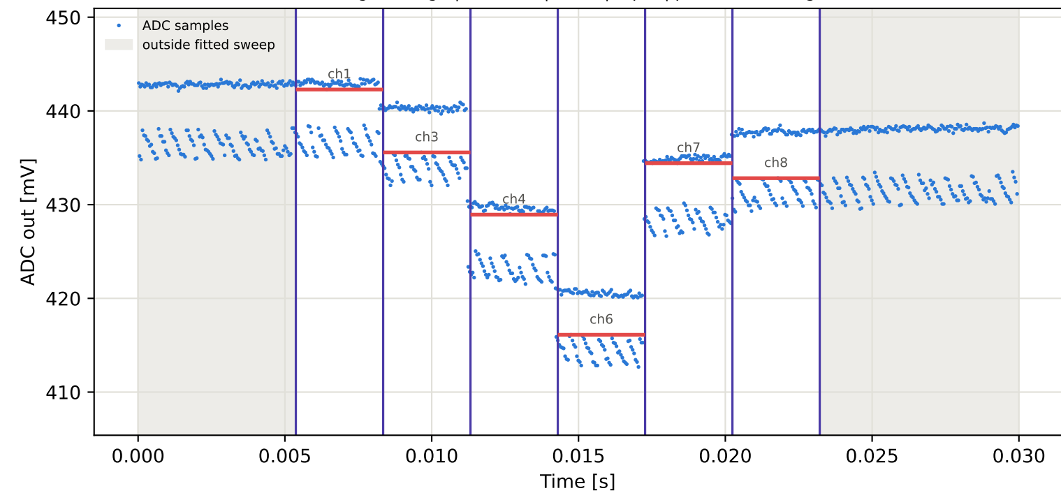
Tag9 &lt;- Tag6 | 935 MHz | run 0 | rep 1 | phase -52.00 deg
