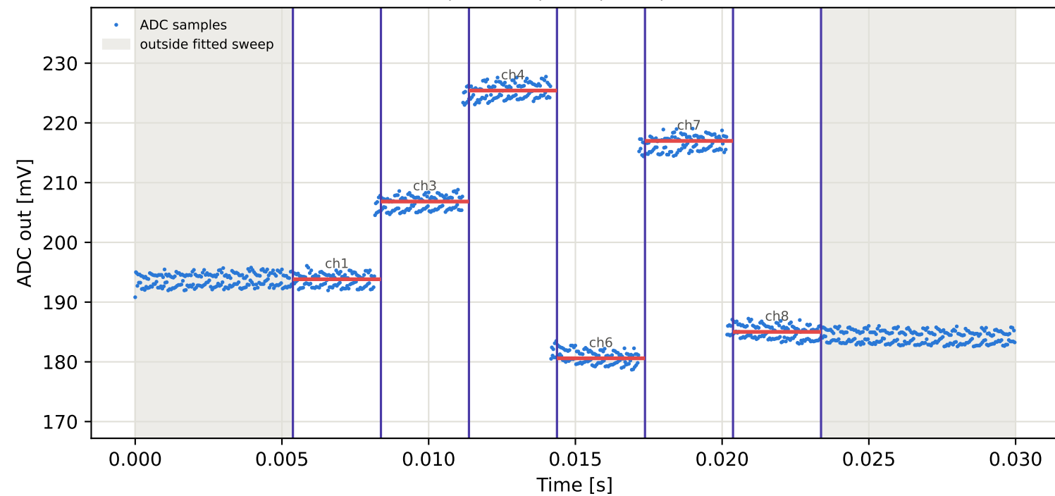
Tag5 &lt;- Tag4 | 995 MHz | run 0 | rep 1 | phase -61.14 deg
