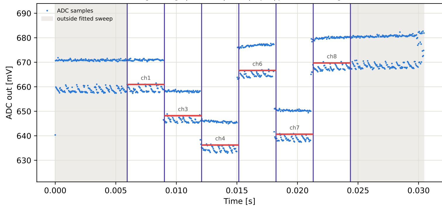
Tag5 &lt;- Tag9 | 945 MHz | run 0 | rep 1 | phase -57.82 deg
