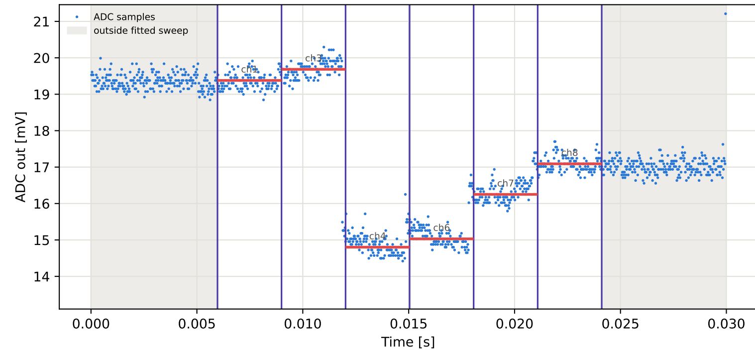
Tag3 &lt;- Tag8 | 795 MHz | run 0 | rep 1 | phase 121.78 deg
