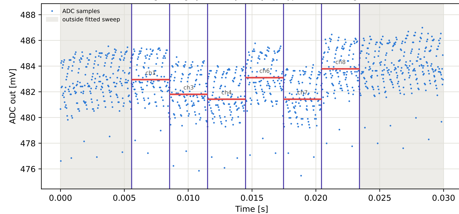
Tag6 &lt;- Tag9 | 845 MHz | run 0 | rep 1 | phase -169.37 deg
