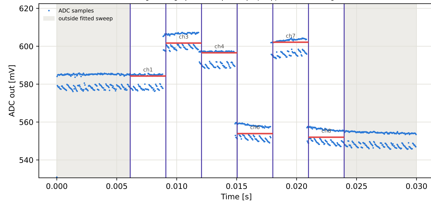
Tag9 &lt;- Tag7 | 875 MHz | run 0 | rep 1 | phase -15.26 deg
