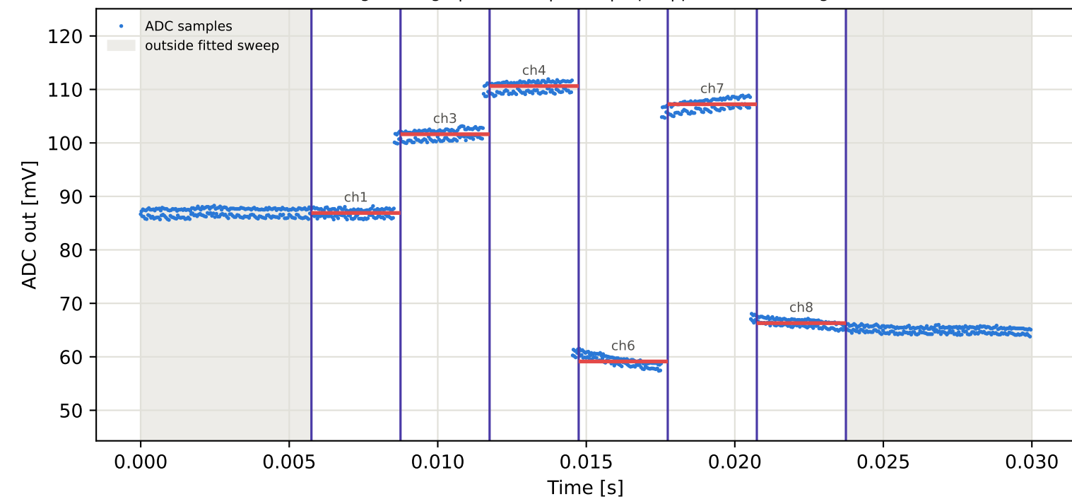
Tag3 &lt;- Tag8 | 925 MHz | run 0 | rep 1 | phase -87.49 deg
