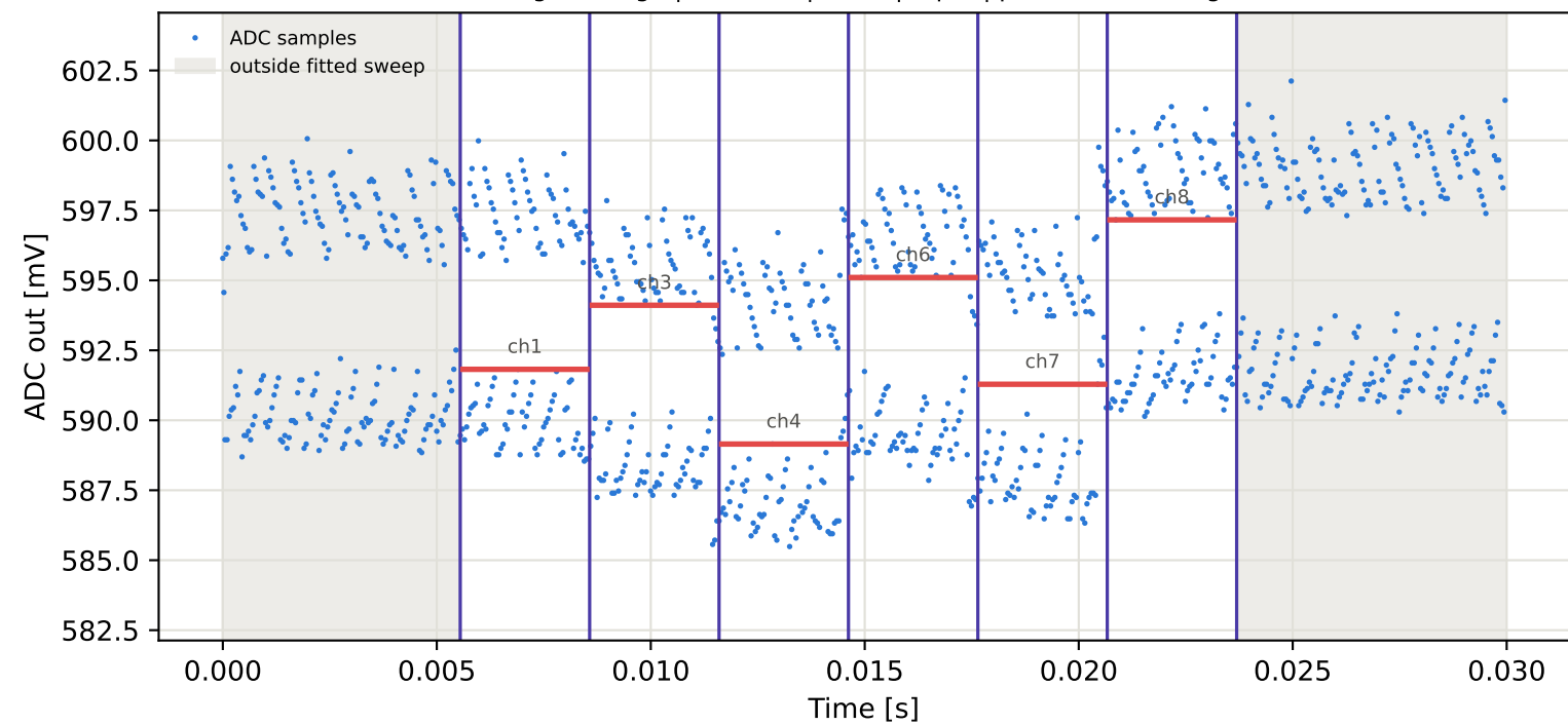
Tag5 &lt;- Tag4 | 925 MHz | run 0 | rep 1 | phase 93.08 deg
