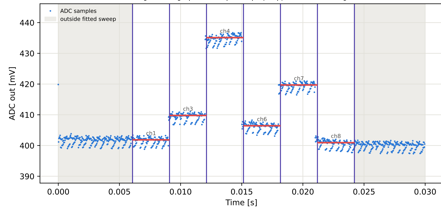
Tag15 &lt;- Tag5 | 995 MHz | run 0 | rep 1 | phase -100.70 deg
