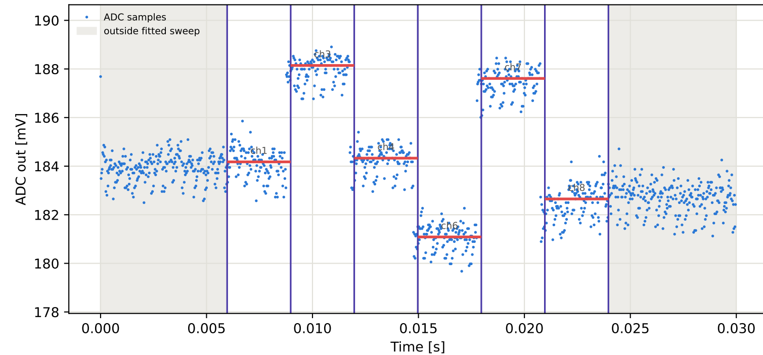
Tag6 &lt;- Tag1 | 775 MHz | run 0 | rep 1 | phase -174.92 deg
