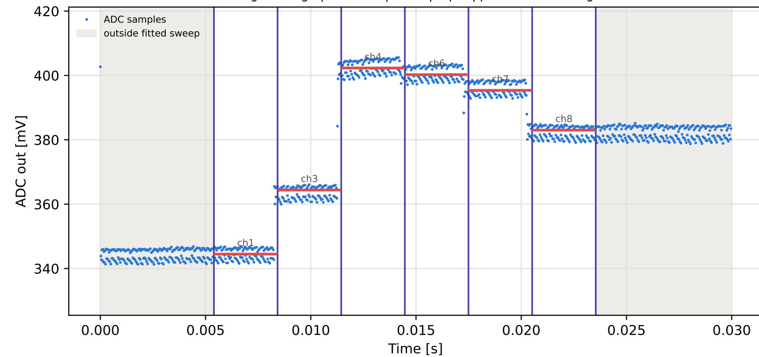
Tag3 &lt;- Tag6 | 835 MHz | run 0 | rep 1 | phase 123.45 deg
