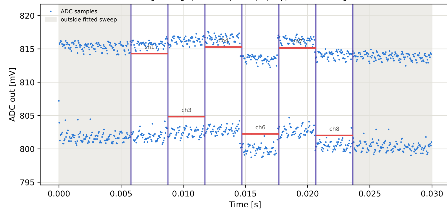
Tag8 &lt;- Tag4 | 935 MHz | run 0 | rep 1 | phase 134.56 deg
