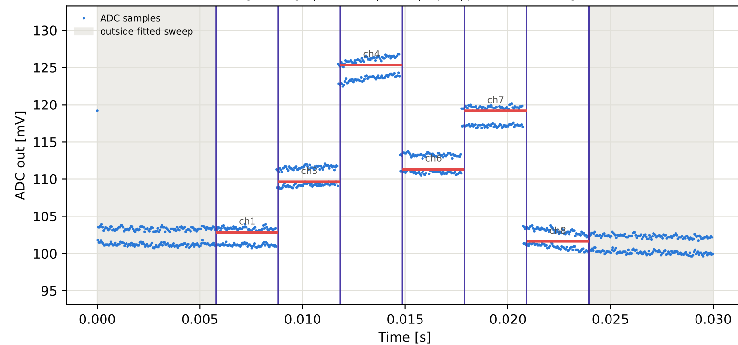
Tag1 &lt;- Tag9 | 945 MHz | run 0 | rep 1 | phase 168.41 deg
