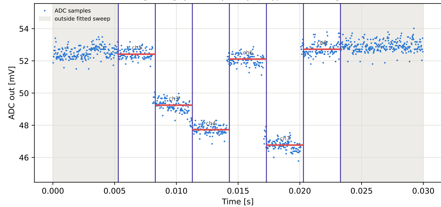
Tag1 &lt;- Tag8 | 775 MHz | run 0 | rep 1 | phase 81.94 deg
