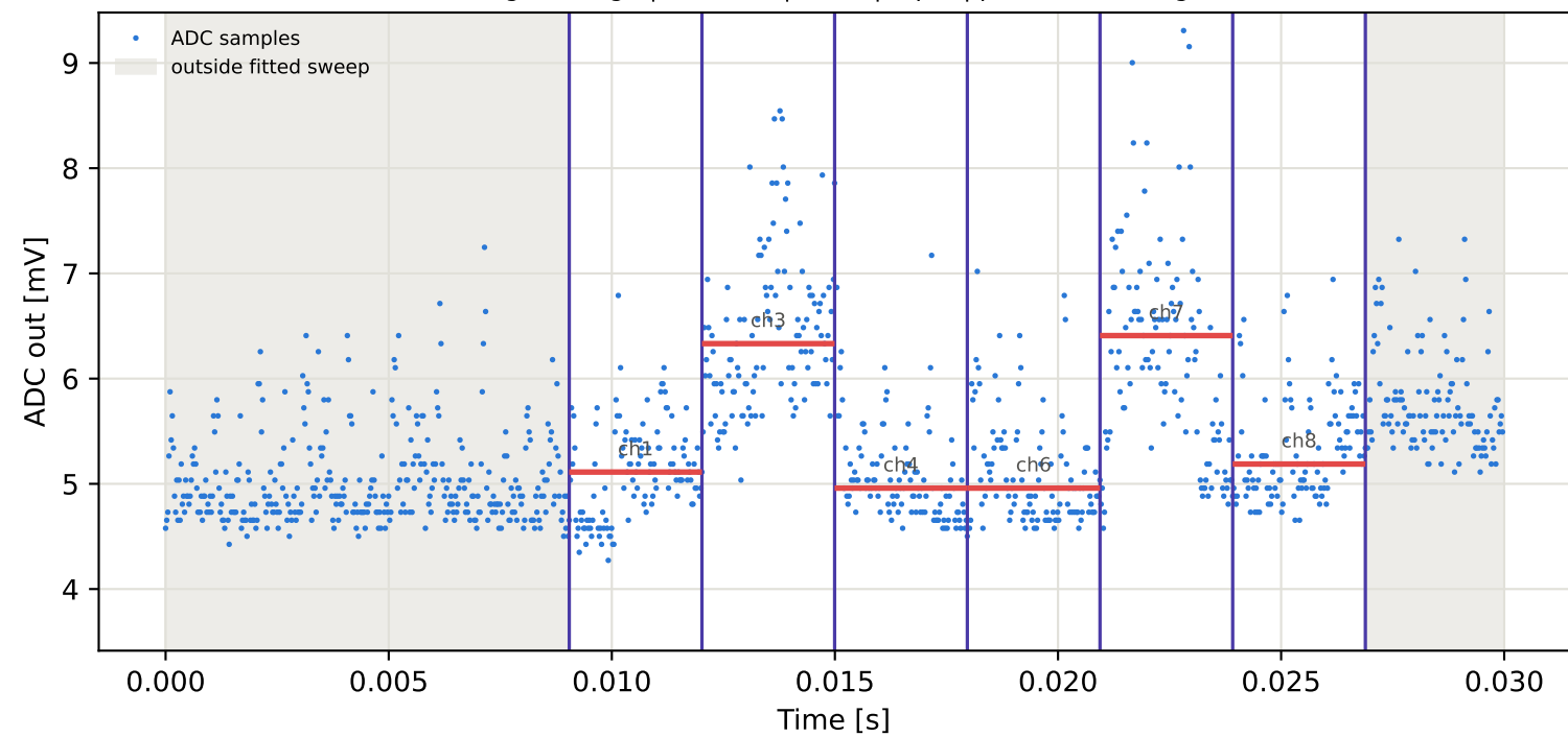
Tag2 &lt;- Tag5 | 775 MHz | run 0 | rep 1 | phase -174.29 deg
