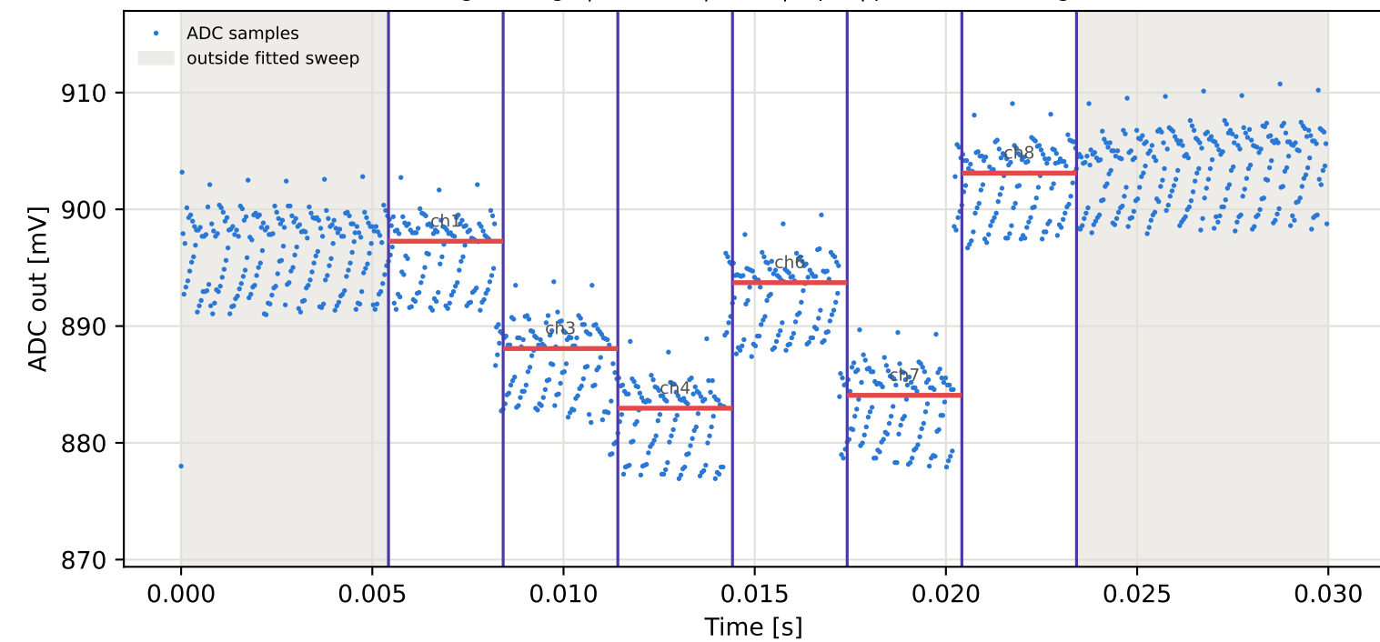
Tag4 &lt;- Tag15 | 895 MHz | run 0 | rep 1 | phase -115.27 deg
