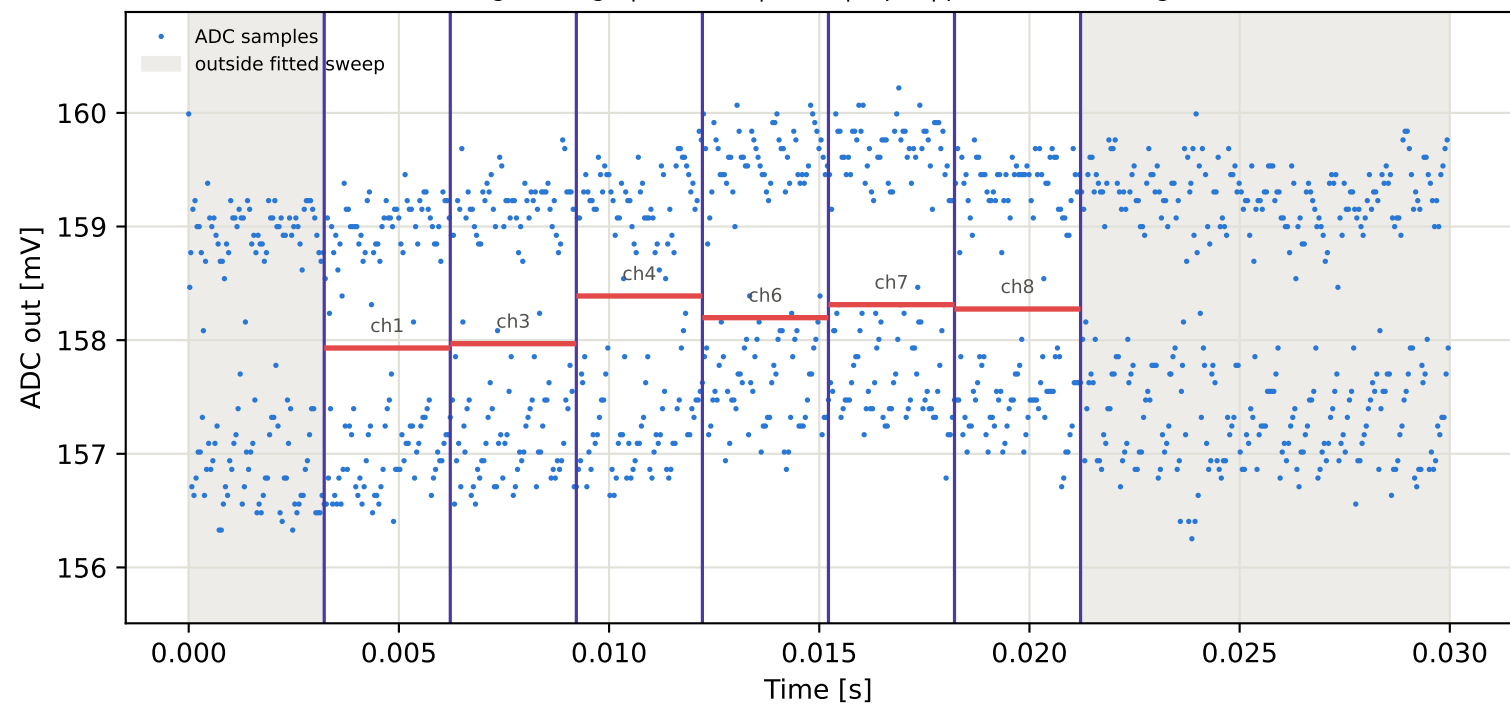
Tag7 &lt;- Tag4 | 845 MHz | run 0 | rep 1 | phase -113.55 deg
