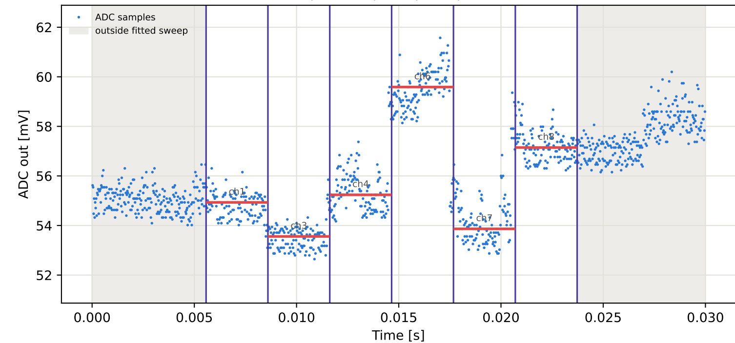
Tag2 &lt;- Tag16 | 975 MHz | run 0 | rep 1 | phase -179.39 deg
