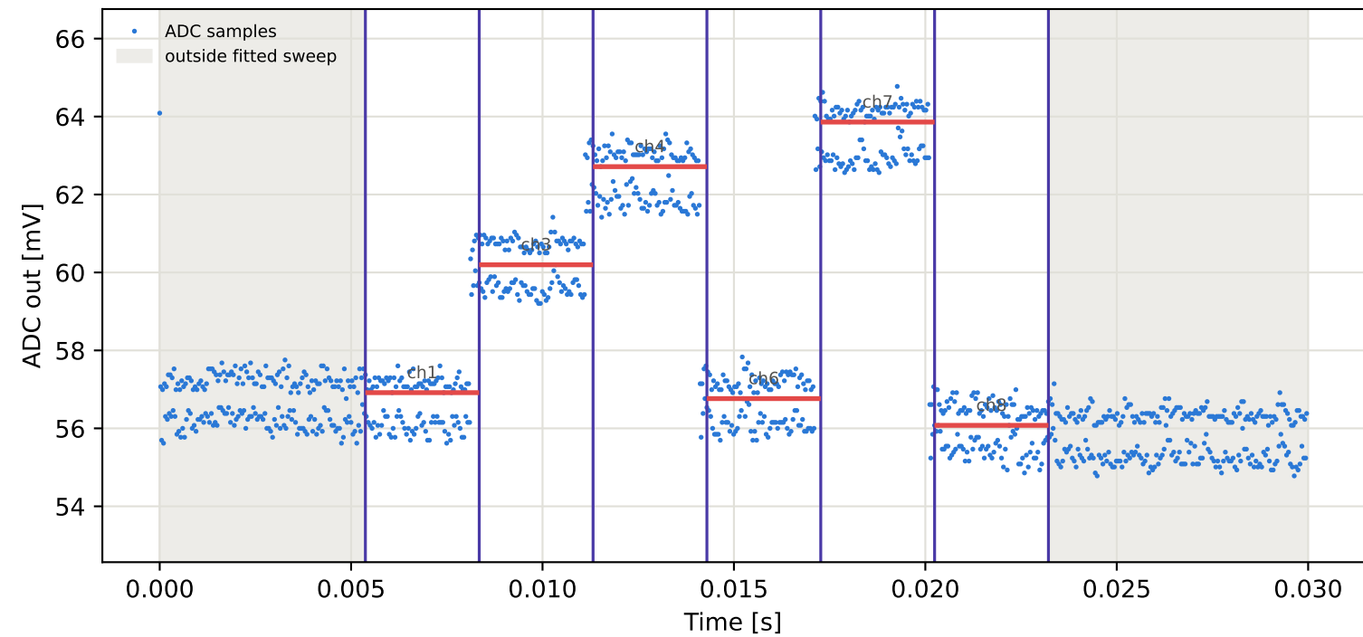
Tag2 &lt;- Tag10 | 785 MHz | run 0 | rep 1 | phase 16.51 deg
