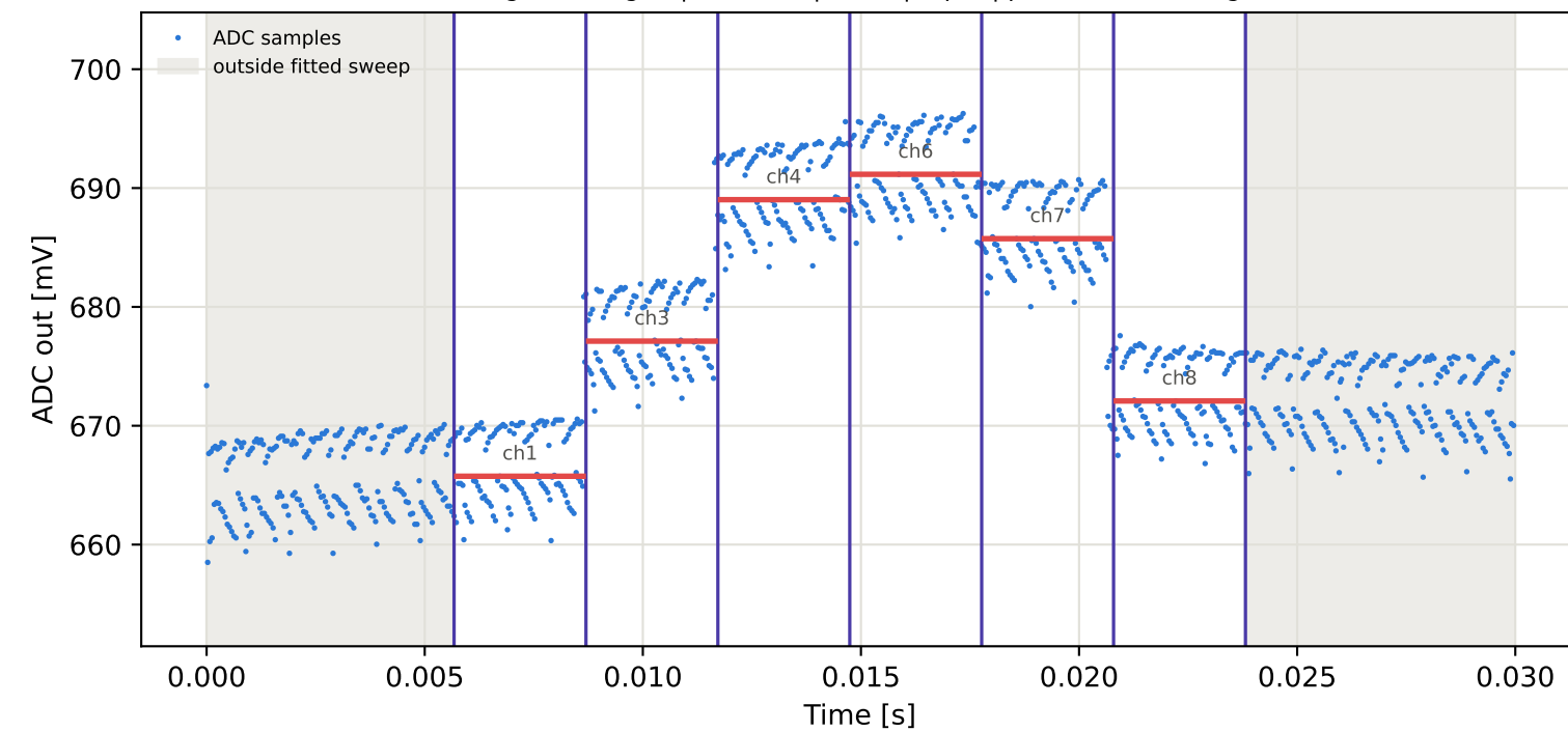
Tag10 &lt;- Tag2 | 895 MHz | run 0 | rep 1 | phase -69.64 deg
