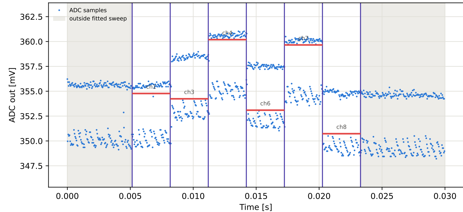
Tag5 &lt;- Tag4 | 825 MHz | run 0 | rep 1 | phase -63.70 deg
