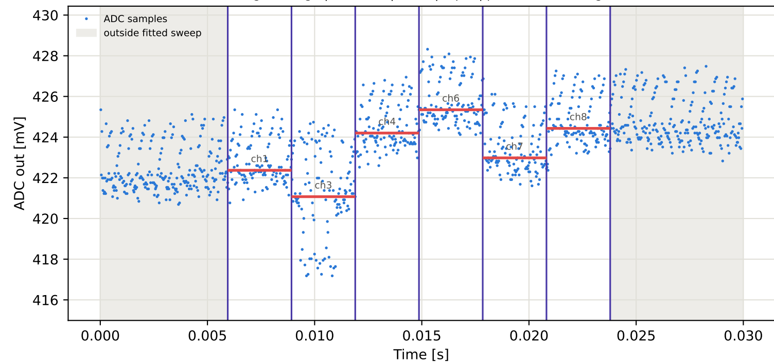
Tag4 &lt;- Tag8 | 835 MHz | run 0 | rep 1 | phase -36.26 deg
