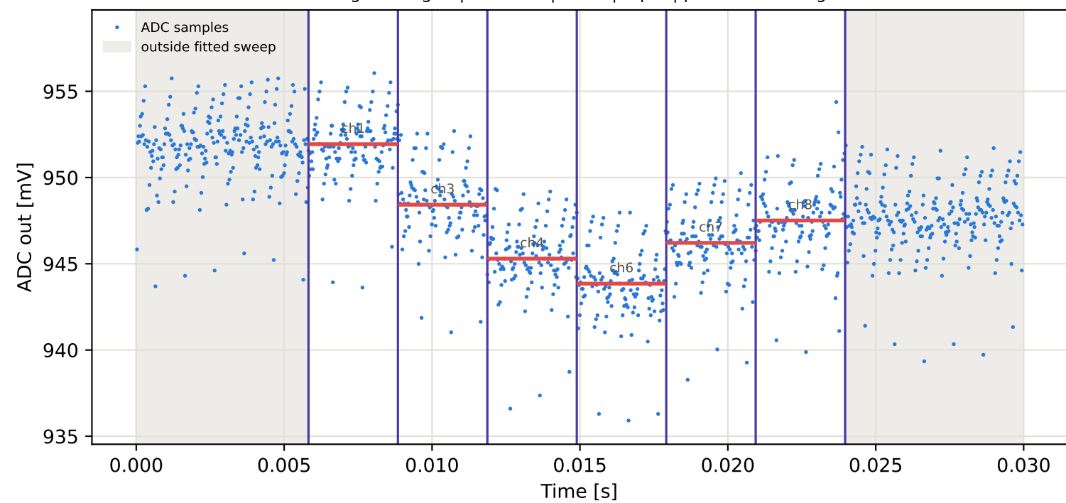
Tag4 &lt;- Tag16 | 875 MHz | run 0 | rep 1 | phase -126.56 deg
