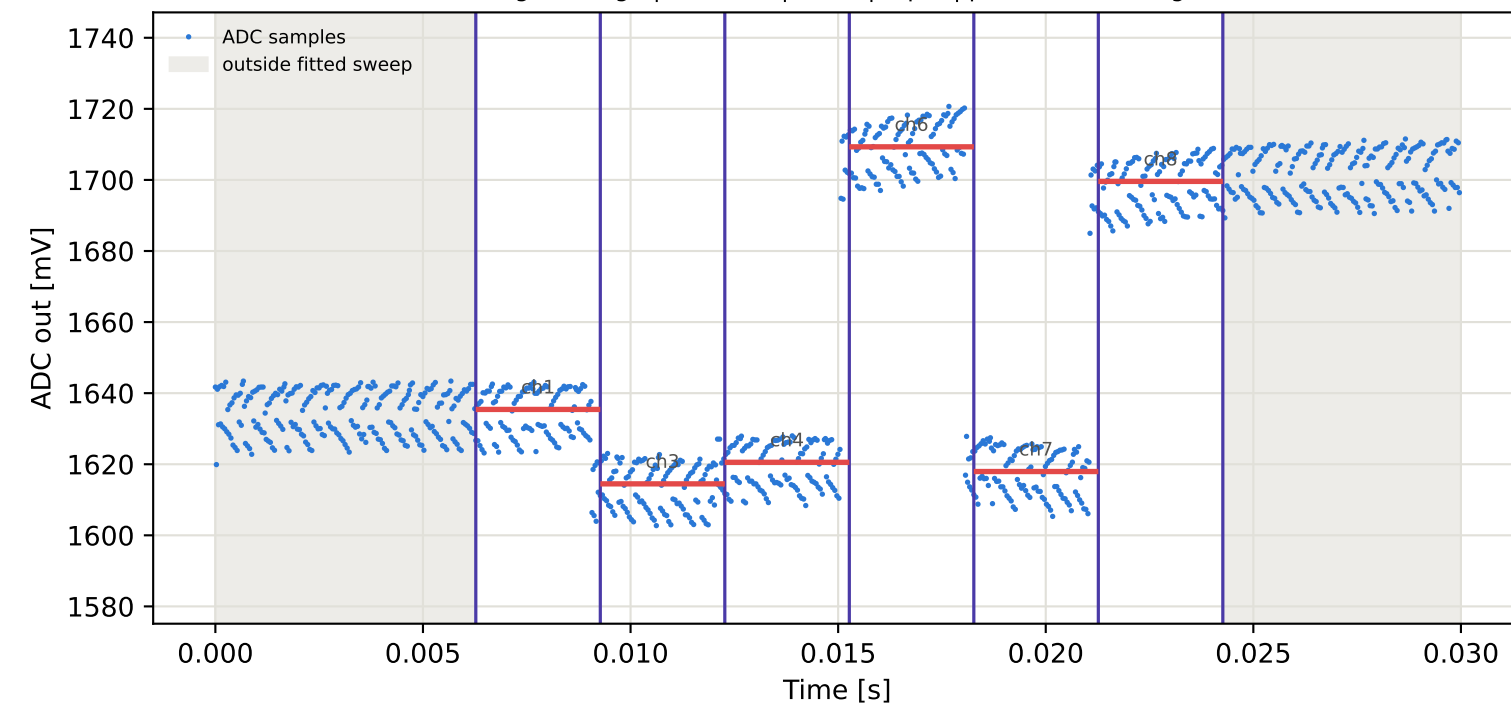
Tag6 &lt;- Tag1 | 905 MHz | run 0 | rep 1 | phase 81.23 deg
