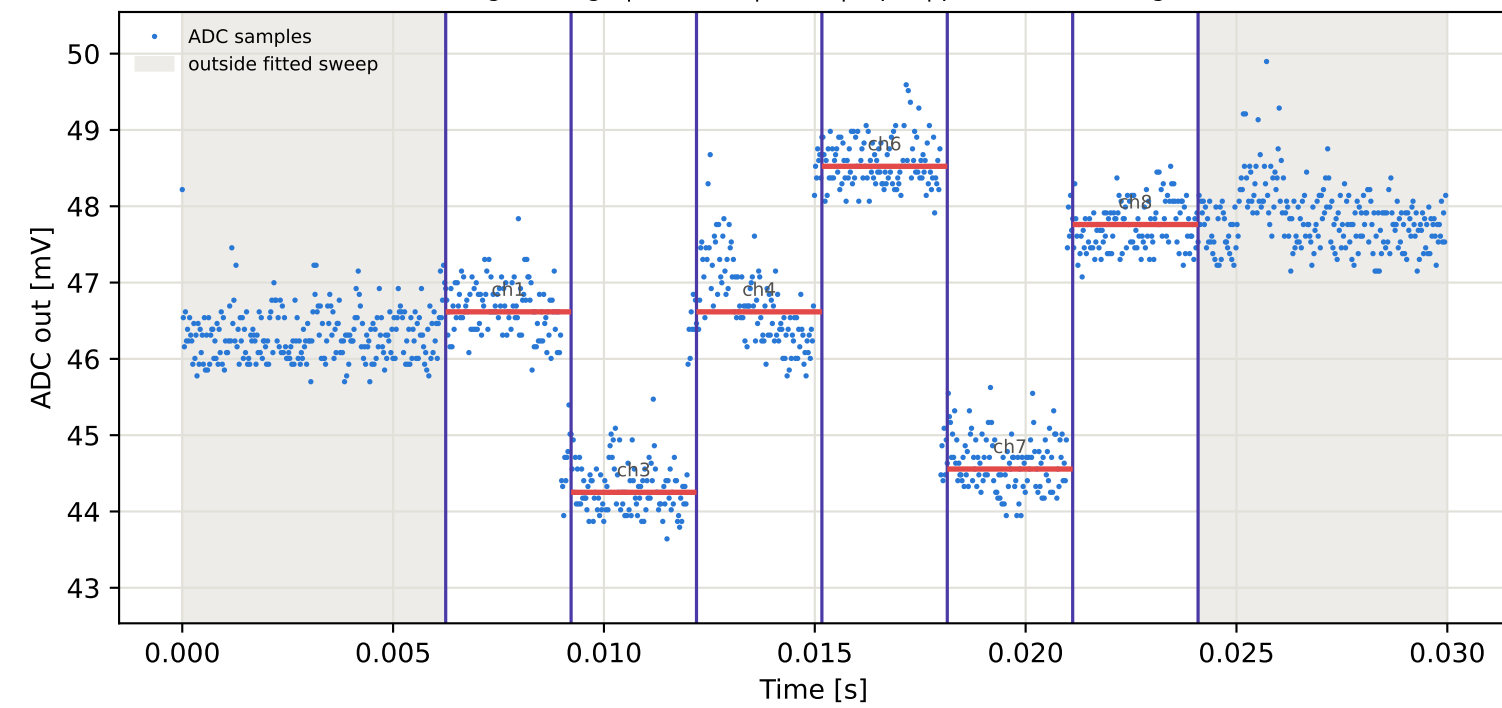
Tag9 &lt;- Tag10 | 775 MHz | run 0 | rep 1 | phase 126.98 deg
