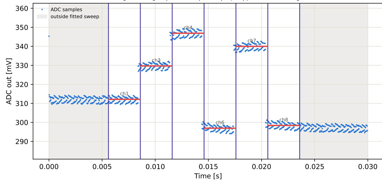
Tag16 &lt;- Tag15 | 985 MHz | run 0 | rep 1 | phase -54.47 deg
