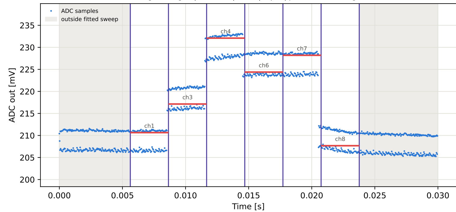
Tag1 &lt;- Tag2 | 915 MHz | run 0 | rep 1 | phase 155.12 deg
