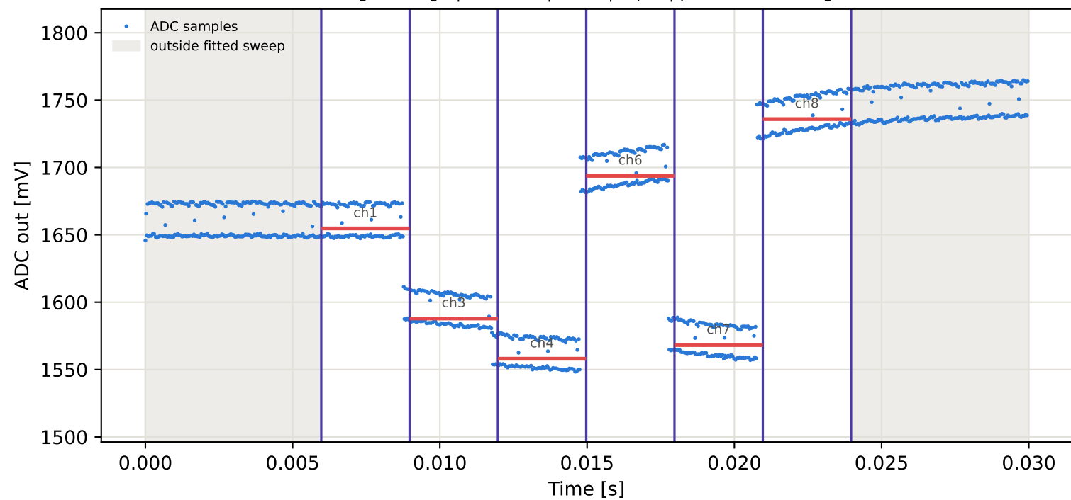
Tag5 &lt;- Tag4 | 905 MHz | run 0 | rep 1 | phase 133.64 deg
