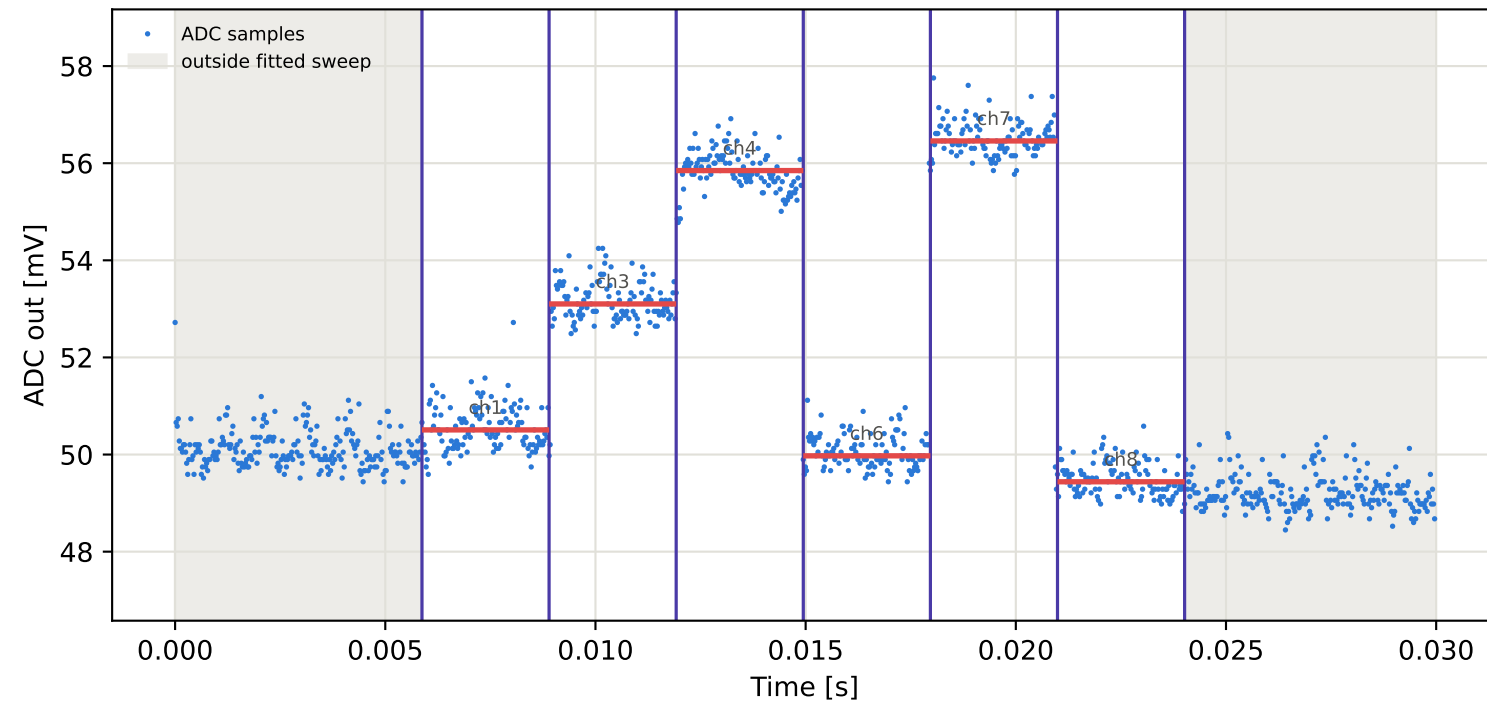
Tag7 &lt;- Tag10 | 775 MHz | run 0 | rep 1 | phase 34.67 deg
