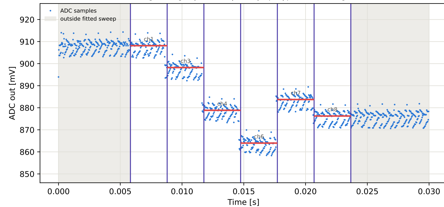
Tag6 &lt;- Tag2 | 875 MHz | run 0 | rep 1 | phase -133.62 deg
