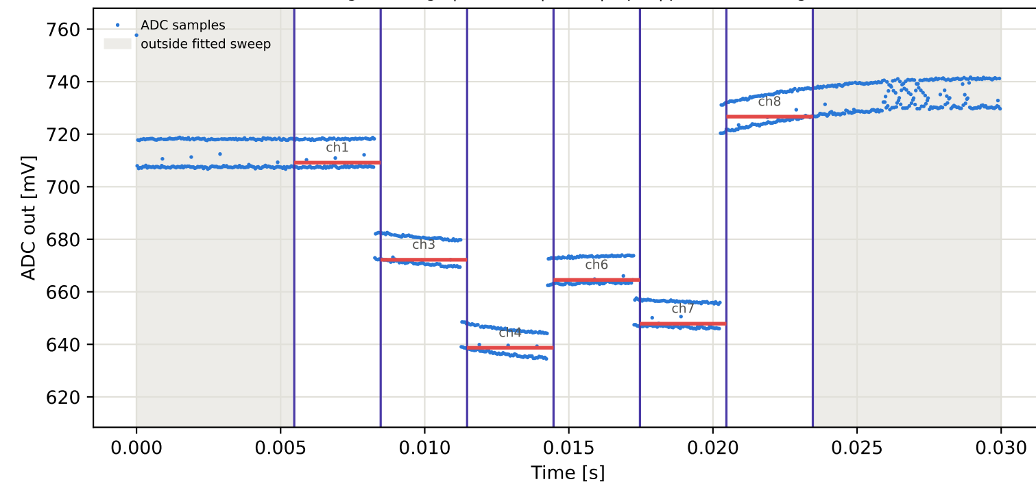
Tag10 &lt;- Tag8 | 895 MHz | run 0 | rep 1 | phase -17.14 deg
