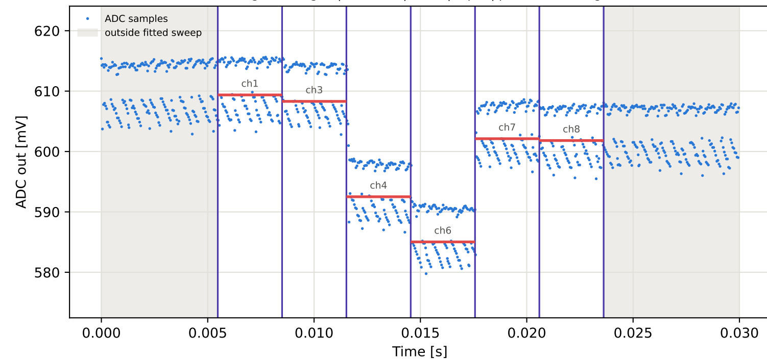
Tag15 &lt;- Tag3 | 955 MHz | run 0 | rep 1 | phase -29.19 deg
