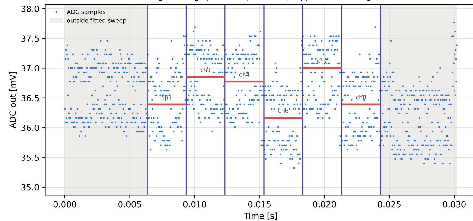
Tag16 &lt;- Tag4 | 775 MHz | run 0 | rep 1 | phase 9.33 deg
