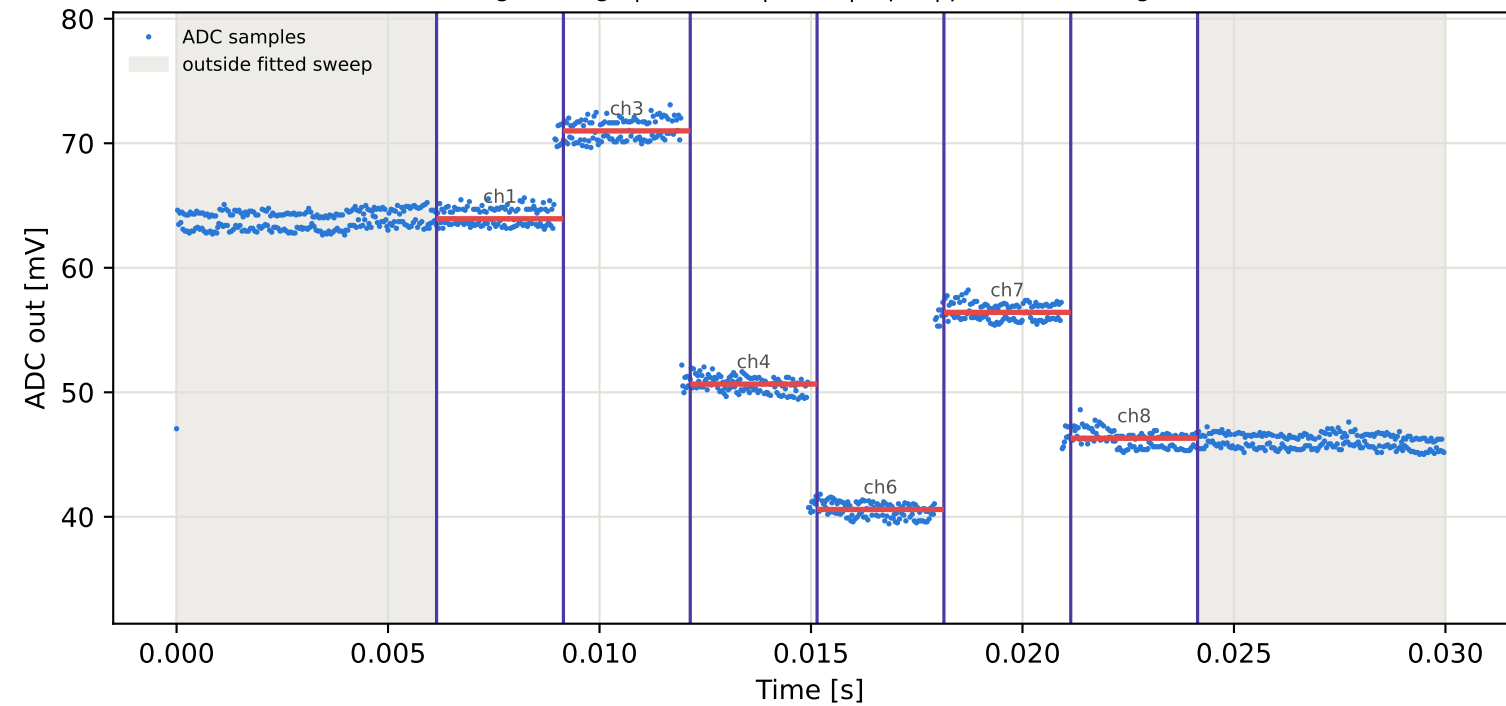
Tag9 &lt;- Tag8 | 835 MHz | run 0 | rep 1 | phase -179.48 deg
