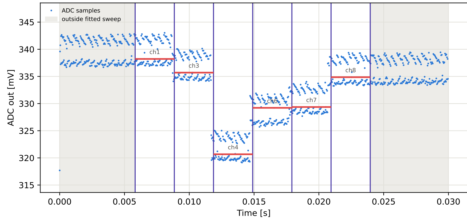
Tag4 &lt;- Tag3 | 985 MHz | run 0 | rep 1 | phase 147.28 deg
