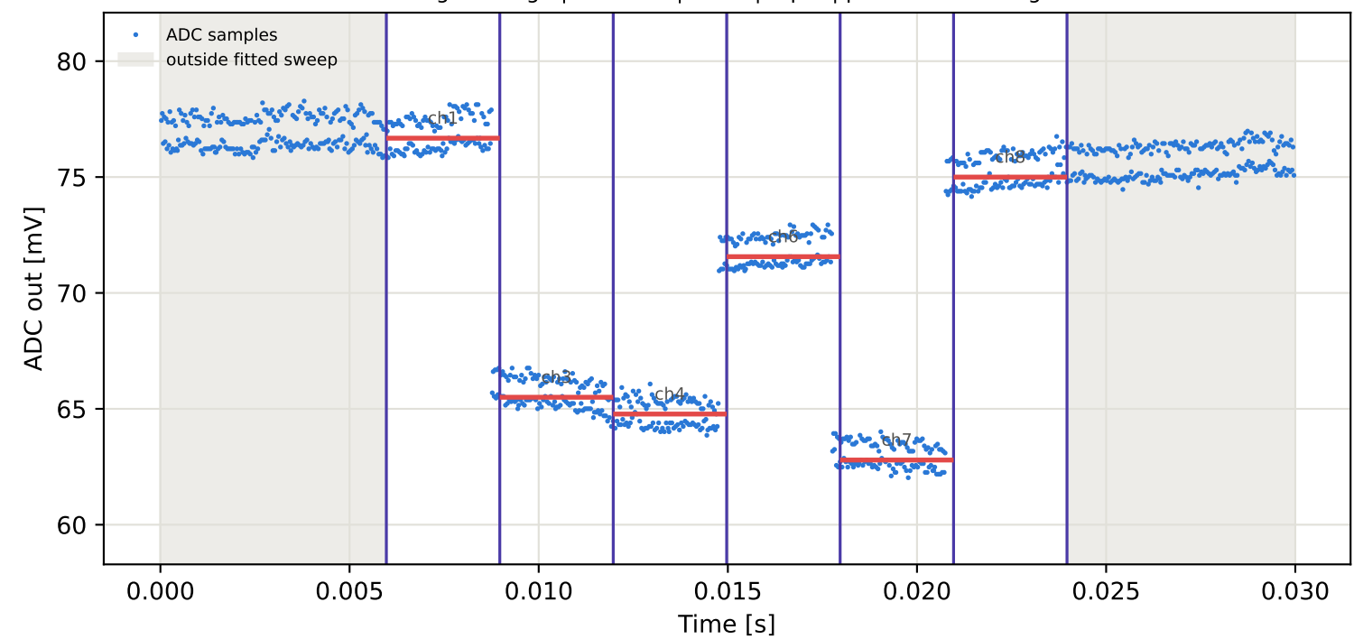
Tag9 &lt;- Tag6 | 825 MHz | run 0 | rep 1 | phase 63.94 deg
