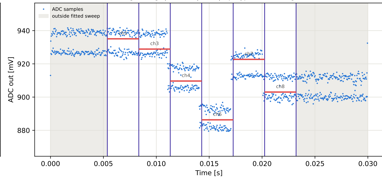
Tag5 &lt;- Tag9 | 885 MHz | run 0 | rep 1 | phase -130.64 deg
