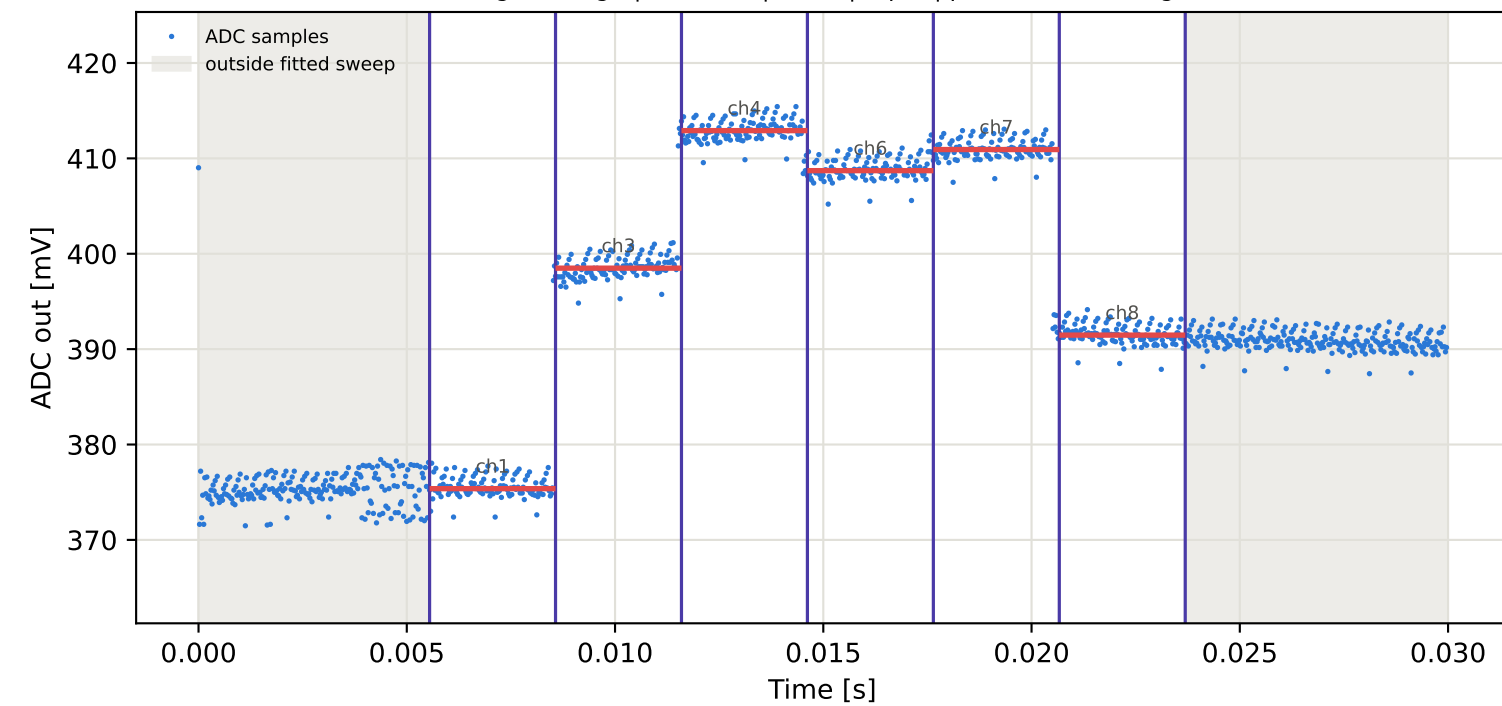
Tag3 &lt;- Tag6 | 855 MHz | run 0 | rep 1 | phase 147.94 deg
