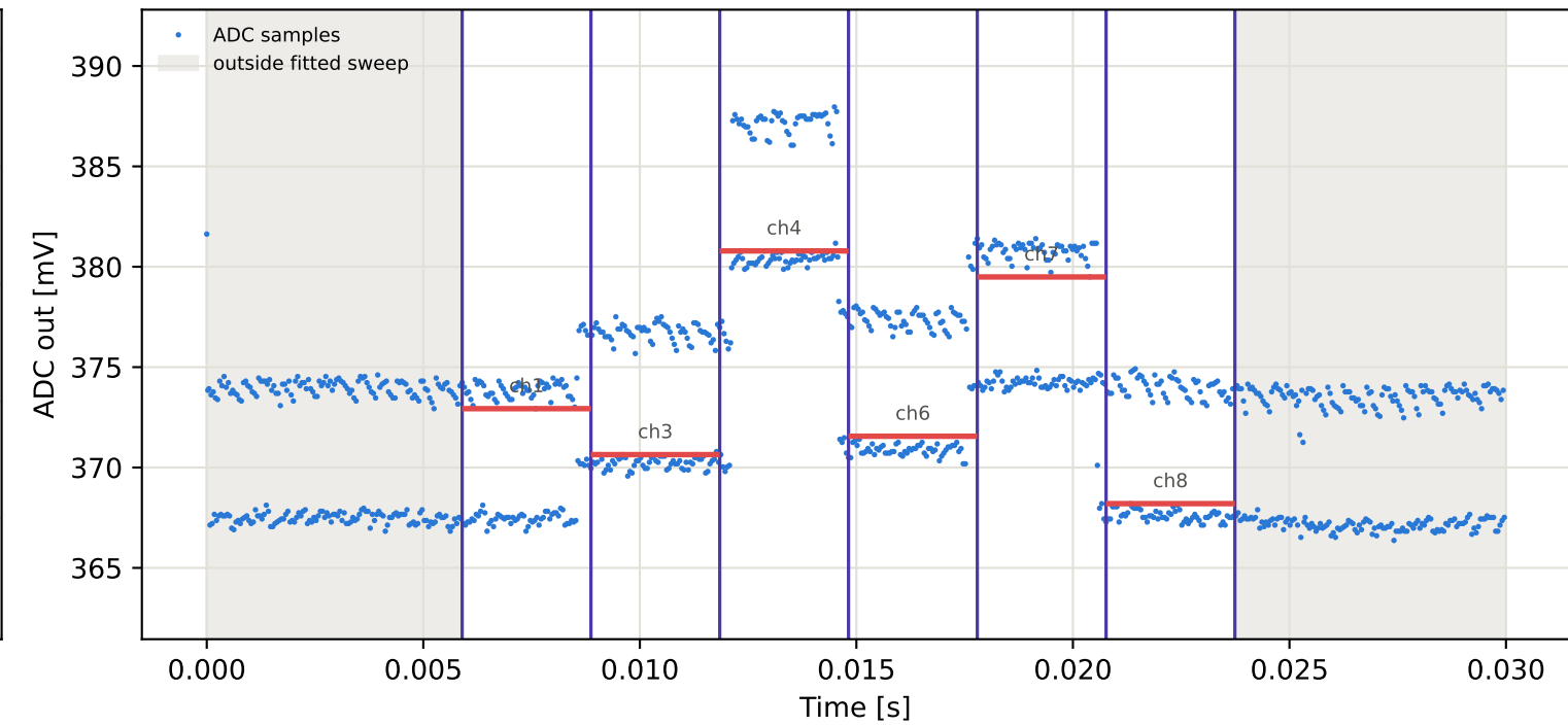
Tag7 &lt;- Tag6 | 985 MHz | run 0 | rep 1 | phase 94.07 deg
