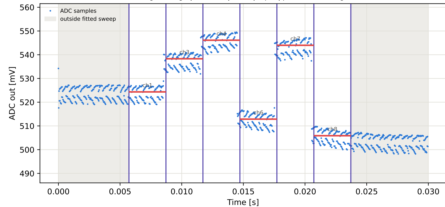
Tag9 &lt;- Tag7 | 915 MHz | run 0 | rep 1 | phase -20.63 deg
