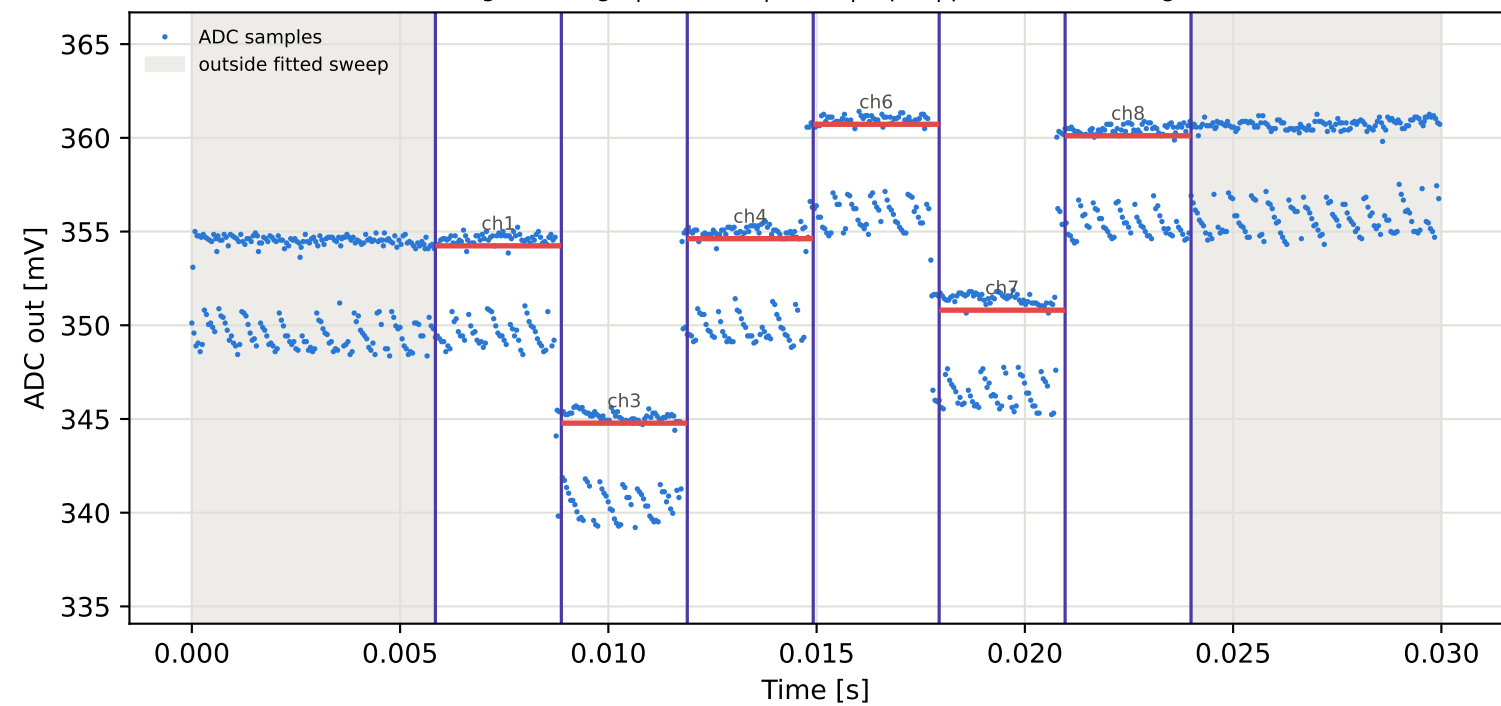
Tag16 &lt;- Tag15 | 845 MHz | run 0 | rep 1 | phase -165.76 deg
