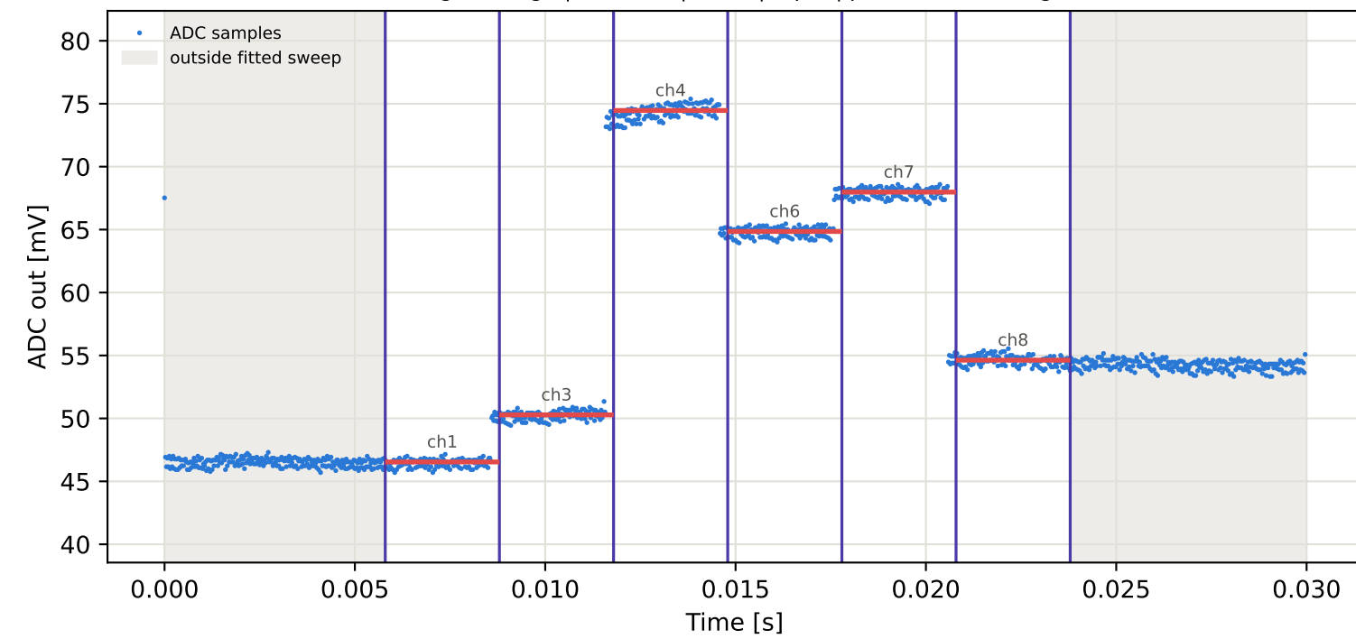
Tag4 &lt;- Tag7 | 805 MHz | run 0 | rep 1 | phase -132.78 deg
