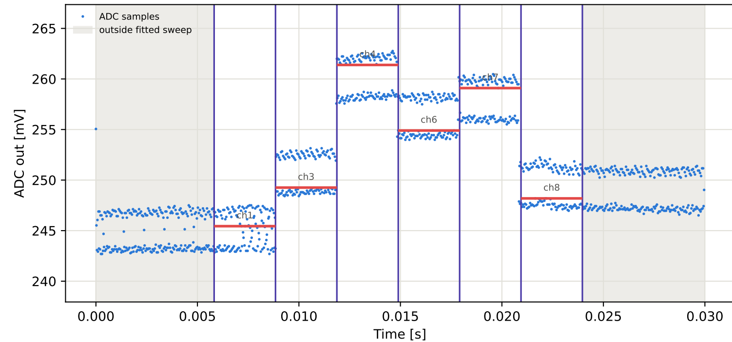
Tag3 &lt;- Tag9 | 825 MHz | run 0 | rep 1 | phase -54.53 deg
