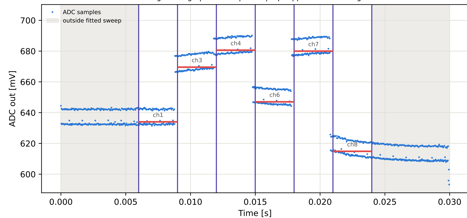
Tag3 &lt;- Tag9 | 875 MHz | run 0 | rep 1 | phase -65.19 deg
