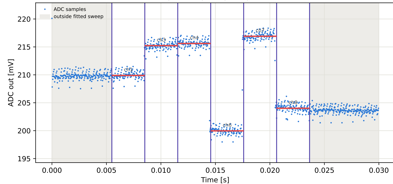
Tag3 &lt;- Tag8 | 995 MHz | run 0 | rep 1 | phase -25.57 deg
