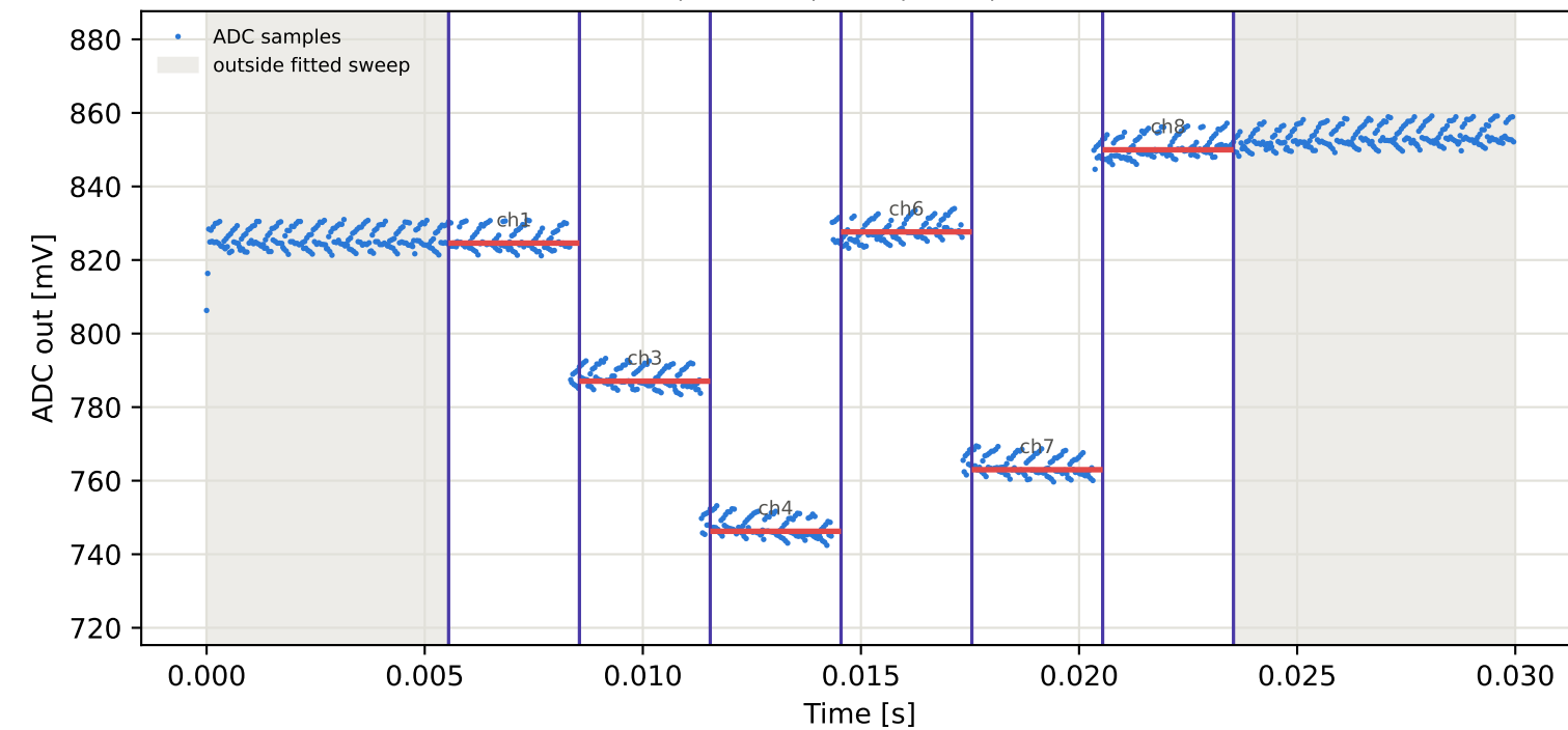
Tag8 &lt;- Tag15 | 945 MHz | run 0 | rep 1 | phase 110.86 deg
