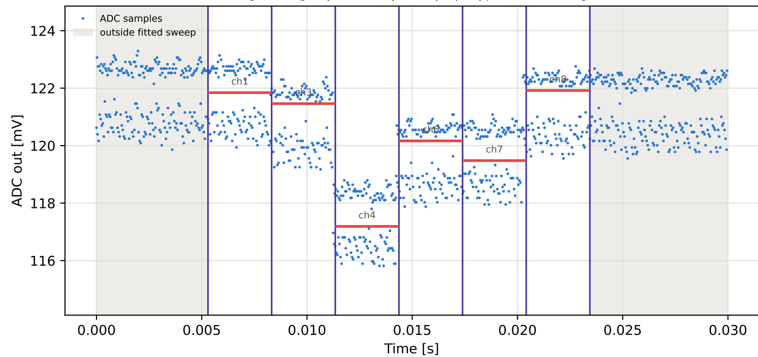
Tag1 &lt;- Tag16 | 995 MHz | run 0 | rep 1 | phase -51.80 deg
