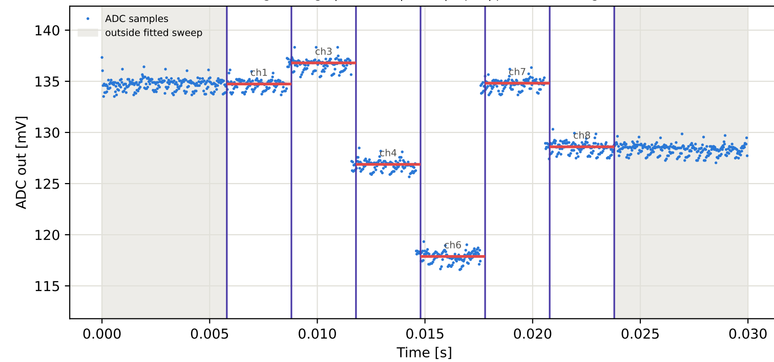
Tag9 &lt;- Tag5 | 995 MHz | run 0 | rep 1 | phase 30.67 deg
