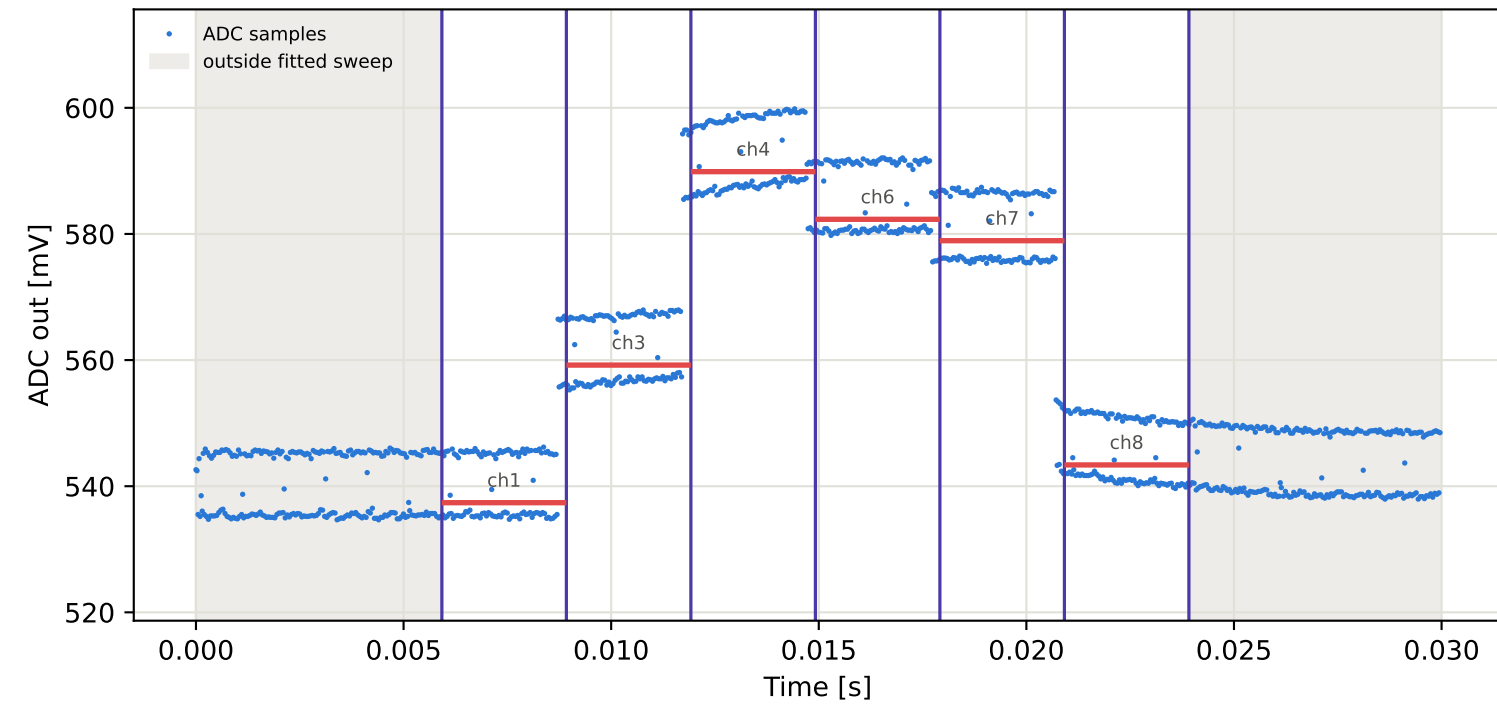
Tag15 &lt;- Tag10 | 925 MHz | run 0 | rep 1 | phase -17.20 deg
