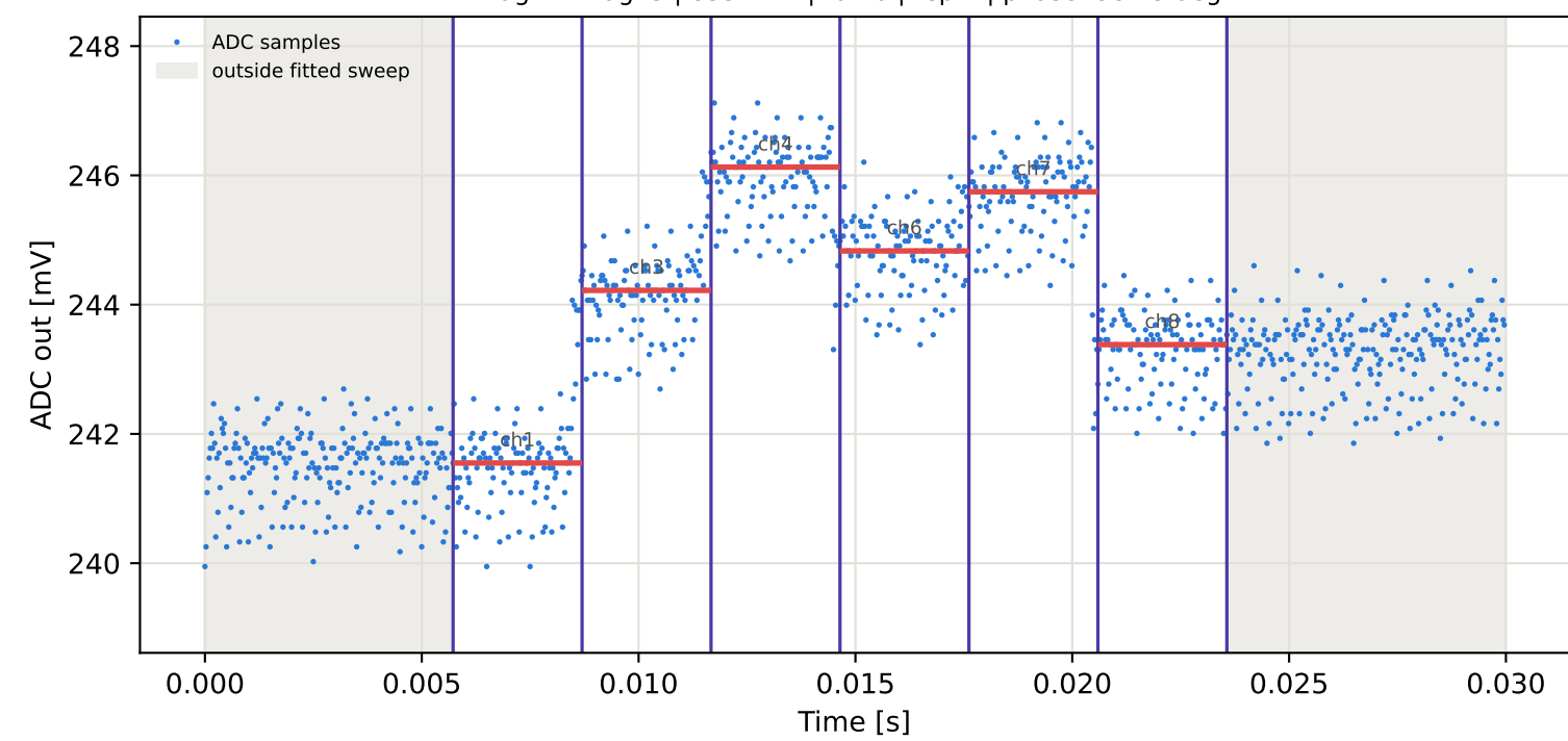
Tag1 &lt;- Tag2 | 855 MHz | run 0 | rep 1 | phase -86.11 deg
