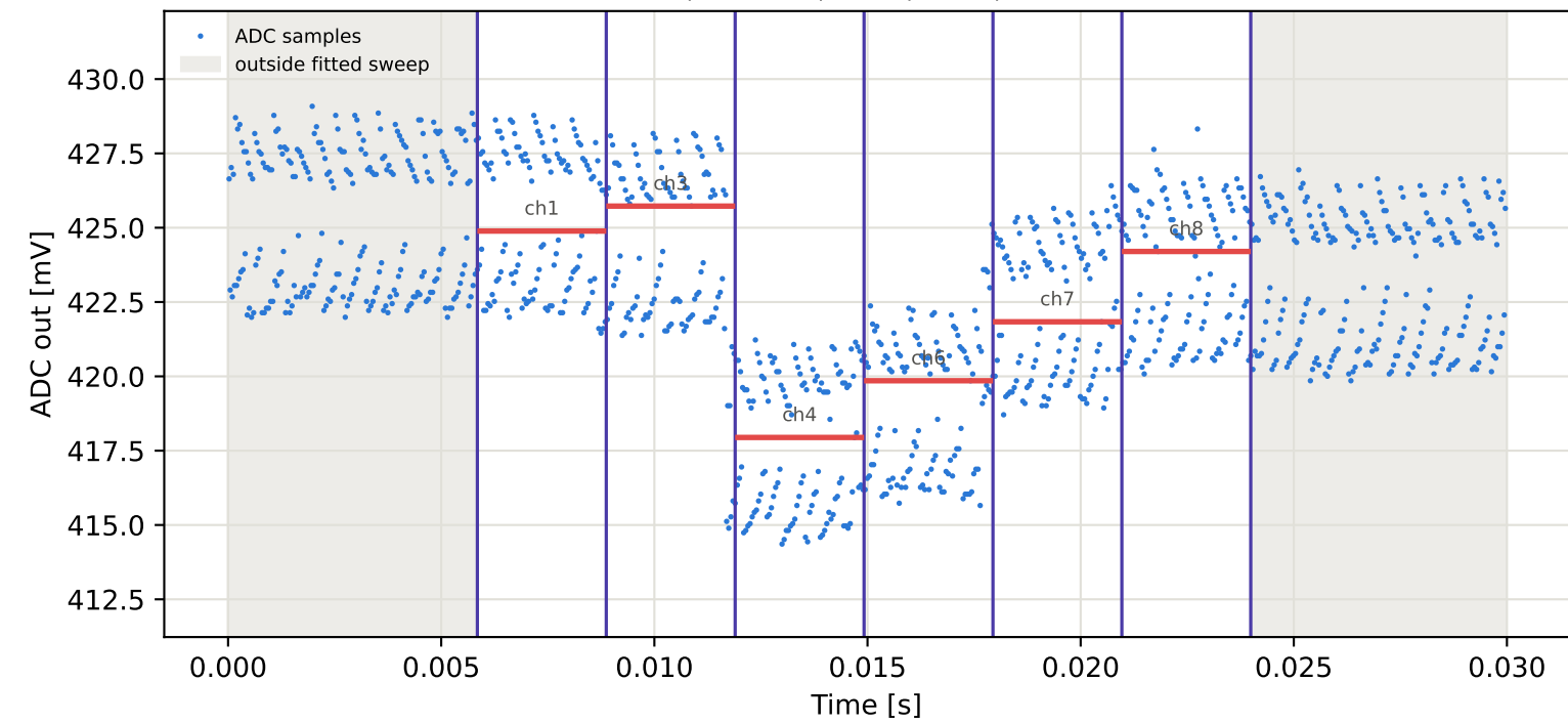
Tag7 &lt;- Tag6 | 975 MHz | run 0 | rep 1 | phase 48.80 deg
