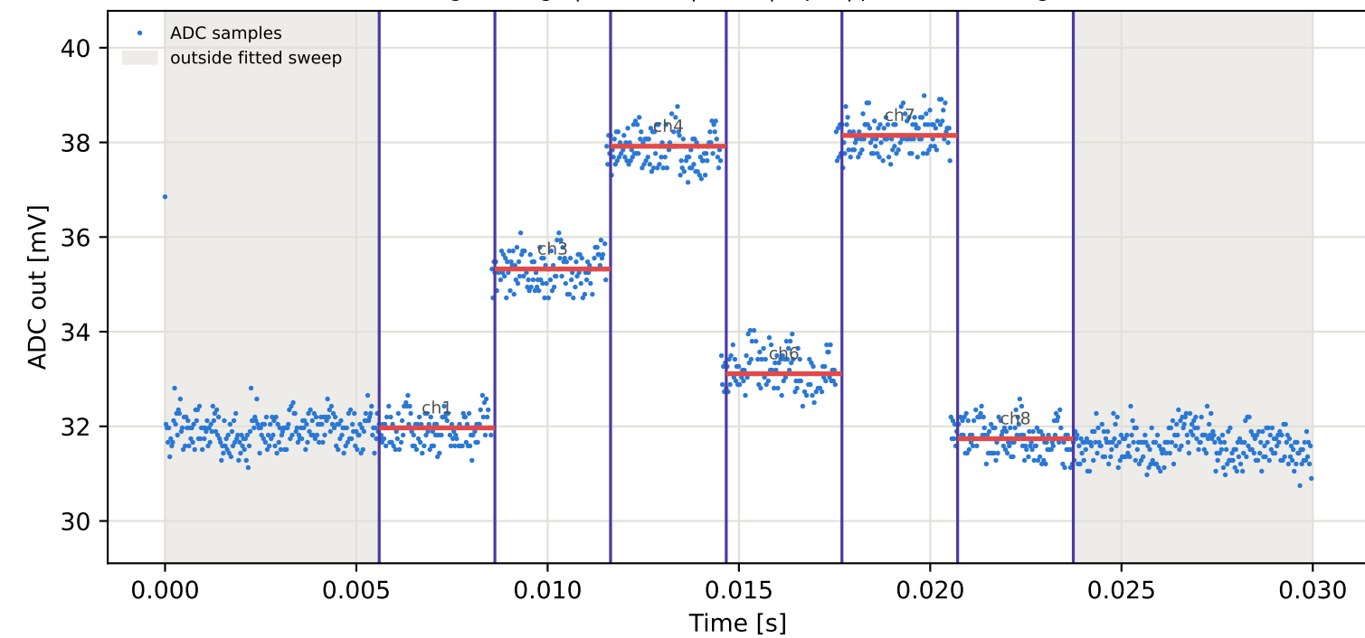
Tag1 &lt;- Tag7 | 785 MHz | run 0 | rep 1 | phase 43.55 deg
