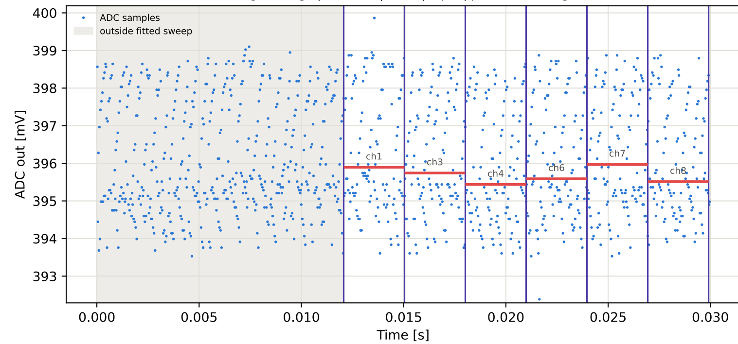
Tag8 &lt;- Tag4 | 995 MHz | run 0 | rep 1 | phase -33.92 deg
