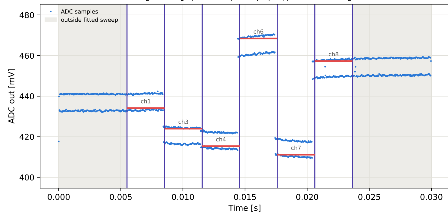
Tag16 &lt;- Tag1 | 995 MHz | run 0 | rep 1 | phase -41.56 deg
