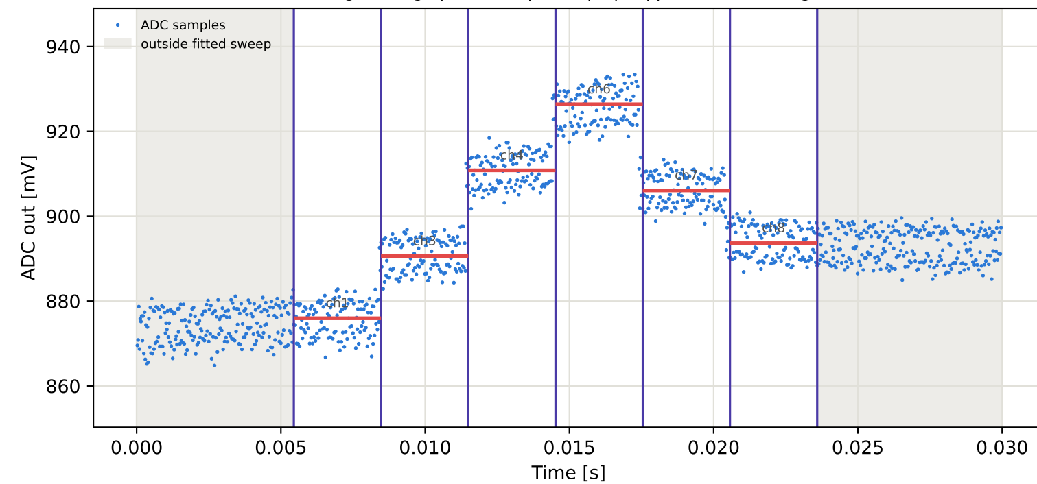
Tag5 &lt;- Tag8 | 885 MHz | run 0 | rep 1 | phase 99.49 deg
