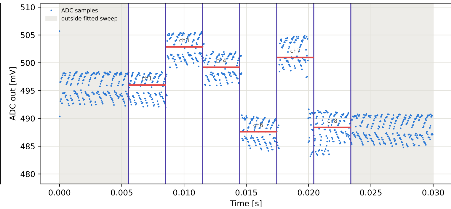
Tag16 &lt;- Tag7 | 855 MHz | run 0 | rep 1 | phase -6.85 deg
