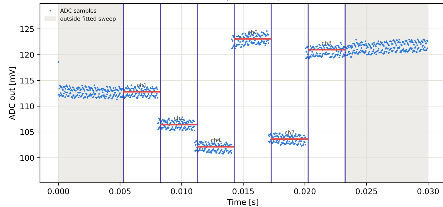
Tag1 &lt;- Tag7 | 935 MHz | run 0 | rep 1 | phase 159.31 deg
