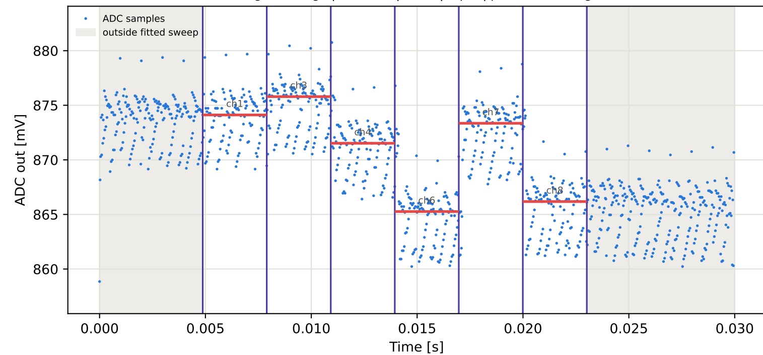
Tag16 &lt;- Tag15 | 875 MHz | run 0 | rep 1 | phase -150.76 deg
