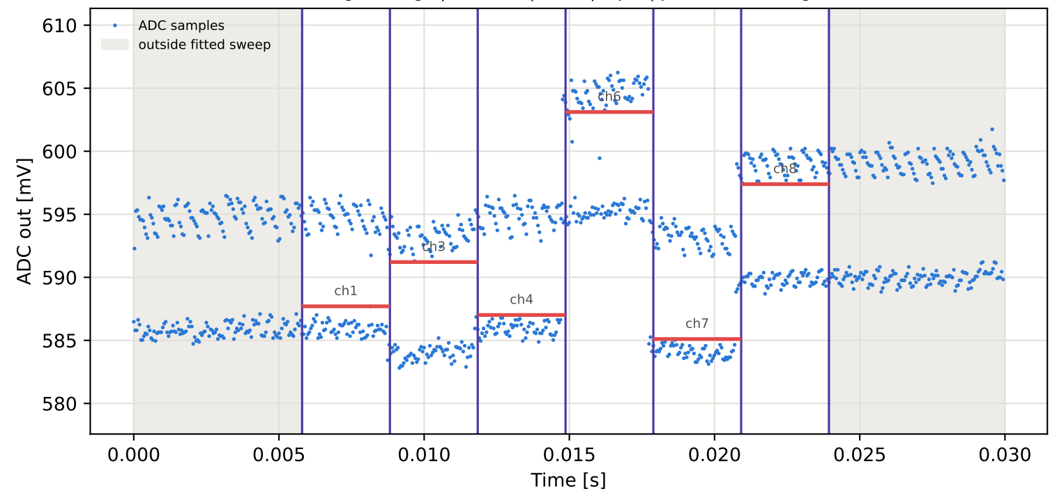
Tag8 &lt;- Tag5 | 965 MHz | run 0 | rep 1 | phase -115.68 deg
