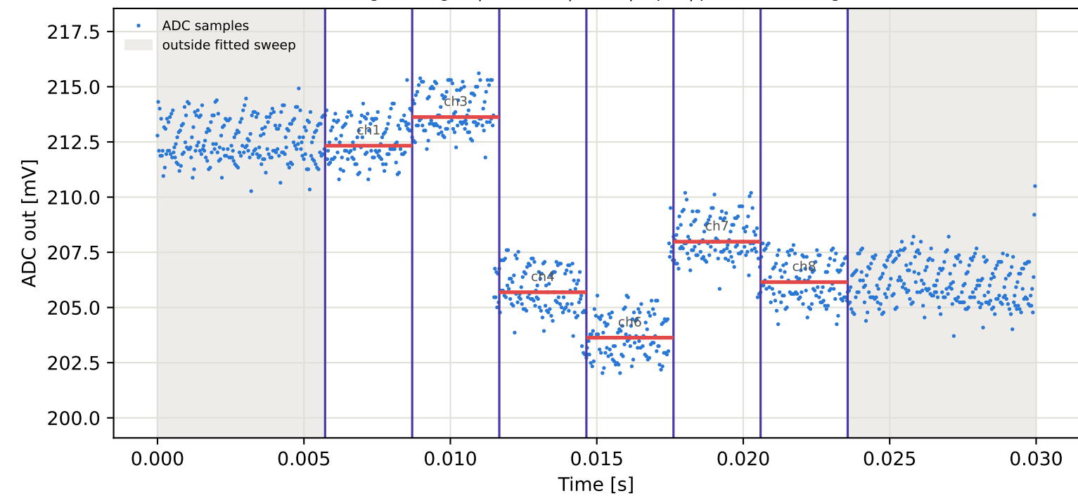
Tag5 &lt;- Tag16 | 835 MHz | run 0 | rep 1 | phase 173.21 deg
