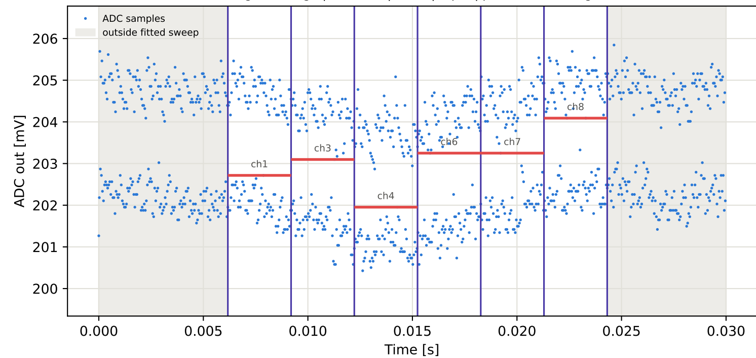
Tag15 &lt;- Tag4 | 805 MHz | run 0 | rep 1 | phase 38.53 deg
