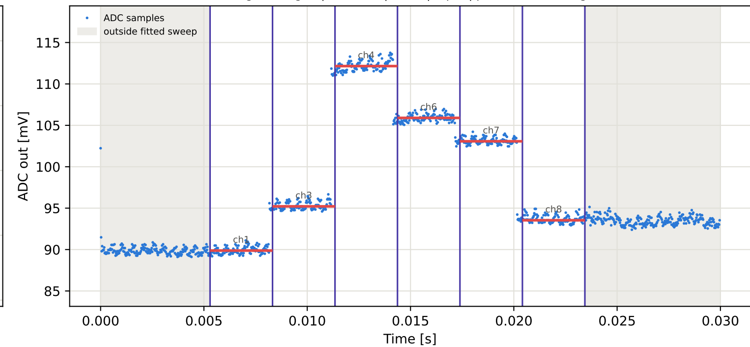
Tag5 &lt;- Tag2 | 975 MHz | run 0 | rep 1 | phase -177.83 deg
