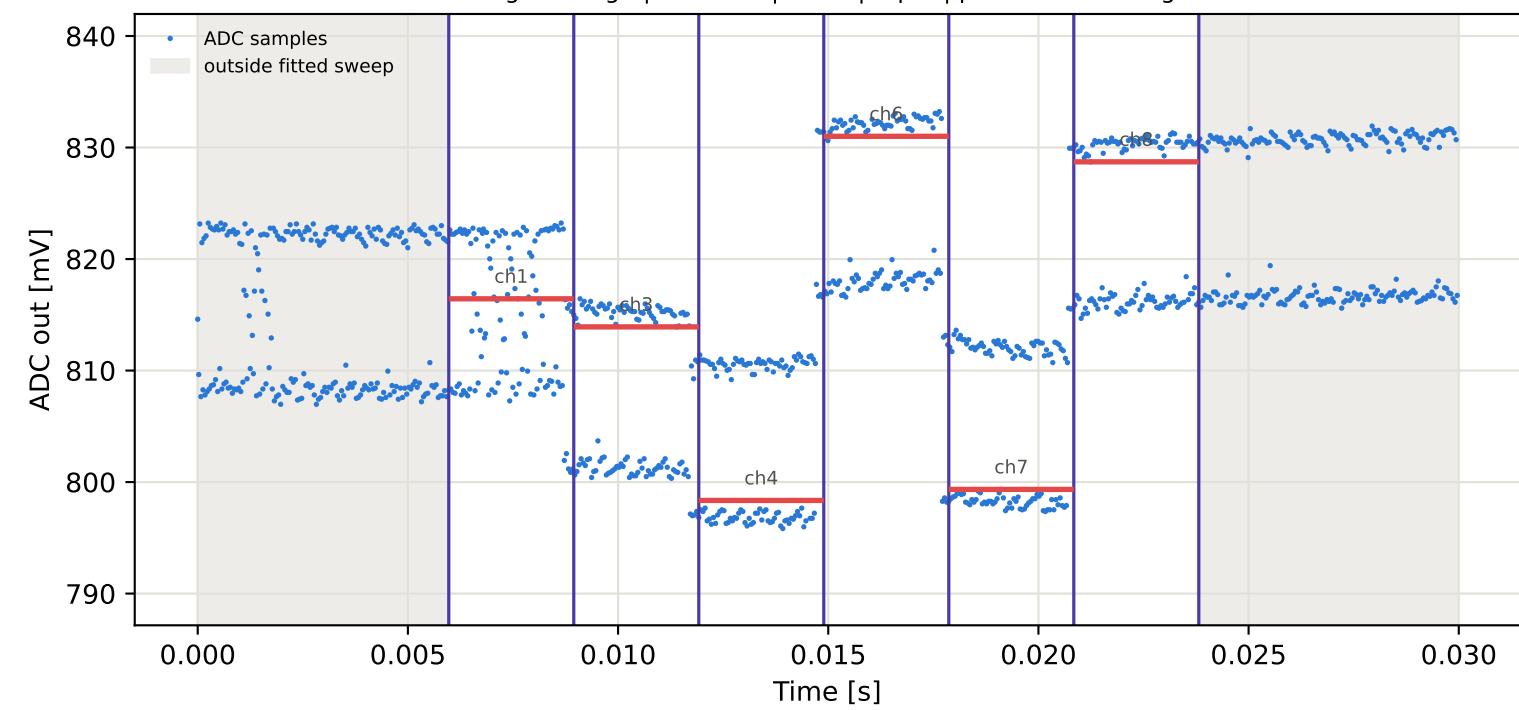
Tag8 &lt;- Tag5 | 935 MHz | run 0 | rep 1 | phase 138.86 deg
