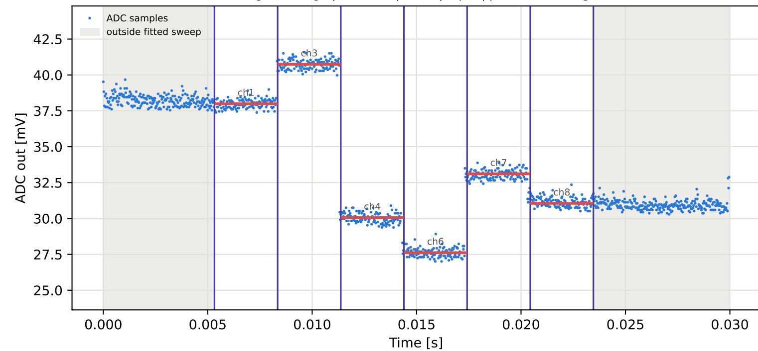
Tag10 &lt;- Tag8 | 825 MHz | run 0 | rep 1 | phase -131.04 deg
