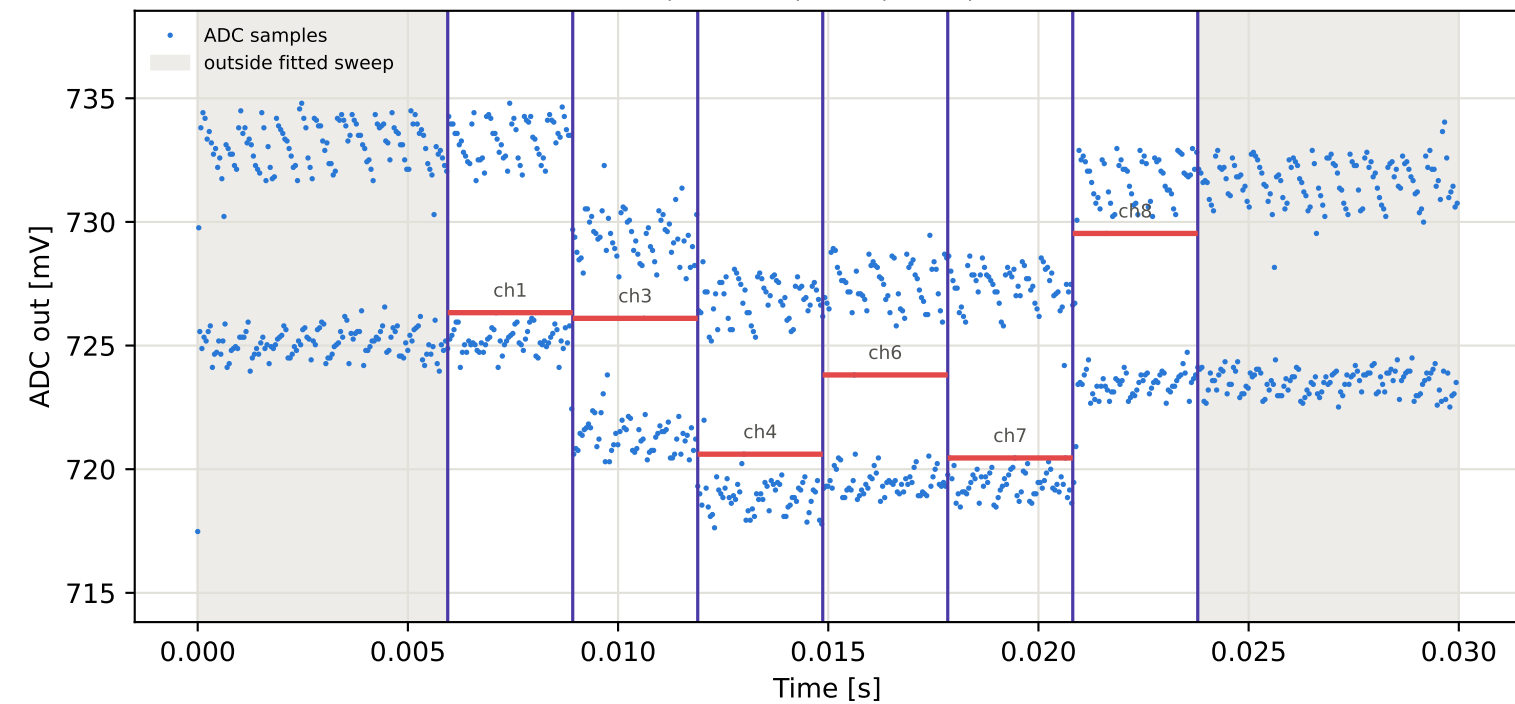
Tag15 &lt;- Tag10 | 875 MHz | run 0 | rep 1 | phase 88.68 deg
