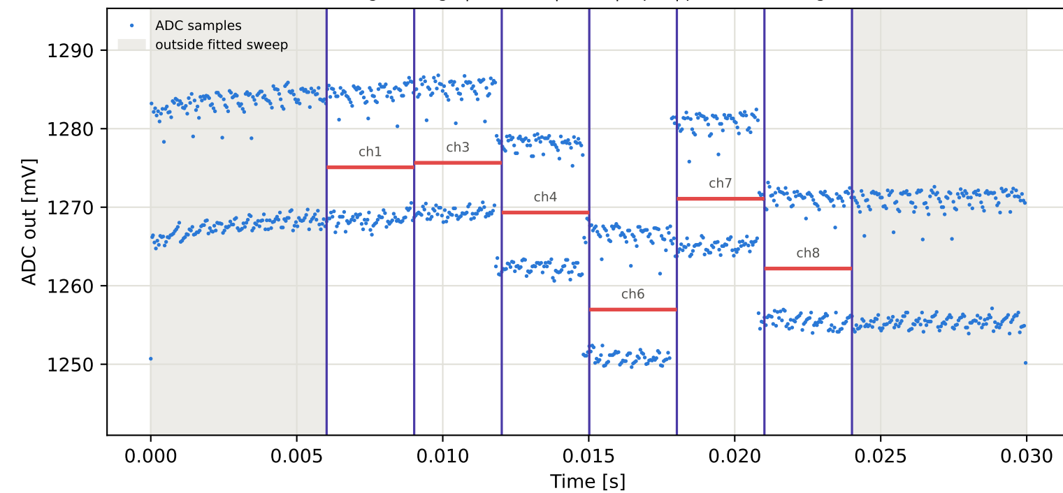
Tag9 &lt;- Tag10 | 875 MHz | run 0 | rep 1 | phase 40.16 deg
