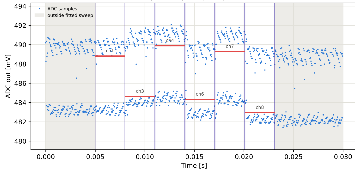
Tag8 &lt;- Tag4 | 825 MHz | run 0 | rep 1 | phase -144.47 deg
