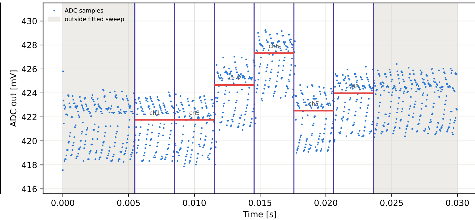
Tag7 &lt;- Tag15 | 975 MHz | run 0 | rep 1 | phase 179.79 deg
