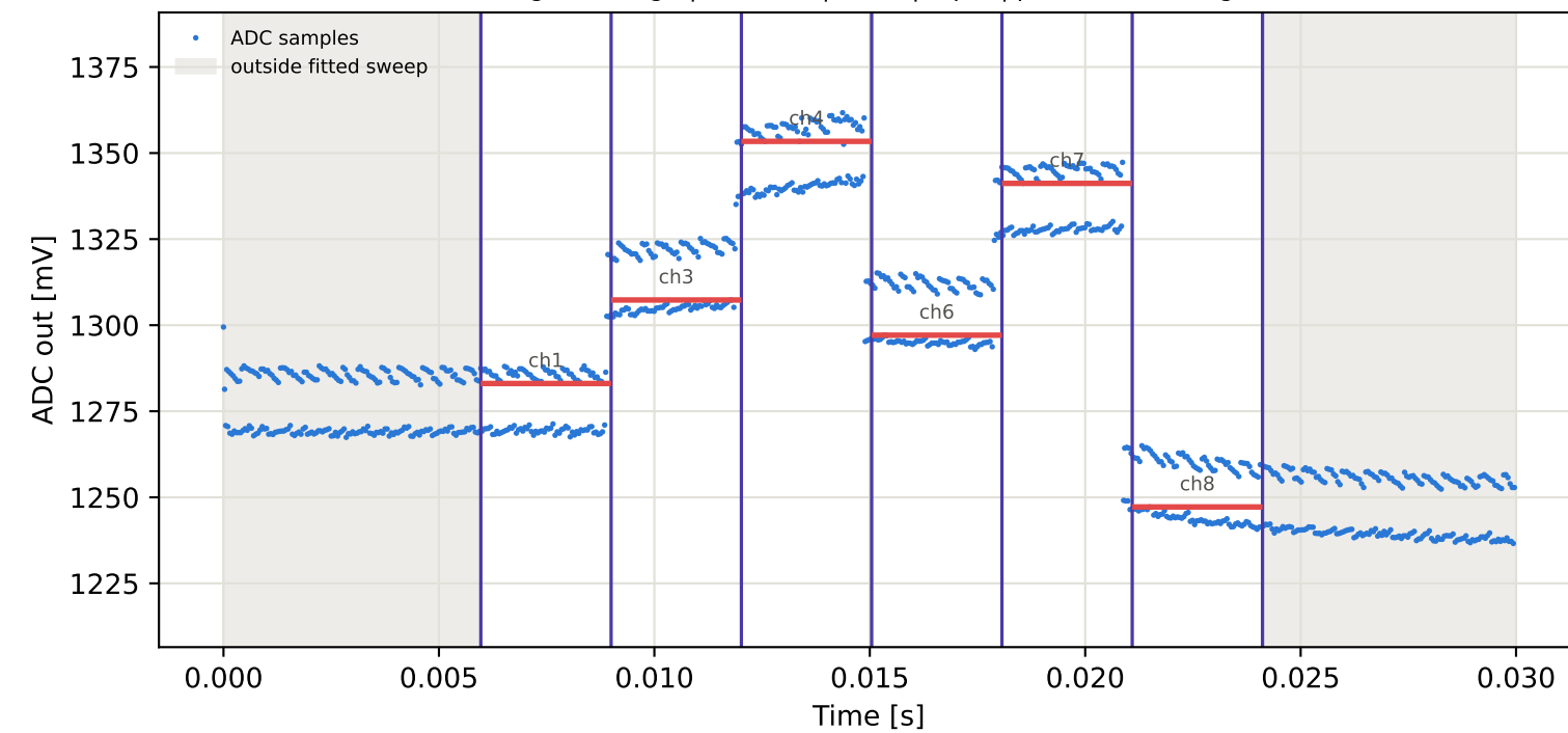
Tag2 &lt;- Tag1 | 915 MHz | run 0 | rep 1 | phase -16.63 deg
