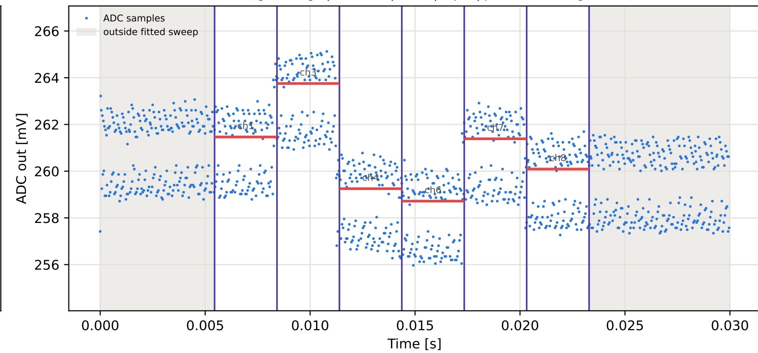
Tag3 &lt;- Tag15 | 825 MHz | run 0 | rep 1 | phase 12.43 deg
