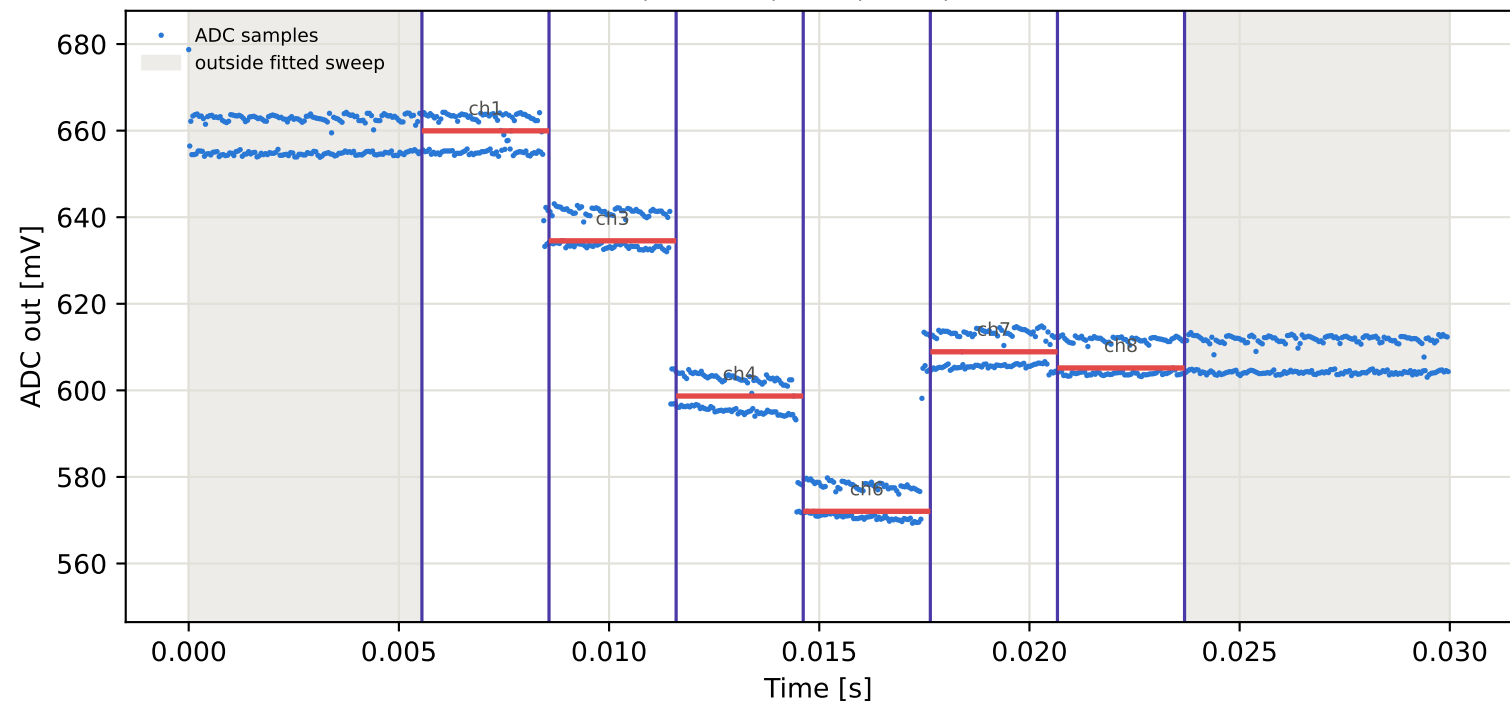
Tag5 &lt;- Tag4 | 865 MHz | run 0 | rep 1 | phase 44.51 deg
