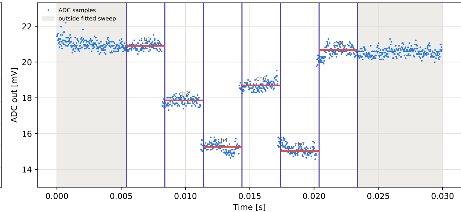
Tag3 &lt;- Tag9 | 795 MHz | run 0 | rep 1 | phase -112.21 deg
