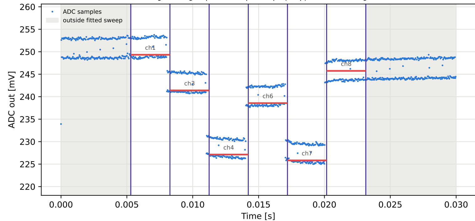
Tag8 &lt;- Tag16 | 805 MHz | run 0 | rep 1 | phase 96.43 deg
