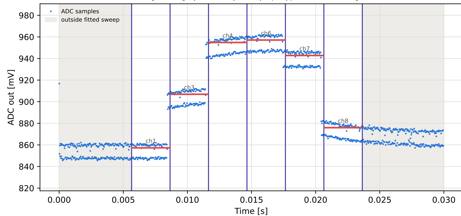
Tag6 &lt;- Tag5 | 885 MHz | run 0 | rep 1 | phase -94.72 deg
