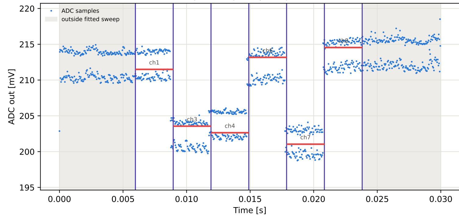
Tag5 &lt;- Tag1 | 835 MHz | run 0 | rep 1 | phase 140.78 deg
