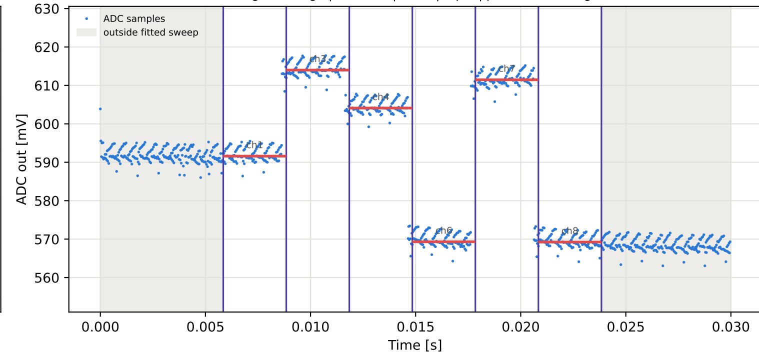
Tag16 &lt;- Tag7 | 865 MHz | run 0 | rep 1 | phase -12.93 deg
