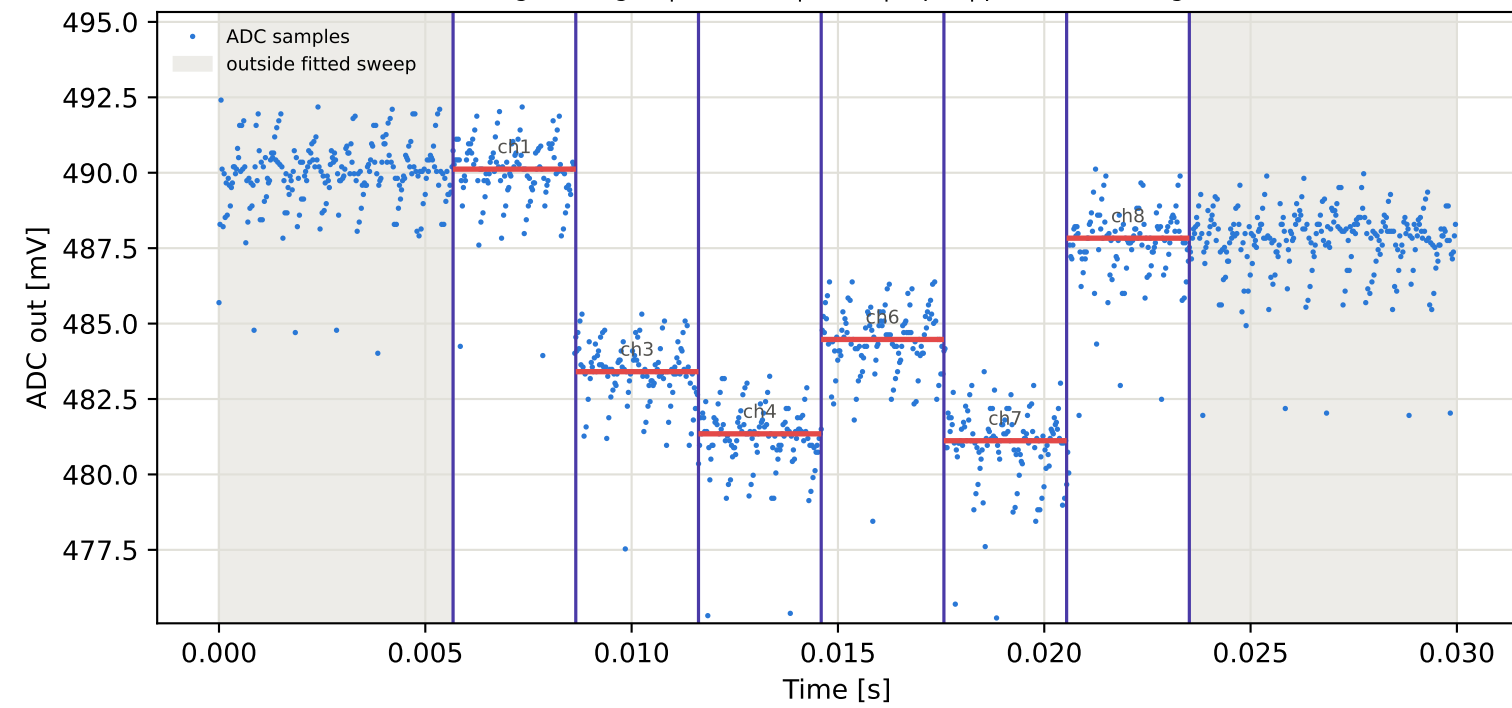
Tag6 &lt;- Tag3 | 845 MHz | run 0 | rep 1 | phase -124.54 deg
