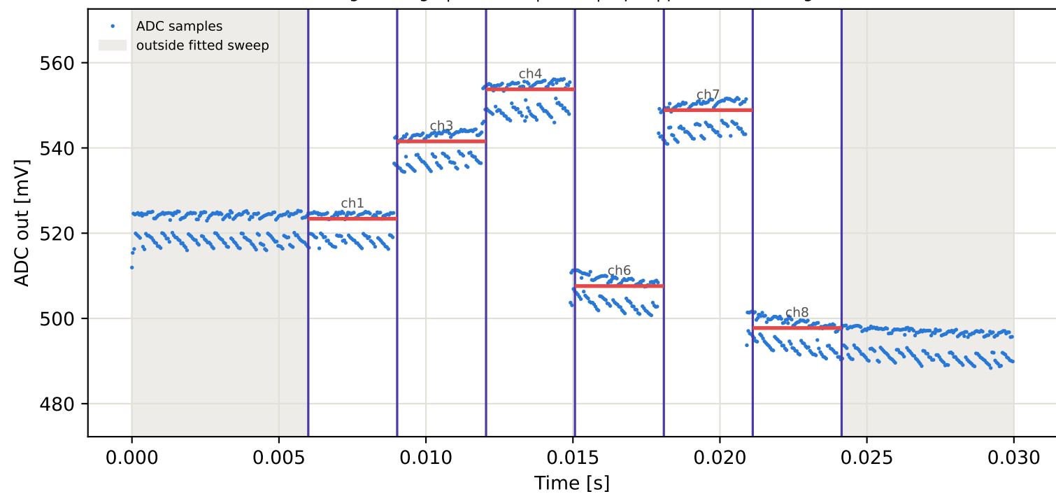
Tag9 &lt;- Tag8 | 915 MHz | run 0 | rep 1 | phase -46.42 deg
