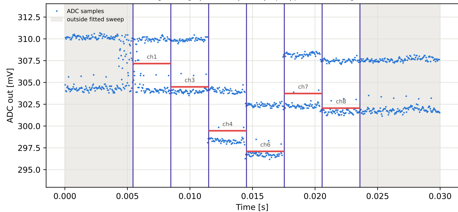
Tag9 &lt;- Tag7 | 985 MHz | run 0 | rep 1 | phase 90.19 deg
