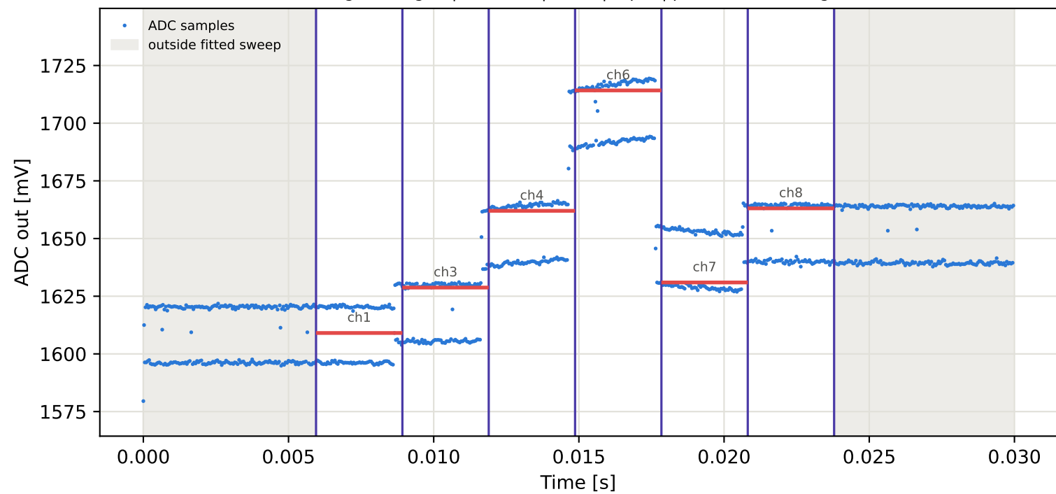
Tag5 &lt;- Tag2 | 905 MHz | run 0 | rep 1 | phase -143.42 deg
