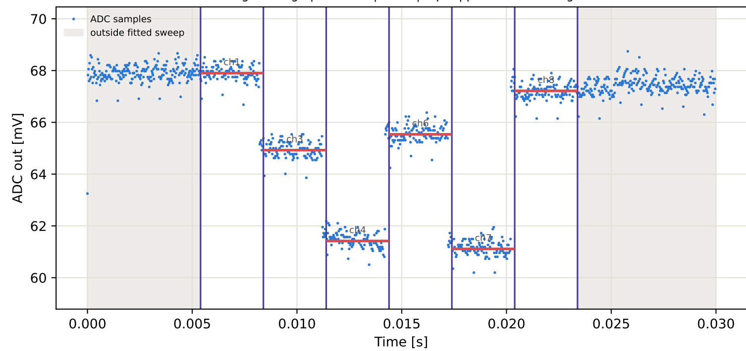
Tag4 &lt;- Tag8 | 785 MHz | run 0 | rep 1 | phase -107.10 deg
