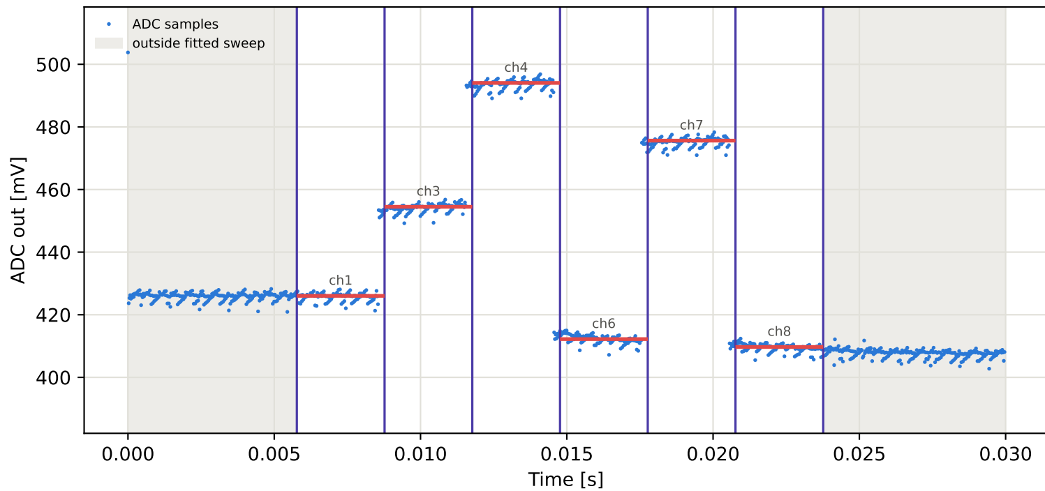
Tag2 &lt;- Tag1 | 975 MHz | run 0 | rep 1 | phase -52.31 deg
