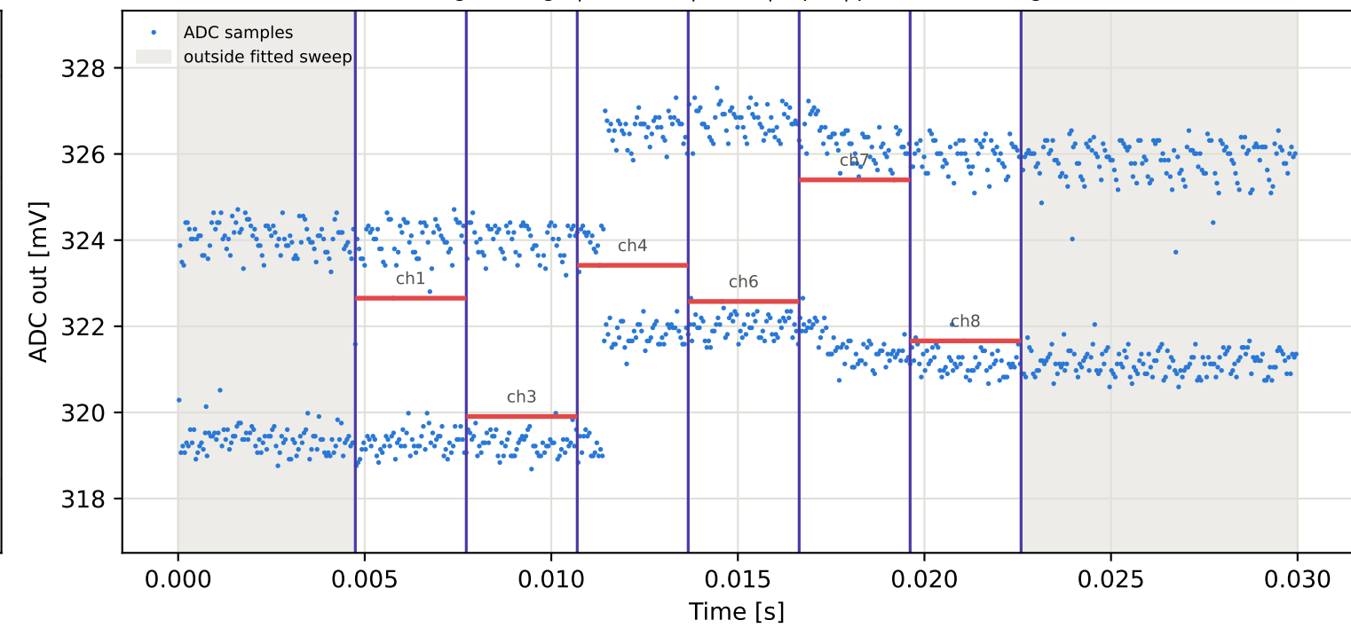
Tag4 &lt;- Tag8 | 825 MHz | run 0 | rep 1 | phase -34.75 deg
