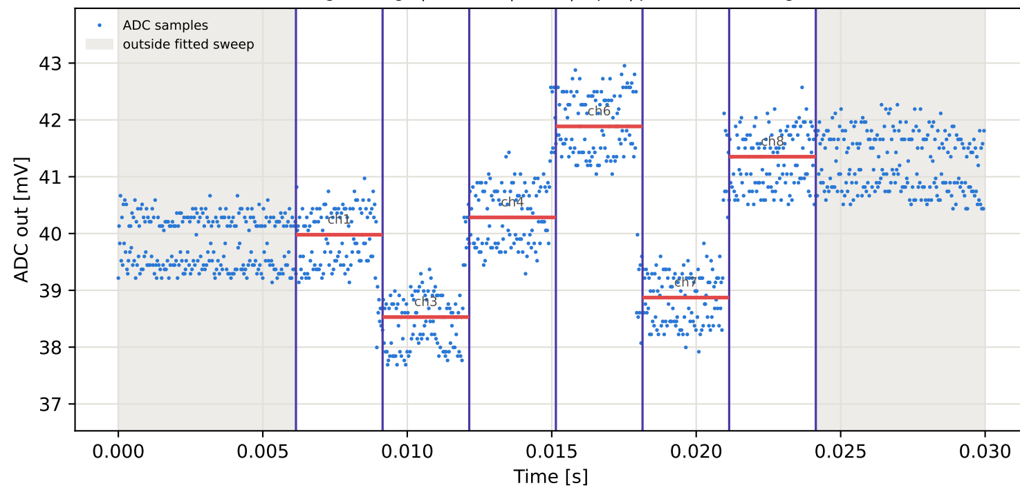
Tag4 &lt;- Tag15 | 775 MHz | run 0 | rep 1 | phase 136.44 deg
