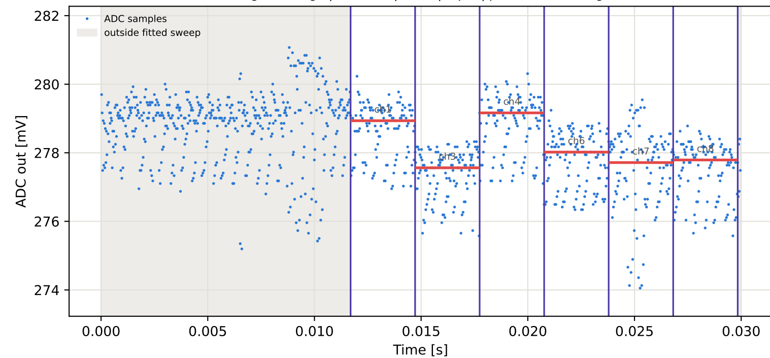
Tag10 &lt;- Tag4 | 845 MHz | run 0 | rep 1 | phase -58.98 deg
