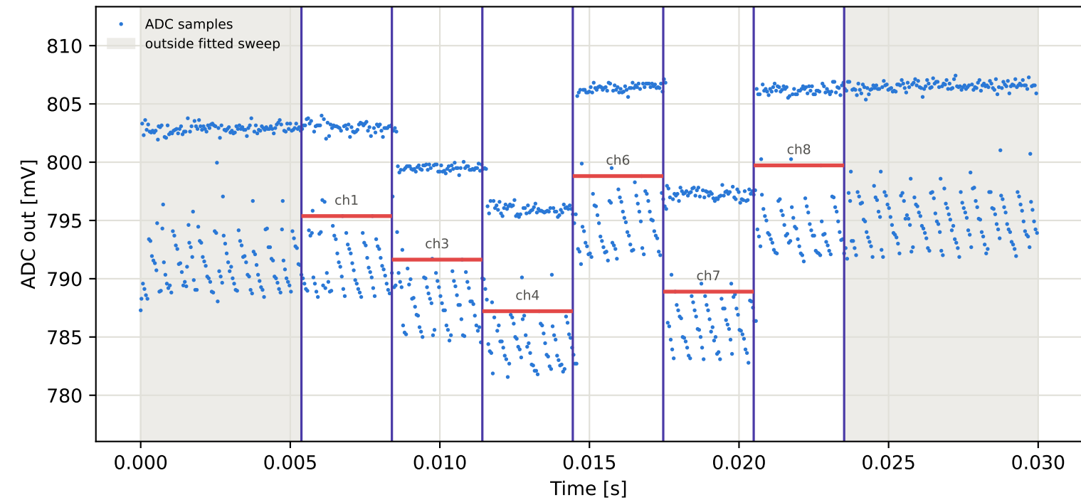
Tag8 &lt;- Tag16 | 945 MHz | run 0 | rep 1 | phase 30.41 deg
