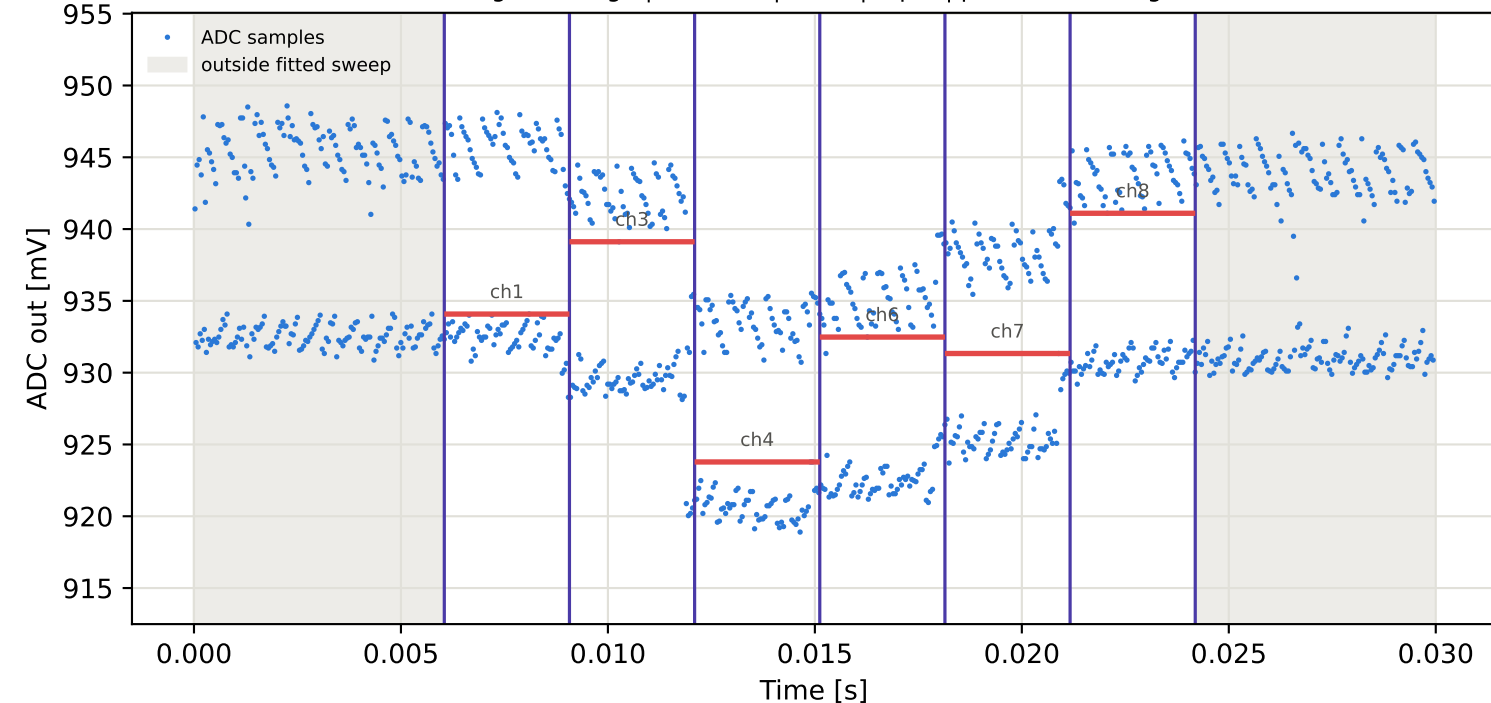
Tag15 &lt;- Tag6 | 945 MHz | run 0 | rep 1 | phase 68.58 deg
