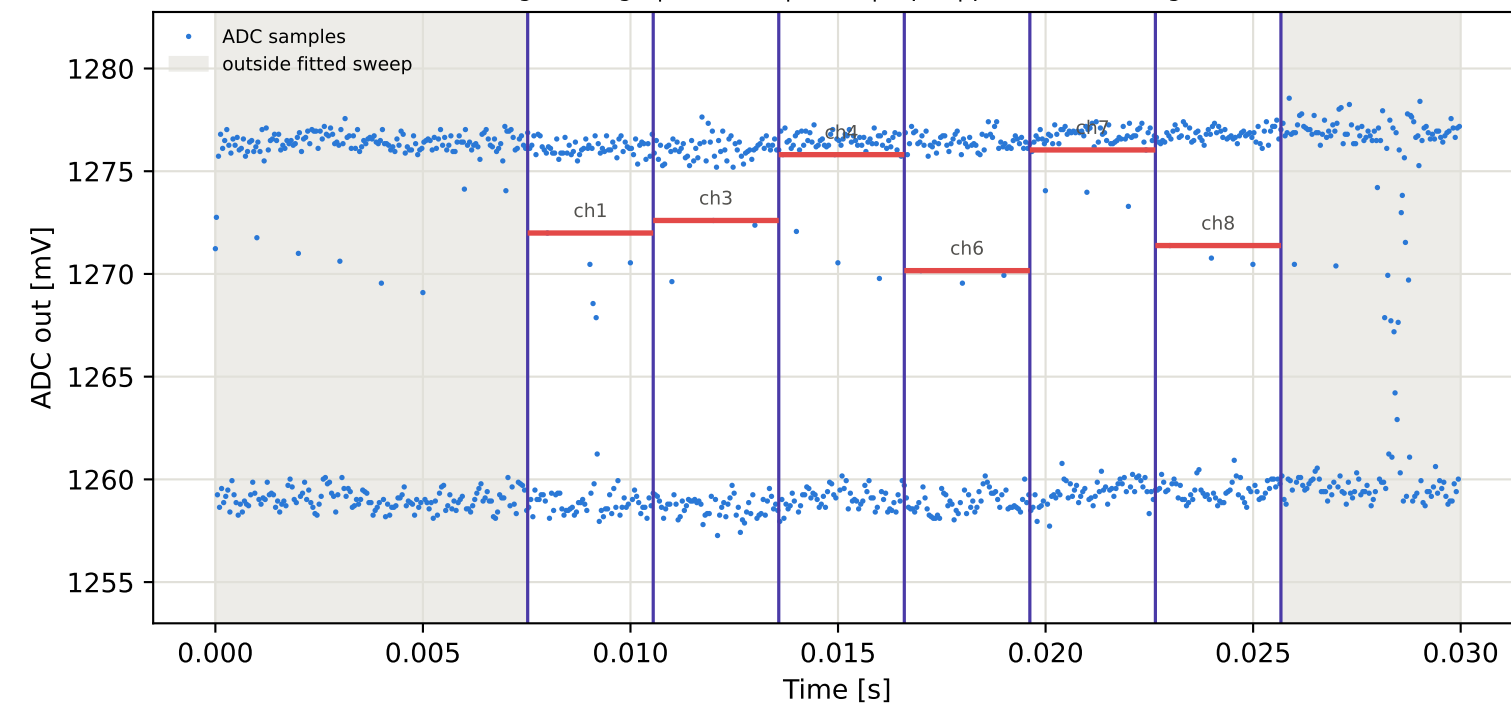
Tag8 &lt;- Tag4 | 875 MHz | run 0 | rep 1 | phase 109.55 deg
