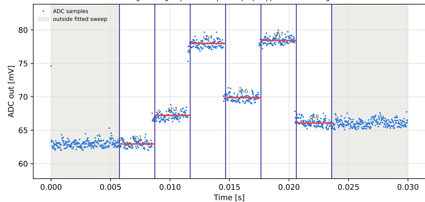
Tag6 &lt;- Tag10 | 795 MHz | run 0 | rep 1 | phase -84.12 deg
