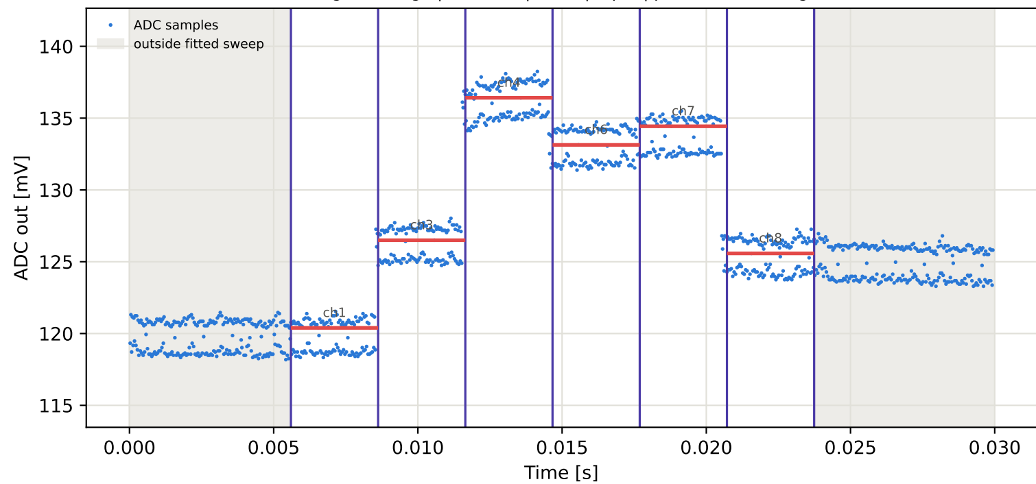
Tag10 &lt;- Tag9 | 865 MHz | run 0 | rep 1 | phase -112.16 deg
