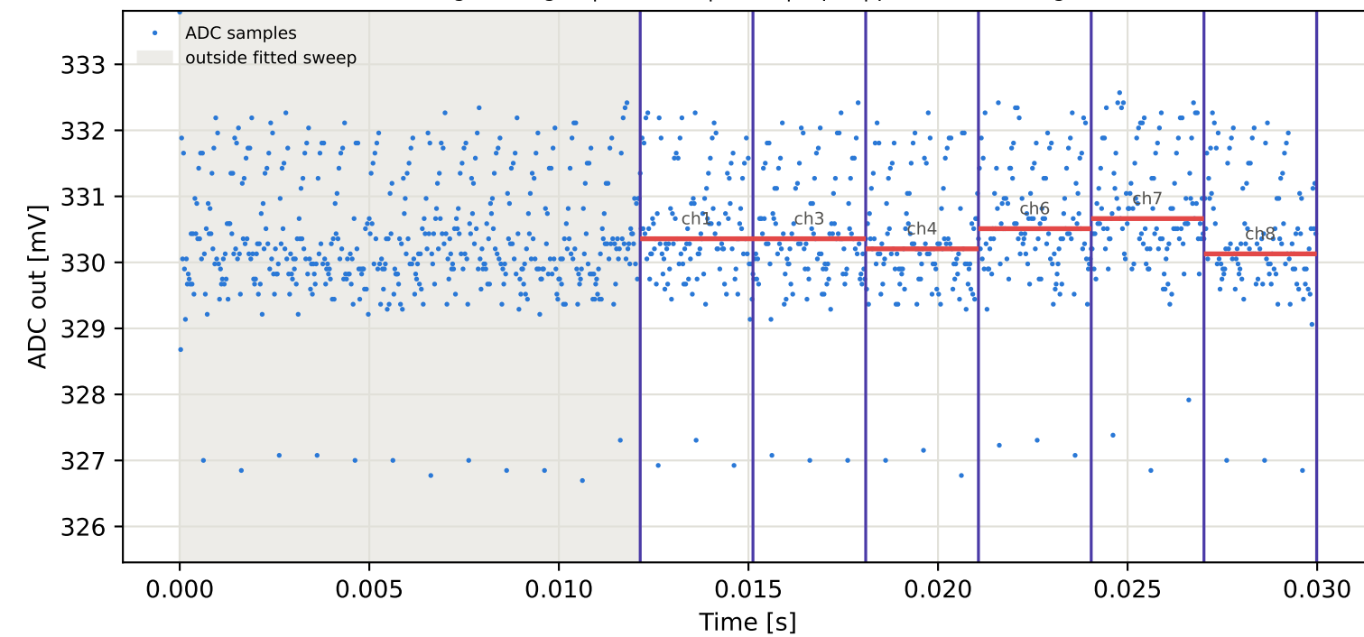
Tag5 &lt;- Tag16 | 805 MHz | run 0 | rep 1 | phase 70.70 deg
