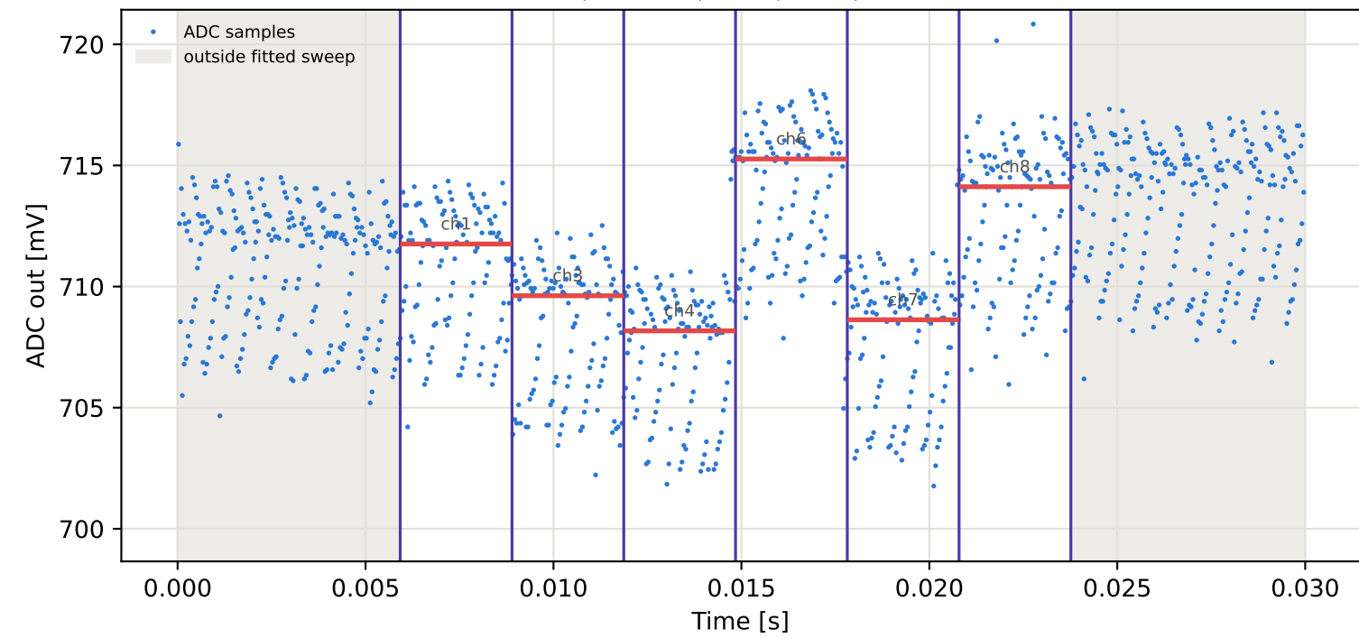
Tag15 &lt;- Tag6 | 975 MHz | run 0 | rep 1 | phase 140.10 deg
