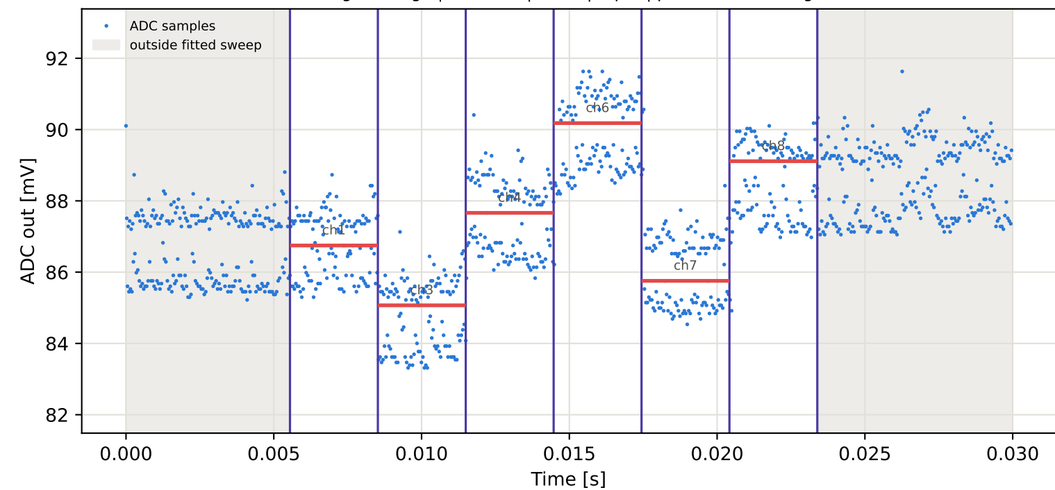
Tag6 &lt;- Tag5 | 785 MHz | run 0 | rep 1 | phase -160.34 deg
