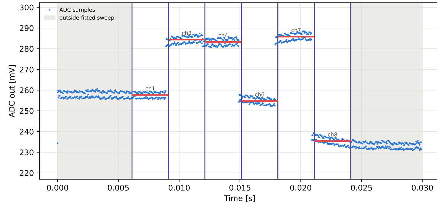
Tag15 &lt;- Tag1 | 875 MHz | run 0 | rep 1 | phase -4.08 deg
