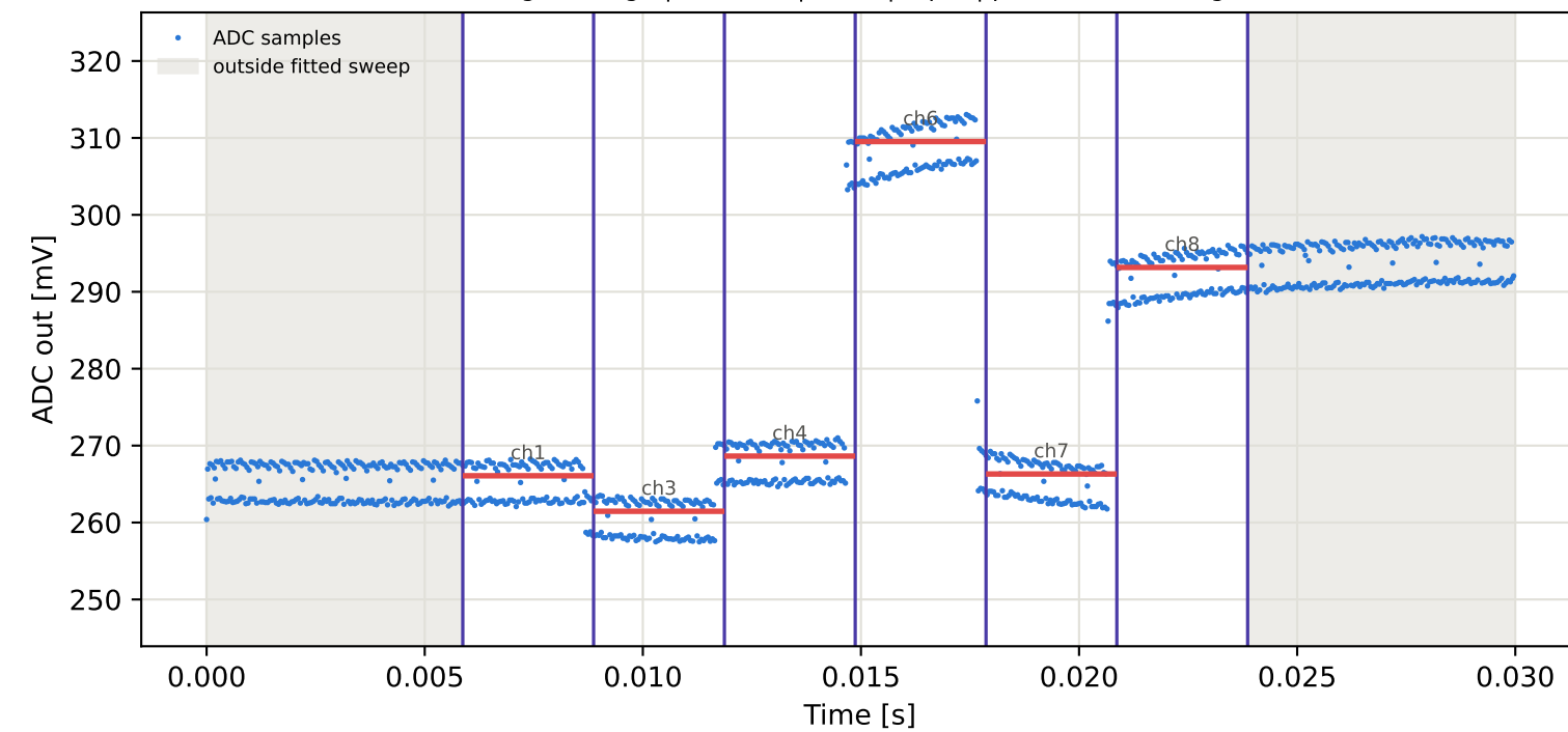
Tag1 &lt;- Tag7 | 905 MHz | run 0 | rep 1 | phase -179.66 deg
