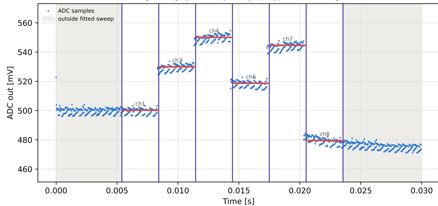
Tag6 &lt;- Tag5 | 895 MHz | run 0 | rep 1 | phase -55.34 deg
