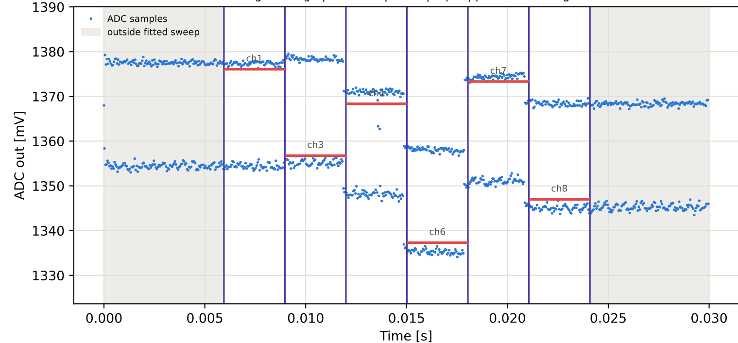
Tag5 &lt;- Tag9 | 915 MHz | run 0 | rep 1 | phase 164.31 deg
