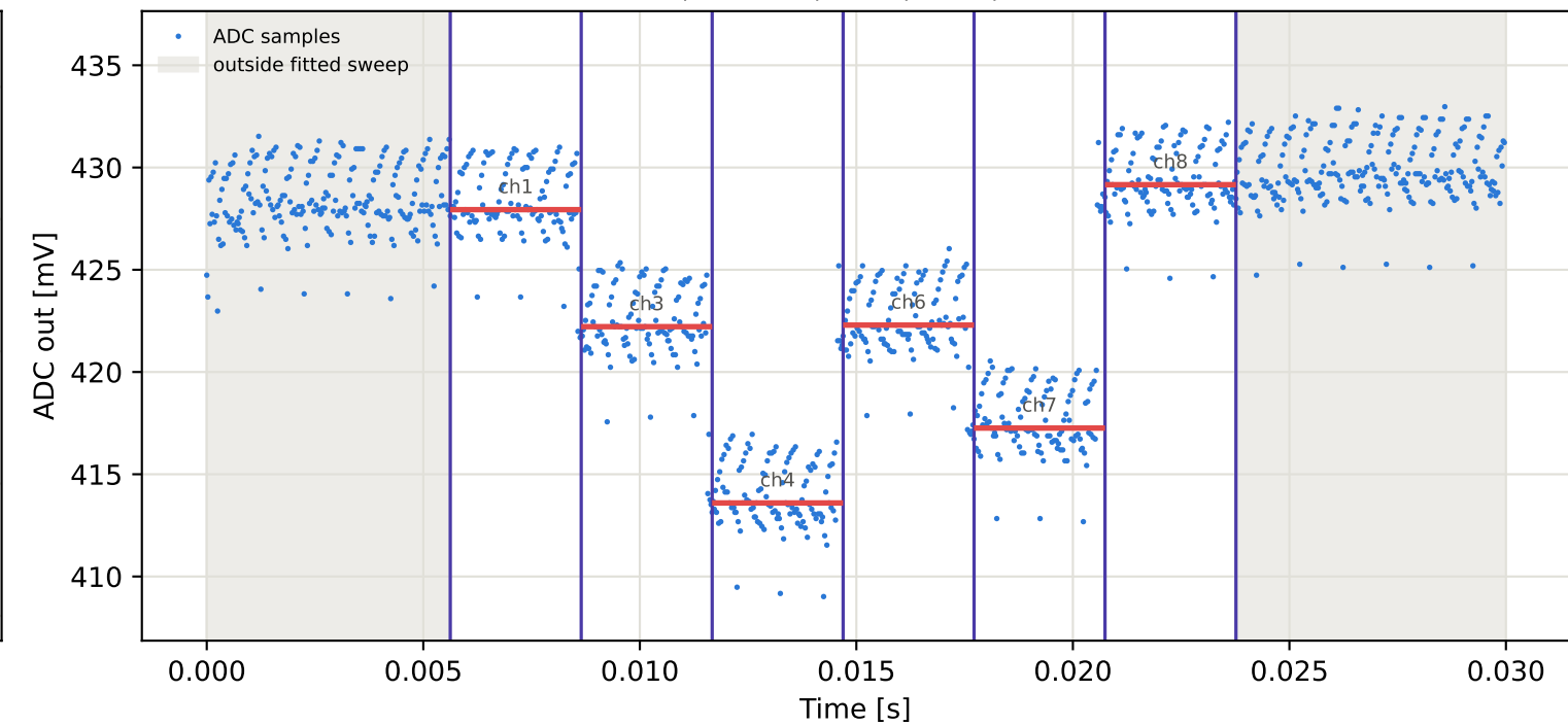
Tag10 &lt;- Tag1 | 935 MHz | run 0 | rep 1 | phase 85.34 deg
