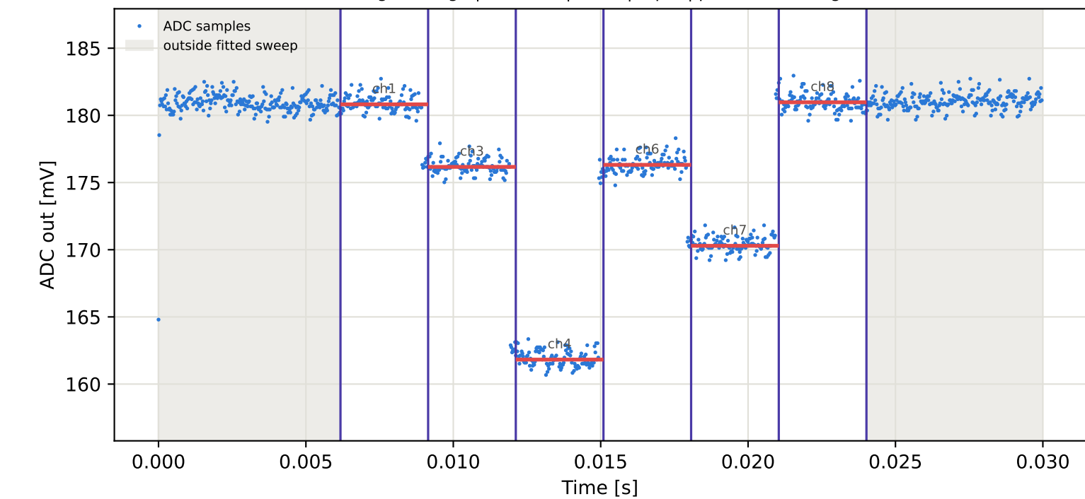
Tag7 &lt;- Tag10 | 995 MHz | run 0 | rep 1 | phase -80.93 deg
