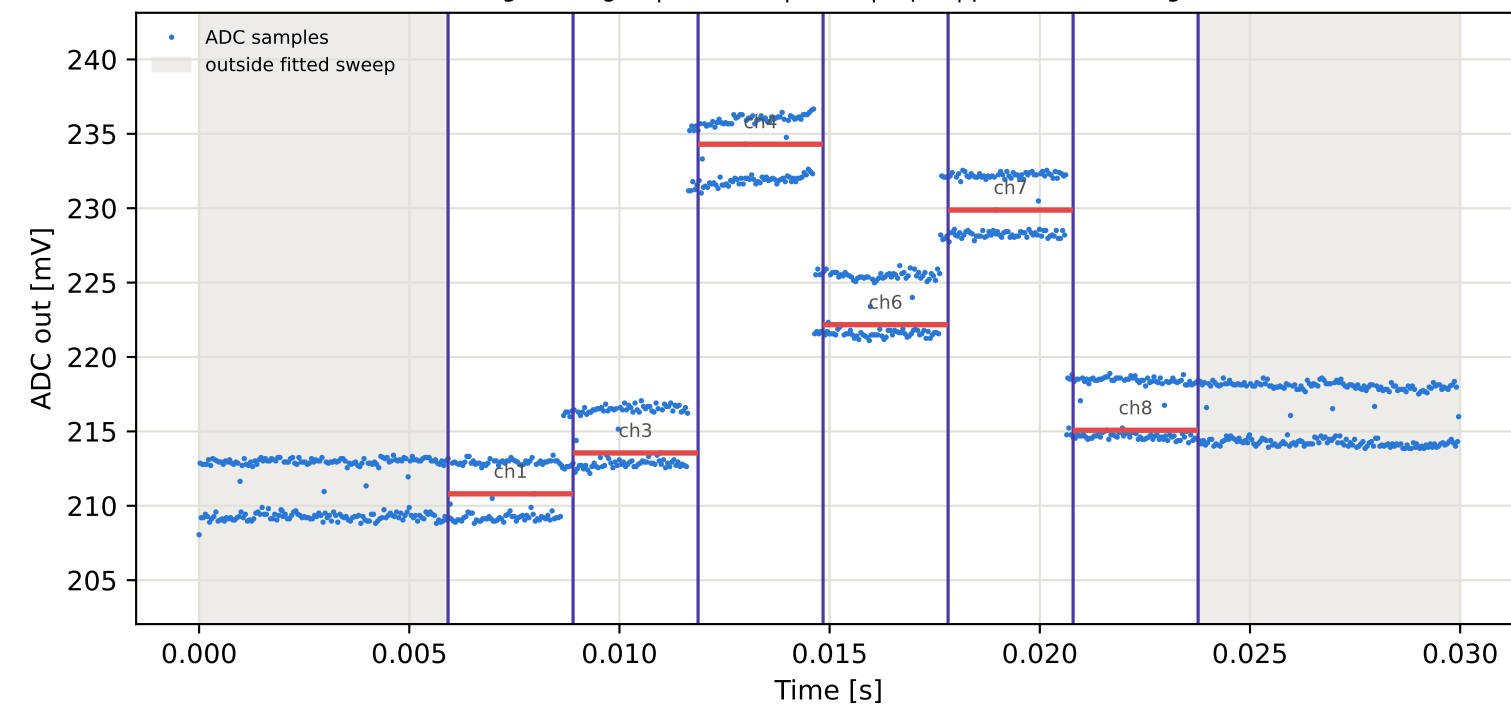
Tag8 &lt;- Tag15 | 805 MHz | run 0 | rep 1 | phase -94.40 deg
