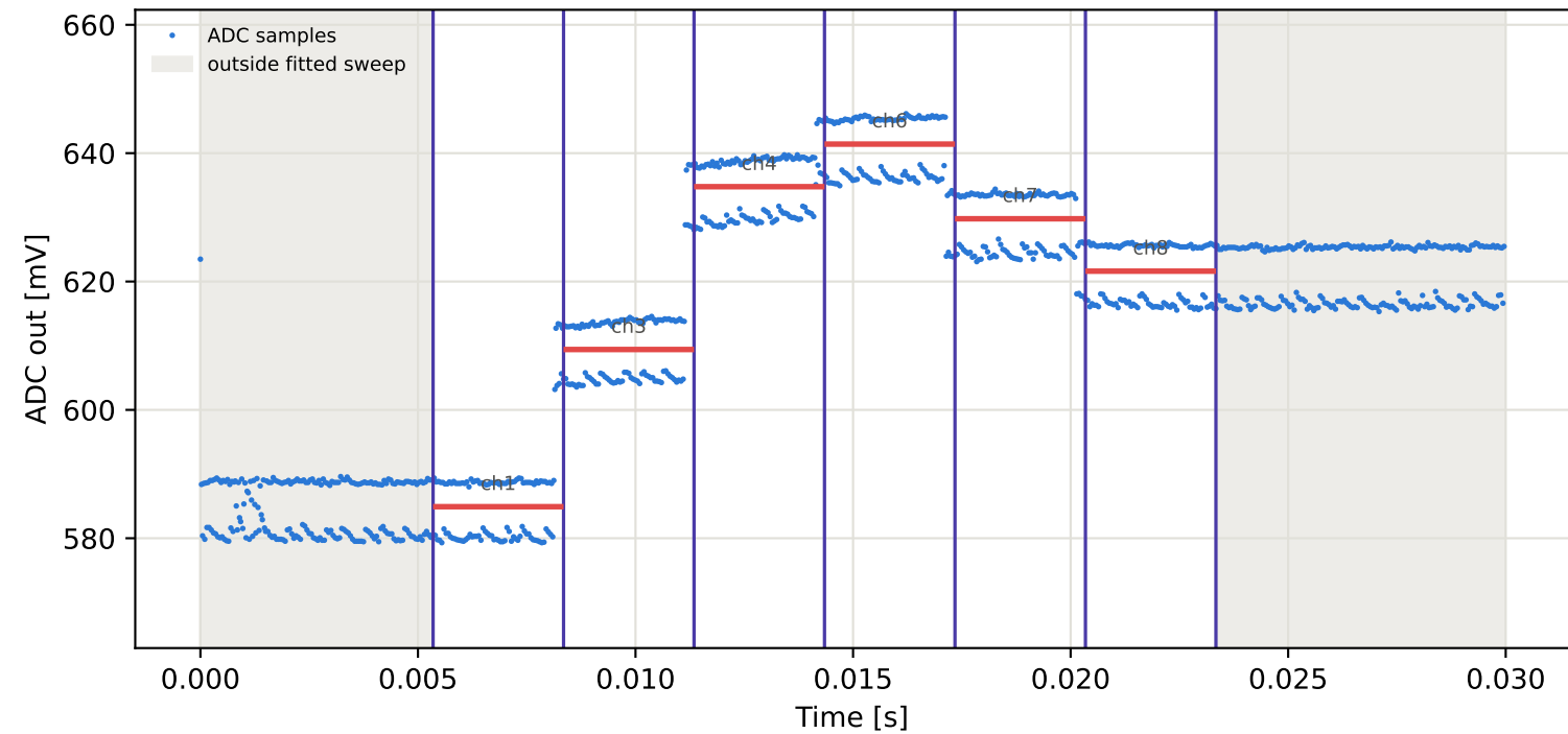
Tag6 &lt;- Tag5 | 855 MHz | run 0 | rep 1 | phase -111.59 deg
