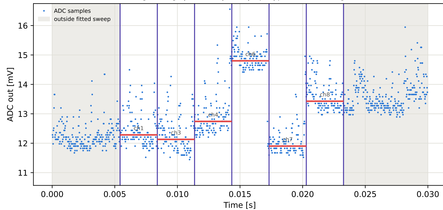
Tag3 &lt;- Tag10 | 955 MHz | run 0 | rep 1 | phase 73.88 deg
