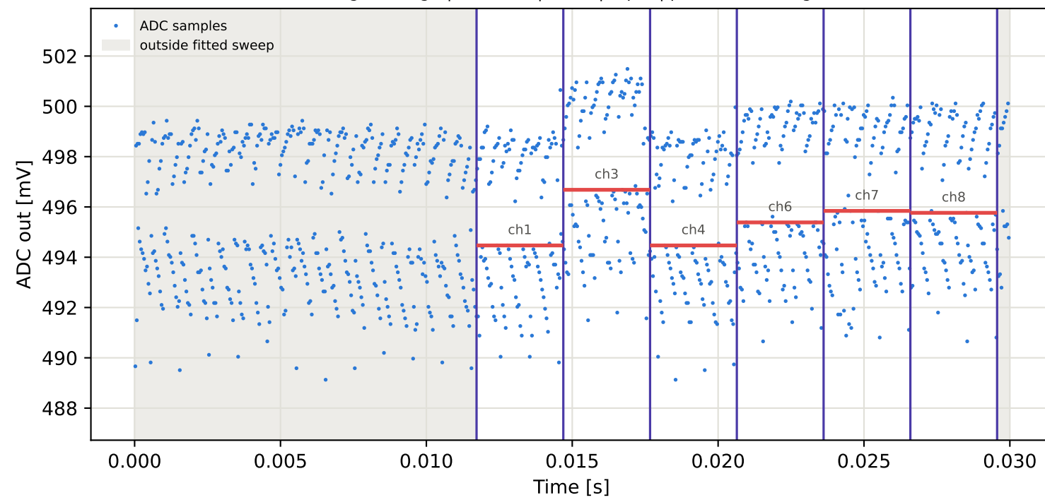
Tag8 &lt;- Tag4 | 975 MHz | run 0 | rep 1 | phase -107.92 deg
