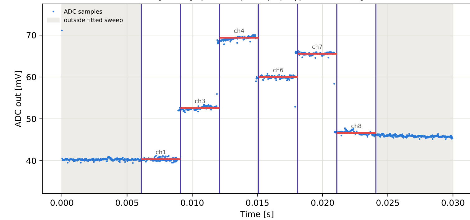
Tag9 &lt;- Tag7 | 825 MHz | run 0 | rep 1 | phase -98.93 deg
