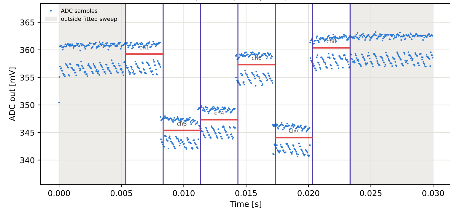
Tag15 &lt;- Tag3 | 825 MHz | run 0 | rep 1 | phase -14.14 deg
