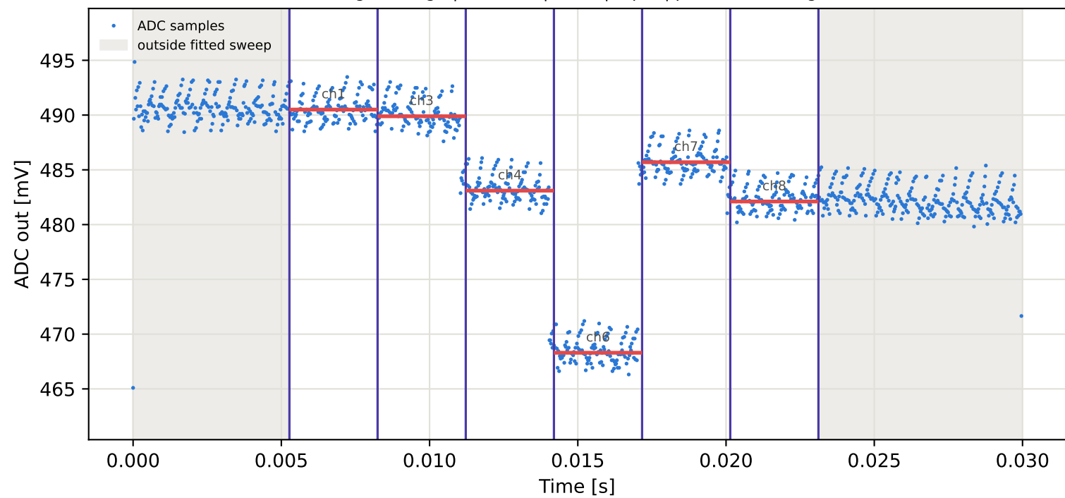
Tag9 &lt;- Tag6 | 925 MHz | run 0 | rep 1 | phase -55.52 deg
