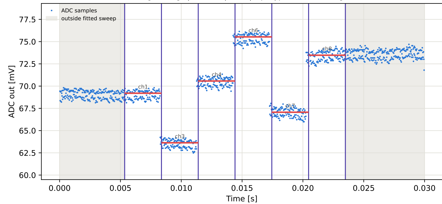
Tag4 &lt;- Tag8 | 805 MHz | run 0 | rep 1 | phase -100.68 deg
