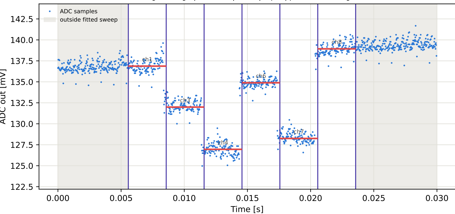
Tag2 &lt;- Tag7 | 925 MHz | run 0 | rep 1 | phase 99.42 deg
