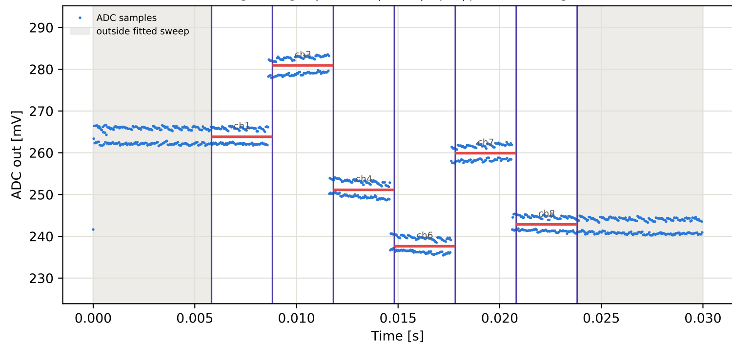
Tag7 &lt;- Tag3 | 835 MHz | run 0 | rep 1 | phase -120.97 deg
