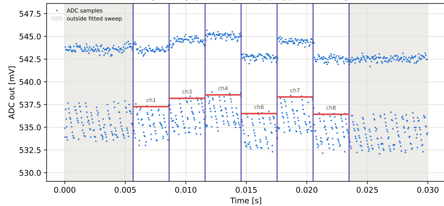
Tag15 &lt;- Tag4 | 965 MHz | run 0 | rep 1 | phase 87.26 deg
