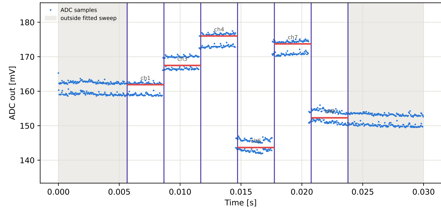
Tag6 &lt;- Tag5 | 995 MHz | run 0 | rep 1 | phase 87.21 deg
