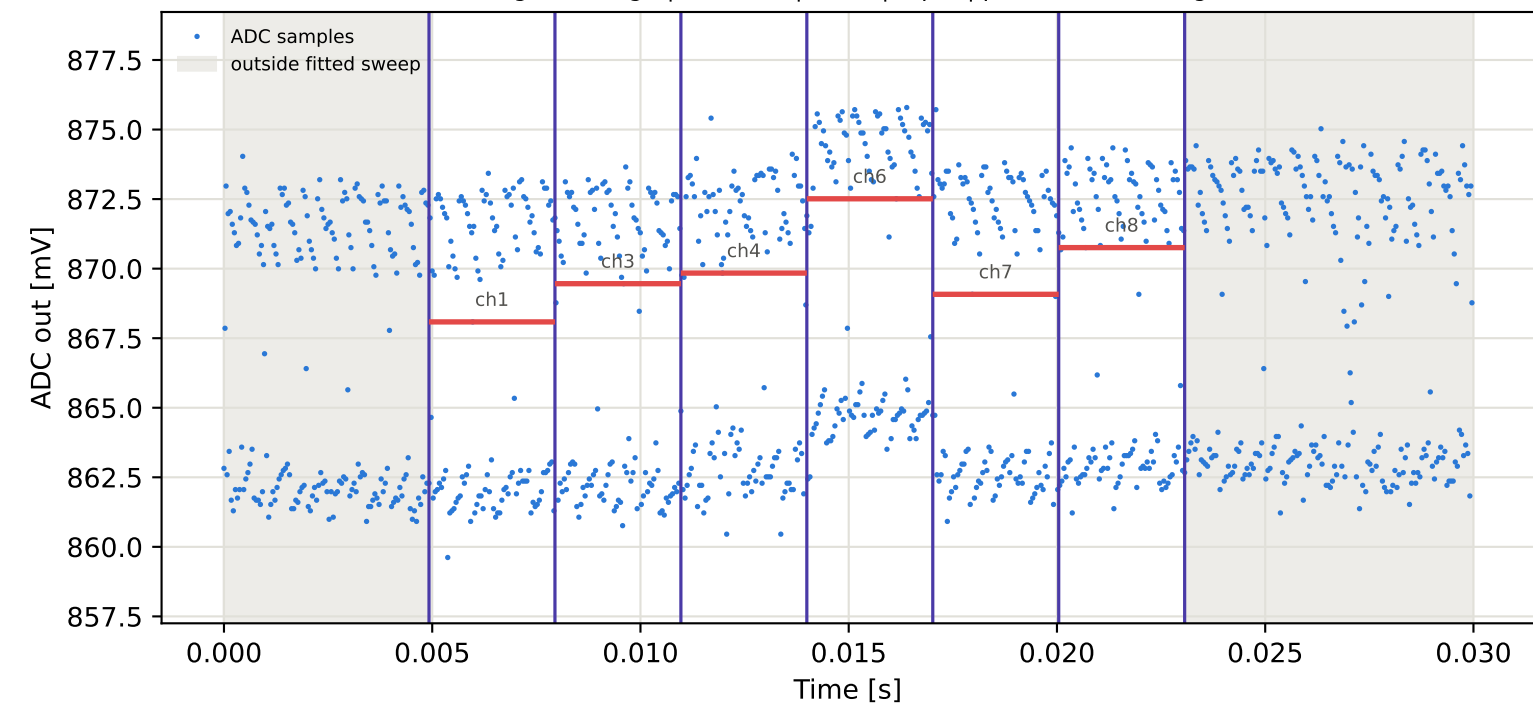
Tag16 &lt;- Tag4 | 875 MHz | run 0 | rep 1 | phase 130.04 deg
