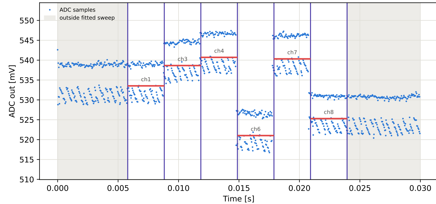
Tag15 &lt;- Tag5 | 965 MHz | run 0 | rep 1 | phase -106.93 deg
