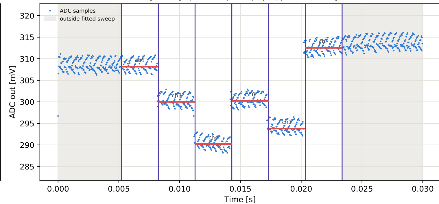
Tag4 &lt;- Tag3 | 915 MHz | run 0 | rep 1 | phase 87.98 deg
