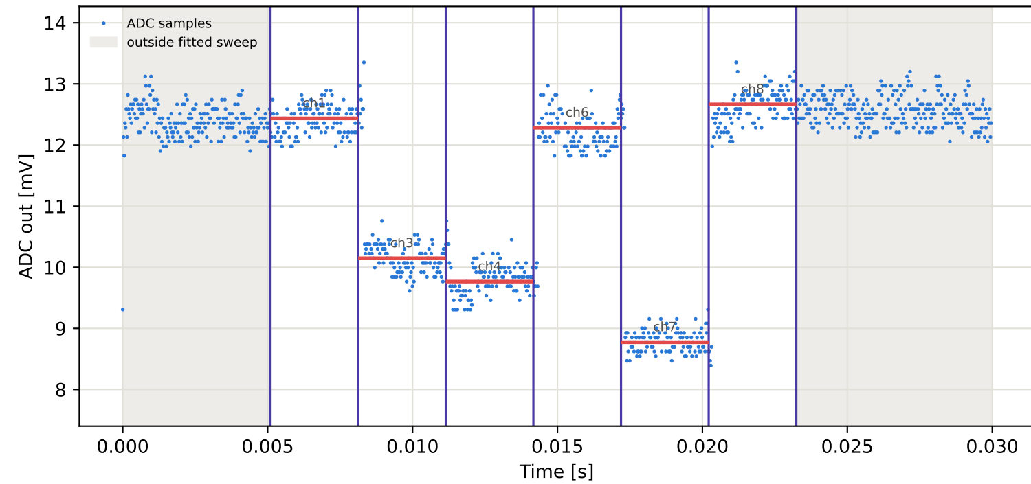
Tag3 &lt;- Tag9 | 775 MHz | run 0 | rep 1 | phase -156.51 deg
