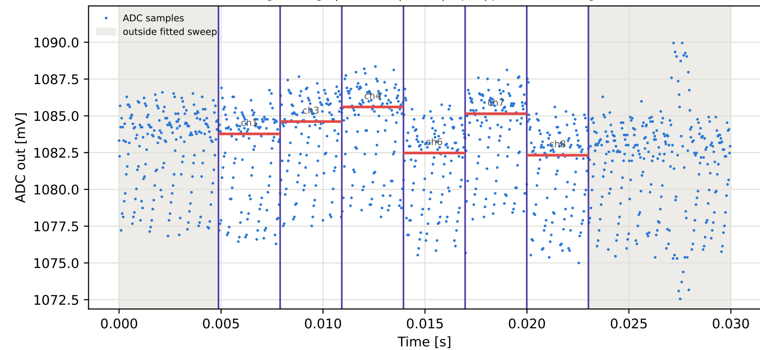
Tag8 &lt;- Tag4 | 905 MHz | run 0 | rep 1 | phase 7.85 deg
