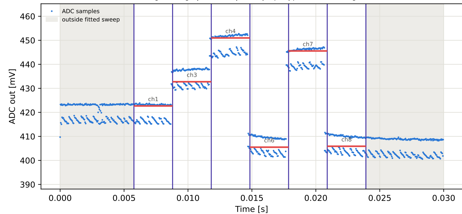
Tag9 &lt;- Tag8 | 935 MHz | run 0 | rep 1 | phase -55.97 deg
