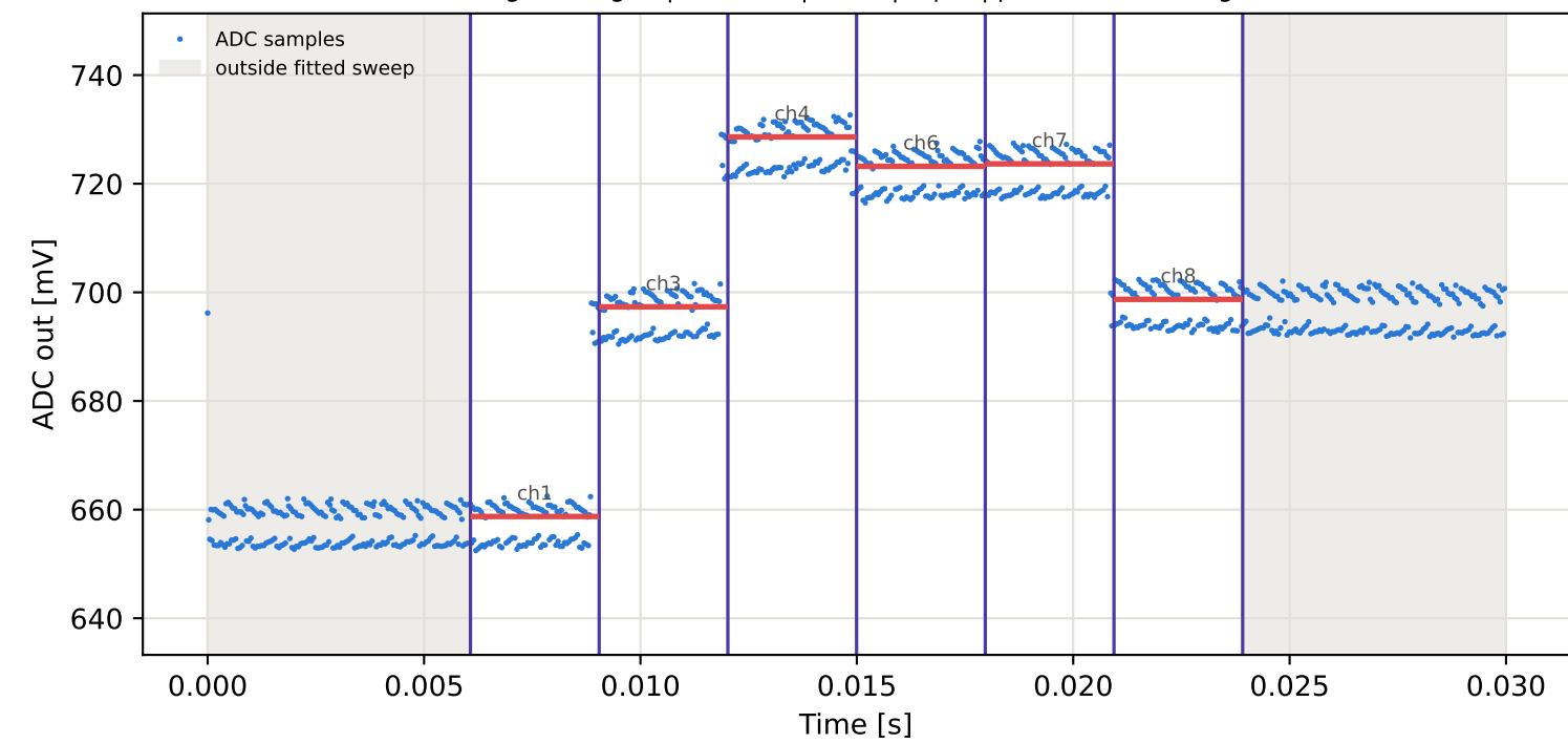
Tag8 &lt;- Tag16 | 855 MHz | run 0 | rep 1 | phase -111.49 deg
