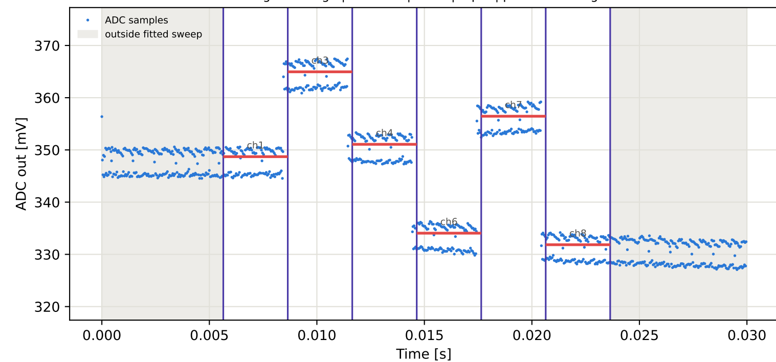
Tag15 &lt;- Tag5 | 855 MHz | run 0 | rep 1 | phase 0.73 deg
