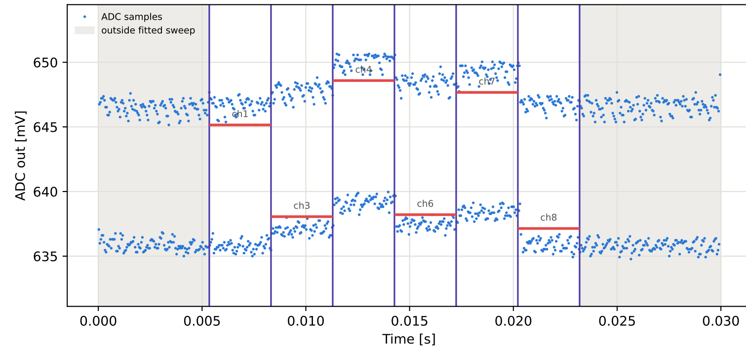
Tag4 &lt;- Tag9 | 925 MHz | run 0 | rep 1 | phase -133.62 deg
