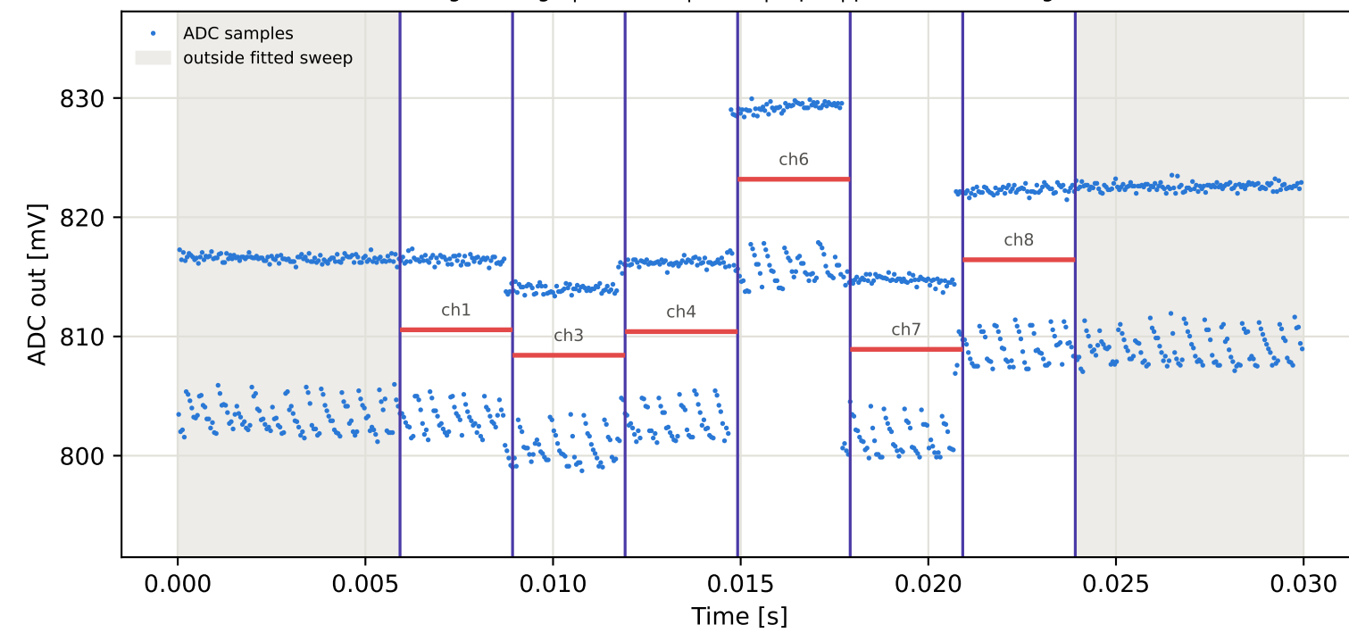
Tag8 &lt;- Tag6 | 935 MHz | run 0 | rep 1 | phase -179.55 deg
