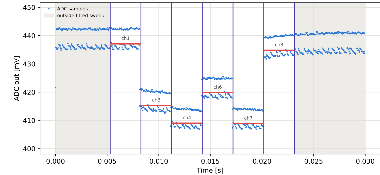
Tag5 &lt;- Tag3 | 855 MHz | run 0 | rep 1 | phase 97.02 deg
