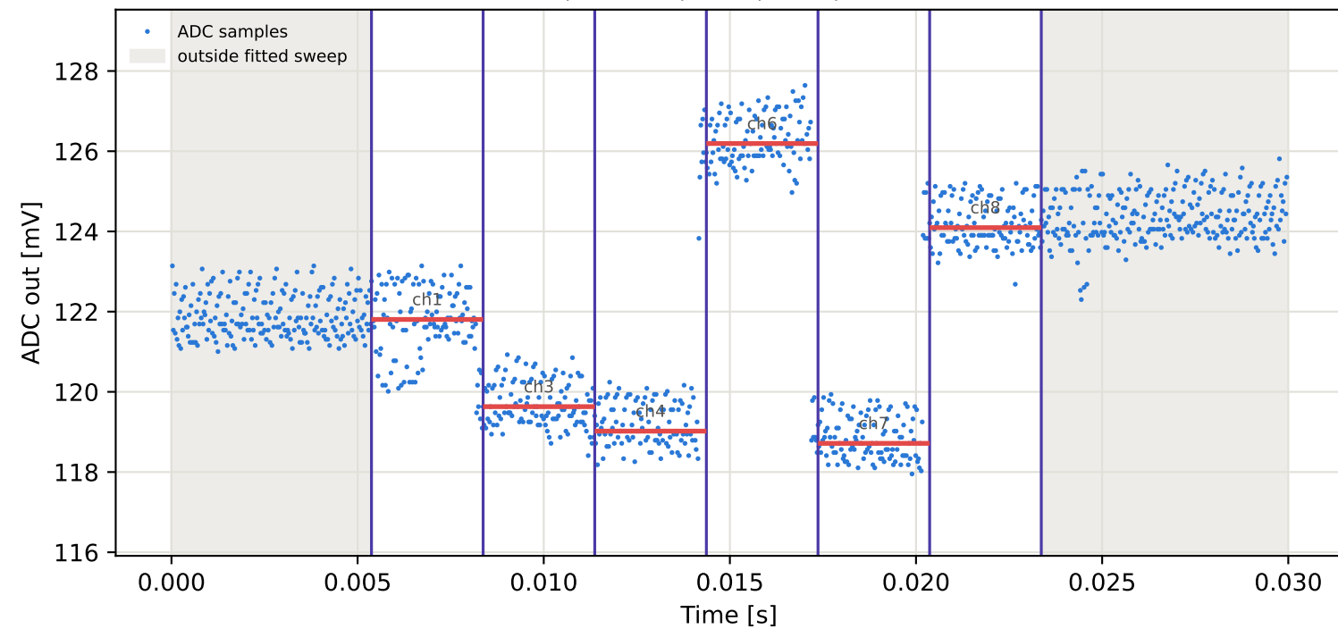
Tag1 &lt;- Tag4 | 995 MHz | run 0 | rep 1 | phase 151.46 deg
