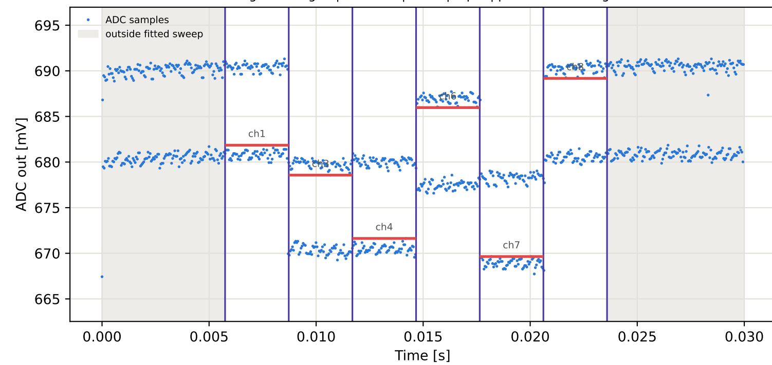
Tag15 &lt;- Tag3 | 835 MHz | run 0 | rep 1 | phase 18.46 deg
