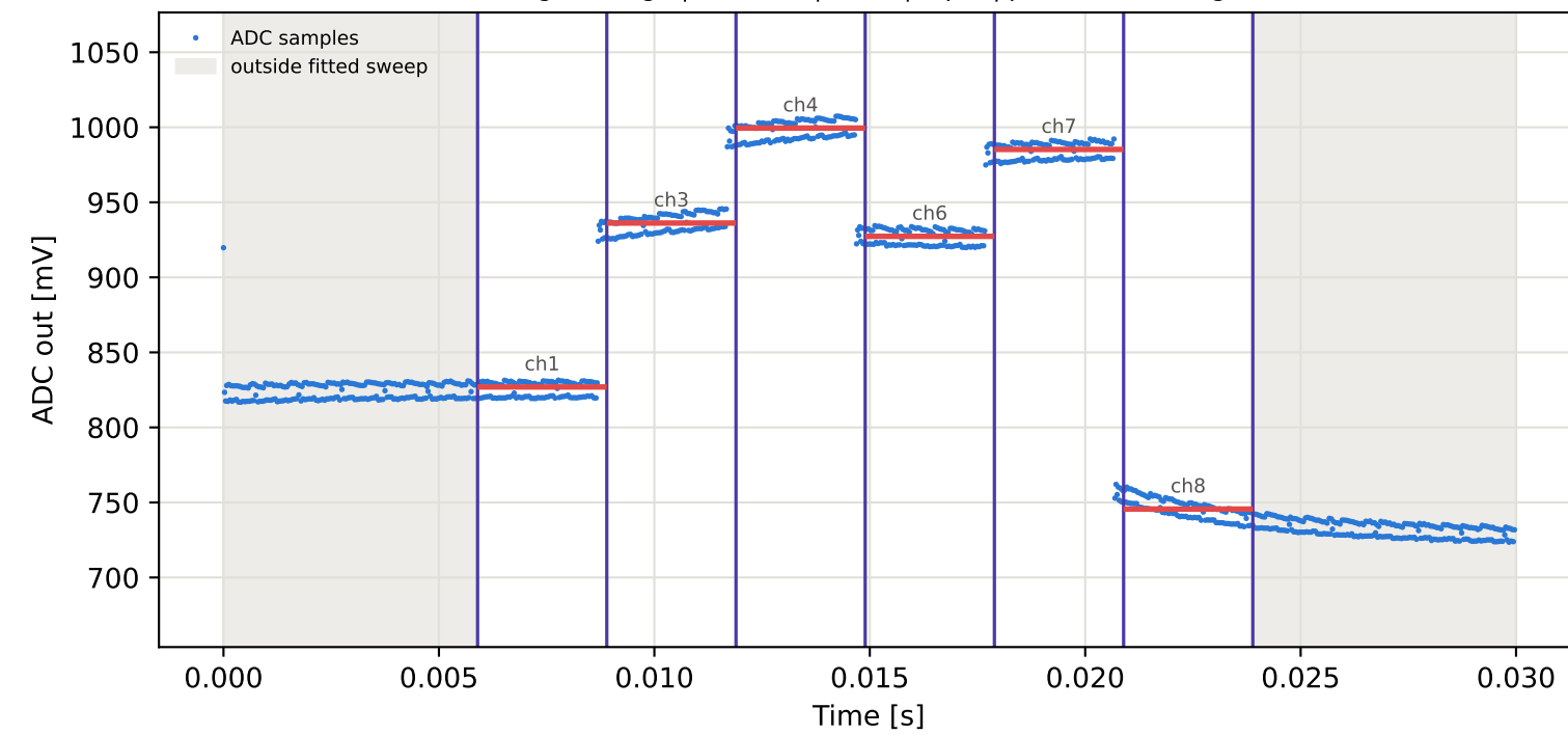
Tag4 &lt;- Tag7 | 895 MHz | run 0 | rep 1 | phase 48.03 deg
