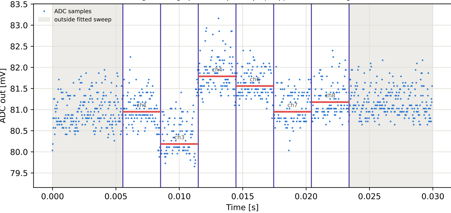
Tag10 &lt;- Tag4 | 775 MHz | run 0 | rep 1 | phase -127.43 deg
