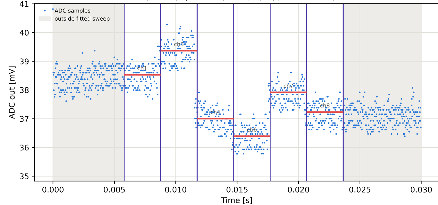
Tag1 &lt;- Tag9 | 785 MHz | run 0 | rep 1 | phase -1.80 deg
