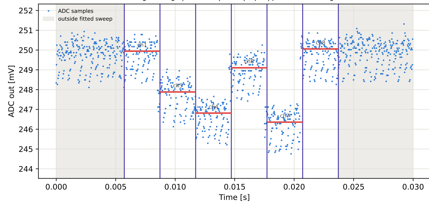
Tag5 &lt;- Tag9 | 785 MHz | run 0 | rep 1 | phase 4.70 deg
