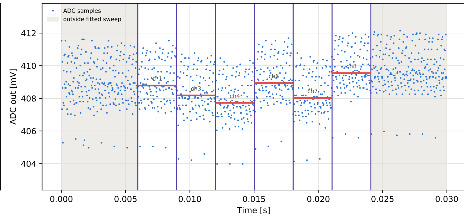
Tag3 &lt;- Tag2 | 855 MHz | run 0 | rep 1 | phase 123.01 deg
