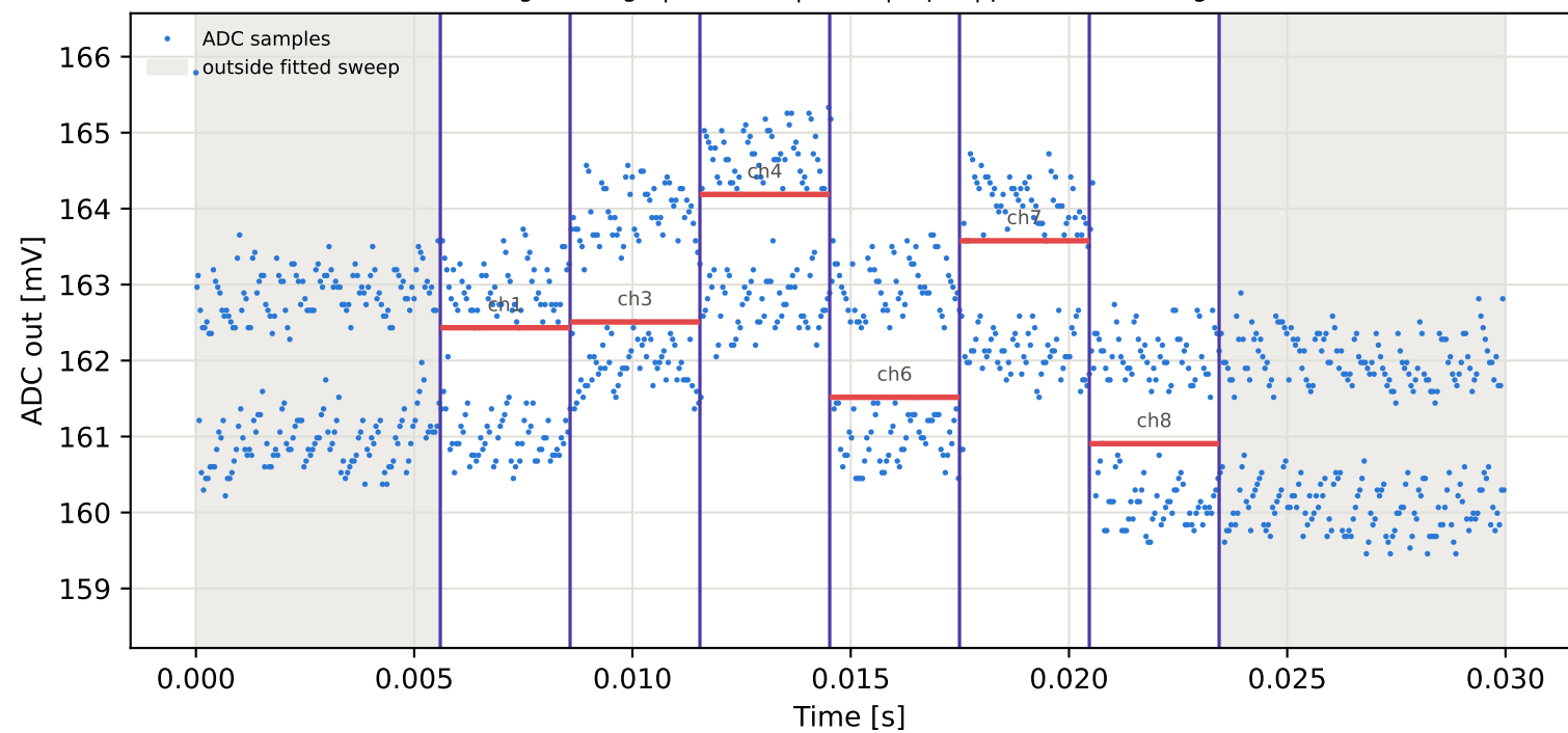
Tag9 &lt;- Tag2 | 965 MHz | run 0 | rep 1 | phase -69.57 deg
