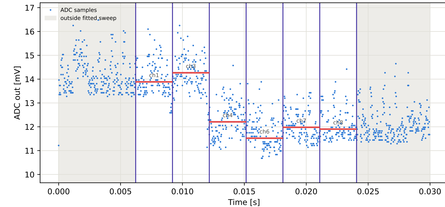
Tag2 &lt;- Tag15 | 855 MHz | run 0 | rep 1 | phase -143.77 deg
