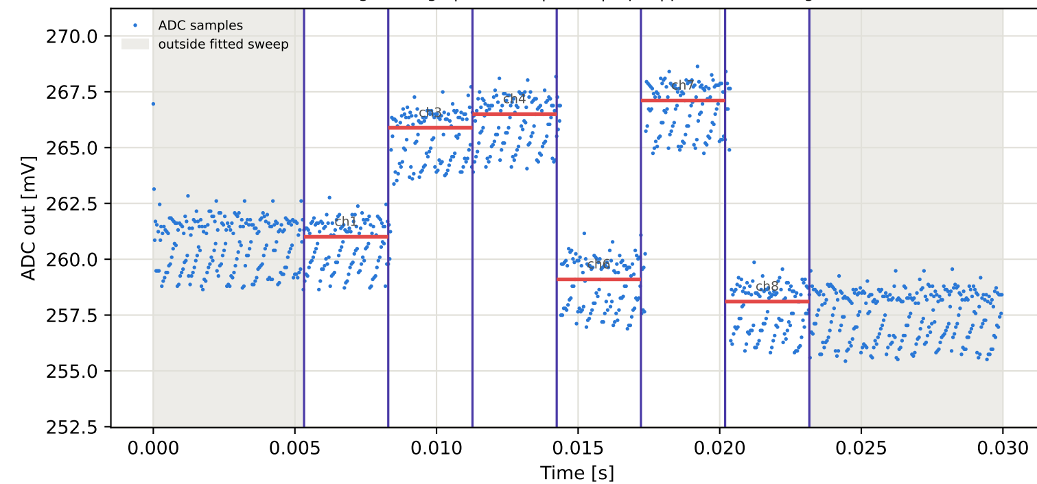
Tag4 &lt;- Tag9 | 845 MHz | run 0 | rep 1 | phase -51.31 deg
