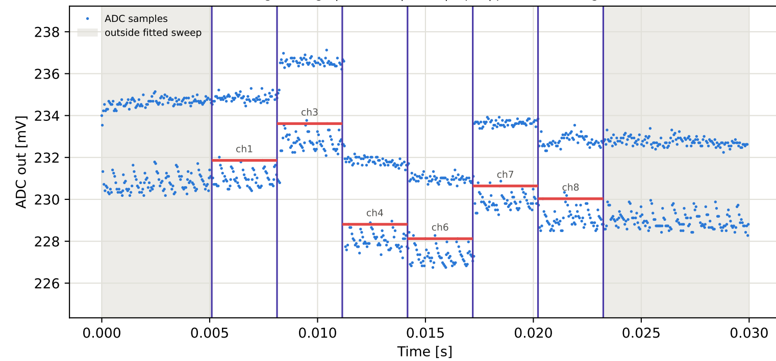
Tag9 &lt;- Tag10 | 805 MHz | run 0 | rep 1 | phase -177.78 deg
