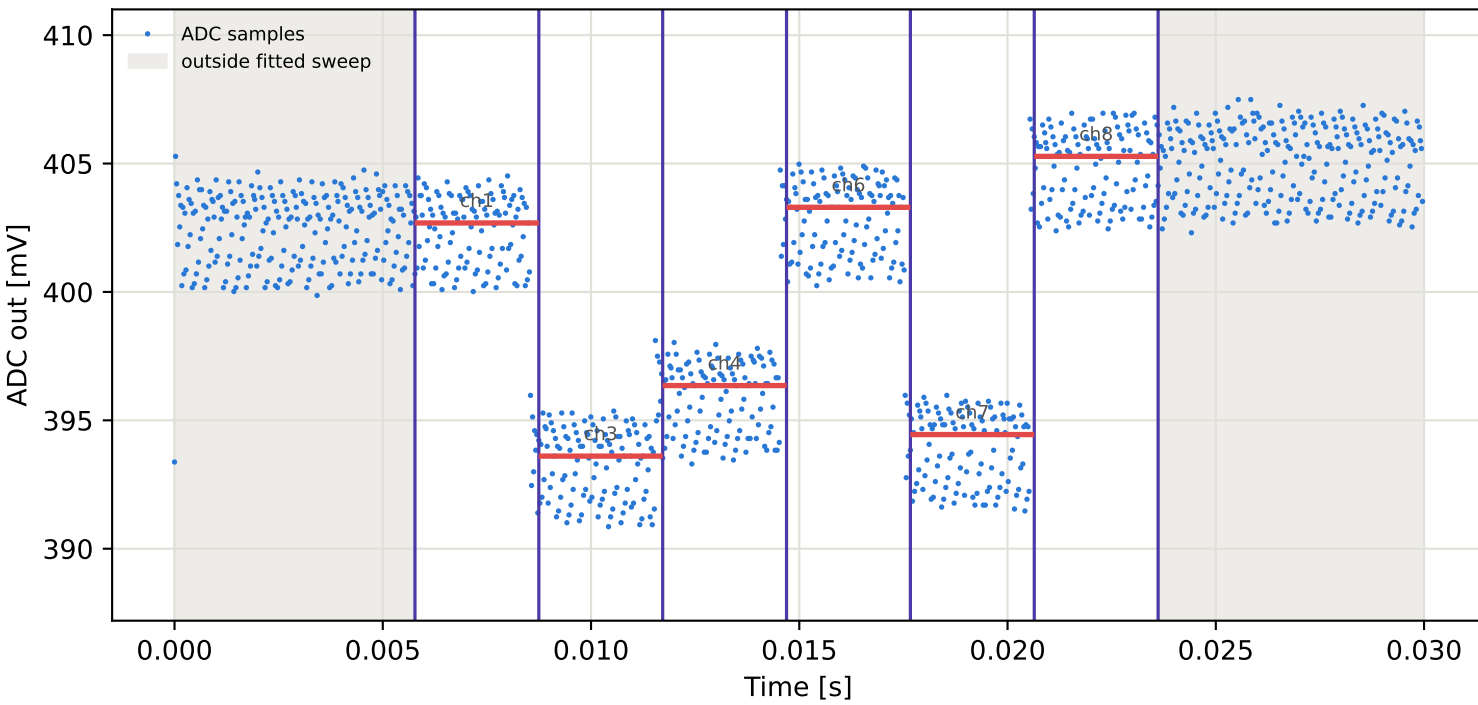
Tag3 &lt;- Tag16 | 835 MHz | run 0 | rep 1 | phase -116.12 deg
