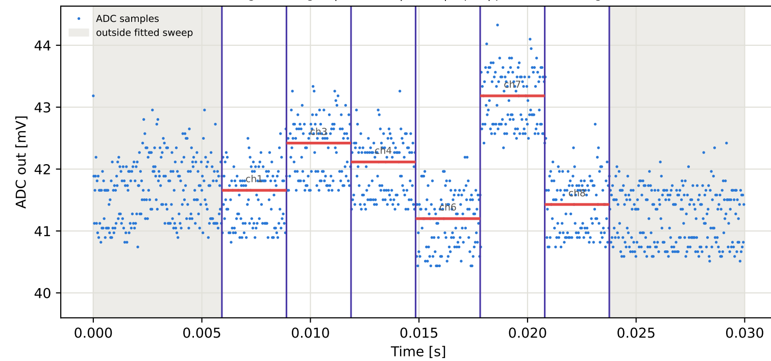
Tag15 &lt;- Tag3 | 775 MHz | run 0 | rep 1 | phase 149.88 deg
