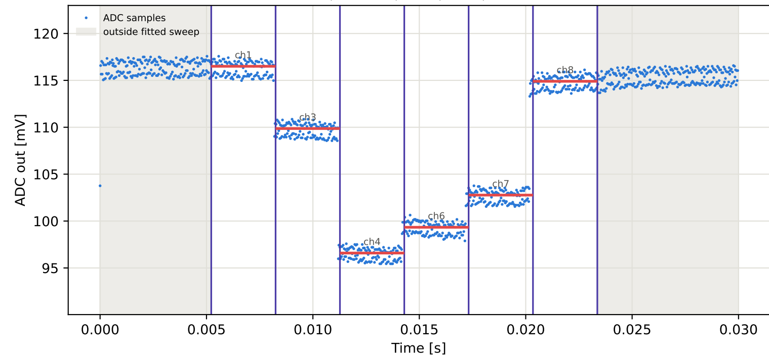
Tag1 &lt;- Tag4 | 935 MHz | run 0 | rep 1 | phase 60.70 deg
