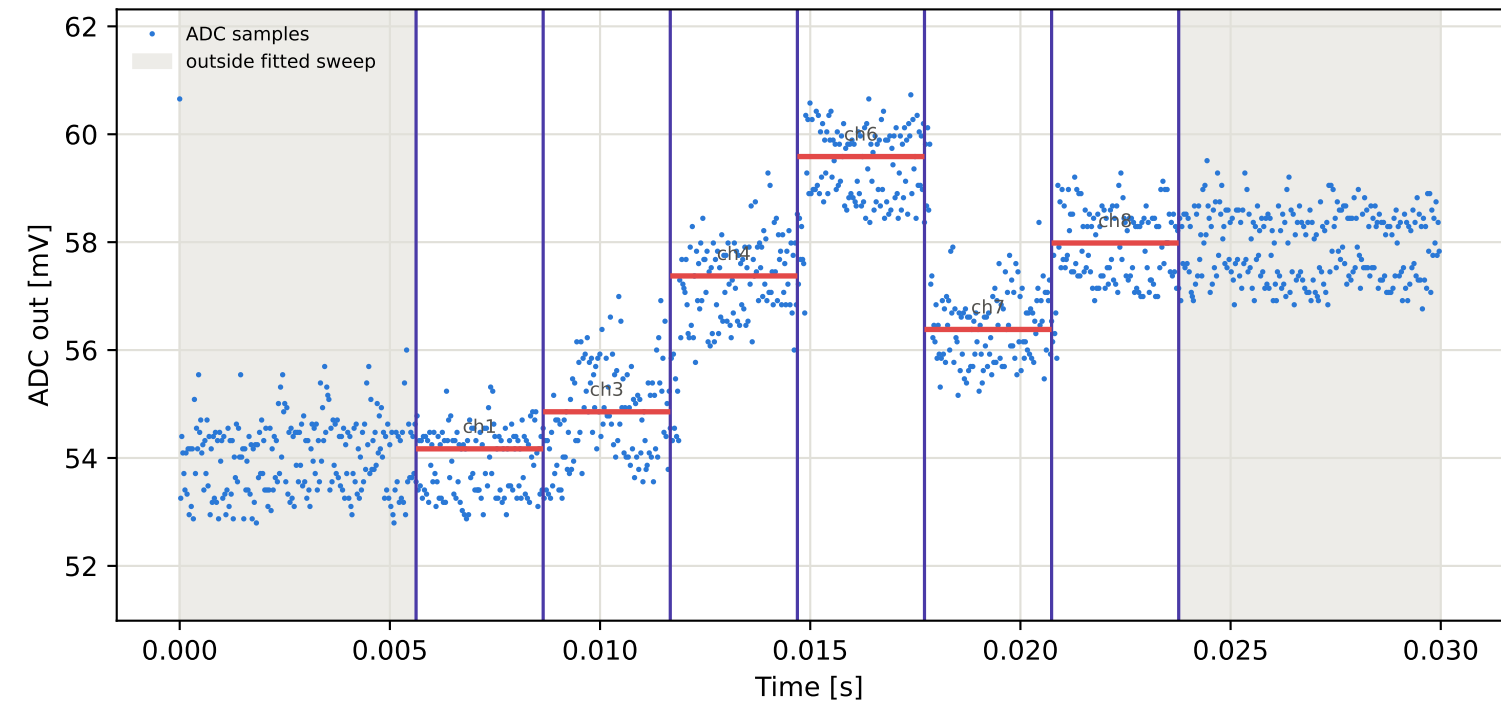
Tag2 &lt;- Tag16 | 875 MHz | run 0 | rep 1 | phase 99.64 deg
