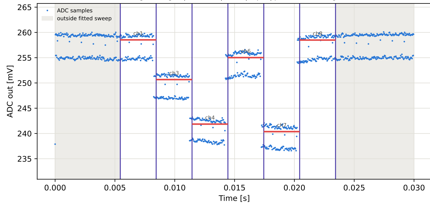
Tag5 &lt;- Tag2 | 795 MHz | run 0 | rep 1 | phase 0.28 deg
