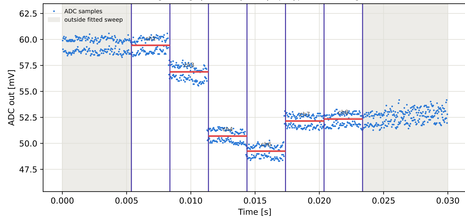
Tag9 &lt;- Tag6 | 845 MHz | run 0 | rep 1 | phase -53.31 deg
