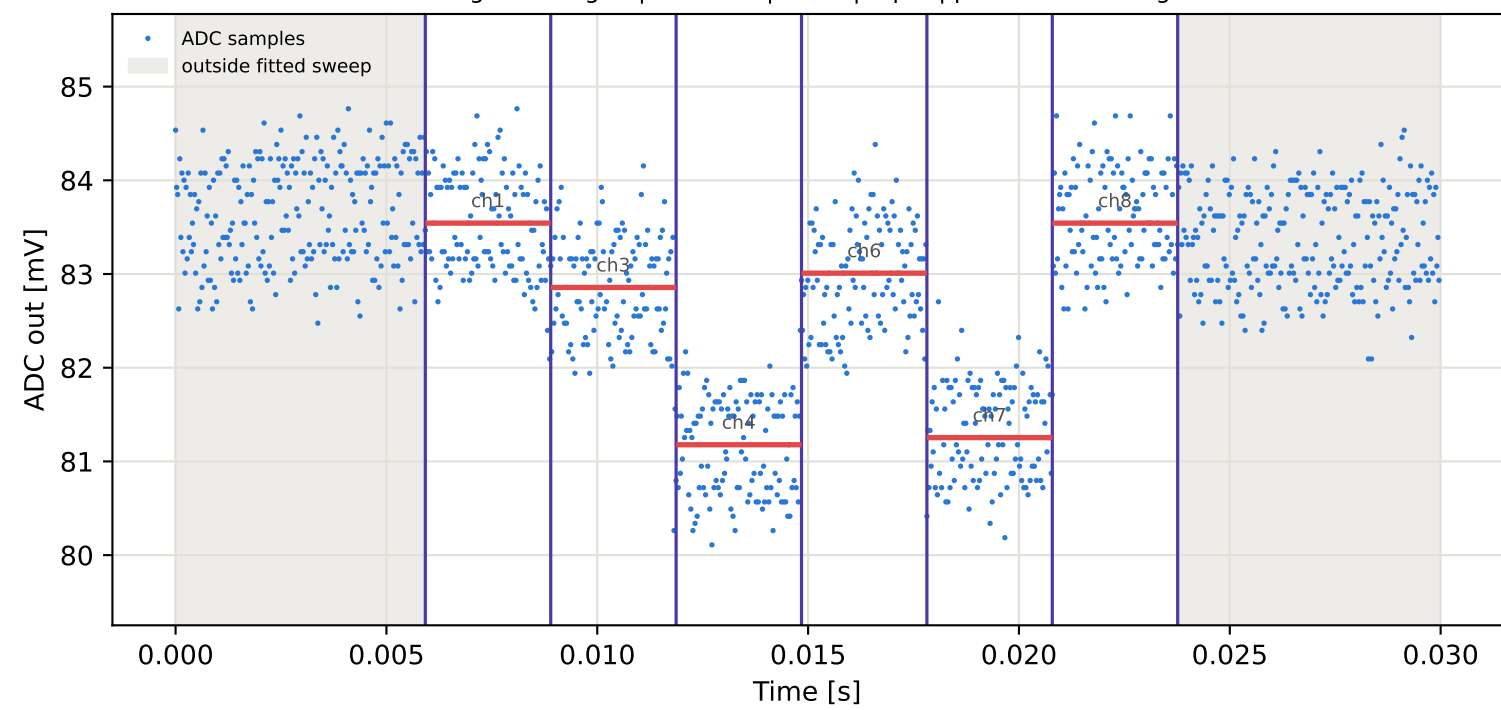
Tag10 &lt;- Tag3 | 775 MHz | run 0 | rep 1 | phase -72.74 deg
