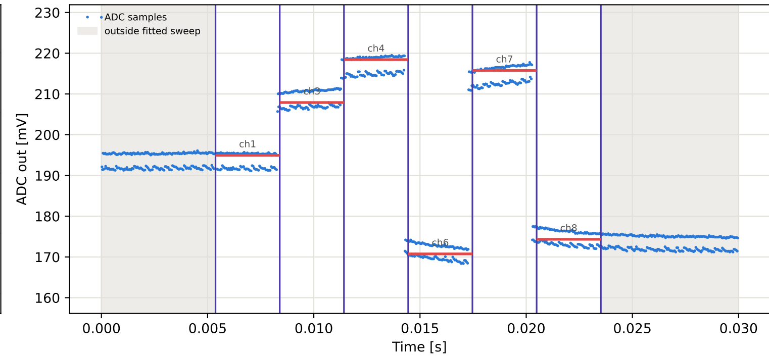
Tag9 &lt;- Tag2 | 945 MHz | run 0 | rep 1 | phase -170.55 deg
