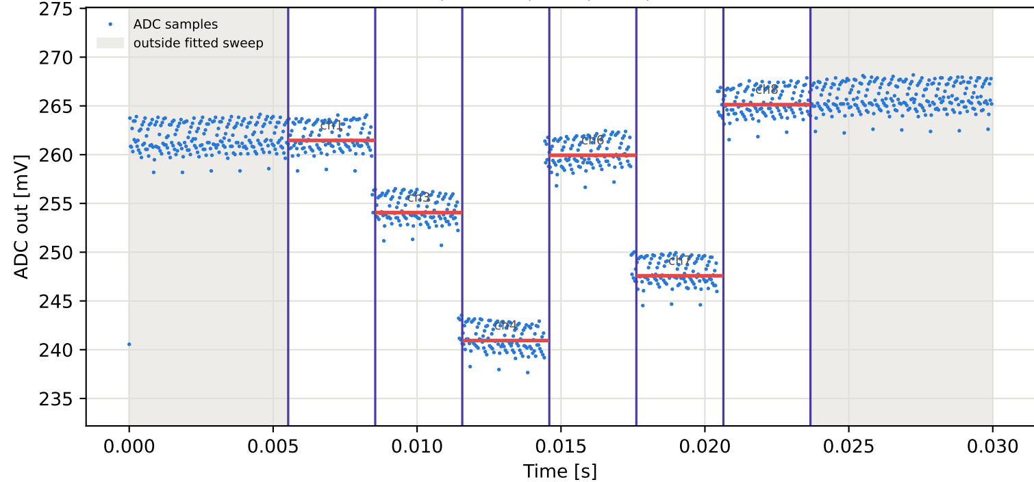
Tag1 &lt;- Tag4 | 955 MHz | run 0 | rep 1 | phase 96.30 deg
