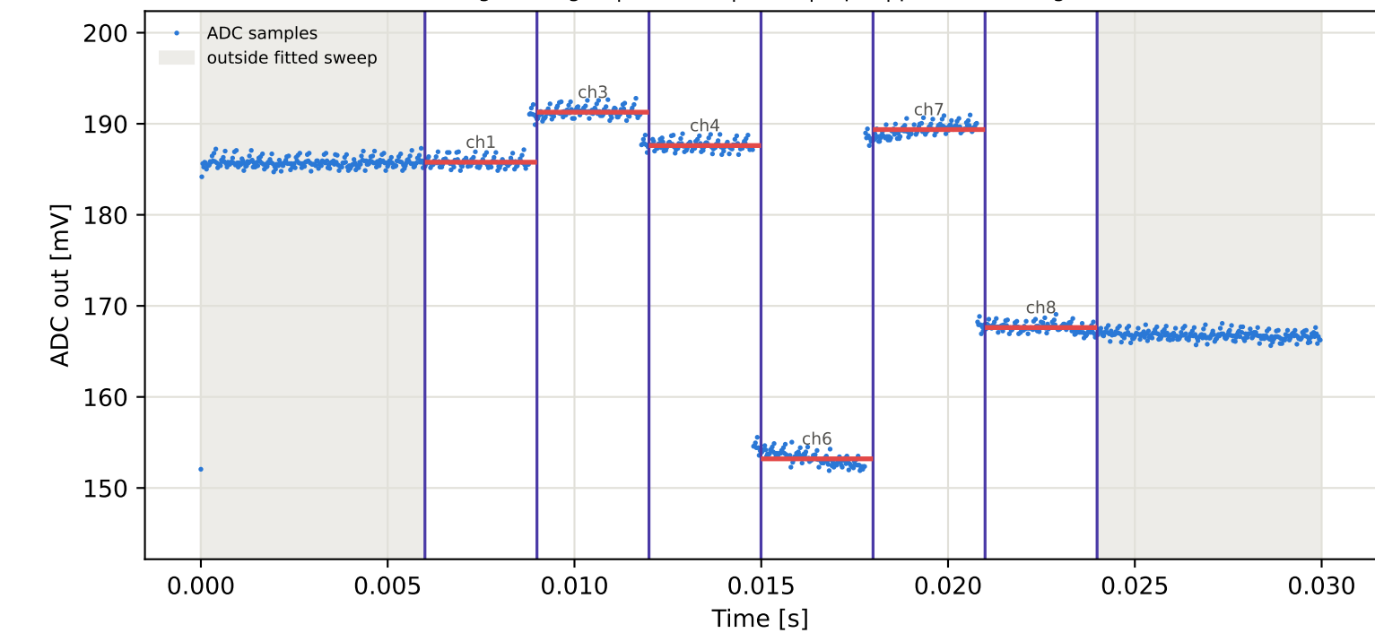
Tag3 &lt;- Tag16 | 915 MHz | run 0 | rep 1 | phase -60.18 deg
