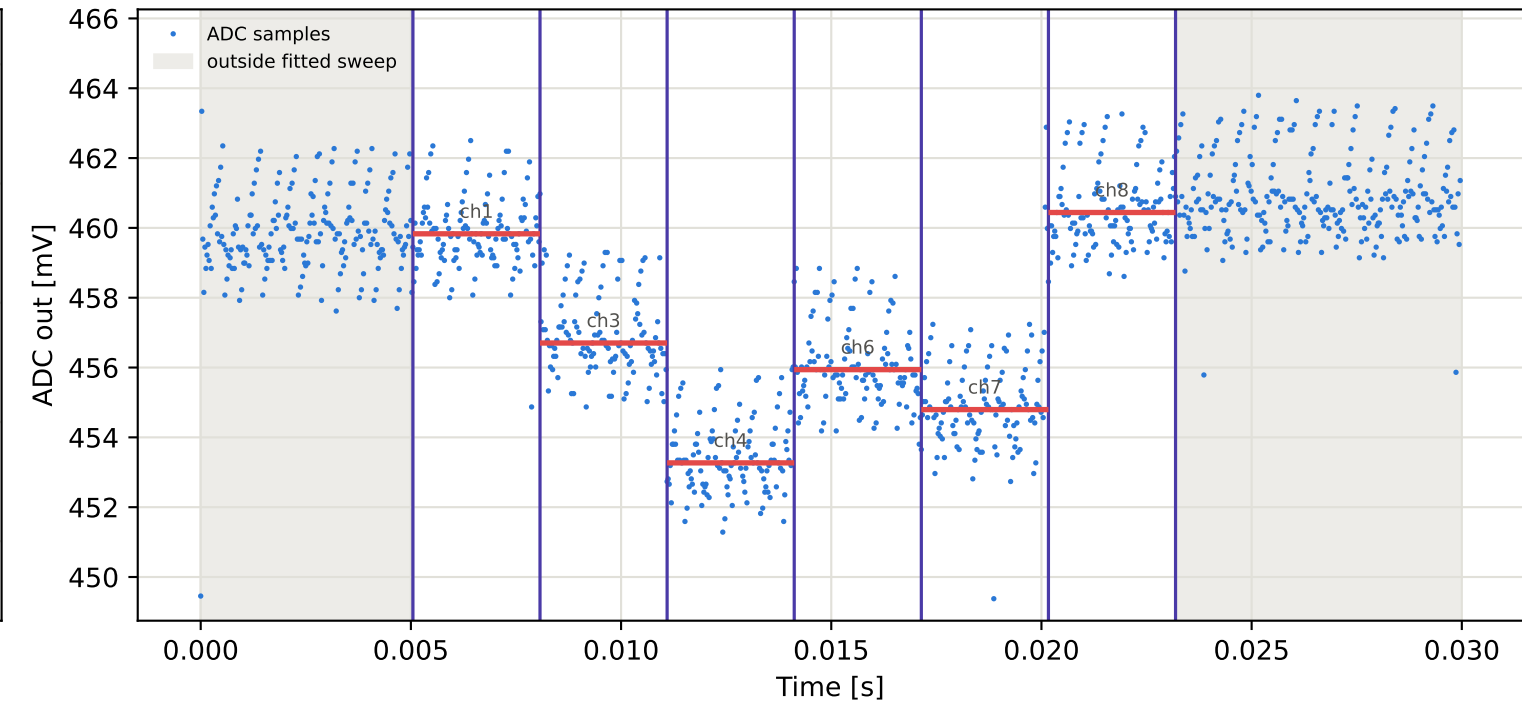
Tag7 &lt;- Tag15 | 915 MHz | run 0 | rep 1 | phase 114.29 deg
