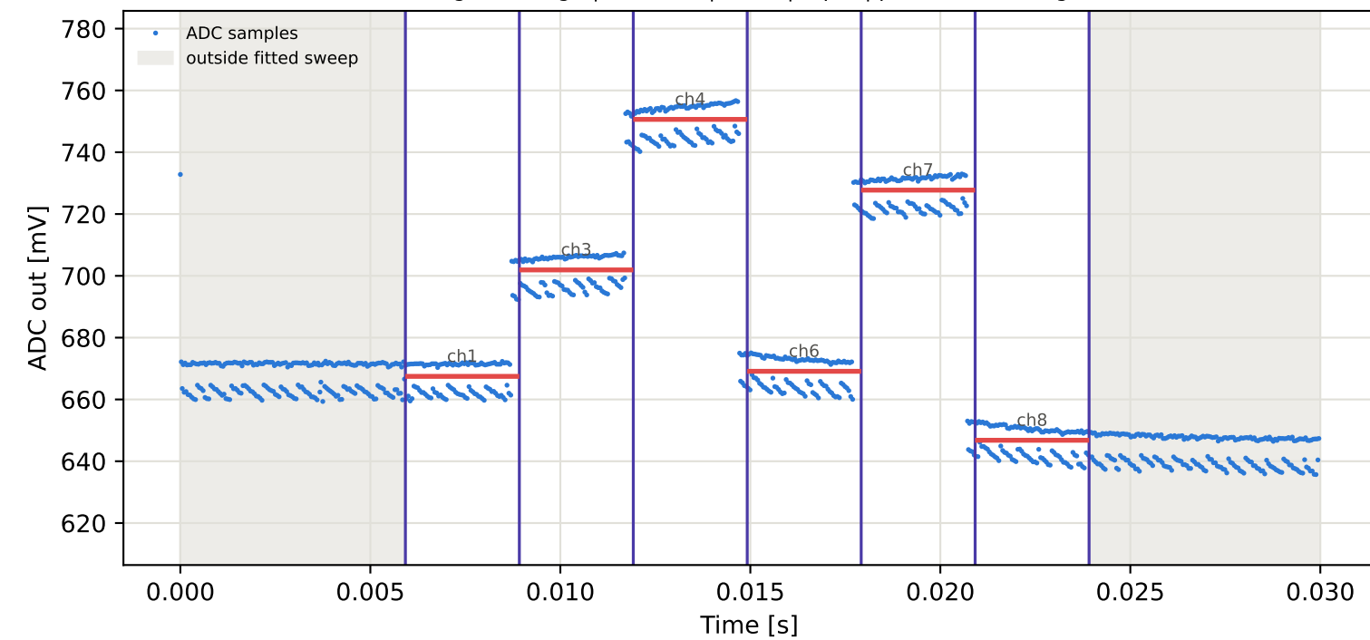
Tag2 &lt;- Tag1 | 945 MHz | run 0 | rep 1 | phase -146.05 deg
