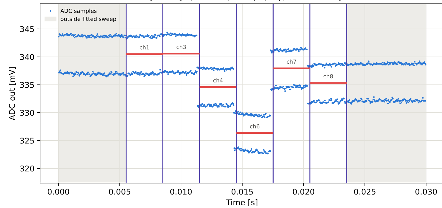
Tag7 &lt;- Tag5 | 955 MHz | run 0 | rep 1 | phase 22.38 deg
