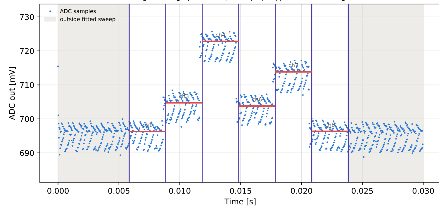
Tag15 &lt;- Tag9 | 975 MHz | run 0 | rep 1 | phase -58.93 deg
