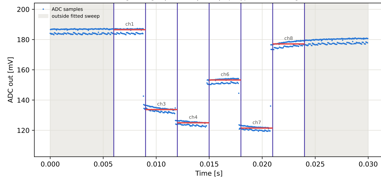
Tag7 &lt;- Tag3 | 855 MHz | run 0 | rep 1 | phase 23.62 deg
