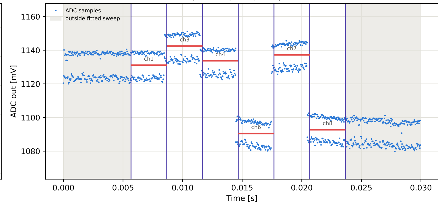
Tag8 &lt;- Tag5 | 885 MHz | run 0 | rep 1 | phase -71.66 deg
