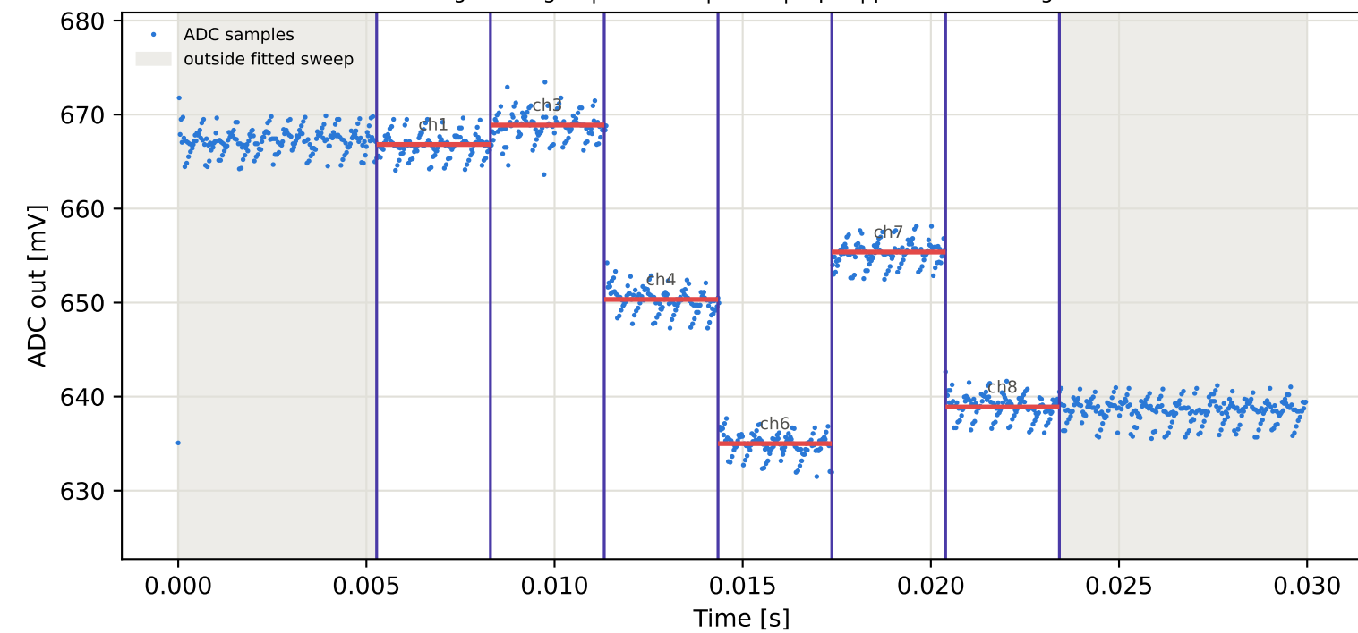
Tag6 &lt;- Tag2 | 865 MHz | run 0 | rep 1 | phase -126.55 deg
