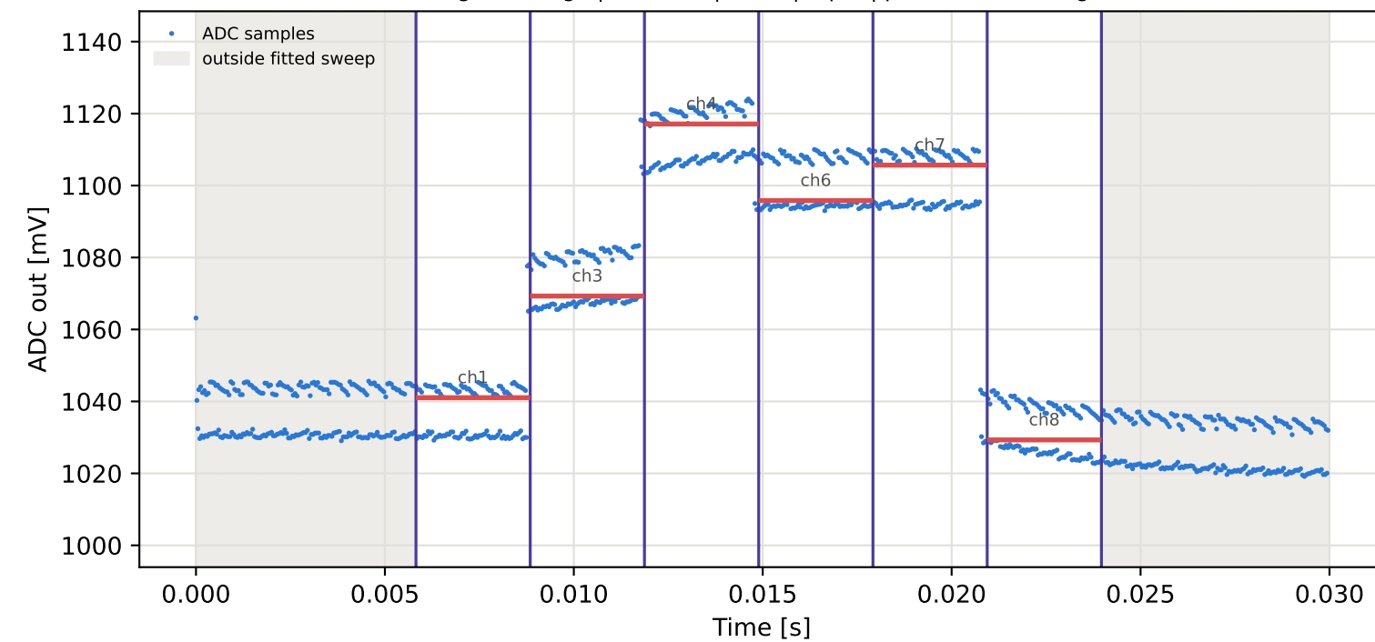
Tag16 &lt;- Tag6 | 905 MHz | run 0 | rep 1 | phase -39.80 deg
