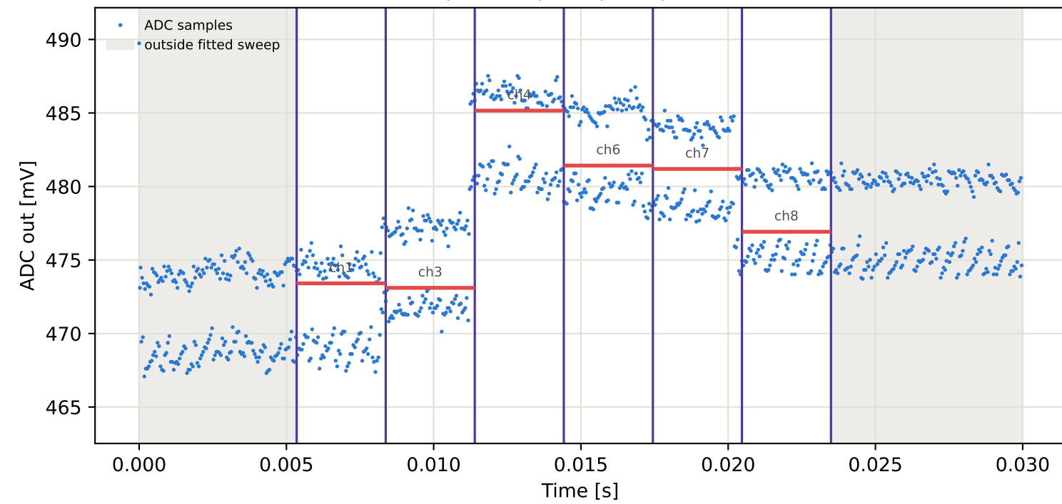
Tag6 &lt;- Tag5 | 845 MHz | run 0 | rep 1 | phase -115.45 deg
