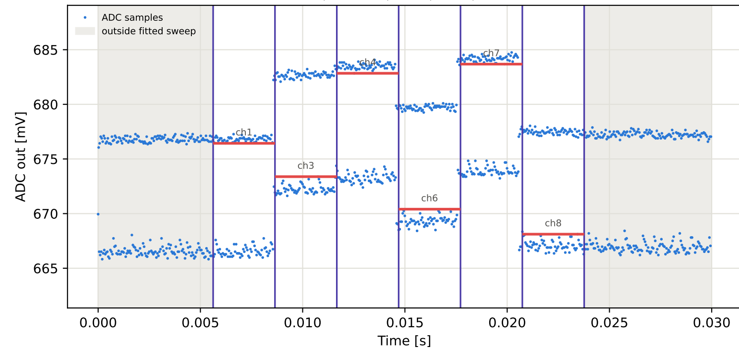
Tag15 &lt;- Tag10 | 835 MHz | run 0 | rep 1 | phase -53.13 deg
