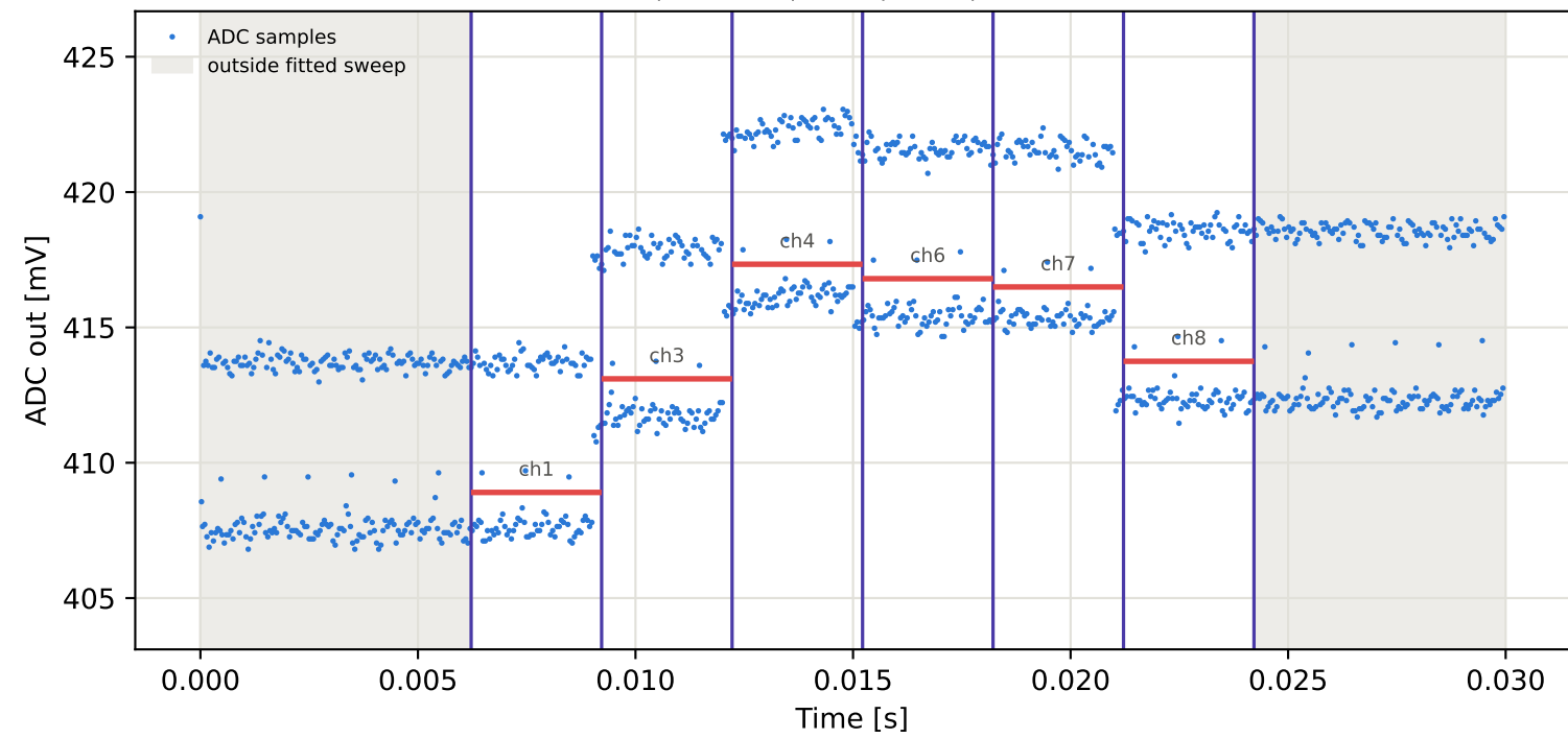
Tag5 &lt;- Tag1 | 855 MHz | run 0 | rep 1 | phase -113.75 deg
