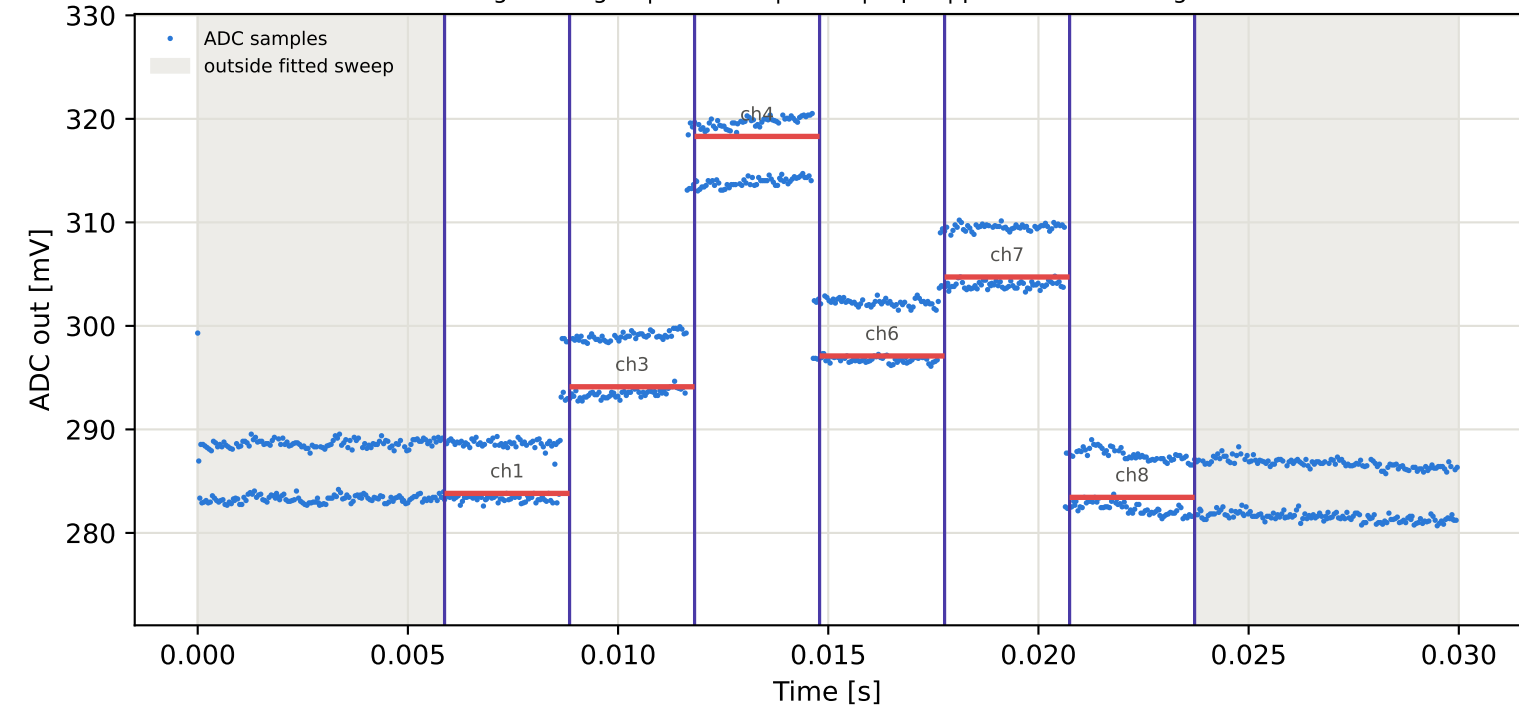
Tag6 &lt;- Tag3 | 945 MHz | run 0 | rep 1 | phase -78.06 deg
