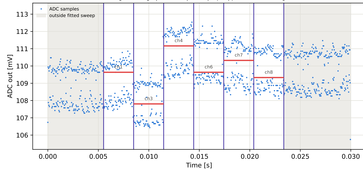
Tag10 &lt;- Tag4 | 785 MHz | run 0 | rep 1 | phase -104.34 deg
