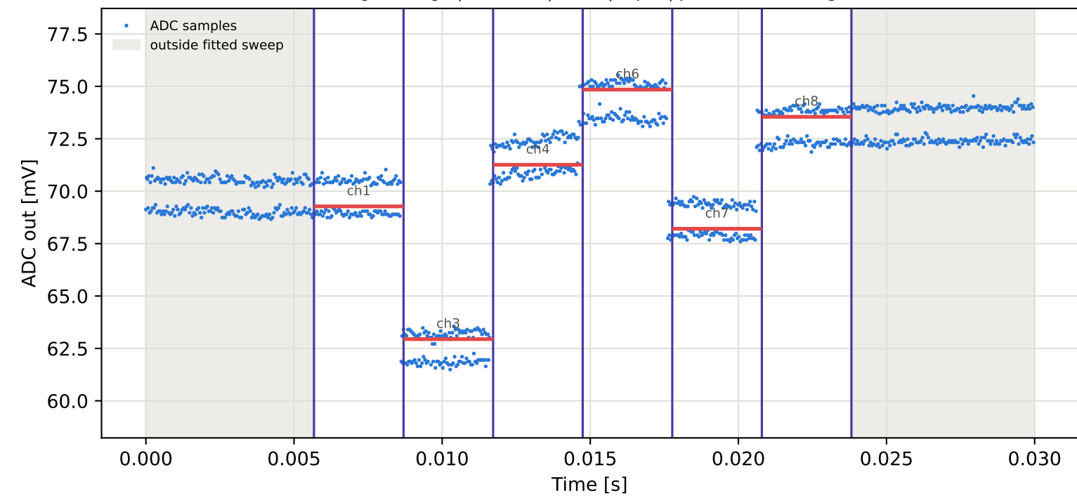
Tag3 &lt;- Tag6 | 805 MHz | run 0 | rep 1 | phase 134.50 deg
