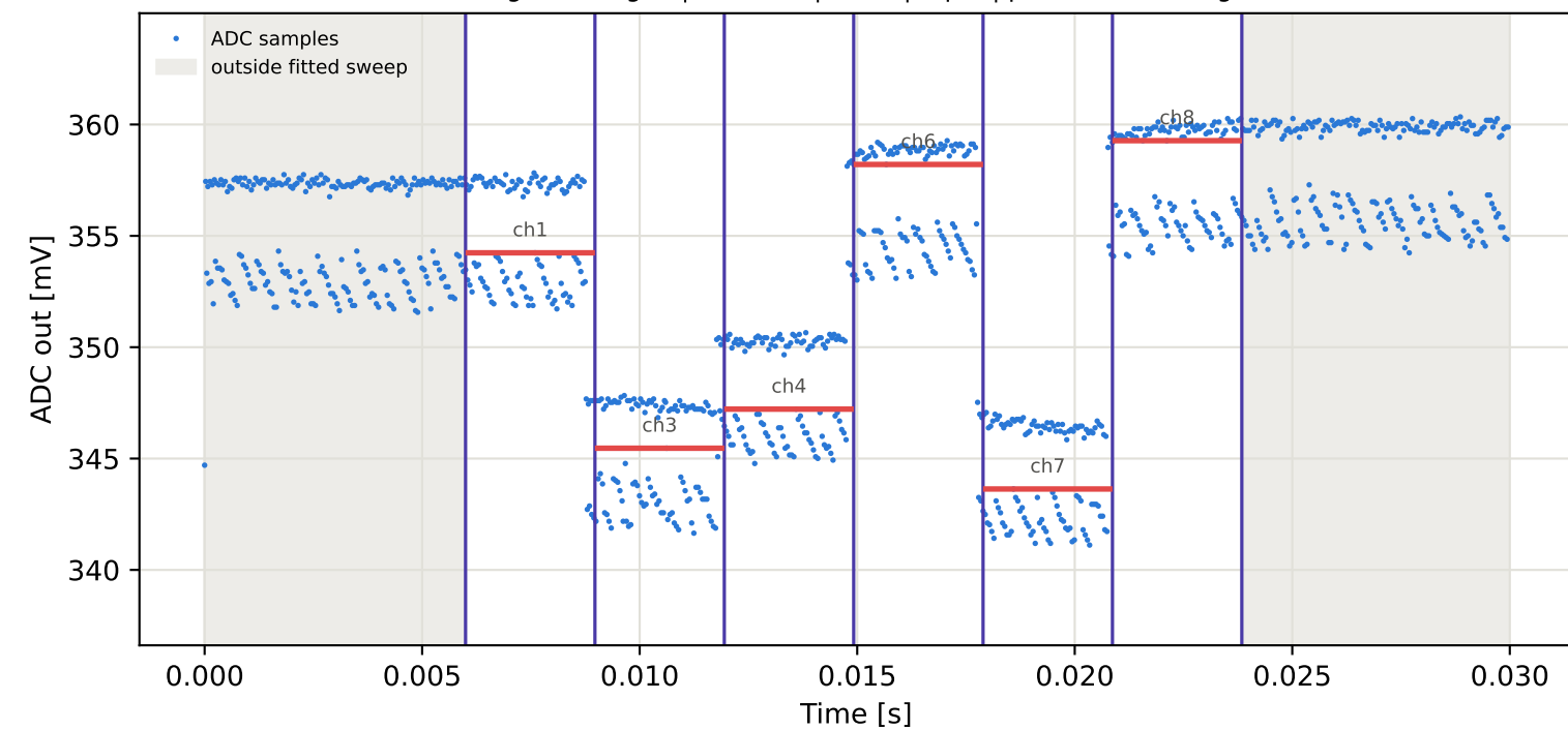
Tag16 &lt;- Tag15 | 825 MHz | run 0 | rep 1 | phase 158.08 deg
