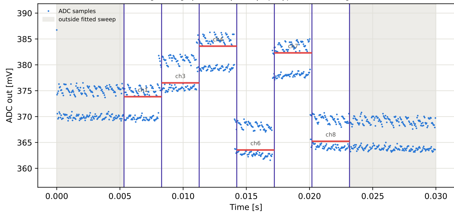
Tag6 &lt;- Tag10 | 965 MHz | run 0 | rep 1 | phase 88.63 deg
