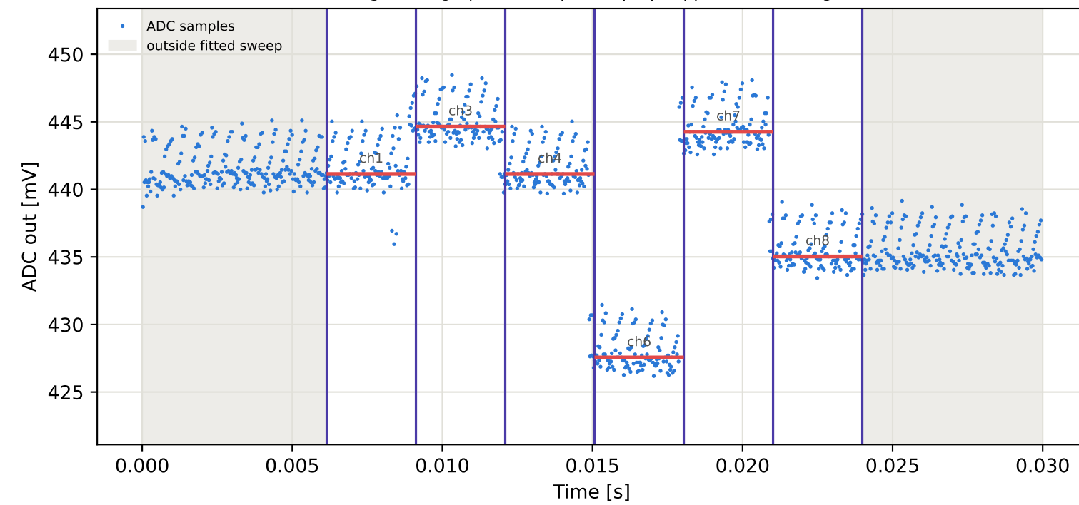
Tag5 &lt;- Tag8 | 955 MHz | run 0 | rep 1 | phase -170.42 deg
