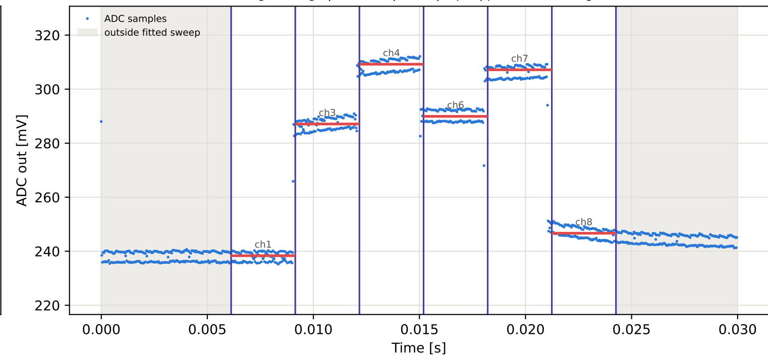
Tag9 &lt;- Tag8 | 865 MHz | run 0 | rep 1 | phase -120.62 deg
