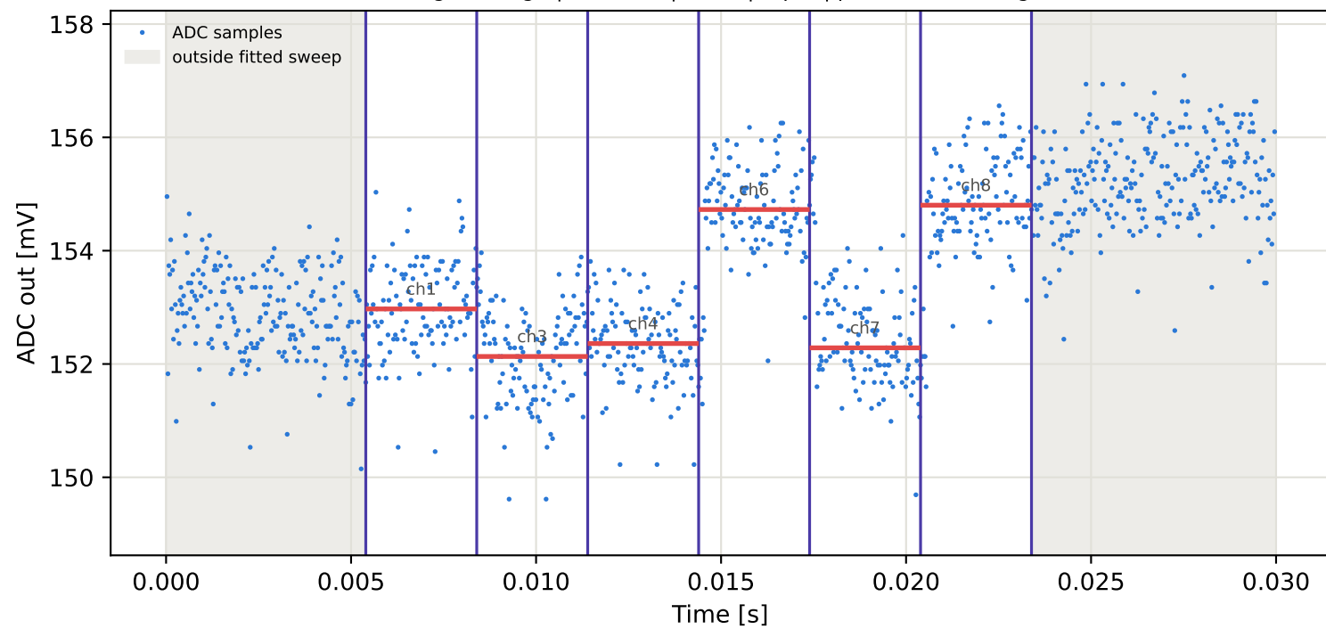
Tag3 &lt;- Tag10 | 885 MHz | run 0 | rep 1 | phase -142.10 deg
