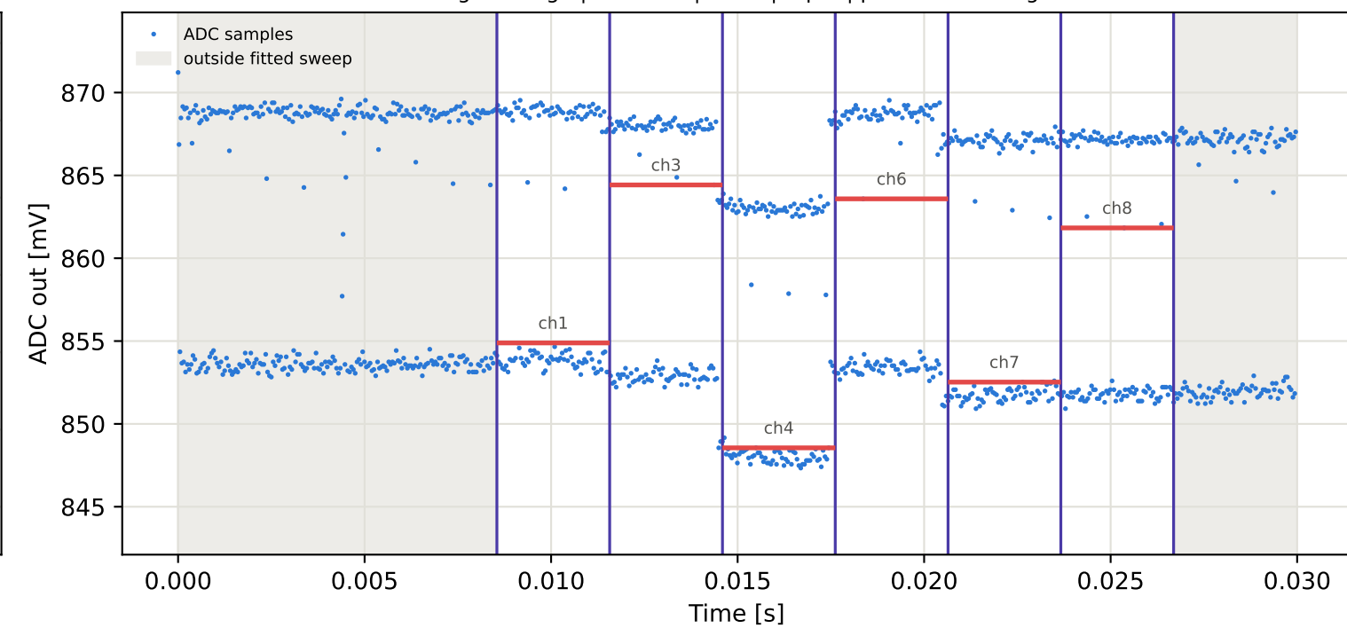
Tag7 &lt;- Tag4 | 925 MHz | run 0 | rep 1 | phase -53.68 deg
