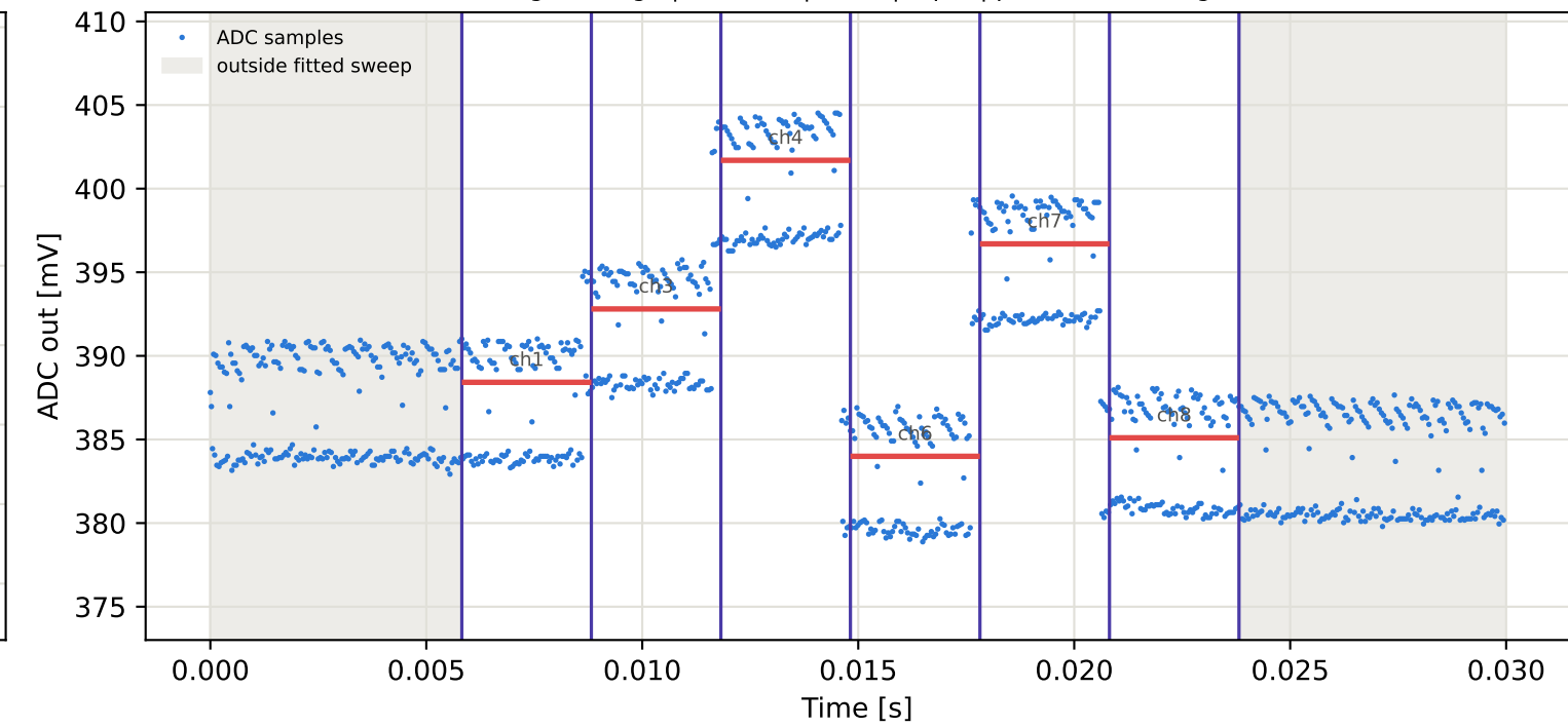
Tag8 &lt;- Tag5 | 995 MHz | run 0 | rep 1 | phase -115.36 deg
