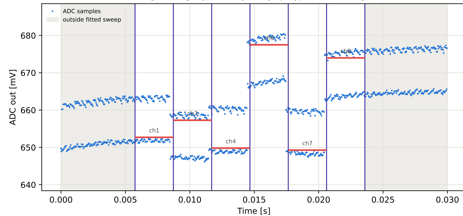
Tag10 &lt;- Tag2 | 915 MHz | run 0 | rep 1 | phase -10.85 deg
