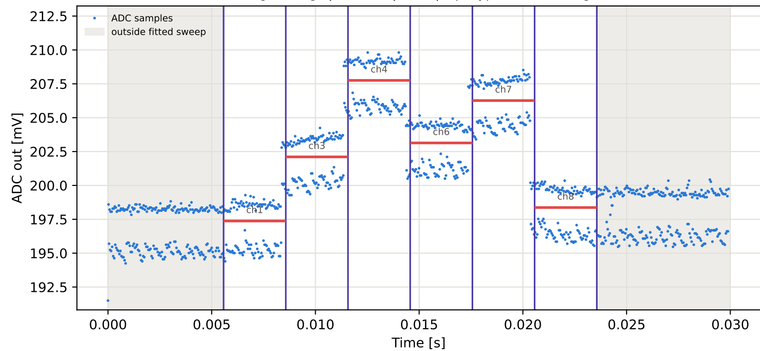
Tag5 &lt;- Tag9 | 835 MHz | run 0 | rep 1 | phase 142.60 deg
