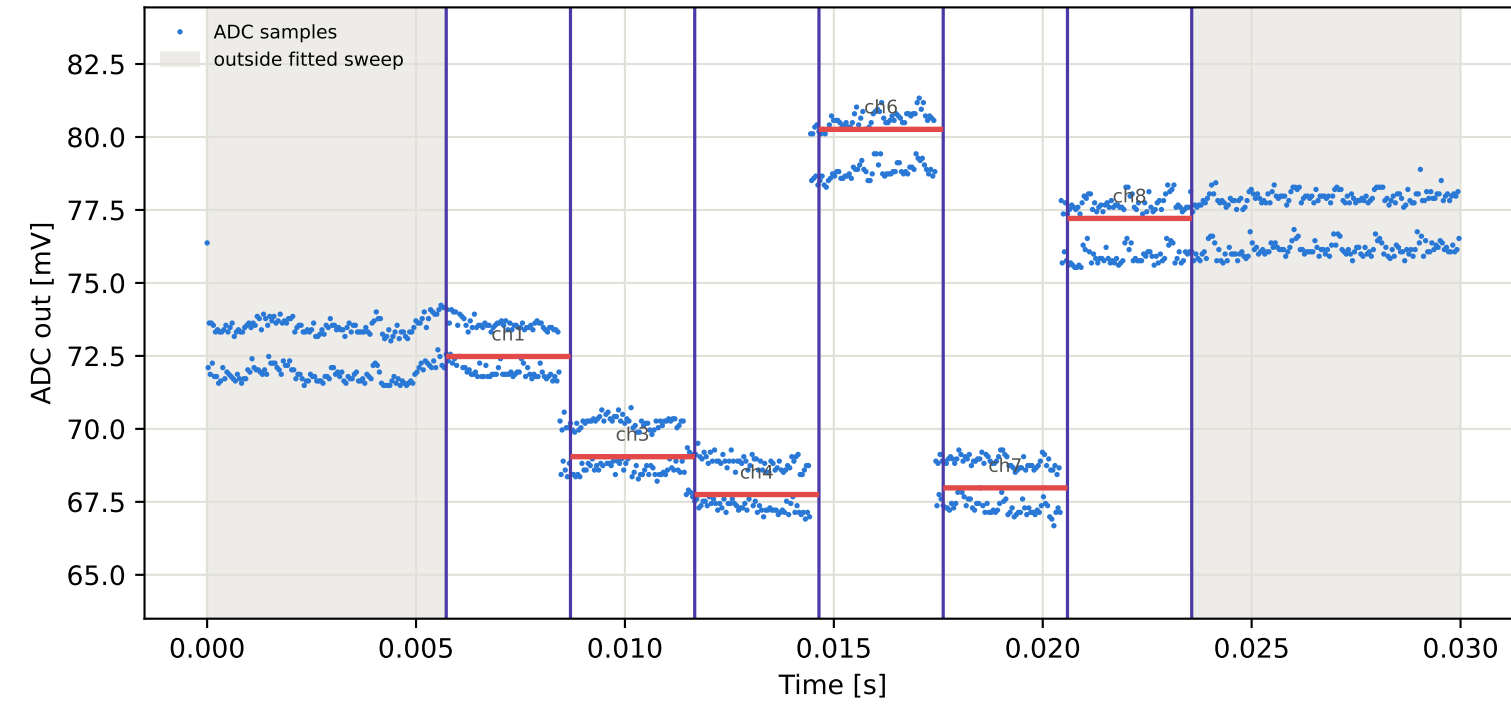
Tag3 &lt;- Tag16 | 965 MHz | run 0 | rep 1 | phase 1.25 deg
