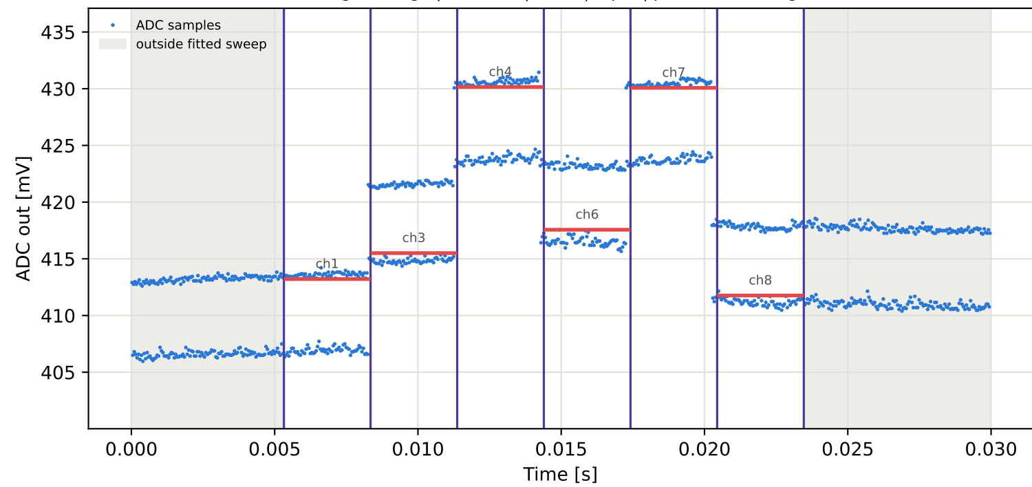
Tag4 &lt;- Tag7 | 835 MHz | run 0 | rep 1 | phase -45.27 deg
