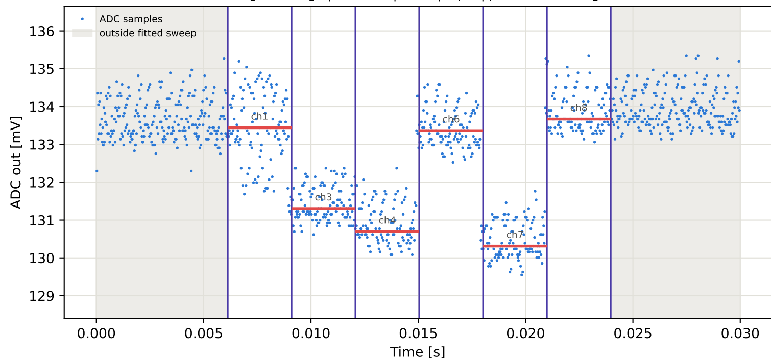
Tag15 &lt;- Tag6 | 795 MHz | run 0 | rep 1 | phase 134.47 deg
