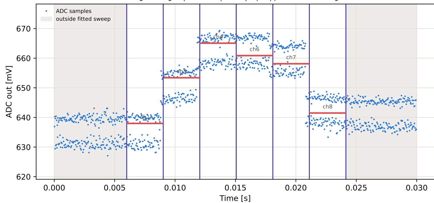
Tag1 &lt;- Tag2 | 885 MHz | run 0 | rep 1 | phase -135.45 deg
