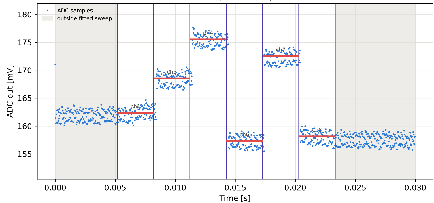
Tag7 &lt;- Tag1 | 995 MHz | run 0 | rep 1 | phase -63.07 deg
