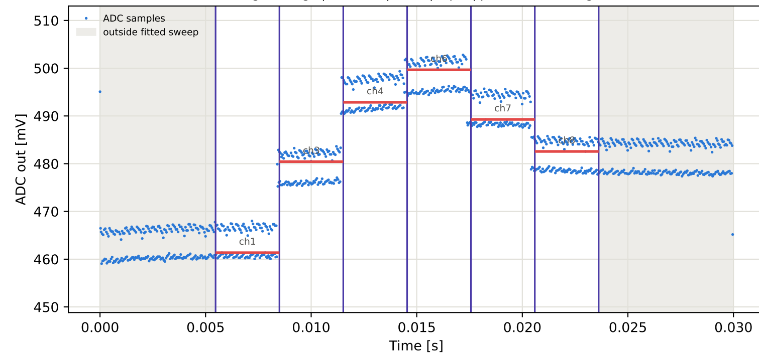
Tag3 &lt;- Tag6 | 865 MHz | run 0 | rep 1 | phase -157.13 deg
