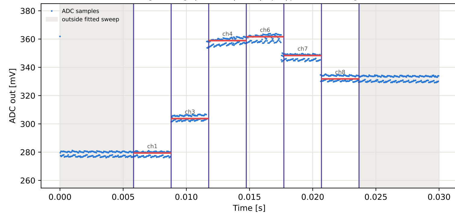
Tag2 &lt;- Tag1 | 845 MHz | run 0 | rep 1 | phase 64.64 deg
