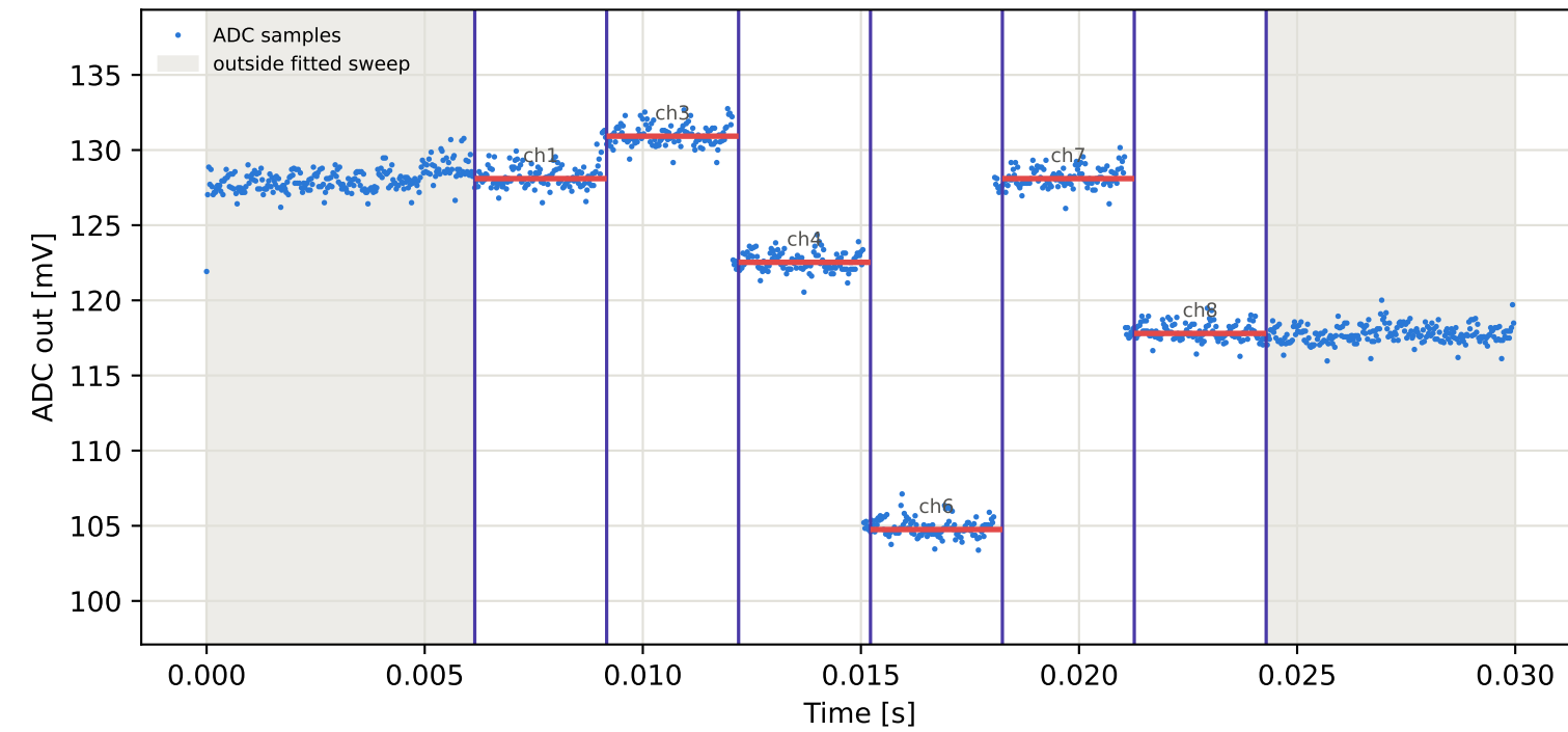
Tag7 &lt;- Tag10 | 975 MHz | run 0 | rep 1 | phase -164.01 deg
