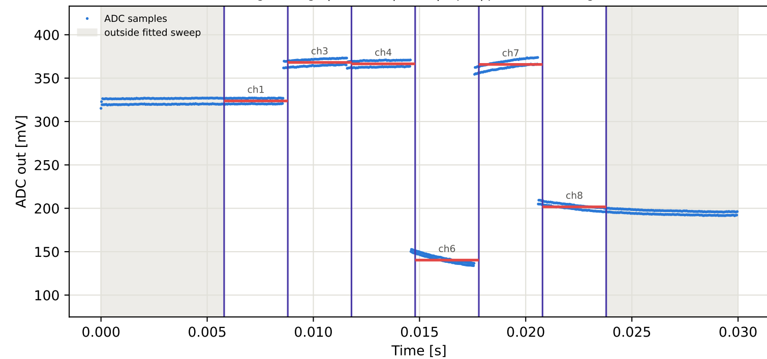
Tag4 &lt;- Tag7 | 915 MHz | run 0 | rep 1 | phase 63.86 deg
