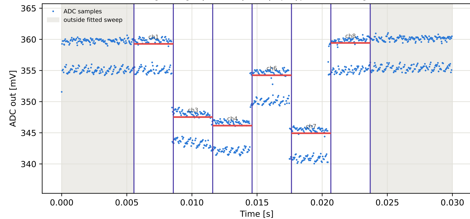
Tag5 &lt;- Tag16 | 845 MHz | run 0 | rep 1 | phase -141.95 deg
