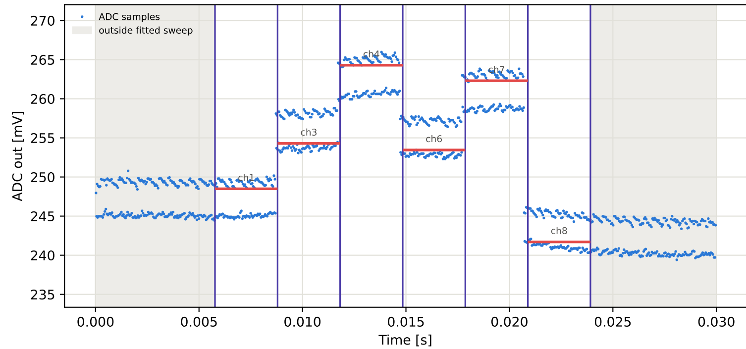
Tag9 &lt;- Tag2 | 905 MHz | run 0 | rep 1 | phase -52.05 deg
