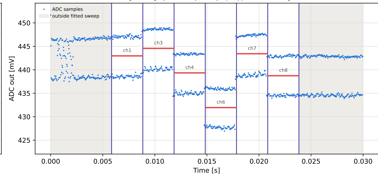
Tag7 &lt;- Tag6 | 965 MHz | run 0 | rep 1 | phase 14.88 deg
