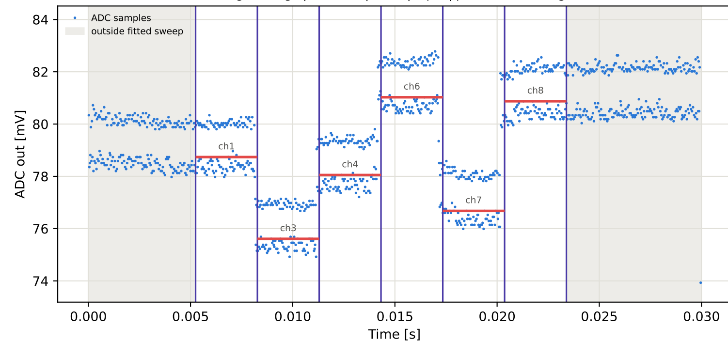
Tag4 &lt;- Tag9 | 795 MHz | run 0 | rep 1 | phase 61.70 deg
