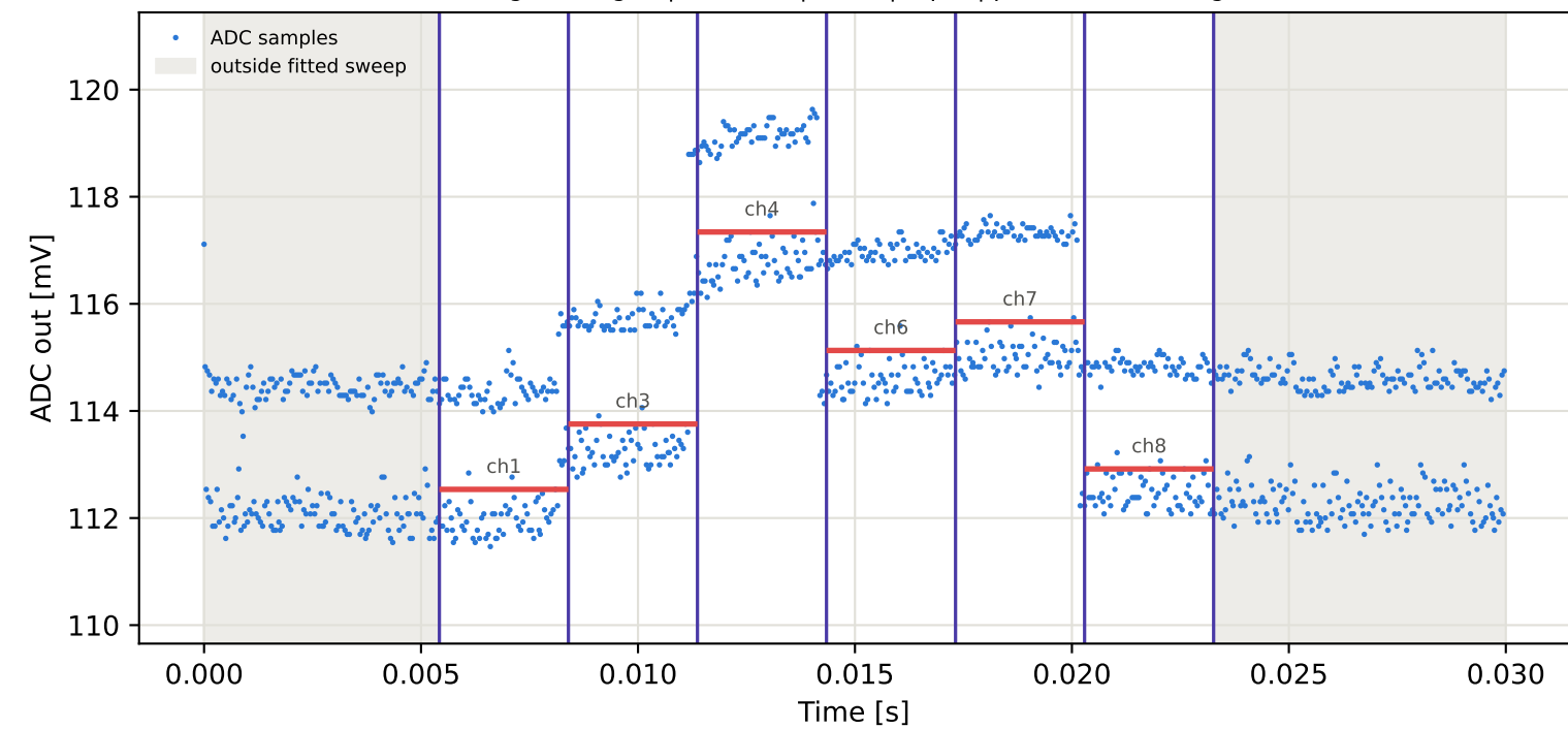
Tag1 &lt;- Tag2 | 975 MHz | run 0 | rep 1 | phase -20.00 deg
