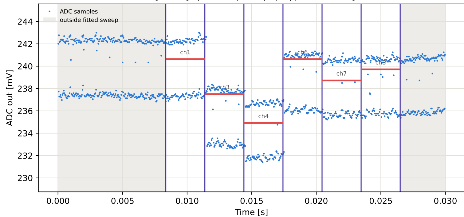
Tag9 &lt;- Tag8 | 975 MHz | run 0 | rep 1 | phase 95.80 deg
