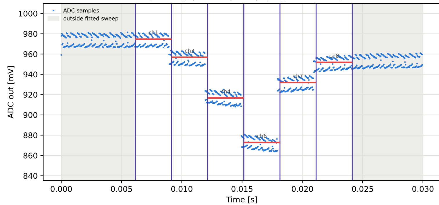
Tag16 &lt;- Tag1 | 915 MHz | run 0 | rep 1 | phase 161.87 deg
