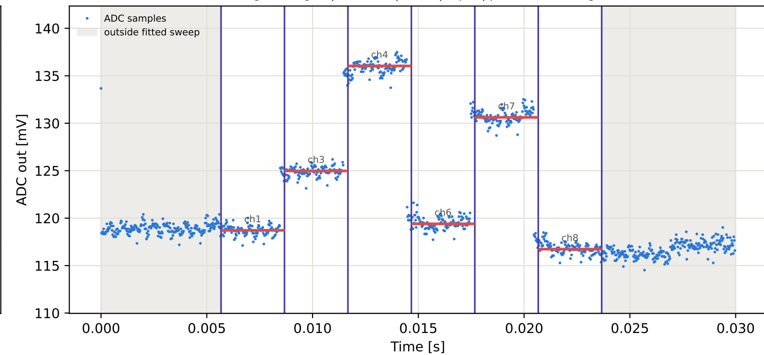
Tag6 &lt;- Tag3 | 975 MHz | run 0 | rep 1 | phase -63.88 deg
