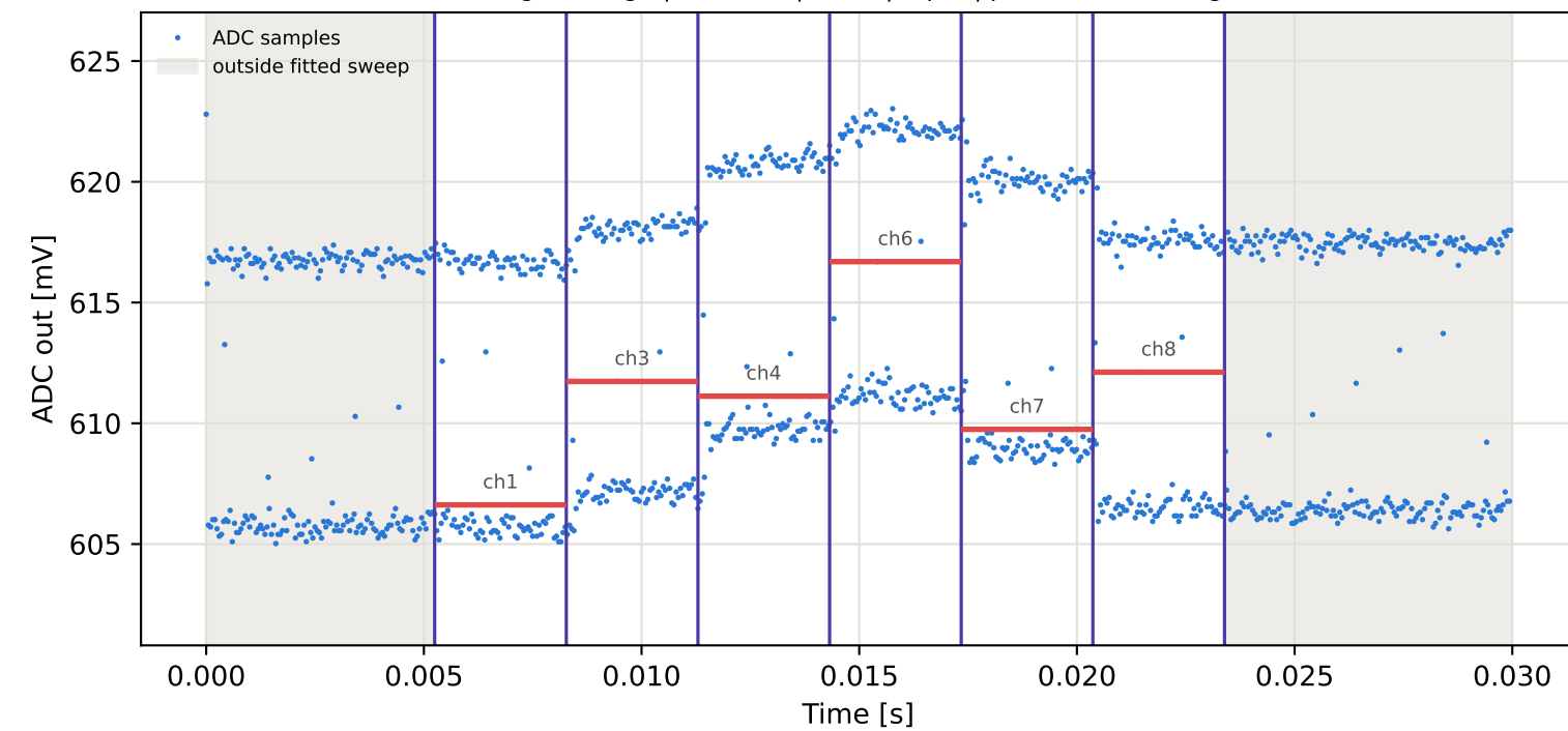
Tag8 &lt;- Tag4 | 925 MHz | run 0 | rep 1 | phase 63.41 deg
