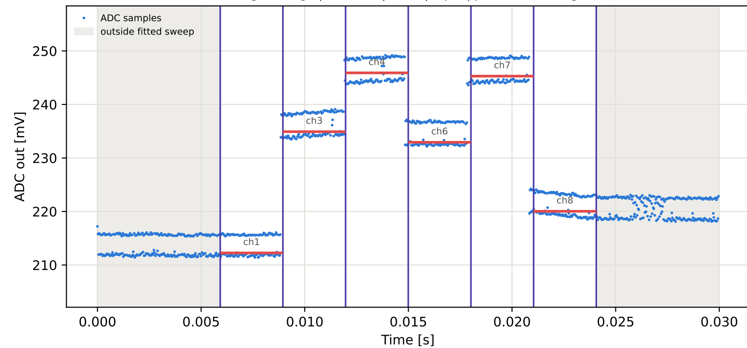
Tag1 &lt;- Tag8 | 845 MHz | run 0 | rep 1 | phase -153.94 deg
