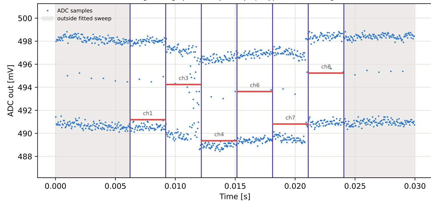
Tag3 &lt;- Tag2 | 865 MHz | run 0 | rep 1 | phase 103.56 deg
