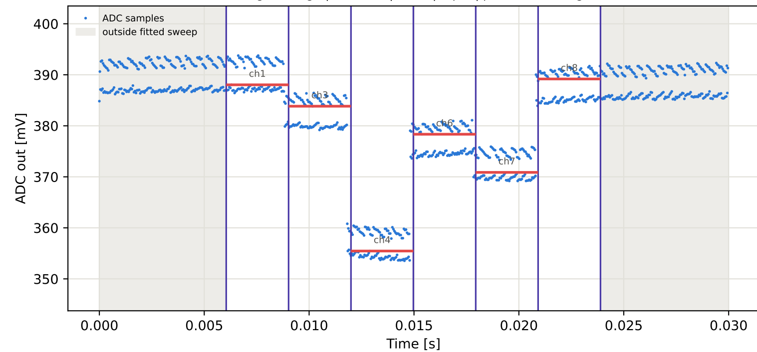
Tag8 &lt;- Tag1 | 985 MHz | run 0 | rep 1 | phase 52.97 deg
