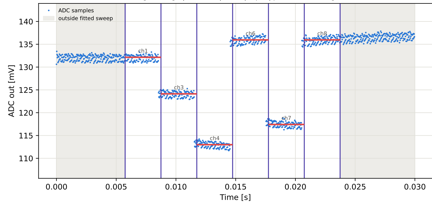
Tag1 &lt;- Tag8 | 995 MHz | run 0 | rep 1 | phase -36.26 deg
