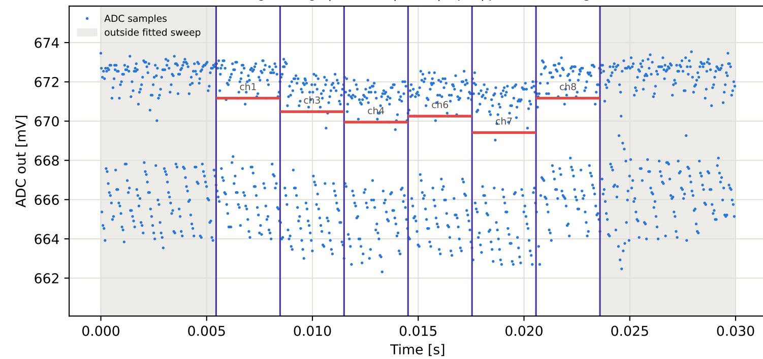
Tag8 &lt;- Tag4 | 835 MHz | run 0 | rep 1 | phase -90.92 deg
