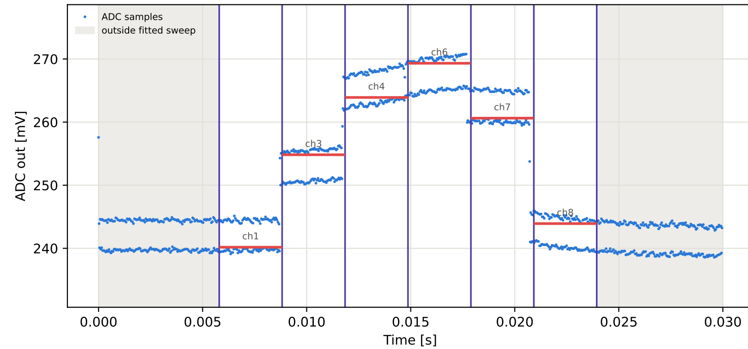
Tag9 &lt;- Tag7 | 905 MHz | run 0 | rep 1 | phase 32.68 deg
