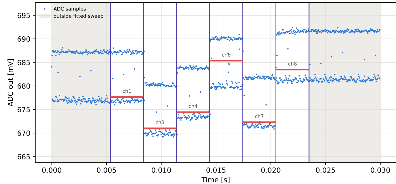
Tag8 &lt;- Tag16 | 845 MHz | run 0 | rep 1 | phase -138.47 deg
