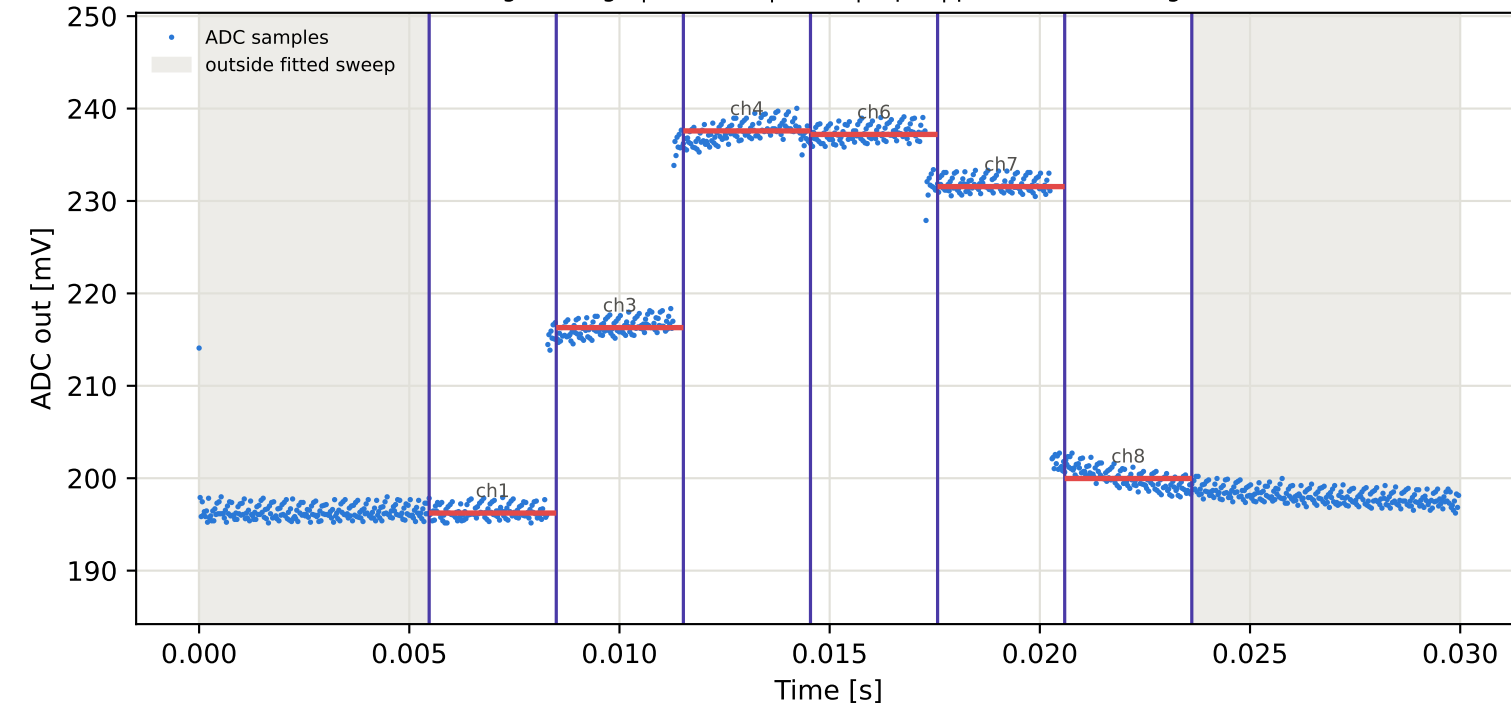
Tag1 &lt;- Tag3 | 895 MHz | run 0 | rep 1 | phase -114.46 deg
