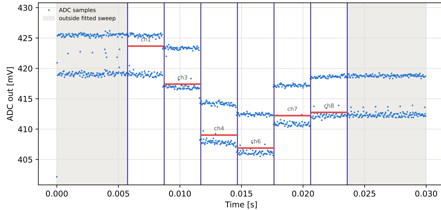
Tag1 &lt;- Tag9 | 865 MHz | run 0 | rep 1 | phase 18.45 deg
