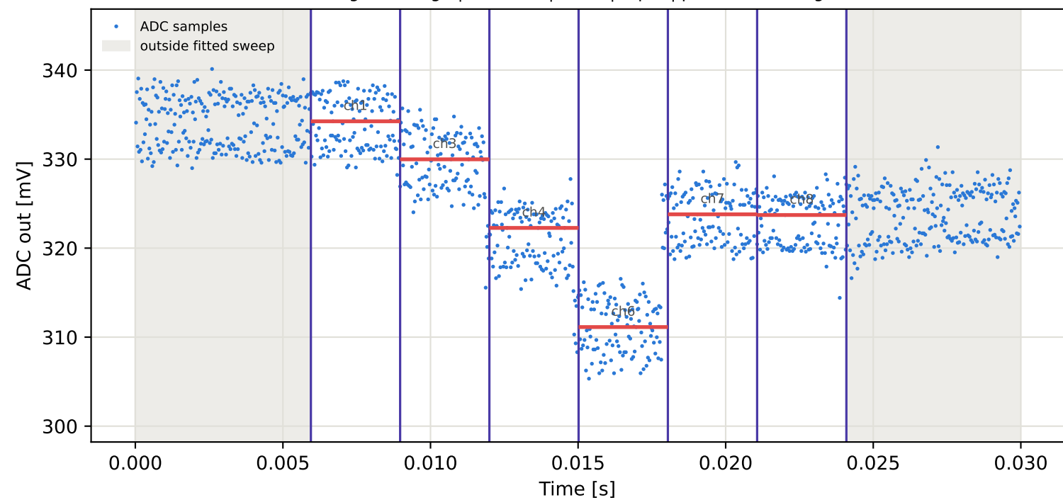
Tag10 &lt;- Tag4 | 885 MHz | run 0 | rep 1 | phase 36.97 deg
