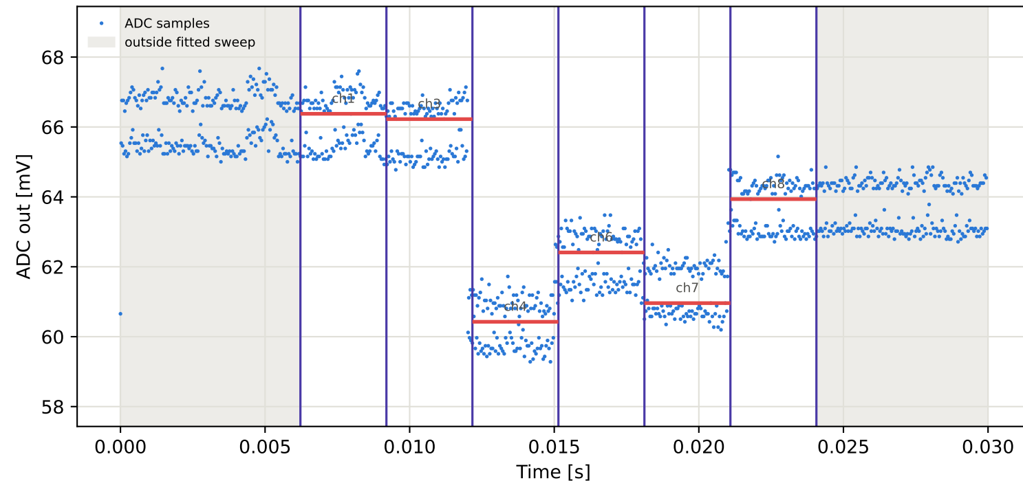
Tag15 &lt;- Tag1 | 805 MHz | run 0 | rep 1 | phase -44.36 deg
