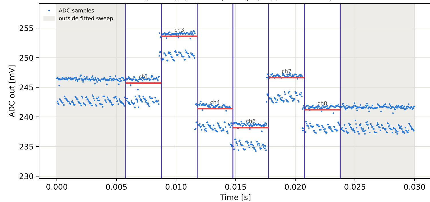
Tag6 &lt;- Tag1 | 795 MHz | run 0 | rep 1 | phase -142.17 deg
