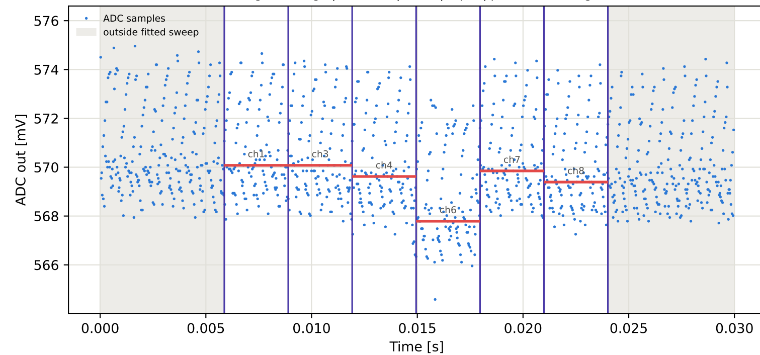
Tag16 &lt;- Tag4 | 955 MHz | run 0 | rep 1 | phase 0.43 deg
