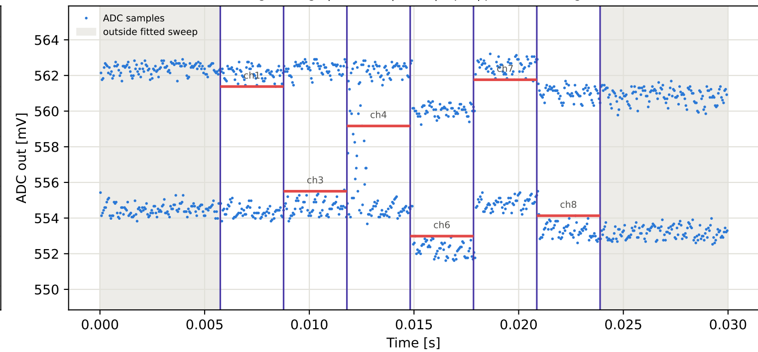
Tag7 &lt;- Tag4 | 865 MHz | run 0 | rep 1 | phase 24.48 deg
