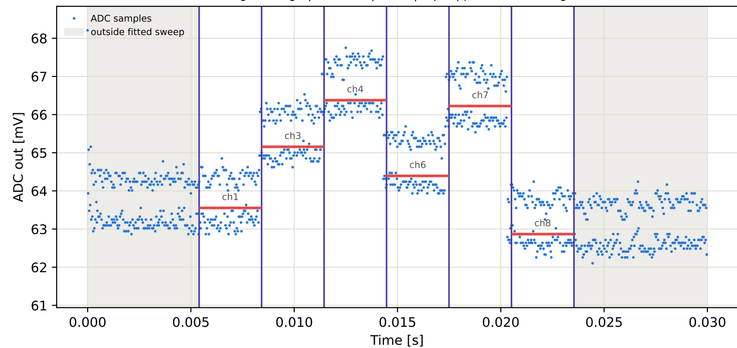
Tag9 &lt;- Tag2 | 825 MHz | run 0 | rep 1 | phase -71.30 deg
