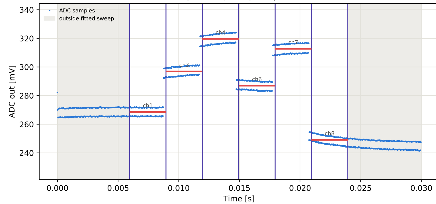
Tag3 &lt;- Tag6 | 905 MHz | run 0 | rep 1 | phase -135.73 deg
