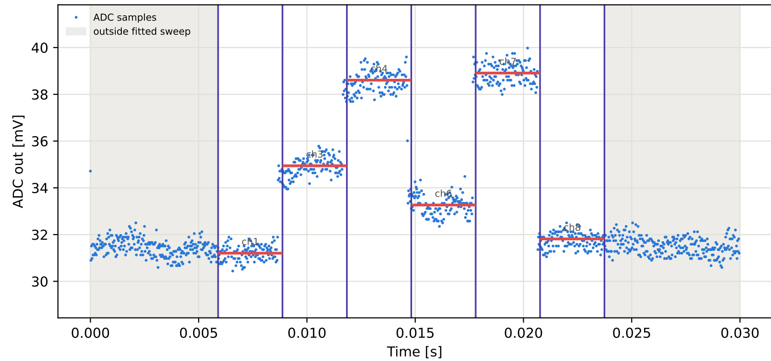
Tag9 &lt;- Tag2 | 805 MHz | run 0 | rep 1 | phase 140.36 deg
