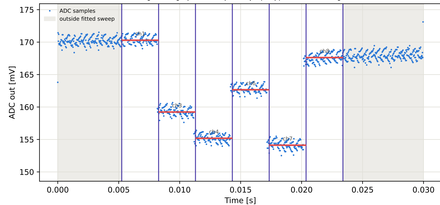
Tag7 &lt;- Tag5 | 845 MHz | run 0 | rep 1 | phase 102.43 deg
