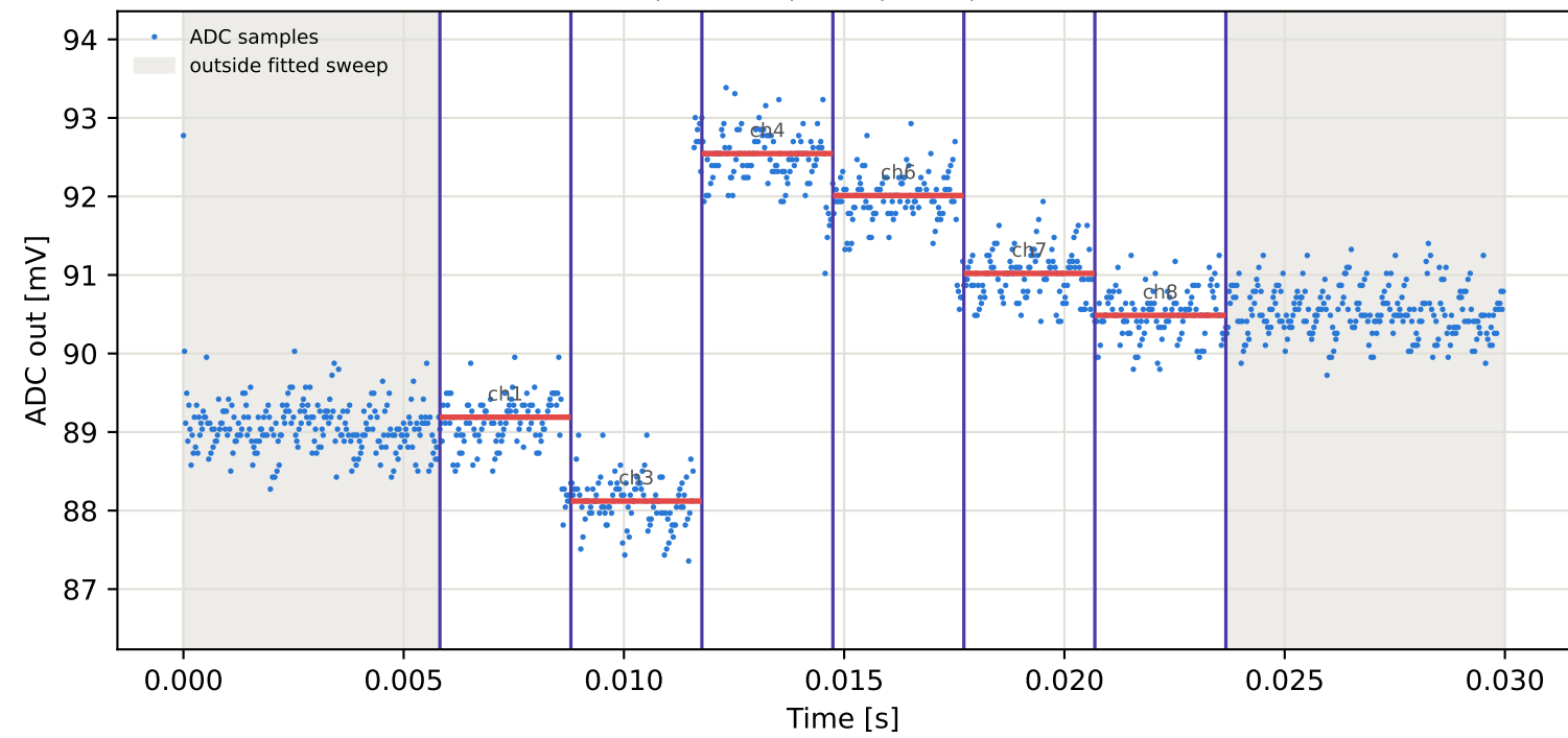
Tag7 &lt;- Tag15 | 785 MHz | run 0 | rep 1 | phase -118.04 deg
