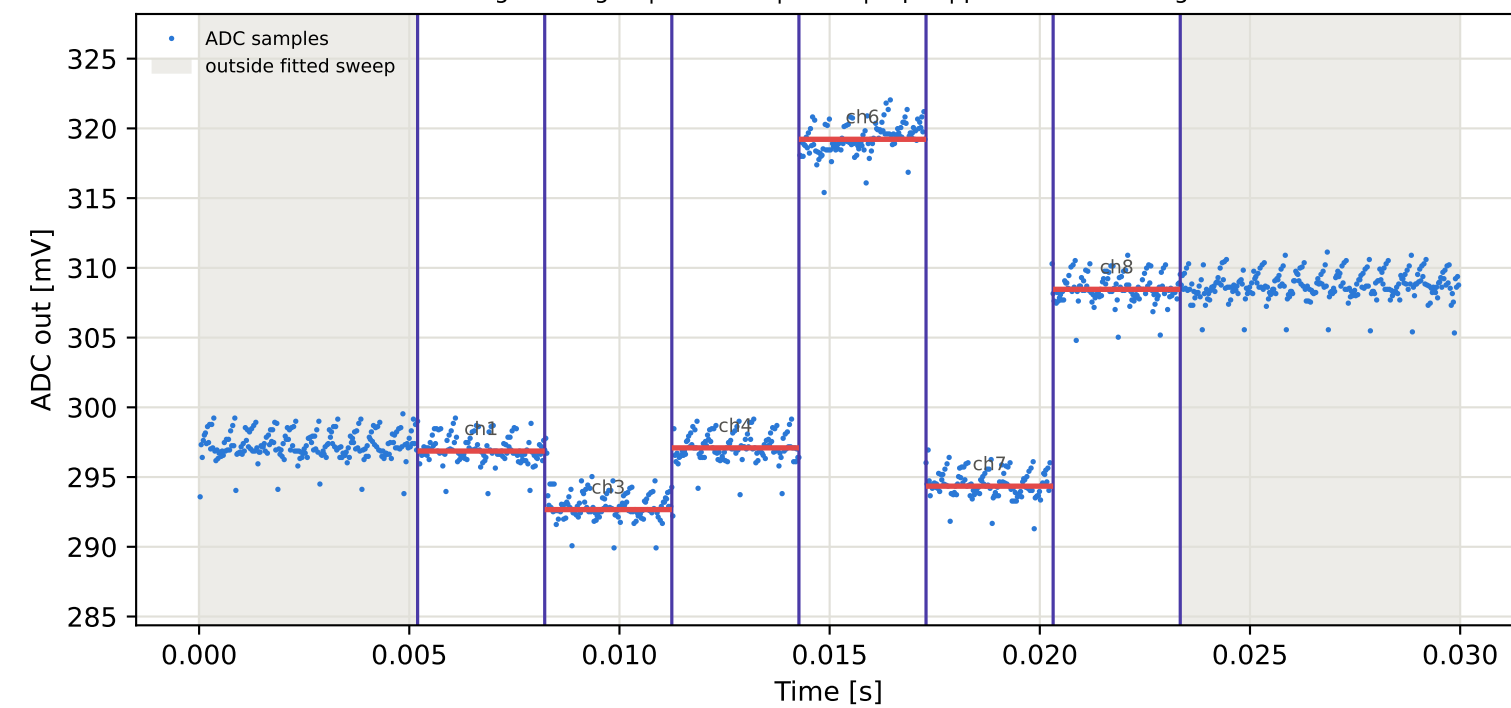
Tag6 &lt;- Tag2 | 945 MHz | run 0 | rep 1 | phase -20.94 deg
