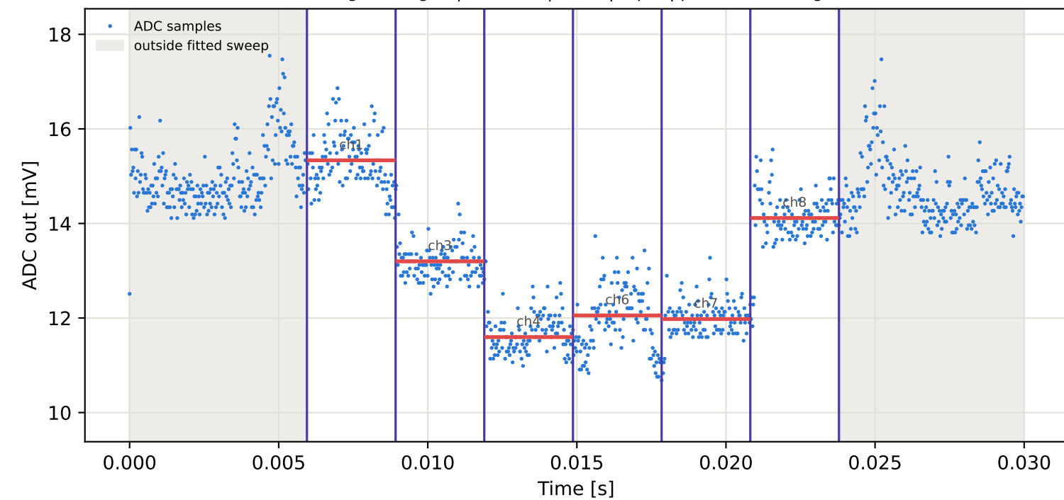
Tag2 &lt;- Tag16 | 895 MHz | run 0 | rep 1 | phase -83.74 deg
