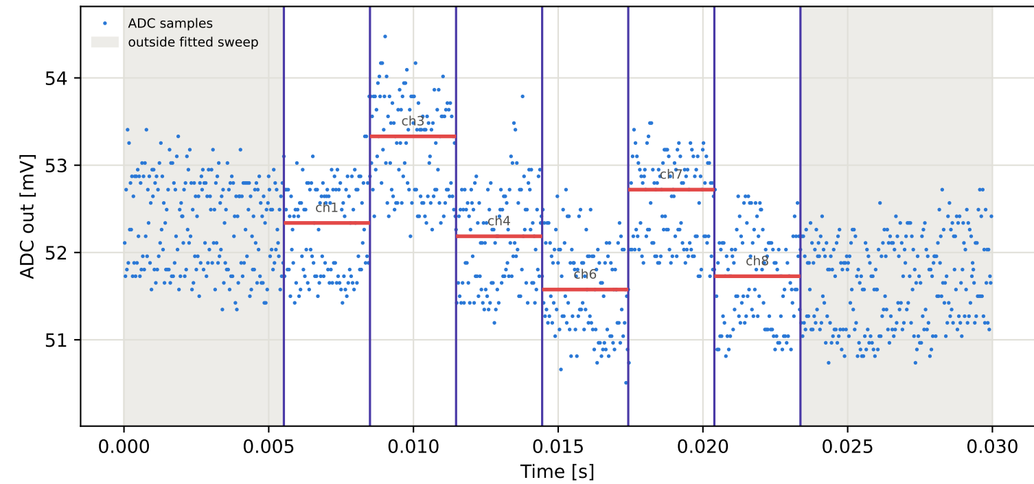
Tag9 &lt;- Tag2 | 775 MHz | run 0 | rep 1 | phase -105.13 deg
