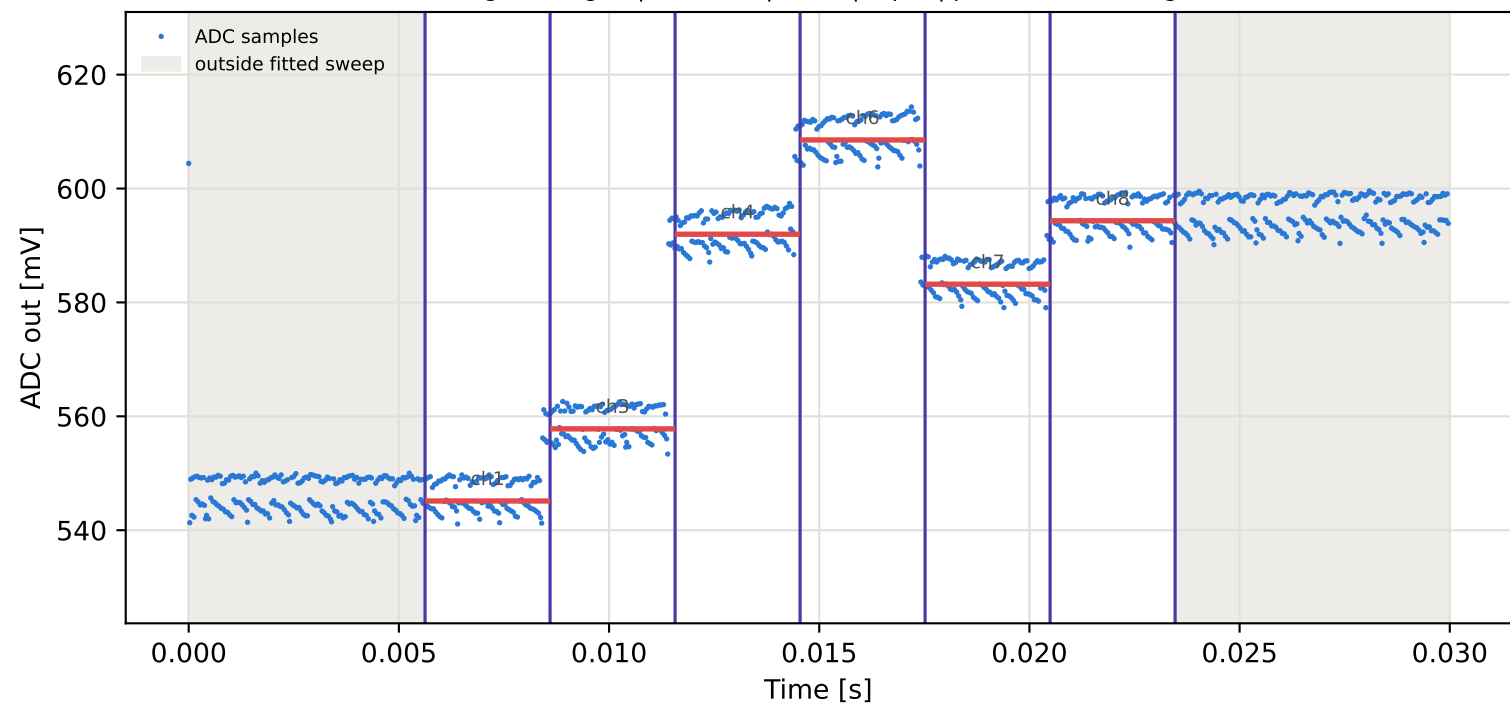
Tag5 &lt;- Tag2 | 865 MHz | run 0 | rep 1 | phase -104.13 deg
