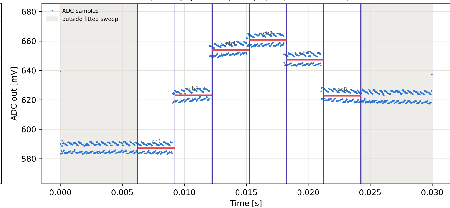
Tag6 &lt;- Tag5 | 865 MHz | run 0 | rep 1 | phase -138.37 deg
