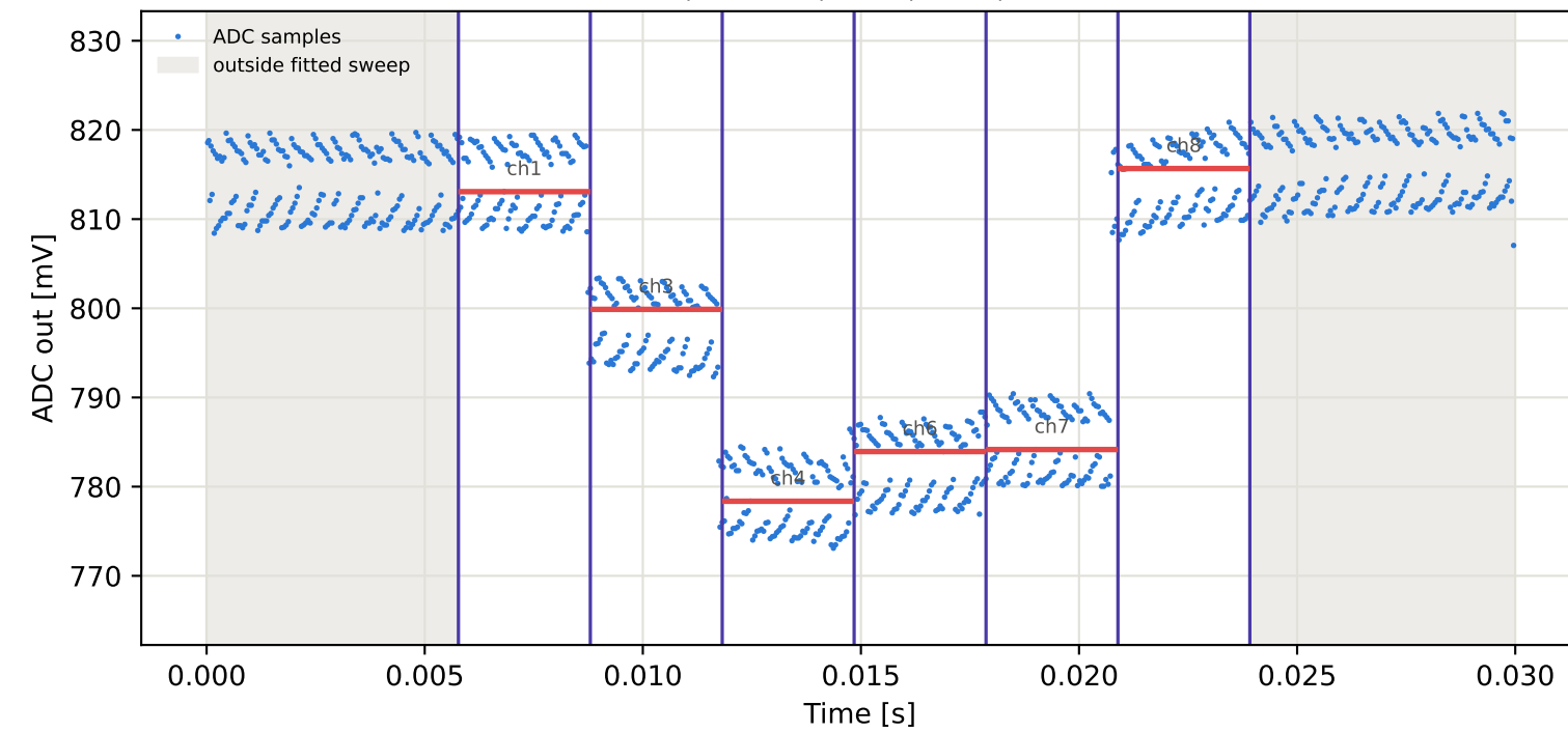
Tag10 &lt;- Tag4 | 905 MHz | run 0 | rep 1 | phase 70.22 deg
