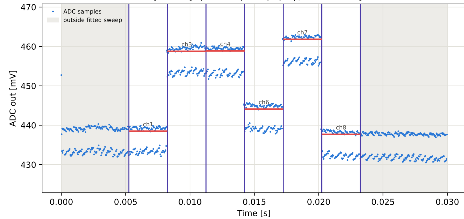
Tag15 &lt;- Tag5 | 845 MHz | run 0 | rep 1 | phase -54.08 deg
