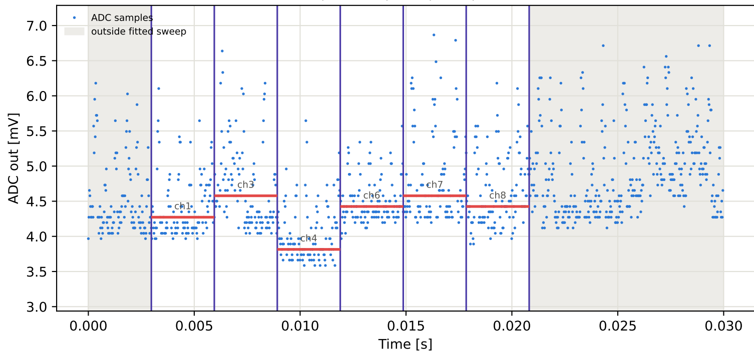
Tag2 &lt;- Tag16 | 785 MHz | run 0 | rep 1 | phase 78.27 deg
