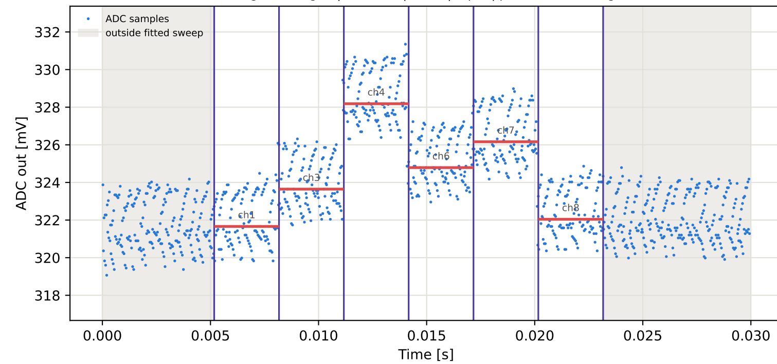
Tag10 &lt;- Tag2 | 965 MHz | run 0 | rep 1 | phase 120.76 deg
