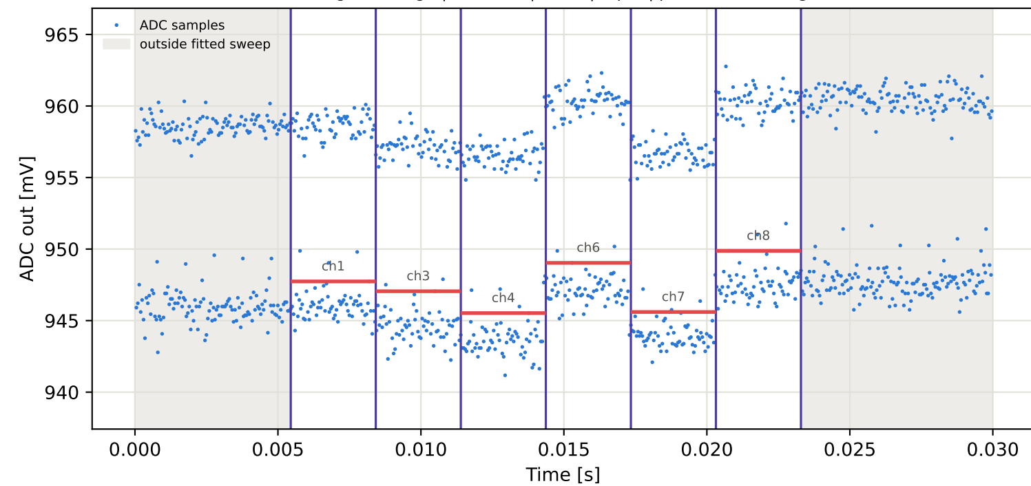
Tag15 &lt;- Tag4 | 885 MHz | run 0 | rep 1 | phase -144.82 deg
