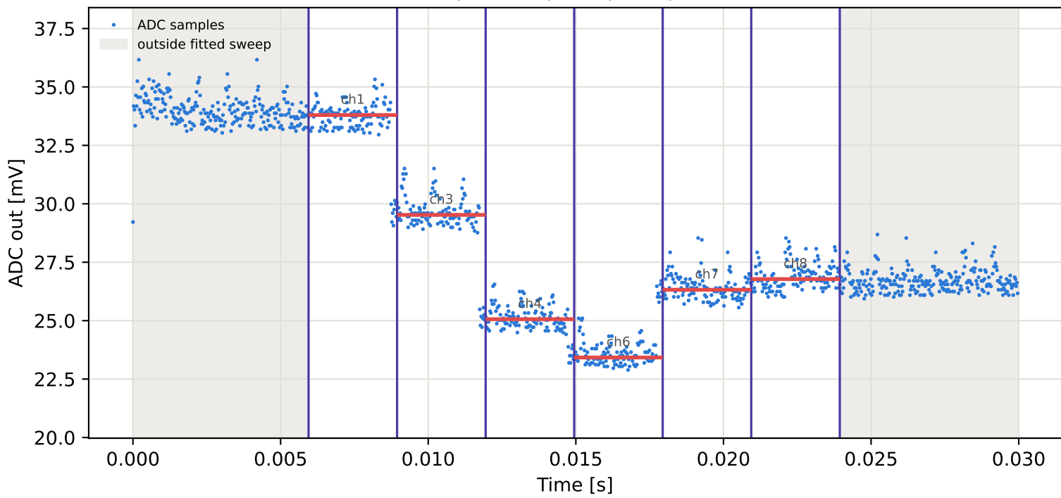
Tag2 &lt;- Tag16 | 865 MHz | run 0 | rep 1 | phase 51.84 deg
