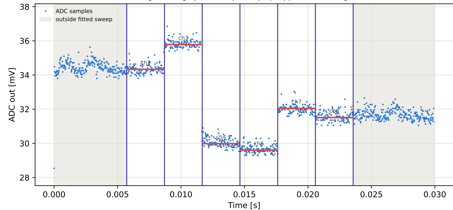
Tag10 &lt;- Tag5 | 825 MHz | run 0 | rep 1 | phase 47.79 deg
