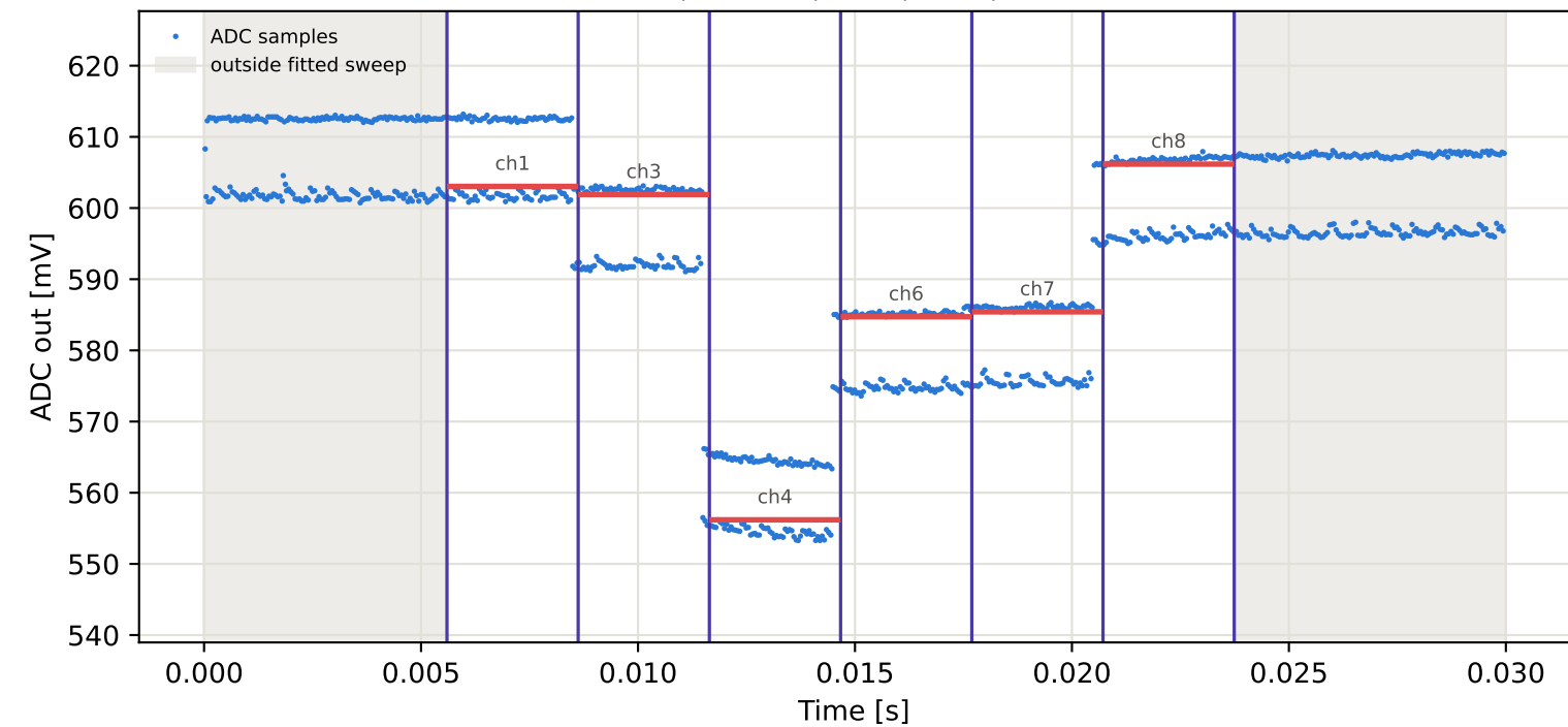
Tag8 &lt;- Tag16 | 965 MHz | run 0 | rep 1 | phase 64.23 deg
