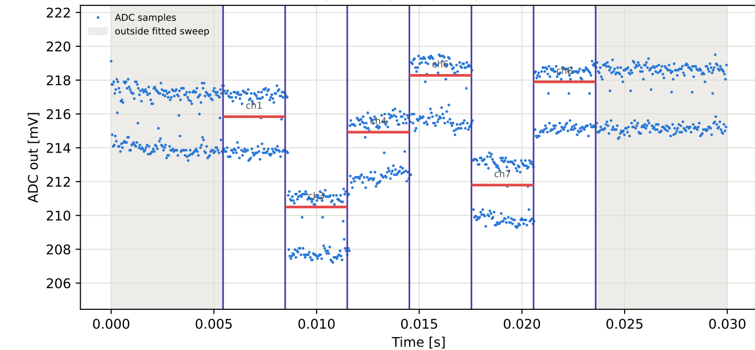
Tag6 &lt;- Tag4 | 805 MHz | run 0 | rep 1 | phase -174.45 deg
