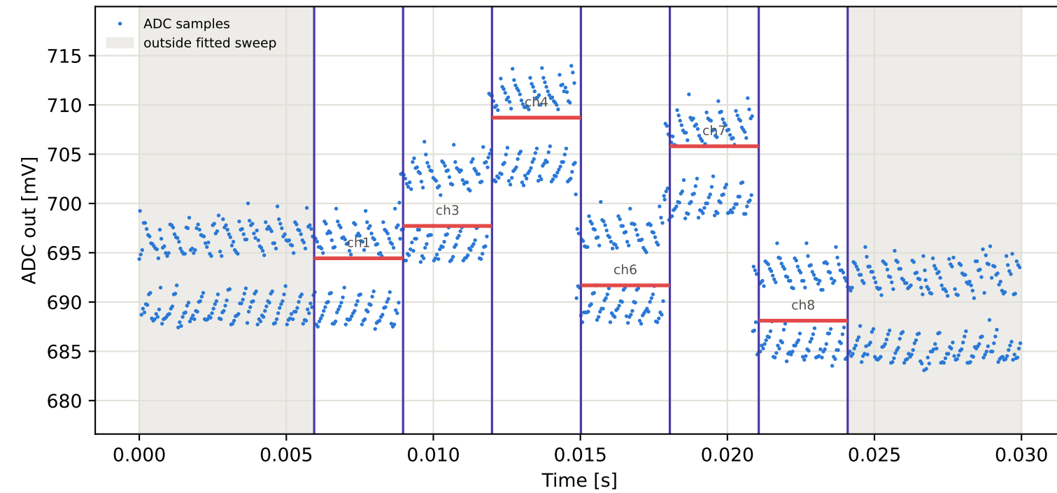
Tag8 &lt;- Tag15 | 955 MHz | run 0 | rep 1 | phase 104.47 deg
