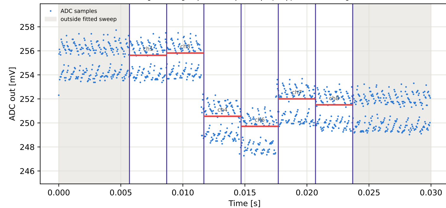
Tag16 &lt;- Tag10 | 835 MHz | run 0 | rep 1 | phase 49.53 deg
