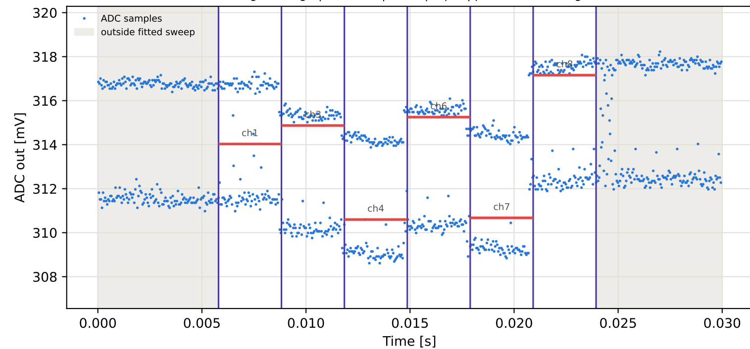
Tag3 &lt;- Tag2 | 845 MHz | run 0 | rep 1 | phase 110.51 deg
