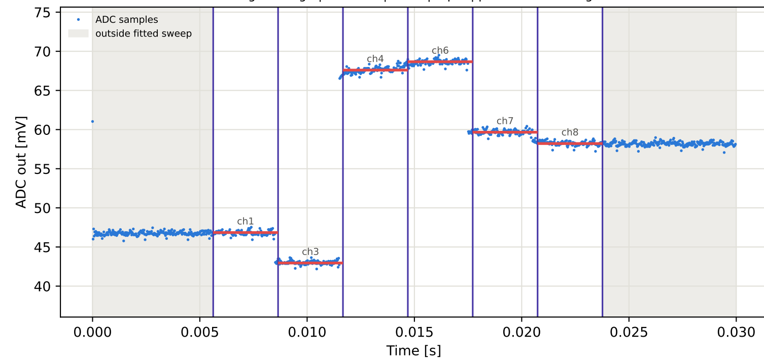
Tag4 &lt;- Tag7 | 785 MHz | run 0 | rep 1 | phase 146.52 deg
