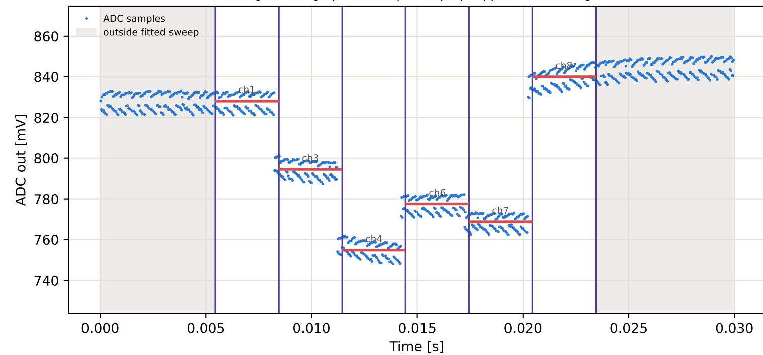
Tag10 &lt;- Tag8 | 905 MHz | run 0 | rep 1 | phase -73.27 deg
