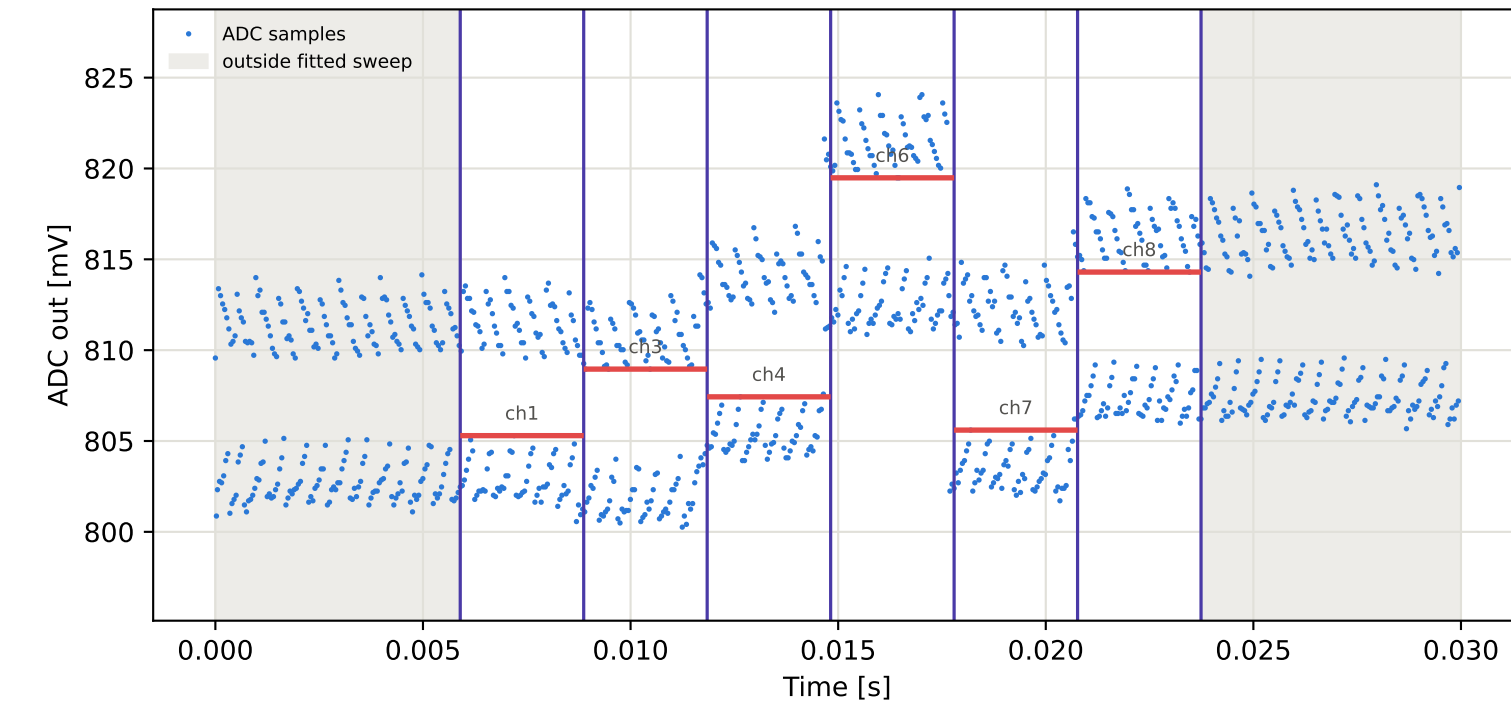
Tag8 &lt;- Tag15 | 935 MHz | run 0 | rep 1 | phase 65.97 deg
