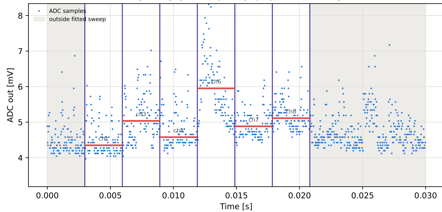
Tag3 &lt;- Tag10 | 775 MHz | run 0 | rep 1 | phase 66.43 deg
