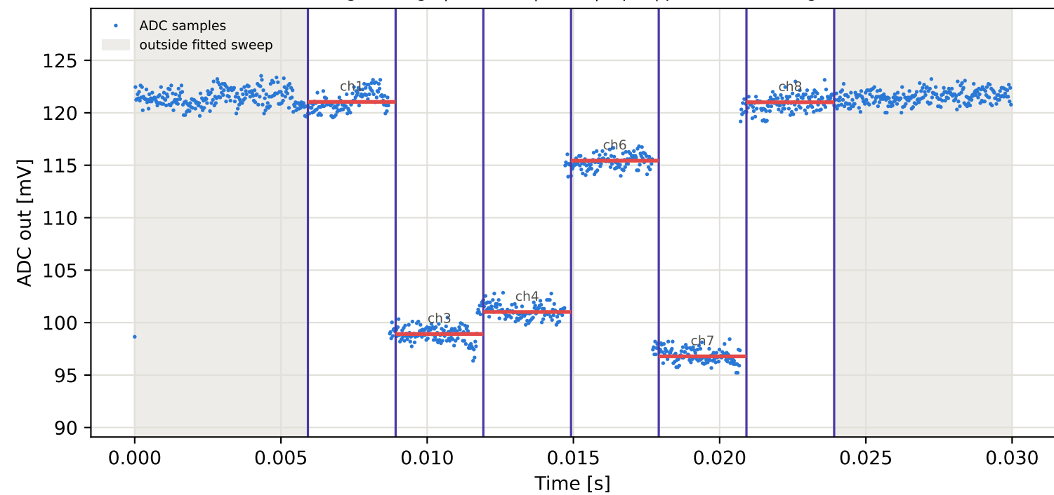
Tag2 &lt;- Tag6 | 825 MHz | run 0 | rep 1 | phase -18.16 deg
