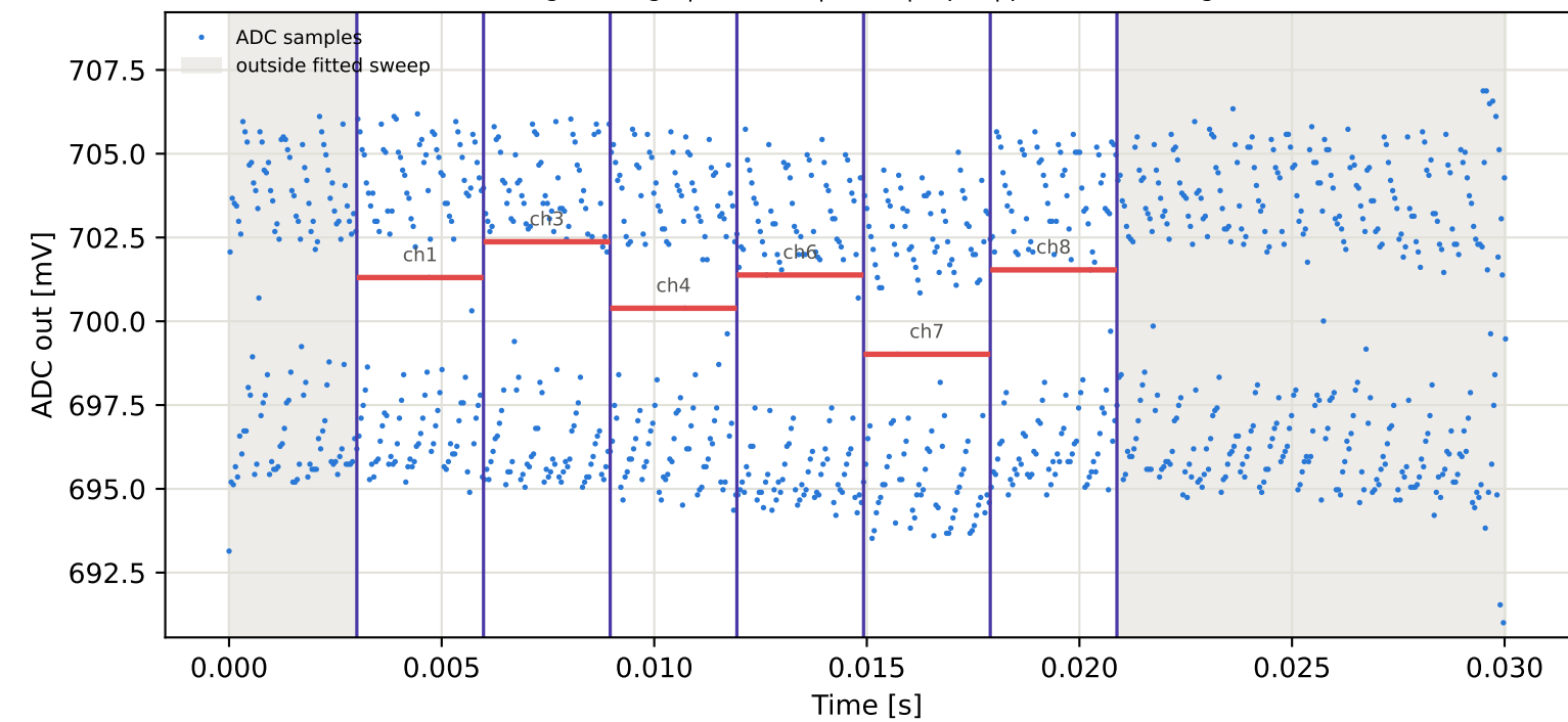
Tag8 &lt;- Tag4 | 955 MHz | run 0 | rep 1 | phase -169.63 deg
