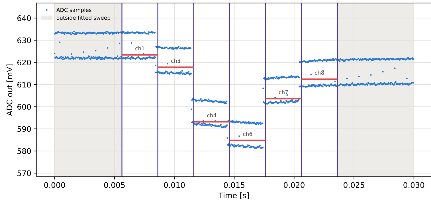
Tag8 &lt;- Tag7 | 925 MHz | run 0 | rep 1 | phase 43.85 deg
