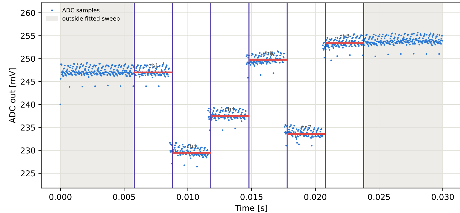
Tag1 &lt;- Tag3 | 845 MHz | run 0 | rep 1 | phase 140.24 deg
