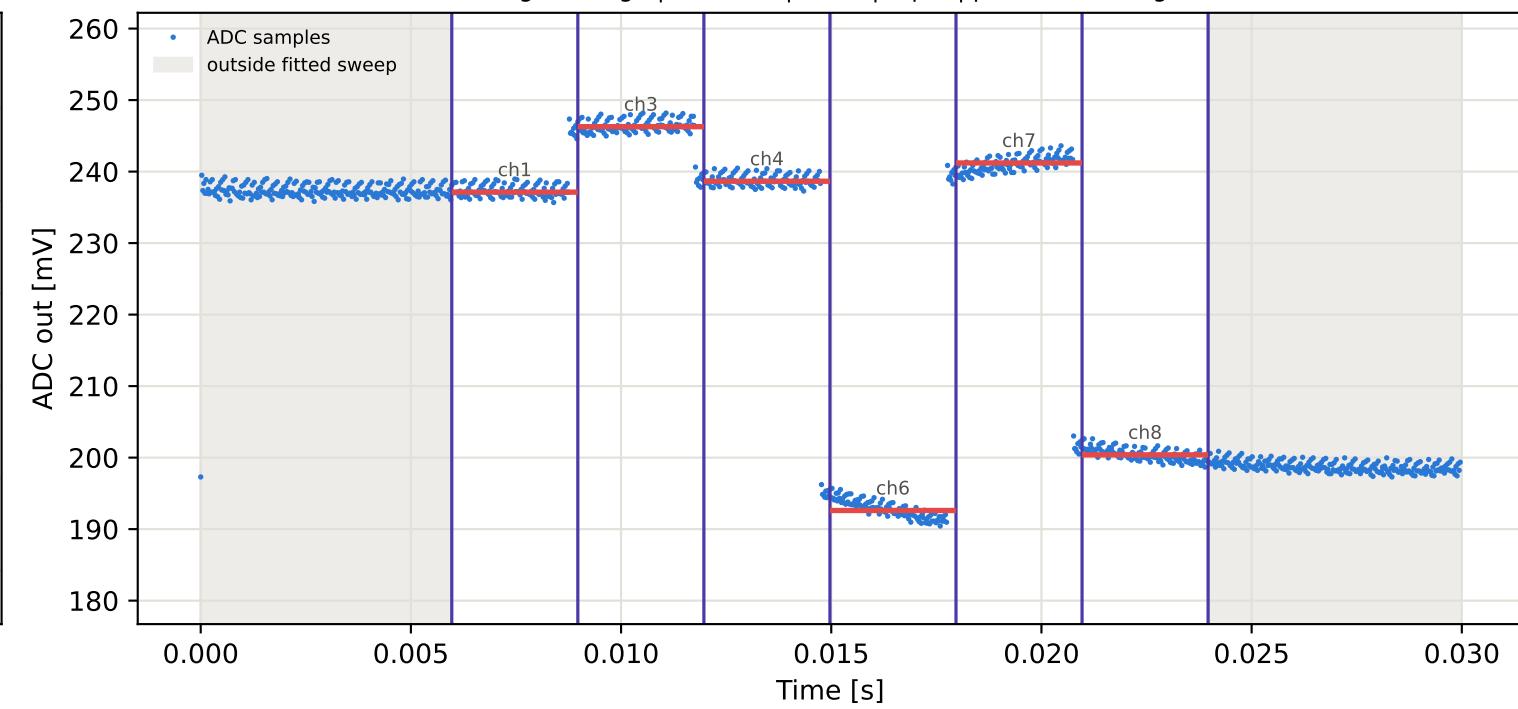
Tag1 &lt;- Tag4 | 895 MHz | run 0 | rep 1 | phase -1.51 deg
