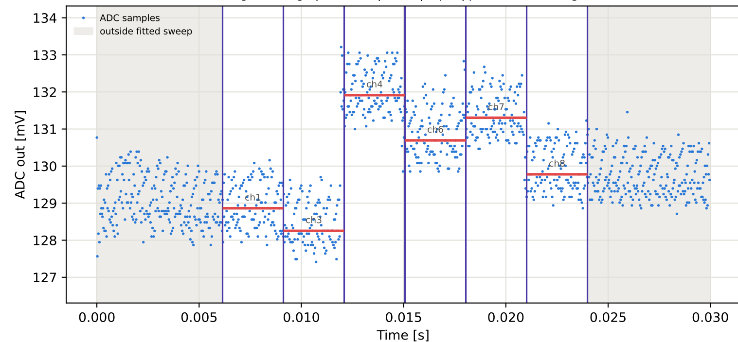
Tag15 &lt;- Tag5 | 795 MHz | run 0 | rep 1 | phase -107.54 deg
