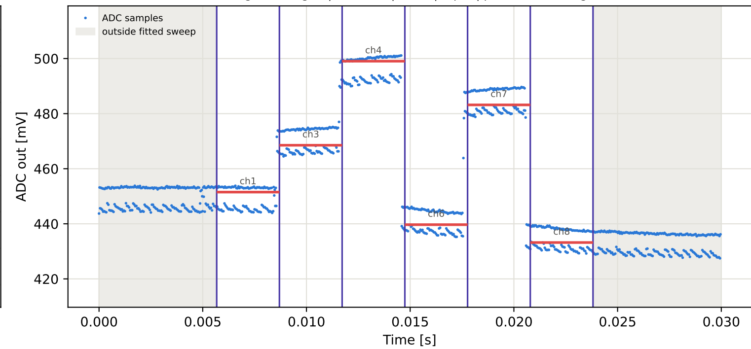
Tag10 &lt;- Tag3 | 945 MHz | run 0 | rep 1 | phase 105.97 deg
