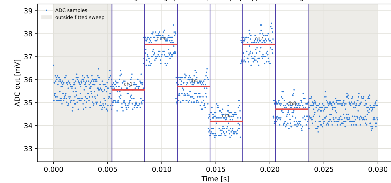
Tag16 &lt;- Tag6 | 775 MHz | run 0 | rep 1 | phase -48.96 deg
