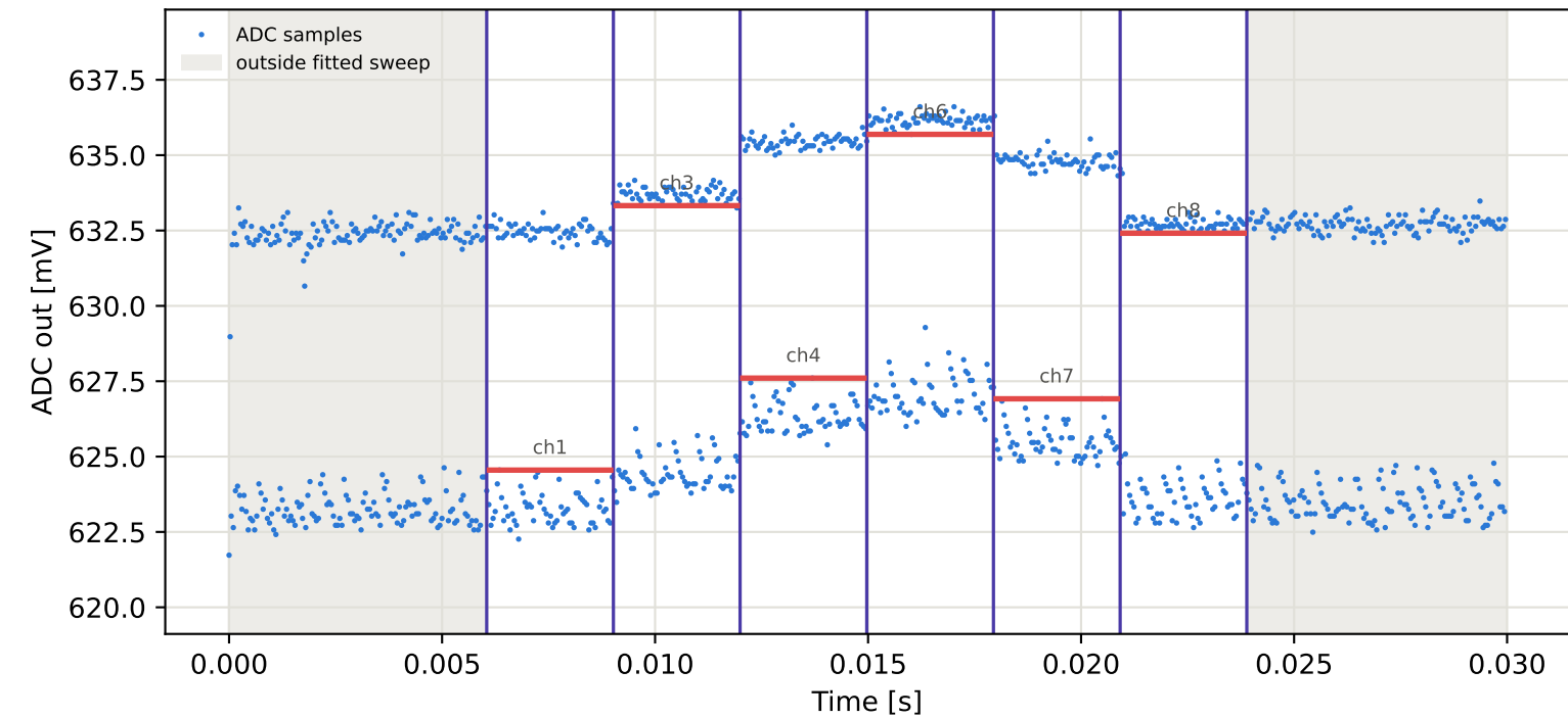
Tag6 &lt;- Tag4 | 855 MHz | run 0 | rep 1 | phase 142.69 deg
