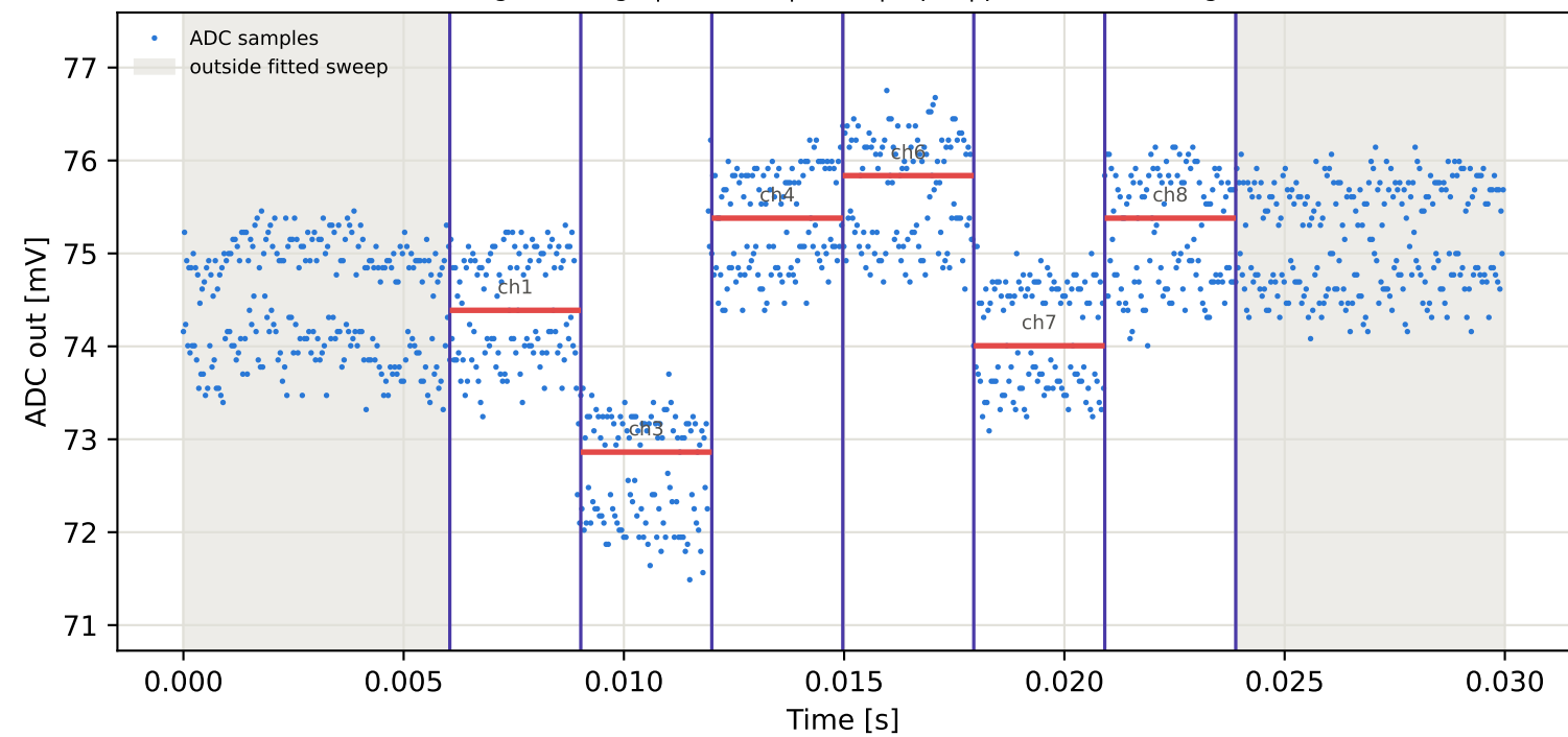
Tag16 &lt;- Tag5 | 795 MHz | run 0 | rep 1 | phase -100.39 deg
