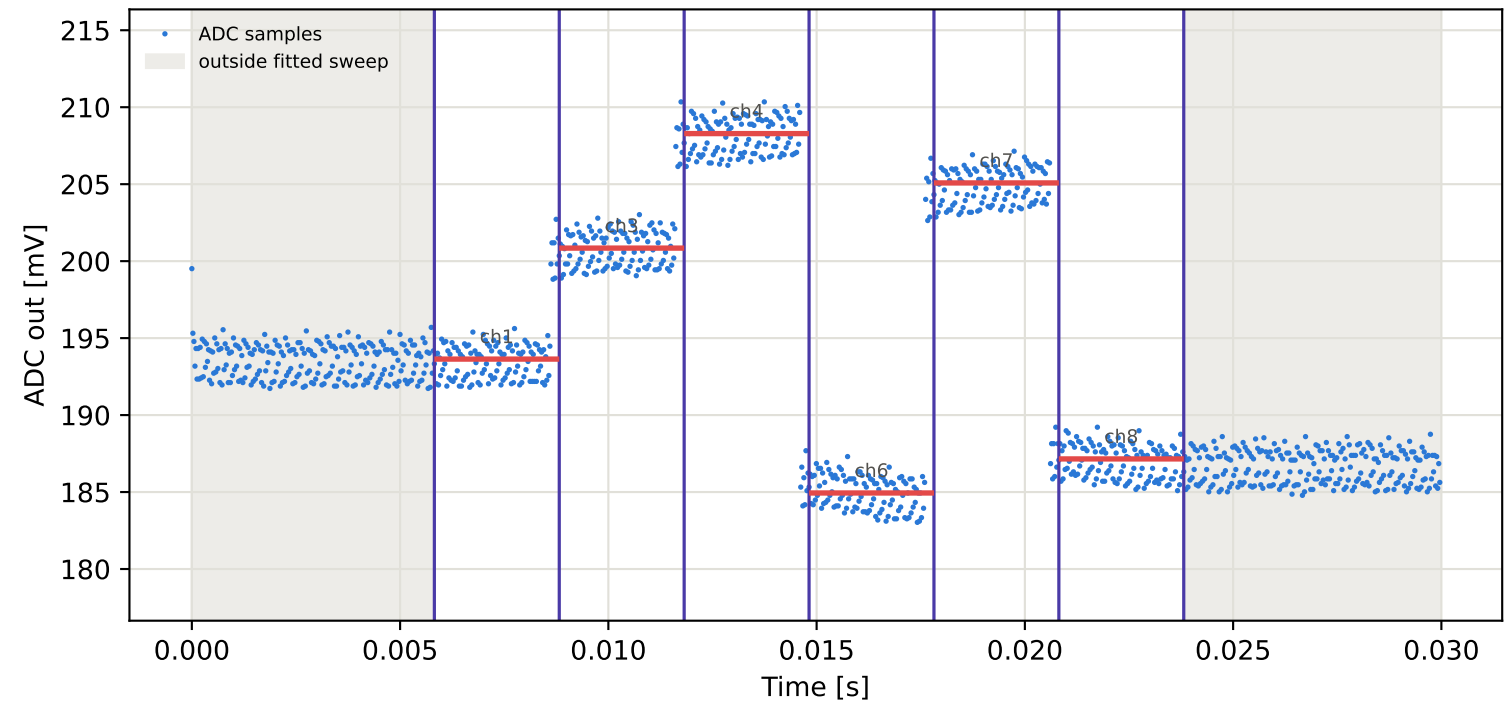
Tag10 &lt;- Tag1 | 965 MHz | run 0 | rep 1 | phase 129.23 deg
