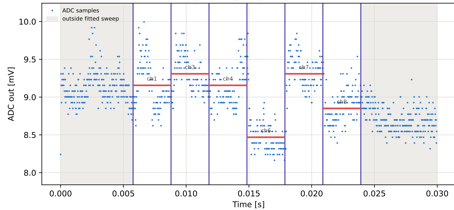
Tag3 &lt;- Tag2 | 775 MHz | run 0 | rep 1 | phase 13.79 deg
