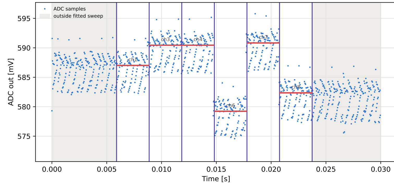
Tag8 &lt;- Tag15 | 965 MHz | run 0 | rep 1 | phase 114.84 deg
