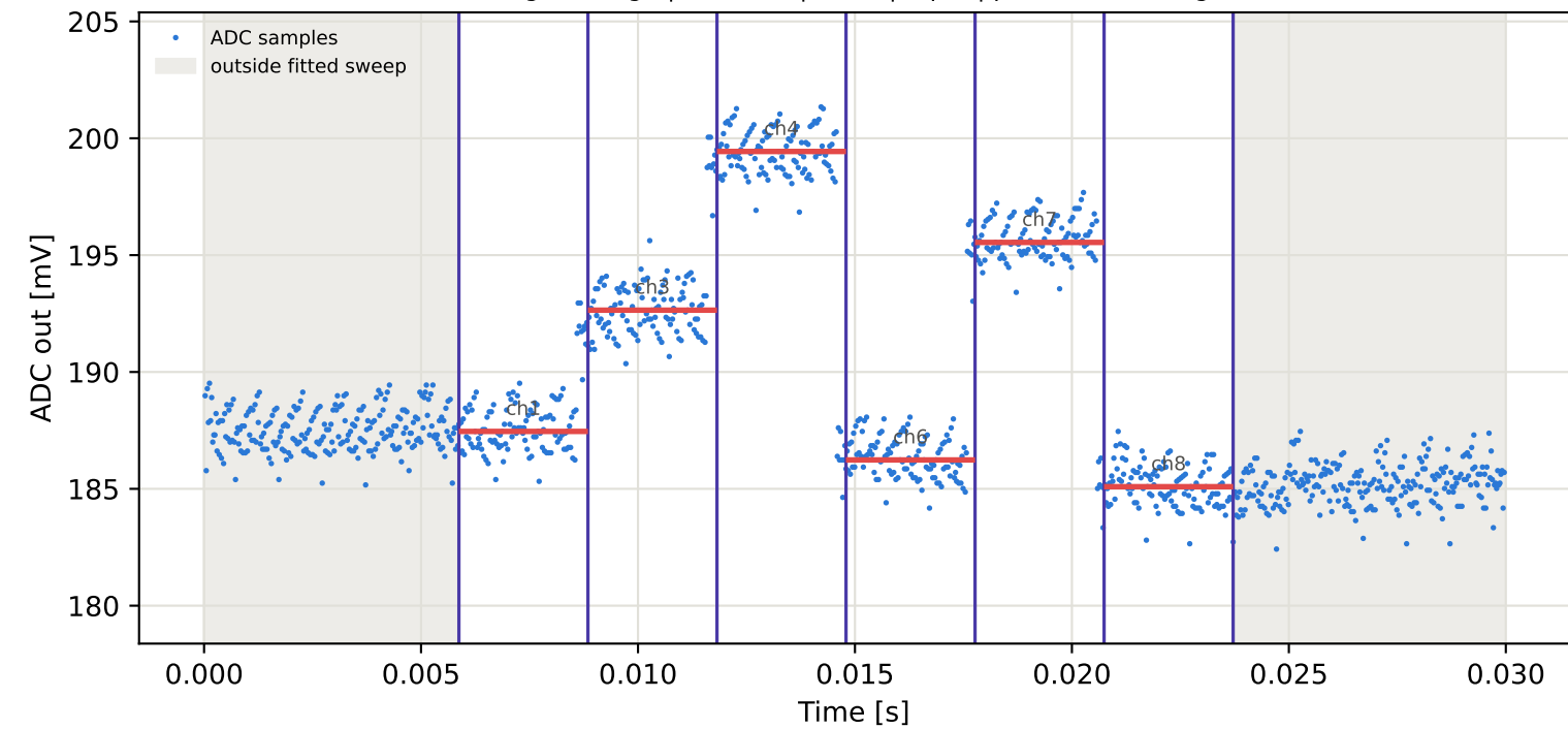
Tag7 &lt;- Tag1 | 965 MHz | run 0 | rep 1 | phase 178.18 deg
