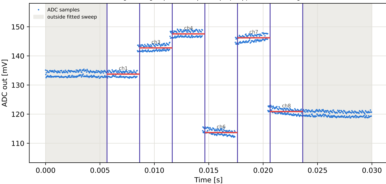
Tag3 &lt;- Tag16 | 935 MHz | run 0 | rep 1 | phase -27.79 deg
