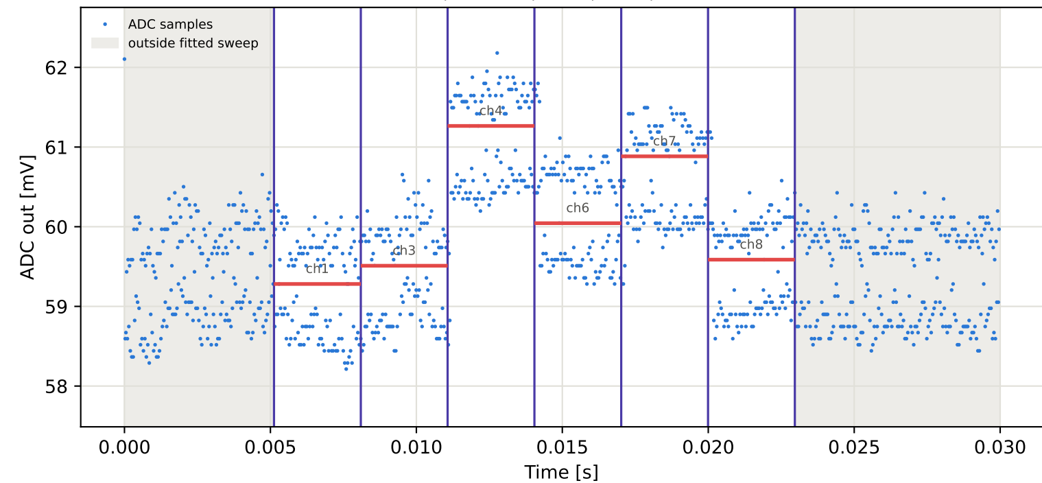
Tag10 &lt;- Tag1 | 805 MHz | run 0 | rep 1 | phase -90.25 deg
