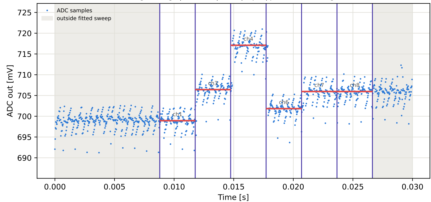
Tag8 &lt;- Tag5 | 955 MHz | run 0 | rep 1 | phase -168.13 deg
