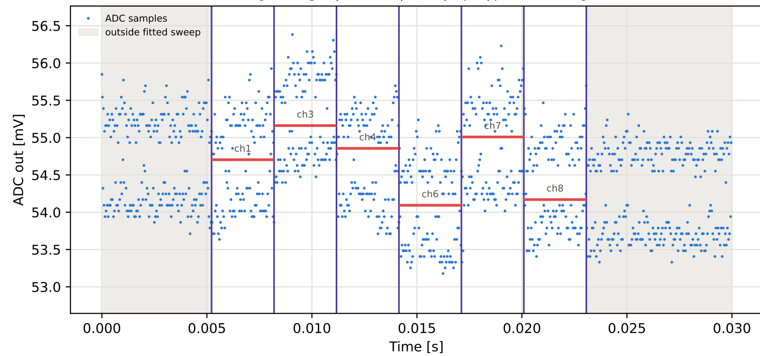
Tag1 &lt;- Tag2 | 795 MHz | run 0 | rep 1 | phase -32.40 deg
