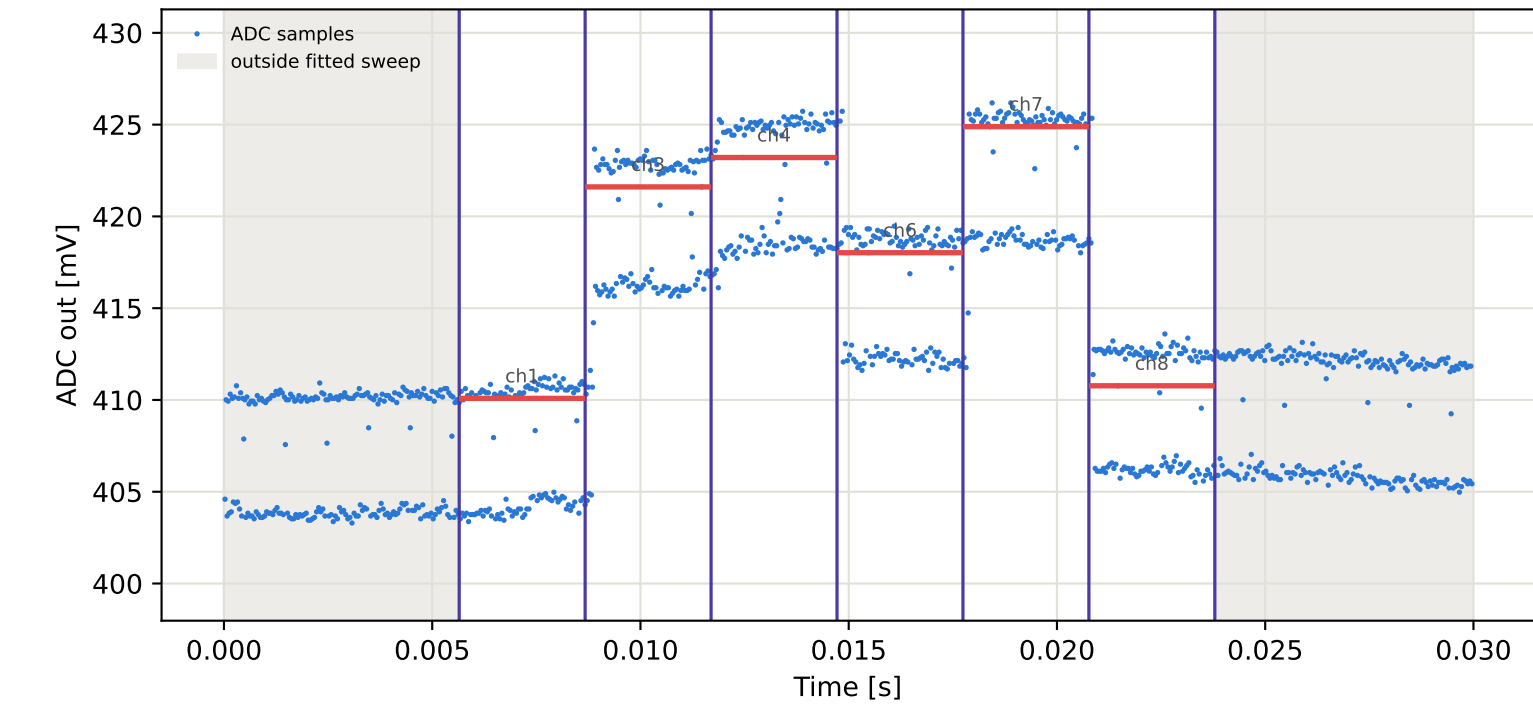
Tag5 &lt;- Tag3 | 855 MHz | run 0 | rep 1 | phase 97.02 deg
