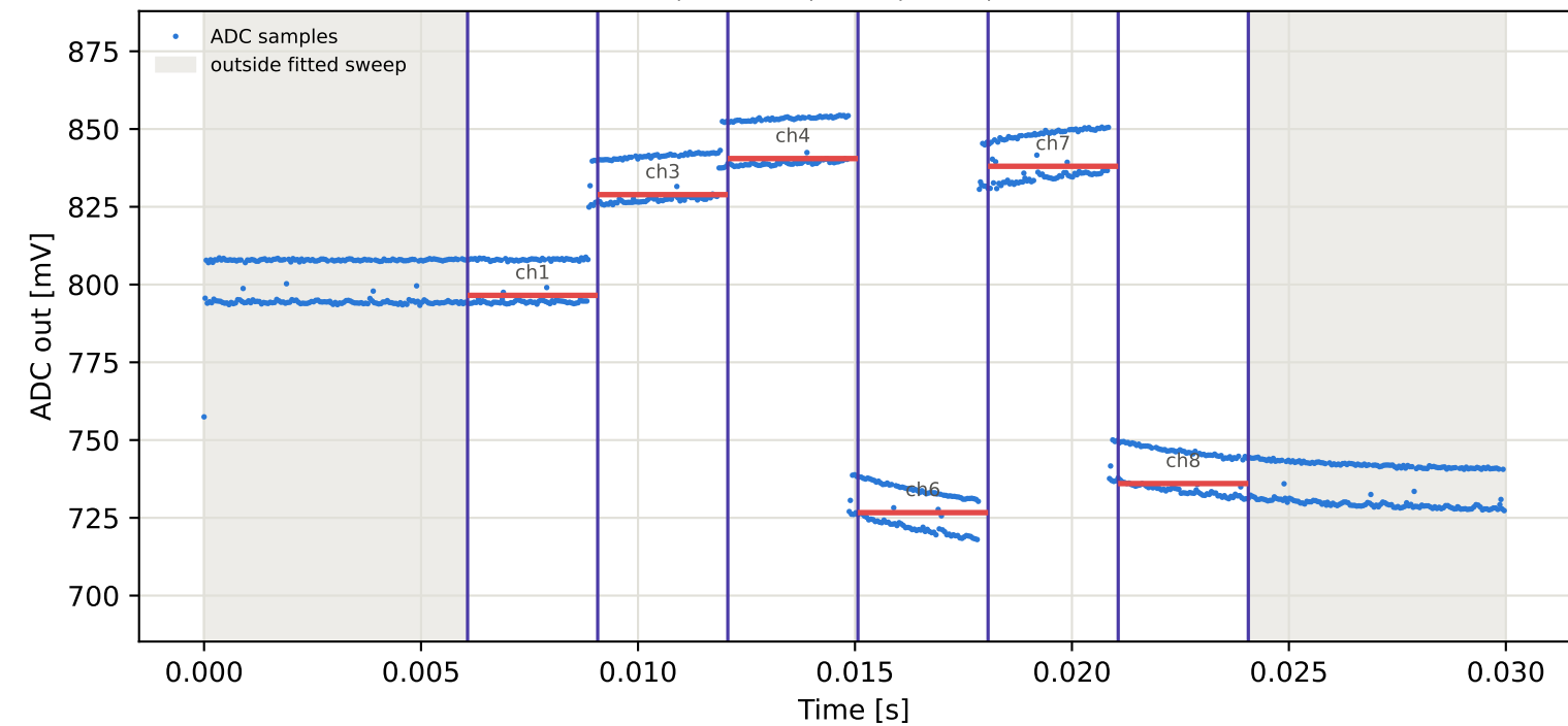
Tag8 &lt;- Tag16 | 915 MHz | run 0 | rep 1 | phase -25.95 deg
