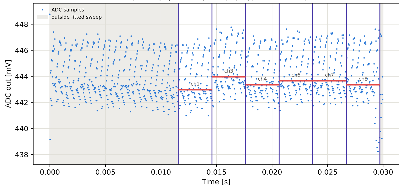
Tag5 &lt;- Tag4 | 955 MHz | run 0 | rep 1 | phase 165.56 deg
