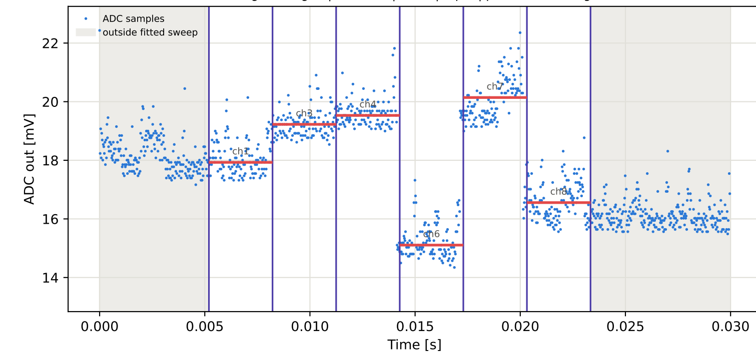
Tag2 &lt;- Tag15 | 965 MHz | run 0 | rep 1 | phase -21.63 deg
