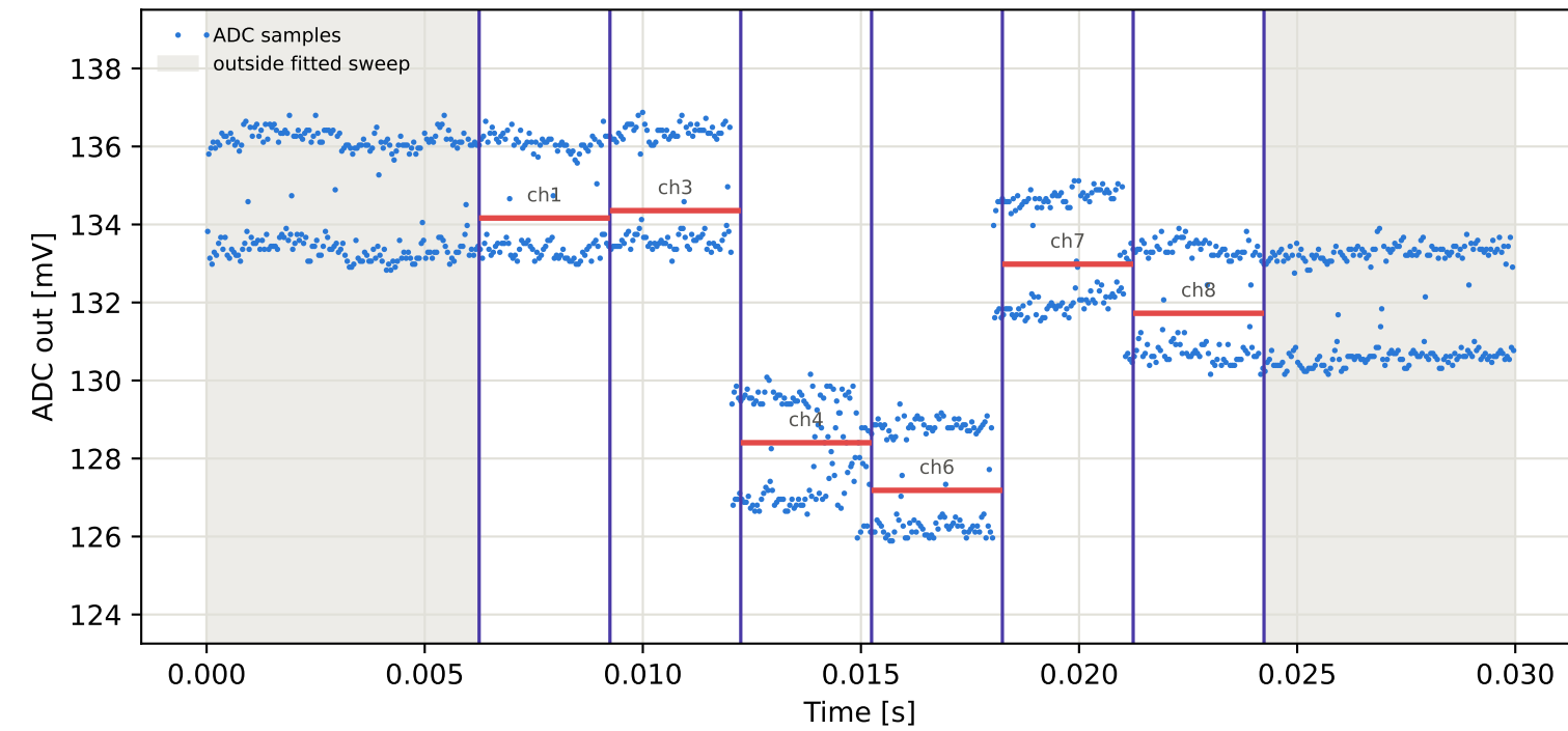
Tag9 &lt;- Tag7 | 995 MHz | run 0 | rep 1 | phase 48.98 deg
