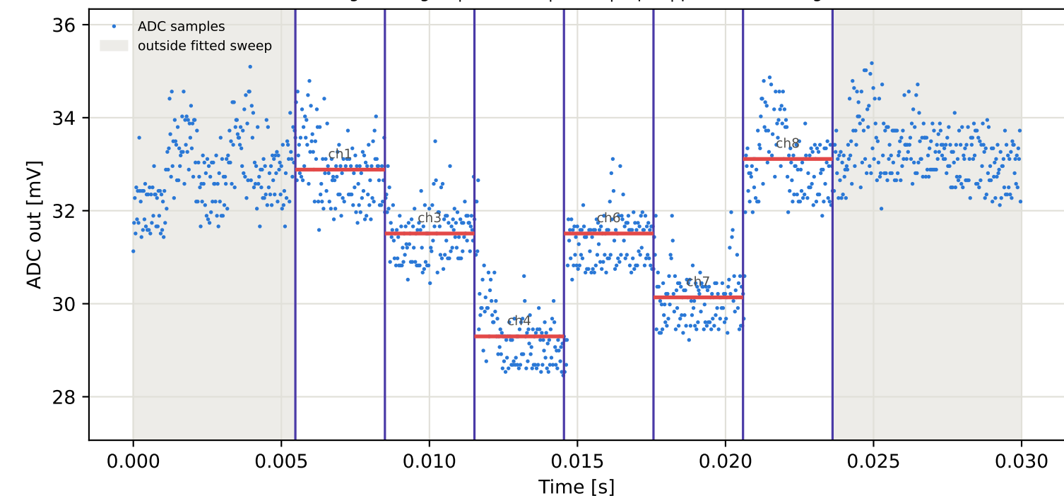
Tag2 &lt;- Tag16 | 945 MHz | run 0 | rep 1 | phase 84.01 deg
