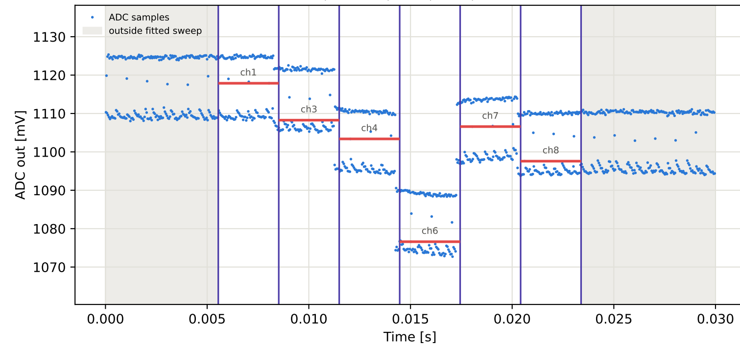
Tag8 &lt;- Tag6 | 895 MHz | run 0 | rep 1 | phase 23.14 deg
