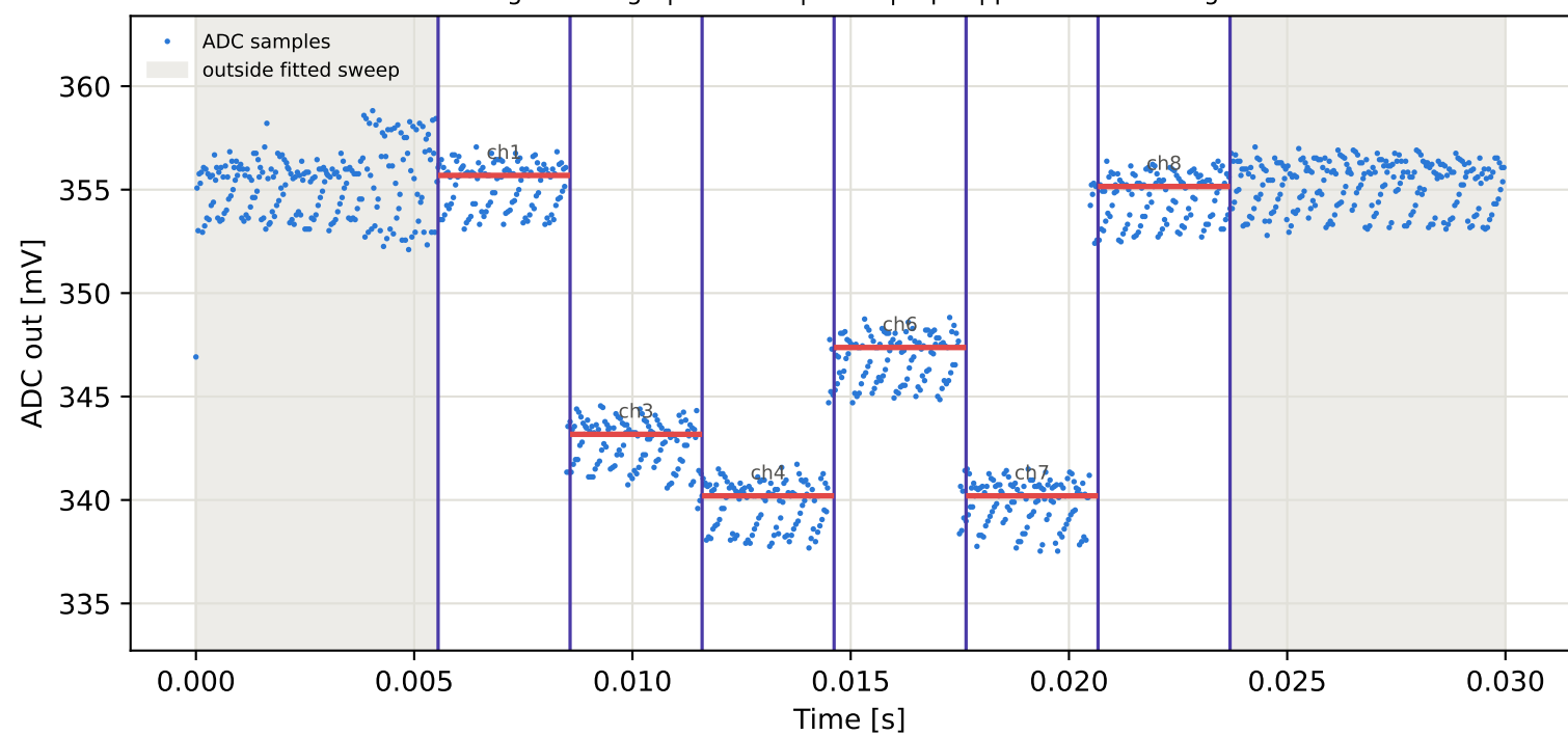
Tag15 &lt;- Tag6 | 855 MHz | run 0 | rep 1 | phase 28.39 deg
