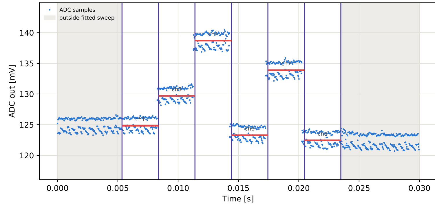
Tag9 &lt;- Tag16 | 995 MHz | run 0 | rep 1 | phase -45.25 deg
