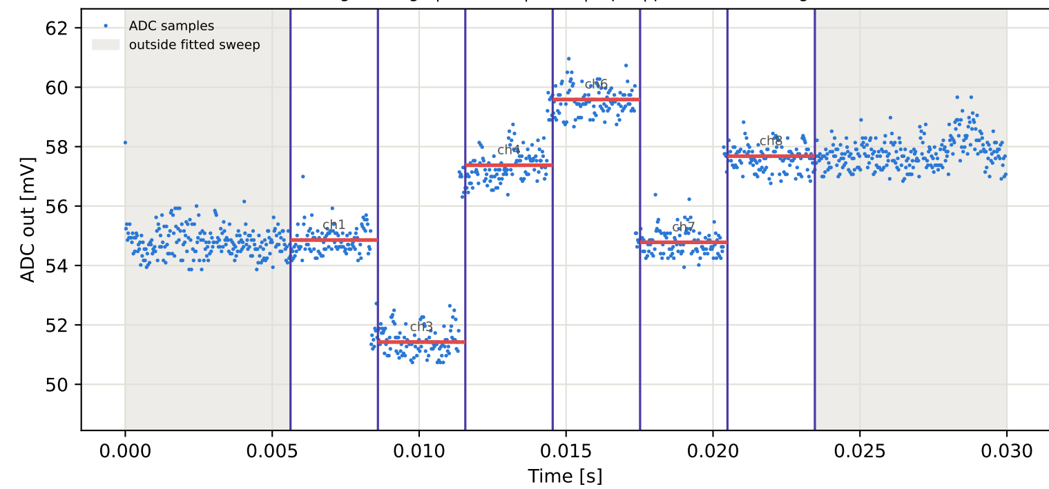
Tag6 &lt;- Tag5 | 775 MHz | run 0 | rep 1 | phase -144.92 deg
