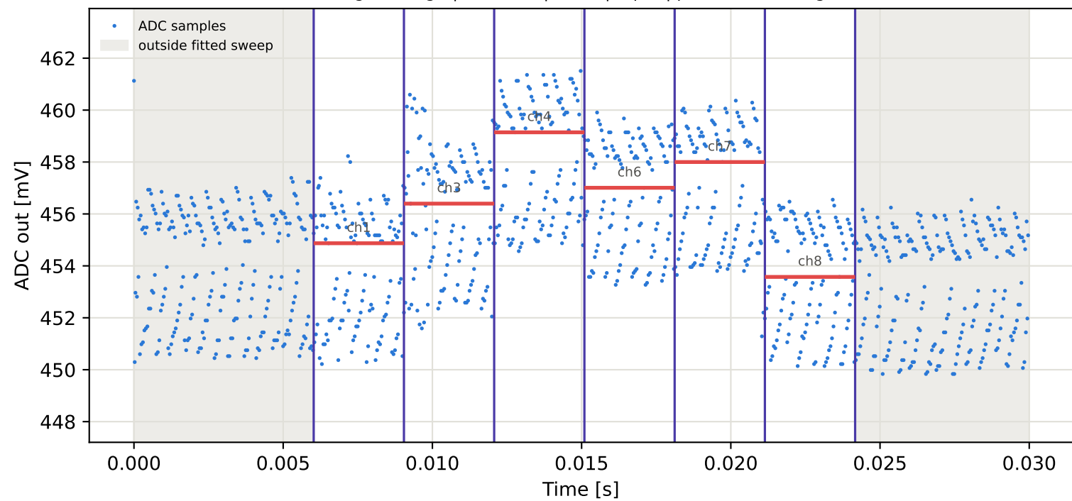
Tag7 &lt;- Tag4 | 915 MHz | run 0 | rep 1 | phase 169.72 deg
