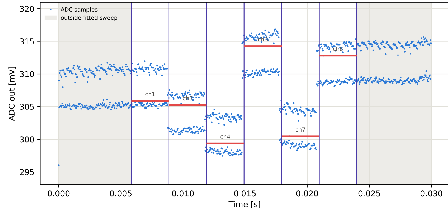
Tag4 &lt;- Tag3 | 965 MHz | run 0 | rep 1 | phase 135.13 deg
