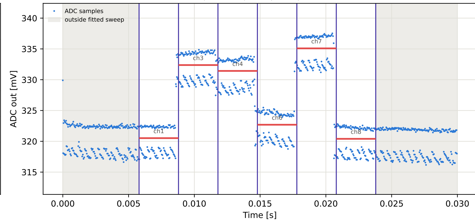
Tag5 &lt;- Tag4 | 805 MHz | run 0 | rep 1 | phase -41.75 deg
