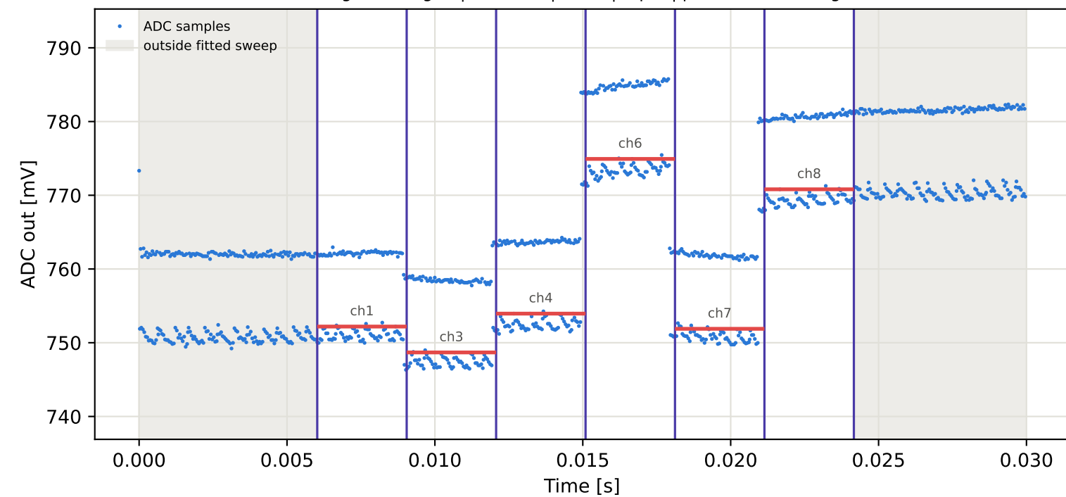
Tag15 &lt;- Tag10 | 895 MHz | run 0 | rep 1 | phase -175.87 deg
