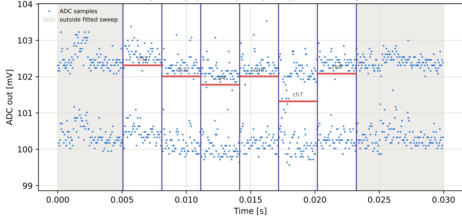
Tag15 &lt;- Tag4 | 785 MHz | run 0 | rep 1 | phase -42.67 deg
