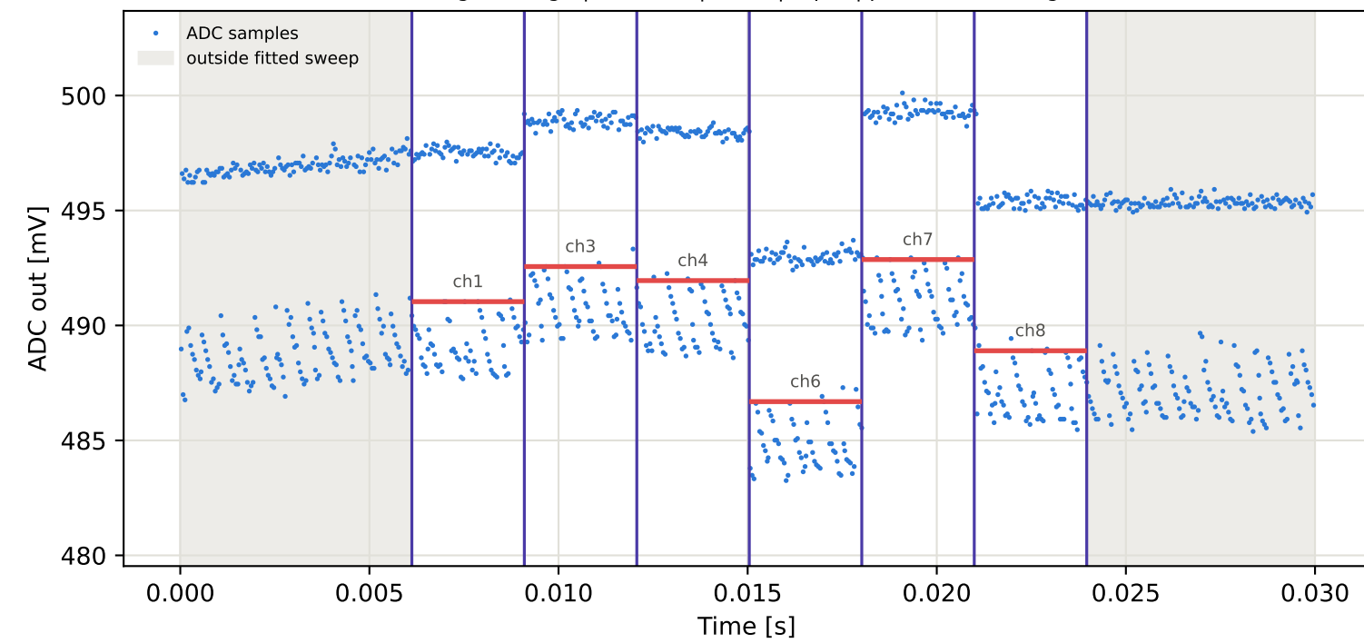
Tag9 &lt;- Tag10 | 975 MHz | run 0 | rep 1 | phase -89.32 deg
