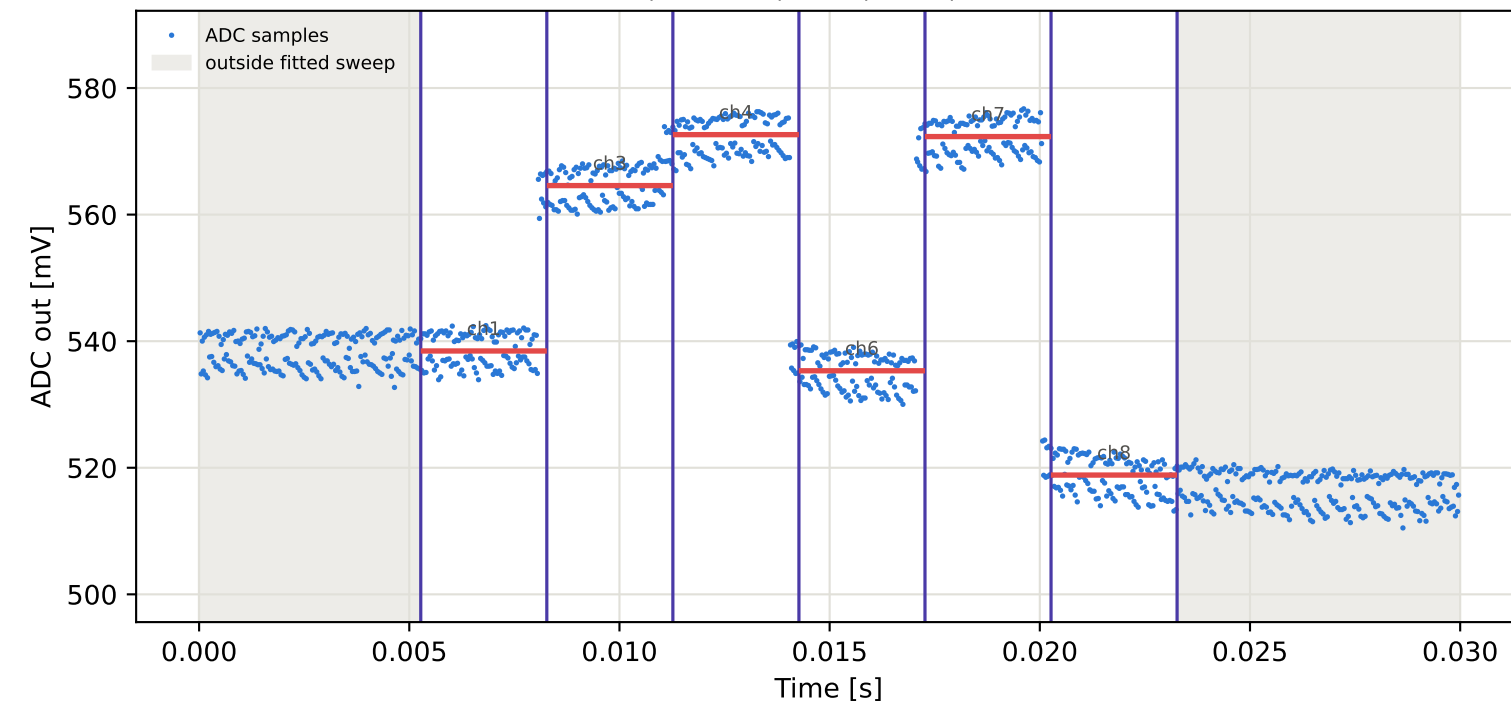
Tag9 &lt;- Tag7 | 885 MHz | run 0 | rep 1 | phase -53.34 deg
