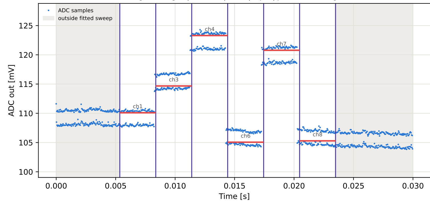
Tag10 &lt;- Tag3 | 995 MHz | run 0 | rep 1 | phase 77.82 deg
