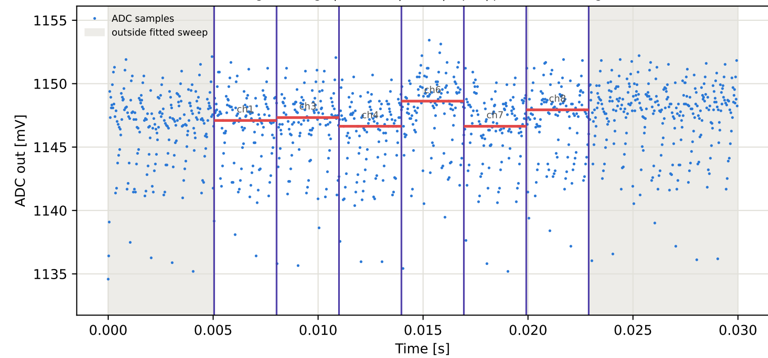
Tag15 &lt;- Tag4 | 935 MHz | run 0 | rep 1 | phase -19.62 deg
