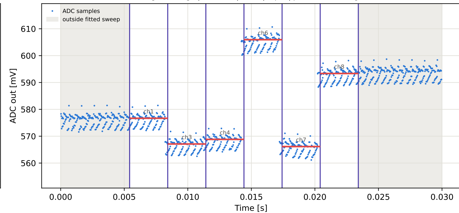
Tag2 &lt;- Tag10 | 955 MHz | run 0 | rep 1 | phase 96.30 deg
