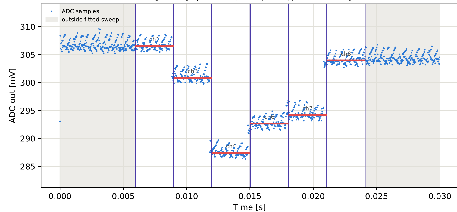
Tag6 &lt;- Tag1 | 945 MHz | run 0 | rep 1 | phase 62.85 deg
