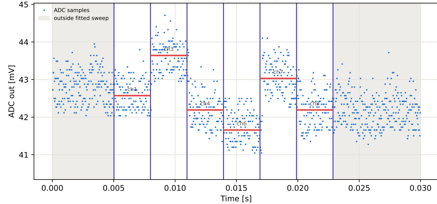
Tag15 &lt;- Tag6 | 775 MHz | run 0 | rep 1 | phase 29.44 deg
