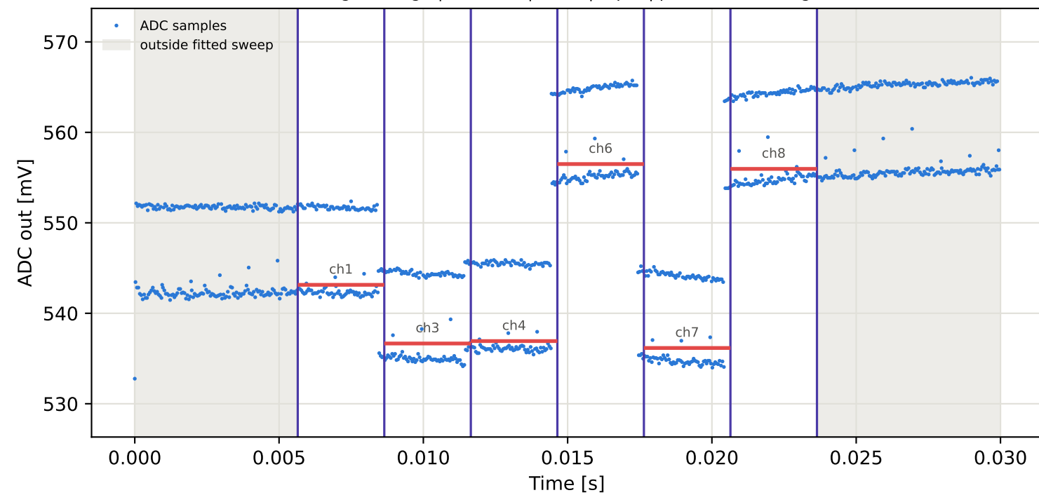
Tag8 &lt;- Tag10 | 905 MHz | run 0 | rep 1 | phase -43.32 deg
