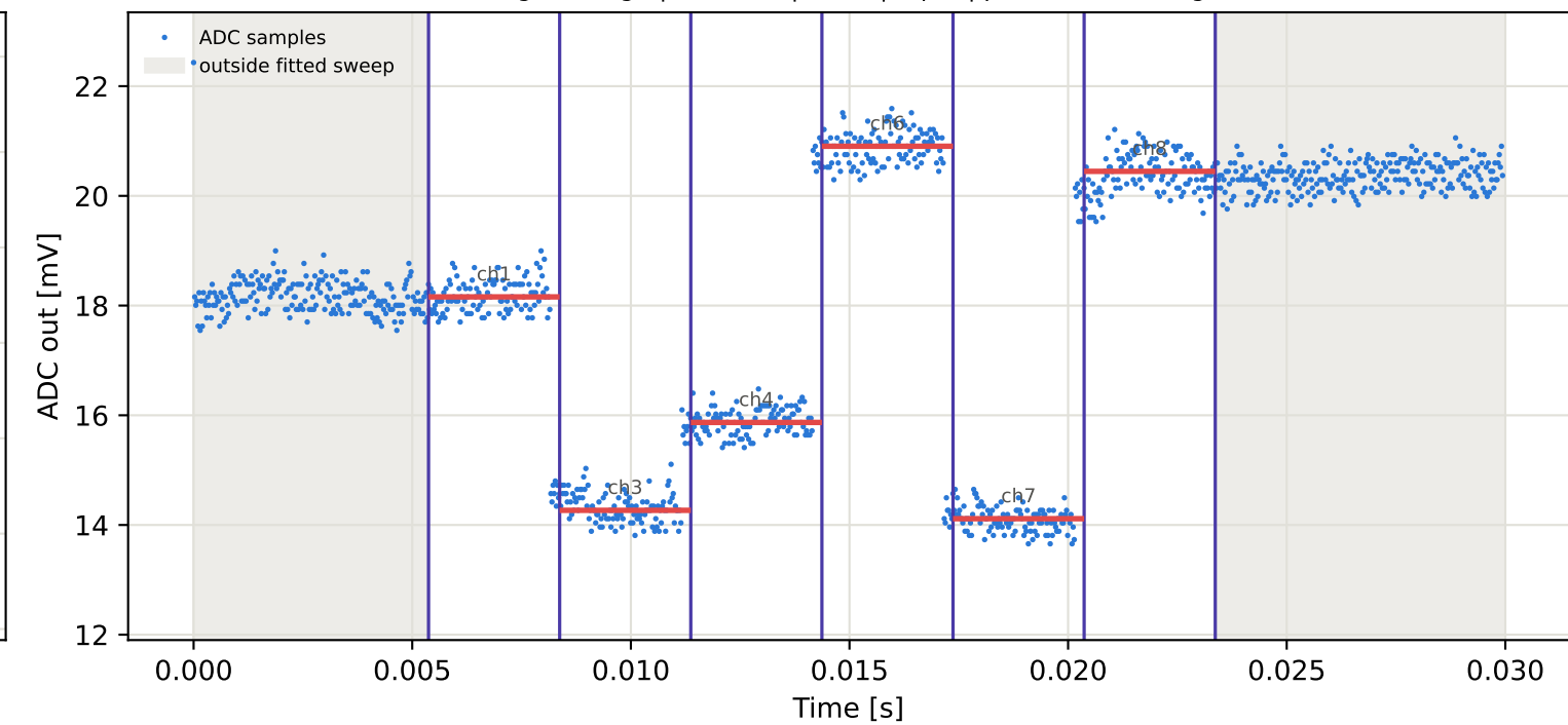
Tag3 &lt;- Tag7 | 795 MHz | run 0 | rep 1 | phase 107.03 deg
