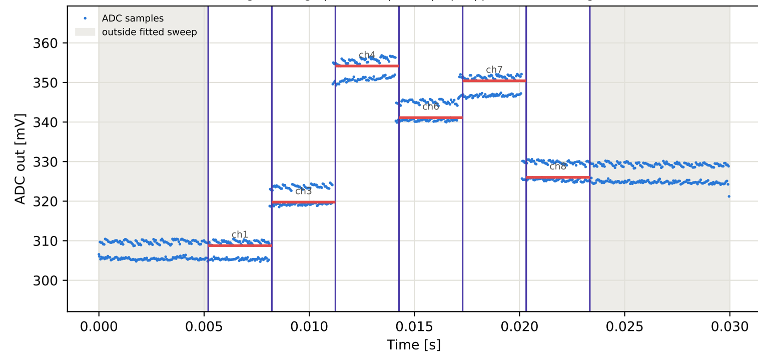
Tag16 &lt;- Tag1 | 825 MHz | run 0 | rep 1 | phase 102.65 deg
