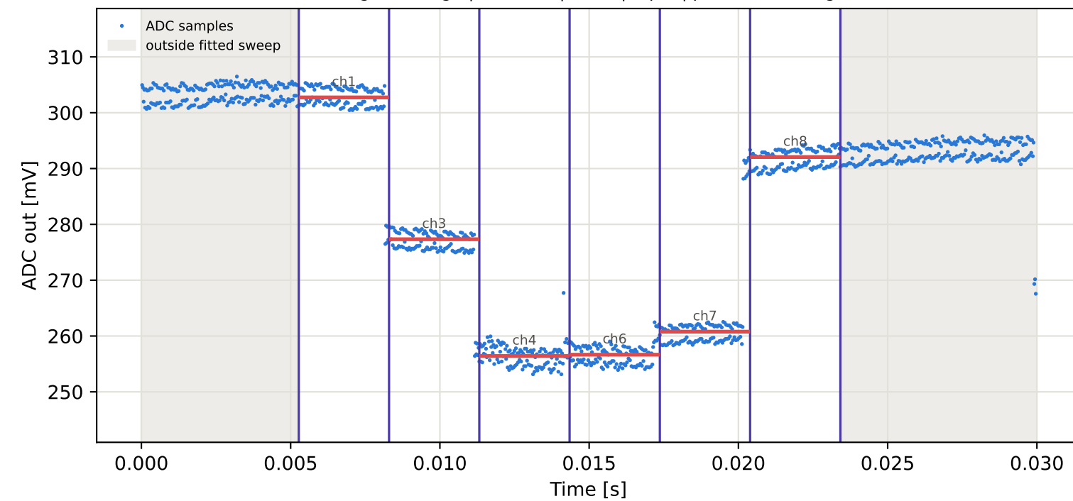
Tag10 &lt;- Tag8 | 875 MHz | run 0 | rep 1 | phase -42.84 deg
