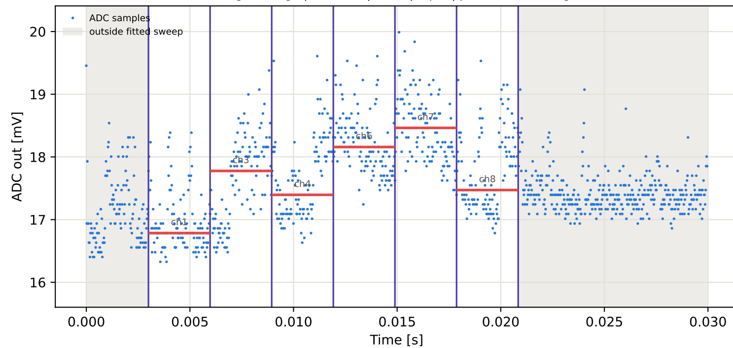
Tag3 &lt;- Tag10 | 845 MHz | run 0 | rep 1 | phase -144.03 deg
