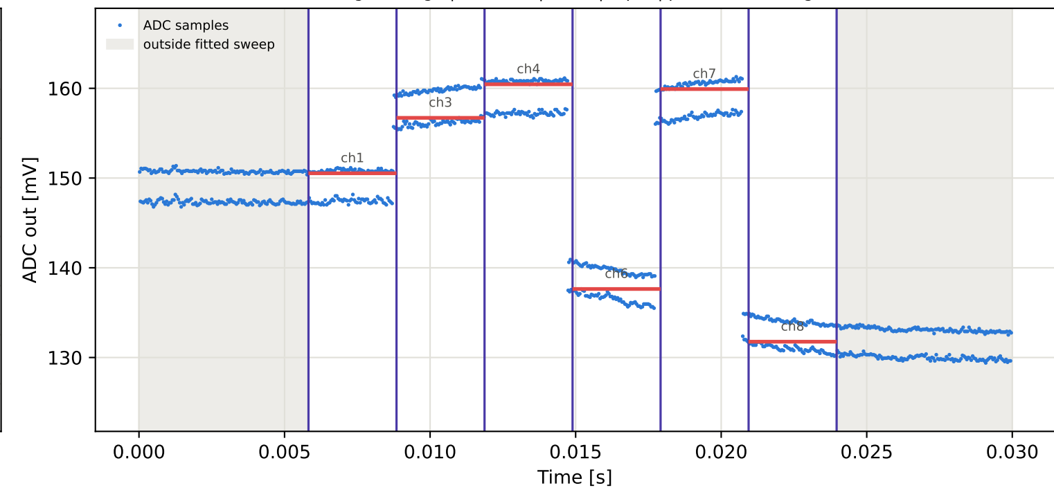
Tag9 &lt;- Tag6 | 895 MHz | run 0 | rep 1 | phase -88.52 deg
