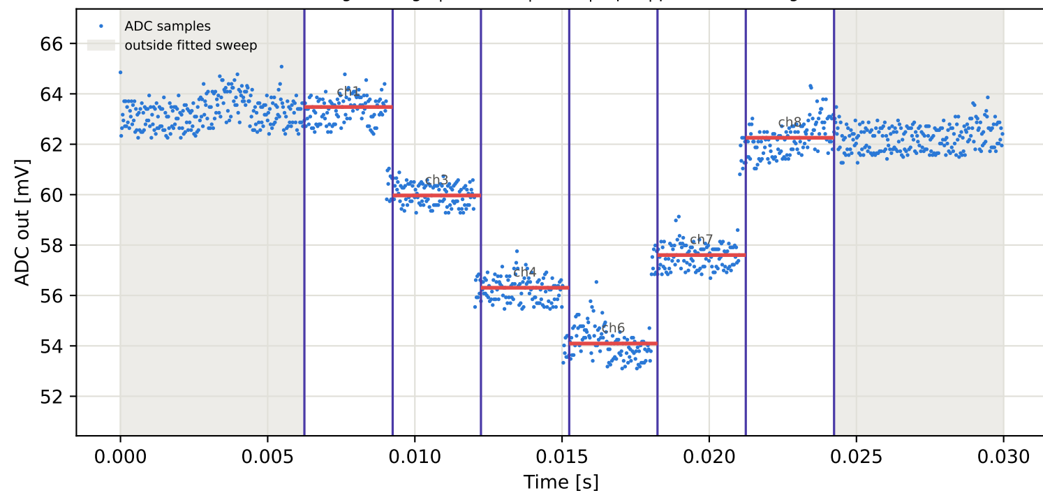
Tag2 &lt;- Tag8 | 905 MHz | run 0 | rep 1 | phase 53.27 deg
