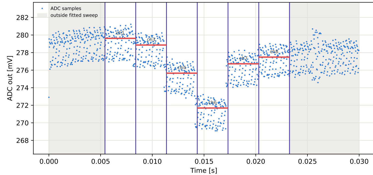
Tag1 &lt;- Tag4 | 905 MHz | run 0 | rep 1 | phase 9.18 deg
