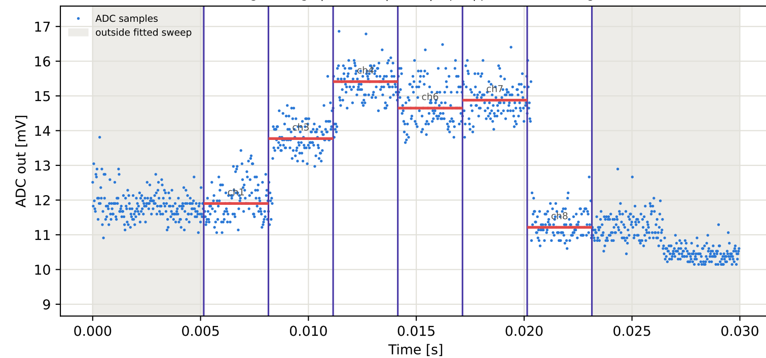
Tag2 &lt;- Tag5 | 895 MHz | run 0 | rep 1 | phase -156.54 deg
