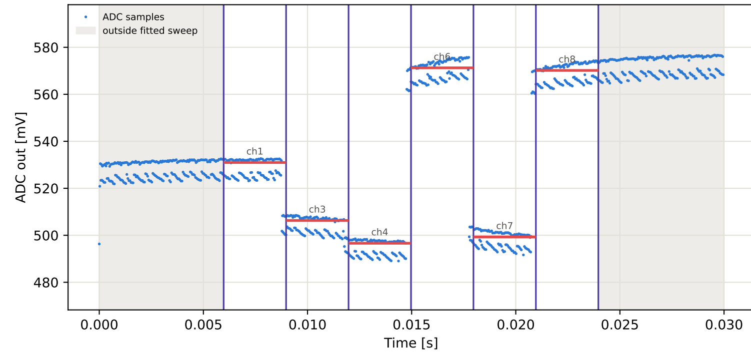
Tag9 &lt;- Tag16 | 915 MHz | run 0 | rep 1 | phase -44.12 deg
