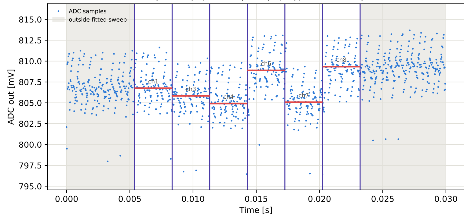
Tag16 &lt;- Tag15 | 925 MHz | run 0 | rep 1 | phase -112.70 deg
