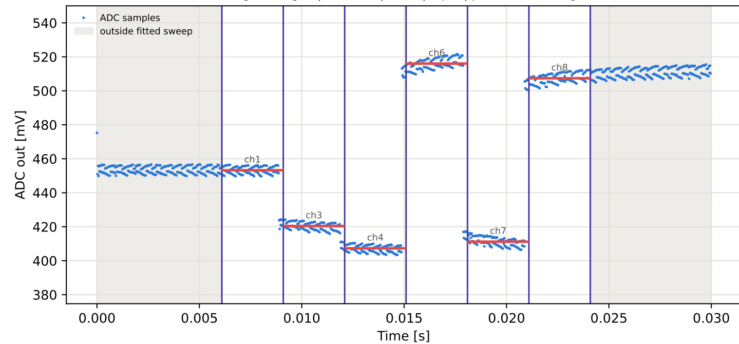
Tag7 &lt;- Tag3 | 915 MHz | run 0 | rep 1 | phase 132.61 deg
