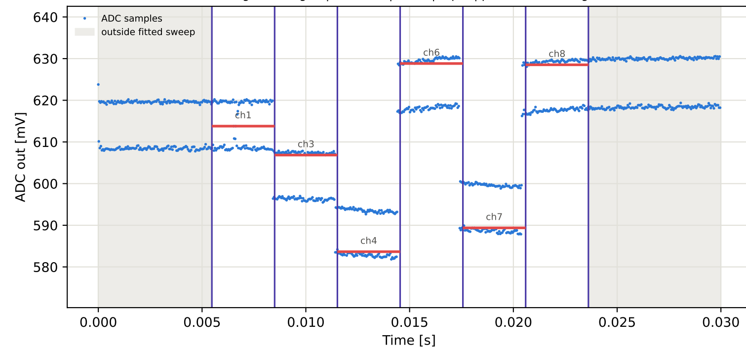
Tag16 &lt;- Tag10 | 965 MHz | run 0 | rep 1 | phase 119.07 deg
