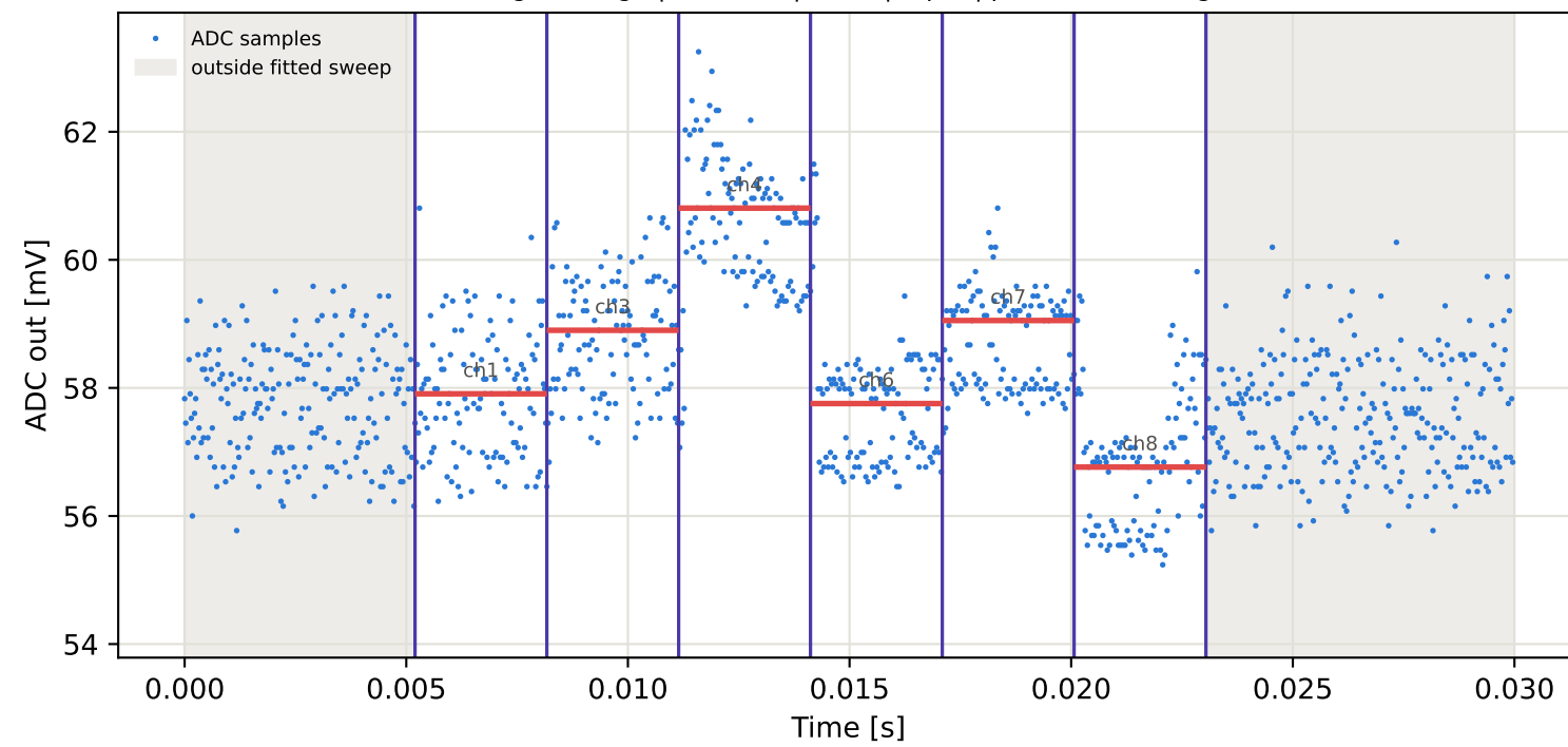
Tag3 &lt;- Tag10 | 985 MHz | run 0 | rep 1 | phase 148.30 deg
