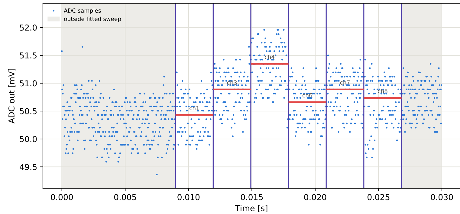
Tag9 &lt;- Tag2 | 845 MHz | run 0 | rep 1 | phase -84.35 deg
