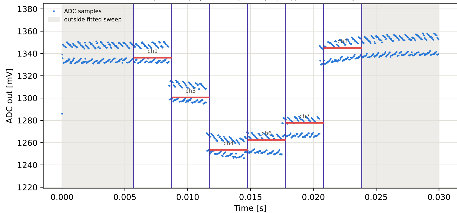
Tag16 &lt;- Tag7 | 915 MHz | run 0 | rep 1 | phase 56.14 deg
