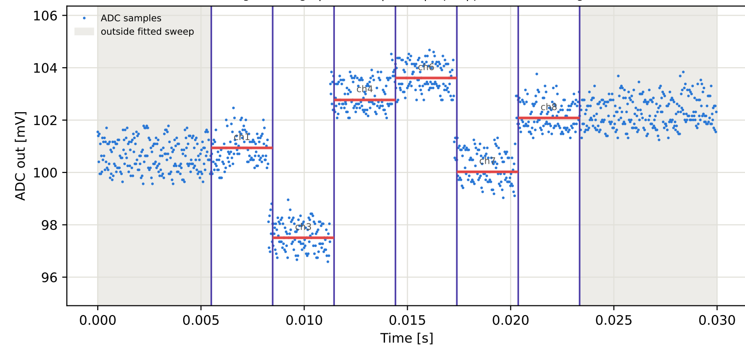
Tag15 &lt;- Tag5 | 785 MHz | run 0 | rep 1 | phase -137.08 deg
