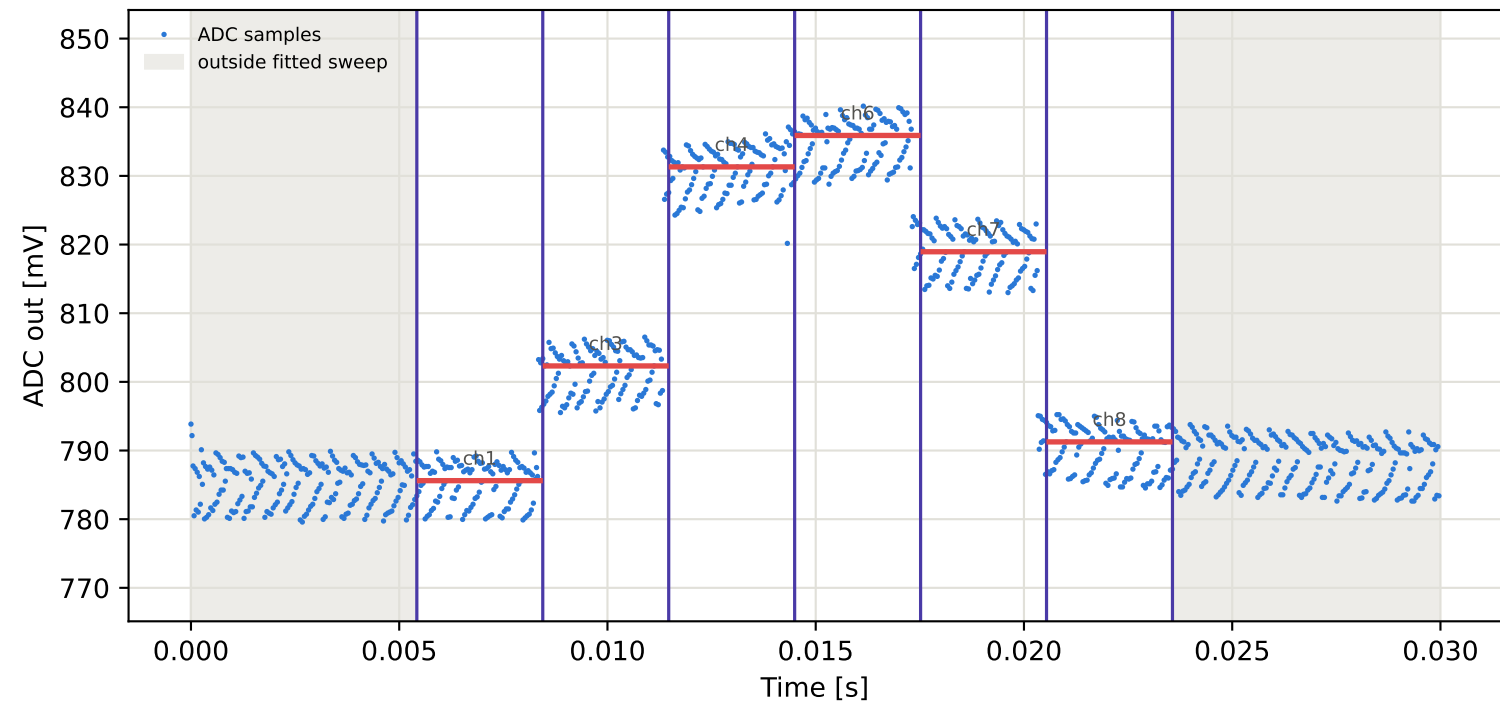
Tag2 &lt;- Tag1 | 925 MHz | run 0 | rep 1 | phase -52.38 deg
