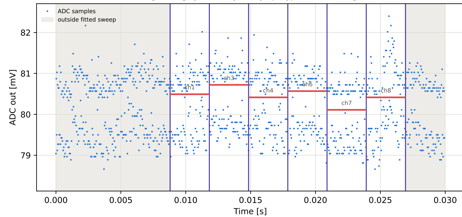
Tag8 &lt;- Tag4 | 785 MHz | run 0 | rep 1 | phase 96.87 deg
