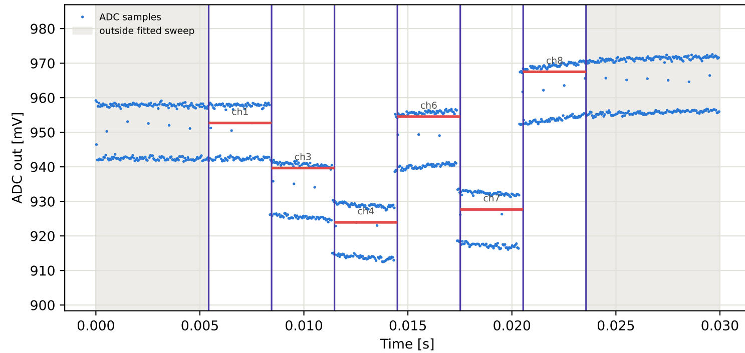
Tag16 &lt;- Tag10 | 915 MHz | run 0 | rep 1 | phase -84.58 deg
