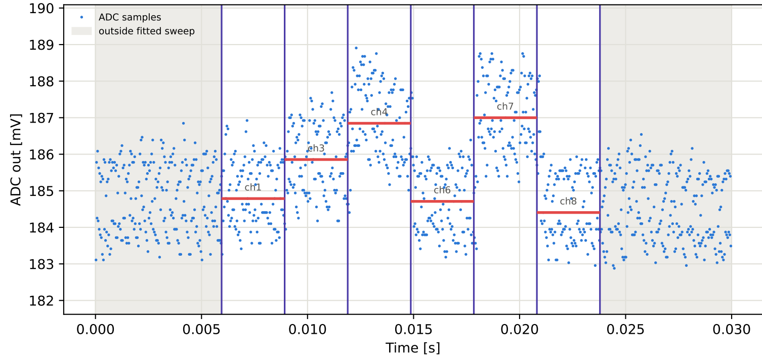
Tag6 &lt;- Tag10 | 775 MHz | run 0 | rep 1 | phase -159.37 deg
