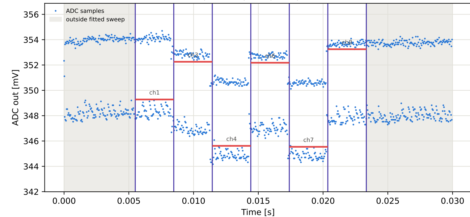
Tag15 &lt;- Tag1 | 825 MHz | run 0 | rep 1 | phase 115.68 deg
