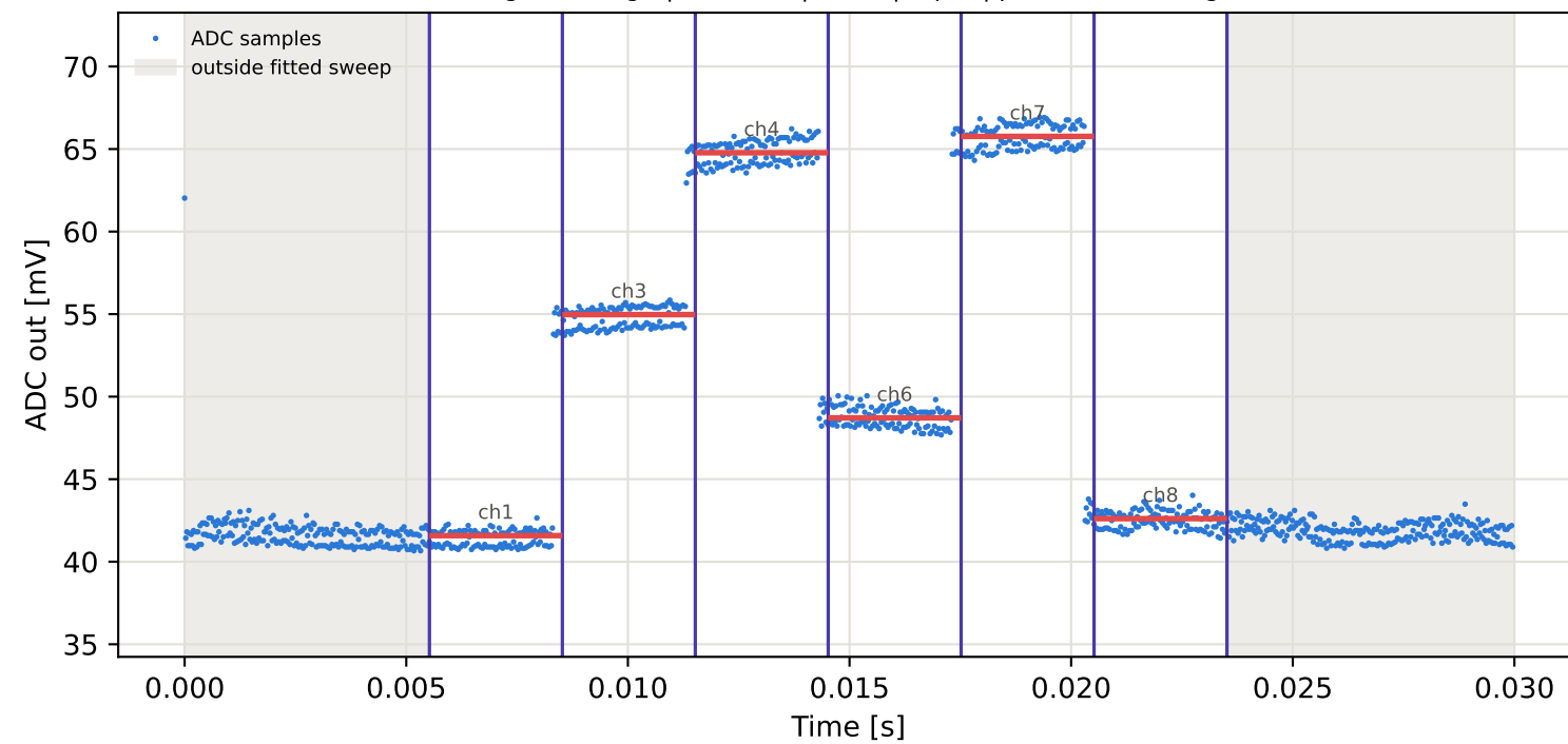
Tag10 &lt;- Tag8 | 805 MHz | run 0 | rep 1 | phase 73.60 deg
