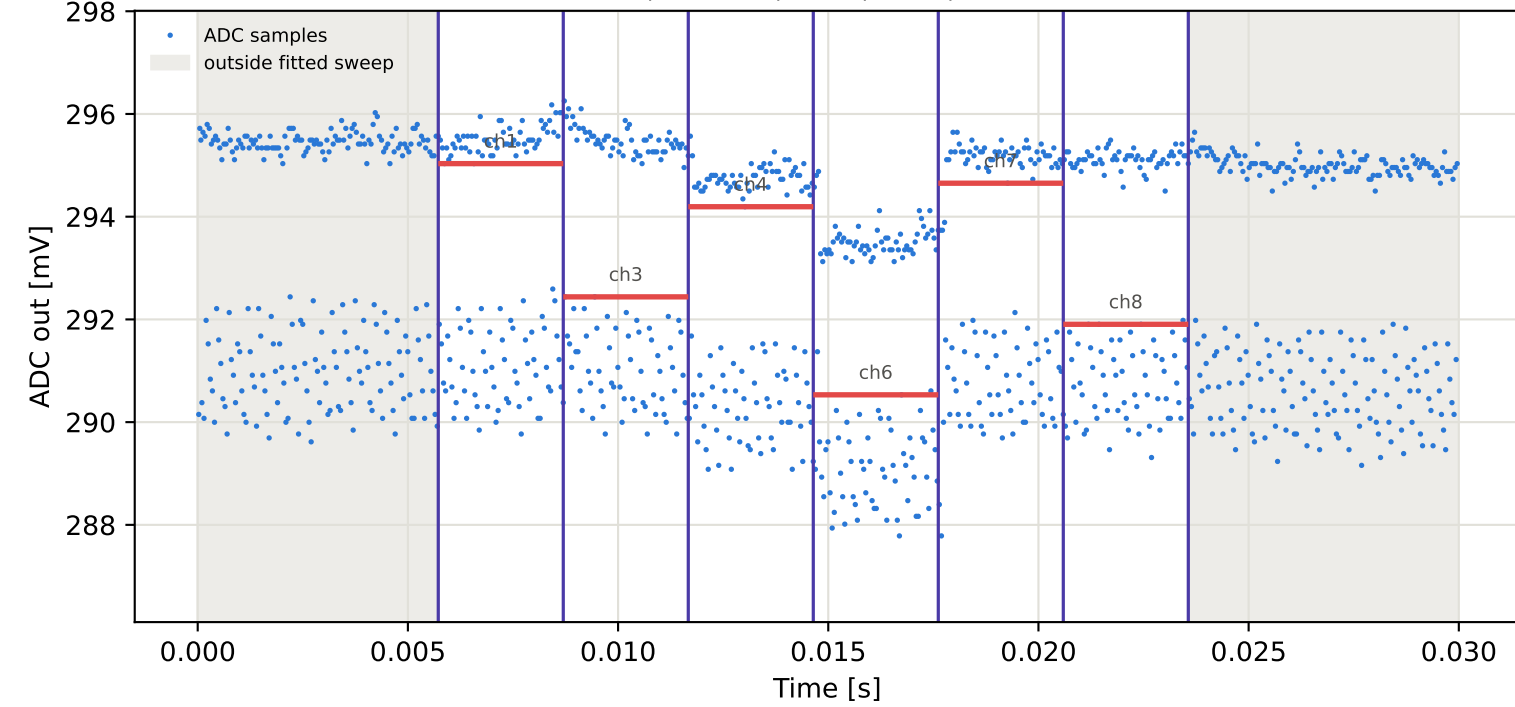
Tag3 &lt;- Tag2 | 985 MHz | run 0 | rep 1 | phase -11.82 deg
