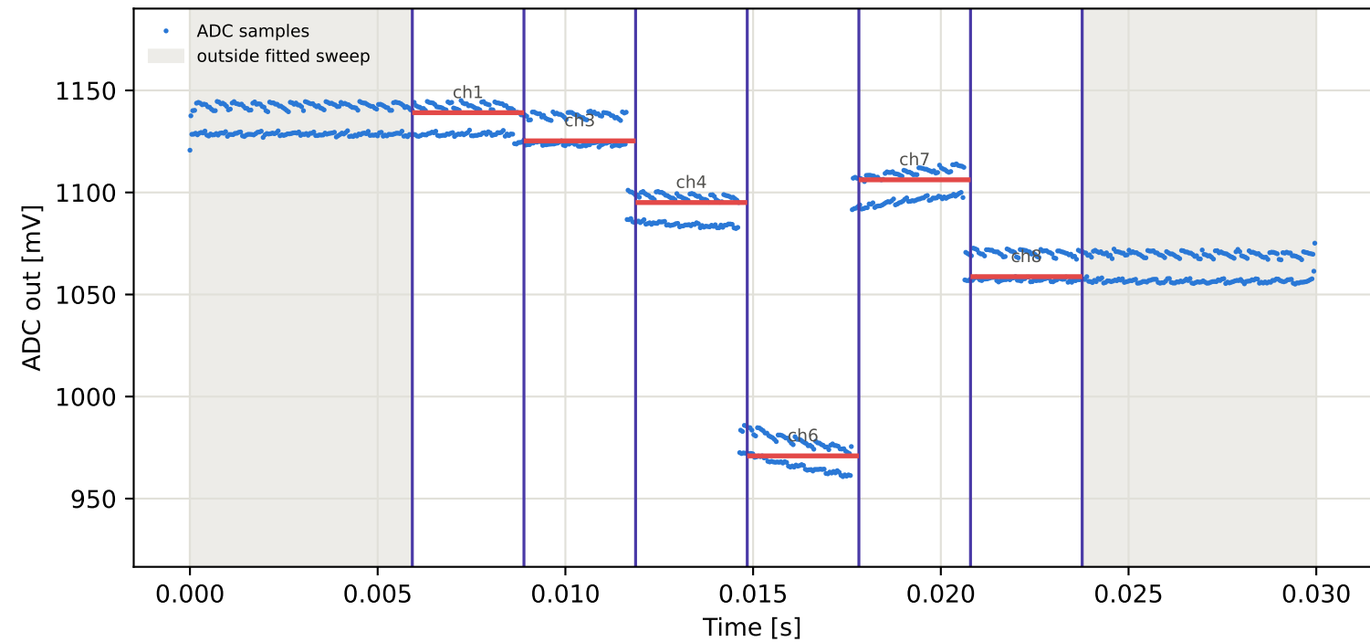
Tag8 &lt;- Tag7 | 905 MHz | run 0 | rep 1 | phase 27.58 deg
