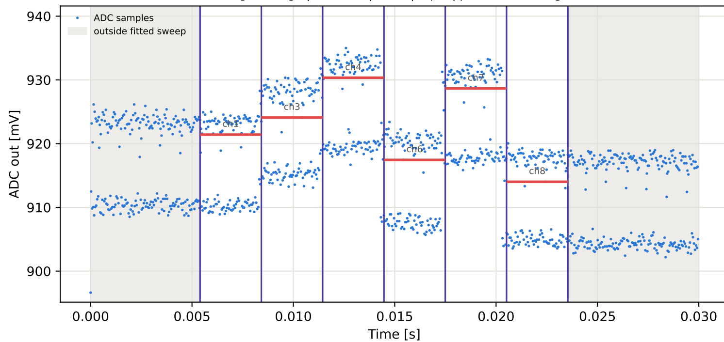
Tag6 &lt;- Tag4 | 885 MHz | run 0 | rep 1 | phase -169.65 deg
