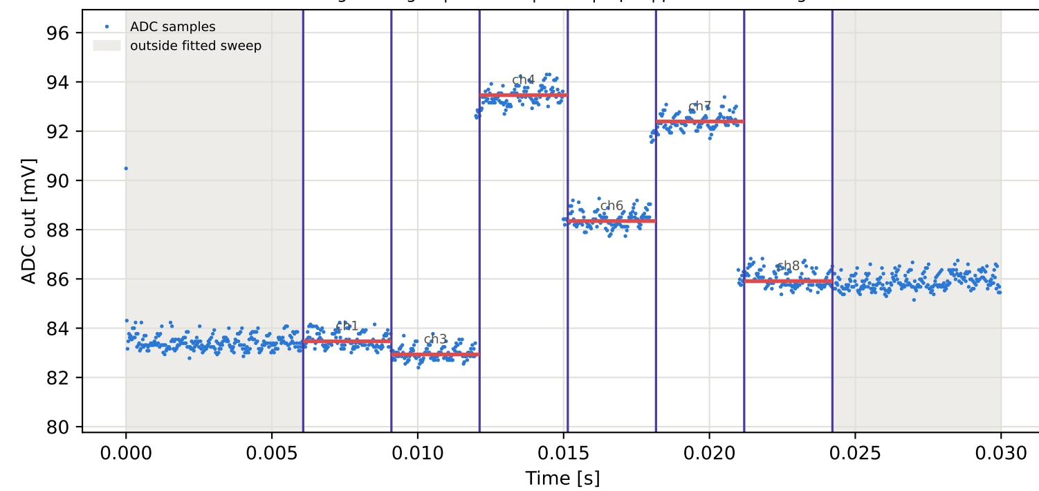
Tag7 &lt;- Tag3 | 785 MHz | run 0 | rep 1 | phase 164.18 deg
