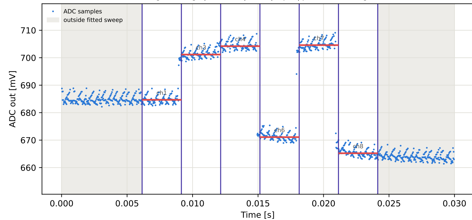
Tag10 &lt;- Tag9 | 895 MHz | run 0 | rep 1 | phase -42.90 deg
