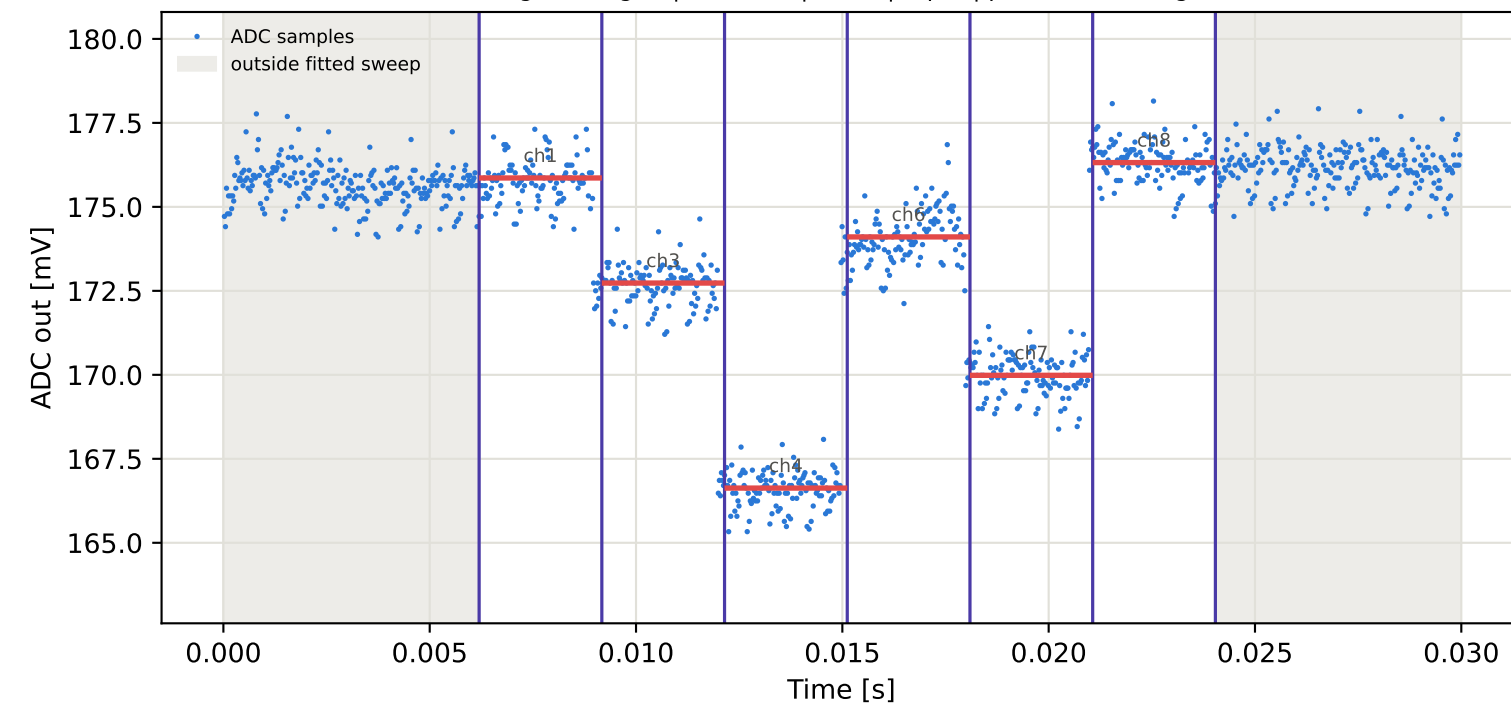
Tag6 &lt;- Tag2 | 995 MHz | run 0 | rep 1 | phase 143.46 deg
