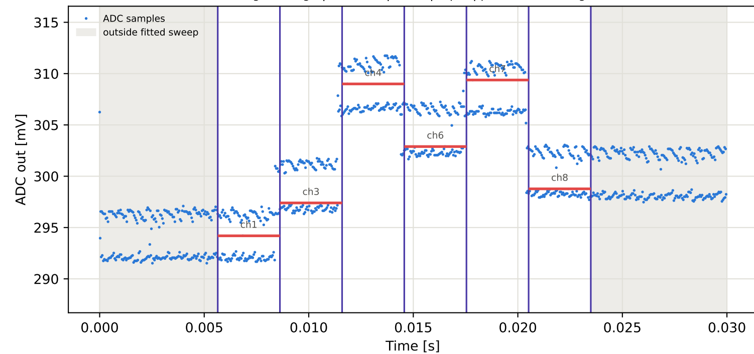
Tag7 &lt;- Tag5 | 825 MHz | run 0 | rep 1 | phase 115.39 deg
