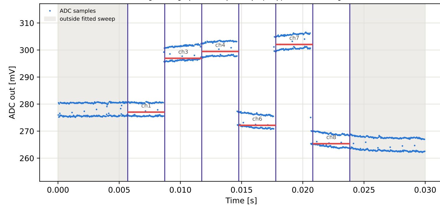
Tag9 &lt;- Tag7 | 865 MHz | run 0 | rep 1 | phase -43.02 deg
