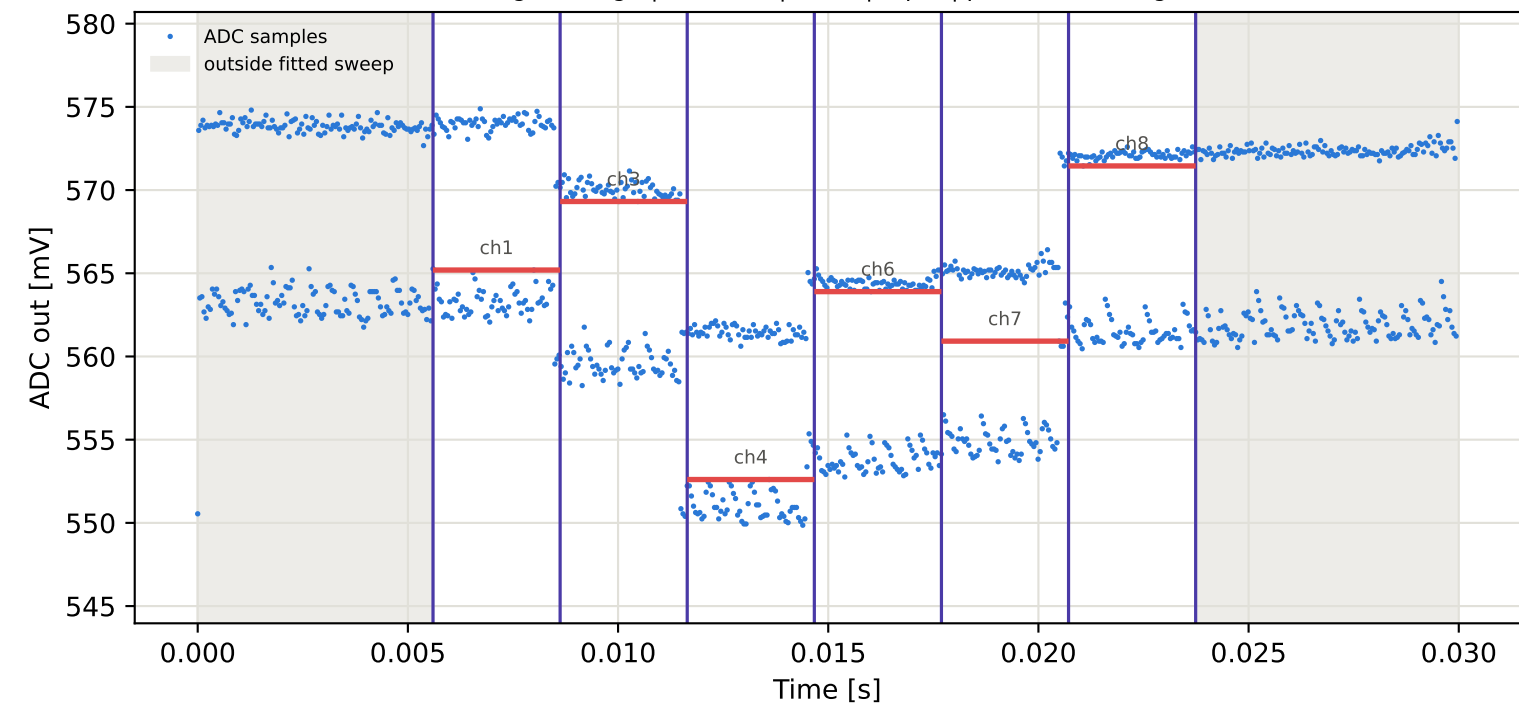
Tag5 &lt;- Tag9 | 935 MHz | run 0 | rep 1 | phase -67.31 deg
