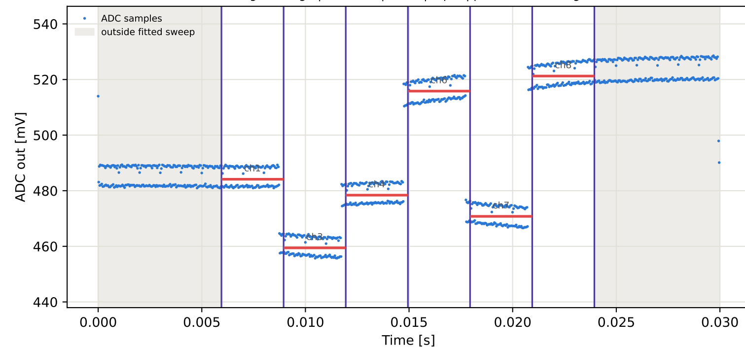
Tag3 &lt;- Tag8 | 865 MHz | run 0 | rep 1 | phase 177.33 deg
