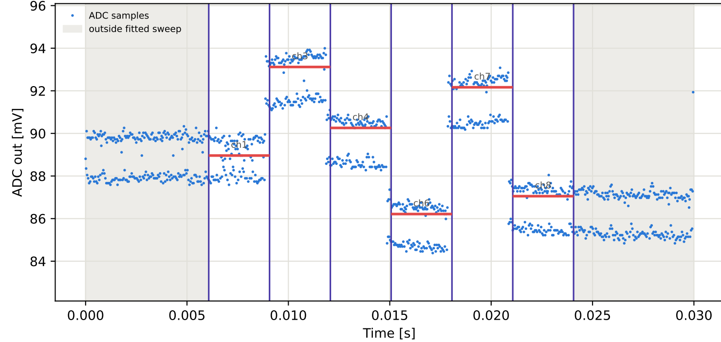
Tag9 &lt;- Tag8 | 795 MHz | run 0 | rep 1 | phase 81.55 deg
