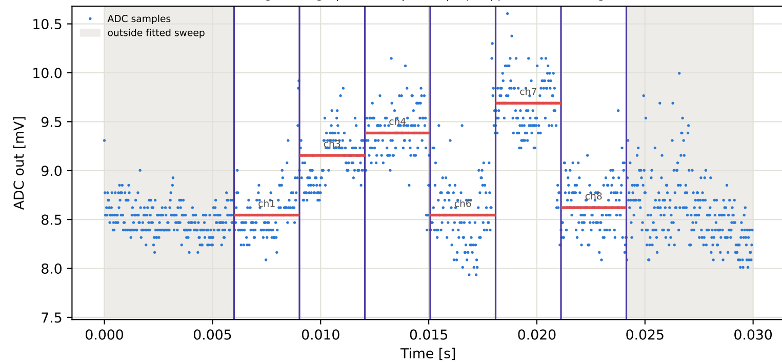
Tag3 &lt;- Tag15 | 775 MHz | run 0 | rep 1 | phase -96.89 deg
