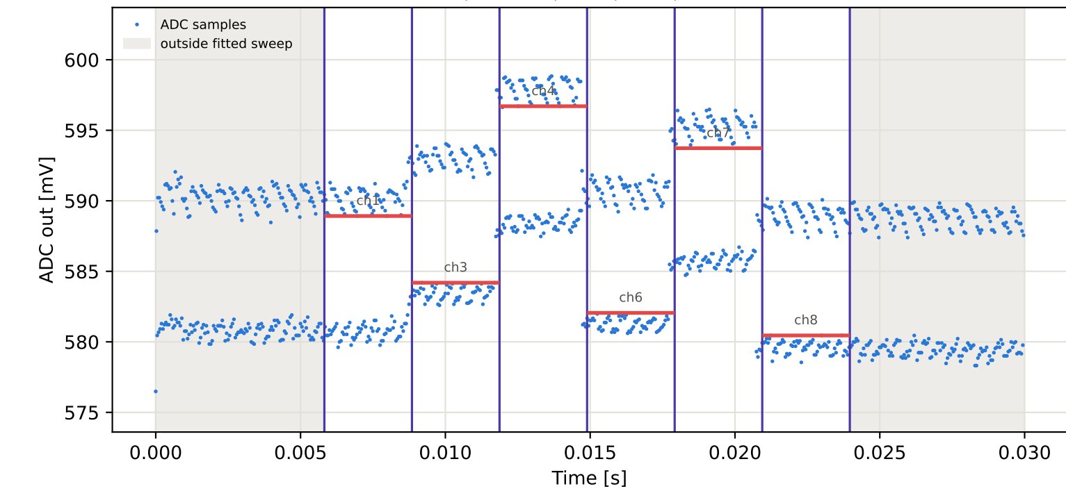
Tag8 &lt;- Tag6 | 965 MHz | run 0 | rep 1 | phase -74.44 deg
