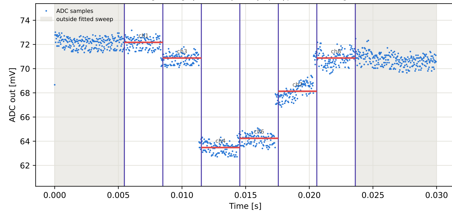
Tag3 &lt;- Tag6 | 965 MHz | run 0 | rep 1 | phase 47.89 deg
