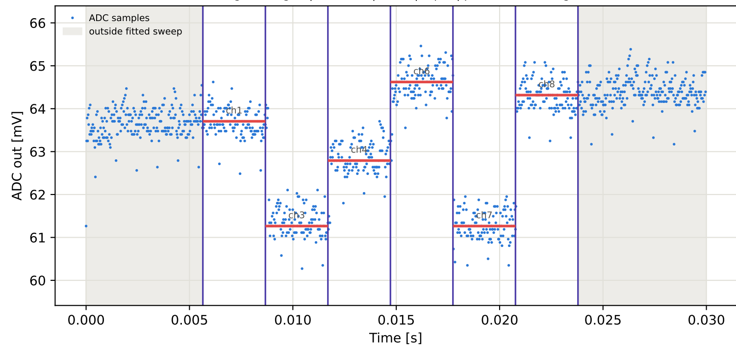
Tag4 &lt;- Tag16 | 785 MHz | run 0 | rep 1 | phase 108.03 deg
