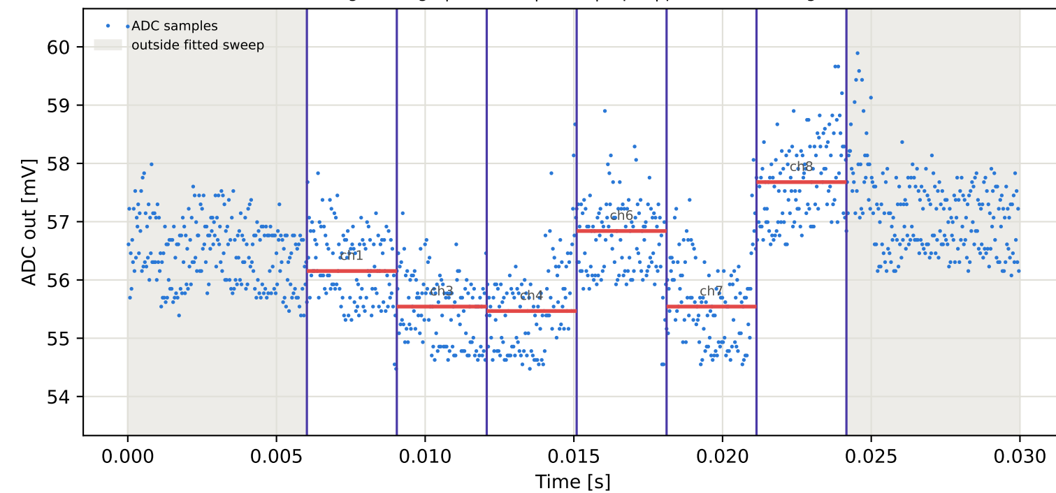
Tag6 &lt;- Tag4 | 775 MHz | run 0 | rep 1 | phase 118.28 deg
