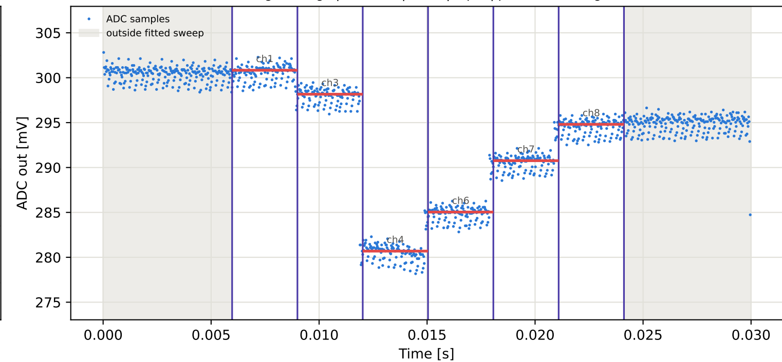
Tag3 &lt;- Tag9 | 985 MHz | run 0 | rep 1 | phase 116.73 deg
