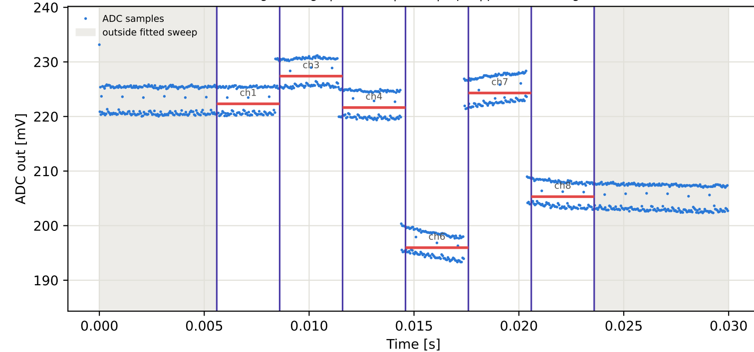
Tag1 &lt;- Tag9 | 915 MHz | run 0 | rep 1 | phase 2.10 deg
