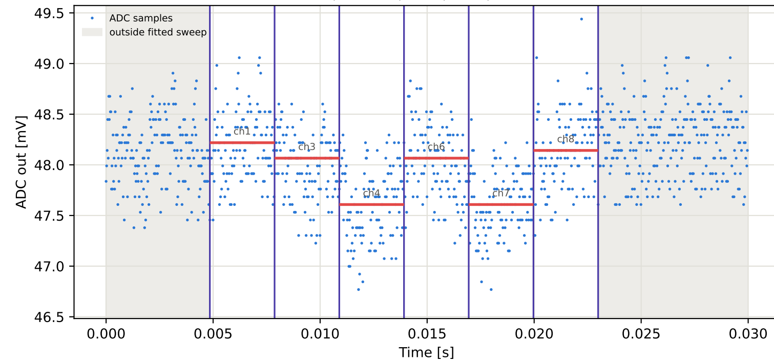
Tag1 &lt;- Tag3 | 775 MHz | run 0 | rep 1 | phase 105.80 deg
