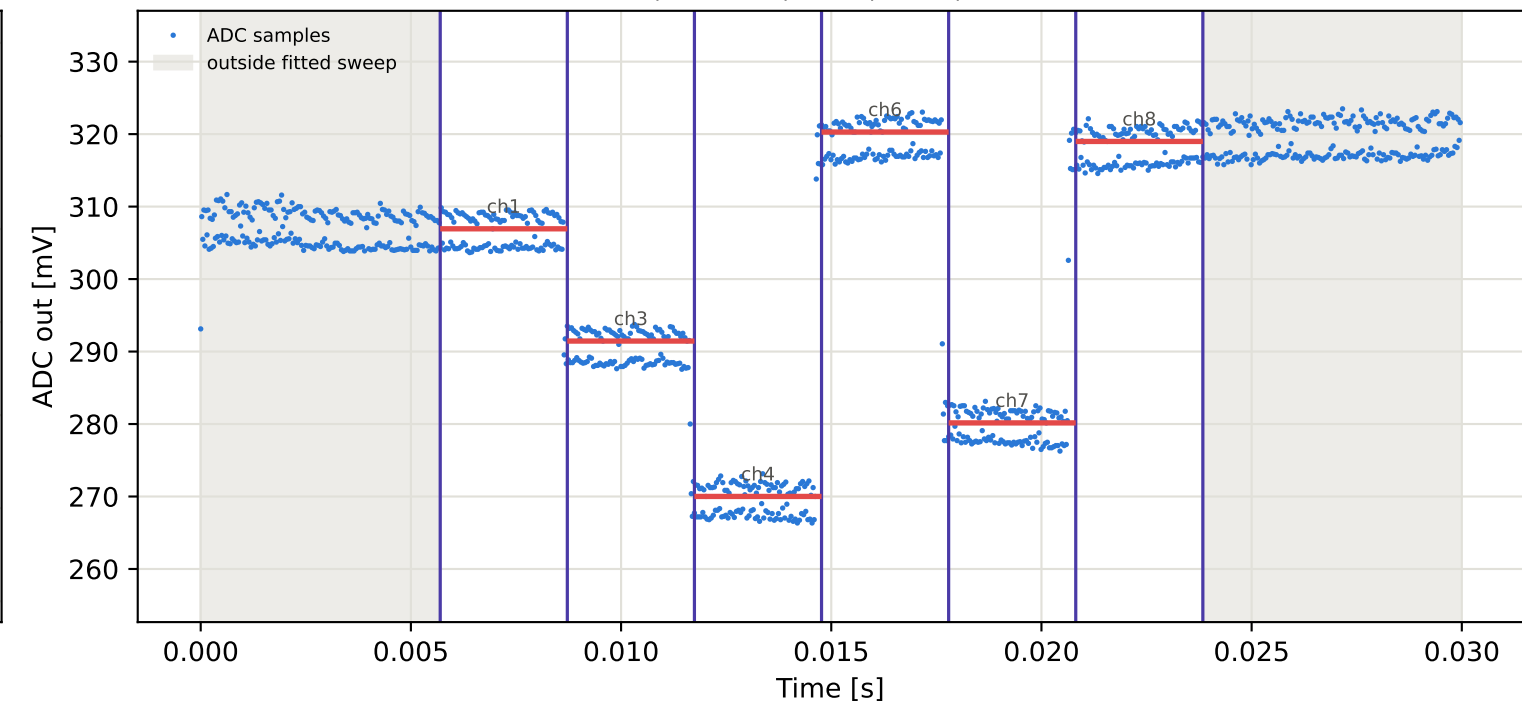
Tag6 &lt;- Tag10 | 985 MHz | run 0 | rep 1 | phase 117.62 deg
