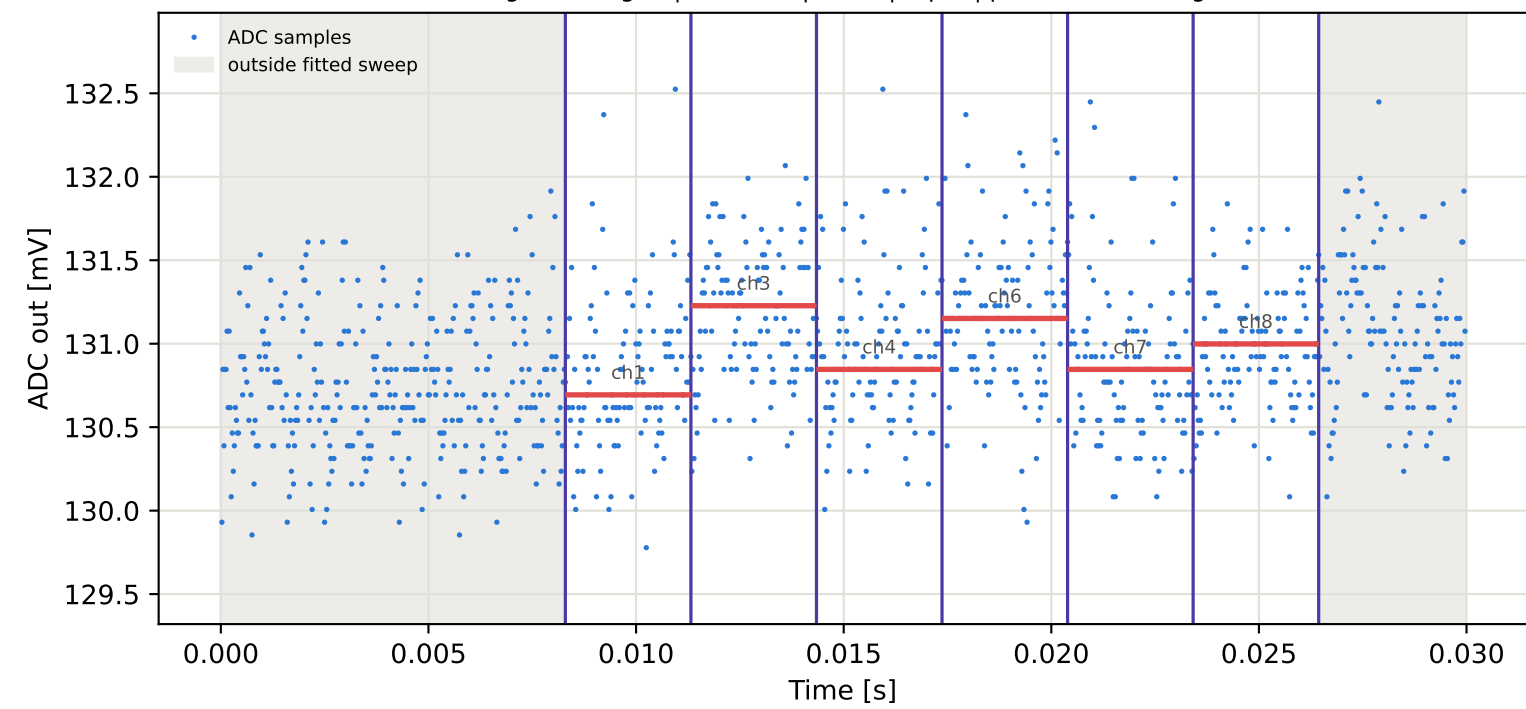
Tag15 &lt;- Tag10 | 795 MHz | run 0 | rep 1 | phase 172.80 deg
