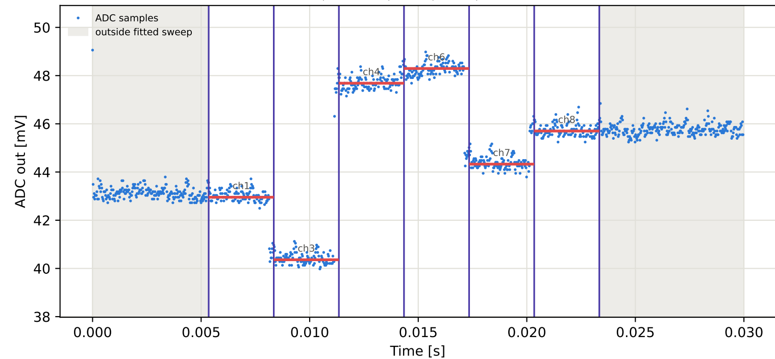
Tag3 &lt;- Tag9 | 785 MHz | run 0 | rep 1 | phase -131.85 deg
