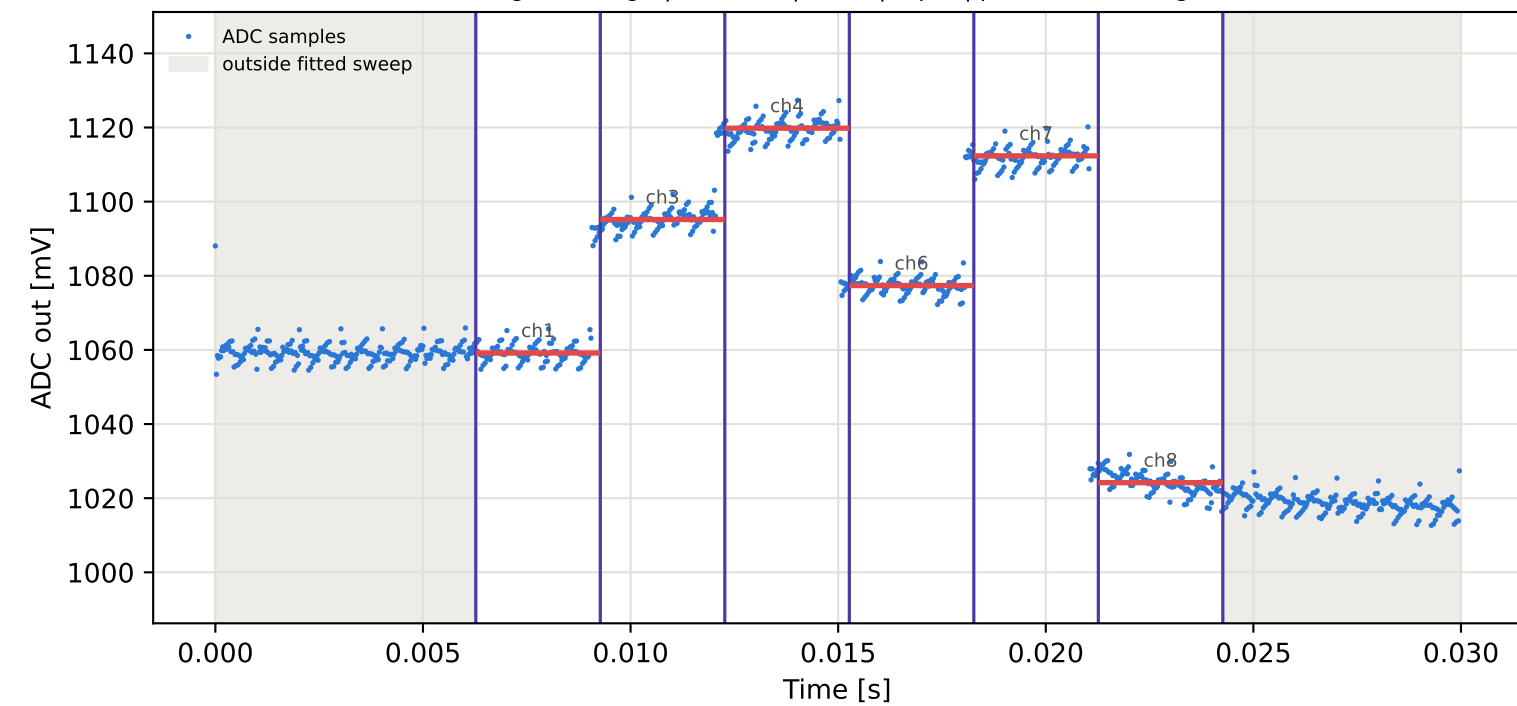
Tag2 &lt;- Tag1 | 905 MHz | run 0 | rep 1 | phase 14.82 deg
