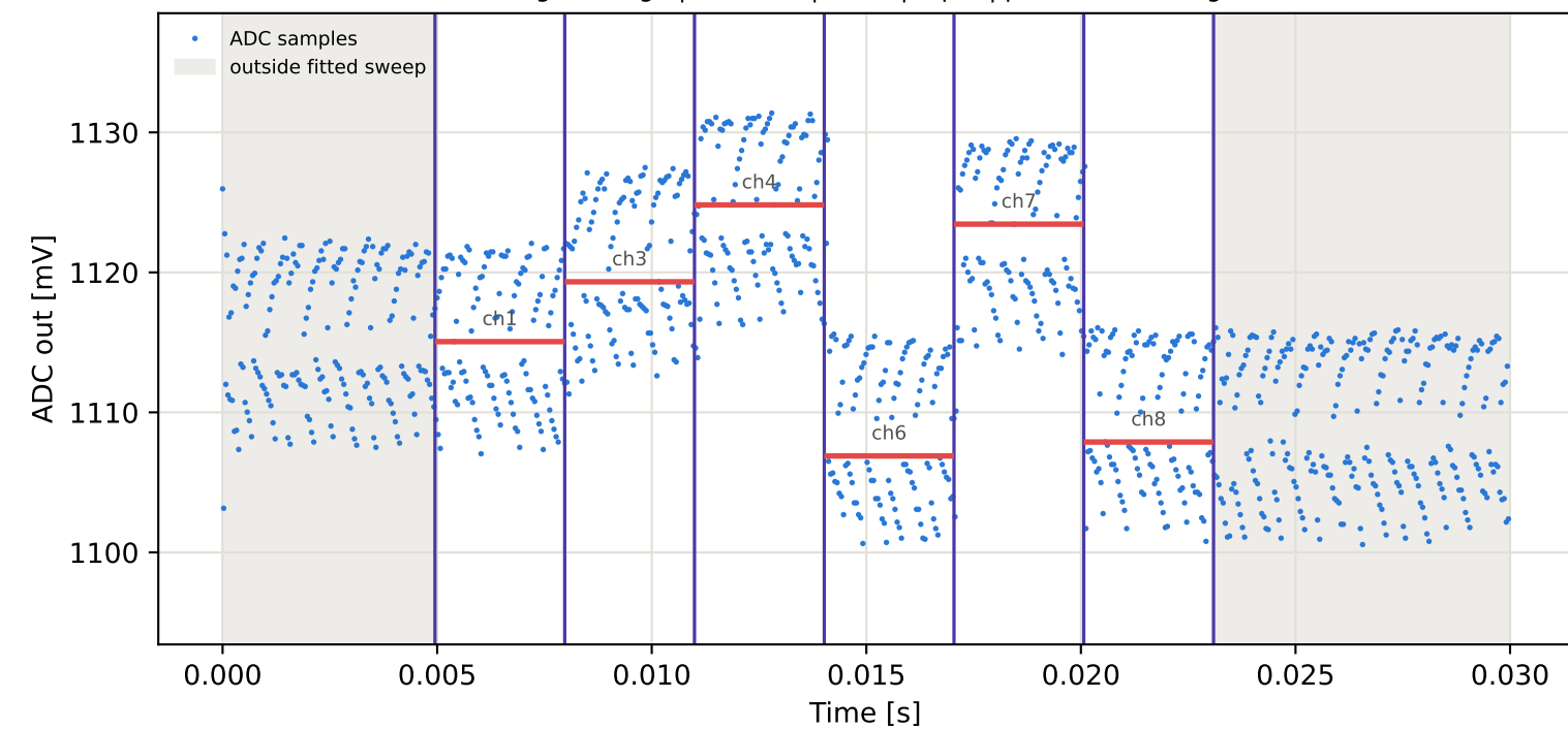
Tag7 &lt;- Tag5 | 935 MHz | run 0 | rep 1 | phase -44.17 deg
