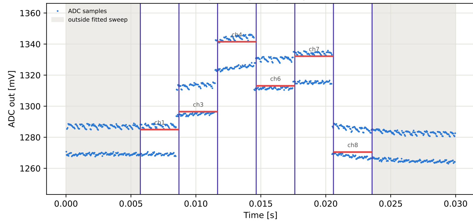
Tag16 &lt;- Tag15 | 915 MHz | run 0 | rep 1 | phase -98.81 deg
