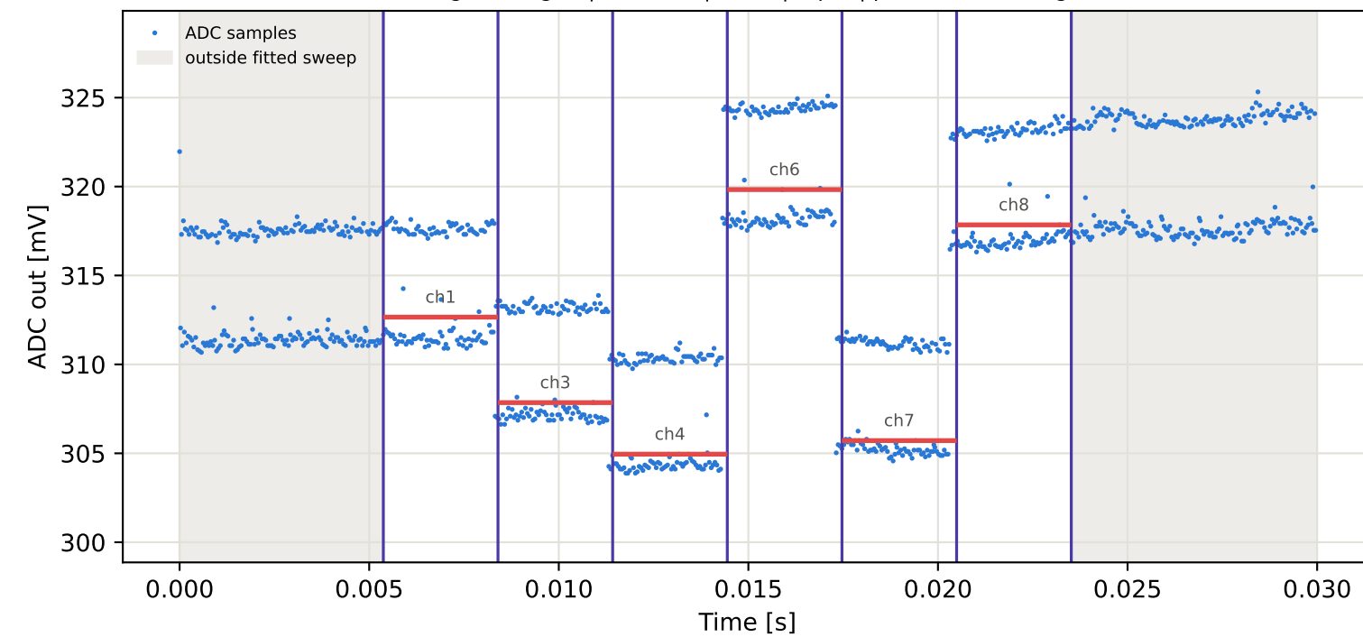
Tag6 &lt;- Tag2 | 955 MHz | run 0 | rep 1 | phase -20.65 deg
