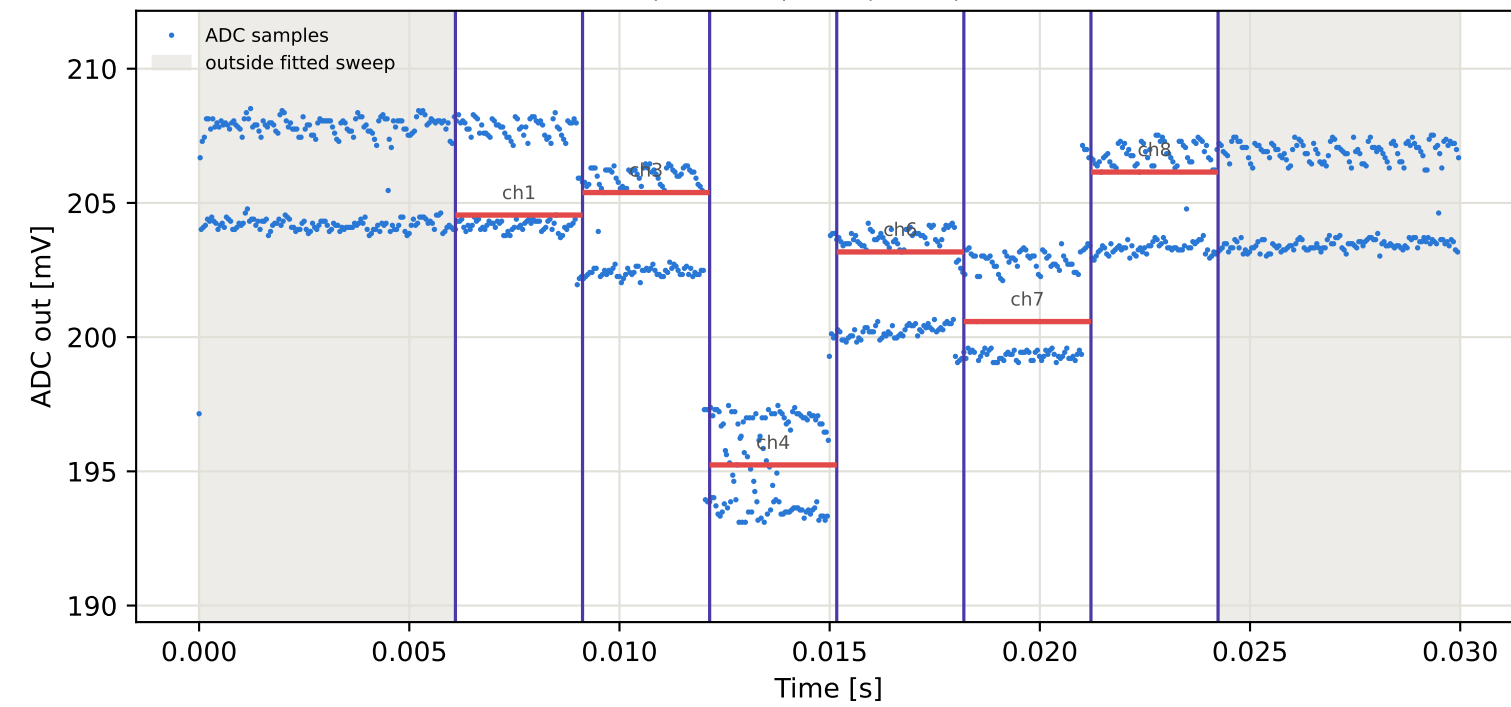
Tag7 &lt;- Tag5 | 995 MHz | run 0 | rep 1 | phase 68.35 deg
