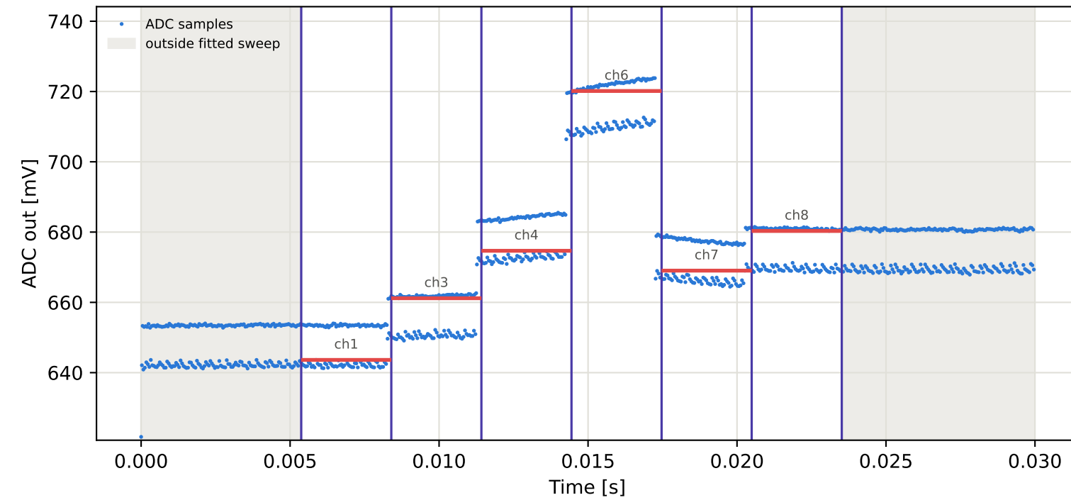
Tag3 &lt;- Tag8 | 895 MHz | run 0 | rep 1 | phase -164.64 deg
