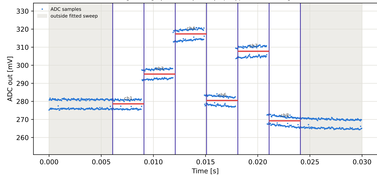
Tag6 &lt;- Tag5 | 945 MHz | run 0 | rep 1 | phase 6.39 deg
