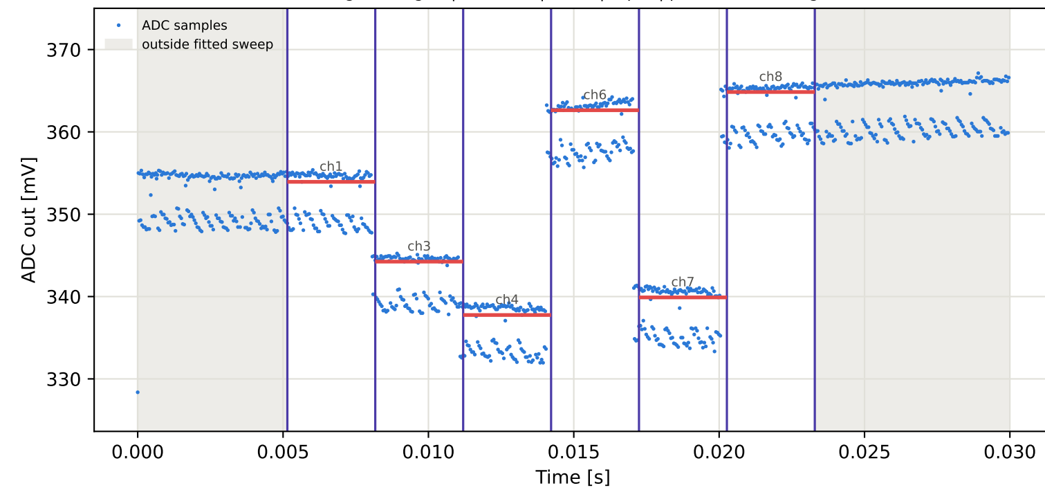
Tag6 &lt;- Tag2 | 935 MHz | run 0 | rep 1 | phase -45.20 deg
