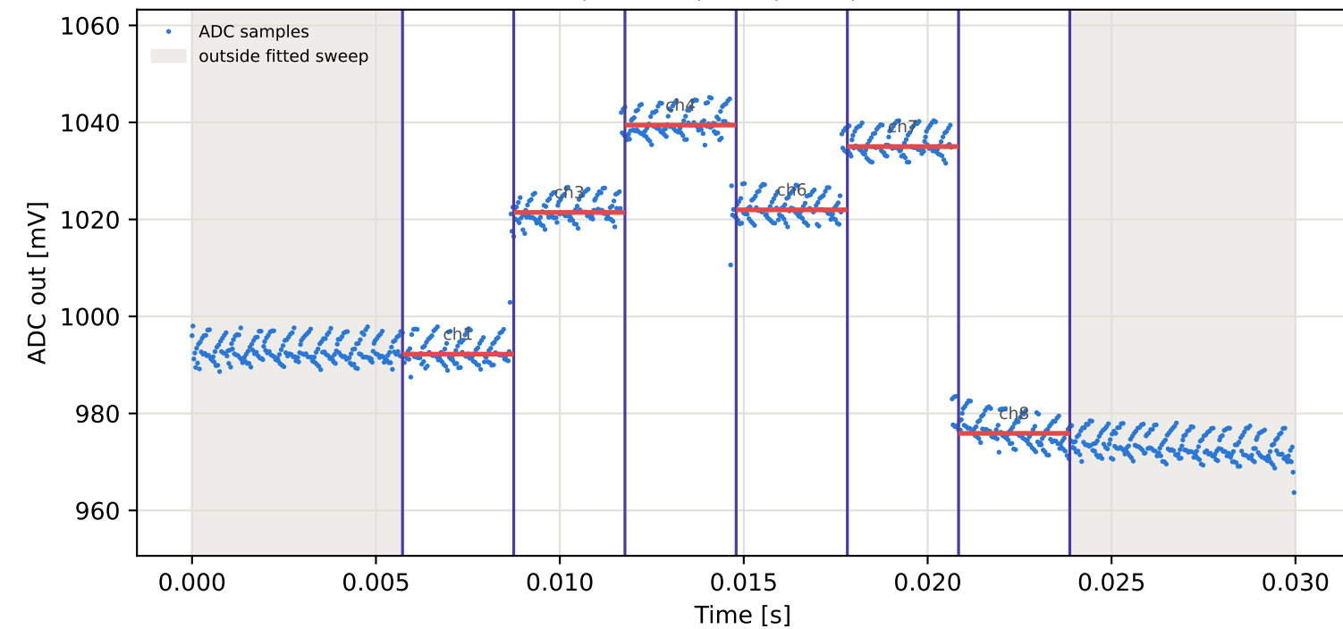
Tag7 &lt;- Tag5 | 895 MHz | run 0 | rep 1 | phase -90.76 deg
