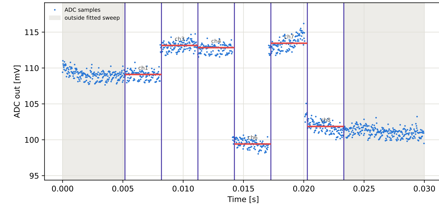
Tag2 &lt;- Tag15 | 915 MHz | run 0 | rep 1 | phase 97.65 deg
