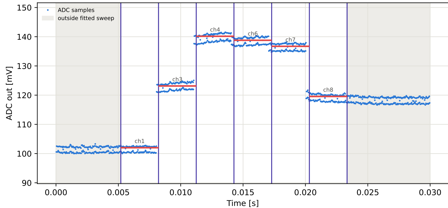
Tag15 &lt;- Tag10 | 865 MHz | run 0 | rep 1 | phase 7.51 deg
