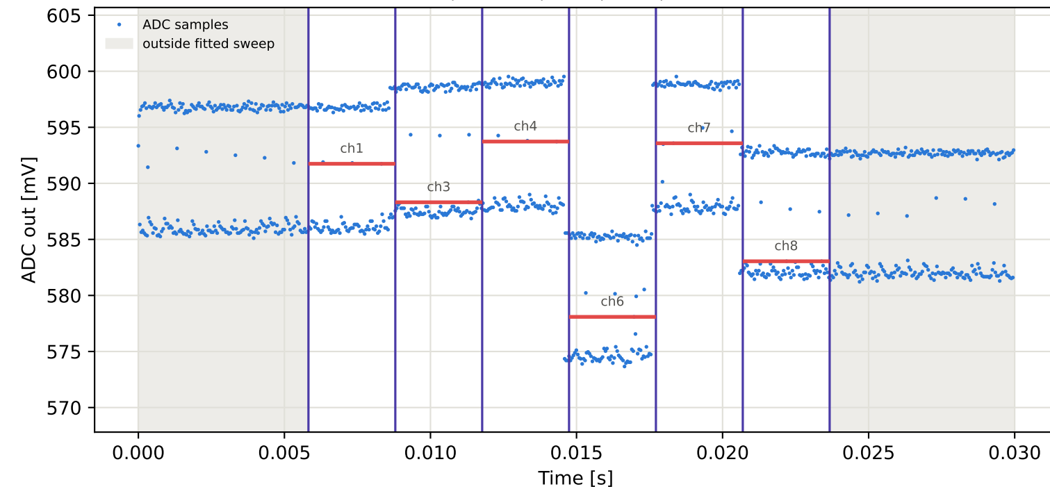
Tag4 &lt;- Tag2 | 975 MHz | run 0 | rep 1 | phase -24.08 deg
