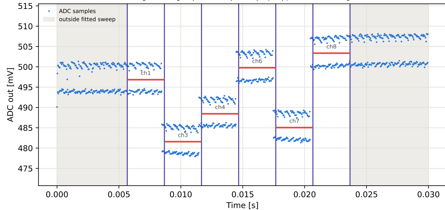
Tag16 &lt;- Tag15 | 855 MHz | run 0 | rep 1 | phase 162.57 deg
