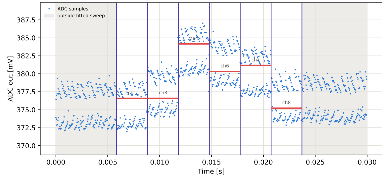
Tag5 &lt;- Tag3 | 965 MHz | run 0 | rep 1 | phase -115.26 deg
