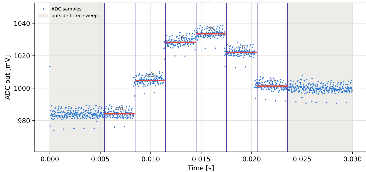
Tag3 &lt;- Tag15 | 885 MHz | run 0 | rep 1 | phase -8.28 deg
