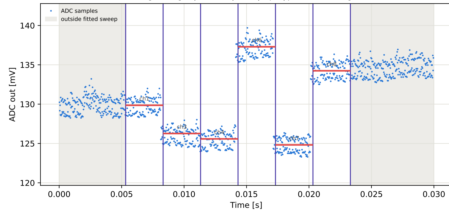
Tag6 &lt;- Tag2 | 975 MHz | run 0 | rep 1 | phase -32.58 deg
