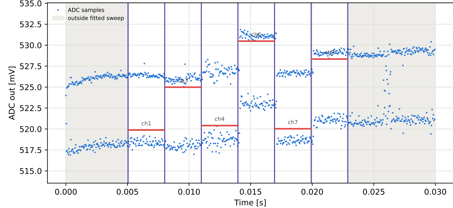
Tag1 &lt;- Tag4 | 875 MHz | run 0 | rep 1 | phase -89.16 deg
