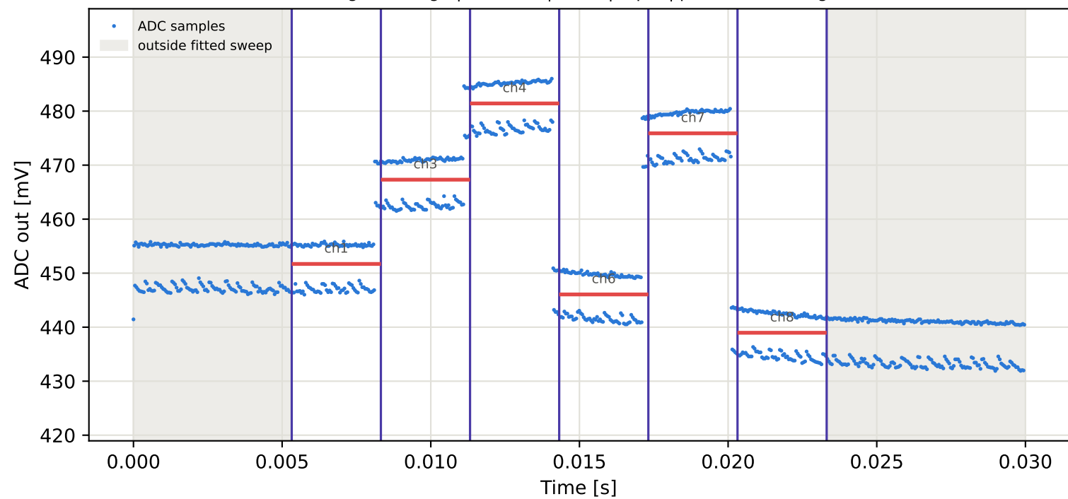
Tag15 &lt;- Tag10 | 945 MHz | run 0 | rep 1 | phase 93.50 deg
