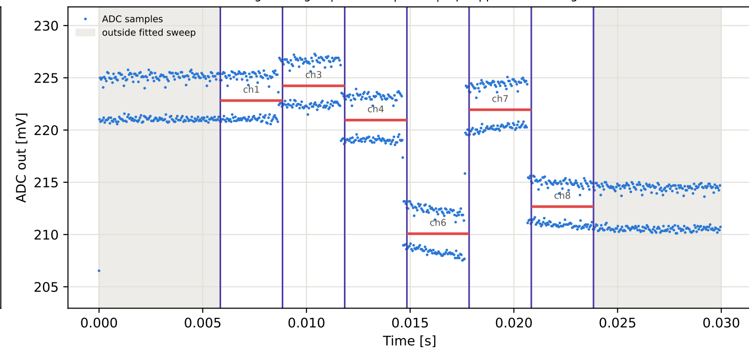
Tag1 &lt;- Tag2 | 895 MHz | run 0 | rep 1 | phase 51.20 deg
