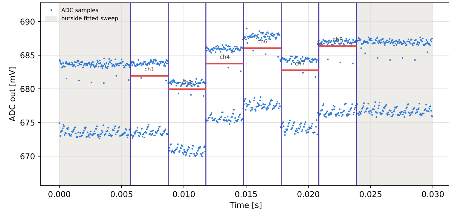
Tag8 &lt;- Tag15 | 845 MHz | run 0 | rep 1 | phase -22.60 deg
