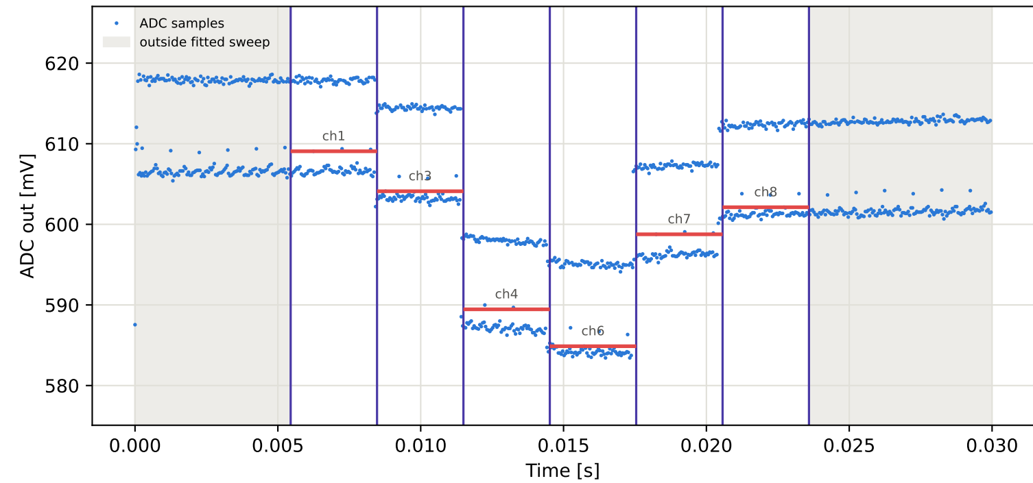
Tag15 &lt;- Tag6 | 955 MHz | run 0 | rep 1 | phase 102.60 deg
