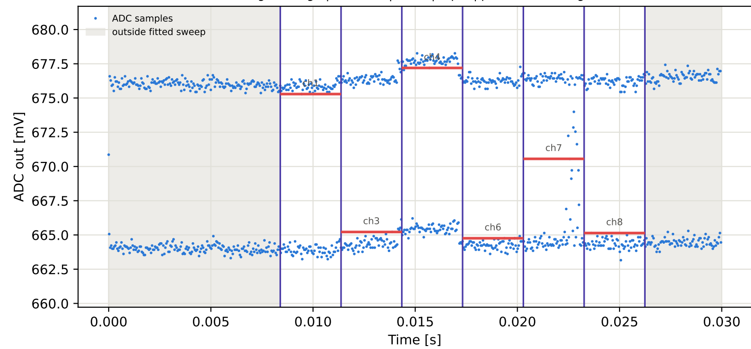
Tag3 &lt;- Tag2 | 895 MHz | run 0 | rep 1 | phase -62.80 deg
