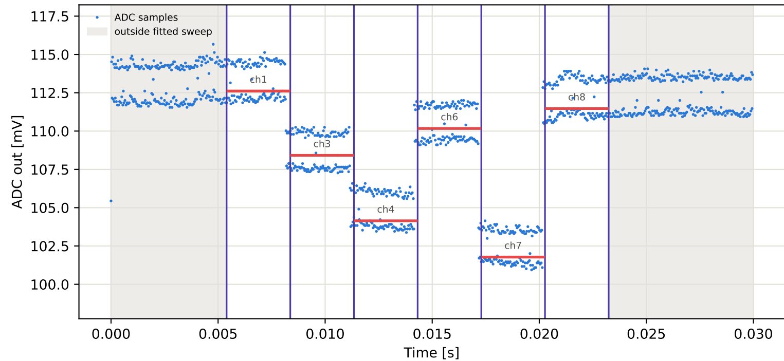
Tag8 &lt;- Tag6 | 795 MHz | run 0 | rep 1 | phase 26.68 deg
