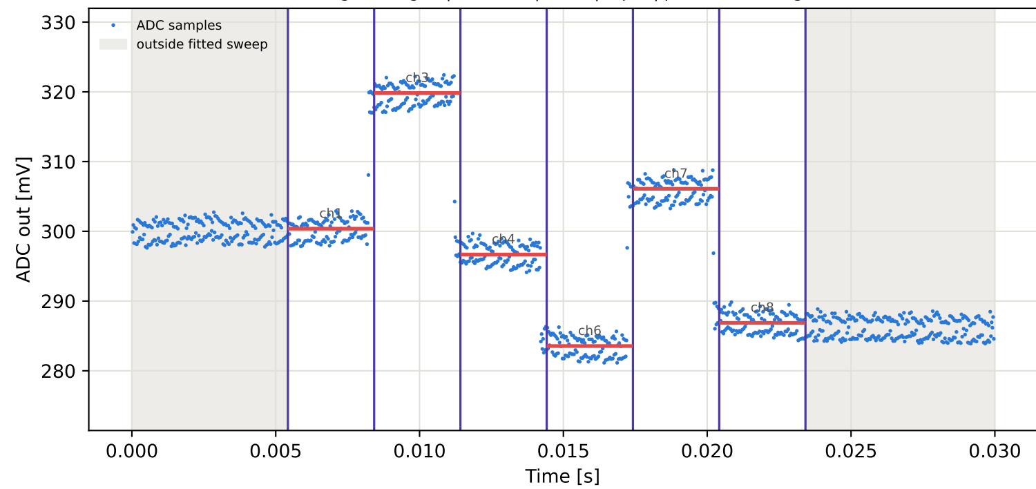
Tag6 &lt;- Tag2 | 835 MHz | run 0 | rep 1 | phase -152.37 deg
