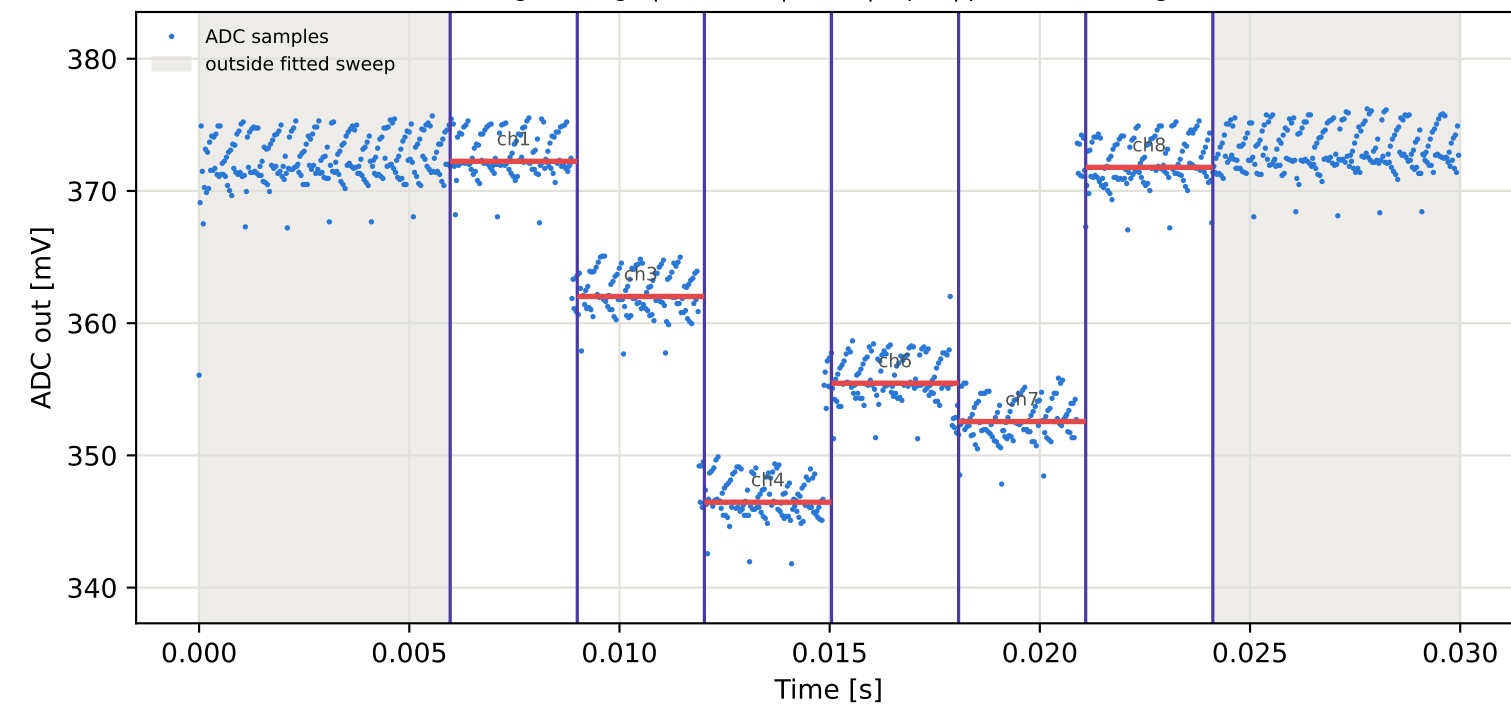
Tag6 &lt;- Tag9 | 915 MHz | run 0 | rep 1 | phase -47.80 deg
