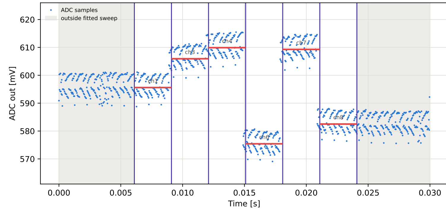
Tag15 &lt;- Tag5 | 955 MHz | run 0 | rep 1 | phase -113.67 deg
