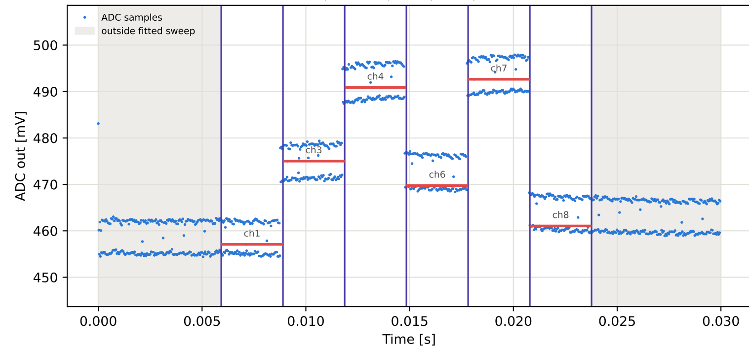
Tag8 &lt;- Tag15 | 825 MHz | run 0 | rep 1 | phase -73.80 deg
