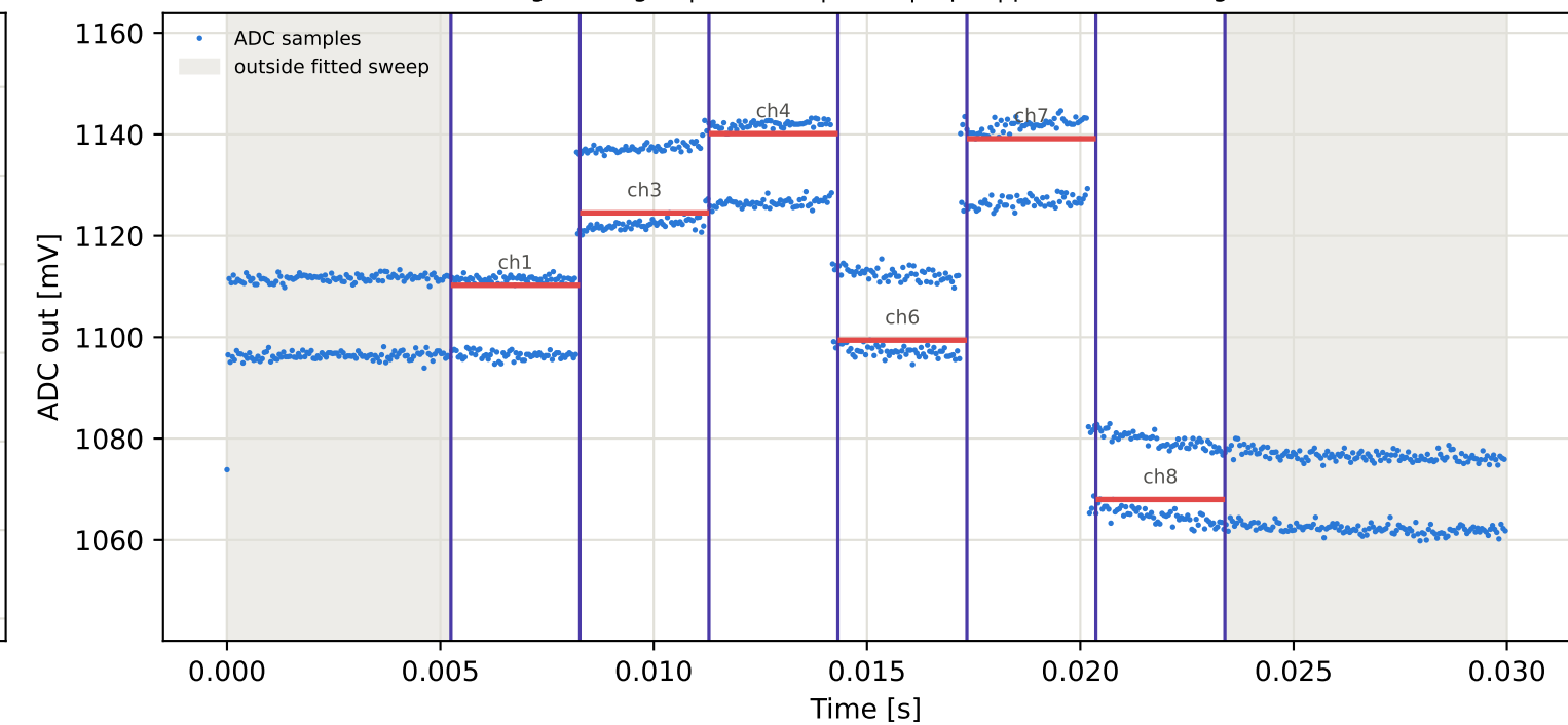
Tag8 &lt;- Tag16 | 885 MHz | run 0 | rep 1 | phase -53.25 deg
