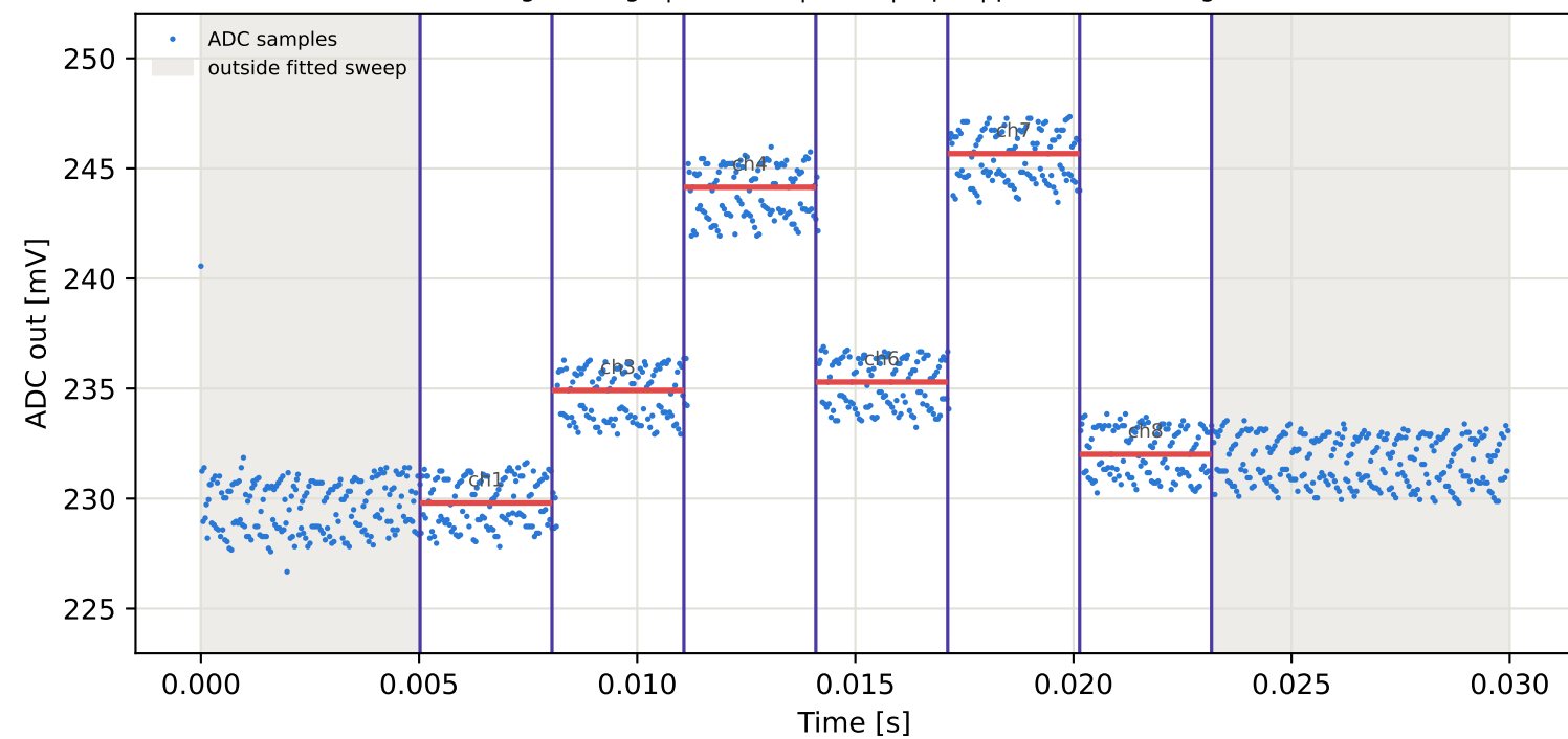
Tag5 &lt;- Tag4 | 795 MHz | run 0 | rep 1 | phase -77.48 deg
