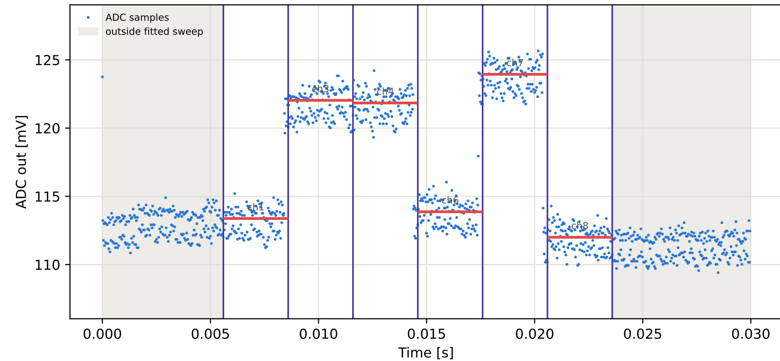
Tag7 &lt;- Tag10 | 825 MHz | run 0 | rep 1 | phase 147.56 deg
