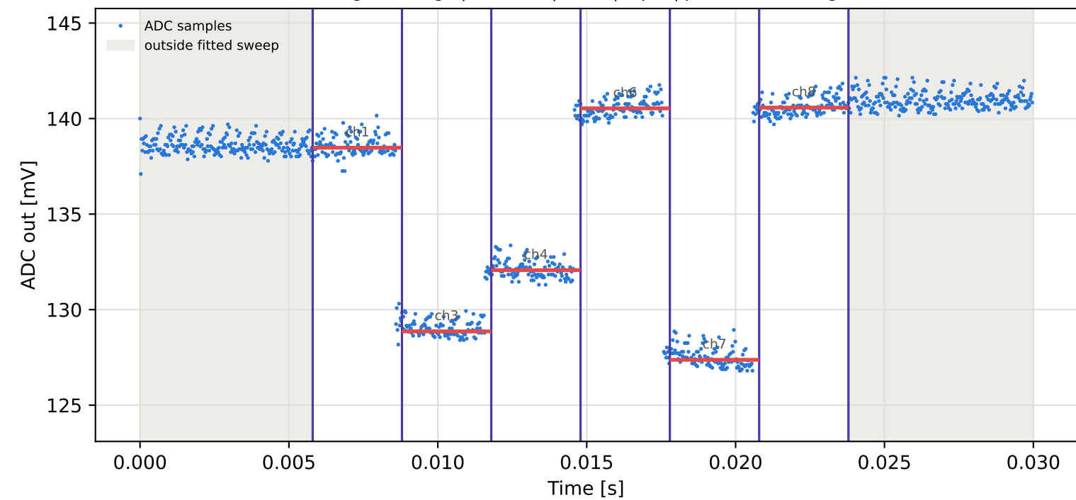
Tag16 &lt;- Tag1 | 795 MHz | run 0 | rep 1 | phase 98.61 deg
