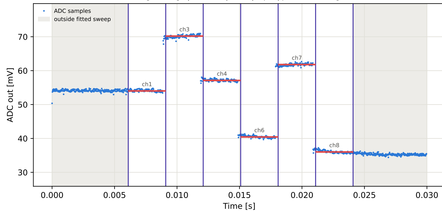
Tag9 &lt;- Tag5 | 845 MHz | run 0 | rep 1 | phase -85.88 deg
