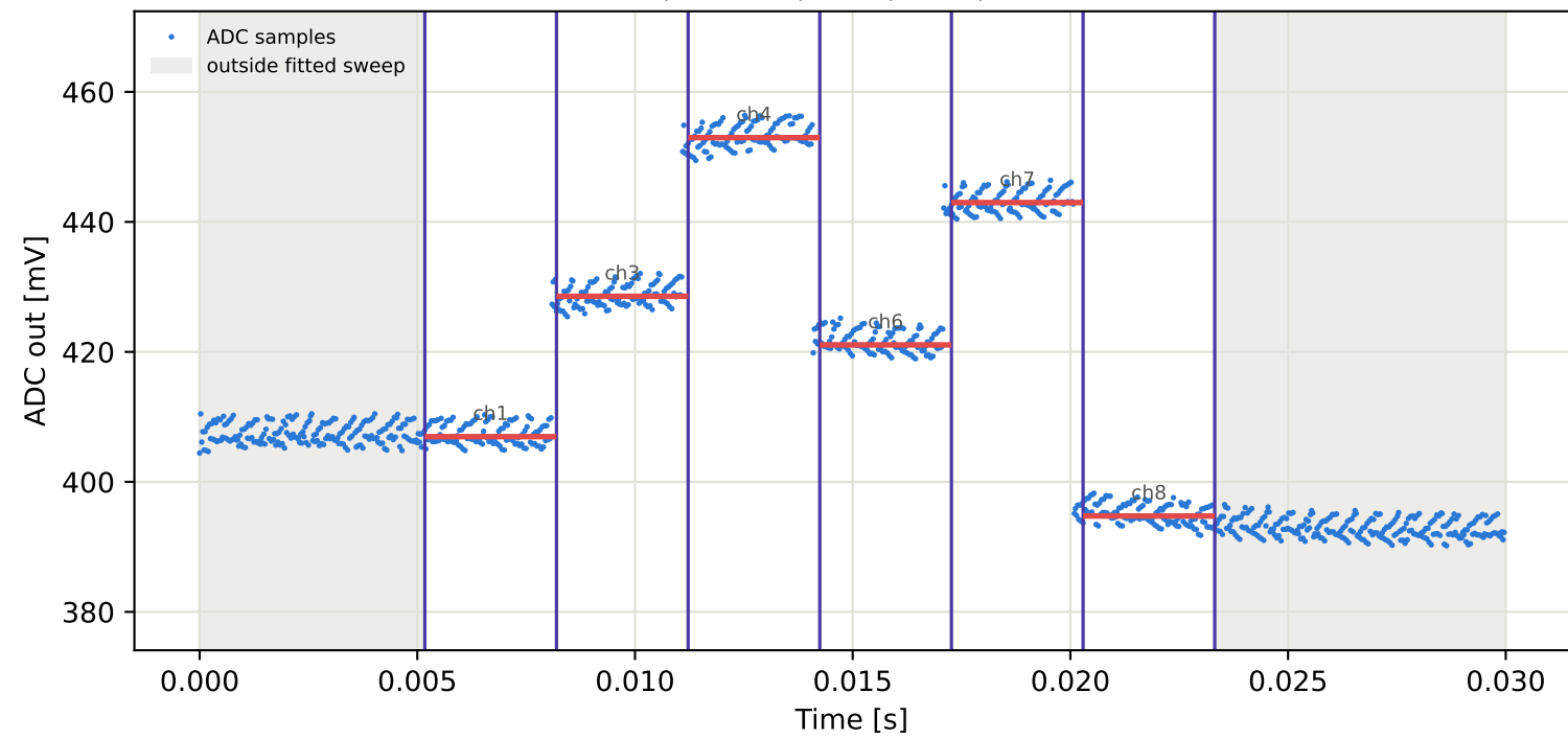
Tag6 &lt;- Tag4 | 925 MHz | run 0 | rep 1 | phase -85.43 deg
