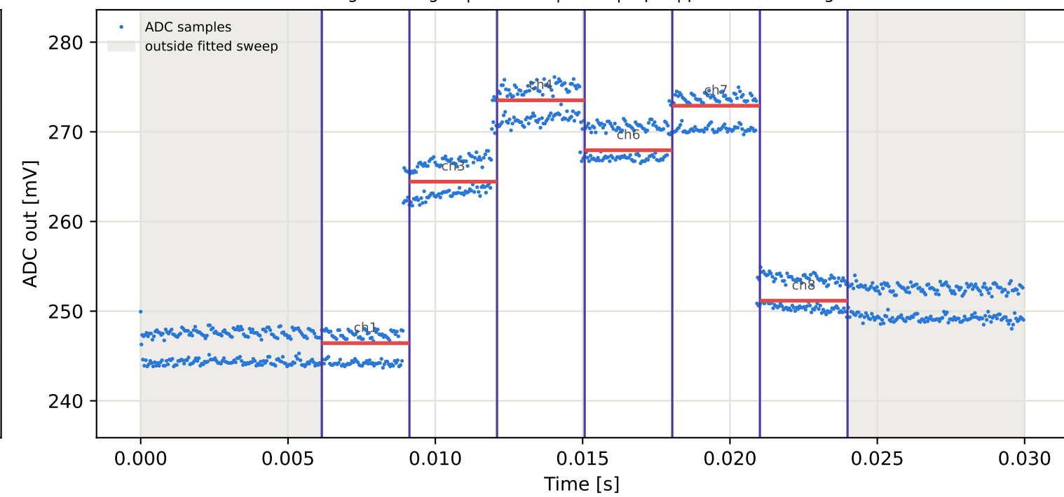
Tag10 &lt;- Tag3 | 875 MHz | run 0 | rep 1 | phase 46.09 deg
