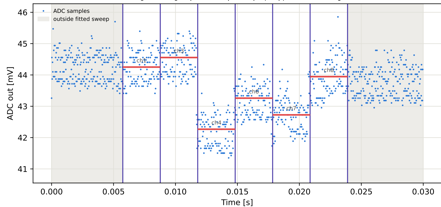
Tag15 &lt;- Tag10 | 775 MHz | run 0 | rep 1 | phase 81.95 deg
