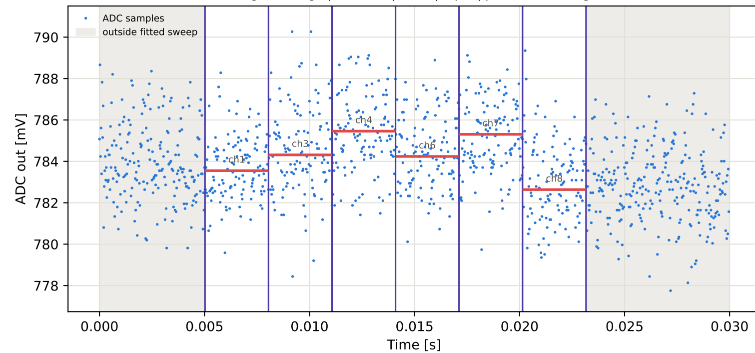
Tag16 &lt;- Tag4 | 885 MHz | run 0 | rep 1 | phase 174.10 deg
