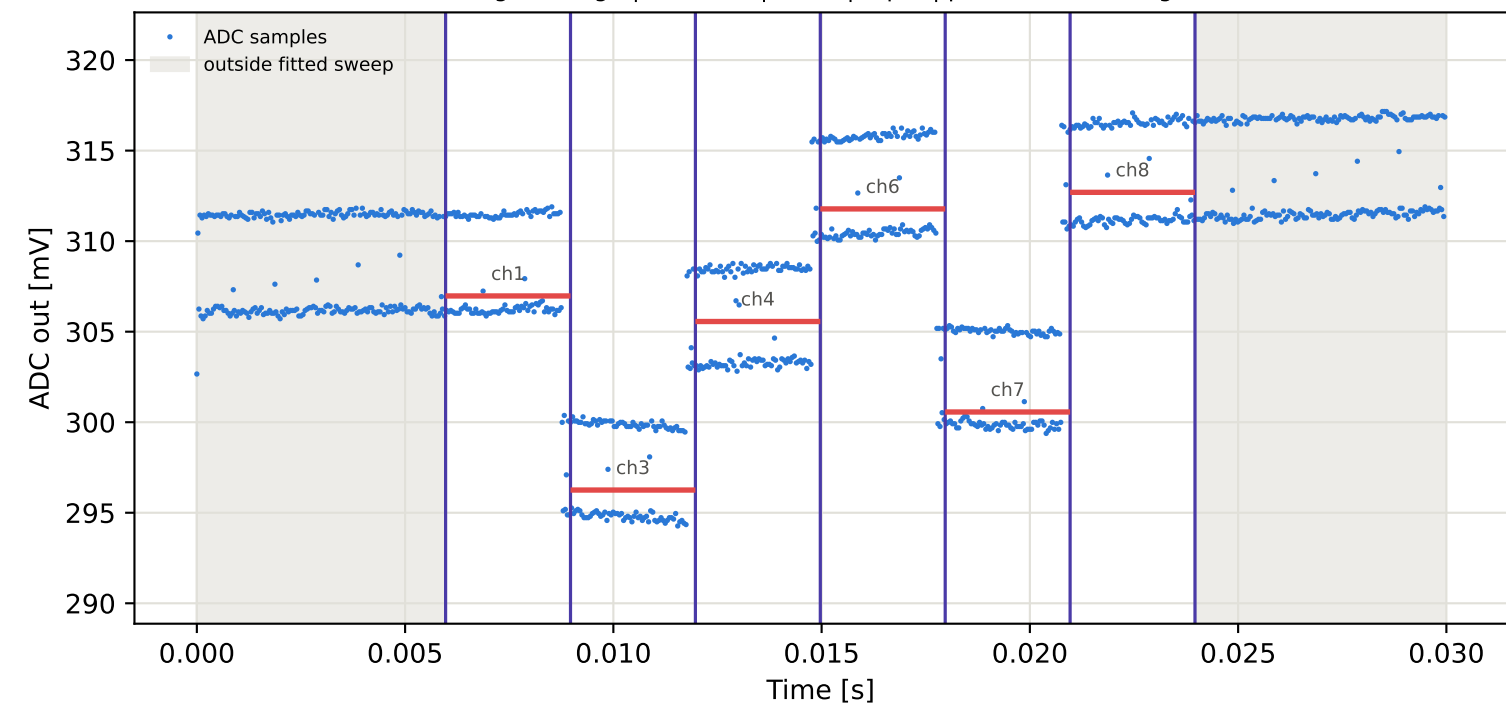
Tag7 &lt;- Tag6 | 825 MHz | run 0 | rep 1 | phase 33.01 deg
