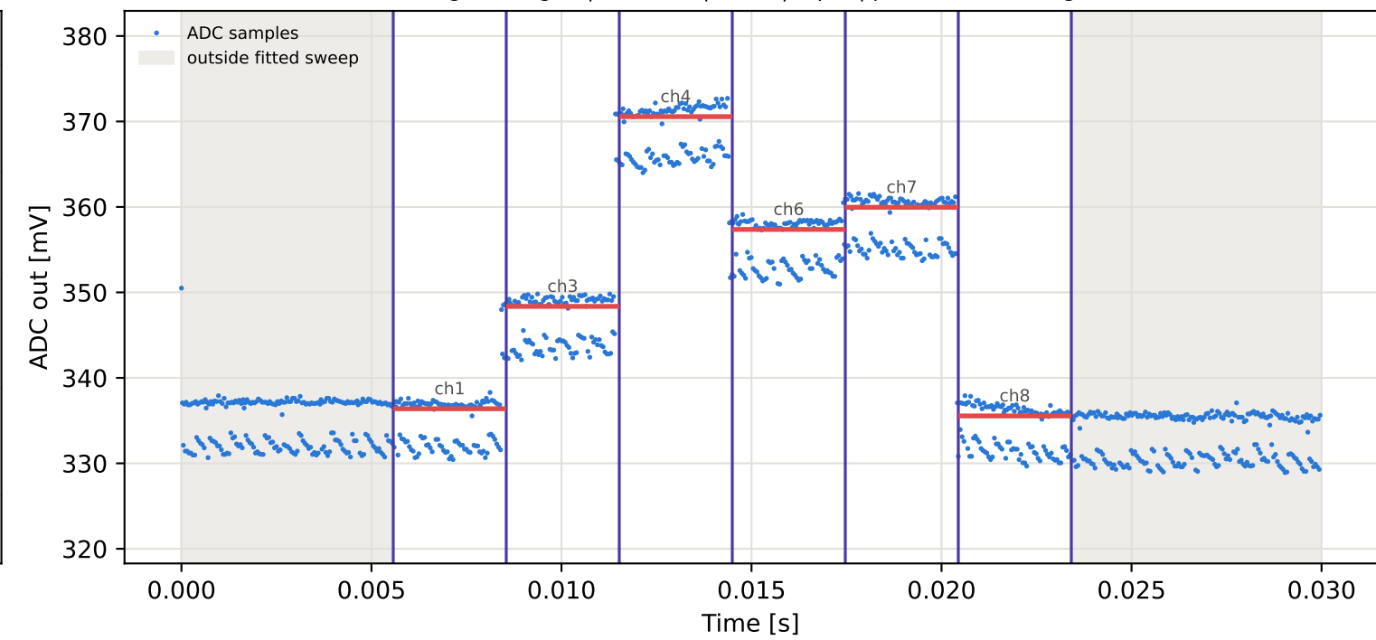
Tag6 &lt;- Tag3 | 935 MHz | run 0 | rep 1 | phase -69.39 deg
