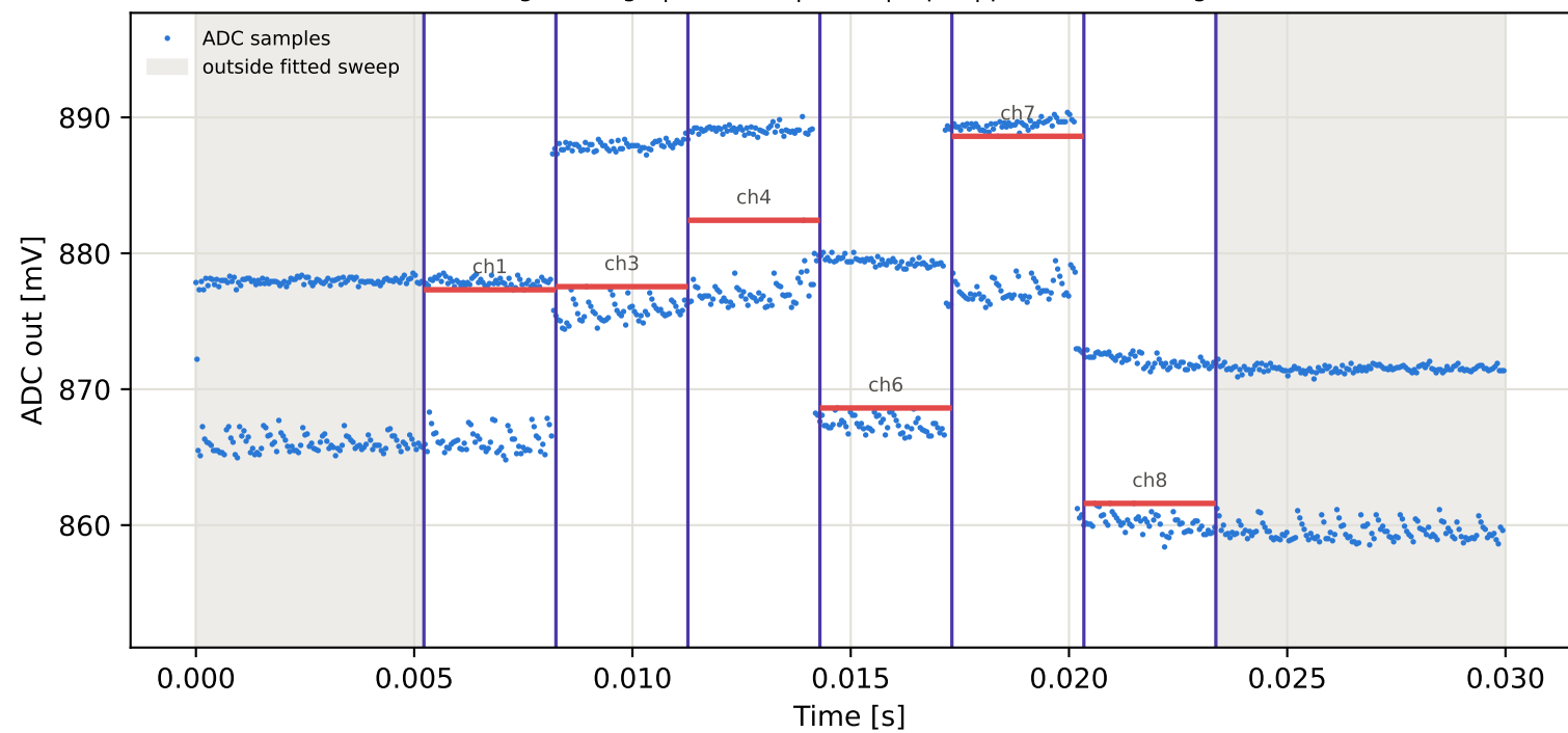
Tag7 &lt;- Tag15 | 875 MHz | run 0 | rep 1 | phase 129.69 deg
