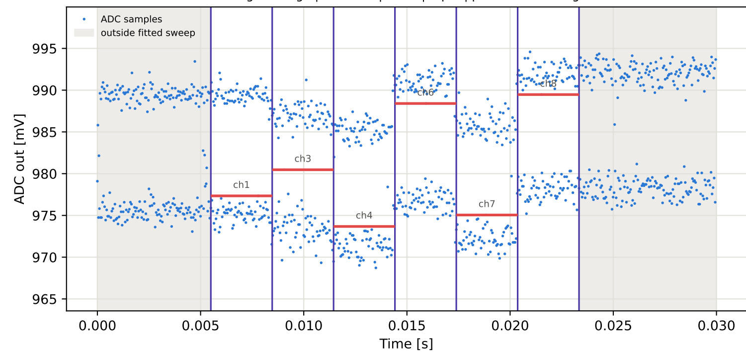
Tag7 &lt;- Tag4 | 885 MHz | run 0 | rep 1 | phase 25.63 deg
