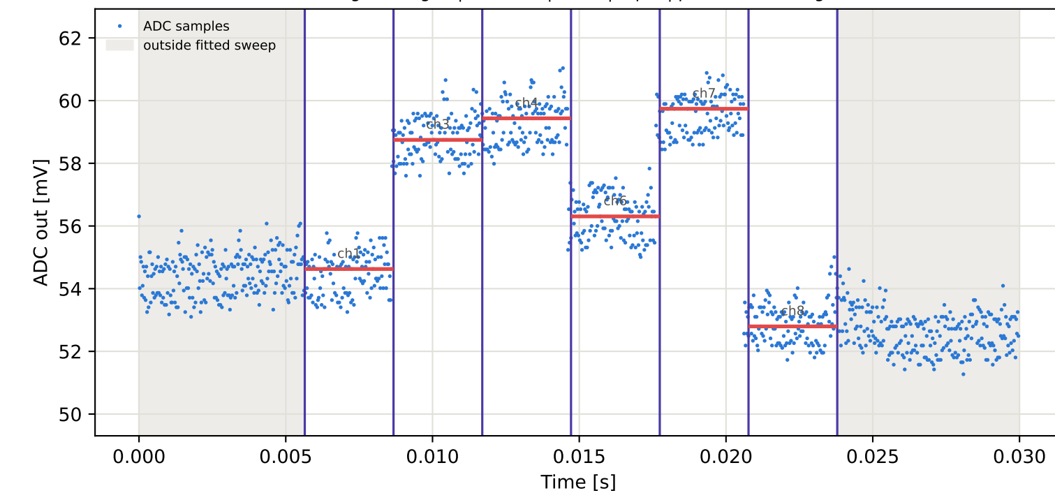
Tag2 &lt;- Tag15 | 875 MHz | run 0 | rep 1 | phase -63.48 deg
