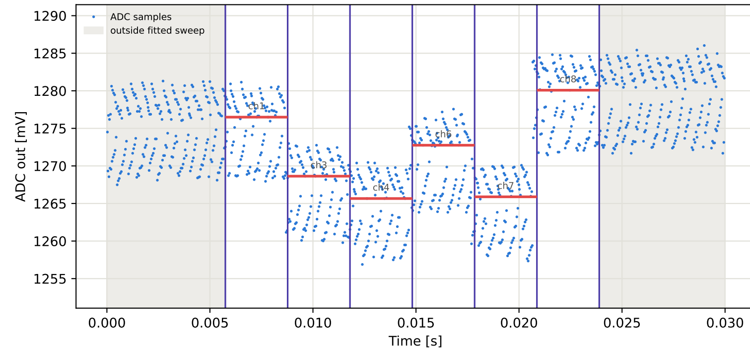
Tag8 &lt;- Tag6 | 875 MHz | run 0 | rep 1 | phase -83.27 deg
