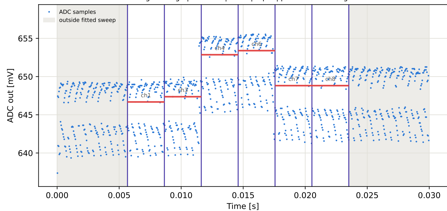
Tag8 &lt;- Tag7 | 985 MHz | run 0 | rep 1 | phase -155.32 deg
