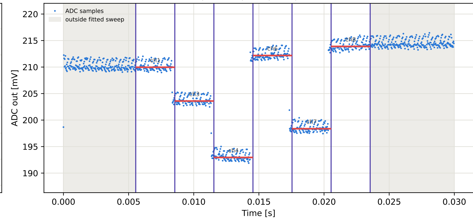
Tag1 &lt;- Tag4 | 965 MHz | run 0 | rep 1 | phase 105.94 deg
