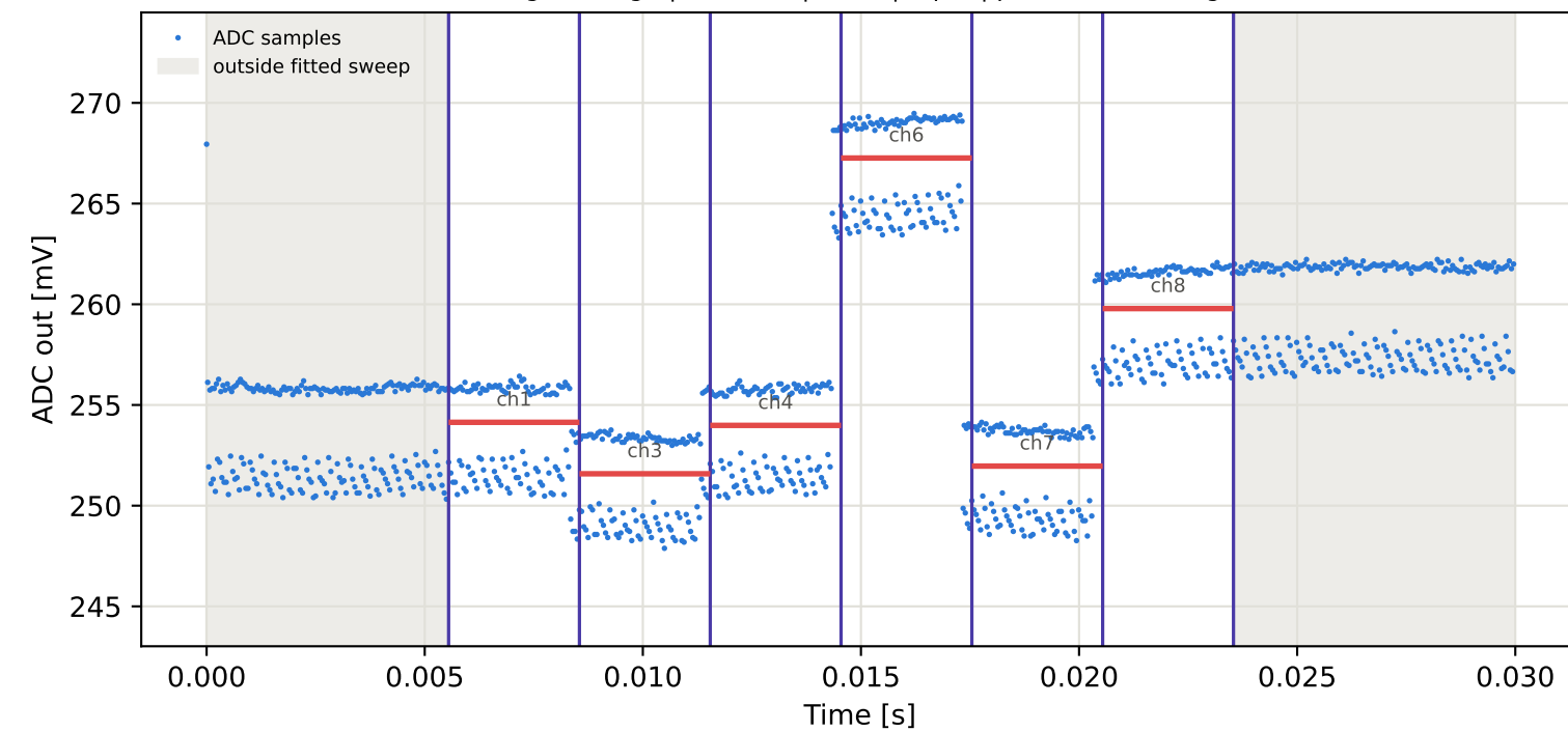
Tag1 &lt;- Tag7 | 955 MHz | run 0 | rep 1 | phase -81.22 deg
