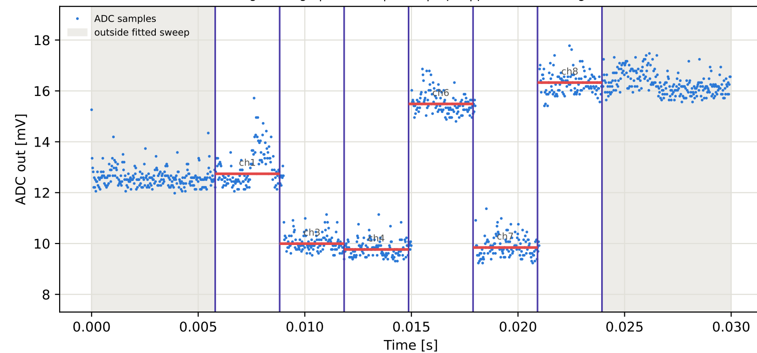
Tag2 &lt;- Tag7 | 895 MHz | run 0 | rep 1 | phase 148.17 deg
