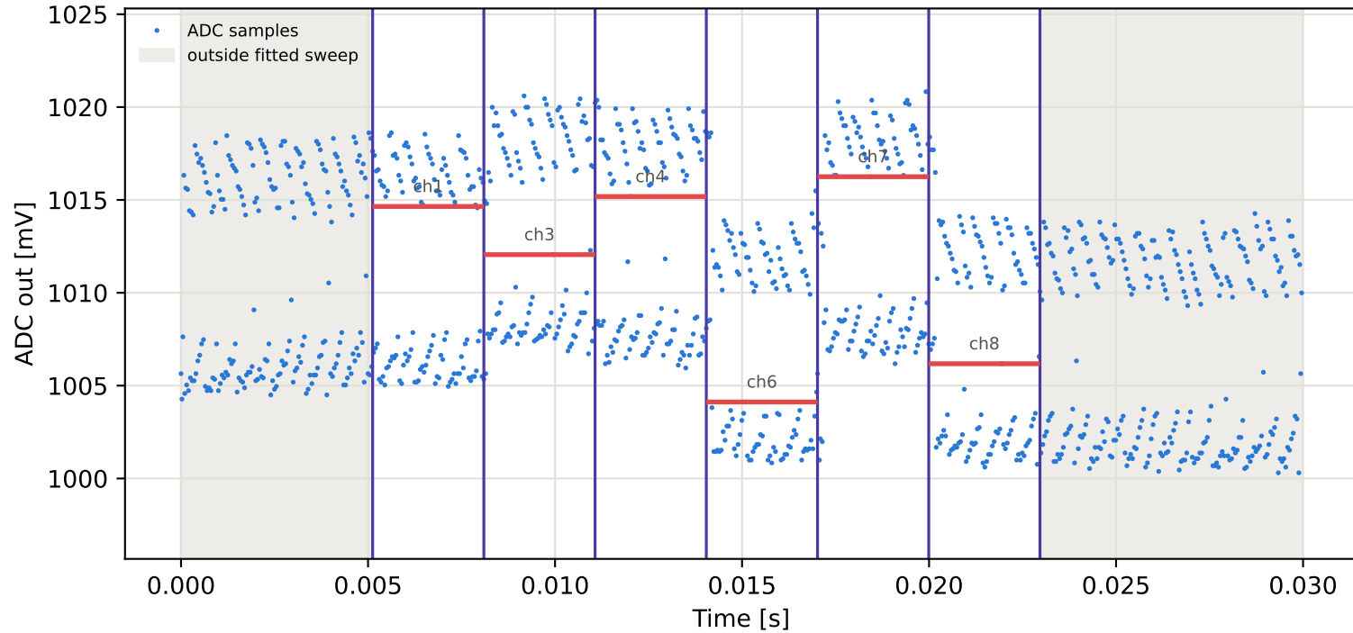
Tag7 &lt;- Tag15 | 895 MHz | run 0 | rep 1 | phase 43.23 deg
