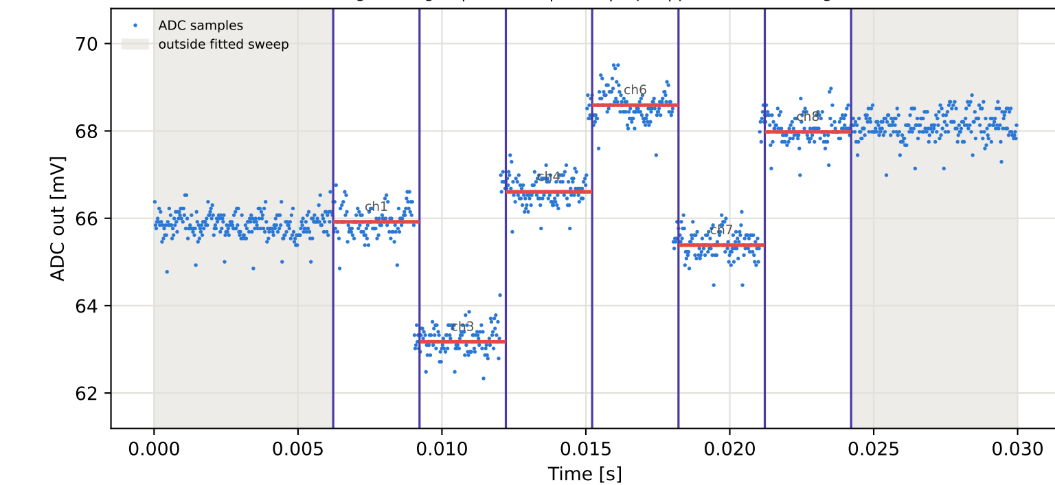
Tag9 &lt;- Tag16 | 825 MHz | run 0 | rep 1 | phase 111.33 deg
