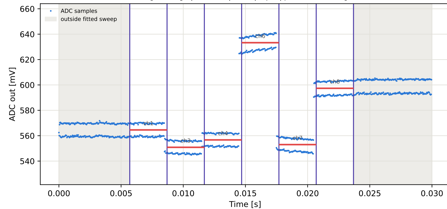
Tag6 &lt;- Tag1 | 935 MHz | run 0 | rep 1 | phase 58.07 deg
