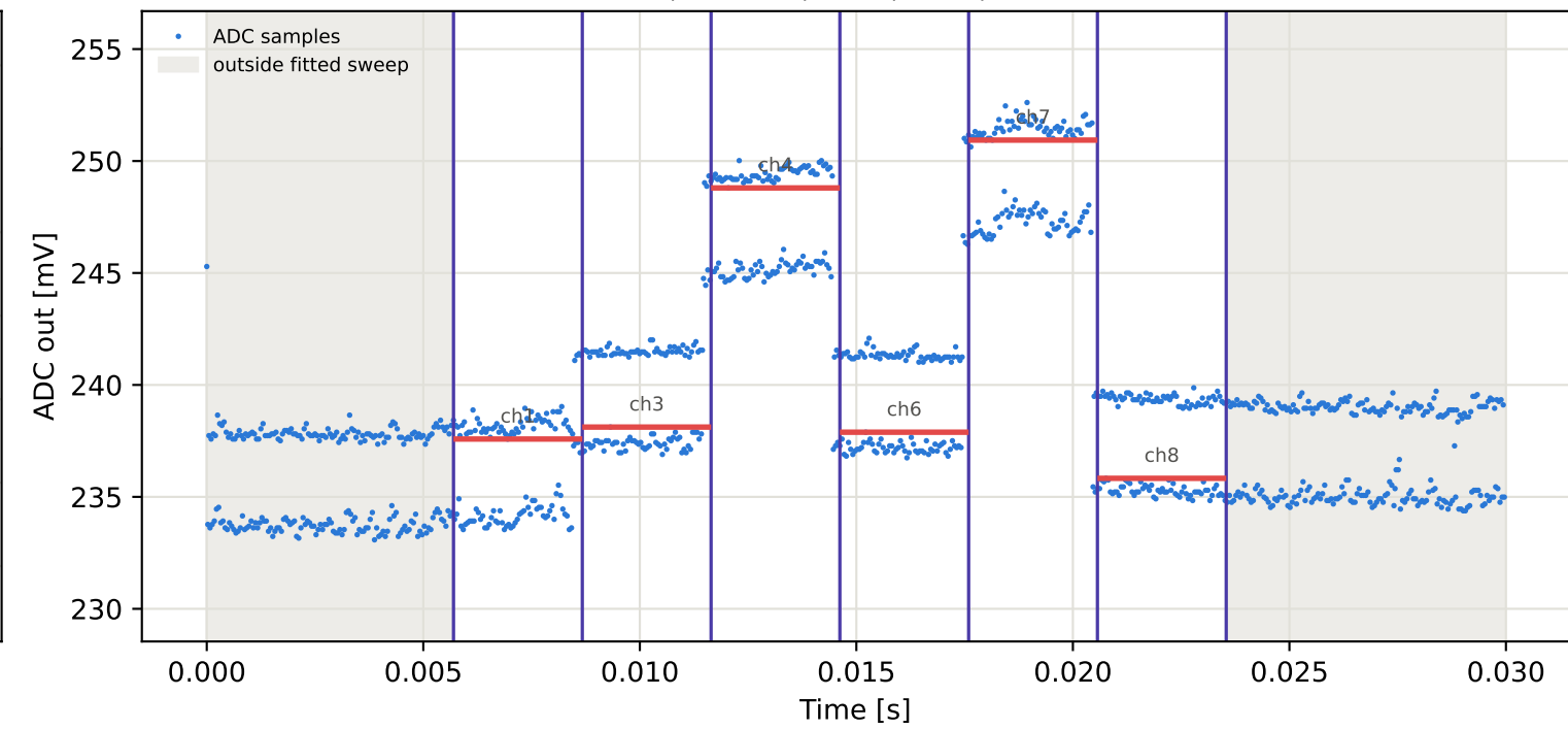
Tag5 &lt;- Tag4 | 785 MHz | run 0 | rep 1 | phase -67.71 deg
