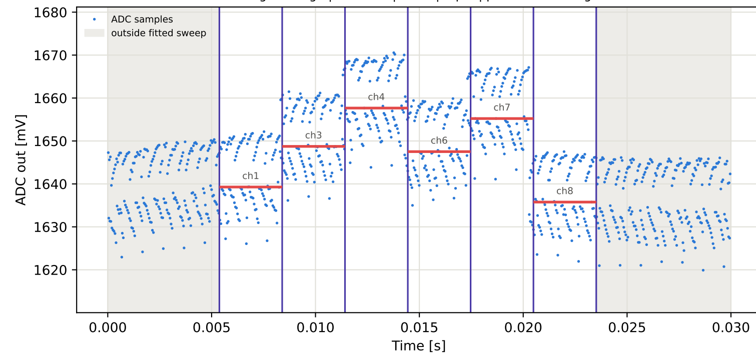
Tag5 &lt;- Tag8 | 905 MHz | run 0 | rep 1 | phase 169.98 deg
