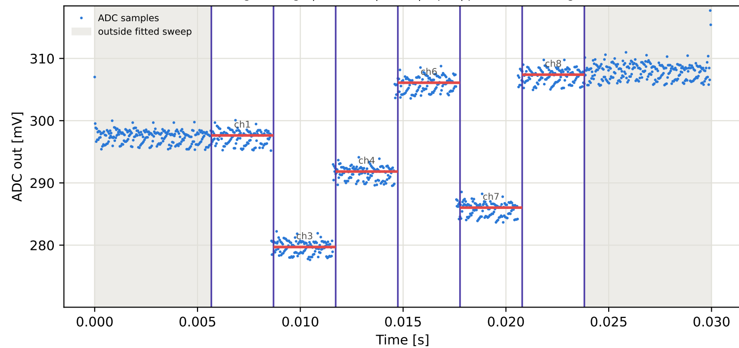
Tag7 &lt;- Tag1 | 835 MHz | run 0 | rep 1 | phase 75.34 deg
