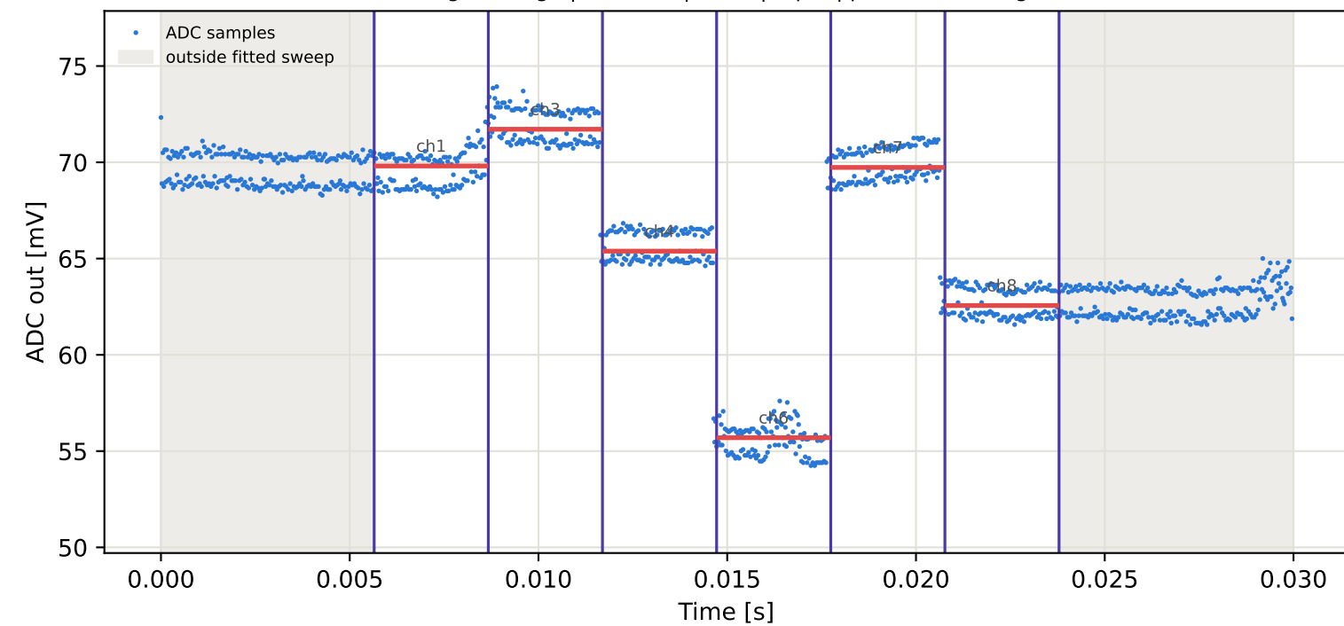
Tag3 &lt;- Tag9 | 965 MHz | run 0 | rep 1 | phase 64.70 deg
