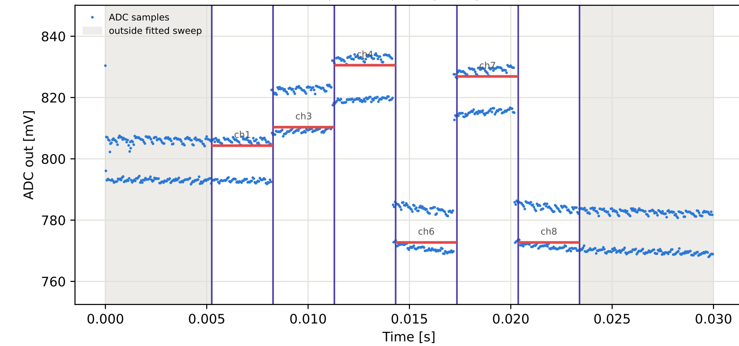
Tag16 &lt;- Tag10 | 925 MHz | run 0 | rep 1 | phase -39.30 deg
