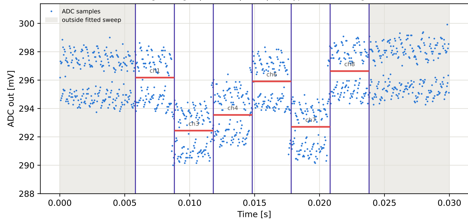
Tag6 &lt;- Tag3 | 835 MHz | run 0 | rep 1 | phase -143.45 deg
