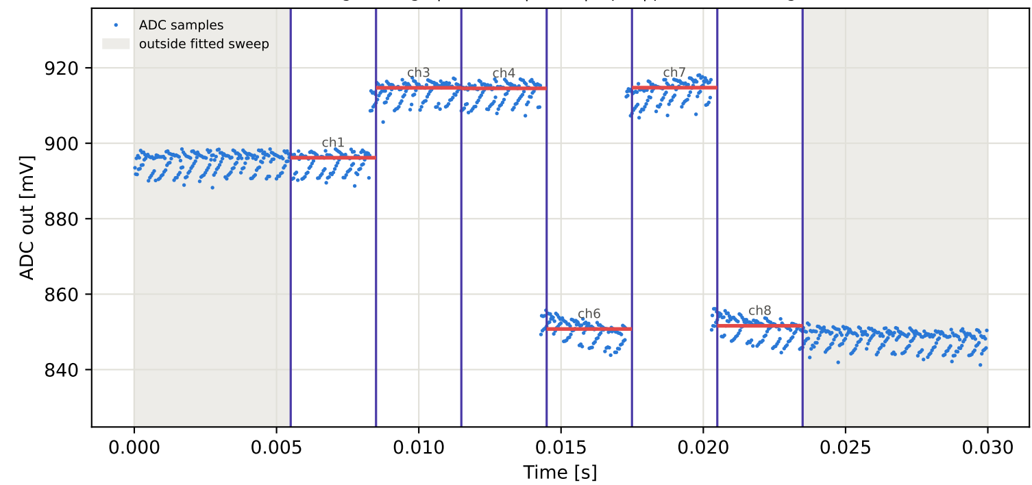
Tag4 &lt;- Tag8 | 895 MHz | run 0 | rep 1 | phase -86.82 deg
