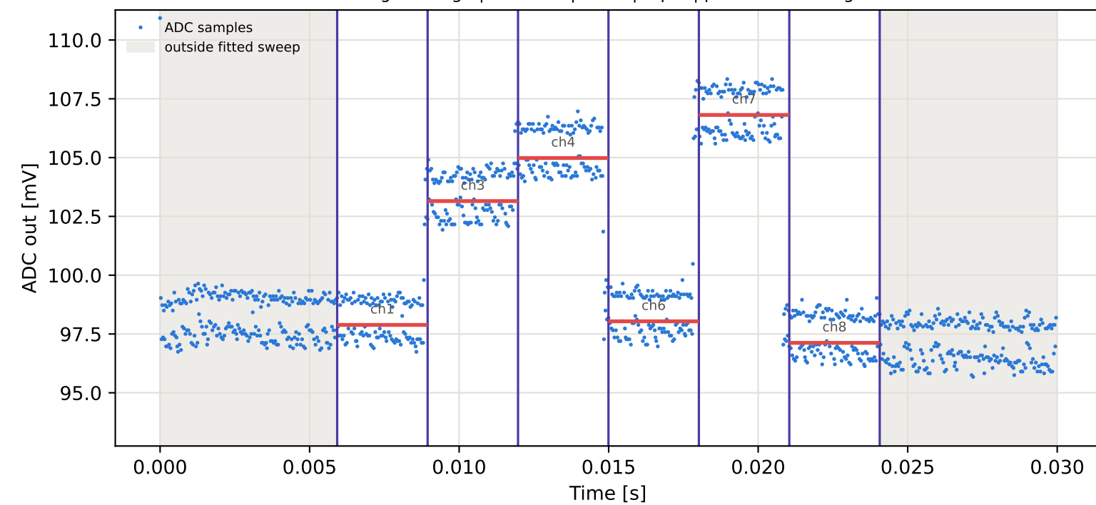
Tag9 &lt;- Tag10 | 795 MHz | run 0 | rep 1 | phase -132.99 deg
