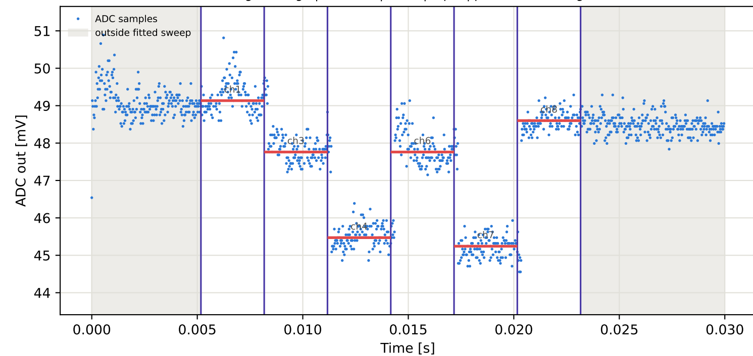
Tag8 &lt;- Tag7 | 775 MHz | run 0 | rep 1 | phase 104.29 deg
