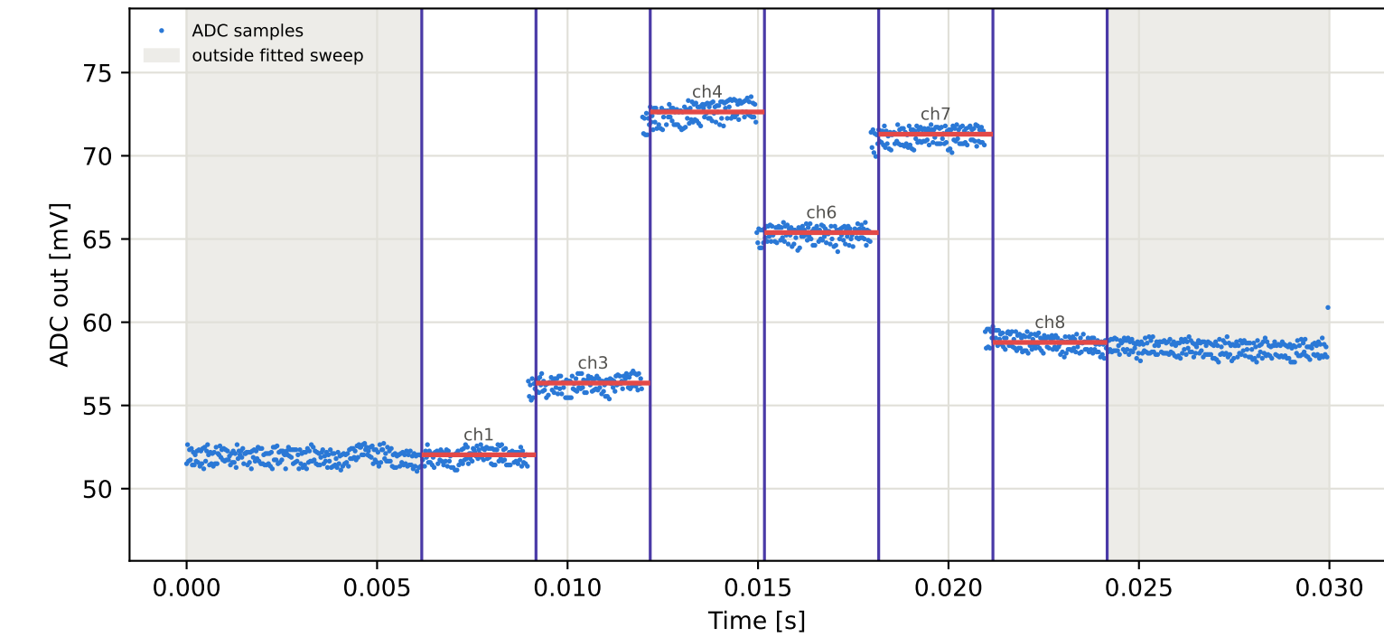
Tag5 &lt;- Tag1 | 805 MHz | run 0 | rep 1 | phase 102.25 deg
