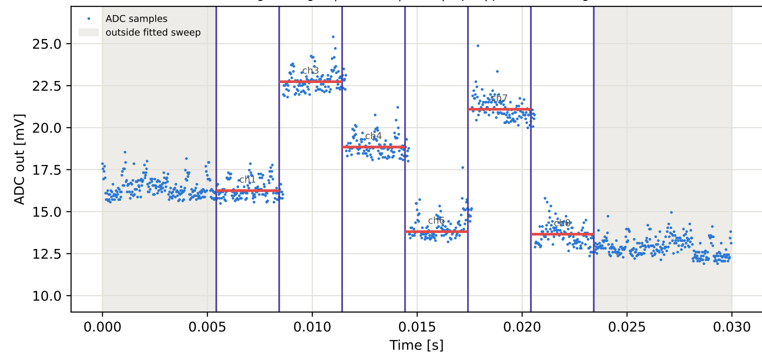
Tag2 &lt;- Tag16 | 845 MHz | run 0 | rep 1 | phase -9.91 deg
