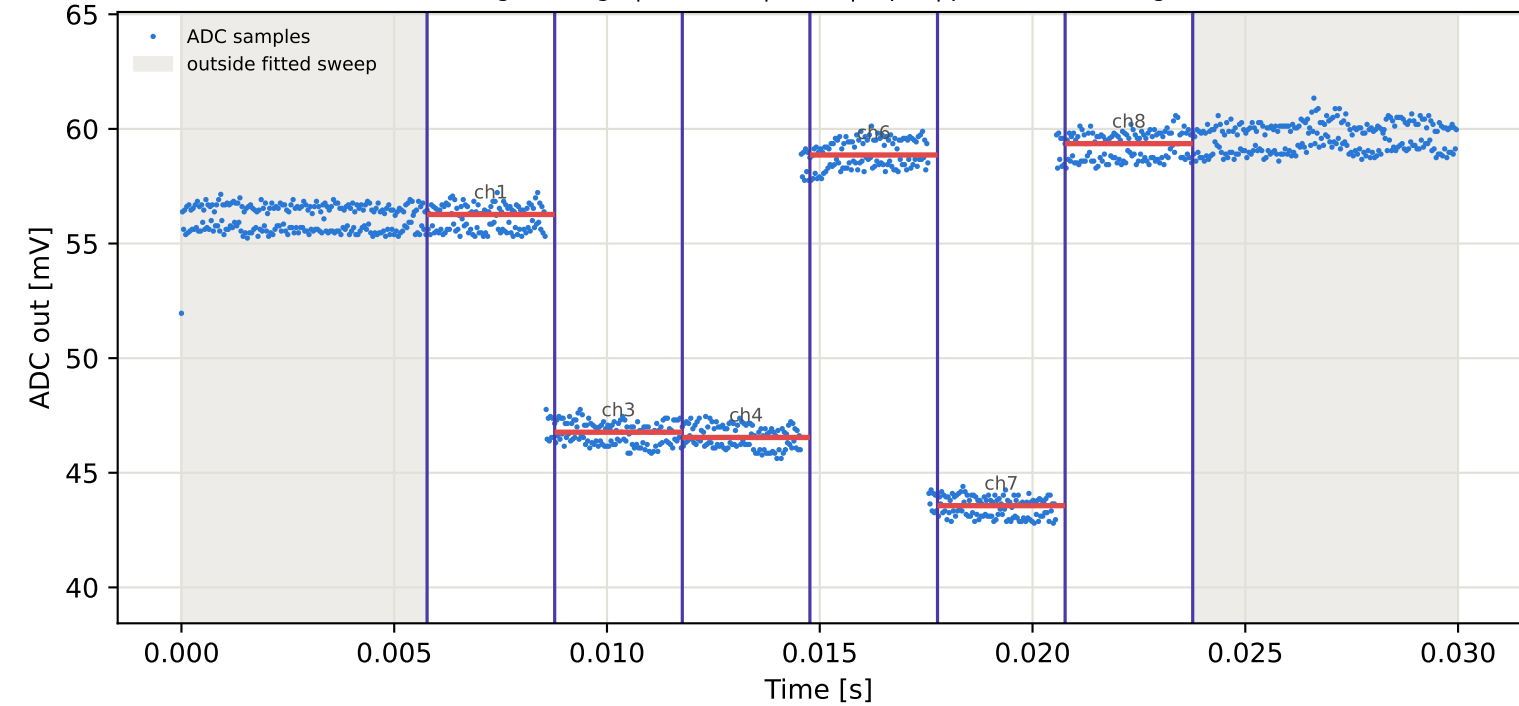
Tag3 &lt;- Tag7 | 785 MHz | run 0 | rep 1 | phase 153.49 deg
