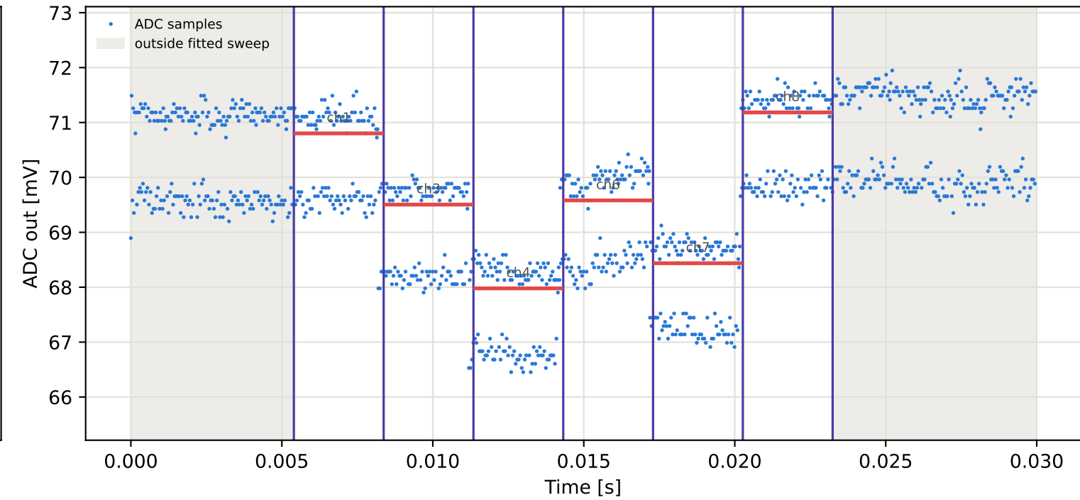
Tag1 &lt;- Tag4 | 805 MHz | run 0 | rep 1 | phase -68.58 deg
