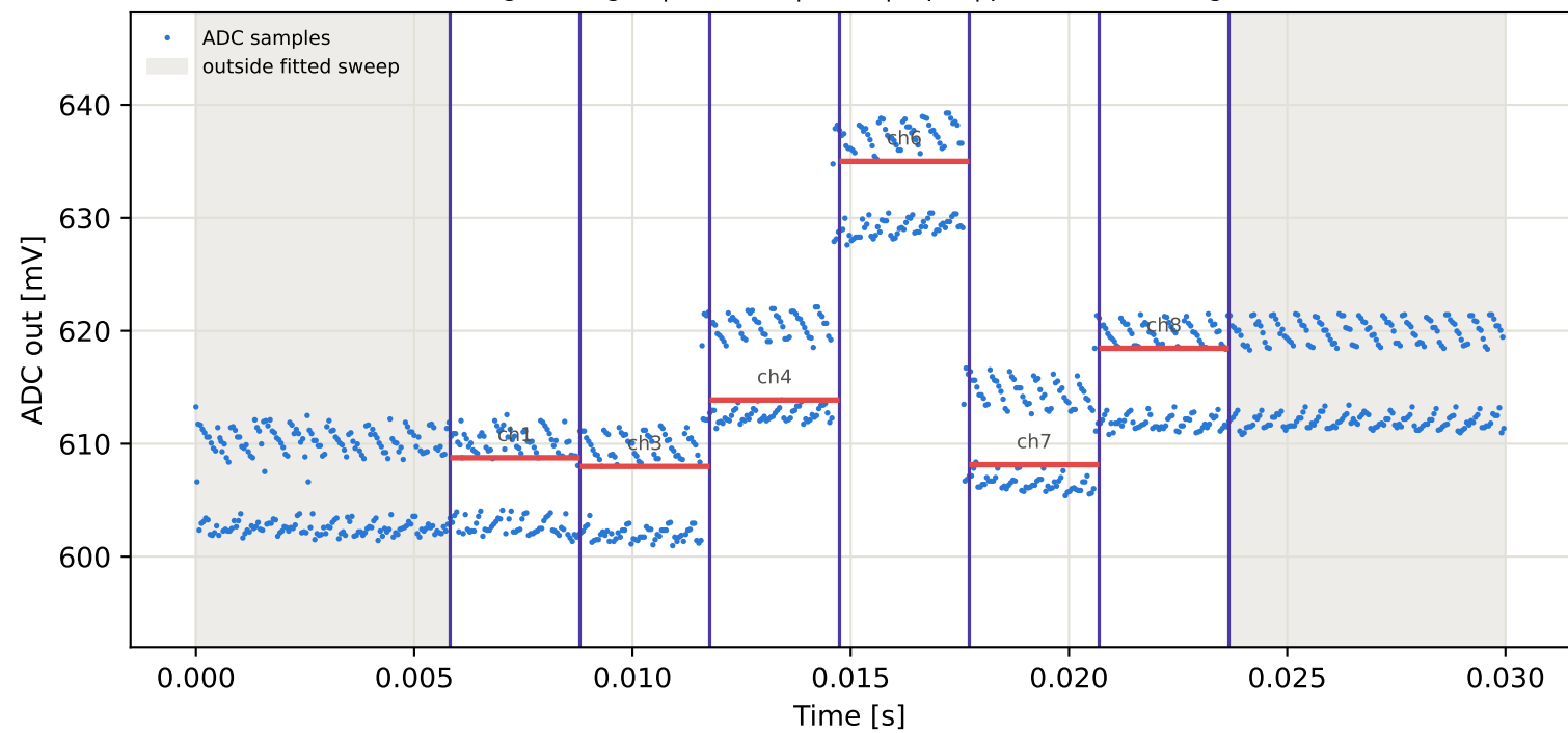
Tag4 &lt;- Tag16 | 945 MHz | run 0 | rep 1 | phase -28.68 deg
