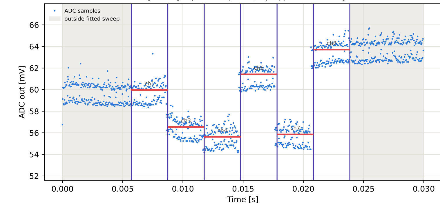
Tag2 &lt;- Tag15 | 905 MHz | run 0 | rep 1 | phase 135.87 deg
