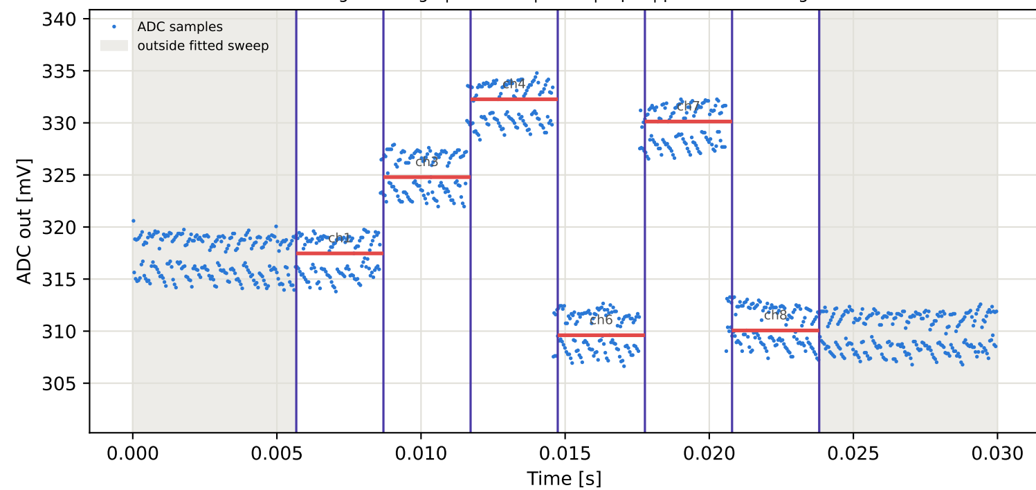
Tag10 &lt;- Tag9 | 965 MHz | run 0 | rep 1 | phase -96.29 deg
