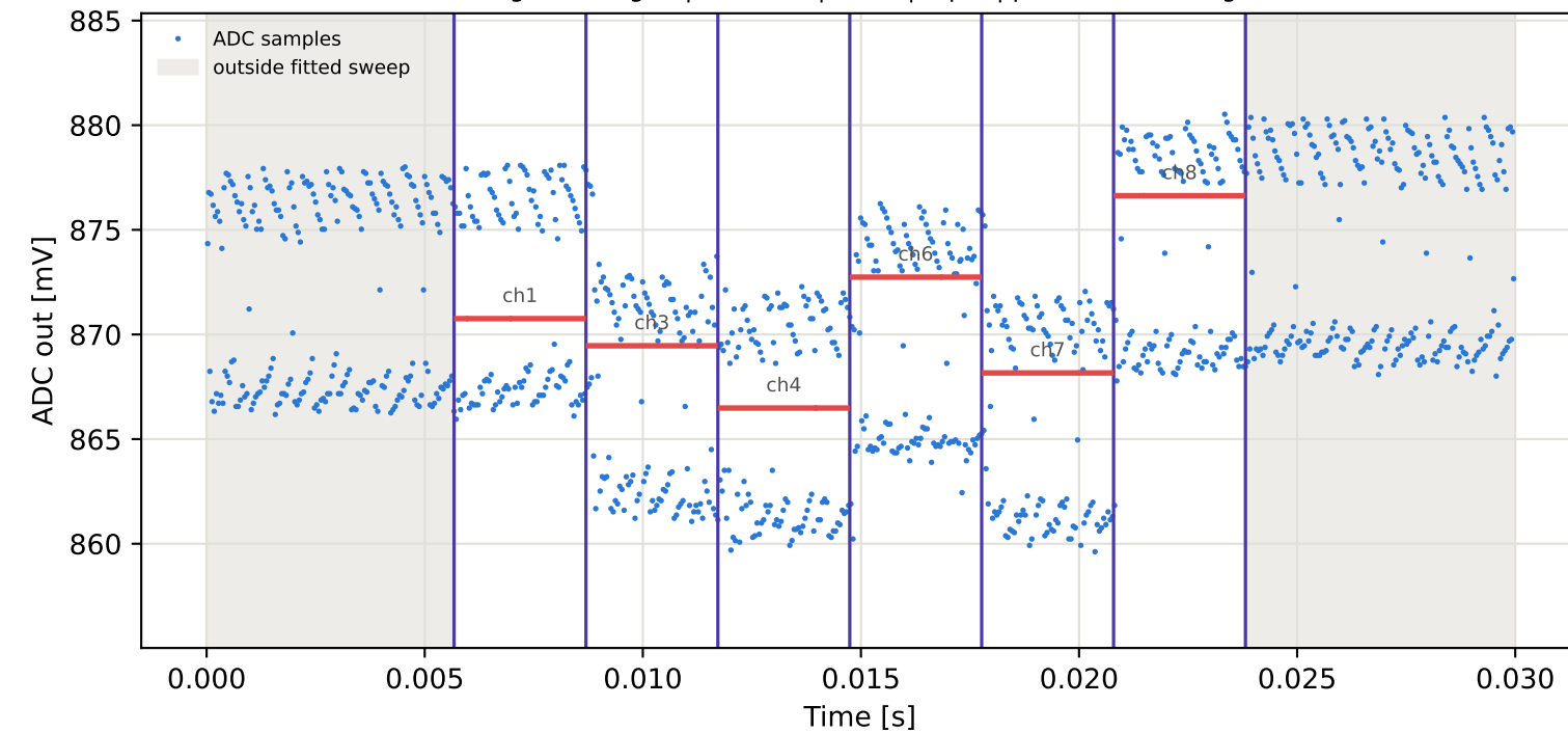
Tag16 &lt;- Tag10 | 875 MHz | run 0 | rep 1 | phase 126.06 deg
