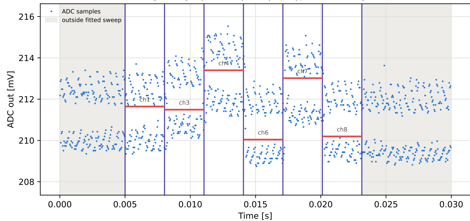
Tag5 &lt;- Tag16 | 995 MHz | run 0 | rep 1 | phase 46.30 deg
