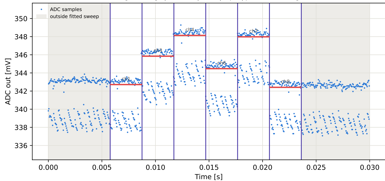
Tag15 &lt;- Tag9 | 855 MHz | run 0 | rep 1 | phase -134.76 deg
