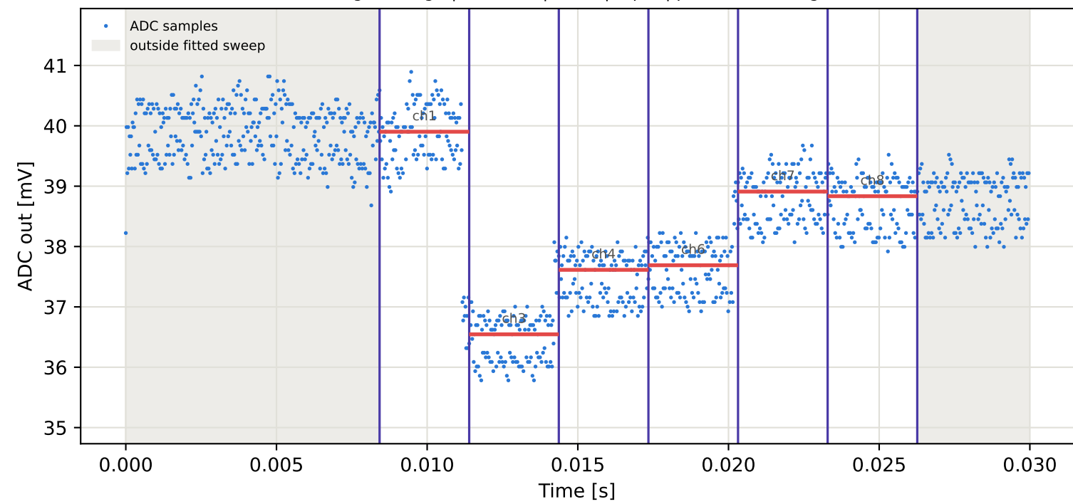
Tag9 &lt;- Tag15 | 805 MHz | run 0 | rep 1 | phase -67.53 deg
