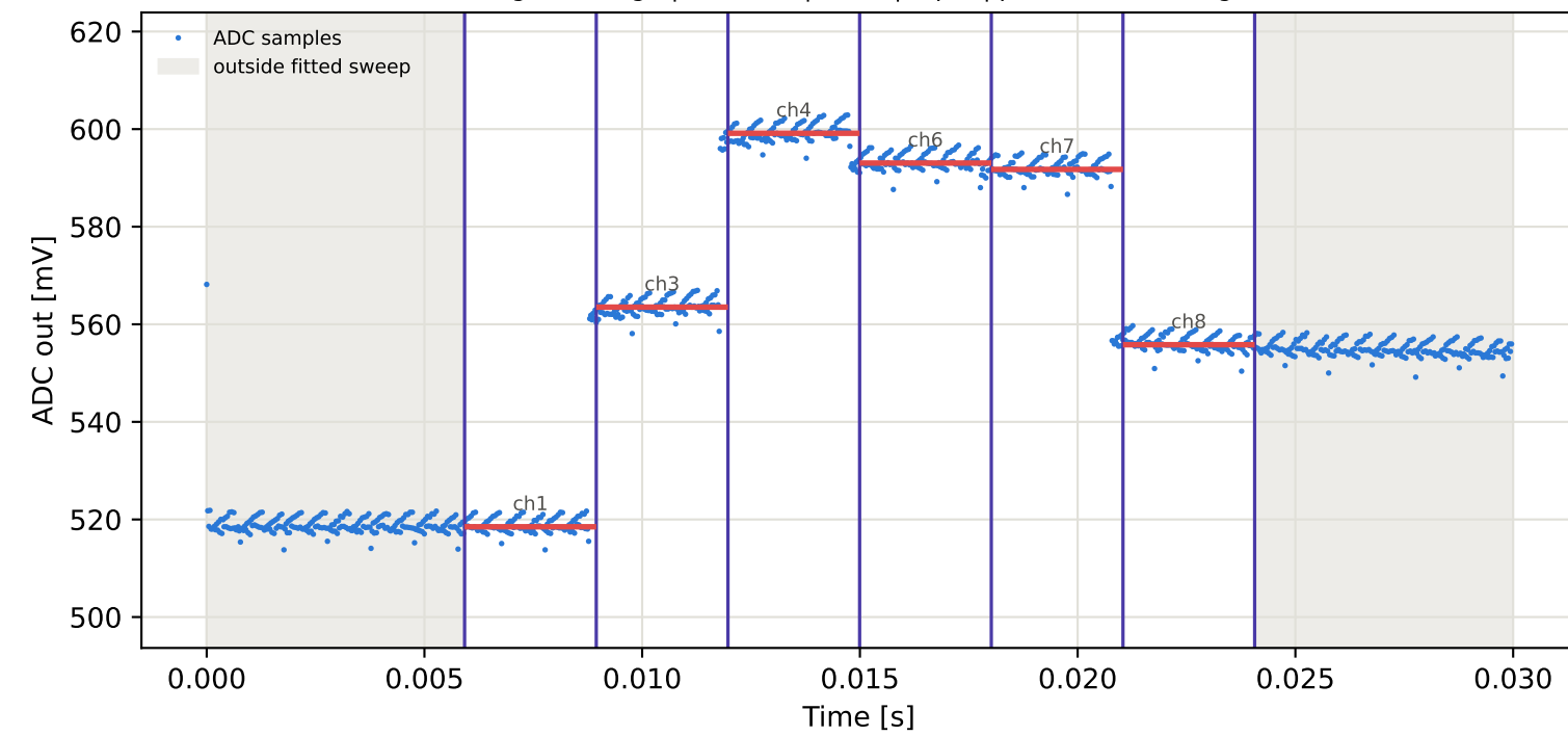
Tag2 &lt;- Tag1 | 865 MHz | run 0 | rep 1 | phase 98.20 deg
