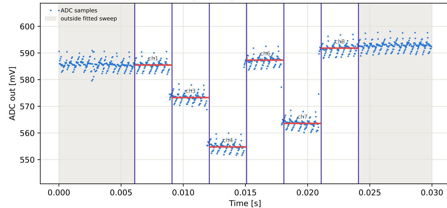
Tag16 &lt;- Tag6 | 955 MHz | run 0 | rep 1 | phase 104.35 deg
