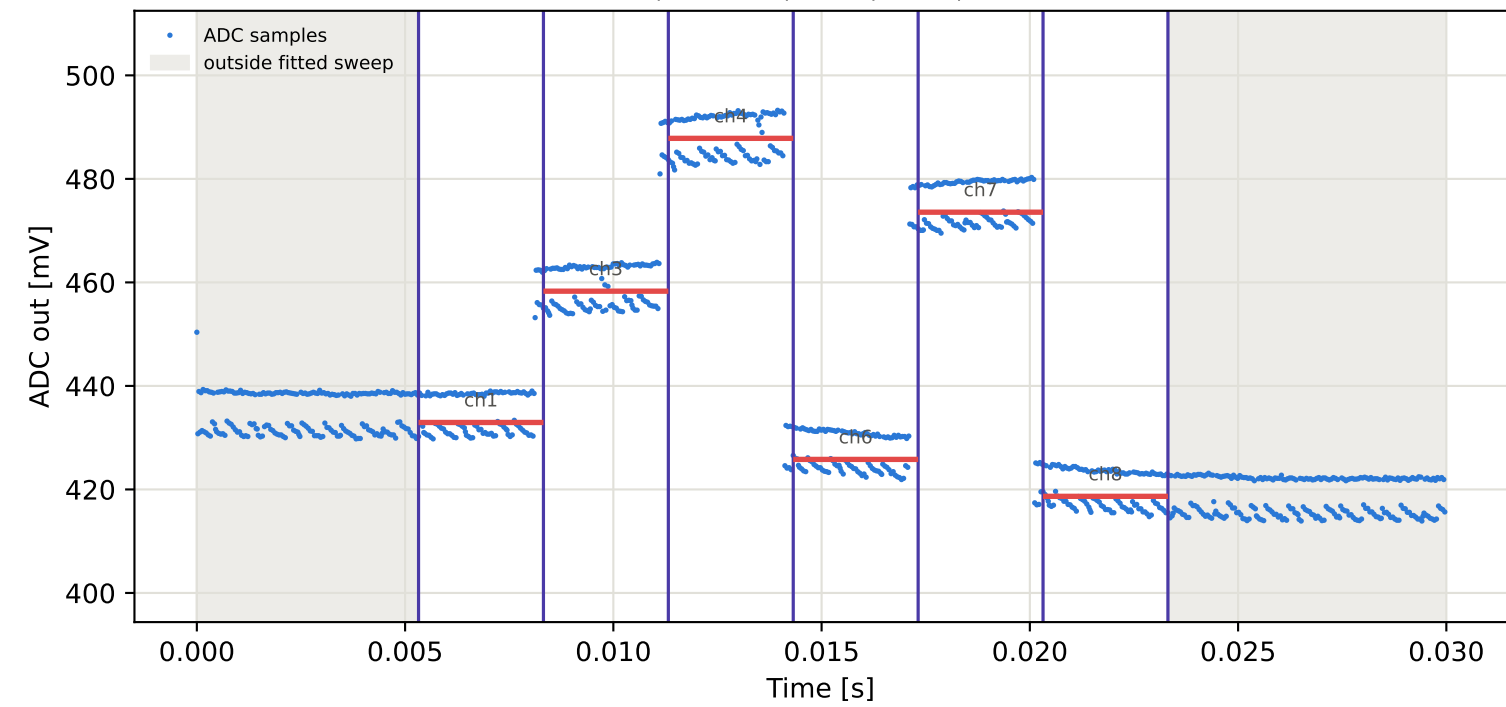
Tag16 &lt;- Tag15 | 975 MHz | run 0 | rep 1 | phase -68.46 deg
