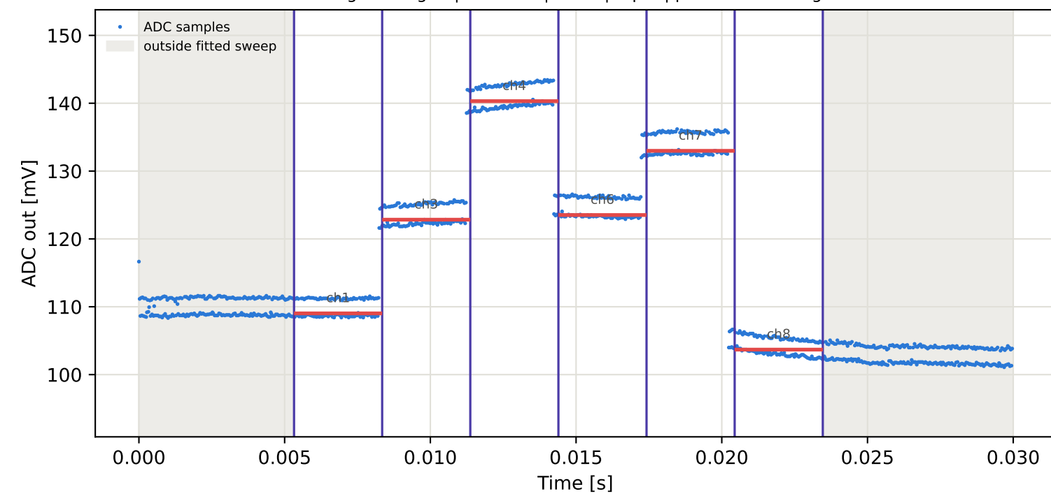
Tag1 &lt;- Tag16 | 925 MHz | run 0 | rep 1 | phase -128.90 deg
