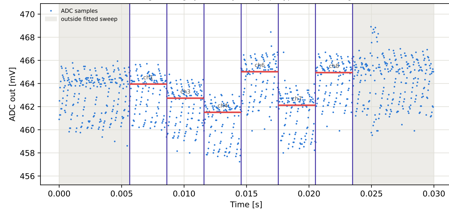
Tag16 &lt;- Tag4 | 975 MHz | run 0 | rep 1 | phase 46.85 deg
