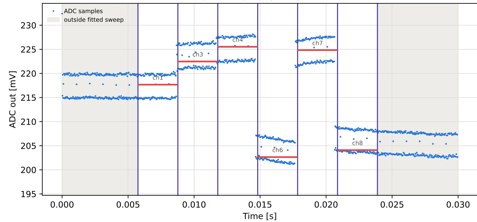
Tag1 &lt;- Tag4 | 915 MHz | run 0 | rep 1 | phase -24.48 deg
