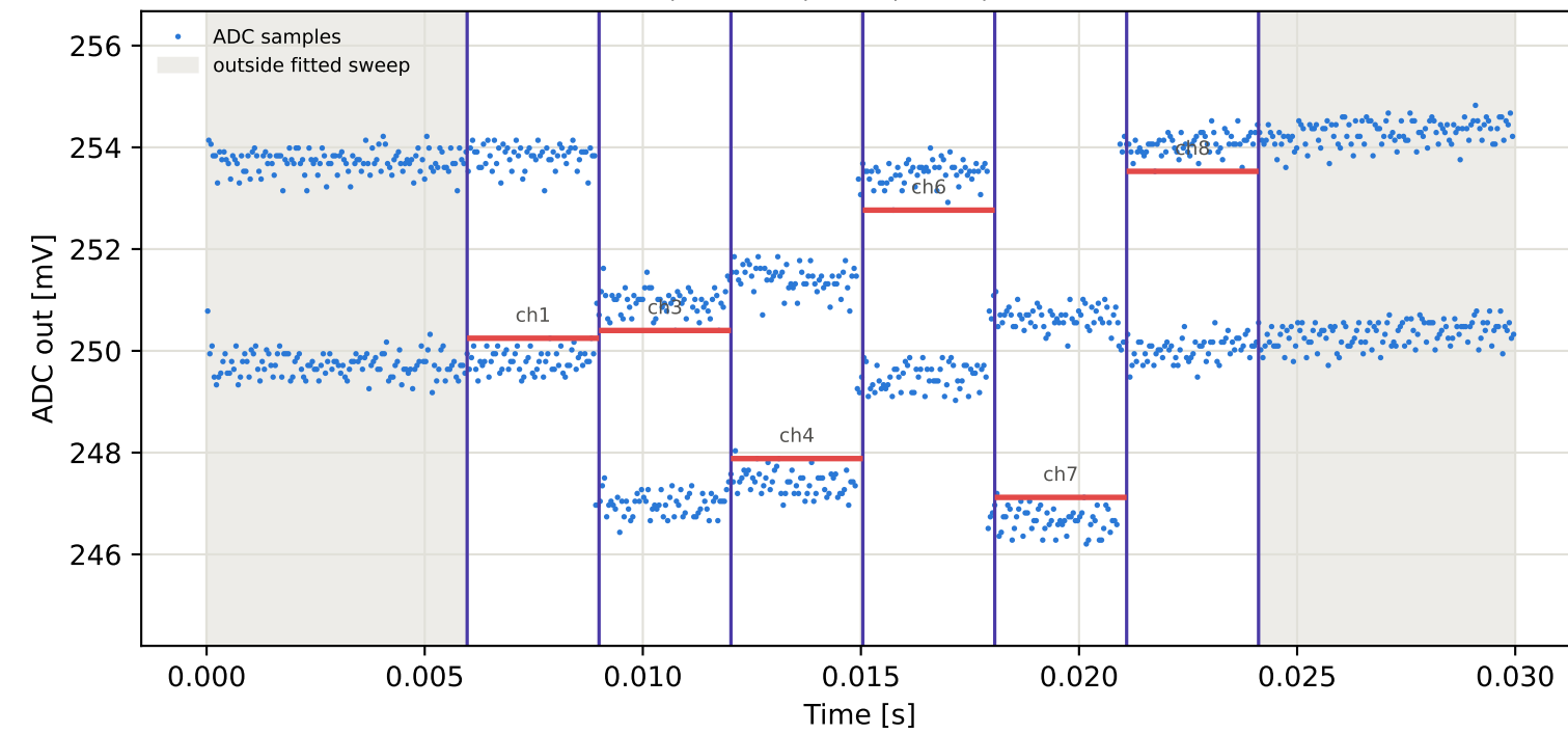
Tag1 &lt;- Tag9 | 835 MHz | run 0 | rep 1 | phase 138.14 deg
