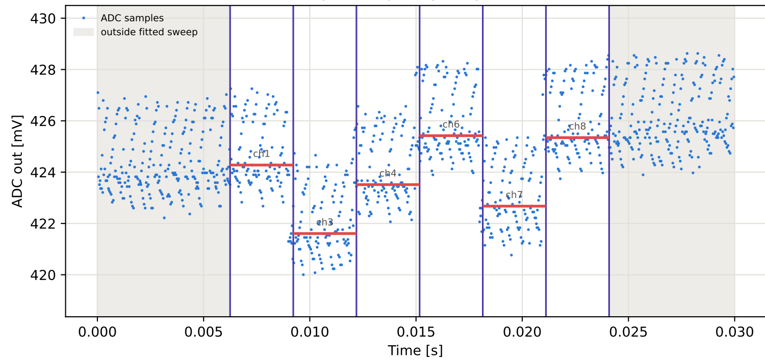
Tag4 &lt;- Tag9 | 835 MHz | run 0 | rep 1 | phase 179.88 deg
