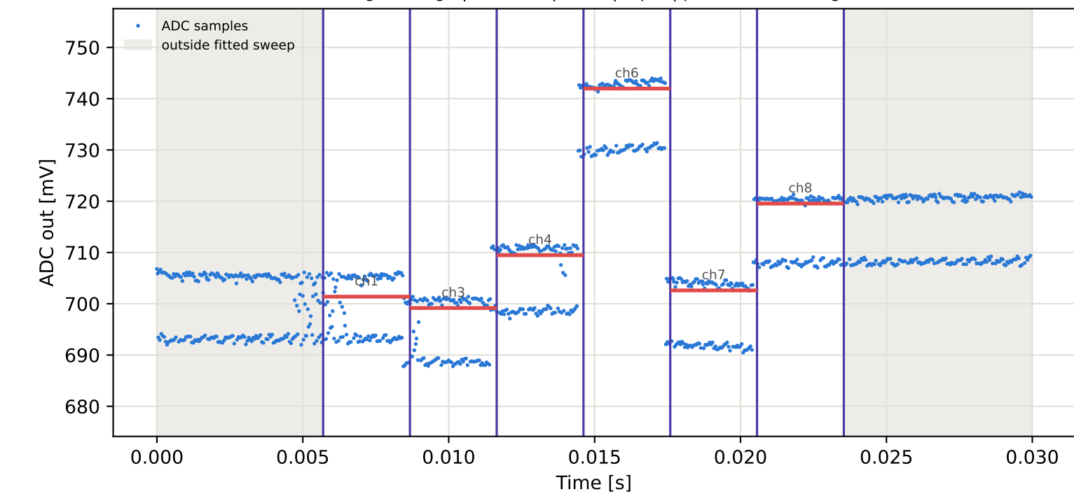
Tag8 &lt;- Tag6 | 955 MHz | run 0 | rep 1 | phase -117.46 deg
