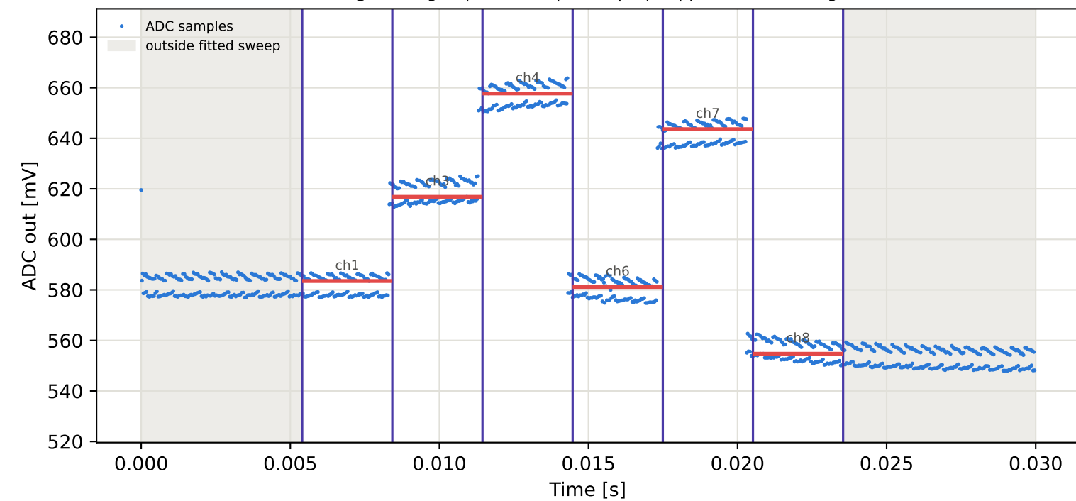
Tag4 &lt;- Tag2 | 945 MHz | run 0 | rep 1 | phase -106.92 deg
