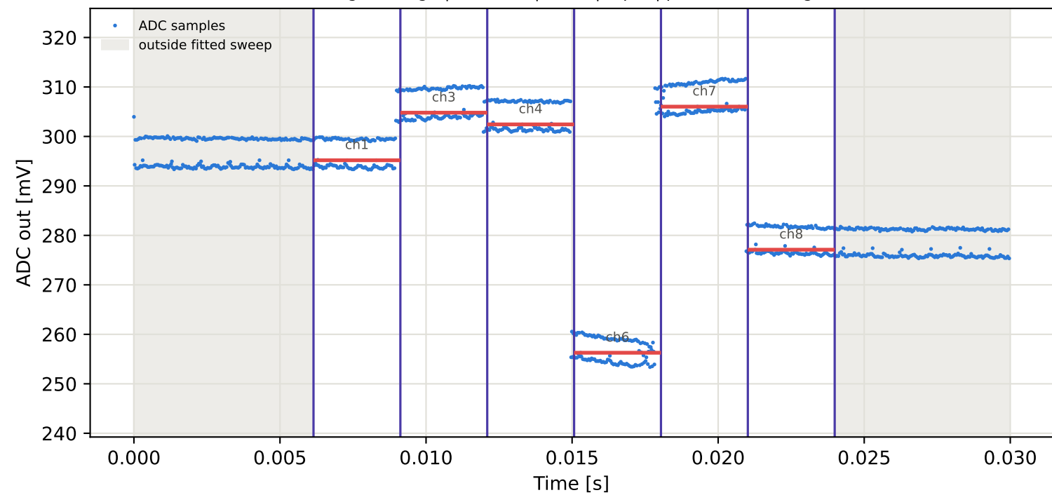
Tag9 &lt;- Tag5 | 985 MHz | run 0 | rep 1 | phase 31.79 deg
