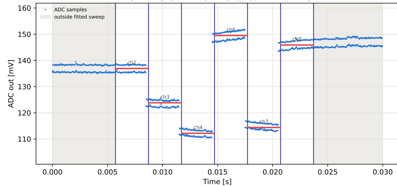
Tag10 &lt;- Tag8 | 995 MHz | run 0 | rep 1 | phase -72.19 deg
