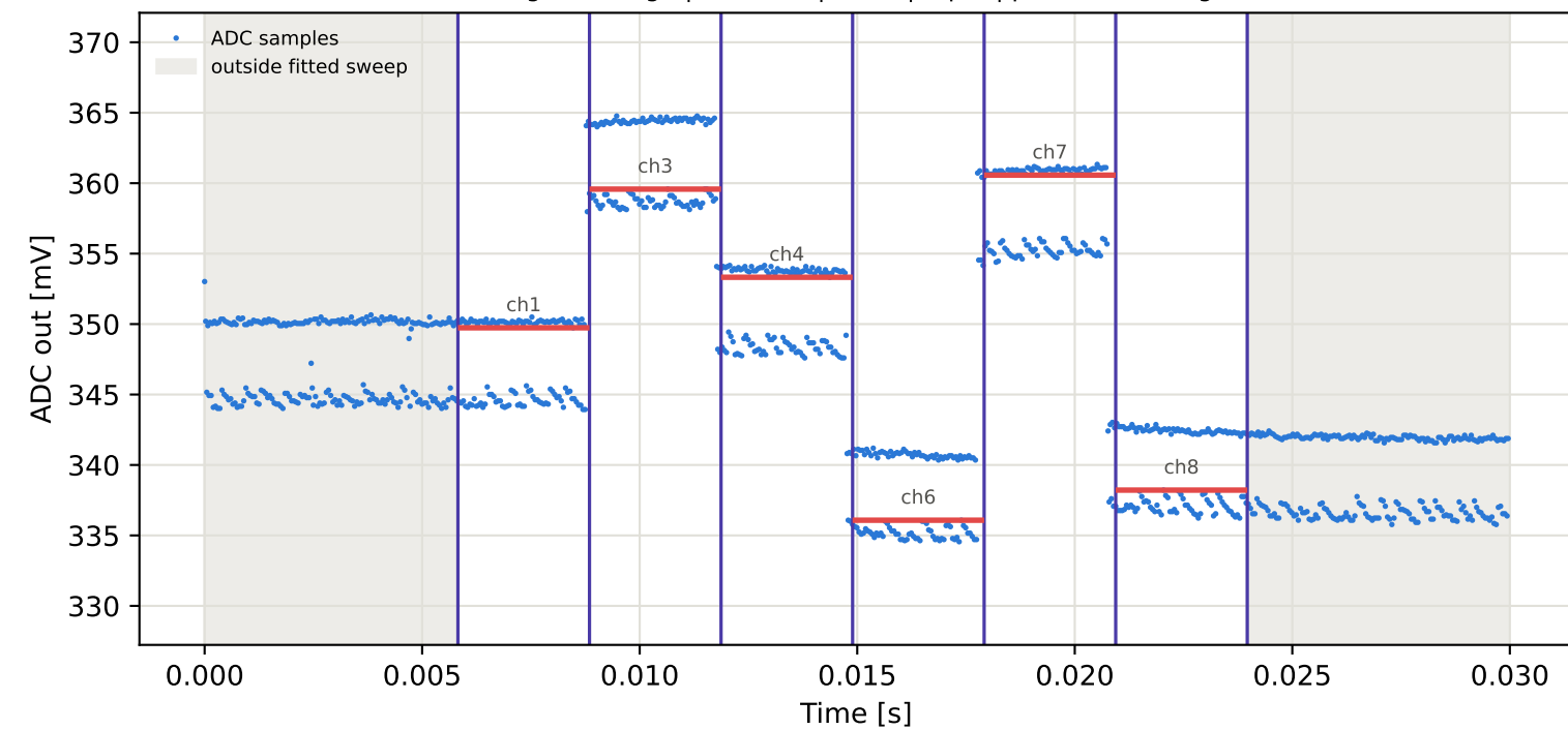
Tag16 &lt;- Tag7 | 825 MHz | run 0 | rep 1 | phase 5.45 deg
