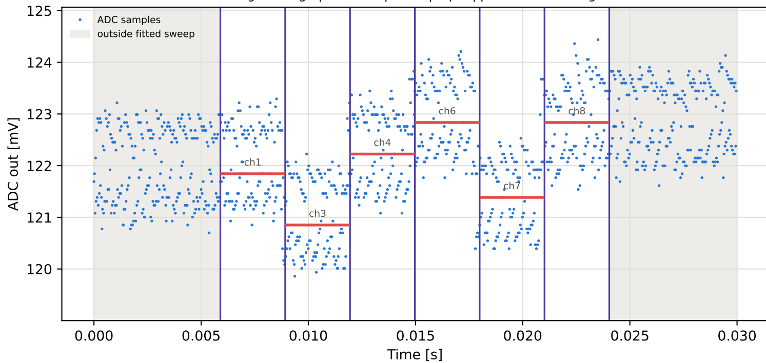
Tag8 &lt;- Tag1 | 775 MHz | run 0 | rep 1 | phase -126.07 deg
