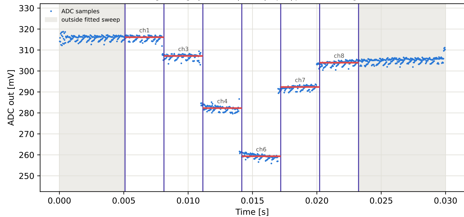
Tag4 &lt;- Tag8 | 915 MHz | run 0 | rep 1 | phase -2.77 deg
