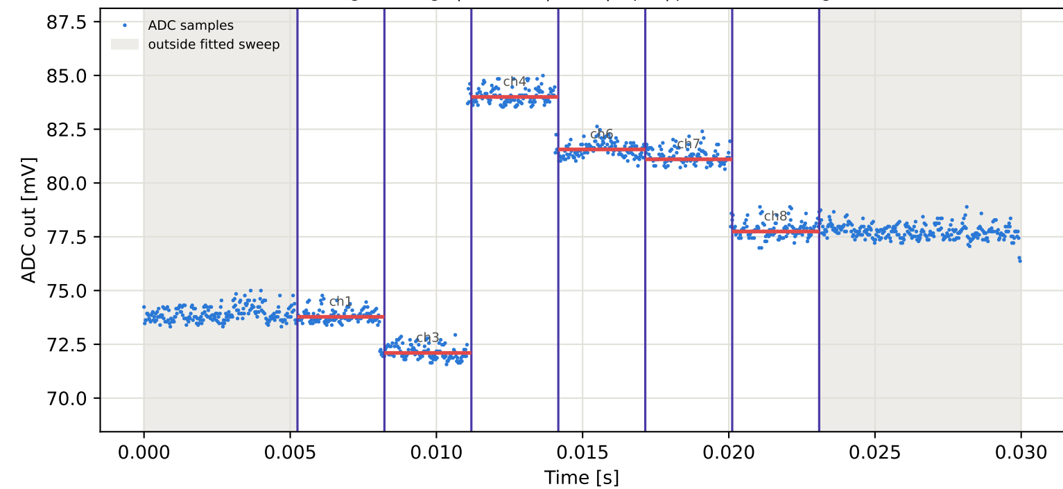
Tag10 &lt;- Tag8 | 775 MHz | run 0 | rep 1 | phase 53.53 deg
