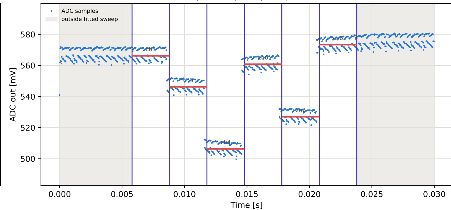
Tag16 &lt;- Tag1 | 965 MHz | run 0 | rep 1 | phase -148.56 deg
