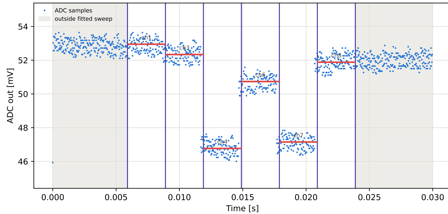
Tag1 &lt;- Tag16 | 775 MHz | run 0 | rep 1 | phase 102.76 deg
