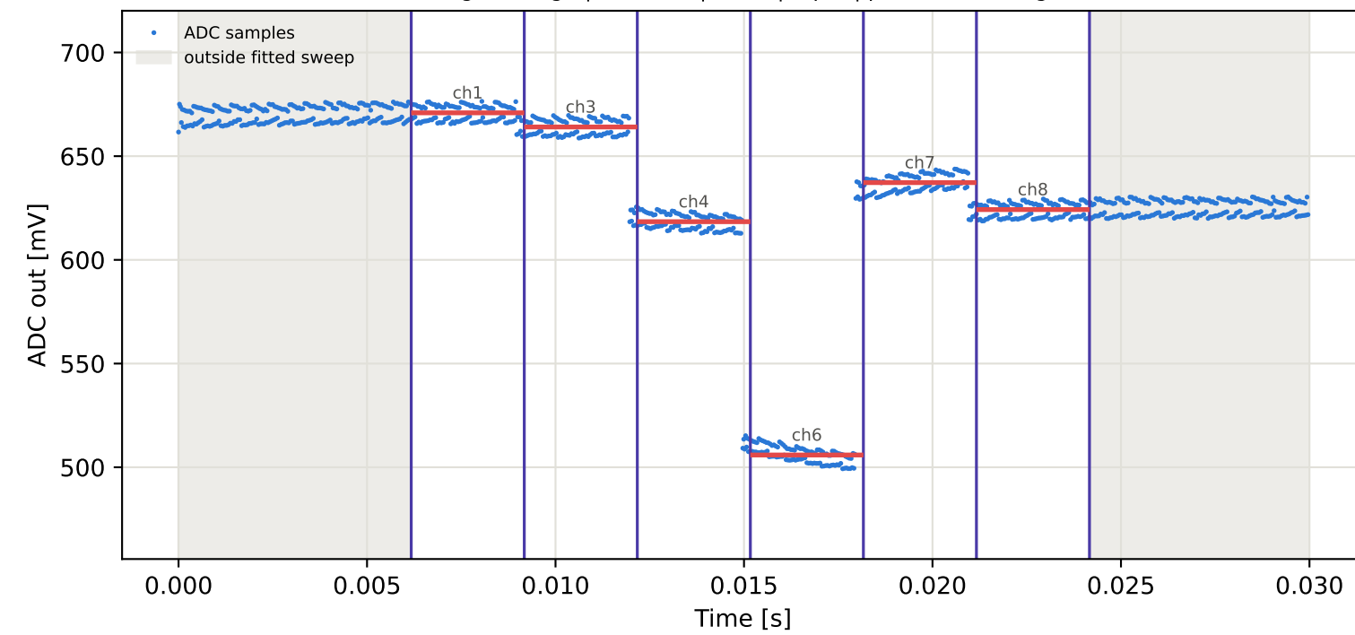
Tag4 &lt;- Tag7 | 925 MHz | run 0 | rep 1 | phase -71.35 deg
