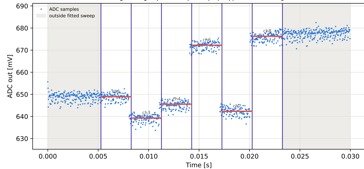
Tag1 &lt;- Tag16 | 885 MHz | run 0 | rep 1 | phase -130.61 deg
