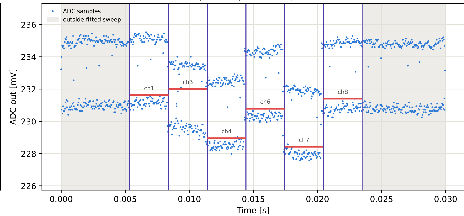
Tag8 &lt;- Tag5 | 805 MHz | run 0 | rep 1 | phase -97.73 deg
