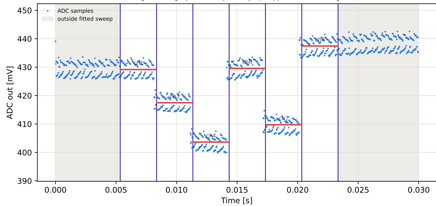
Tag10 &lt;- Tag4 | 935 MHz | run 0 | rep 1 | phase 108.21 deg
