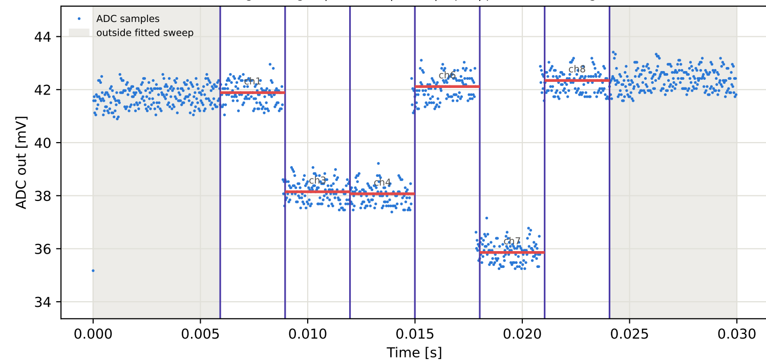
Tag1 &lt;- Tag16 | 785 MHz | run 0 | rep 1 | phase 93.30 deg
