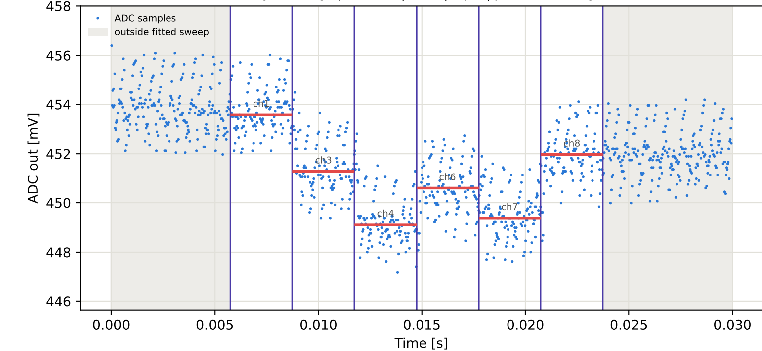
Tag16 &lt;- Tag10 | 845 MHz | run 0 | rep 1 | phase 138.52 deg
