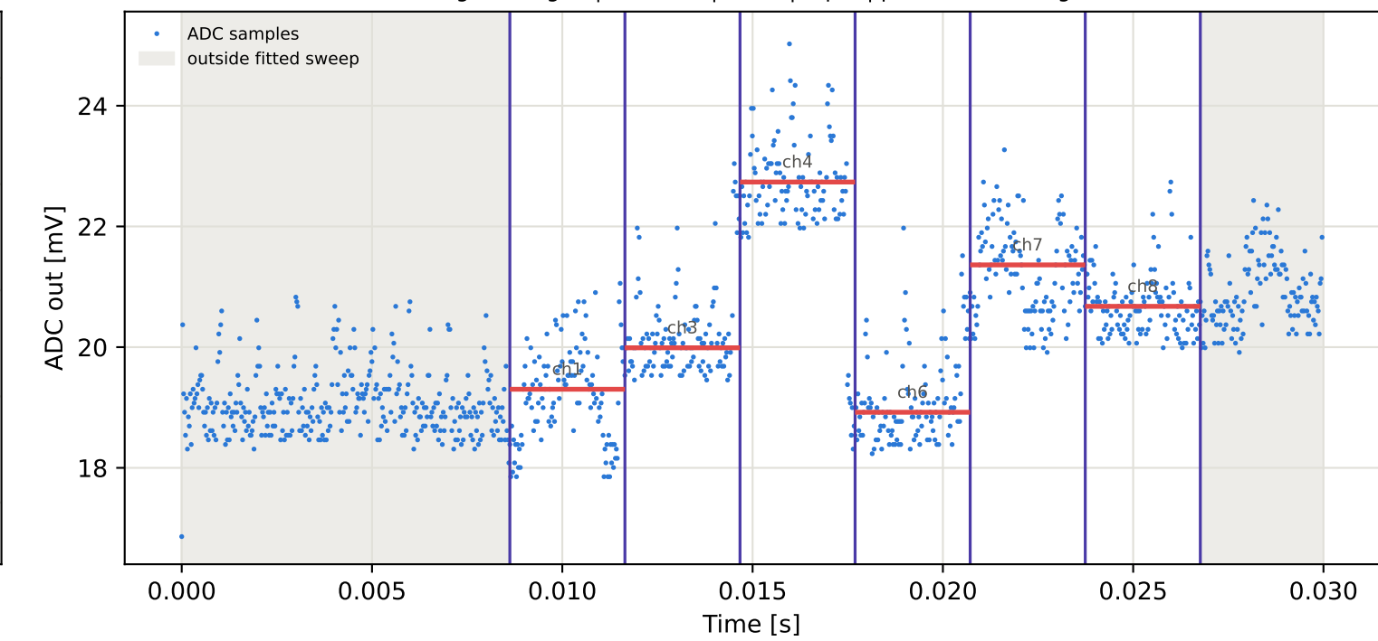
Tag2 &lt;- Tag16 | 965 MHz | run 0 | rep 1 | phase -87.95 deg
