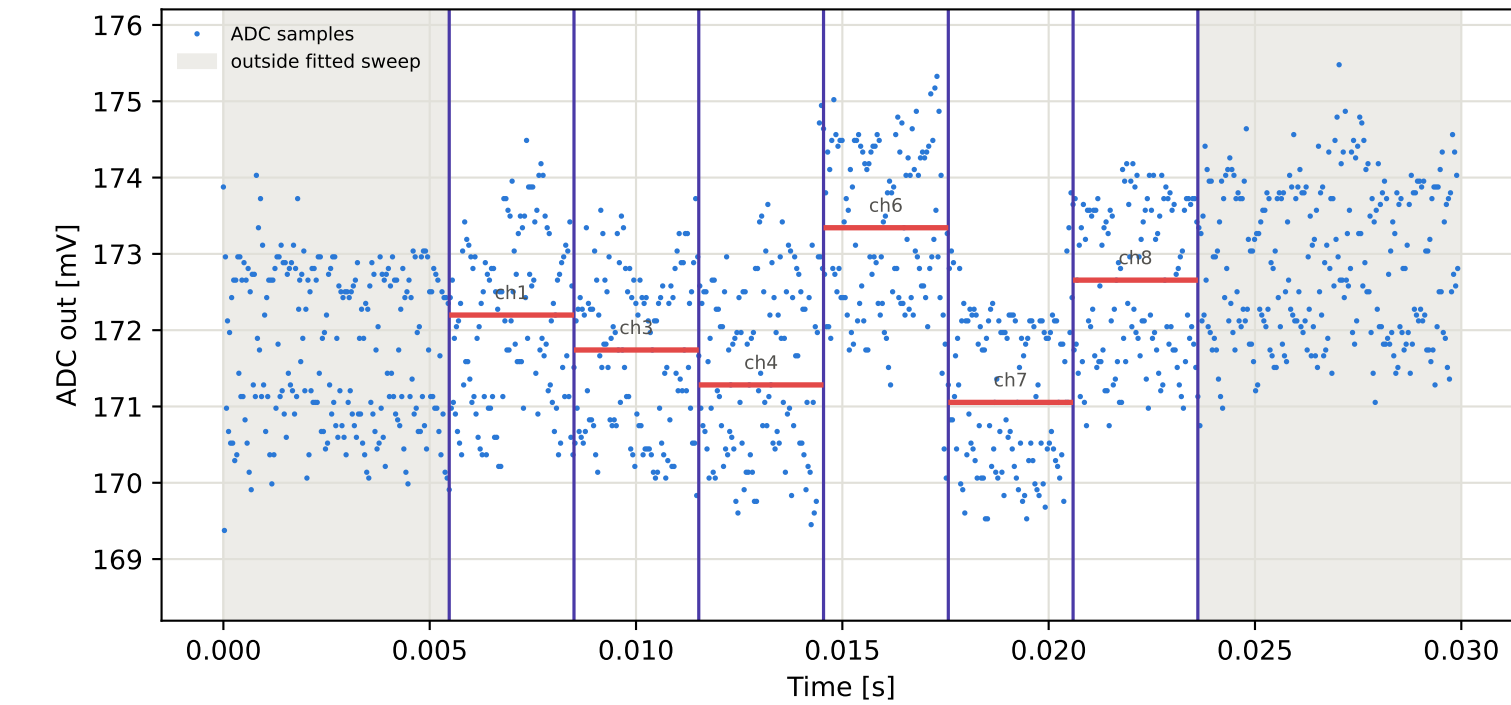
Tag6 &lt;- Tag4 | 995 MHz | run 0 | rep 1 | phase 60.46 deg
