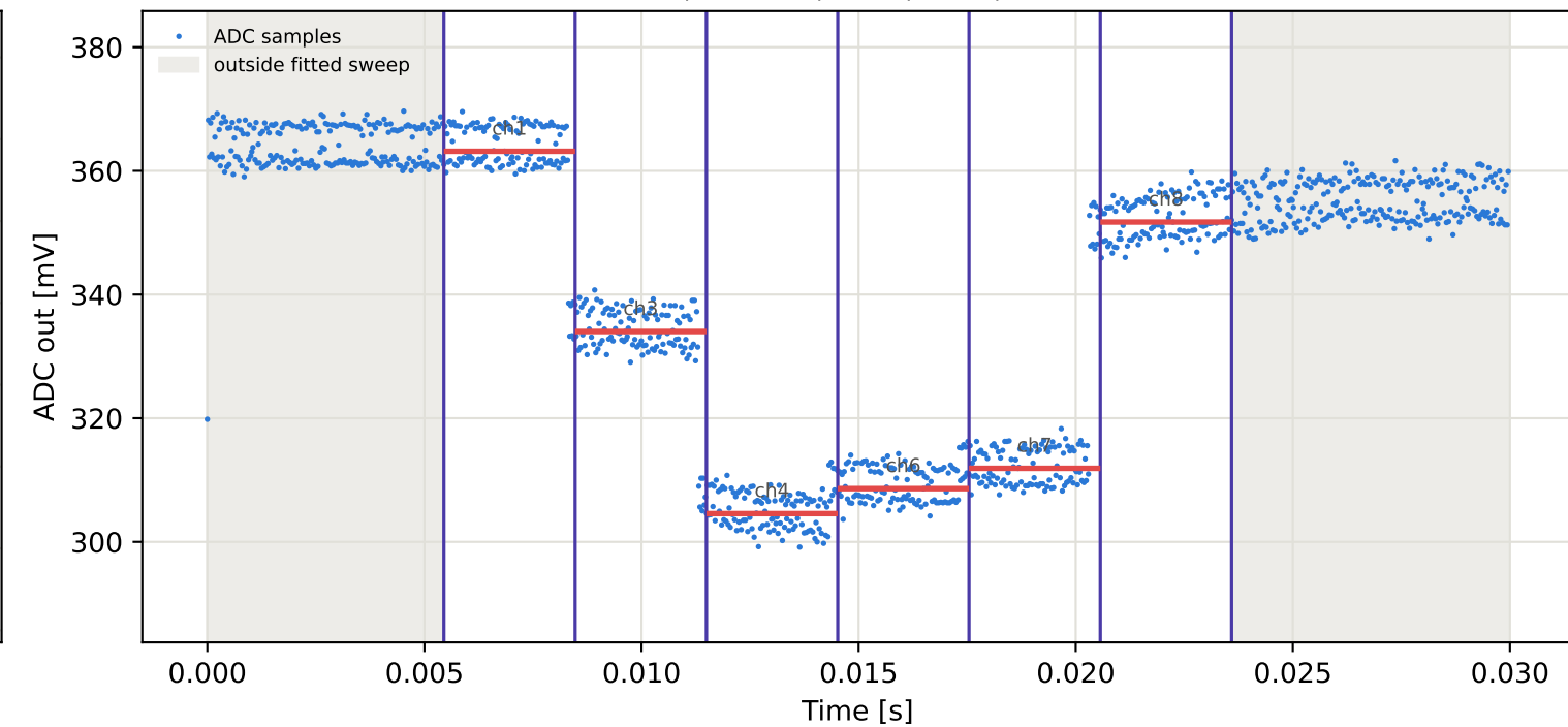
Tag10 &lt;- Tag1 | 885 MHz | run 0 | rep 1 | phase 69.42 deg
