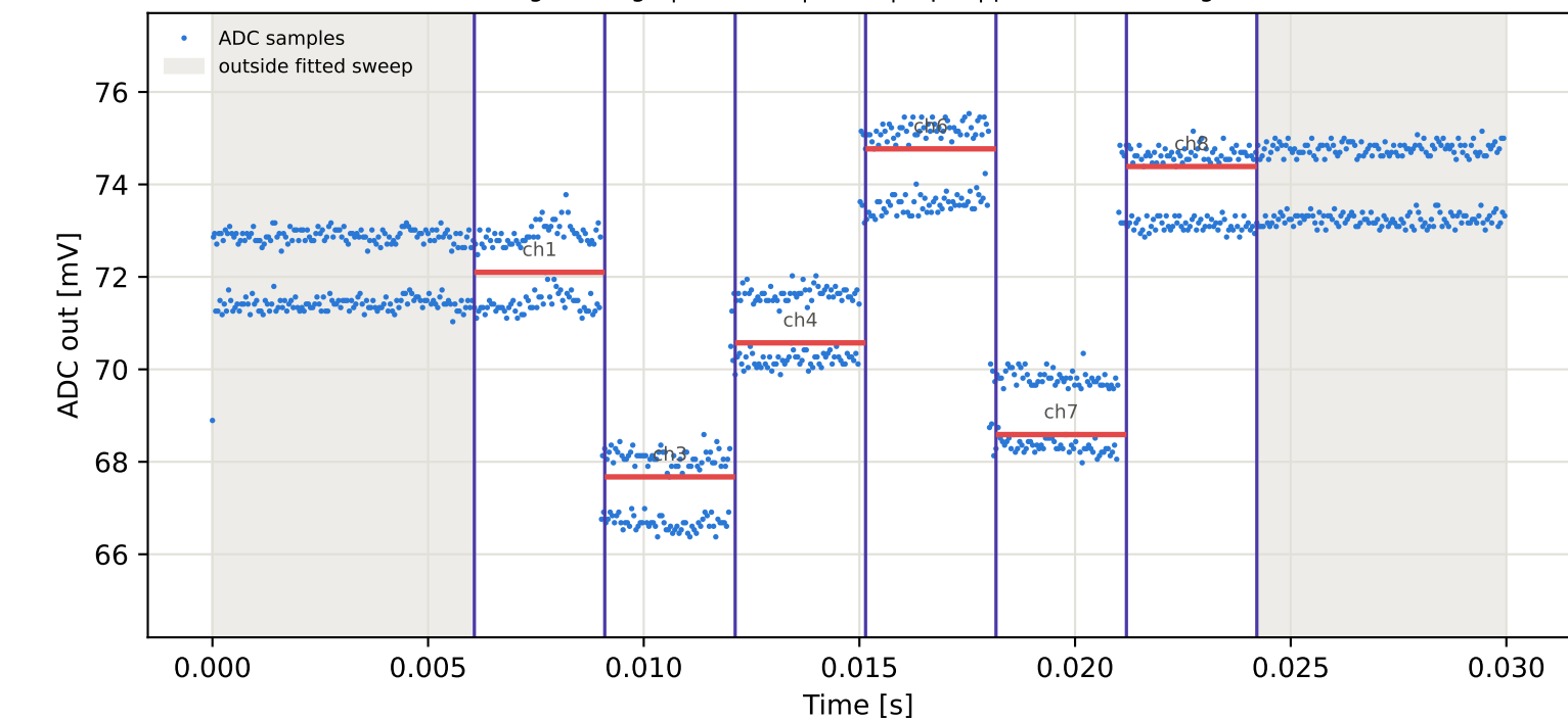
Tag3 &lt;- Tag8 | 805 MHz | run 0 | rep 1 | phase 179.65 deg
