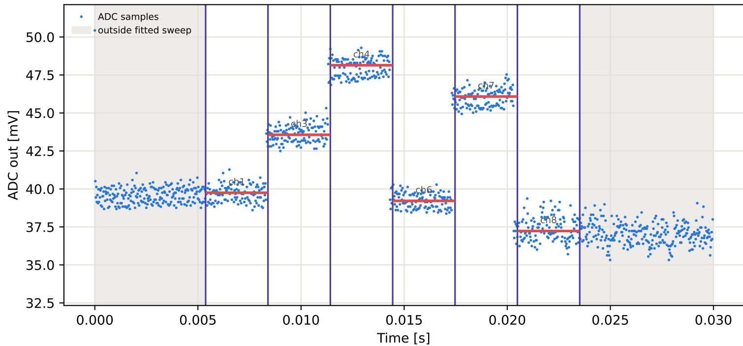
Tag2 &lt;- Tag16 | 935 MHz | run 0 | rep 1 | phase 141.17 deg
