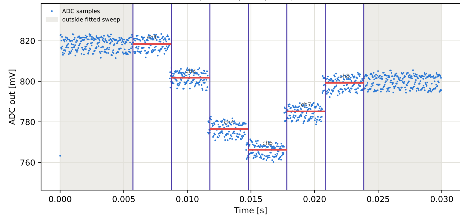
Tag2 &lt;- Tag10 | 885 MHz | run 0 | rep 1 | phase 120.59 deg
