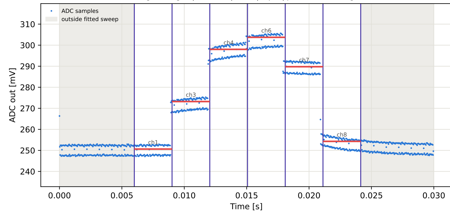
Tag1 &lt;- Tag16 | 905 MHz | run 0 | rep 1 | phase -129.95 deg
