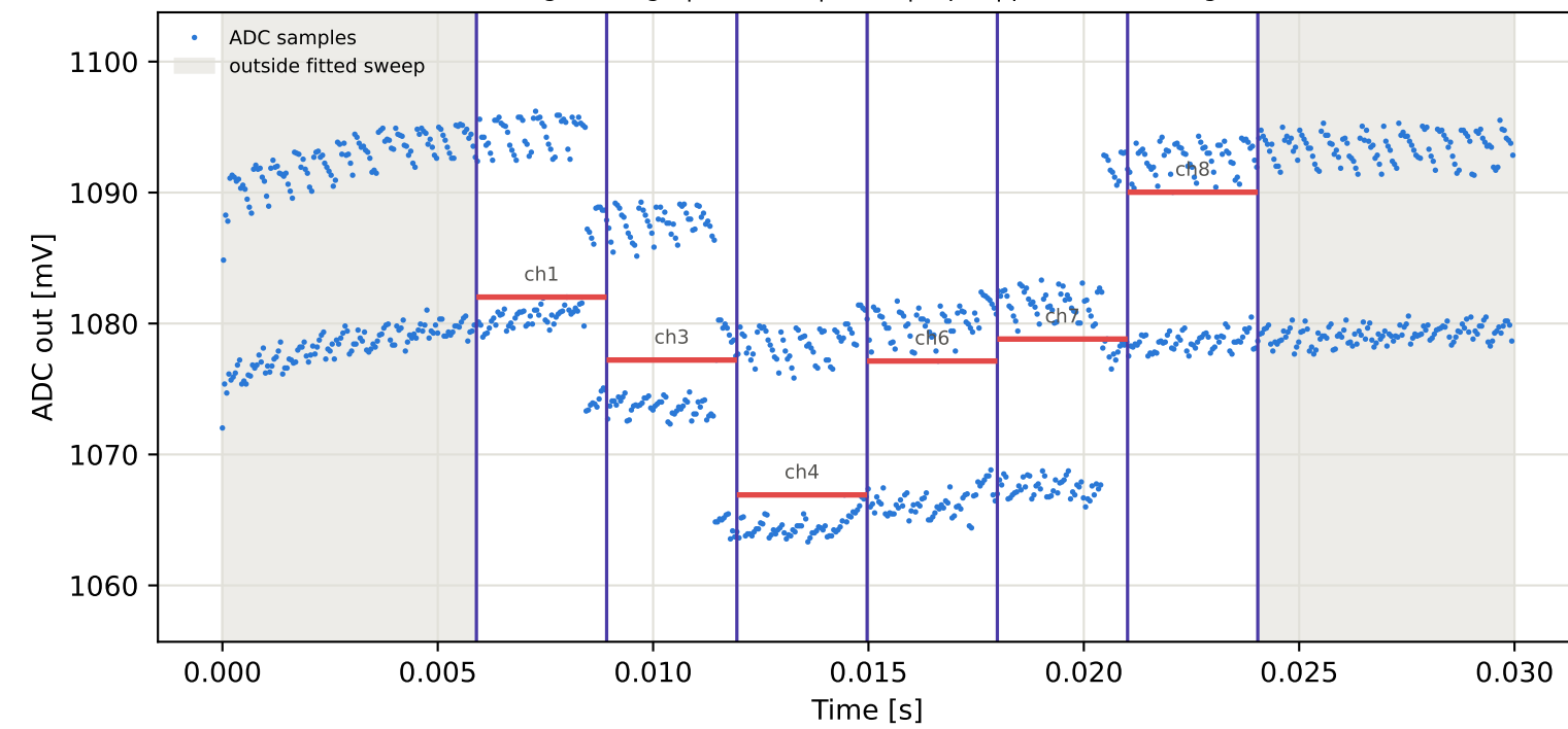
Tag9 &lt;- Tag10 | 905 MHz | run 0 | rep 1 | phase 130.56 deg
