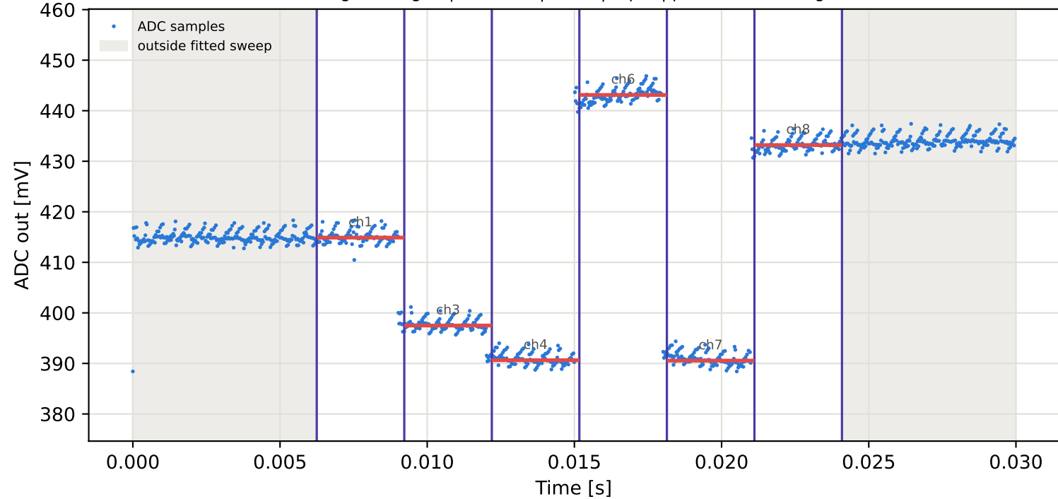
Tag8 &lt;- Tag15 | 995 MHz | run 0 | rep 1 | phase 146.60 deg
