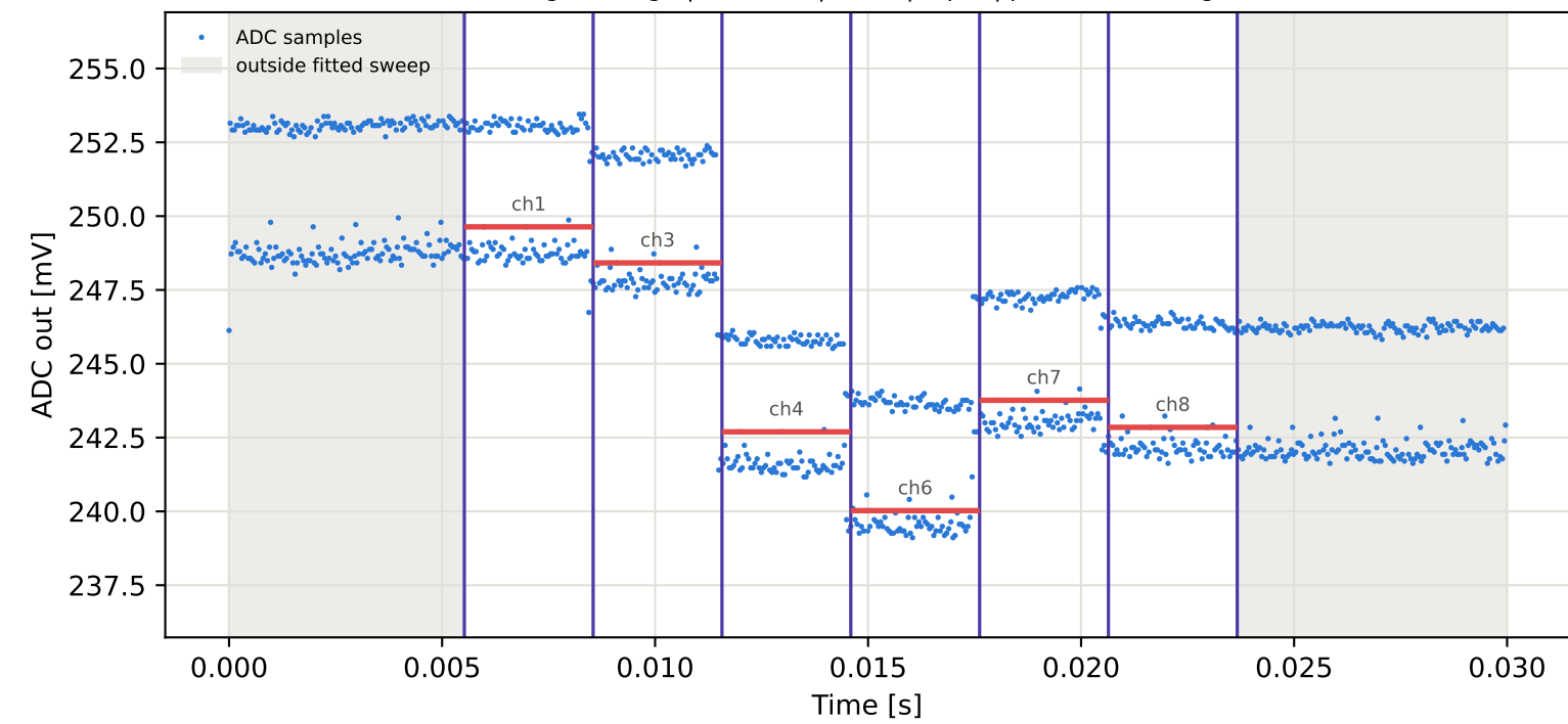
Tag1 &lt;- Tag7 | 855 MHz | run 0 | rep 1 | phase 60.83 deg
