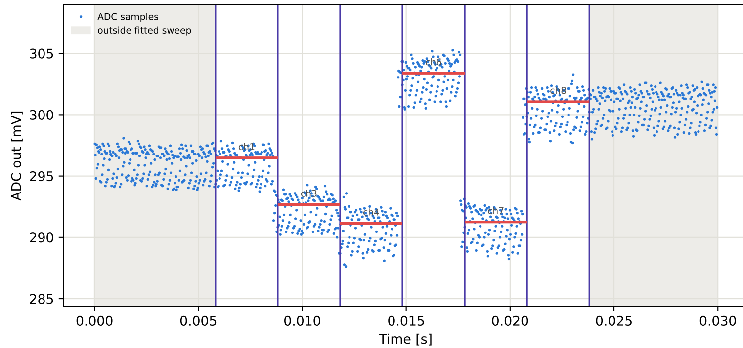
Tag3 &lt;- Tag16 | 985 MHz | run 0 | rep 1 | phase 15.66 deg
