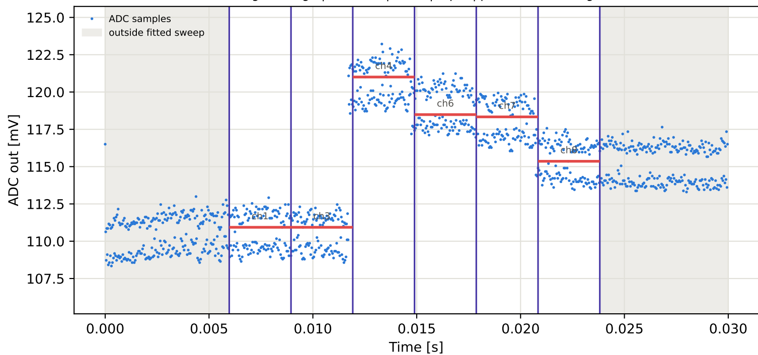
Tag6 &lt;- Tag5 | 825 MHz | run 0 | rep 1 | phase -115.65 deg
