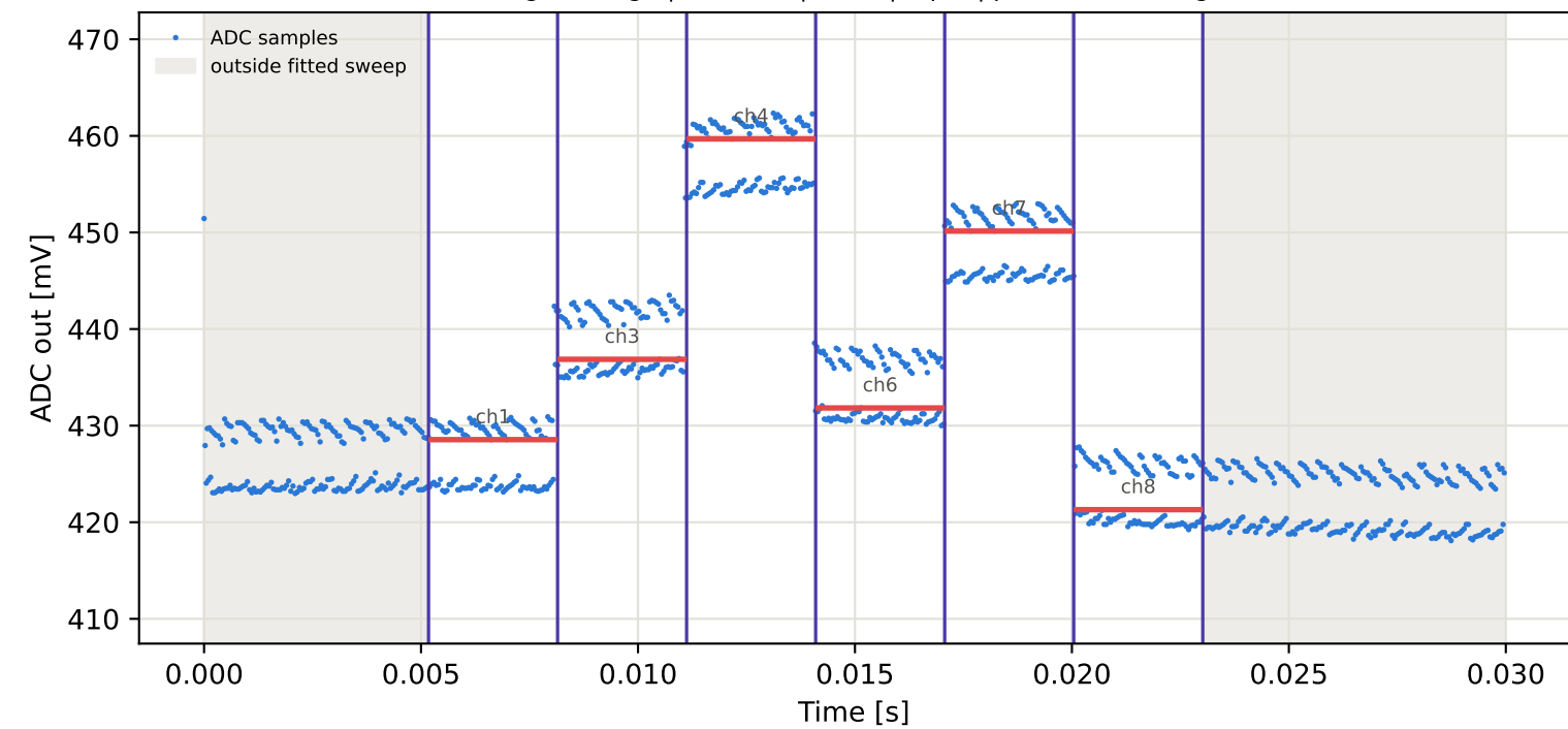
Tag8 &lt;- Tag10 | 965 MHz | run 0 | rep 1 | phase -169.23 deg
