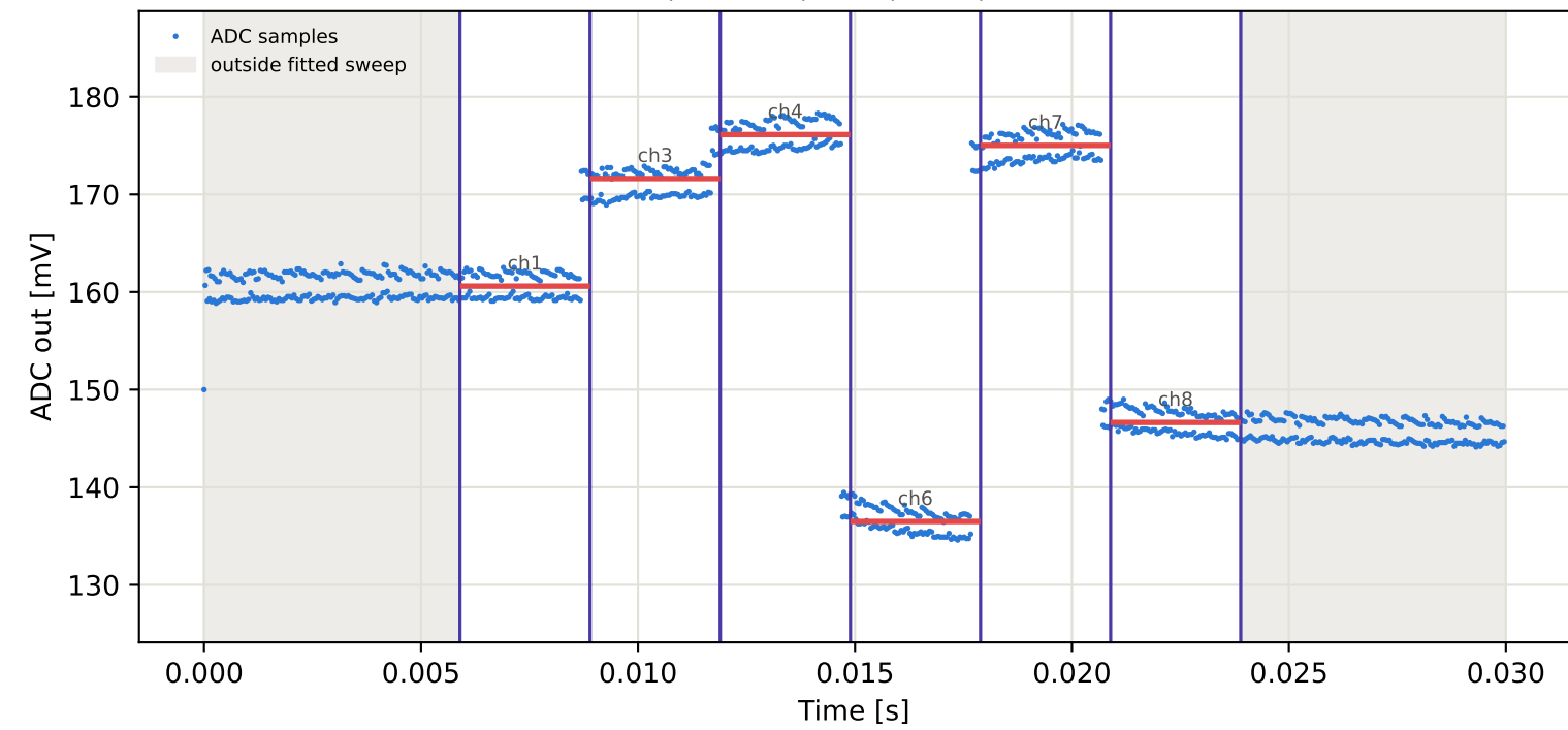
Tag9 &lt;- Tag8 | 955 MHz | run 0 | rep 1 | phase -25.74 deg
