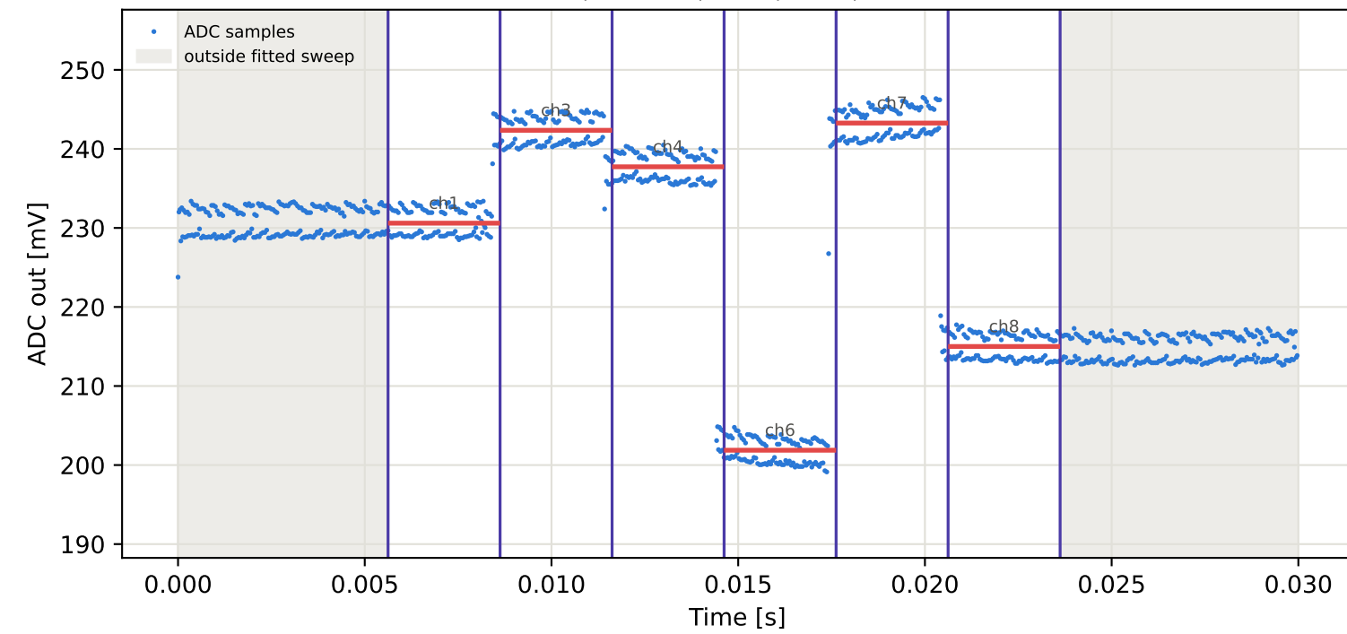
Tag9 &lt;- Tag16 | 975 MHz | run 0 | rep 1 | phase -13.53 deg
