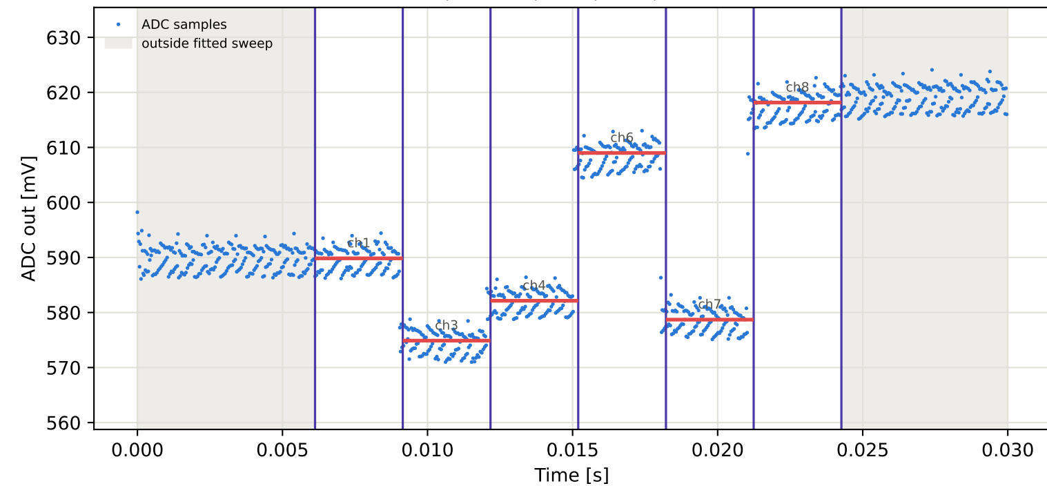
Tag5 &lt;- Tag3 | 865 MHz | run 0 | rep 1 | phase 165.14 deg
