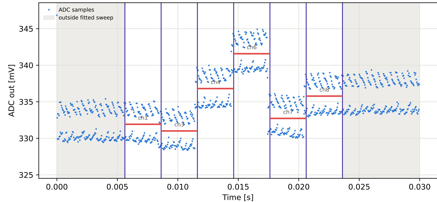
Tag16 &lt;- Tag7 | 985 MHz | run 0 | rep 1 | phase 147.89 deg
