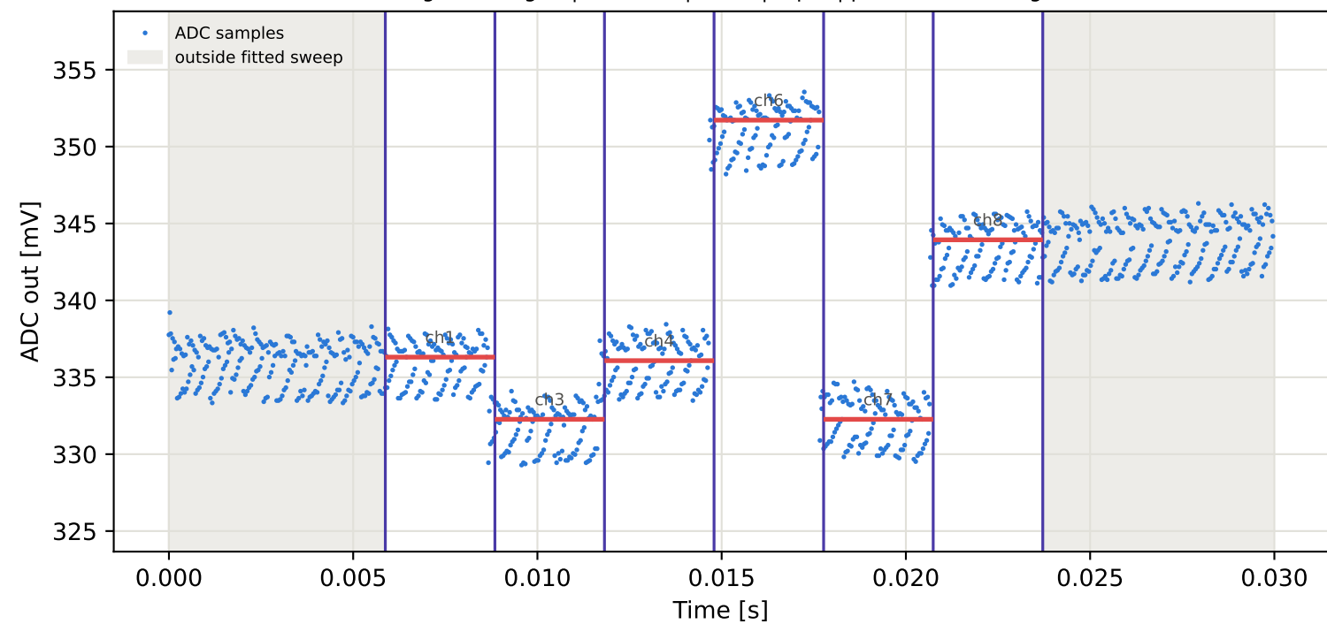
Tag16 &lt;- Tag10 | 985 MHz | run 0 | rep 1 | phase 177.55 deg
