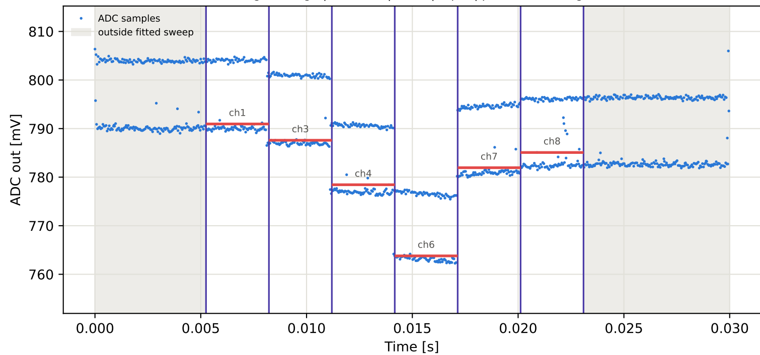
Tag8 &lt;- Tag5 | 915 MHz | run 0 | rep 1 | phase 62.81 deg
