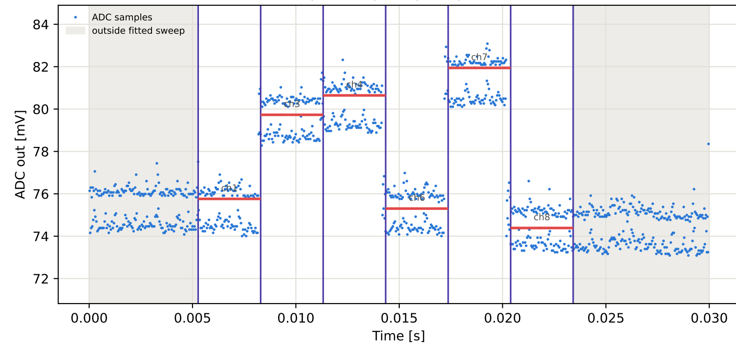
Tag8 &lt;- Tag6 | 785 MHz | run 0 | rep 1 | phase -39.57 deg
