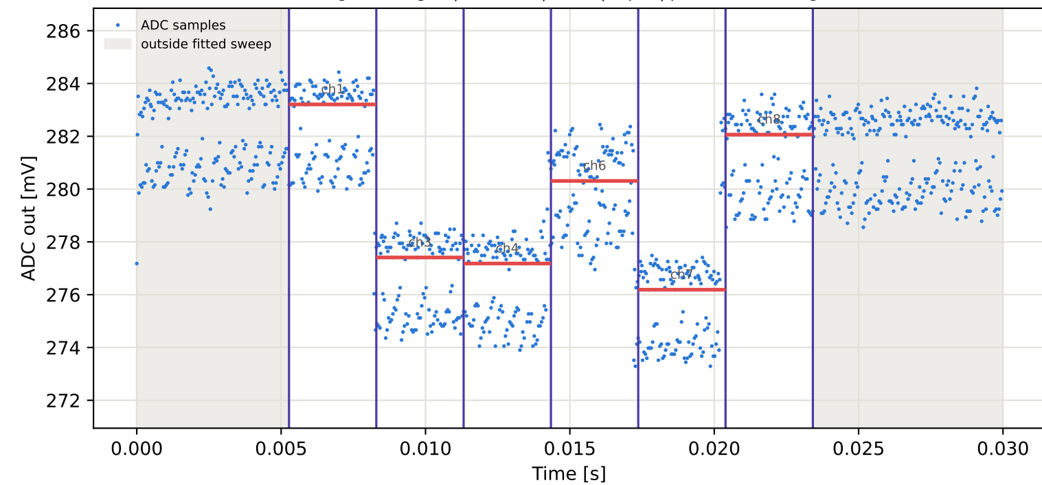
Tag10 &lt;- Tag2 | 845 MHz | run 0 | rep 1 | phase -108.41 deg
