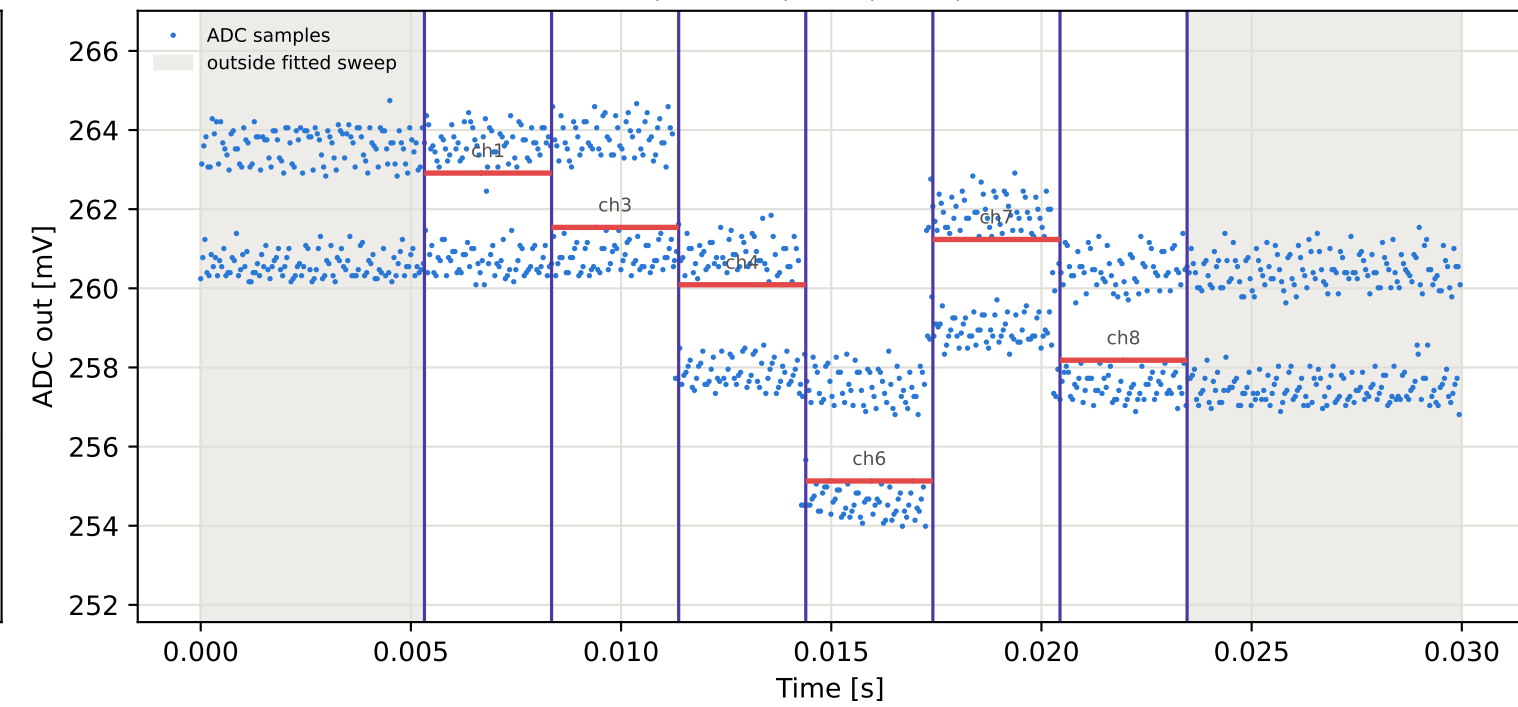
Tag3 &lt;- Tag2 | 825 MHz | run 0 | rep 1 | phase 25.72 deg
