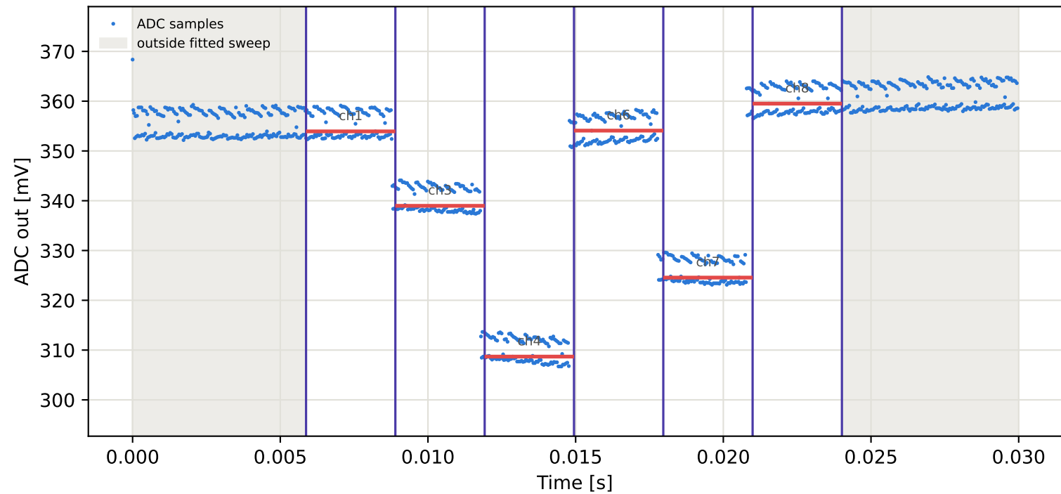
Tag5 &lt;- Tag1 | 985 MHz | run 0 | rep 1 | phase -74.39 deg
