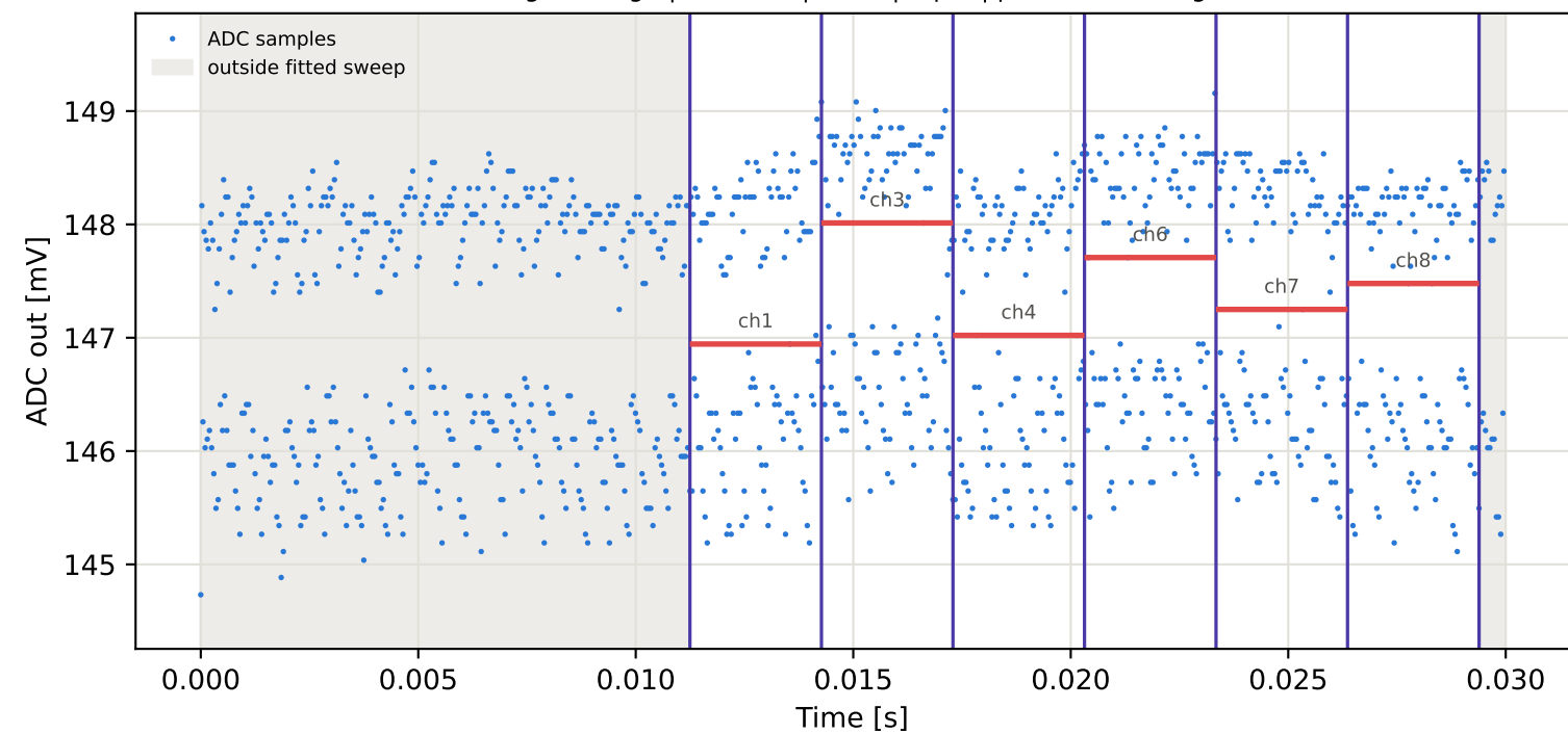
Tag9 &lt;- Tag2 | 895 MHz | run 0 | rep 1 | phase 94.43 deg
