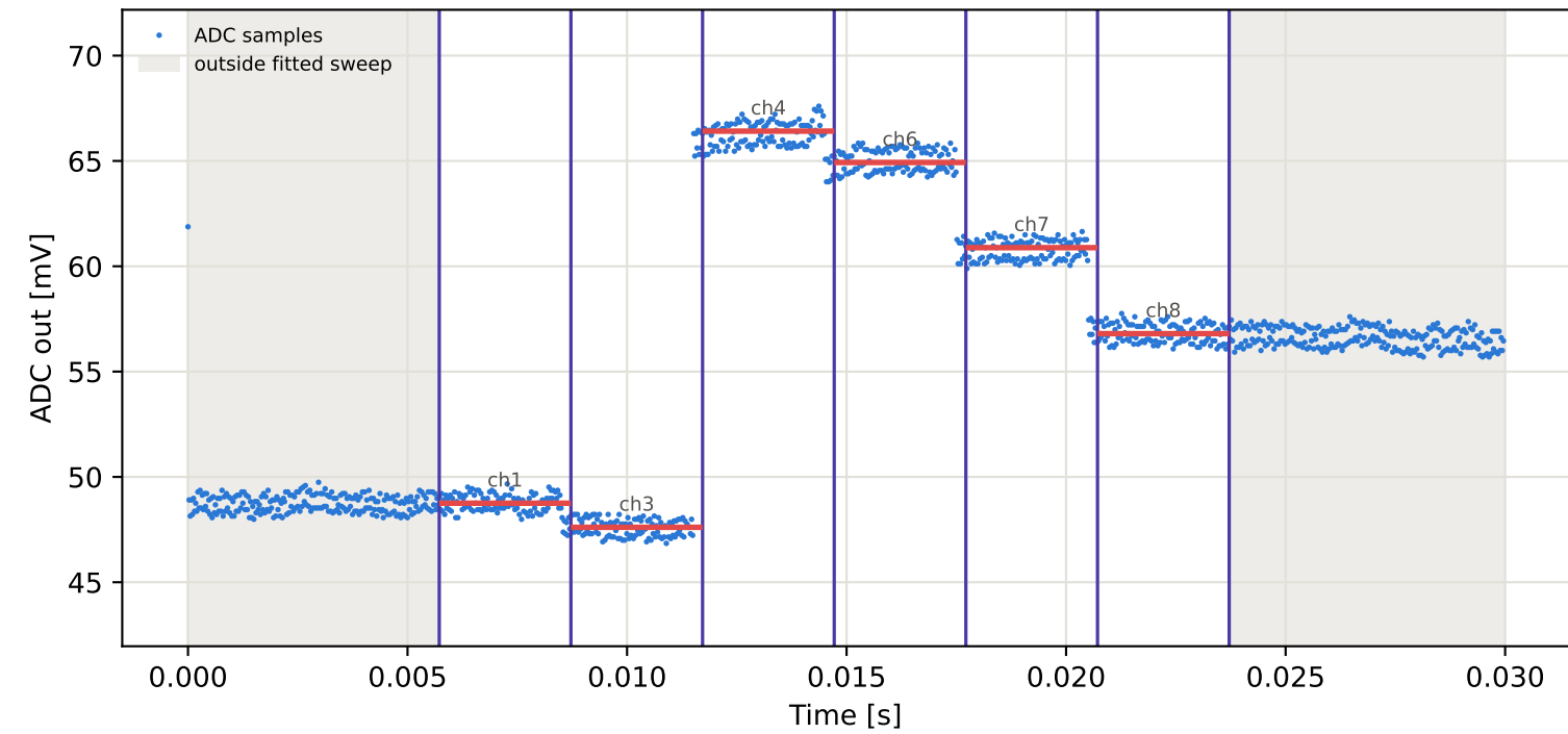
Tag16 &lt;- Tag7 | 785 MHz | run 0 | rep 1 | phase -83.70 deg
