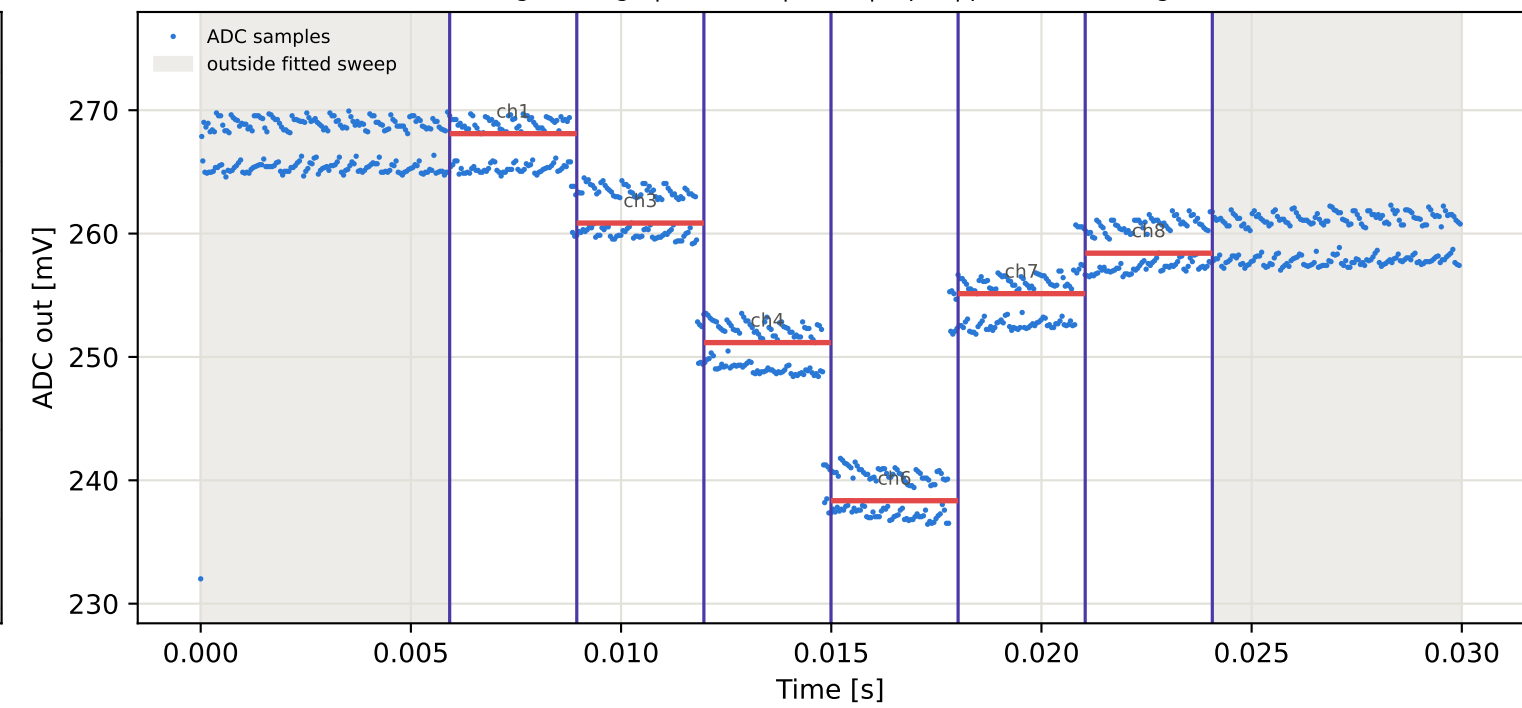
Tag9 &lt;- Tag6 | 905 MHz | run 0 | rep 1 | phase -11.91 deg
