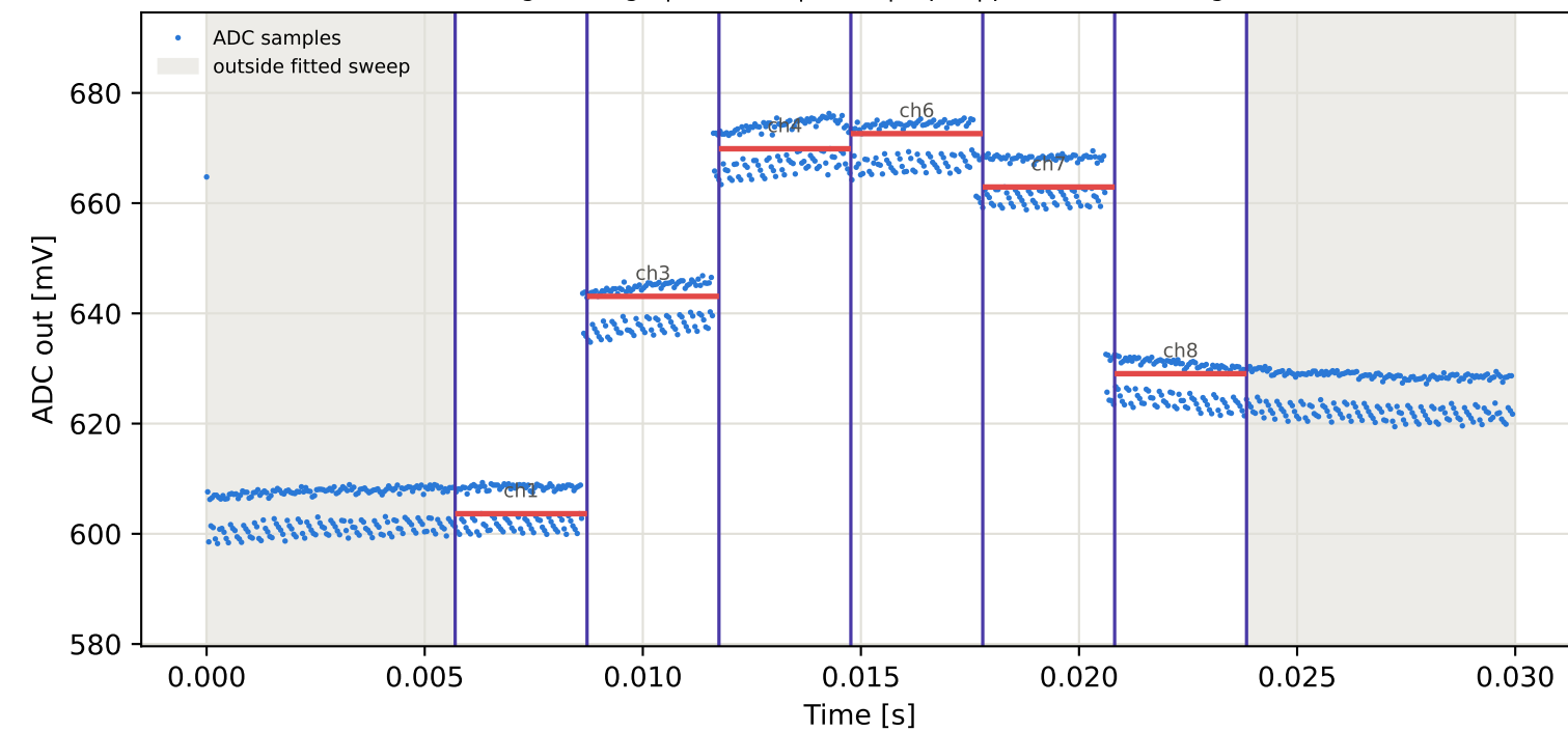
Tag3 &lt;- Tag6 | 875 MHz | run 0 | rep 1 | phase -132.31 deg
