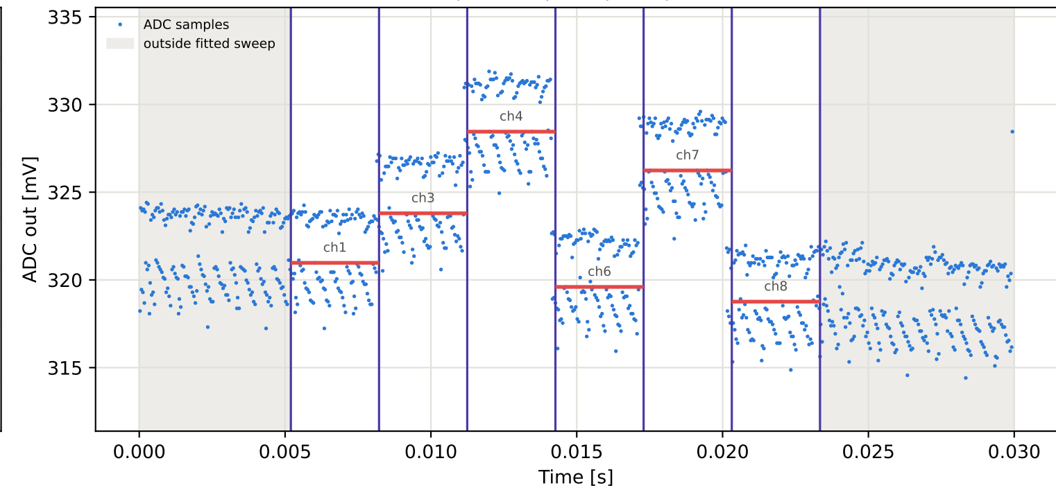
Tag10 &lt;- Tag5 | 965 MHz | run 0 | rep 1 | phase -71.96 deg
