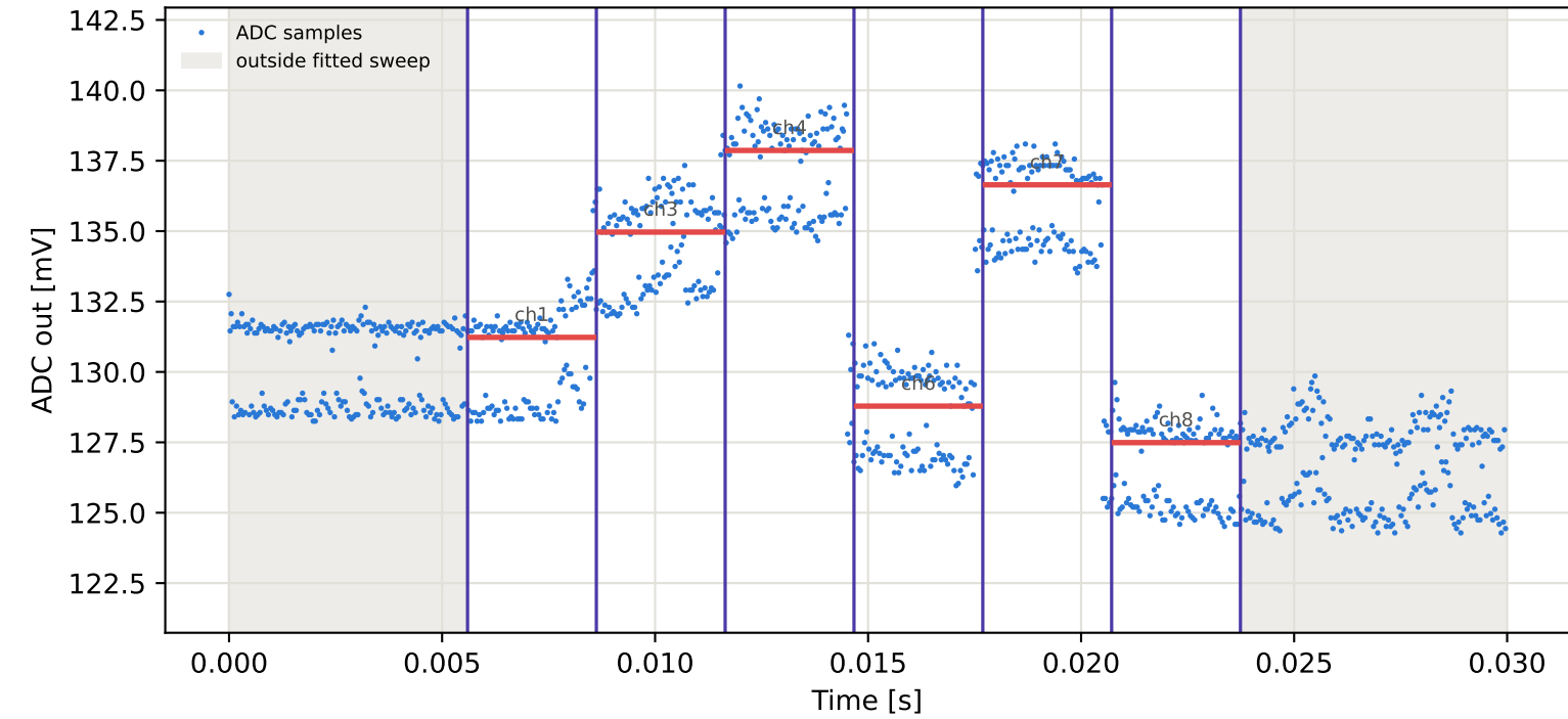
Tag2 &lt;- Tag15 | 925 MHz | run 0 | rep 1 | phase -86.59 deg
