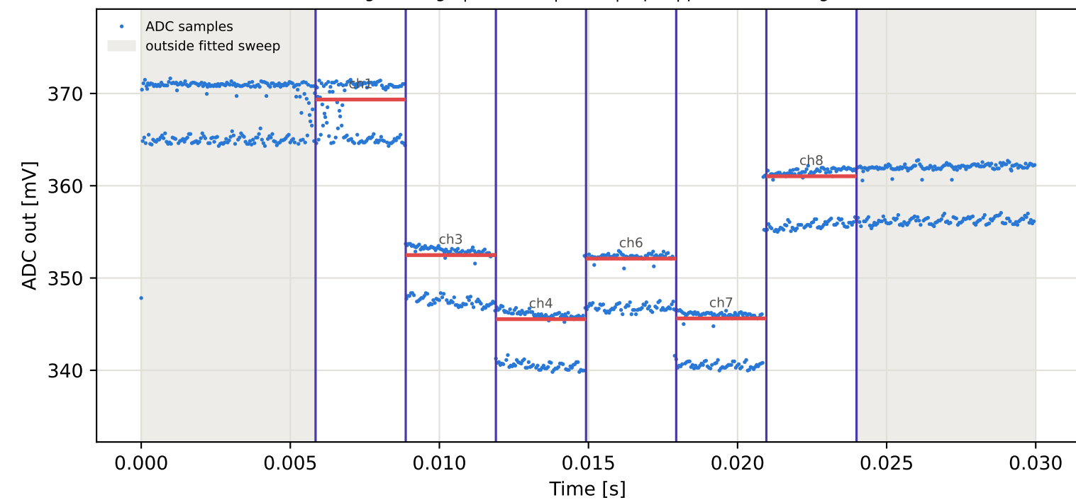
Tag5 &lt;- Tag3 | 845 MHz | run 0 | rep 1 | phase 86.62 deg
