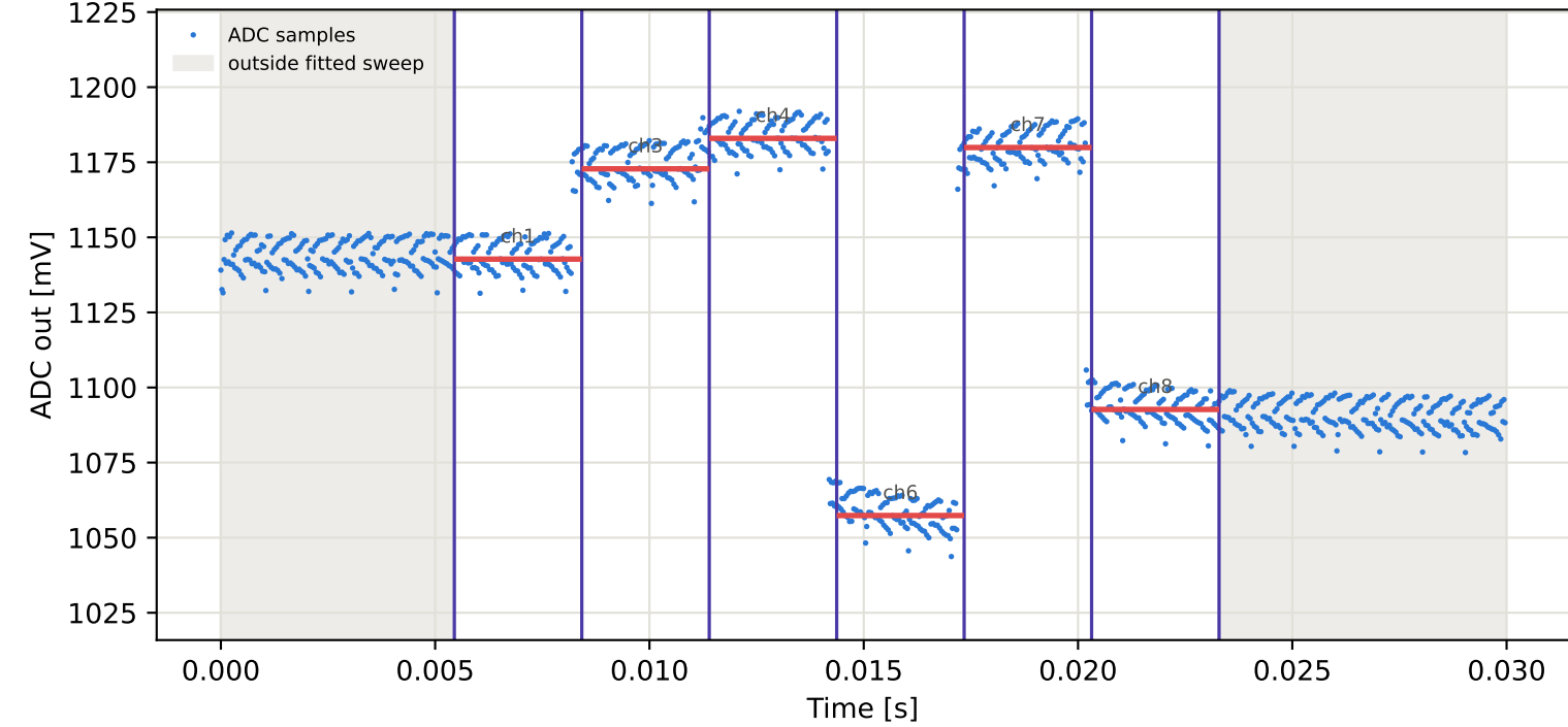
Tag15 &lt;- Tag6 | 935 MHz | run 0 | rep 1 | phase 7.53 deg
