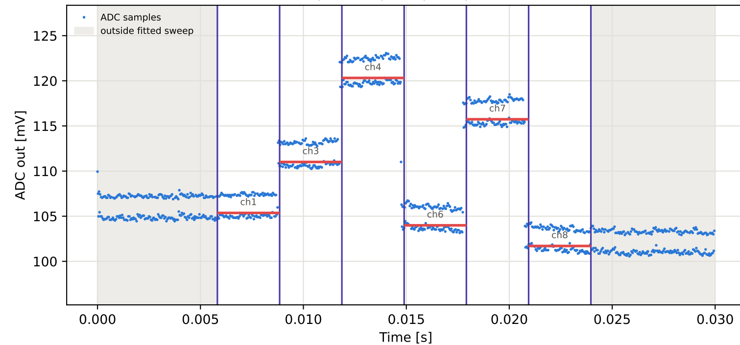
Tag1 &lt;- Tag3 | 975 MHz | run 0 | rep 1 | phase -76.63 deg
