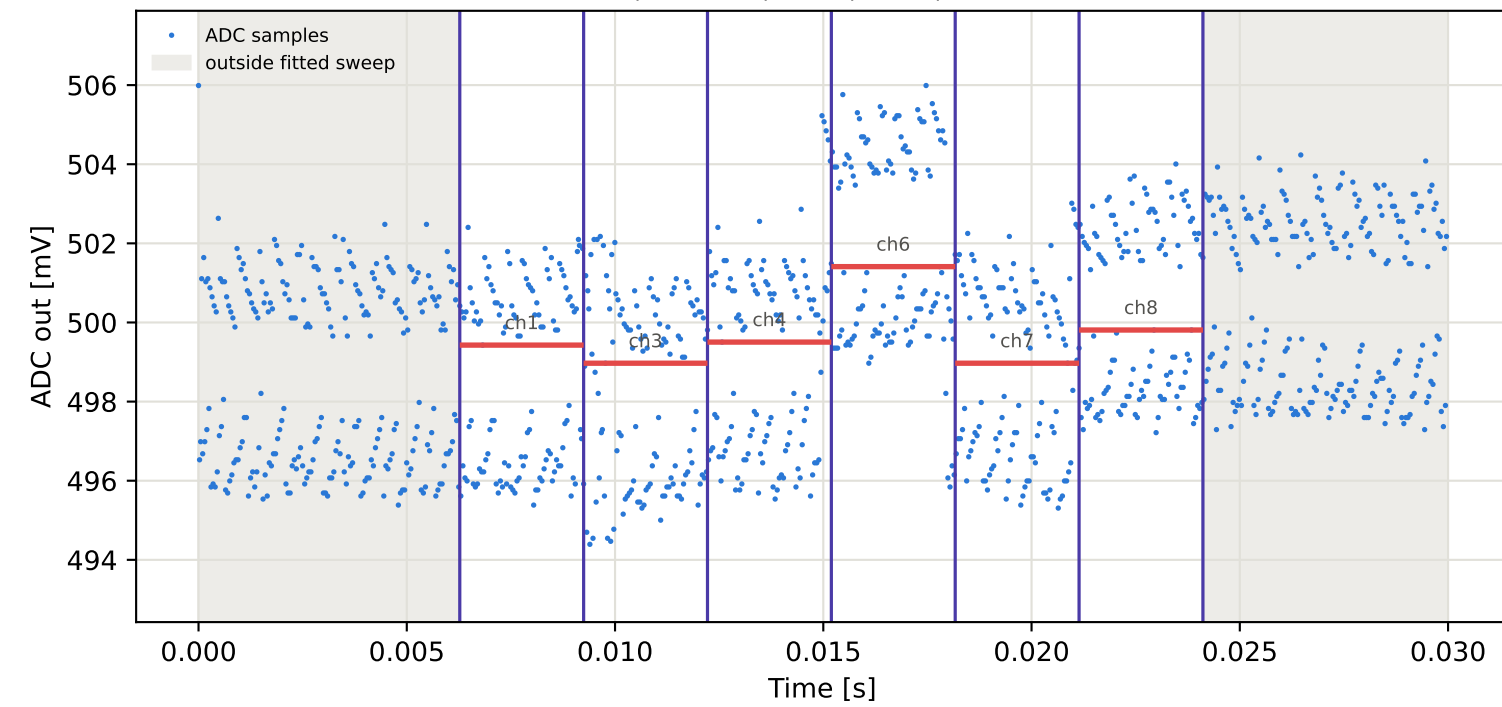
Tag4 &lt;- Tag2 | 865 MHz | run 0 | rep 1 | phase -166.62 deg
