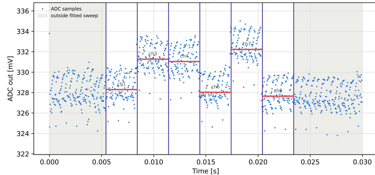
Tag5 &lt;- Tag3 | 805 MHz | run 0 | rep 1 | phase -34.27 deg
