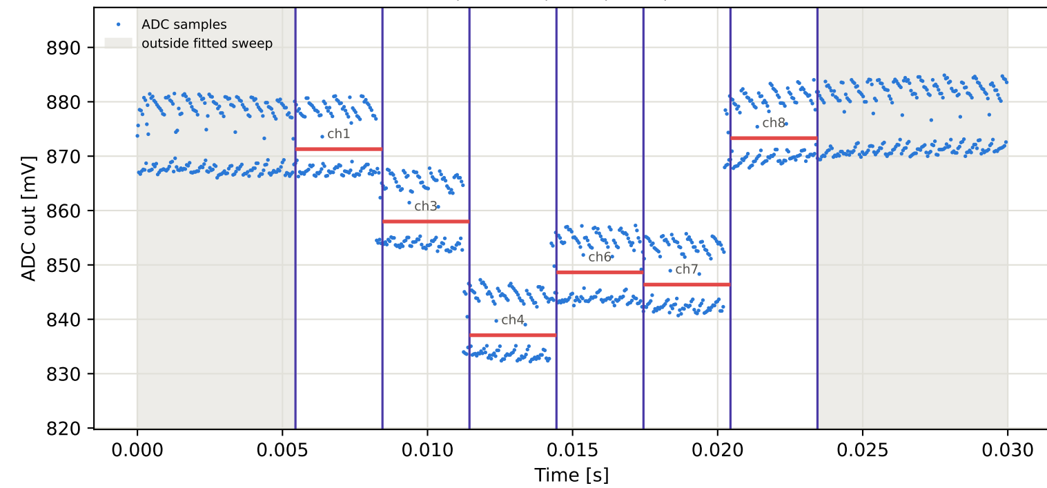
Tag7 &lt;- Tag10 | 925 MHz | run 0 | rep 1 | phase 74.18 deg
