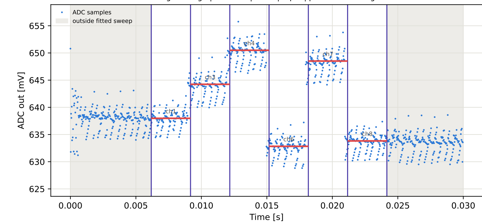
Tag8 &lt;- Tag6 | 985 MHz | run 0 | rep 1 | phase -58.13 deg
