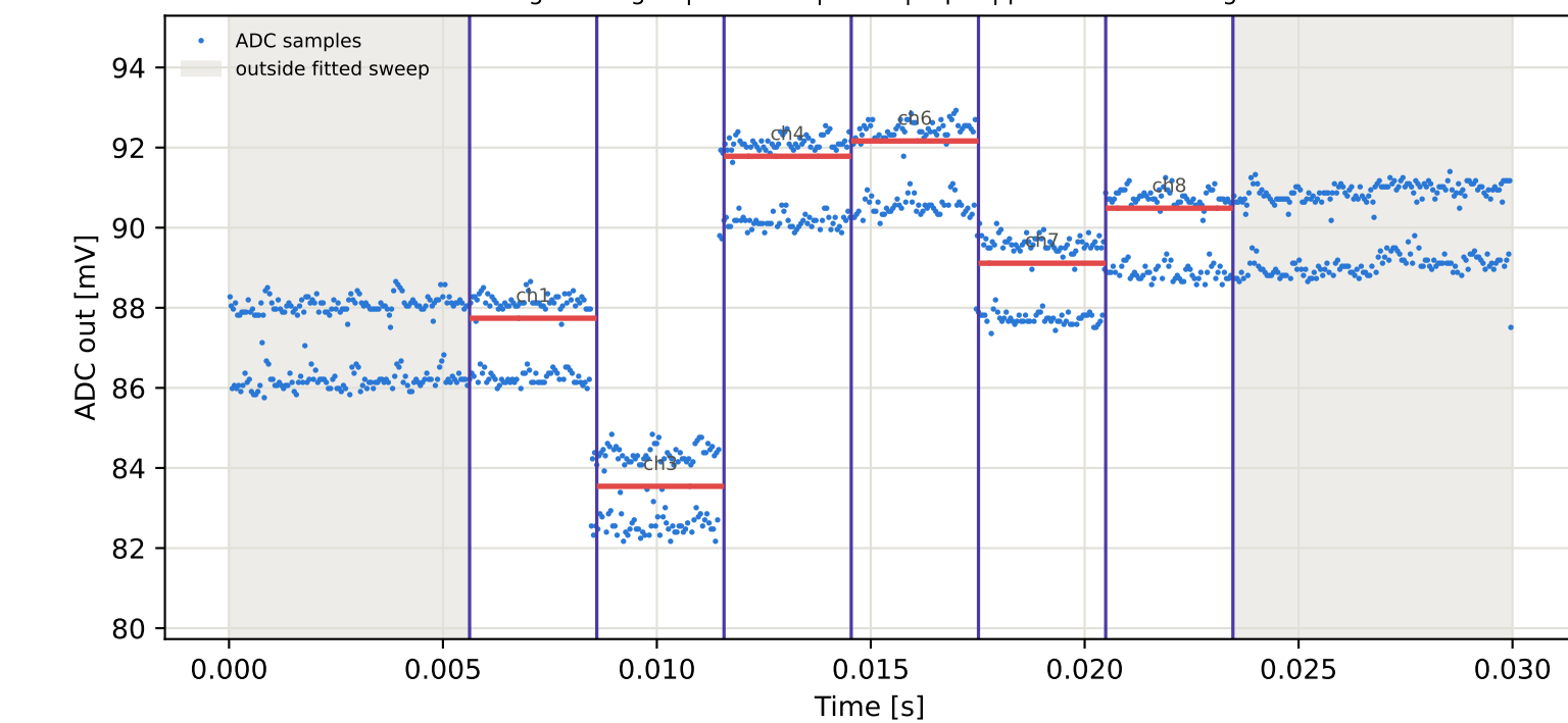
Tag9 &lt;- Tag16 | 795 MHz | run 0 | rep 1 | phase 84.18 deg
