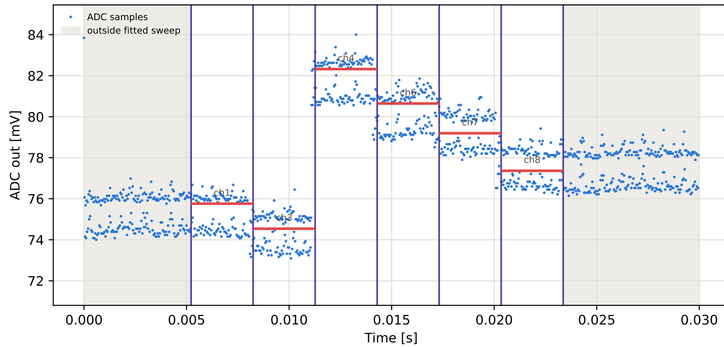
Tag9 &lt;- Tag10 | 785 MHz | run 0 | rep 1 | phase -159.27 deg
