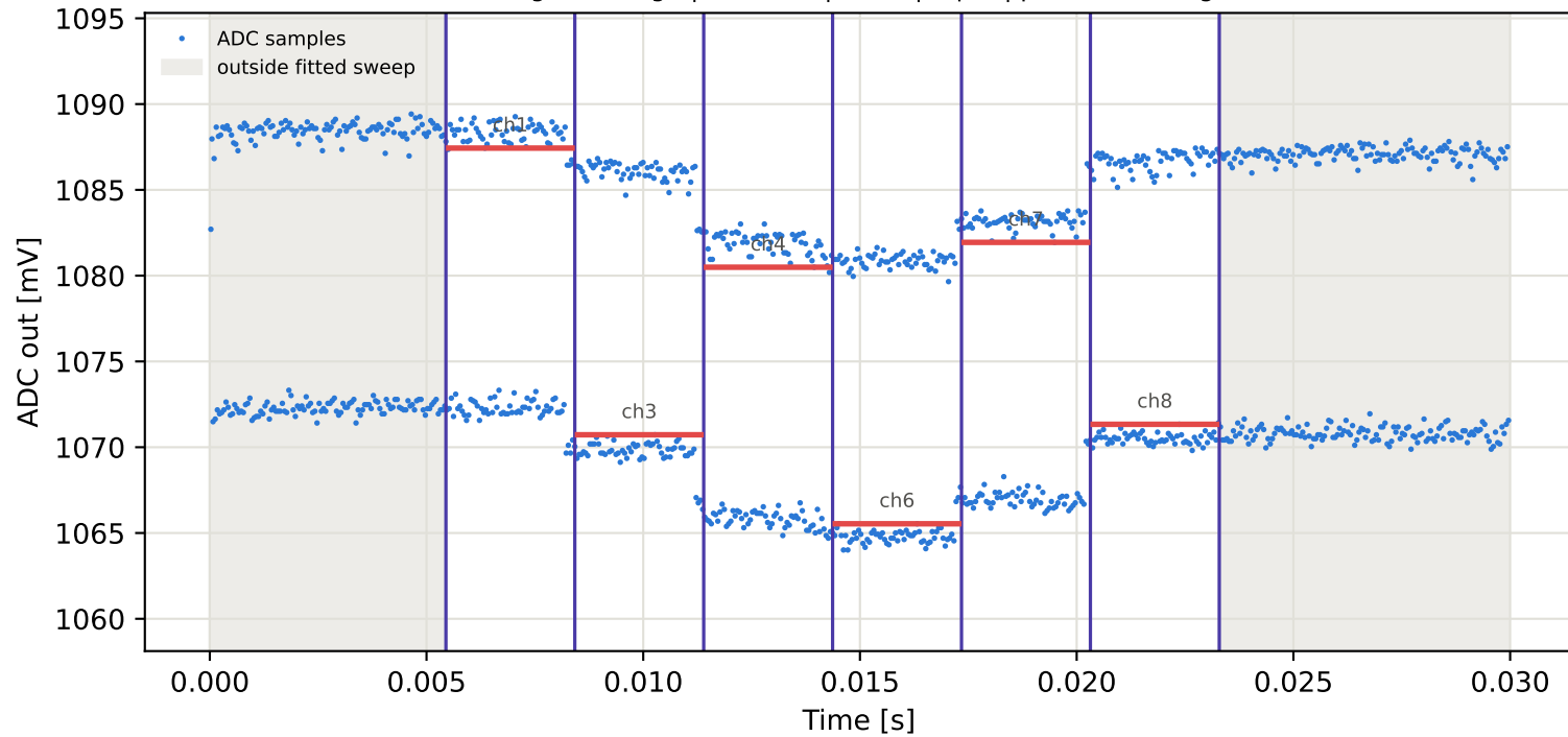
Tag16 &lt;- Tag15 | 905 MHz | run 0 | rep 1 | phase -116.70 deg
