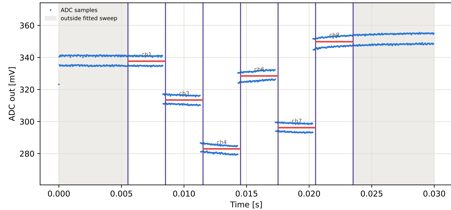
Tag3 &lt;- Tag2 | 945 MHz | run 0 | rep 1 | phase -140.25 deg
