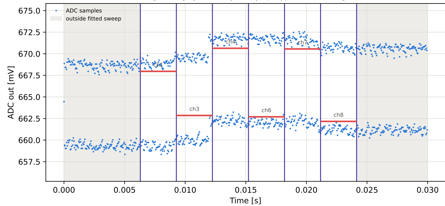
Tag8 &lt;- Tag5 | 835 MHz | run 0 | rep 1 | phase -4.91 deg
