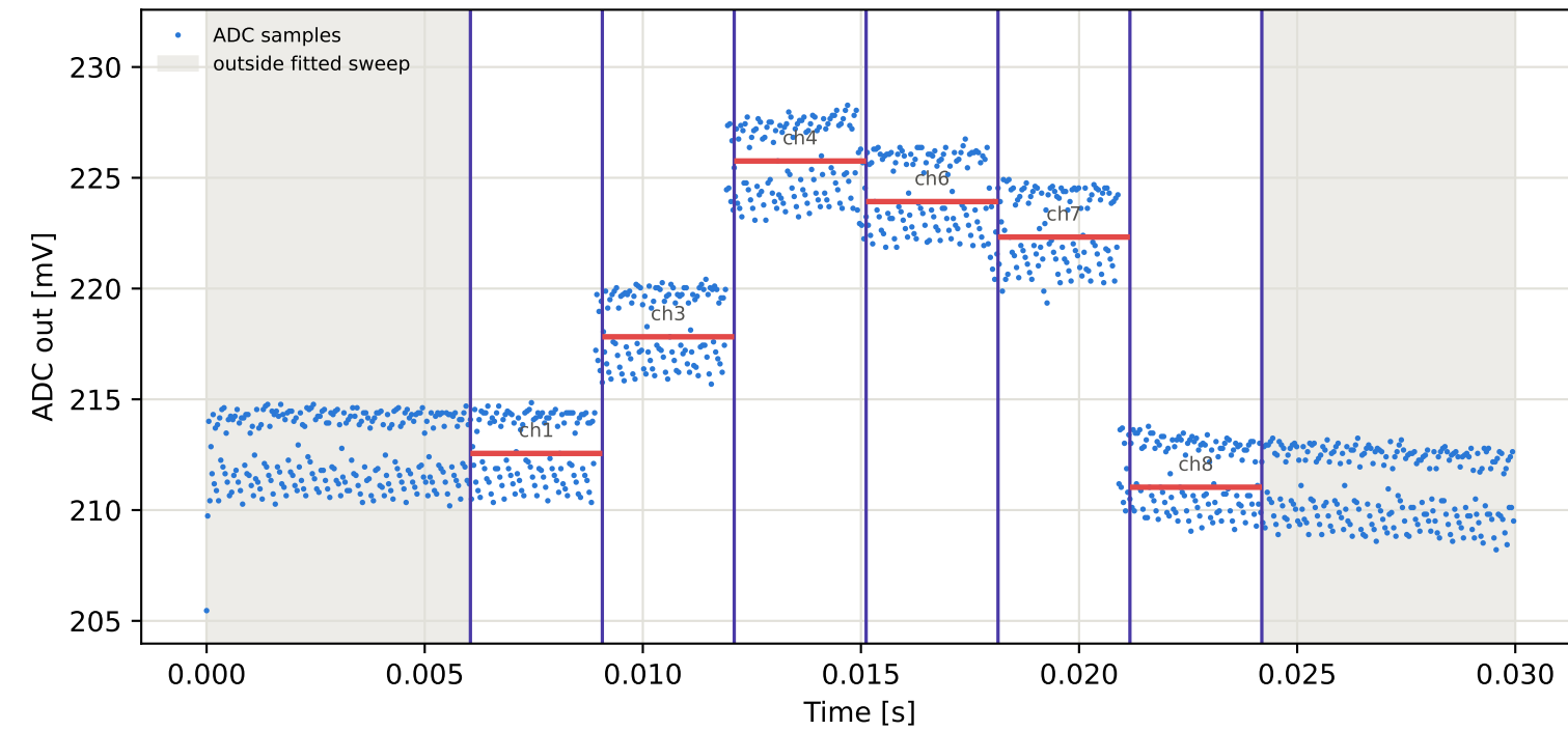
Tag1 &lt;- Tag3 | 915 MHz | run 0 | rep 1 | phase -179.17 deg
