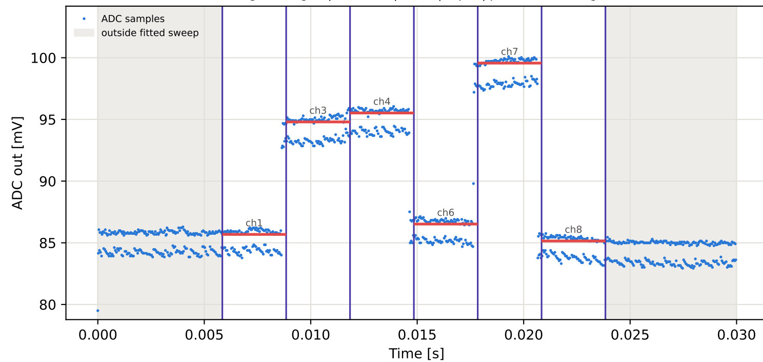
Tag7 &lt;- Tag3 | 795 MHz | run 0 | rep 1 | phase -122.73 deg
