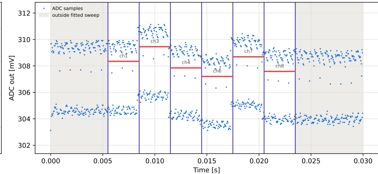
Tag7 &lt;- Tag15 | 825 MHz | run 0 | rep 1 | phase -56.63 deg
