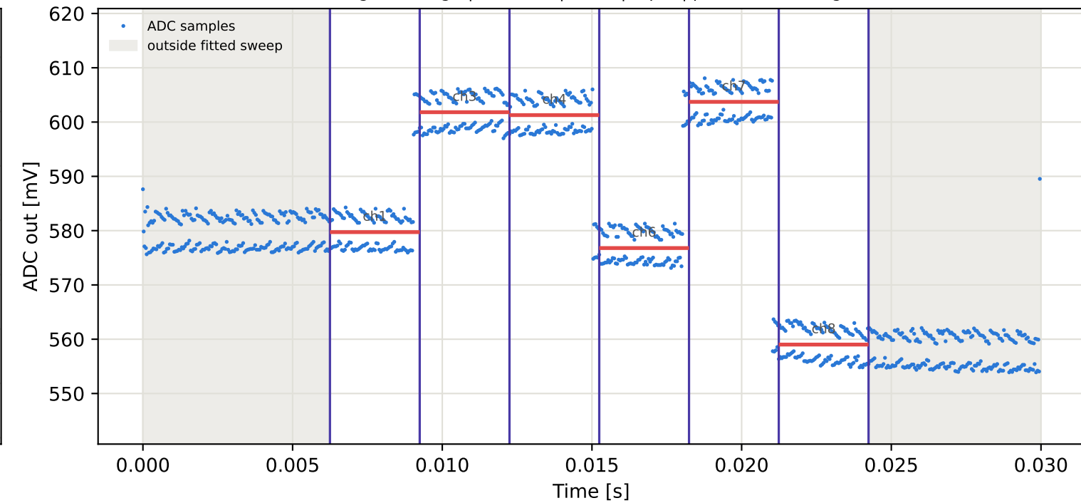
Tag16 &lt;- Tag5 | 865 MHz | run 0 | rep 1 | phase -129.84 deg
