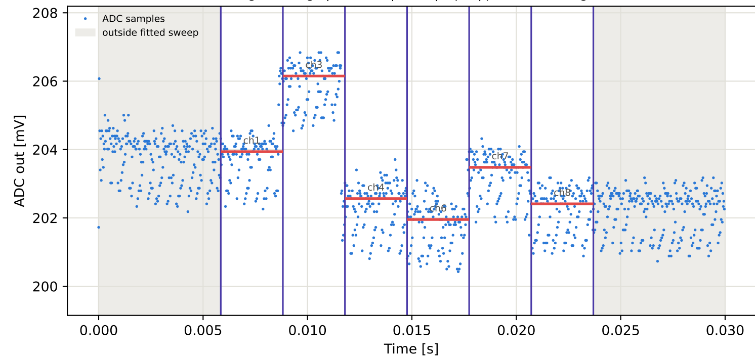
Tag15 &lt;- Tag6 | 805 MHz | run 0 | rep 1 | phase -173.34 deg
