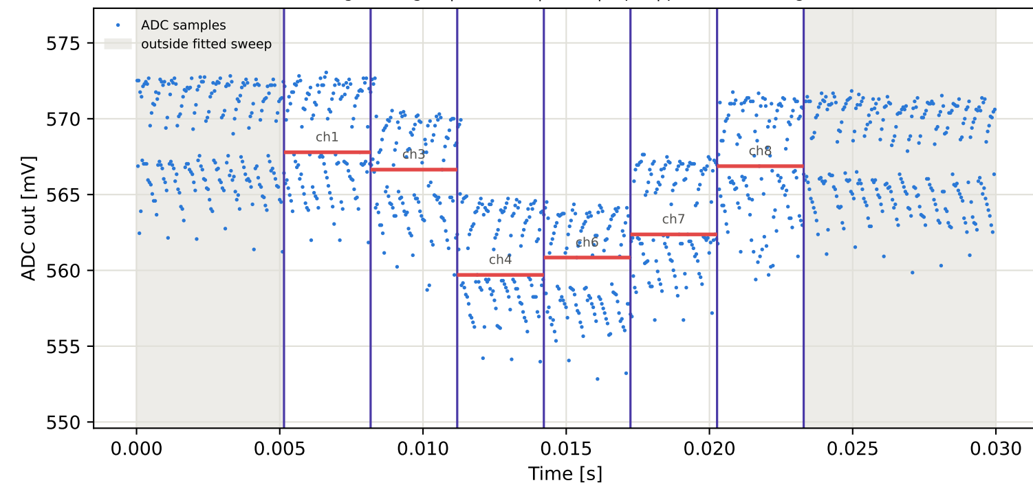
Tag5 &lt;- Tag16 | 935 MHz | run 0 | rep 1 | phase -89.46 deg
