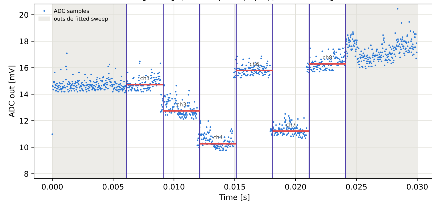
Tag2 &lt;- Tag5 | 955 MHz | run 0 | rep 1 | phase -87.28 deg
