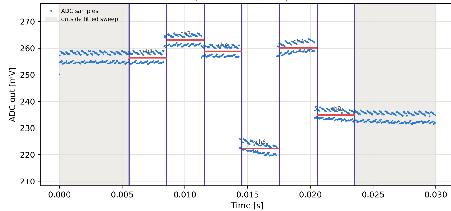
Tag9 &lt;- Tag5 | 905 MHz | run 0 | rep 1 | phase -121.45 deg
