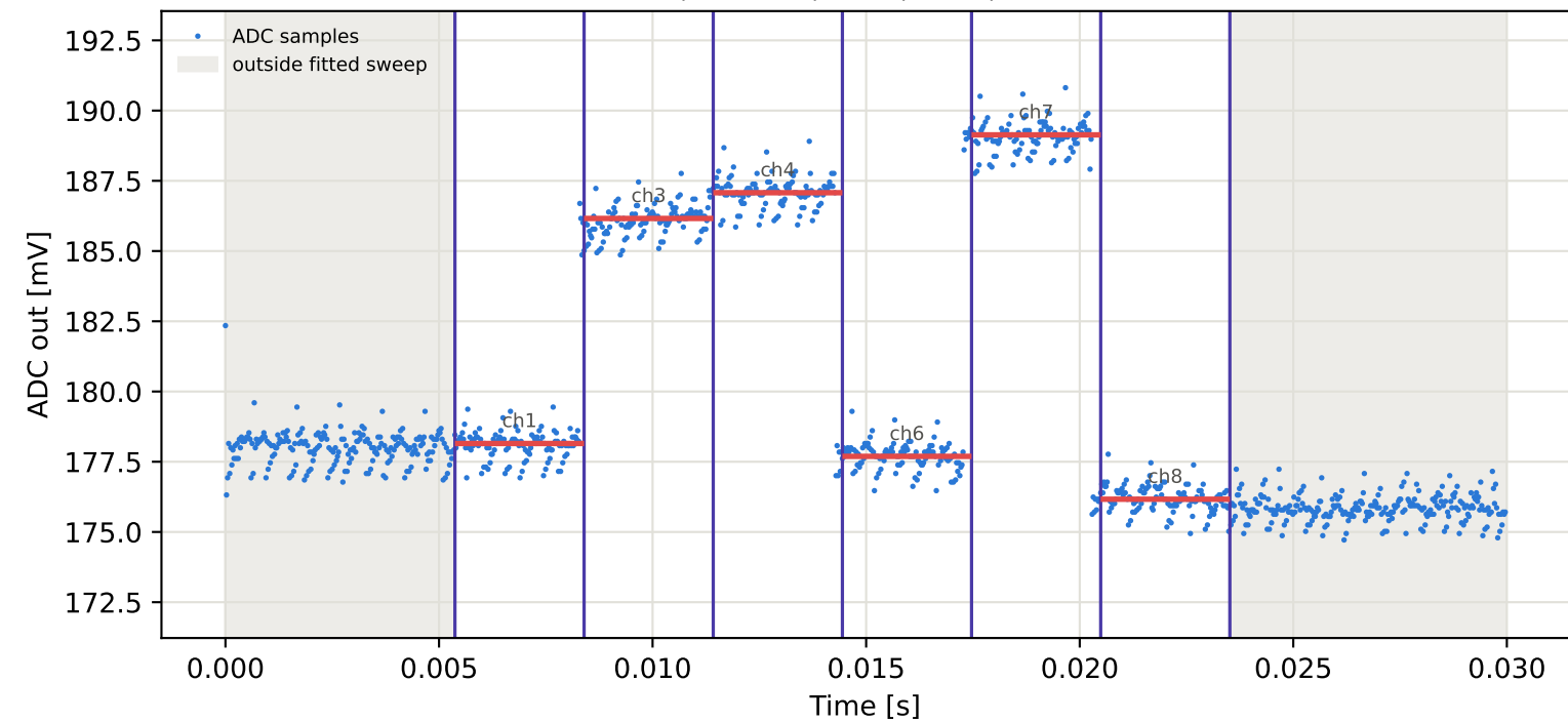
Tag7 &lt;- Tag6 | 805 MHz | run 0 | rep 1 | phase -40.58 deg
