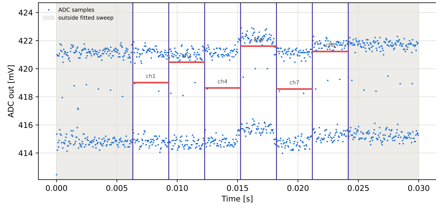
Tag5 &lt;- Tag4 | 855 MHz | run 0 | rep 1 | phase 36.20 deg
