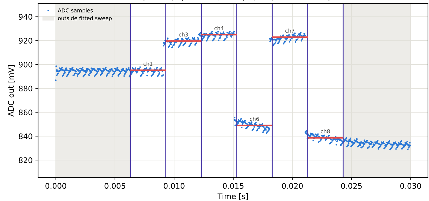
Tag5 &lt;- Tag1 | 905 MHz | run 0 | rep 1 | phase -174.04 deg
