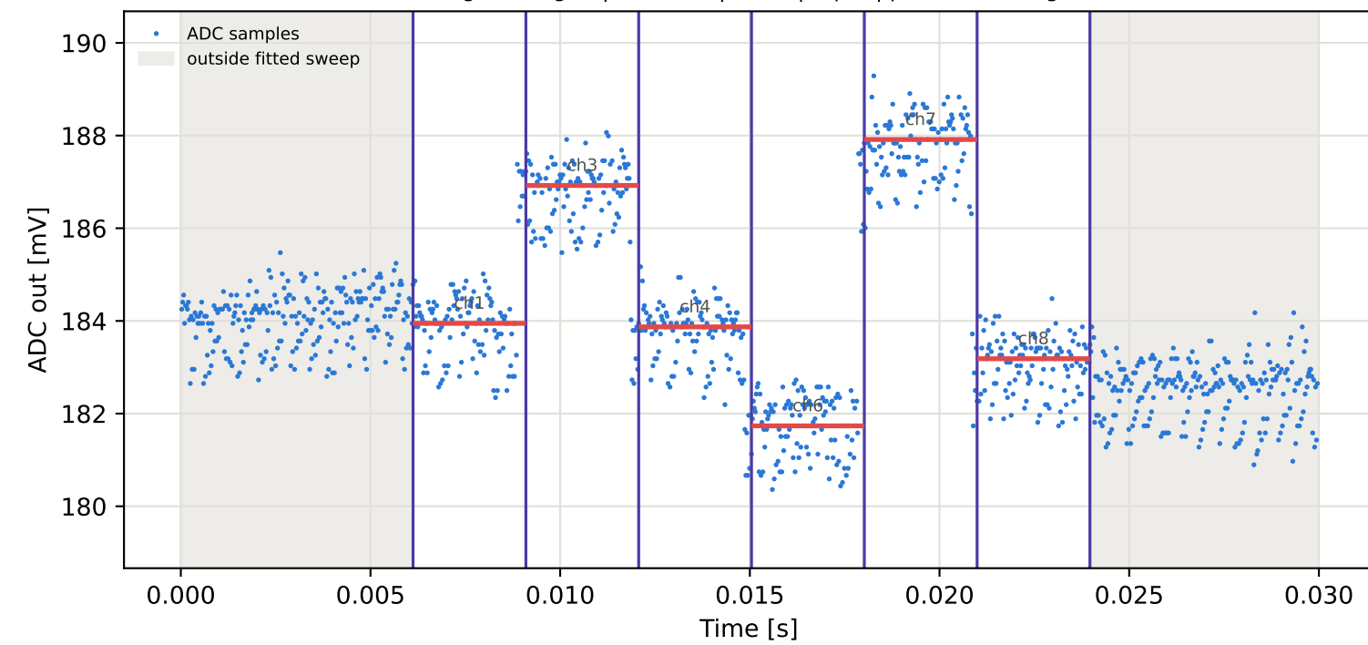
Tag5 &lt;- Tag3 | 775 MHz | run 0 | rep 1 | phase -62.13 deg
