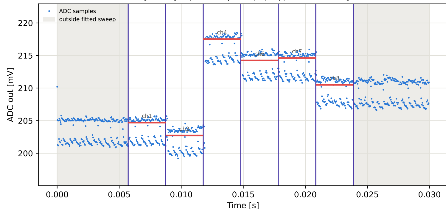
Tag6 &lt;- Tag10 | 805 MHz | run 0 | rep 1 | phase -113.14 deg
