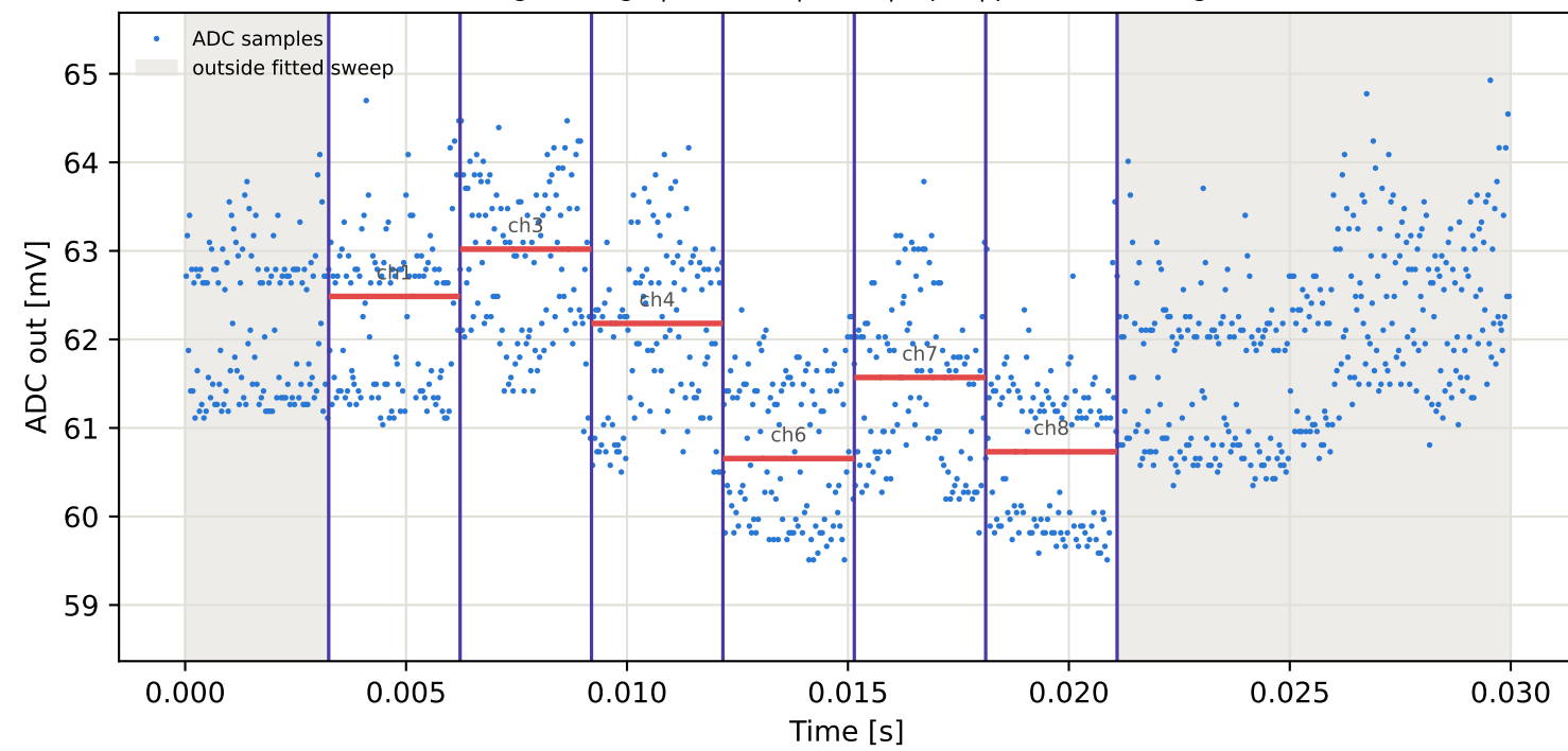
Tag3 &lt;- Tag10 | 835 MHz | run 0 | rep 1 | phase 153.09 deg
