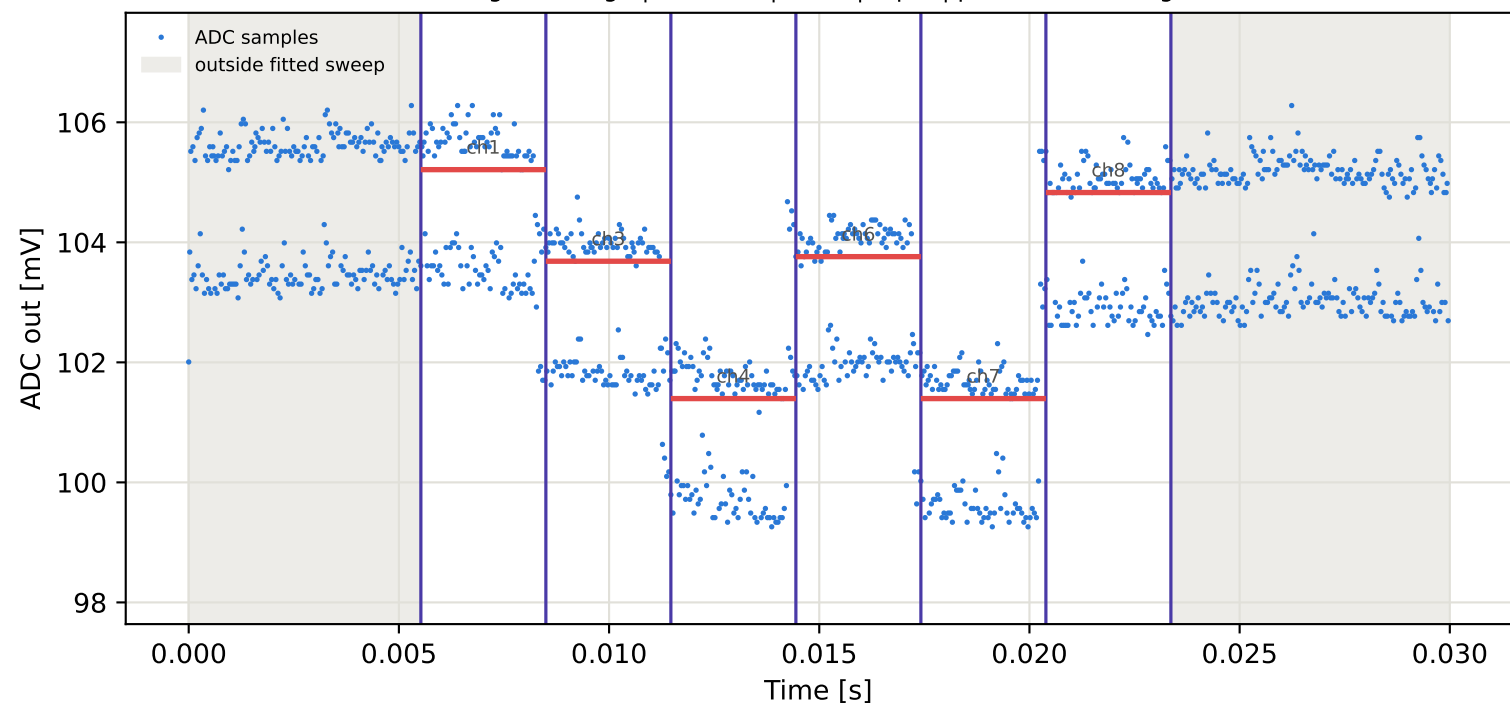
Tag15 &lt;- Tag6 | 785 MHz | run 0 | rep 1 | phase 103.84 deg
