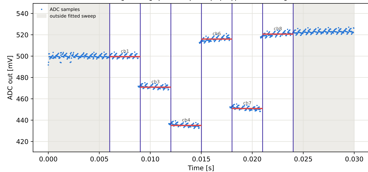
Tag10 &lt;- Tag8 | 945 MHz | run 0 | rep 1 | phase -60.36 deg
