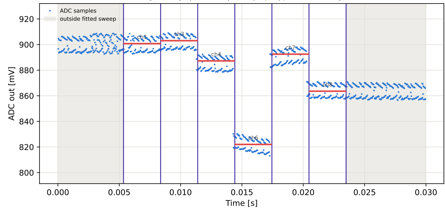
Tag4 &lt;- Tag8 | 905 MHz | run 0 | rep 1 | phase -26.39 deg
