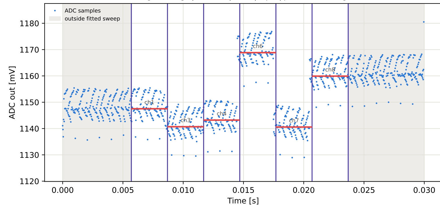
Tag15 &lt;- Tag9 | 935 MHz | run 0 | rep 1 | phase -147.73 deg
