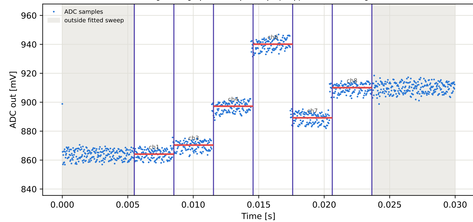
Tag5 &lt;- Tag3 | 885 MHz | run 0 | rep 1 | phase -153.34 deg
