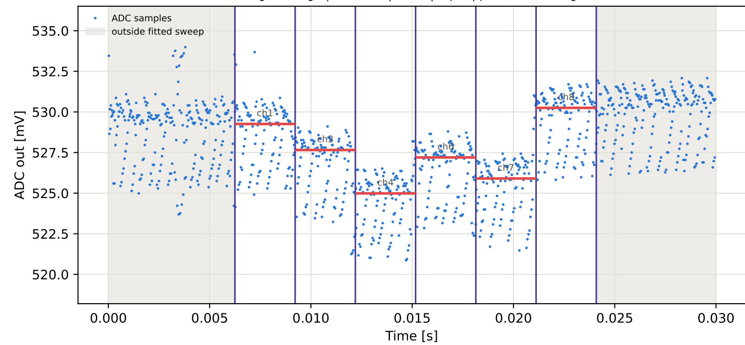
Tag9 &lt;- Tag2 | 915 MHz | run 0 | rep 1 | phase 82.19 deg
