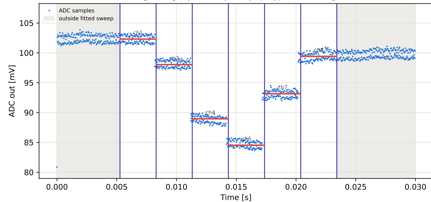
Tag3 &lt;- Tag16 | 925 MHz | run 0 | rep 1 | phase -0.54 deg
