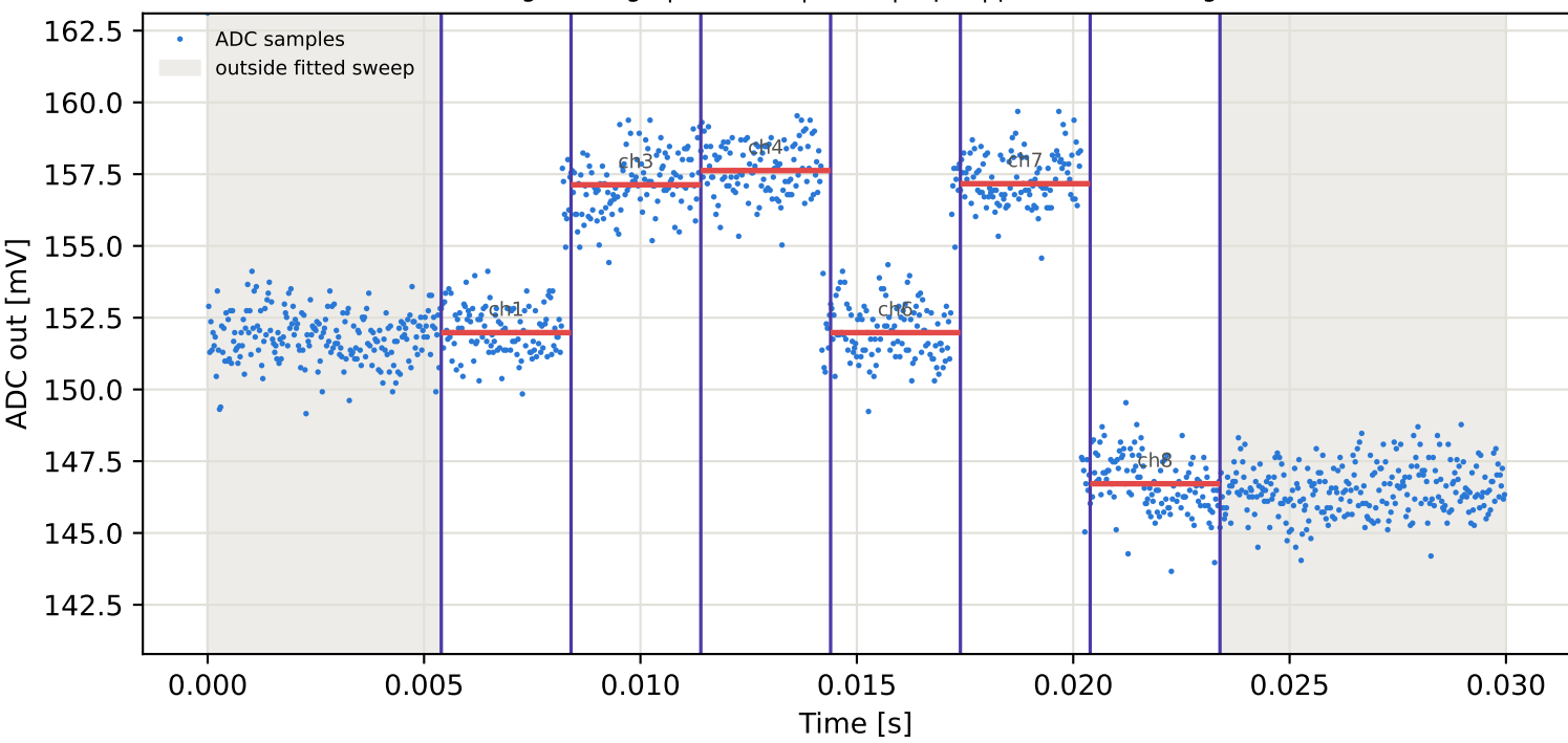
Tag2 &lt;- Tag8 | 885 MHz | run 0 | rep 1 | phase -52.04 deg
