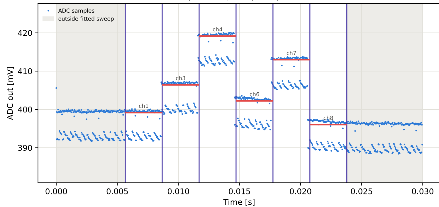
Tag4 &lt;- Tag16 | 955 MHz | run 0 | rep 1 | phase -4.18 deg
