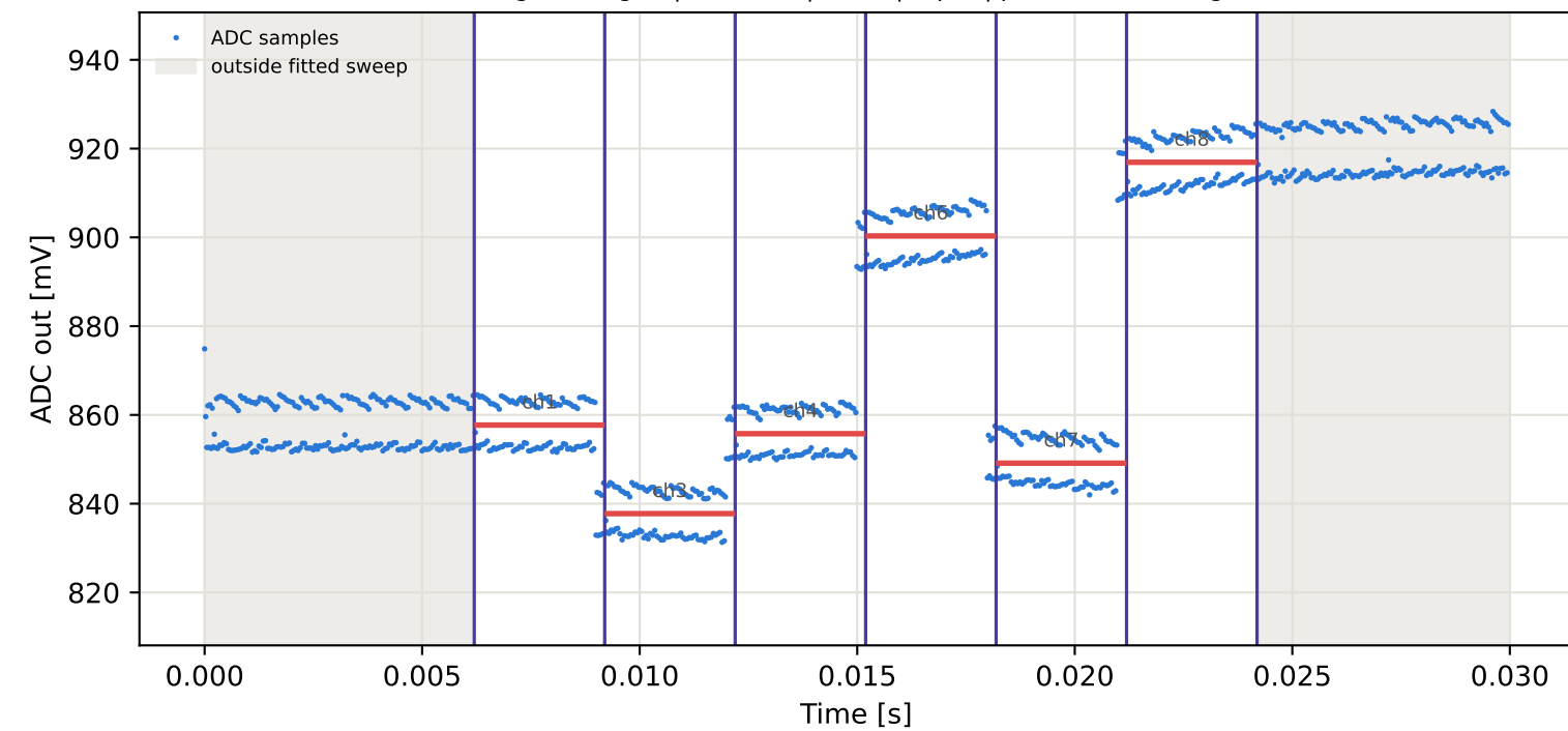
Tag6 &lt;- Tag3 | 875 MHz | run 0 | rep 1 | phase -112.63 deg
