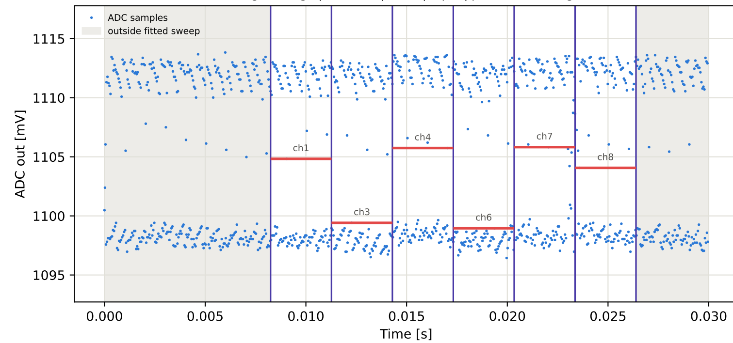
Tag8 &lt;- Tag4 | 895 MHz | run 0 | rep 1 | phase -37.71 deg
