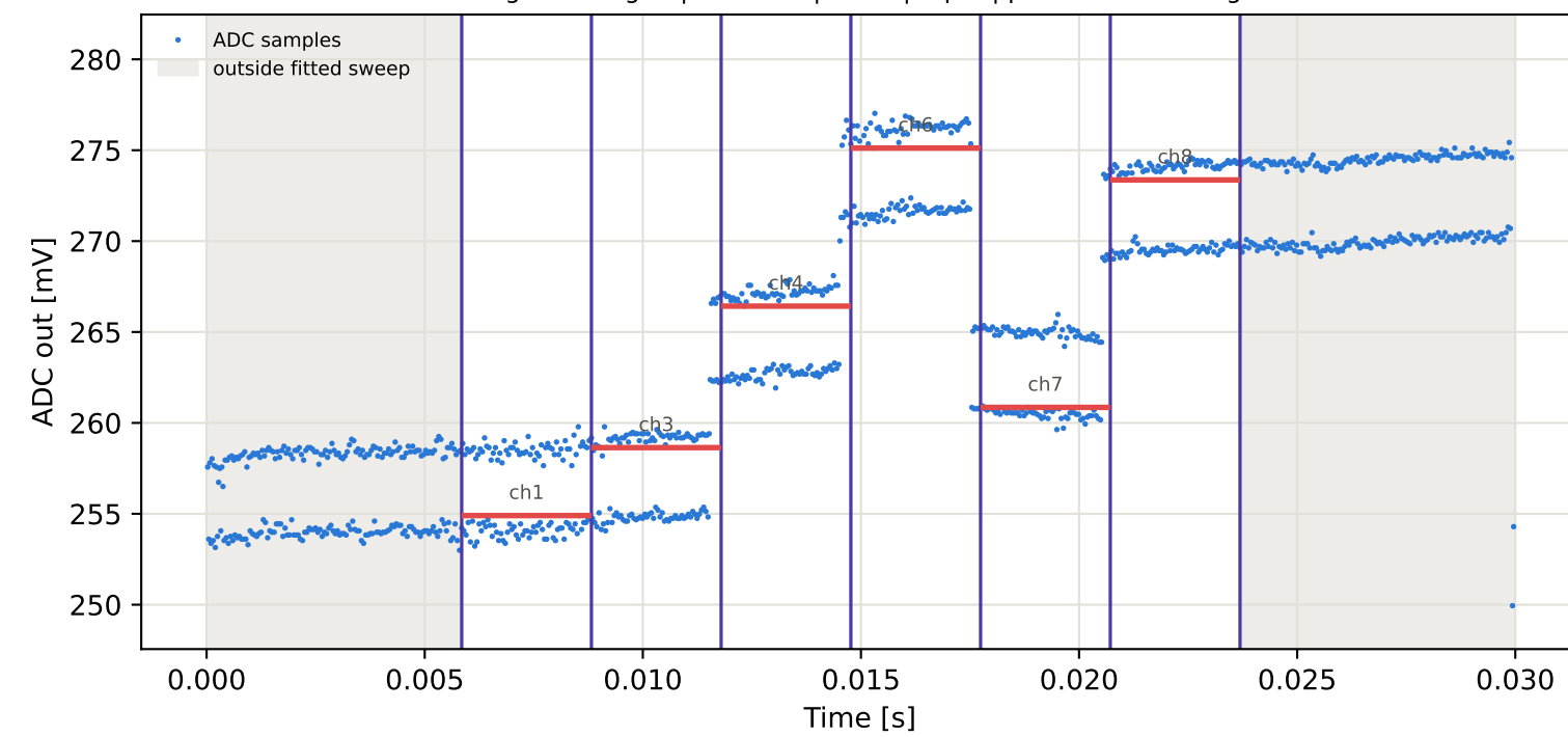
Tag10 &lt;- Tag2 | 875 MHz | run 0 | rep 1 | phase 86.84 deg
