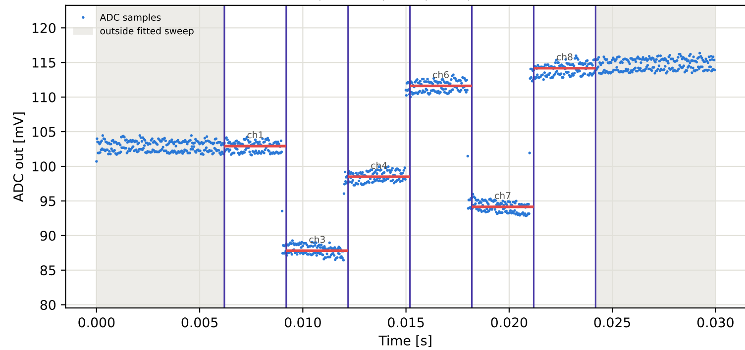
Tag10 &lt;- Tag1 | 855 MHz | run 0 | rep 1 | phase 174.31 deg
