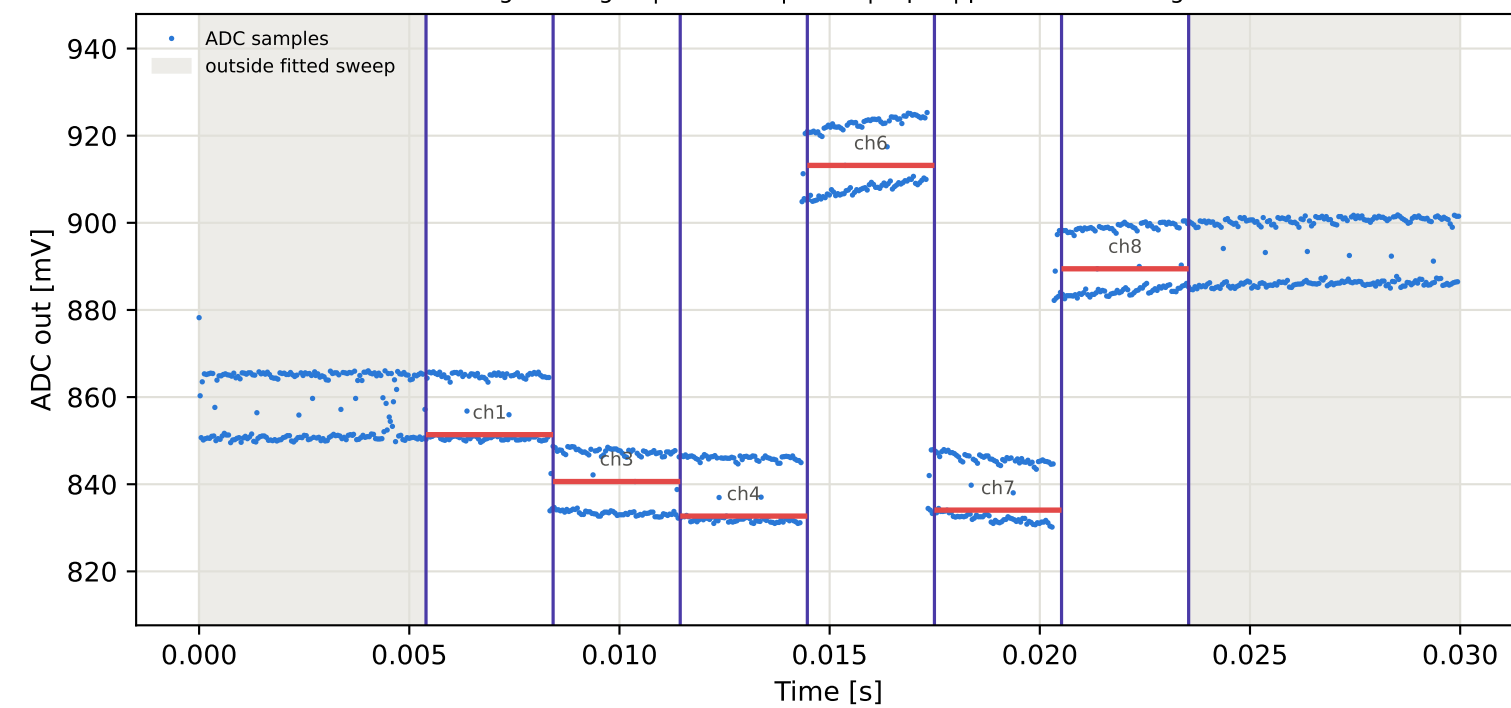
Tag7 &lt;- Tag3 | 925 MHz | run 0 | rep 1 | phase 130.29 deg
