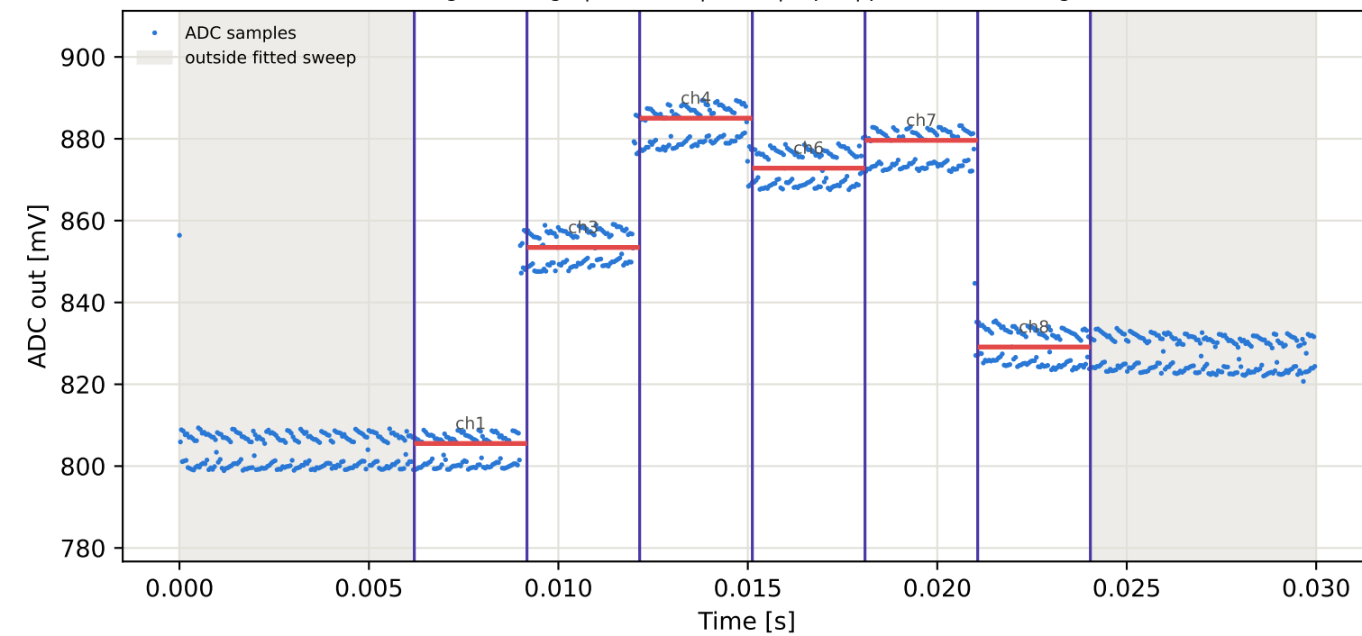
Tag2 &lt;- Tag1 | 875 MHz | run 0 | rep 1 | phase -178.75 deg
