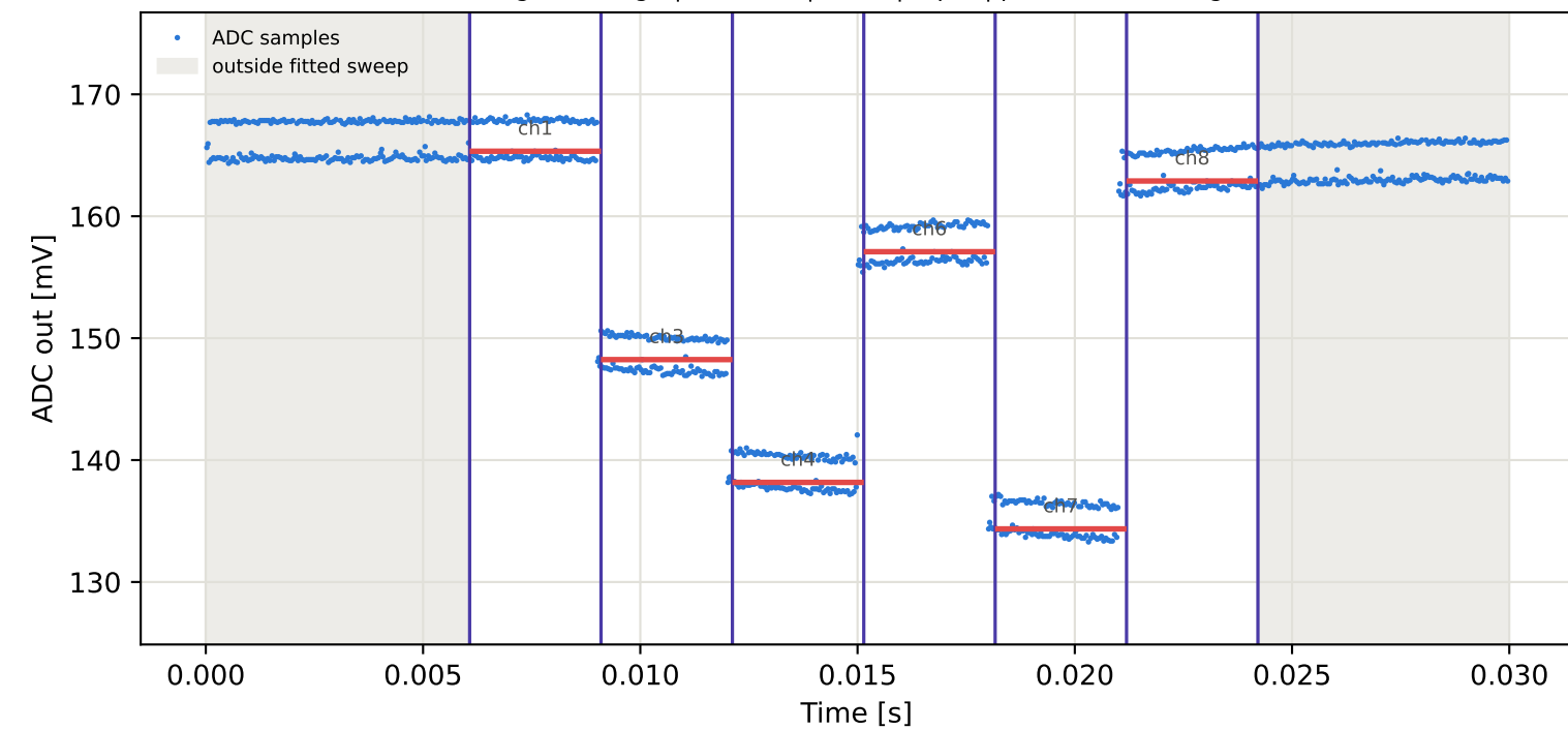
Tag2 &lt;- Tag1 | 805 MHz | run 0 | rep 1 | phase 38.00 deg
