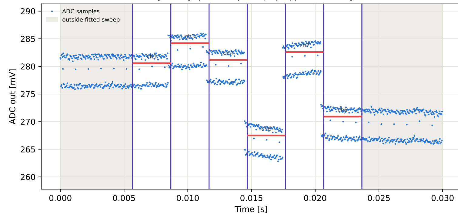
Tag1 &lt;- Tag9 | 905 MHz | run 0 | rep 1 | phase -1.64 deg
