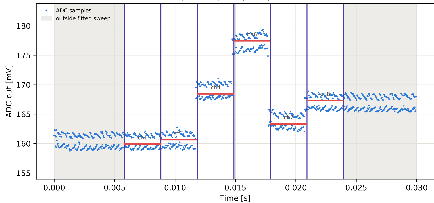
Tag9 &lt;- Tag15 | 965 MHz | run 0 | rep 1 | phase -8.28 deg
