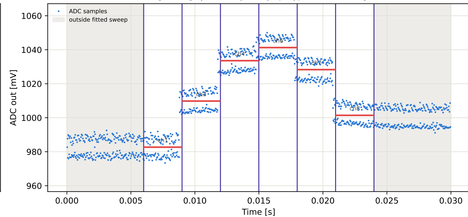
Tag3 &lt;- Tag7 | 885 MHz | run 0 | rep 1 | phase -131.07 deg
