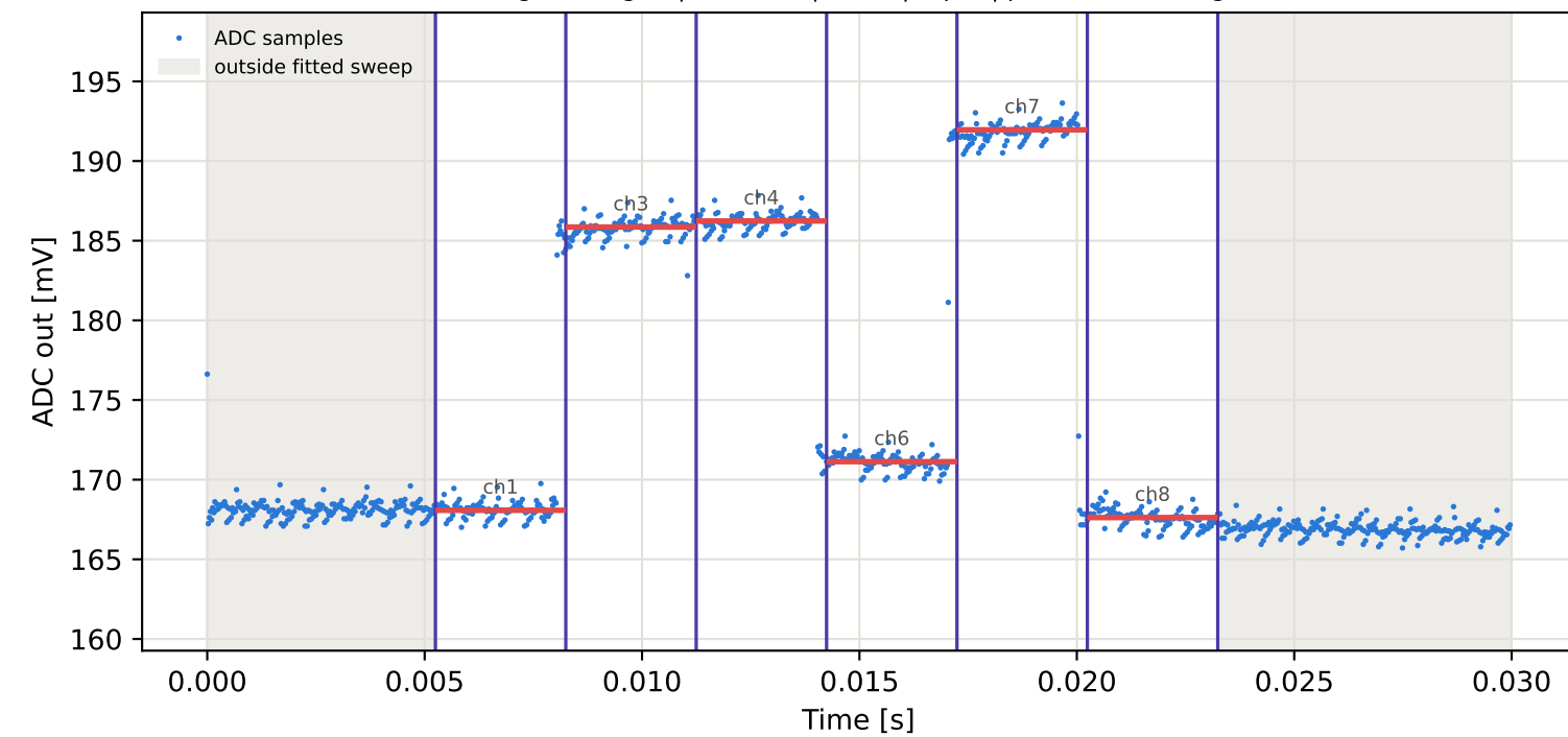
Tag7 &lt;- Tag3 | 805 MHz | run 0 | rep 1 | phase -150.52 deg
