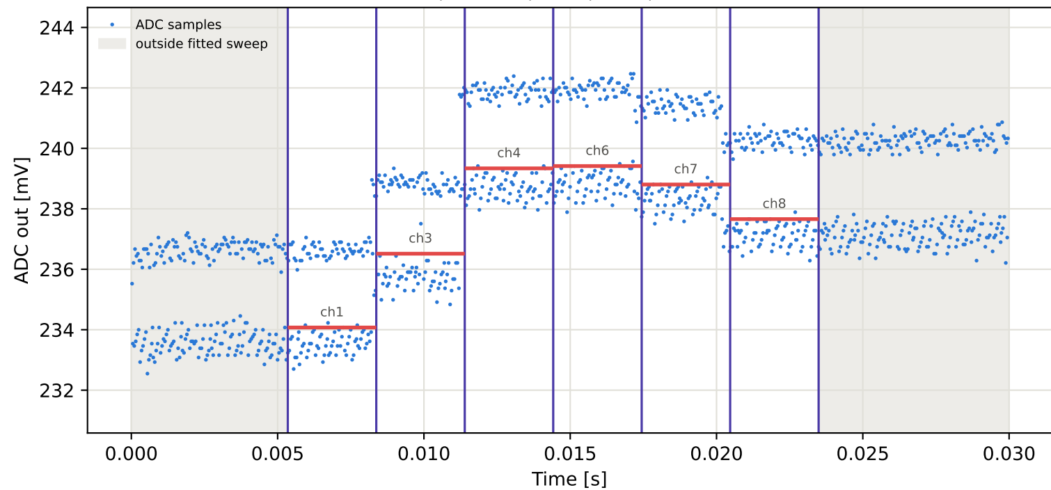
Tag1 &lt;- Tag4 | 845 MHz | run 0 | rep 1 | phase -118.44 deg
