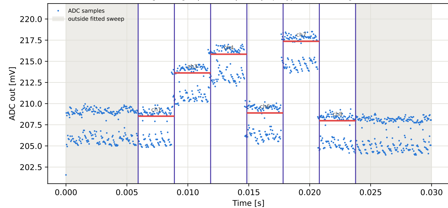
Tag6 &lt;- Tag2 | 805 MHz | run 0 | rep 1 | phase 94.60 deg
