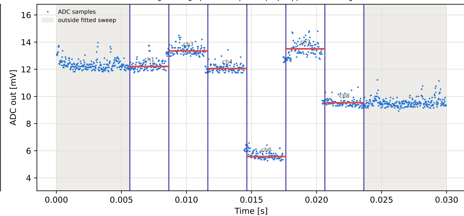
Tag2 &lt;- Tag6 | 955 MHz | run 0 | rep 1 | phase -98.52 deg
