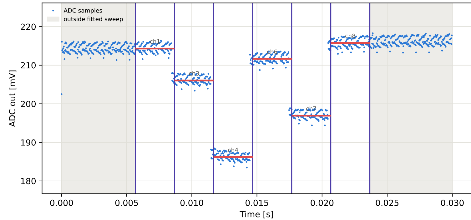
Tag5 &lt;- Tag1 | 995 MHz | run 0 | rep 1 | phase 74.90 deg
