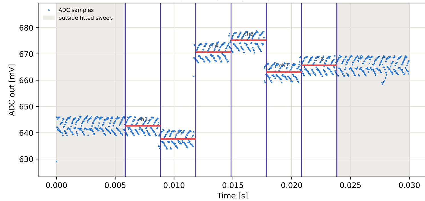
Tag8 &lt;- Tag16 | 835 MHz | run 0 | rep 1 | phase -132.33 deg
