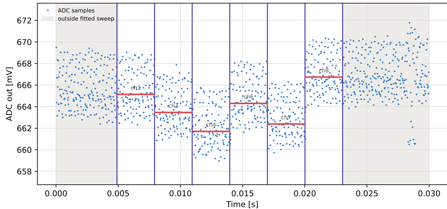
Tag3 &lt;- Tag2 | 875 MHz | run 0 | rep 1 | phase 102.13 deg
