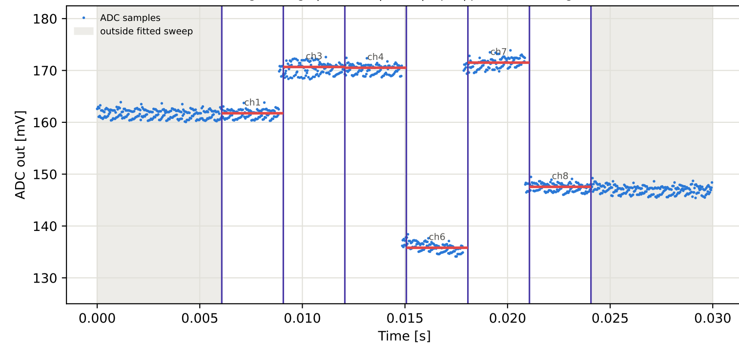
Tag9 &lt;- Tag5 | 955 MHz | run 0 | rep 1 | phase -12.82 deg
