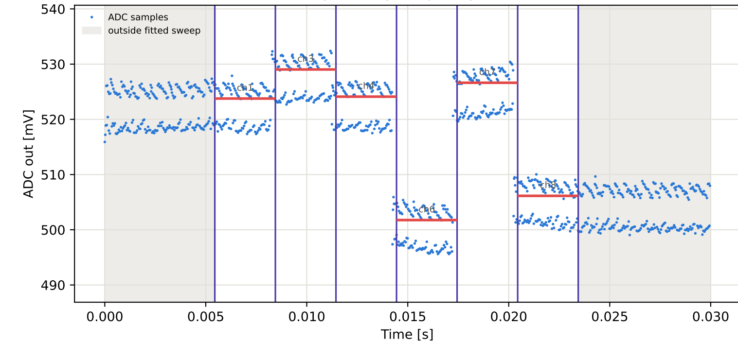
Tag6 &lt;- Tag1 | 895 MHz | run 0 | rep 1 | phase -1.72 deg
