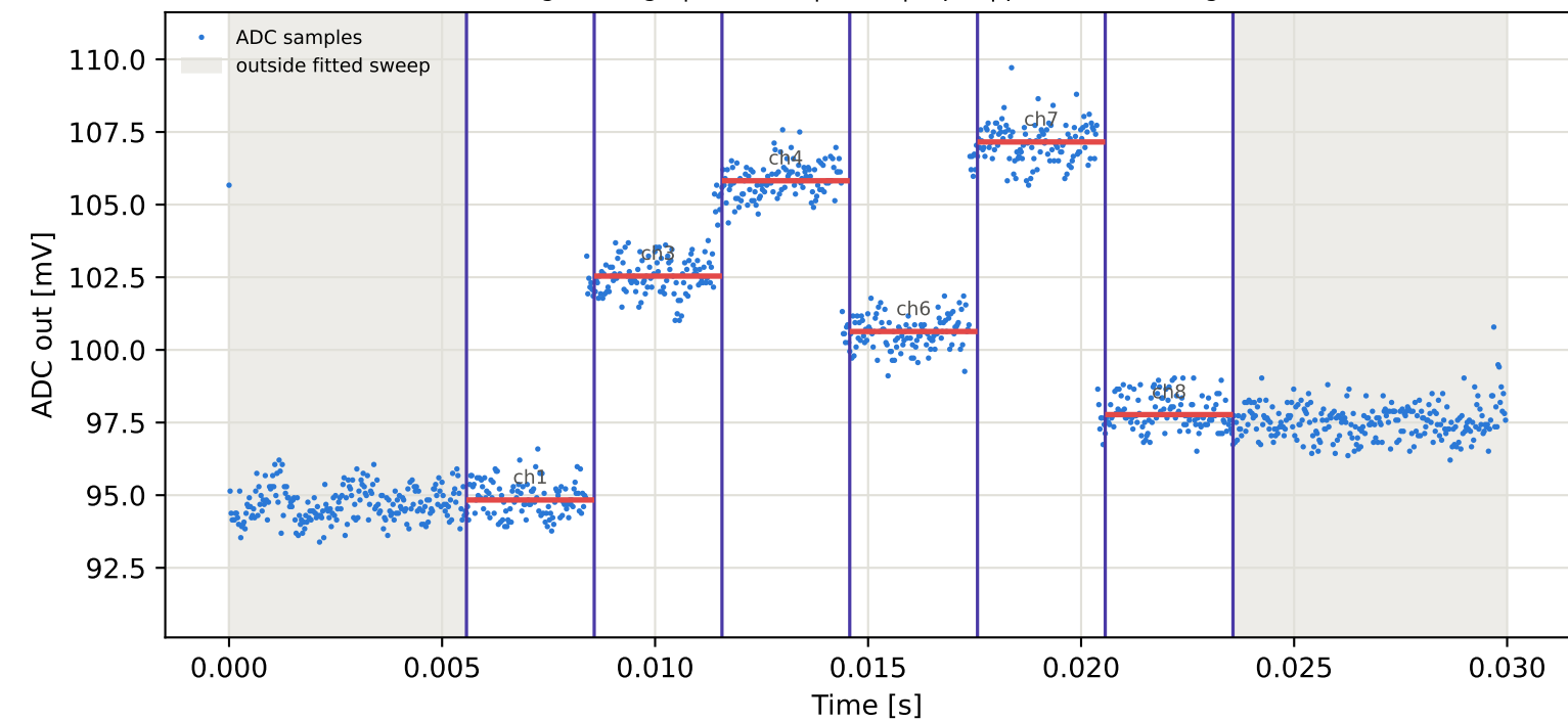
Tag2 &lt;- Tag5 | 825 MHz | run 0 | rep 1 | phase 80.05 deg
