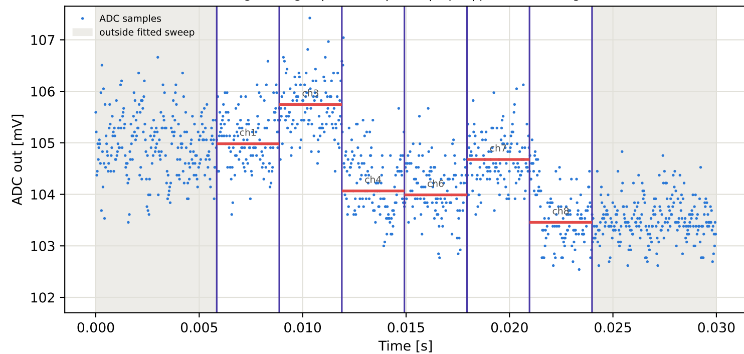
Tag2 &lt;- Tag16 | 825 MHz | run 0 | rep 1 | phase -68.46 deg
