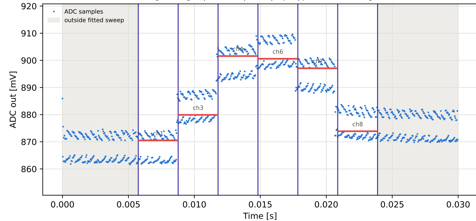
Tag4 &lt;- Tag2 | 895 MHz | run 0 | rep 1 | phase -38.82 deg
