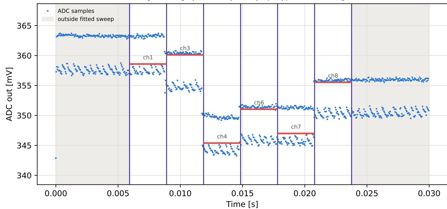
Tag15 &lt;- Tag6 | 825 MHz | run 0 | rep 1 | phase -74.30 deg
