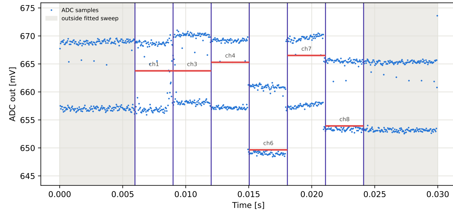
Tag10 &lt;- Tag4 | 915 MHz | run 0 | rep 1 | phase 118.08 deg
