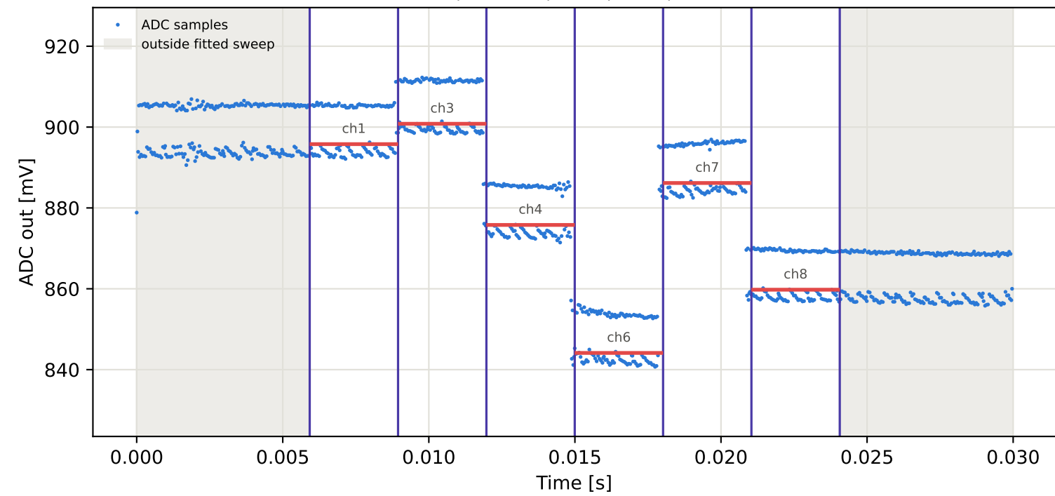
Tag16 &lt;- Tag7 | 875 MHz | run 0 | rep 1 | phase 22.14 deg
