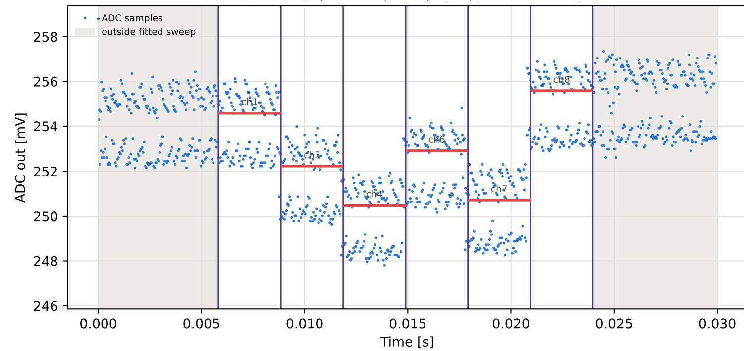
Tag16 &lt;- Tag4 | 835 MHz | run 0 | rep 1 | phase -79.06 deg
