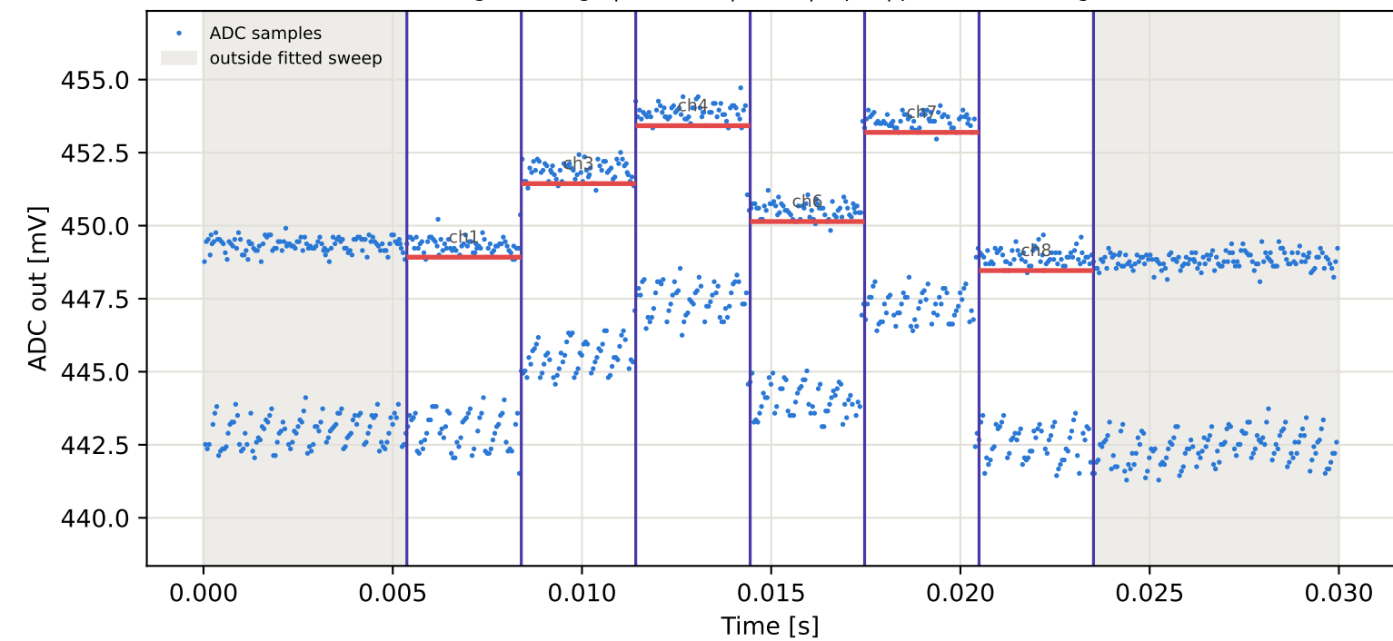
Tag15 &lt;- Tag9 | 845 MHz | run 0 | rep 1 | phase 83.83 deg
