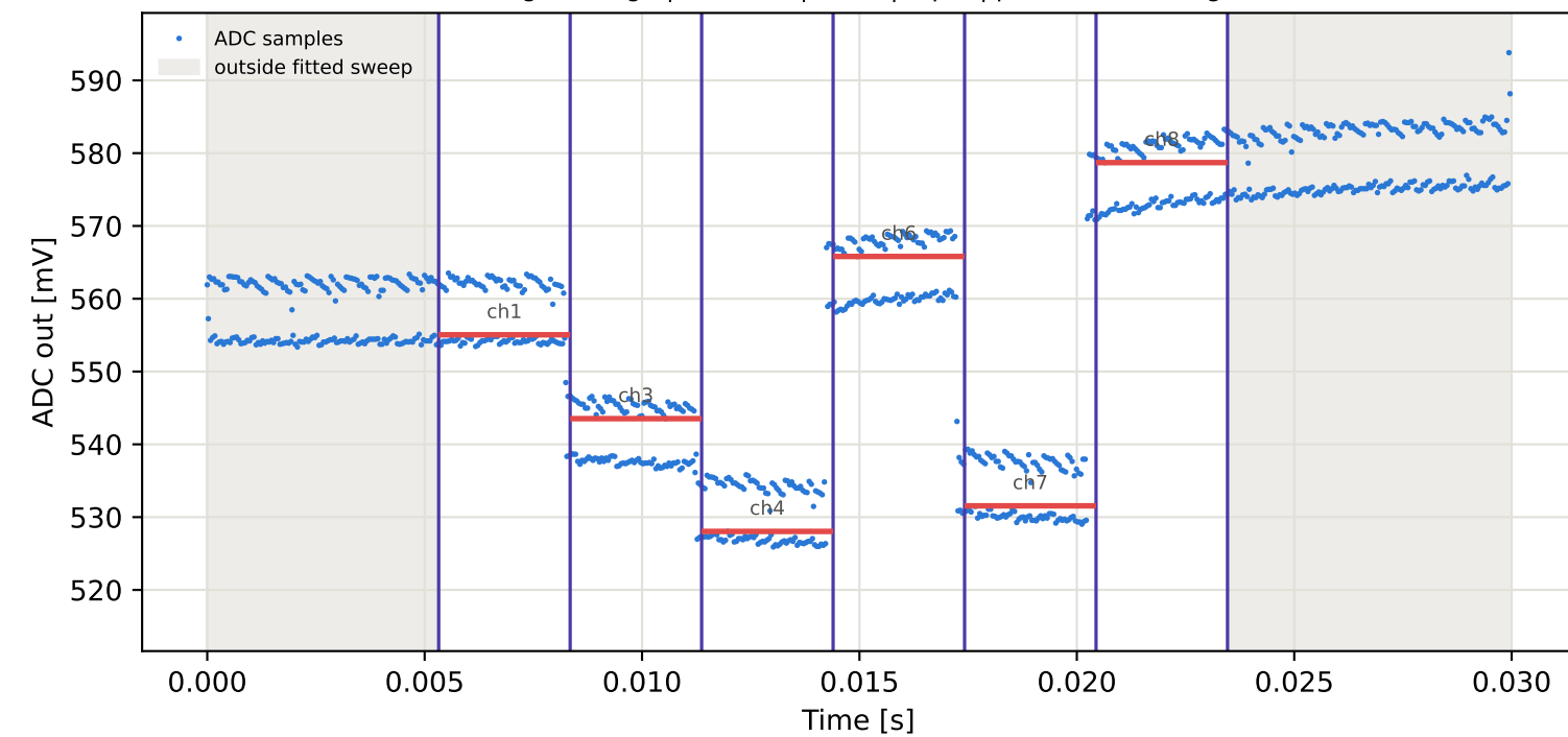
Tag7 &lt;- Tag5 | 905 MHz | run 0 | rep 1 | phase -125.74 deg
