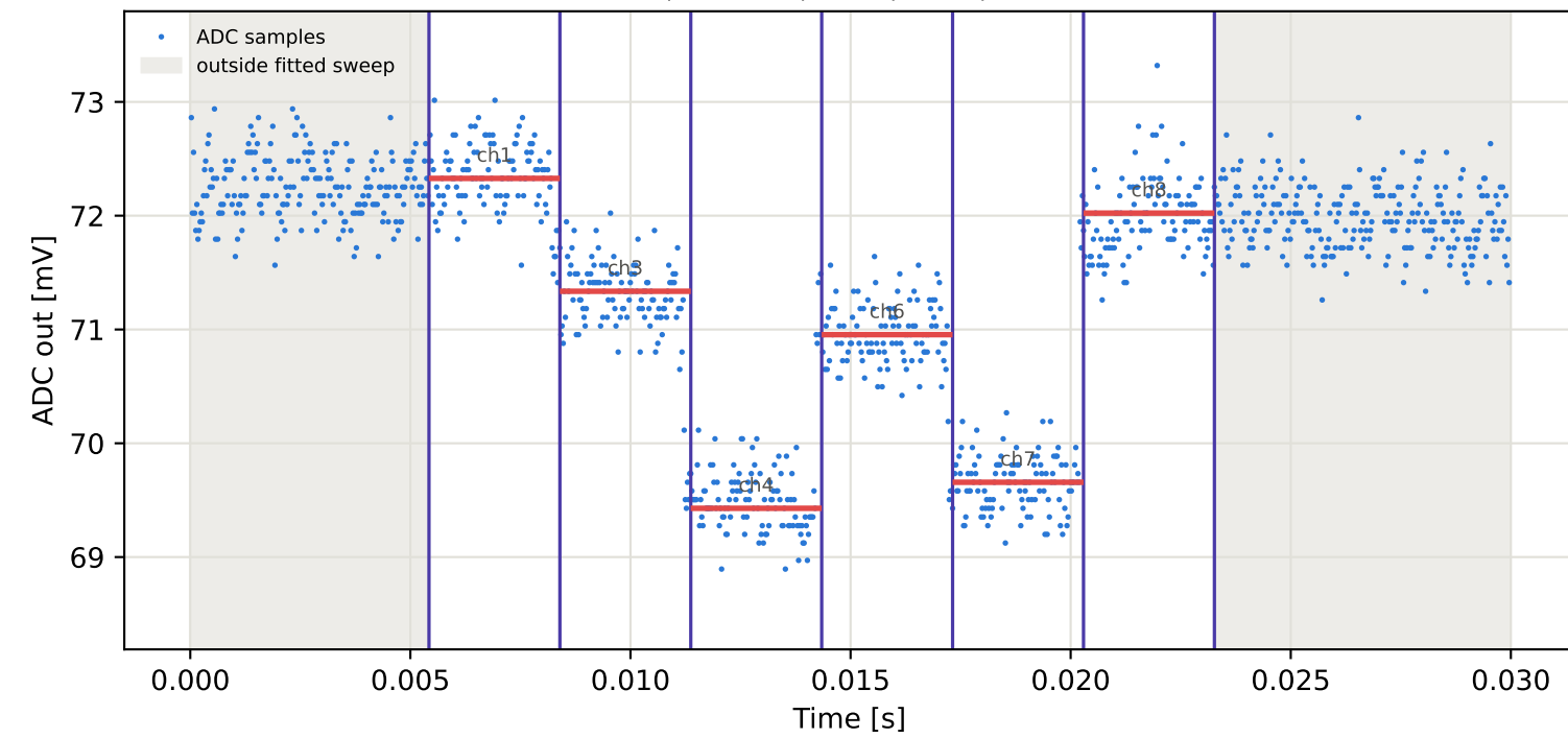
Tag4 &lt;- Tag9 | 805 MHz | run 0 | rep 1 | phase 95.00 deg
