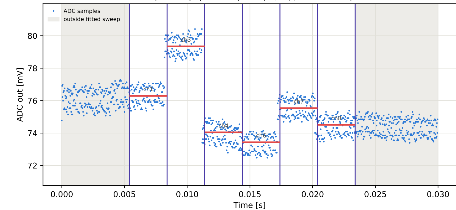
Tag16 &lt;- Tag6 | 795 MHz | run 0 | rep 1 | phase 61.25 deg
