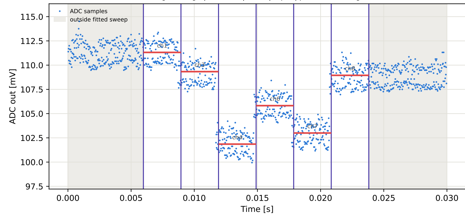
Tag2 &lt;- Tag7 | 825 MHz | run 0 | rep 1 | phase 69.90 deg
