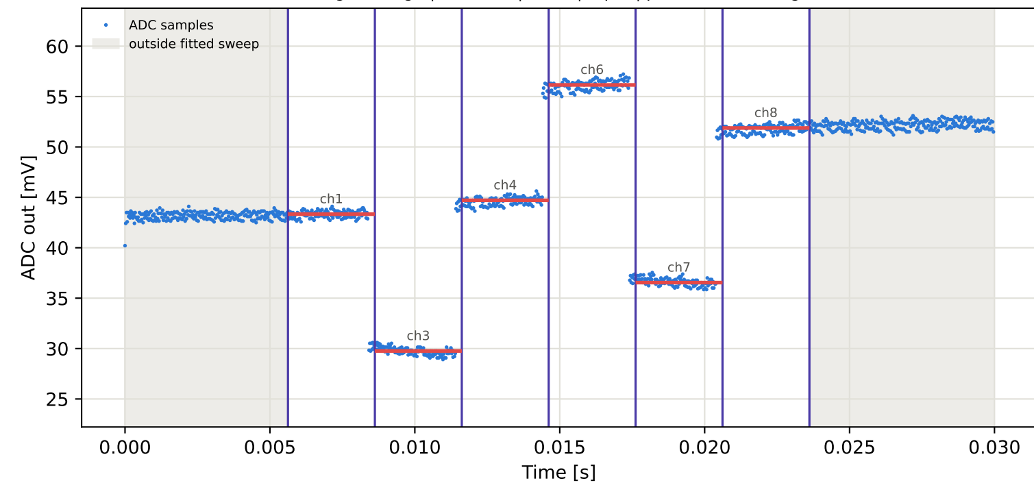
Tag4 &lt;- Tag7 | 775 MHz | run 0 | rep 1 | phase 130.08 deg
