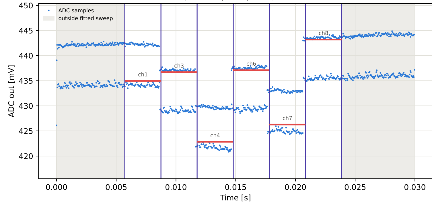
Tag9 &lt;- Tag15 | 935 MHz | run 0 | rep 1 | phase -85.16 deg
