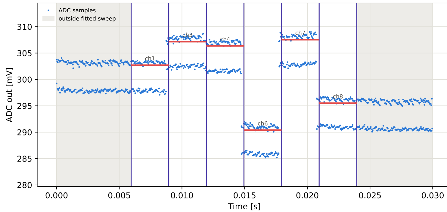
Tag4 &lt;- Tag15 | 965 MHz | run 0 | rep 1 | phase -51.98 deg
