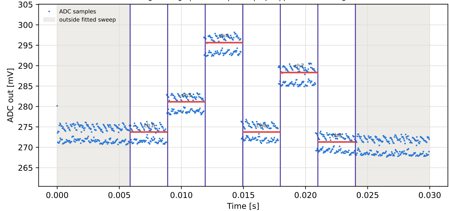
Tag7 &lt;- Tag1 | 985 MHz | run 0 | rep 1 | phase -116.01 deg
