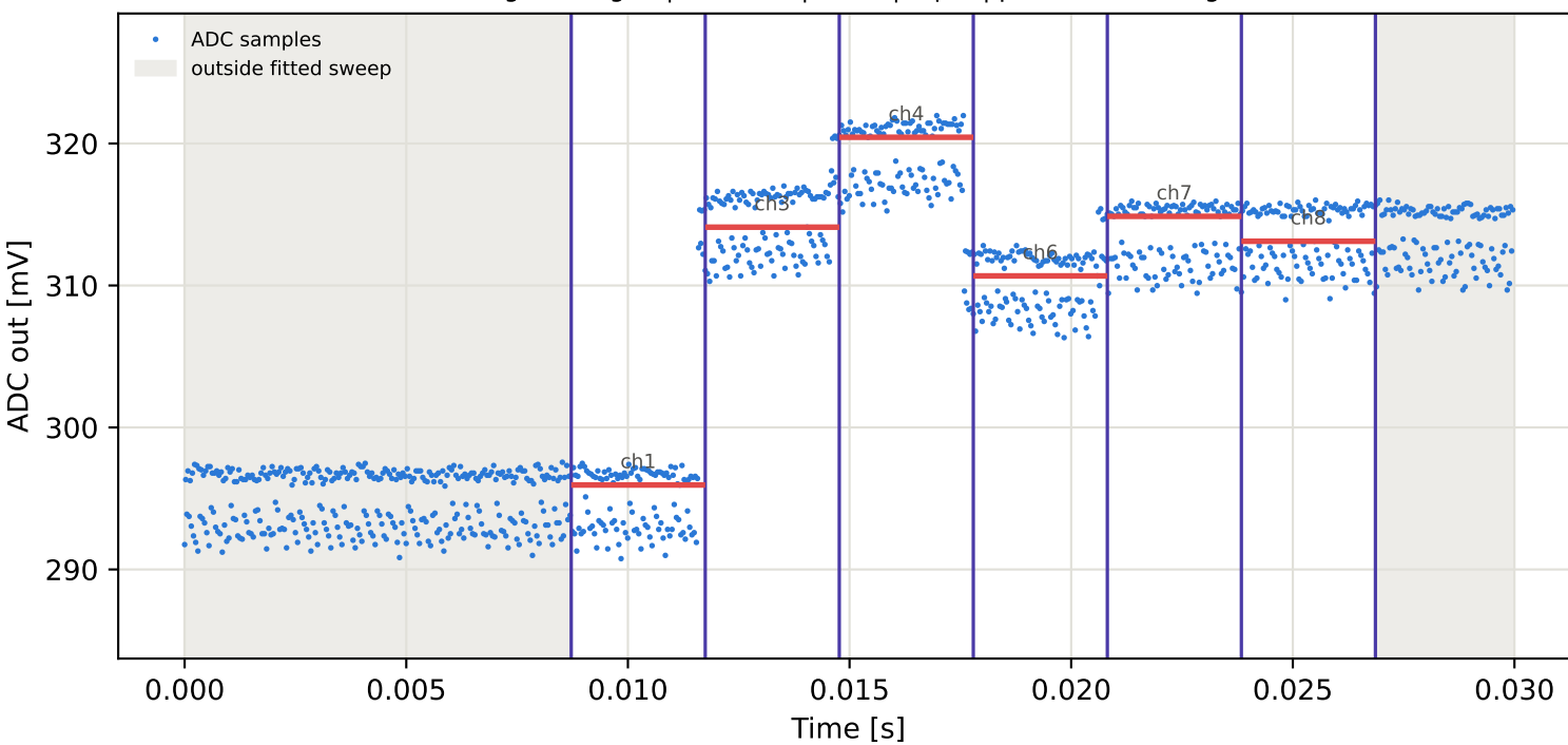
Tag3 &lt;- Tag16 | 845 MHz | run 0 | rep 1 | phase -94.41 deg
