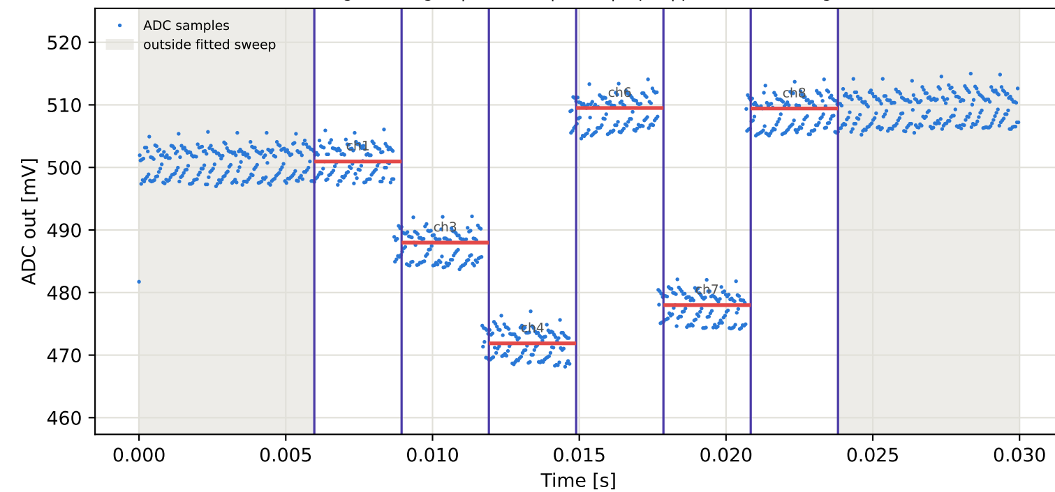
Tag15 &lt;- Tag3 | 985 MHz | run 0 | rep 1 | phase 74.28 deg
