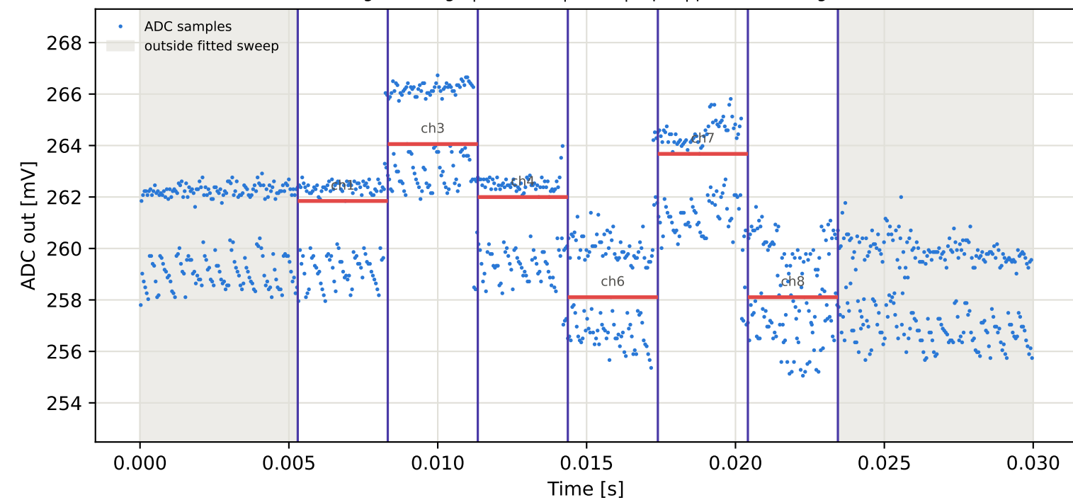
Tag10 &lt;- Tag5 | 835 MHz | run 0 | rep 1 | phase 0.63 deg
