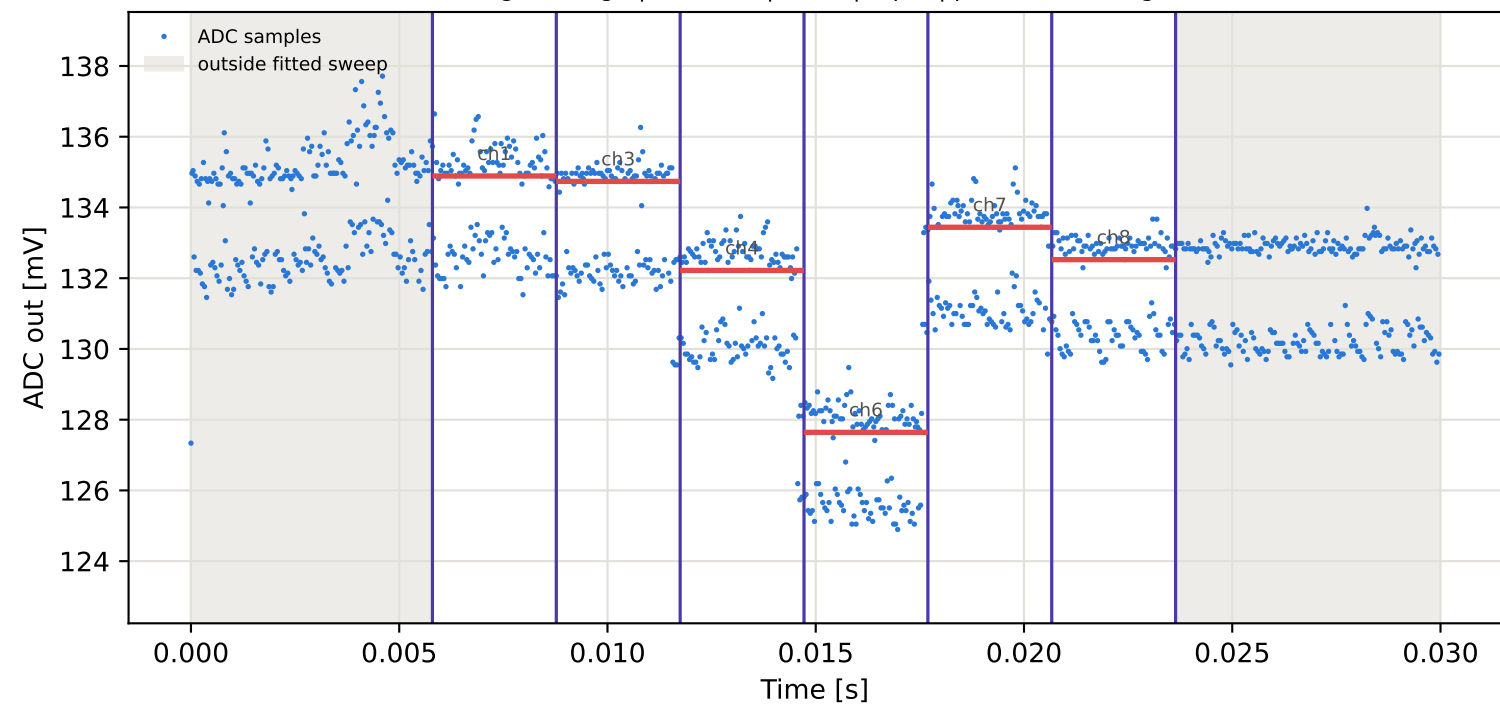
Tag2 &lt;- Tag5 | 925 MHz | run 0 | rep 1 | phase 162.88 deg
