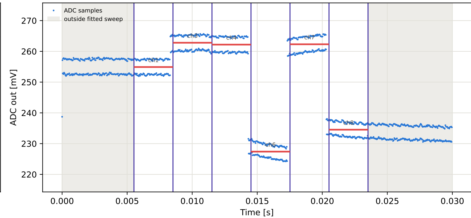
Tag9 &lt;- Tag8 | 905 MHz | run 0 | rep 1 | phase -61.41 deg
