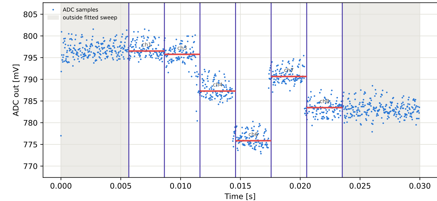
Tag16 &lt;- Tag15 | 885 MHz | run 0 | rep 1 | phase -155.17 deg
