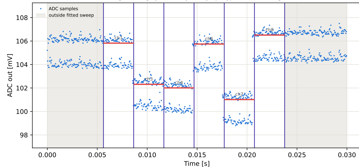
Tag15 &lt;- Tag9 | 785 MHz | run 0 | rep 1 | phase 138.09 deg
