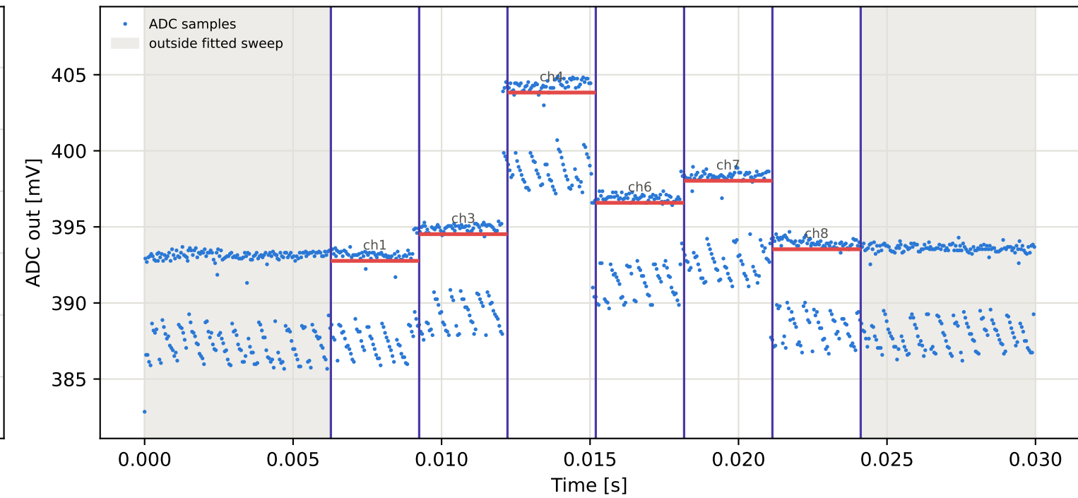
Tag8 &lt;- Tag7 | 995 MHz | run 0 | rep 1 | phase -144.81 deg
