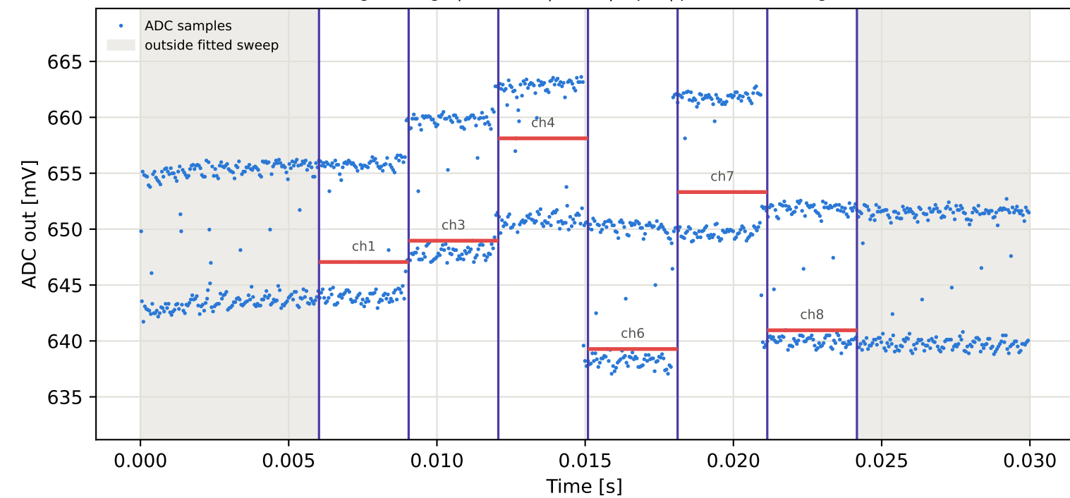
Tag5 &lt;- Tag8 | 945 MHz | run 0 | rep 1 | phase 178.24 deg
