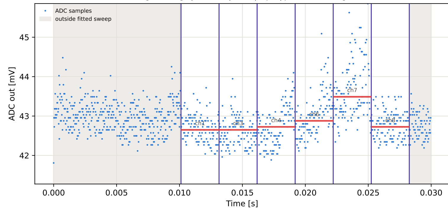
Tag15 &lt;- Tag4 | 775 MHz | run 0 | rep 1 | phase -74.69 deg
