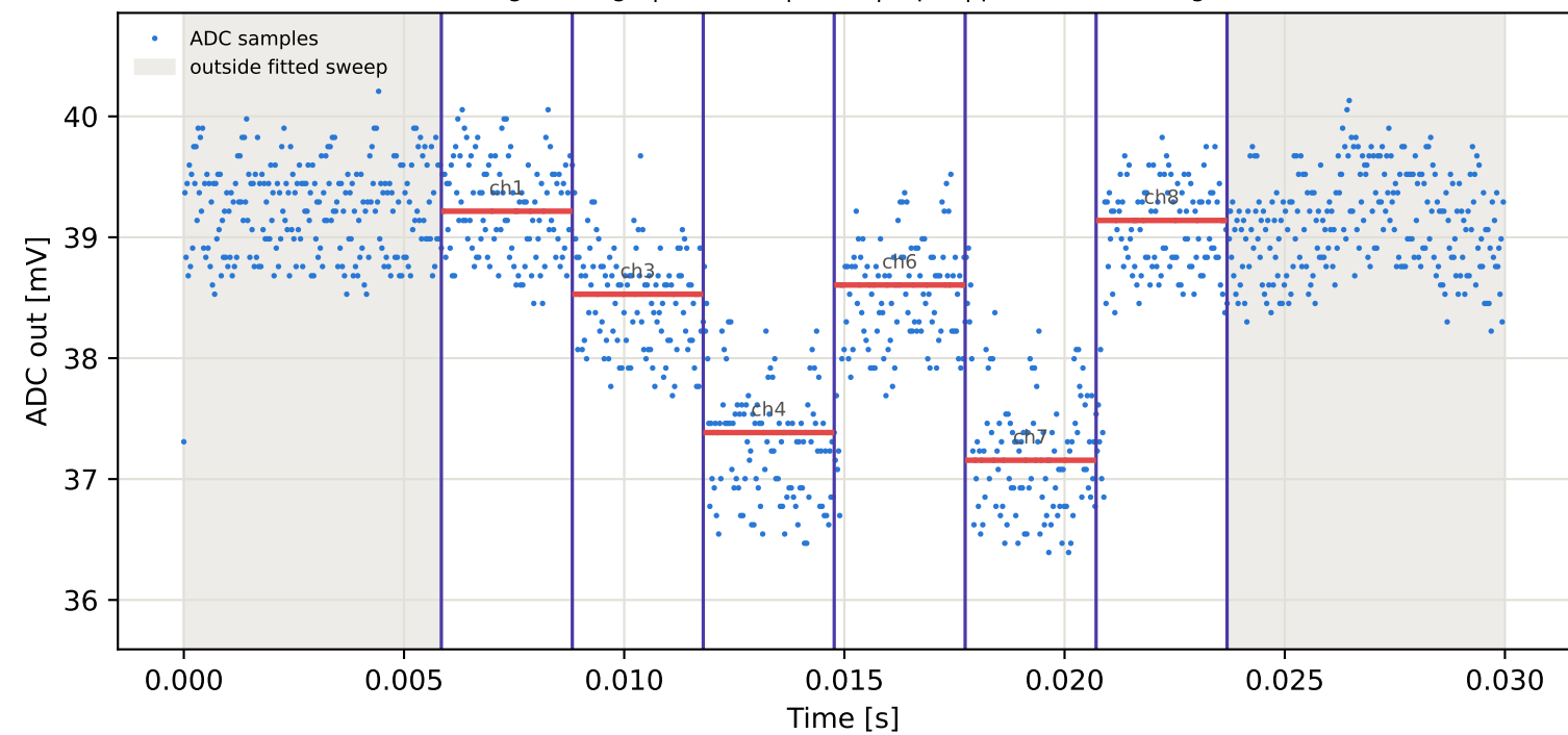
Tag10 &lt;- Tag1 | 785 MHz | run 0 | rep 1 | phase -154.17 deg
