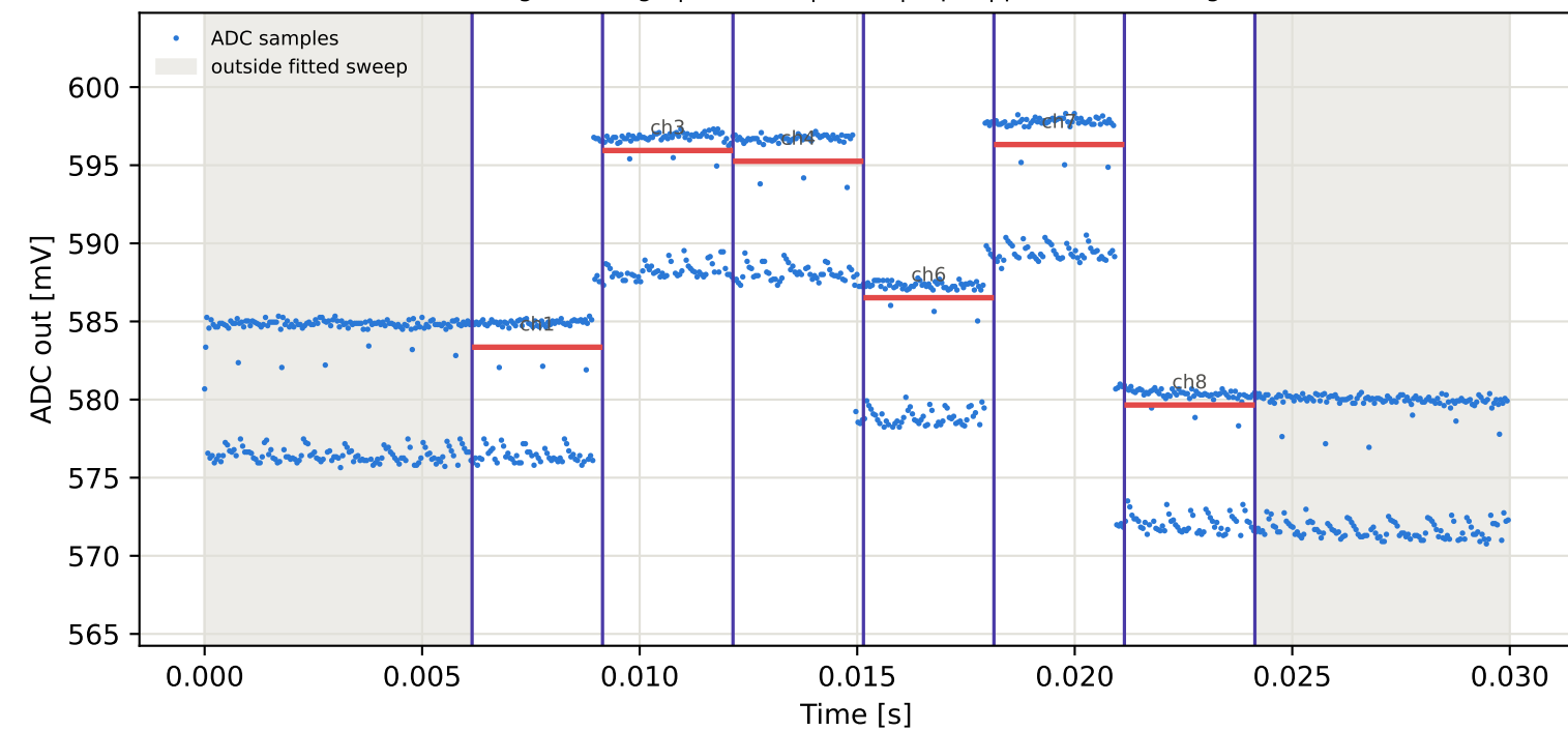
Tag16 &lt;- Tag15 | 865 MHz | run 0 | rep 1 | phase 178.65 deg
