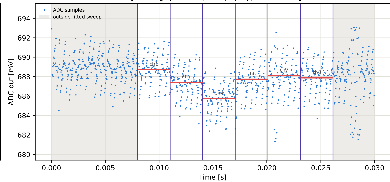
Tag15 &lt;- Tag4 | 905 MHz | run 0 | rep 1 | phase -83.70 deg
