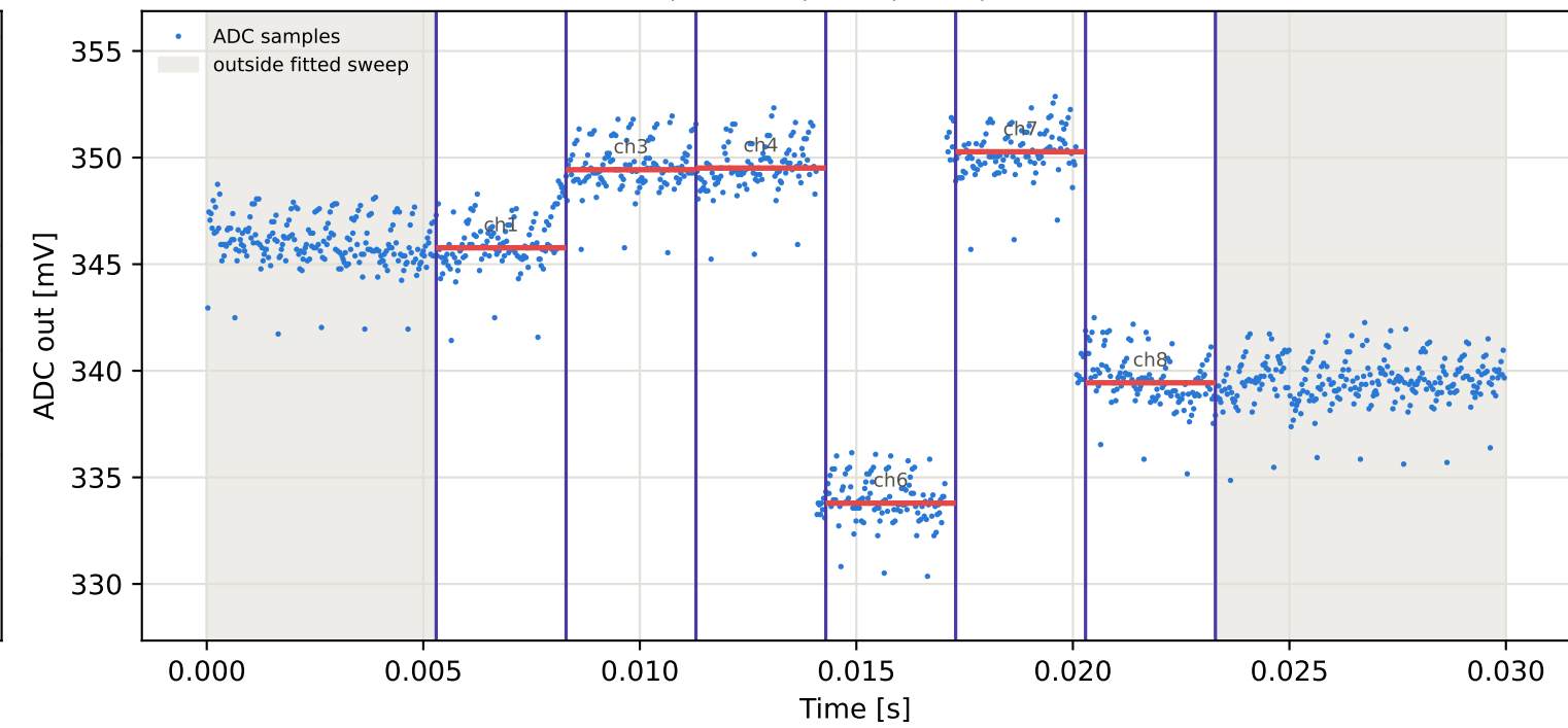
Tag6 &lt;- Tag5 | 935 MHz | run 0 | rep 1 | phase -14.07 deg
