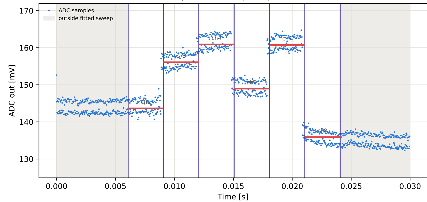
Tag2 &lt;- Tag6 | 885 MHz | run 0 | rep 1 | phase 170.56 deg
