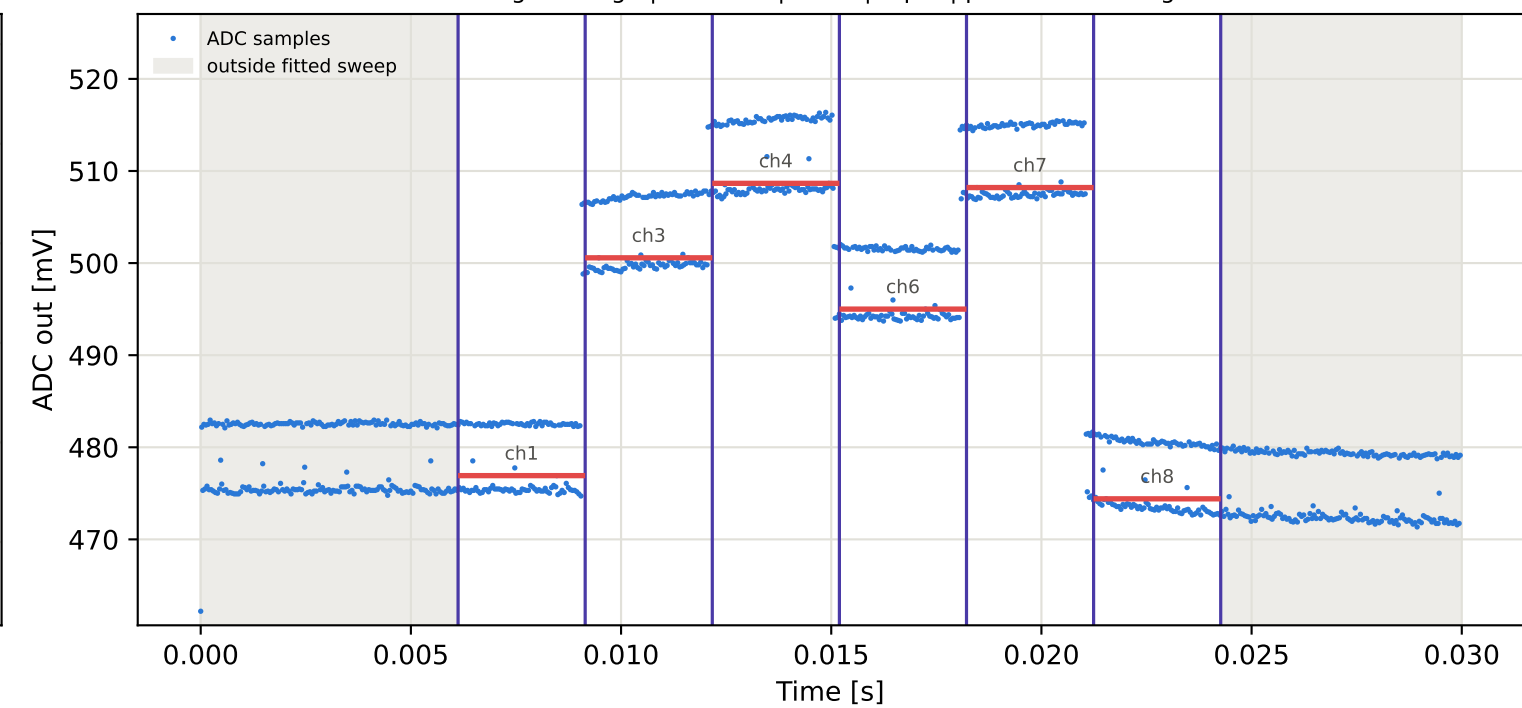
Tag4 &lt;- Tag8 | 865 MHz | run 0 | rep 1 | phase 117.47 deg
