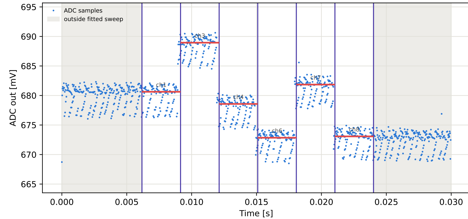
Tag15 &lt;- Tag5 | 835 MHz | run 0 | rep 1 | phase -17.18 deg
