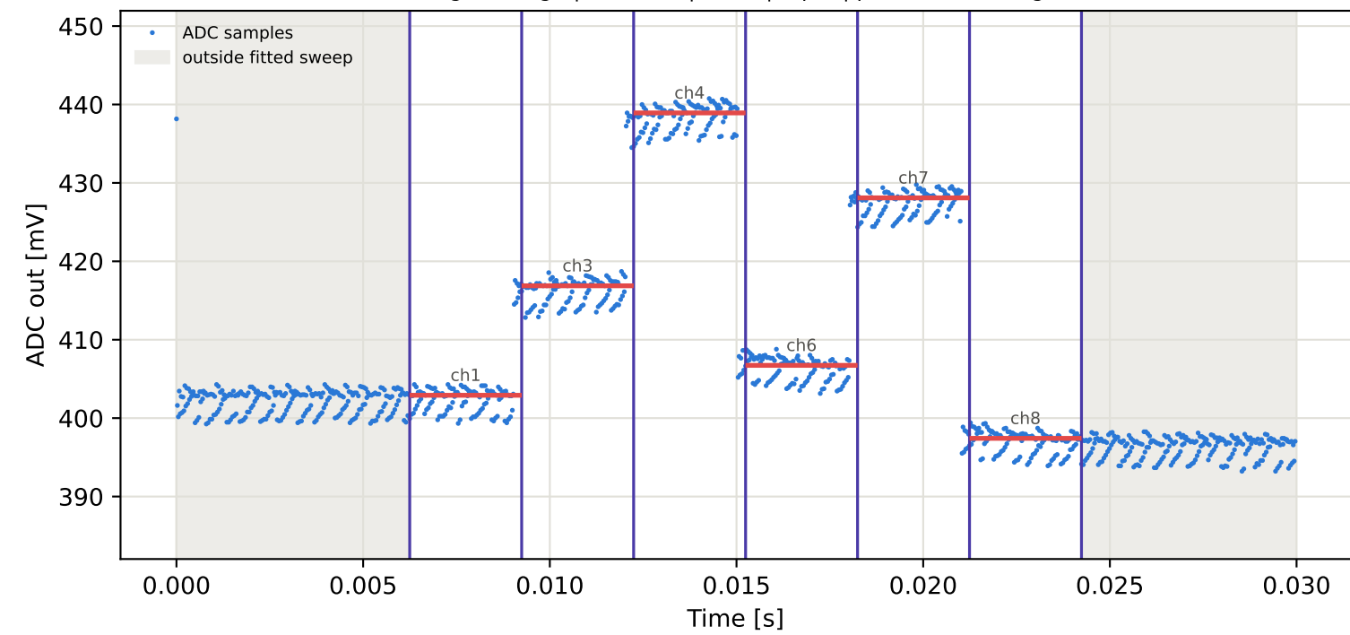
Tag8 &lt;- Tag10 | 975 MHz | run 0 | rep 1 | phase -158.87 deg
