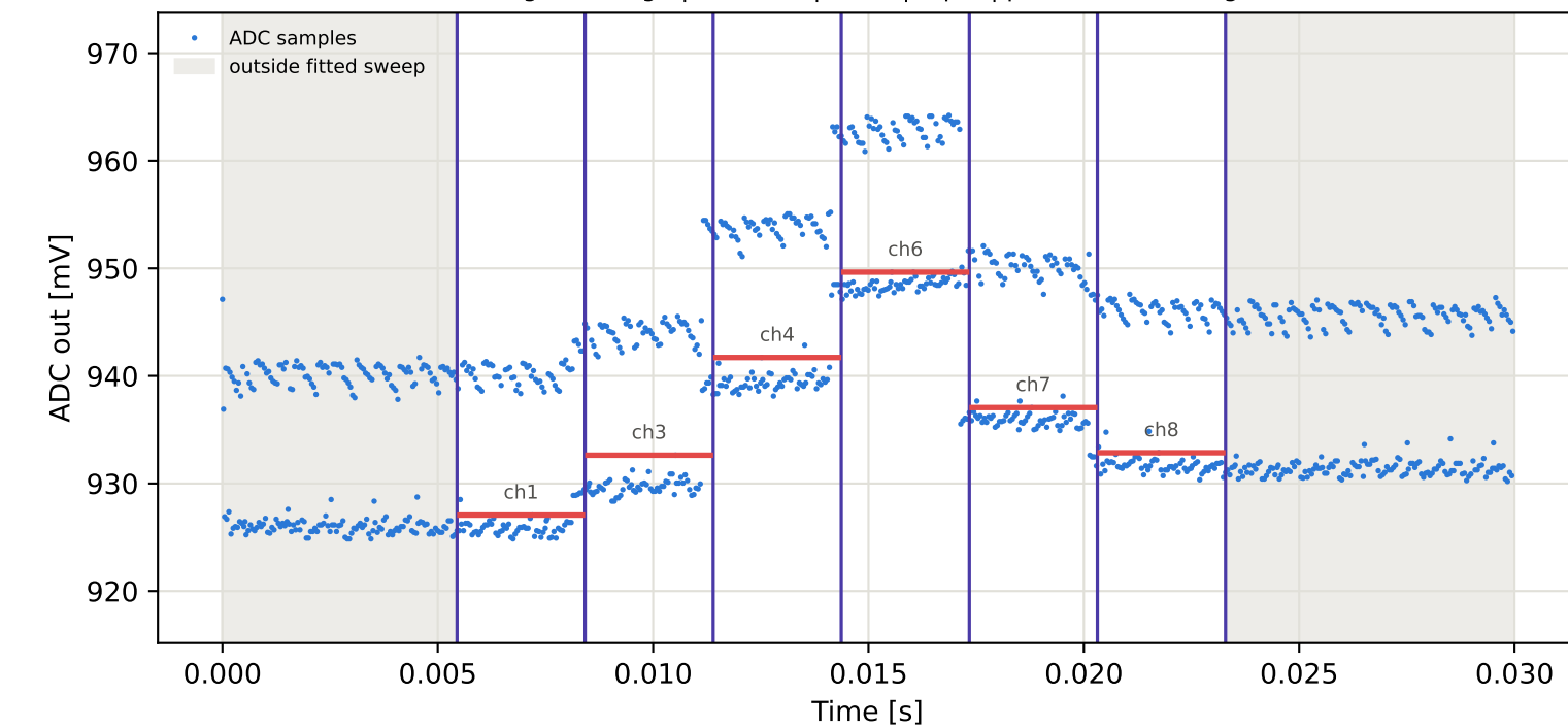
Tag15 &lt;- Tag5 | 915 MHz | run 0 | rep 1 | phase 178.95 deg
