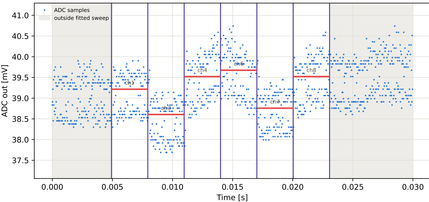
Tag4 &lt;- Tag3 | 775 MHz | run 0 | rep 1 | phase -153.75 deg
