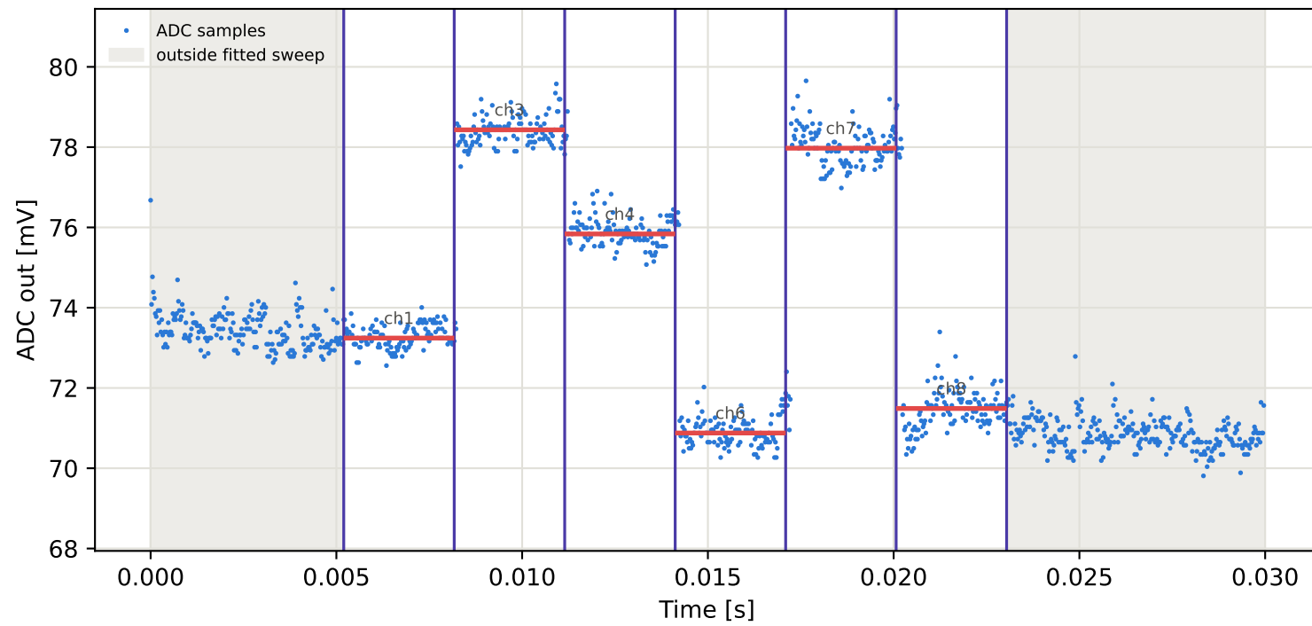
Tag6 &lt;- Tag9 | 795 MHz | run 0 | rep 1 | phase 16.37 deg
