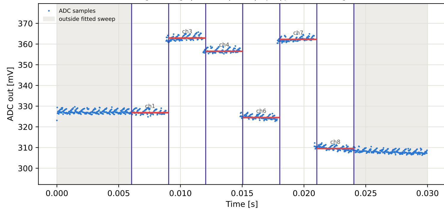
Tag16 &lt;- Tag1 | 855 MHz | run 0 | rep 1 | phase -111.95 deg
