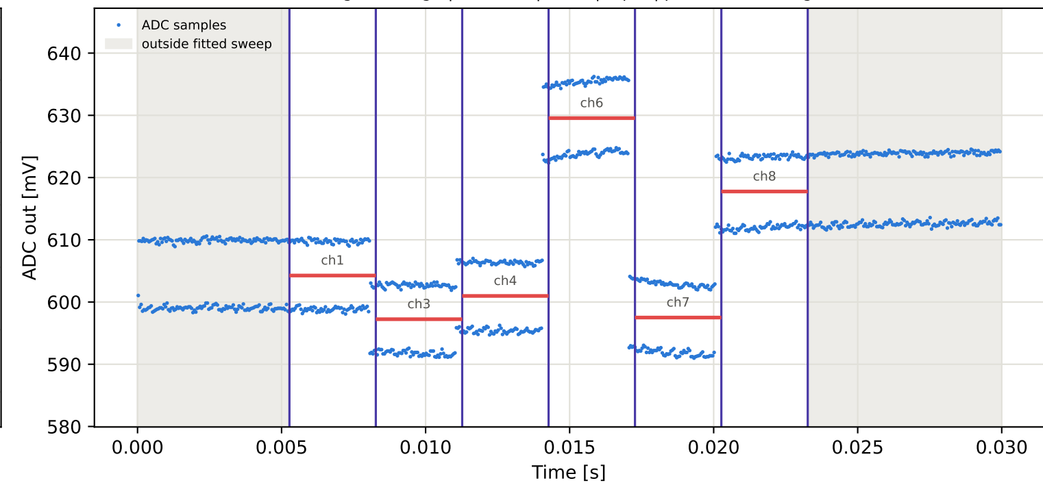
Tag2 &lt;- Tag10 | 965 MHz | run 0 | rep 1 | phase 97.09 deg
