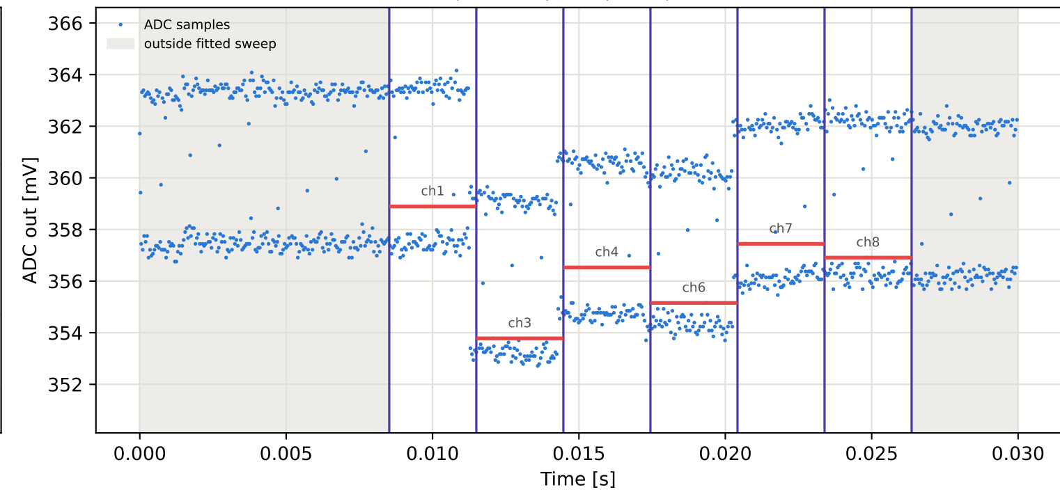
Tag5 &lt;- Tag1 | 825 MHz | run 0 | rep 1 | phase 67.89 deg
