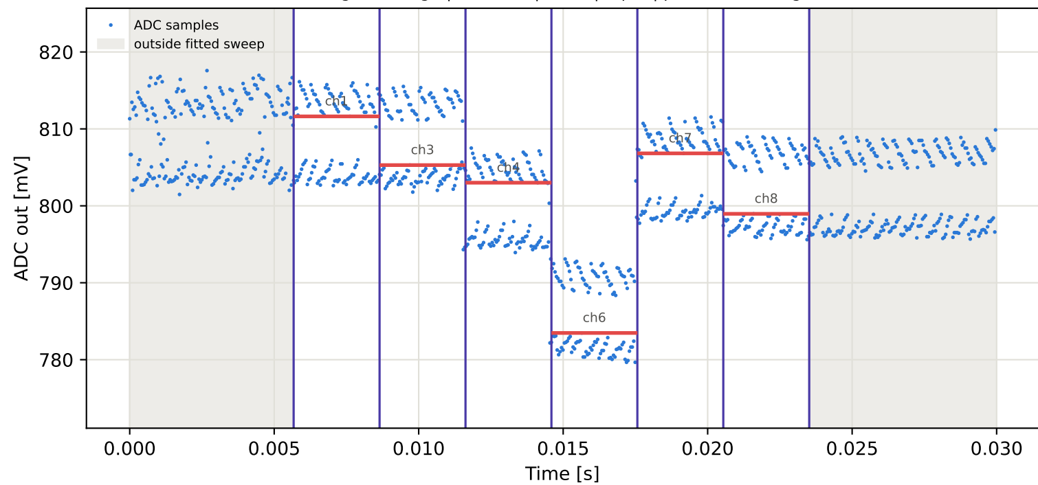
Tag16 &lt;- Tag5 | 925 MHz | run 0 | rep 1 | phase 84.39 deg
