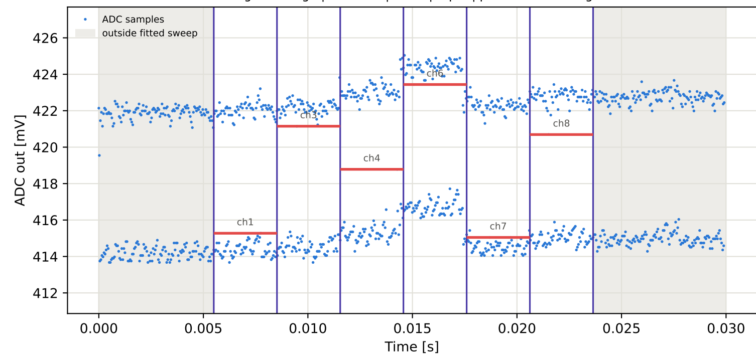
Tag15 &lt;- Tag4 | 995 MHz | run 0 | rep 1 | phase 169.47 deg
