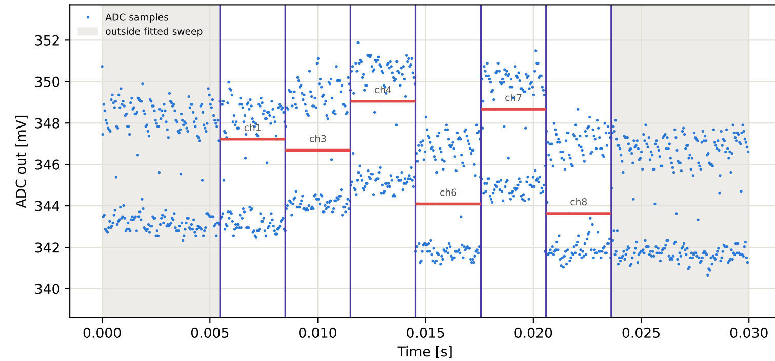
Tag6 &lt;- Tag4 | 935 MHz | run 0 | rep 1 | phase -52.57 deg
