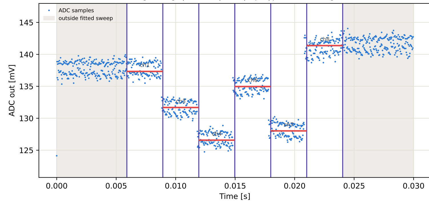
Tag3 &lt;- Tag10 | 925 MHz | run 0 | rep 1 | phase 48.61 deg
