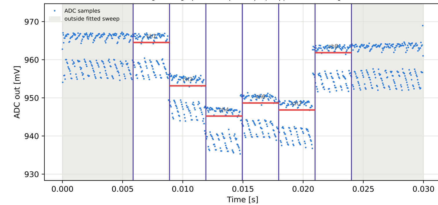
Tag4 &lt;- Tag9 | 875 MHz | run 0 | rep 1 | phase 78.56 deg
