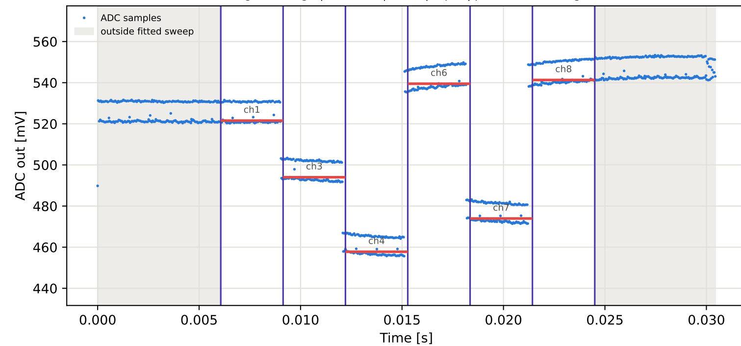
Tag10 &lt;- Tag8 | 955 MHz | run 0 | rep 1 | phase -99.16 deg
