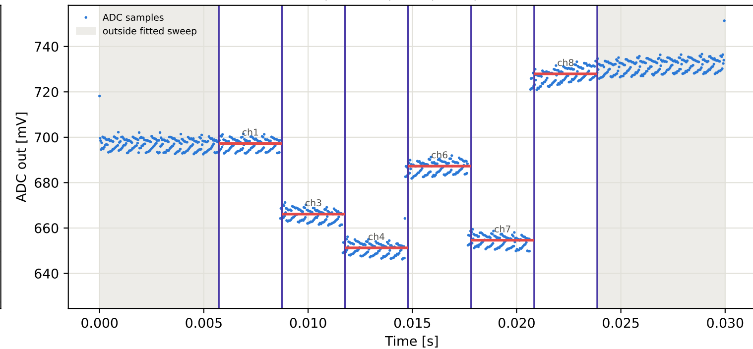
Tag10 &lt;- Tag5 | 895 MHz | run 0 | rep 1 | phase 110.98 deg
