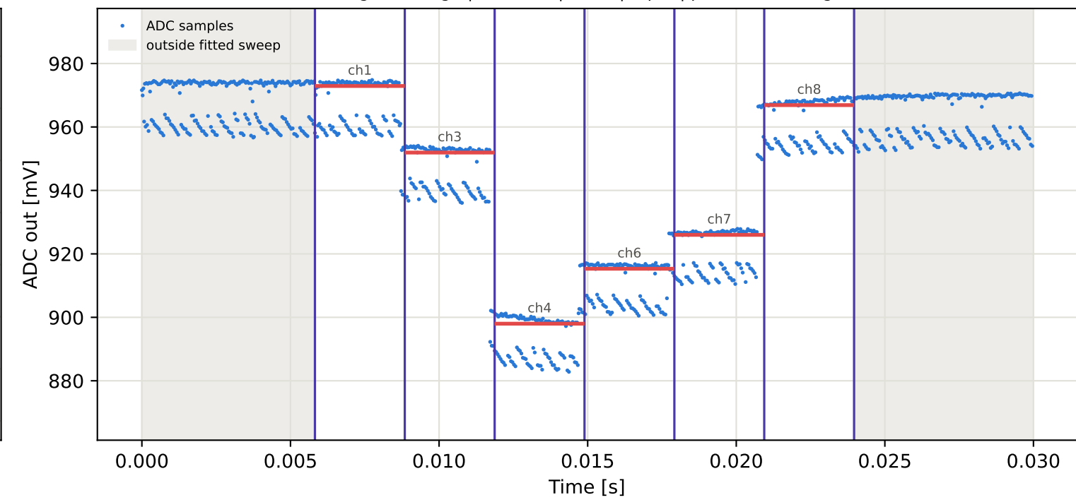
Tag16 &lt;- Tag1 | 945 MHz | run 0 | rep 1 | phase 146.06 deg
