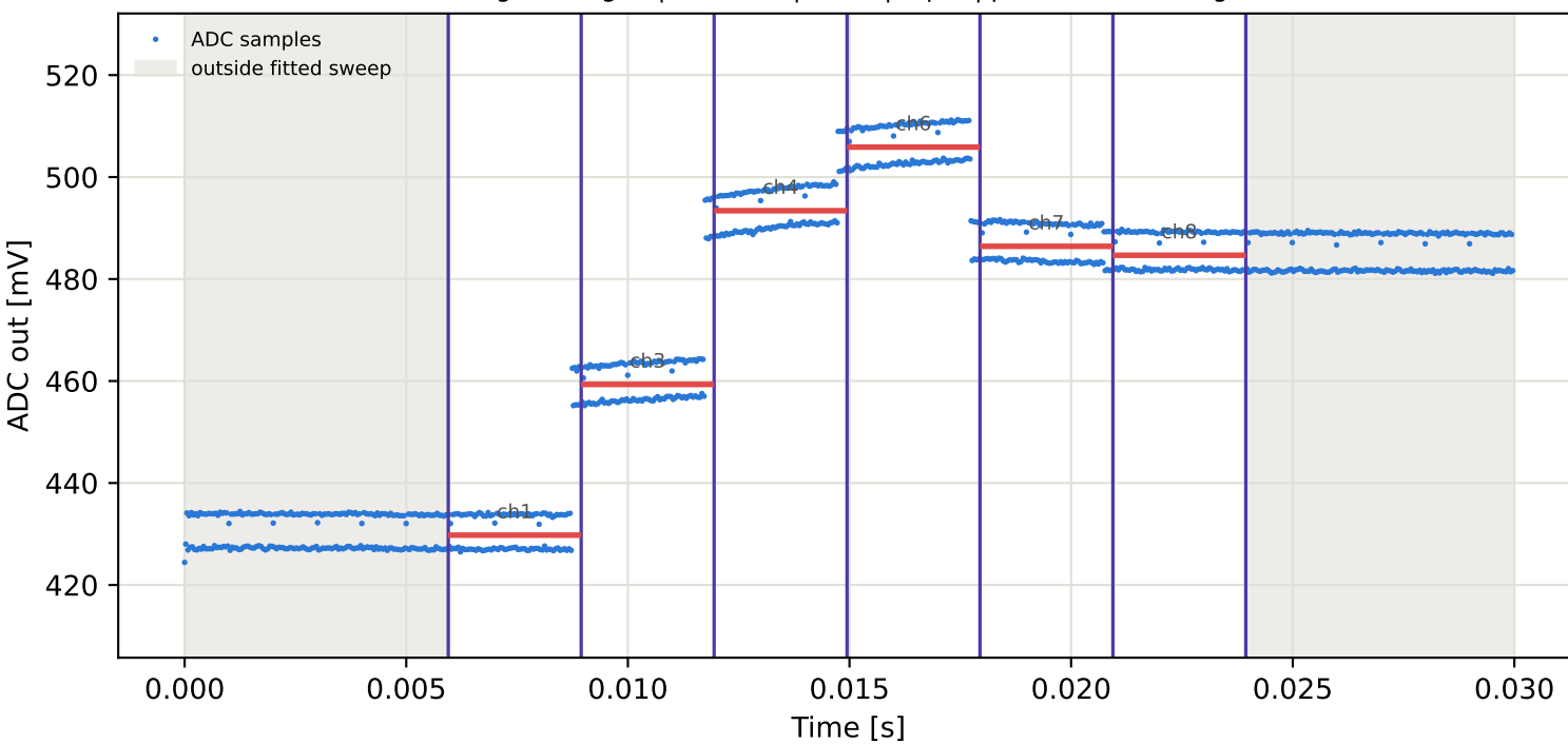
Tag3 &lt;- Tag16 | 865 MHz | run 0 | rep 1 | phase -128.62 deg
