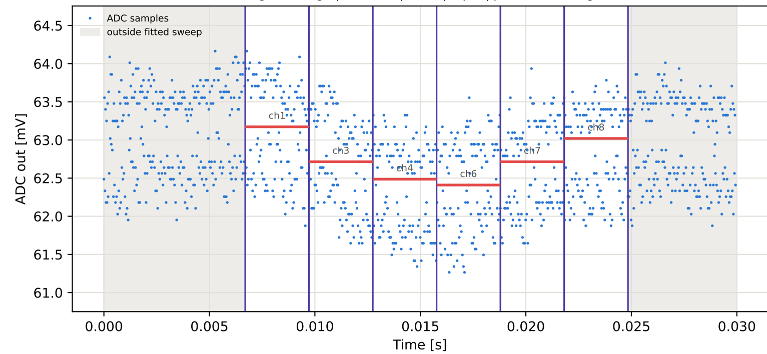
Tag16 &lt;- Tag4 | 785 MHz | run 0 | rep 1 | phase 41.86 deg
