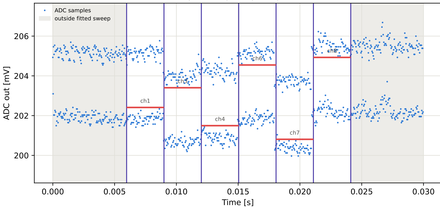
Tag15 &lt;- Tag10 | 805 MHz | run 0 | rep 1 | phase 143.52 deg
