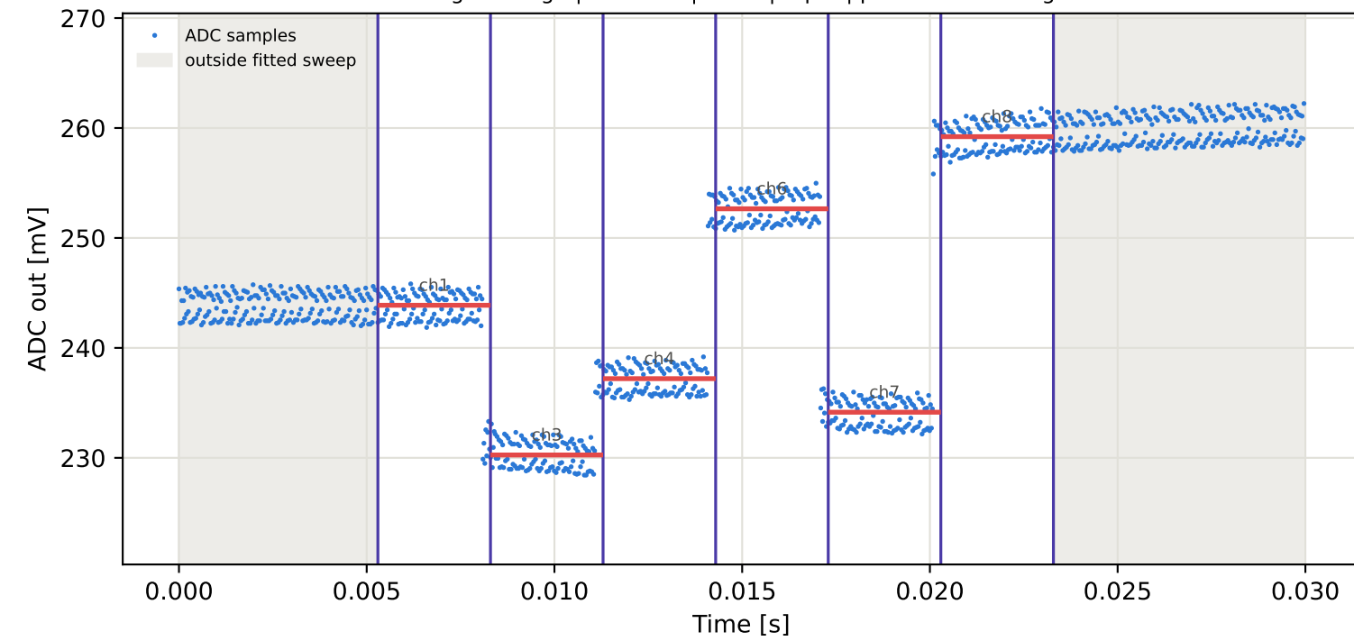
Tag1 &lt;- Tag3 | 855 MHz | run 0 | rep 1 | phase 164.07 deg
