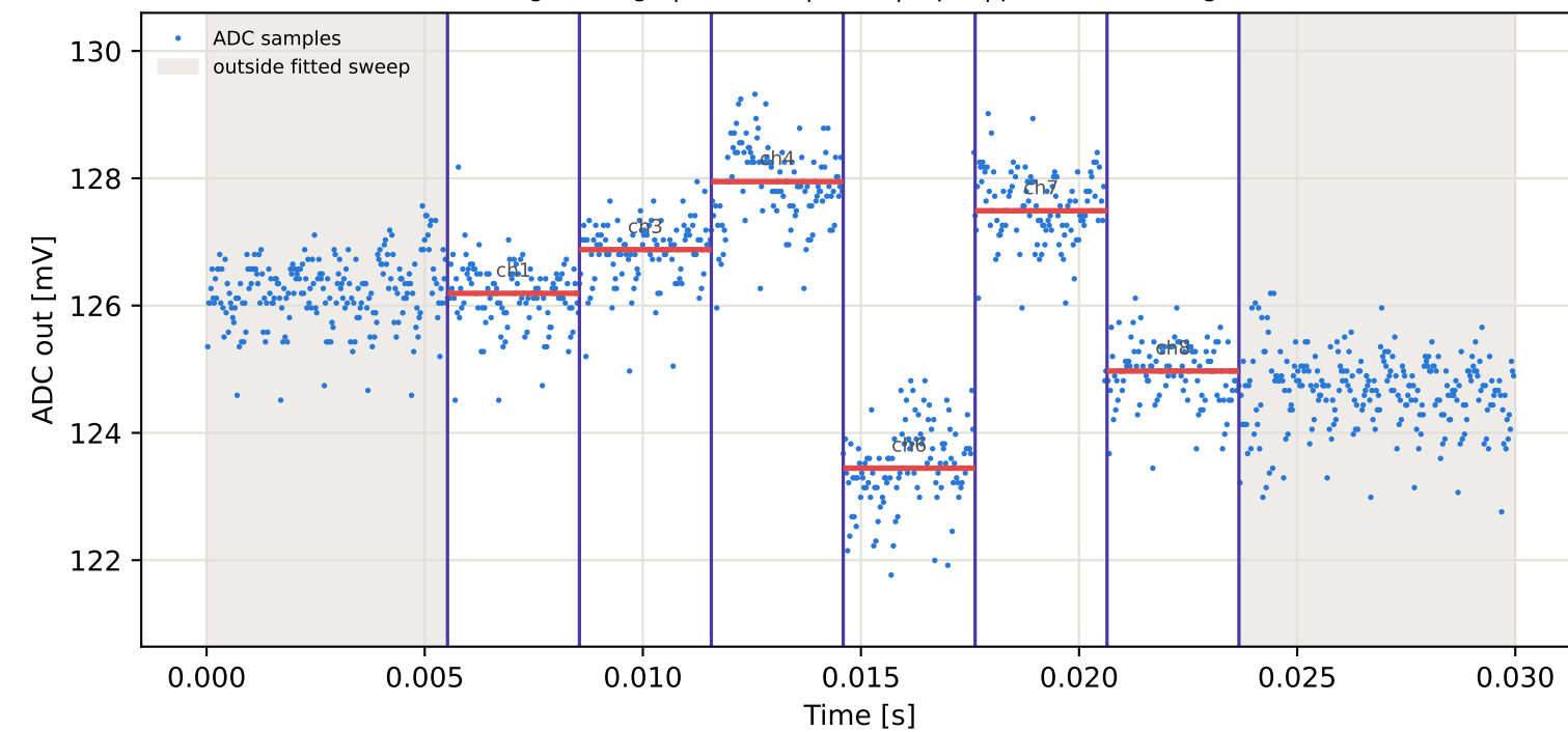
Tag6 &lt;- Tag4 | 975 MHz | run 0 | rep 1 | phase -21.68 deg
