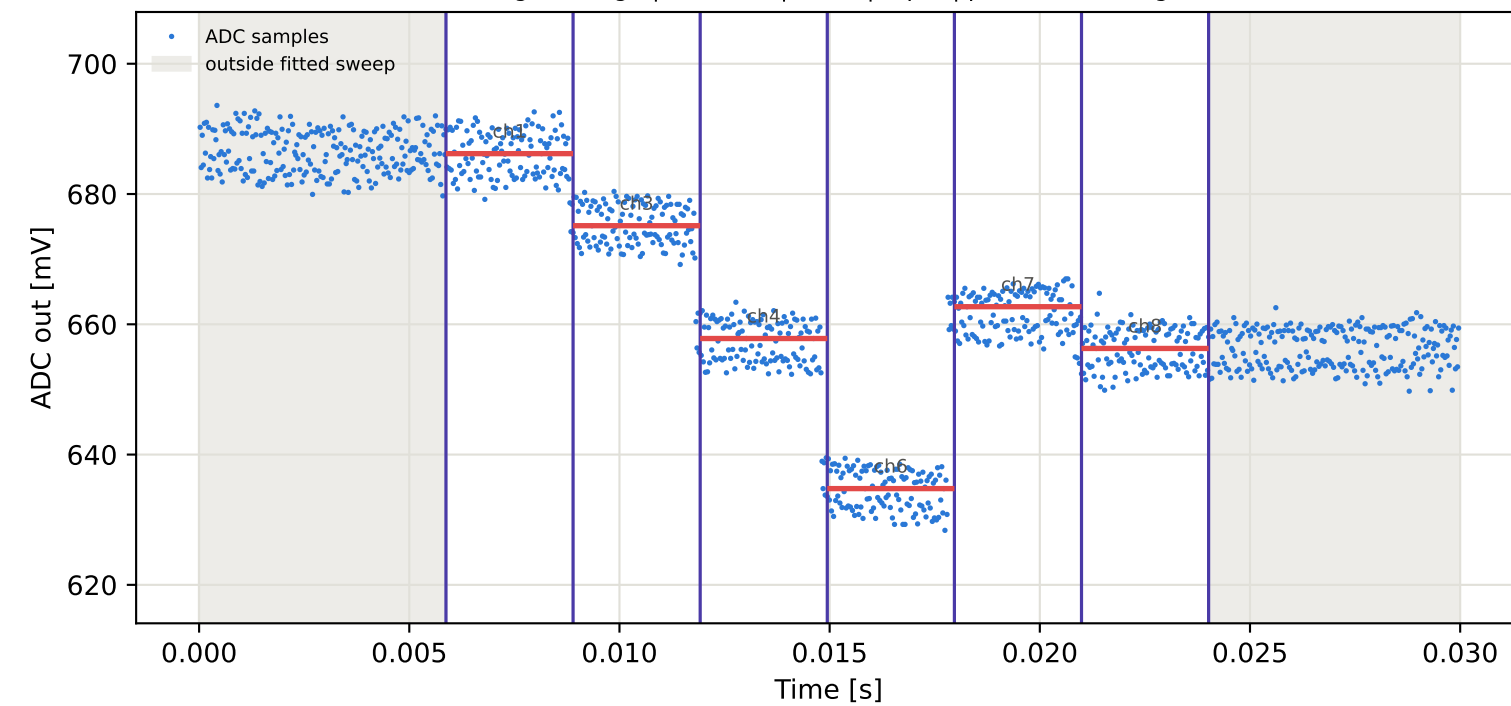
Tag1 &lt;- Tag7 | 885 MHz | run 0 | rep 1 | phase 97.61 deg
