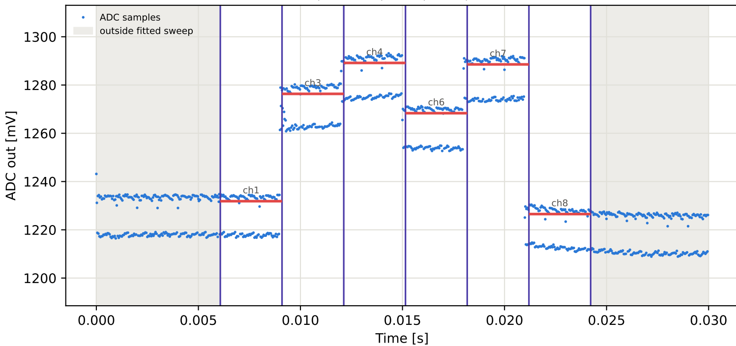
Tag8 &lt;- Tag16 | 875 MHz | run 0 | rep 1 | phase -83.56 deg
