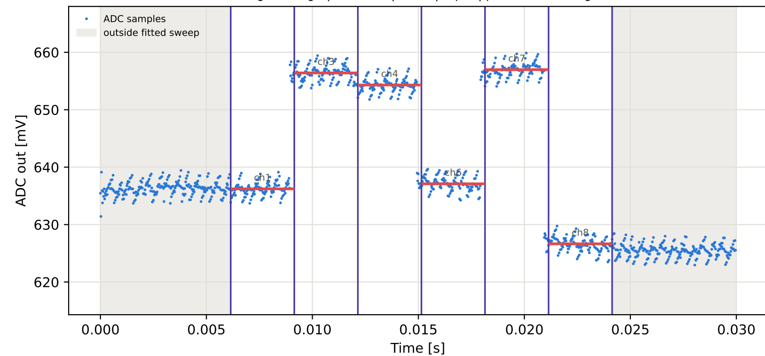
Tag6 &lt;- Tag1 | 865 MHz | run 0 | rep 1 | phase -44.52 deg
