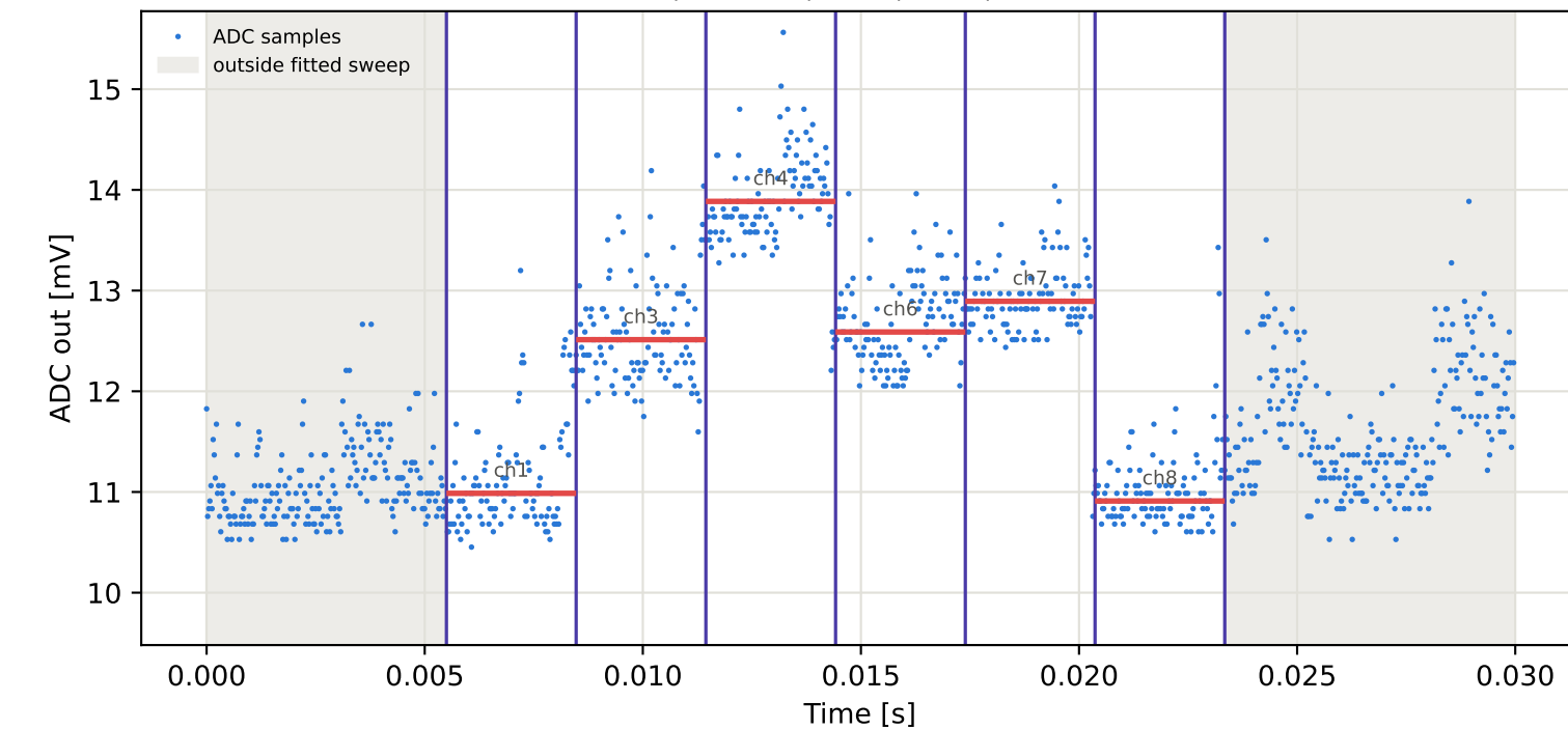
Tag2 &lt;- Tag15 | 955 MHz | run 0 | rep 1 | phase -101.34 deg
