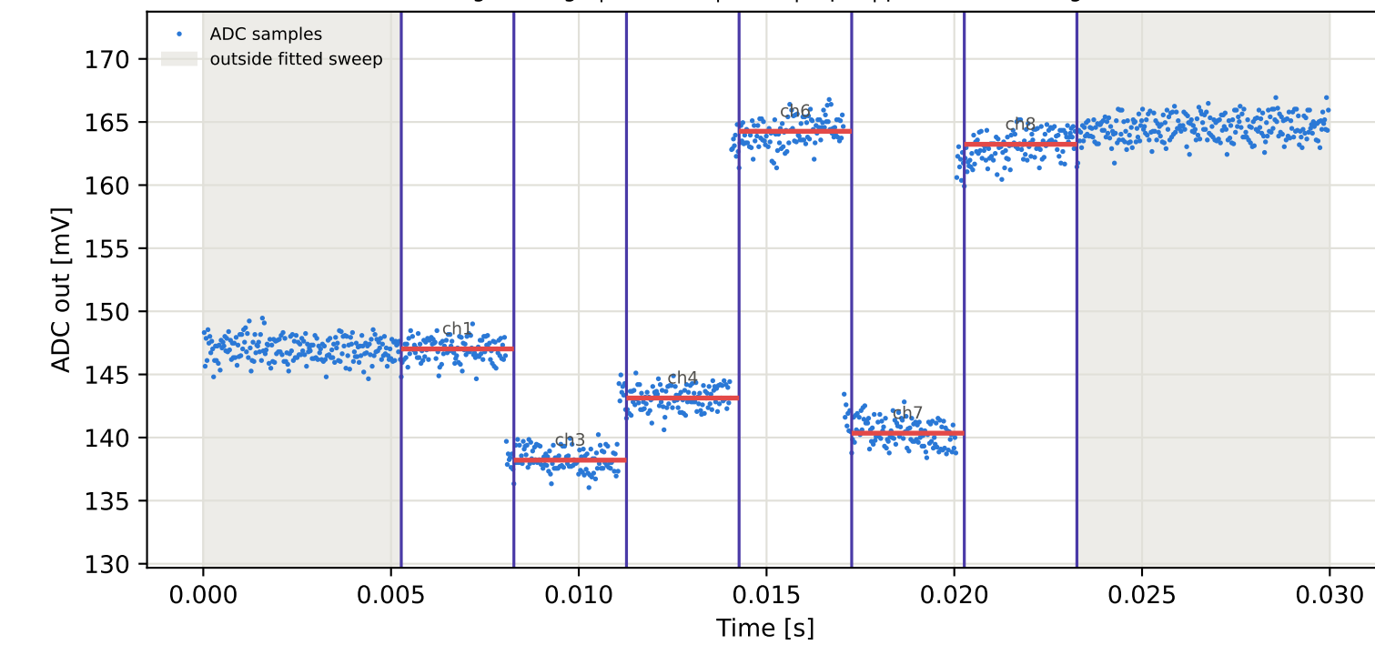
Tag2 &lt;- Tag7 | 885 MHz | run 0 | rep 1 | phase 171.94 deg
