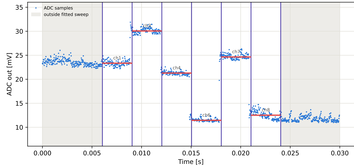
Tag2 &lt;- Tag8 | 845 MHz | run 0 | rep 1 | phase 63.96 deg
