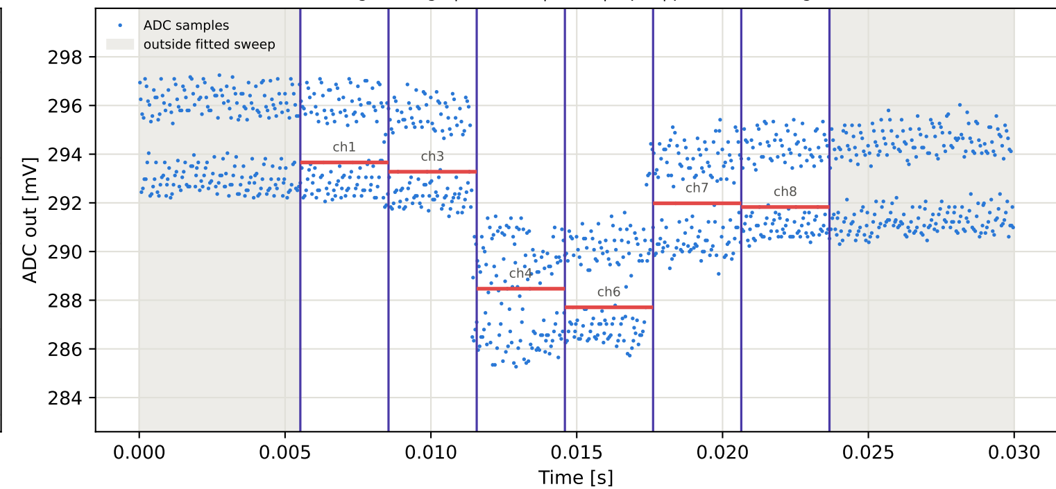
Tag3 &lt;- Tag7 | 985 MHz | run 0 | rep 1 | phase 46.91 deg
