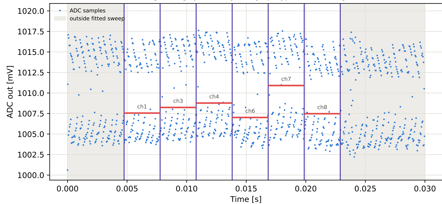
Tag7 &lt;- Tag4 | 895 MHz | run 0 | rep 1 | phase 82.75 deg
