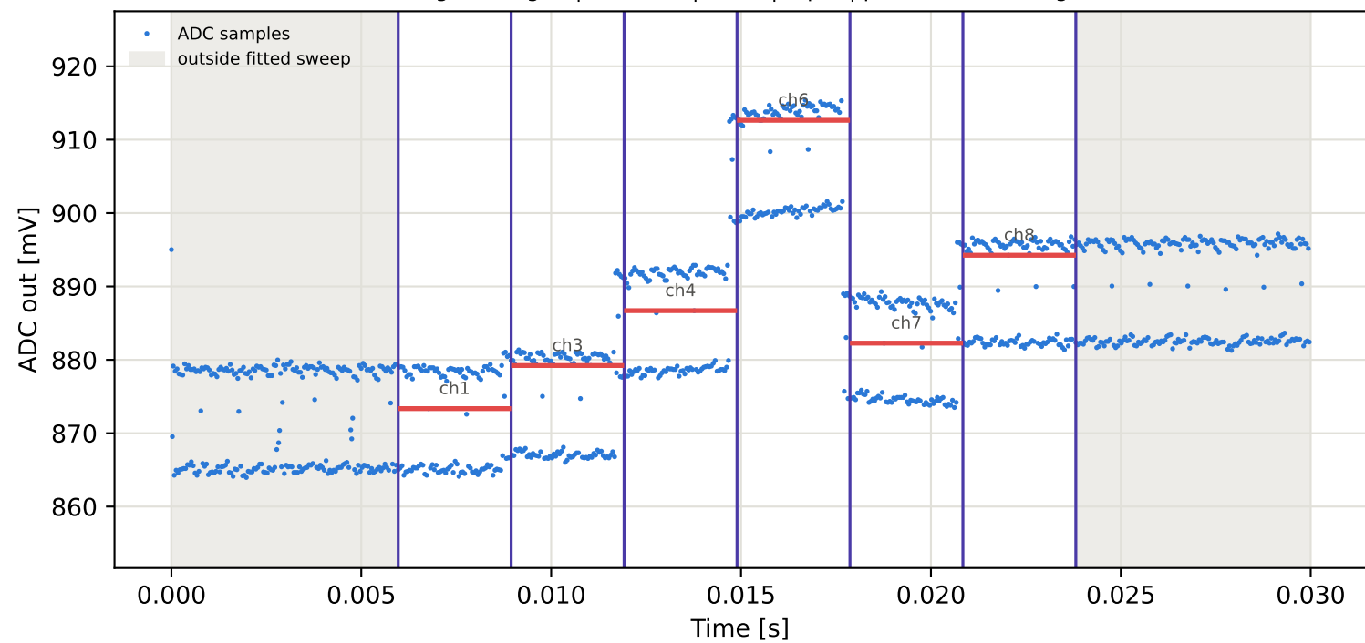
Tag4 &lt;- Tag2 | 905 MHz | run 0 | rep 1 | phase 99.57 deg
