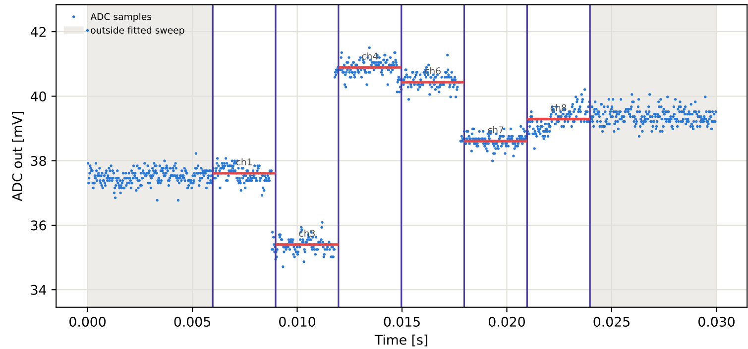
Tag5 &lt;- Tag1 | 775 MHz | run 0 | rep 1 | phase -62.32 deg
