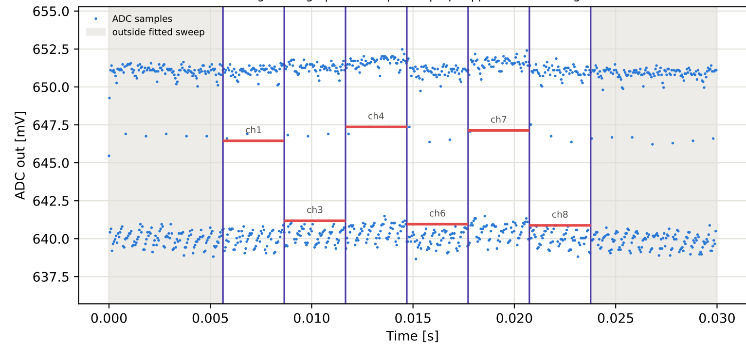
Tag8 &lt;- Tag4 | 985 MHz | run 0 | rep 1 | phase -35.32 deg
