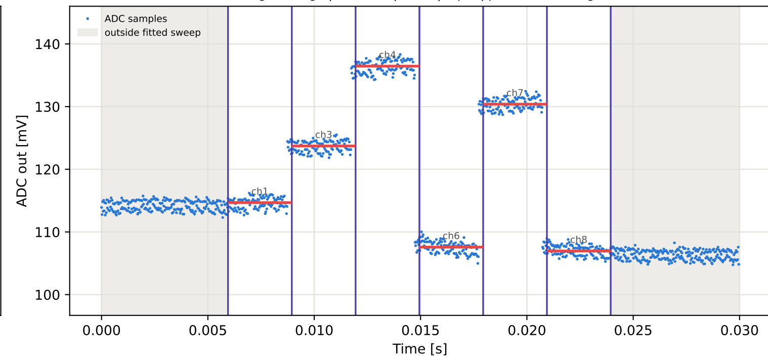
Tag6 &lt;- Tag5 | 975 MHz | run 0 | rep 1 | phase 73.96 deg
