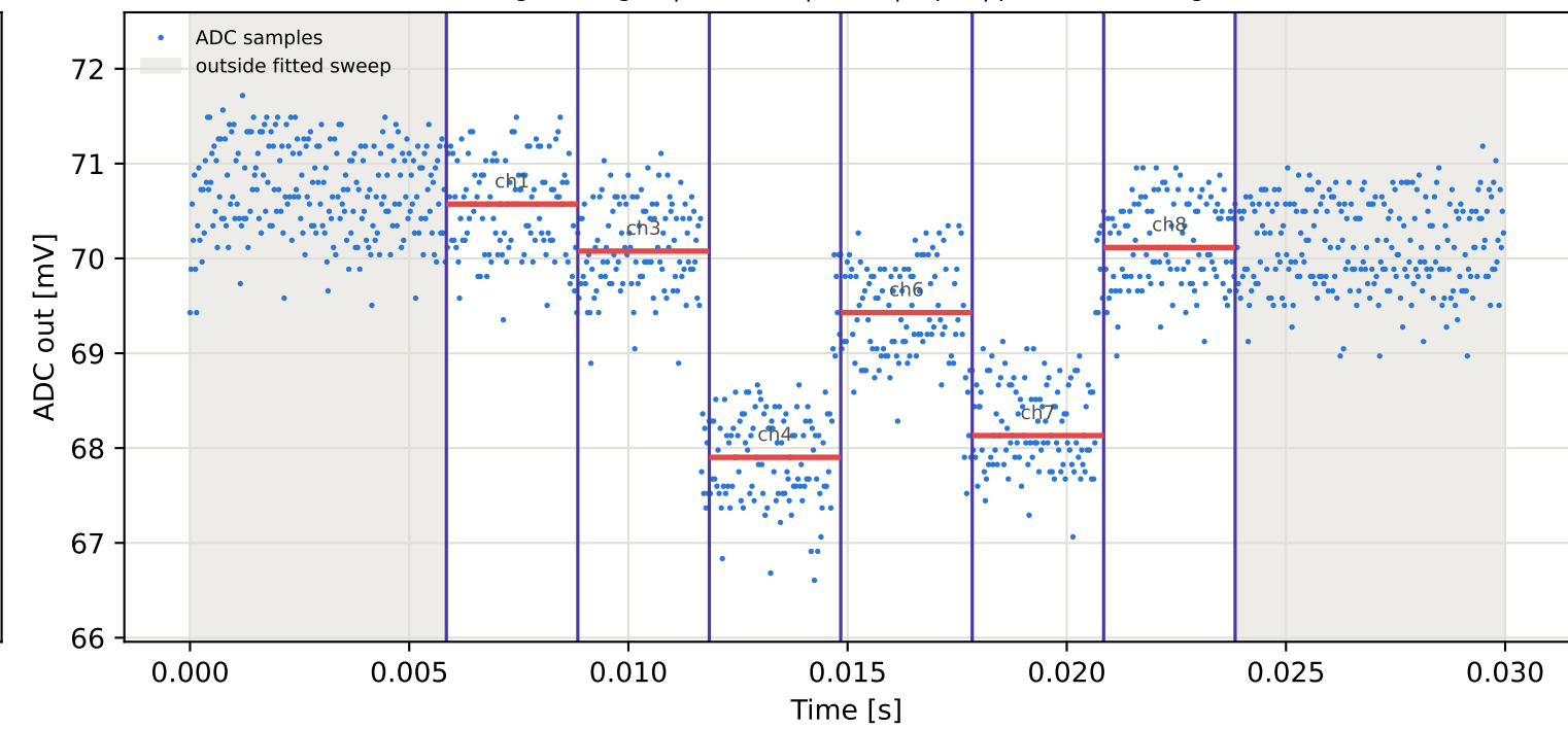
Tag1 &lt;- Tag2 | 805 MHz | run 0 | rep 1 | phase 99.08 deg
