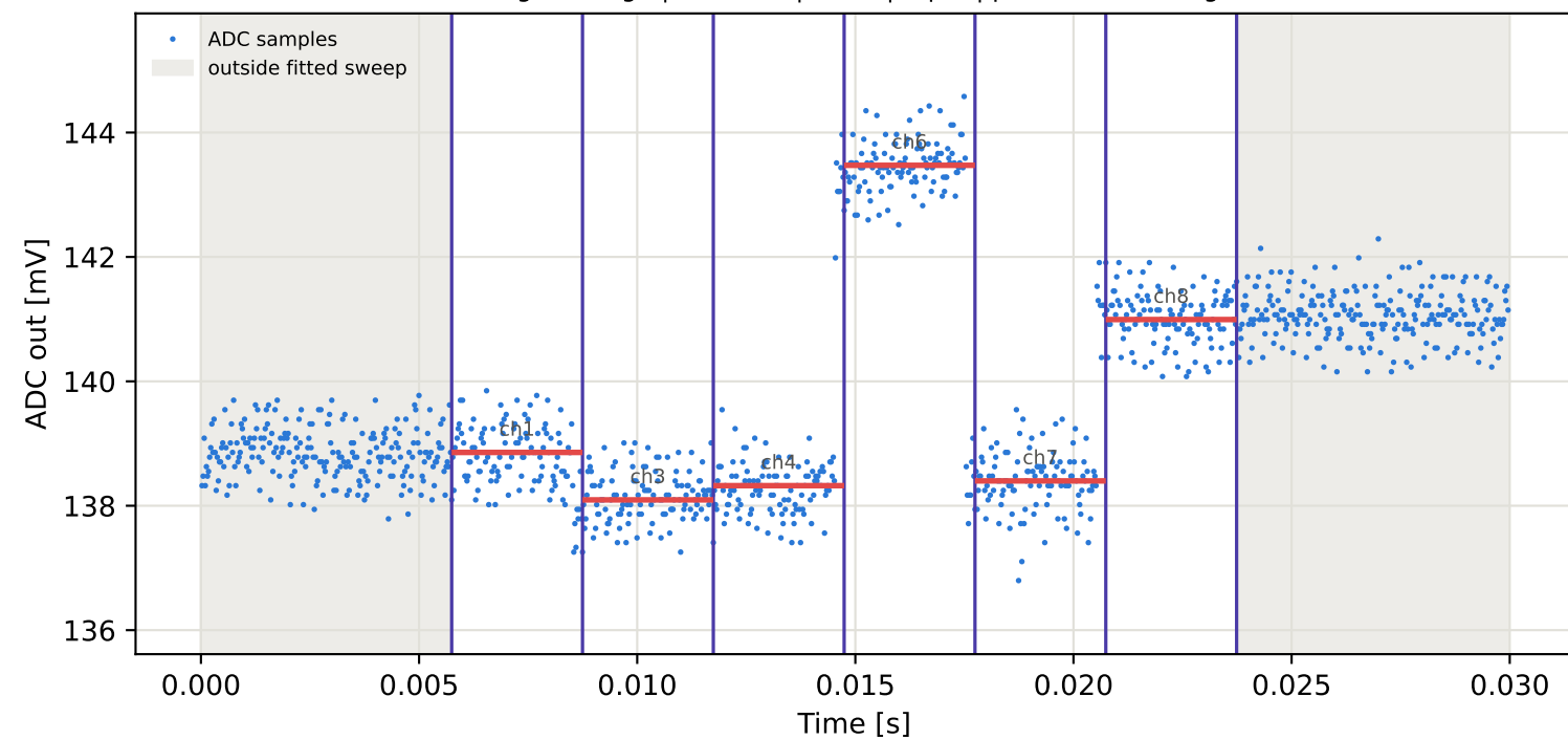
Tag3 &lt;- Tag2 | 935 MHz | run 0 | rep 1 | phase 176.38 deg
