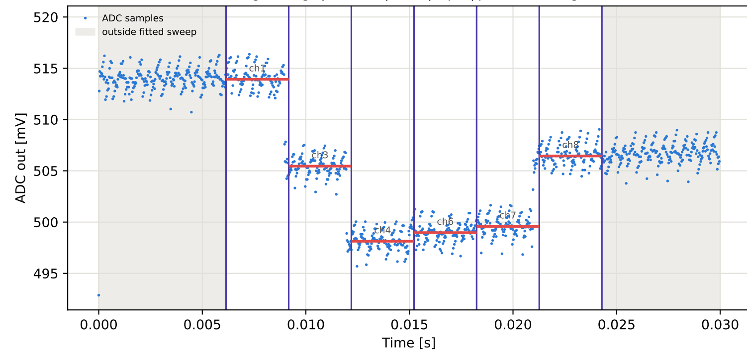
Tag4 &lt;- Tag15 | 865 MHz | run 0 | rep 1 | phase -137.50 deg
