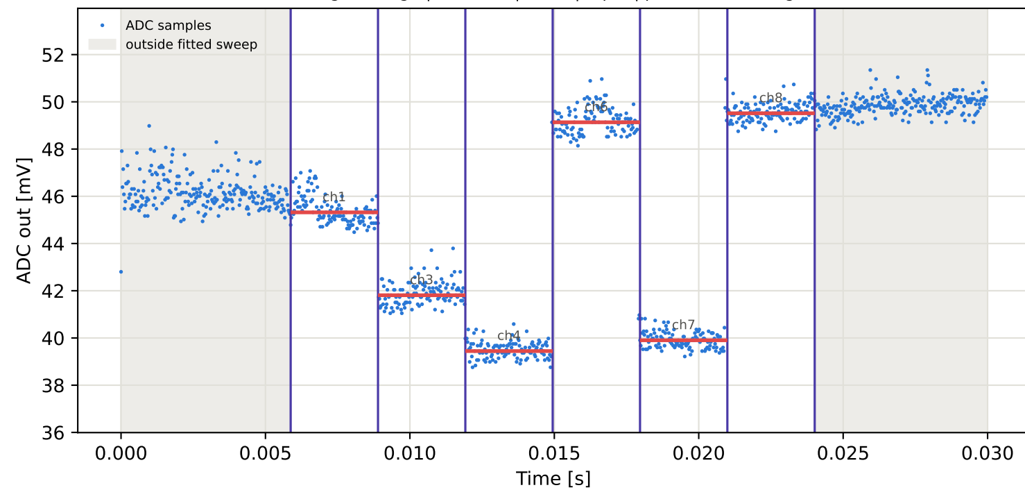
Tag3 &lt;- Tag10 | 935 MHz | run 0 | rep 1 | phase 44.58 deg
