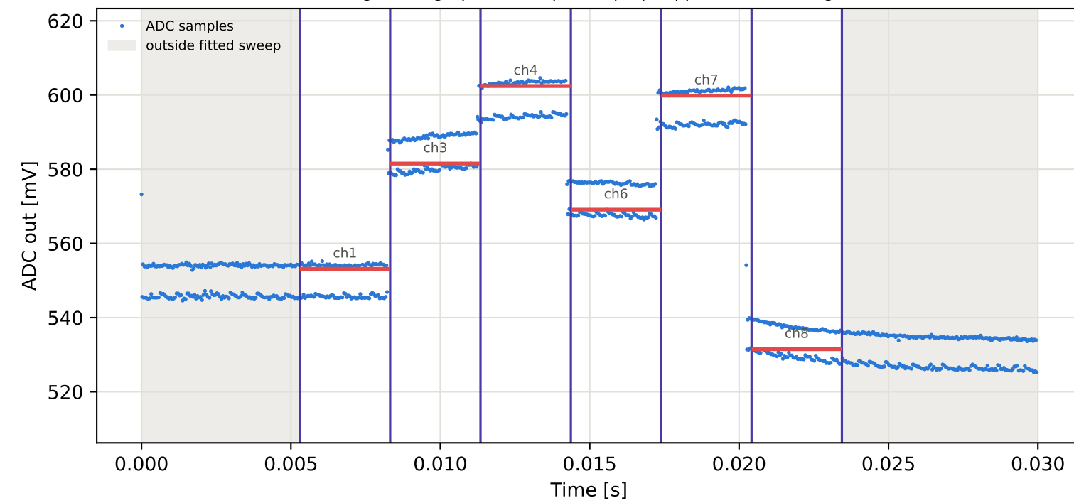
Tag9 &lt;- Tag5 | 875 MHz | run 0 | rep 1 | phase -116.75 deg
