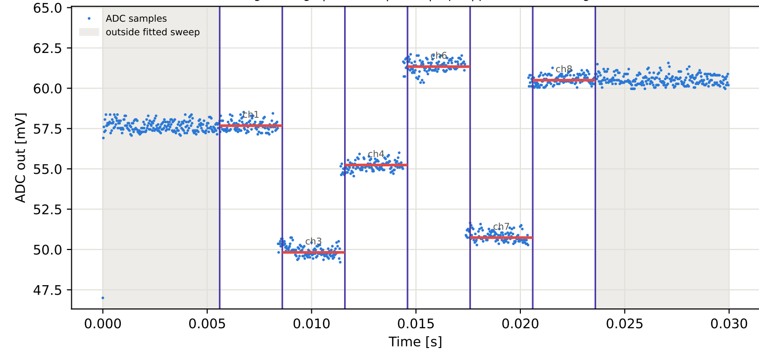
Tag9 &lt;- Tag7 | 775 MHz | run 0 | rep 1 | phase -178.61 deg
