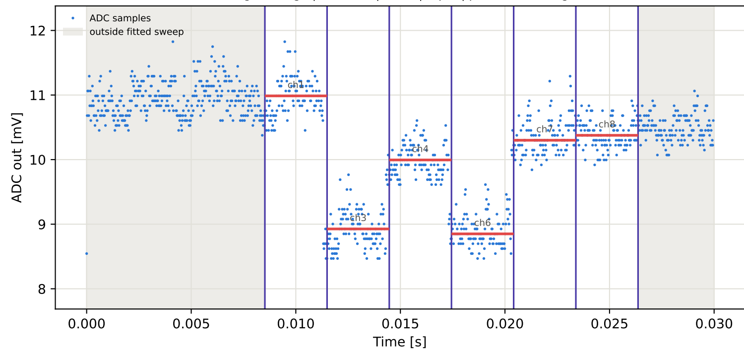
Tag3 &lt;- Tag6 | 775 MHz | run 0 | rep 1 | phase 19.77 deg
