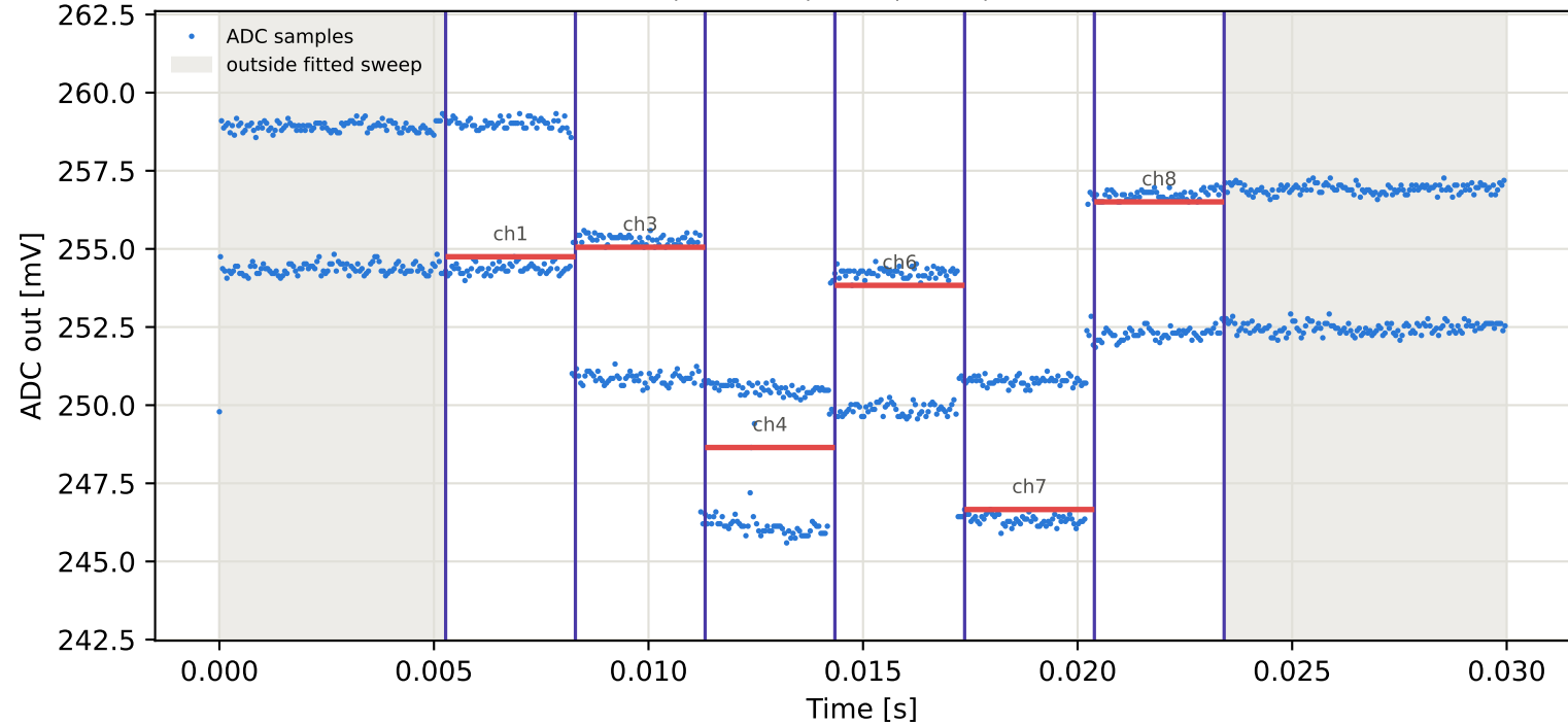
Tag7 &lt;- Tag5 | 835 MHz | run 0 | rep 1 | phase 100.23 deg
