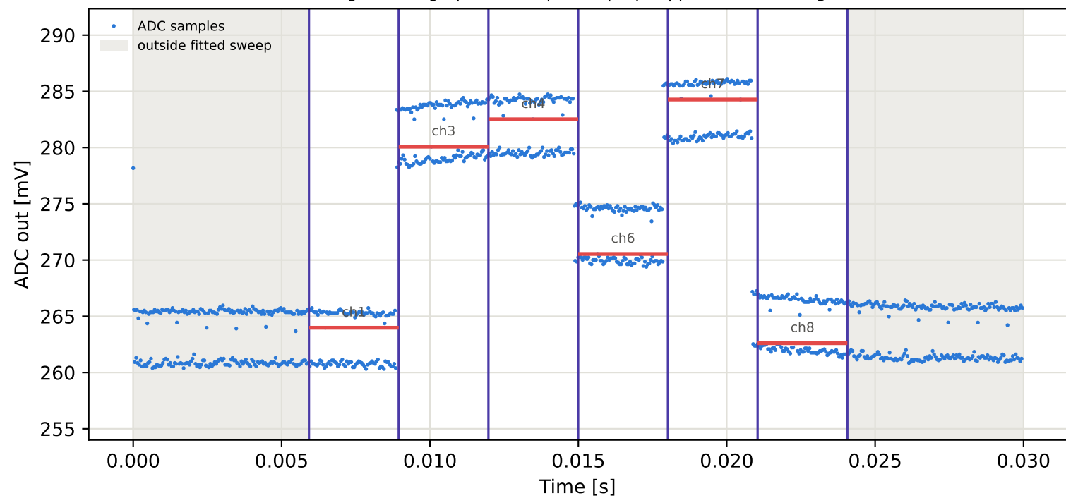
Tag10 &lt;- Tag5 | 845 MHz | run 0 | rep 1 | phase -60.60 deg
