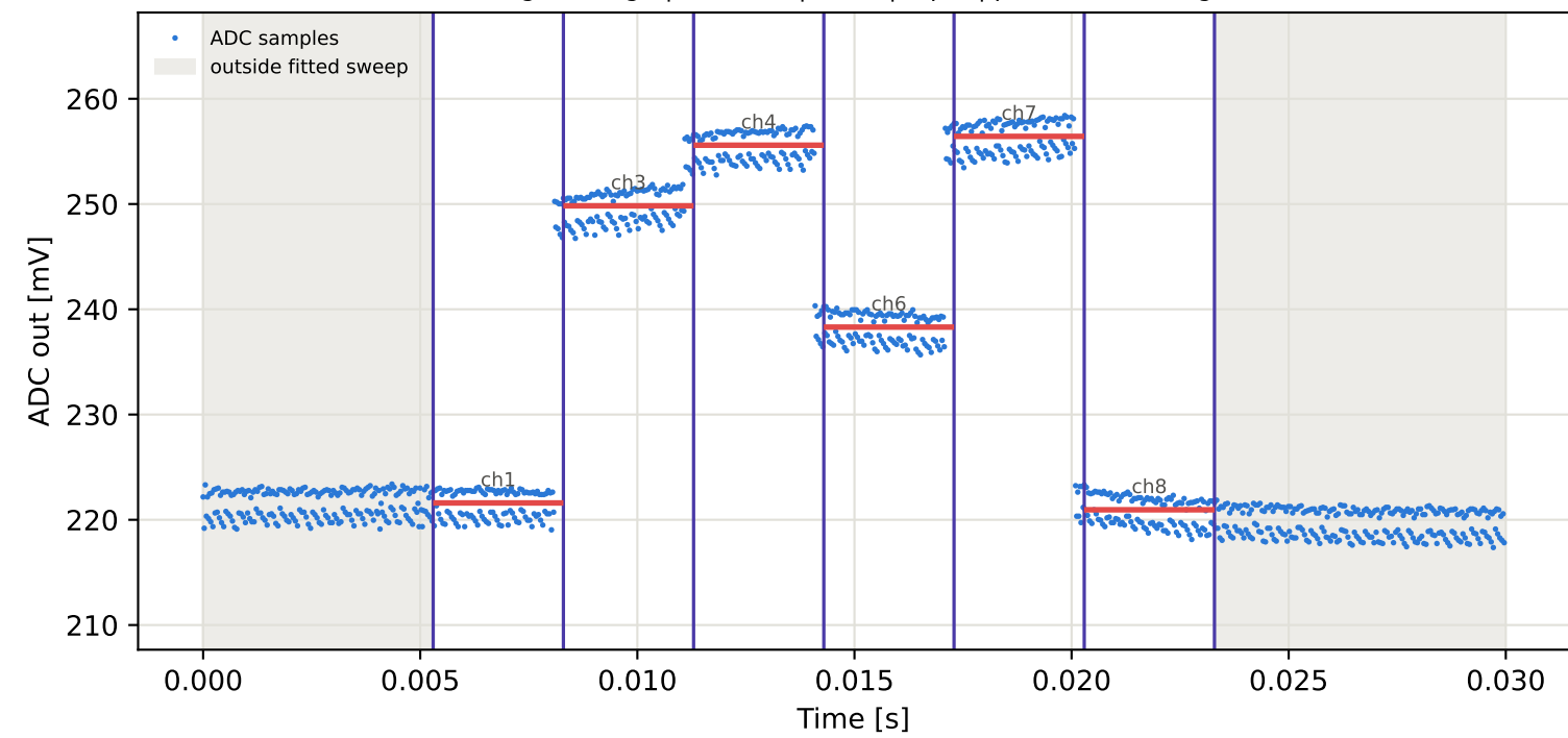
Tag1 &lt;- Tag8 | 855 MHz | run 0 | rep 1 | phase -106.07 deg
