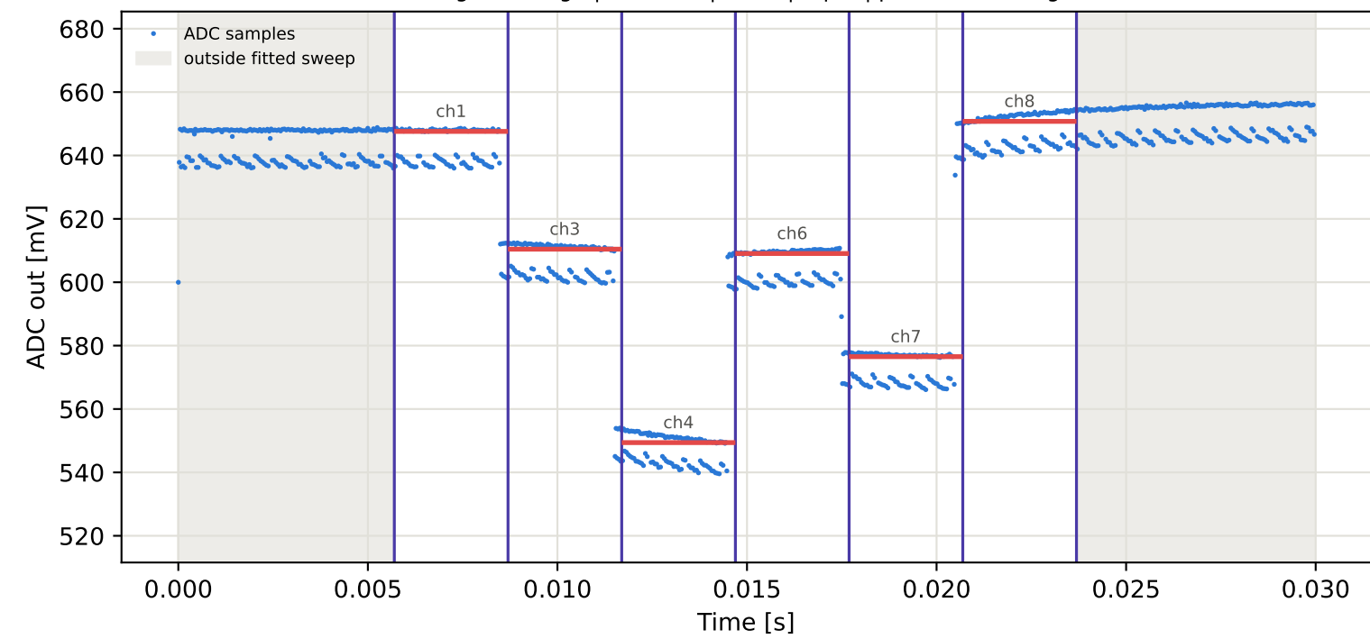
Tag16 &lt;- Tag7 | 935 MHz | run 0 | rep 1 | phase 81.05 deg
