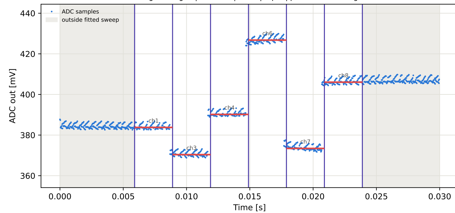
Tag7 &lt;- Tag3 | 985 MHz | run 0 | rep 1 | phase -170.10 deg
