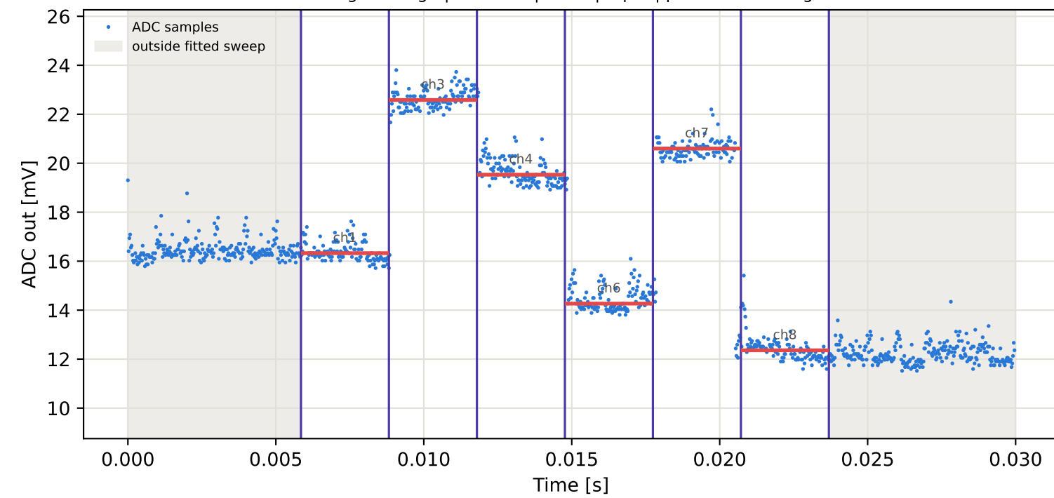
Tag2 &lt;- Tag5 | 845 MHz | run 0 | rep 1 | phase 114.71 deg
