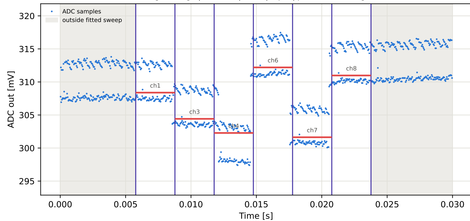
Tag9 &lt;- Tag6 | 985 MHz | run 0 | rep 1 | phase 28.70 deg
