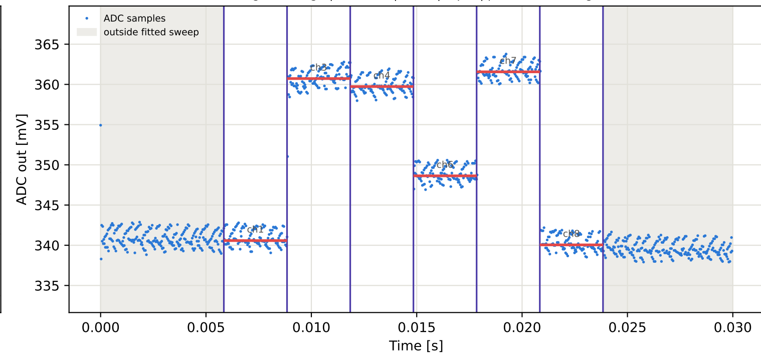
Tag16 &lt;- Tag5 | 845 MHz | run 0 | rep 1 | phase 43.27 deg
