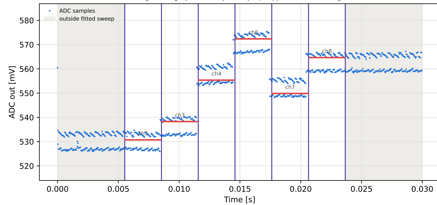
Tag7 &lt;- Tag5 | 865 MHz | run 0 | rep 1 | phase -147.59 deg
