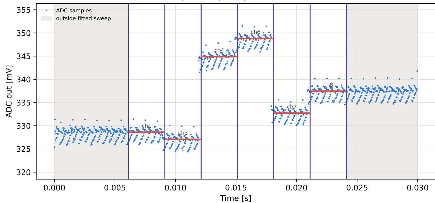
Tag4 &lt;- Tag8 | 985 MHz | run 0 | rep 1 | phase 94.05 deg
