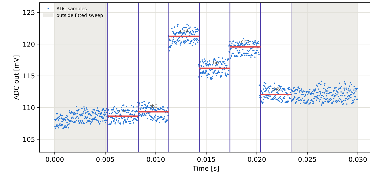
Tag6 &lt;- Tag1 | 825 MHz | run 0 | rep 1 | phase -103.35 deg
