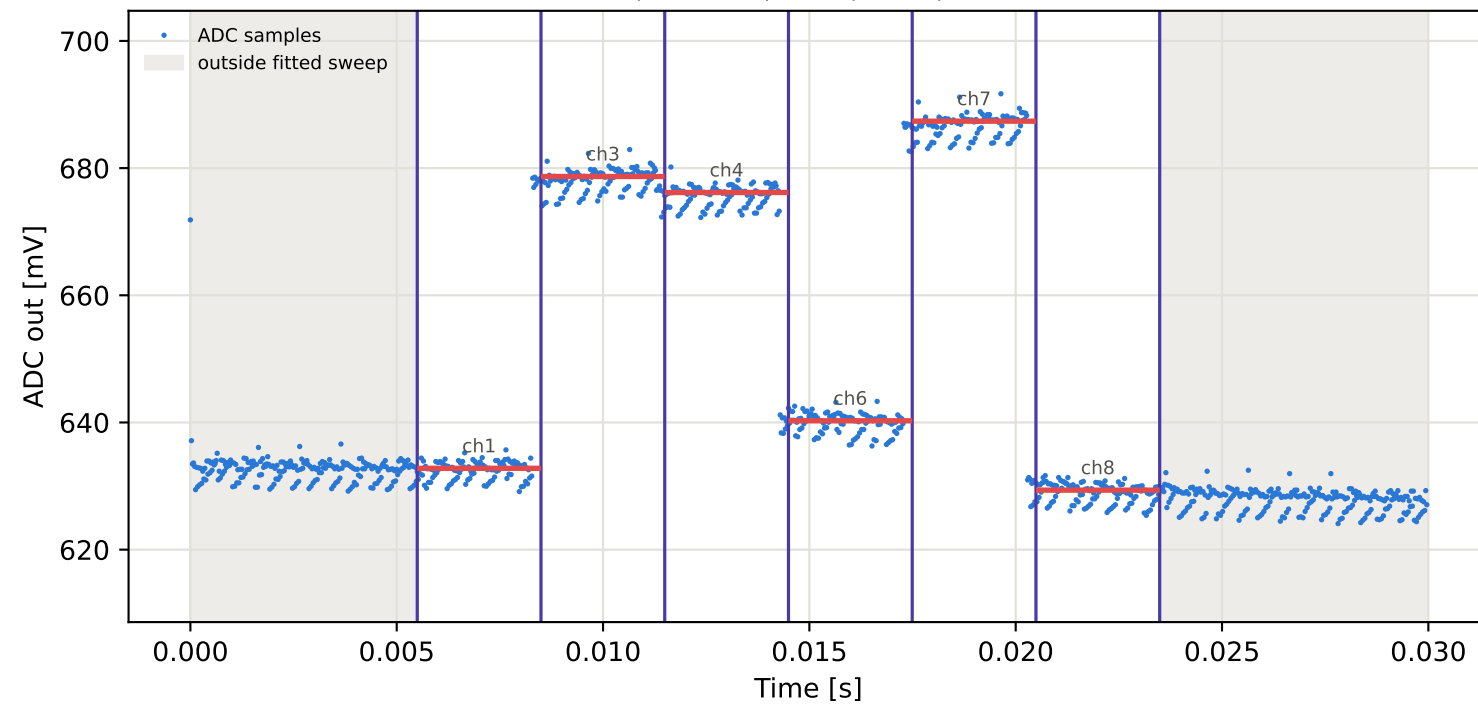
Tag8 &lt;- Tag15 | 835 MHz | run 0 | rep 1 | phase -43.38 deg
