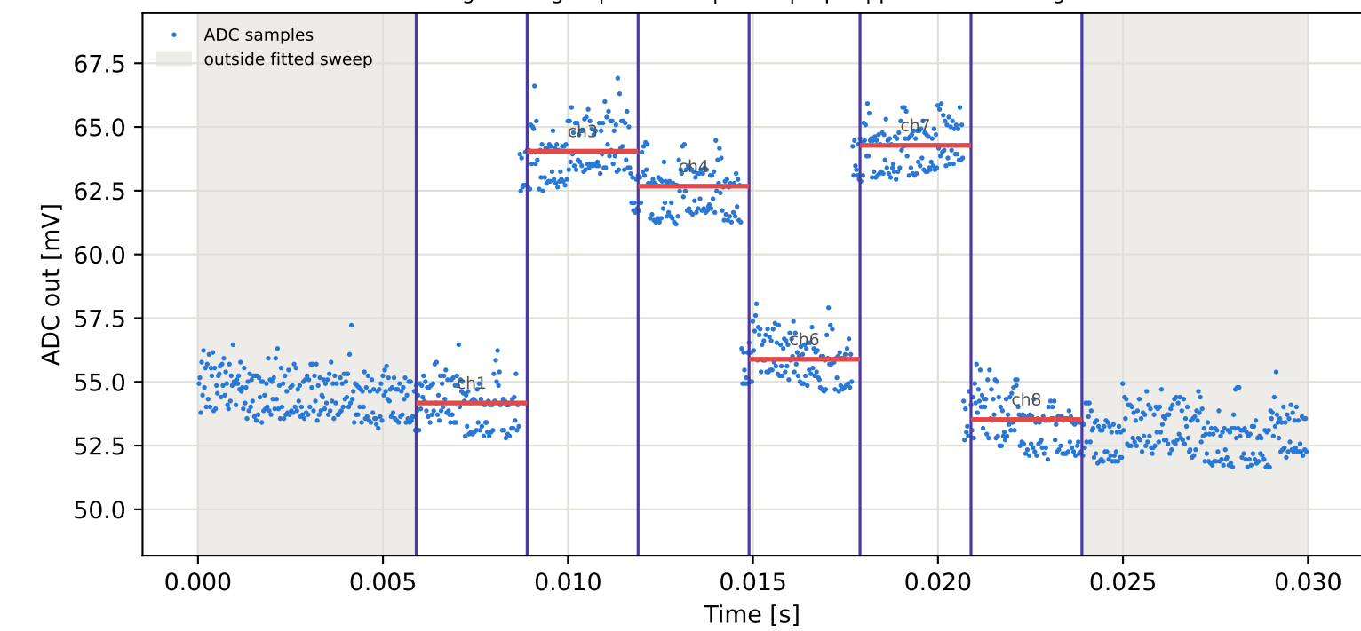
Tag2 &lt;- Tag16 | 835 MHz | run 0 | rep 1 | phase -43.76 deg
