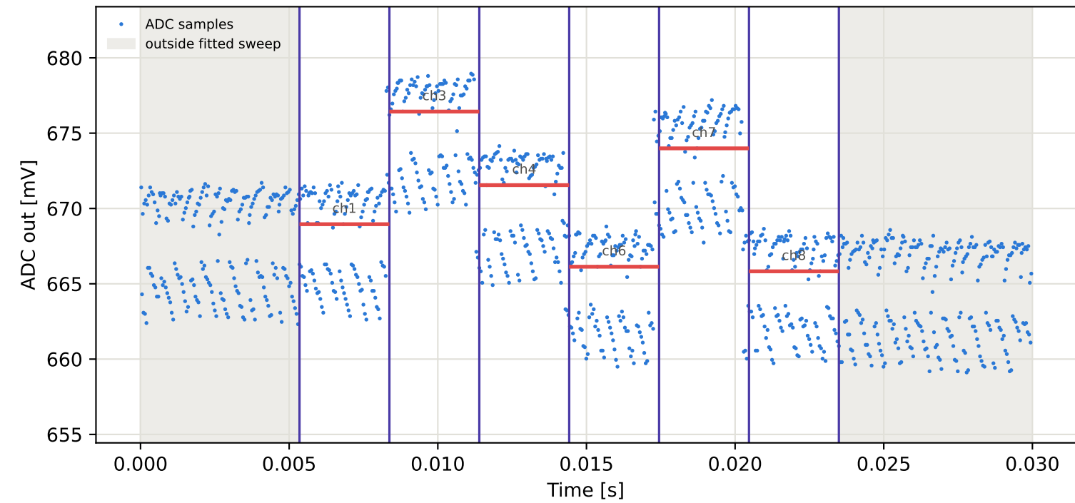
Tag8 &lt;- Tag7 | 835 MHz | run 0 | rep 1 | phase -54.63 deg
