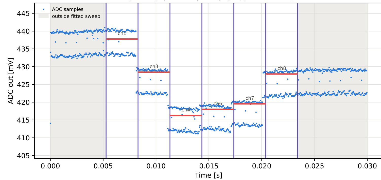
Tag5 &lt;- Tag8 | 855 MHz | run 0 | rep 1 | phase -87.36 deg
