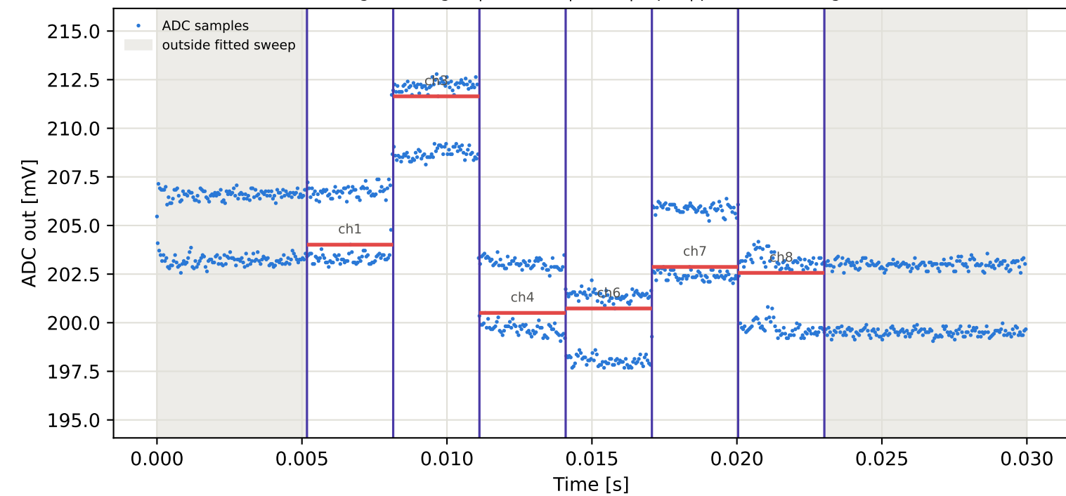
Tag15 &lt;- Tag3 | 805 MHz | run 0 | rep 1 | phase -103.60 deg
