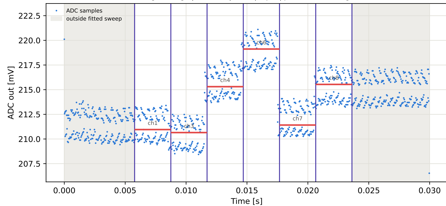
Tag5 &lt;- Tag9 | 995 MHz | run 0 | rep 1 | phase 110.96 deg
