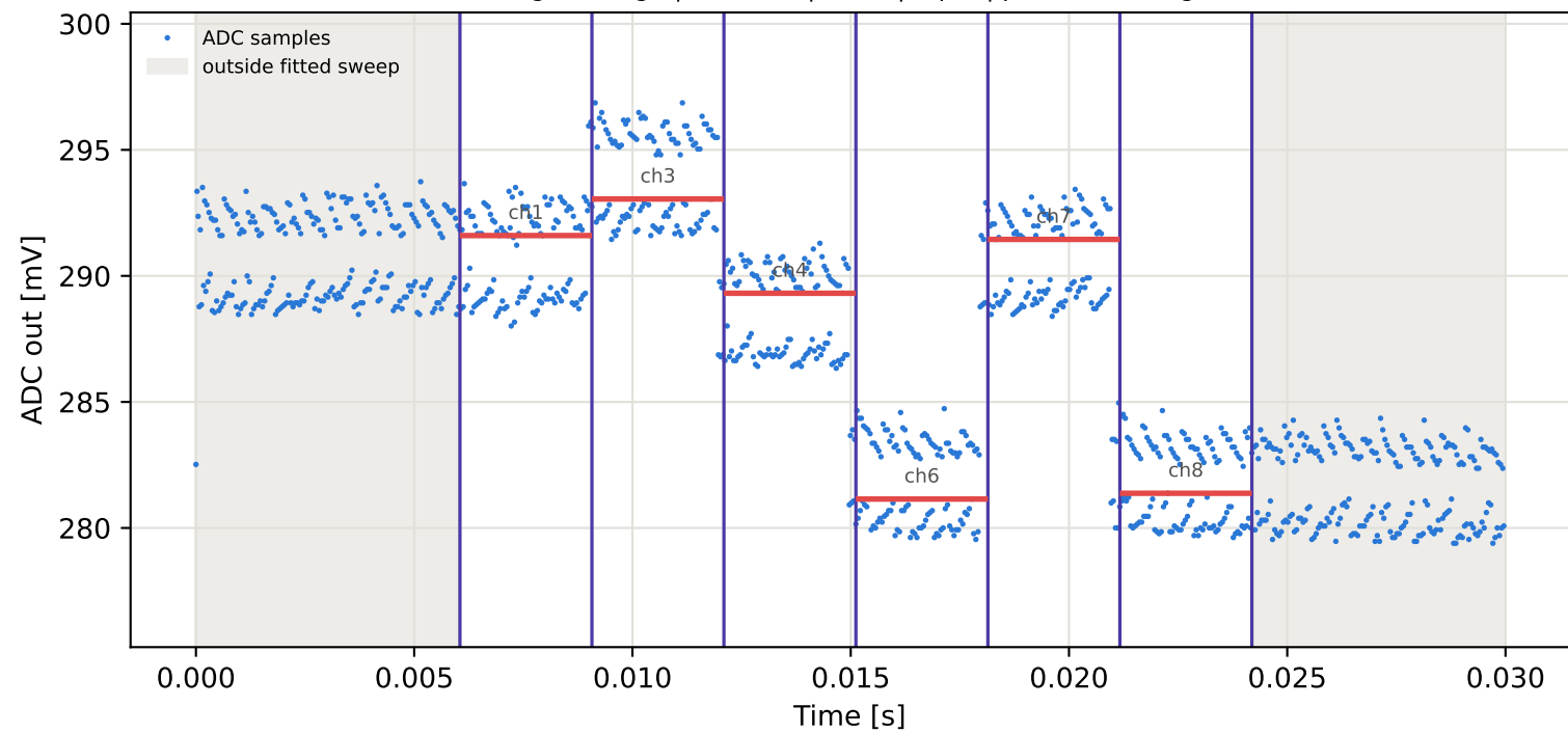
Tag9 &lt;- Tag15 | 865 MHz | run 0 | rep 1 | phase -138.02 deg
