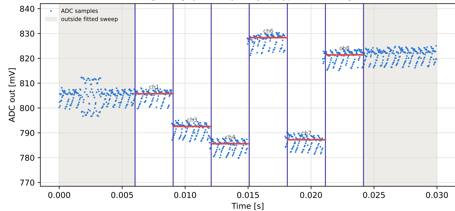
Tag8 &lt;- Tag5 | 945 MHz | run 0 | rep 1 | phase 159.12 deg
