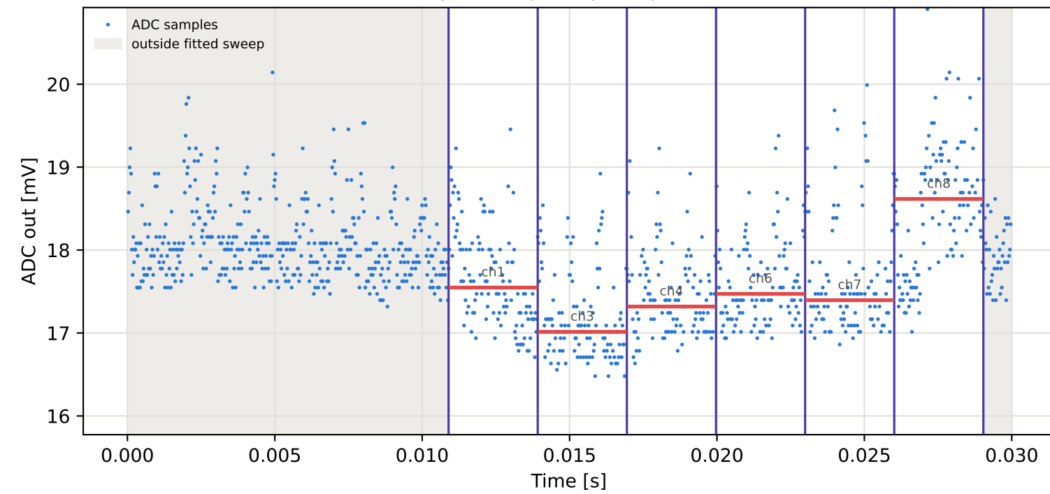
Tag2 &lt;- Tag7 | 845 MHz | run 0 | rep 1 | phase 138.44 deg
