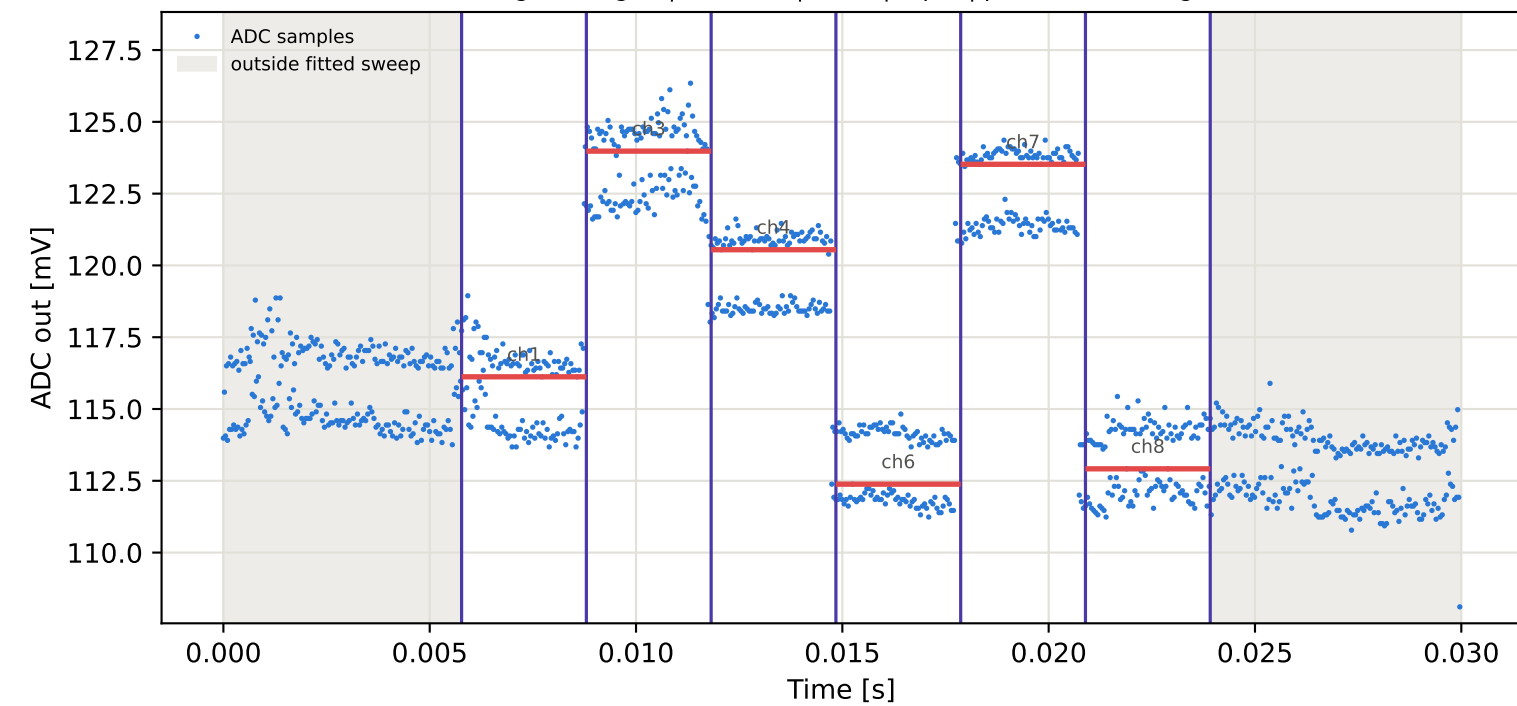
Tag6 &lt;- Tag2 | 825 MHz | run 0 | rep 1 | phase 130.70 deg
