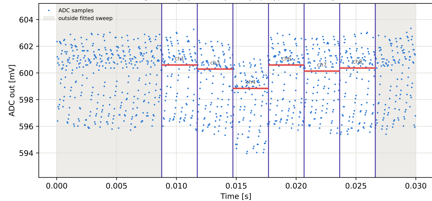
Tag16 &lt;- Tag4 | 965 MHz | run 0 | rep 1 | phase 22.99 deg
