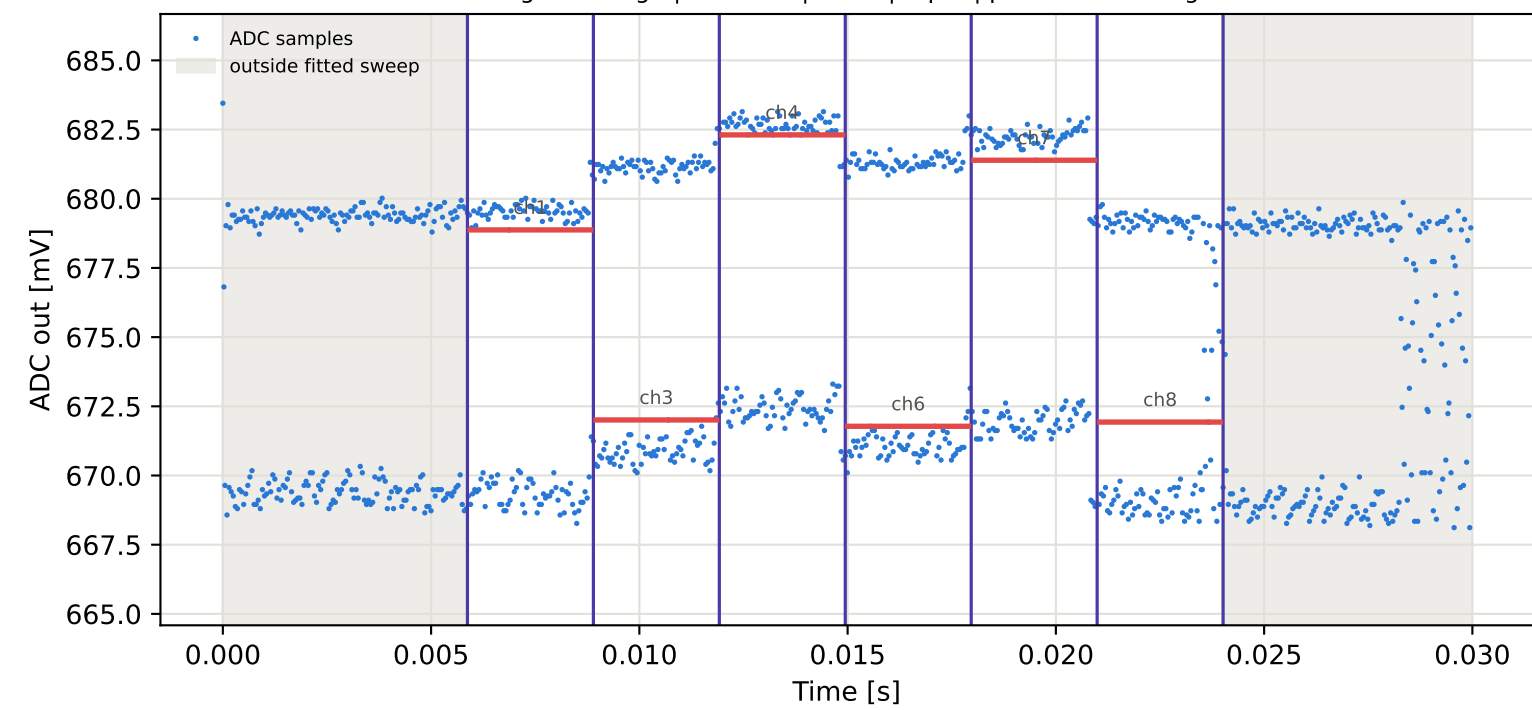
Tag15 &lt;- Tag4 | 835 MHz | run 0 | rep 1 | phase 73.87 deg
