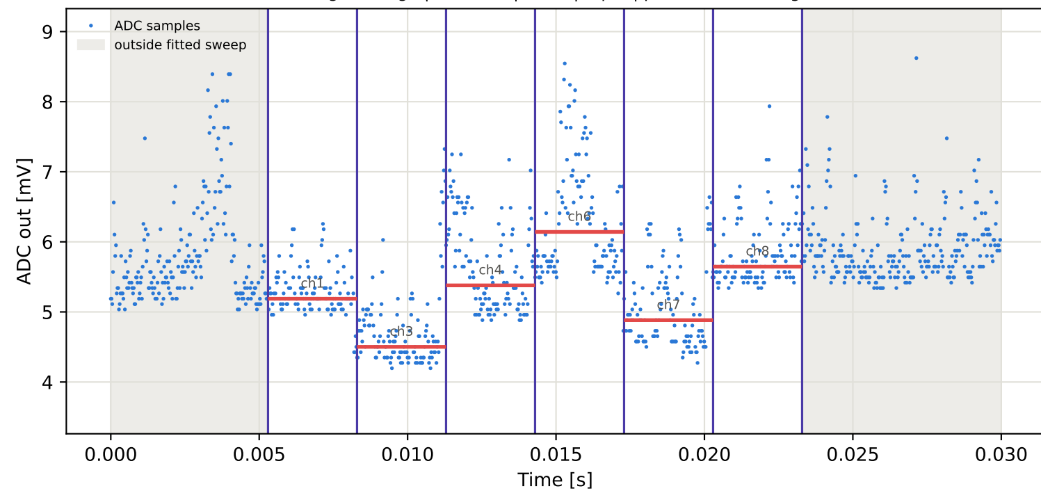
Tag2 &lt;- Tag8 | 775 MHz | run 0 | rep 1 | phase 106.31 deg
