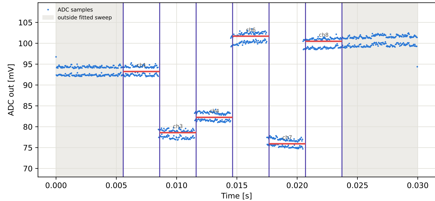
Tag8 &lt;- Tag7 | 785 MHz | run 0 | rep 1 | phase 131.65 deg
