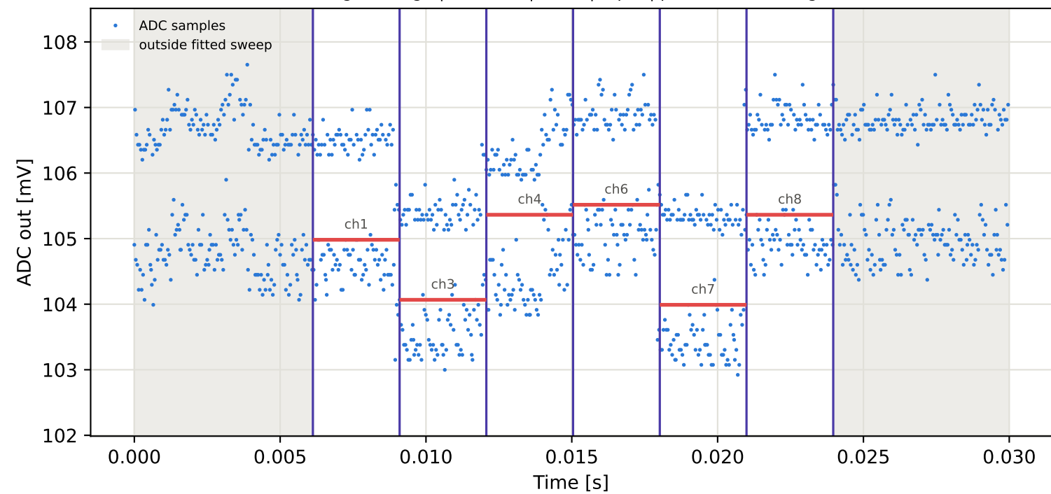
Tag8 &lt;- Tag5 | 795 MHz | run 0 | rep 1 | phase -133.56 deg
