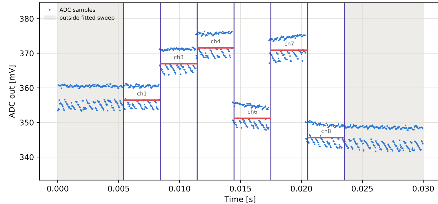
Tag7 &lt;- Tag10 | 915 MHz | run 0 | rep 1 | phase 48.02 deg
