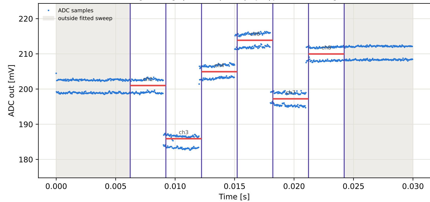
Tag16 &lt;- Tag1 | 805 MHz | run 0 | rep 1 | phase 109.84 deg
