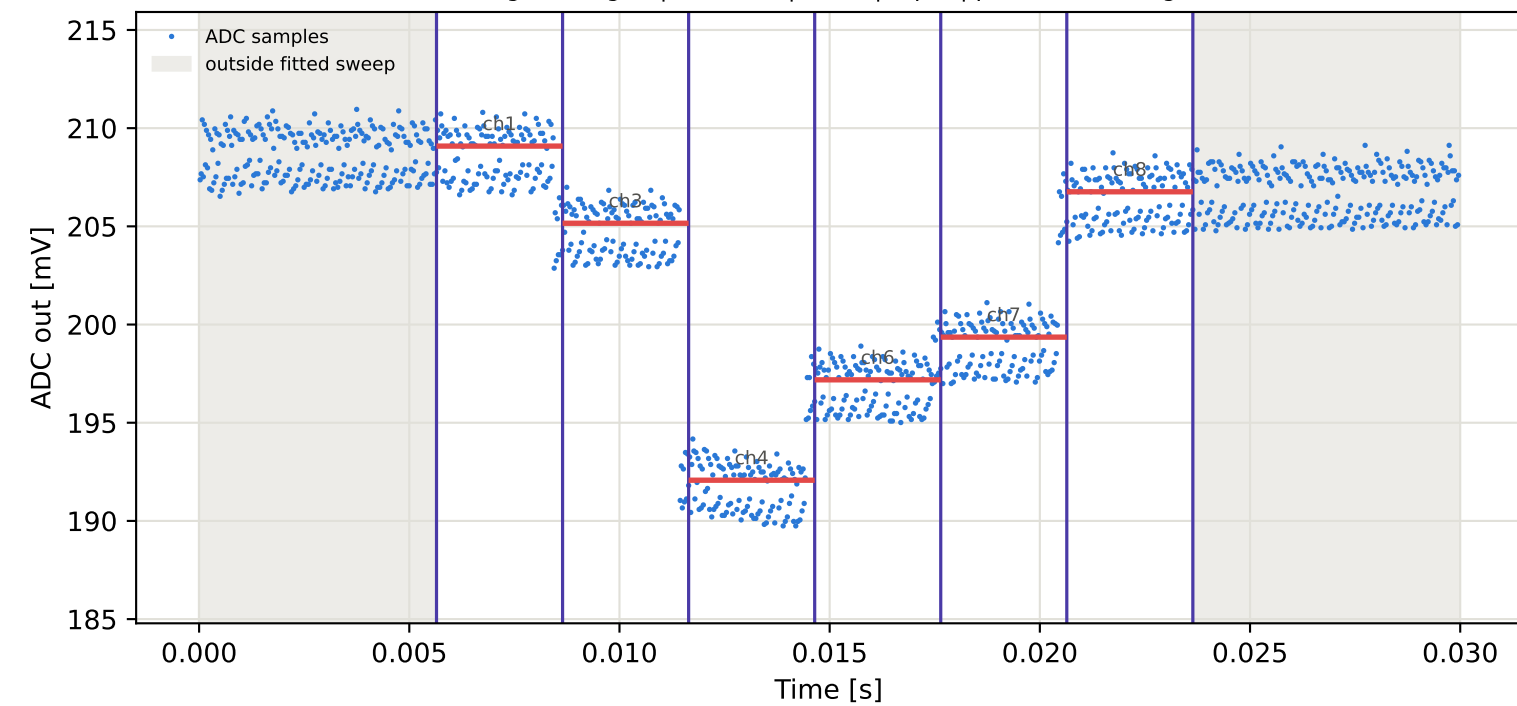
Tag1 &lt;- Tag16 | 965 MHz | run 0 | rep 1 | phase -38.34 deg
