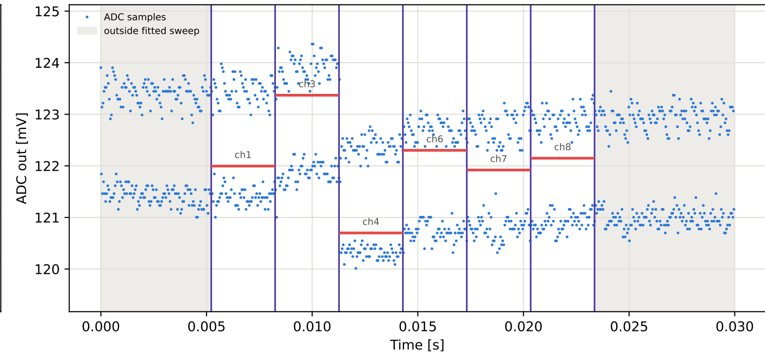
Tag7 &lt;- Tag6 | 775 MHz | run 0 | rep 1 | phase -144.15 deg
