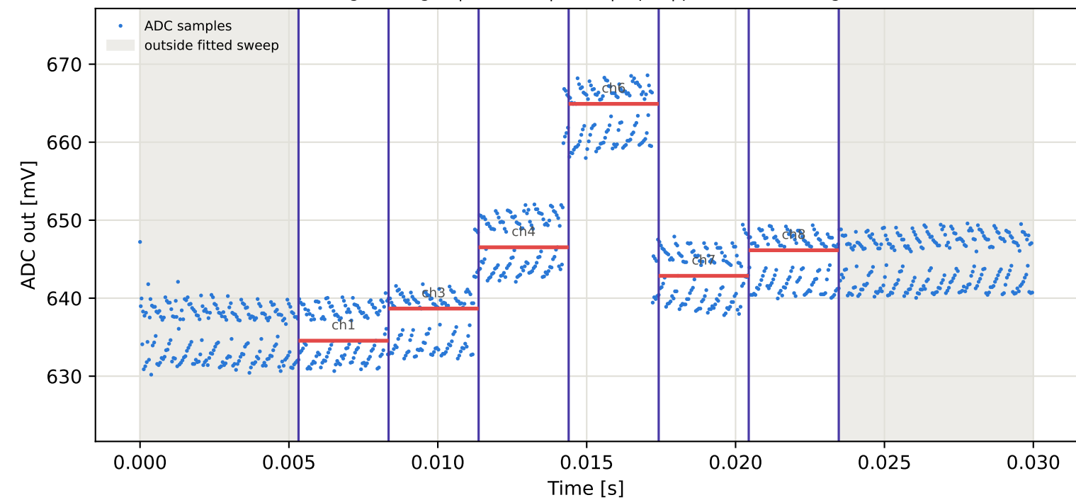
Tag4 &lt;- Tag16 | 925 MHz | run 0 | rep 1 | phase -4.72 deg
