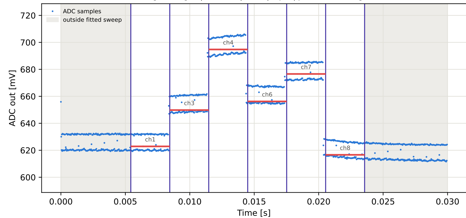
Tag5 &lt;- Tag2 | 945 MHz | run 0 | rep 1 | phase 126.72 deg
