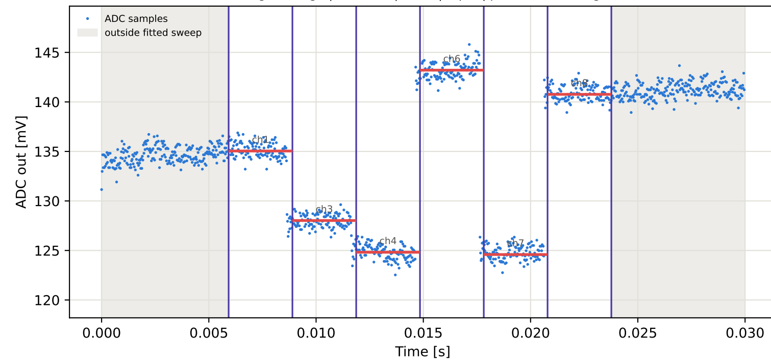
Tag6 &lt;- Tag9 | 975 MHz | run 0 | rep 1 | phase 10.44 deg
