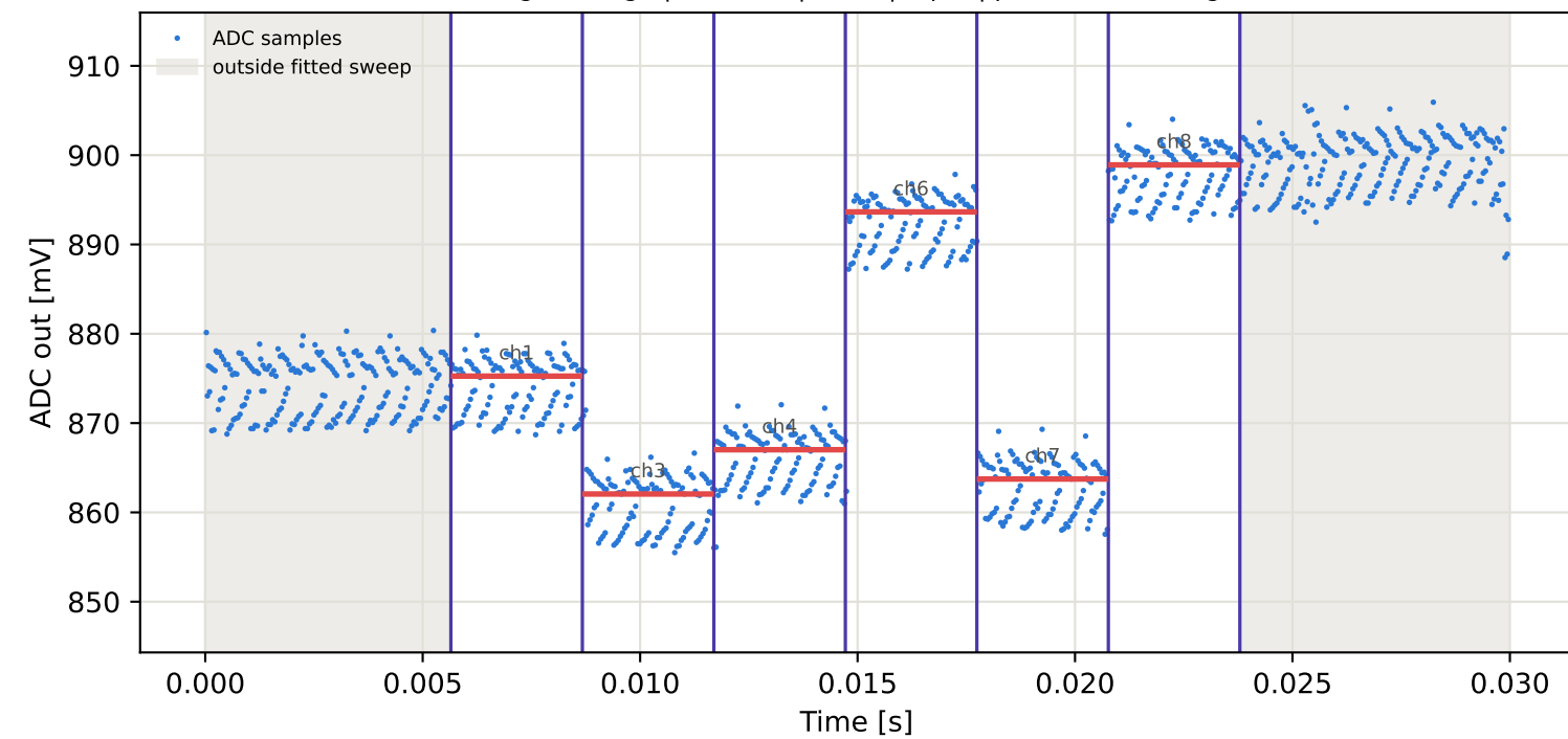
Tag8 &lt;- Tag10 | 875 MHz | run 0 | rep 1 | phase -88.85 deg
