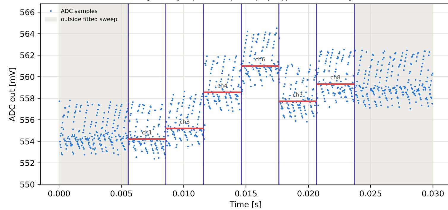
Tag7 &lt;- Tag10 | 865 MHz | run 0 | rep 1 | phase -141.26 deg
