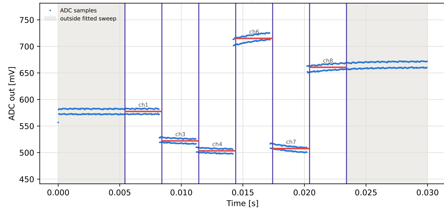
Tag5 &lt;- Tag4 | 935 MHz | run 0 | rep 1 | phase 157.41 deg
