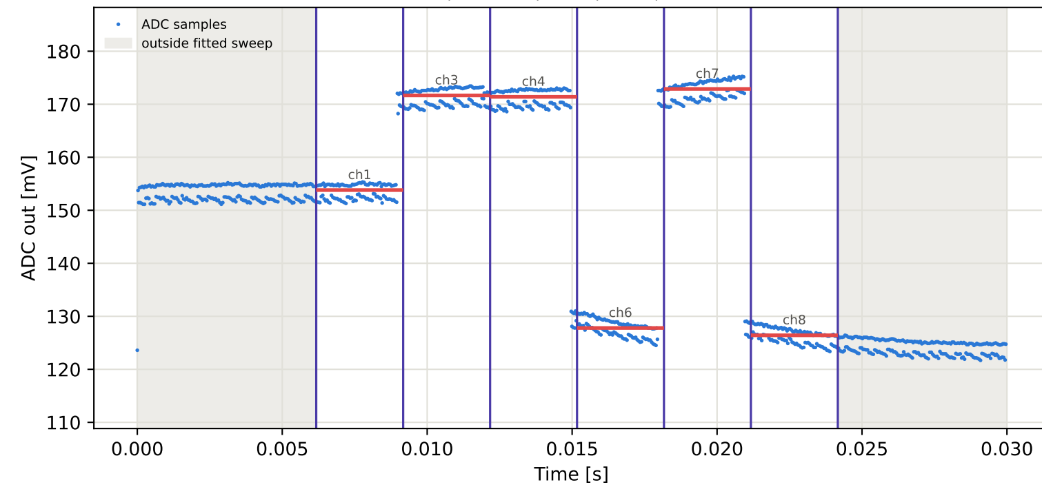
Tag9 &lt;- Tag7 | 895 MHz | run 0 | rep 1 | phase -23.16 deg
