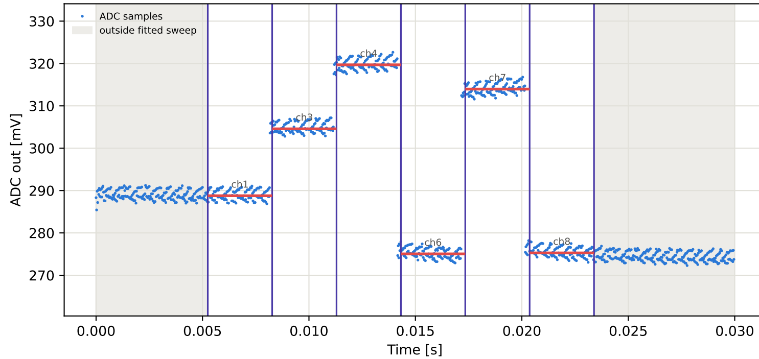
Tag4 &lt;- Tag2 | 965 MHz | run 0 | rep 1 | phase -61.80 deg
