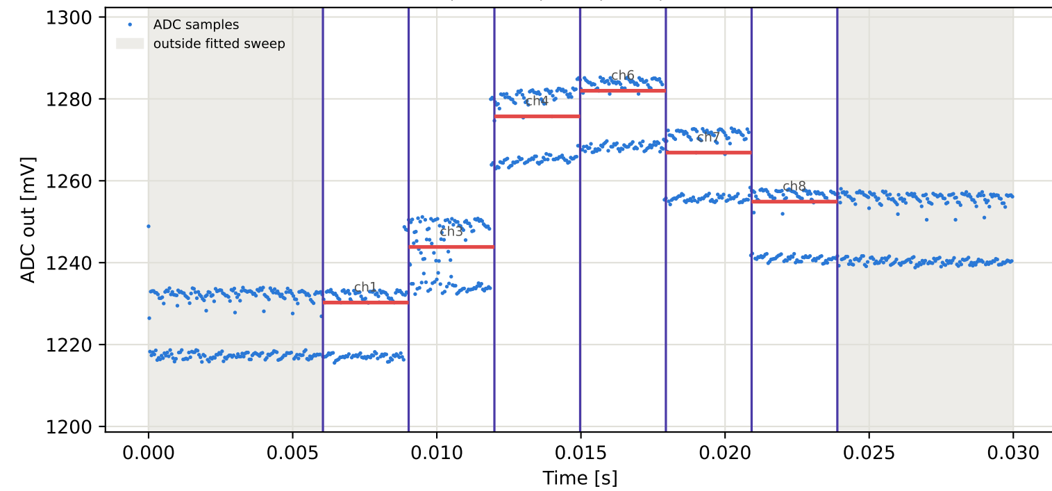
Tag8 &lt;- Tag7 | 875 MHz | run 0 | rep 1 | phase -127.51 deg
