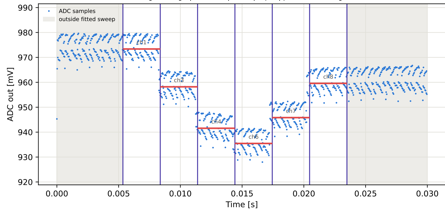
Tag4 &lt;- Tag3 | 875 MHz | run 0 | rep 1 | phase 56.22 deg
