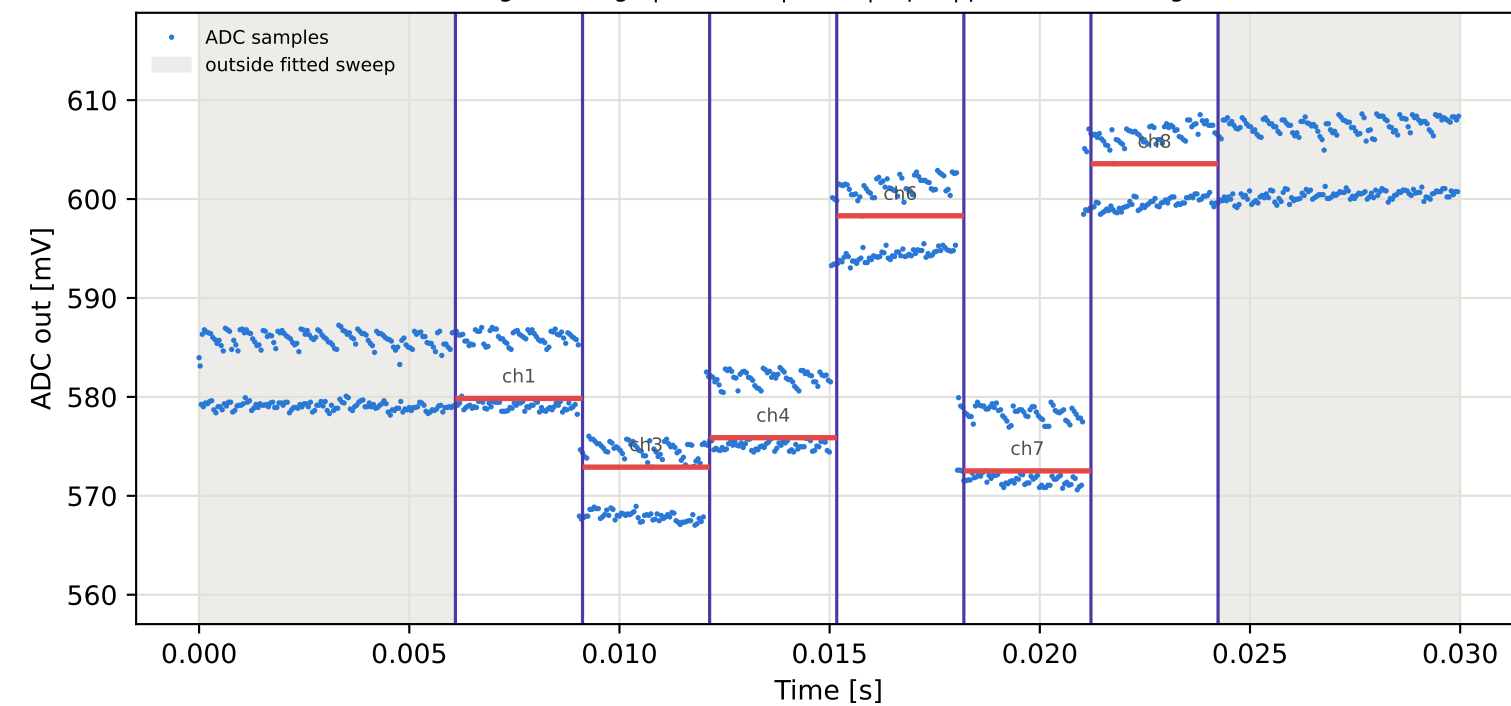
Tag16 &lt;- Tag6 | 865 MHz | run 0 | rep 1 | phase 166.66 deg
