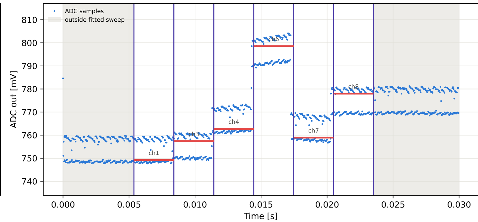
Tag15 &lt;- Tag6 | 895 MHz | run 0 | rep 1 | phase -164.22 deg
