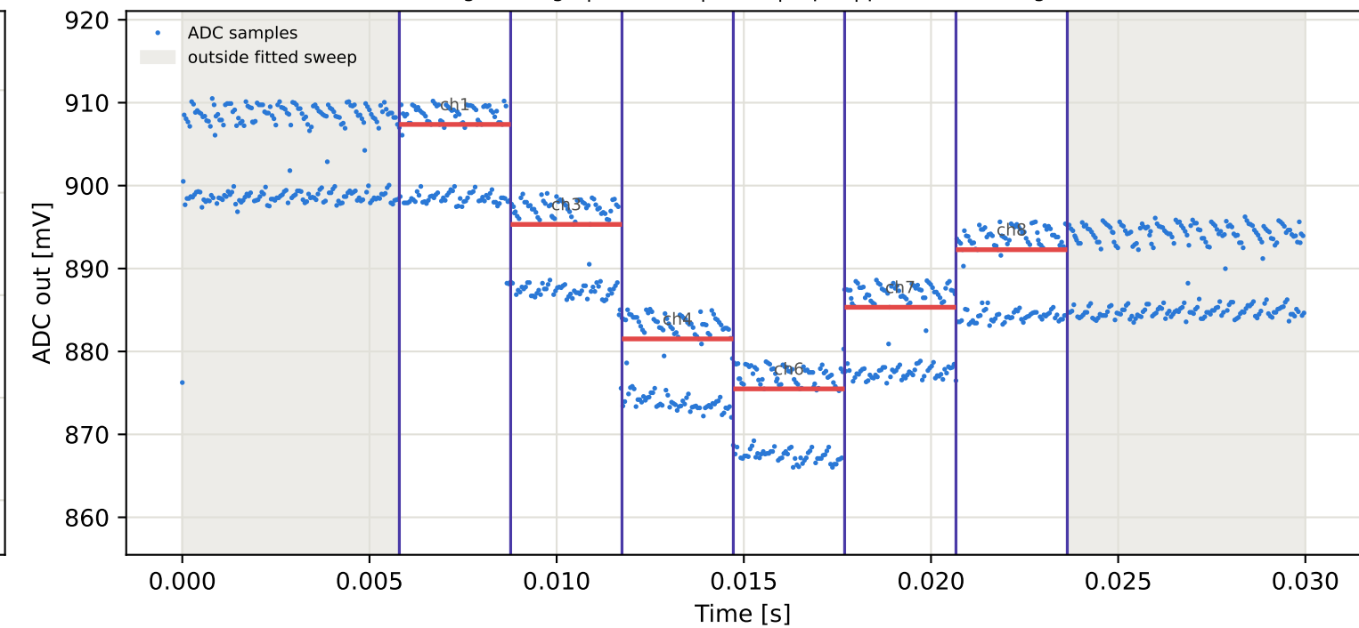
Tag7 &lt;- Tag6 | 875 MHz | run 0 | rep 1 | phase 108.80 deg
