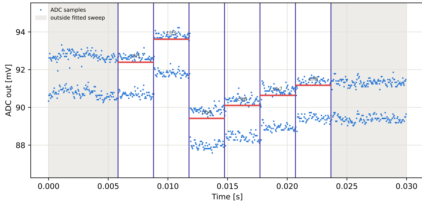
Tag9 &lt;- Tag5 | 795 MHz | run 0 | rep 1 | phase 25.52 deg
