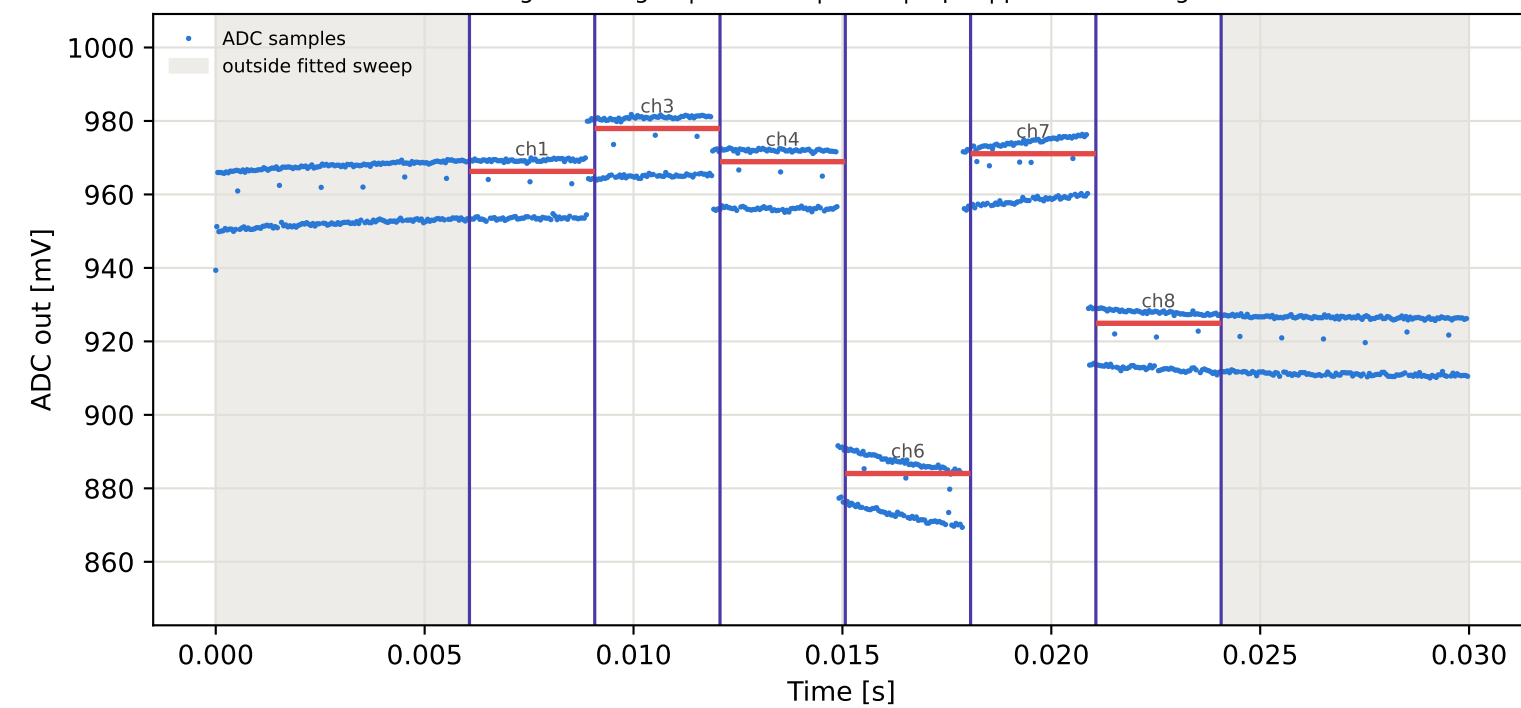
Tag15 &lt;- Tag3 | 915 MHz | run 0 | rep 1 | phase -138.27 deg
