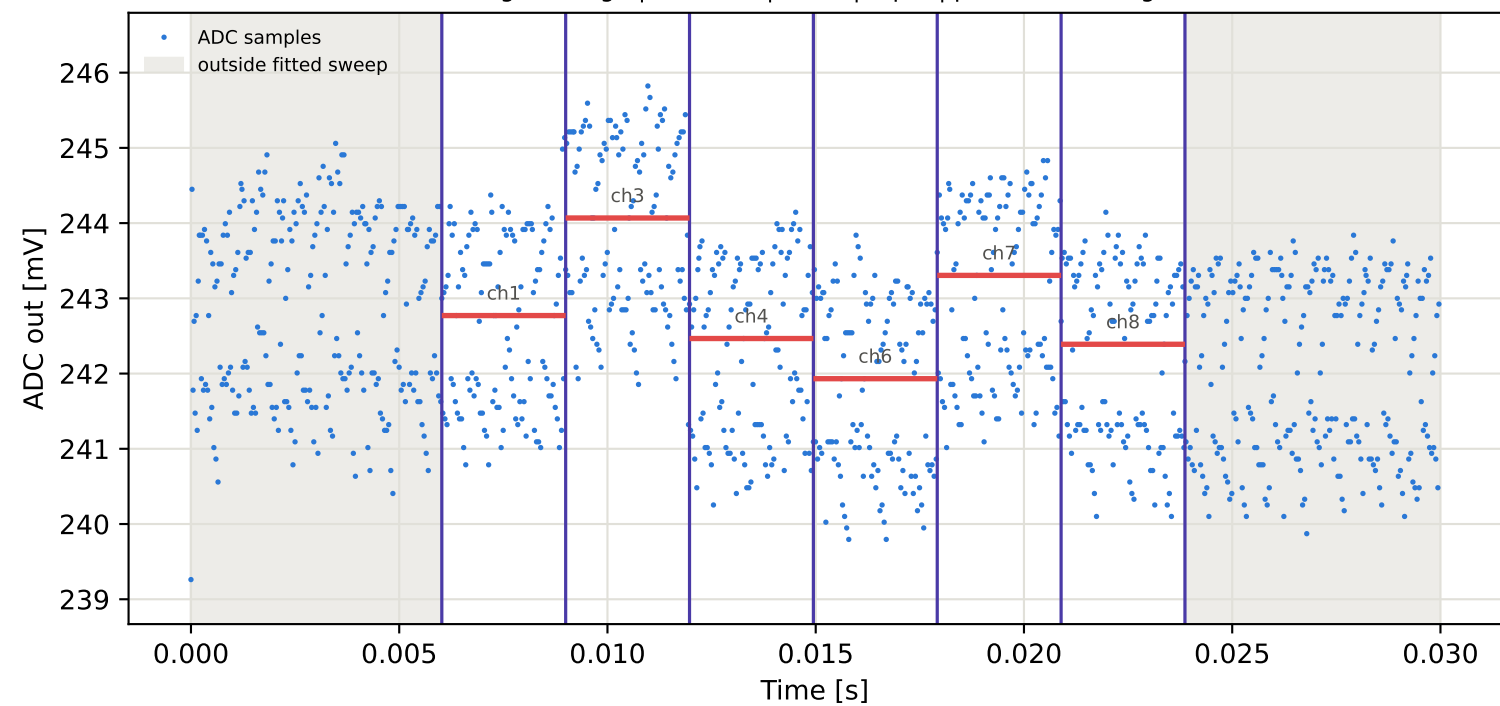
Tag5 &lt;- Tag3 | 795 MHz | run 0 | rep 1 | phase 26.48 deg
