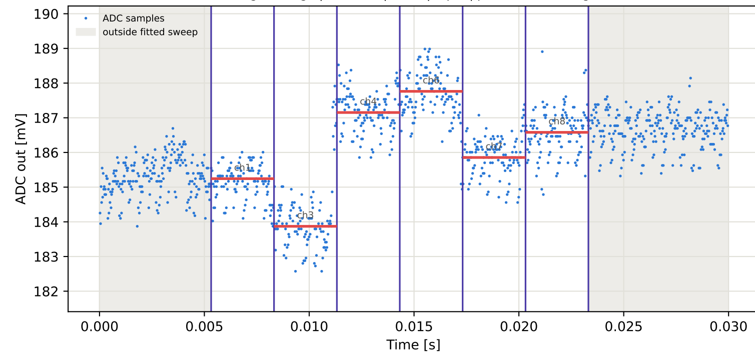
Tag5 &lt;- Tag8 | 775 MHz | run 0 | rep 1 | phase 14.05 deg
