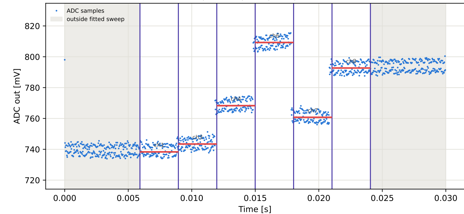
Tag16 &lt;- Tag15 | 885 MHz | run 0 | rep 1 | phase -155.17 deg
