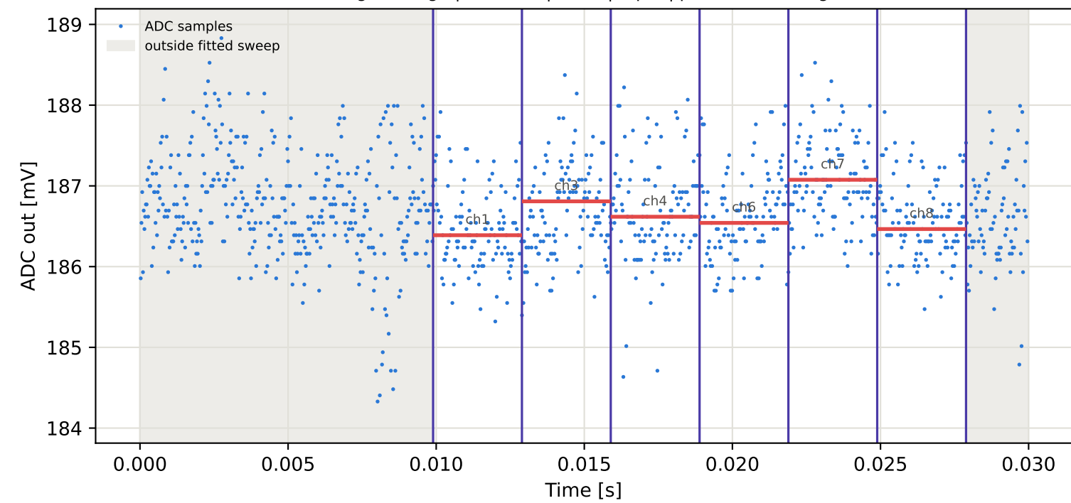
Tag5 &lt;- Tag4 | 775 MHz | run 0 | rep 1 | phase -81.32 deg
