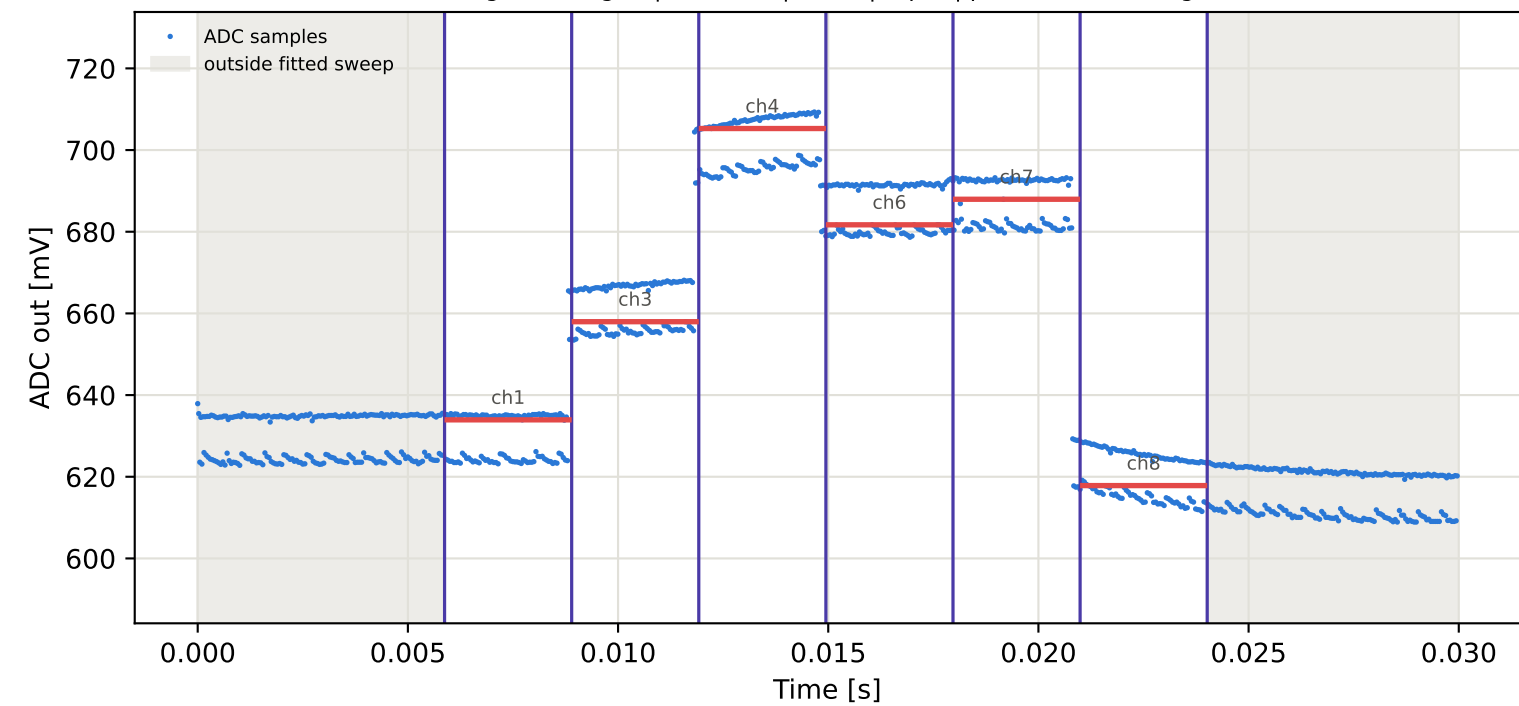
Tag10 &lt;- Tag3 | 915 MHz | run 0 | rep 1 | phase 92.30 deg
