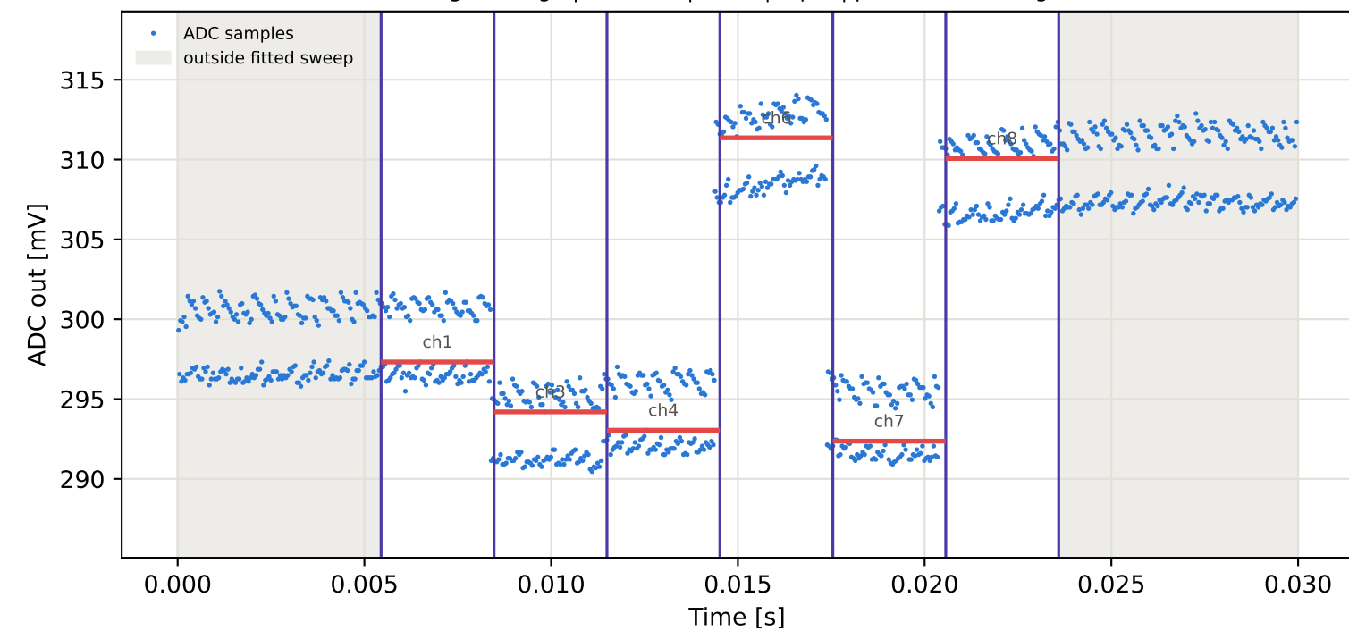
Tag4 &lt;- Tag9 | 915 MHz | run 0 | rep 1 | phase 161.71 deg
