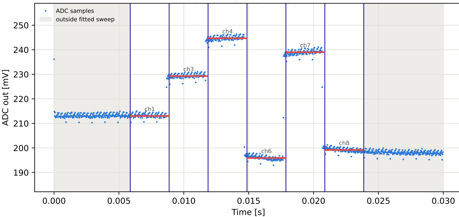
Tag3 &lt;- Tag16 | 955 MHz | run 0 | rep 1 | phase -50.22 deg
