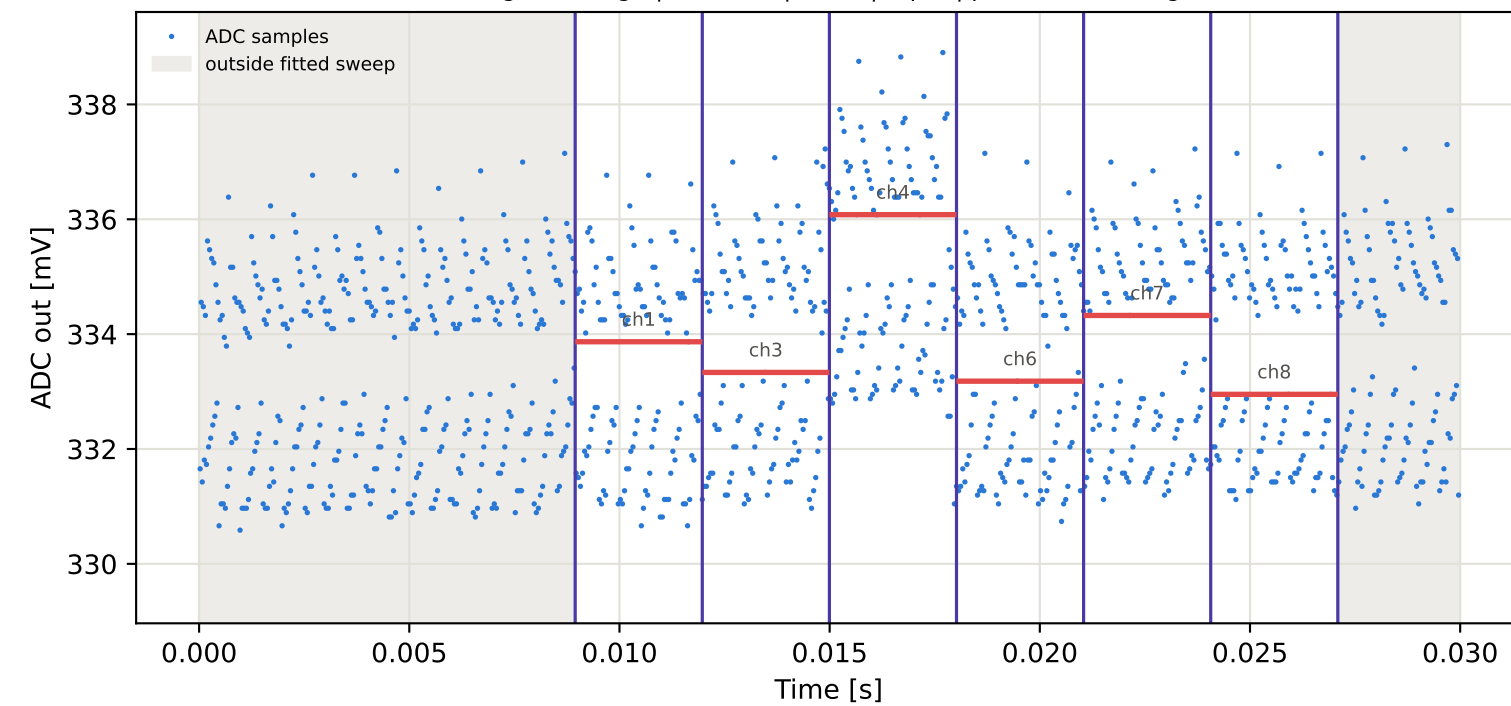
Tag16 &lt;- Tag4 | 985 MHz | run 0 | rep 1 | phase 100.82 deg
