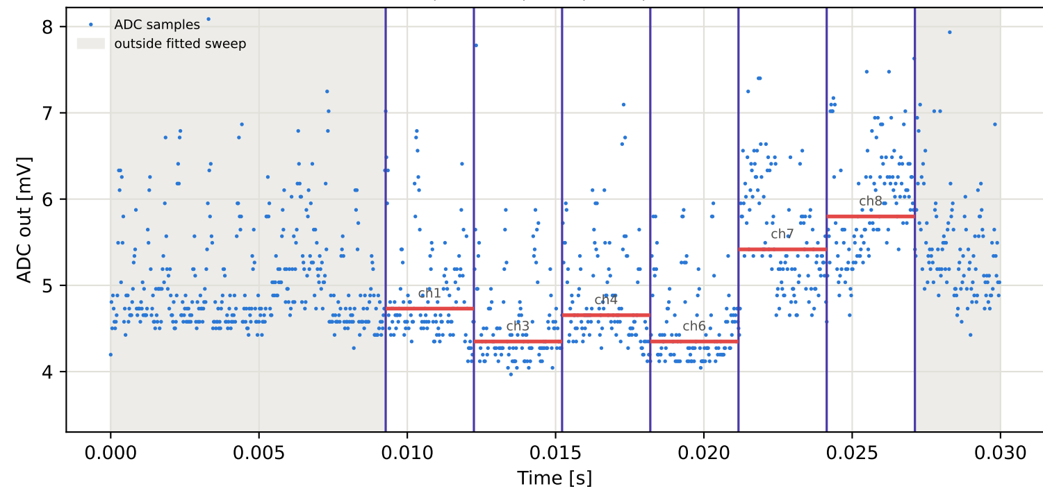
Tag2 &lt;- Tag8 | 785 MHz | run 0 | rep 1 | phase 56.14 deg
