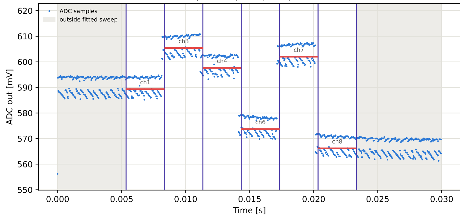
Tag2 &lt;- Tag10 | 865 MHz | run 0 | rep 1 | phase 84.23 deg
