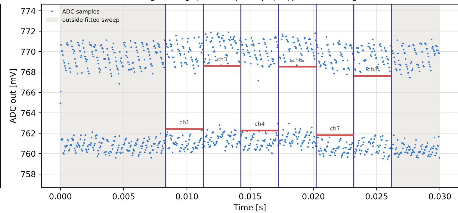
Tag15 &lt;- Tag4 | 895 MHz | run 0 | rep 1 | phase -126.47 deg
