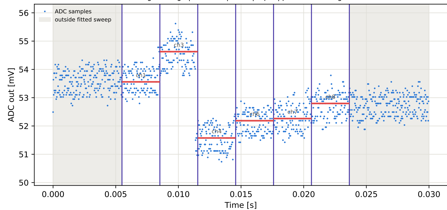
Tag9 &lt;- Tag6 | 775 MHz | run 0 | rep 1 | phase -52.62 deg
