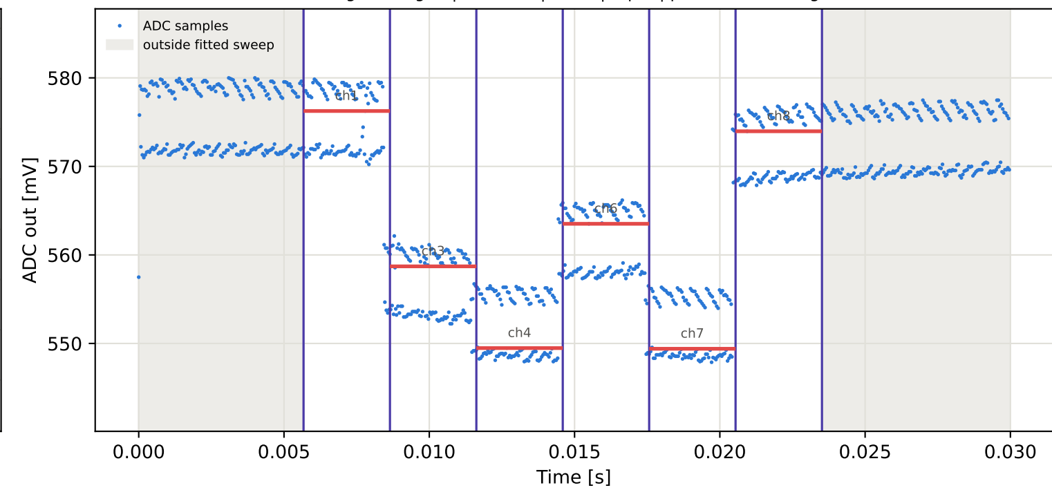
Tag7 &lt;- Tag15 | 865 MHz | run 0 | rep 1 | phase 100.86 deg
