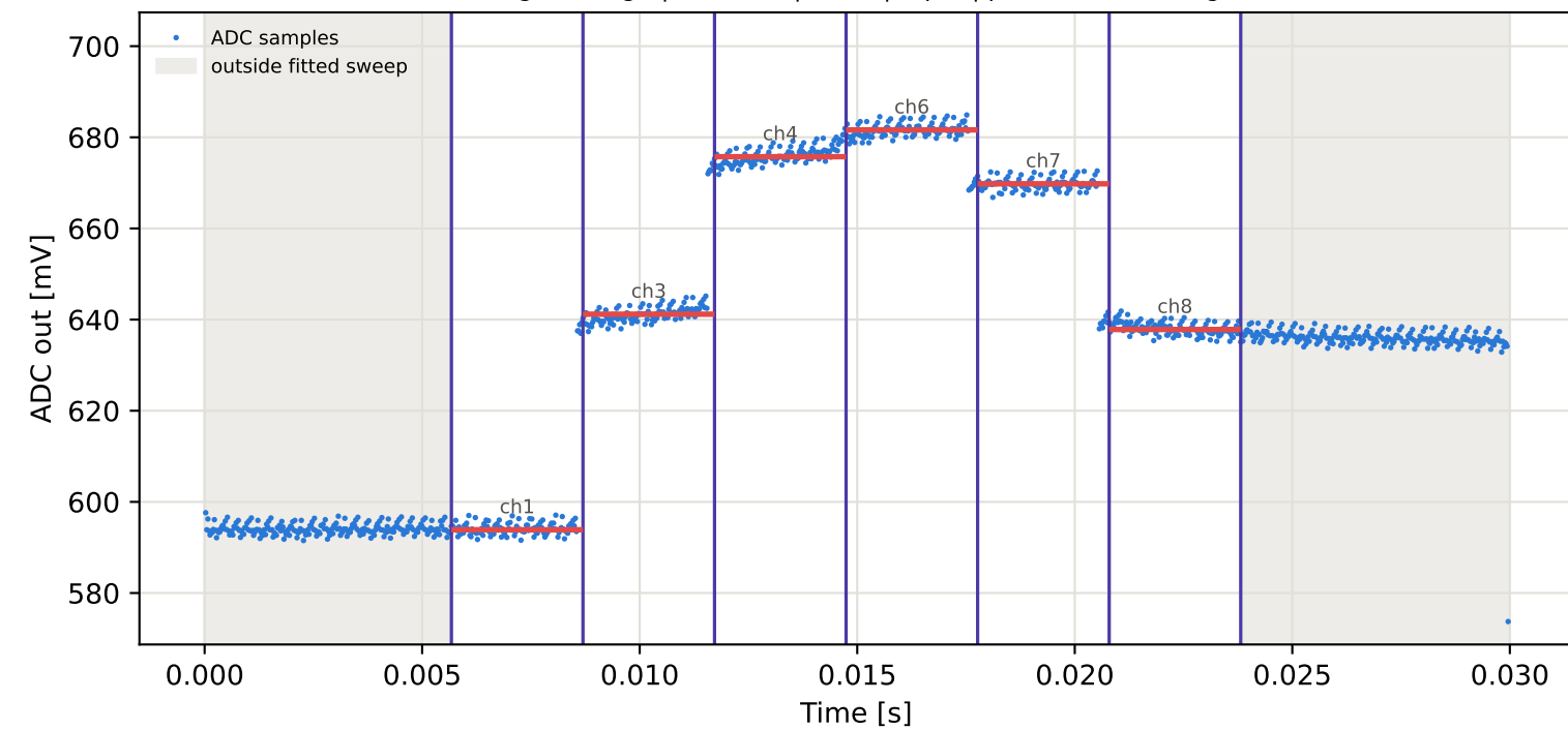
Tag3 &lt;- Tag7 | 875 MHz | run 0 | rep 1 | phase -146.50 deg
