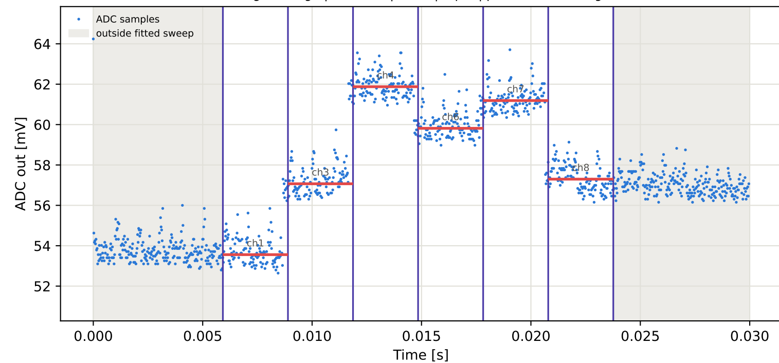
Tag2 &lt;- Tag8 | 835 MHz | run 0 | rep 1 | phase -105.21 deg
