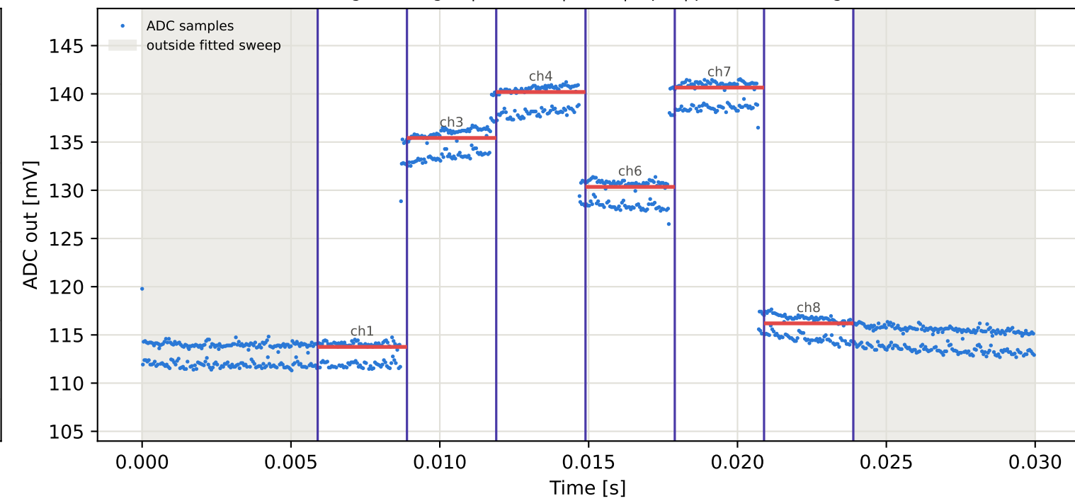
Tag10 &lt;- Tag3 | 865 MHz | run 0 | rep 1 | phase 46.73 deg
