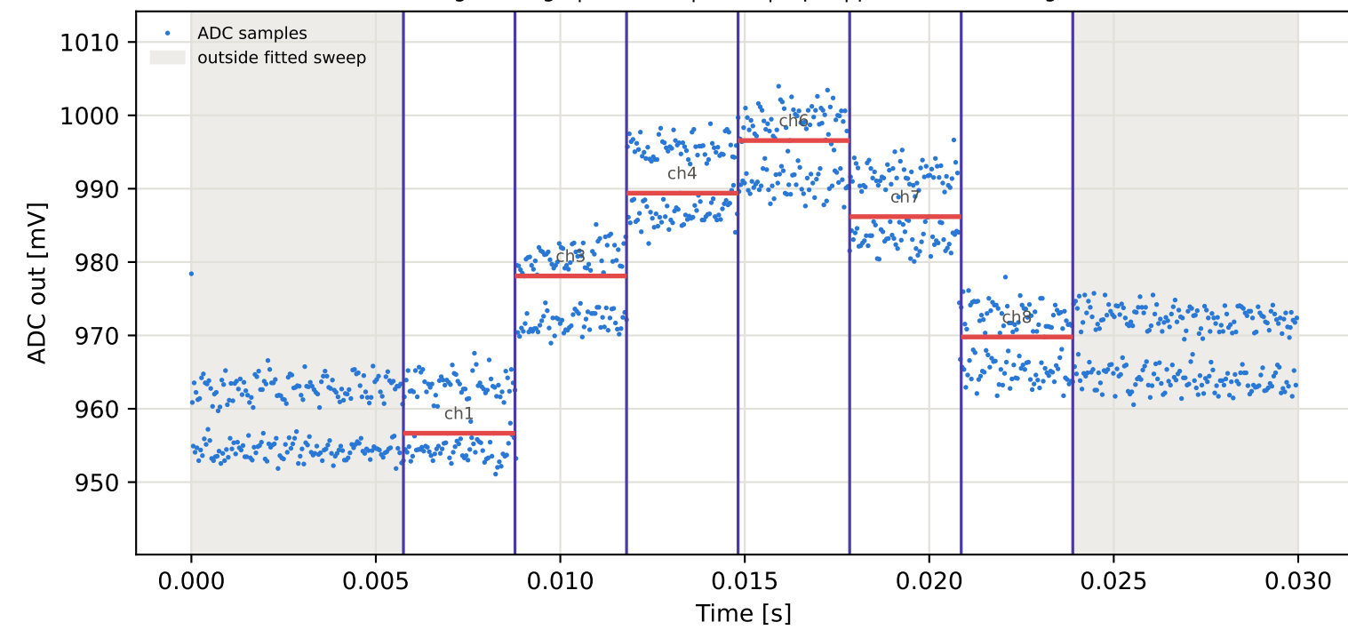
Tag7 &lt;- Tag5 | 885 MHz | run 0 | rep 1 | phase -121.81 deg
