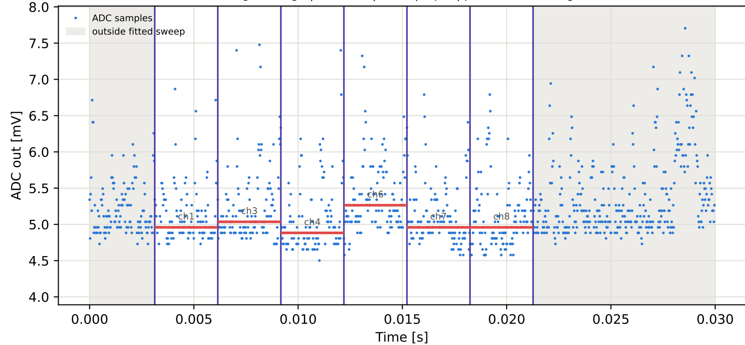
Tag2 &lt;- Tag7 | 775 MHz | run 0 | rep 1 | phase -174.34 deg
