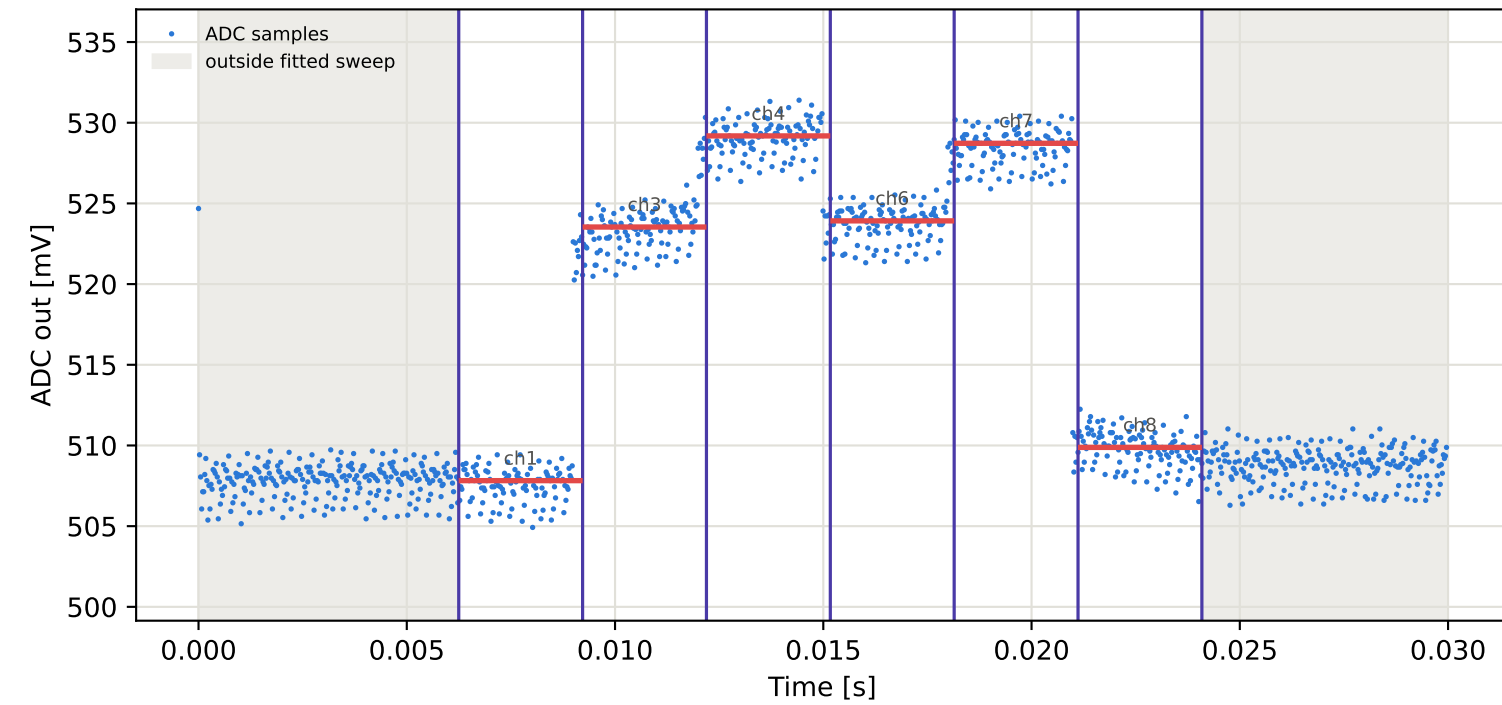
Tag1 &lt;- Tag3 | 875 MHz | run 0 | rep 1 | phase -179.15 deg
