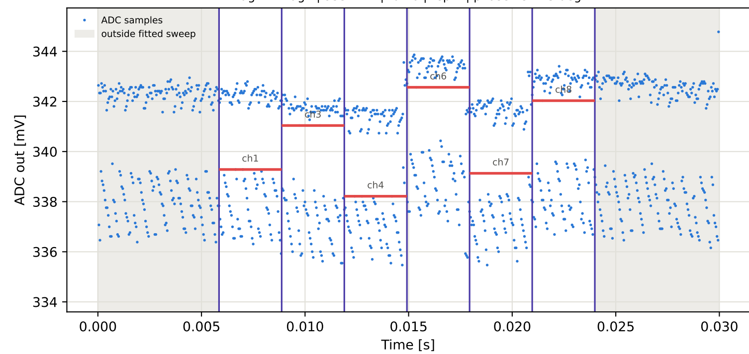
Tag7 &lt;- Tag4 | 955 MHz | run 0 | rep 1 | phase 120.42 deg
