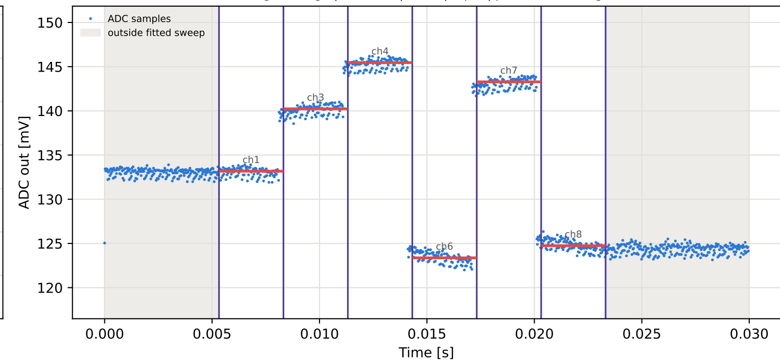
Tag3 &lt;- Tag7 | 935 MHz | run 0 | rep 1 | phase -30.54 deg
