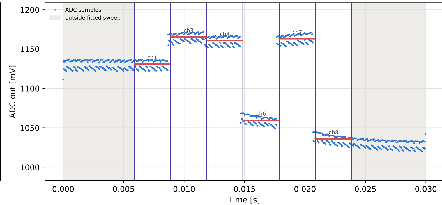
Tag8 &lt;- Tag7 | 895 MHz | run 0 | rep 1 | phase 4.95 deg
