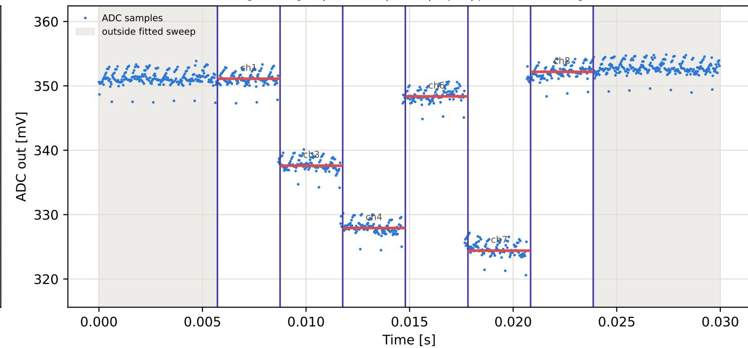
Tag5 &lt;- Tag2 | 805 MHz | run 0 | rep 1 | phase 152.15 deg
