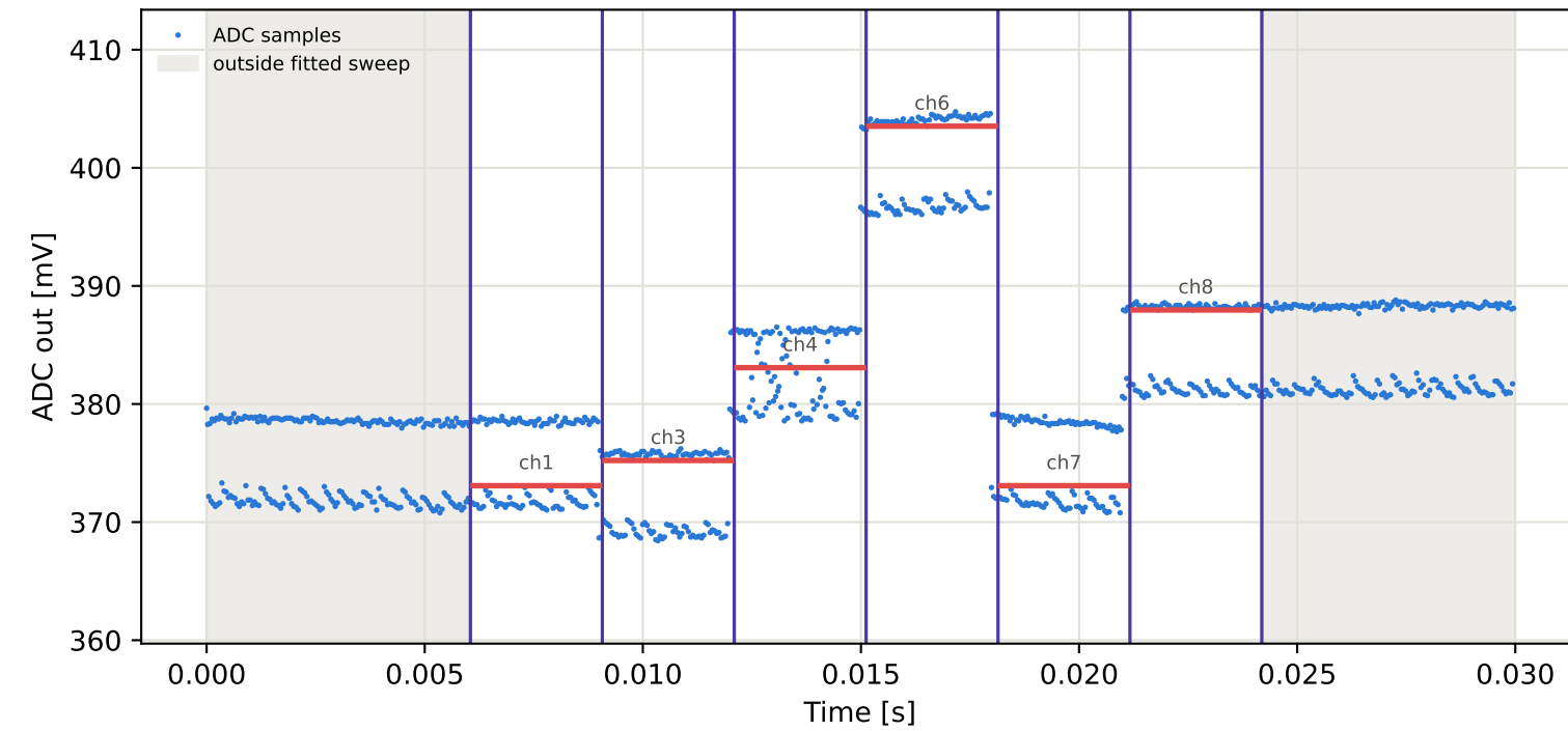
Tag7 &lt;- Tag5 | 985 MHz | run 0 | rep 1 | phase 53.05 deg
