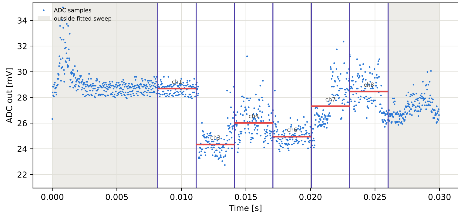
Tag2 &lt;- Tag8 | 805 MHz | run 0 | rep 1 | phase -91.96 deg
