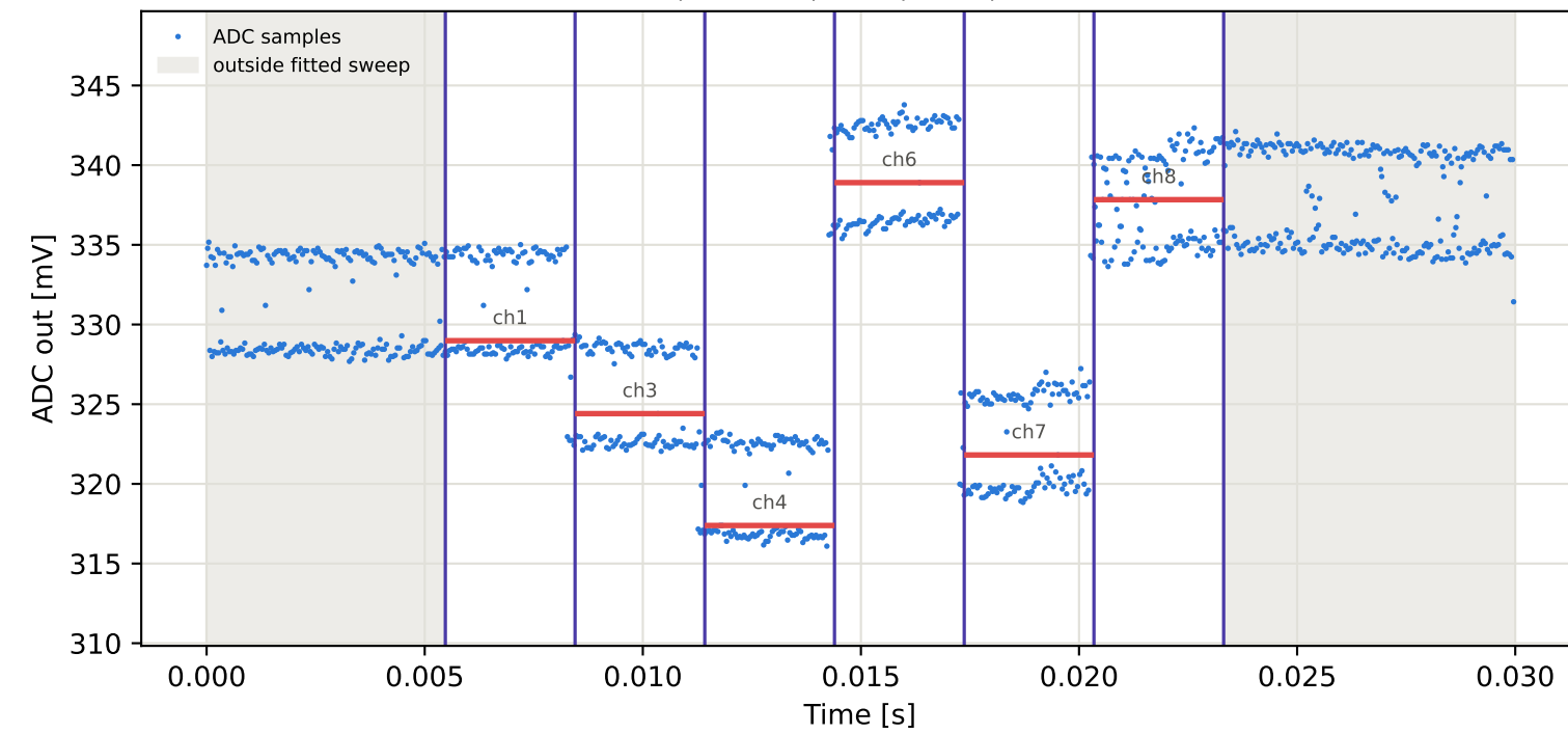
Tag10 &lt;- Tag4 | 965 MHz | run 0 | rep 1 | phase 132.93 deg
