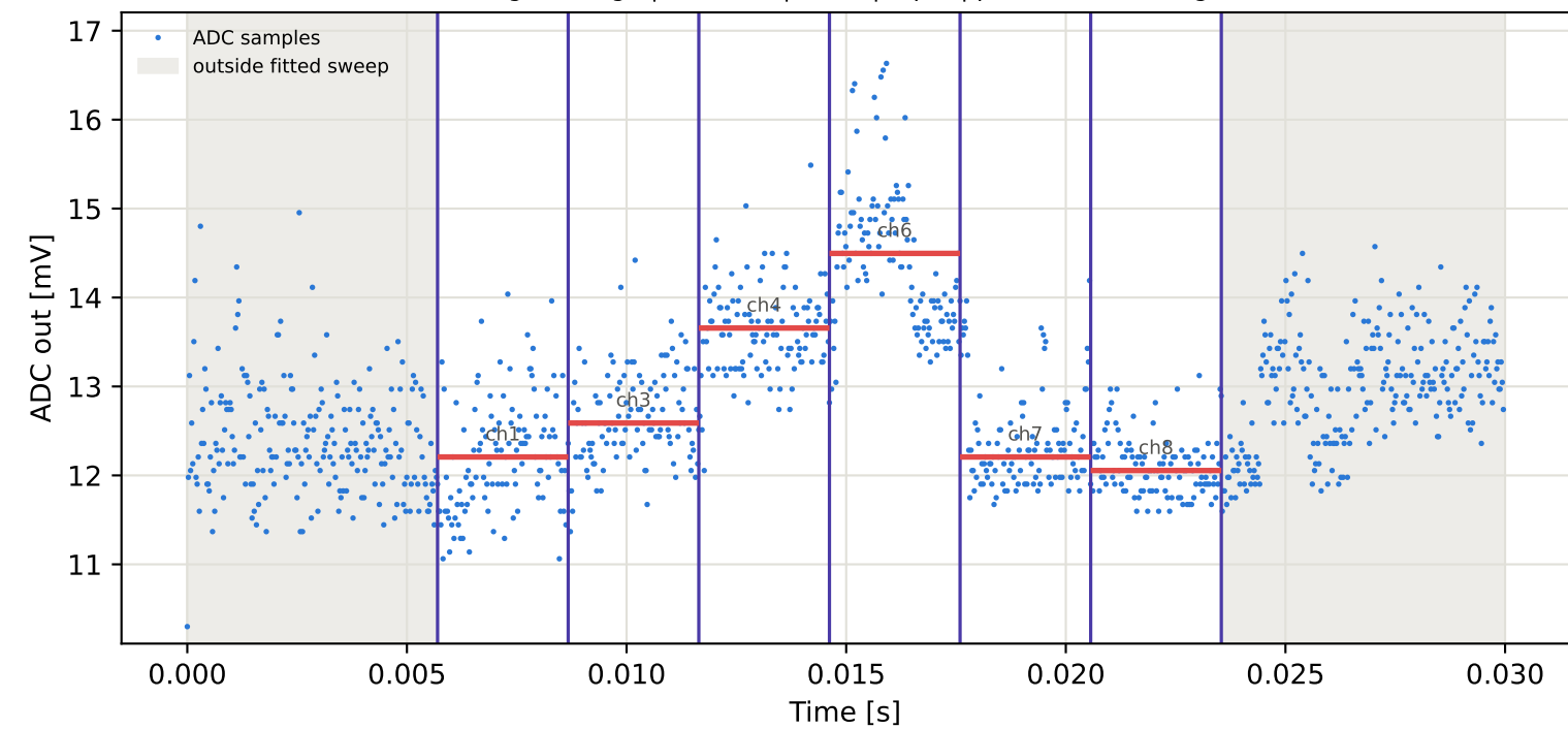
Tag2 &lt;- Tag6 | 895 MHz | run 0 | rep 1 | phase 78.58 deg
