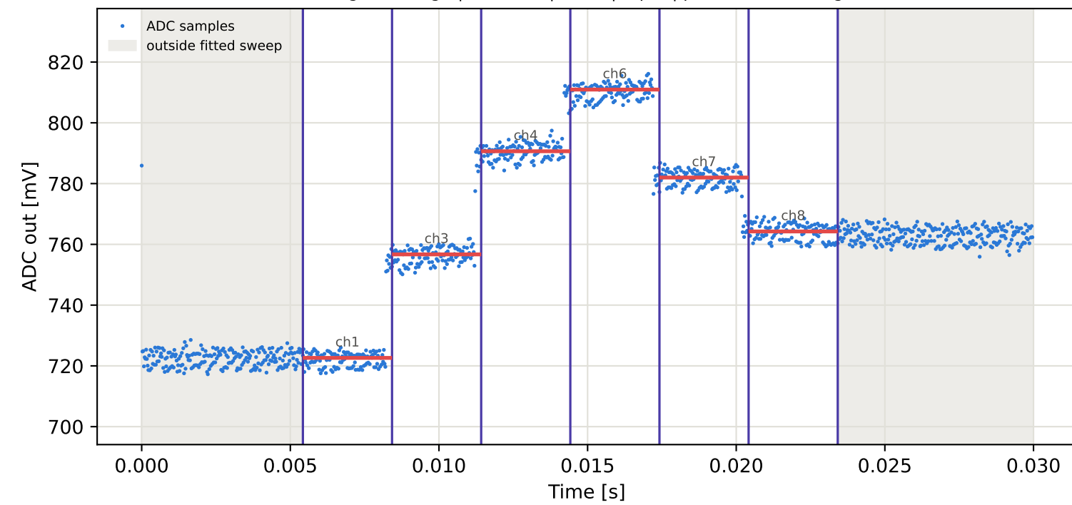
Tag2 &lt;- Tag1 | 885 MHz | run 0 | rep 1 | phase 169.65 deg
