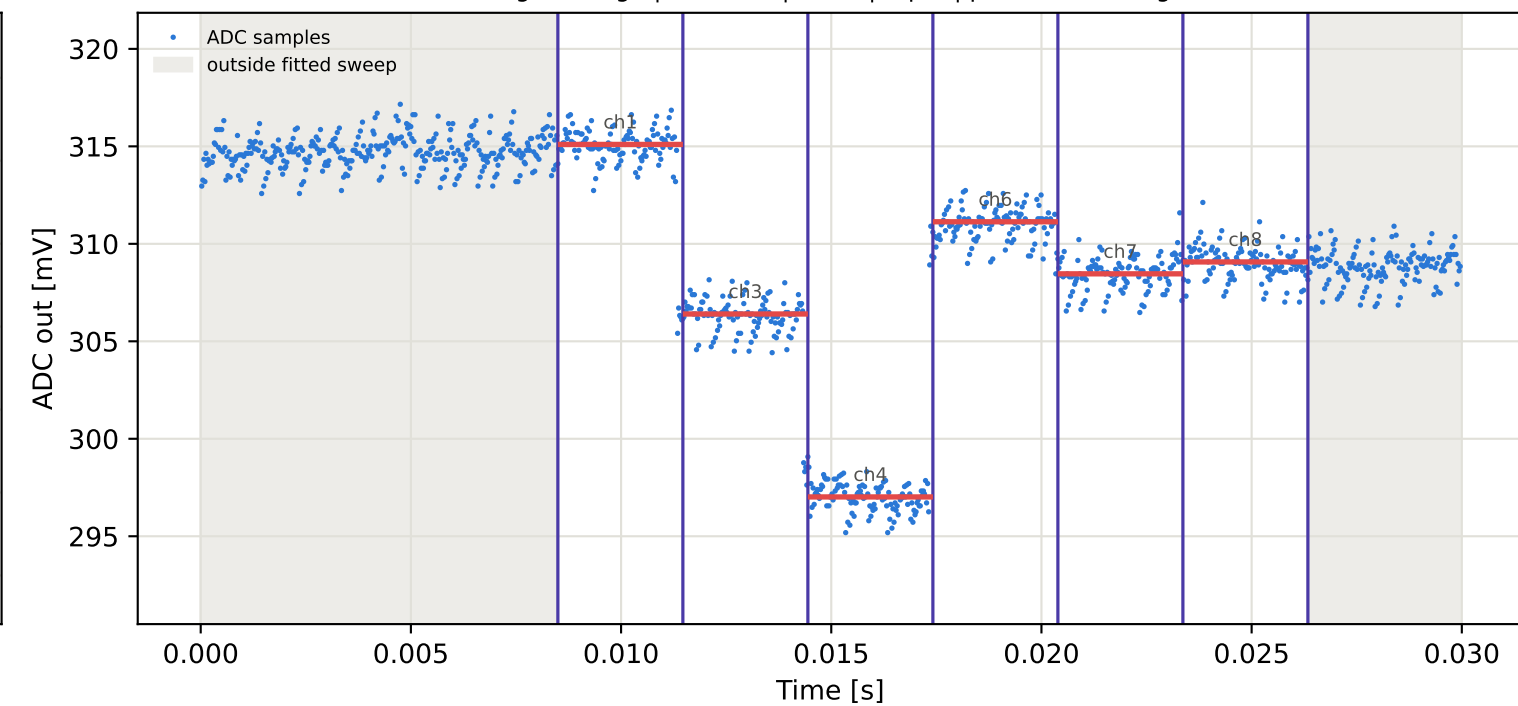
Tag6 &lt;- Tag5 | 955 MHz | run 0 | rep 1 | phase 79.21 deg
