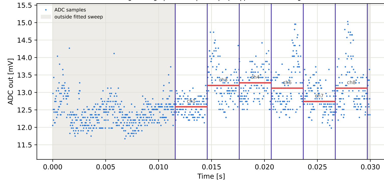
Tag3 &lt;- Tag10 | 895 MHz | run 0 | rep 1 | phase -135.27 deg
