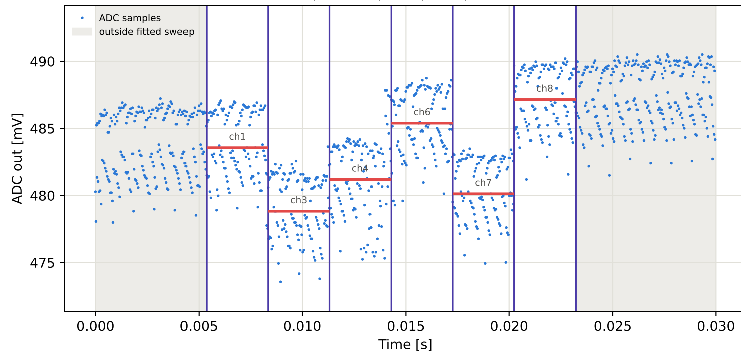
Tag6 &lt;- Tag4 | 845 MHz | run 0 | rep 1 | phase 164.55 deg
