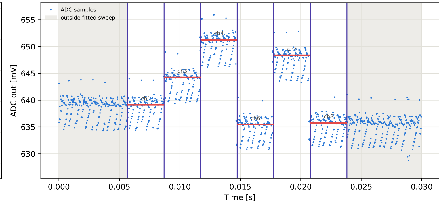
Tag8 &lt;- Tag16 | 985 MHz | run 0 | rep 1 | phase 108.73 deg
