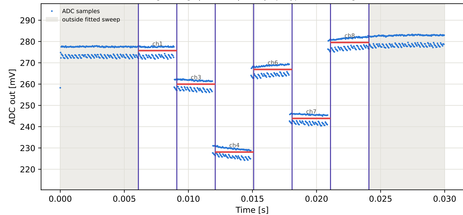
Tag1 &lt;- Tag8 | 955 MHz | run 0 | rep 1 | phase -38.38 deg
