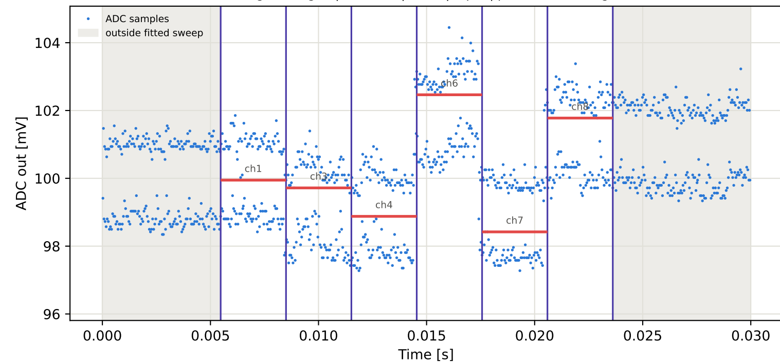
Tag5 &lt;- Tag16 | 975 MHz | run 0 | rep 1 | phase -31.49 deg
