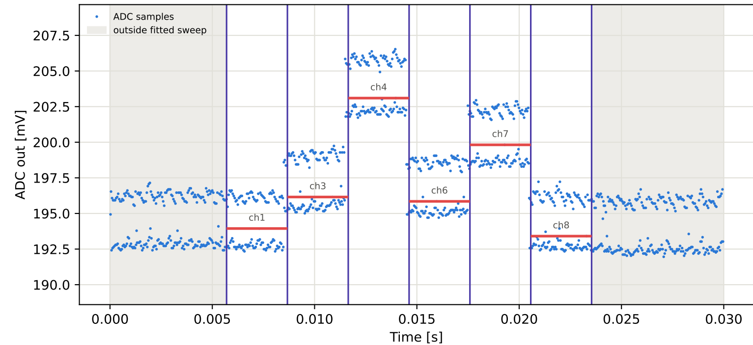
Tag15 &lt;- Tag1 | 975 MHz | run 0 | rep 1 | phase -95.41 deg
