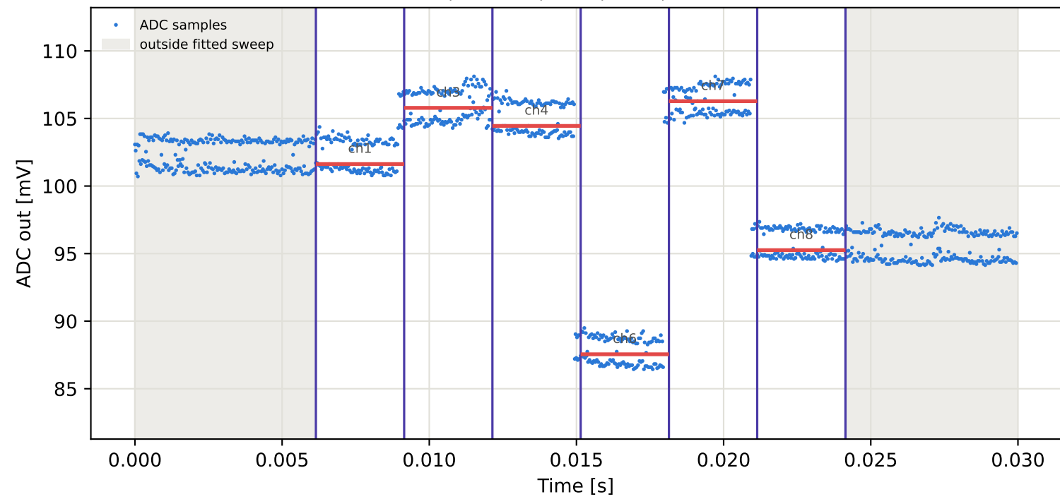
Tag5 &lt;- Tag3 | 985 MHz | run 0 | rep 1 | phase -12.19 deg
