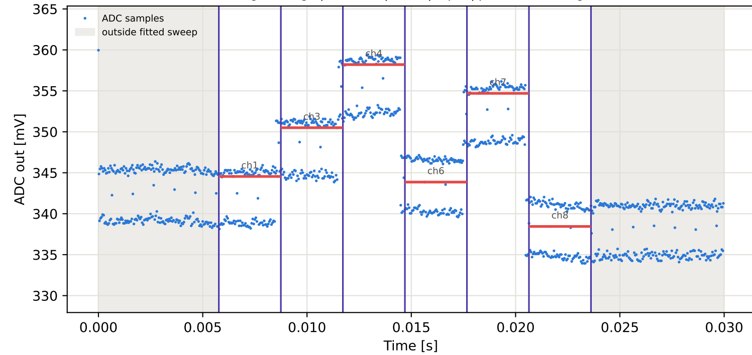
Tag7 &lt;- Tag1 | 935 MHz | run 0 | rep 1 | phase -18.03 deg
