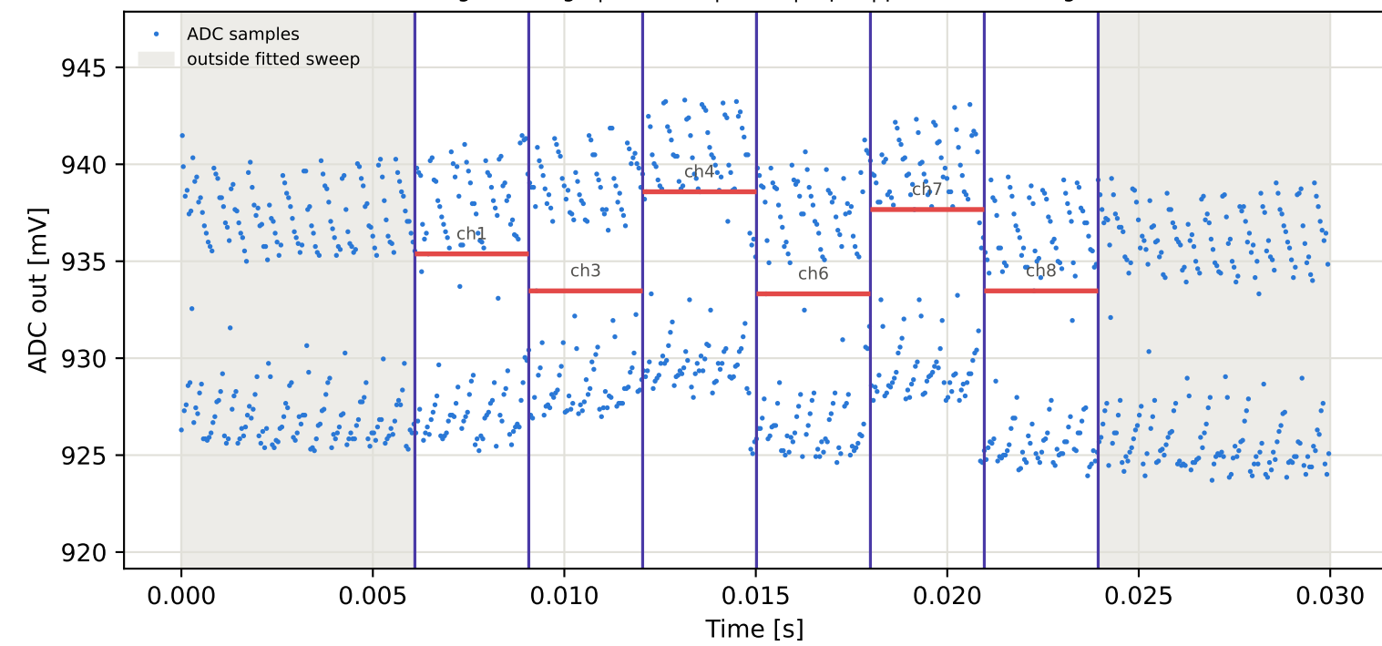
Tag15 &lt;- Tag1 | 945 MHz | run 0 | rep 1 | phase -79.61 deg
