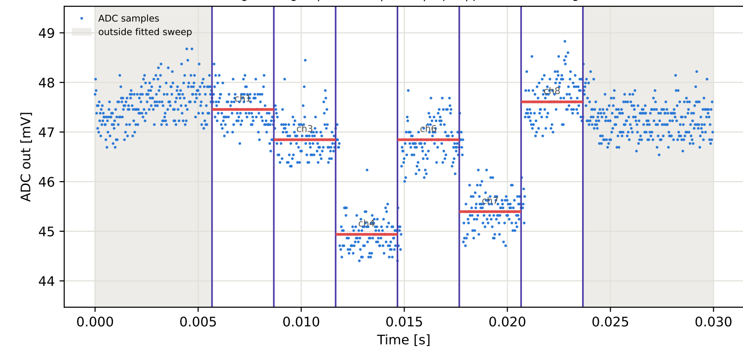
Tag8 &lt;- Tag16 | 775 MHz | run 0 | rep 1 | phase 106.22 deg
