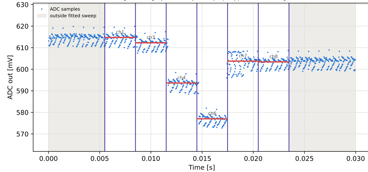
Tag16 &lt;- Tag6 | 935 MHz | run 0 | rep 1 | phase 32.62 deg
