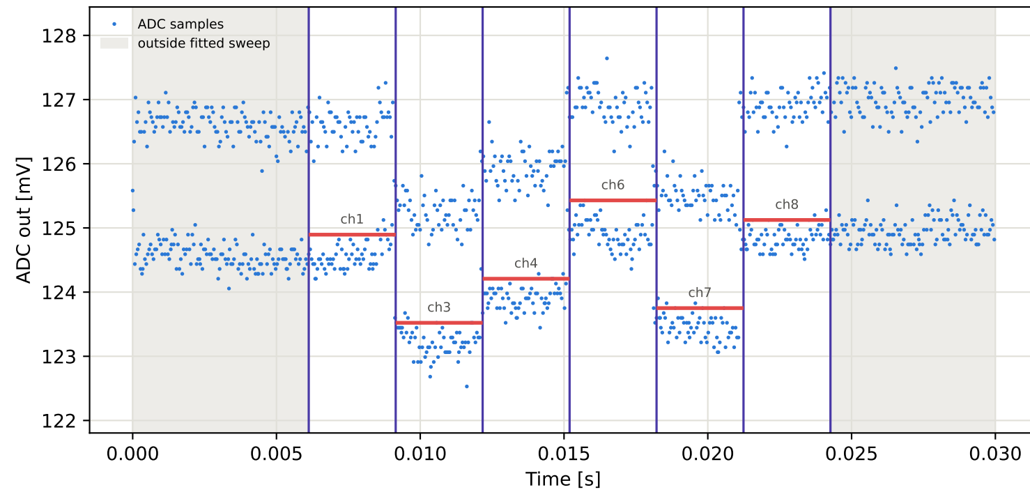
Tag1 &lt;- Tag16 | 825 MHz | run 0 | rep 1 | phase -179.54 deg
