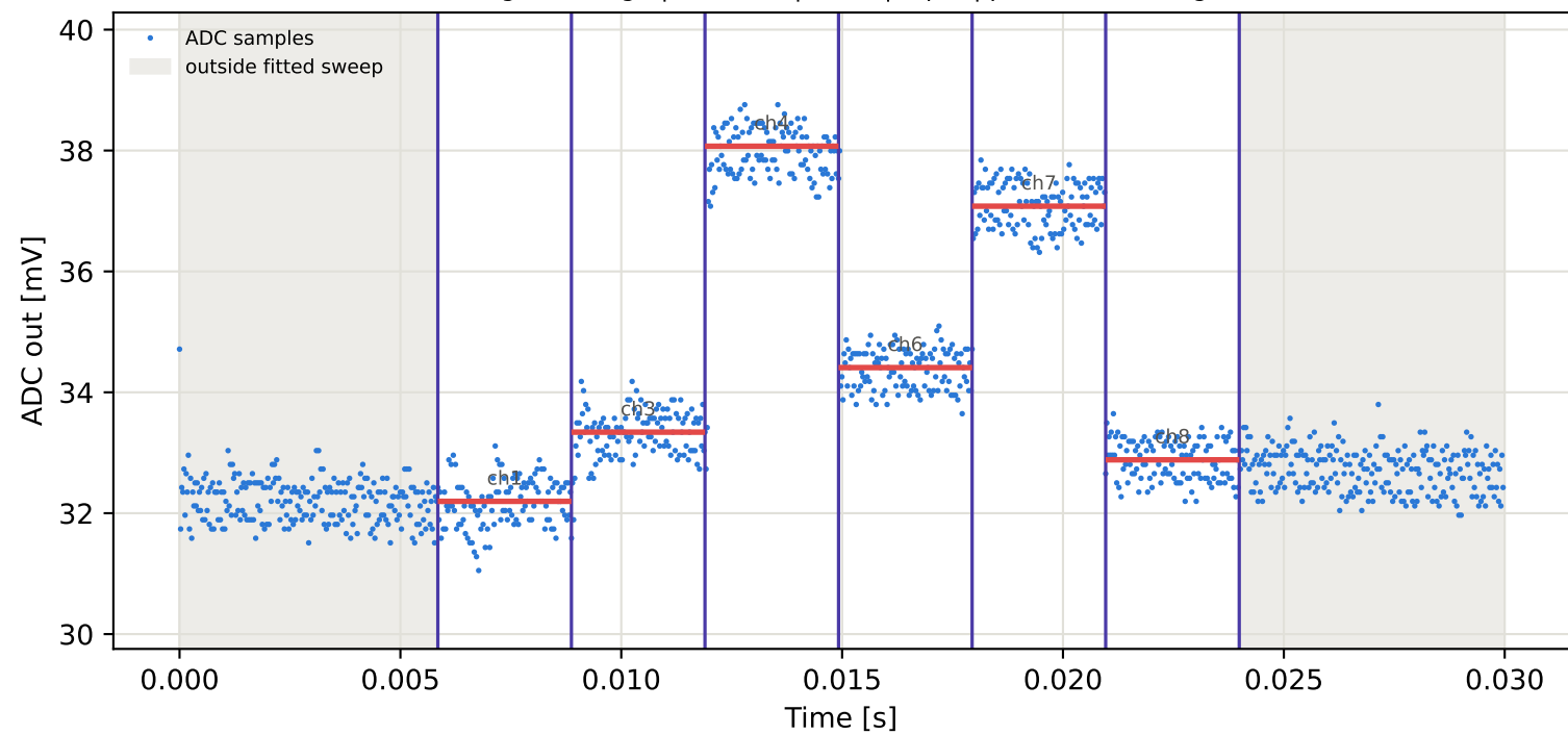
Tag2 &lt;- Tag10 | 775 MHz | run 0 | rep 1 | phase -147.92 deg
