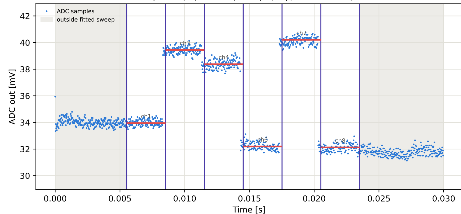
Tag9 &lt;- Tag8 | 805 MHz | run 0 | rep 1 | phase 71.49 deg
