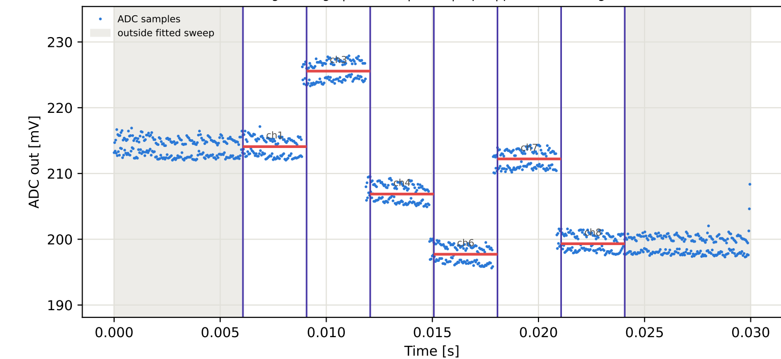
Tag5 &lt;- Tag3 | 835 MHz | run 0 | rep 1 | phase 25.14 deg
