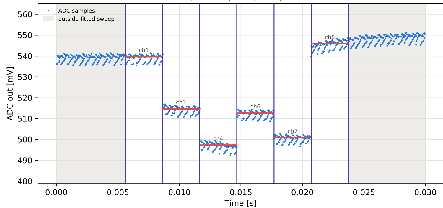
Tag6 &lt;- Tag2 | 895 MHz | run 0 | rep 1 | phase 89.40 deg
