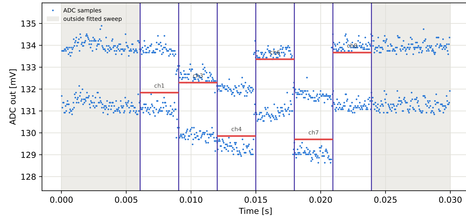
Tag16 &lt;- Tag10 | 795 MHz | run 0 | rep 1 | phase 42.52 deg
