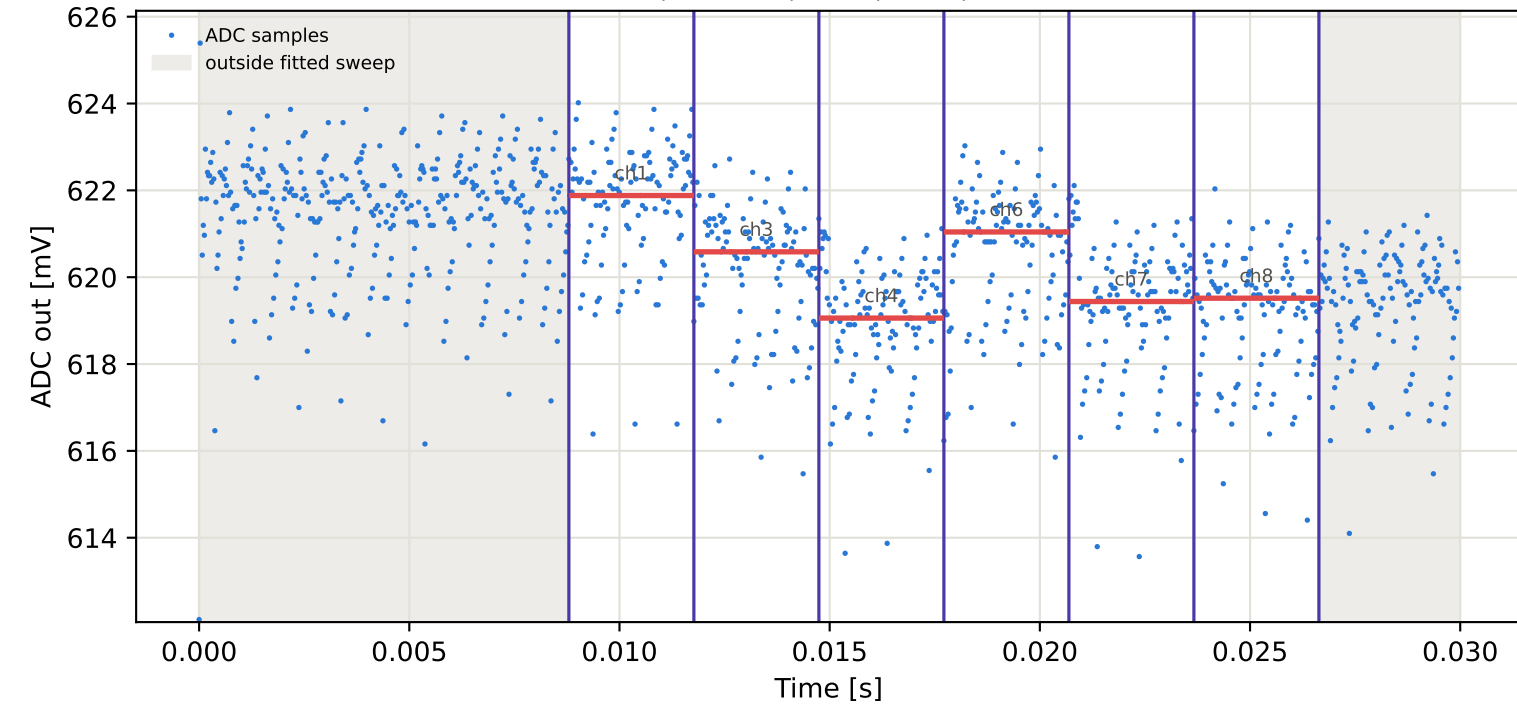
Tag15 &lt;- Tag1 | 865 MHz | run 0 | rep 1 | phase 90.64 deg
