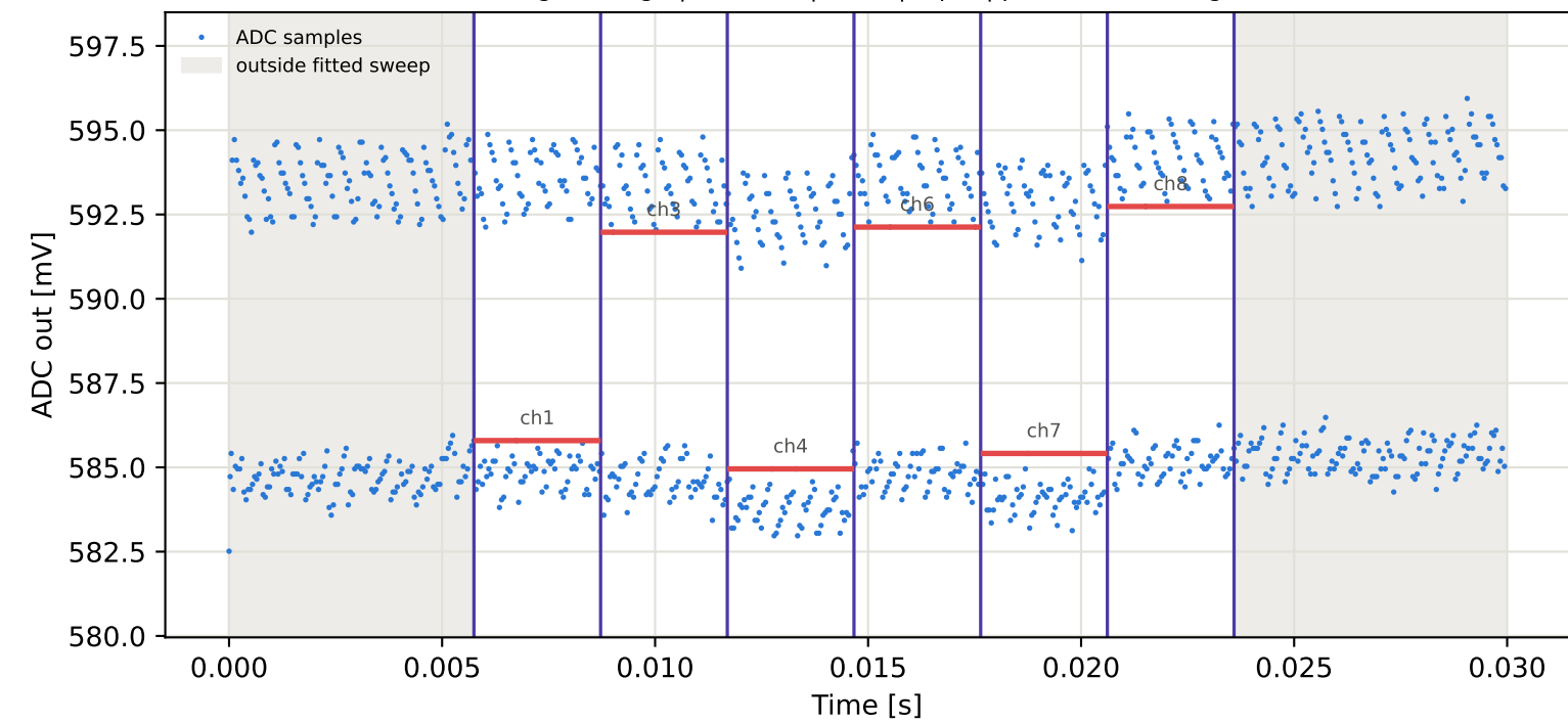
Tag8 &lt;- Tag4 | 965 MHz | run 0 | rep 1 | phase -142.68 deg
