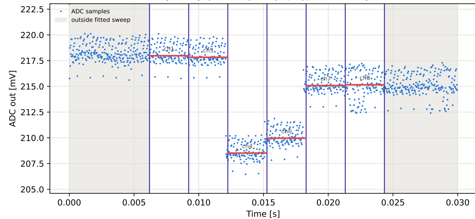
Tag3 &lt;- Tag7 | 995 MHz | run 0 | rep 1 | phase 58.07 deg
