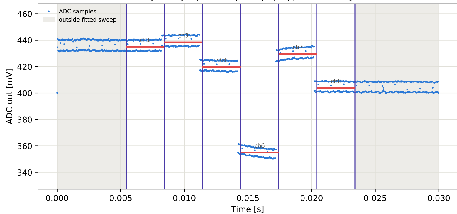
Tag6 &lt;- Tag10 | 925 MHz | run 0 | rep 1 | phase 15.11 deg
