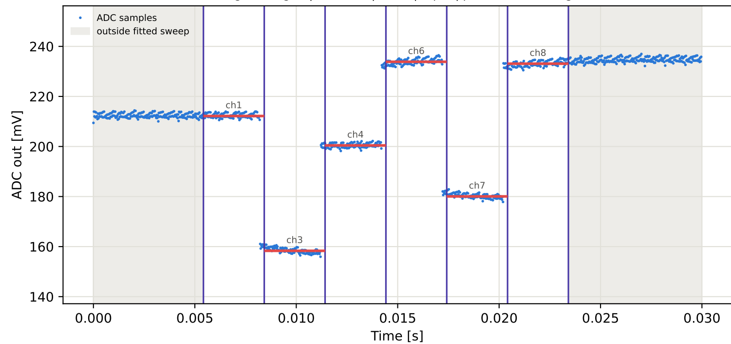
Tag5 &lt;- Tag2 | 835 MHz | run 0 | rep 1 | phase 44.84 deg
