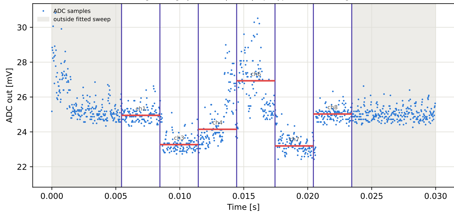
Tag2 &lt;- Tag6 | 805 MHz | run 0 | rep 1 | phase 79.57 deg
