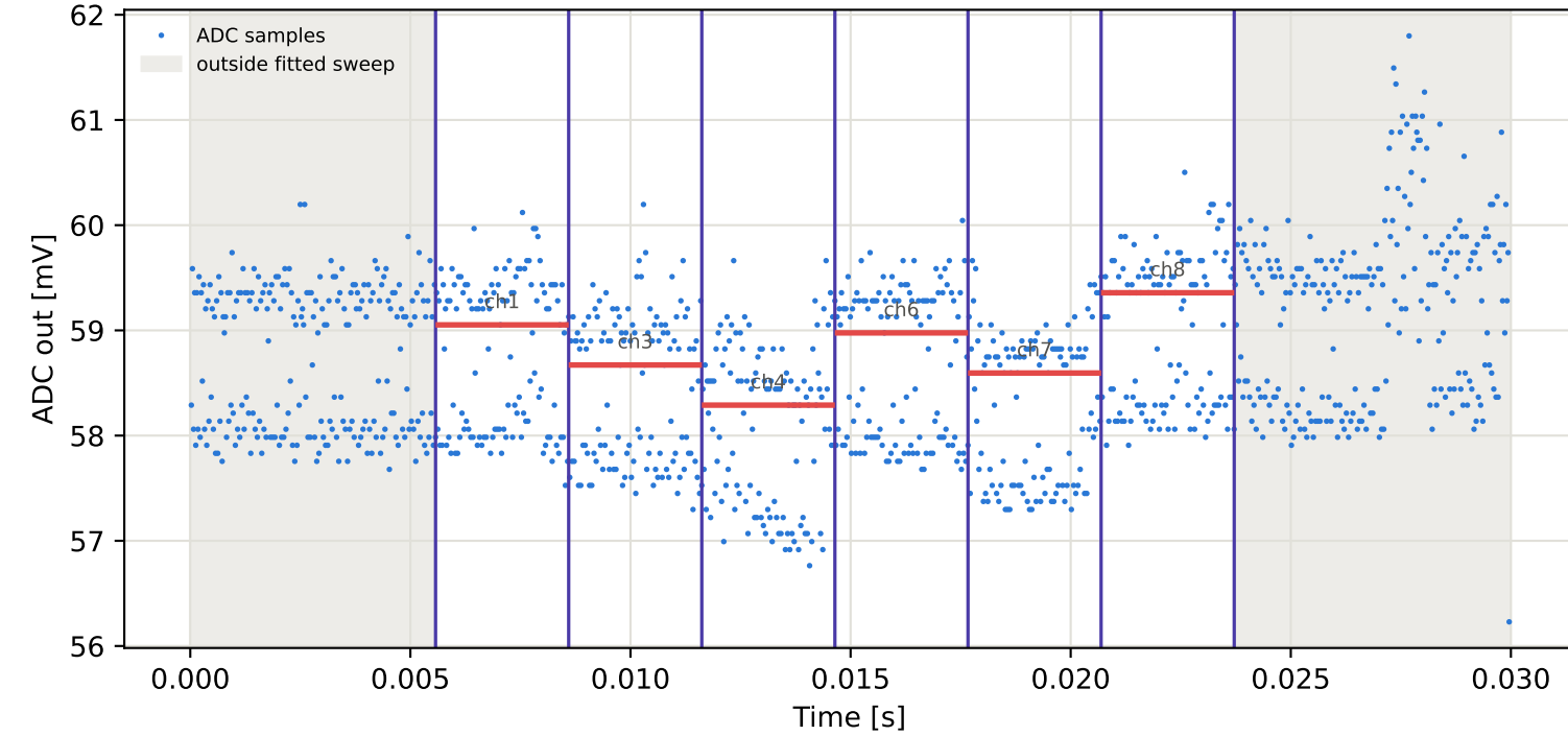
Tag2 &lt;- Tag7 | 985 MHz | run 0 | rep 1 | phase -13.84 deg
