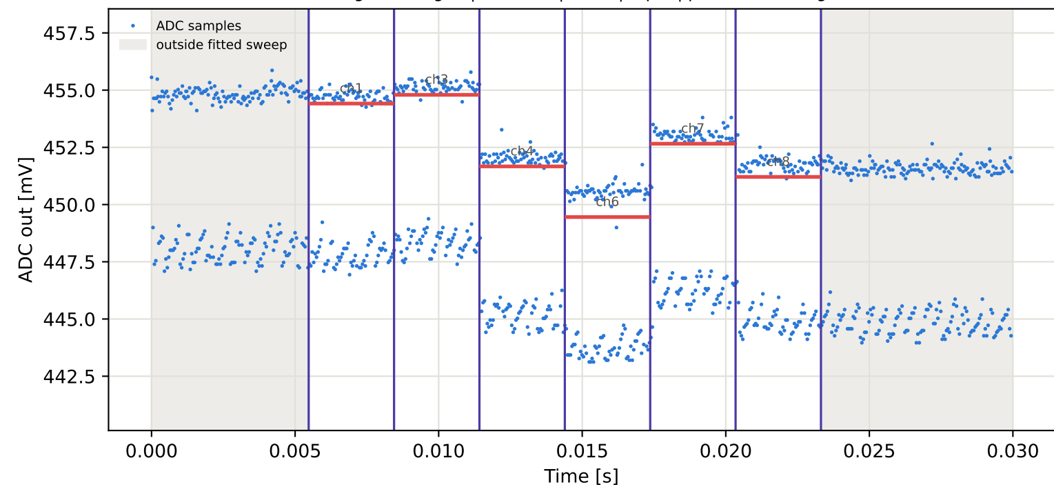
Tag15 &lt;- Tag10 | 845 MHz | run 0 | rep 1 | phase 36.16 deg
