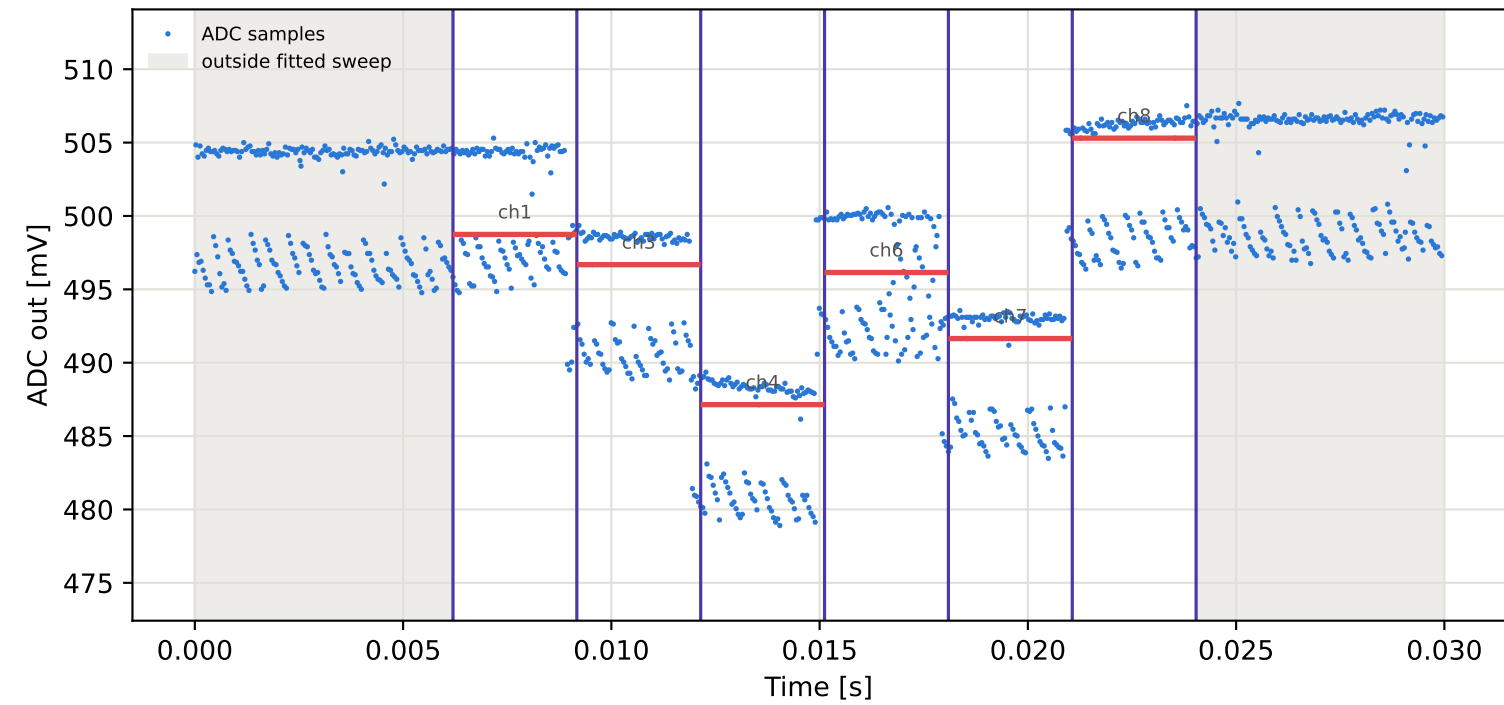
Tag10 &lt;- Tag5 | 955 MHz | run 0 | rep 1 | phase -160.20 deg
