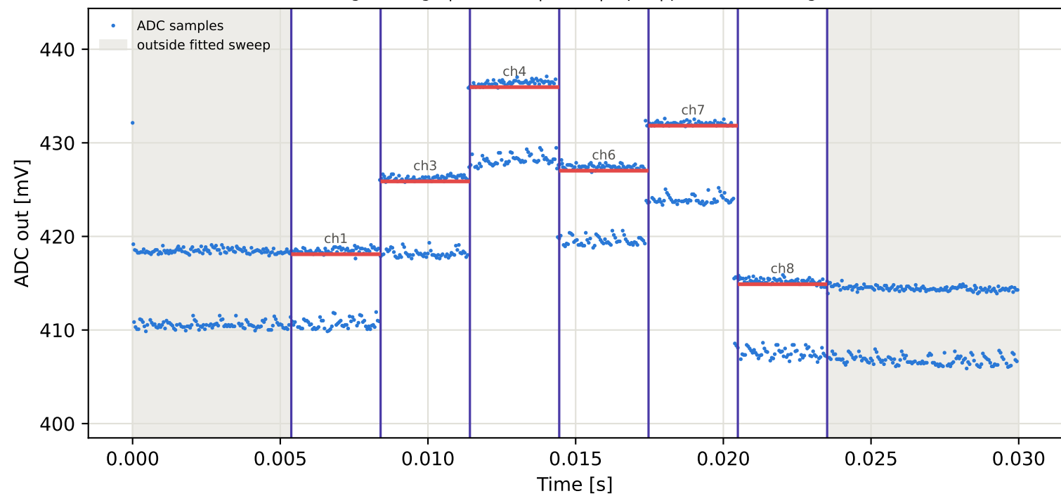
Tag7 &lt;- Tag1 | 925 MHz | run 0 | rep 1 | phase 145.95 deg
