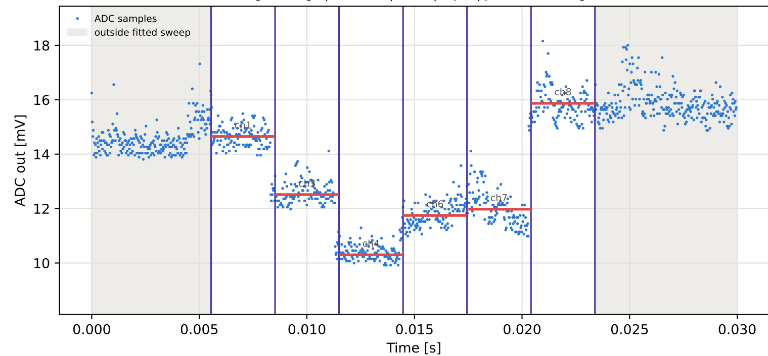
Tag2 &lt;- Tag8 | 895 MHz | run 0 | rep 1 | phase 23.72 deg
