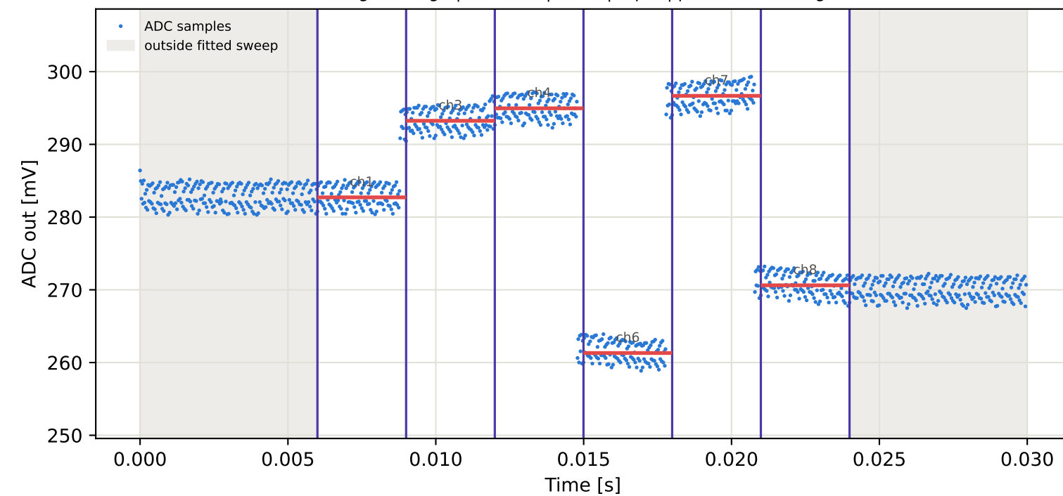
Tag3 &lt;- Tag8 | 985 MHz | run 0 | rep 1 | phase -25.12 deg
