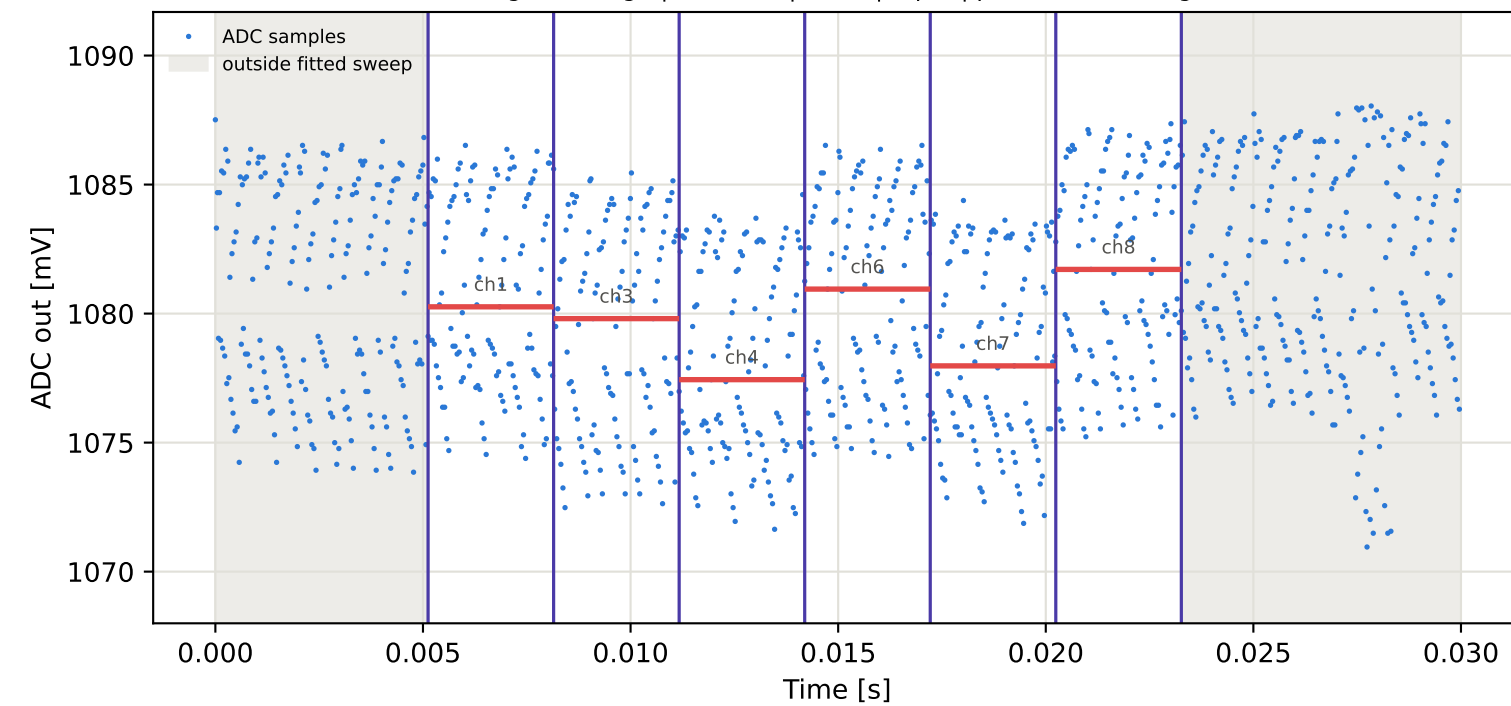
Tag16 &lt;- Tag4 | 905 MHz | run 0 | rep 1 | phase -104.35 deg
