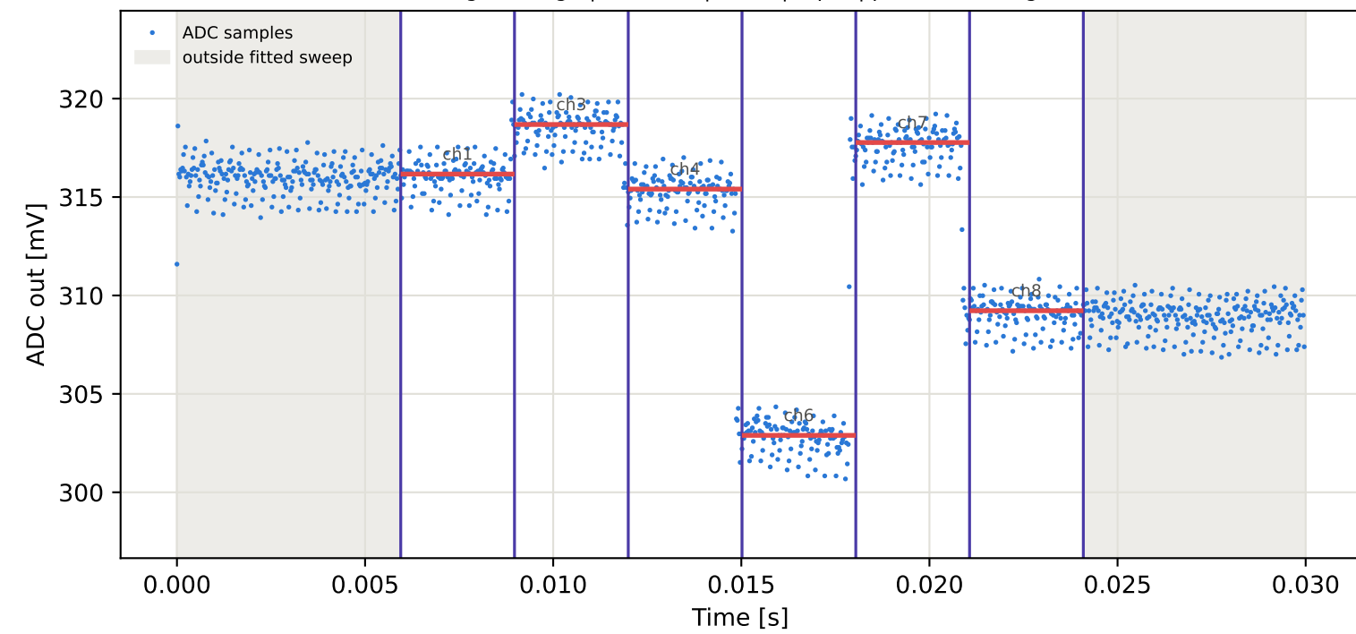
Tag3 &lt;- Tag15 | 945 MHz | run 0 | rep 1 | phase 98.73 deg
