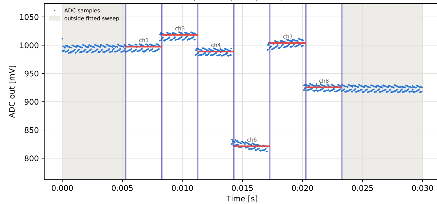
Tag4 &lt;- Tag7 | 935 MHz | run 0 | rep 1 | phase 77.46 deg
