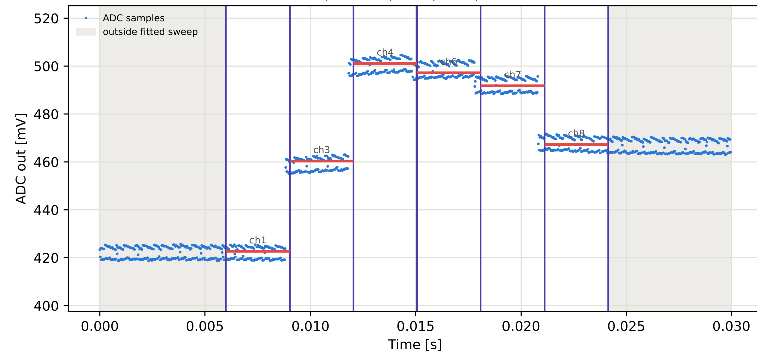
Tag2 &lt;- Tag1 | 855 MHz | run 0 | rep 1 | phase 43.31 deg
