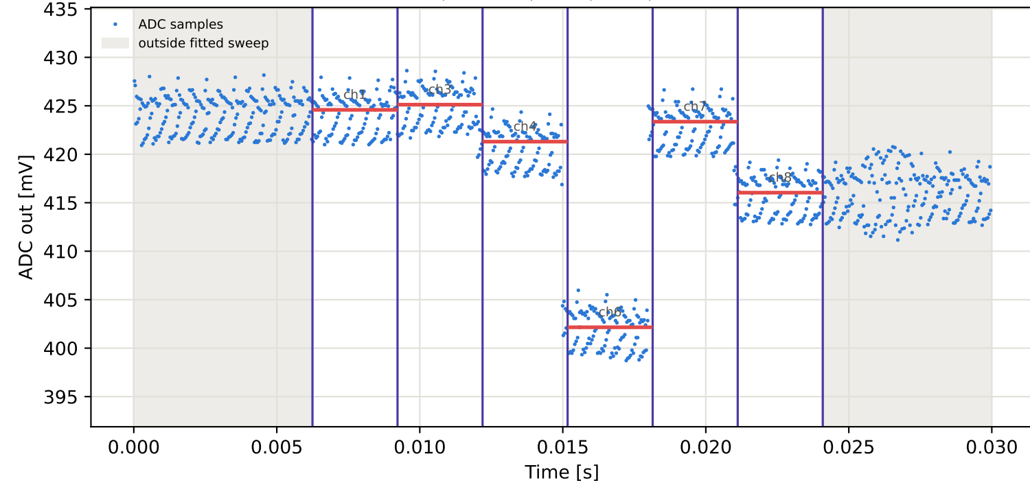
Tag6 &lt;- Tag5 | 925 MHz | run 0 | rep 1 | phase 10.90 deg
