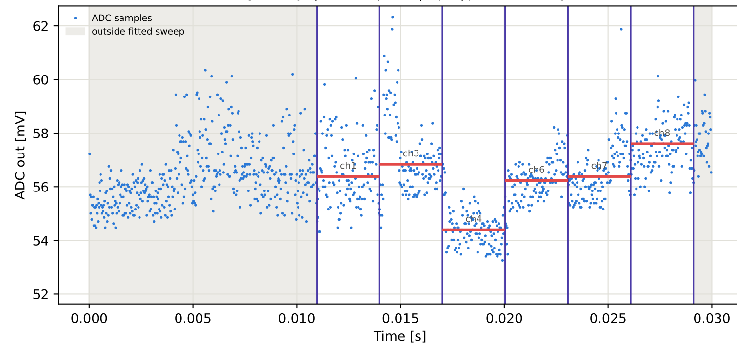
Tag2 &lt;- Tag7 | 975 MHz | run 0 | rep 1 | phase 0.65 deg
