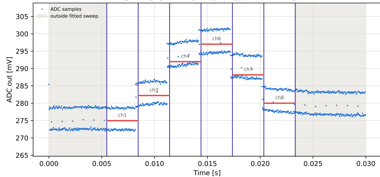
Tag3 &lt;- Tag15 | 905 MHz | run 0 | rep 1 | phase -15.76 deg
