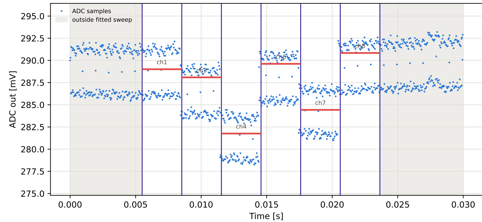
Tag6 &lt;- Tag5 | 985 MHz | run 0 | rep 1 | phase 90.94 deg
