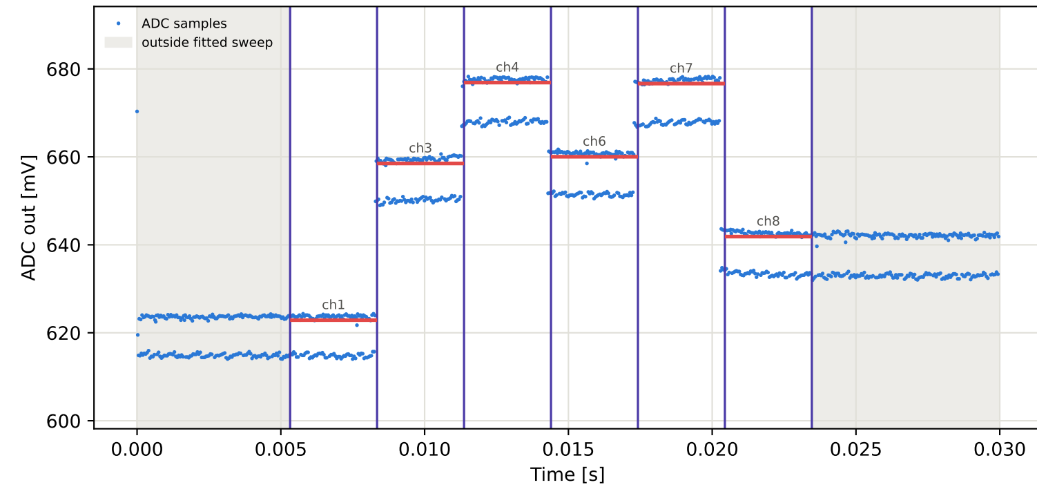
Tag8 &lt;- Tag6 | 835 MHz | run 0 | rep 1 | phase 128.24 deg
