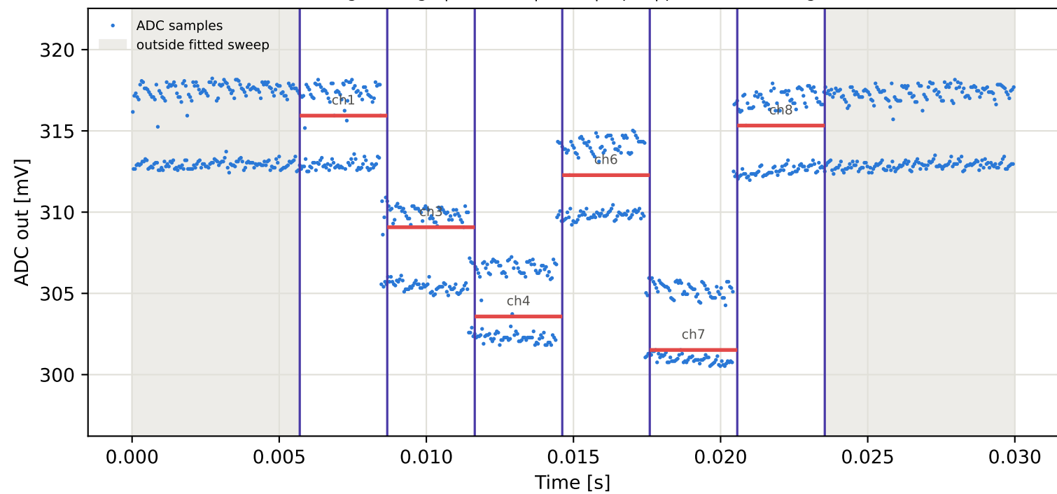
Tag8 &lt;- Tag10 | 825 MHz | run 0 | rep 1 | phase -21.07 deg
