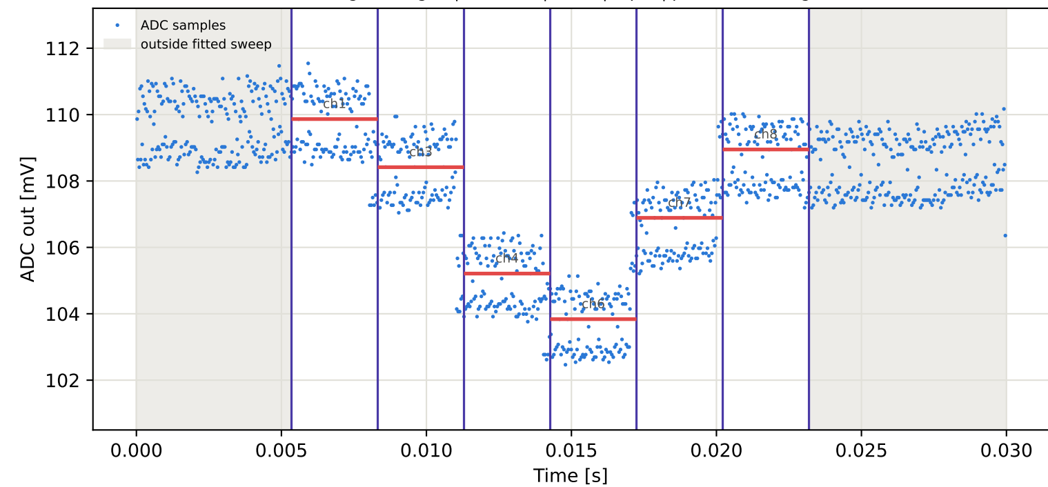
Tag1 &lt;- Tag2 | 935 MHz | run 0 | rep 1 | phase -32.65 deg
