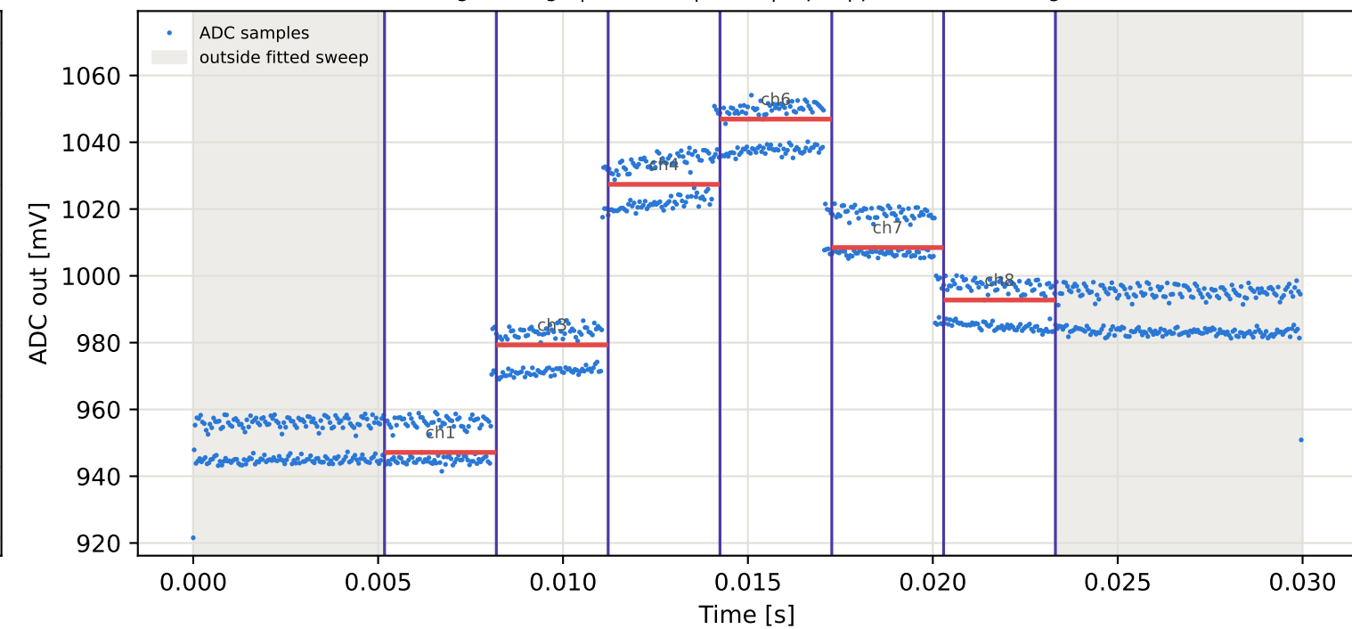
Tag3 &lt;- Tag9 | 885 MHz | run 0 | rep 1 | phase -24.59 deg
