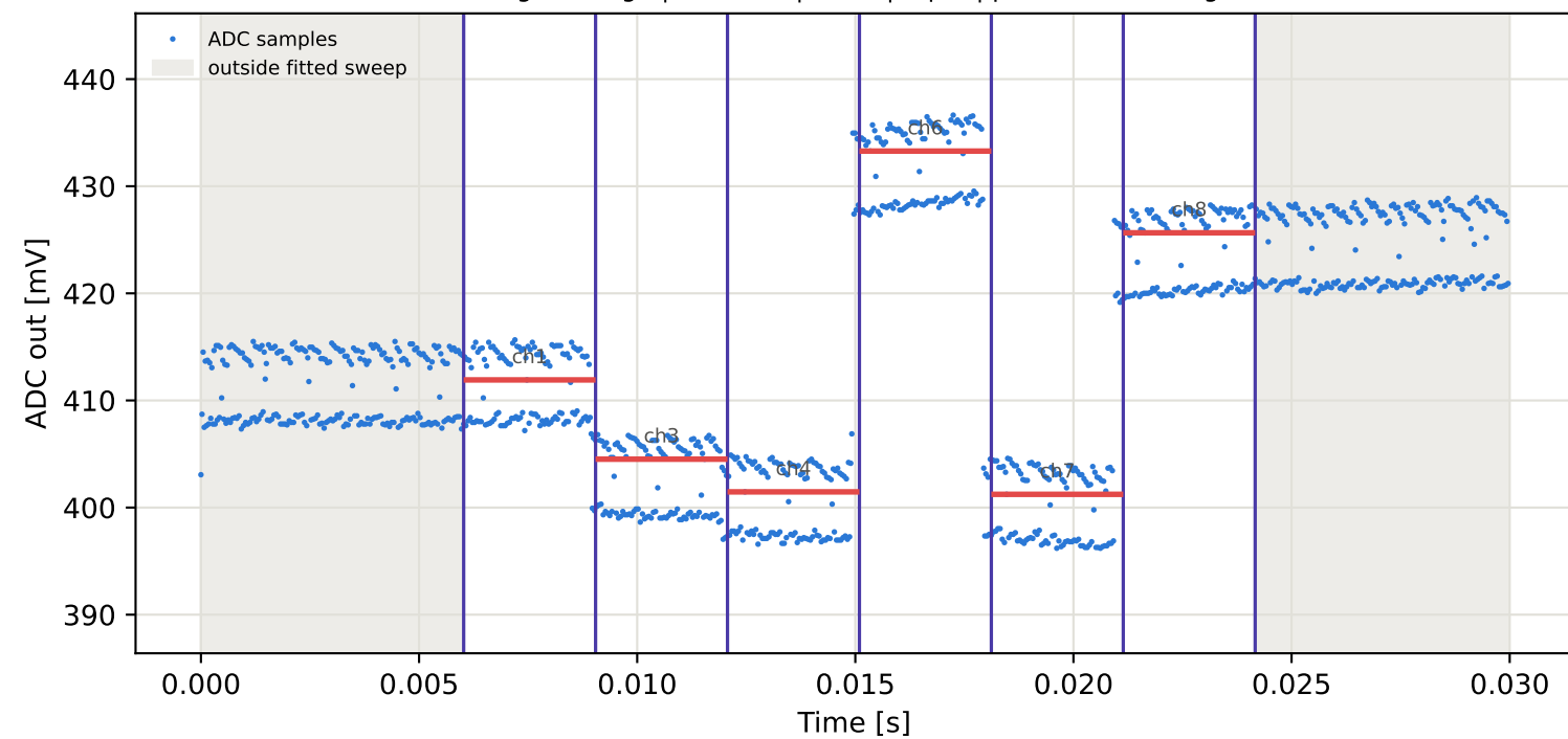
Tag4 &lt;- Tag3 | 955 MHz | run 0 | rep 1 | phase 155.62 deg
