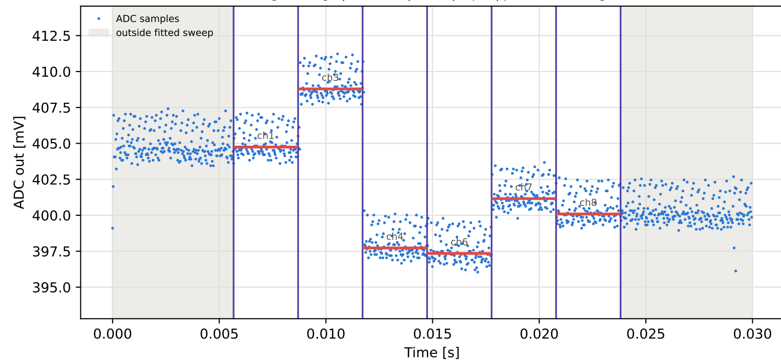
Tag3 &lt;- Tag15 | 835 MHz | run 0 | rep 1 | phase 40.82 deg
