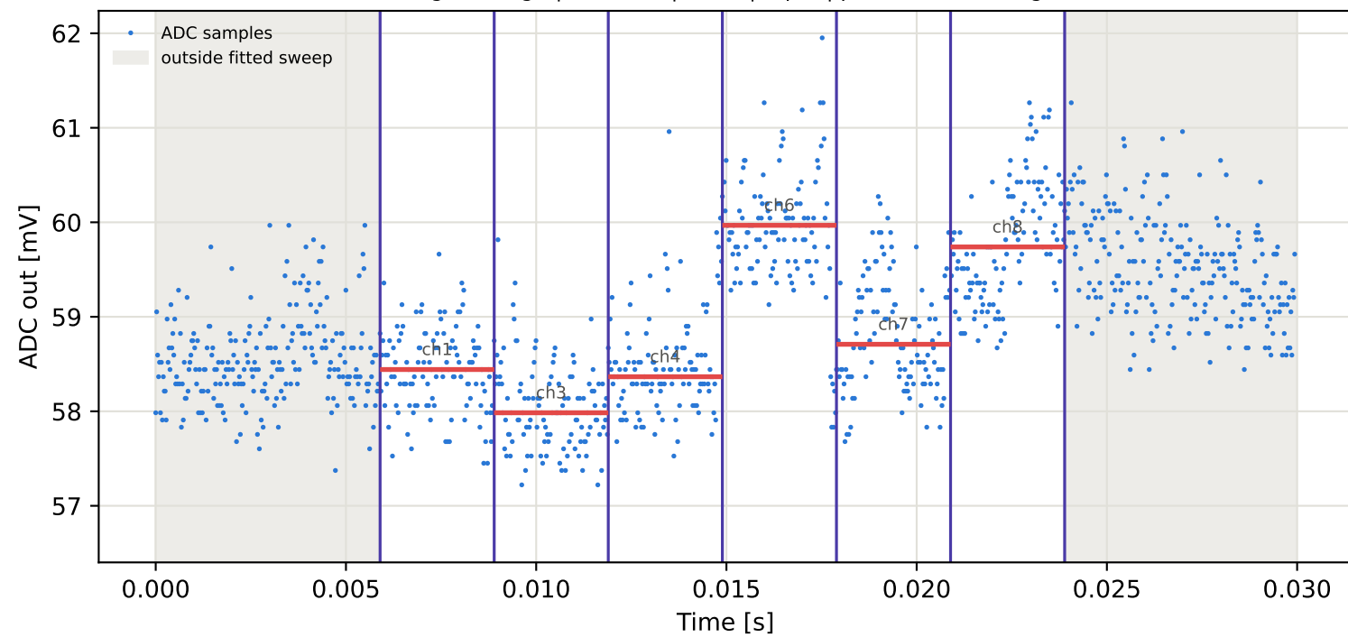
Tag2 &lt;- Tag6 | 905 MHz | run 0 | rep 1 | phase 85.86 deg
