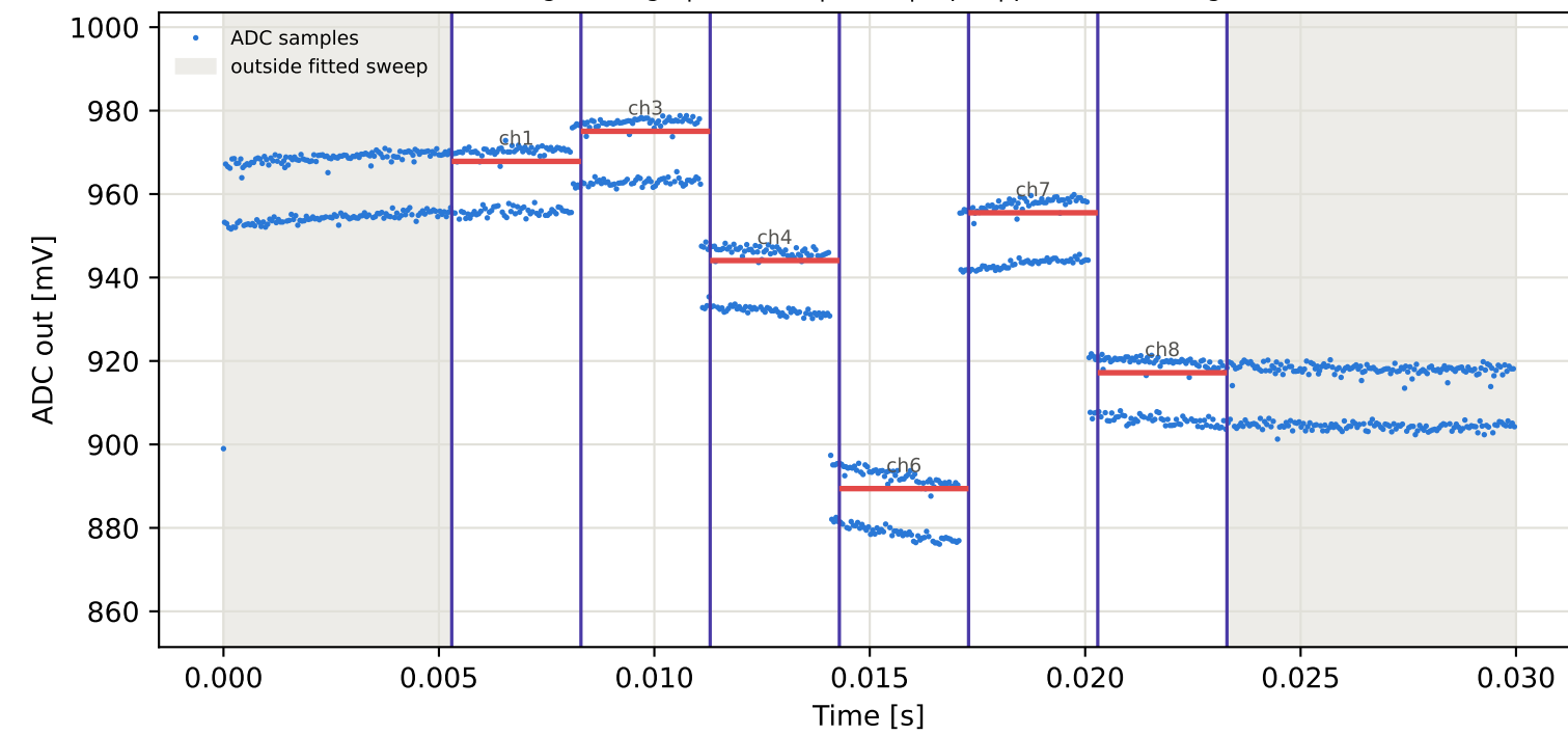
Tag6 &lt;- Tag9 | 885 MHz | run 0 | rep 1 | phase -1.86 deg
