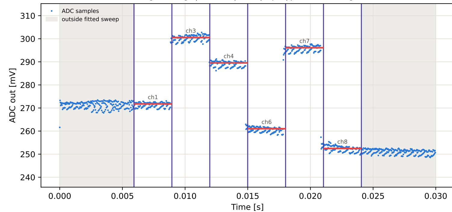
Tag10 &lt;- Tag8 | 845 MHz | run 0 | rep 1 | phase -165.43 deg
