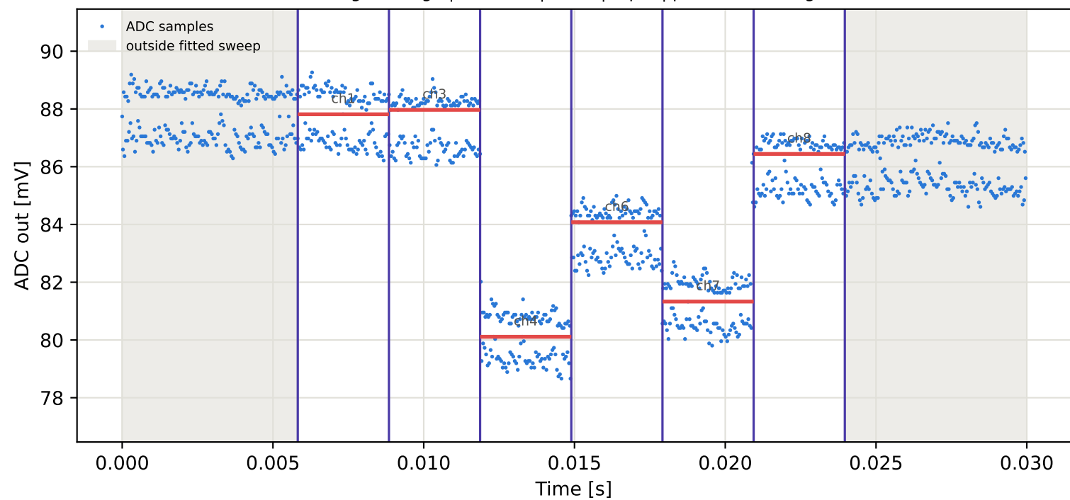
Tag9 &lt;- Tag8 | 785 MHz | run 0 | rep 1 | phase 83.16 deg
