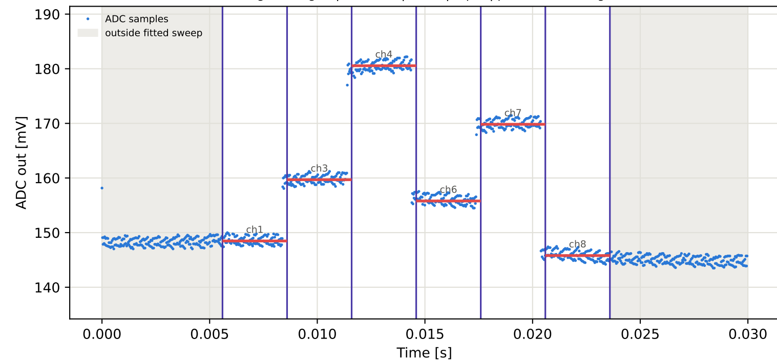
Tag9 &lt;- Tag16 | 965 MHz | run 0 | rep 1 | phase -8.80 deg
