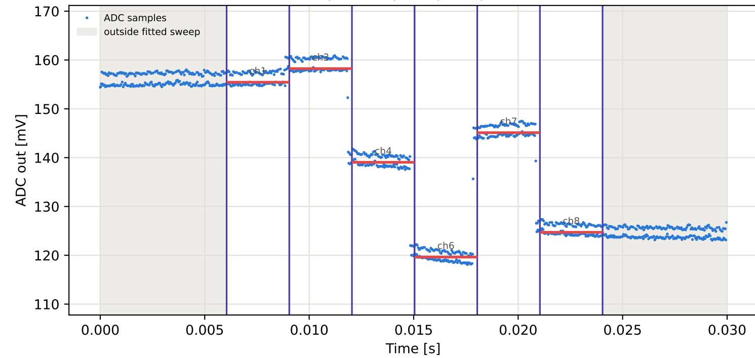
Tag10 &lt;- Tag1 | 865 MHz | run 0 | rep 1 | phase 23.58 deg
