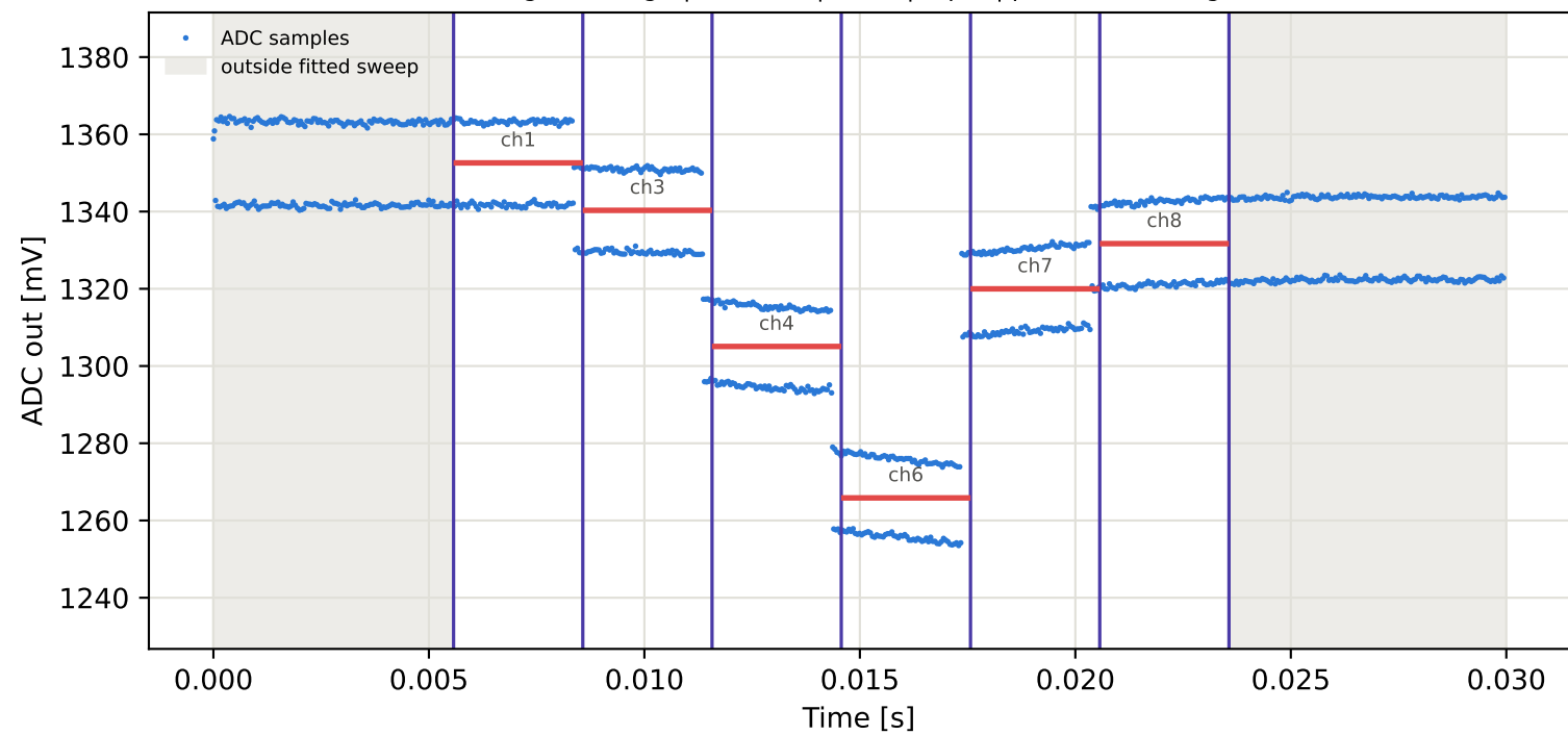
Tag16 &lt;- Tag1 | 925 MHz | run 0 | rep 1 | phase 142.58 deg
