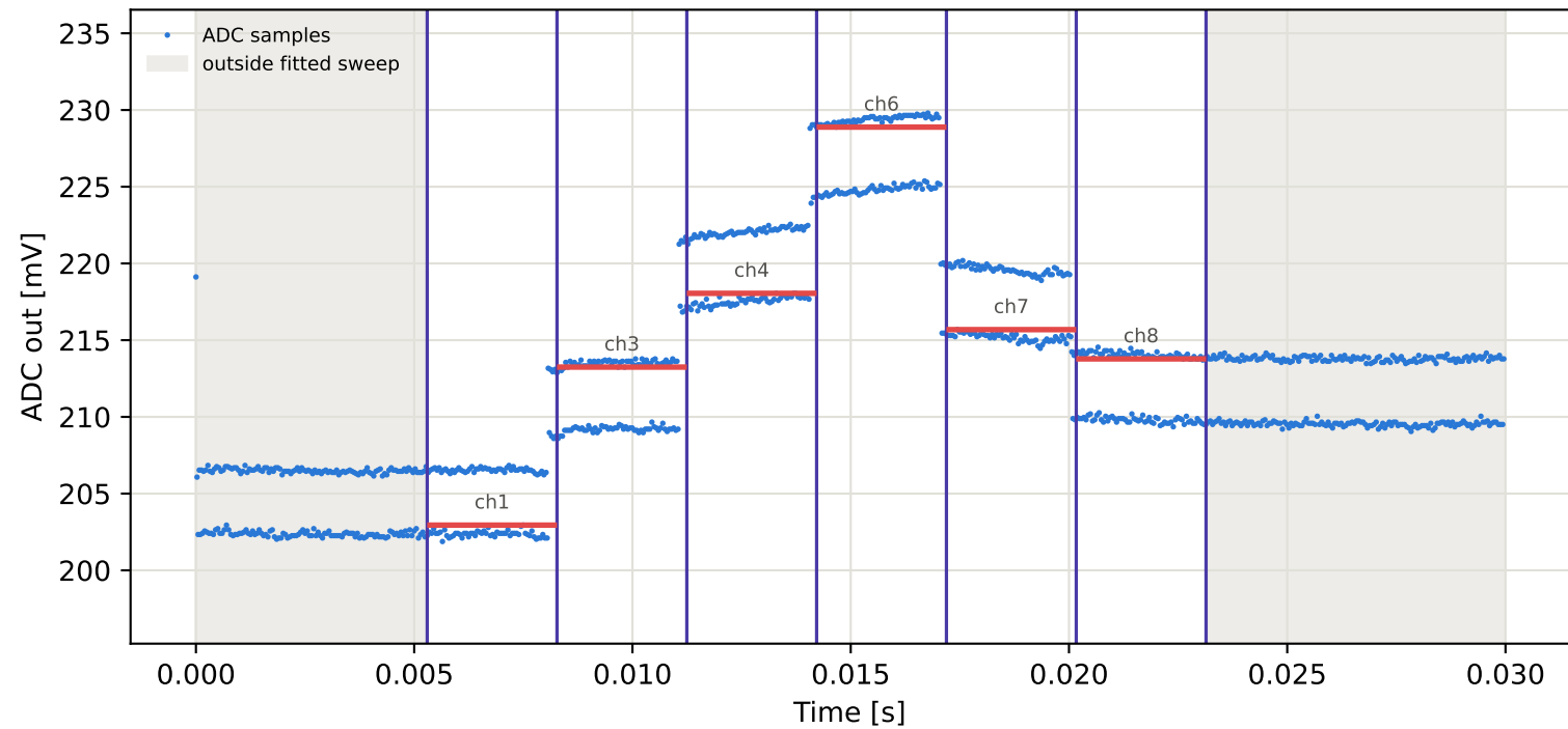
Tag10 &lt;- Tag1 | 895 MHz | run 0 | rep 1 | phase 53.39 deg
