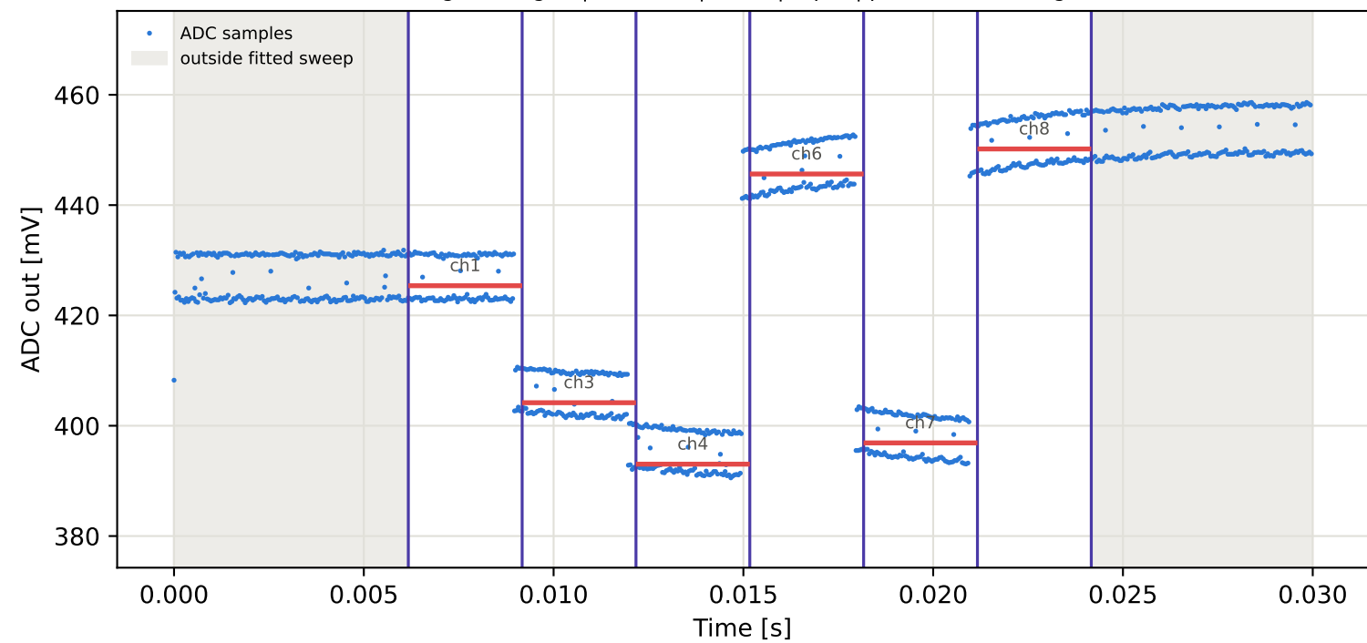
Tag6 &lt;- Tag2 | 925 MHz | run 0 | rep 1 | phase -90.45 deg
