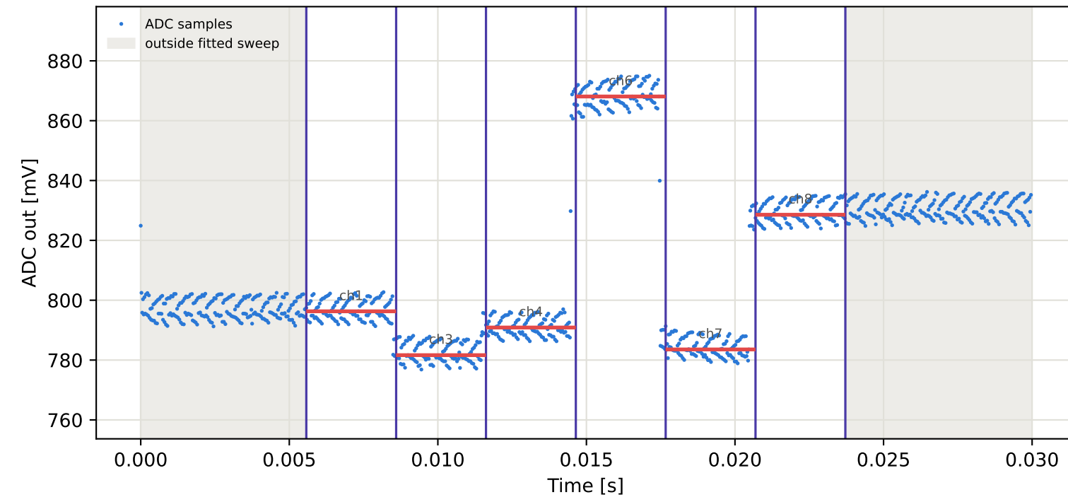
Tag8 &lt;- Tag6 | 945 MHz | run 0 | rep 1 | phase 174.28 deg
