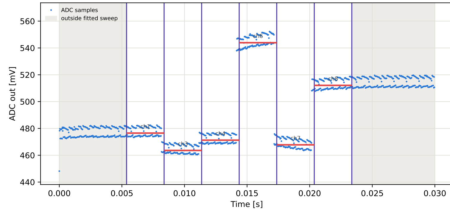
Tag9 &lt;- Tag16 | 925 MHz | run 0 | rep 1 | phase -30.36 deg
