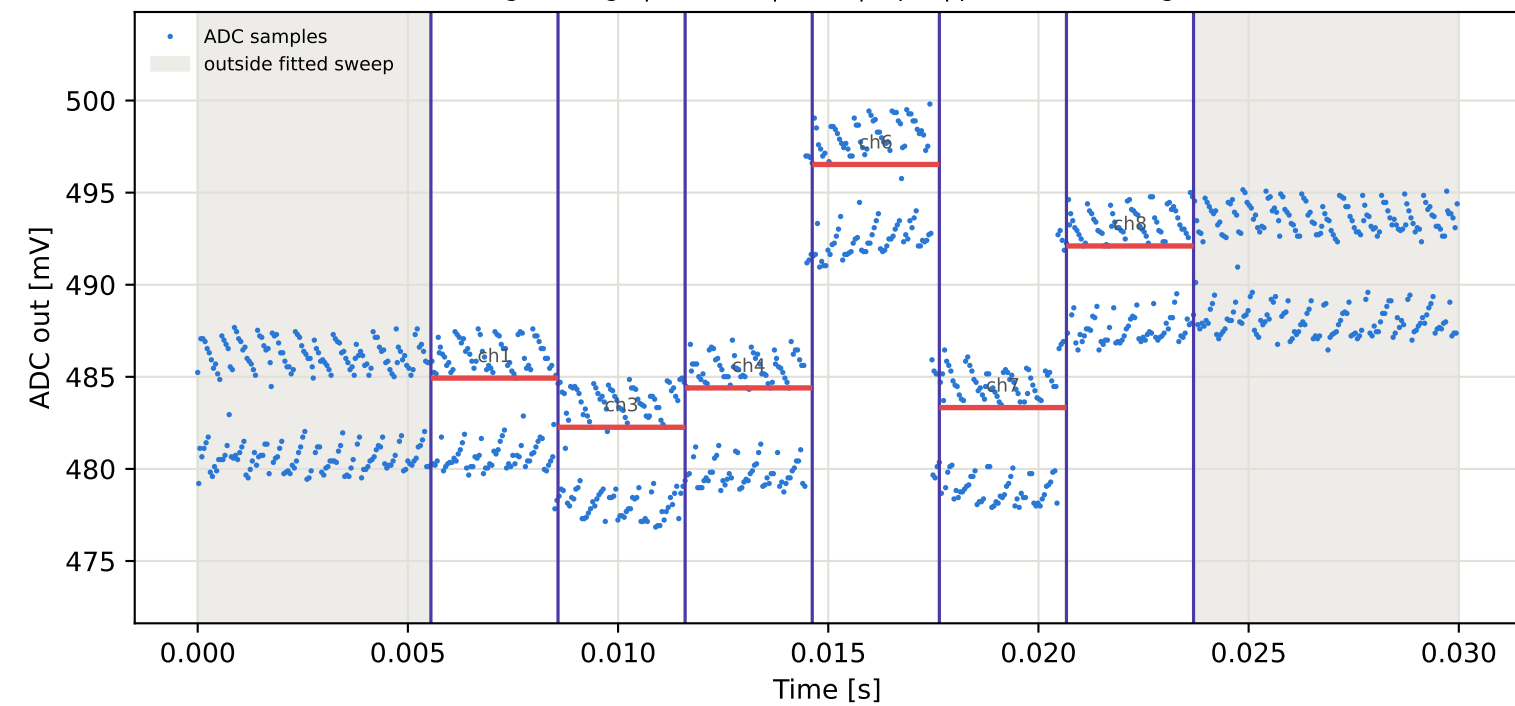
Tag9 &lt;- Tag15 | 925 MHz | run 0 | rep 1 | phase -64.47 deg
