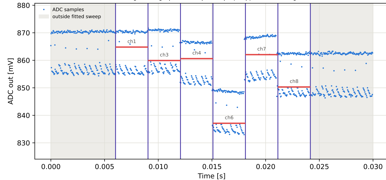
Tag7 &lt;- Tag5 | 925 MHz | run 0 | rep 1 | phase 5.67 deg
