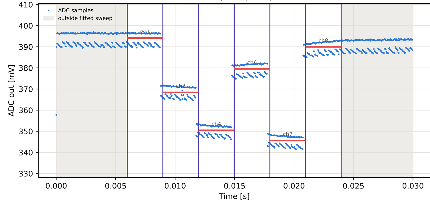
Tag5 &lt;- Tag2 | 825 MHz | run 0 | rep 1 | phase -65.77 deg
