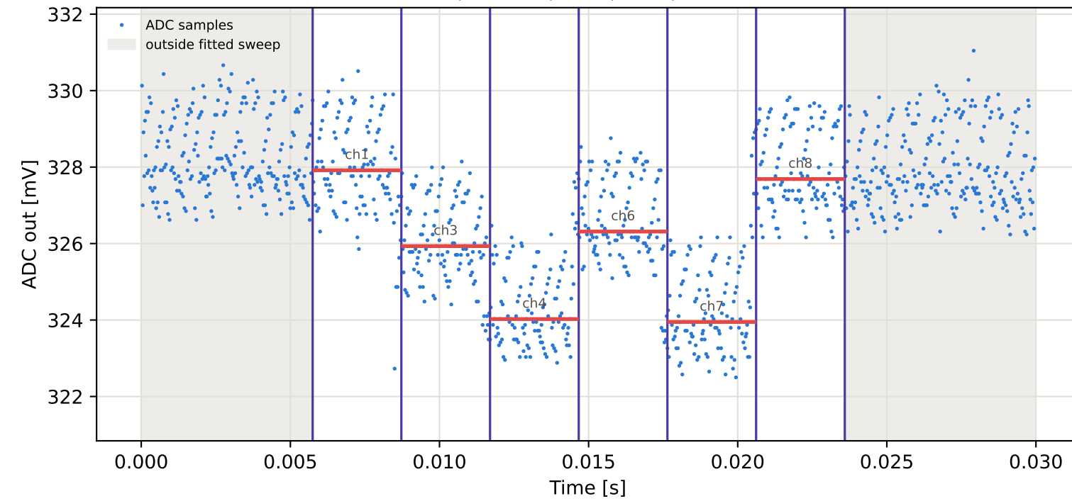
Tag4 &lt;- Tag9 | 825 MHz | run 0 | rep 1 | phase 103.18 deg
