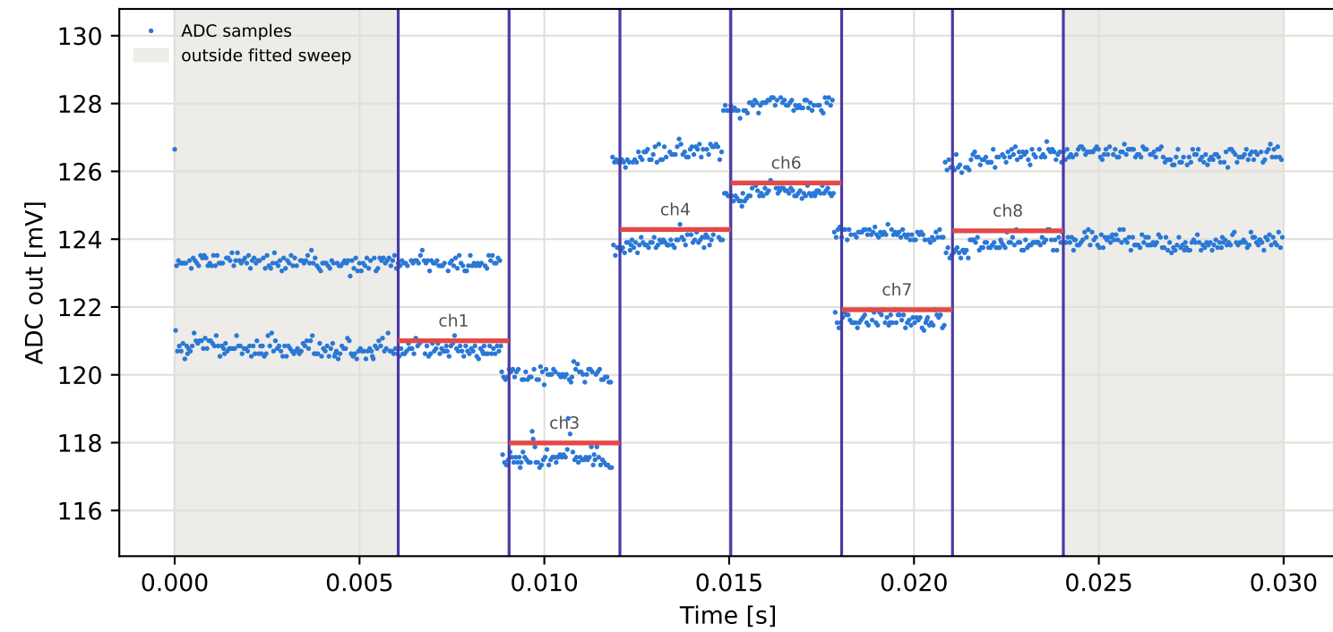
Tag1 &lt;- Tag2 | 825 MHz | run 0 | rep 1 | phase -138.19 deg
