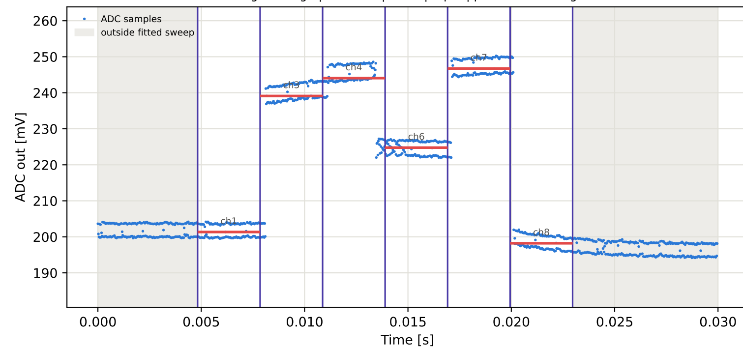
Tag9 &lt;- Tag5 | 855 MHz | run 0 | rep 1 | phase -124.36 deg
