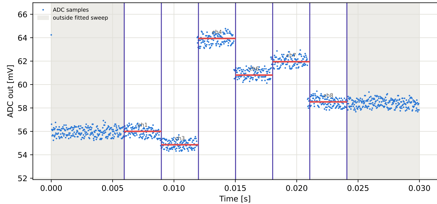
Tag5 &lt;- Tag1 | 785 MHz | run 0 | rep 1 | phase 5.22 deg
