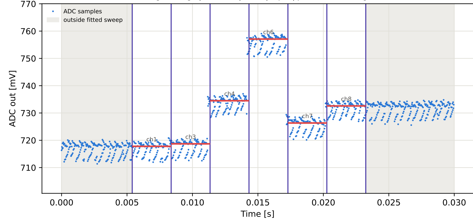
Tag8 &lt;- Tag10 | 945 MHz | run 0 | rep 1 | phase 125.37 deg
