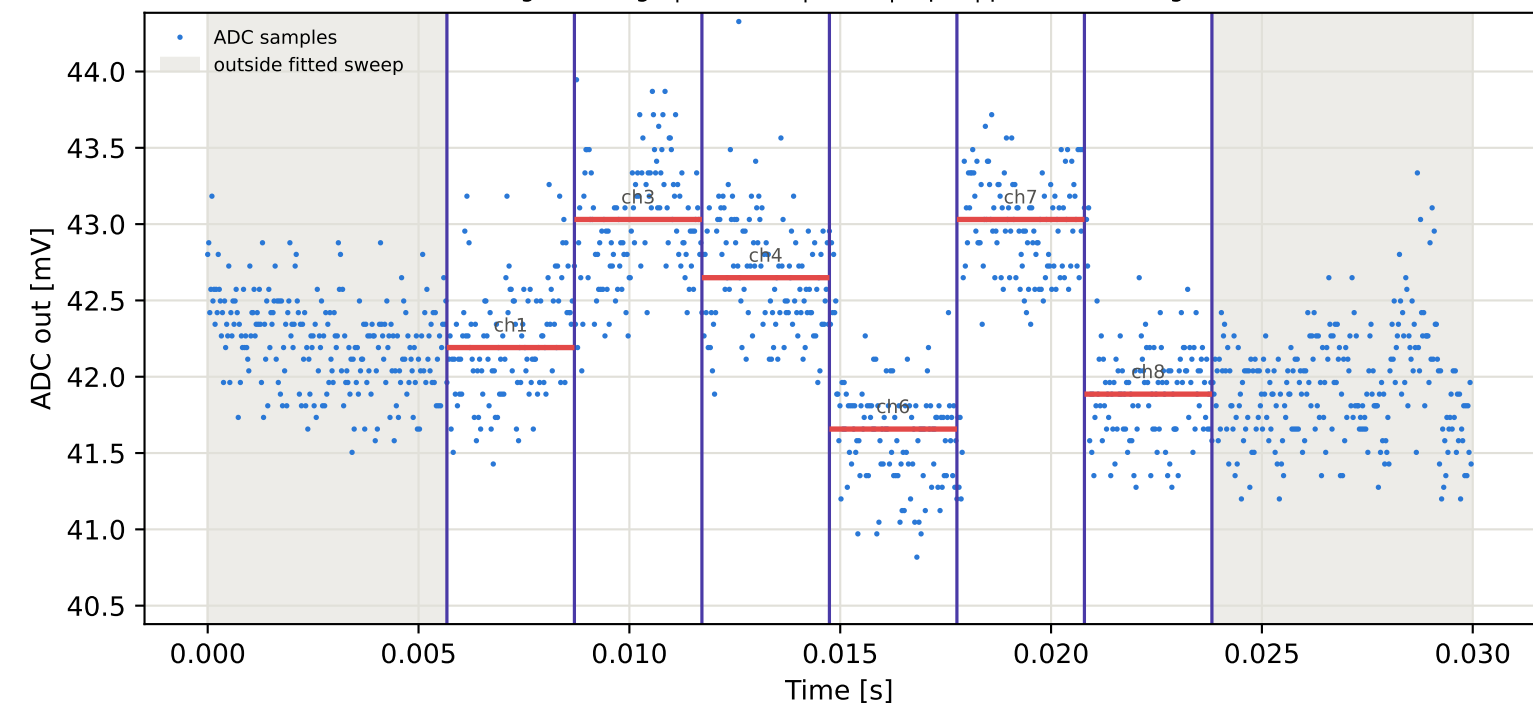
Tag15 &lt;- Tag1 | 775 MHz | run 0 | rep 1 | phase -5.76 deg
