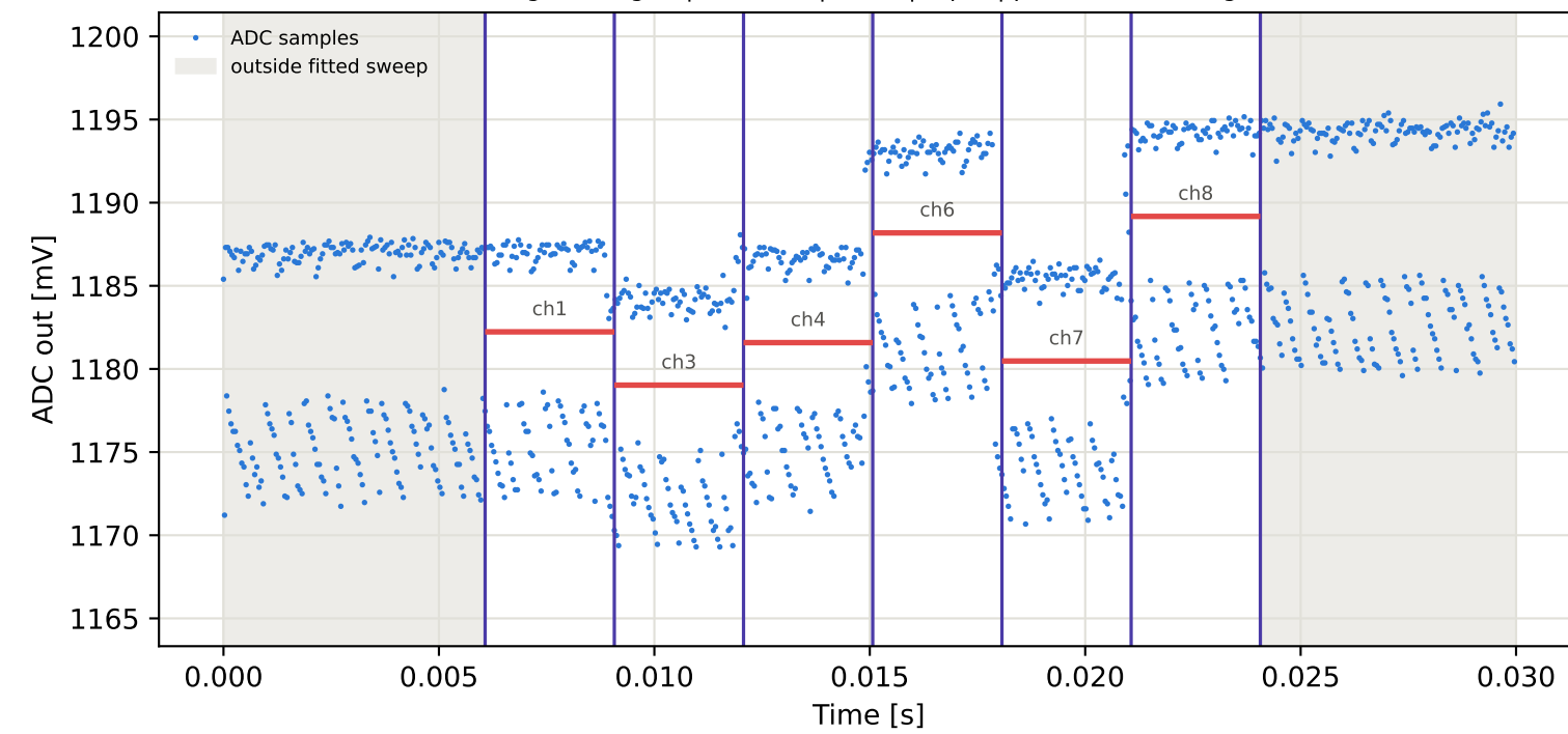
Tag5 &lt;- Tag16 | 875 MHz | run 0 | rep 1 | phase 179.35 deg
