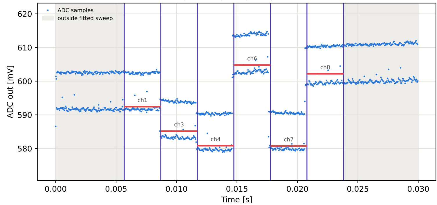
Tag8 &lt;- Tag7 | 965 MHz | run 0 | rep 1 | phase 142.86 deg
