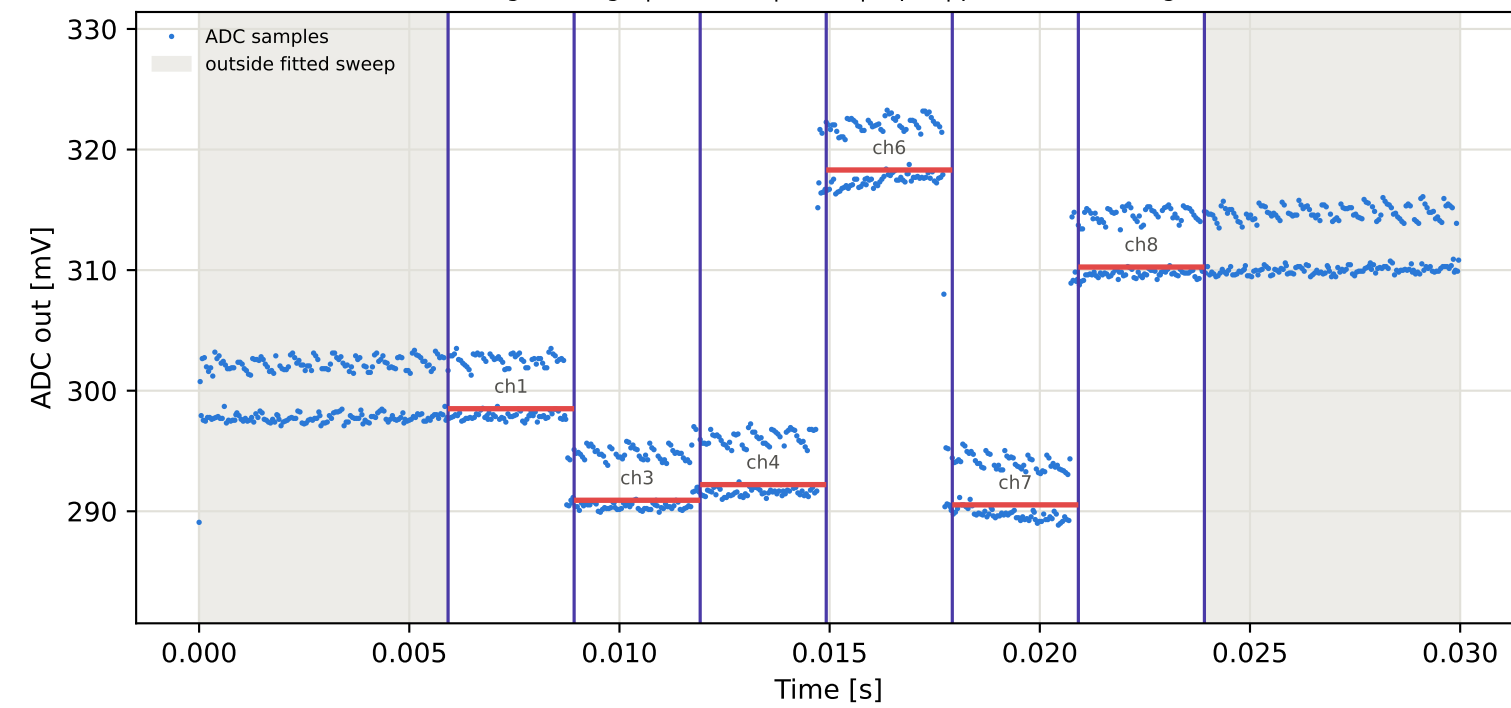
Tag6 &lt;- Tag9 | 945 MHz | run 0 | rep 1 | phase -10.07 deg
