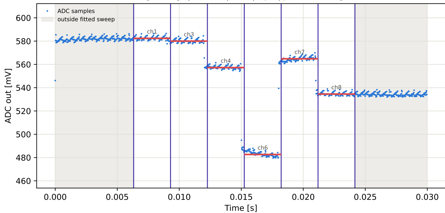
Tag8 &lt;- Tag1 | 905 MHz | run 0 | rep 1 | phase 28.85 deg
