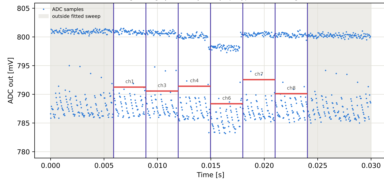
Tag8 &lt;- Tag4 | 945 MHz | run 0 | rep 1 | phase 177.63 deg
