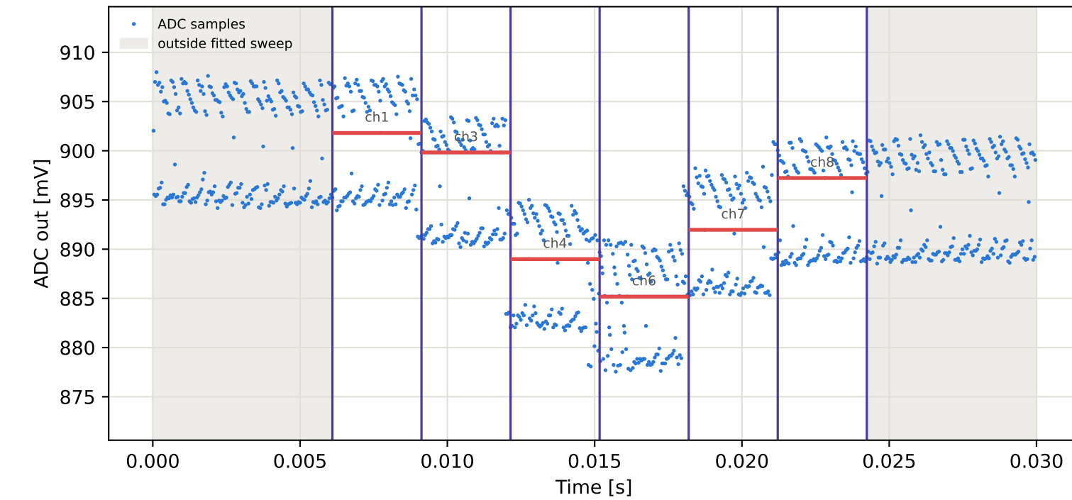
Tag4 &lt;- Tag9 | 895 MHz | run 0 | rep 1 | phase 165.92 deg
