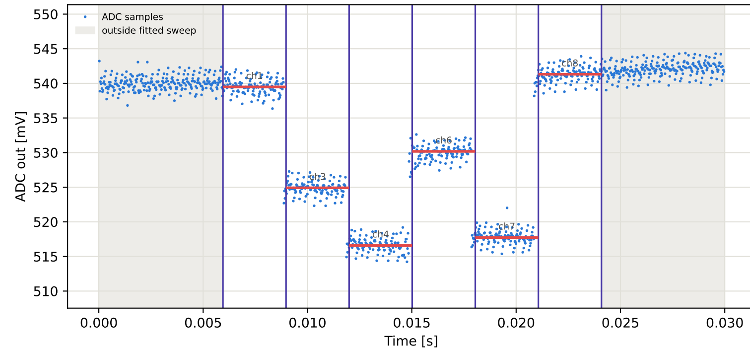
Tag1 &lt;- Tag9 | 875 MHz | run 0 | rep 1 | phase -0.53 deg
