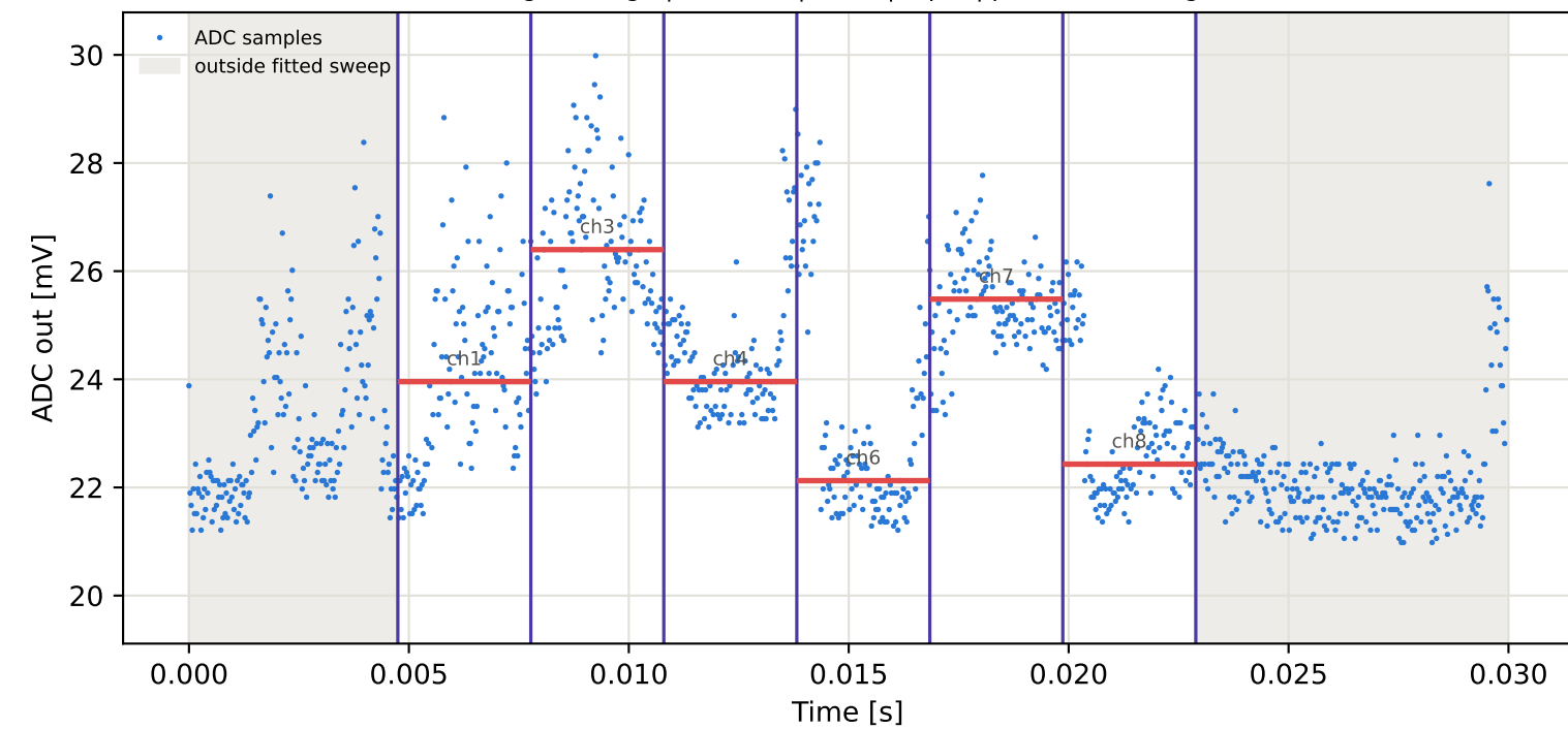
Tag2 &lt;- Tag5 | 805 MHz | run 0 | rep 1 | phase 35.21 deg
