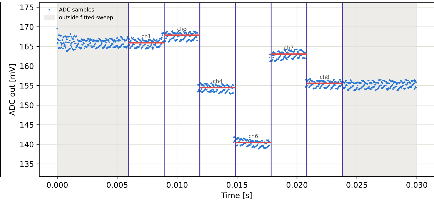
Tag9 &lt;- Tag8 | 965 MHz | run 0 | rep 1 | phase 24.48 deg
