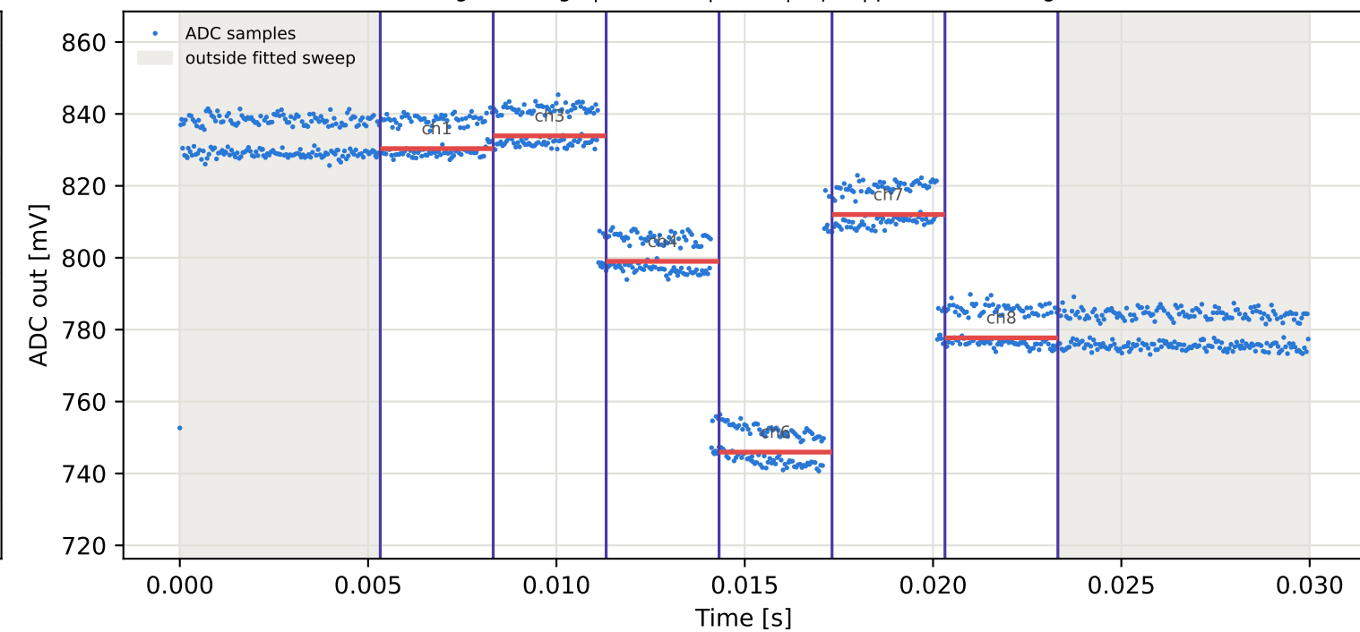
Tag16 &lt;- Tag7 | 885 MHz | run 0 | rep 1 | phase 22.36 deg
