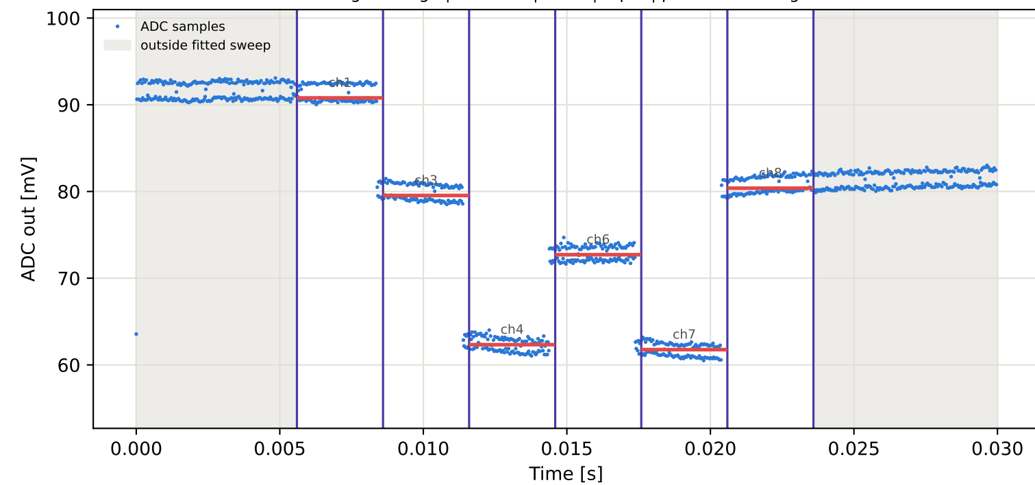
Tag9 &lt;- Tag5 | 825 MHz | run 0 | rep 1 | phase 68.09 deg
