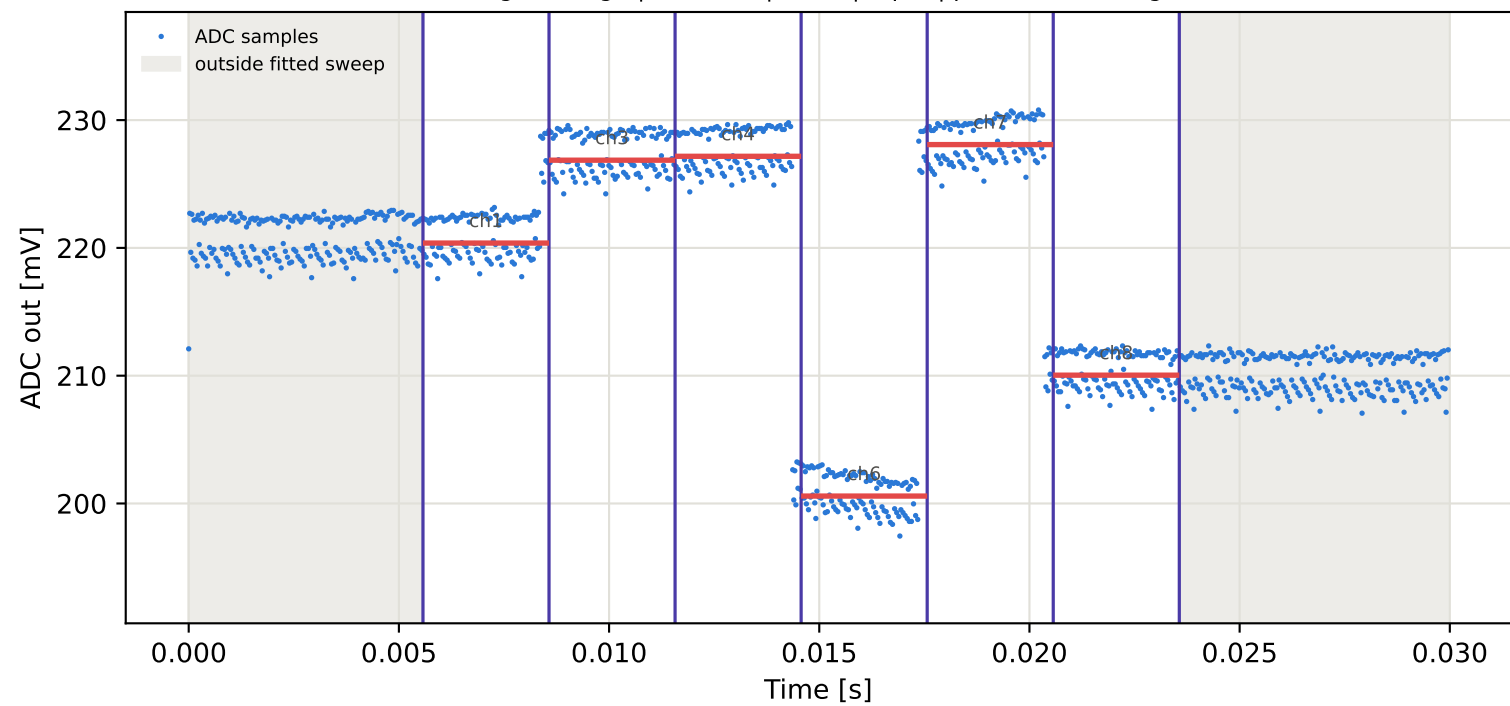
Tag3 &lt;- Tag7 | 955 MHz | run 0 | rep 1 | phase 0.27 deg
