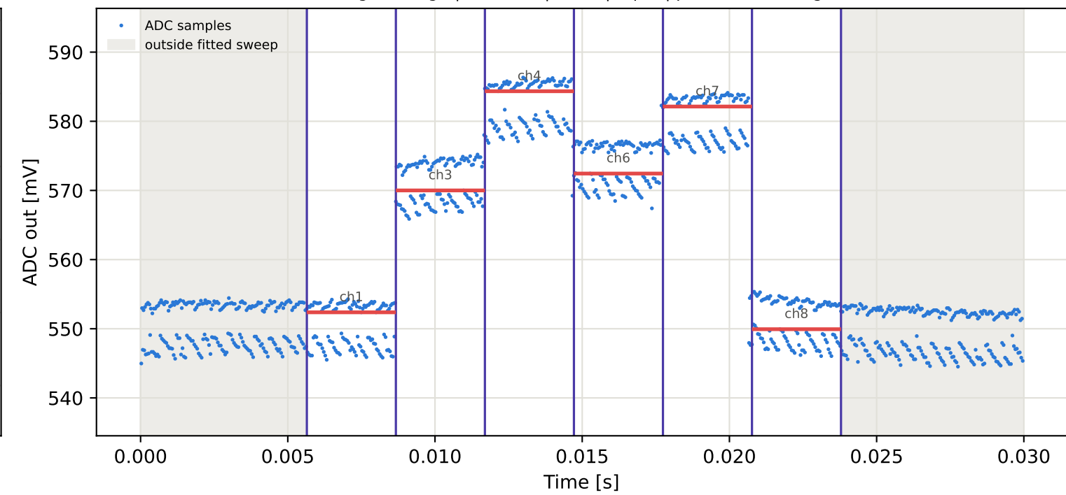
Tag9 &lt;- Tag6 | 875 MHz | run 0 | rep 1 | phase -80.94 deg
