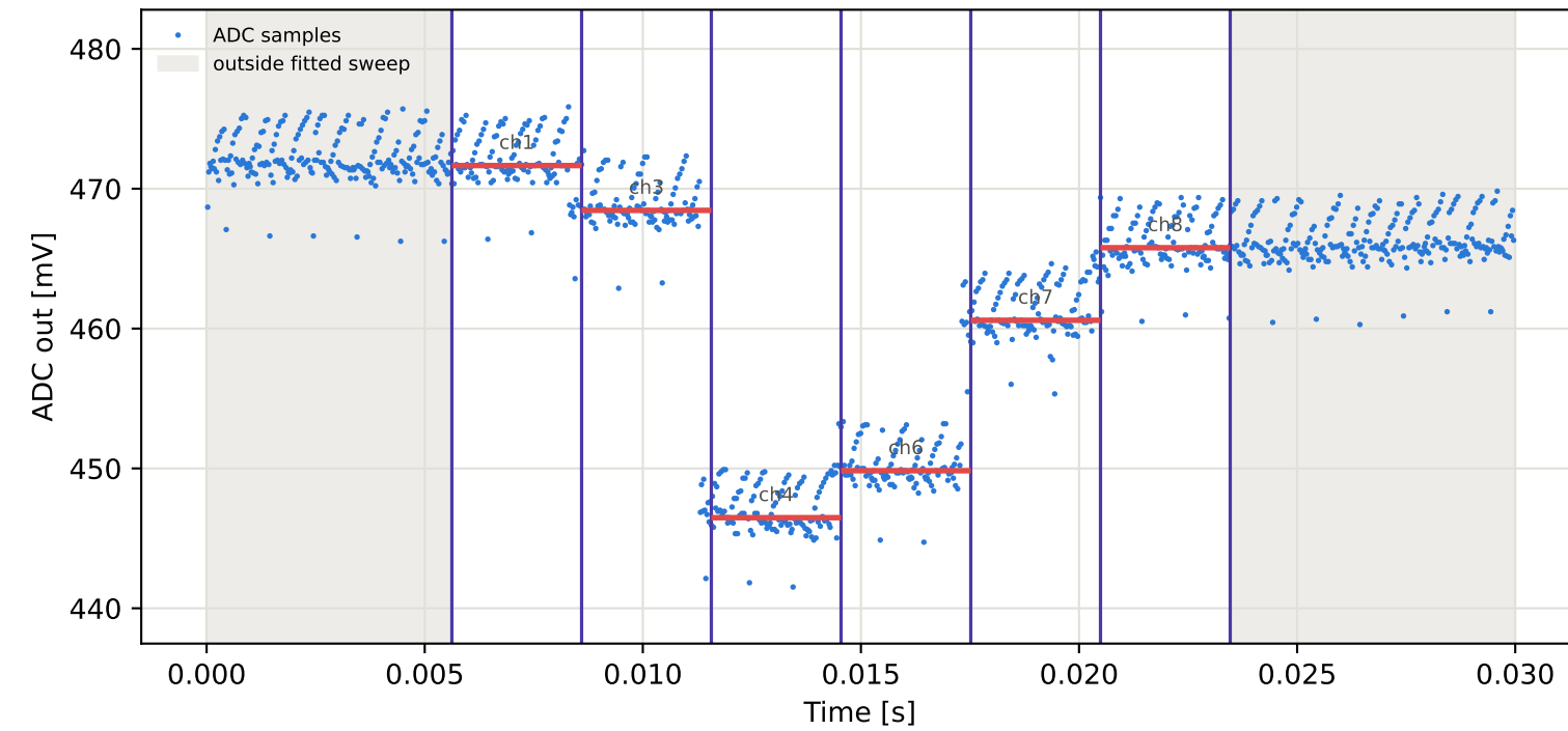
Tag16 &lt;- Tag6 | 975 MHz | run 0 | rep 1 | phase 136.86 deg
