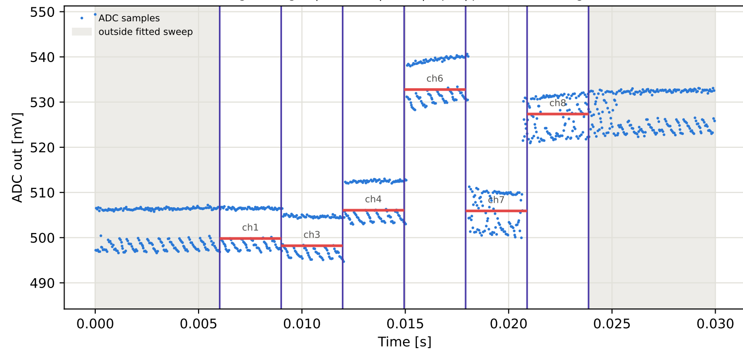
Tag6 &lt;- Tag3 | 895 MHz | run 0 | rep 1 | phase -79.22 deg
