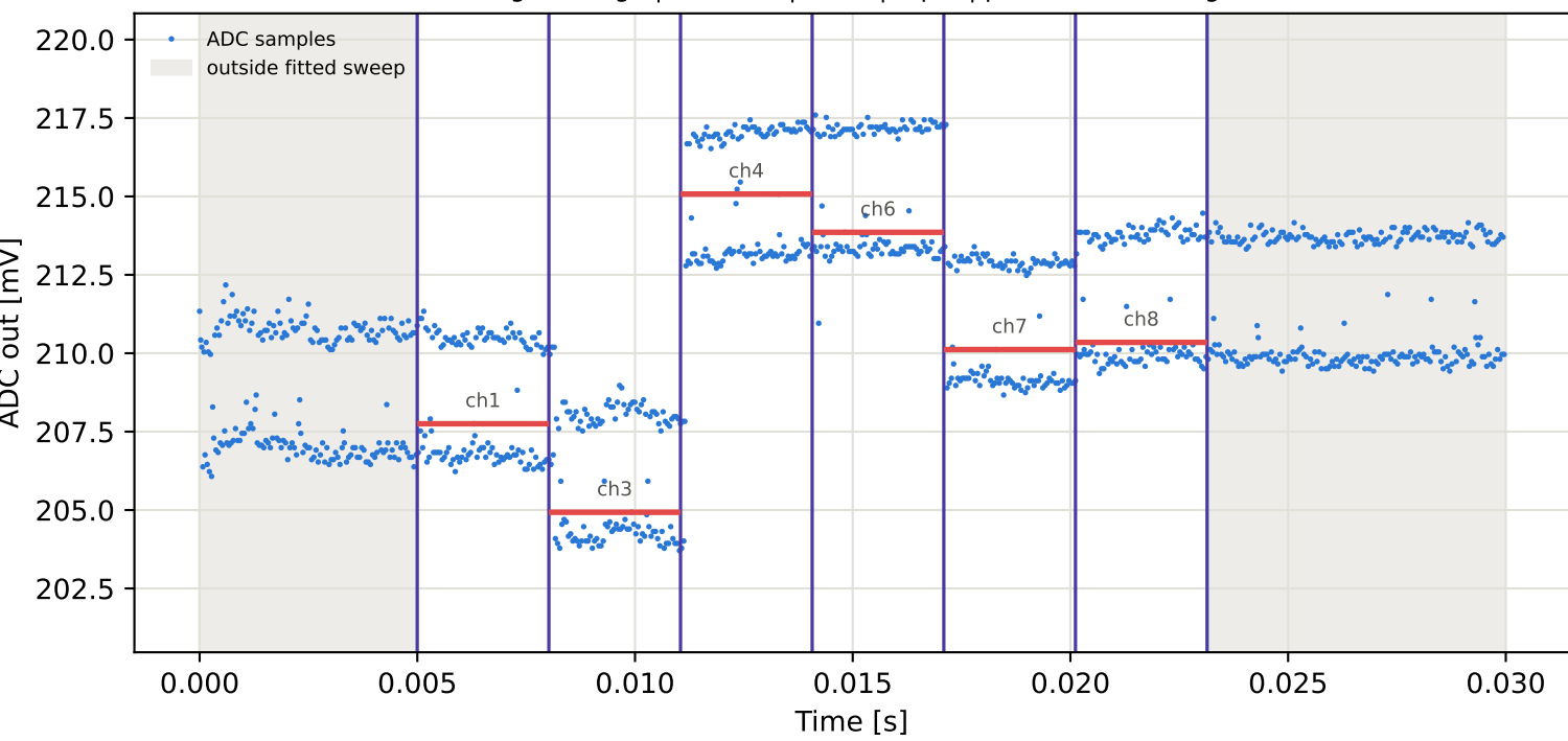
Tag6 &lt;- Tag1 | 805 MHz | run 0 | rep 1 | phase -125.23 deg
