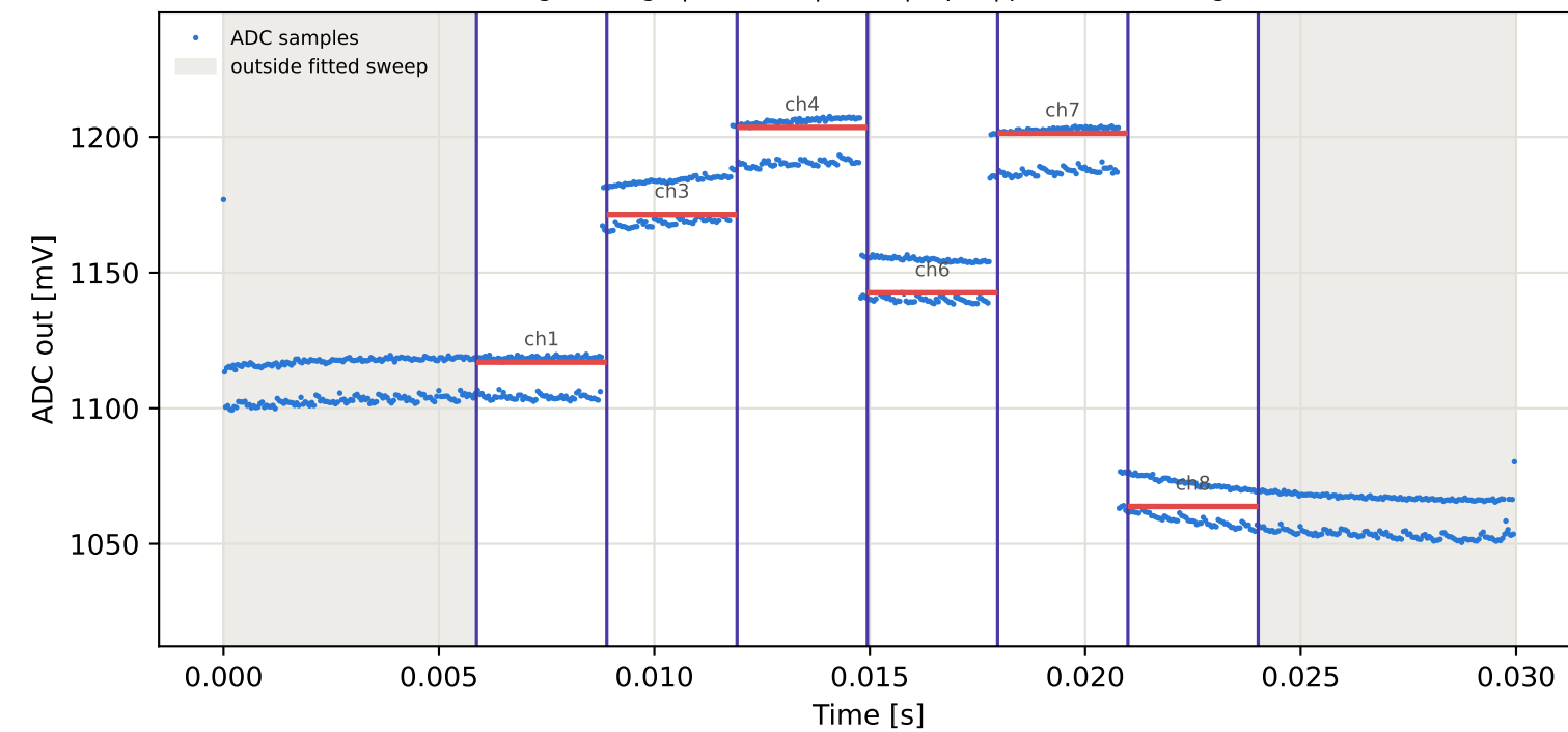
Tag4 &lt;- Tag7 | 885 MHz | run 0 | rep 1 | phase 11.32 deg
