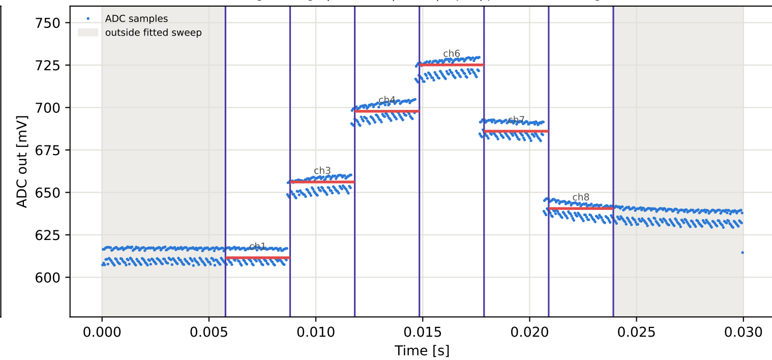
Tag3 &lt;- Tag7 | 895 MHz | run 0 | rep 1 | phase -124.48 deg
