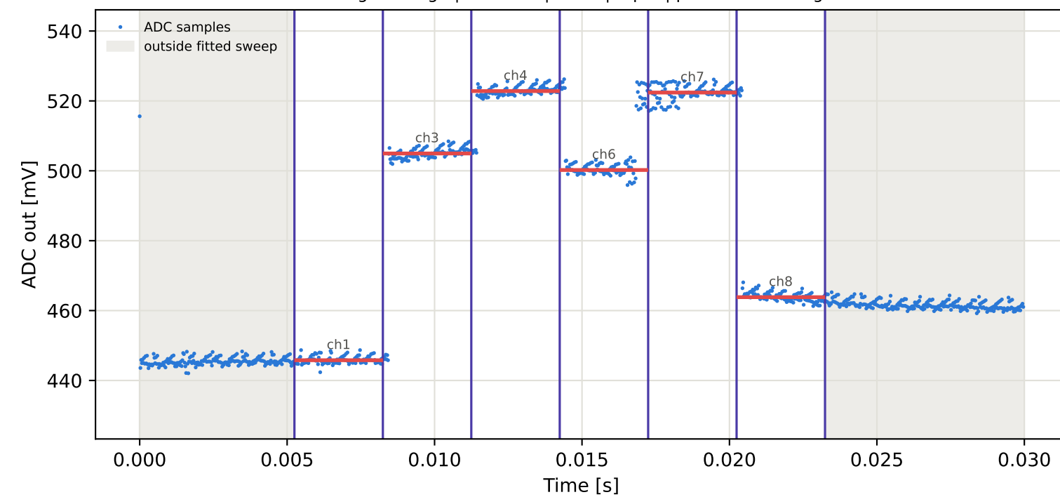
Tag4 &lt;- Tag7 | 865 MHz | run 0 | rep 1 | phase -11.75 deg
