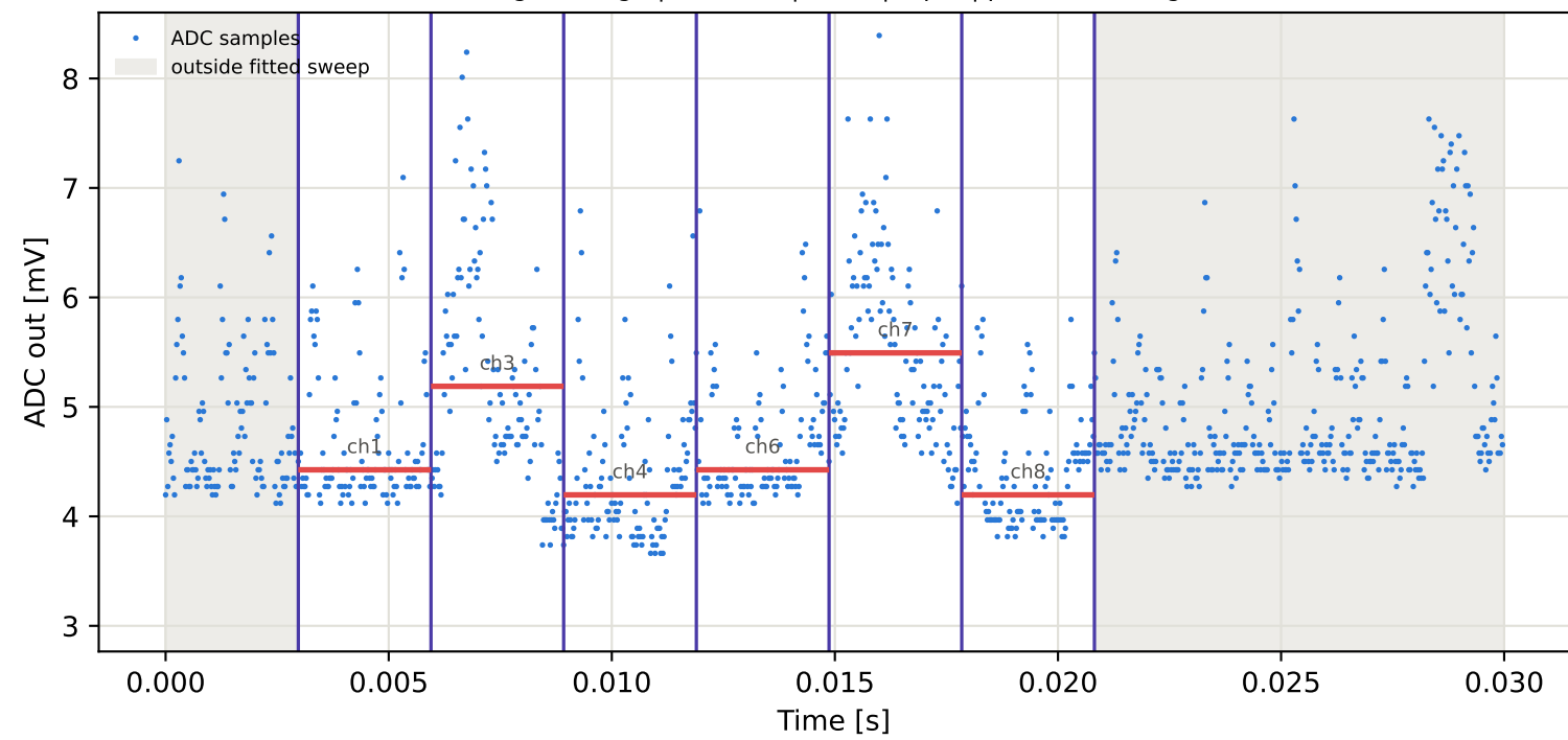
Tag2 &lt;- Tag5 | 785 MHz | run 0 | rep 1 | phase 100.09 deg
