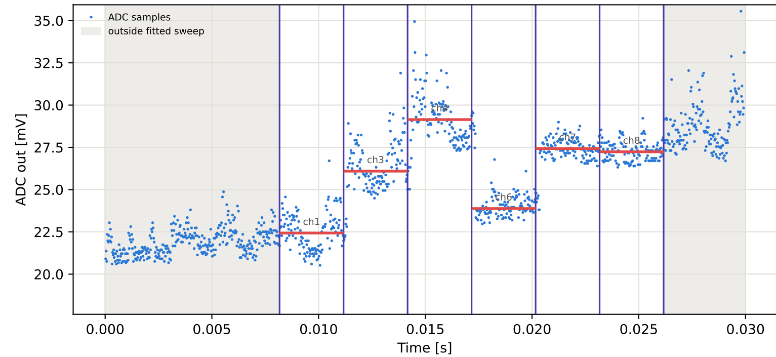
Tag2 &lt;- Tag7 | 865 MHz | run 0 | rep 1 | phase 54.59 deg
