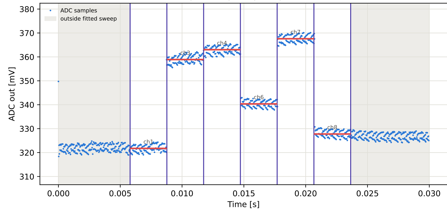
Tag5 &lt;- Tag4 | 825 MHz | run 0 | rep 1 | phase -63.70 deg
