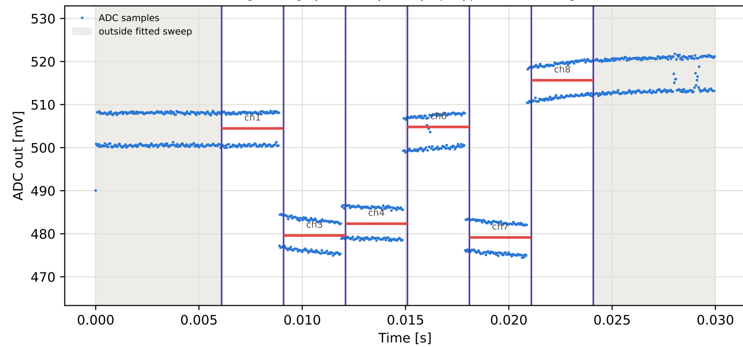
Tag3 &lt;- Tag15 | 865 MHz | run 0 | rep 1 | phase -5.16 deg
