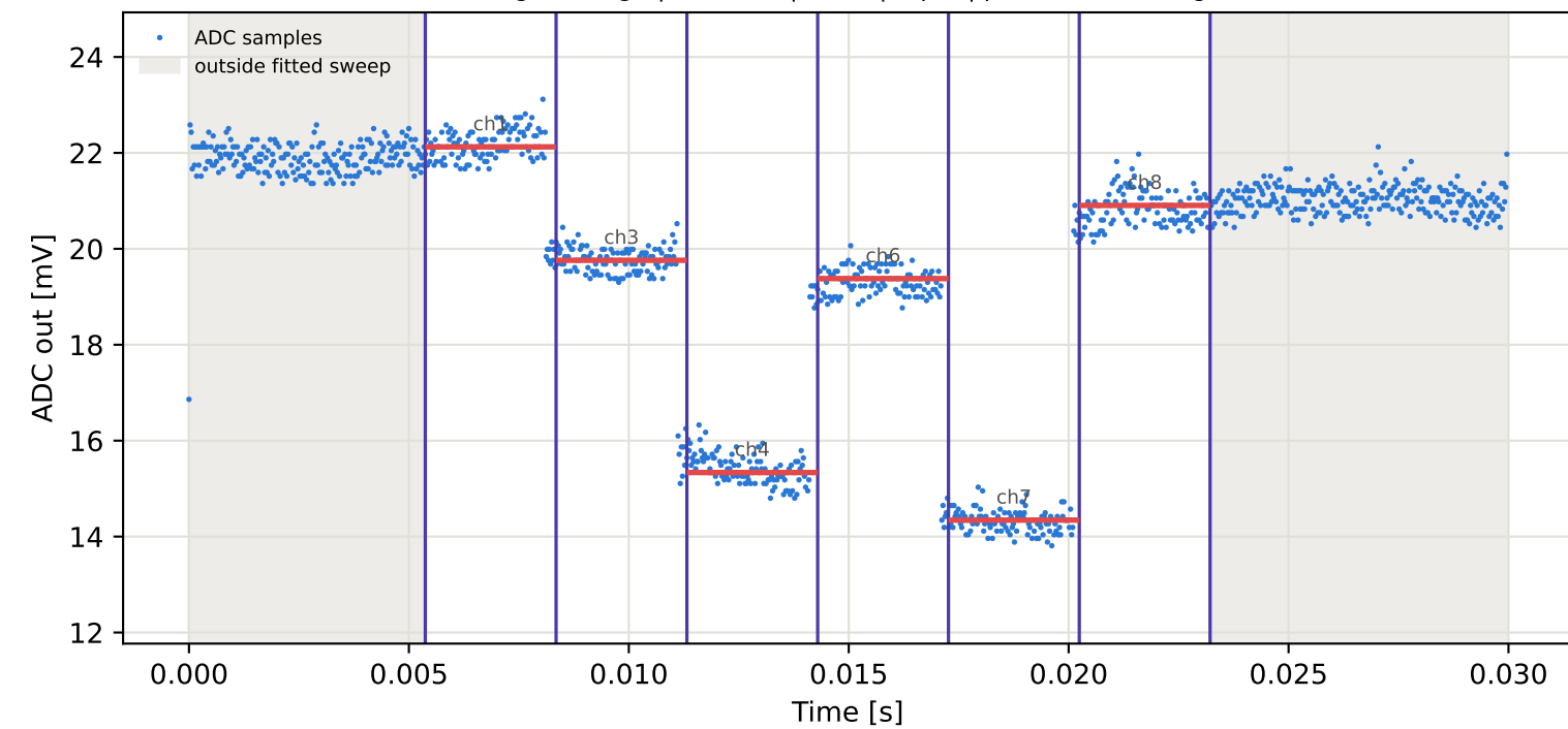
Tag3 &lt;- Tag6 | 795 MHz | run 0 | rep 1 | phase 59.88 deg
