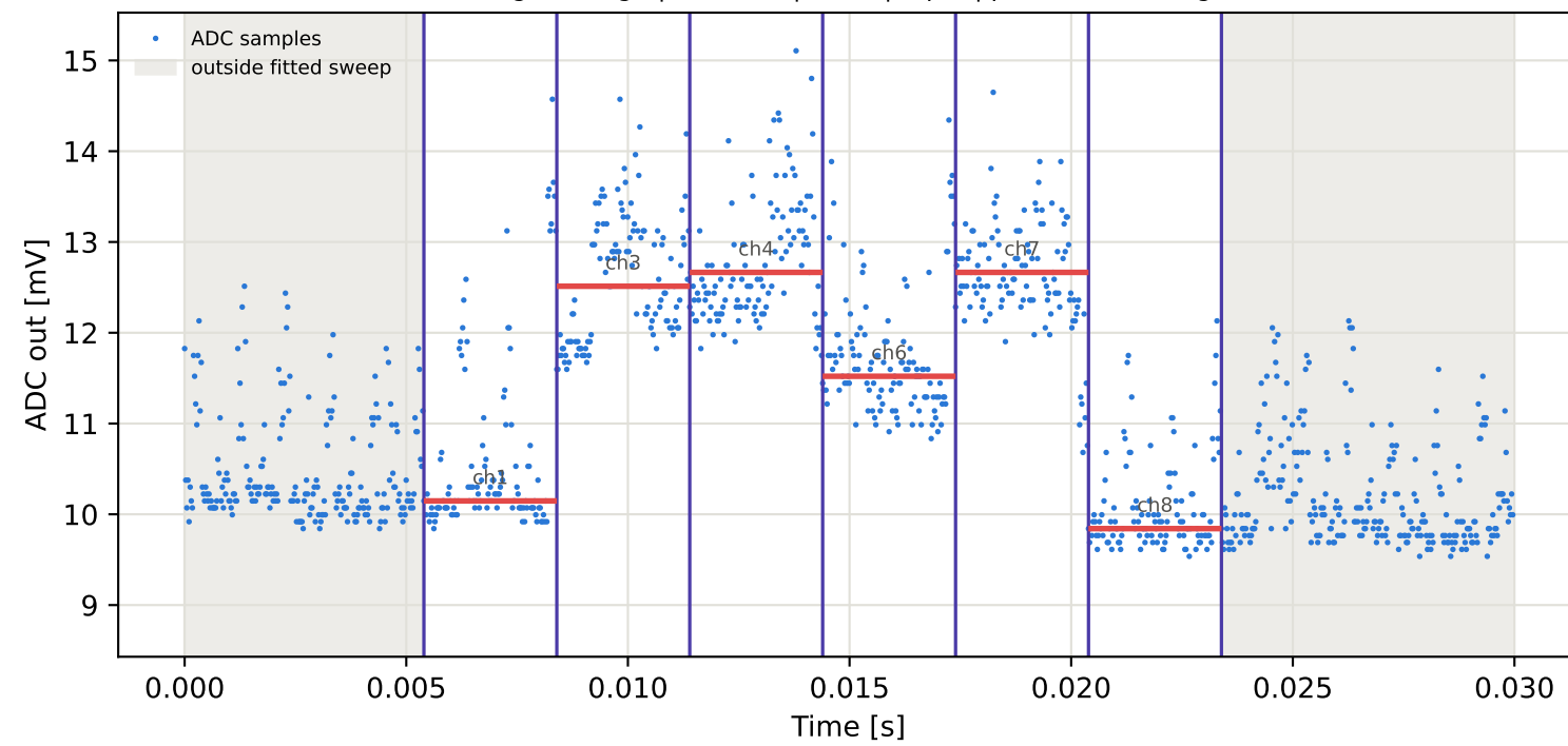
Tag3 &lt;- Tag10 | 855 MHz | run 0 | rep 1 | phase -73.16 deg
