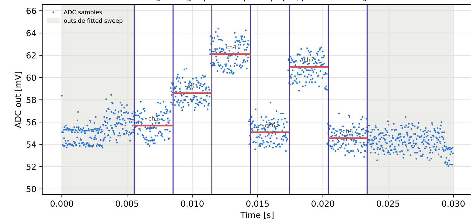
Tag2 &lt;- Tag15 | 985 MHz | run 0 | rep 1 | phase -70.49 deg
