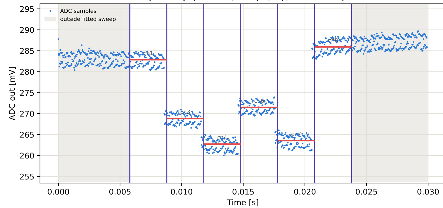
Tag10 &lt;- Tag4 | 875 MHz | run 0 | rep 1 | phase 96.75 deg
