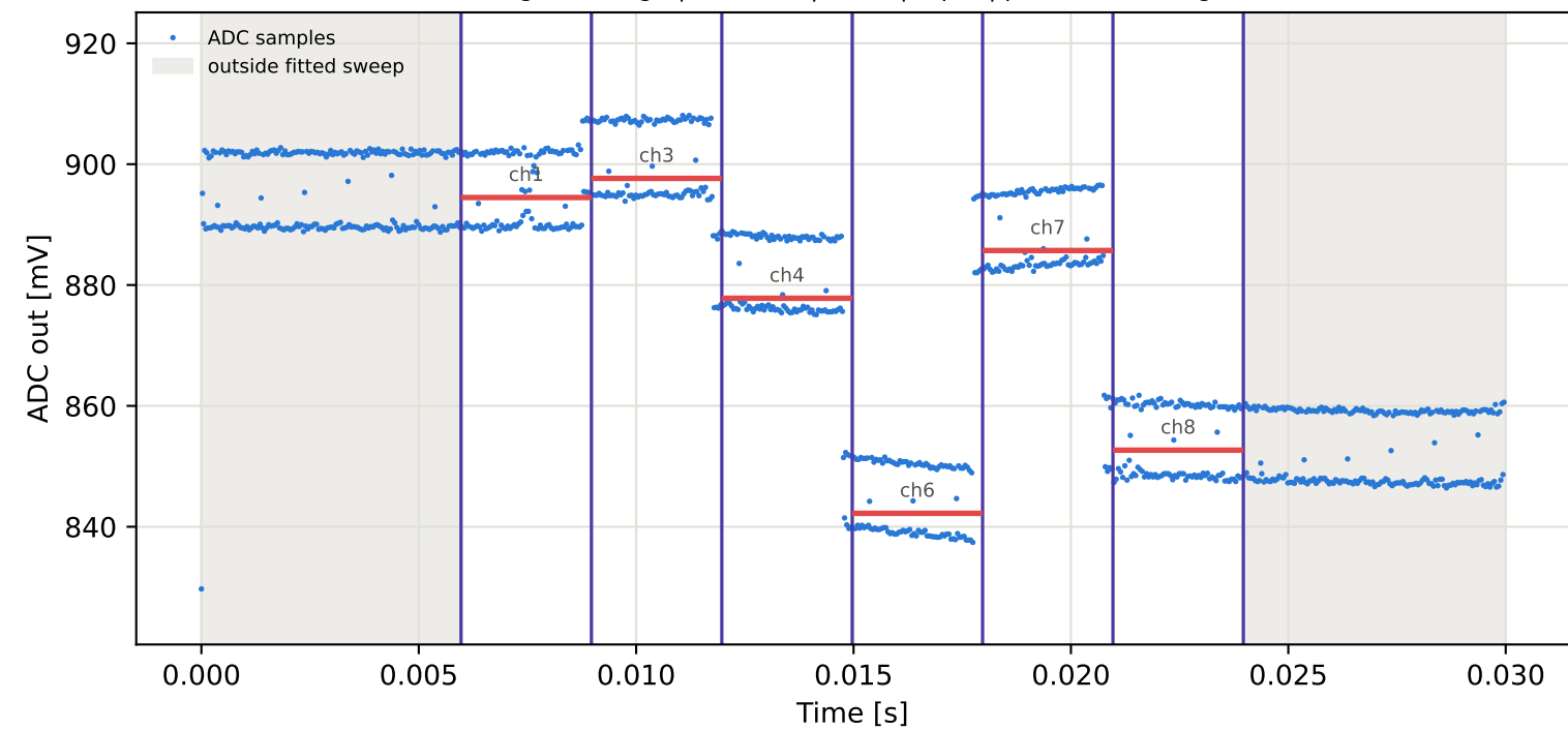
Tag2 &lt;- Tag10 | 875 MHz | run 0 | rep 1 | phase -145.01 deg
