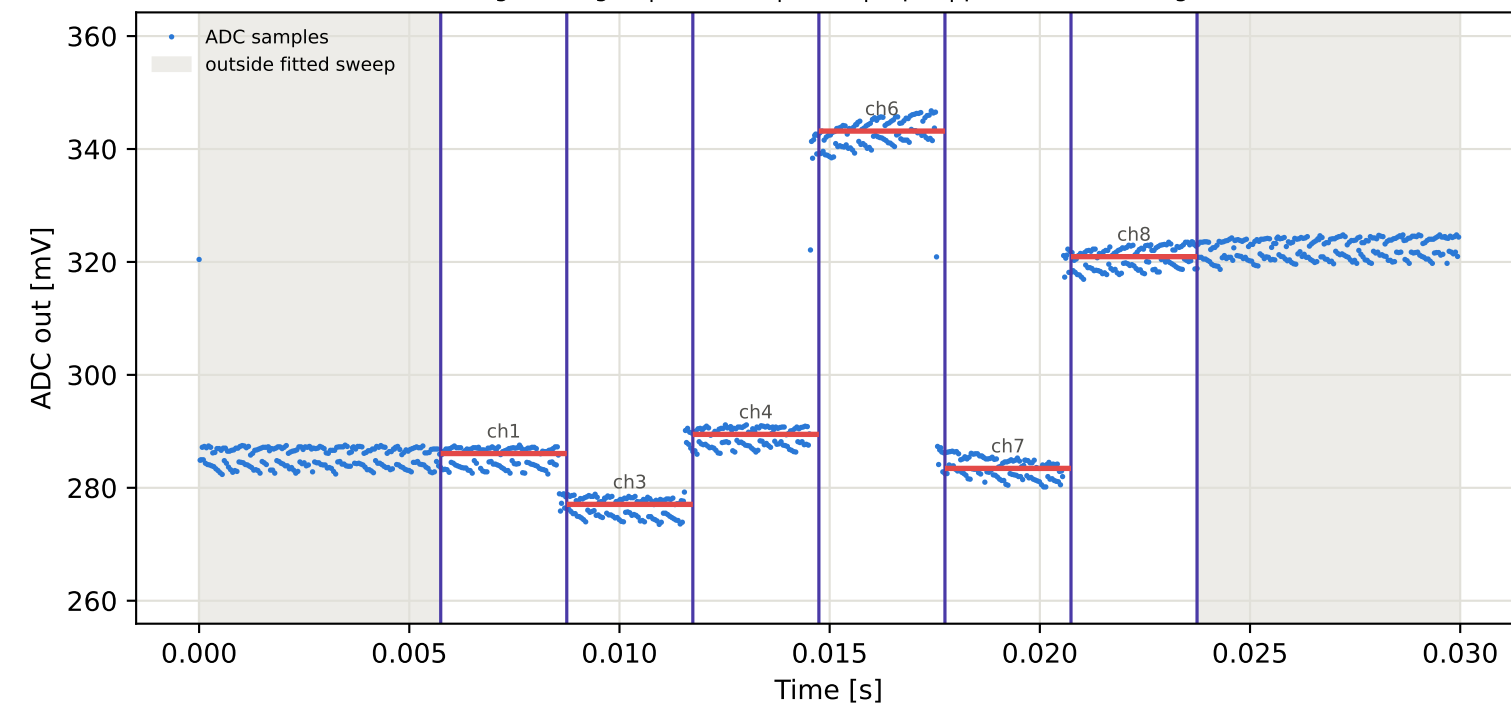
Tag4 &lt;- Tag2 | 915 MHz | run 0 | rep 1 | phase -2.88 deg
