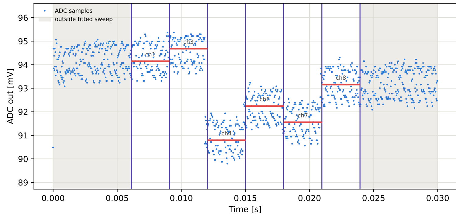
Tag7 &lt;- Tag10 | 785 MHz | run 0 | rep 1 | phase 76.47 deg
