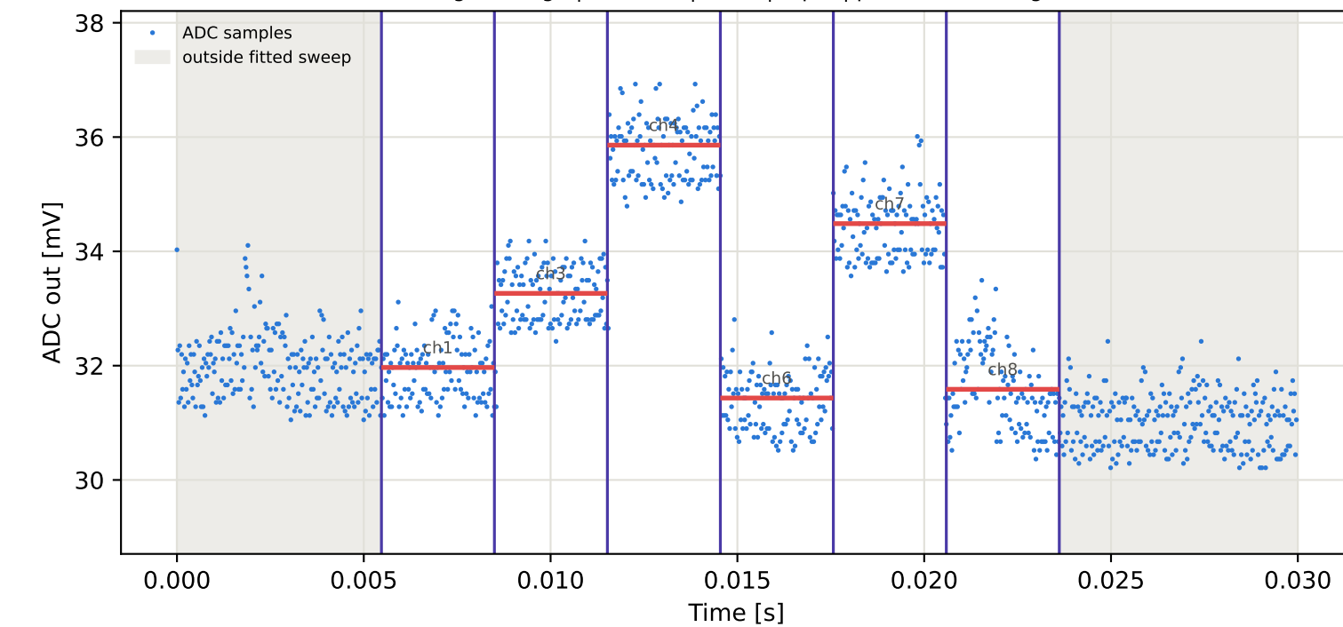
Tag2 &lt;- Tag15 | 995 MHz | run 0 | rep 1 | phase -93.66 deg
