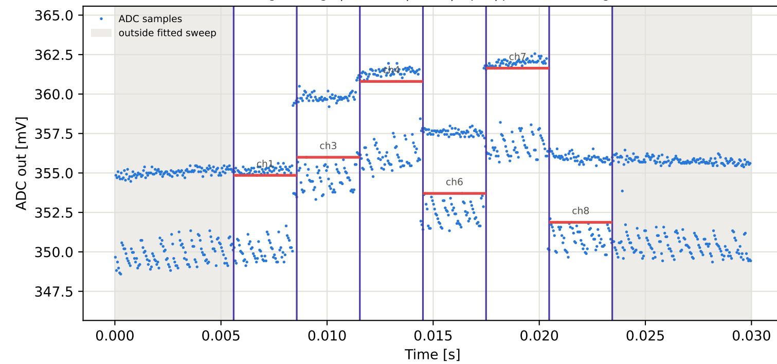
Tag5 &lt;- Tag8 | 825 MHz | run 0 | rep 1 | phase 75.10 deg
