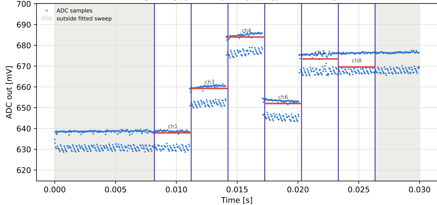
Tag3 &lt;- Tag15 | 875 MHz | run 0 | rep 1 | phase -2.67 deg
