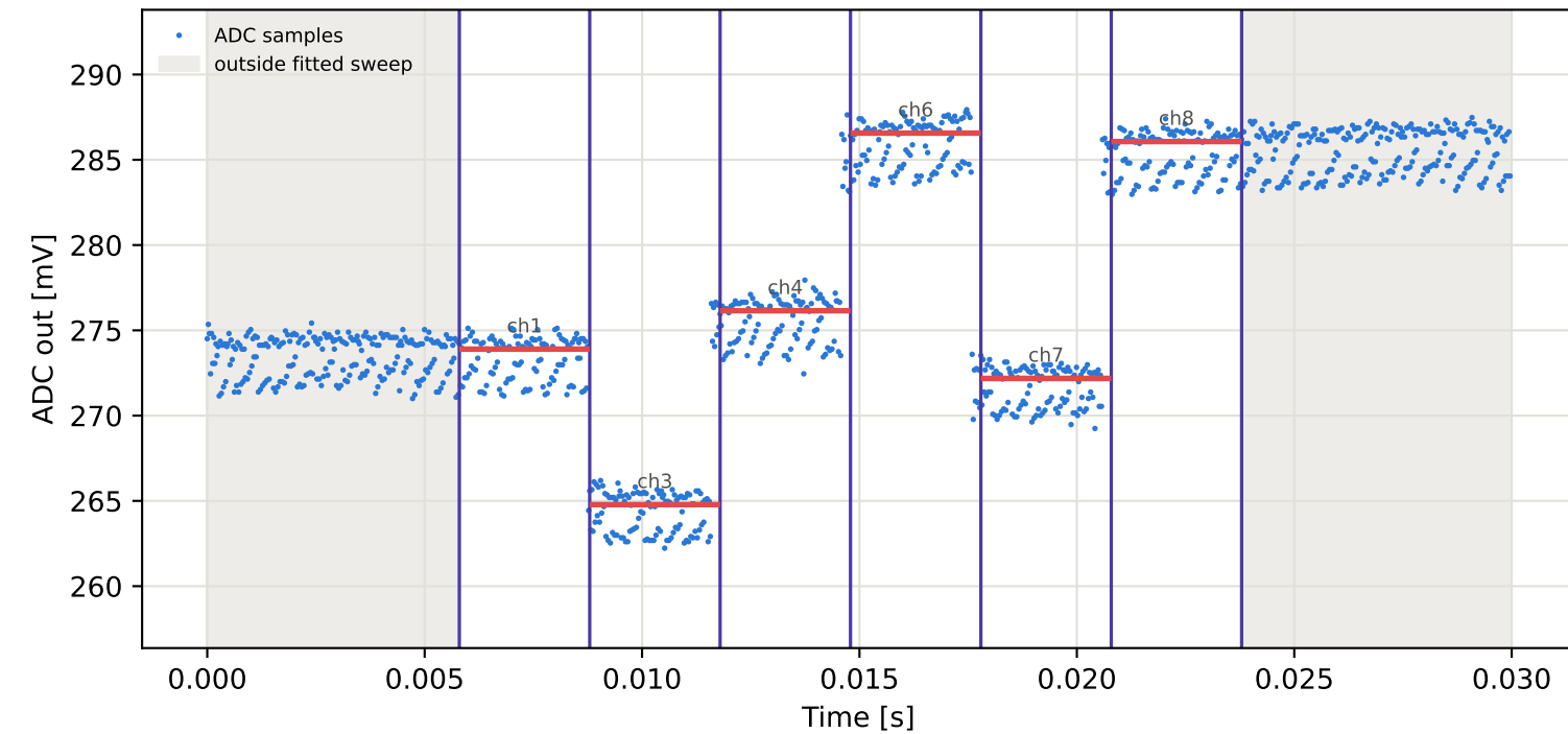
Tag15 &lt;- Tag1 | 845 MHz | run 0 | rep 1 | phase -94.43 deg
