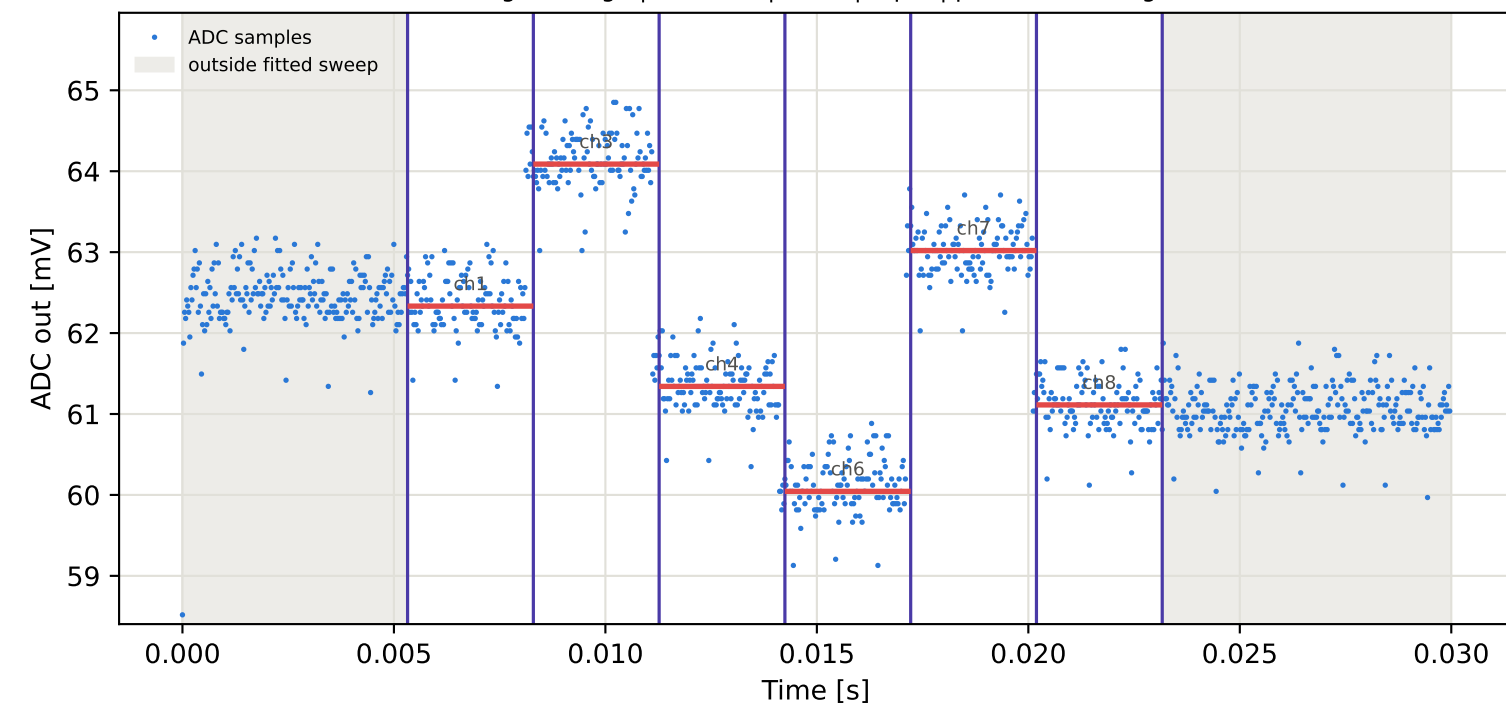
Tag4 &lt;- Tag9 | 785 MHz | run 0 | rep 1 | phase 29.01 deg
