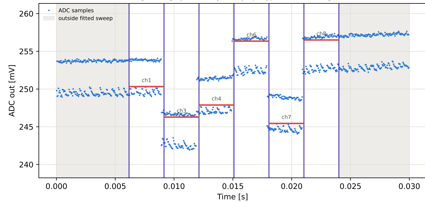
Tag8 &lt;- Tag10 | 835 MHz | run 0 | rep 1 | phase 83.48 deg
