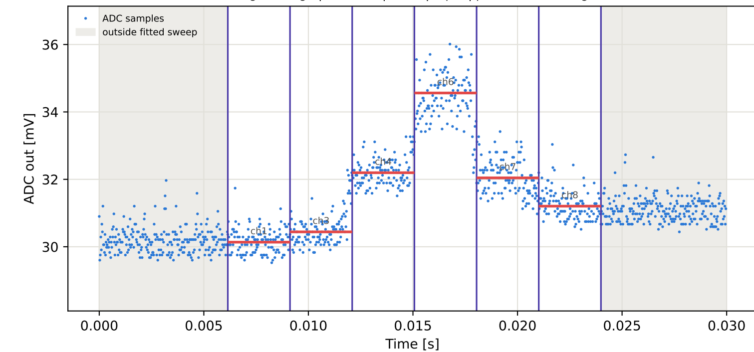
Tag2 &lt;- Tag15 | 945 MHz | run 0 | rep 1 | phase -140.56 deg
