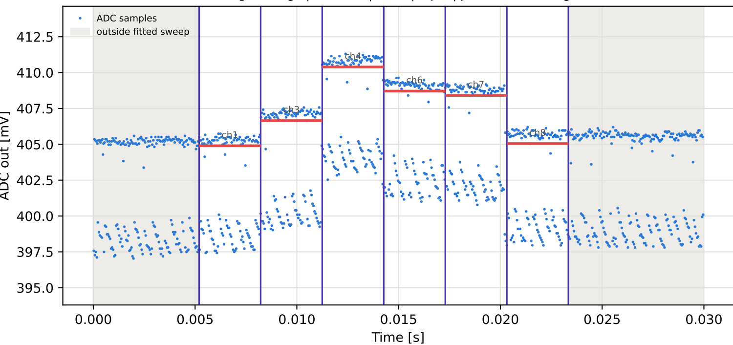
Tag4 &lt;- Tag9 | 955 MHz | run 0 | rep 1 | phase -114.79 deg
