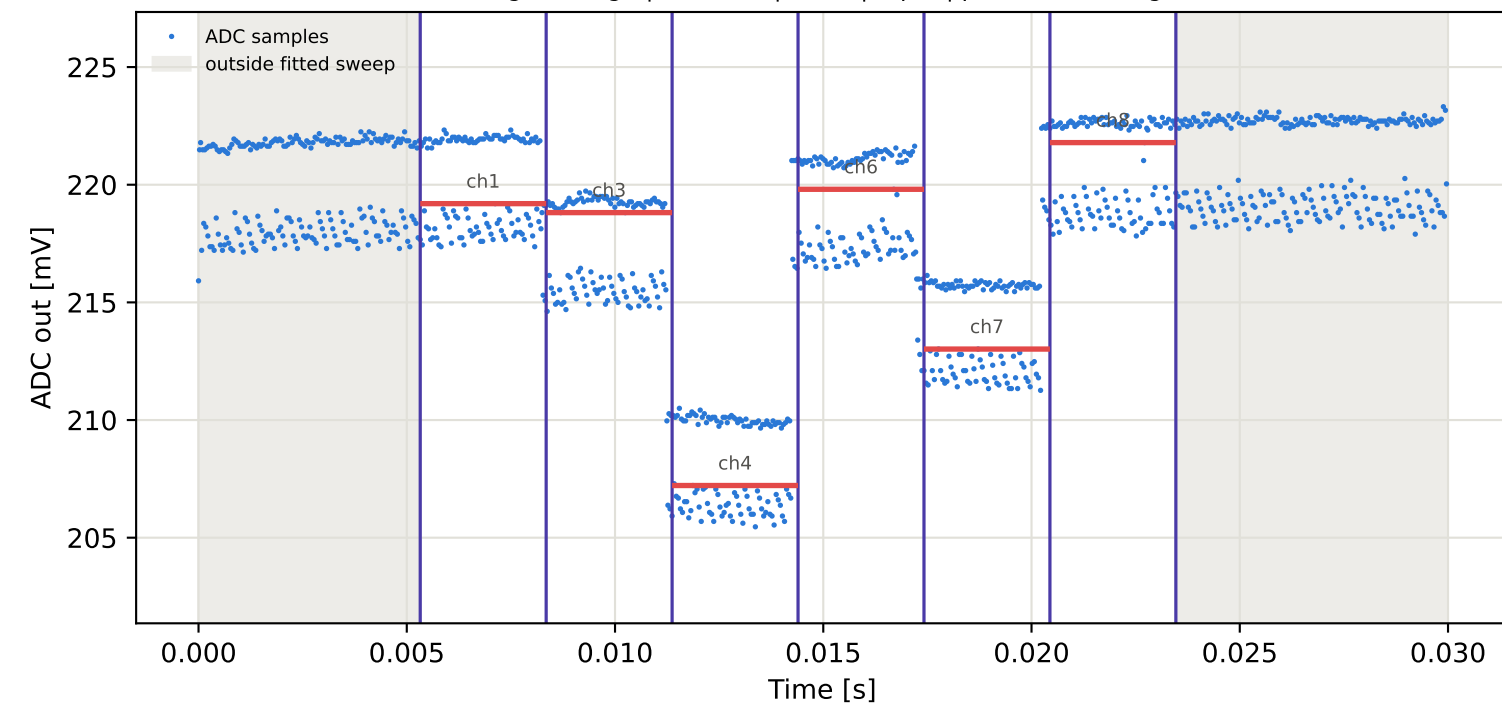
Tag3 &lt;- Tag6 | 995 MHz | run 0 | rep 1 | phase 65.56 deg
