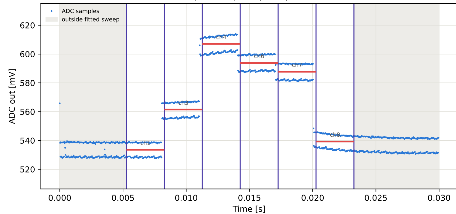
Tag5 &lt;- Tag2 | 935 MHz | run 0 | rep 1 | phase 138.23 deg
