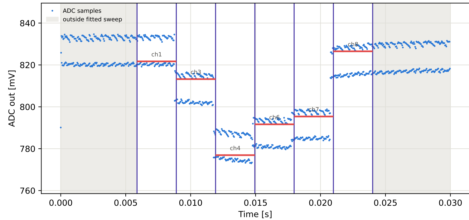
Tag2 &lt;- Tag10 | 925 MHz | run 0 | rep 1 | phase -63.94 deg
