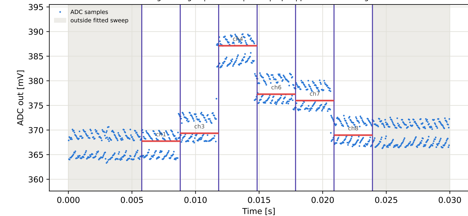
Tag7 &lt;- Tag10 | 985 MHz | run 0 | rep 1 | phase -120.24 deg
