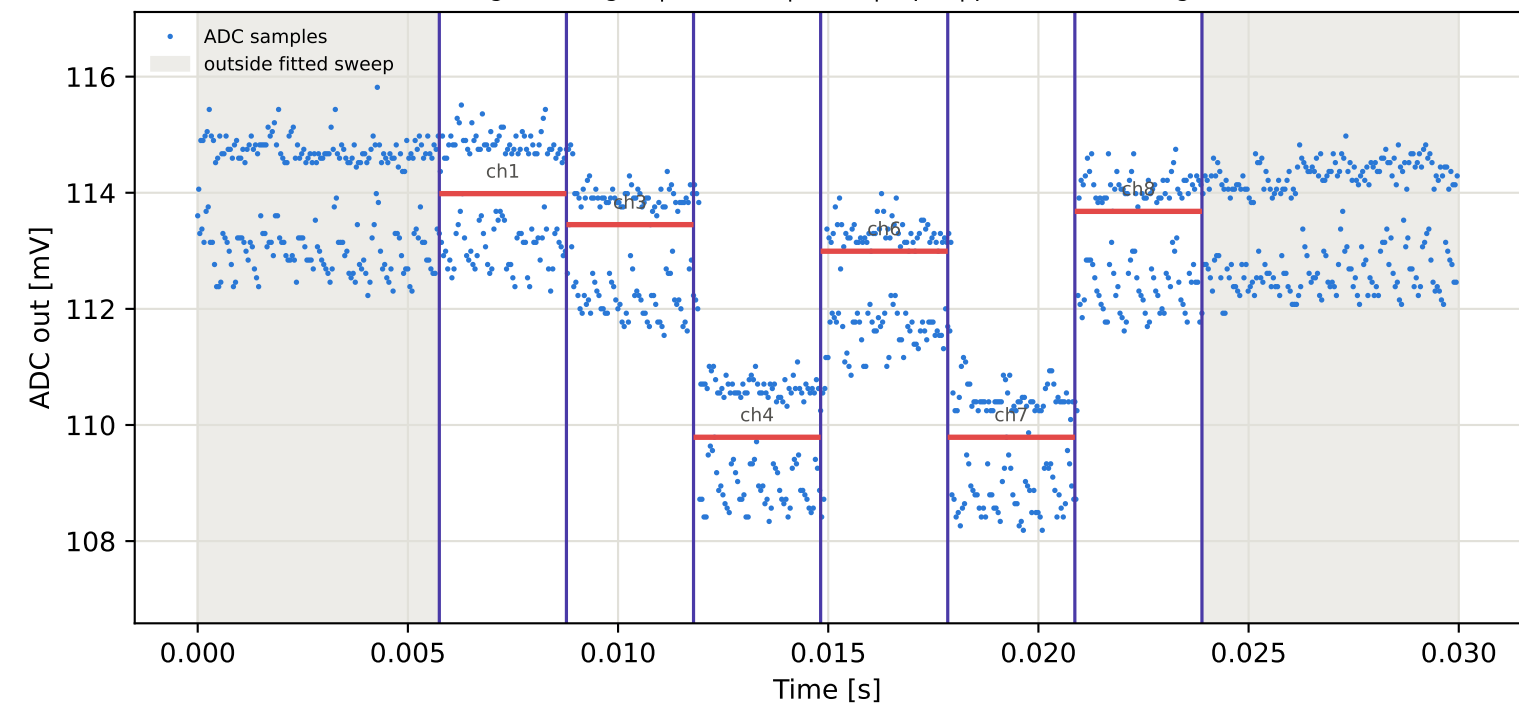
Tag10 &lt;- Tag3 | 785 MHz | run 0 | rep 1 | phase -152.53 deg
