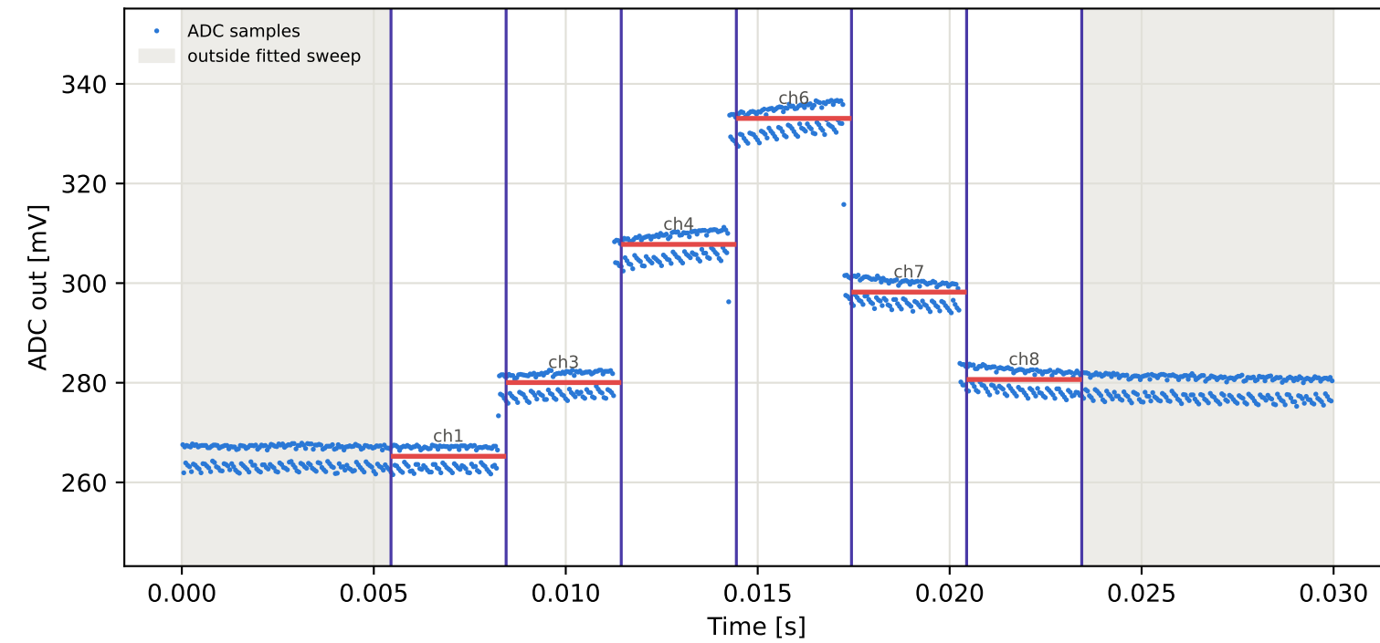
Tag3 &lt;- Tag8 | 905 MHz | run 0 | rep 1 | phase -158.87 deg
