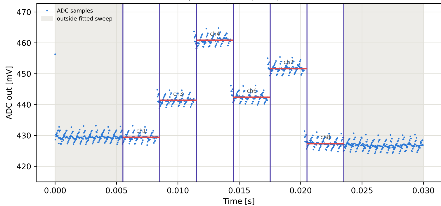
Tag5 &lt;- Tag2 | 955 MHz | run 0 | rep 1 | phase -60.11 deg
