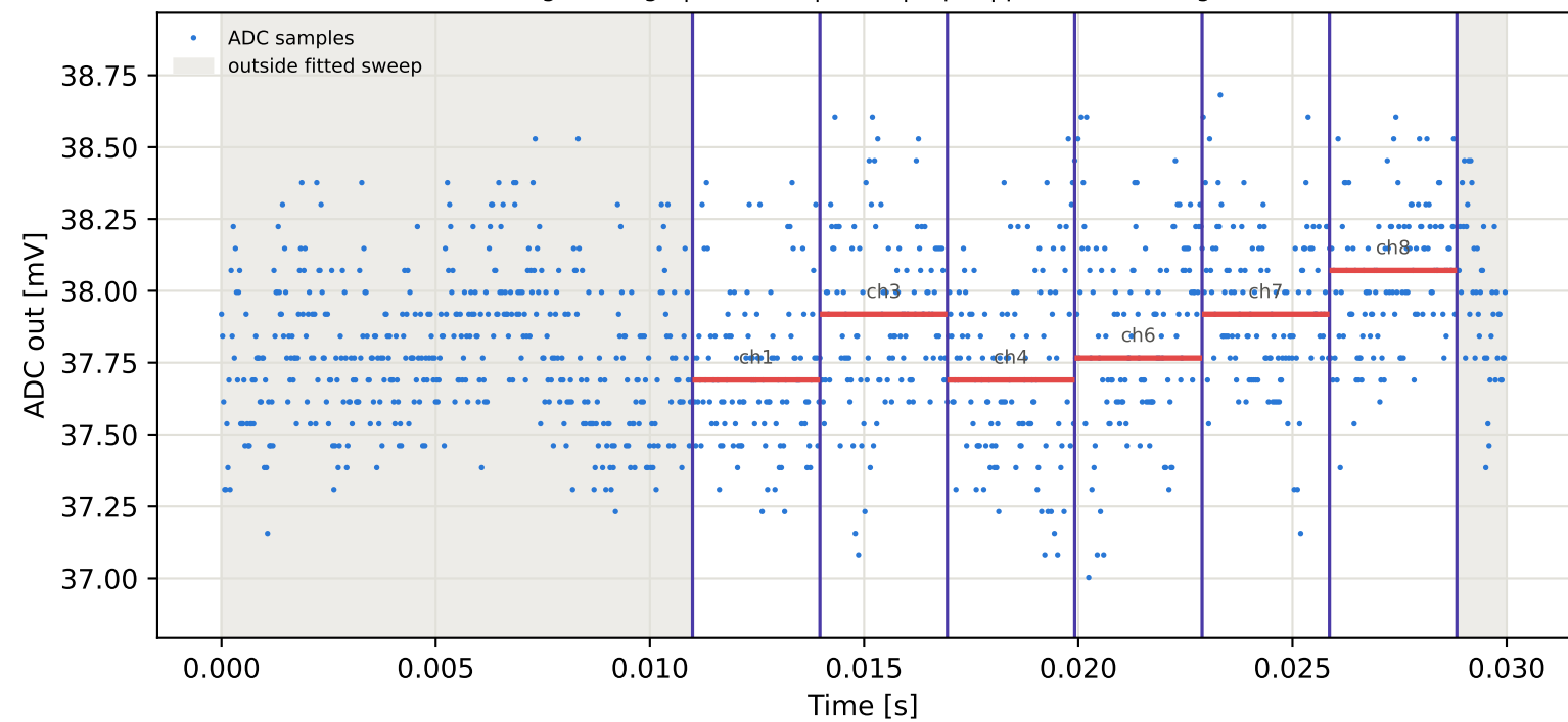
Tag1 &lt;- Tag4 | 785 MHz | run 0 | rep 1 | phase -110.66 deg
