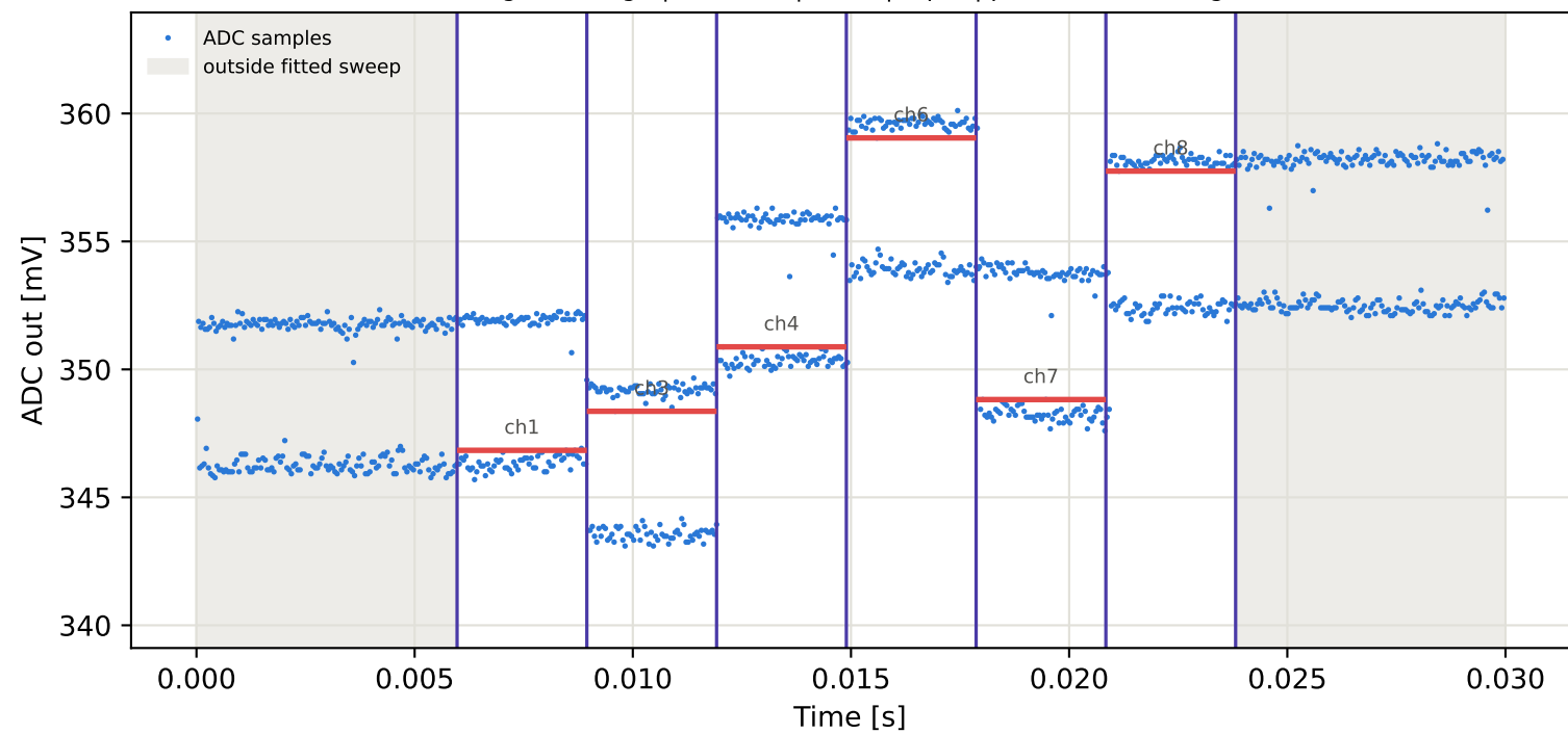
Tag2 &lt;- Tag10 | 845 MHz | run 0 | rep 1 | phase 123.35 deg
