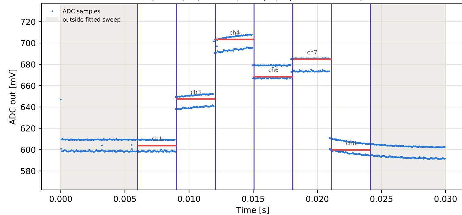
Tag4 &lt;- Tag2 | 925 MHz | run 0 | rep 1 | phase 152.57 deg
