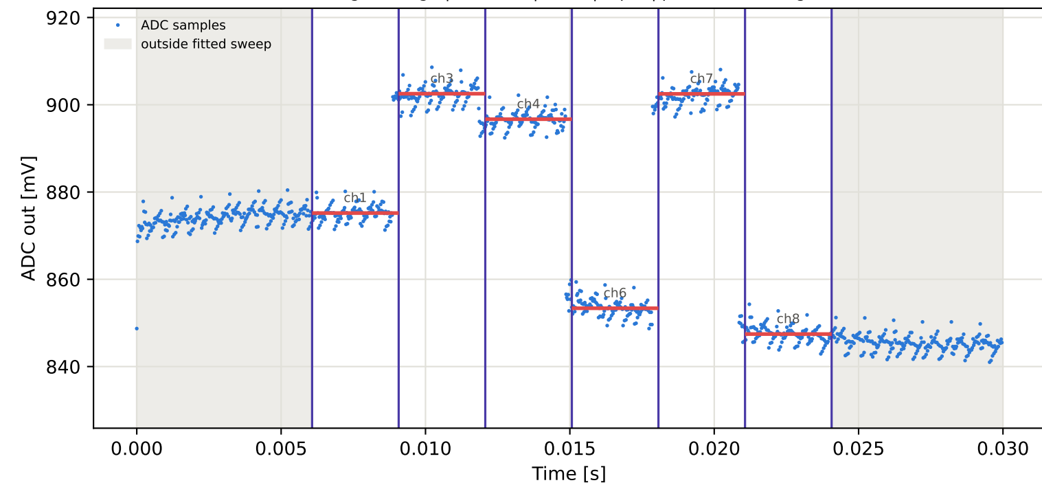
Tag6 &lt;- Tag9 | 875 MHz | run 0 | rep 1 | phase -35.67 deg
