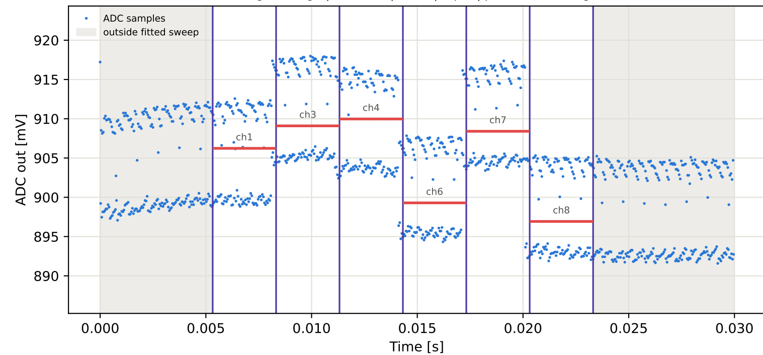
Tag9 &lt;- Tag10 | 865 MHz | run 0 | rep 1 | phase 3.73 deg
