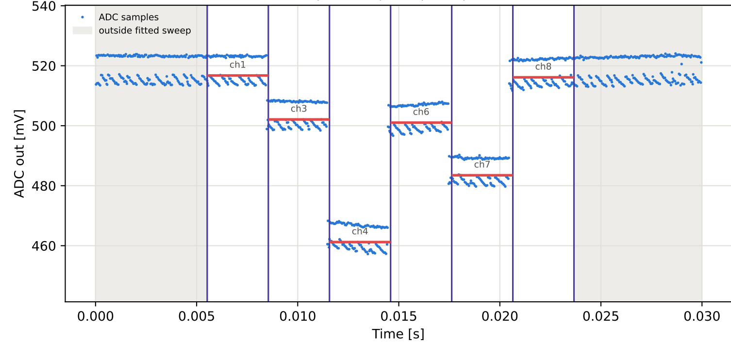
Tag8 &lt;- Tag16 | 975 MHz | run 0 | rep 1 | phase 77.59 deg
