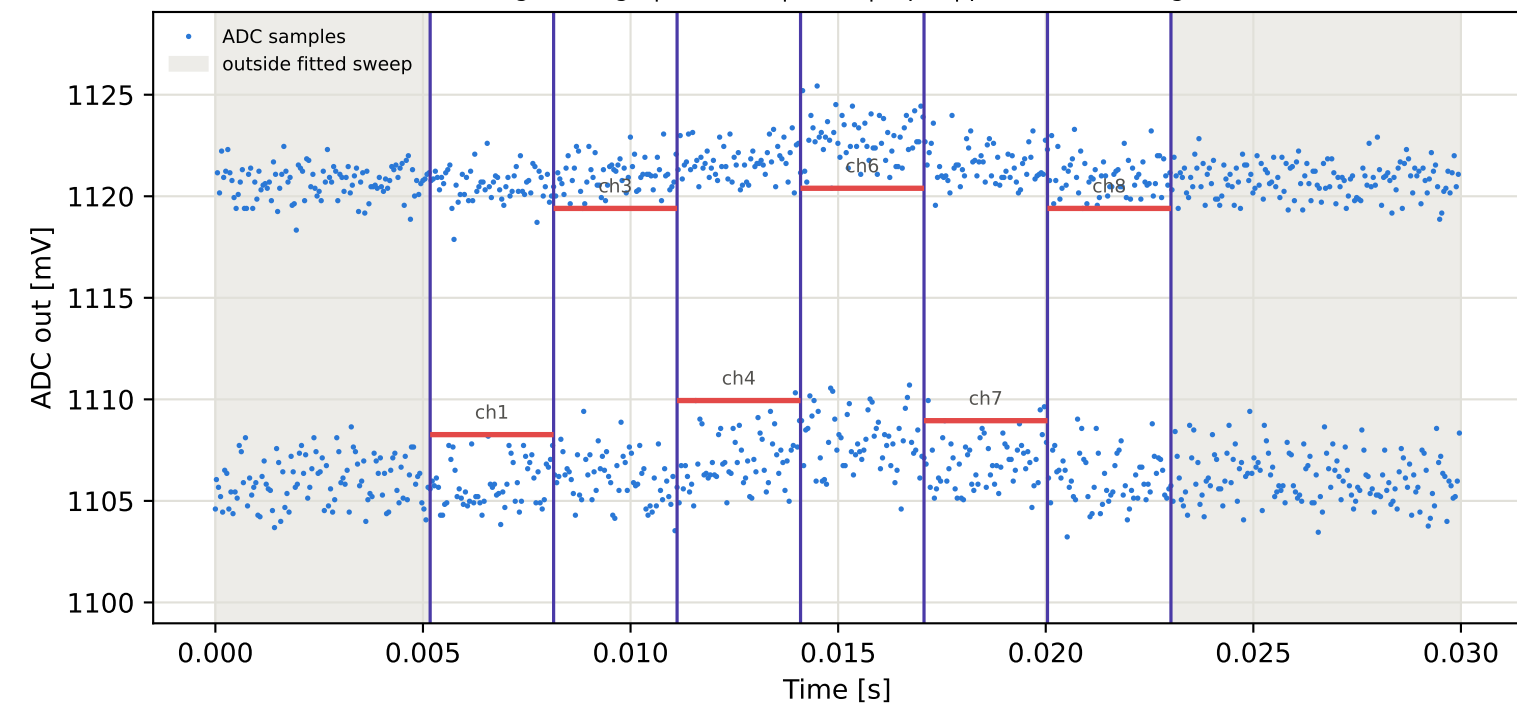
Tag8 &lt;- Tag4 | 885 MHz | run 0 | rep 1 | phase -131.35 deg
