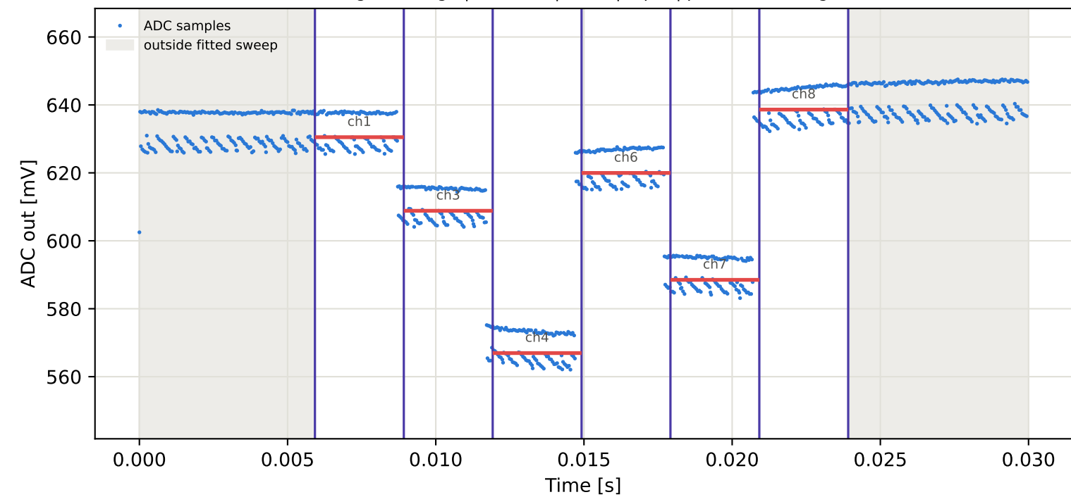
Tag16 &lt;- Tag1 | 955 MHz | run 0 | rep 1 | phase 145.29 deg
