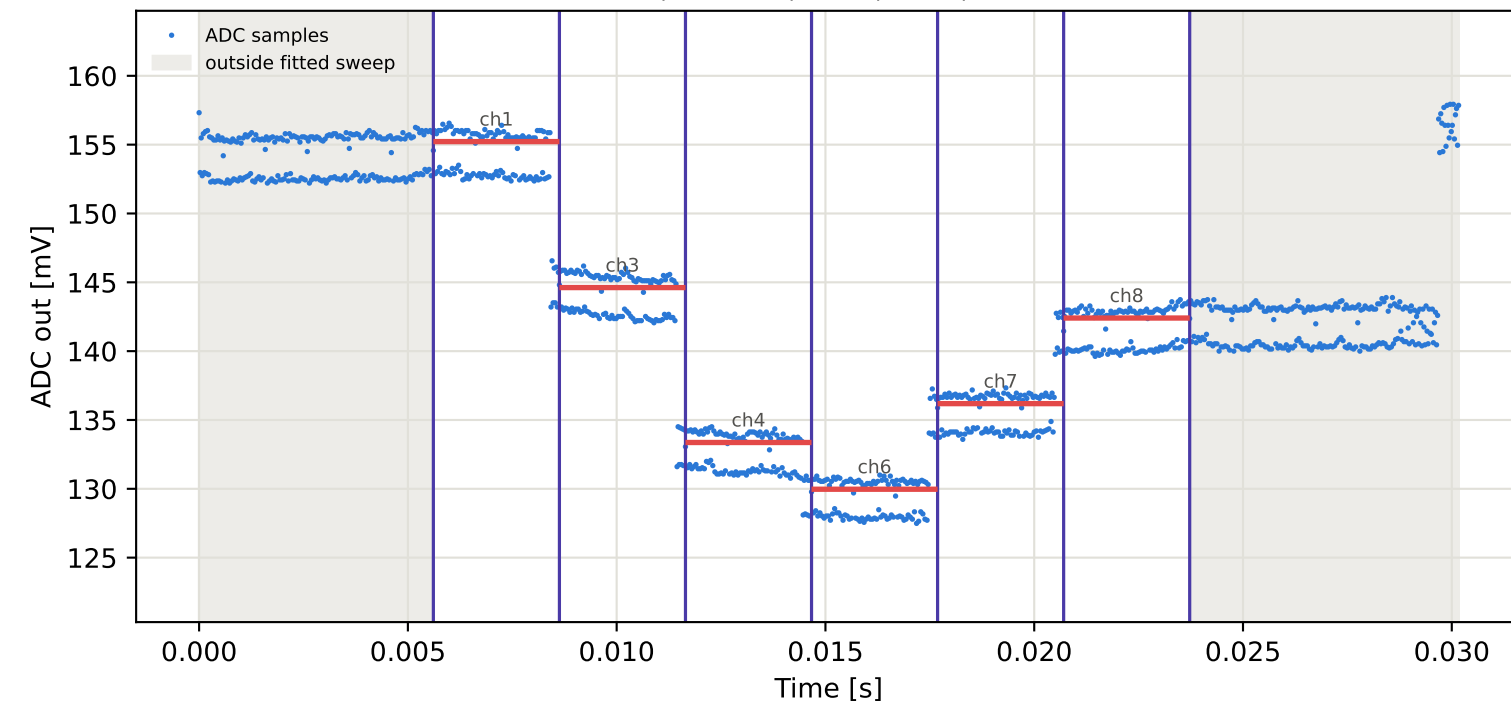
Tag10 &lt;- Tag4 | 865 MHz | run 0 | rep 1 | phase 56.77 deg
