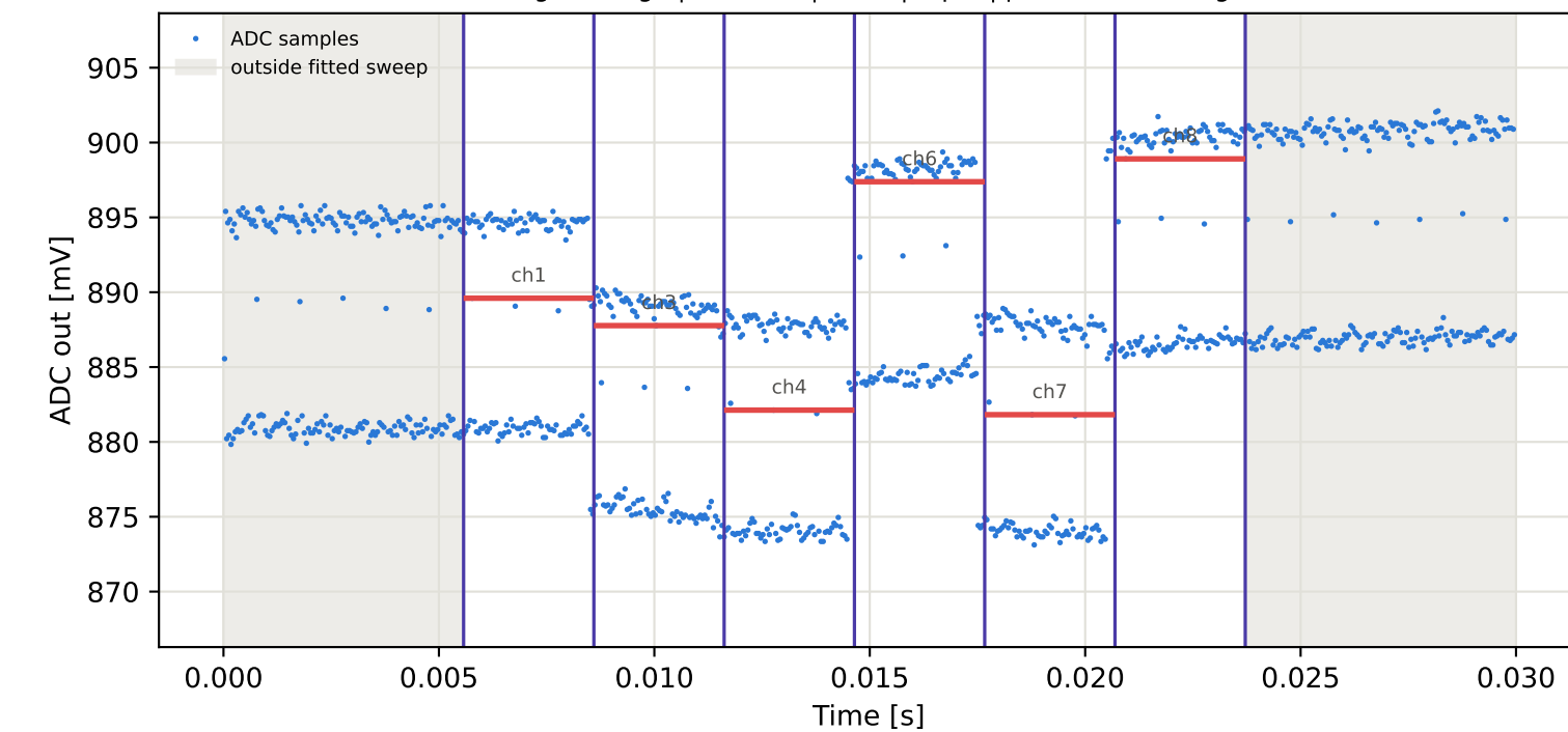
Tag4 &lt;- Tag9 | 905 MHz | run 0 | rep 1 | phase 137.79 deg
