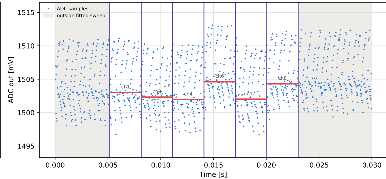
Tag5 &lt;- Tag4 | 895 MHz | run 0 | rep 1 | phase 110.22 deg
