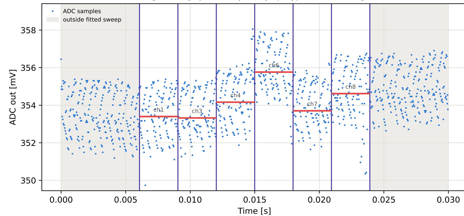
Tag16 &lt;- Tag4 | 845 MHz | run 0 | rep 1 | phase 62.86 deg
