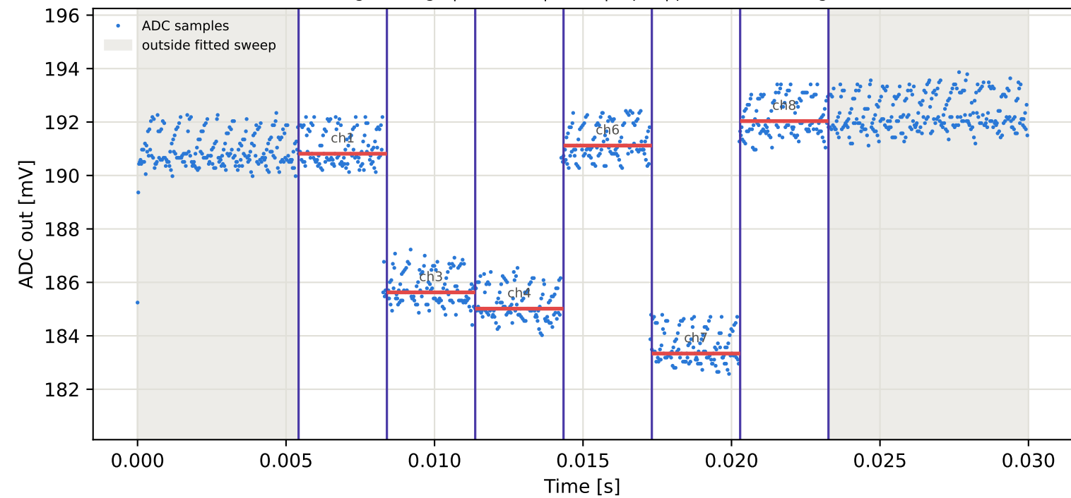
Tag8 &lt;- Tag10 | 805 MHz | run 0 | rep 1 | phase -52.64 deg
