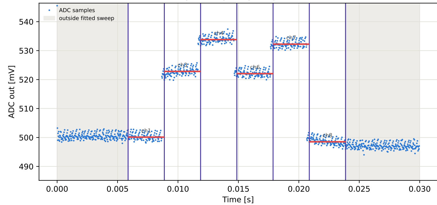
Tag1 &lt;- Tag4 | 875 MHz | run 0 | rep 1 | phase -89.16 deg
