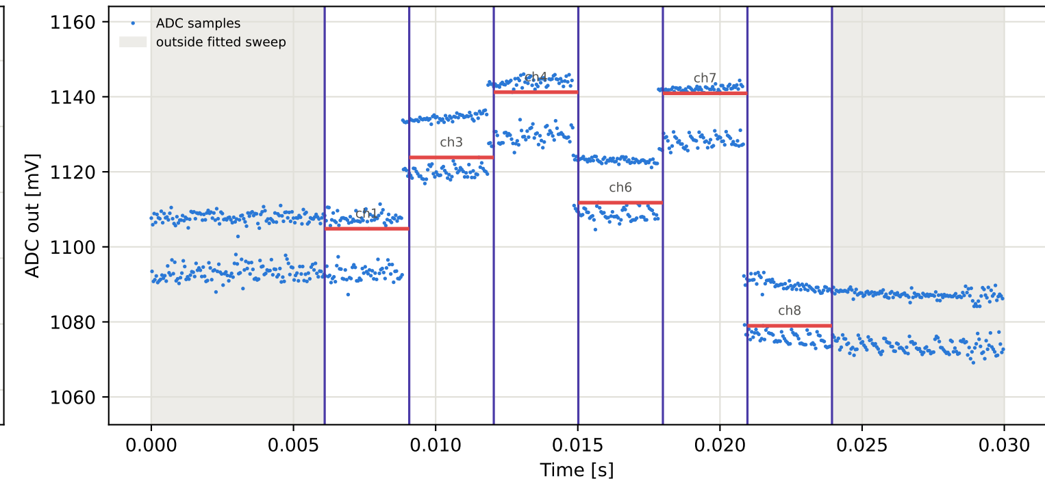
Tag8 &lt;- Tag7 | 885 MHz | run 0 | rep 1 | phase -56.96 deg
