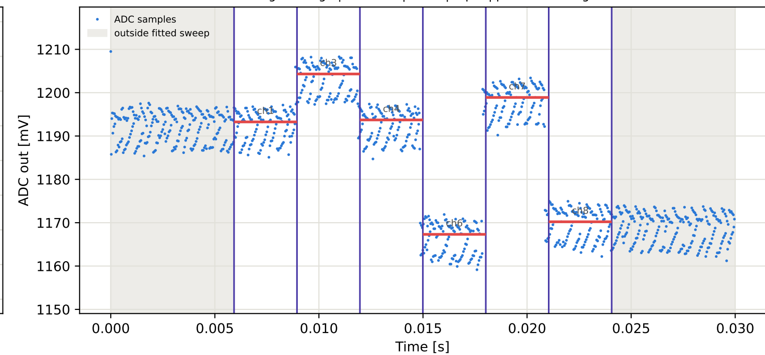
Tag5 &lt;- Tag9 | 875 MHz | run 0 | rep 1 | phase -172.82 deg
