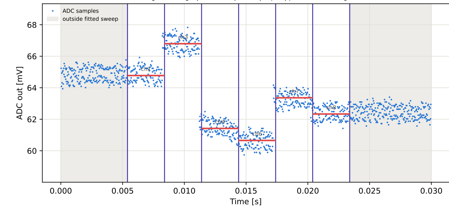
Tag16 &lt;- Tag6 | 785 MHz | run 0 | rep 1 | phase 46.17 deg
