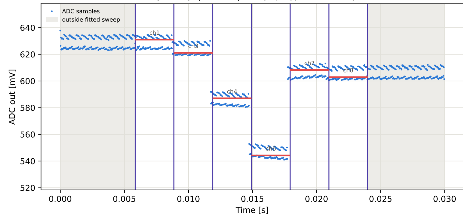
Tag5 &lt;- Tag1 | 945 MHz | run 0 | rep 1 | phase 158.09 deg
