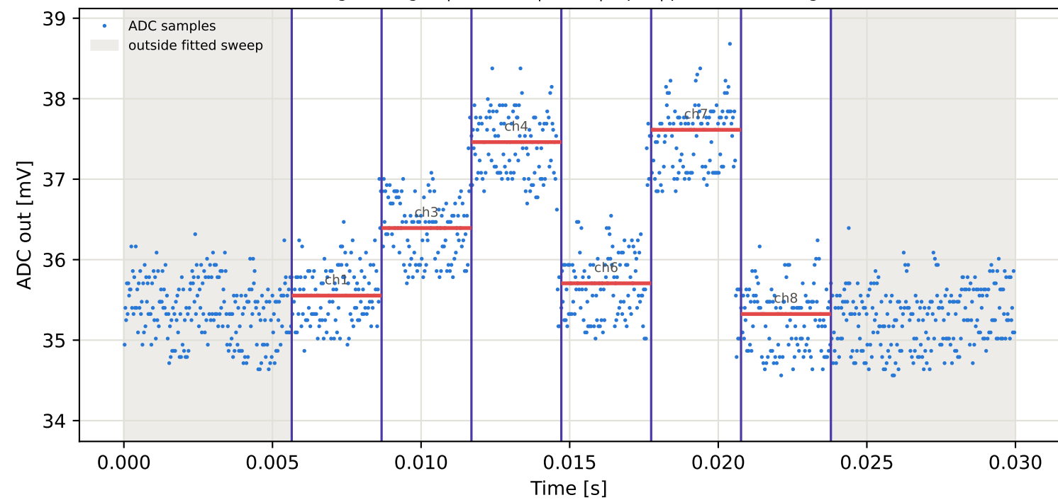
Tag1 &lt;- Tag2 | 785 MHz | run 0 | rep 1 | phase 71.25 deg
