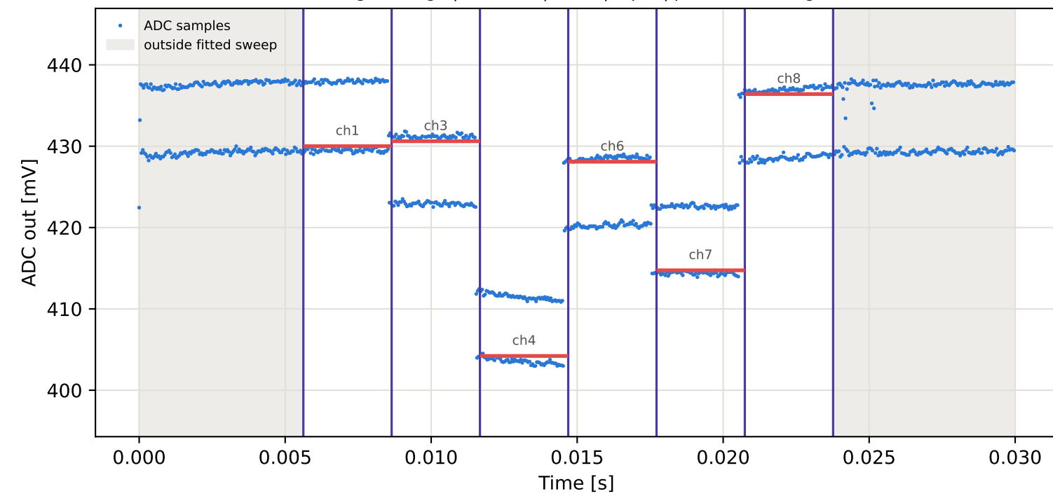
Tag8 &lt;- Tag1 | 975 MHz | run 0 | rep 1 | phase -7.22 deg
