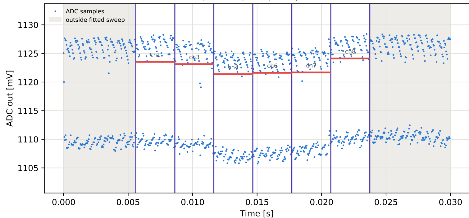
Tag7 &lt;- Tag4 | 935 MHz | run 0 | rep 1 | phase 113.54 deg
