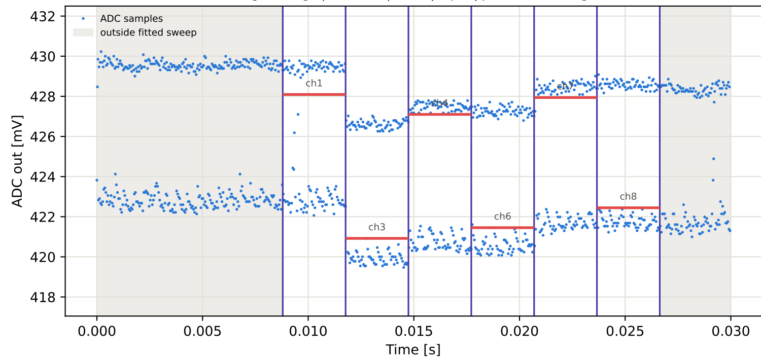
Tag4 &lt;- Tag15 | 835 MHz | run 0 | rep 1 | phase -170.67 deg
