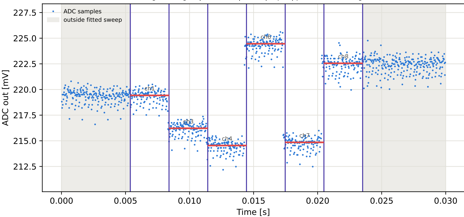
Tag3 &lt;- Tag16 | 995 MHz | run 0 | rep 1 | phase 7.27 deg
