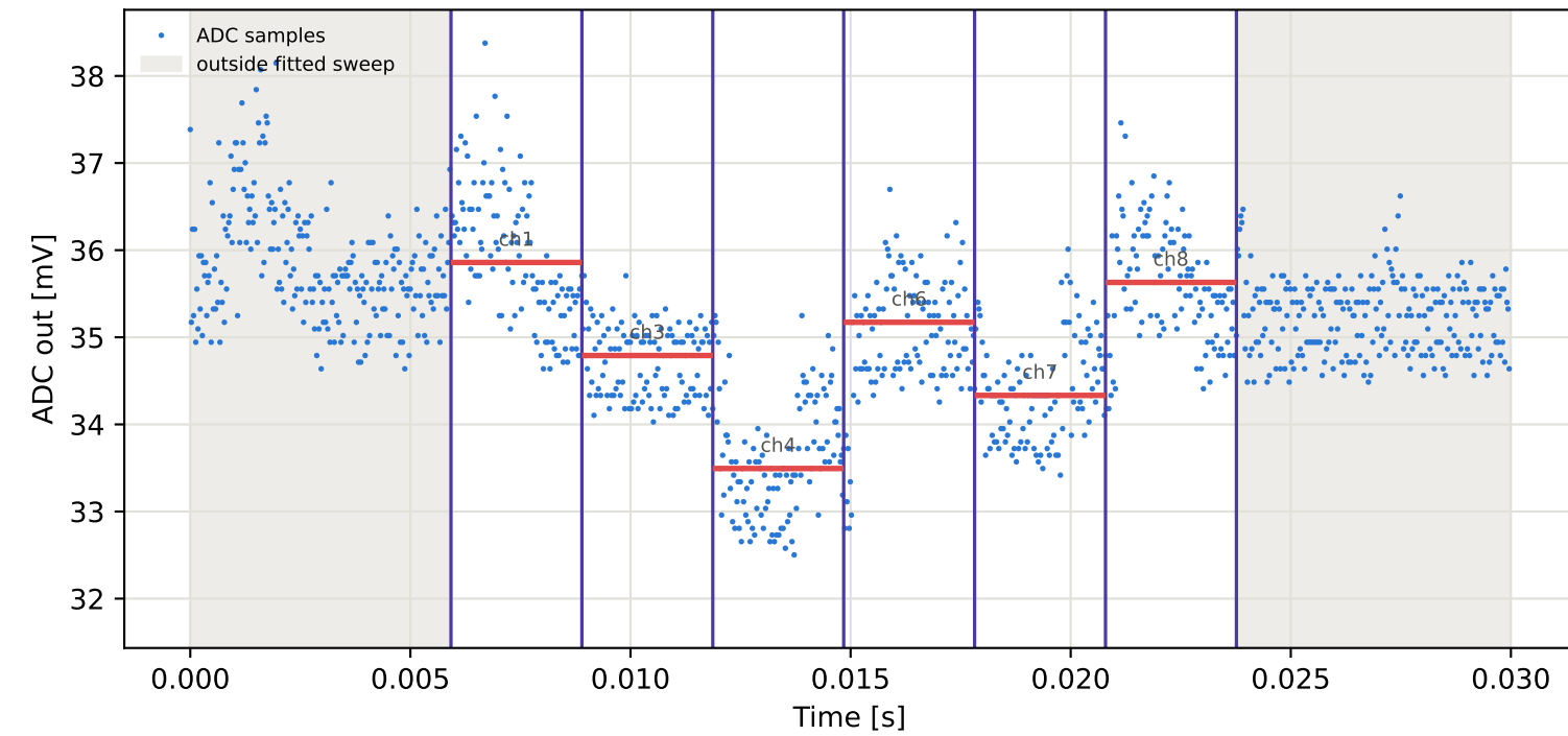
Tag2 &lt;- Tag7 | 995 MHz | run 0 | rep 1 | phase 3.49 deg
