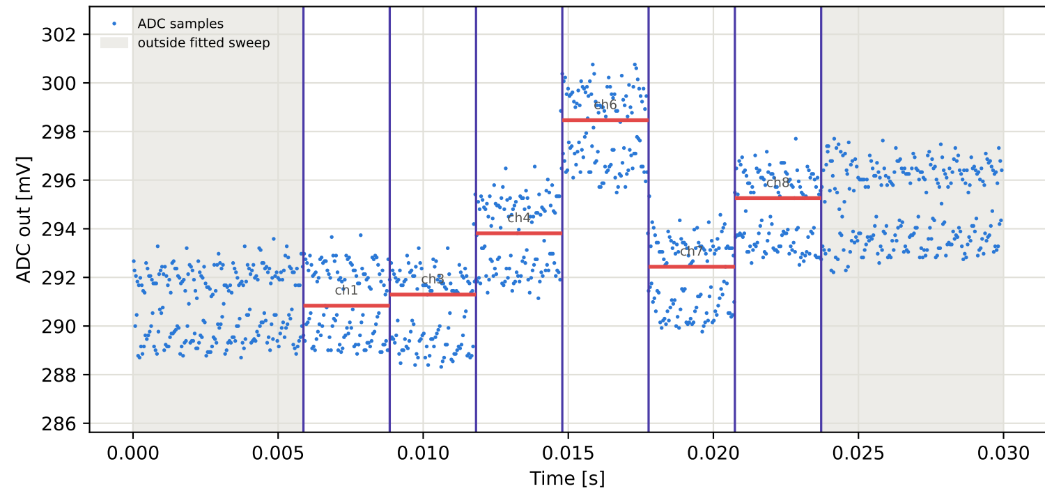
Tag6 &lt;- Tag4 | 835 MHz | run 0 | rep 1 | phase -158.71 deg
