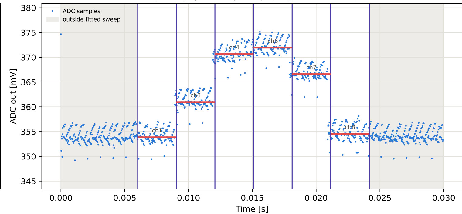
Tag7 &lt;- Tag1 | 915 MHz | run 0 | rep 1 | phase 81.50 deg
