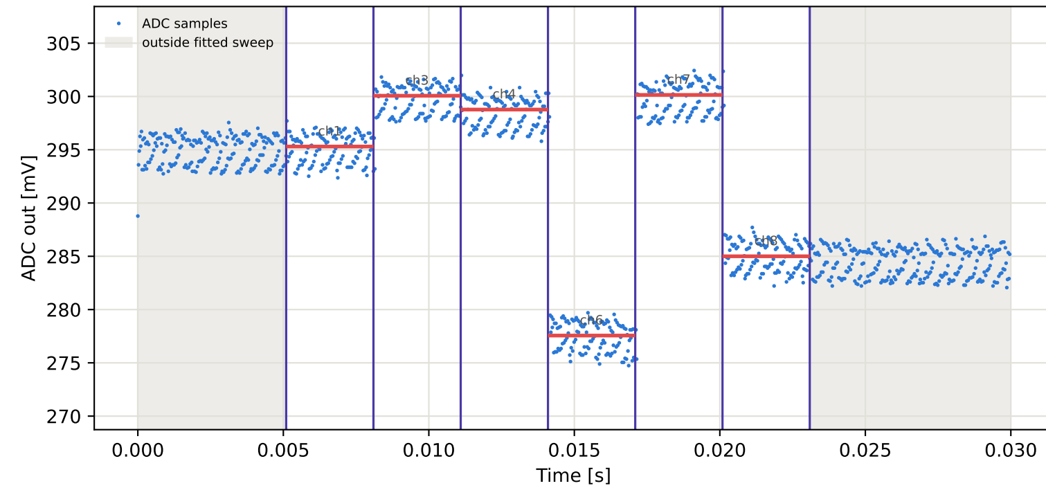
Tag7 &lt;- Tag10 | 945 MHz | run 0 | rep 1 | phase 88.03 deg
