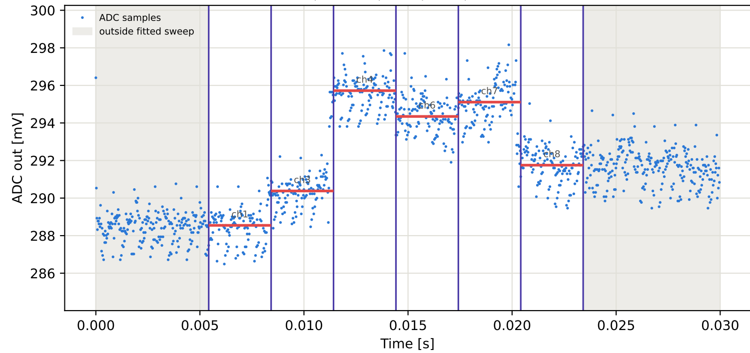
Tag6 &lt;- Tag5 | 835 MHz | run 0 | rep 1 | phase -110.85 deg
