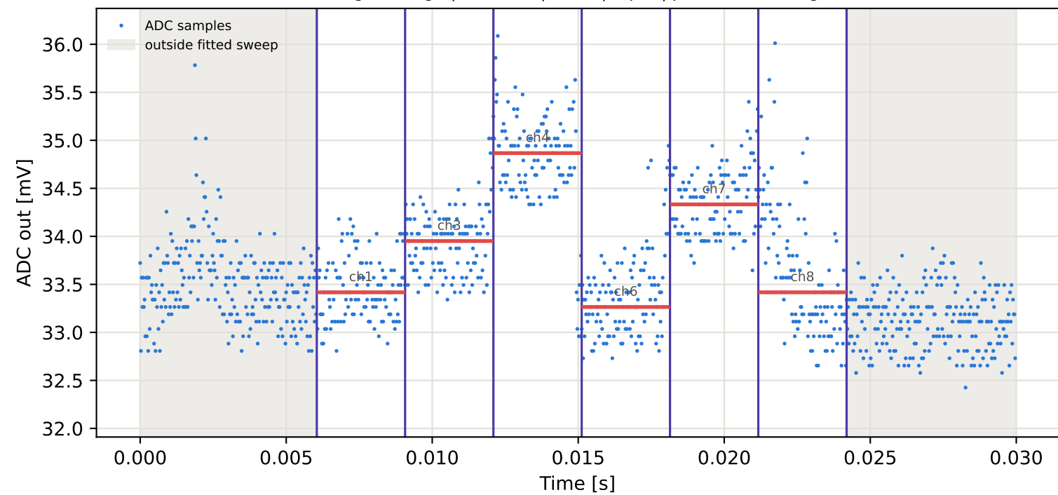
Tag3 &lt;- Tag10 | 995 MHz | run 0 | rep 1 | phase 142.82 deg
