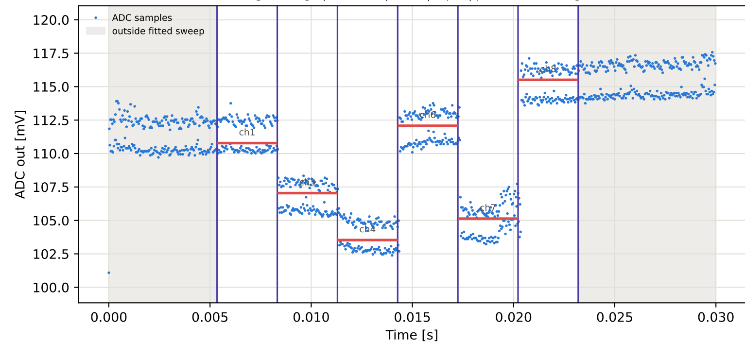
Tag3 &lt;- Tag10 | 915 MHz | run 0 | rep 1 | phase 0.34 deg
