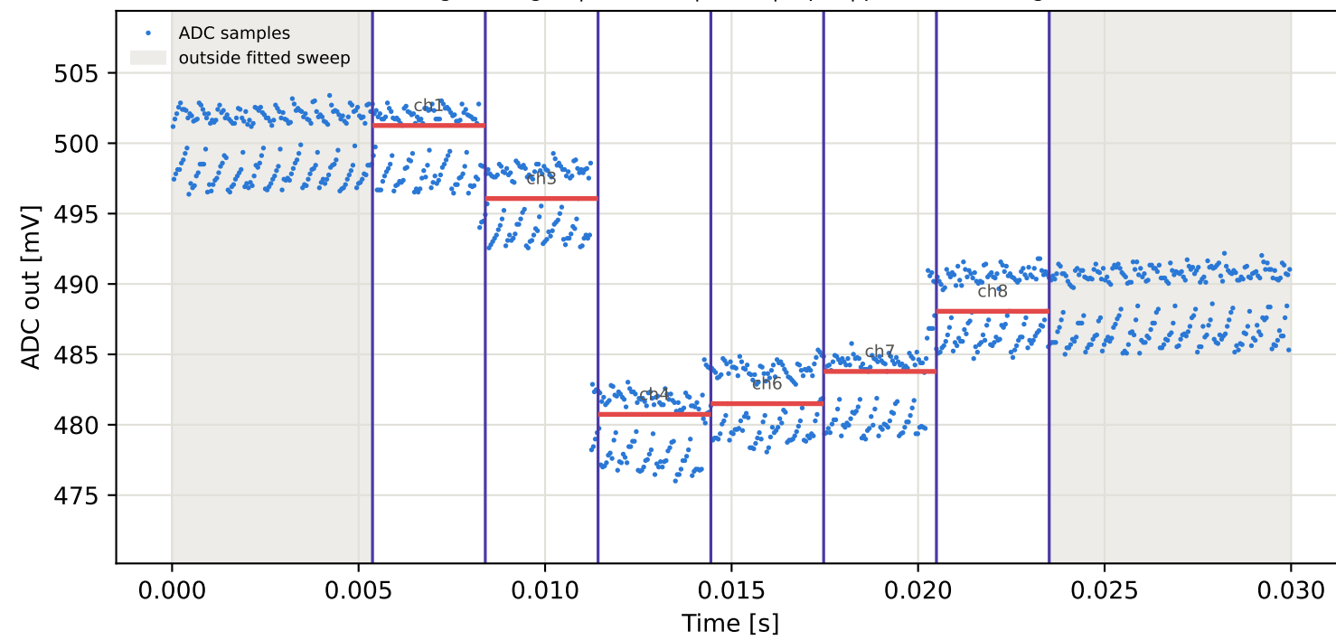
Tag6 &lt;- Tag2 | 845 MHz | run 0 | rep 1 | phase -120.18 deg
