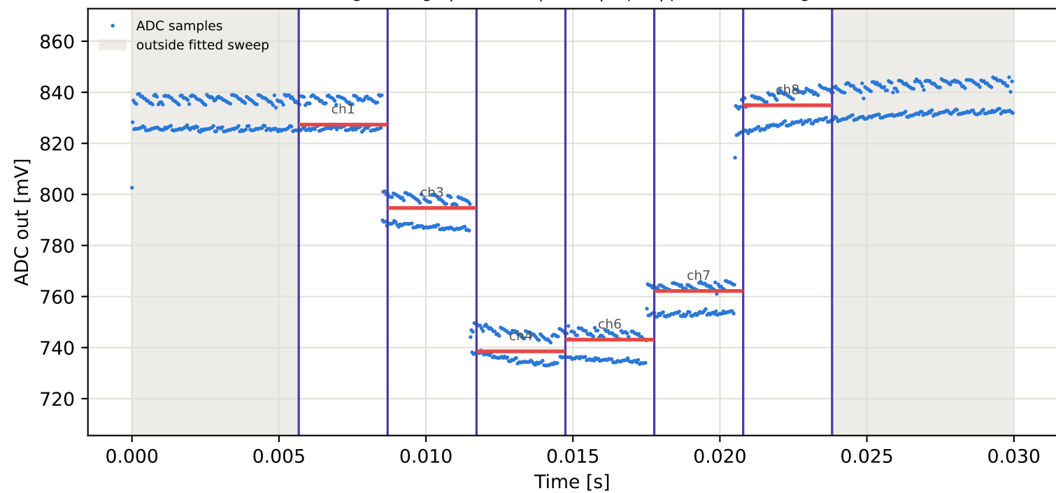
Tag8 &lt;- Tag7 | 915 MHz | run 0 | rep 1 | phase 16.63 deg
