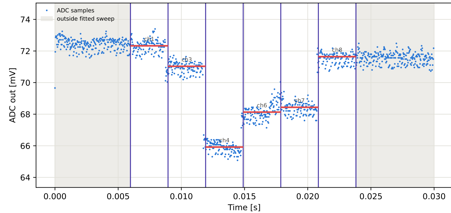
Tag3 &lt;- Tag15 | 965 MHz | run 0 | rep 1 | phase 130.43 deg
