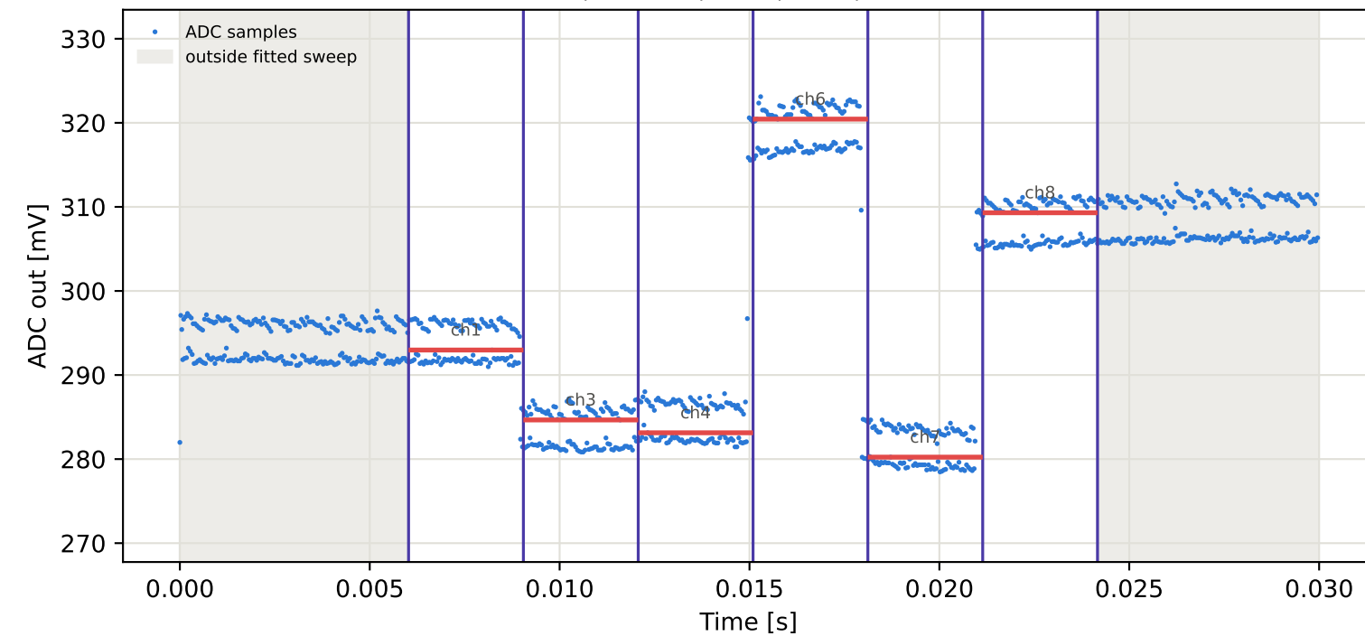
Tag6 &lt;- Tag1 | 985 MHz | run 0 | rep 1 | phase 157.66 deg
