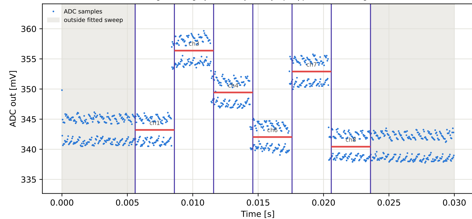
Tag15 &lt;- Tag5 | 825 MHz | run 0 | rep 1 | phase -2.37 deg
