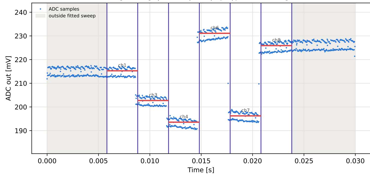
Tag10 &lt;- Tag8 | 975 MHz | run 0 | rep 1 | phase -99.38 deg
