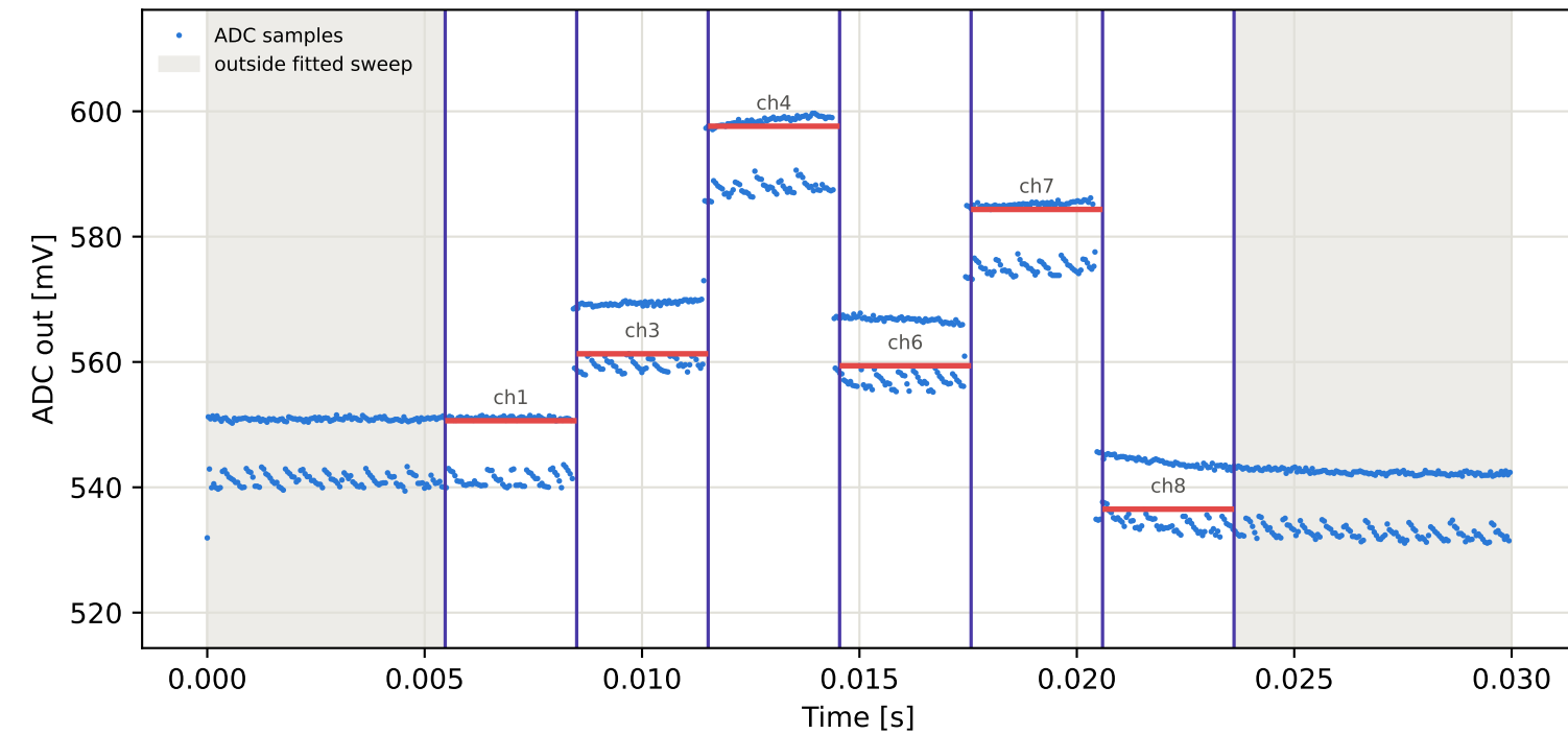
Tag5 &lt;- Tag3 | 935 MHz | run 0 | rep 1 | phase -170.84 deg
