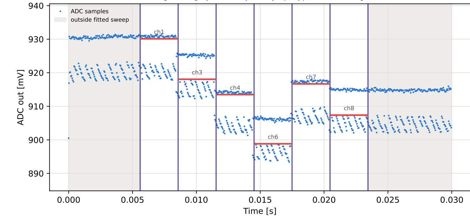
Tag8 &lt;- Tag6 | 865 MHz | run 0 | rep 1 | phase -100.84 deg
