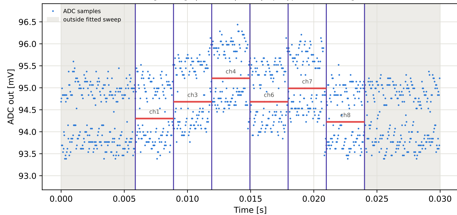
Tag7 &lt;- Tag4 | 795 MHz | run 0 | rep 1 | phase 114.84 deg
