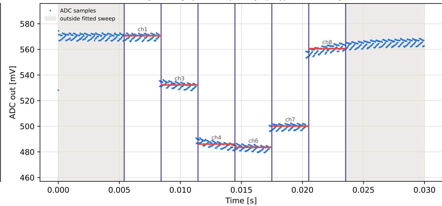
Tag16 &lt;- Tag5 | 895 MHz | run 0 | rep 1 | phase 6.11 deg
