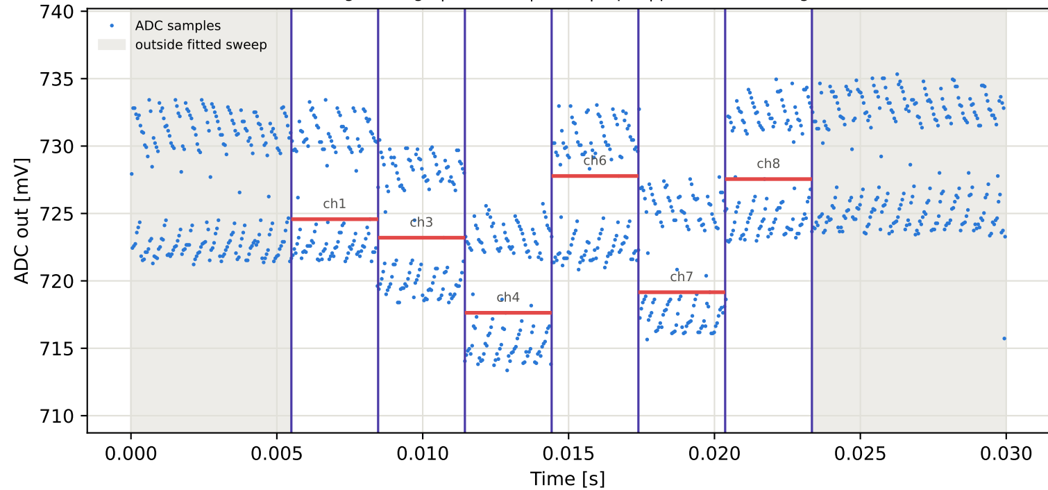
Tag7 &lt;- Tag6 | 945 MHz | run 0 | rep 1 | phase -29.71 deg
