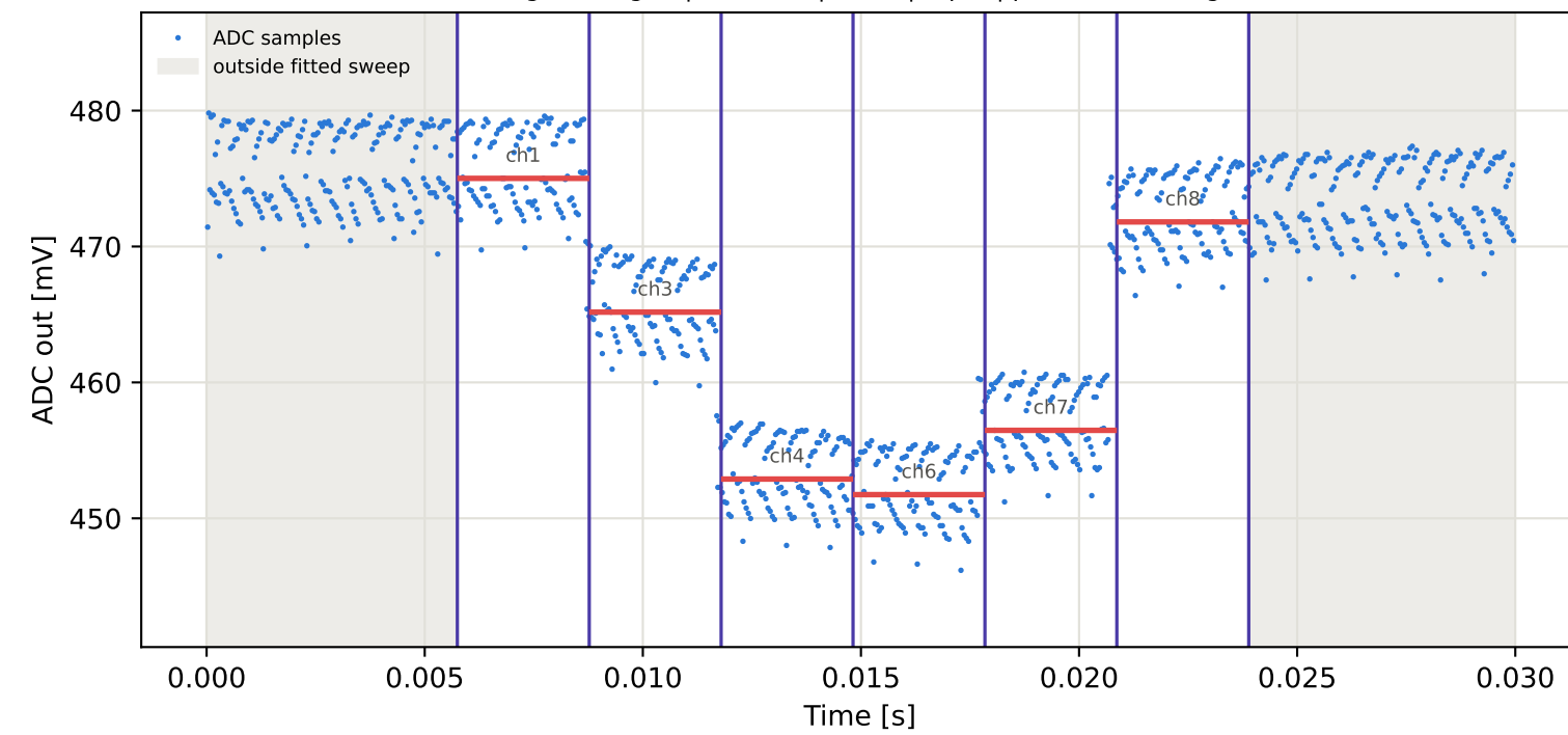
Tag6 &lt;- Tag2 | 905 MHz | run 0 | rep 1 | phase 88.52 deg
