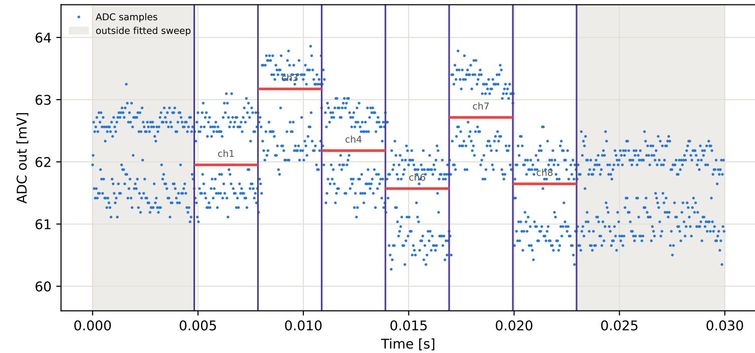
Tag16 &lt;- Tag15 | 785 MHz | run 0 | rep 1 | phase 114.19 deg
