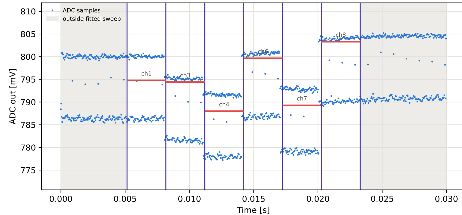
Tag8 &lt;- Tag15 | 915 MHz | run 0 | rep 1 | phase 3.05 deg
