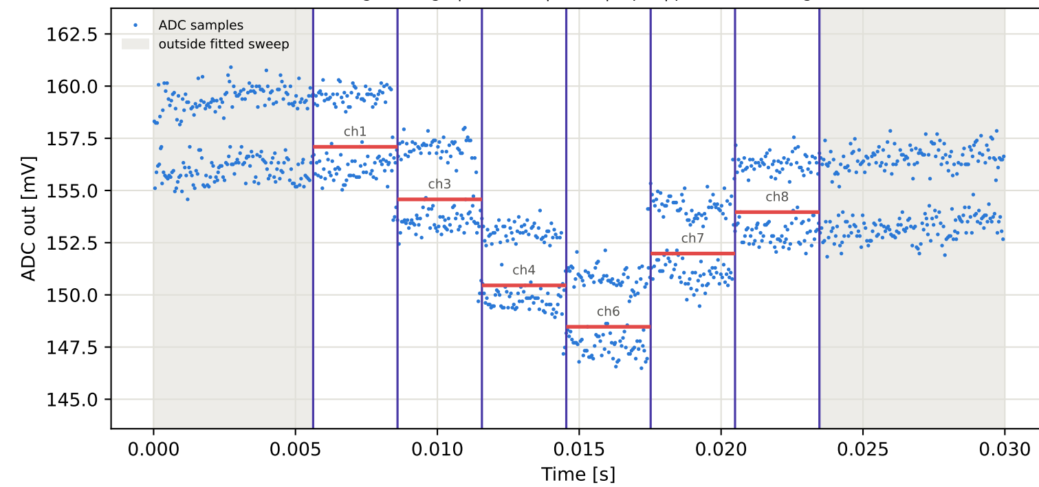
Tag2 &lt;- Tag5 | 885 MHz | run 0 | rep 1 | phase -106.74 deg
