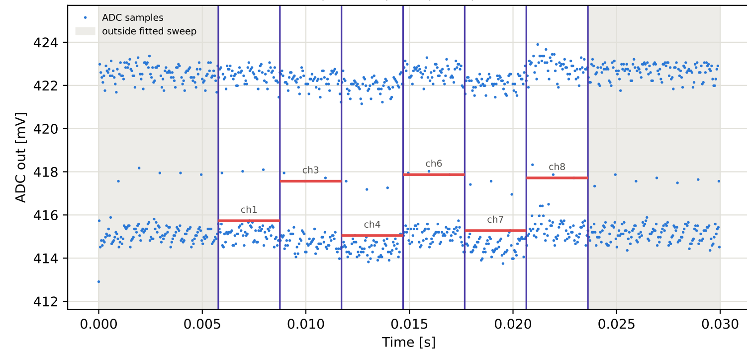
Tag15 &lt;- Tag1 | 995 MHz | run 0 | rep 1 | phase 116.80 deg
