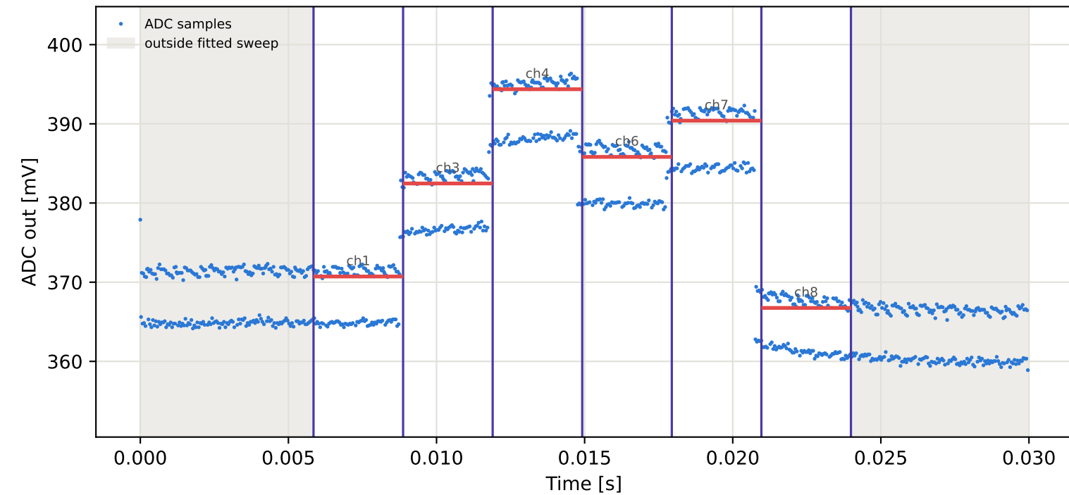
Tag4 &lt;- Tag2 | 915 MHz | run 0 | rep 1 | phase -105.64 deg
