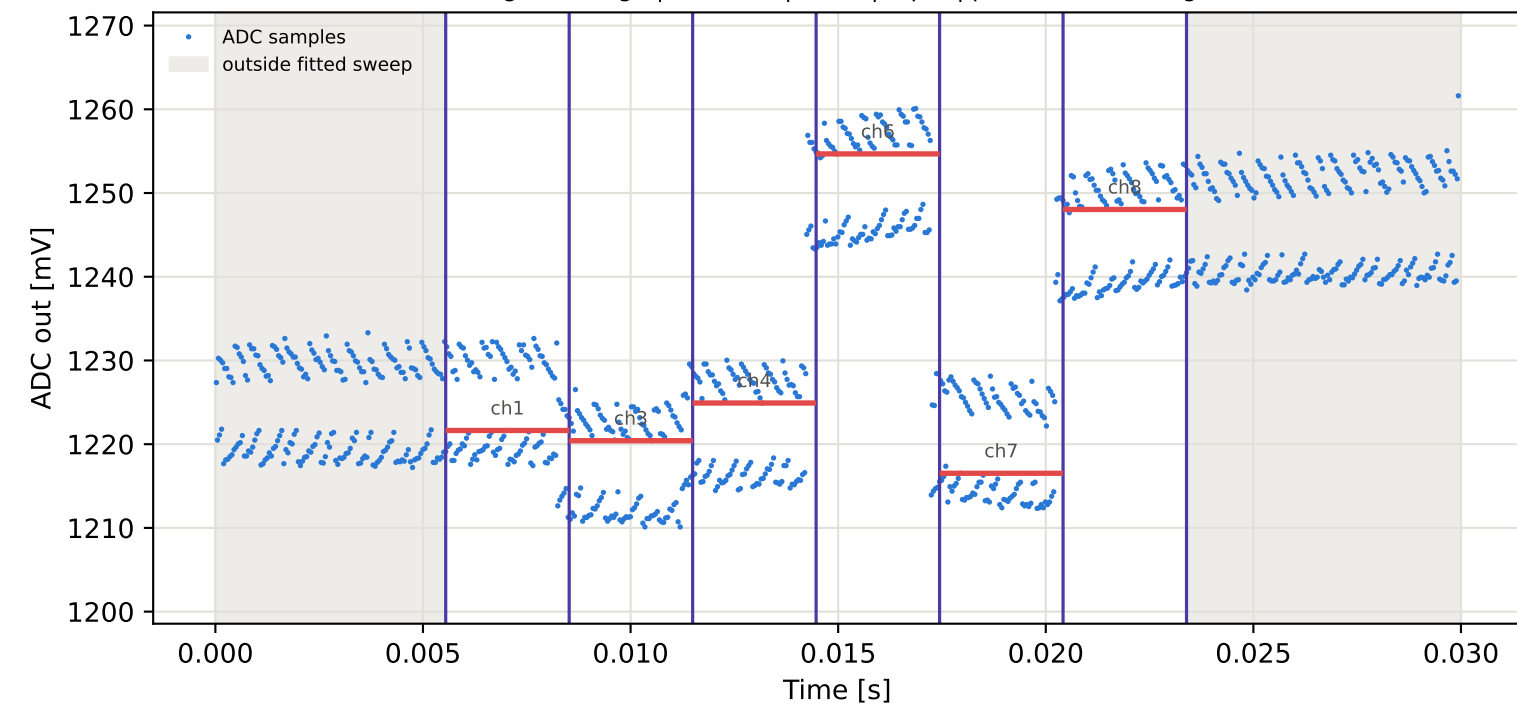
Tag16 &lt;- Tag6 | 895 MHz | run 0 | rep 1 | phase 91.33 deg
