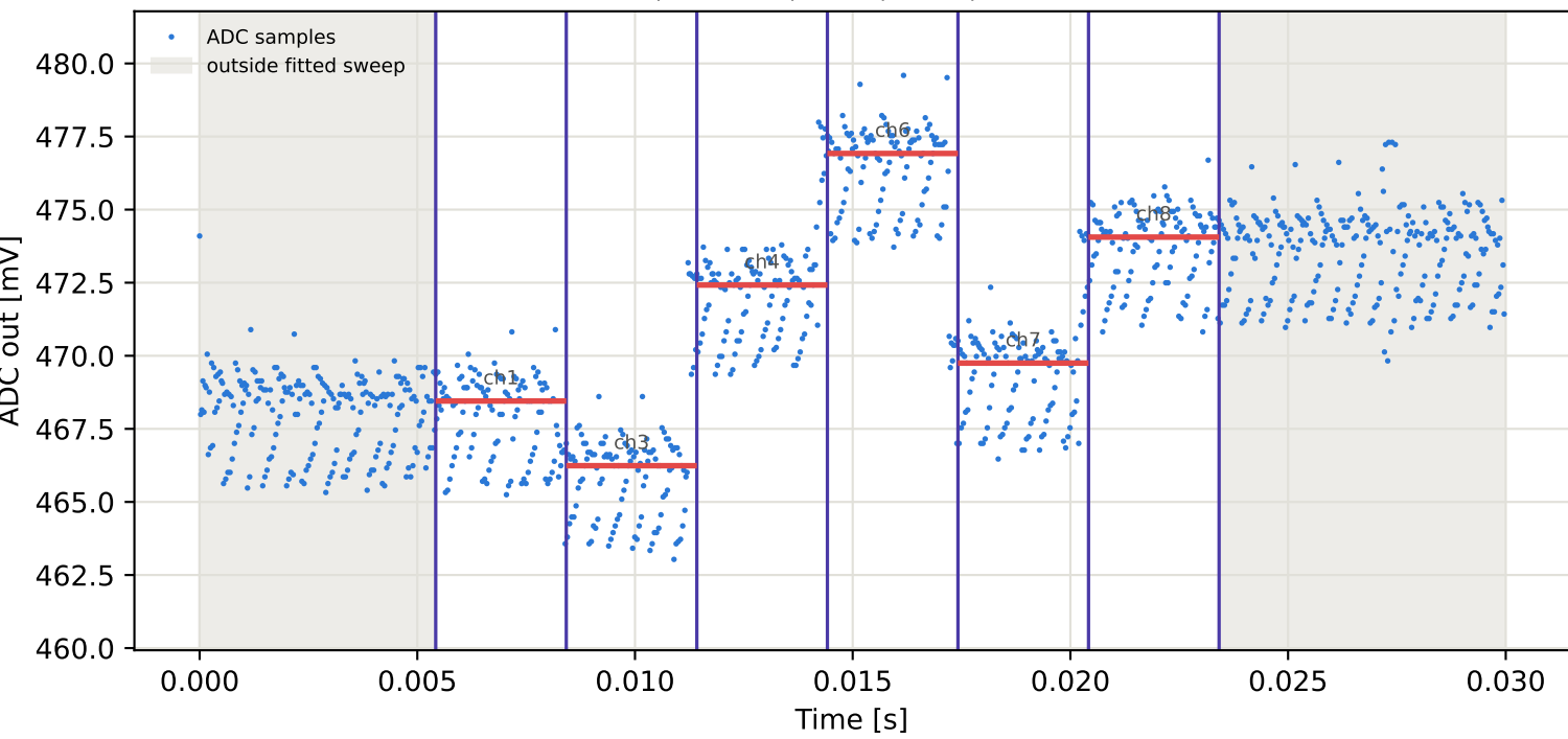
Tag4 &lt;- Tag9 | 855 MHz | run 0 | rep 1 | phase -152.30 deg
