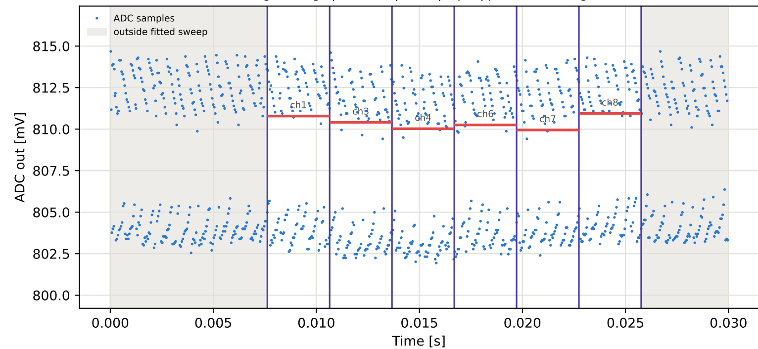
Tag7 &lt;- Tag15 | 895 MHz | run 0 | rep 1 | phase 74.25 deg
