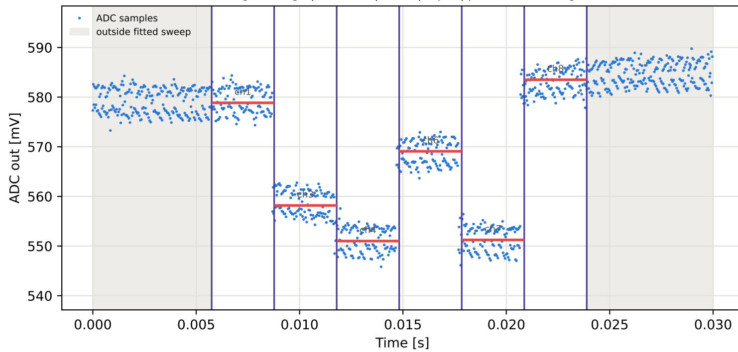
Tag3 &lt;- Tag10 | 885 MHz | run 0 | rep 1 | phase 166.60 deg
