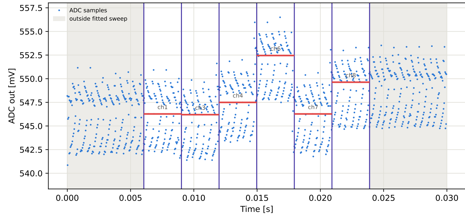
Tag7 &lt;- Tag15 | 955 MHz | run 0 | rep 1 | phase -178.21 deg
