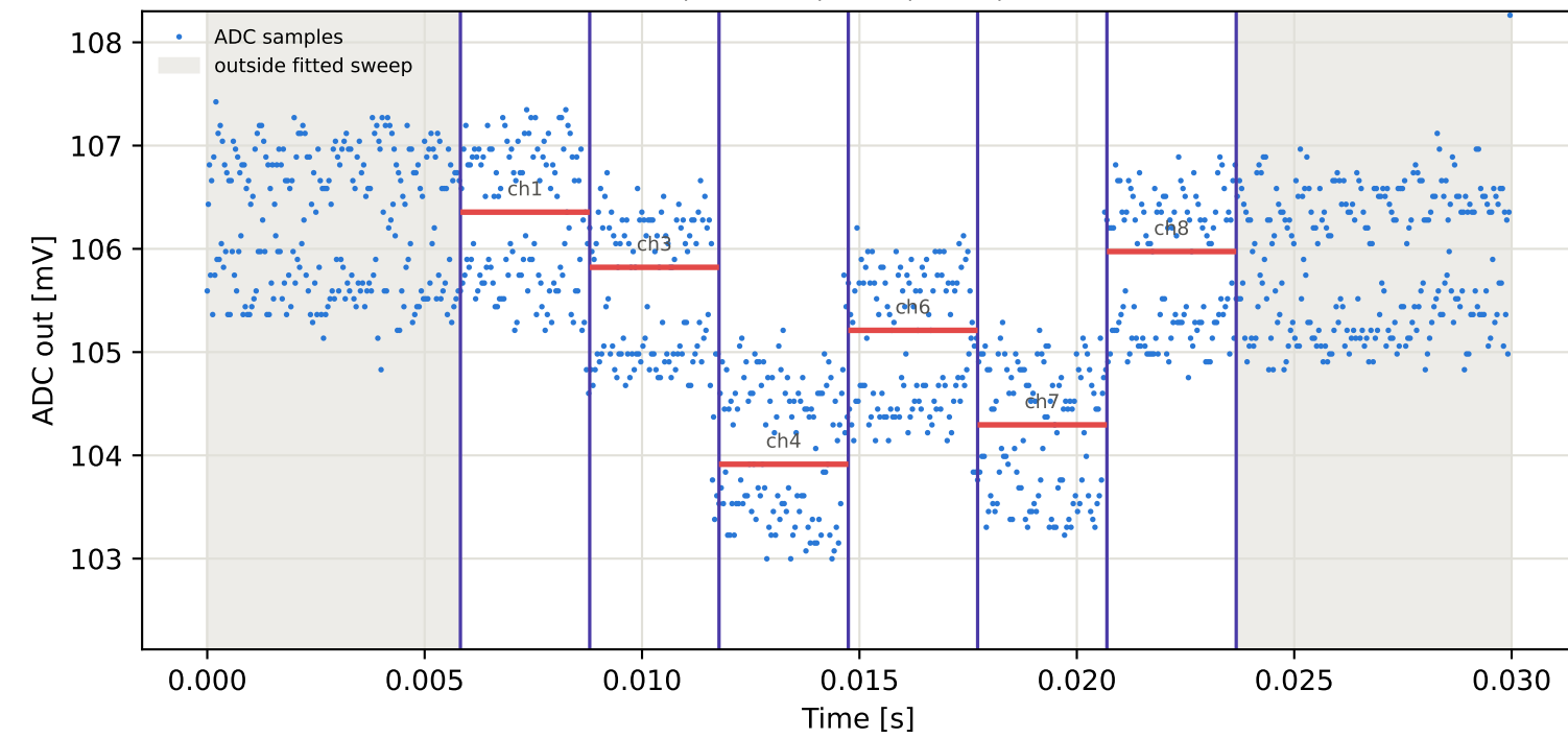
Tag16 &lt;- Tag6 | 795 MHz | run 0 | rep 1 | phase 89.51 deg
