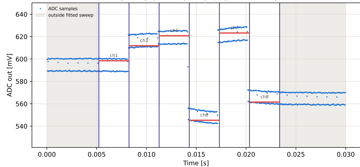
Tag8 &lt;- Tag10 | 965 MHz | run 0 | rep 1 | phase 99.76 deg
