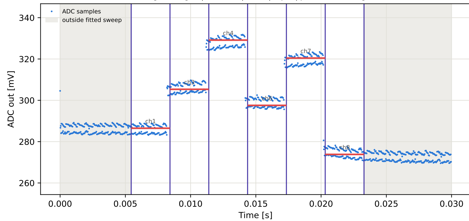
Tag6 &lt;- Tag3 | 925 MHz | run 0 | rep 1 | phase -48.82 deg
