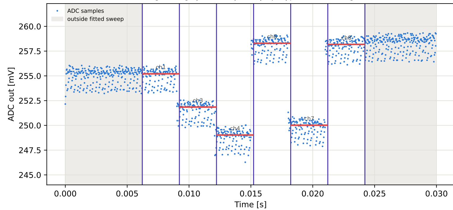
Tag3 &lt;- Tag15 | 965 MHz | run 0 | rep 1 | phase 32.77 deg
