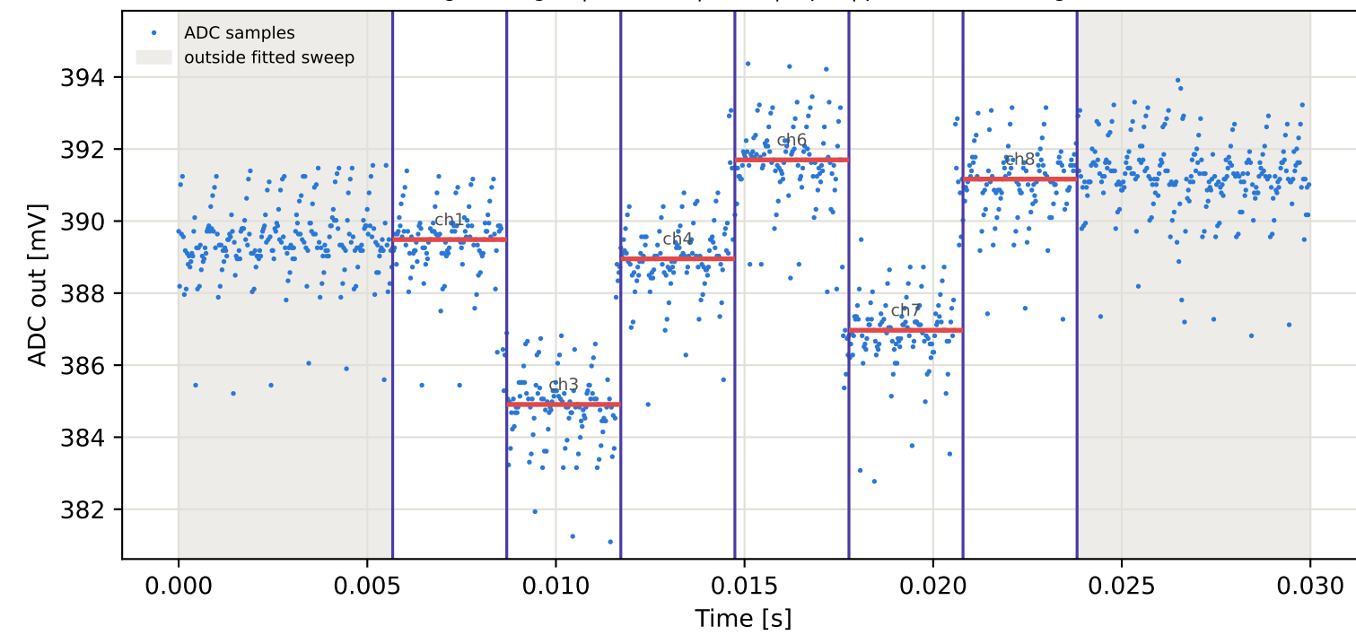
Tag5 &lt;- Tag16 | 805 MHz | run 0 | rep 1 | phase -87.56 deg
