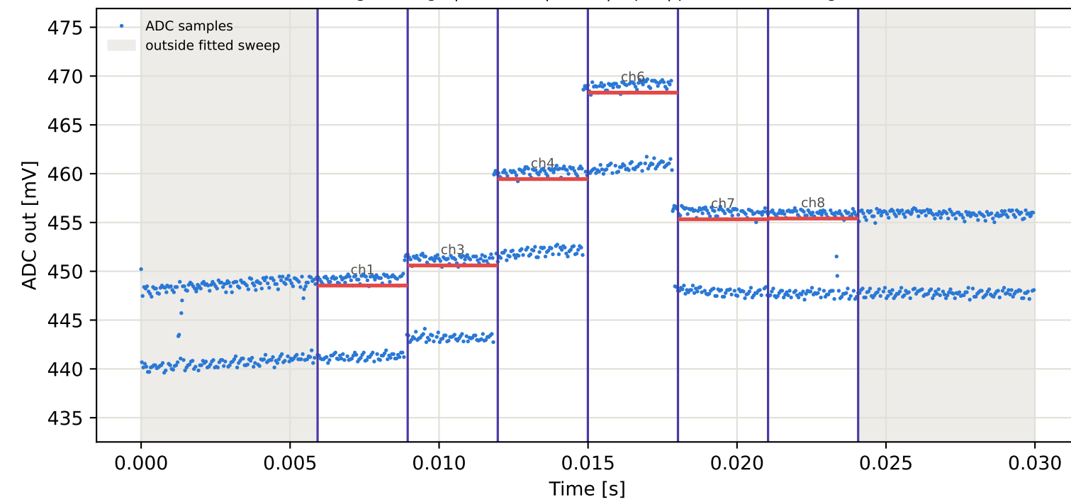
Tag3 &lt;- Tag6 | 935 MHz | run 0 | rep 1 | phase -33.34 deg
