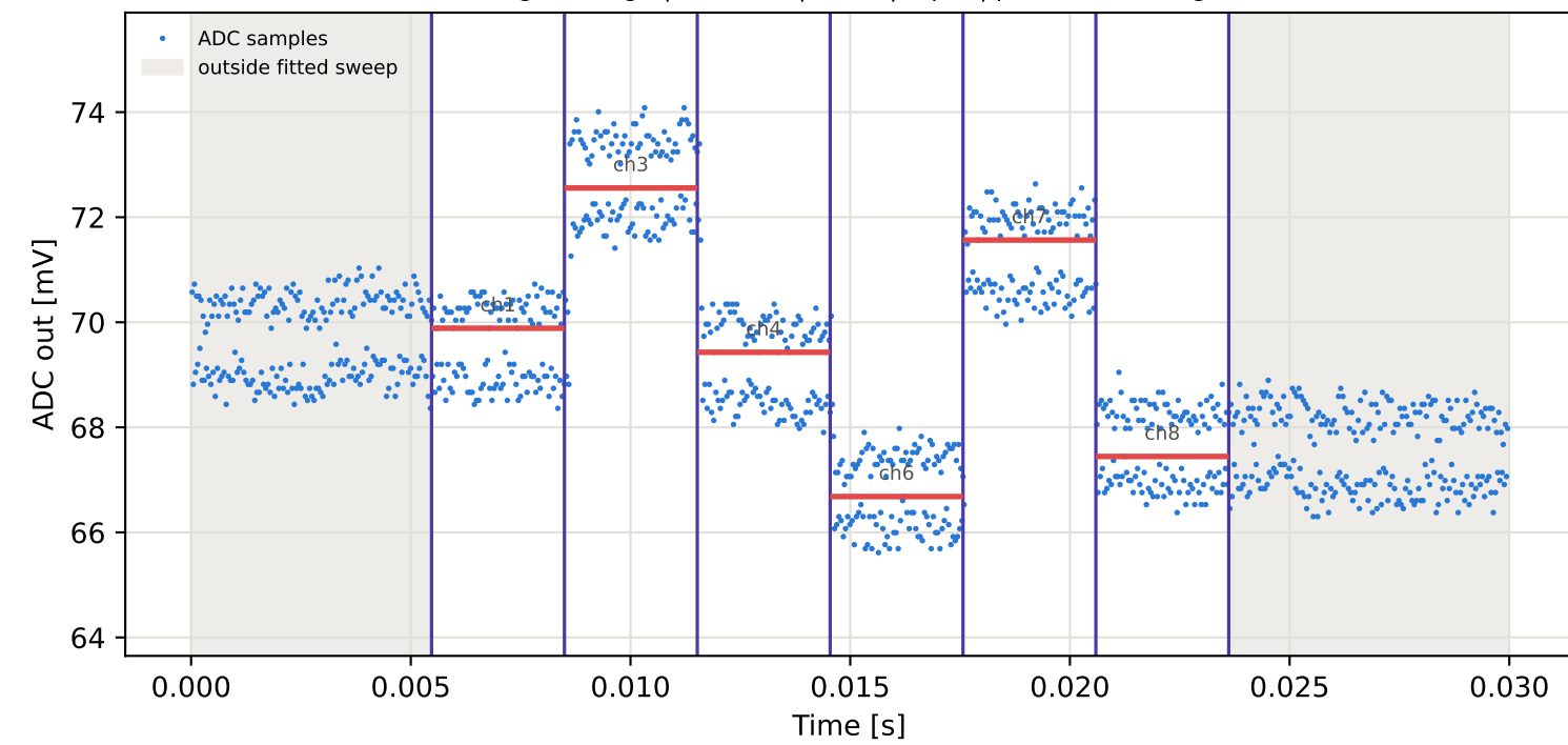
Tag4 &lt;- Tag8 | 785 MHz | run 0 | rep 1 | phase -15.23 deg
