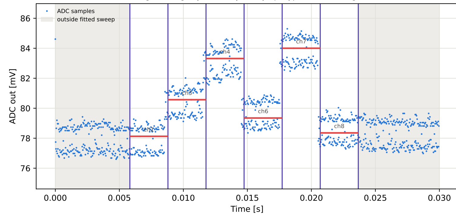
Tag15 &lt;- Tag3 | 795 MHz | run 0 | rep 1 | phase -122.44 deg
