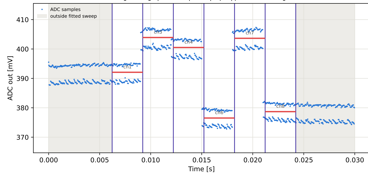
Tag6 &lt;- Tag9 | 845 MHz | run 0 | rep 1 | phase -96.95 deg
