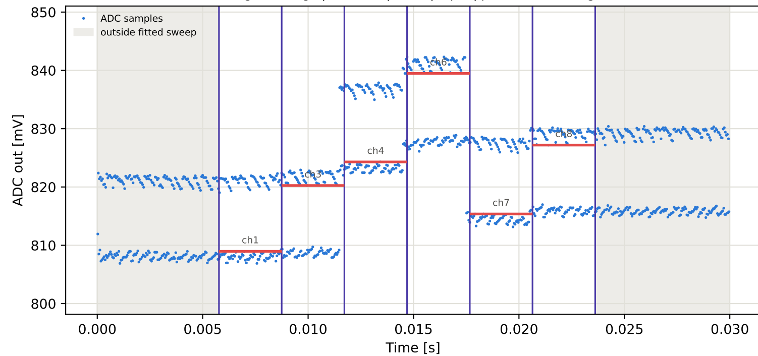
Tag2 &lt;- Tag10 | 985 MHz | run 0 | rep 1 | phase 92.33 deg
