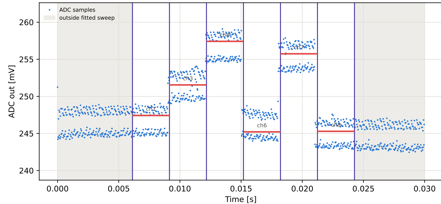
Tag1 &lt;- Tag4 | 825 MHz | run 0 | rep 1 | phase -103.88 deg
