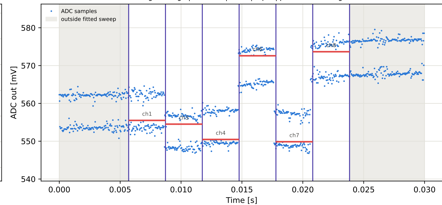
Tag2 &lt;- Tag6 | 885 MHz | run 0 | rep 1 | phase -64.27 deg
