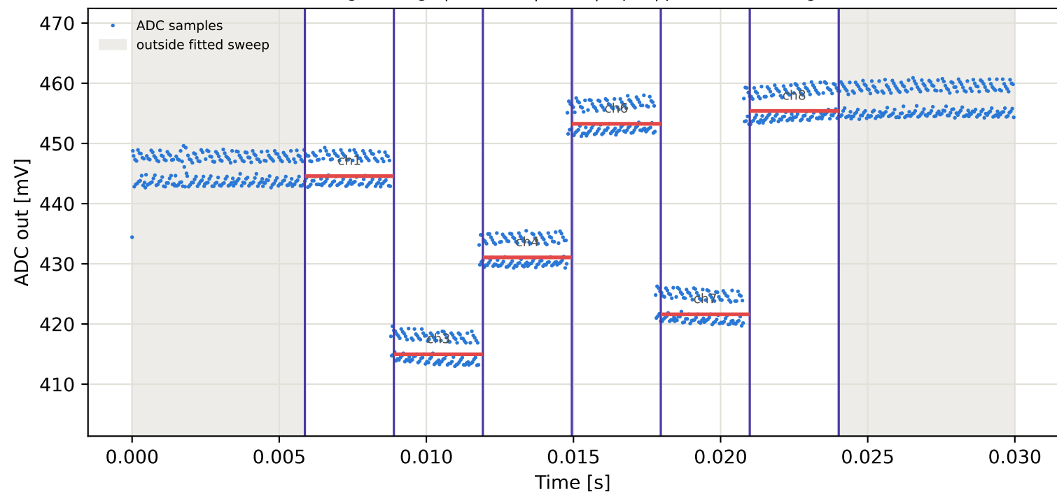
Tag3 &lt;- Tag7 | 835 MHz | run 0 | rep 1 | phase 93.20 deg
