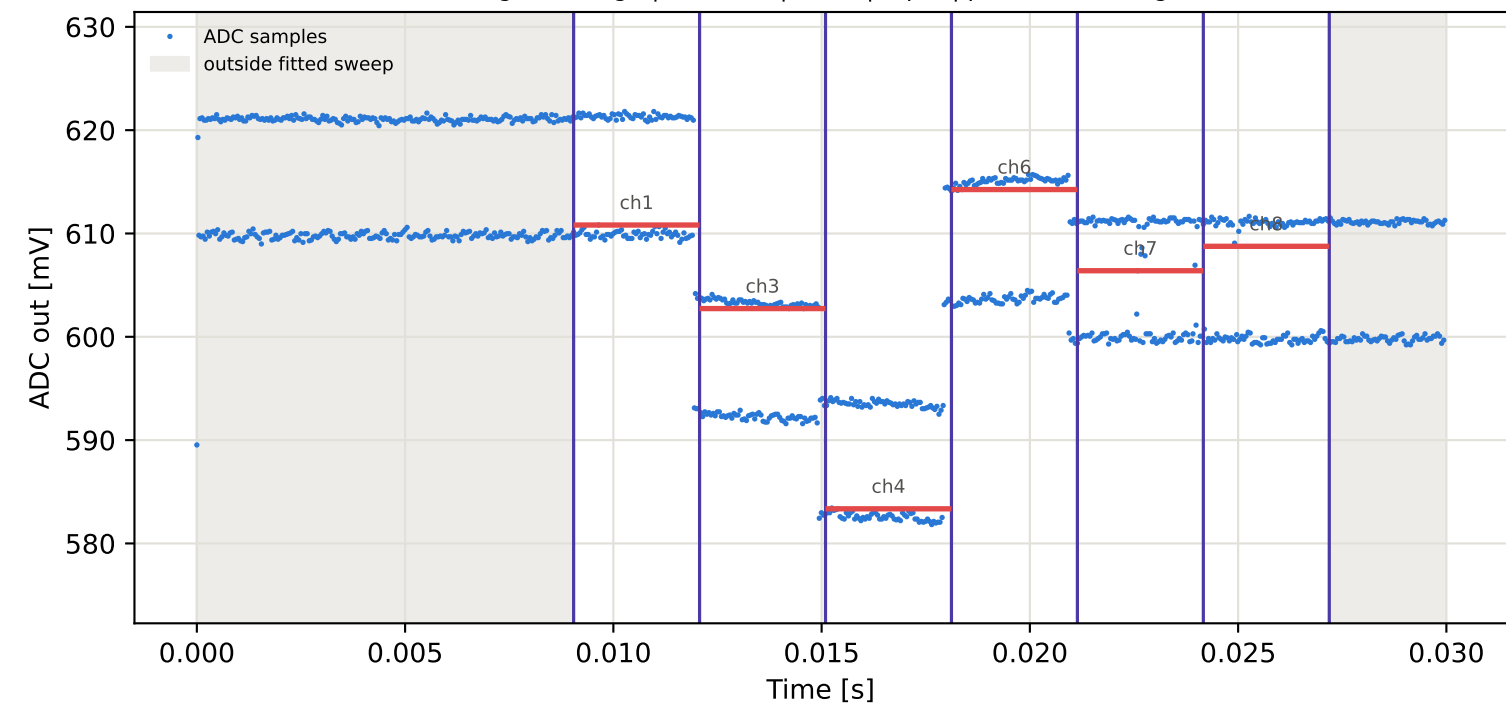
Tag16 &lt;- Tag1 | 965 MHz | run 0 | rep 1 | phase 56.61 deg
