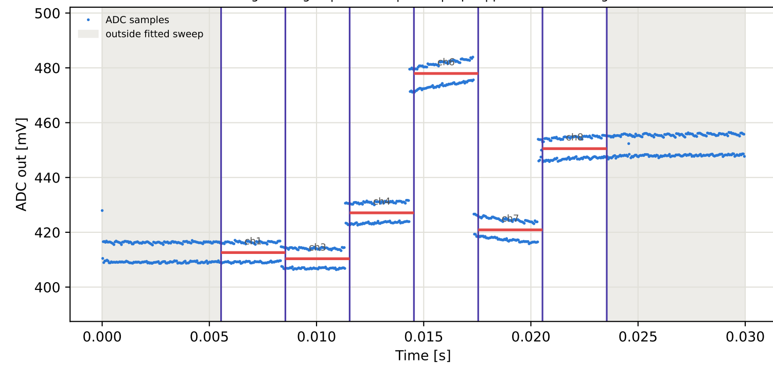
Tag7 &lt;- Tag3 | 905 MHz | run 0 | rep 1 | phase -8.55 deg
