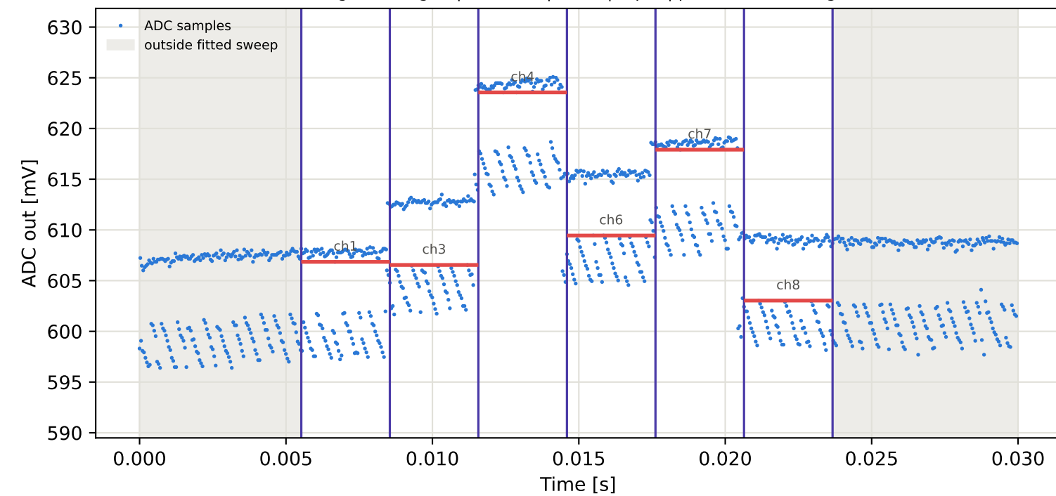
Tag15 &lt;- Tag3 | 965 MHz | run 0 | rep 1 | phase -62.60 deg
