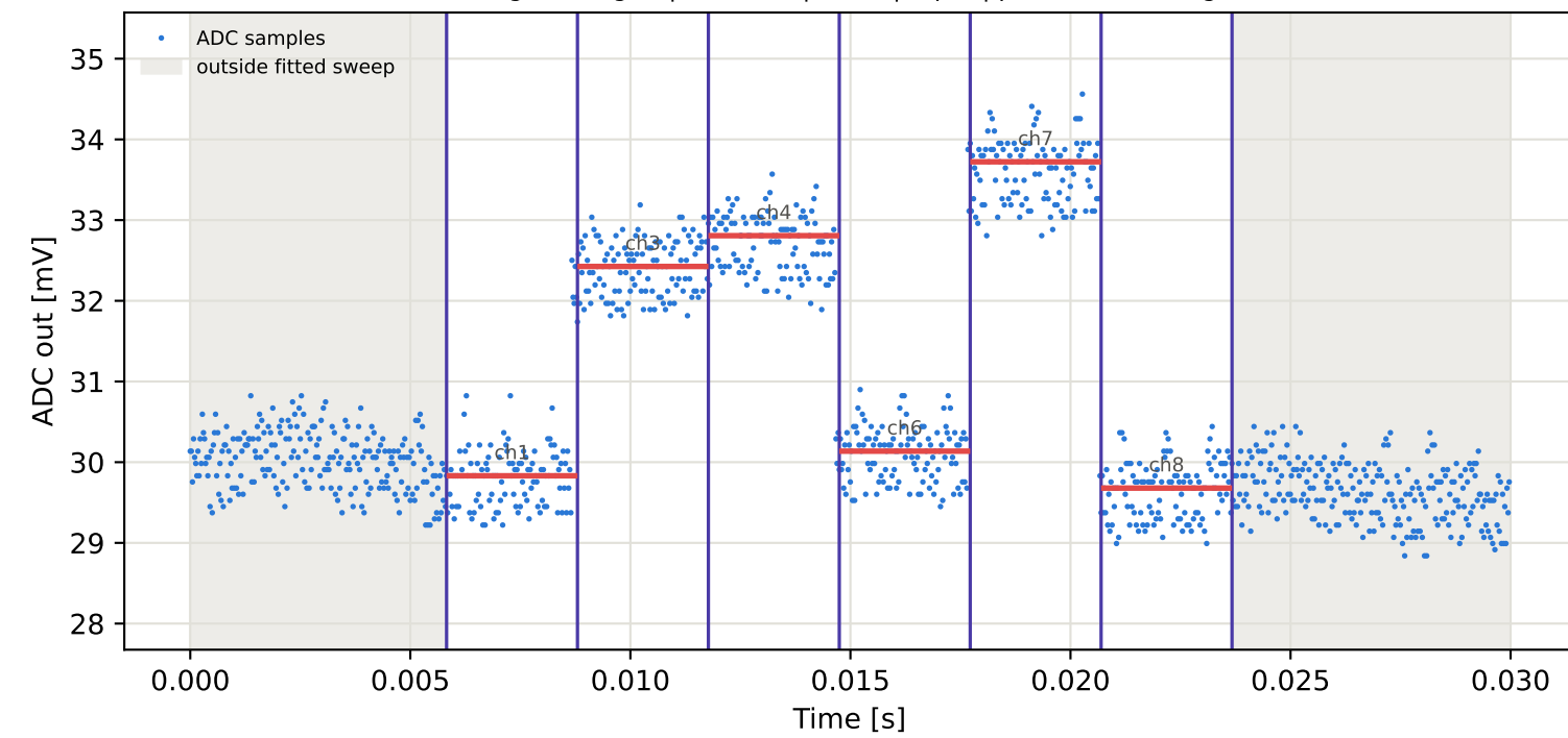
Tag1 &lt;- Tag16 | 795 MHz | run 0 | rep 1 | phase 139.21 deg
