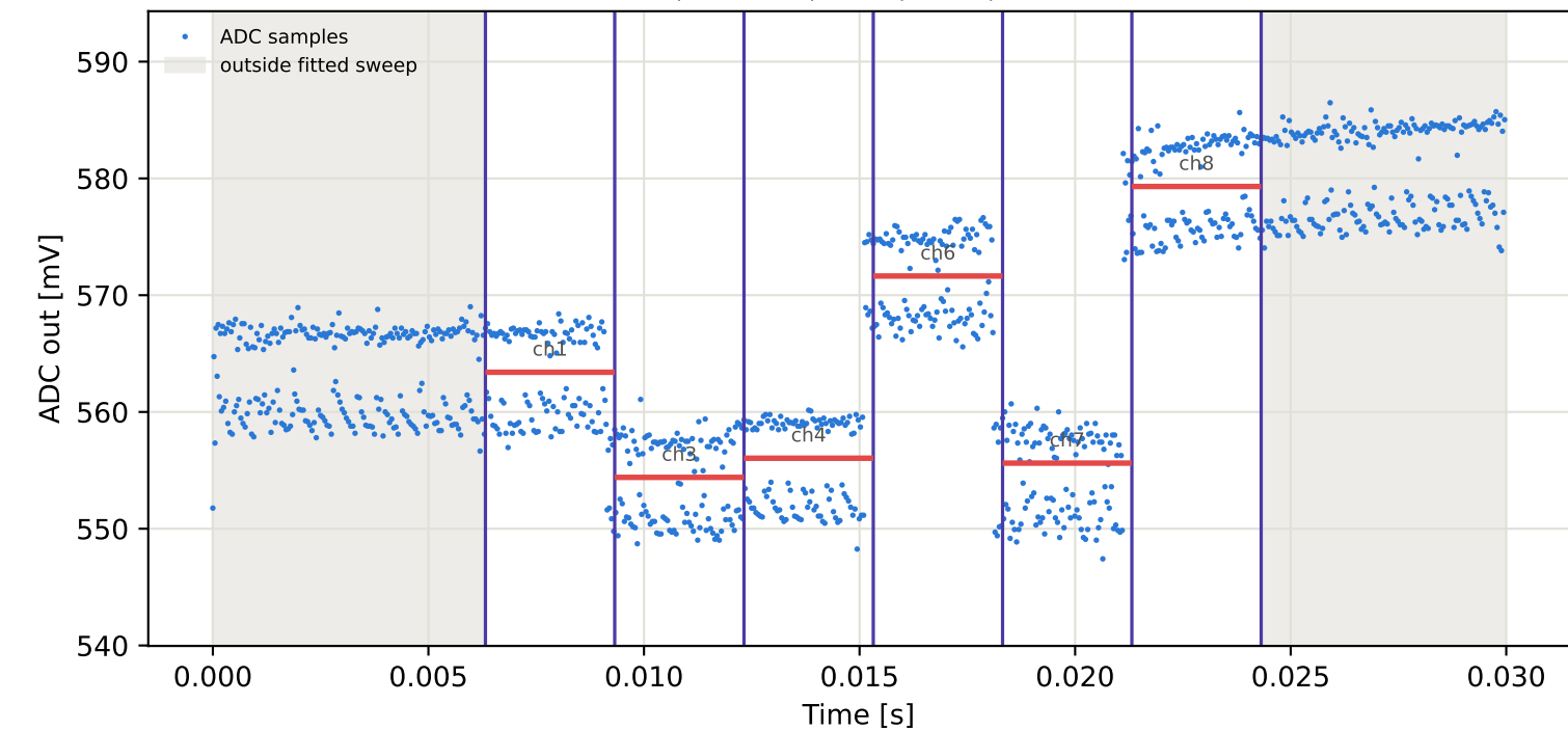
Tag2 &lt;- Tag16 | 885 MHz | run 0 | rep 1 | phase 152.00 deg
