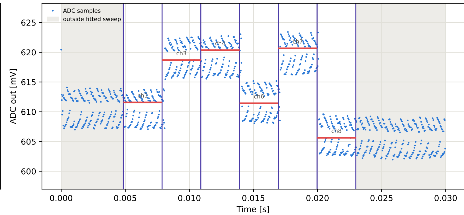
Tag15 &lt;- Tag10 | 865 MHz | run 0 | rep 1 | phase -50.57 deg
