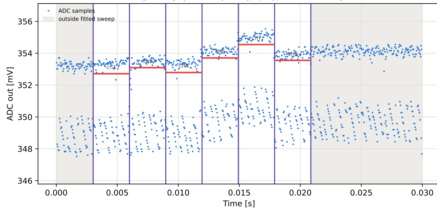
Tag8 &lt;- Tag4 | 805 MHz | run 0 | rep 1 | phase -151.40 deg
