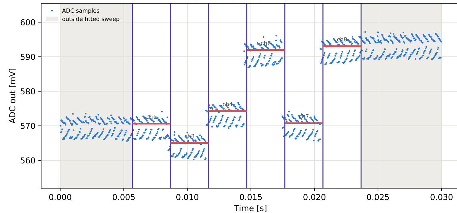
Tag6 &lt;- Tag4 | 865 MHz | run 0 | rep 1 | phase -172.52 deg
