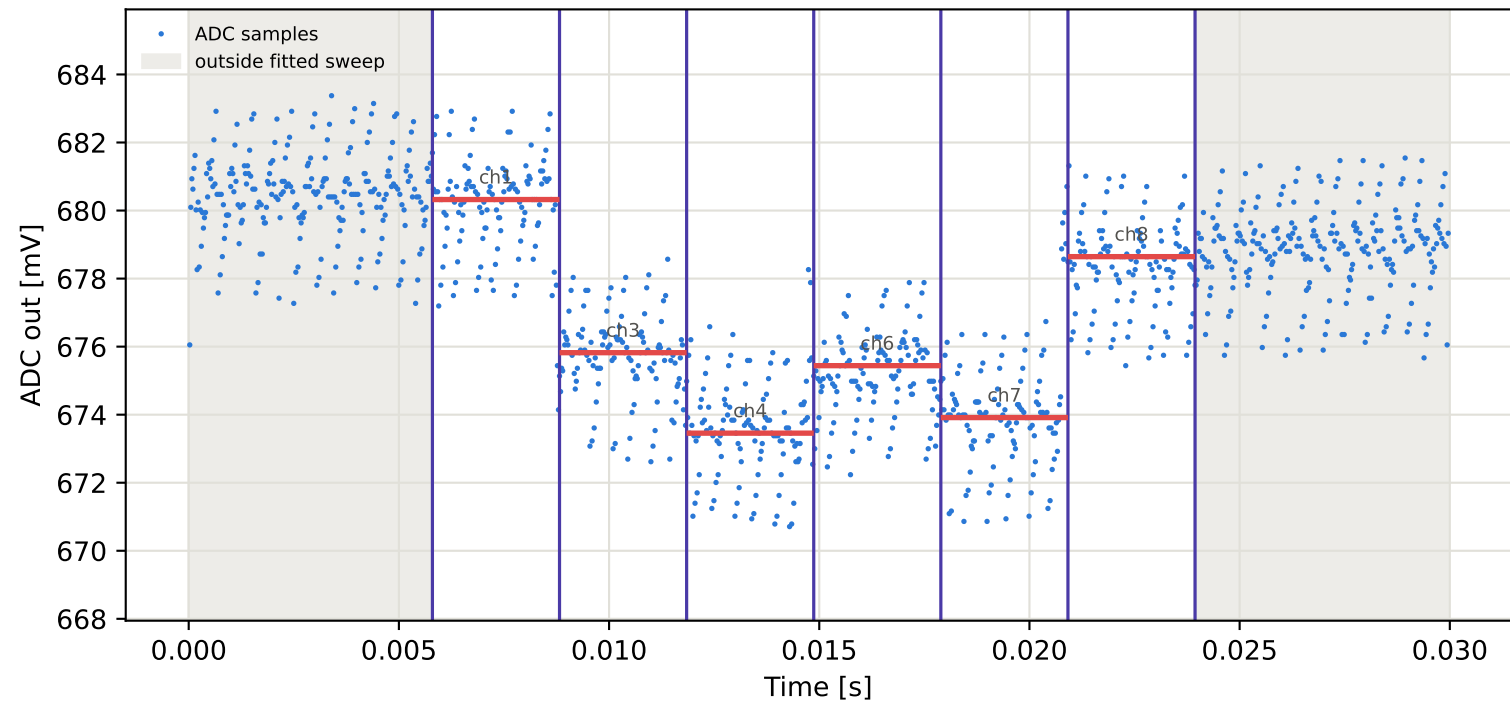
Tag8 &lt;- Tag7 | 855 MHz | run 0 | rep 1 | phase -149.06 deg
