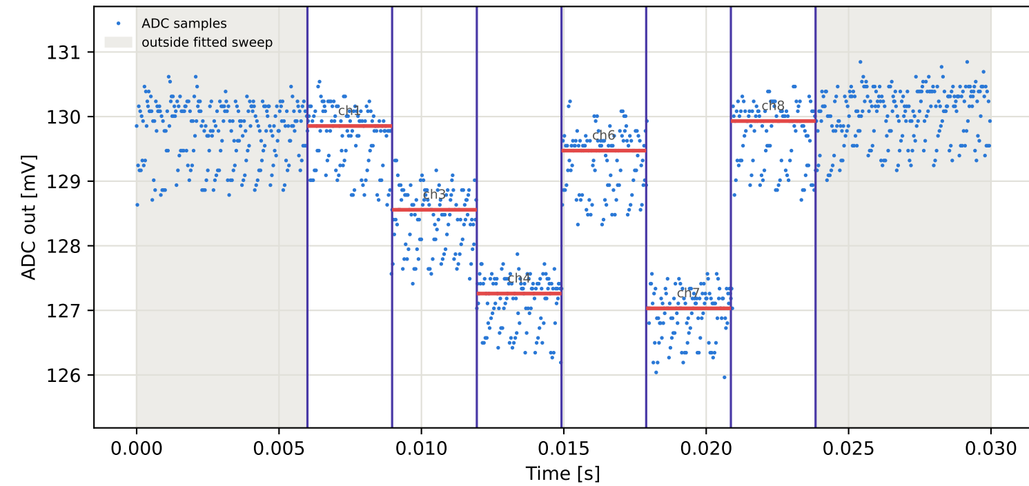
Tag7 &lt;- Tag15 | 805 MHz | run 0 | rep 1 | phase -87.42 deg
