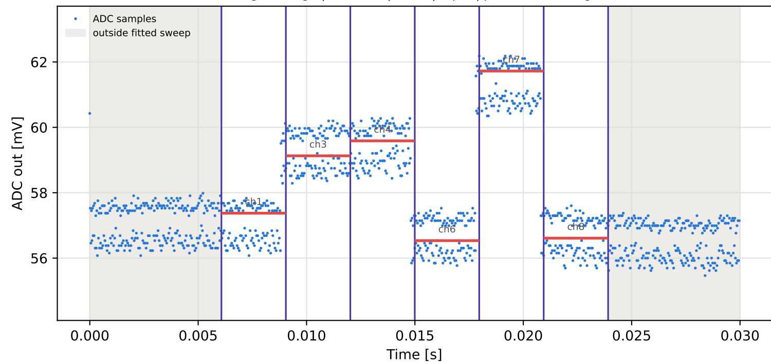
Tag3 &lt;- Tag6 | 775 MHz | run 0 | rep 1 | phase -62.15 deg
