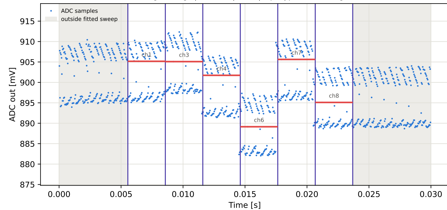
Tag9 &lt;- Tag10 | 985 MHz | run 0 | rep 1 | phase -23.11 deg
