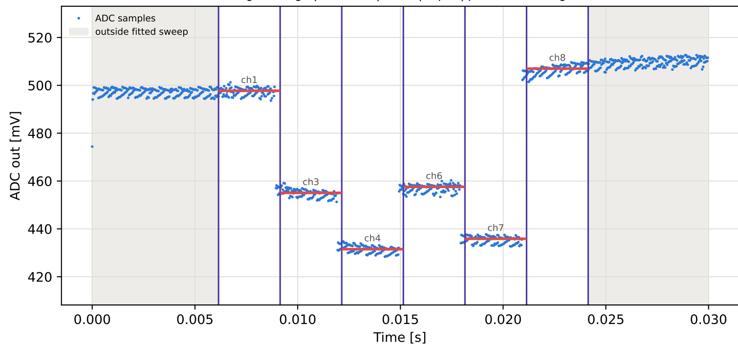
Tag4 &lt;- Tag3 | 875 MHz | run 0 | rep 1 | phase 91.66 deg
