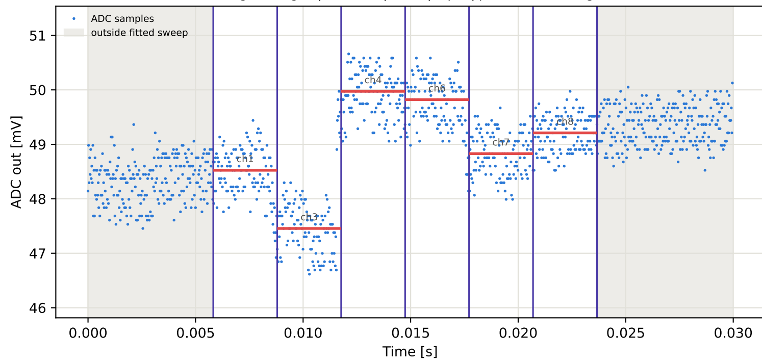
Tag1 &lt;- Tag2 | 775 MHz | run 0 | rep 1 | phase 133.52 deg
