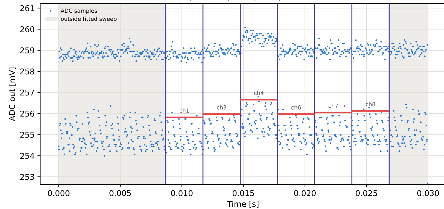
Tag8 &lt;- Tag4 | 785 MHz | run 0 | rep 1 | phase 14.60 deg
