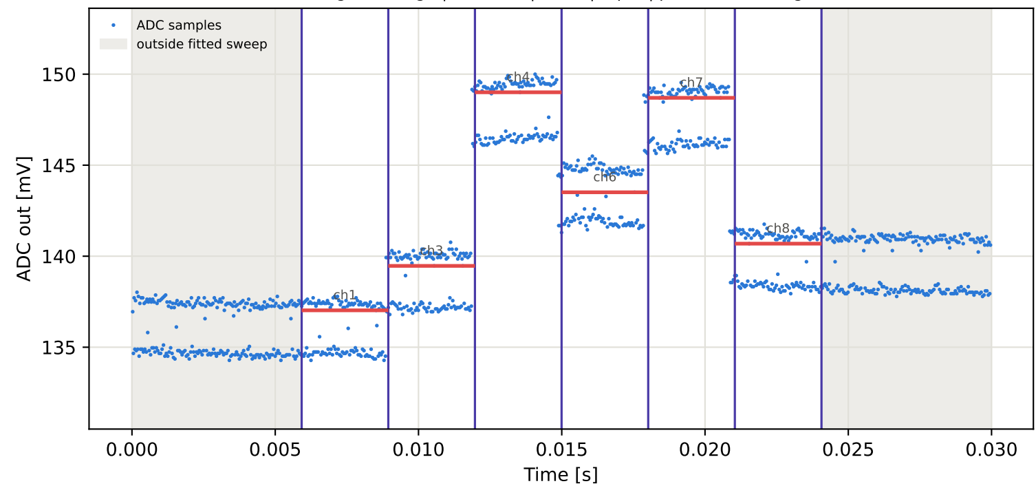
Tag16 &lt;- Tag1 | 805 MHz | run 0 | rep 1 | phase -77.78 deg
