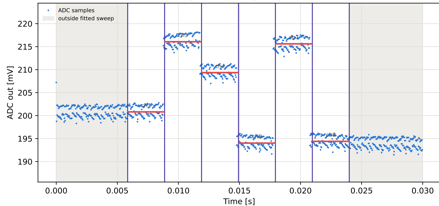
Tag16 &lt;- Tag15 | 825 MHz | run 0 | rep 1 | phase -11.19 deg
