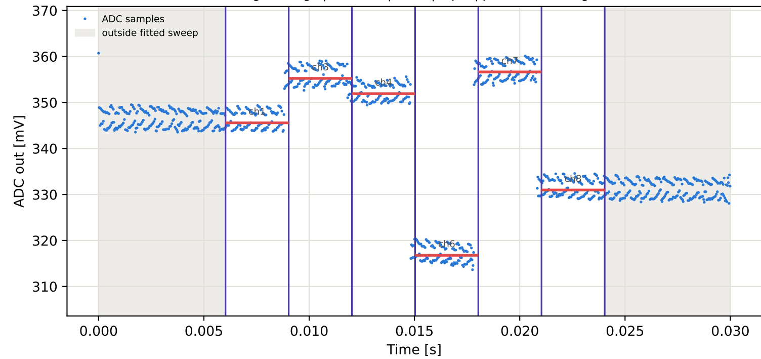
Tag6 &lt;- Tag5 | 985 MHz | run 0 | rep 1 | phase -13.24 deg
