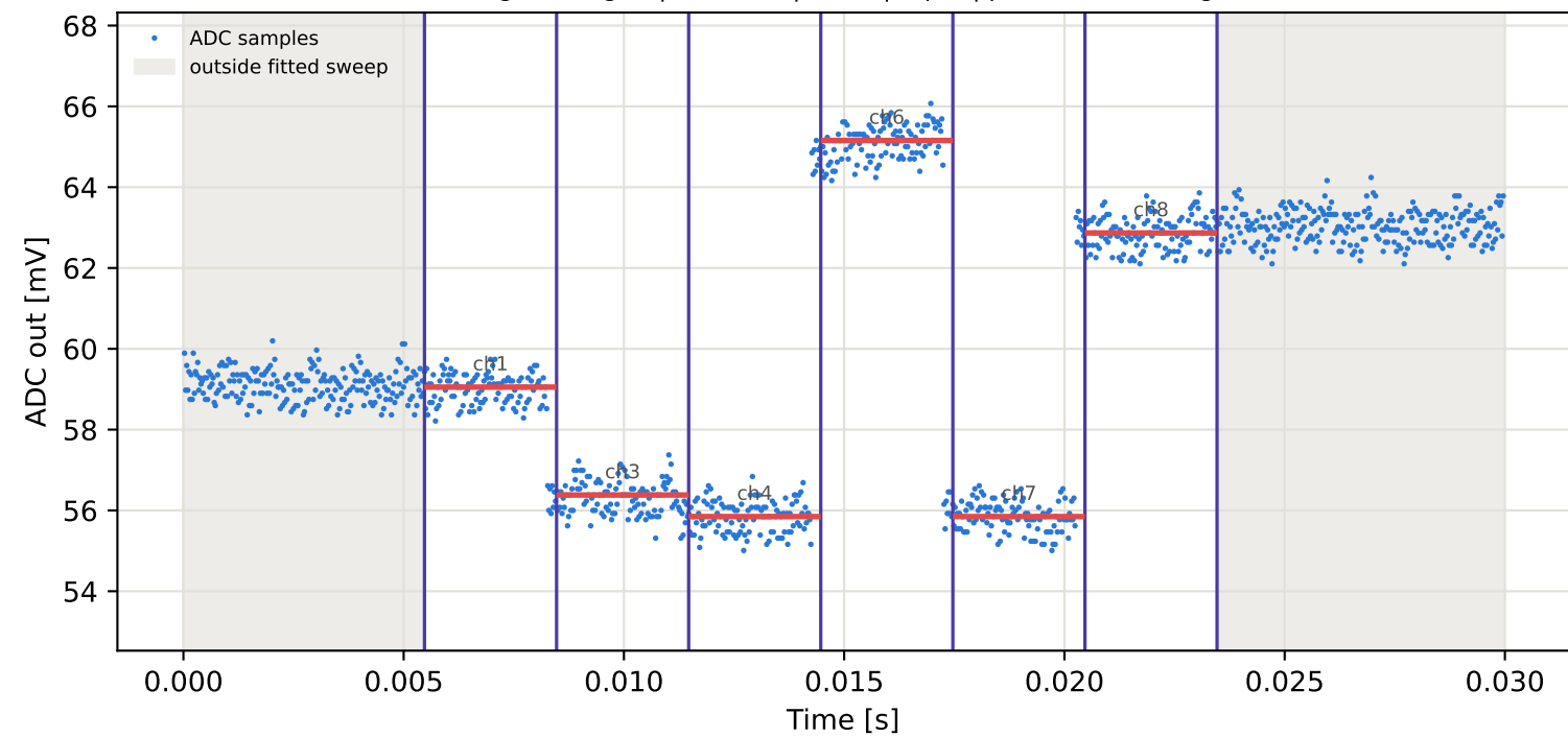
Tag1 &lt;- Tag2 | 955 MHz | run 0 | rep 1 | phase -121.92 deg
