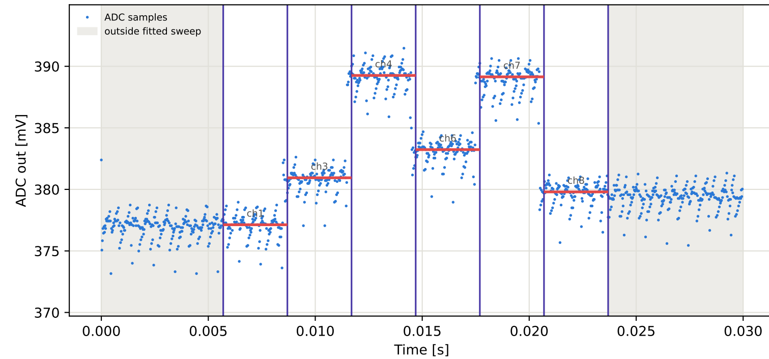
Tag5 &lt;- Tag3 | 805 MHz | run 0 | rep 1 | phase -91.54 deg
