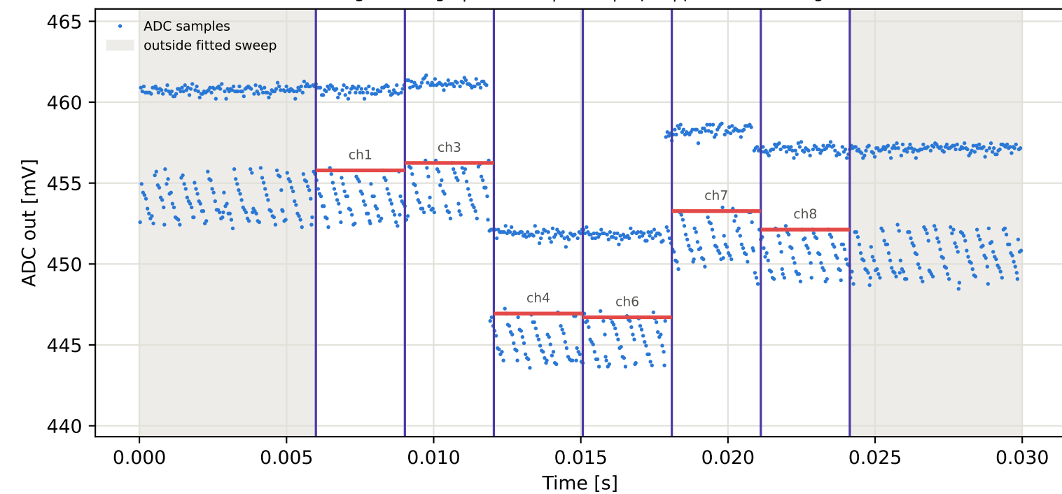
Tag16 &lt;- Tag6 | 995 MHz | run 0 | rep 1 | phase 34.78 deg
