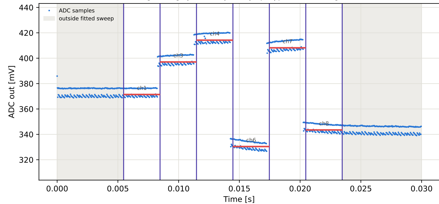
Tag3 &lt;- Tag7 | 955 MHz | run 0 | rep 1 | phase -142.23 deg
