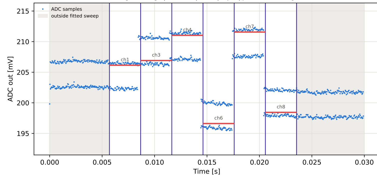
Tag15 &lt;- Tag9 | 975 MHz | run 0 | rep 1 | phase 94.10 deg
