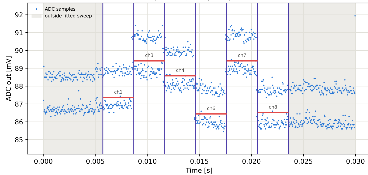
Tag5 &lt;- Tag8 | 775 MHz | run 0 | rep 1 | phase -174.56 deg
