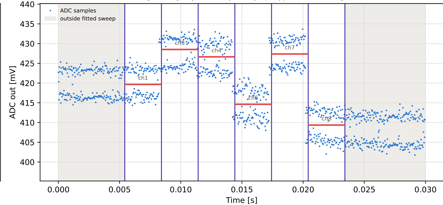
Tag1 &lt;- Tag2 | 885 MHz | run 0 | rep 1 | phase -87.38 deg
