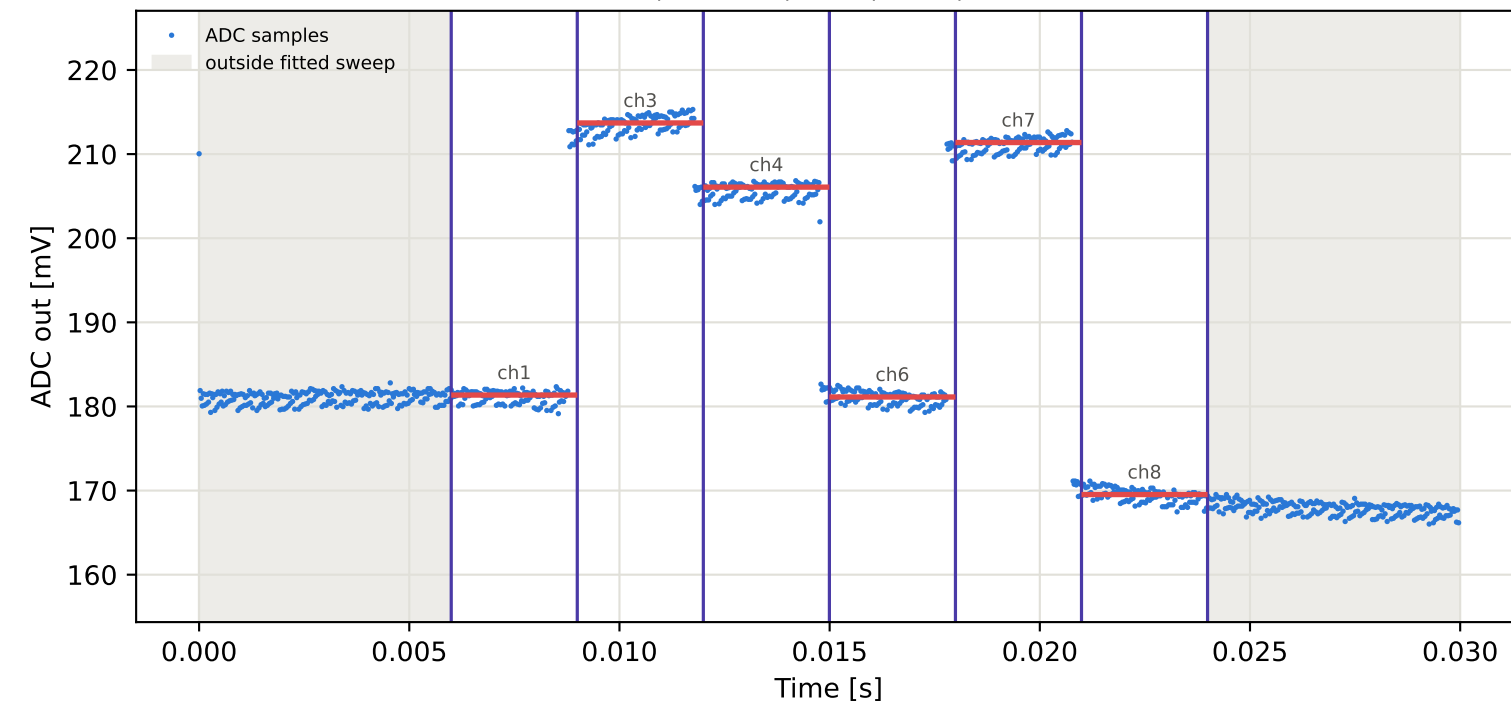
Tag9 &lt;- Tag16 | 855 MHz | run 0 | rep 1 | phase -36.62 deg
