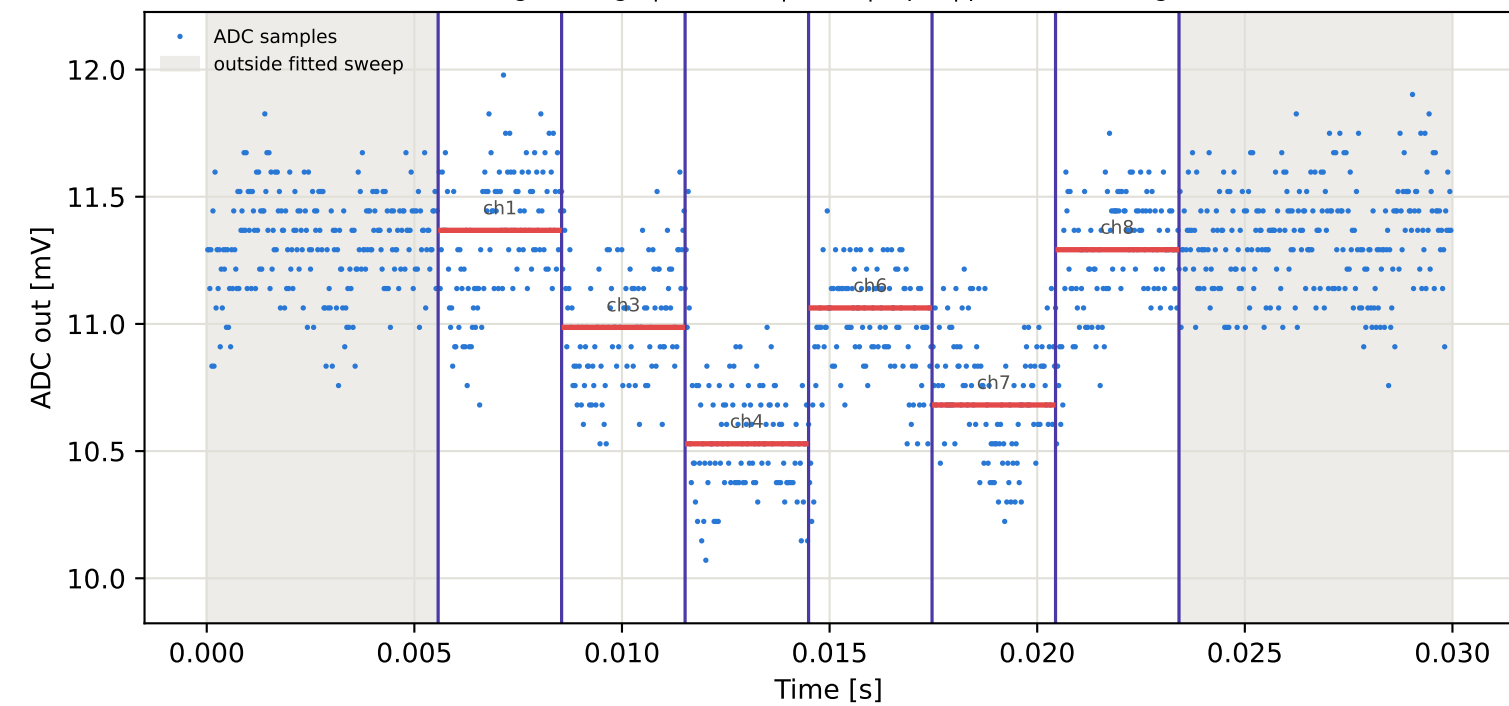
Tag3 &lt;- Tag10 | 995 MHz | run 0 | rep 1 | phase 88.34 deg
