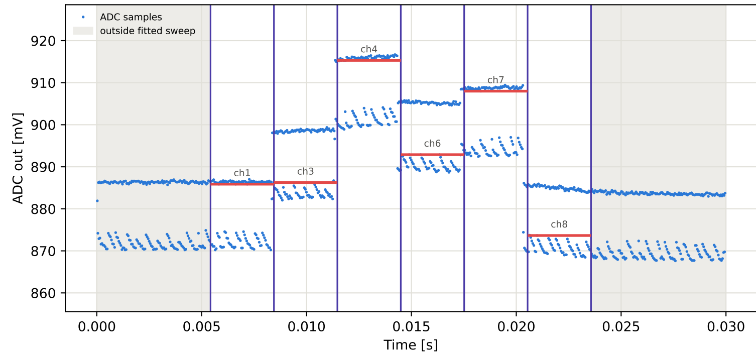
Tag9 &lt;- Tag2 | 935 MHz | run 0 | rep 1 | phase -175.92 deg
