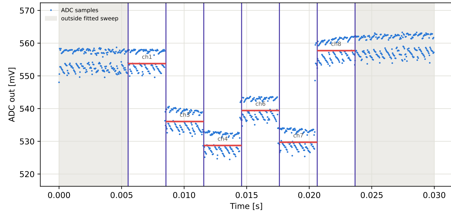
Tag2 &lt;- Tag16 | 875 MHz | run 0 | rep 1 | phase 136.85 deg
