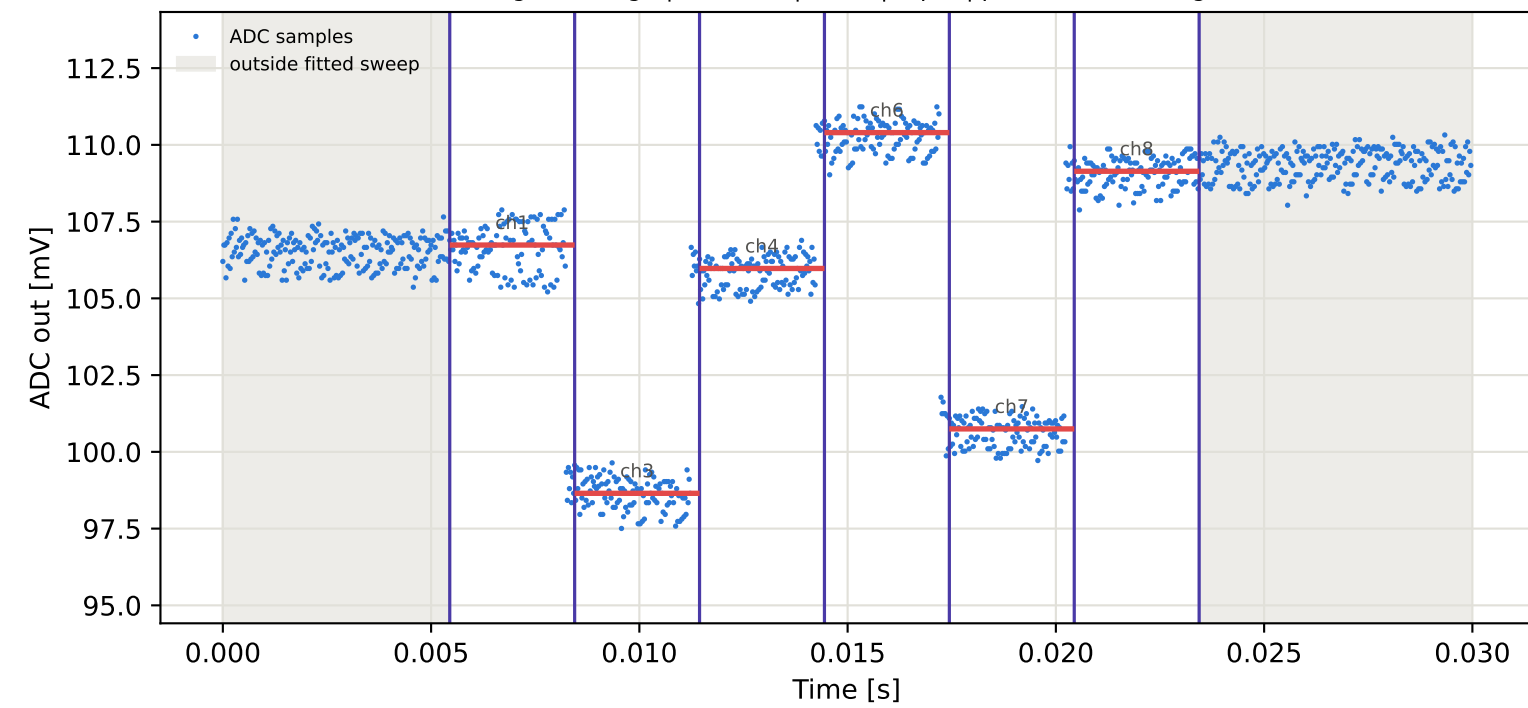
Tag16 &lt;- Tag5 | 795 MHz | run 0 | rep 1 | phase -160.47 deg
