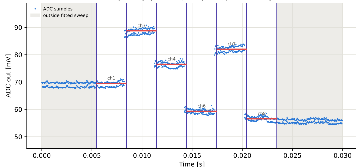
Tag9 &lt;- Tag8 | 835 MHz | run 0 | rep 1 | phase -4.94 deg
