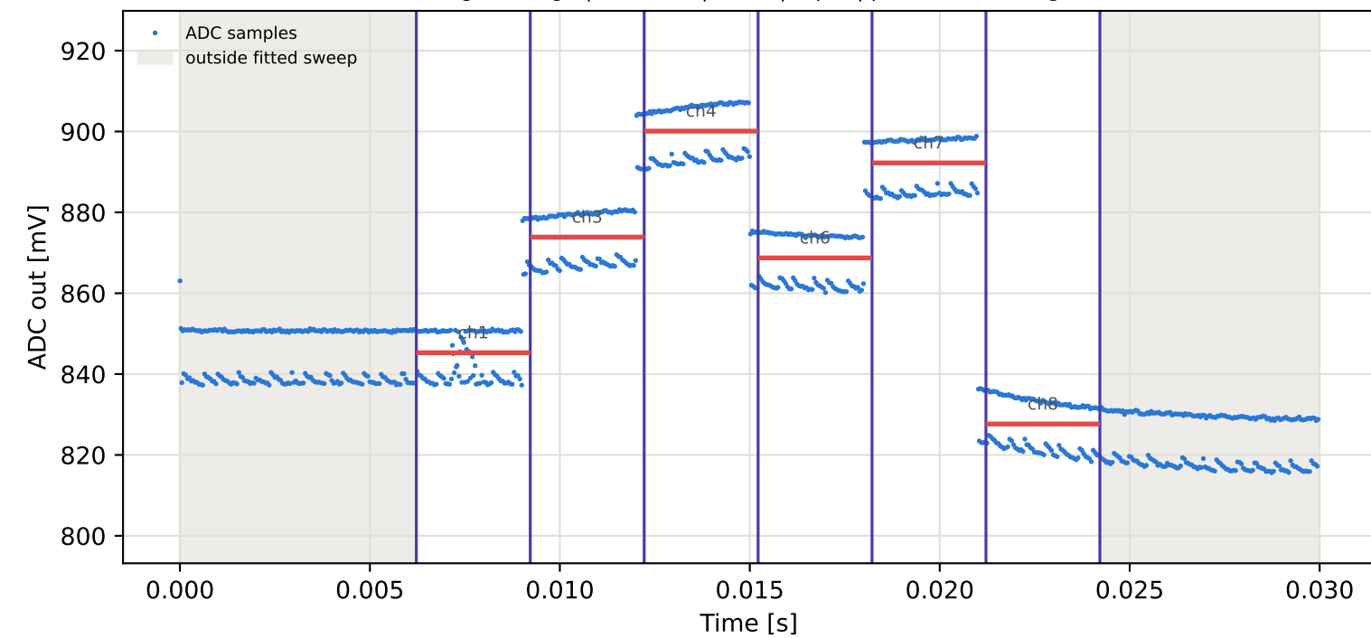
Tag9 &lt;- Tag5 | 905 MHz | run 0 | rep 1 | phase -40.72 deg
