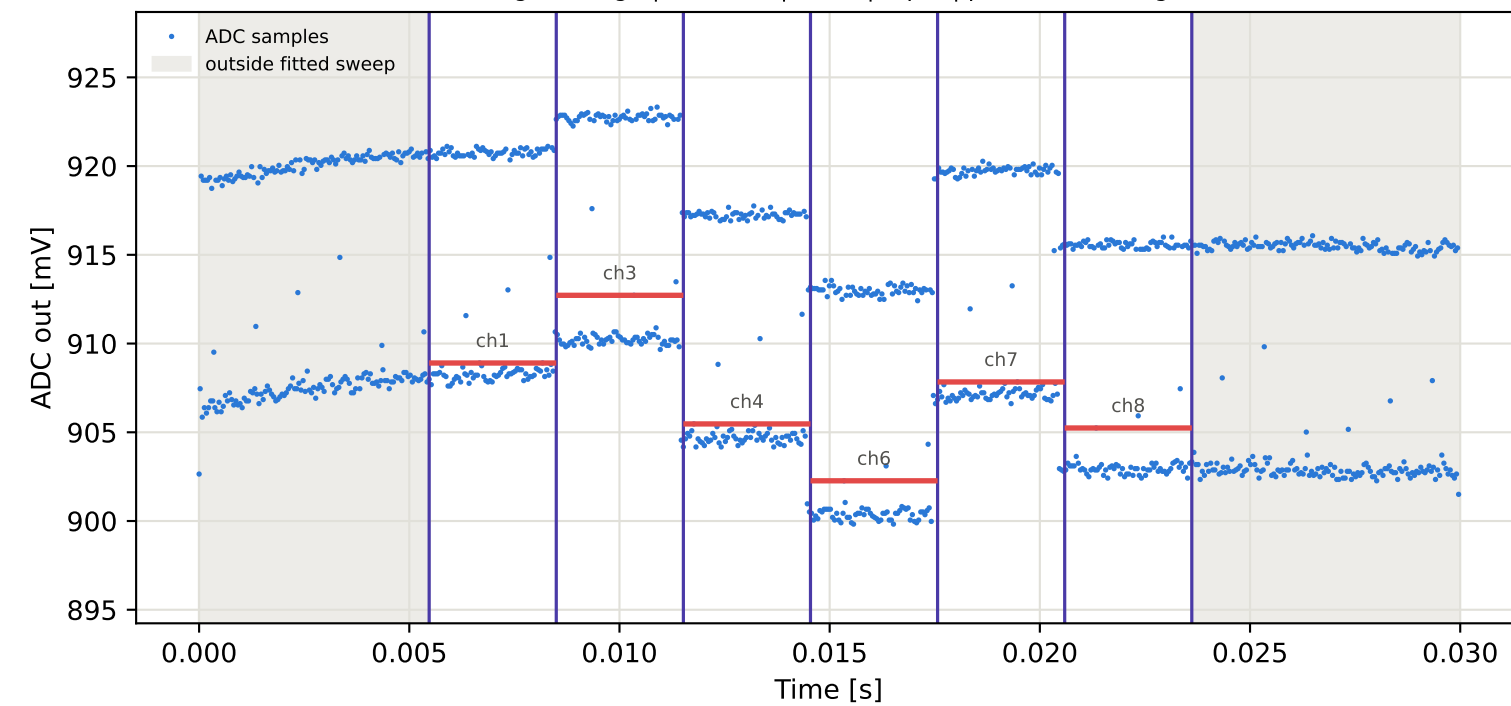
Tag9 &lt;- Tag10 | 865 MHz | run 0 | rep 1 | phase -175.44 deg
