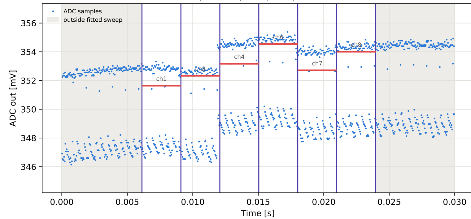
Tag9 &lt;- Tag10 | 805 MHz | run 0 | rep 1 | phase 63.64 deg
