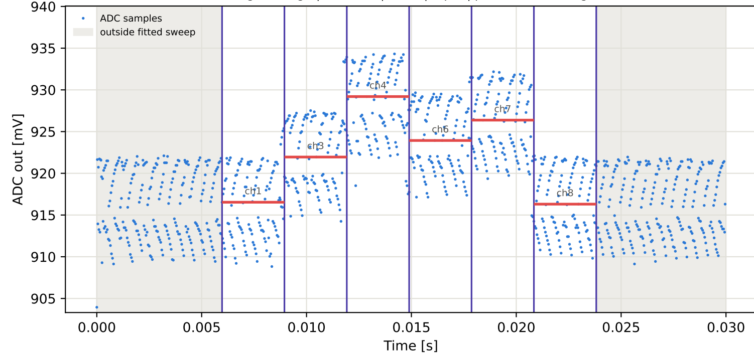
Tag5 &lt;- Tag9 | 925 MHz | run 0 | rep 1 | phase -116.82 deg
