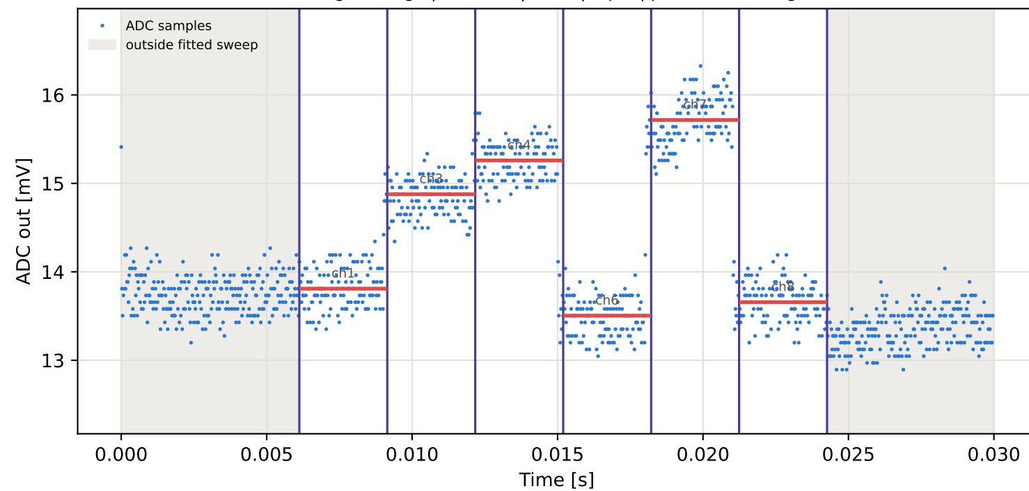
Tag2 &lt;- Tag15 | 795 MHz | run 0 | rep 1 | phase -88.84 deg
