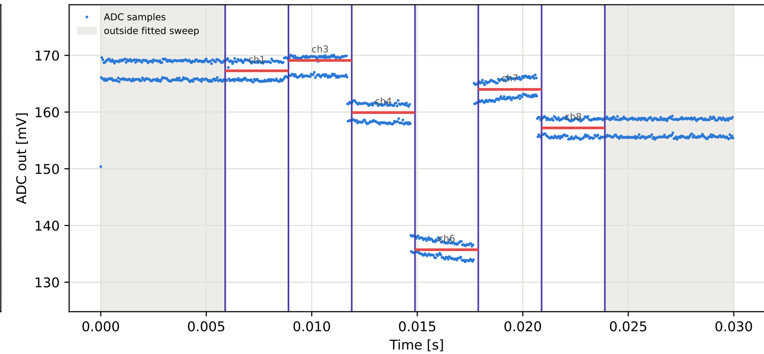
Tag5 &lt;- Tag1 | 935 MHz | run 0 | rep 1 | phase -79.27 deg
