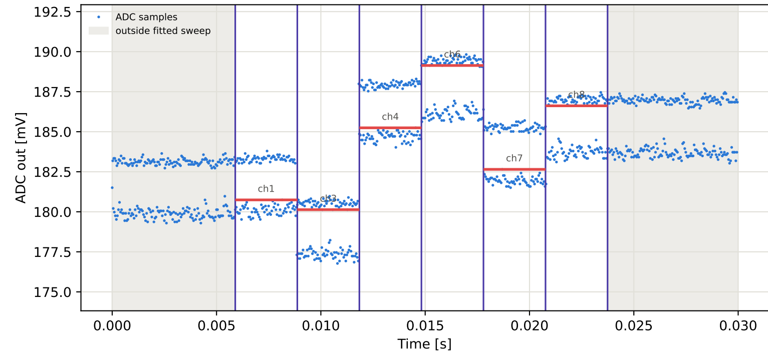
Tag4 &lt;- Tag2 | 825 MHz | run 0 | rep 1 | phase 32.36 deg
