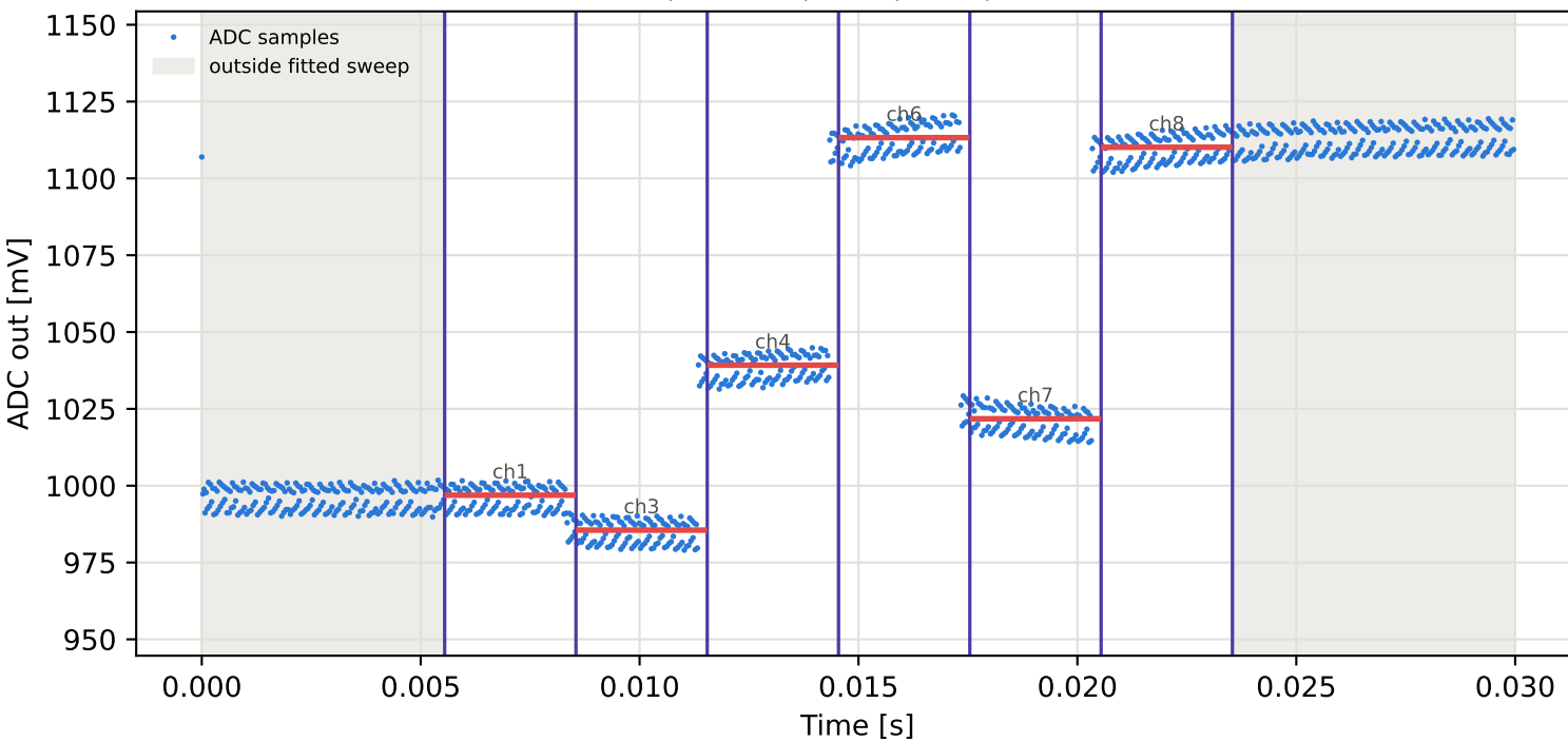
Tag3 &lt;- Tag16 | 875 MHz | run 0 | rep 1 | phase -164.04 deg
