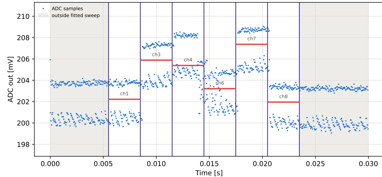
Tag4 &lt;- Tag9 | 805 MHz | run 0 | rep 1 | phase 178.99 deg
