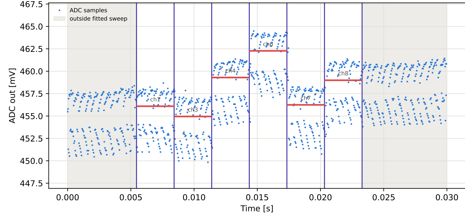
Tag16 &lt;- Tag15 | 995 MHz | run 0 | rep 1 | phase -133.07 deg
