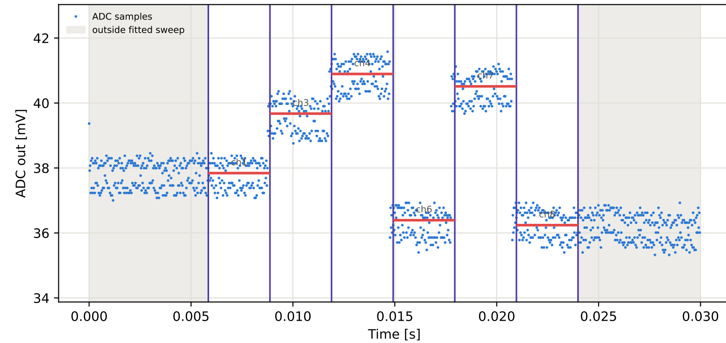
Tag2 &lt;- Tag15 | 955 MHz | run 0 | rep 1 | phase 139.02 deg
