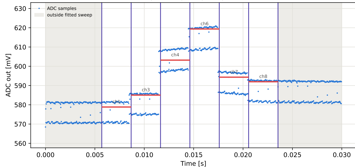
Tag10 &lt;- Tag5 | 945 MHz | run 0 | rep 1 | phase -145.47 deg
