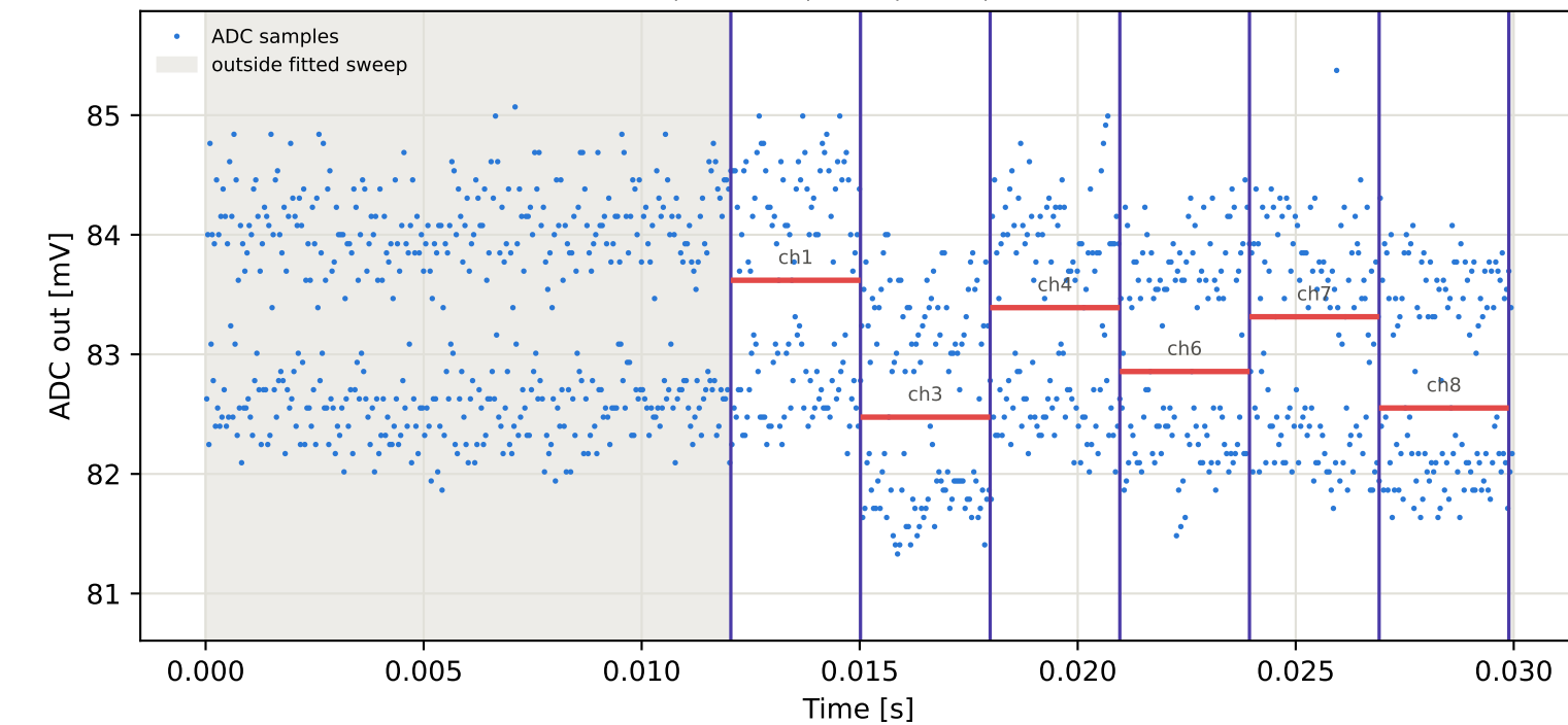
Tag4 &lt;- Tag2 | 985 MHz | run 0 | rep 1 | phase -82.71 deg
