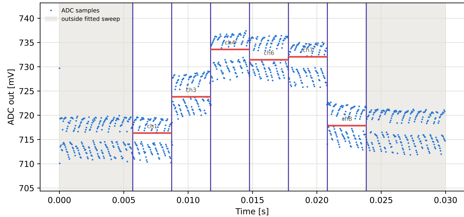
Tag9 &lt;- Tag2 | 895 MHz | run 0 | rep 1 | phase 14.18 deg
