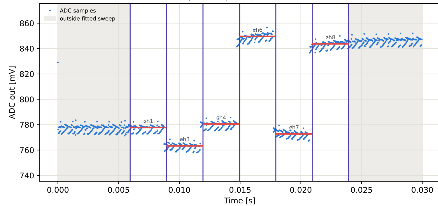
Tag7 &lt;- Tag3 | 895 MHz | run 0 | rep 1 | phase -6.91 deg
