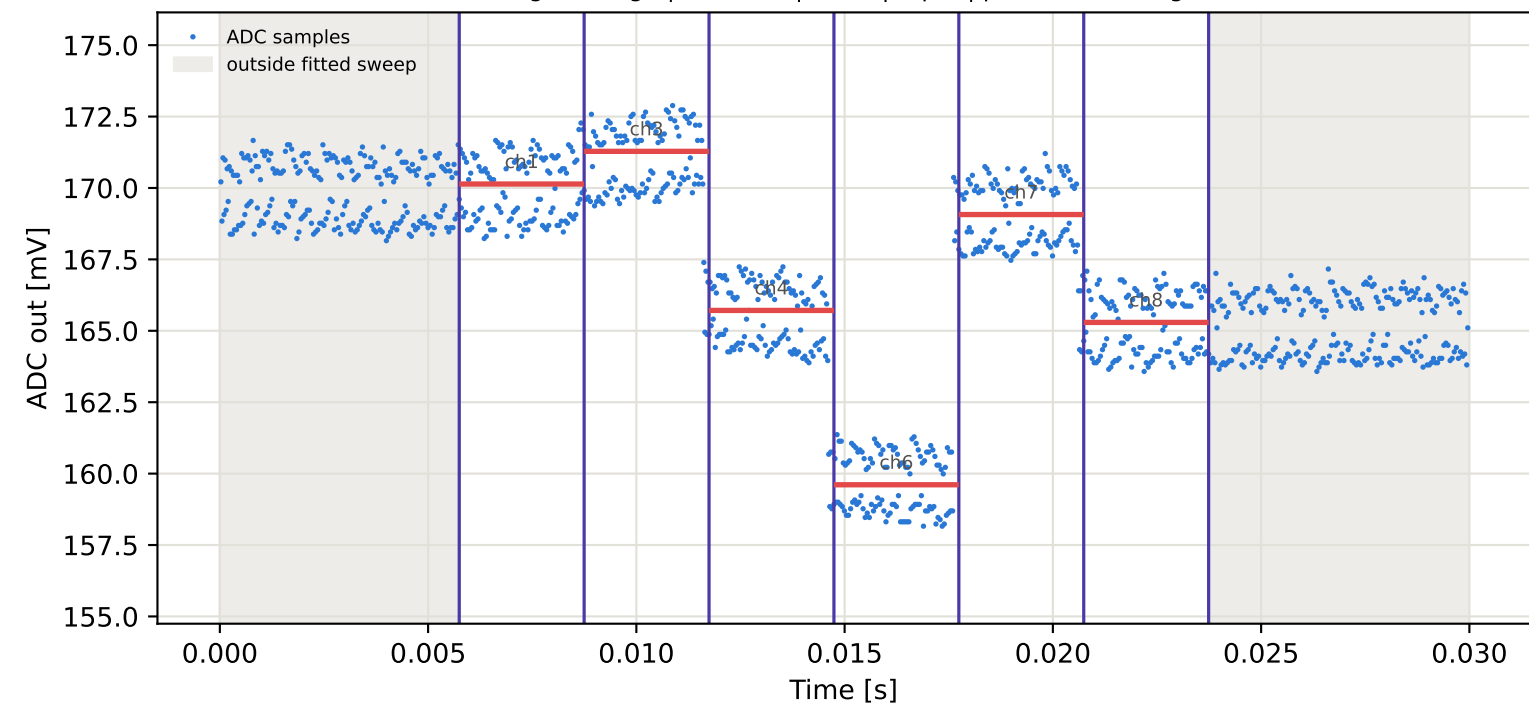
Tag6 &lt;- Tag10 | 995 MHz | run 0 | rep 1 | phase -96.18 deg
