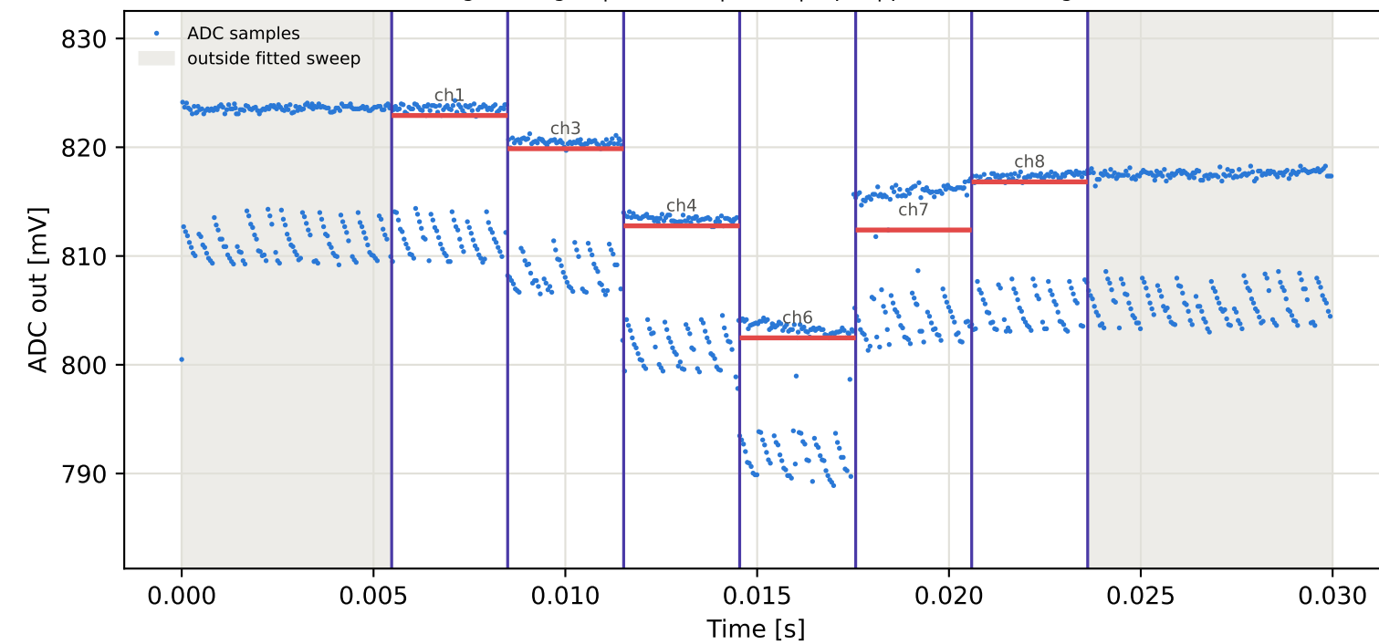
Tag5 &lt;- Tag16 | 905 MHz | run 0 | rep 1 | phase 45.65 deg
