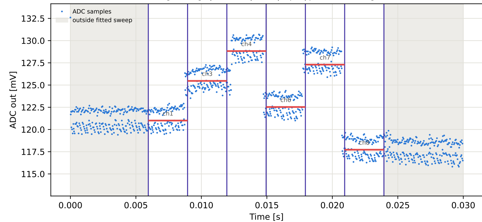
Tag1 &lt;- Tag7 | 915 MHz | run 0 | rep 1 | phase -138.10 deg
