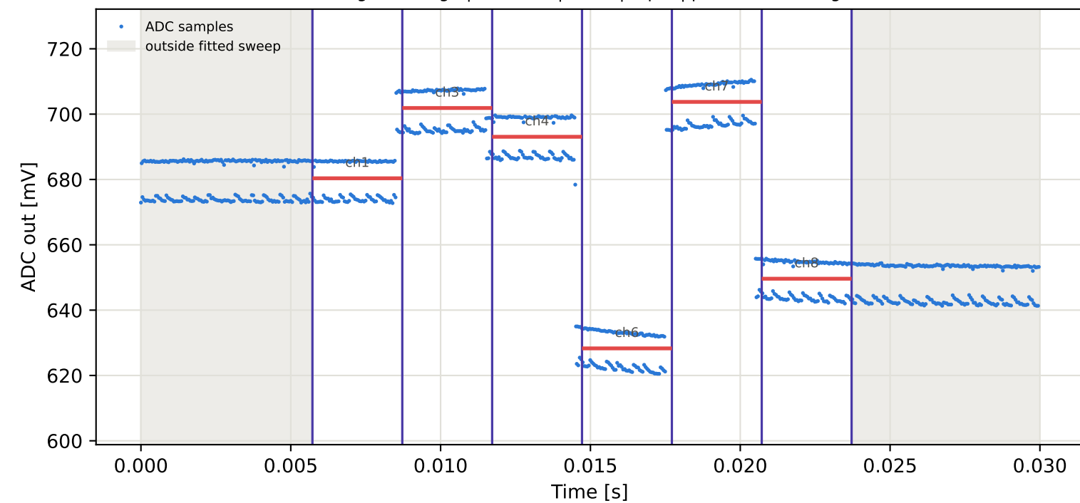
Tag16 &lt;- Tag7 | 975 MHz | run 0 | rep 1 | phase -12.85 deg
