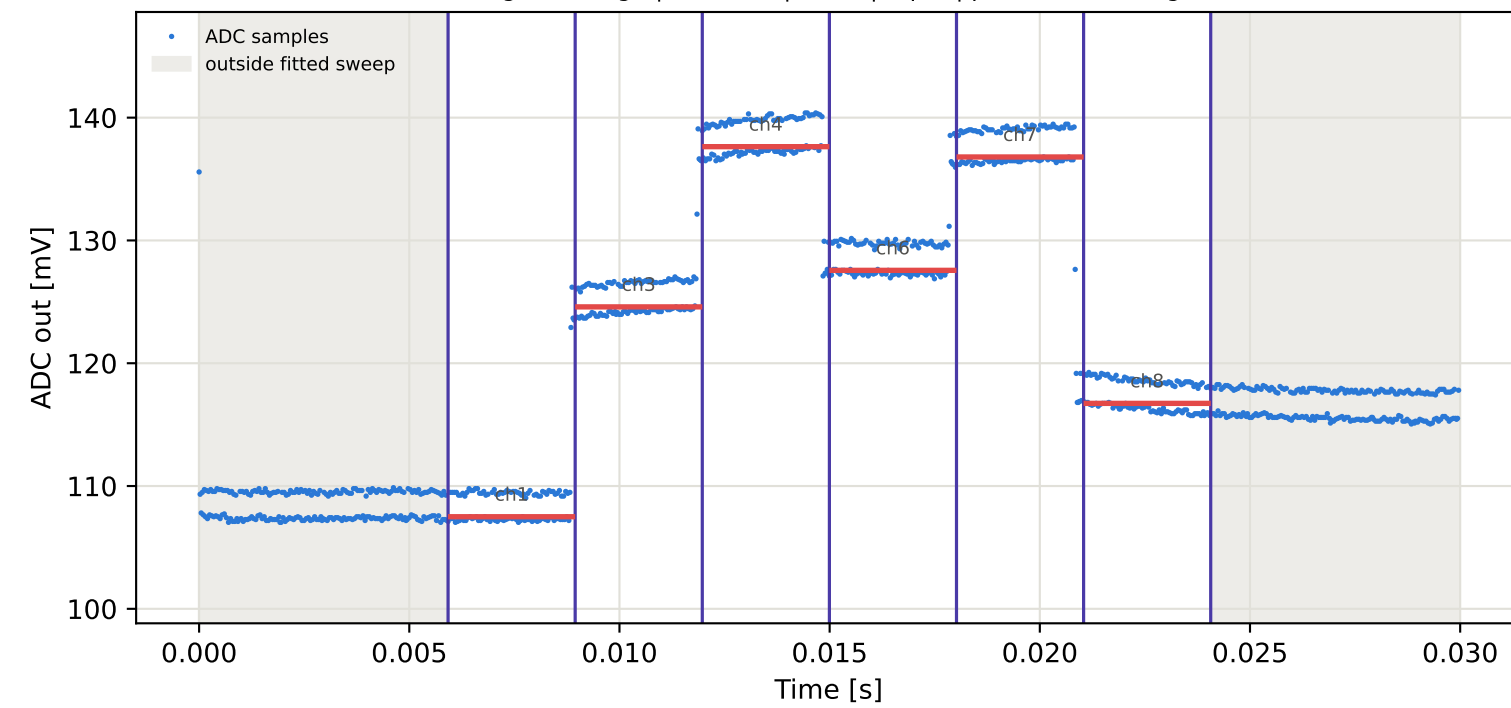
Tag10 &lt;- Tag8 | 835 MHz | run 0 | rep 1 | phase -50.70 deg
