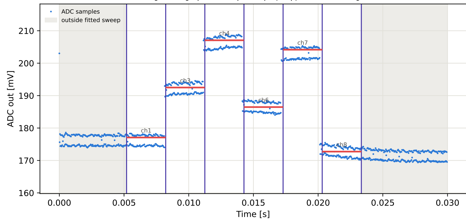
Tag9 &lt;- Tag7 | 855 MHz | run 0 | rep 1 | phase -78.11 deg
