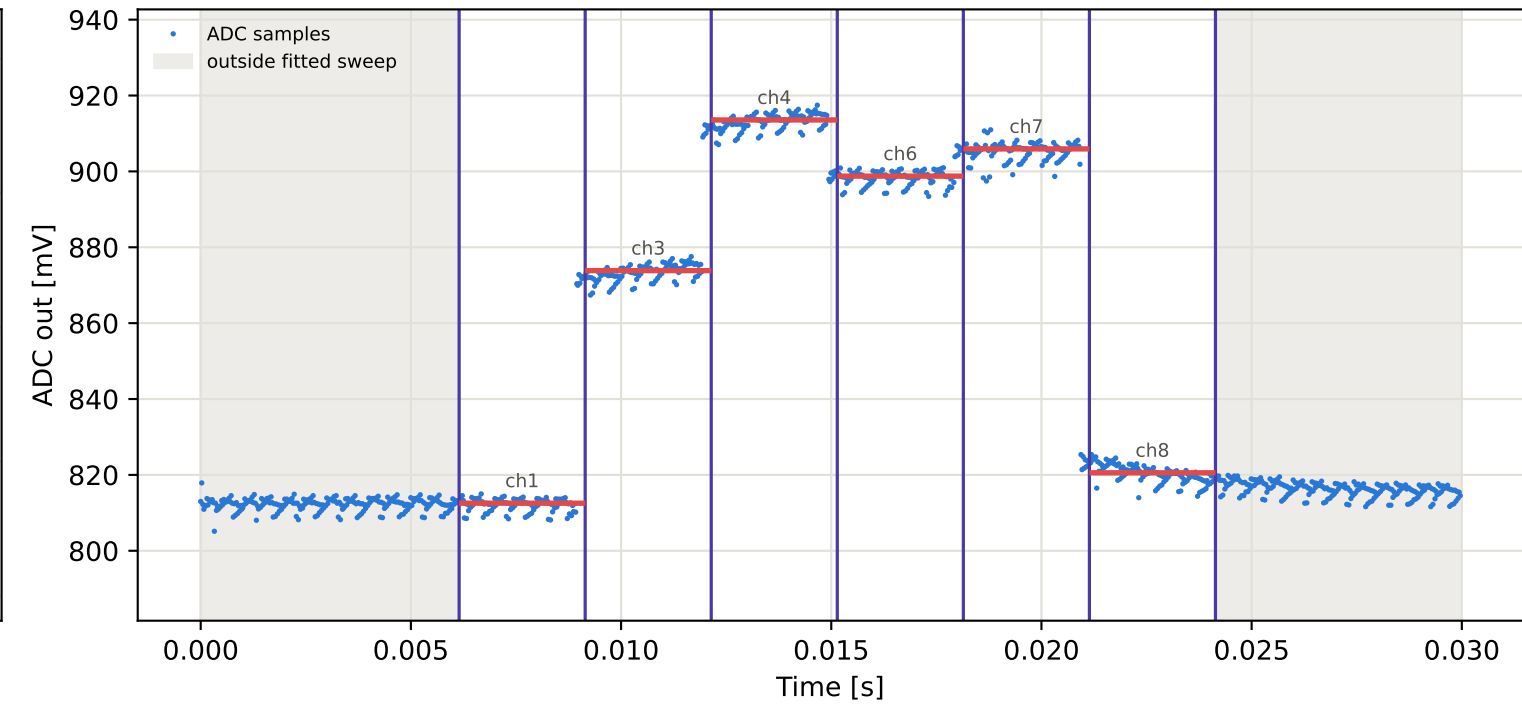
Tag6 &lt;- Tag5 | 875 MHz | run 0 | rep 1 | phase 99.18 deg
