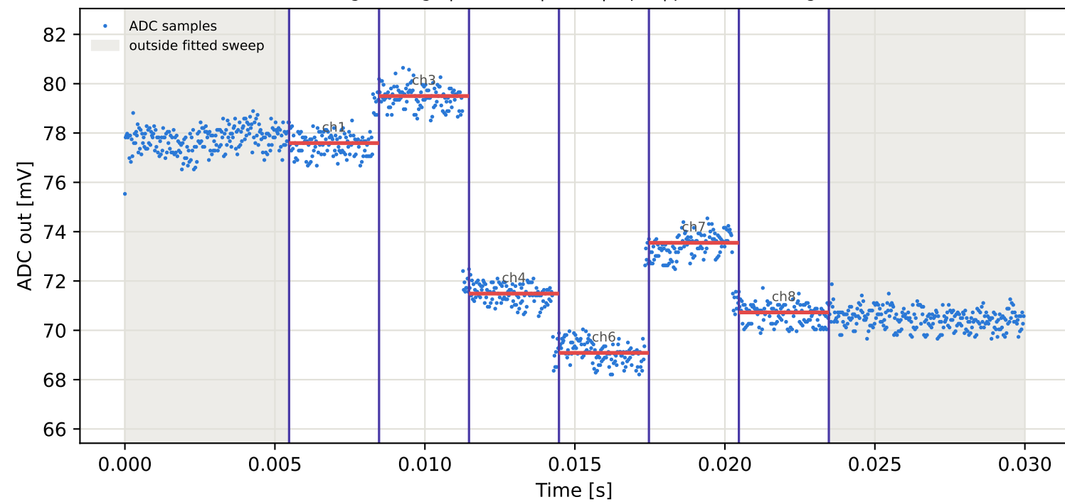
Tag9 &lt;- Tag6 | 835 MHz | run 0 | rep 1 | phase 44.48 deg
