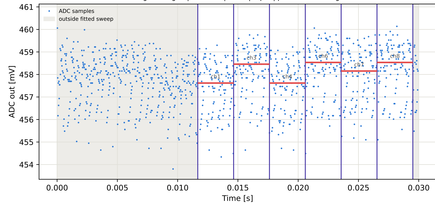
Tag5 &lt;- Tag16 | 845 MHz | run 0 | rep 1 | phase -85.86 deg
