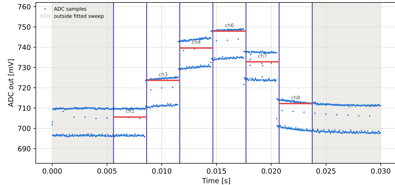
Tag3 &lt;- Tag16 | 905 MHz | run 0 | rep 1 | phase -126.18 deg
