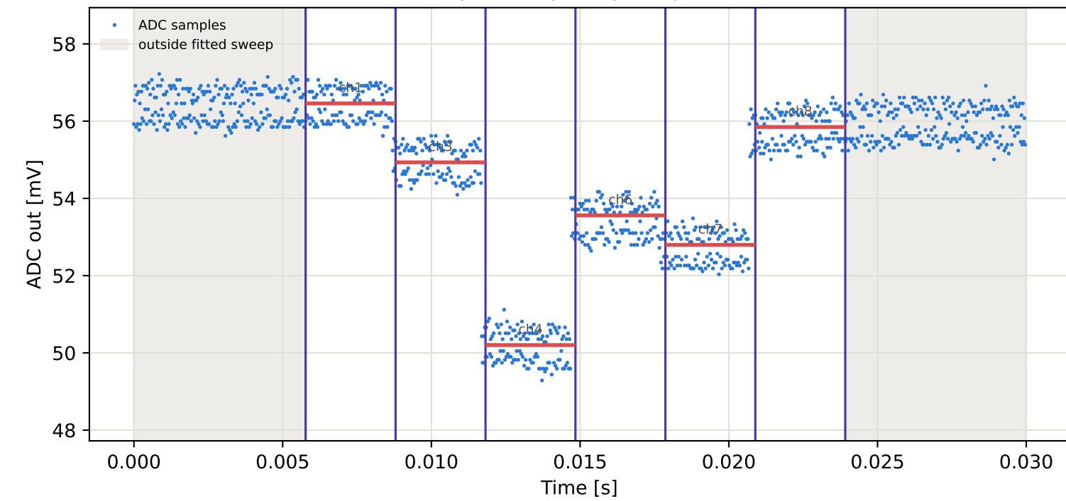
Tag2 &lt;- Tag16 | 975 MHz | run 0 | rep 1 | phase 67.60 deg
