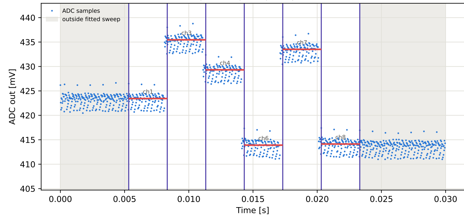
Tag3 &lt;- Tag9 | 825 MHz | run 0 | rep 1 | phase -8.05 deg
