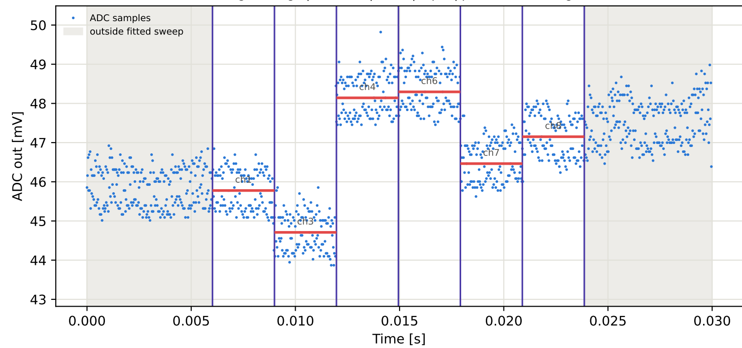
Tag9 &lt;- Tag15 | 805 MHz | run 0 | rep 1 | phase -21.77 deg
