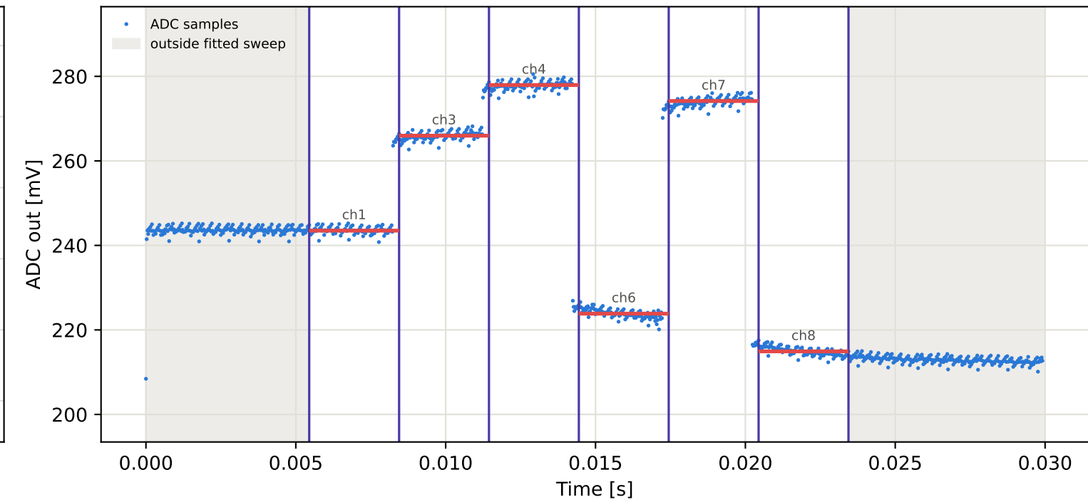
Tag3 &lt;- Tag2 | 925 MHz | run 0 | rep 1 | phase -174.72 deg
