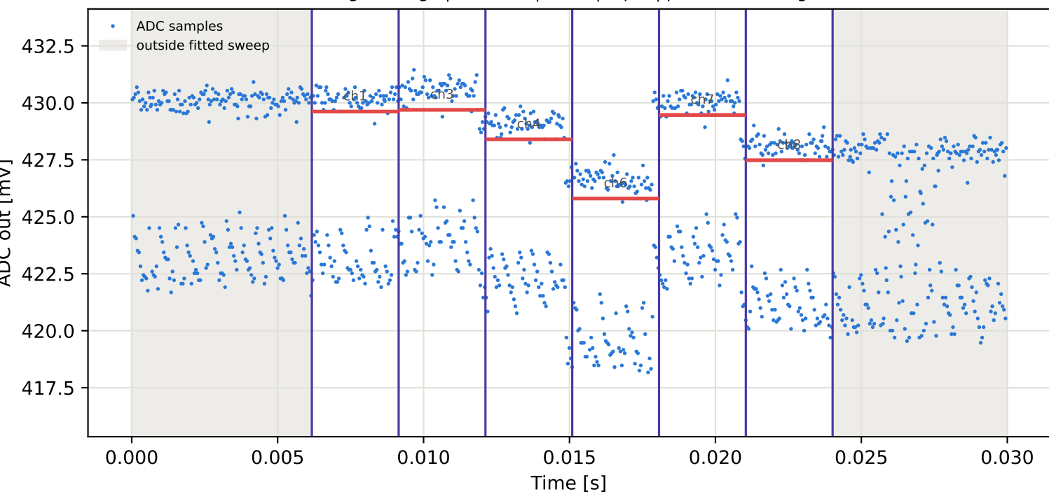
Tag2 &lt;- Tag7 | 905 MHz | run 0 | rep 1 | phase 16.44 deg
