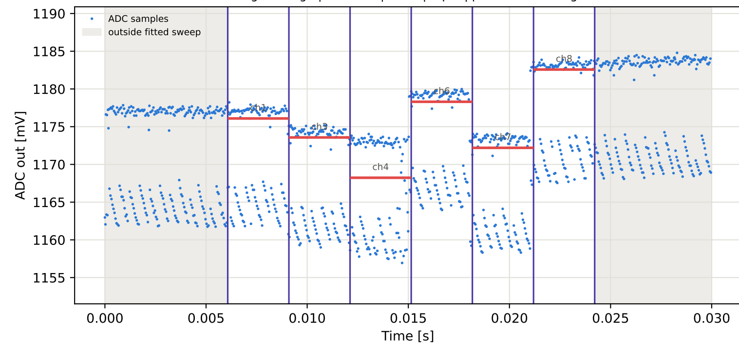
Tag8 &lt;- Tag4 | 895 MHz | run 0 | rep 1 | phase -84.79 deg
