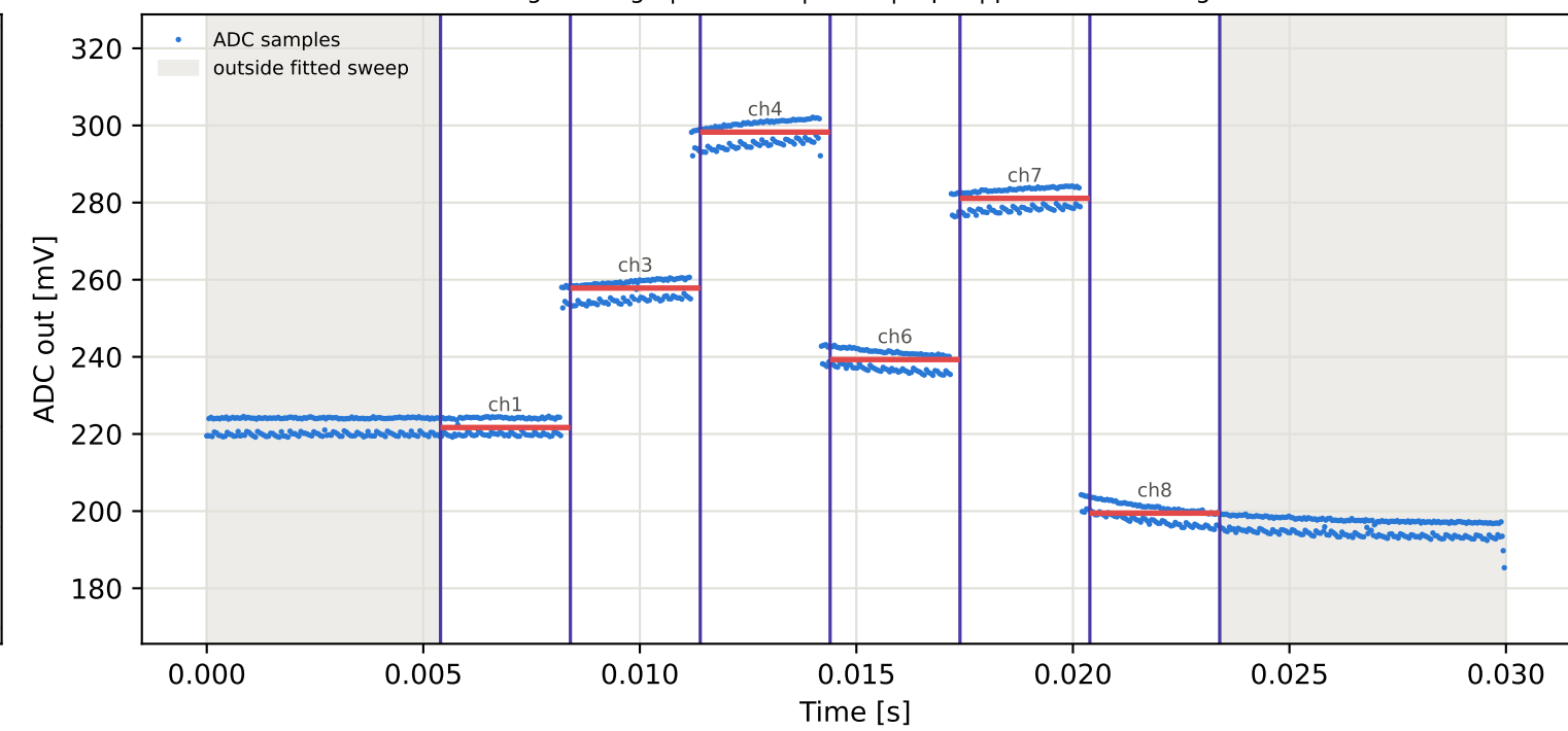
Tag3 &lt;- Tag7 | 925 MHz | run 0 | rep 1 | phase -155.88 deg
