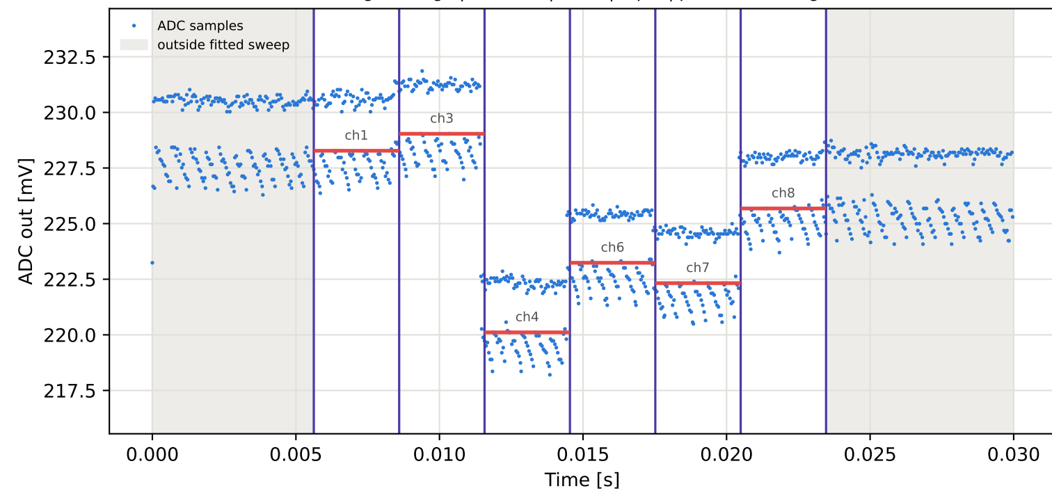
Tag8 &lt;- Tag7 | 775 MHz | run 0 | rep 1 | phase -1.51 deg
