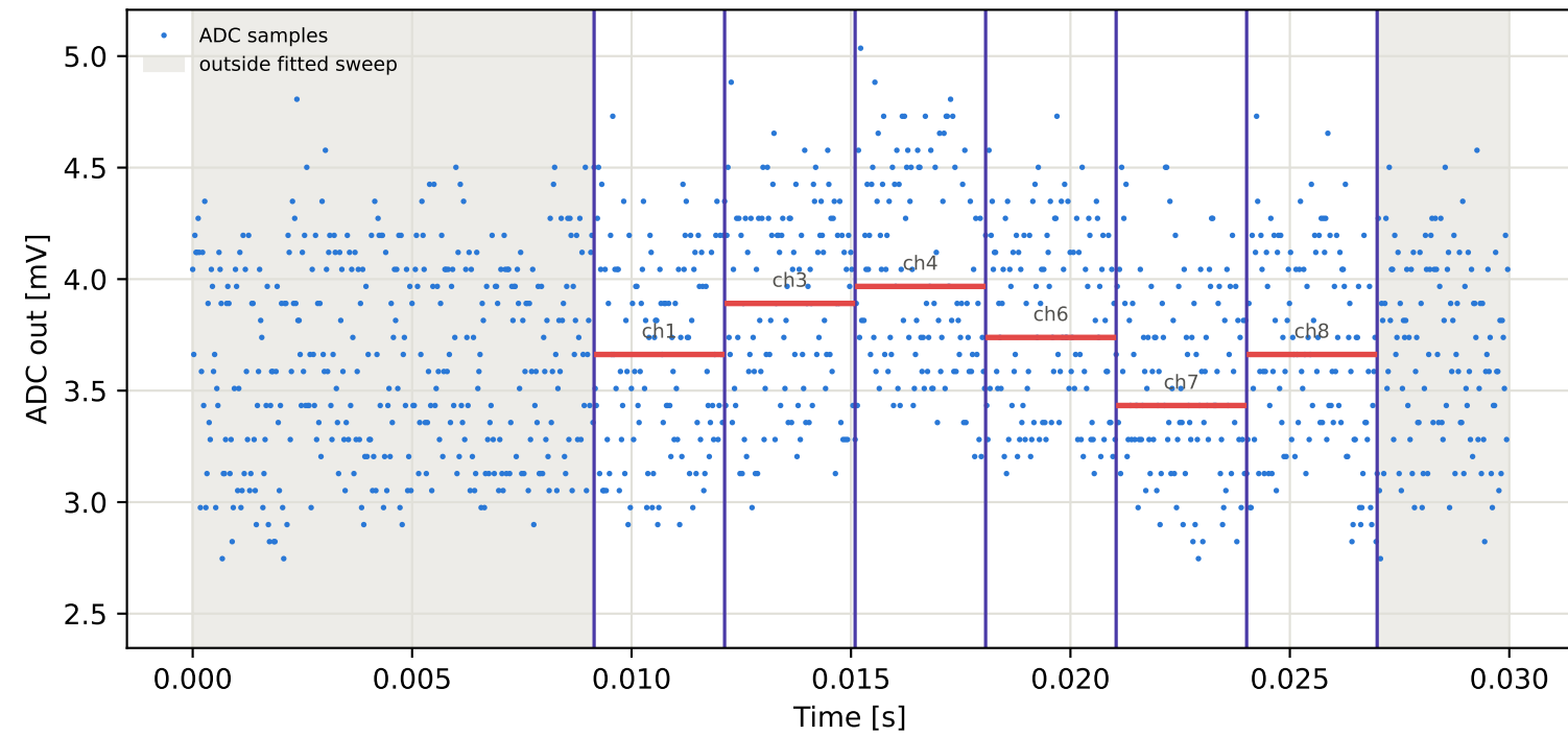
Tag1 &lt;- Tag4 | 785 MHz | run 0 | rep 1 | phase -136.16 deg
