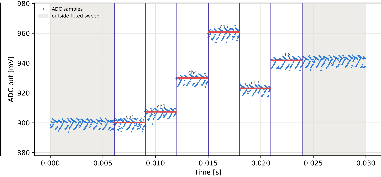
Tag8 &lt;- Tag5 | 875 MHz | run 0 | rep 1 | phase -106.56 deg
