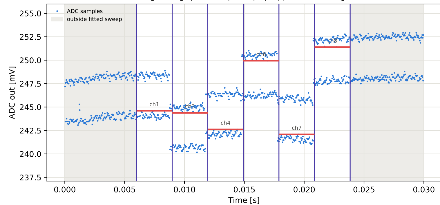
Tag5 &lt;- Tag8 | 855 MHz | run 0 | rep 1 | phase -3.95 deg
