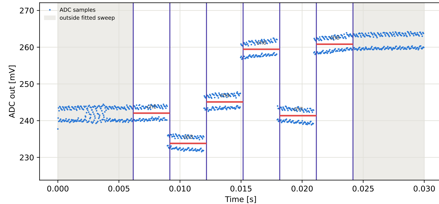
Tag1 &lt;- Tag3 | 865 MHz | run 0 | rep 1 | phase -122.31 deg
