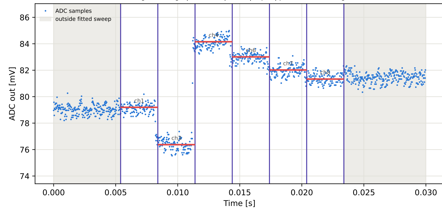
Tag15 &lt;- Tag5 | 795 MHz | run 0 | rep 1 | phase -120.18 deg
