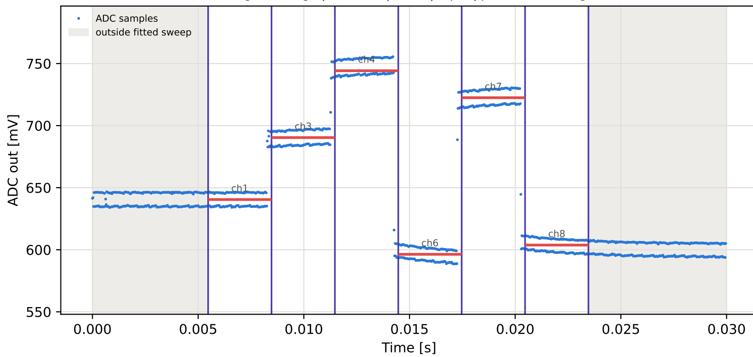
Tag2 &lt;- Tag1 | 975 MHz | run 0 | rep 1 | phase 53.24 deg
