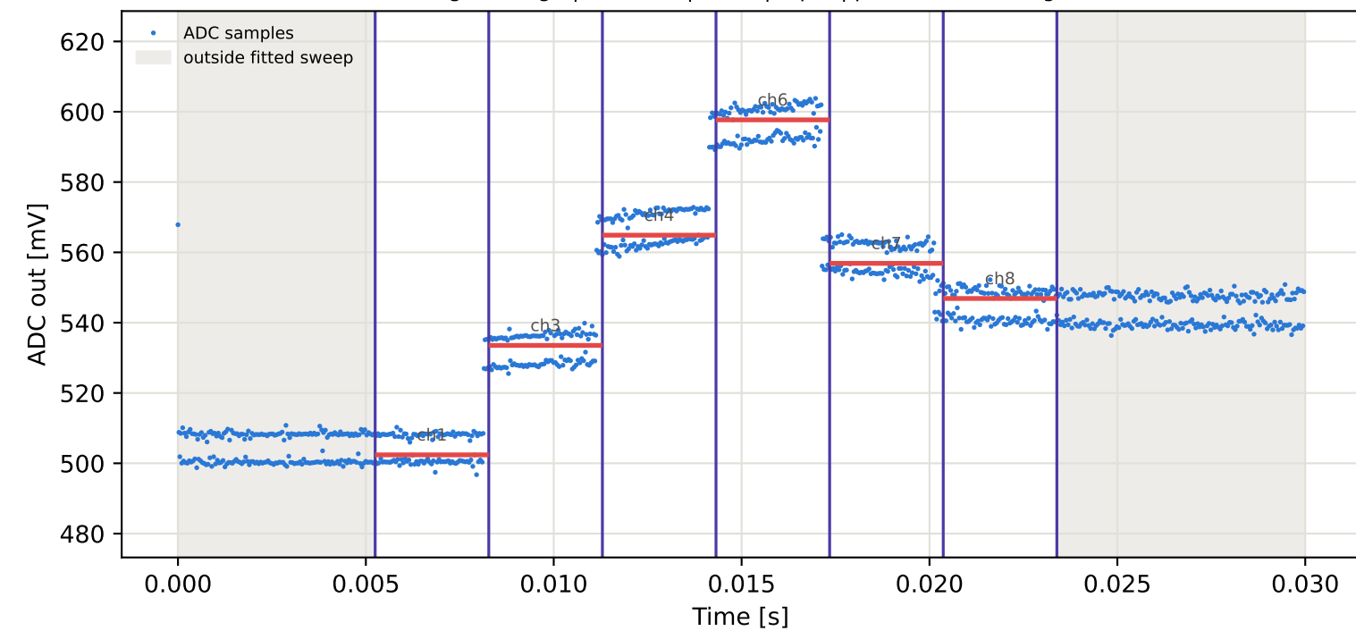
Tag2 &lt;- Tag7 | 885 MHz | run 0 | rep 1 | phase 11.33 deg
