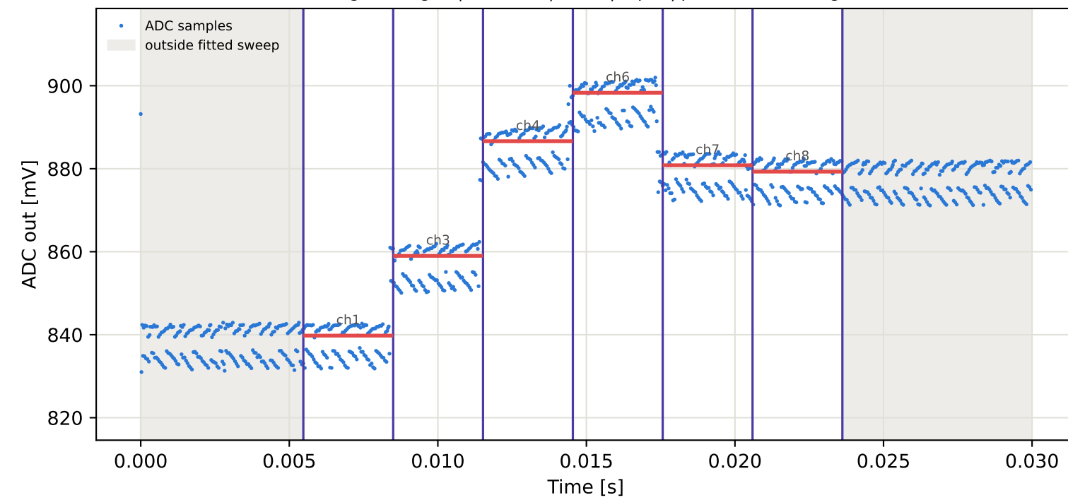
Tag6 &lt;- Tag2 | 875 MHz | run 0 | rep 1 | phase -119.65 deg
