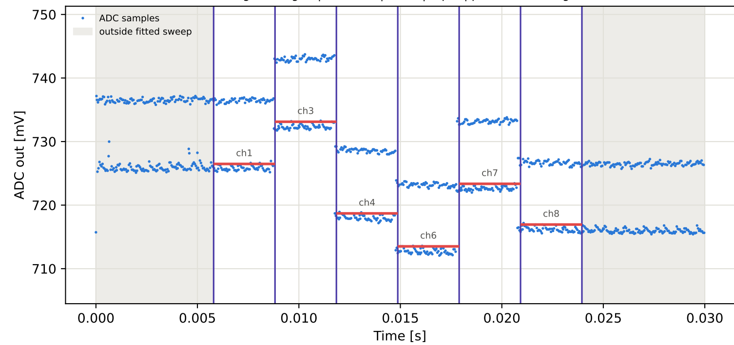
Tag7 &lt;- Tag15 | 845 MHz | run 0 | rep 1 | phase 35.09 deg
