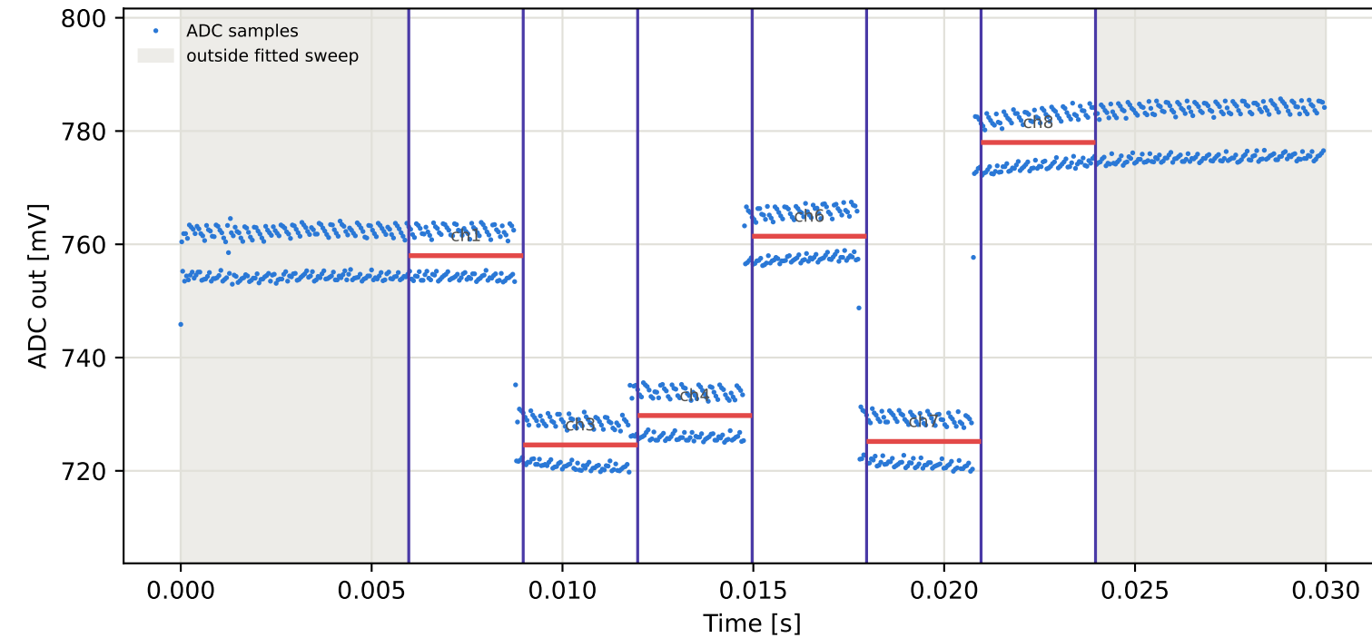
Tag3 &lt;- Tag8 | 855 MHz | run 0 | rep 1 | phase -98.02 deg
