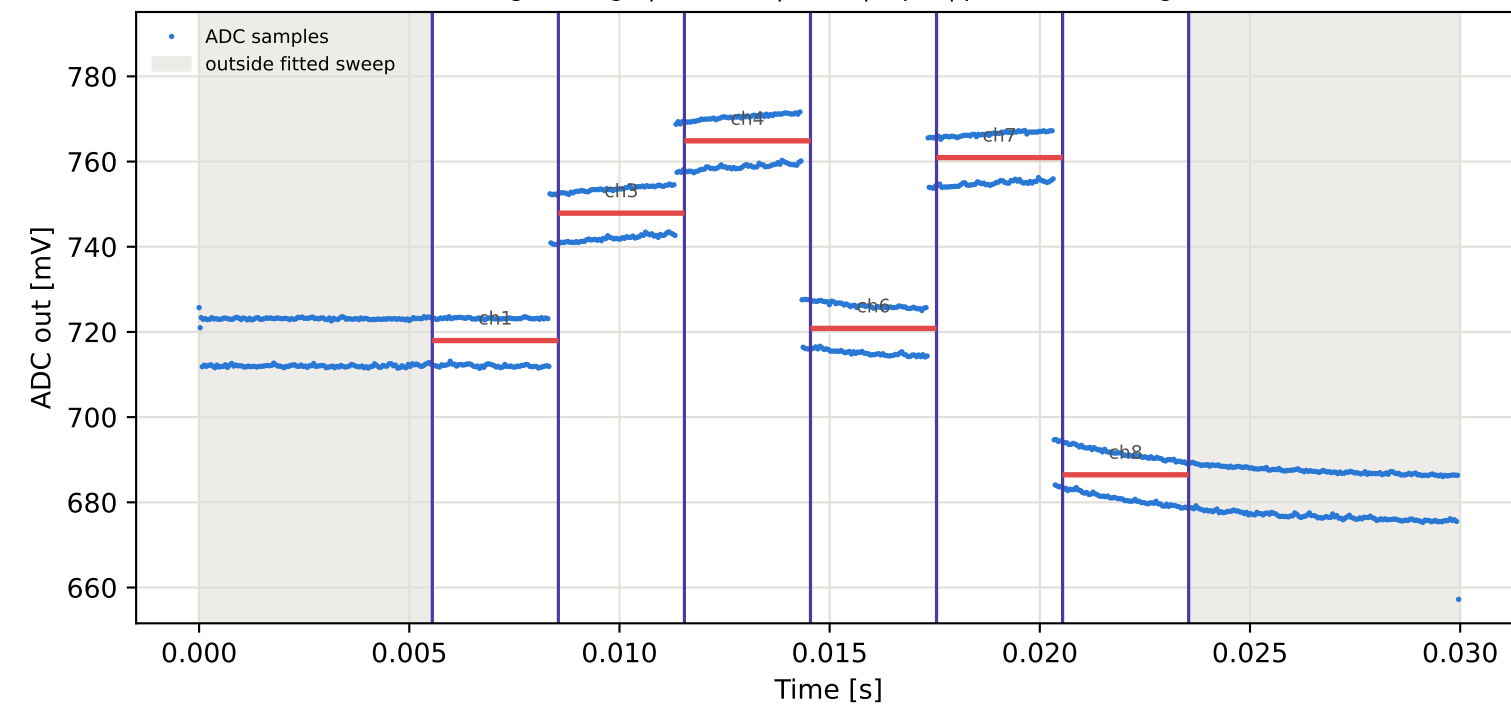
Tag9 &lt;- Tag5 | 895 MHz | run 0 | rep 1 | phase -53.79 deg
