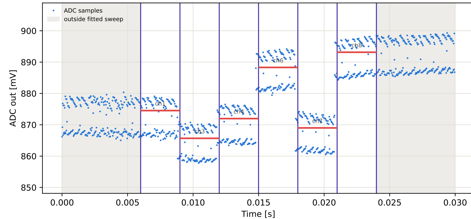
Tag6 &lt;- Tag1 | 875 MHz | run 0 | rep 1 | phase 1.42 deg
