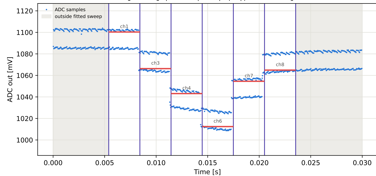
Tag2 &lt;- Tag10 | 915 MHz | run 0 | rep 1 | phase 75.99 deg
