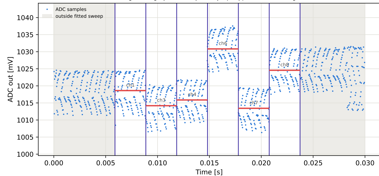
Tag8 &lt;- Tag6 | 975 MHz | run 0 | rep 1 | phase 167.68 deg
