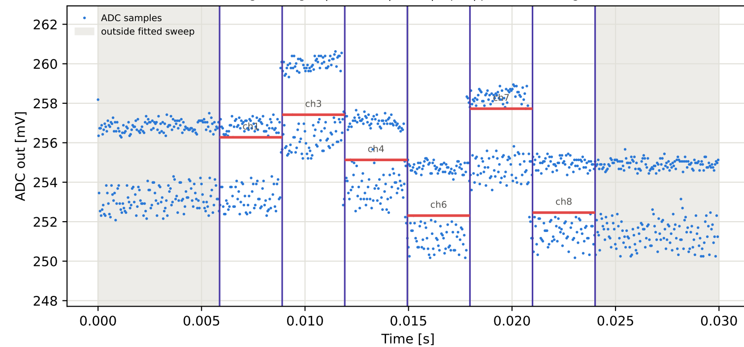
Tag1 &lt;- Tag16 | 825 MHz | run 0 | rep 1 | phase -174.99 deg
