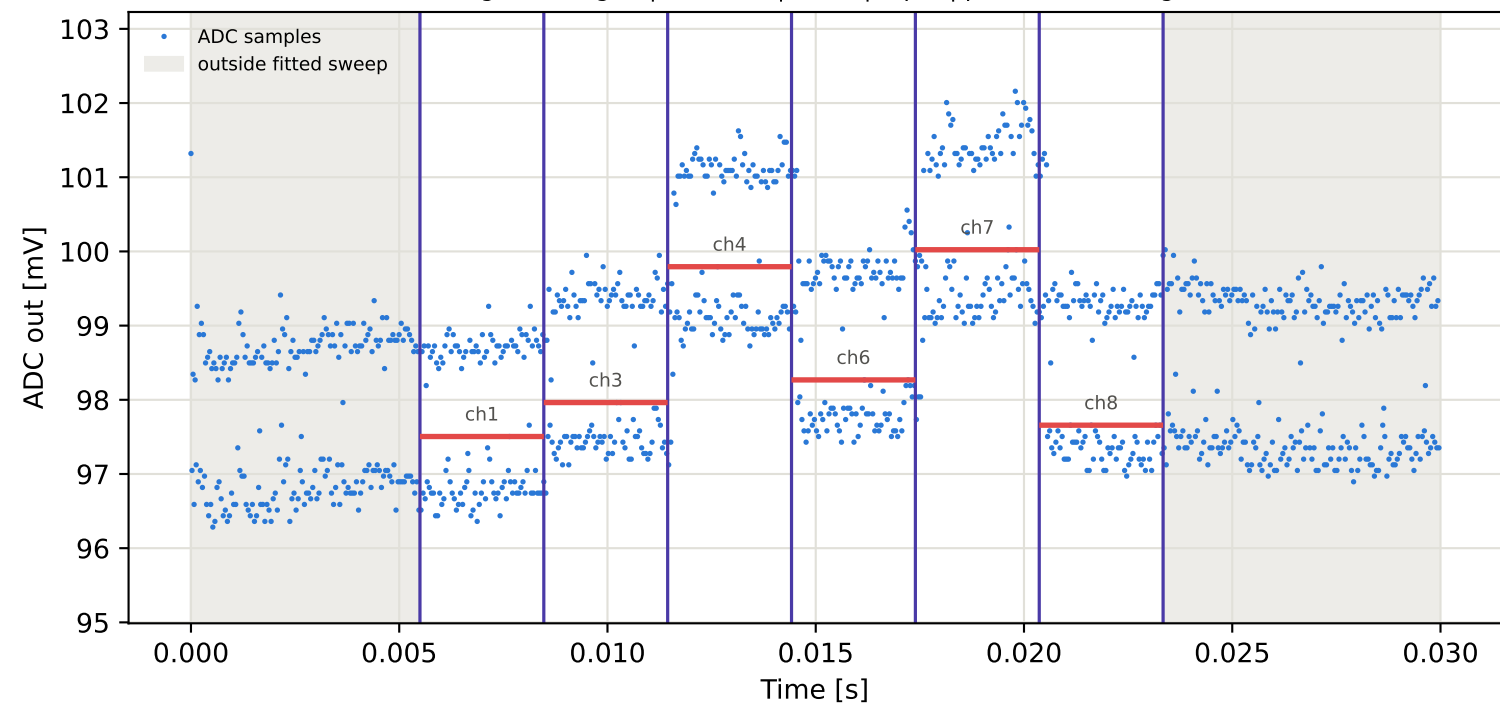
Tag15 &lt;- Tag3 | 785 MHz | run 0 | rep 1 | phase -149.62 deg
