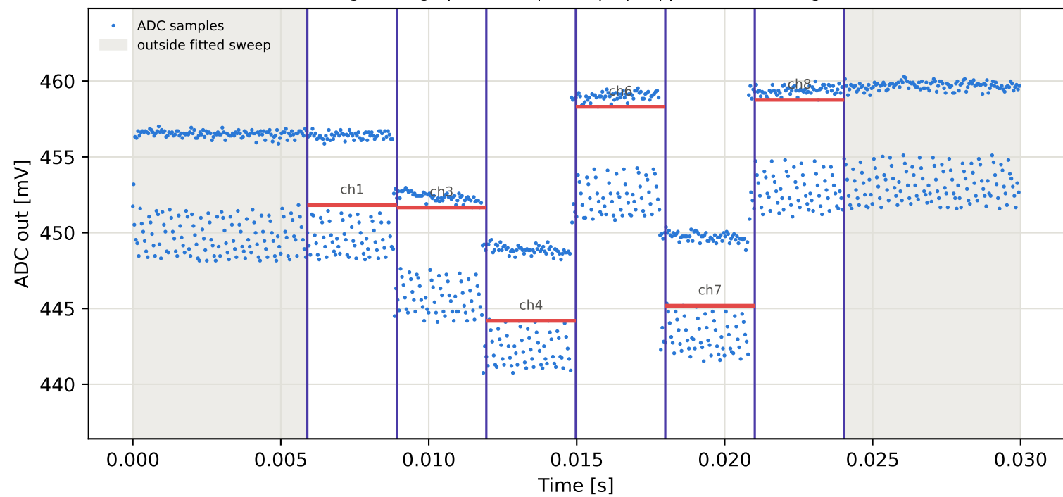
Tag3 &lt;- Tag15 | 935 MHz | run 0 | rep 1 | phase -51.75 deg
