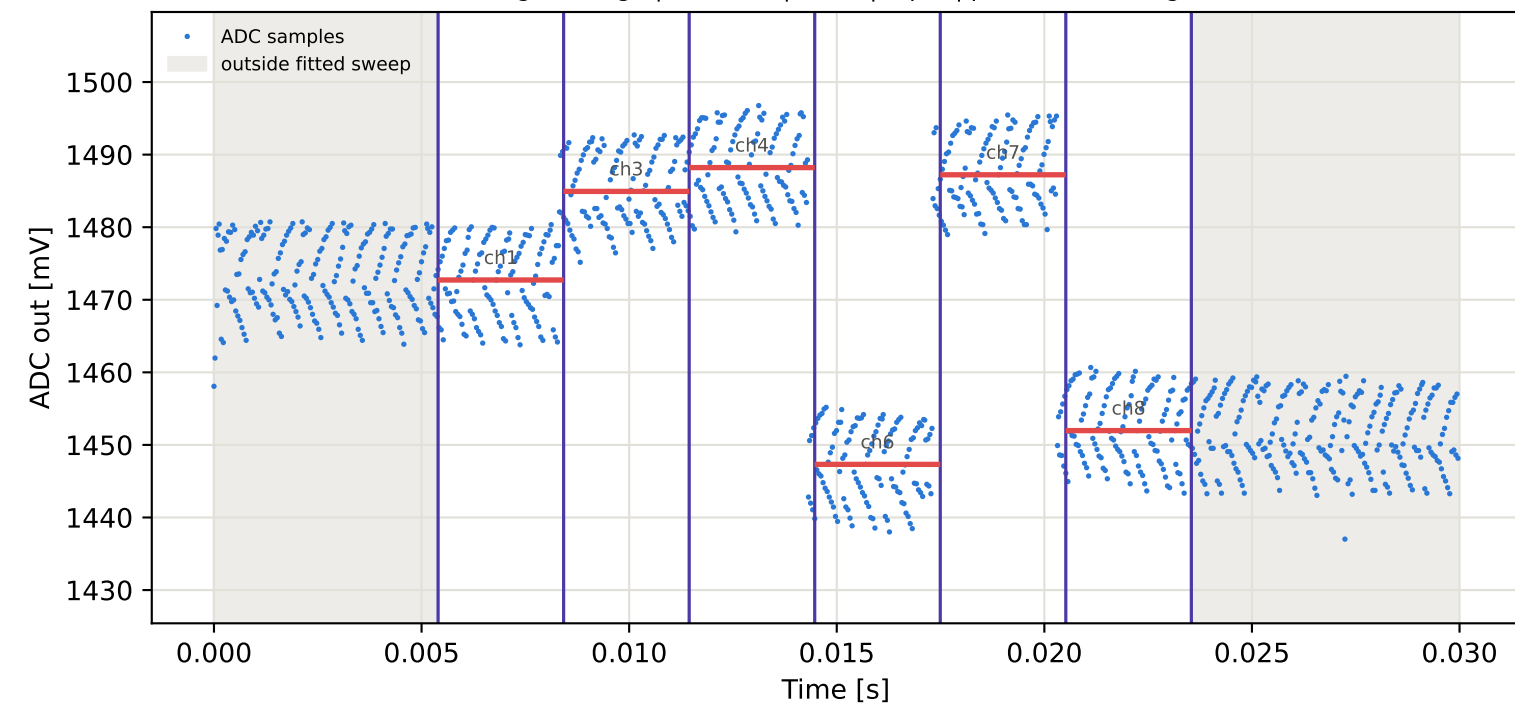
Tag8 &lt;- Tag5 | 915 MHz | run 0 | rep 1 | phase 113.03 deg
