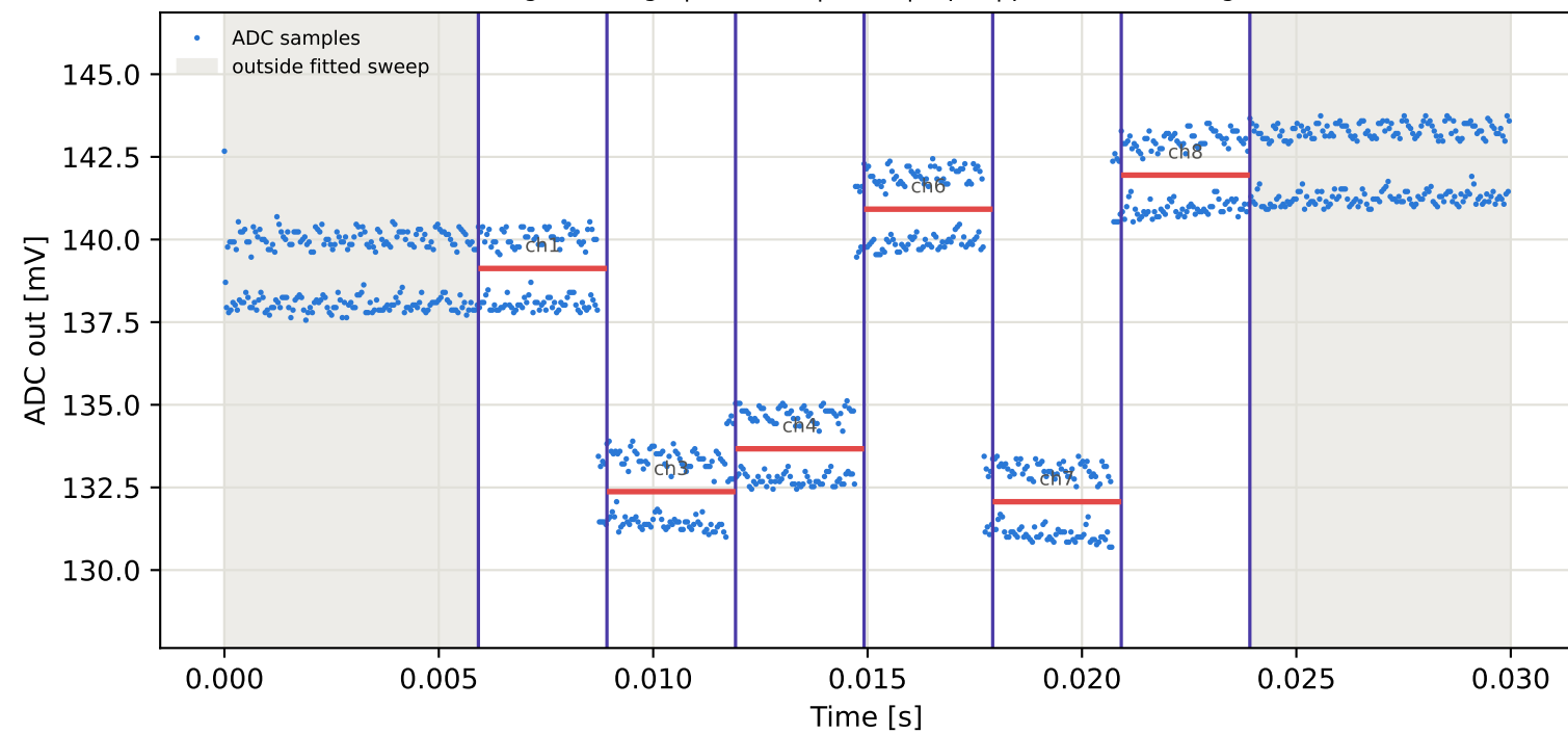
Tag10 &lt;- Tag9 | 805 MHz | run 0 | rep 1 | phase -160.40 deg
