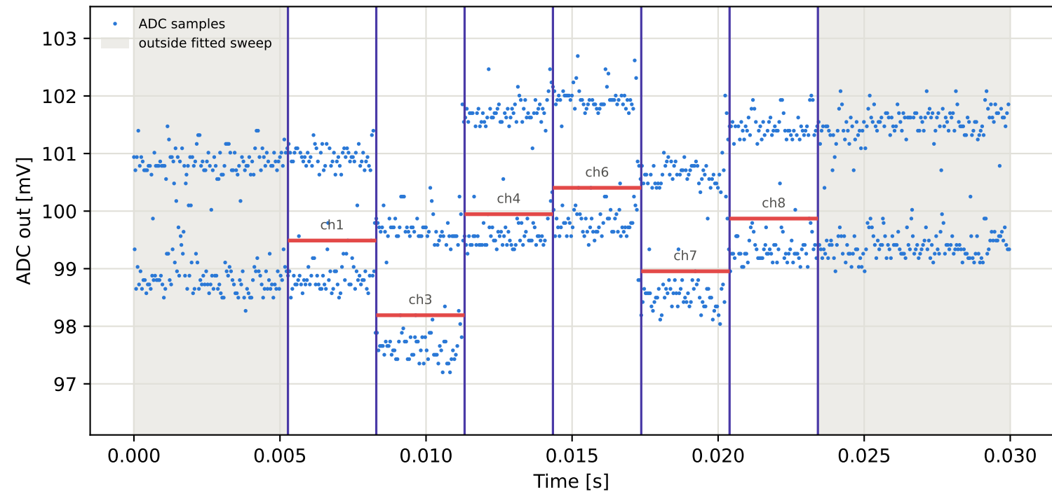
Tag15 &lt;- Tag5 | 785 MHz | run 0 | rep 1 | phase -138.78 deg
