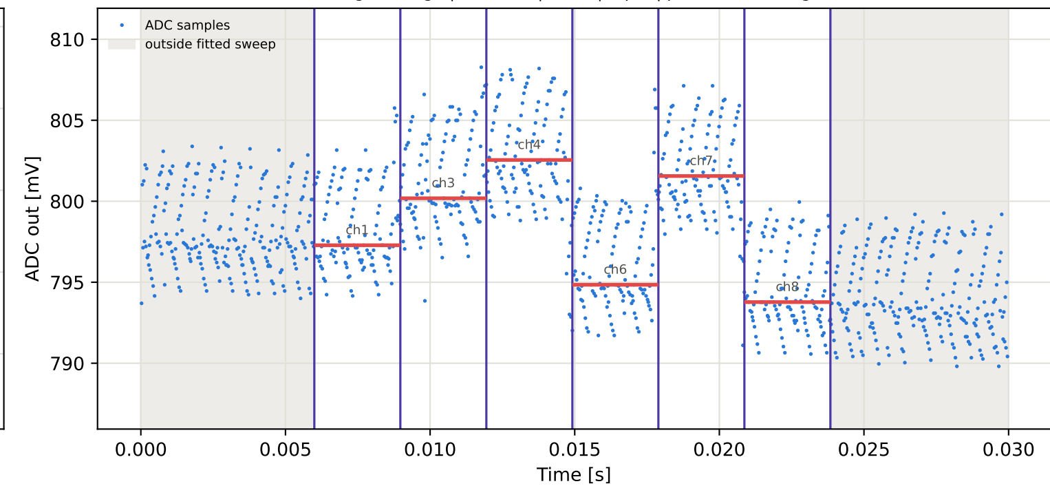
Tag9 &lt;- Tag6 | 925 MHz | run 0 | rep 1 | phase -174.65 deg
