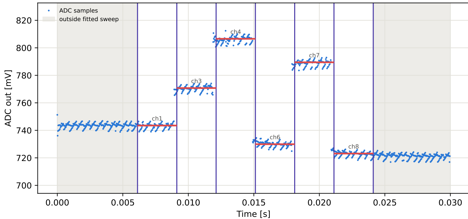
Tag6 &lt;- Tag1 | 945 MHz | run 0 | rep 1 | phase 148.27 deg
