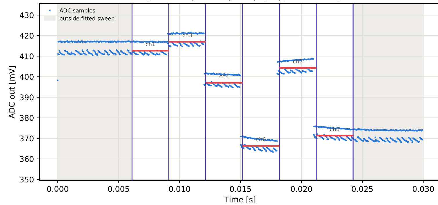
Tag10 &lt;- Tag8 | 865 MHz | run 0 | rep 1 | phase 41.90 deg
