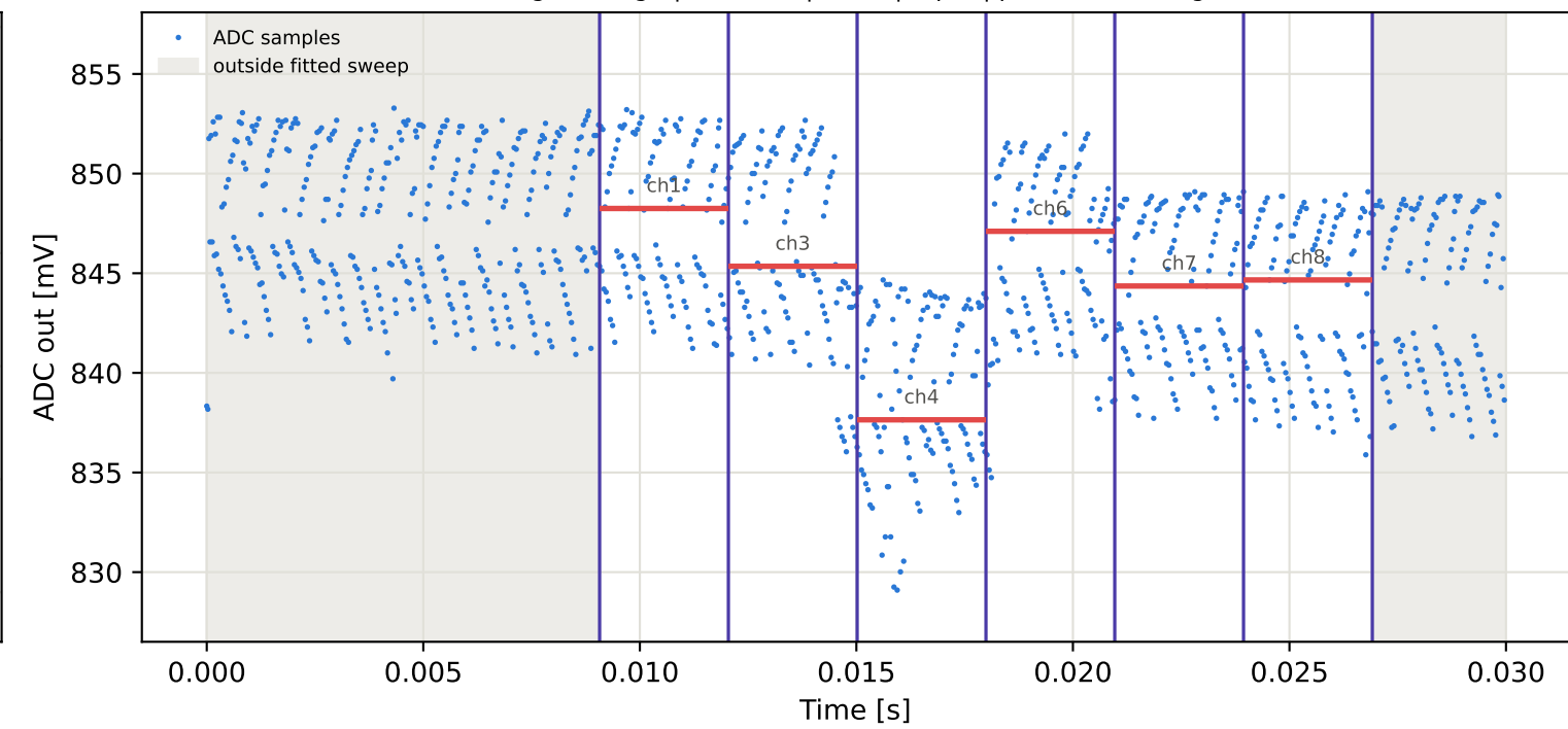
Tag7 &lt;- Tag4 | 935 MHz | run 0 | rep 1 | phase 91.66 deg
