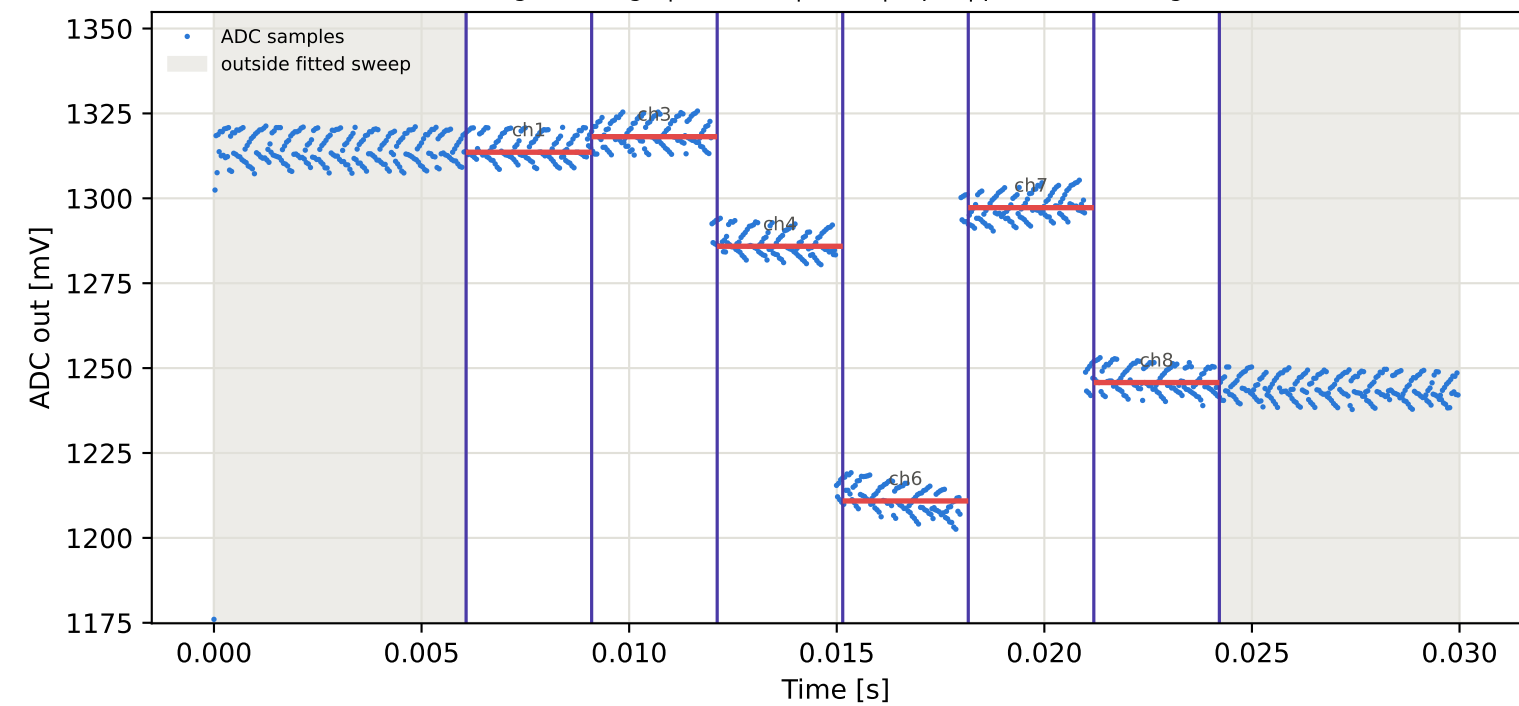
Tag2 &lt;- Tag10 | 905 MHz | run 0 | rep 1 | phase 144.08 deg
