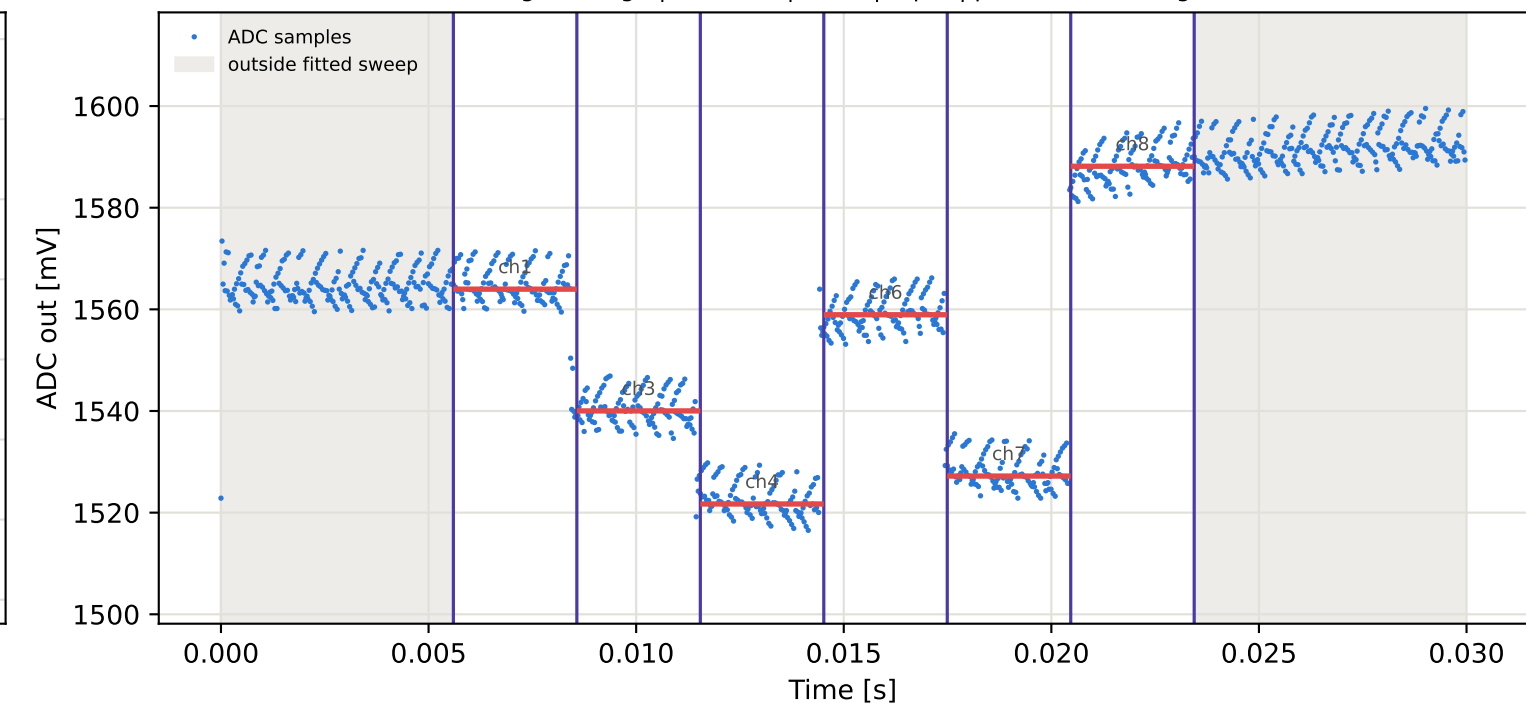
Tag8 &lt;- Tag7 | 905 MHz | run 0 | rep 1 | phase -70.86 deg
