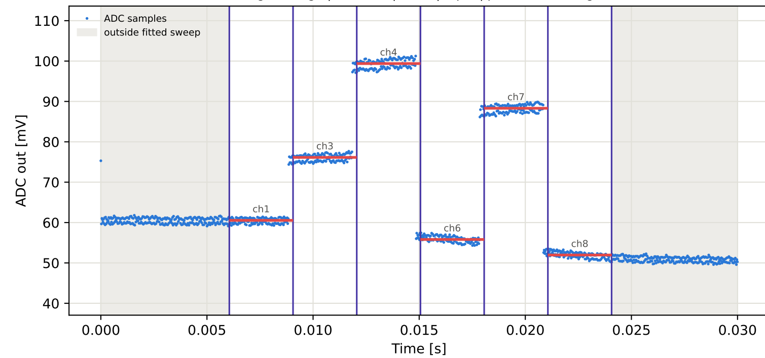
Tag4 &lt;- Tag7 | 985 MHz | run 0 | rep 1 | phase -118.39 deg
