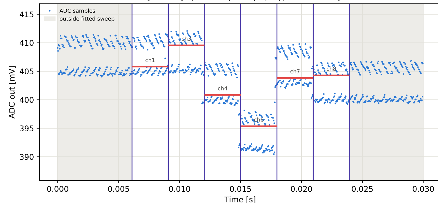
Tag10 &lt;- Tag4 | 955 MHz | run 0 | rep 1 | phase 29.11 deg
