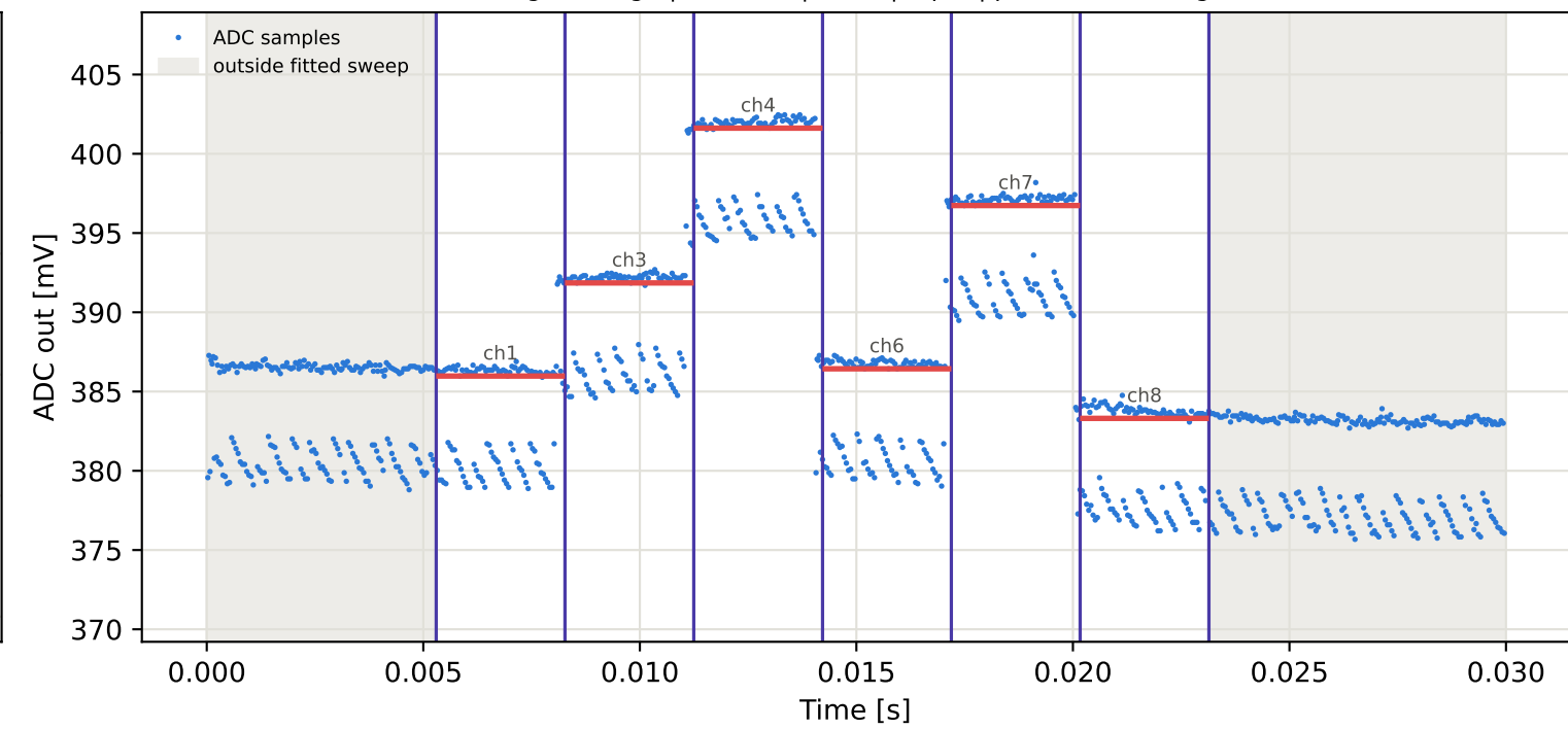
Tag9 &lt;- Tag6 | 965 MHz | run 0 | rep 1 | phase 177.46 deg
