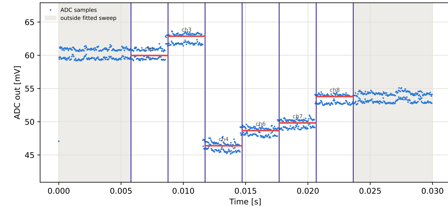
Tag9 &lt;- Tag16 | 805 MHz | run 0 | rep 1 | phase -85.16 deg
