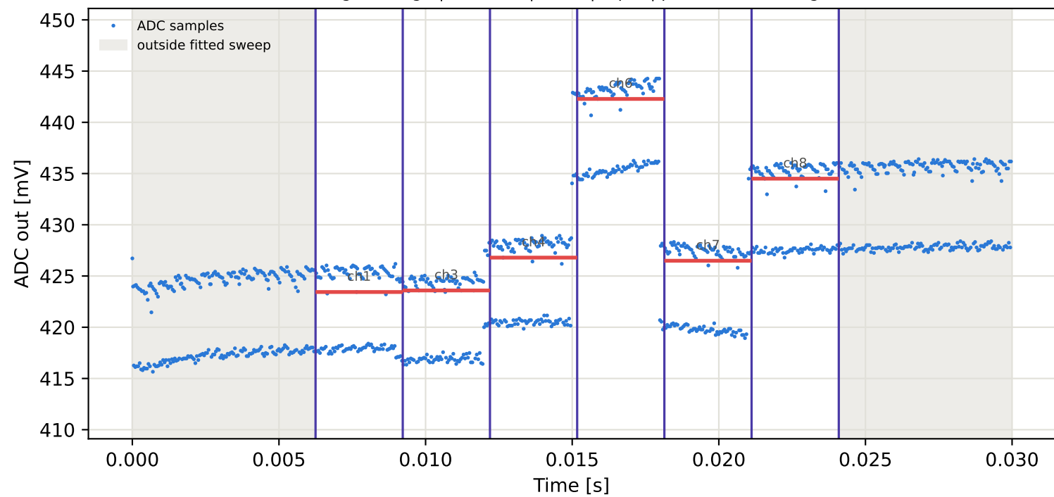
Tag2 &lt;- Tag5 | 905 MHz | run 0 | rep 1 | phase -82.70 deg
