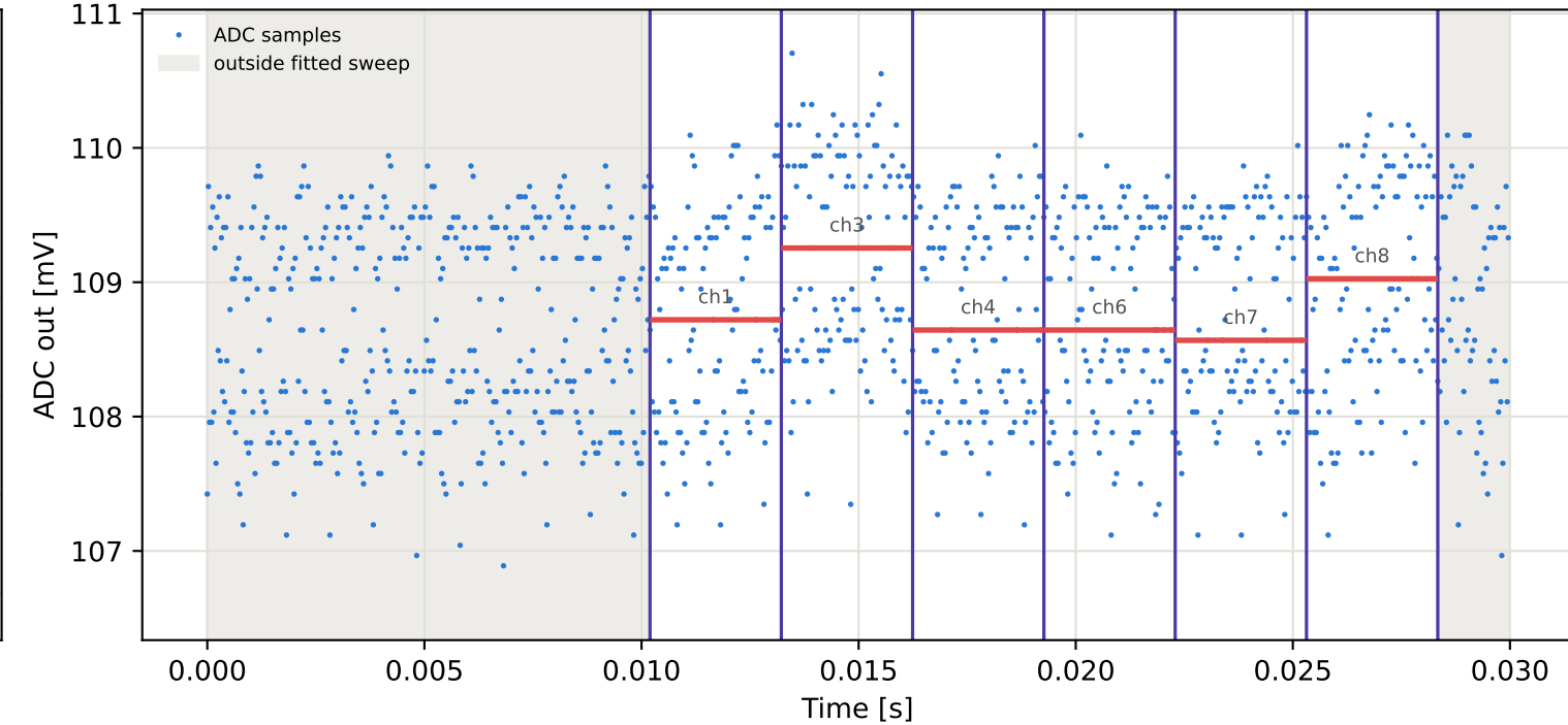
Tag5 &lt;- Tag1 | 775 MHz | run 0 | rep 1 | phase -41.72 deg
