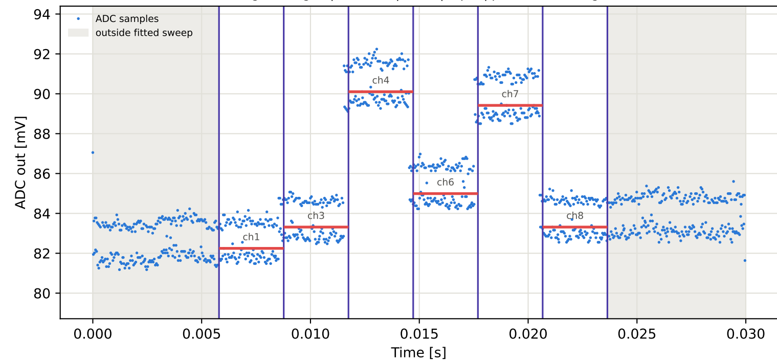
Tag5 &lt;- Tag2 | 775 MHz | run 0 | rep 1 | phase -38.55 deg
