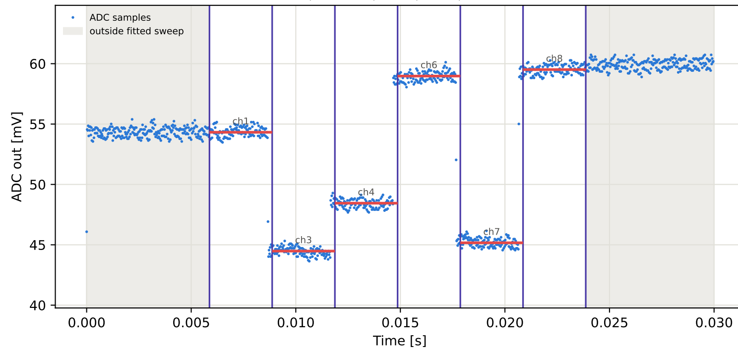
Tag9 &lt;- Tag7 | 805 MHz | run 0 | rep 1 | phase 166.21 deg
