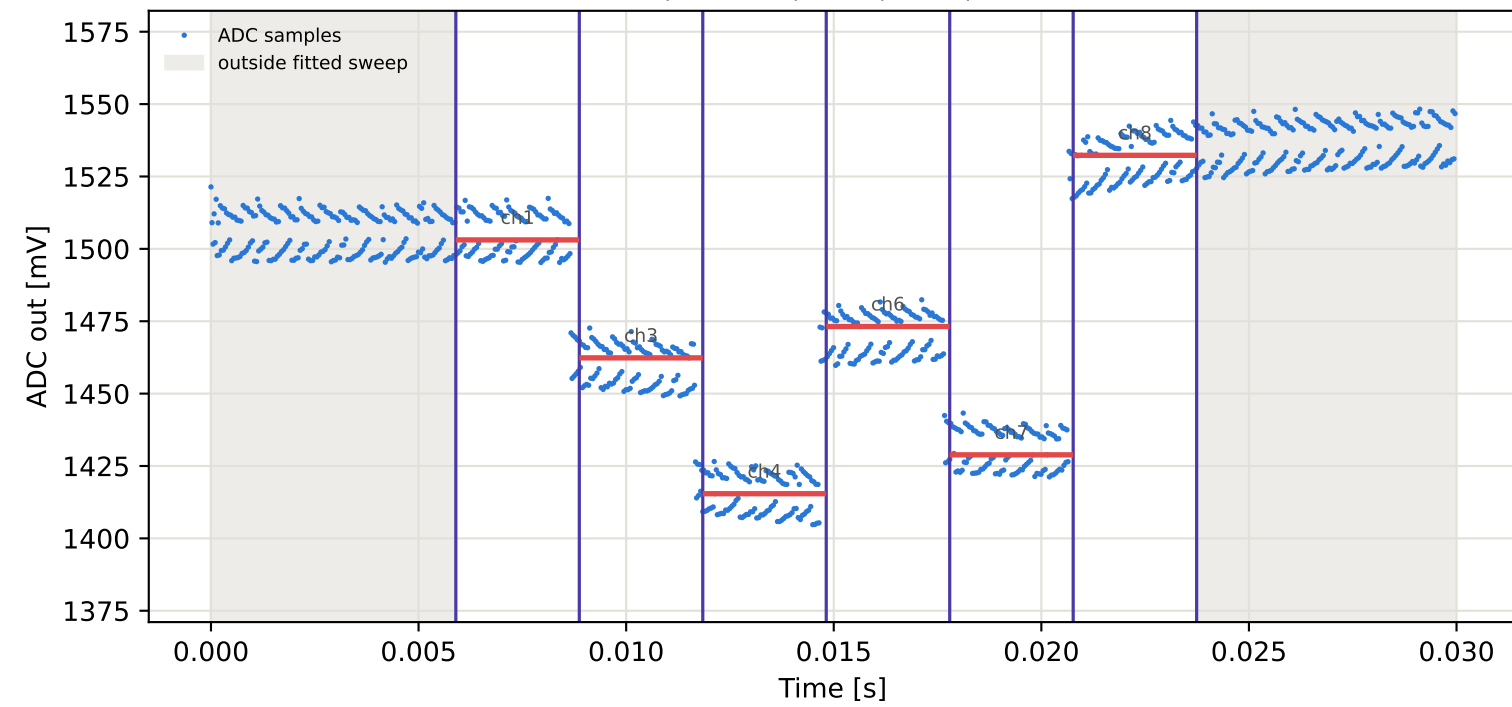
Tag8 &lt;- Tag16 | 915 MHz | run 0 | rep 1 | phase 95.56 deg
