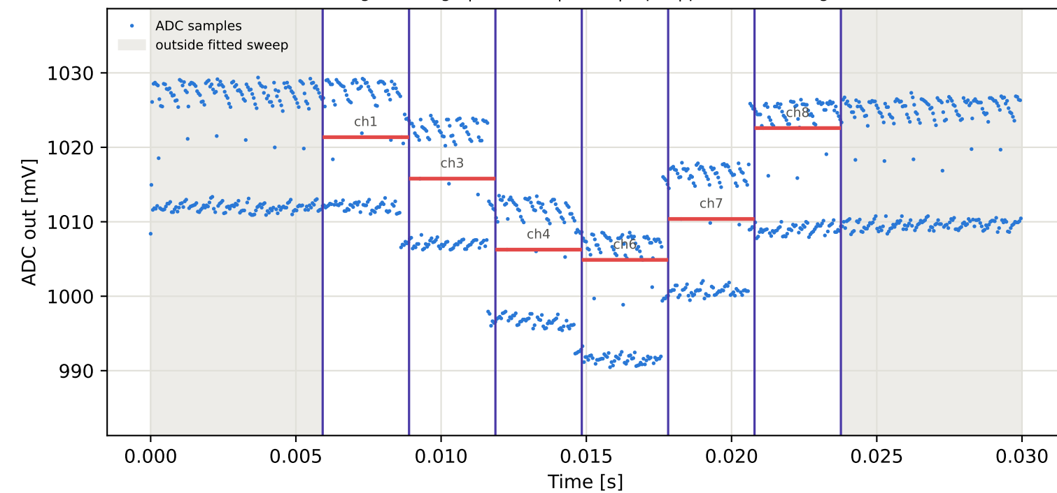
Tag15 &lt;- Tag1 | 925 MHz | run 0 | rep 1 | phase -8.66 deg
