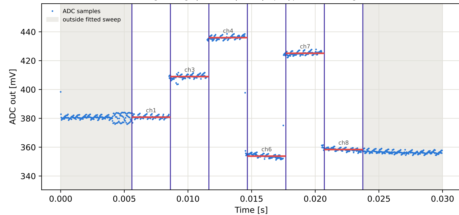
Tag4 &lt;- Tag7 | 965 MHz | run 0 | rep 1 | phase -126.37 deg
