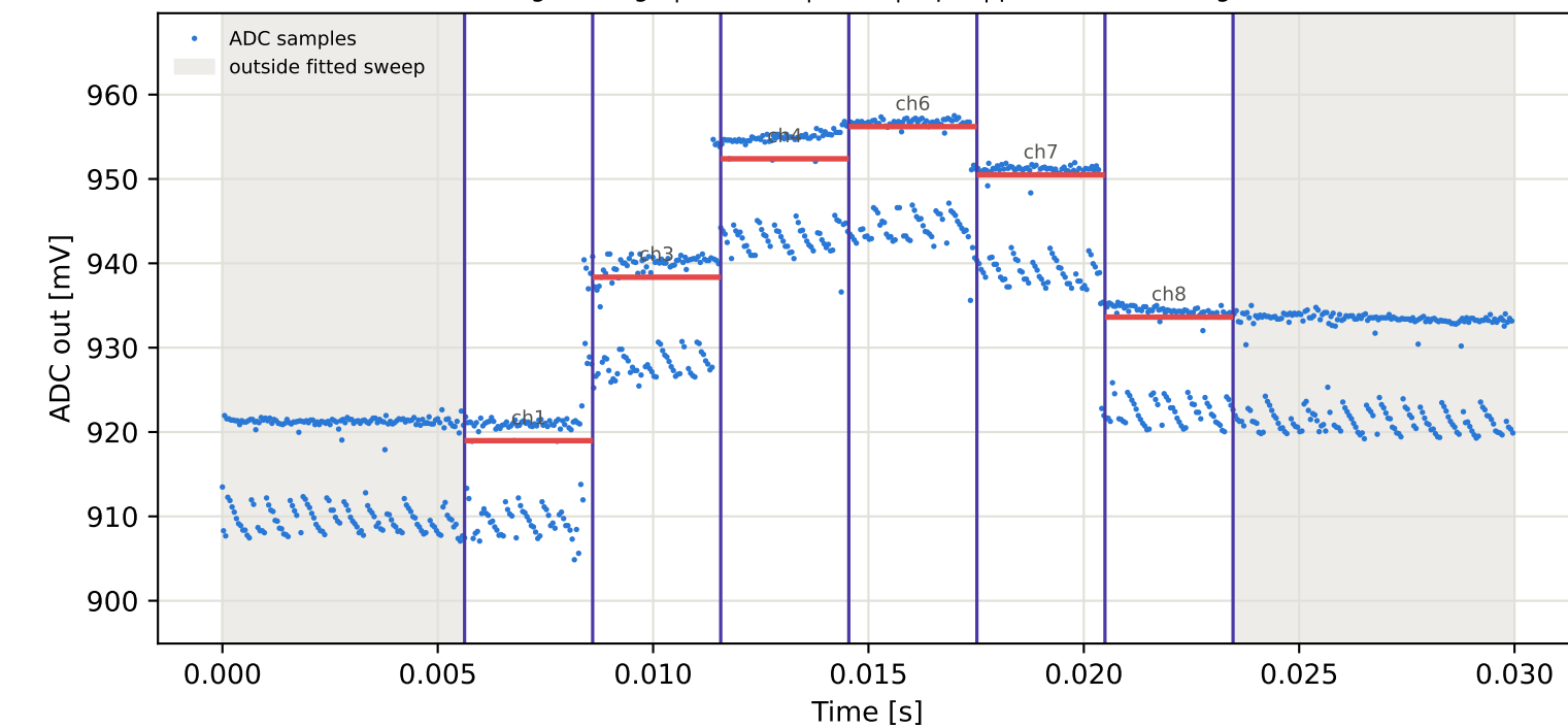
Tag7 &lt;- Tag5 | 875 MHz | run 0 | rep 1 | phase -118.51 deg
