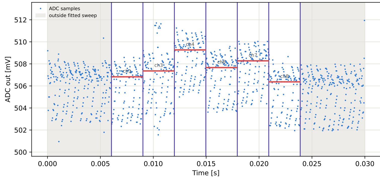
Tag5 &lt;- Tag4 | 975 MHz | run 0 | rep 1 | phase -176.76 deg
