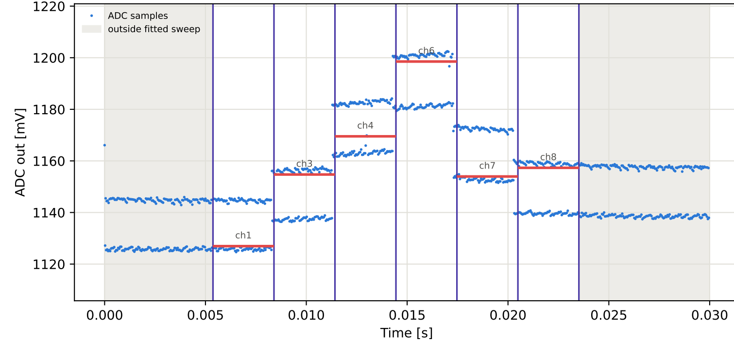
Tag8 &lt;- Tag15 | 925 MHz | run 0 | rep 1 | phase -142.89 deg
