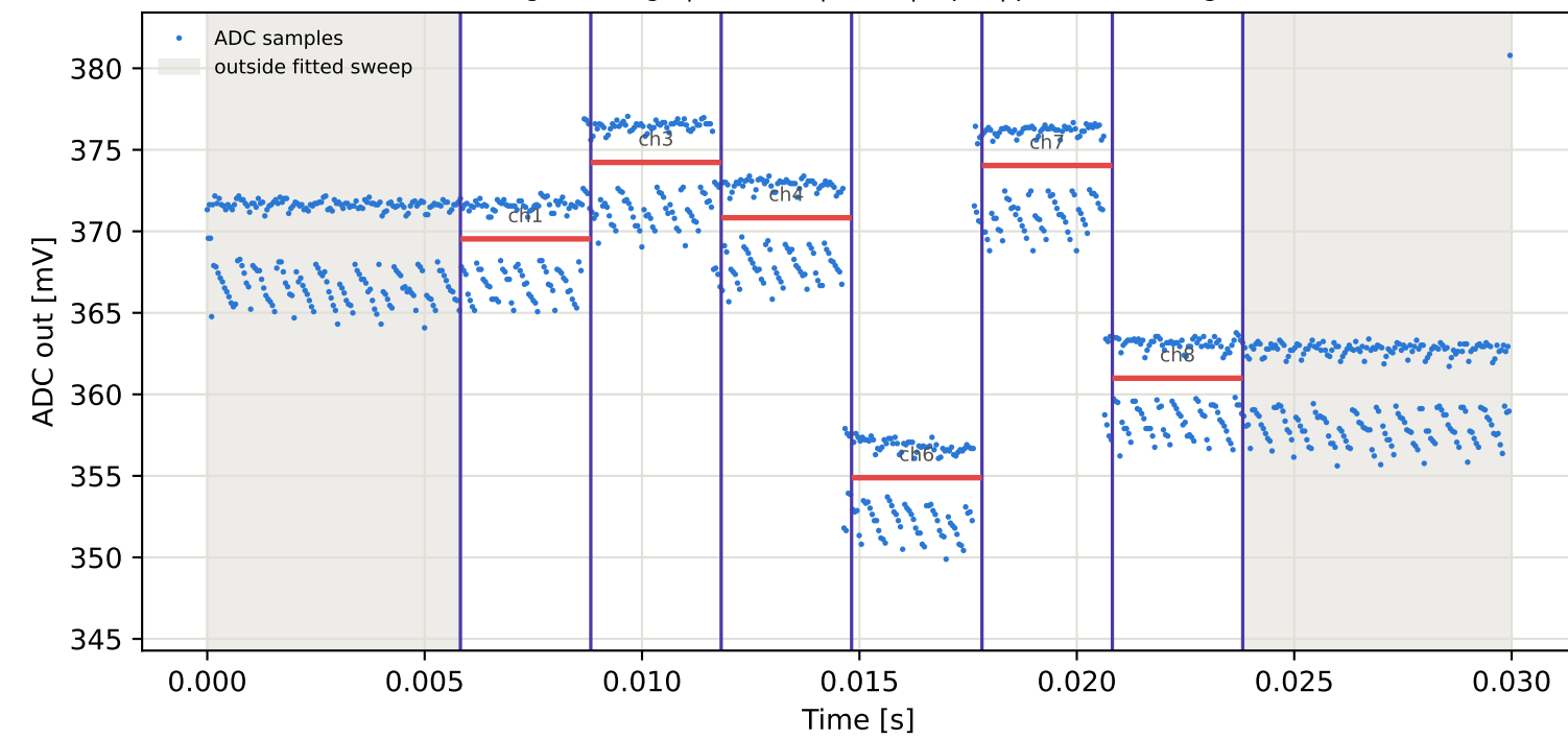
Tag15 &lt;- Tag9 | 995 MHz | run 0 | rep 1 | phase 138.12 deg
