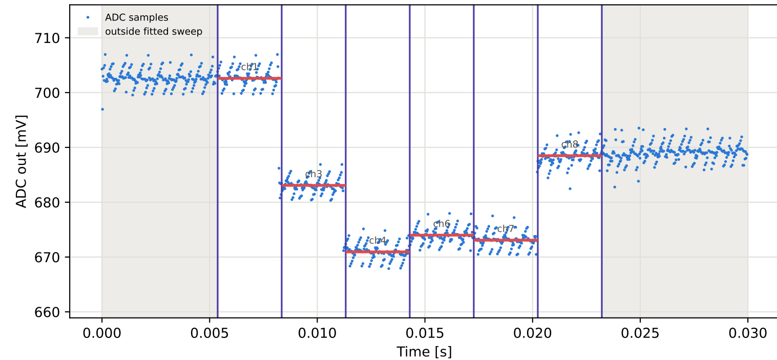
Tag8 &lt;- Tag6 | 855 MHz | run 0 | rep 1 | phase 77.96 deg
