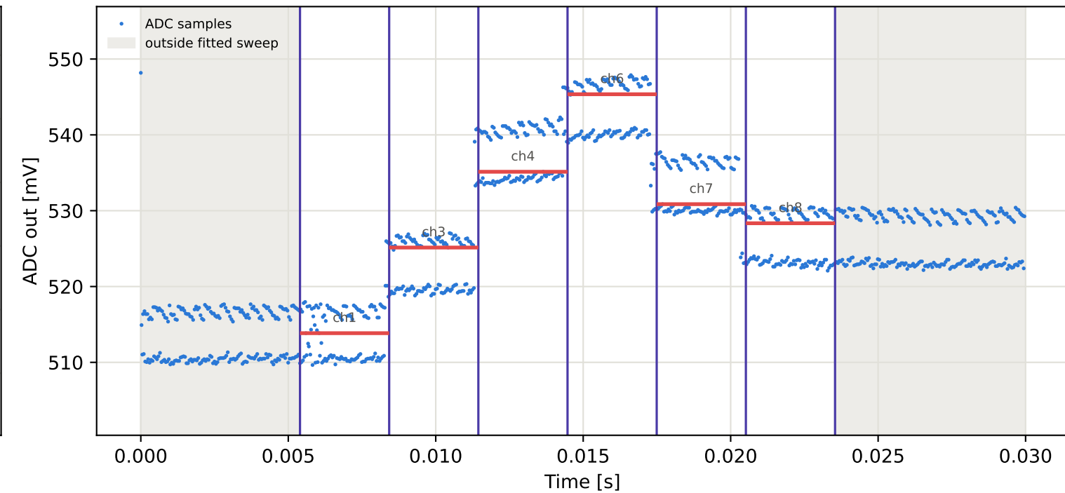
Tag5 &lt;- Tag4 | 865 MHz | run 0 | rep 1 | phase 48.59 deg
