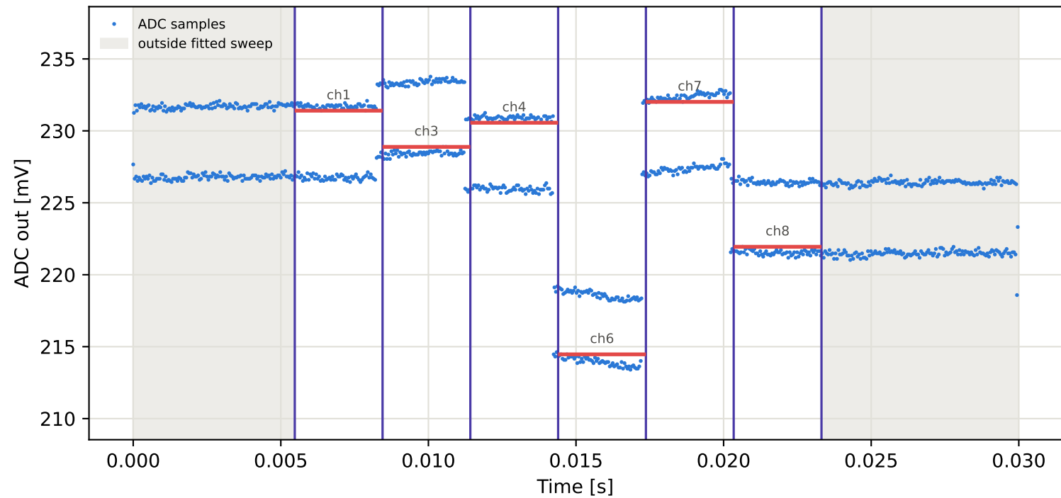
Tag2 &lt;- Tag7 | 935 MHz | run 0 | rep 1 | phase -114.44 deg
