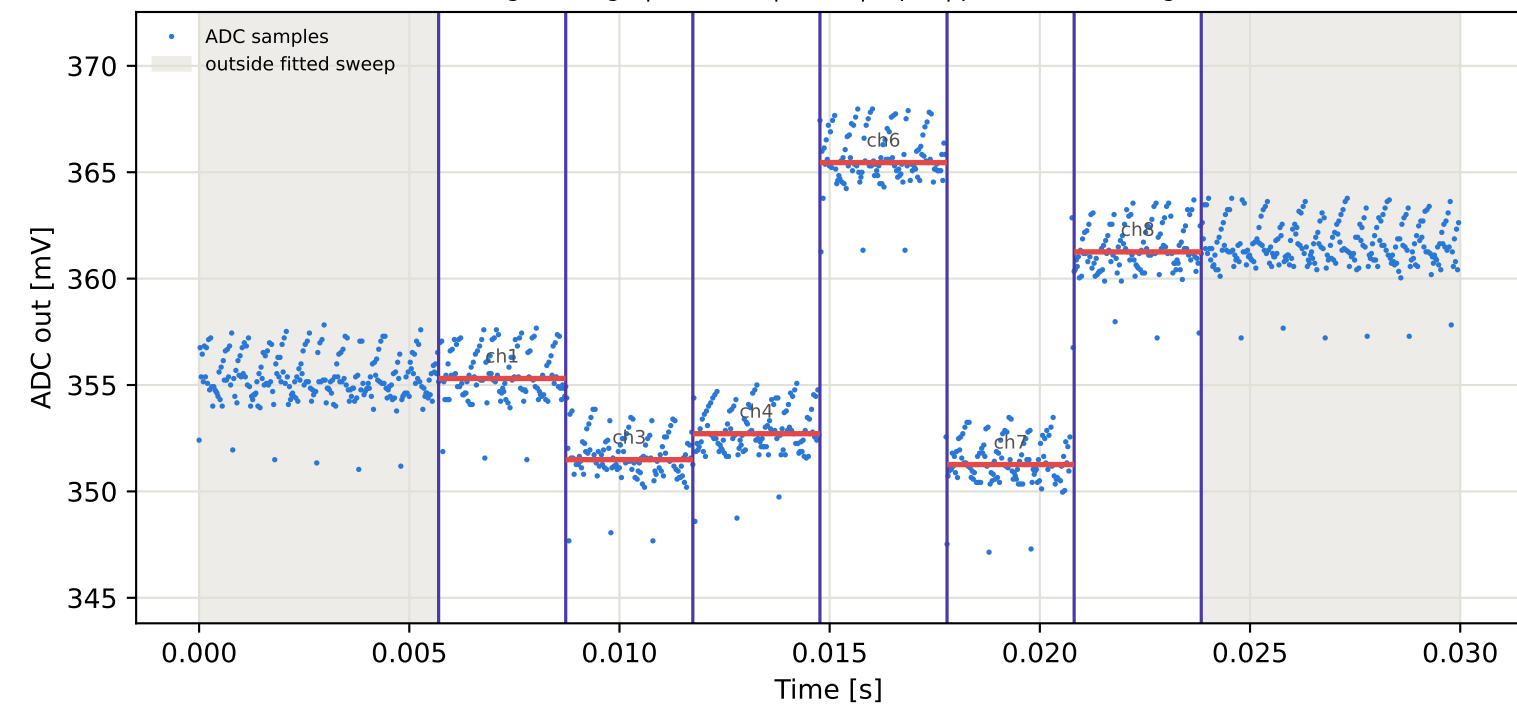
Tag4 &lt;- Tag15 | 955 MHz | run 0 | rep 1 | phase -9.87 deg
