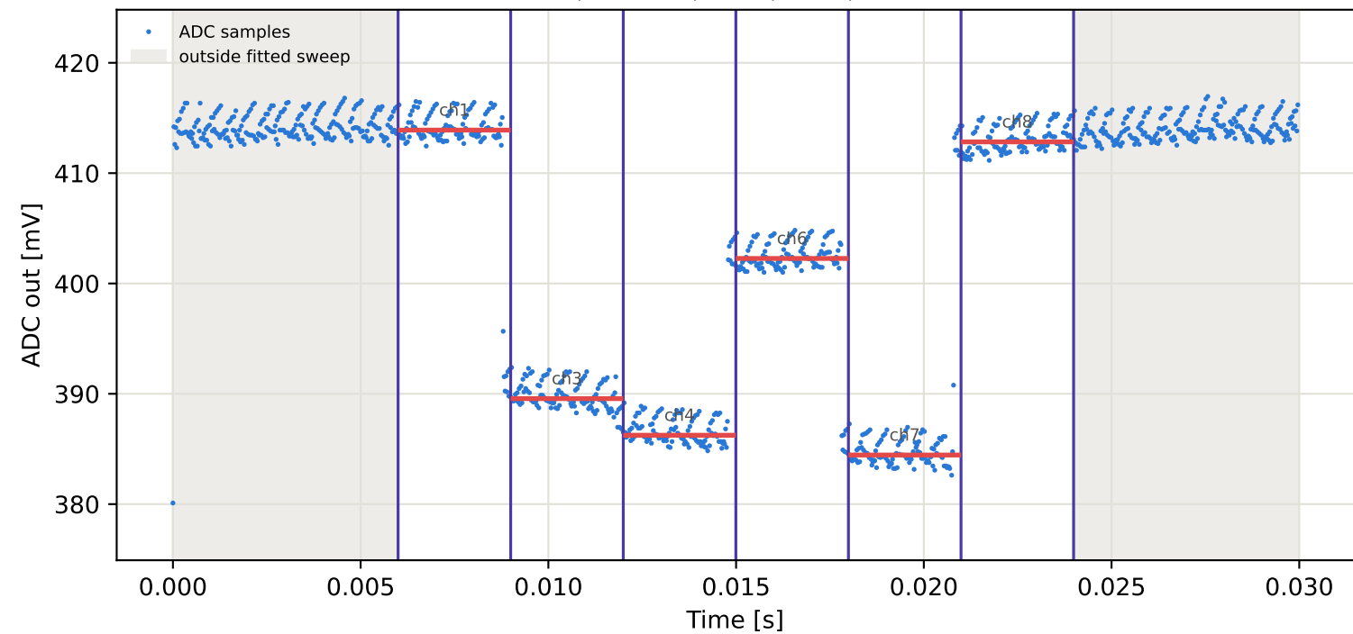
Tag6 &lt;- Tag10 | 845 MHz | run 0 | rep 1 | phase 115.49 deg
