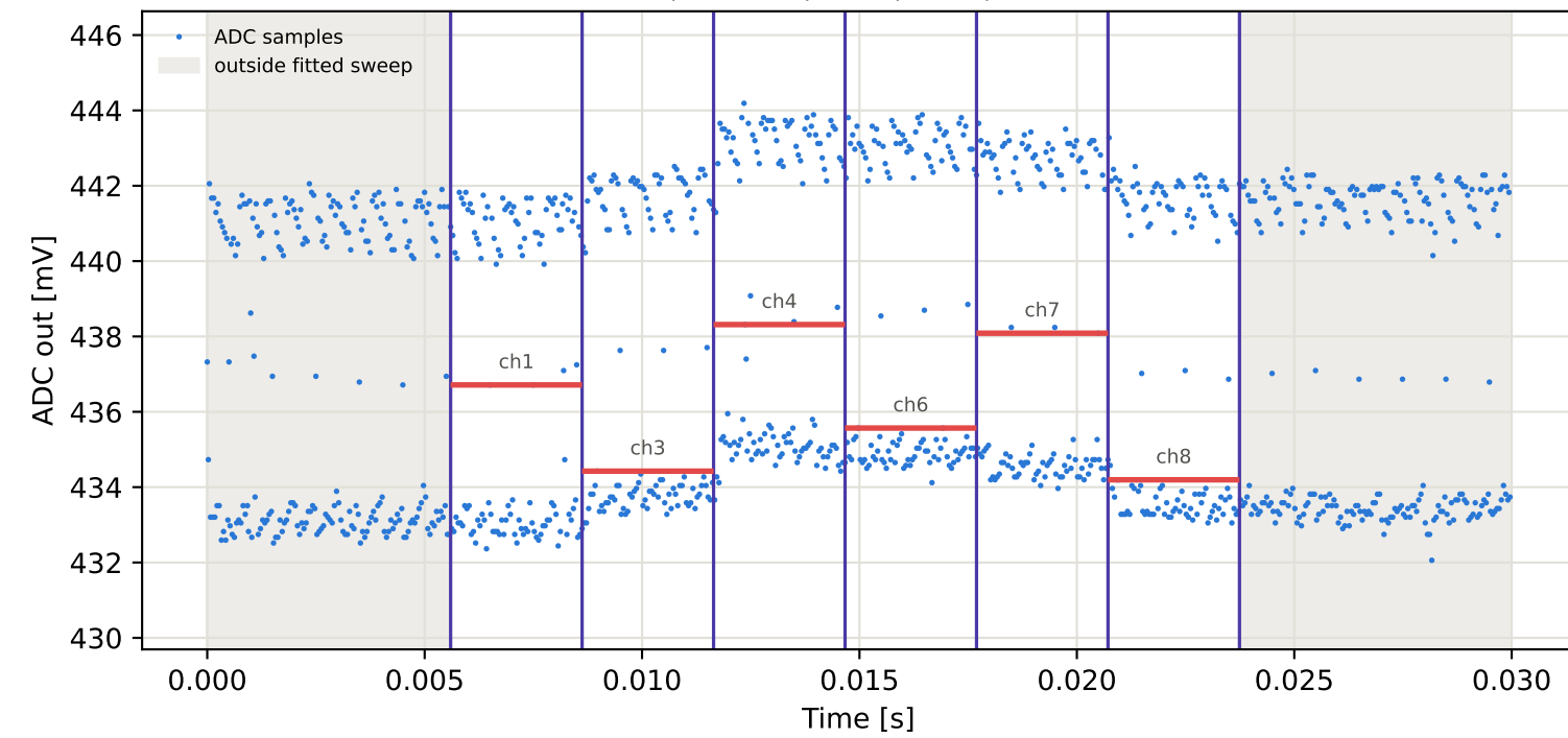
Tag2 &lt;- Tag7 | 925 MHz | run 0 | rep 1 | phase -91.21 deg
