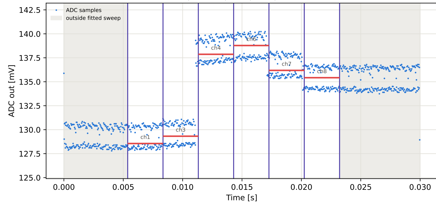
Tag2 &lt;- Tag8 | 825 MHz | run 0 | rep 1 | phase -125.96 deg
