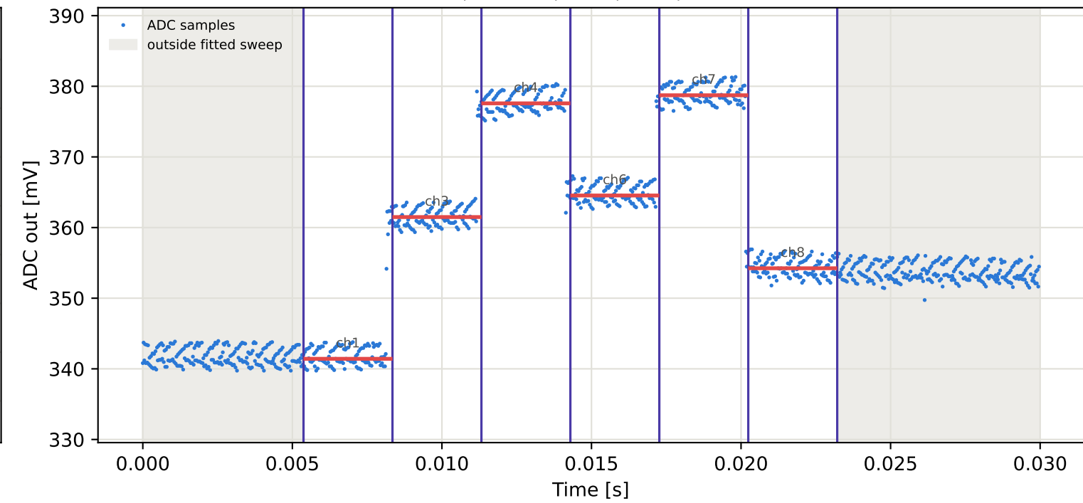
Tag5 &lt;- Tag4 | 825 MHz | run 0 | rep 1 | phase -90.24 deg
