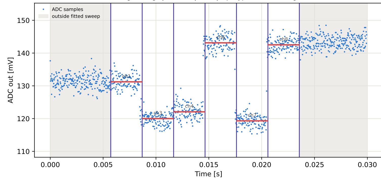
Tag4 &lt;- Tag9 | 885 MHz | run 0 | rep 1 | phase -67.41 deg
