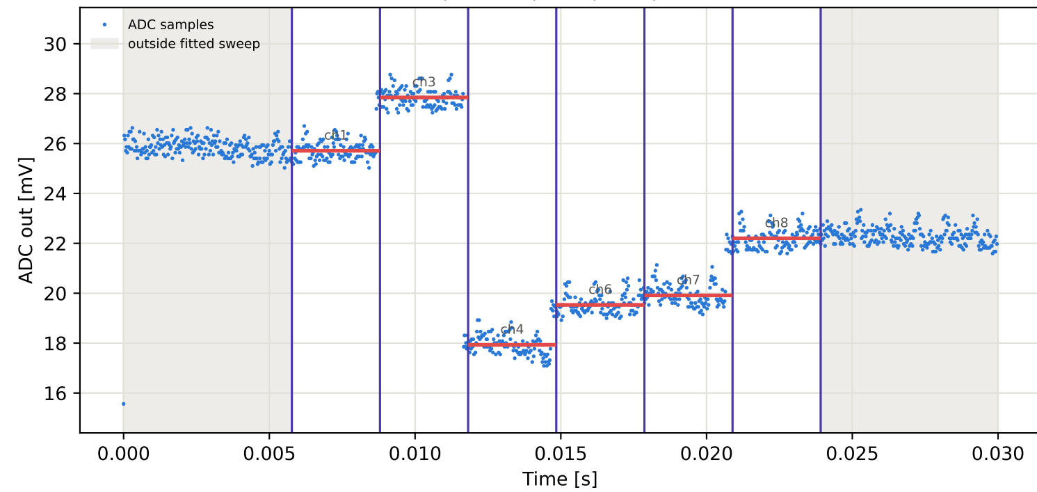
Tag6 &lt;- Tag10 | 795 MHz | run 0 | rep 1 | phase 64.97 deg
