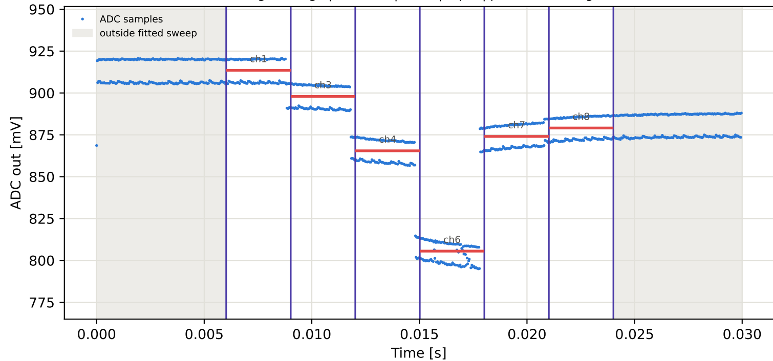
Tag9 &lt;- Tag8 | 905 MHz | run 0 | rep 1 | phase 32.75 deg
