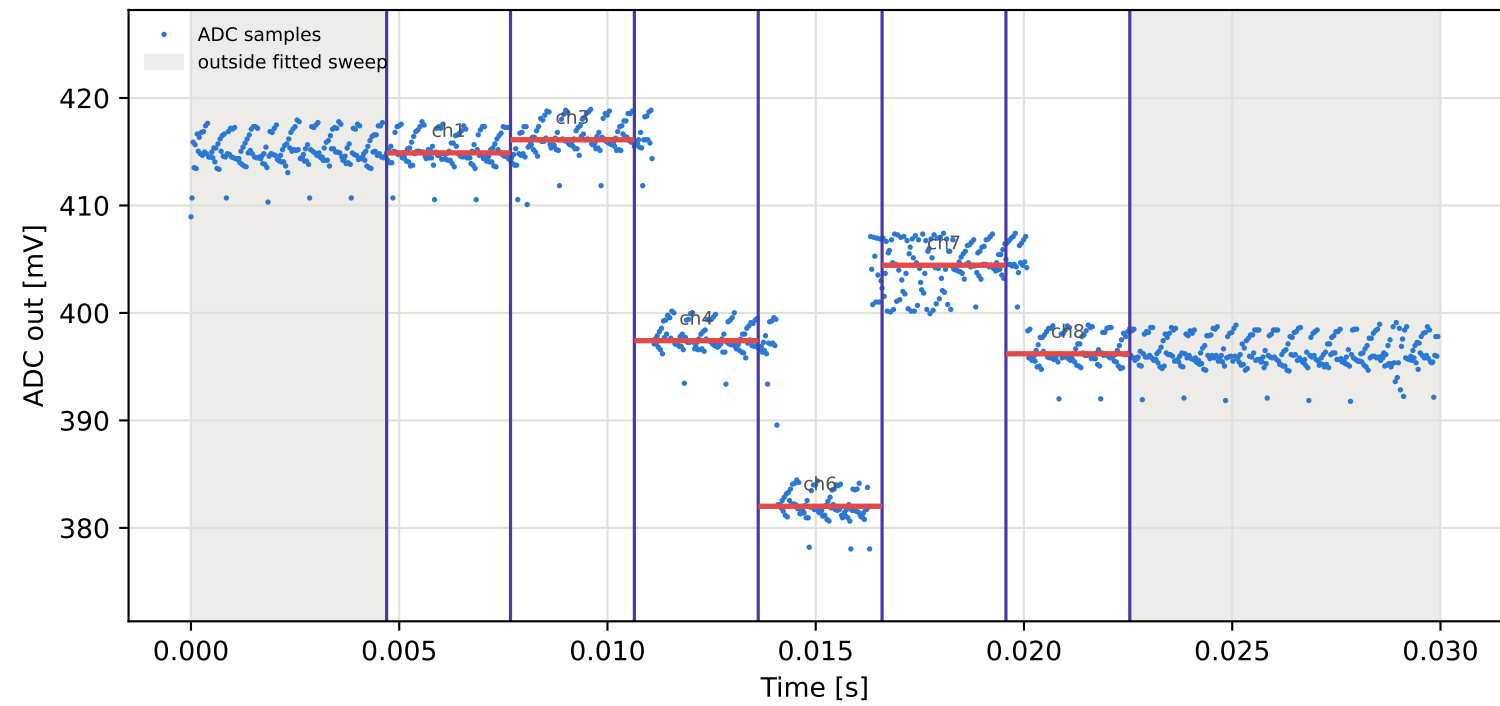
Tag15 &lt;- Tag9 | 835 MHz | run 0 | rep 1 | phase 6.18 deg
