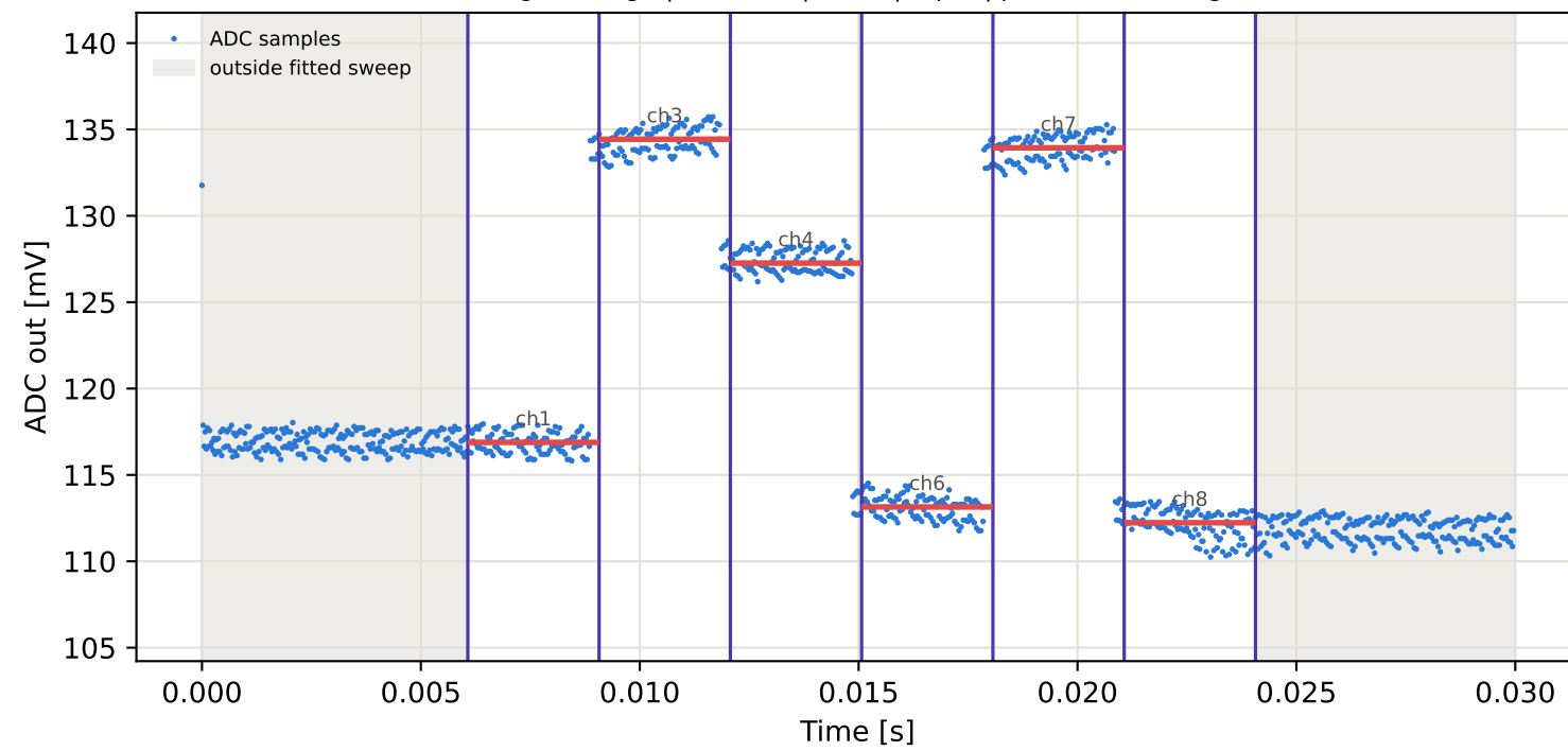
Tag8 &lt;- Tag1 | 805 MHz | run 0 | rep 1 | phase -61.19 deg
