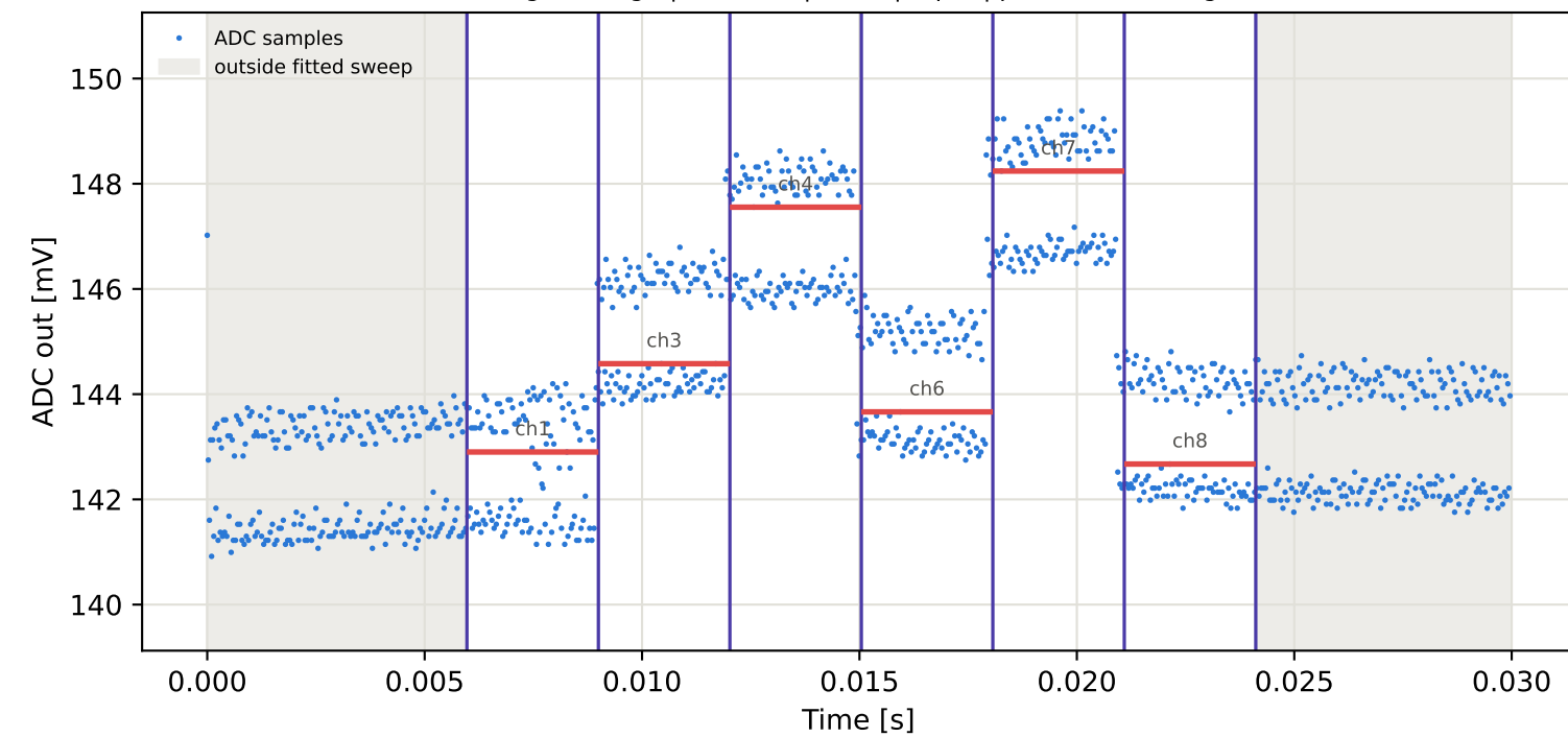
Tag3 &lt;- Tag6 | 805 MHz | run 0 | rep 1 | phase -51.63 deg
