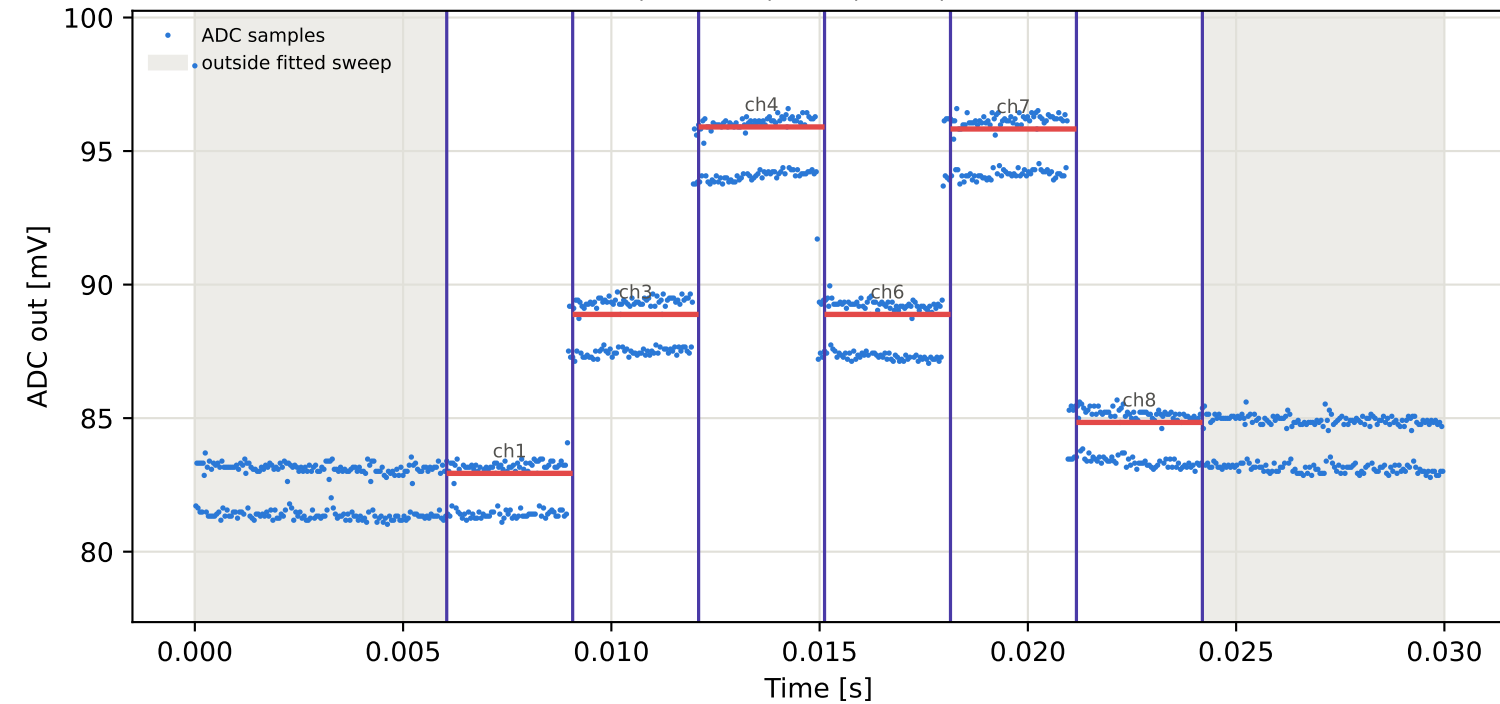
Tag3 &lt;- Tag9 | 795 MHz | run 0 | rep 1 | phase -78.46 deg
