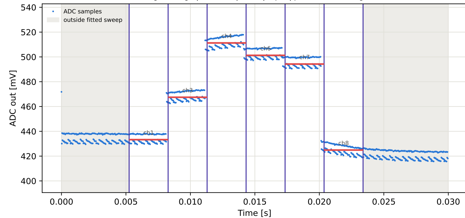
Tag6 &lt;- Tag1 | 915 MHz | run 0 | rep 1 | phase 13.81 deg
