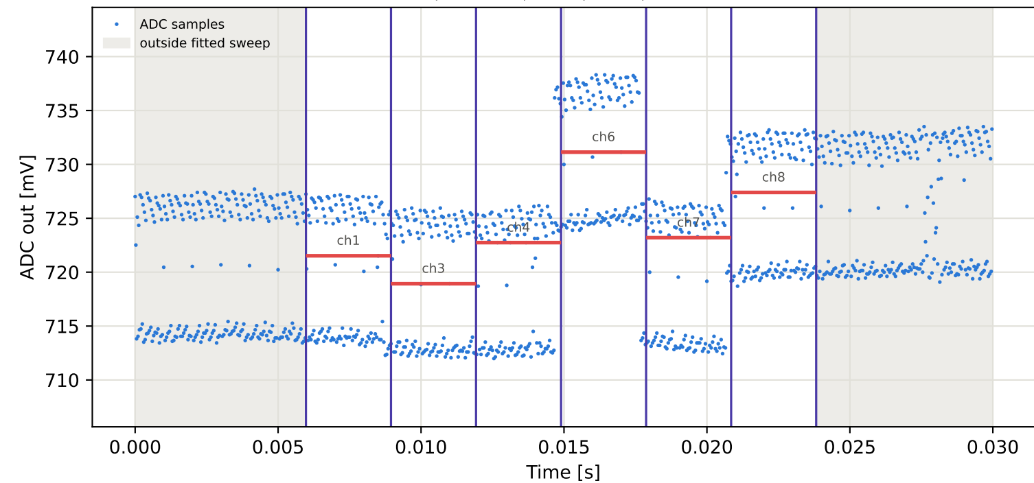
Tag3 &lt;- Tag2 | 905 MHz | run 0 | rep 1 | phase -166.98 deg
