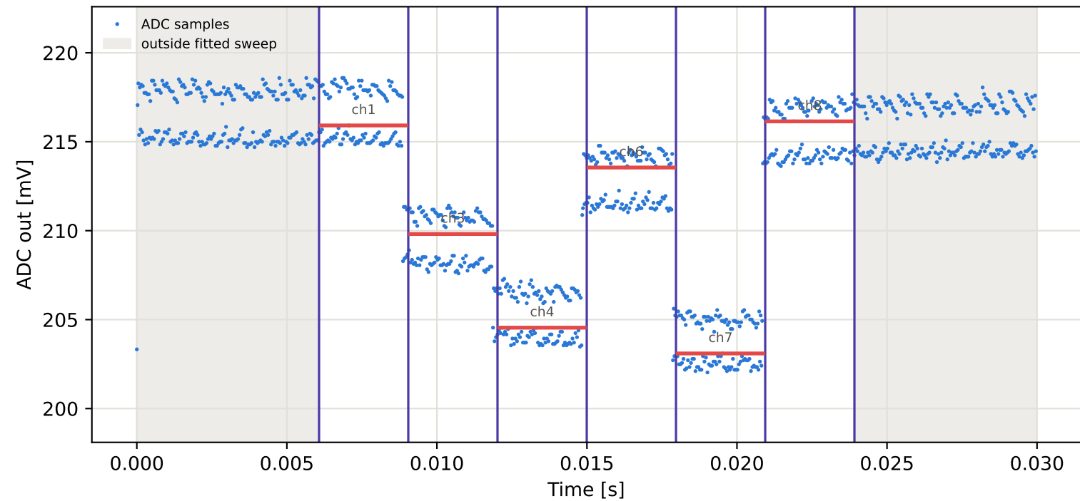
Tag5 &lt;- Tag1 | 805 MHz | run 0 | rep 1 | phase -42.09 deg
