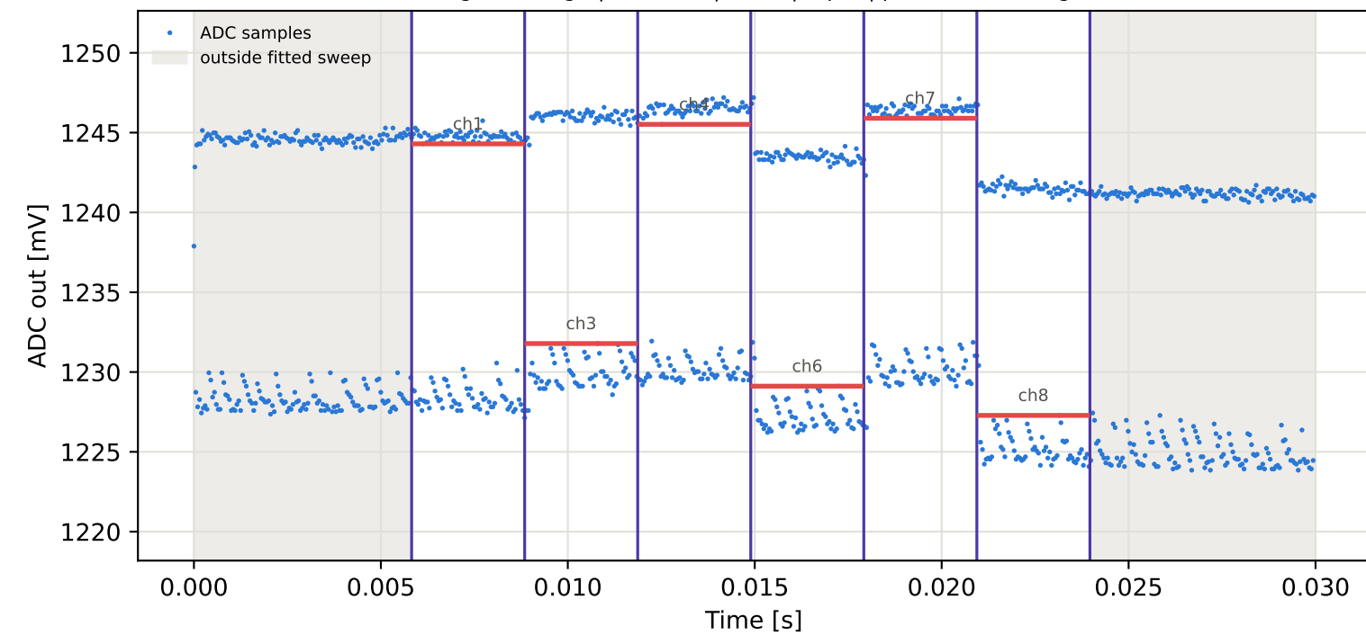
Tag16 &lt;- Tag4 | 895 MHz | run 0 | rep 1 | phase -179.45 deg
