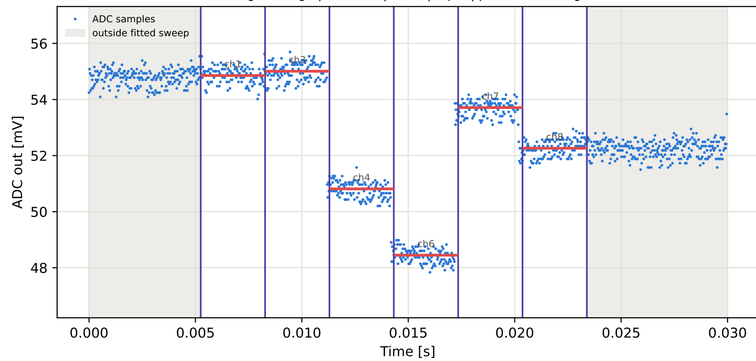
Tag2 &lt;- Tag8 | 975 MHz | run 0 | rep 1 | phase 27.04 deg
