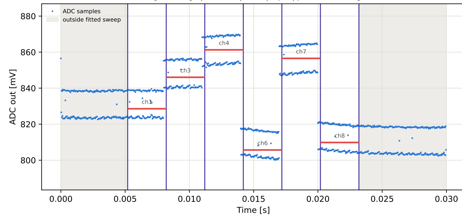
Tag16 &lt;- Tag6 | 945 MHz | run 0 | rep 1 | phase -136.88 deg
