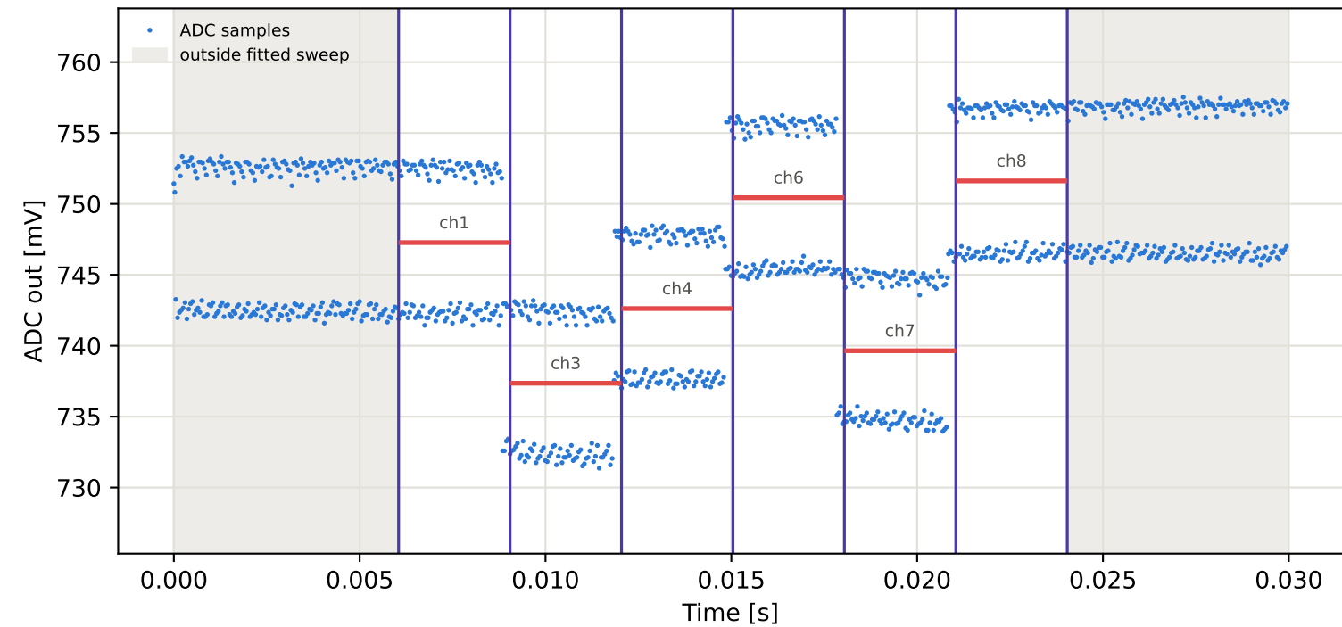
Tag3 &lt;- Tag2 | 855 MHz | run 0 | rep 1 | phase -65.21 deg
