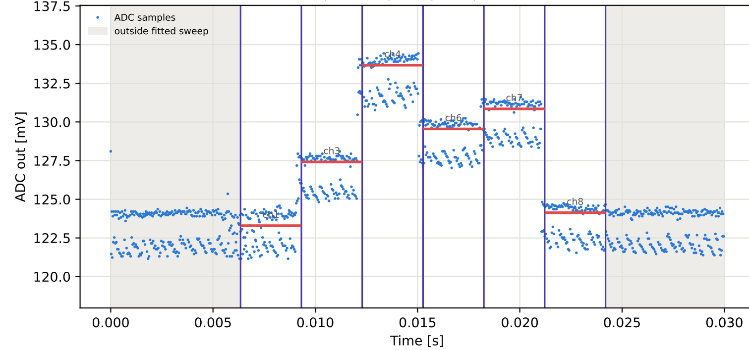
Tag2 &lt;- Tag7 | 945 MHz | run 0 | rep 1 | phase -110.04 deg
