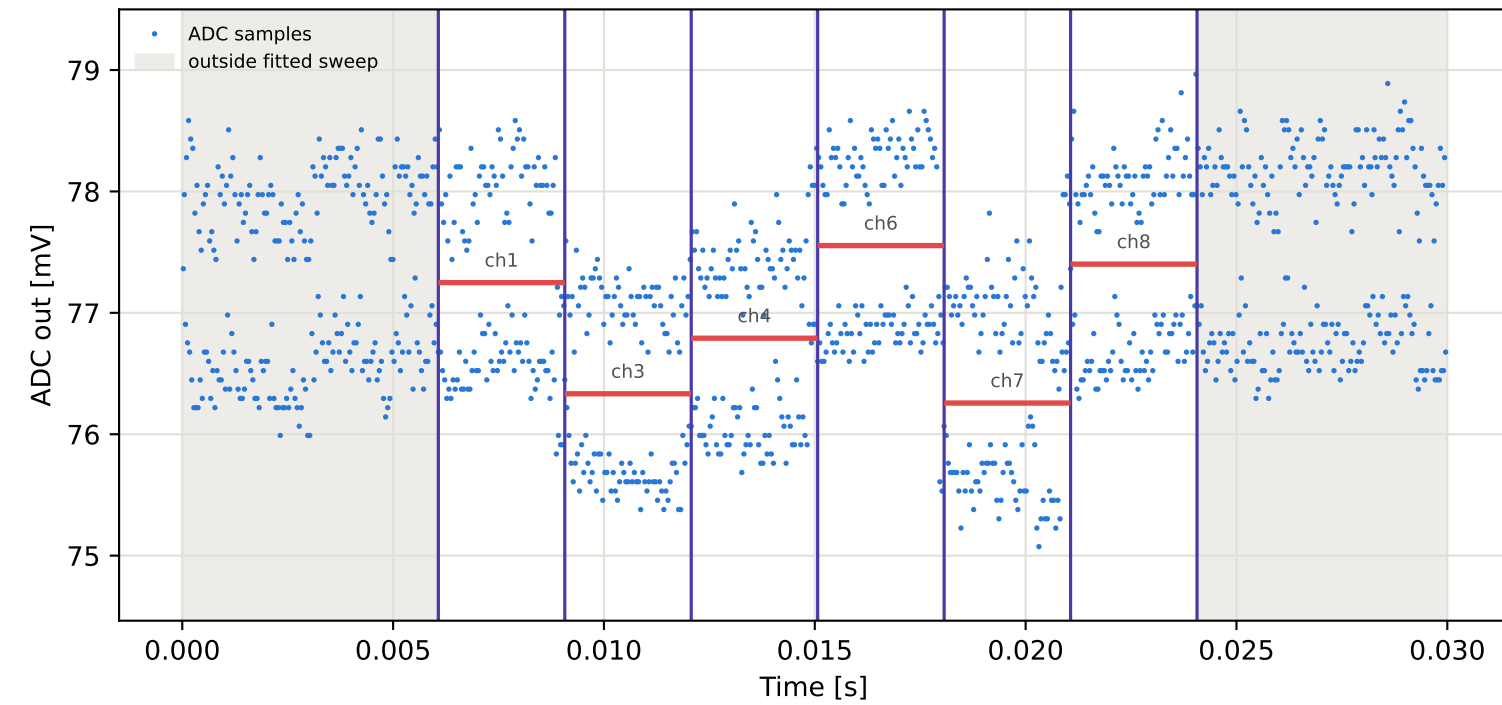
Tag16 &lt;- Tag10 | 775 MHz | run 0 | rep 1 | phase -34.88 deg
