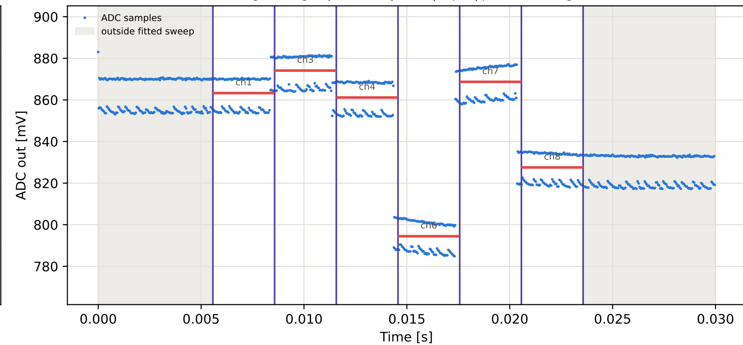
Tag5 &lt;- Tag2 | 935 MHz | run 0 | rep 1 | phase 59.16 deg
