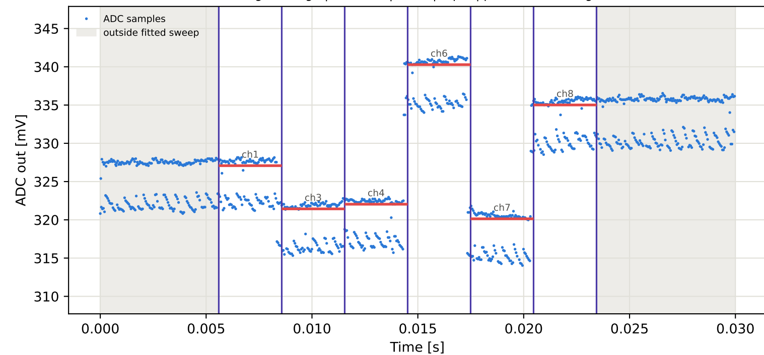
Tag6 &lt;- Tag1 | 975 MHz | run 0 | rep 1 | phase 159.79 deg
