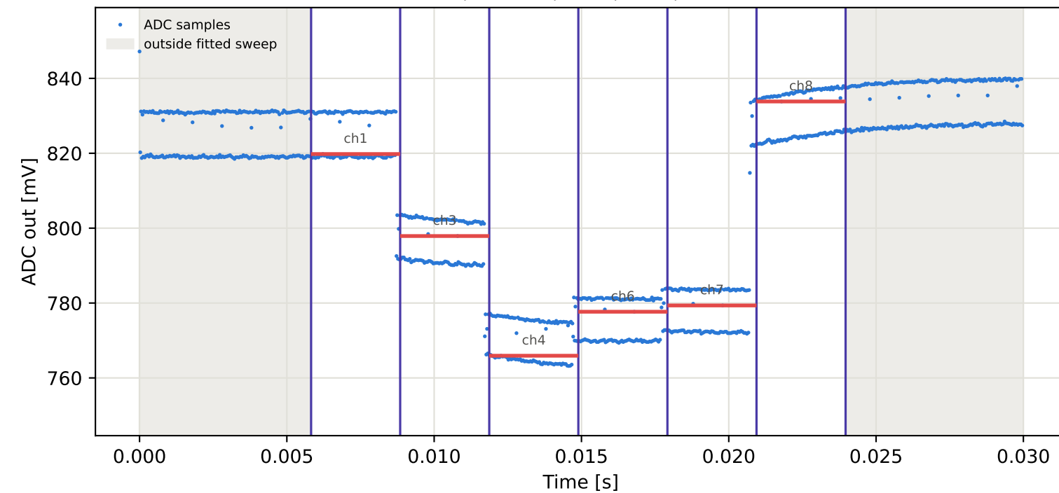
Tag15 &lt;- Tag5 | 895 MHz | run 0 | rep 1 | phase 73.84 deg
