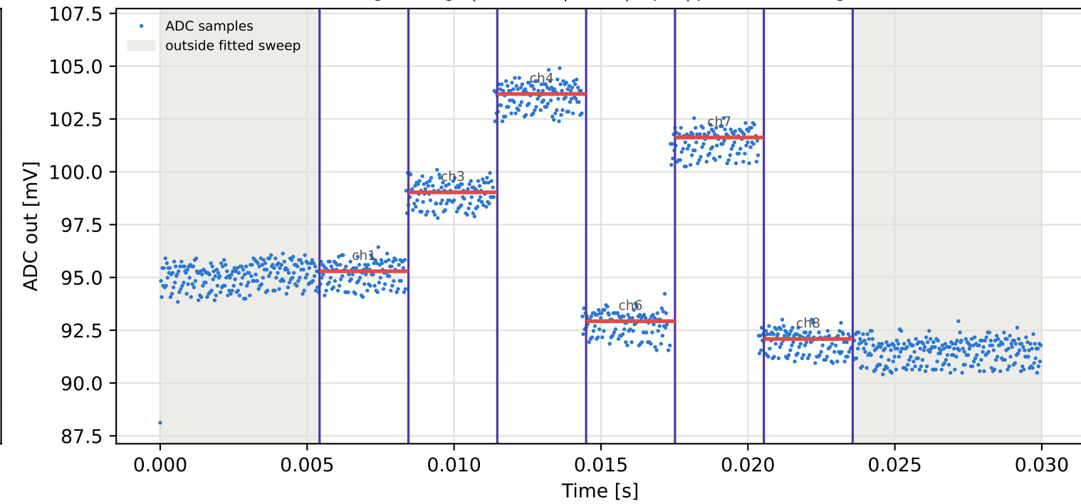
Tag1 &lt;- Tag8 | 945 MHz | run 0 | rep 1 | phase -161.82 deg
