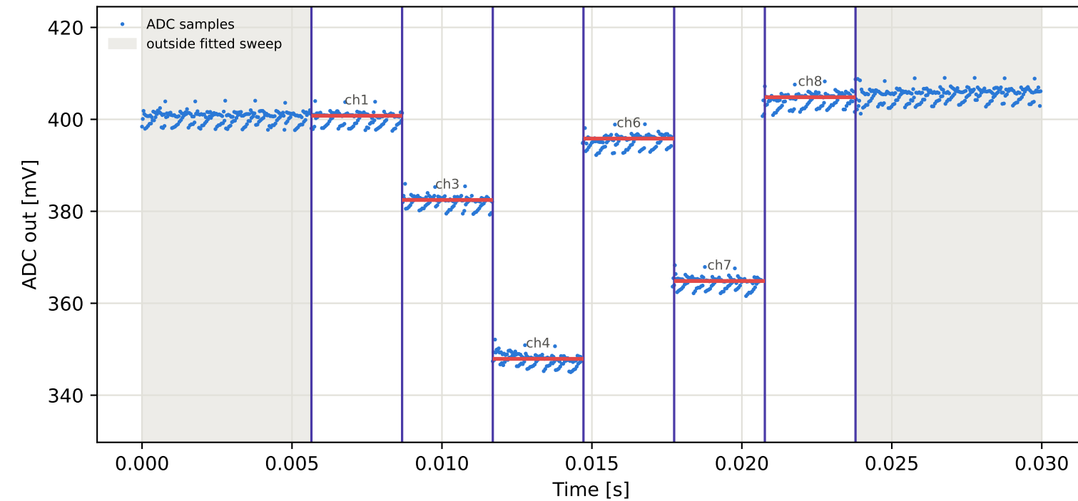
Tag5 &lt;- Tag3 | 985 MHz | run 0 | rep 1 | phase 174.48 deg
