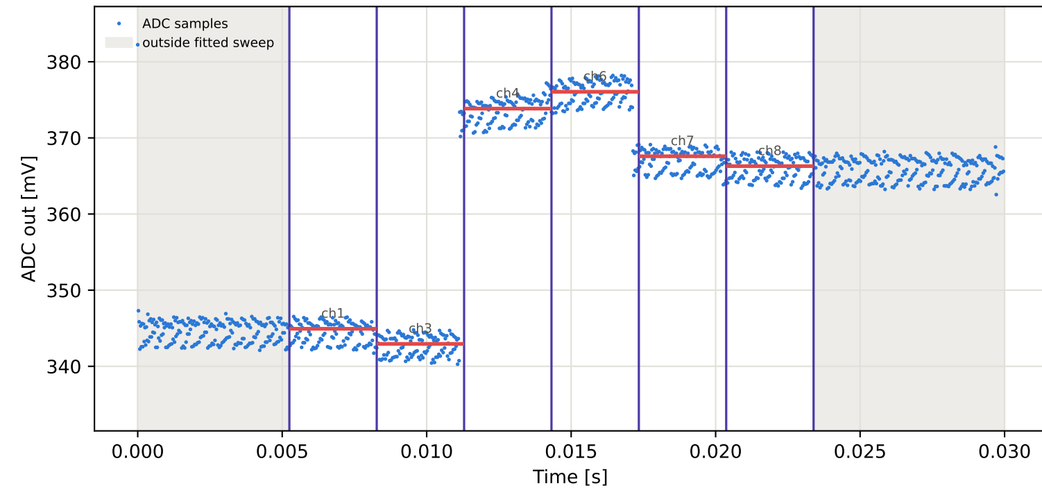
Tag6 &lt;- Tag1 | 825 MHz | run 0 | rep 1 | phase -62.27 deg
