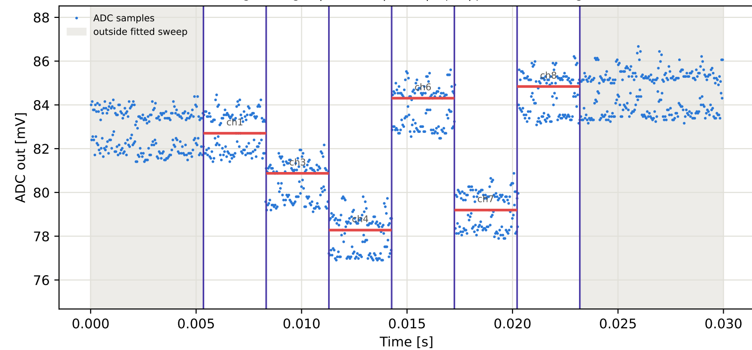
Tag6 &lt;- Tag2 | 955 MHz | run 0 | rep 1 | phase -73.10 deg
