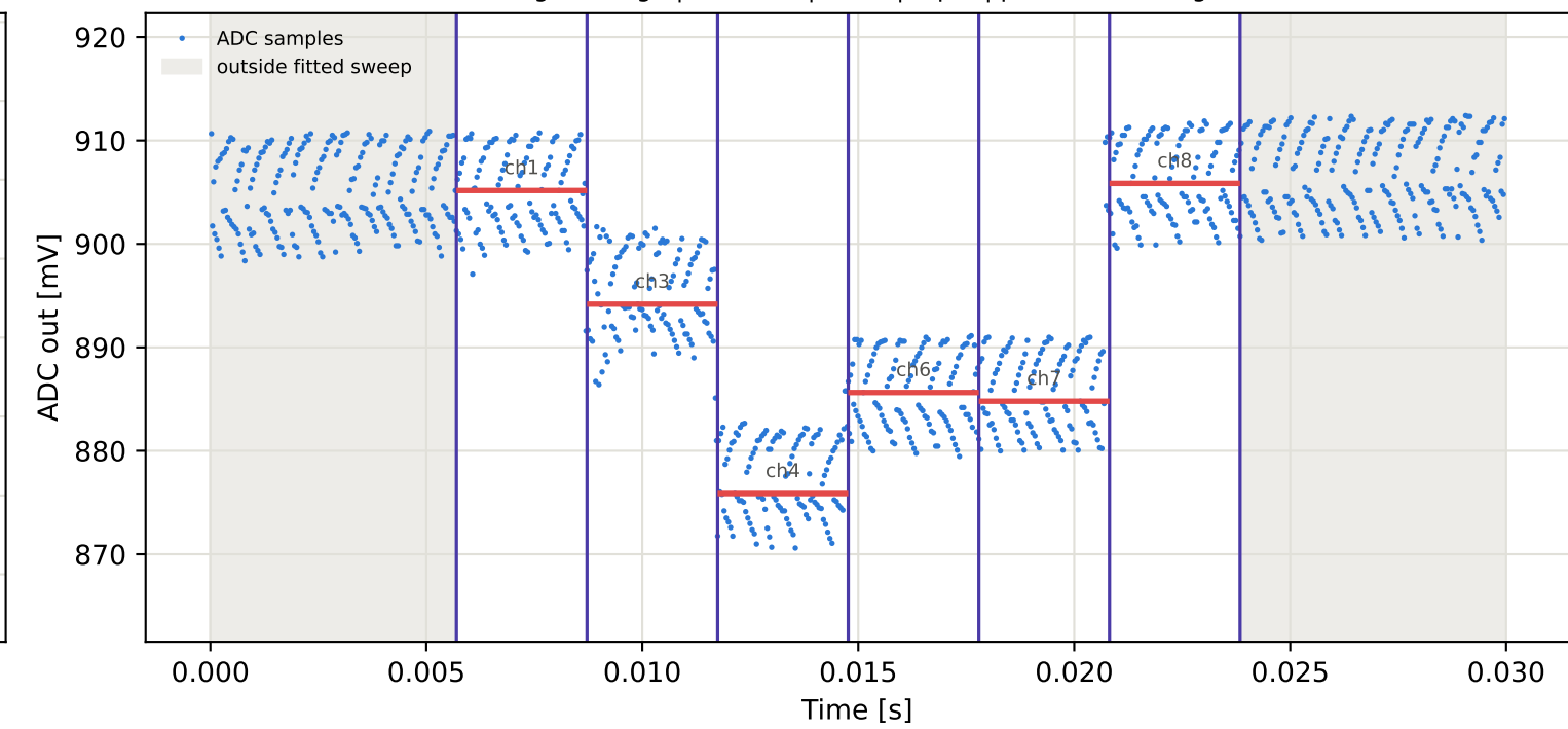
Tag9 &lt;- Tag8 | 935 MHz | run 0 | rep 1 | phase 69.16 deg
