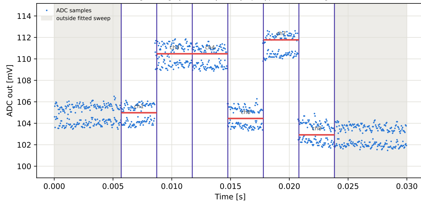
Tag6 &lt;- Tag9 | 805 MHz | run 0 | rep 1 | phase -32.24 deg
