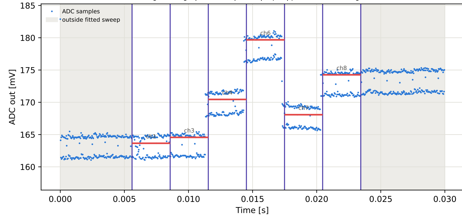
Tag9 &lt;- Tag2 | 865 MHz | run 0 | rep 1 | phase -153.74 deg
