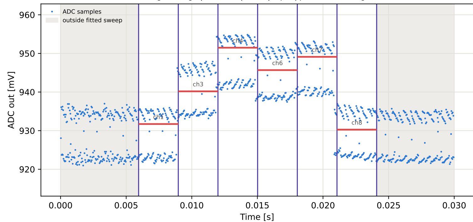
Tag7 &lt;- Tag6 | 875 MHz | run 0 | rep 1 | phase 32.91 deg
