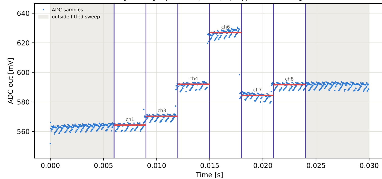
Tag10 &lt;- Tag2 | 915 MHz | run 0 | rep 1 | phase 150.48 deg
