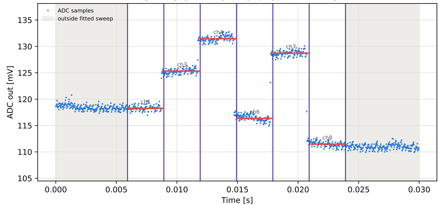
Tag1 &lt;- Tag8 | 915 MHz | run 0 | rep 1 | phase -77.22 deg
