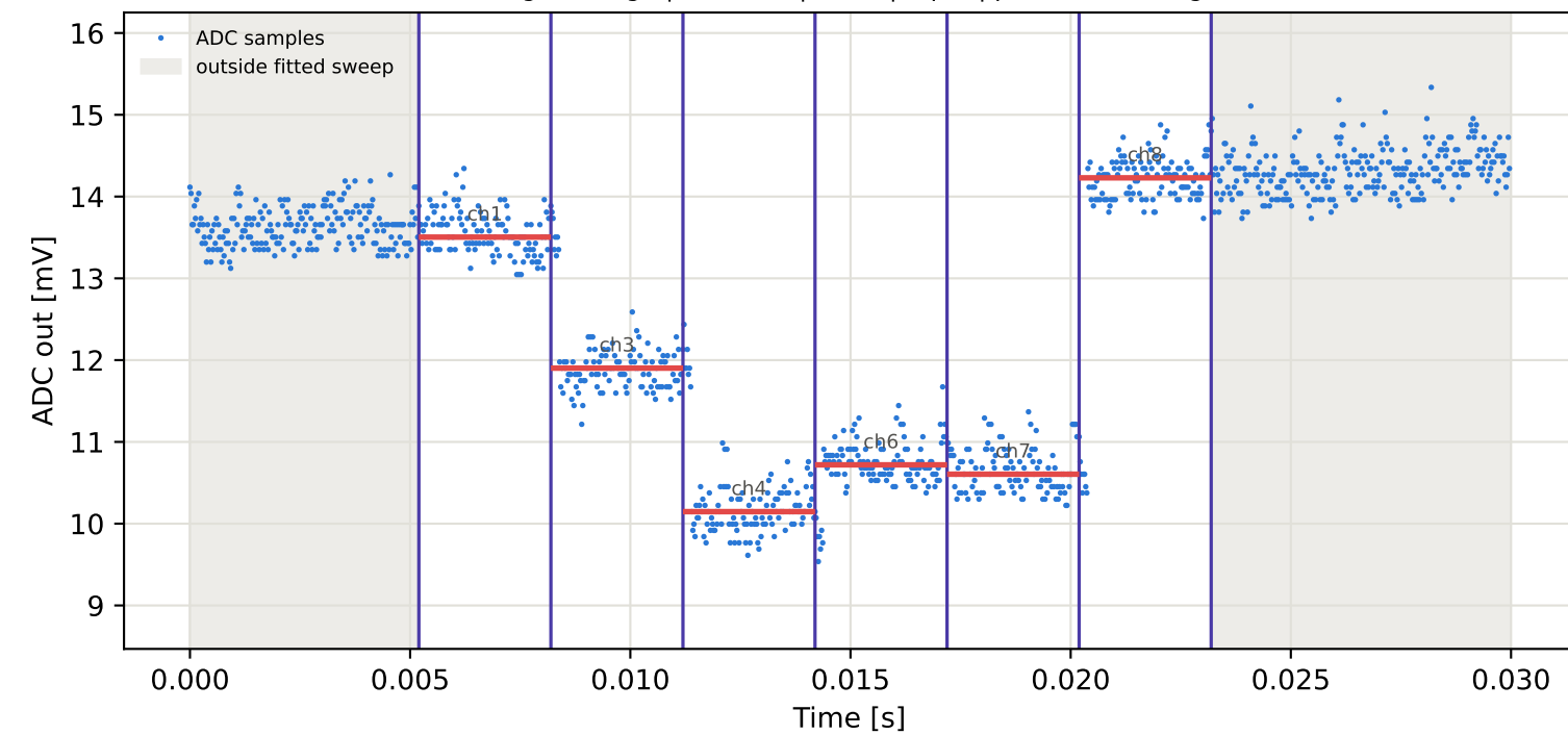
Tag1 &lt;- Tag7 | 905 MHz | run 0 | rep 1 | phase -81.14 deg
