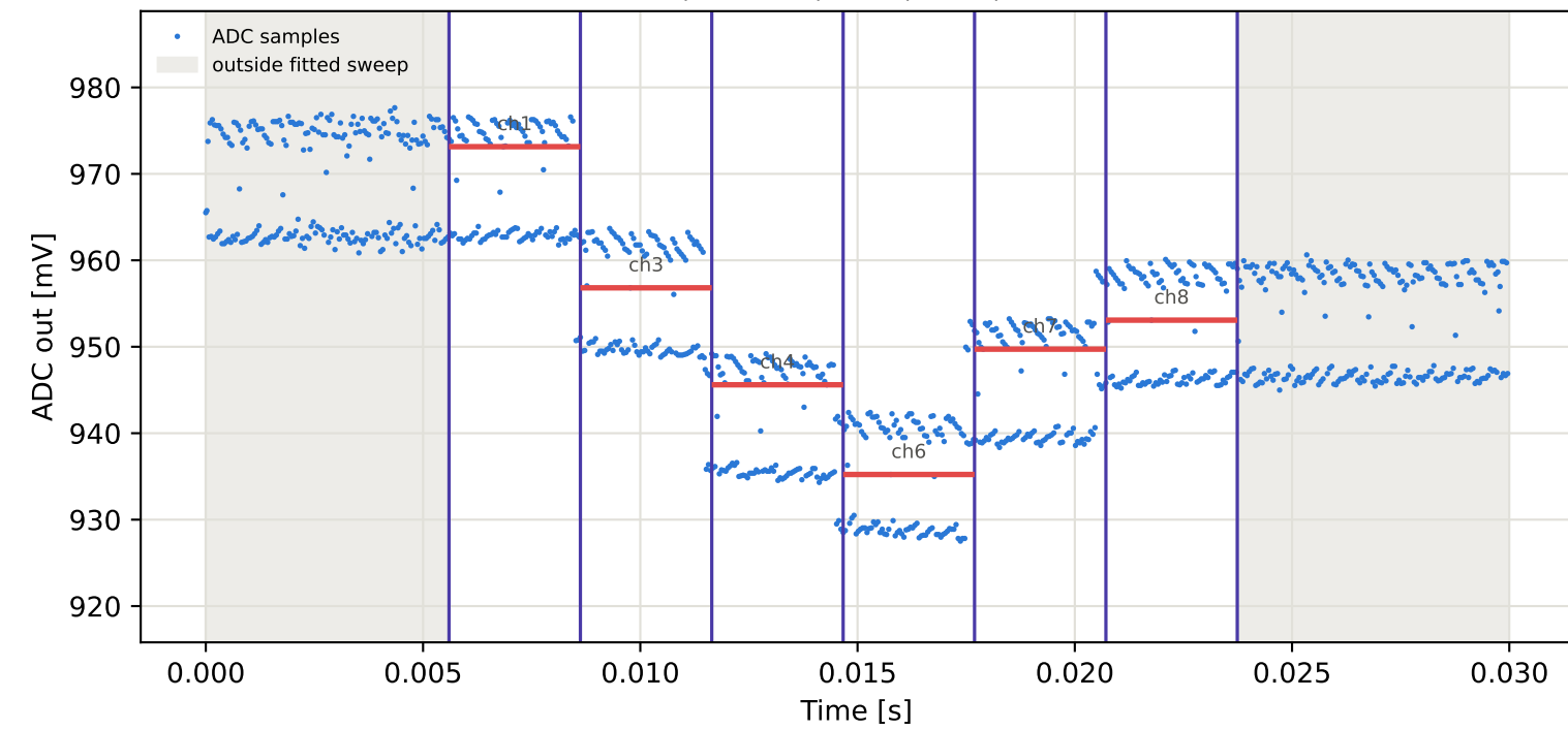
Tag7 &lt;- Tag10 | 875 MHz | run 0 | rep 1 | phase 50.06 deg
