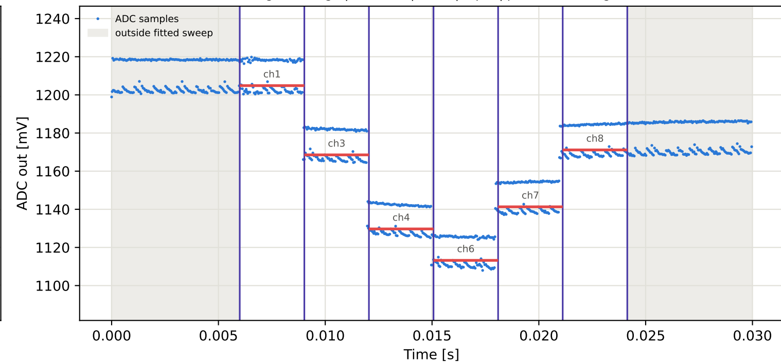
Tag16 &lt;- Tag5 | 875 MHz | run 0 | rep 1 | phase 26.48 deg
