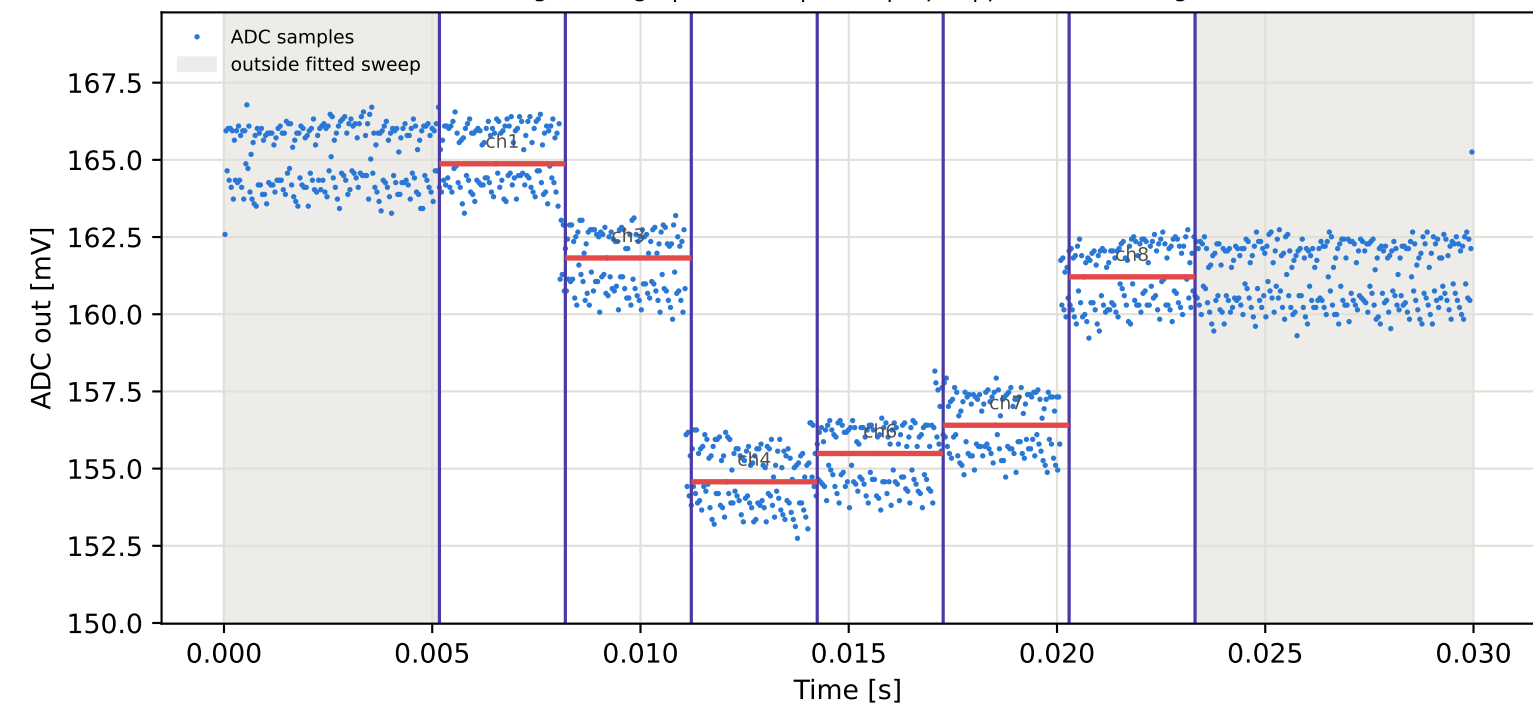
Tag1 &lt;- Tag9 | 835 MHz | run 0 | rep 1 | phase 38.38 deg
