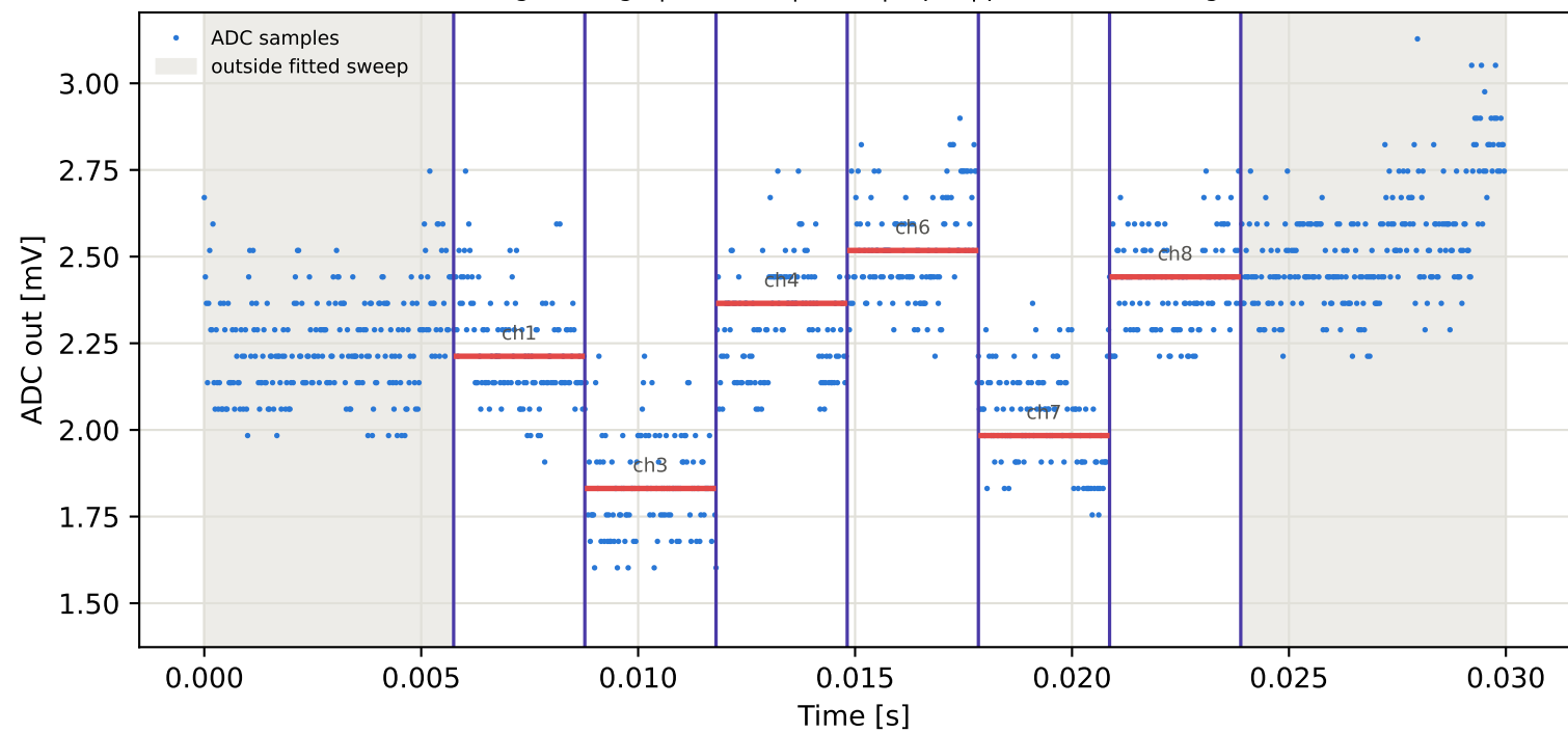
Tag2 &lt;- Tag6 | 775 MHz | run 0 | rep 1 | phase 121.97 deg
