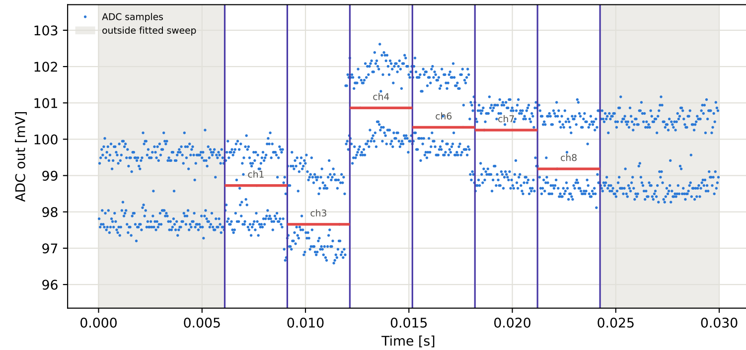
Tag16 &lt;- Tag10 | 785 MHz | run 0 | rep 1 | phase -18.16 deg
