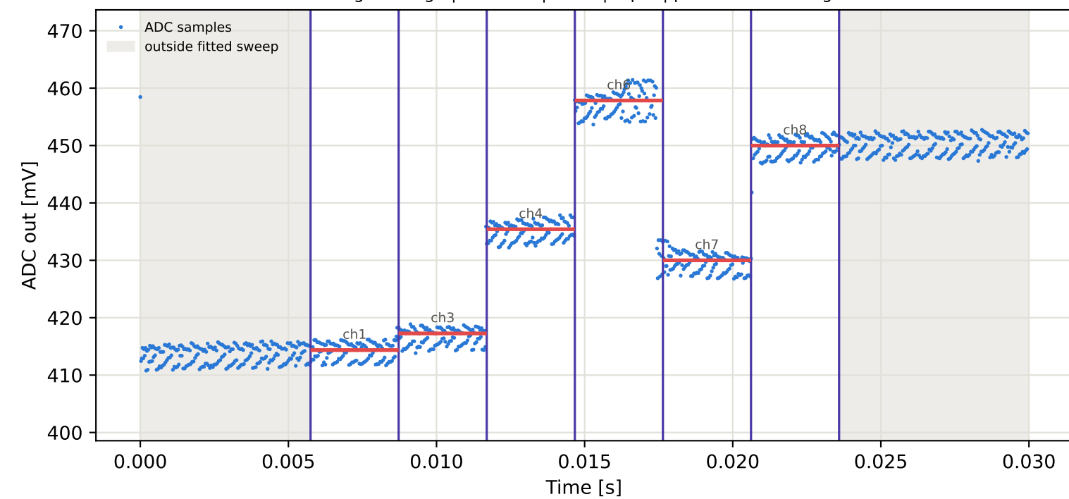
Tag2 &lt;- Tag5 | 865 MHz | run 0 | rep 1 | phase -138.76 deg
