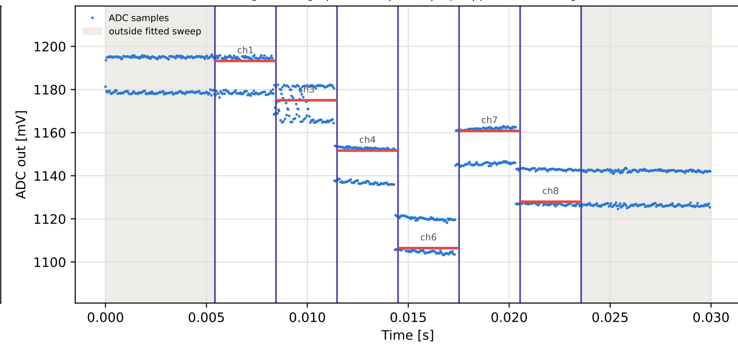
Tag16 &lt;- Tag7 | 875 MHz | run 0 | rep 1 | phase -112.71 deg
