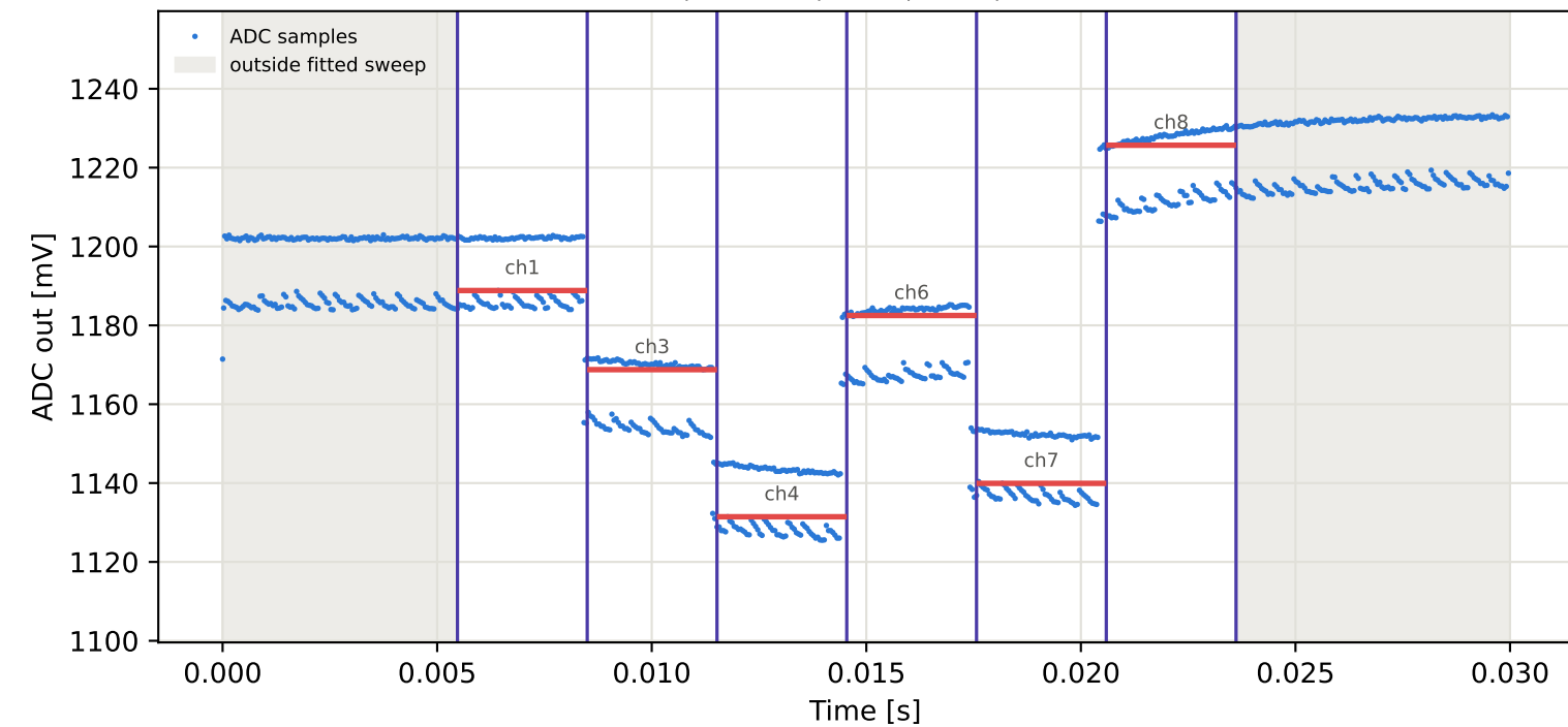
Tag15 &lt;- Tag5 | 905 MHz | run 0 | rep 1 | phase 102.87 deg
