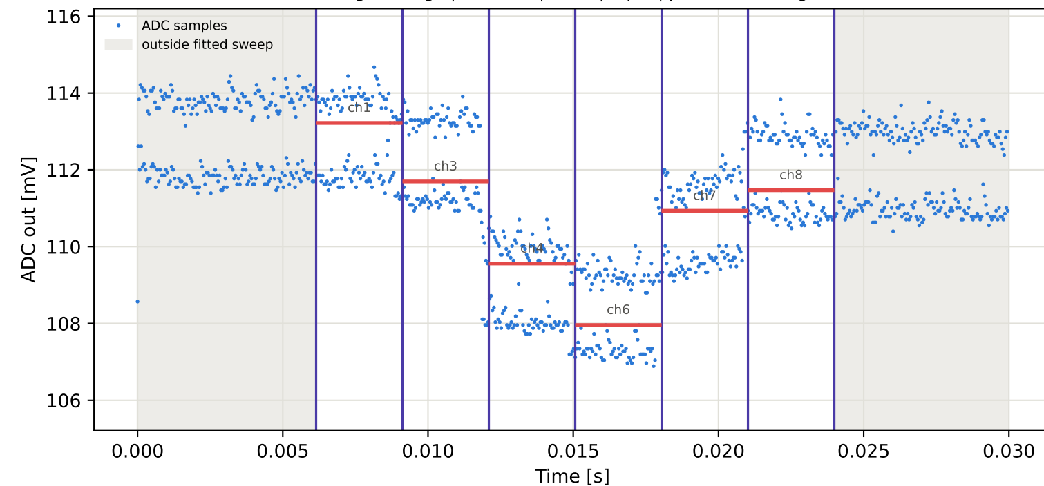
Tag6 &lt;- Tag4 | 805 MHz | run 0 | rep 1 | phase 179.46 deg
