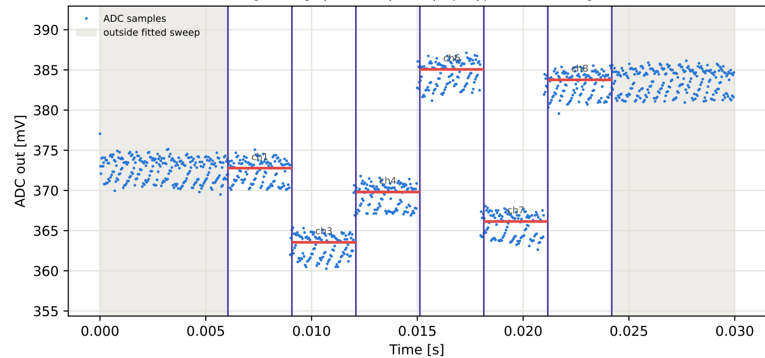
Tag5 &lt;- Tag9 | 825 MHz | run 0 | rep 1 | phase 101.33 deg
