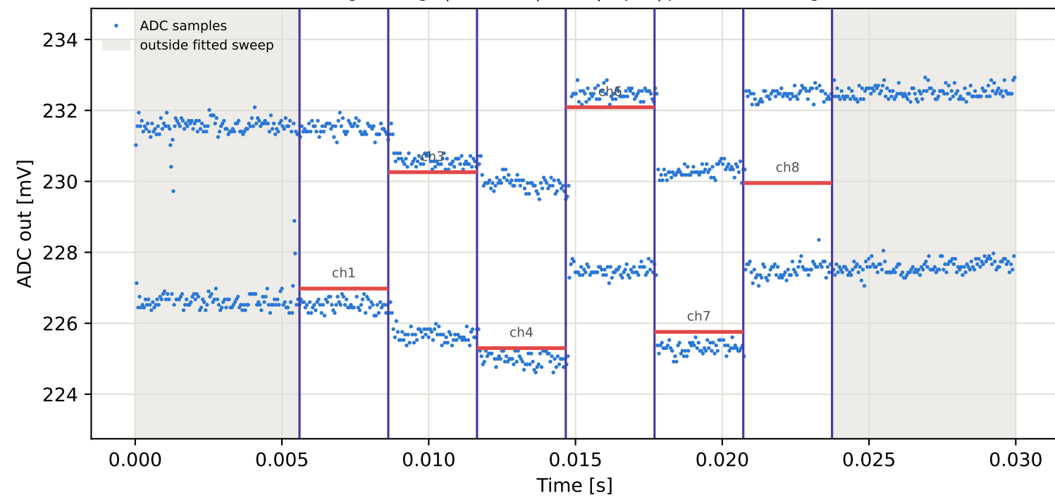
Tag2 &lt;- Tag6 | 935 MHz | run 0 | rep 1 | phase -150.00 deg
