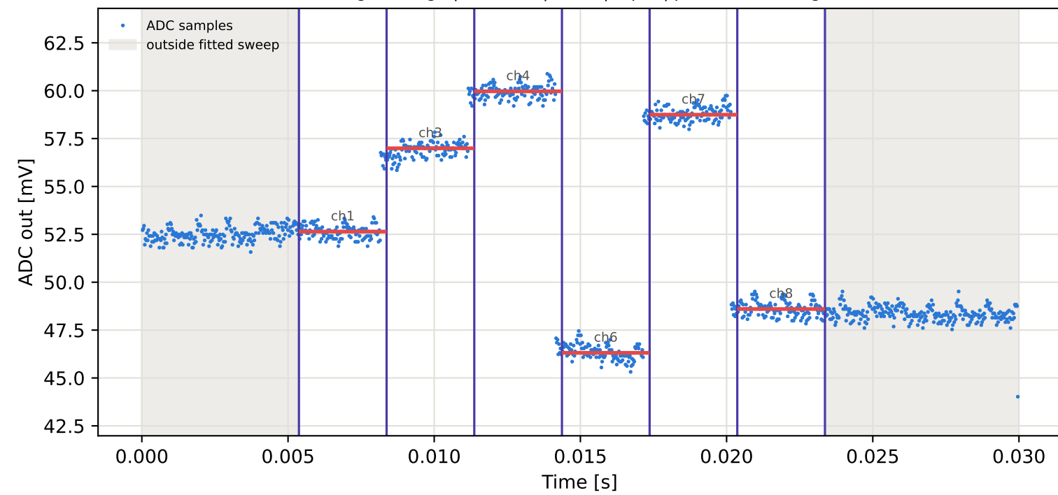
Tag1 &lt;- Tag8 | 955 MHz | run 0 | rep 1 | phase -22.96 deg
