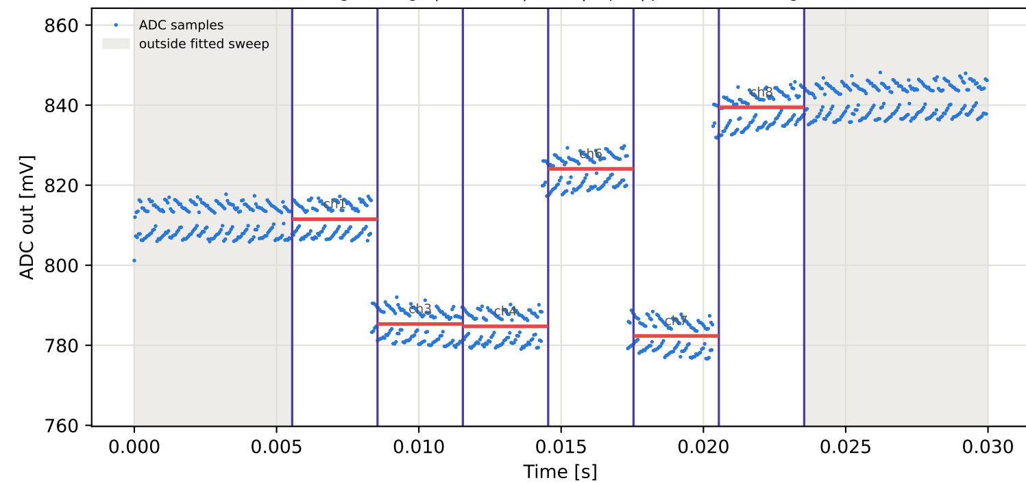
Tag8 &lt;- Tag10 | 895 MHz | run 0 | rep 1 | phase 92.02 deg
