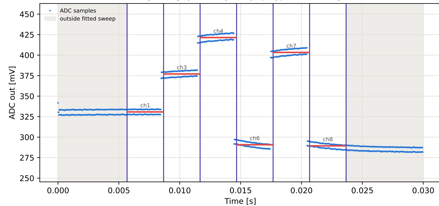
Tag4 &lt;- Tag7 | 945 MHz | run 0 | rep 1 | phase -131.51 deg
