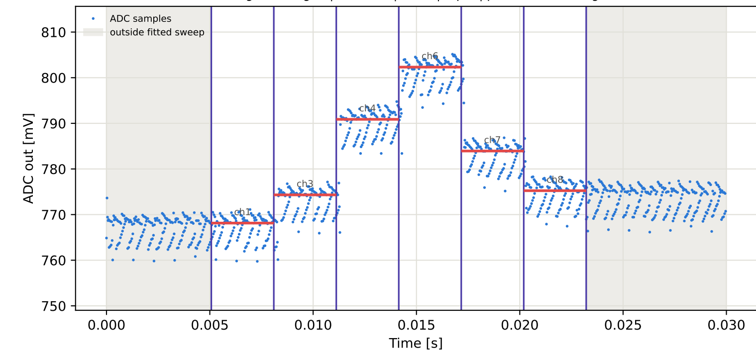
Tag15 &lt;- Tag10 | 925 MHz | run 0 | rep 1 | phase -135.62 deg
