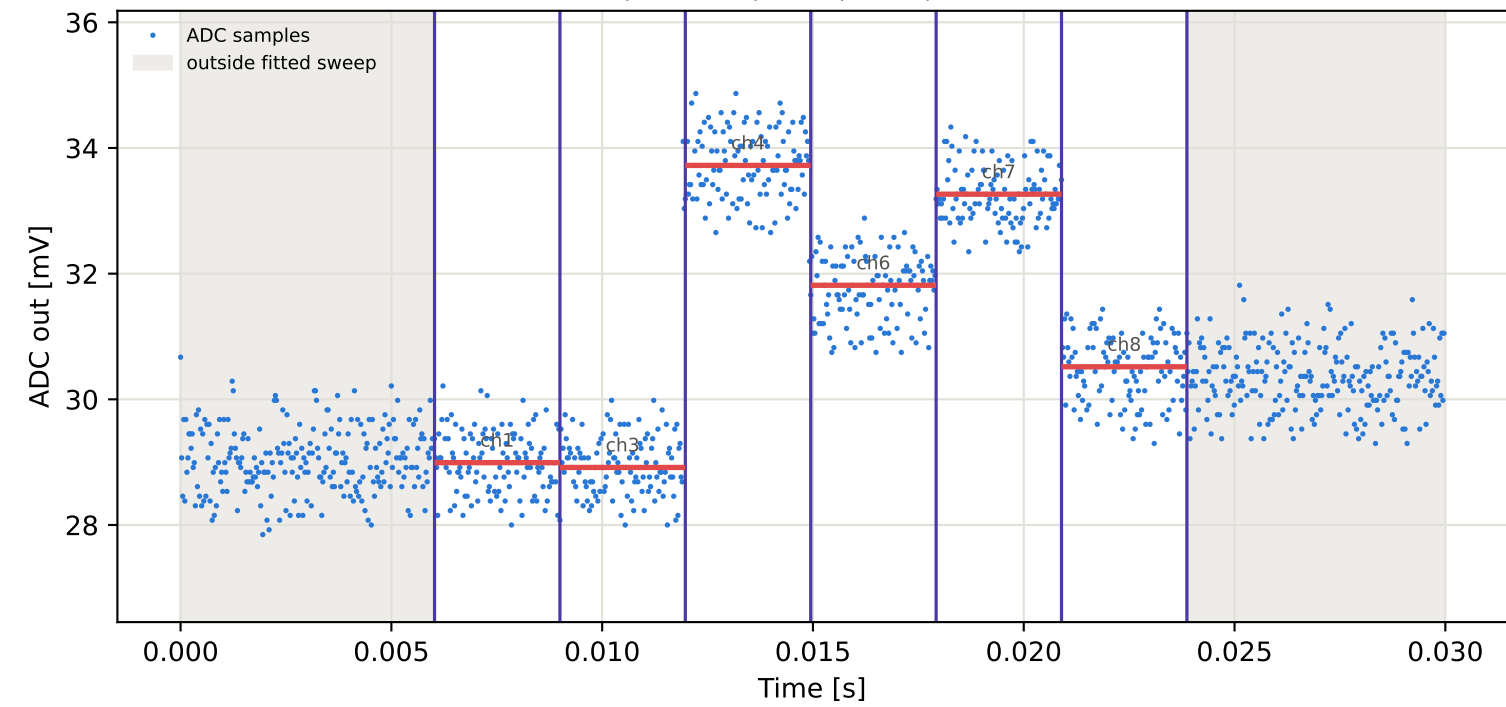
Tag1 &lt;- Tag4 | 795 MHz | run 0 | rep 1 | phase -102.24 deg
