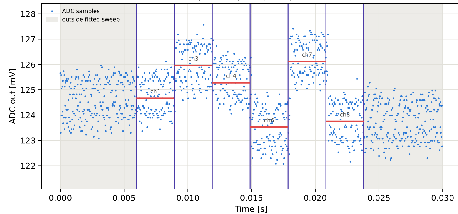
Tag4 &lt;- Tag15 | 795 MHz | run 0 | rep 1 | phase -166.32 deg
