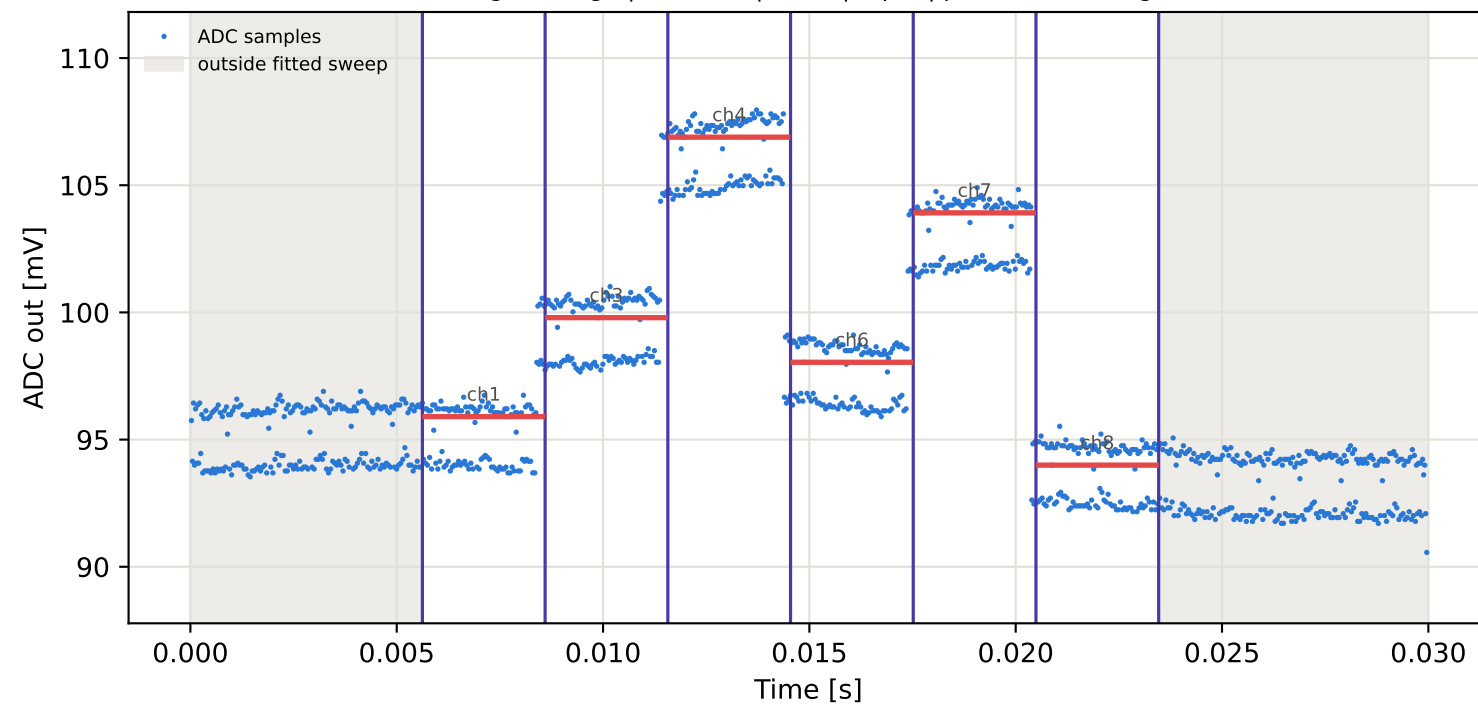
Tag1 &lt;- Tag7 | 945 MHz | run 0 | rep 1 | phase -177.35 deg
