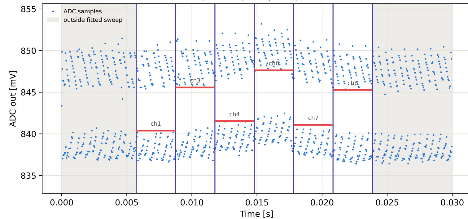
Tag16 &lt;- Tag4 | 945 MHz | run 0 | rep 1 | phase -44.11 deg
