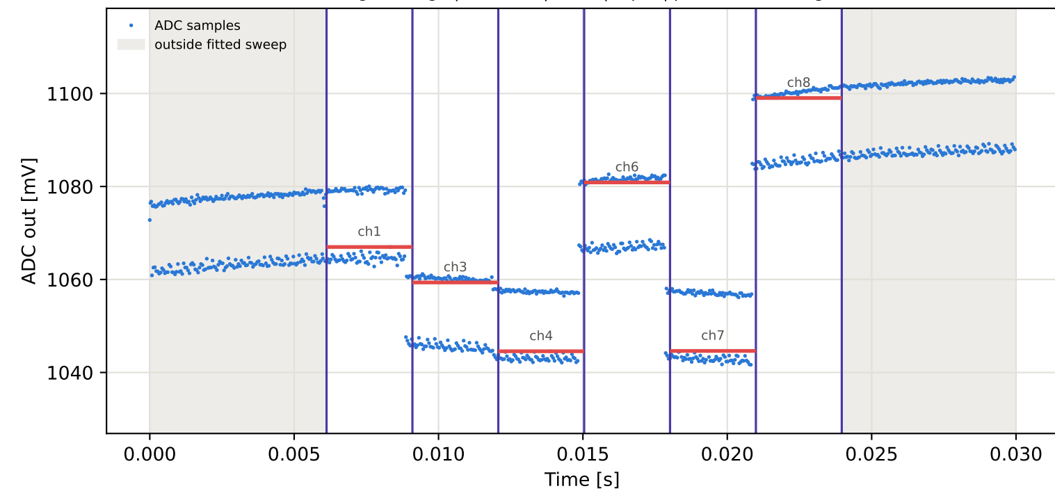
Tag3 &lt;- Tag6 | 875 MHz | run 0 | rep 1 | phase -169.45 deg
