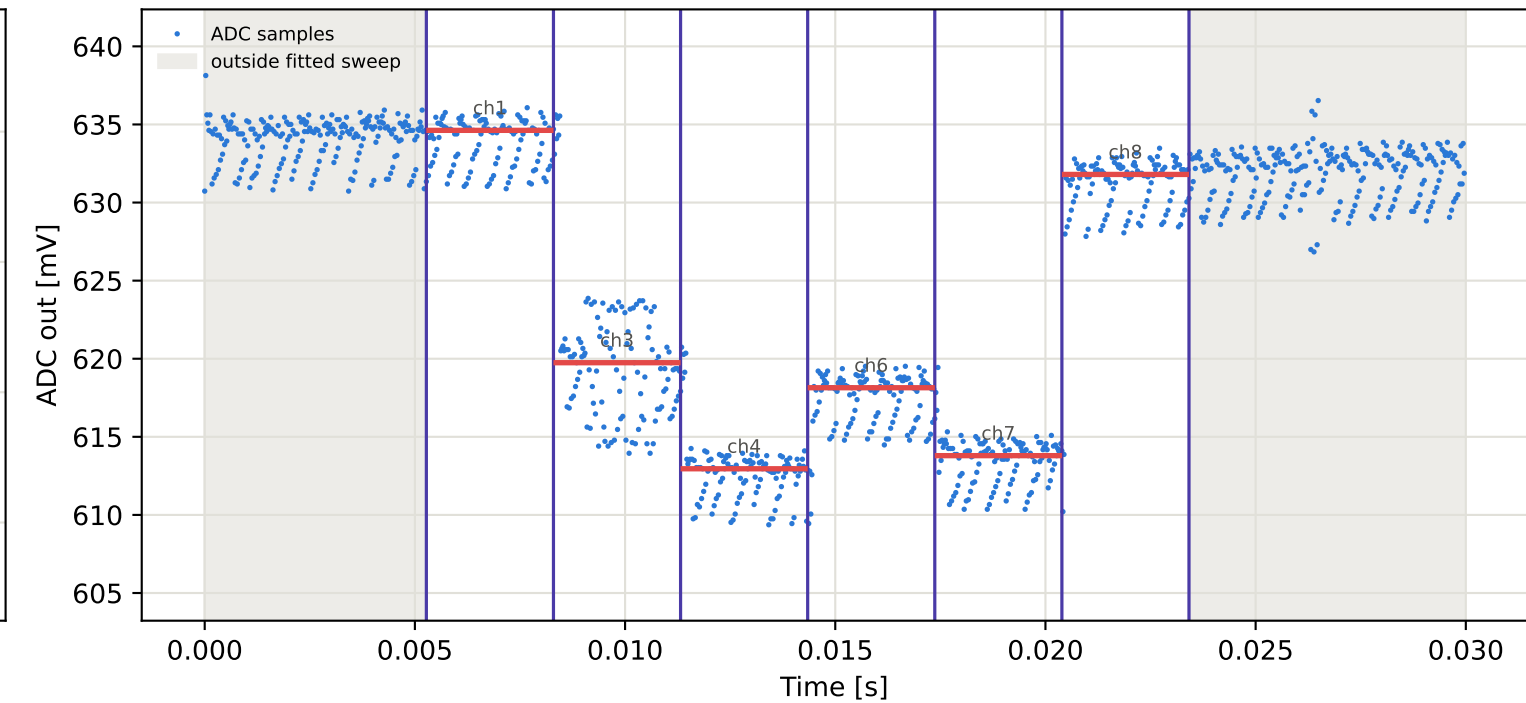
Tag15 &lt;- Tag6 | 865 MHz | run 0 | rep 1 | phase 97.82 deg
