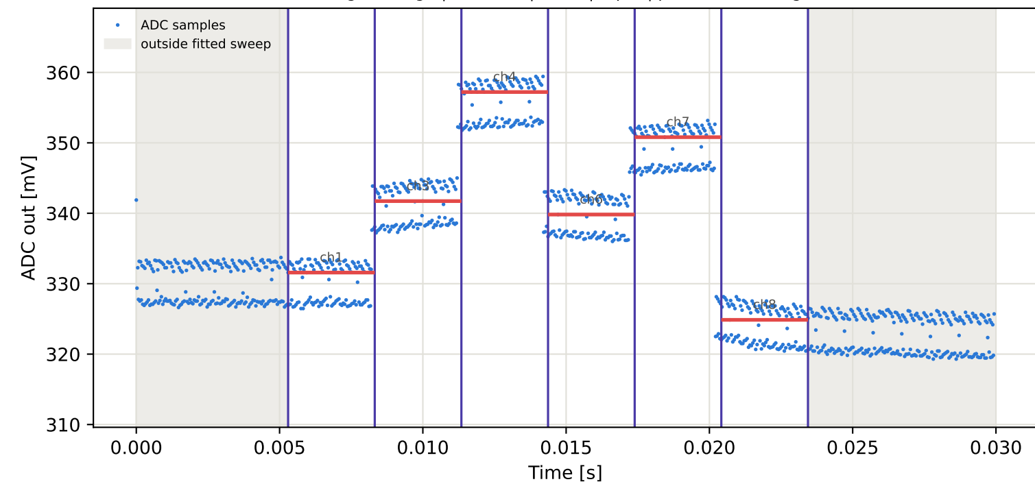
Tag1 &lt;- Tag7 | 925 MHz | run 0 | rep 1 | phase -179.12 deg
