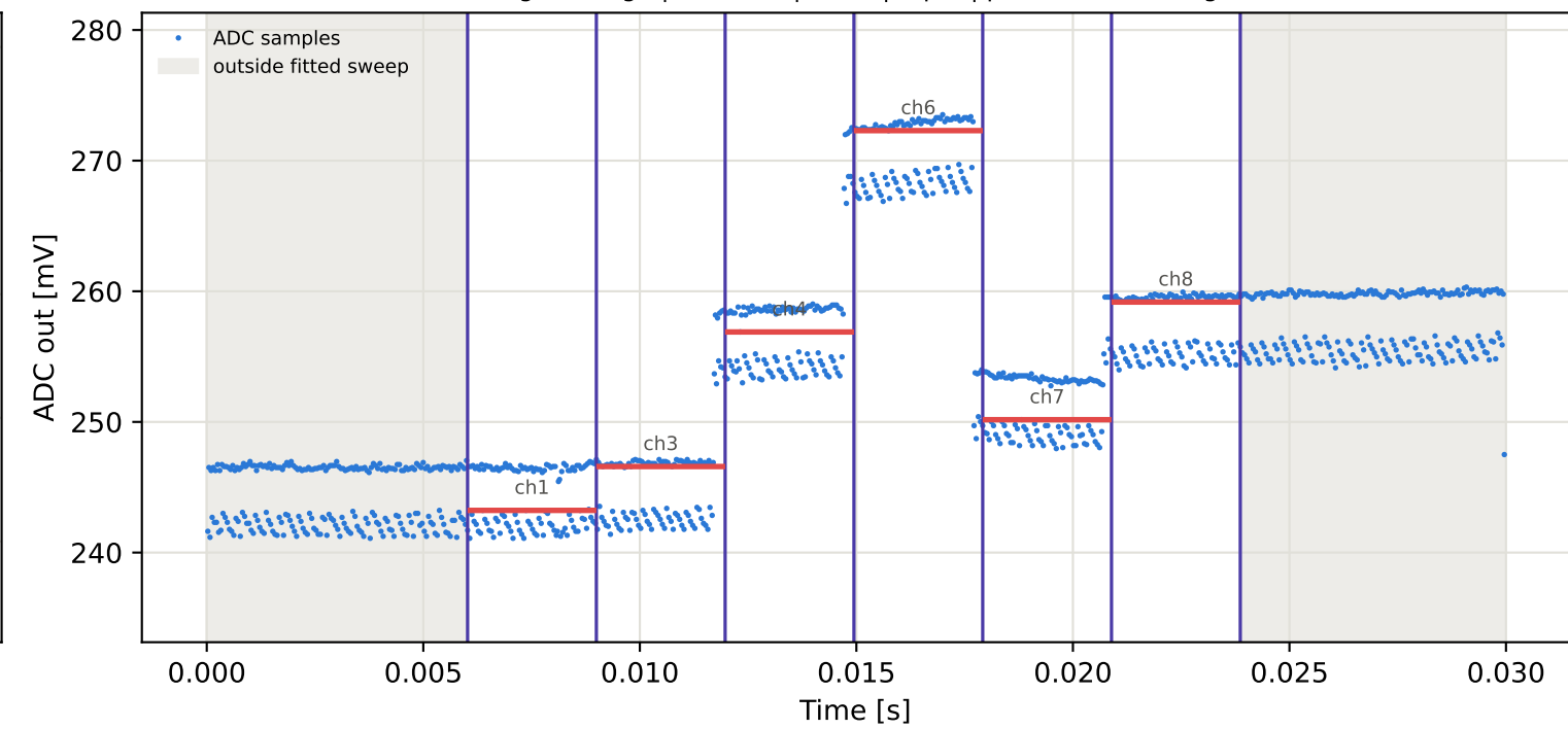
Tag3 &lt;- Tag9 | 925 MHz | run 0 | rep 1 | phase 40.26 deg
