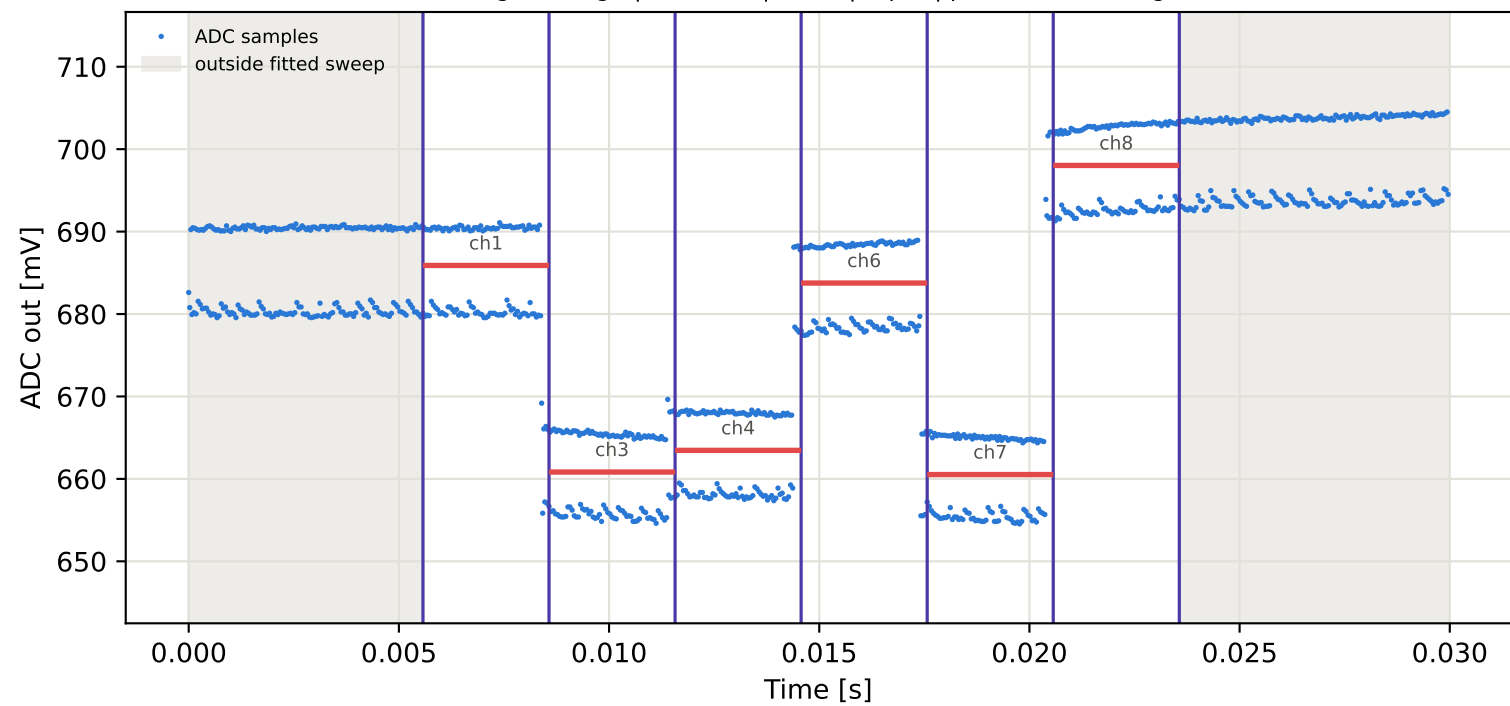
Tag8 &lt;- Tag5 | 855 MHz | run 0 | rep 1 | phase 84.57 deg
