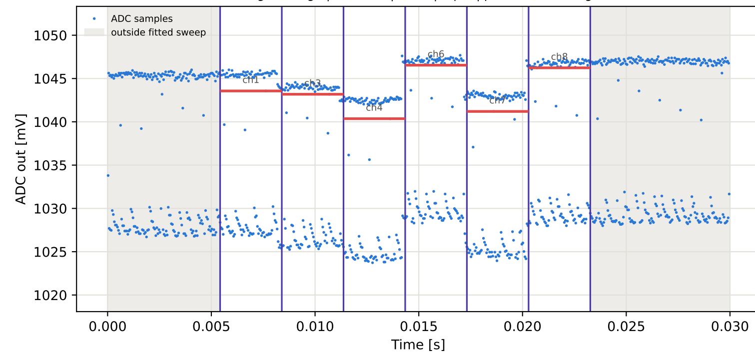
Tag8 &lt;- Tag6 | 955 MHz | run 0 | rep 1 | phase 128.17 deg
