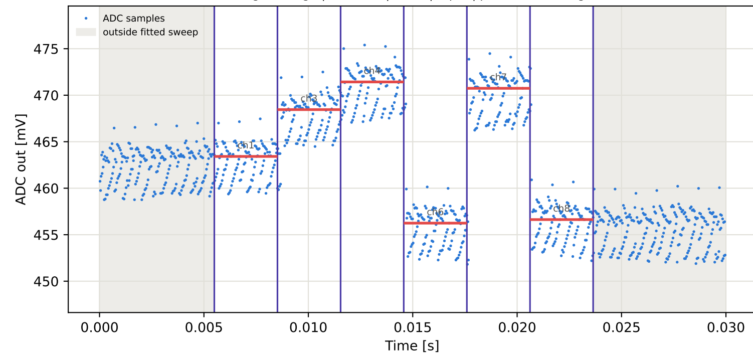
Tag5 &lt;- Tag8 | 915 MHz | run 0 | rep 1 | phase -112.03 deg
