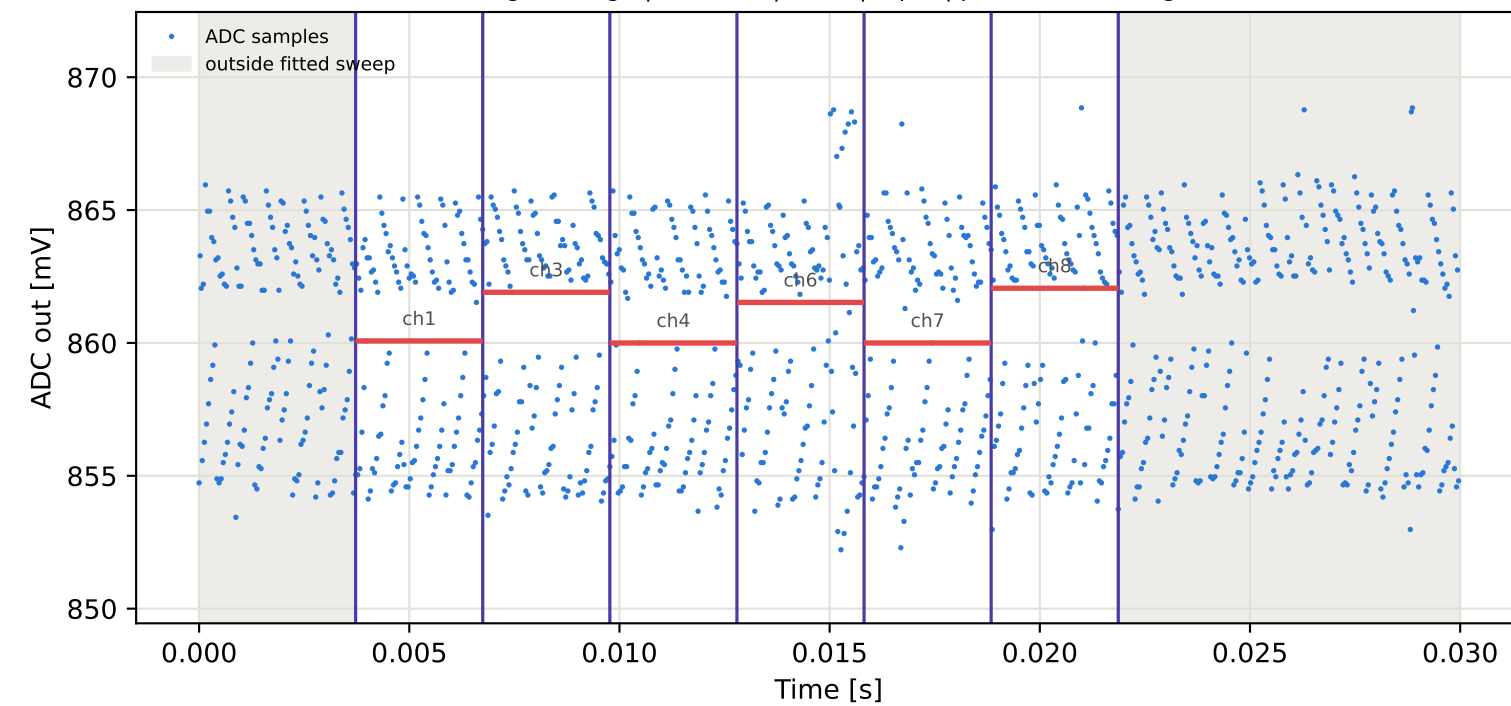
Tag8 &lt;- Tag4 | 965 MHz | run 0 | rep 1 | phase -179.82 deg
