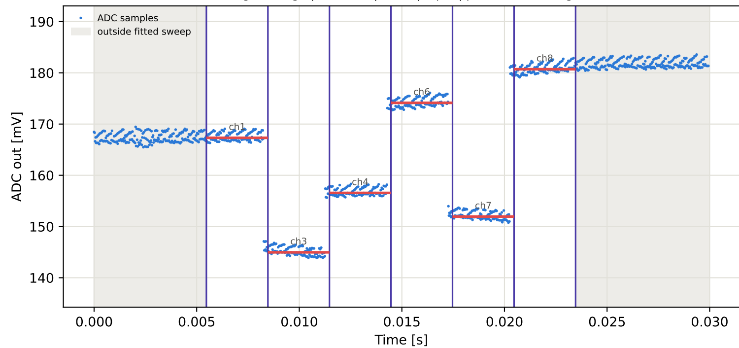
Tag2 &lt;- Tag5 | 845 MHz | run 0 | rep 1 | phase -110.77 deg
