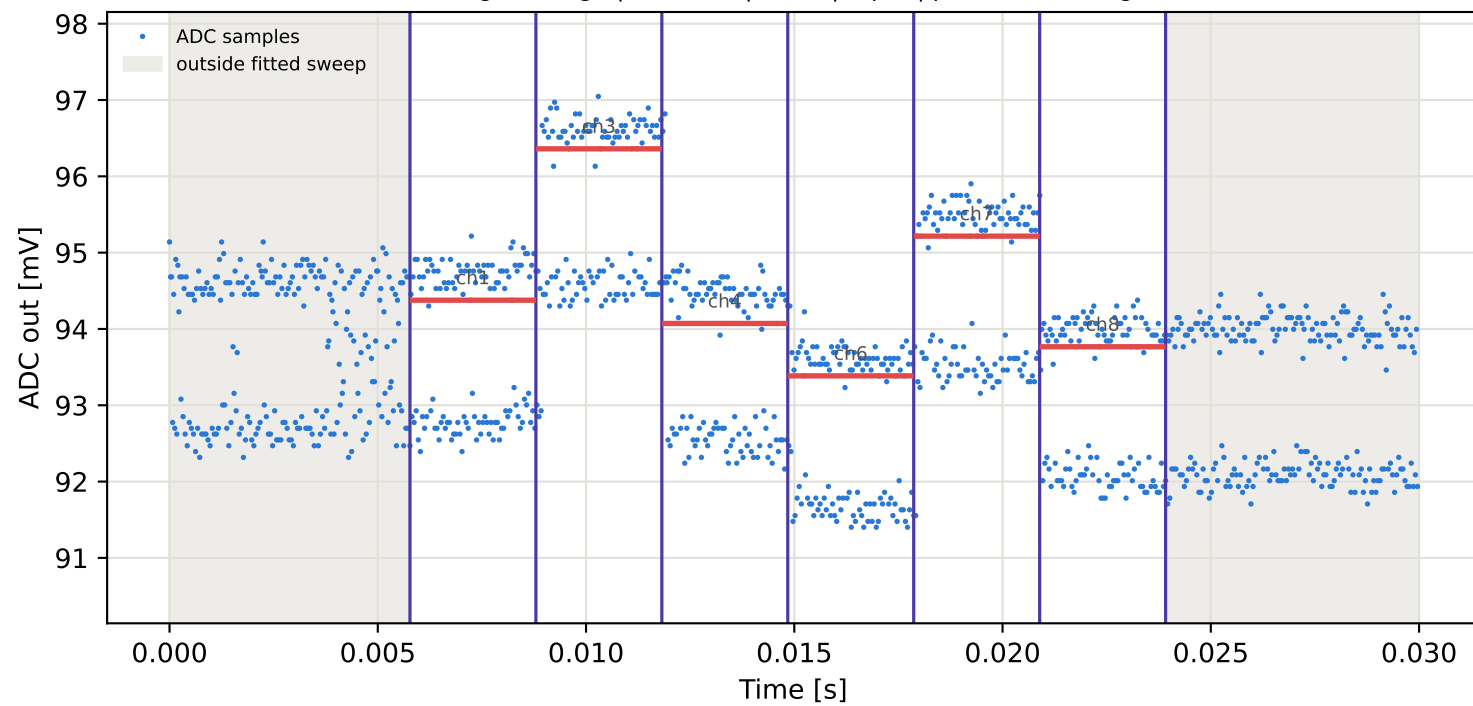
Tag3 &lt;- Tag6 | 795 MHz | run 0 | rep 1 | phase -0.57 deg
