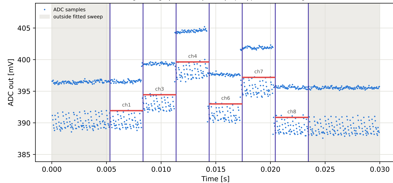
Tag3 &lt;- Tag8 | 955 MHz | run 0 | rep 1 | phase -66.60 deg
