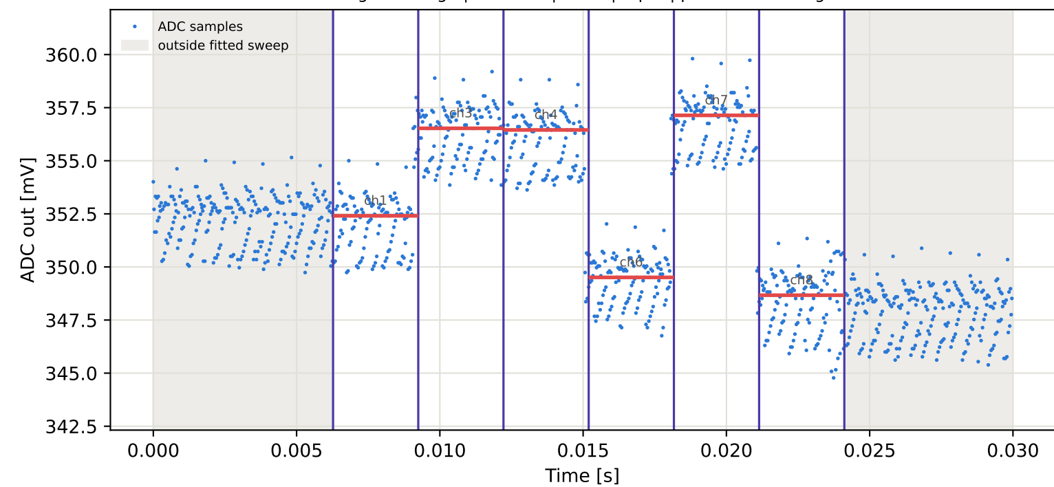
Tag15 &lt;- Tag4 | 855 MHz | run 0 | rep 1 | phase 77.91 deg
