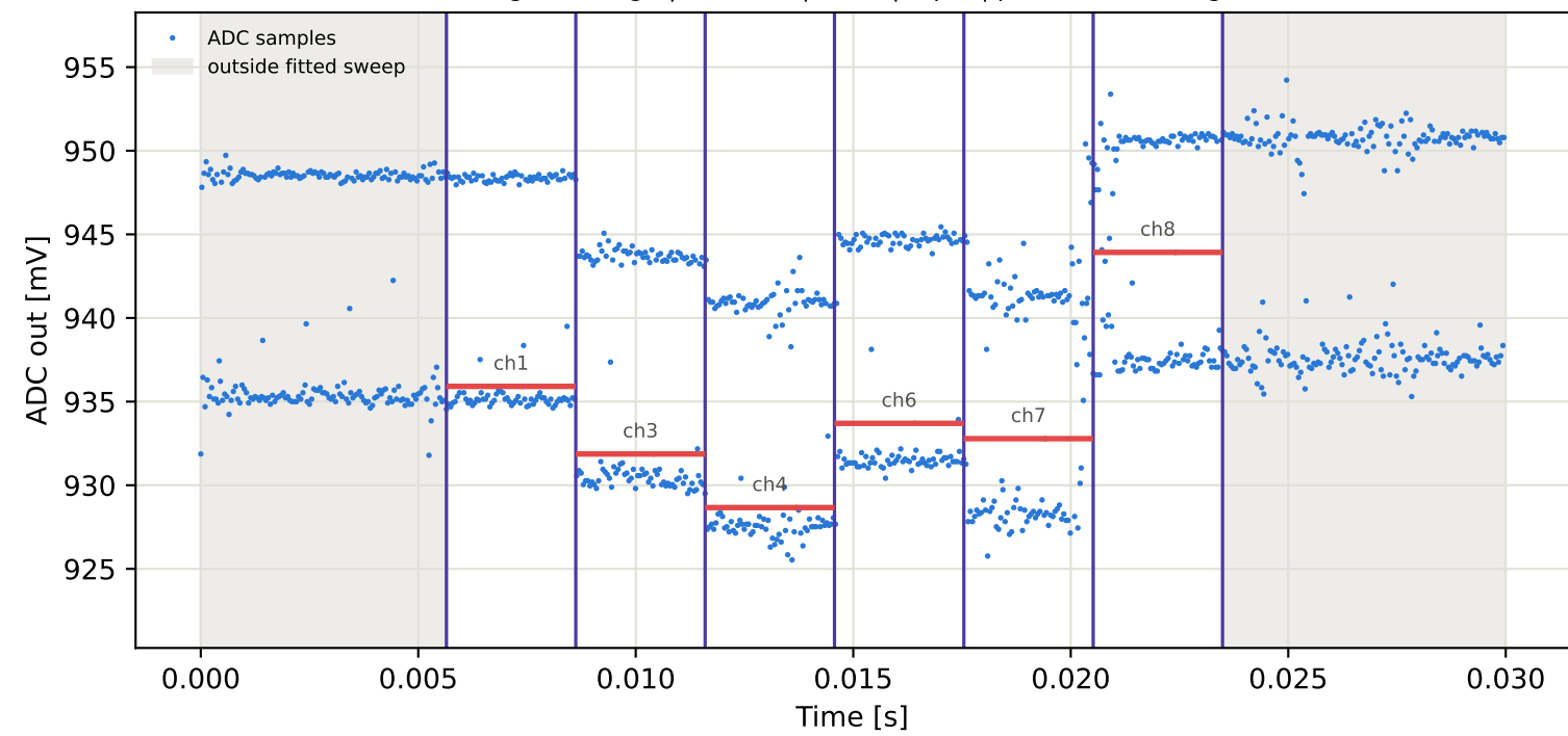
Tag15 &lt;- Tag4 | 875 MHz | run 0 | rep 1 | phase 170.50 deg
