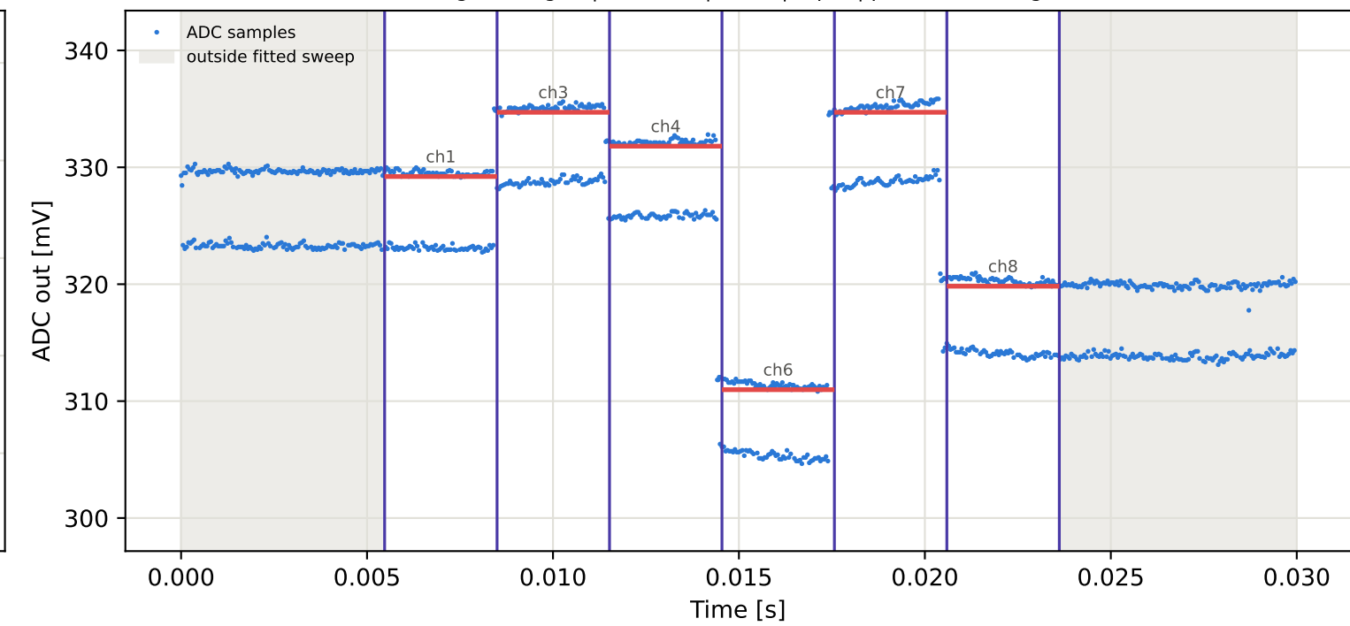
Tag6 &lt;- Tag3 | 965 MHz | run 0 | rep 1 | phase -10.43 deg
