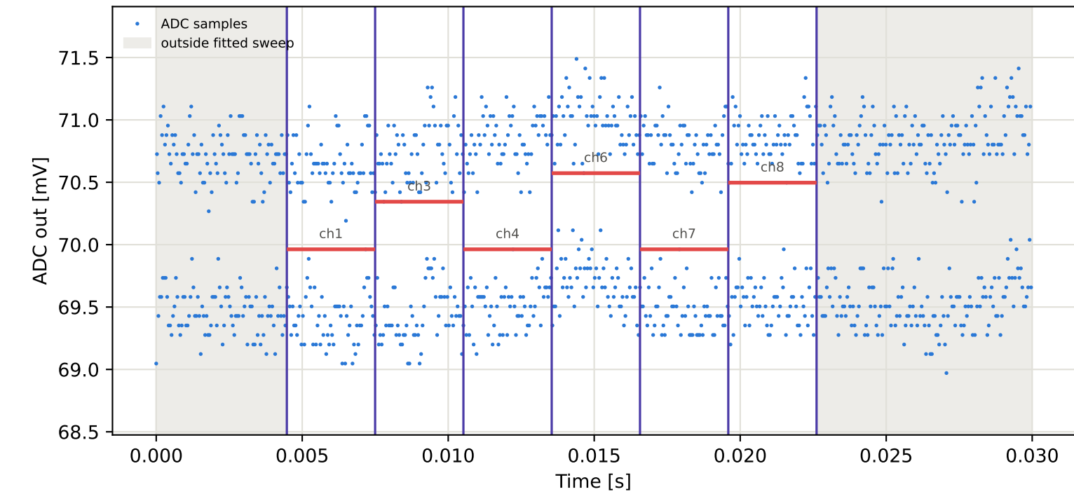
Tag16 &lt;- Tag15 | 785 MHz | run 0 | rep 1 | phase -75.46 deg
