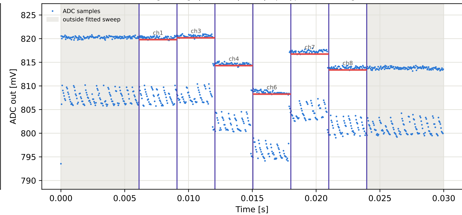
Tag5 &lt;- Tag9 | 905 MHz | run 0 | rep 1 | phase -139.79 deg
