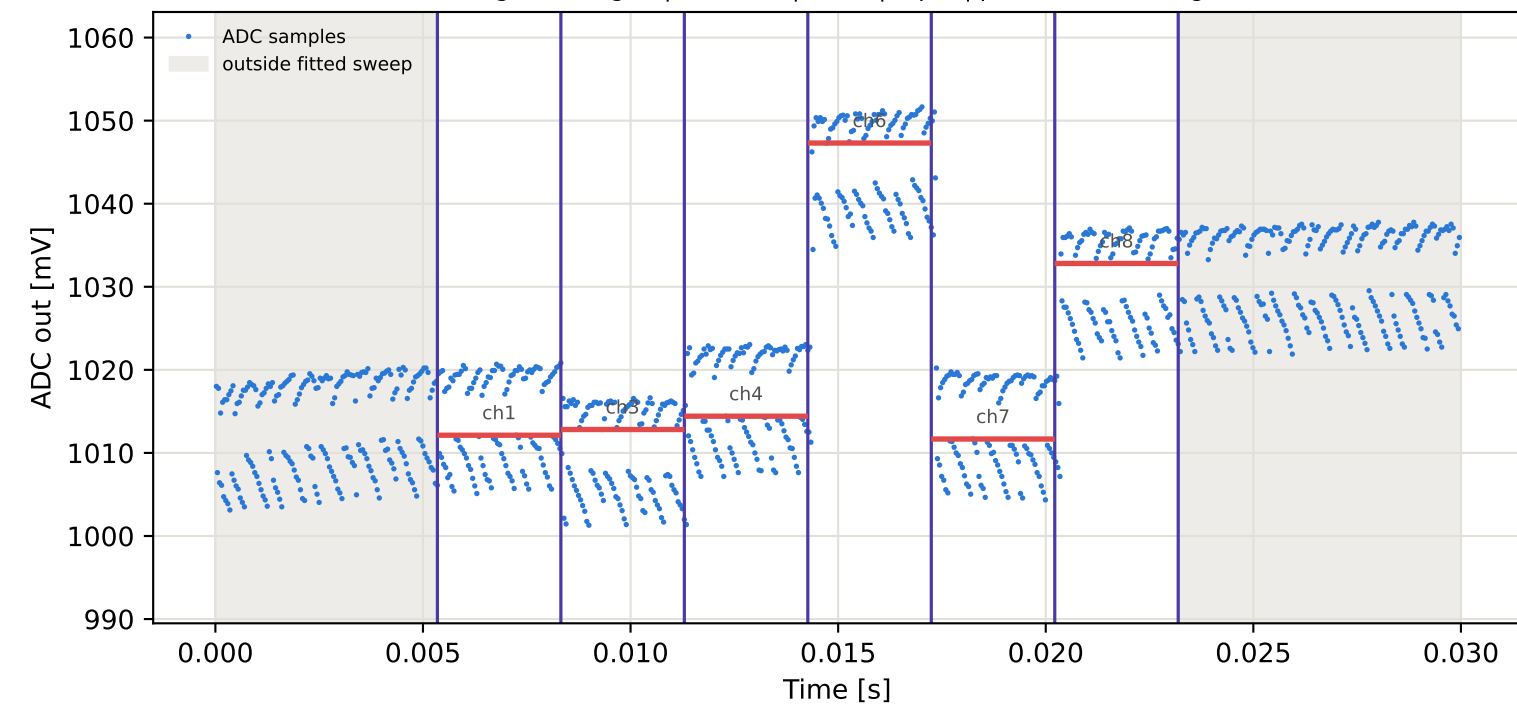
Tag10 &lt;- Tag2 | 935 MHz | run 0 | rep 1 | phase -80.50 deg
