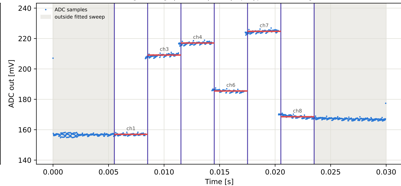
Tag16 &lt;- Tag5 | 825 MHz | run 0 | rep 1 | phase -59.41 deg
