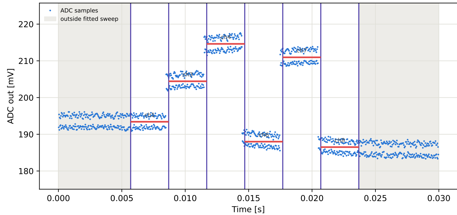
Tag10 &lt;- Tag9 | 985 MHz | run 0 | rep 1 | phase -44.86 deg
