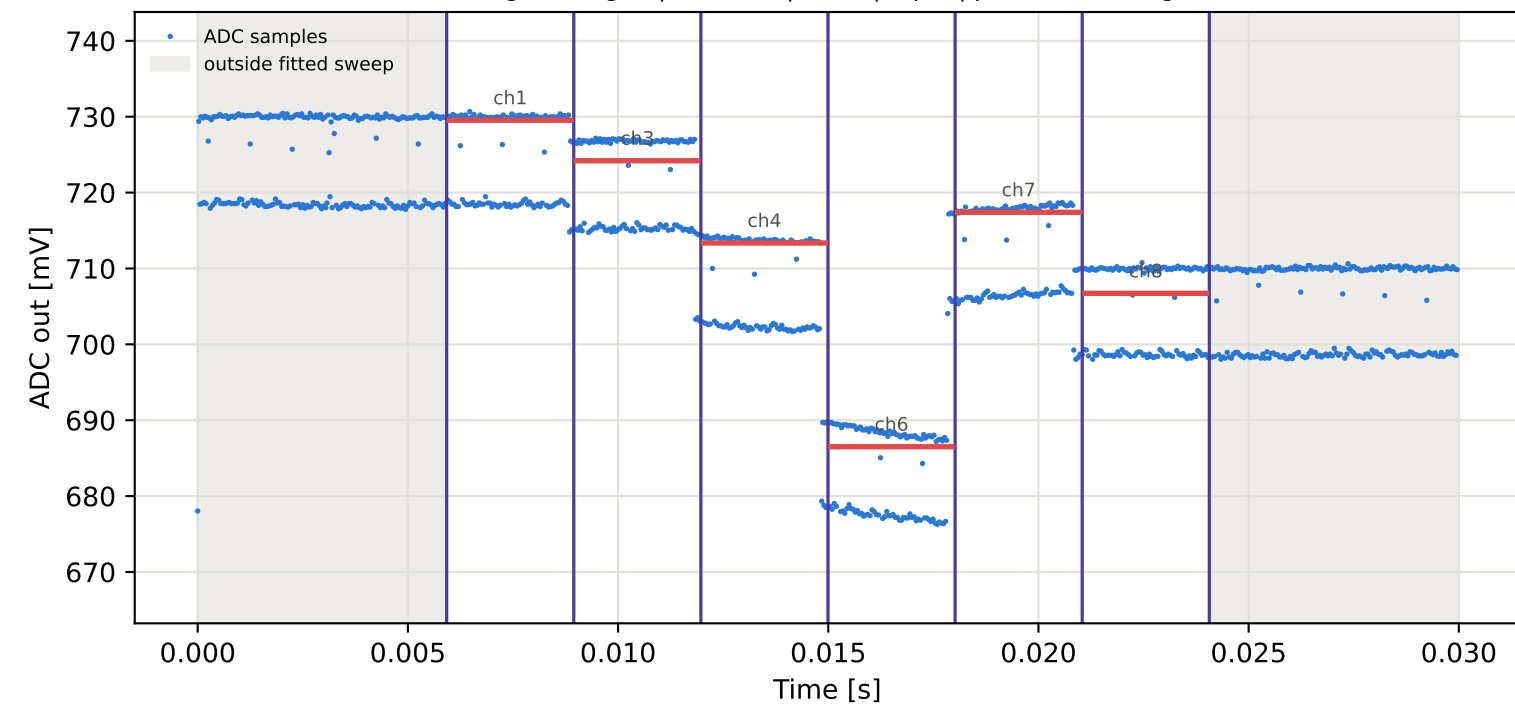
Tag4 &lt;- Tag16 | 895 MHz | run 0 | rep 1 | phase -37.64 deg
