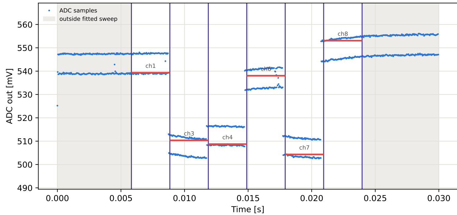
Tag7 &lt;- Tag3 | 855 MHz | run 0 | rep 1 | phase -98.99 deg
