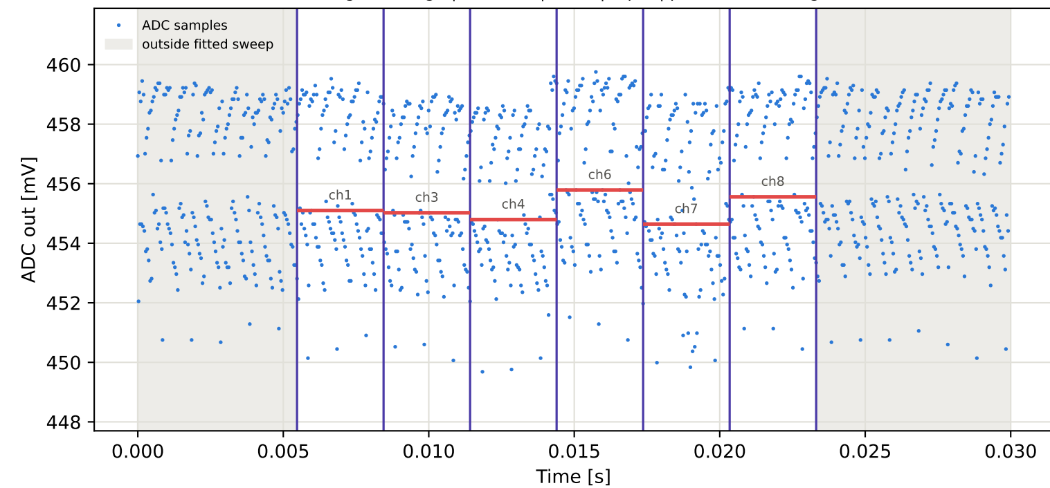
Tag16 &lt;- Tag4 | 995 MHz | run 0 | rep 1 | phase 87.71 deg
