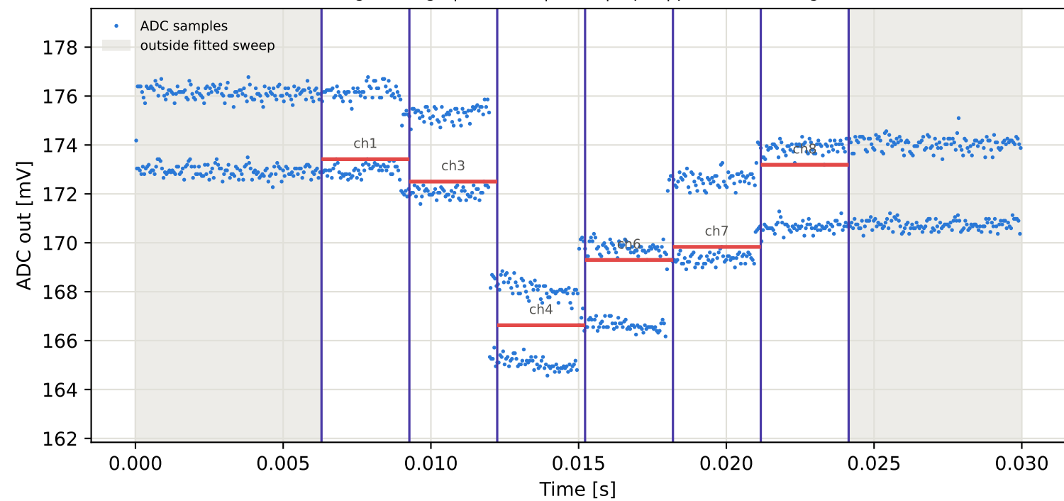
Tag1 &lt;- Tag7 | 995 MHz | run 0 | rep 1 | phase -36.39 deg
