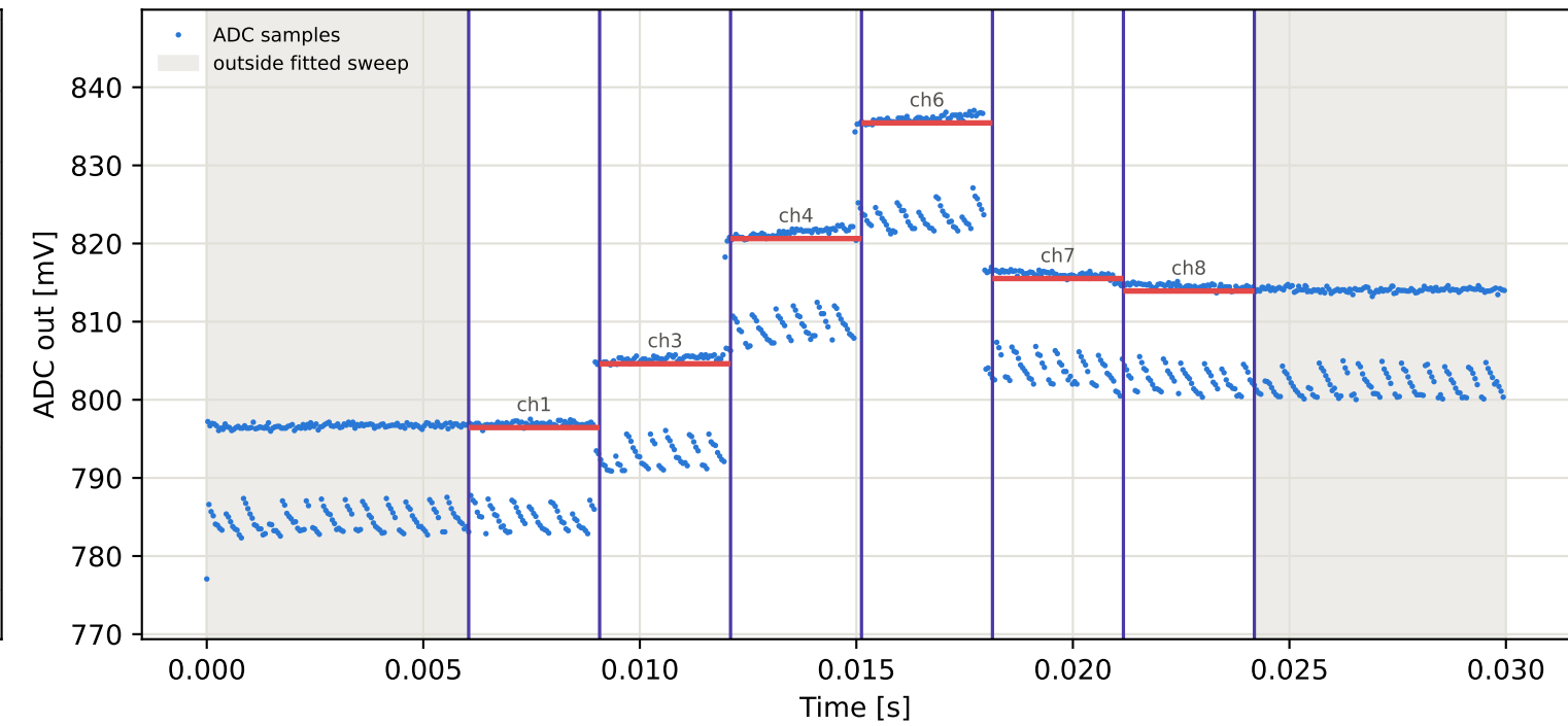
Tag6 &lt;- Tag10 | 905 MHz | run 0 | rep 1 | phase 119.86 deg
