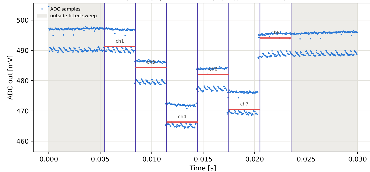
Tag4 &lt;- Tag9 | 865 MHz | run 0 | rep 1 | phase -162.72 deg
