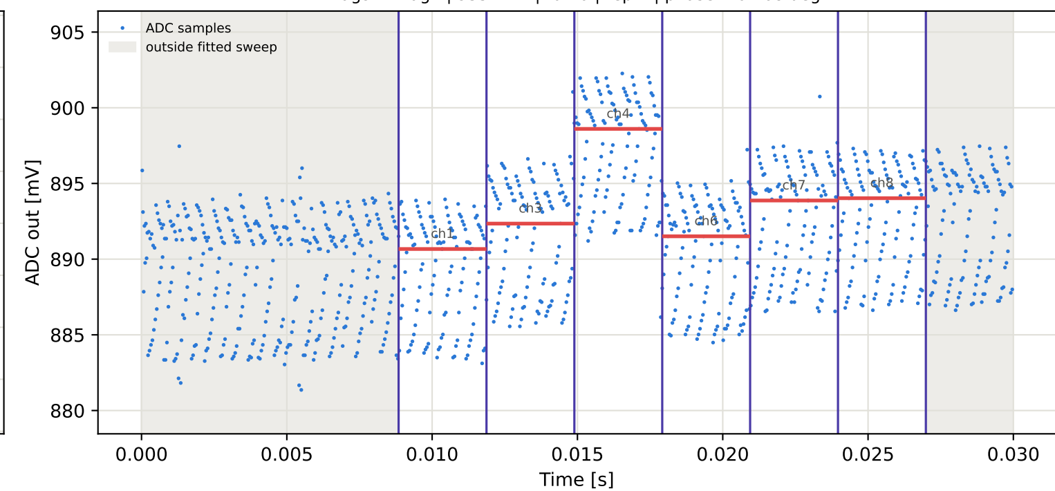
Tag9 &lt;- Tag6 | 935 MHz | run 0 | rep 1 | phase 158.31 deg
