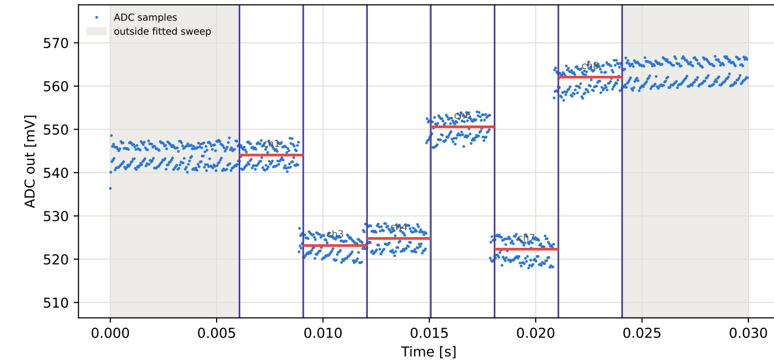
Tag2 &lt;- Tag15 | 875 MHz | run 0 | rep 1 | phase -6.96 deg
