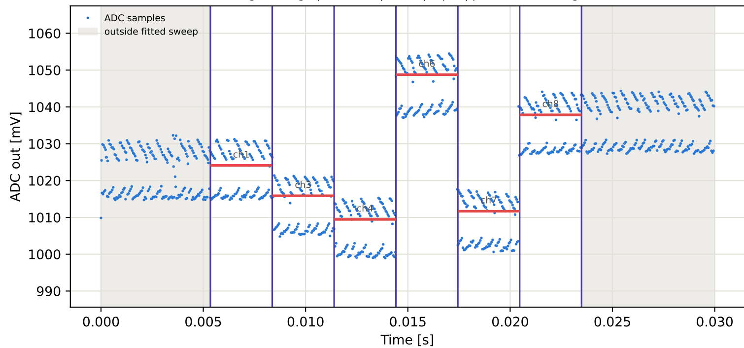
Tag8 &lt;- Tag5 | 975 MHz | run 0 | rep 1 | phase -43.38 deg
