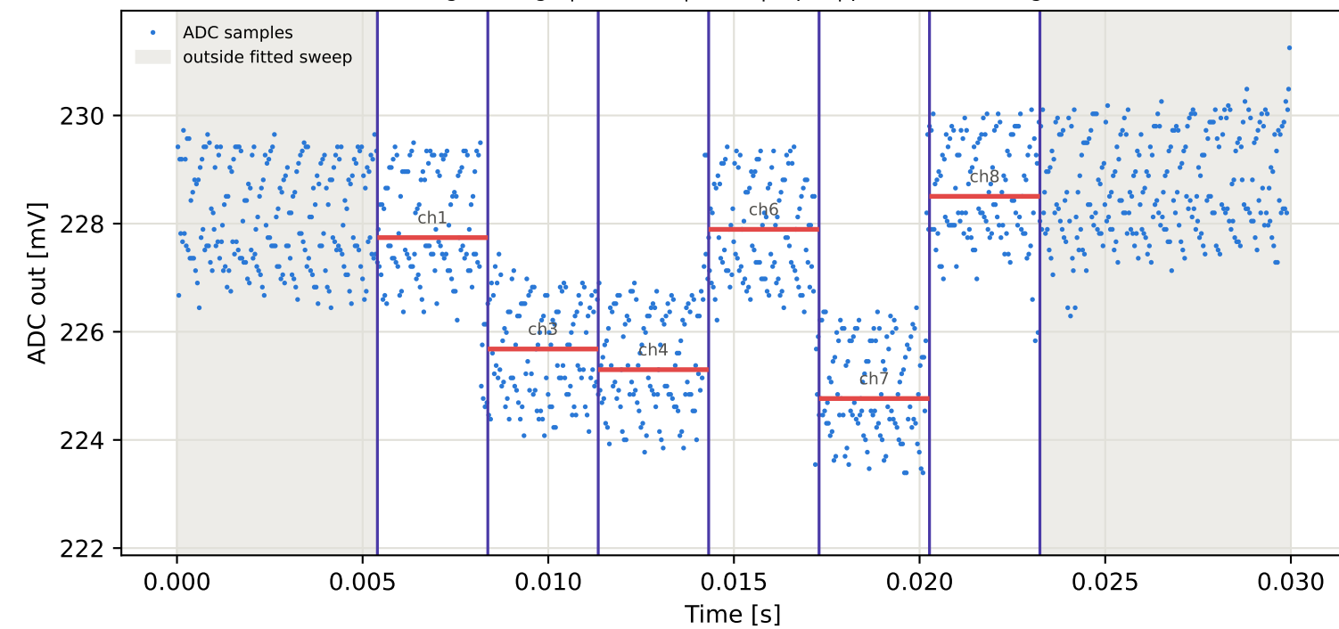
Tag3 &lt;- Tag10 | 855 MHz | run 0 | rep 1 | phase 103.42 deg
