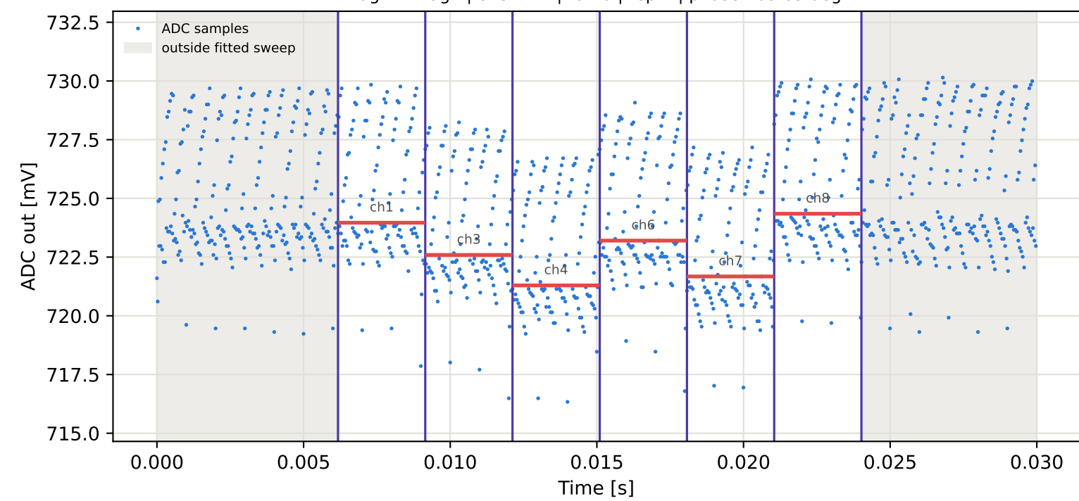
Tag7 &lt;- Tag4 | 845 MHz | run 0 | rep 1 | phase 105.47 deg
