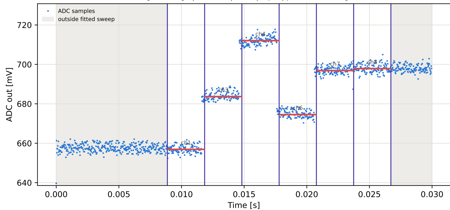
Tag15 &lt;- Tag10 | 885 MHz | run 0 | rep 1 | phase 51.03 deg
