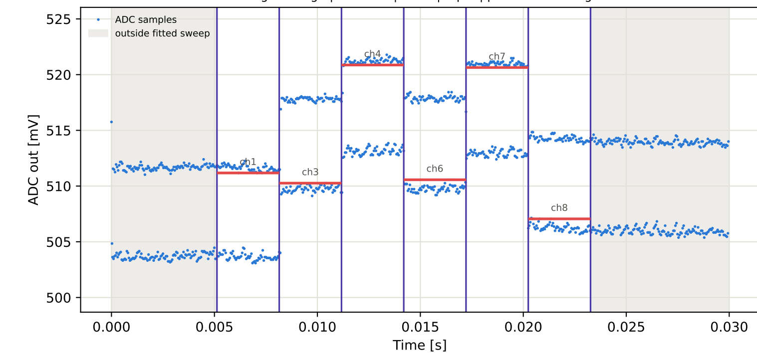
Tag6 &lt;- Tag1 | 855 MHz | run 0 | rep 1 | phase -76.07 deg
