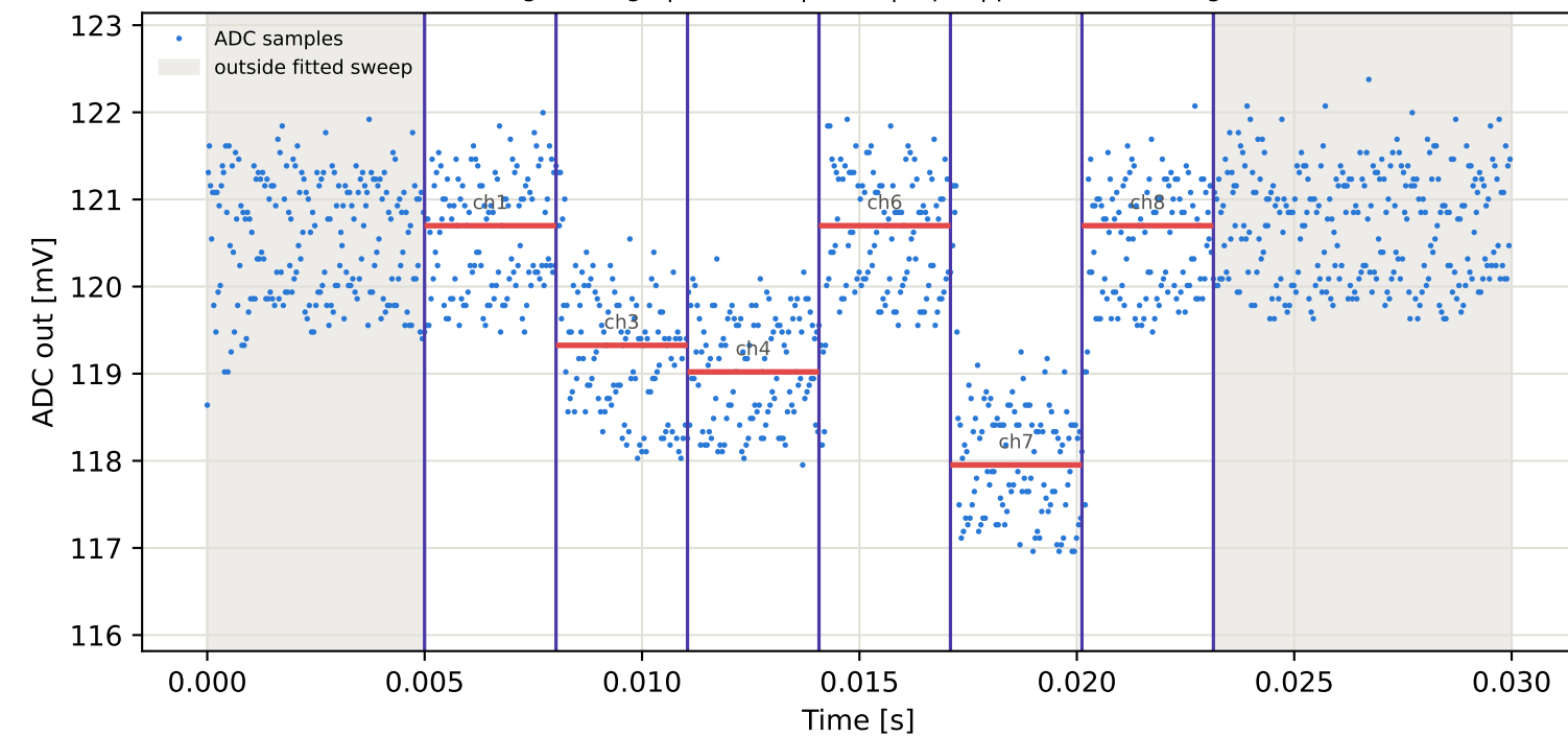
Tag7 &lt;- Tag5 | 785 MHz | run 0 | rep 1 | phase 41.81 deg
