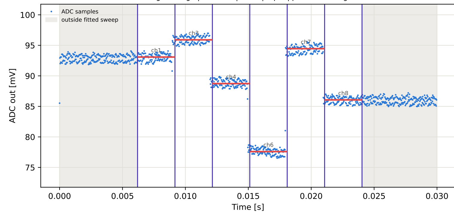
Tag4 &lt;- Tag7 | 995 MHz | run 0 | rep 1 | phase -46.72 deg
