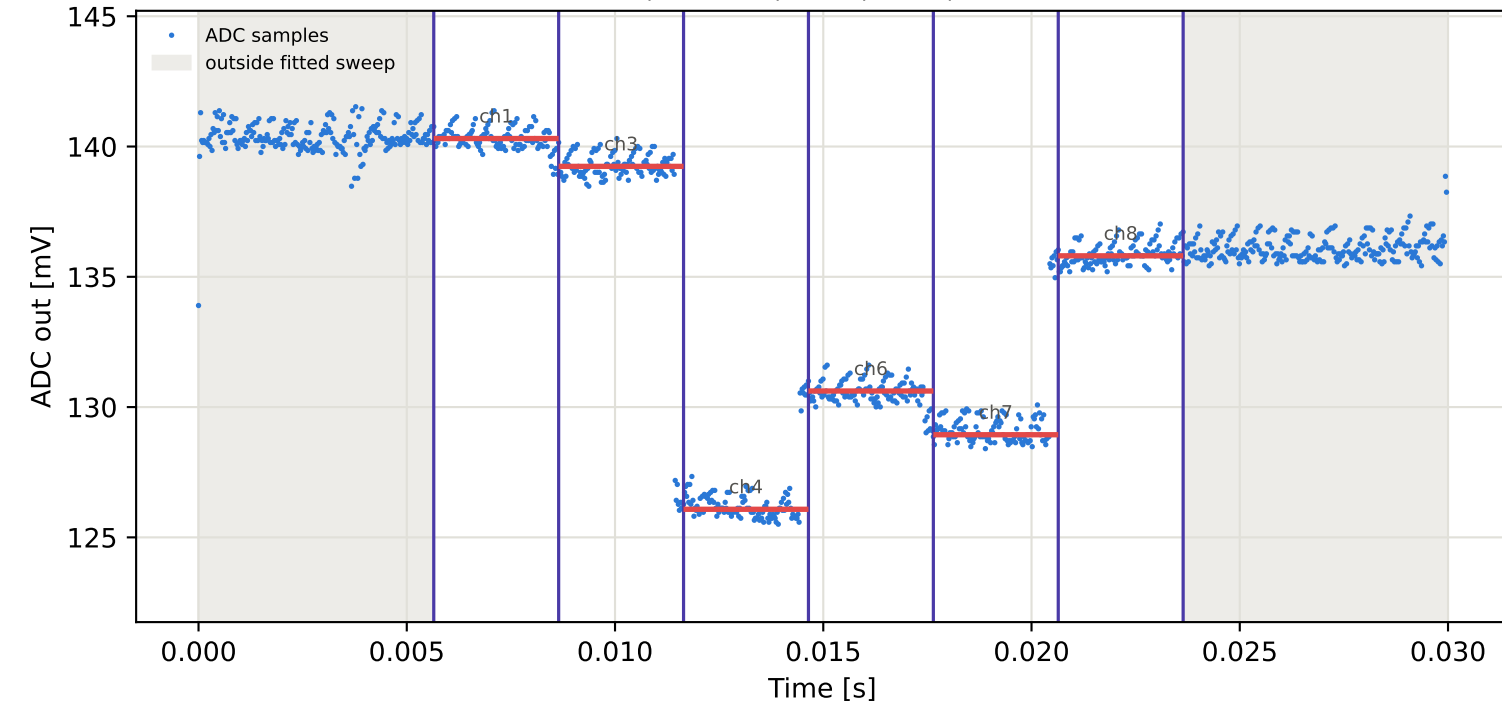
Tag7 &lt;- Tag5 | 805 MHz | run 0 | rep 1 | phase 73.14 deg
