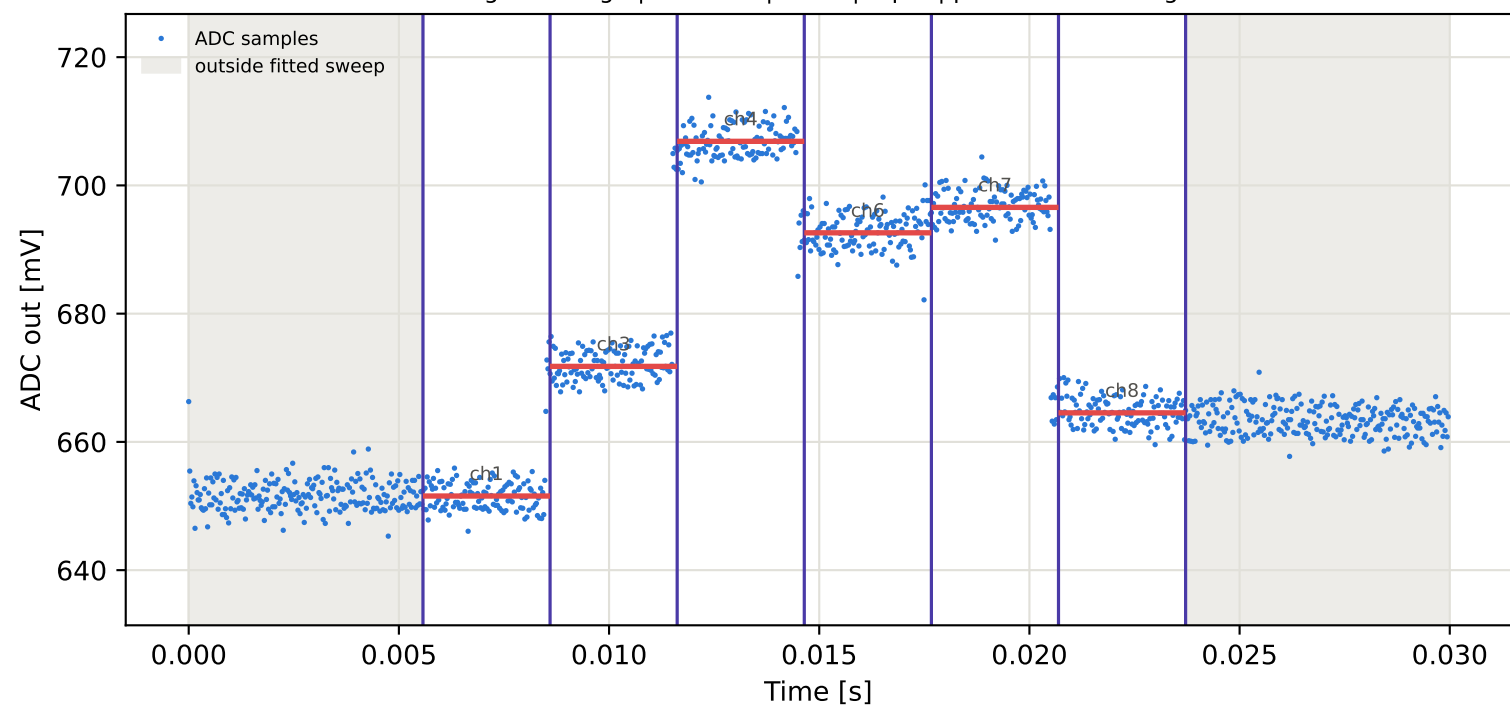
Tag10 &lt;- Tag9 | 885 MHz | run 0 | rep 1 | phase -94.33 deg
