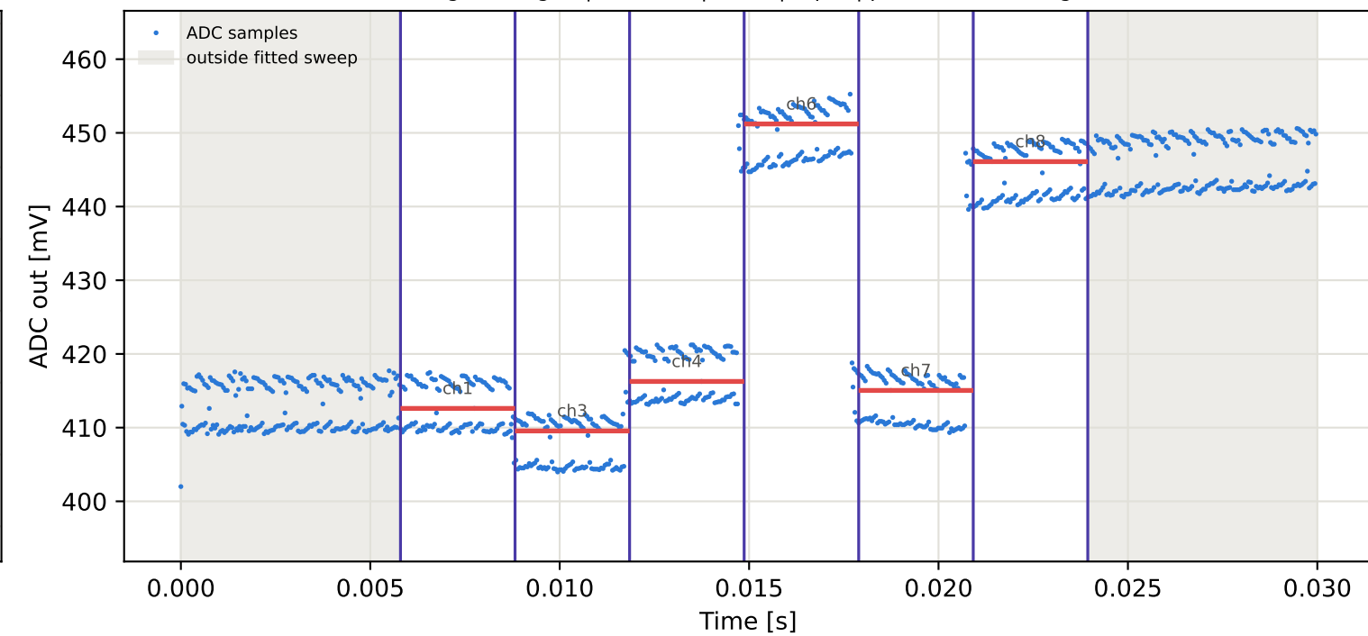
Tag6 &lt;- Tag3 | 895 MHz | run 0 | rep 1 | phase -97.66 deg
