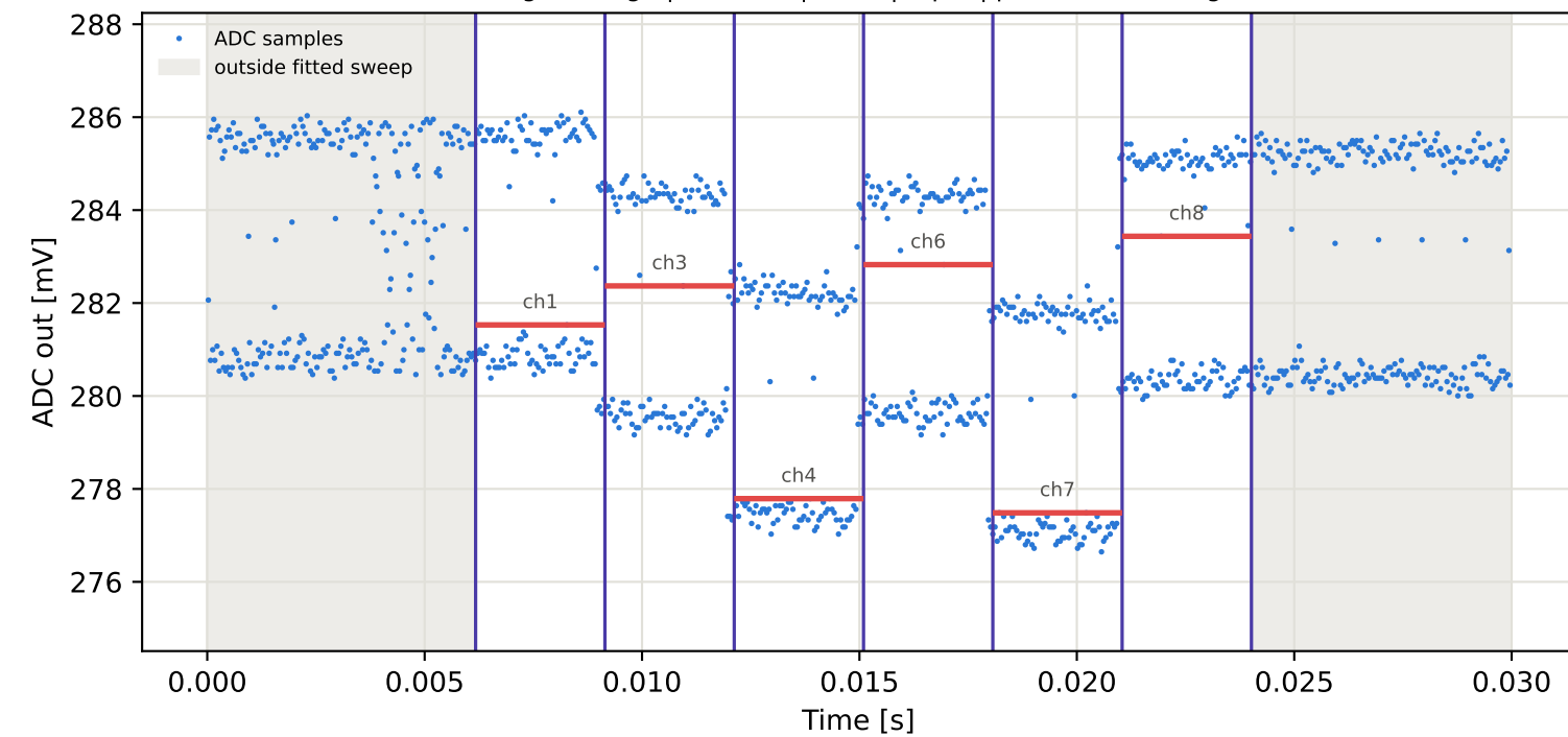
Tag8 &lt;- Tag6 | 795 MHz | run 0 | rep 1 | phase 162.96 deg
