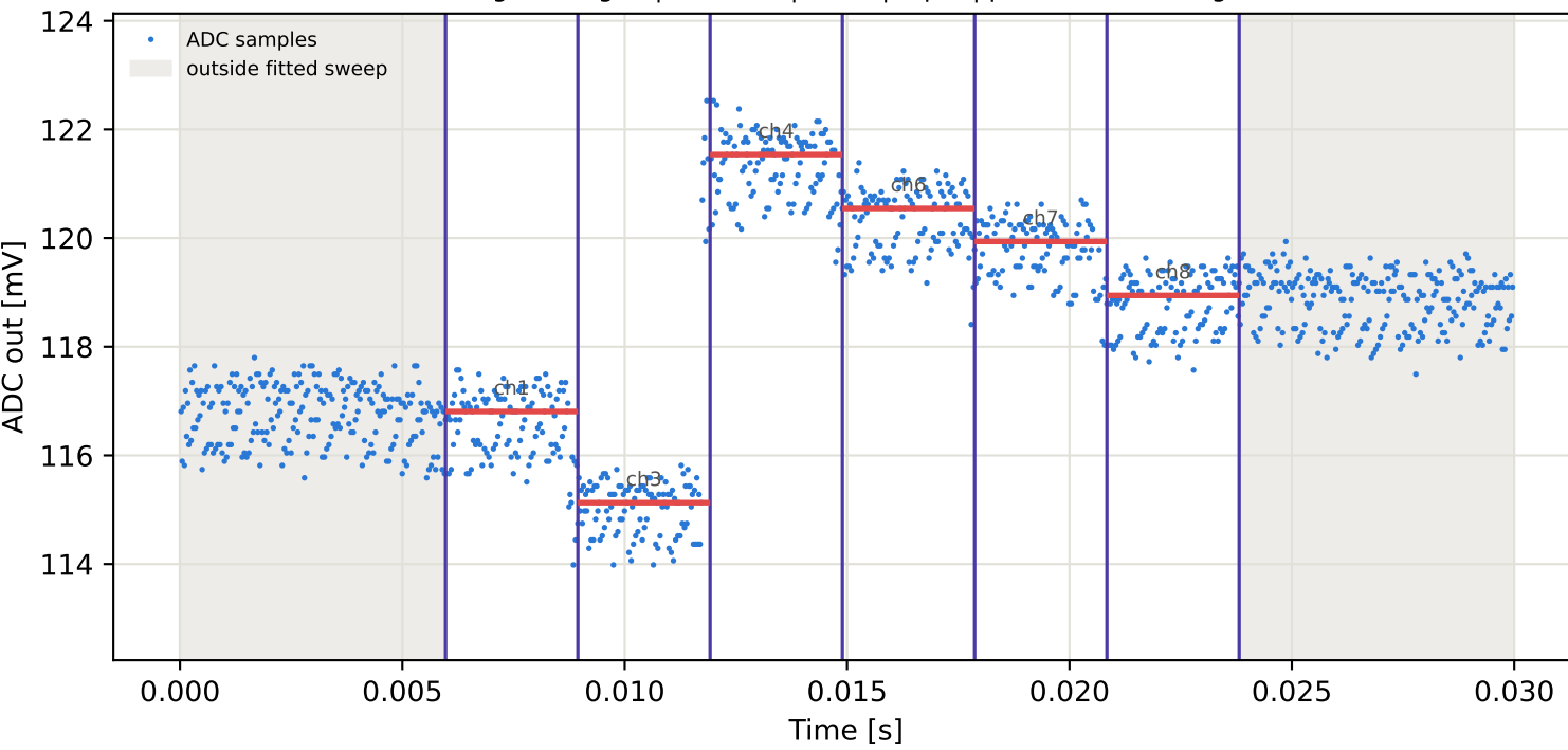
Tag7 &lt;- Tag10 | 795 MHz | run 0 | rep 1 | phase -117.65 deg
