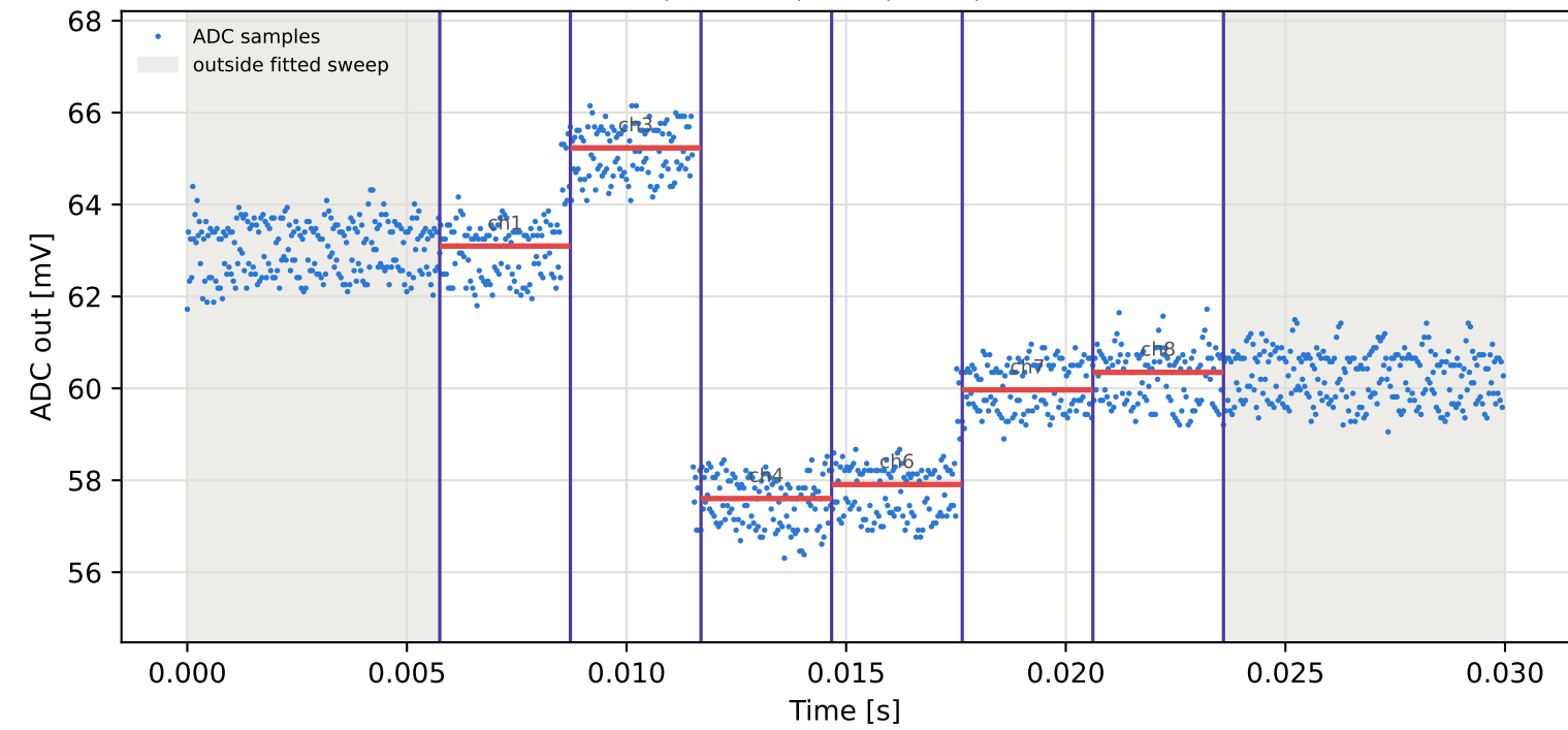
Tag6 &lt;- Tag5 | 785 MHz | run 0 | rep 1 | phase 56.25 deg
