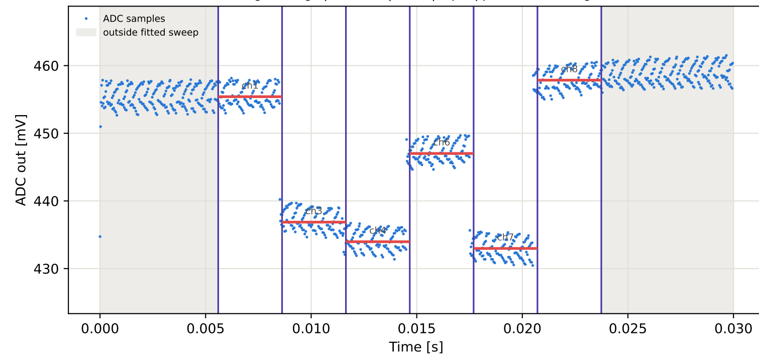
Tag2 &lt;- Tag15 | 865 MHz | run 0 | rep 1 | phase 9.29 deg
