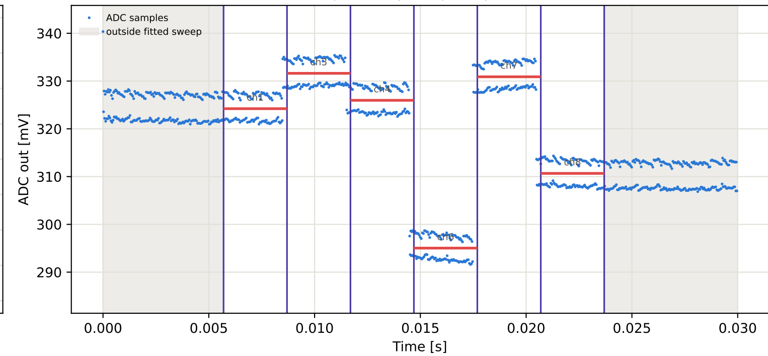
Tag6 &lt;- Tag5 | 965 MHz | run 0 | rep 1 | phase -4.04 deg
