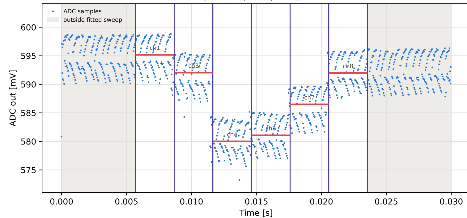
Tag10 &lt;- Tag8 | 945 MHz | run 0 | rep 1 | phase 45.42 deg
