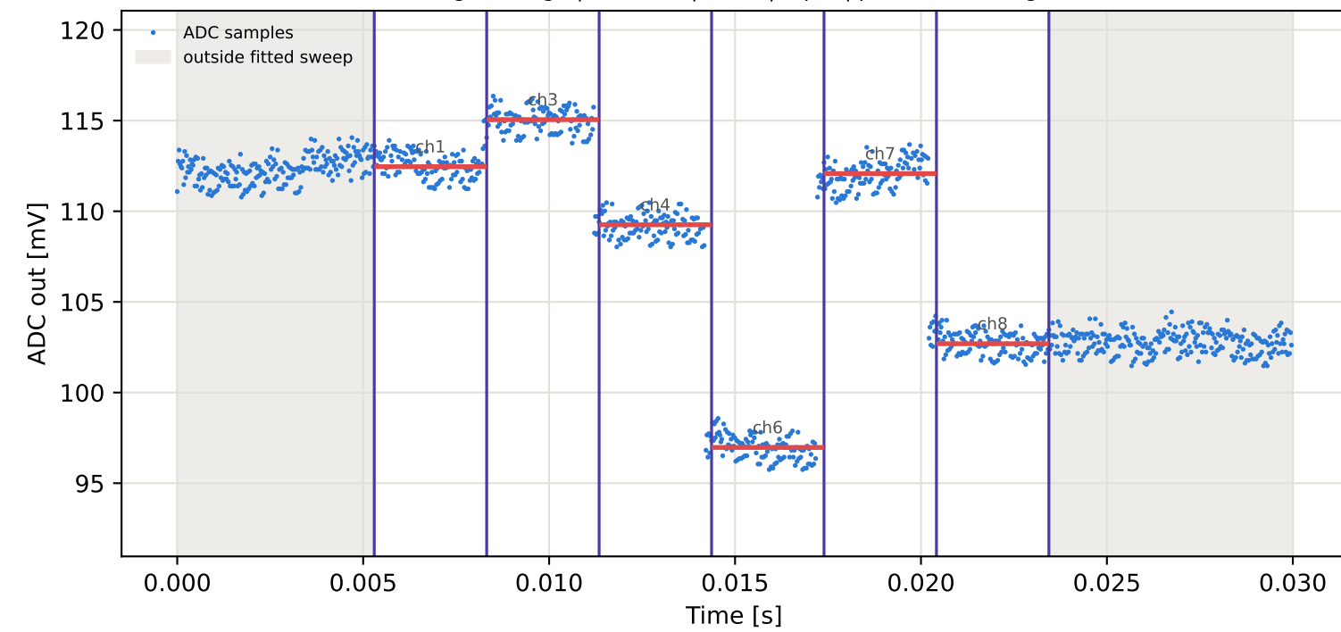
Tag6 &lt;- Tag9 | 915 MHz | run 0 | rep 1 | phase -2.58 deg
