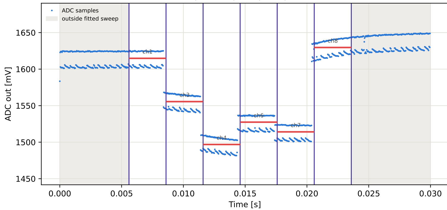
Tag8 &lt;- Tag16 | 905 MHz | run 0 | rep 1 | phase 78.60 deg
