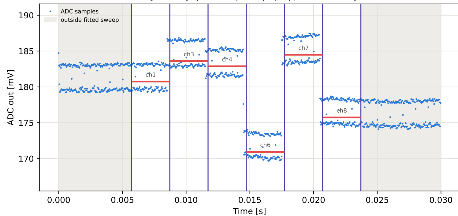
Tag10 &lt;- Tag1 | 995 MHz | run 0 | rep 1 | phase -15.46 deg
