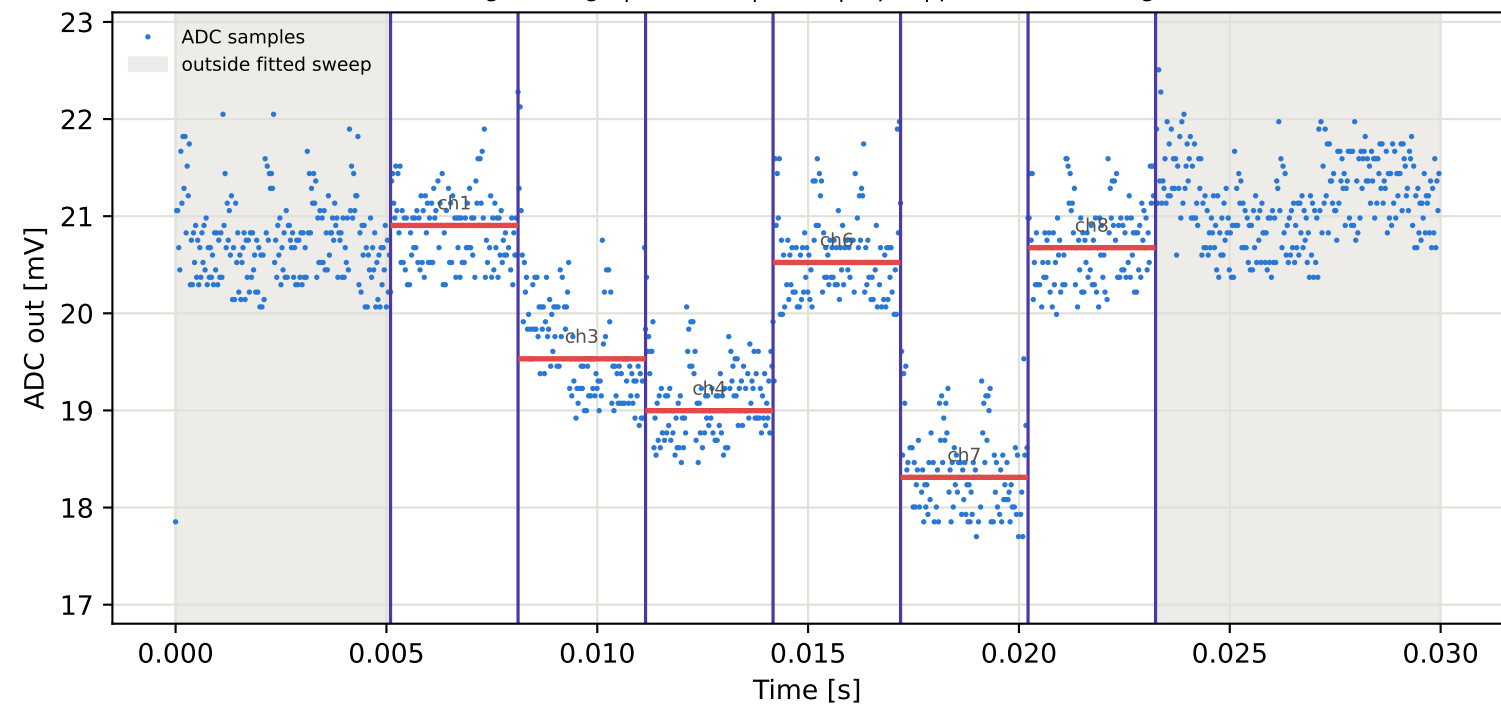
Tag6 &lt;- Tag5 | 795 MHz | run 0 | rep 1 | phase 84.30 deg
