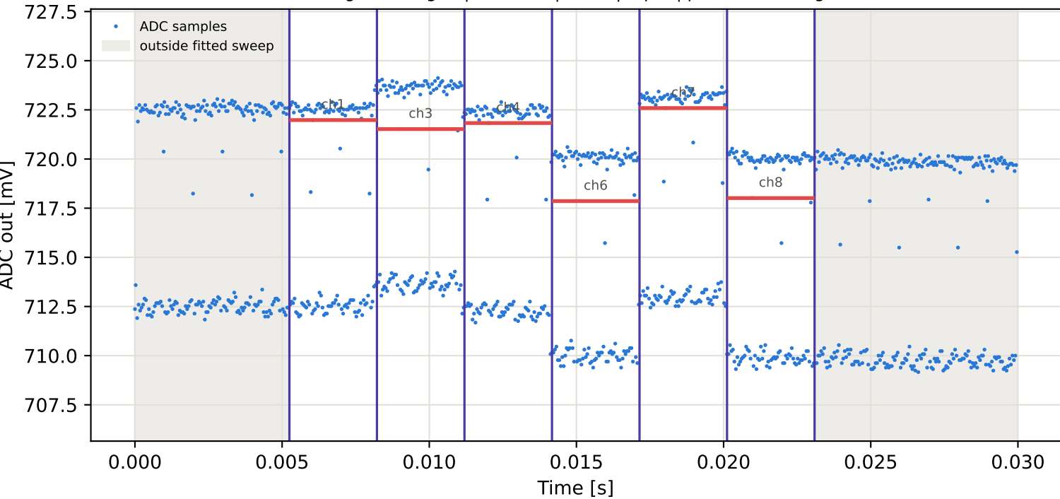
Tag16 &lt;- Tag10 | 865 MHz | run 0 | rep 1 | phase -5.84 deg
