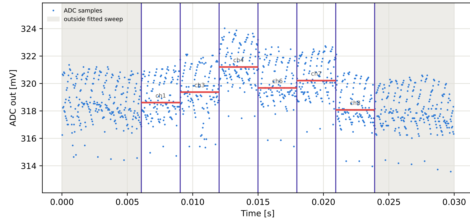
Tag6 &lt;- Tag4 | 975 MHz | run 0 | rep 1 | phase 100.78 deg
