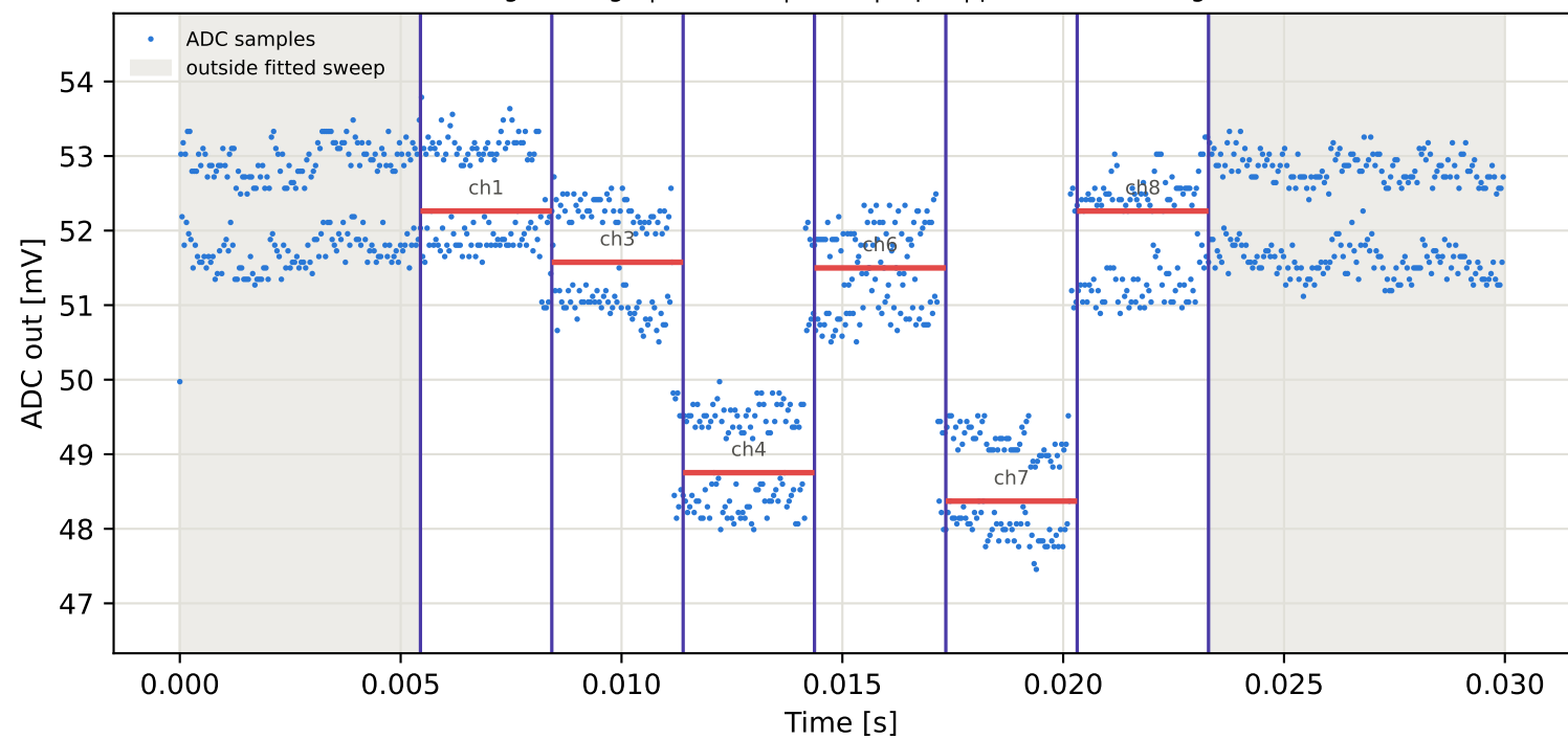
Tag1 &lt;- Tag3 | 775 MHz | run 0 | rep 1 | phase 107.73 deg
