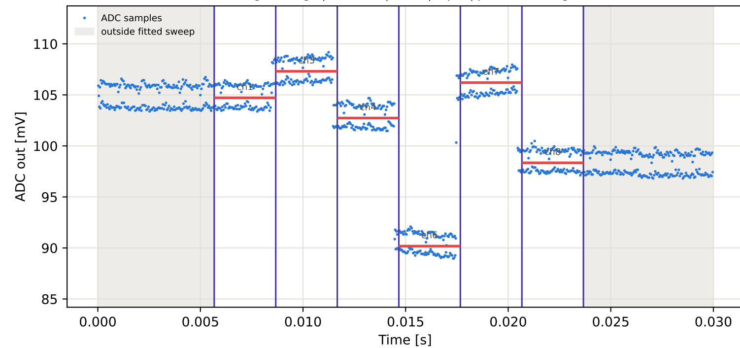
Tag1 &lt;- Tag7 | 965 MHz | run 0 | rep 1 | phase -62.65 deg
