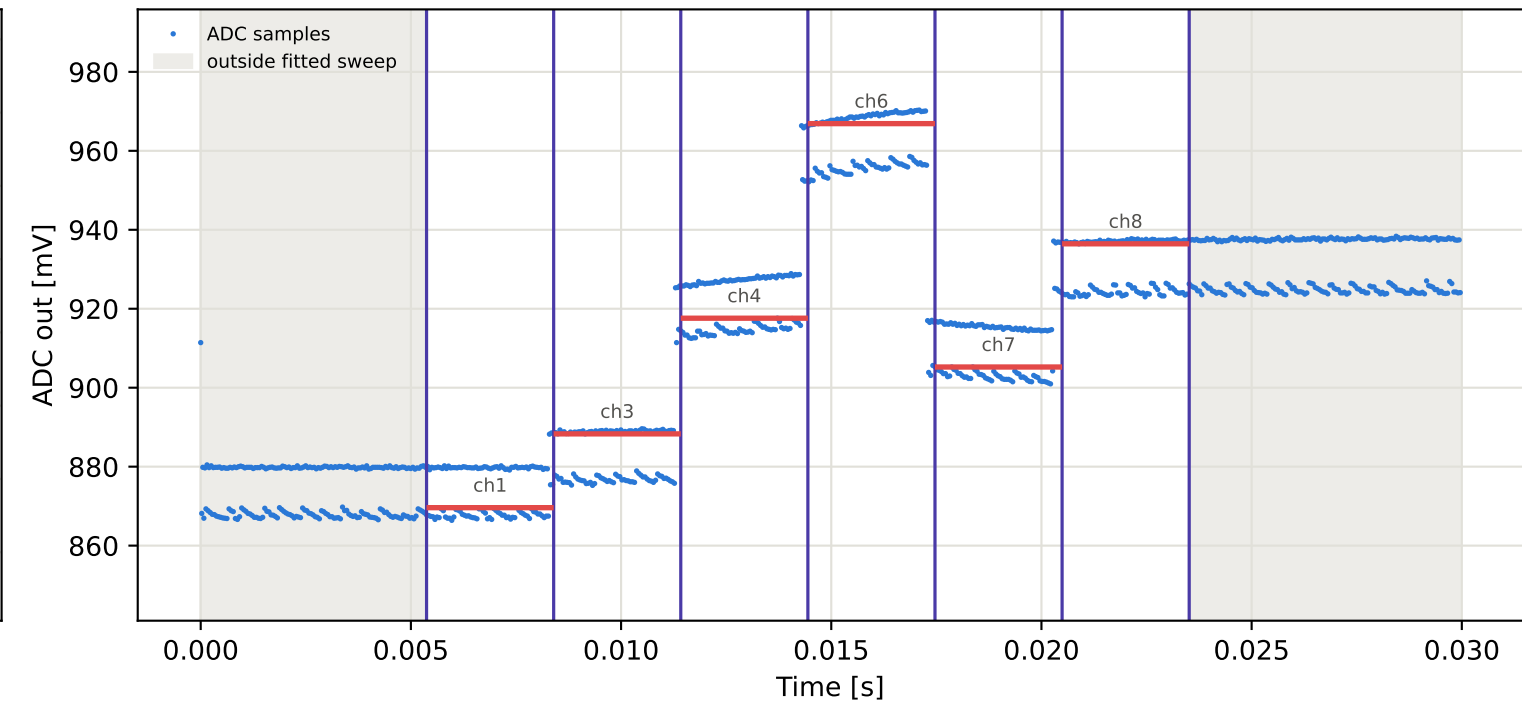
Tag15 &lt;- Tag10 | 895 MHz | run 0 | rep 1 | phase 104.61 deg
