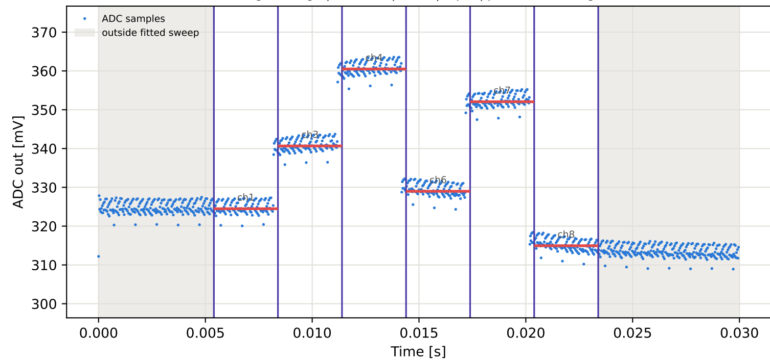
Tag1 &lt;- Tag8 | 925 MHz | run 0 | rep 1 | phase -129.74 deg
