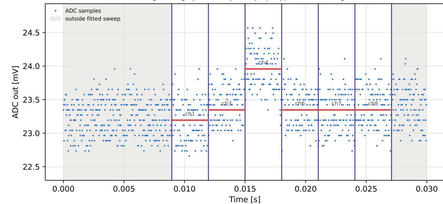
Tag3 &lt;- Tag2 | 785 MHz | run 0 | rep 1 | phase -90.32 deg
