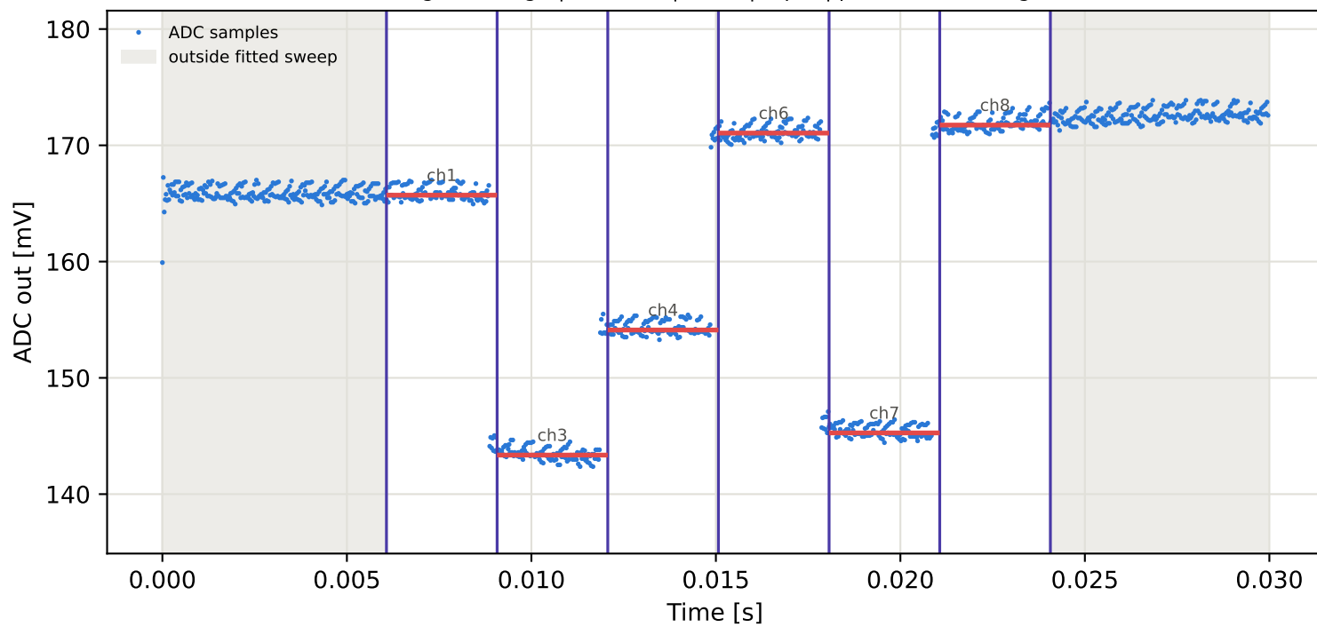
Tag2 &lt;- Tag1 | 805 MHz | run 0 | rep 1 | phase -85.52 deg
