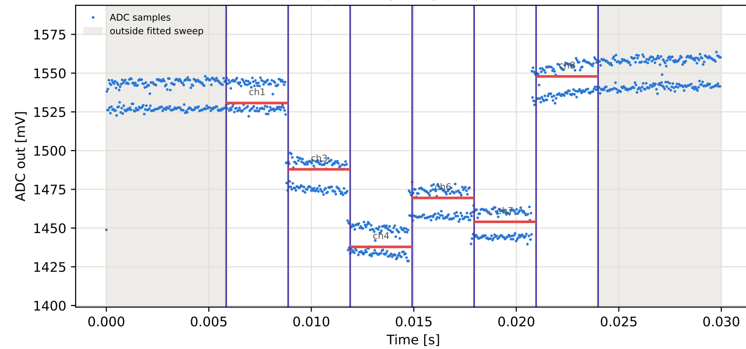
Tag5 &lt;- Tag3 | 885 MHz | run 0 | rep 1 | phase 81.40 deg
