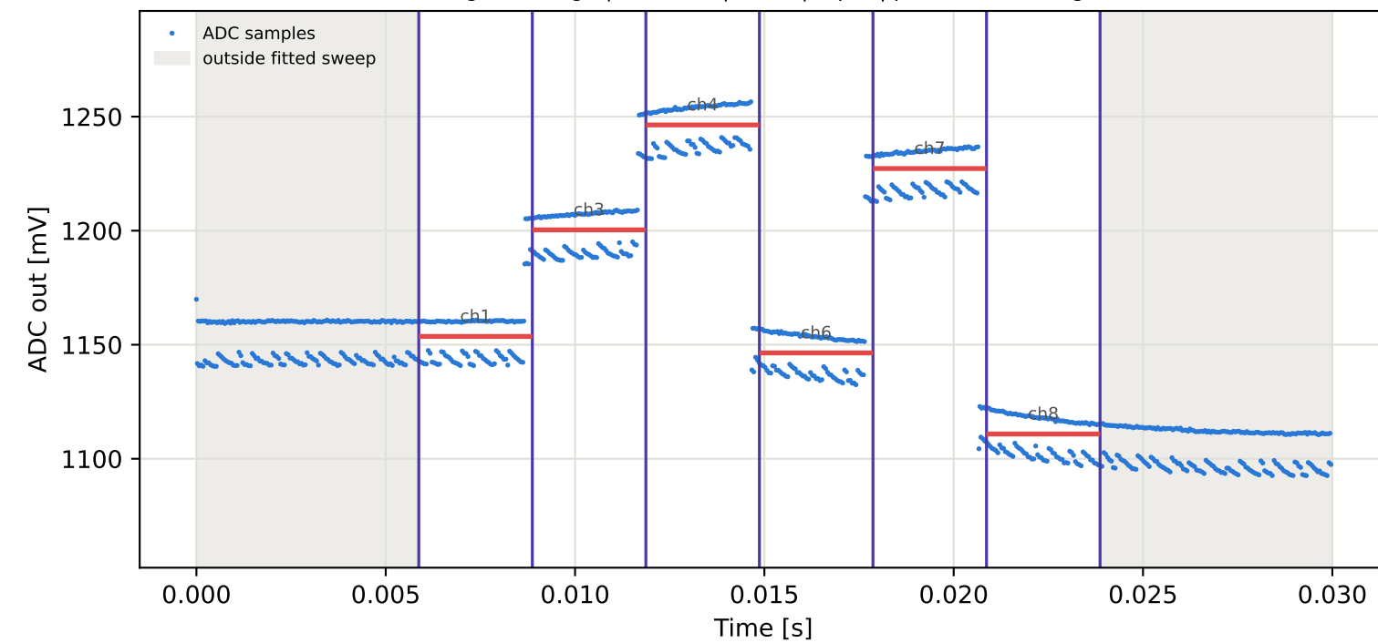
Tag2 &lt;- Tag1 | 925 MHz | run 0 | rep 1 | phase 125.78 deg
