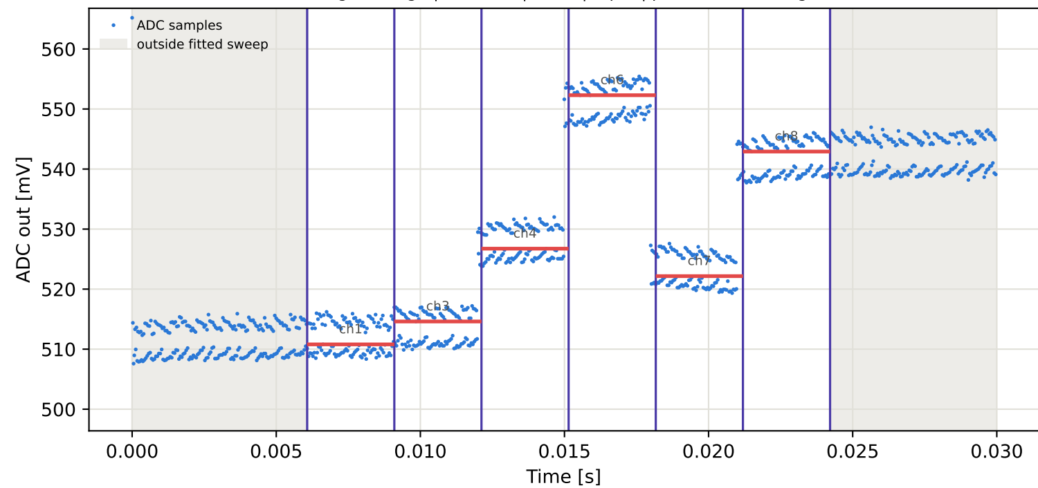
Tag2 &lt;- Tag5 | 875 MHz | run 0 | rep 1 | phase -143.01 deg
