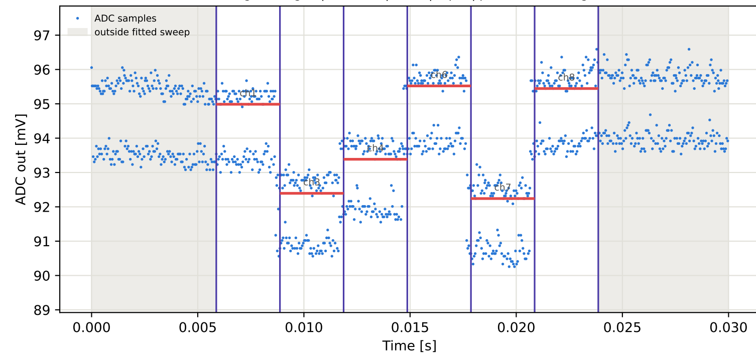
Tag5 &lt;- Tag16 | 795 MHz | run 0 | rep 1 | phase -73.29 deg
