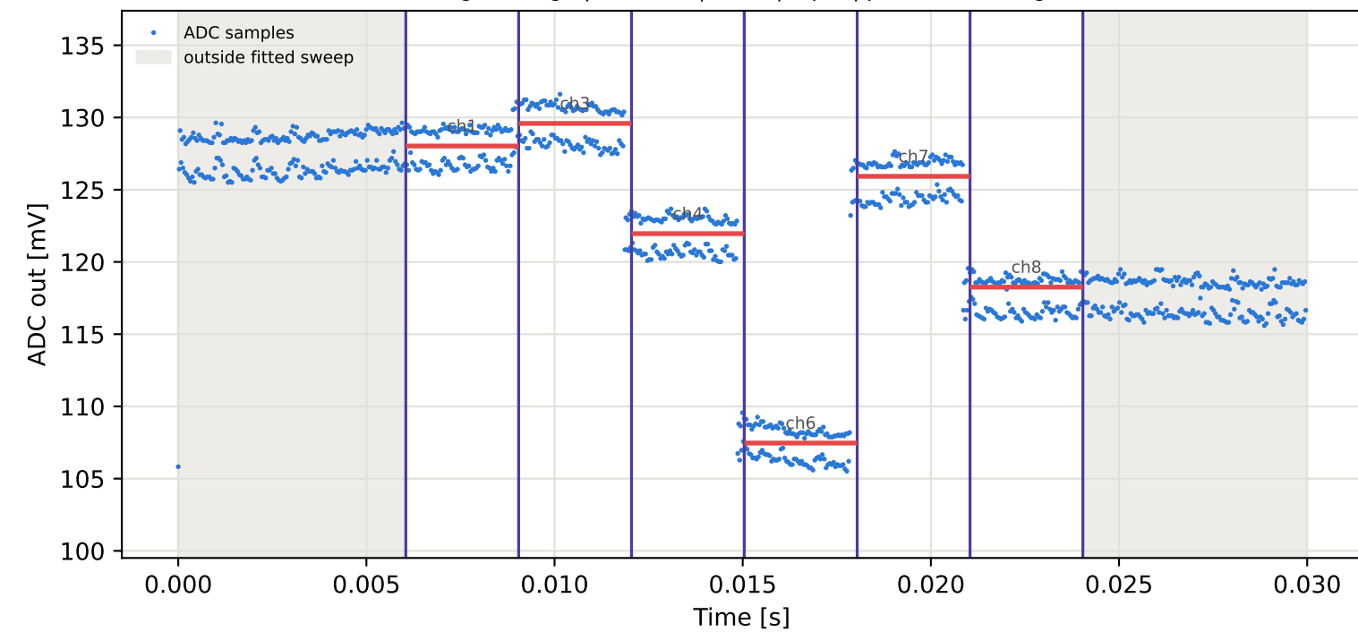
Tag6 &lt;- Tag9 | 935 MHz | run 0 | rep 1 | phase -12.12 deg
