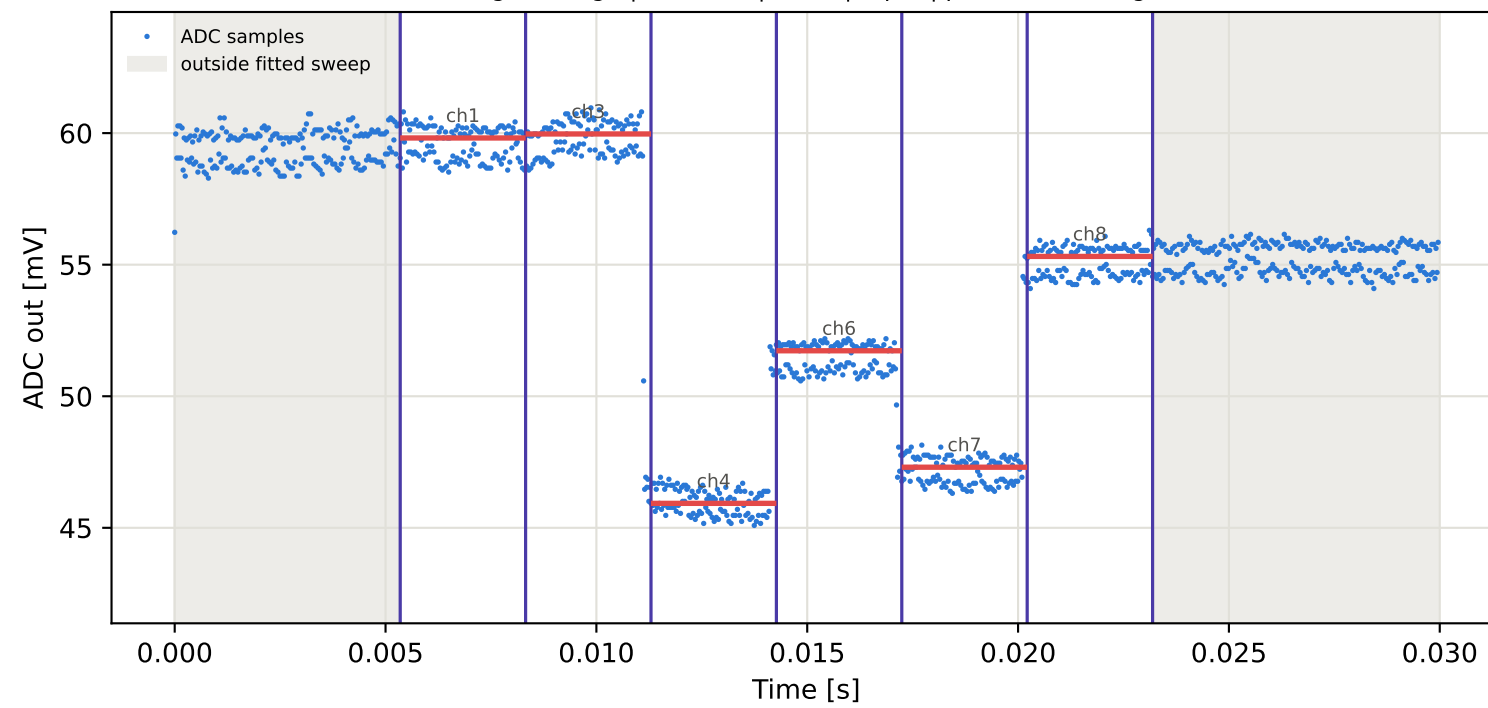
Tag9 &lt;- Tag5 | 805 MHz | run 0 | rep 1 | phase 87.94 deg
