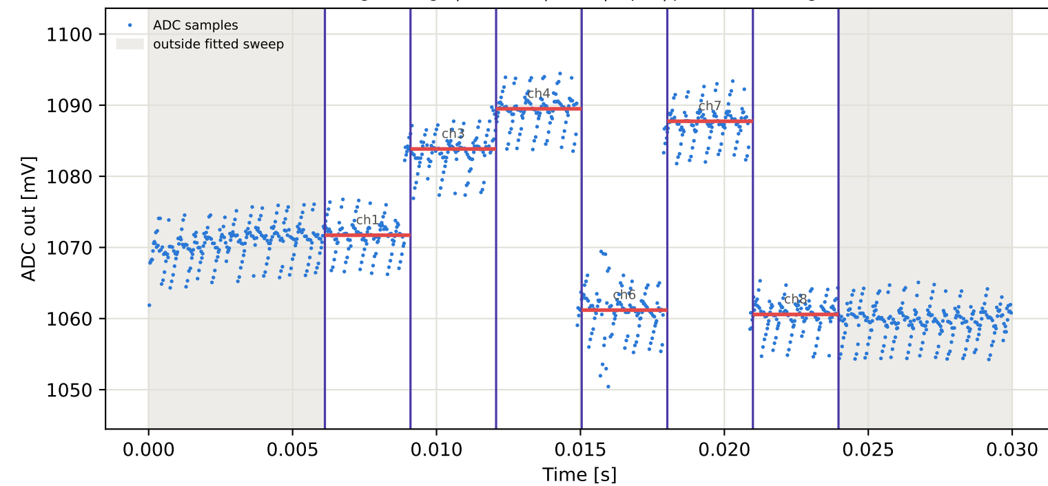
Tag9 &lt;- Tag10 | 935 MHz | run 0 | rep 1 | phase -90.97 deg
