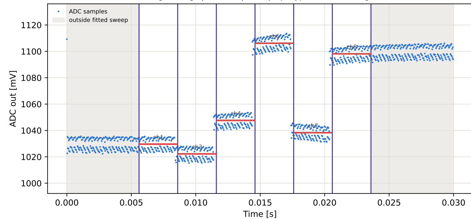
Tag3 &lt;- Tag8 | 875 MHz | run 0 | rep 1 | phase -128.83 deg
