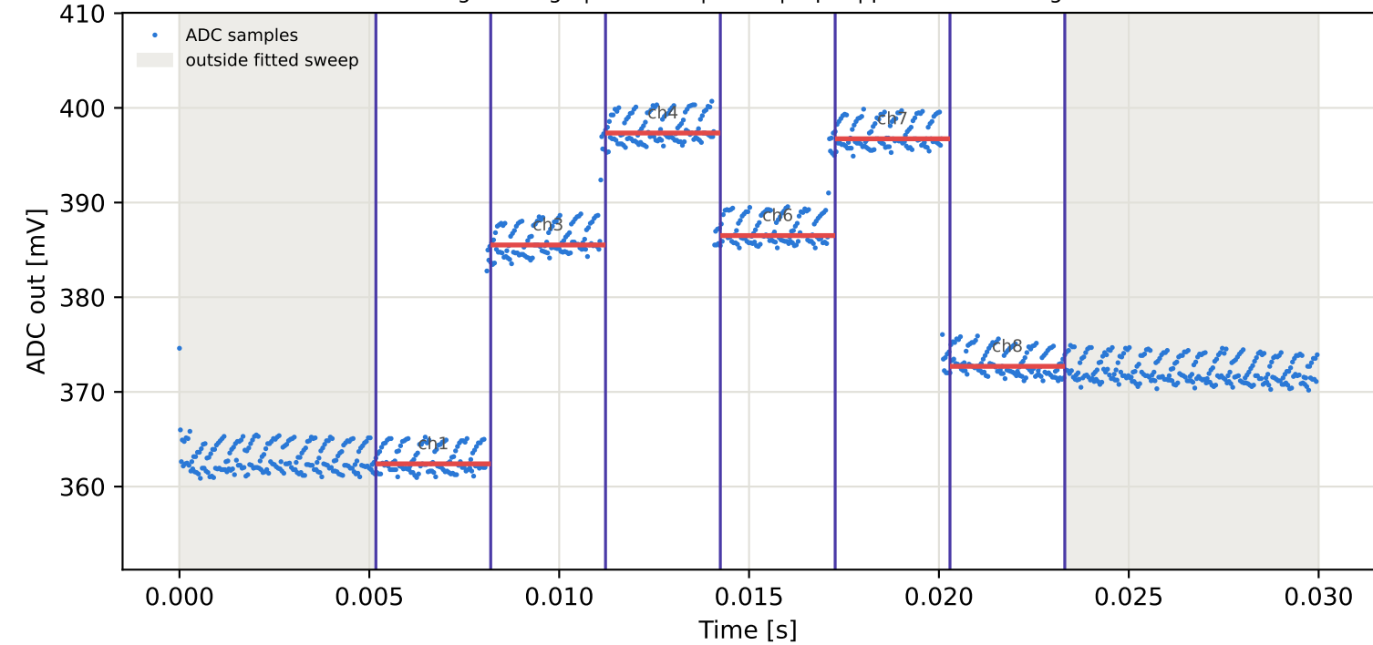
Tag7 &lt;- Tag1 | 845 MHz | run 0 | rep 1 | phase -37.32 deg
