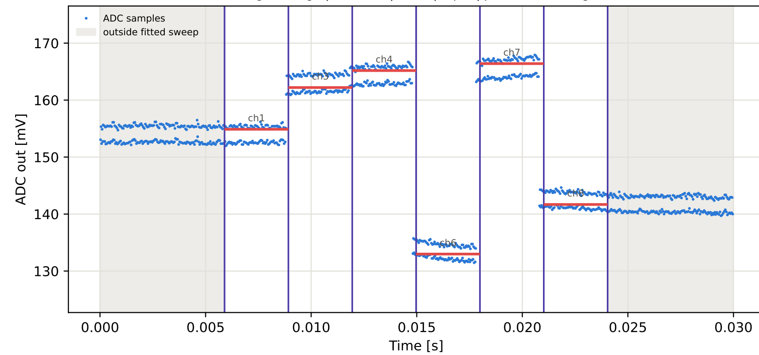
Tag1 &lt;- Tag7 | 975 MHz | run 0 | rep 1 | phase -52.20 deg
