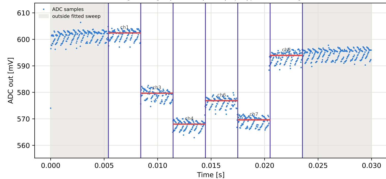
Tag10 &lt;- Tag2 | 875 MHz | run 0 | rep 1 | phase -81.55 deg
