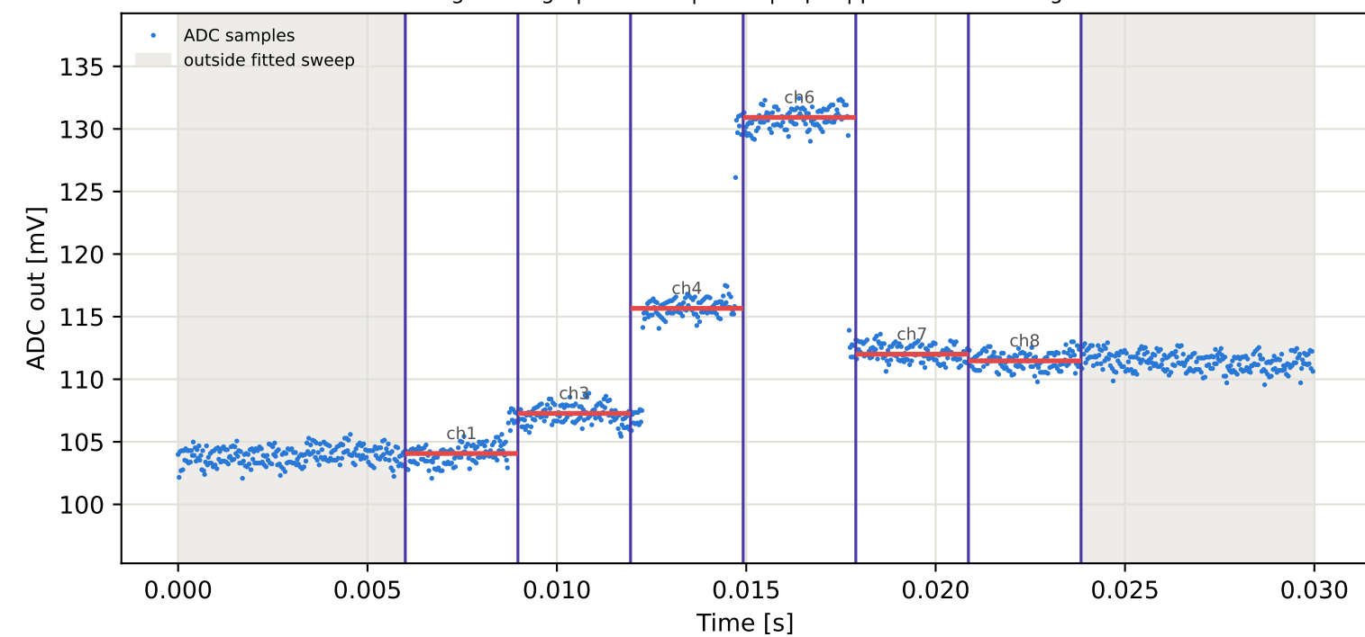
Tag6 &lt;- Tag5 | 915 MHz | run 0 | rep 1 | phase -149.03 deg
