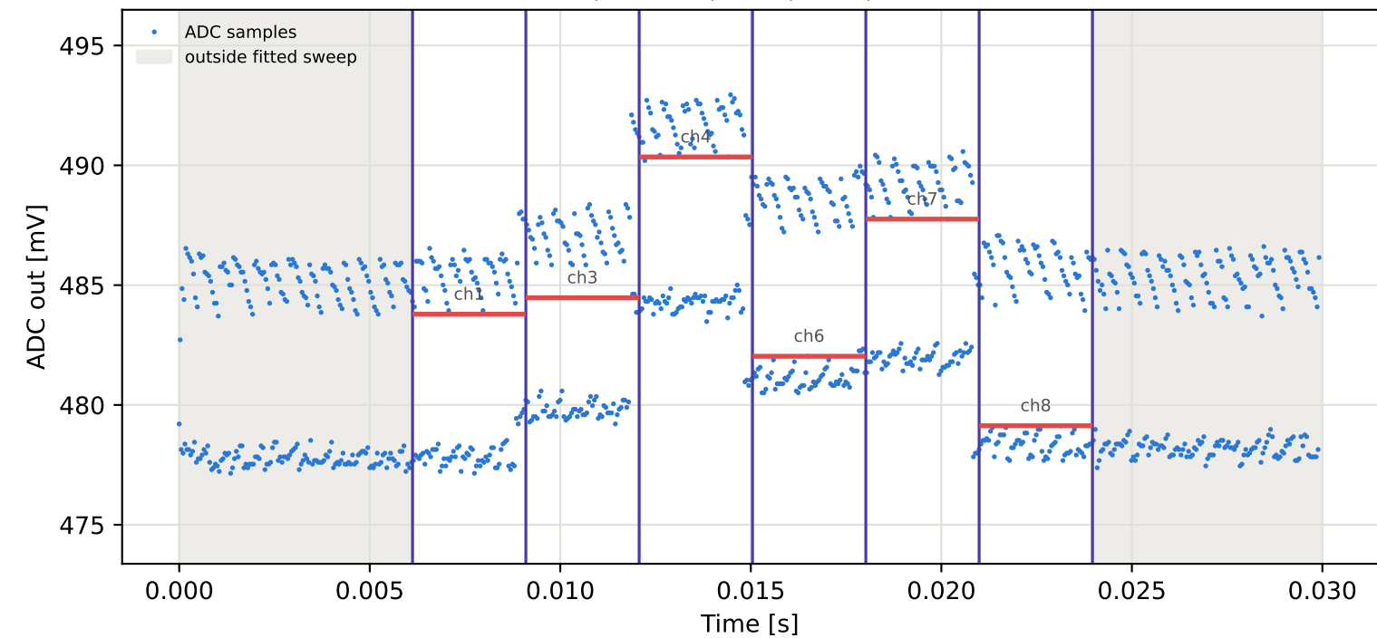
Tag7 &lt;- Tag15 | 975 MHz | run 0 | rep 1 | phase -75.86 deg
