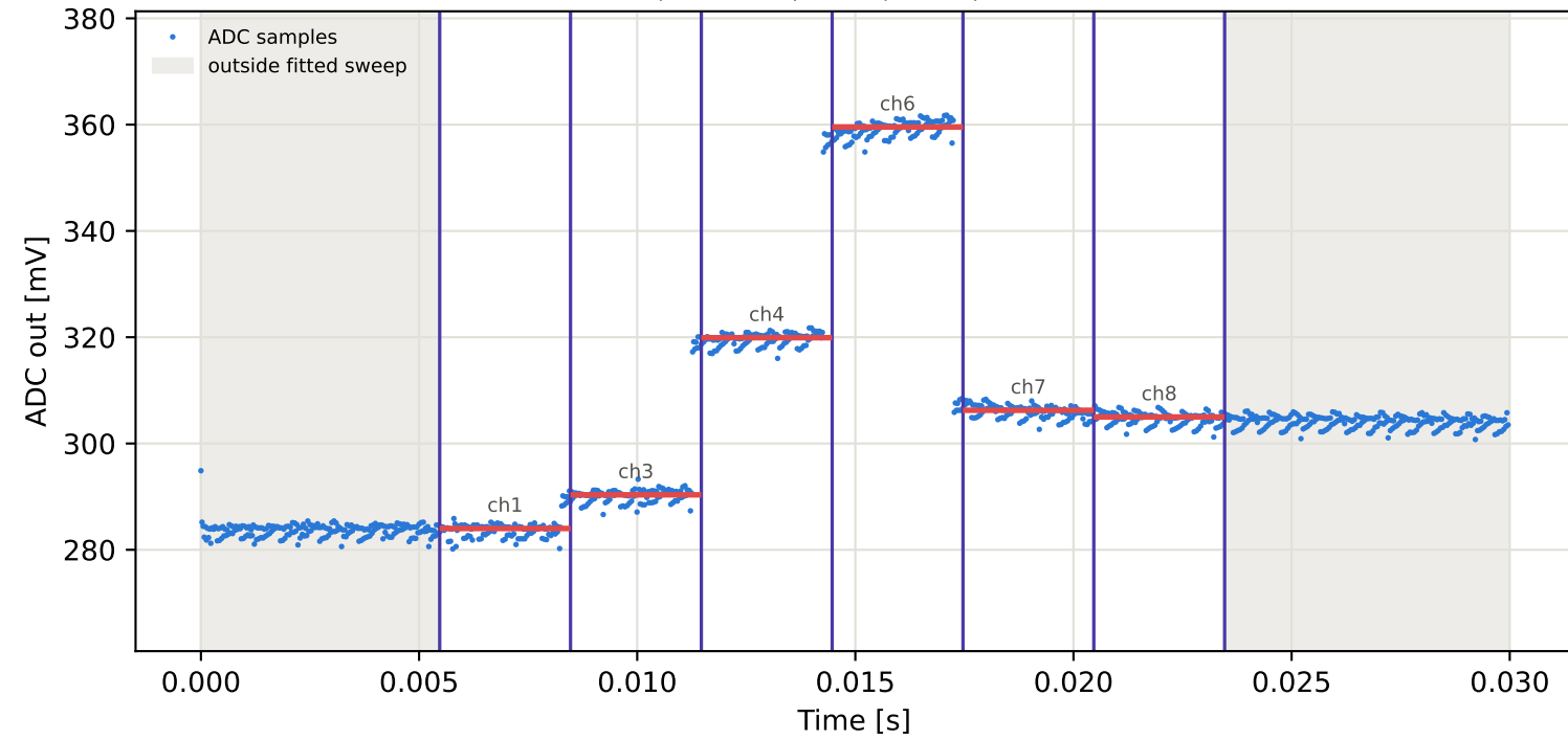
Tag6 &lt;- Tag5 | 925 MHz | run 0 | rep 1 | phase -148.58 deg
