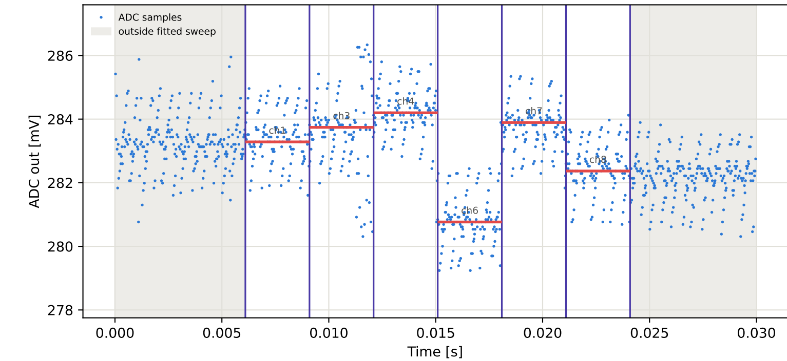
Tag10 &lt;- Tag4 | 975 MHz | run 0 | rep 1 | phase 122.05 deg
