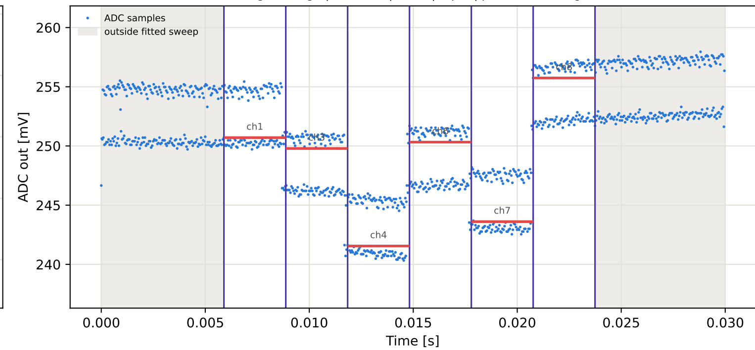
Tag3 &lt;- Tag15 | 925 MHz | run 0 | rep 1 | phase -41.95 deg
