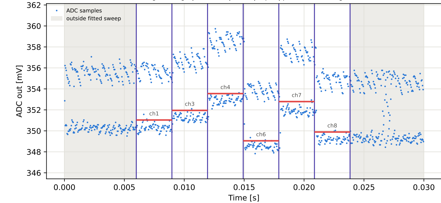
Tag6 &lt;- Tag4 | 985 MHz | run 0 | rep 1 | phase 126.22 deg
