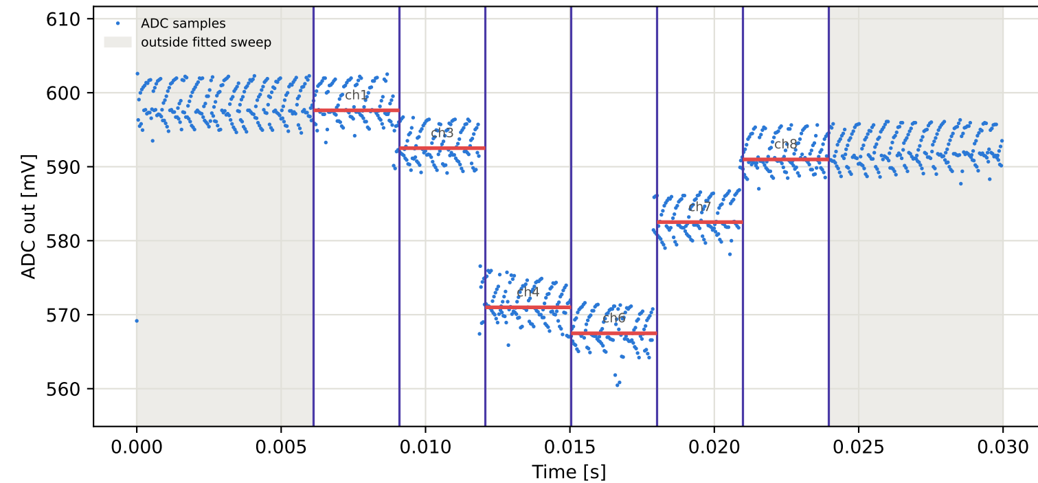
Tag15 &lt;- Tag1 | 945 MHz | run 0 | rep 1 | phase -77.07 deg
