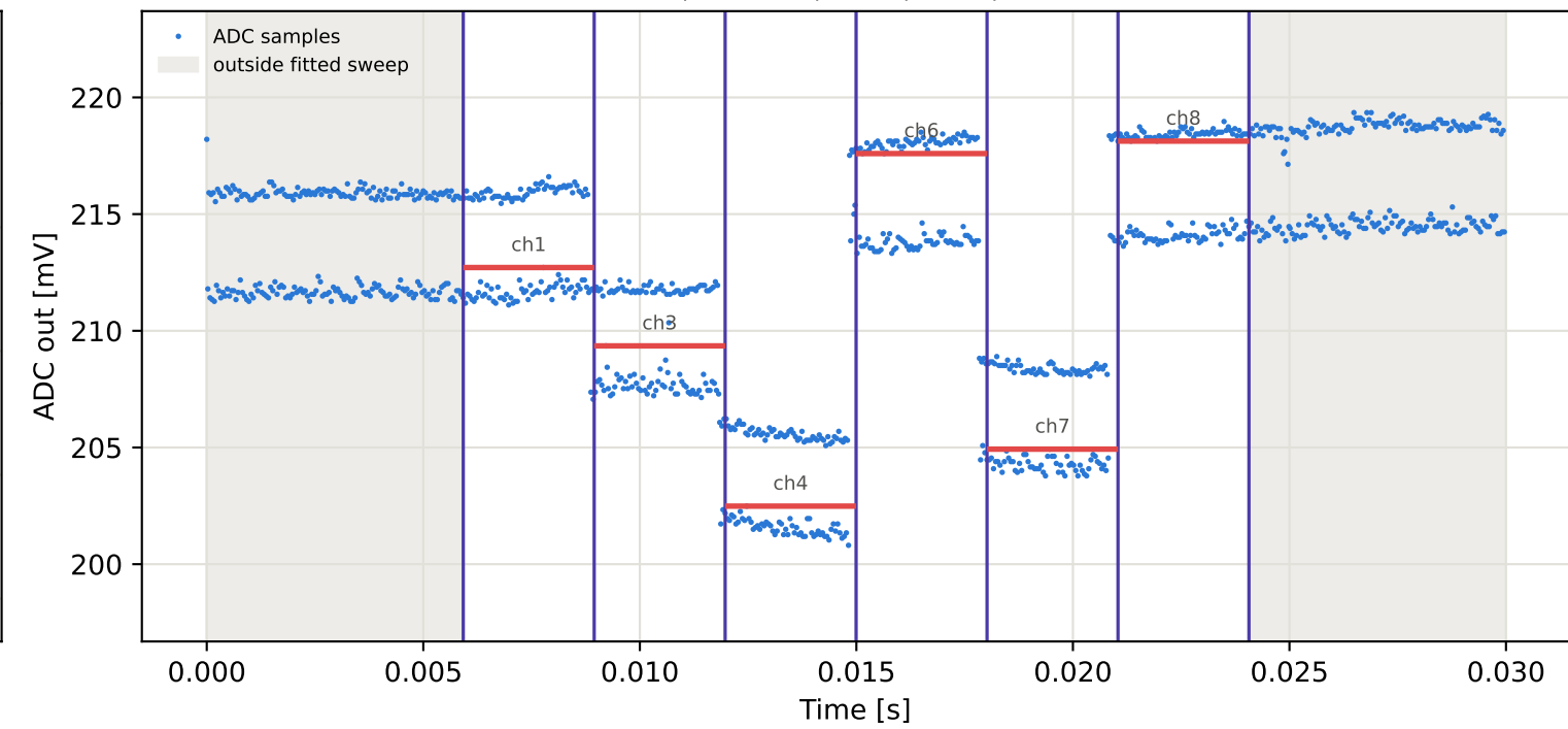
Tag15 &lt;- Tag10 | 975 MHz | run 0 | rep 1 | phase 120.34 deg
