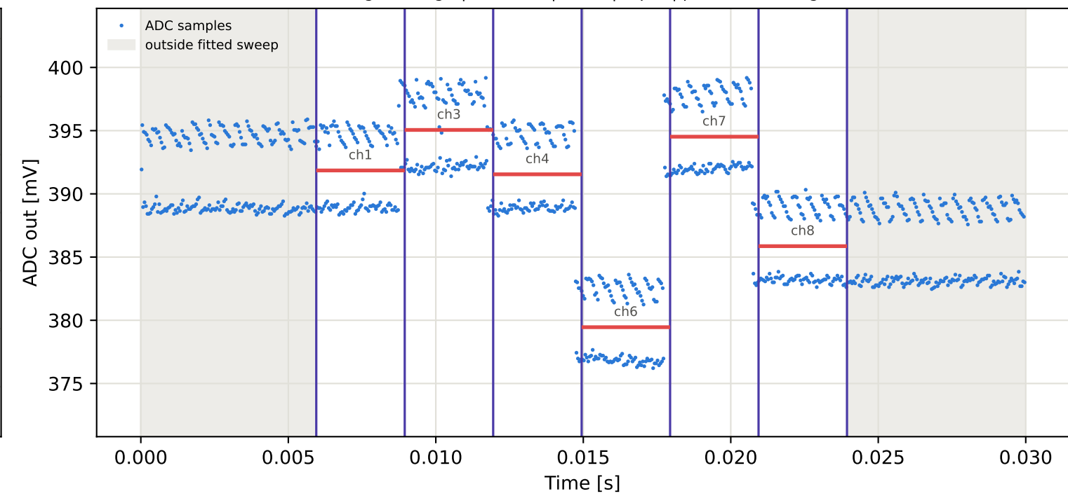
Tag4 &lt;- Tag8 | 975 MHz | run 0 | rep 1 | phase -65.75 deg
