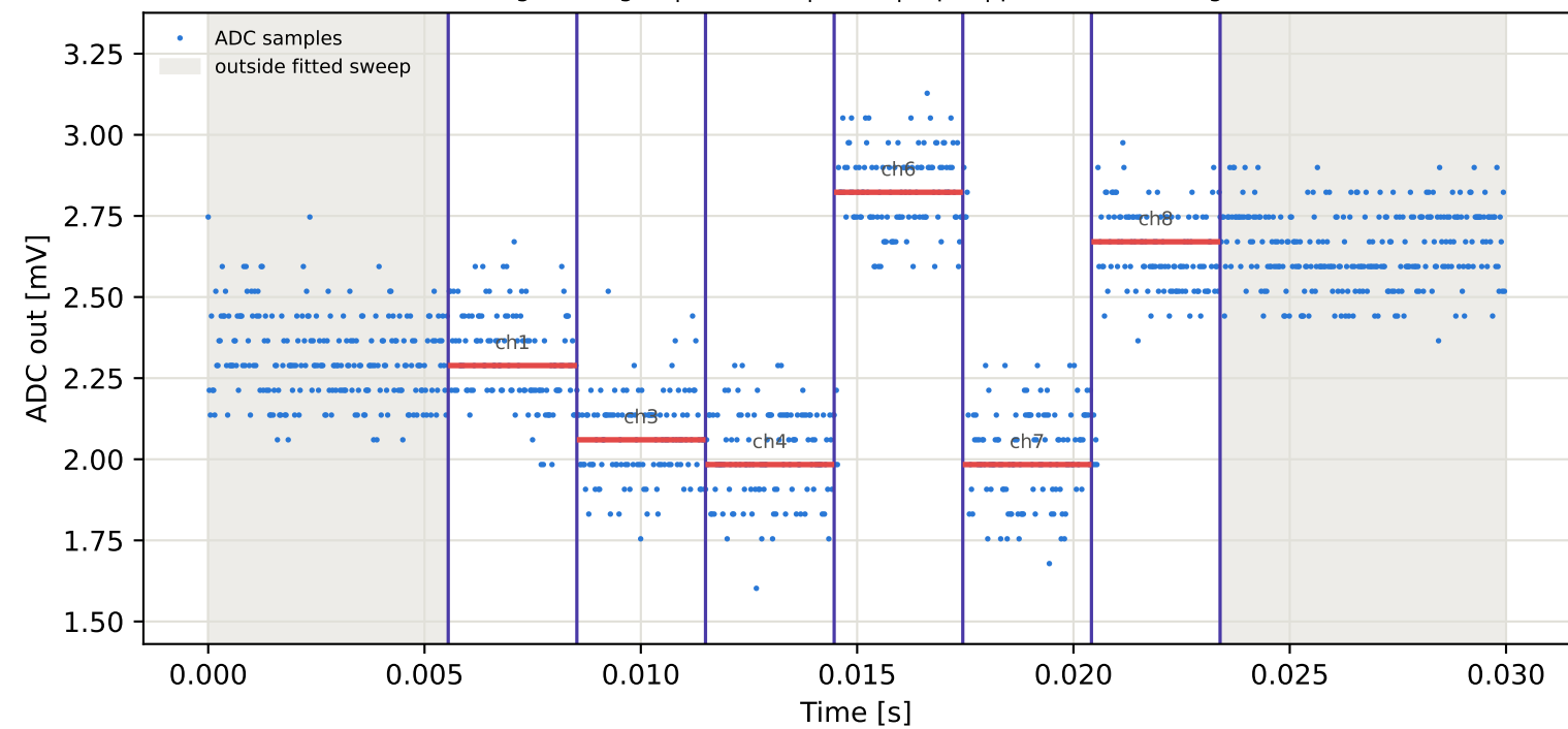
Tag2 &lt;- Tag16 | 965 MHz | run 0 | rep 1 | phase 7.68 deg
