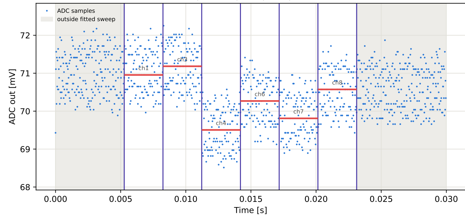
Tag4 &lt;- Tag3 | 785 MHz | run 0 | rep 1 | phase 78.46 deg
