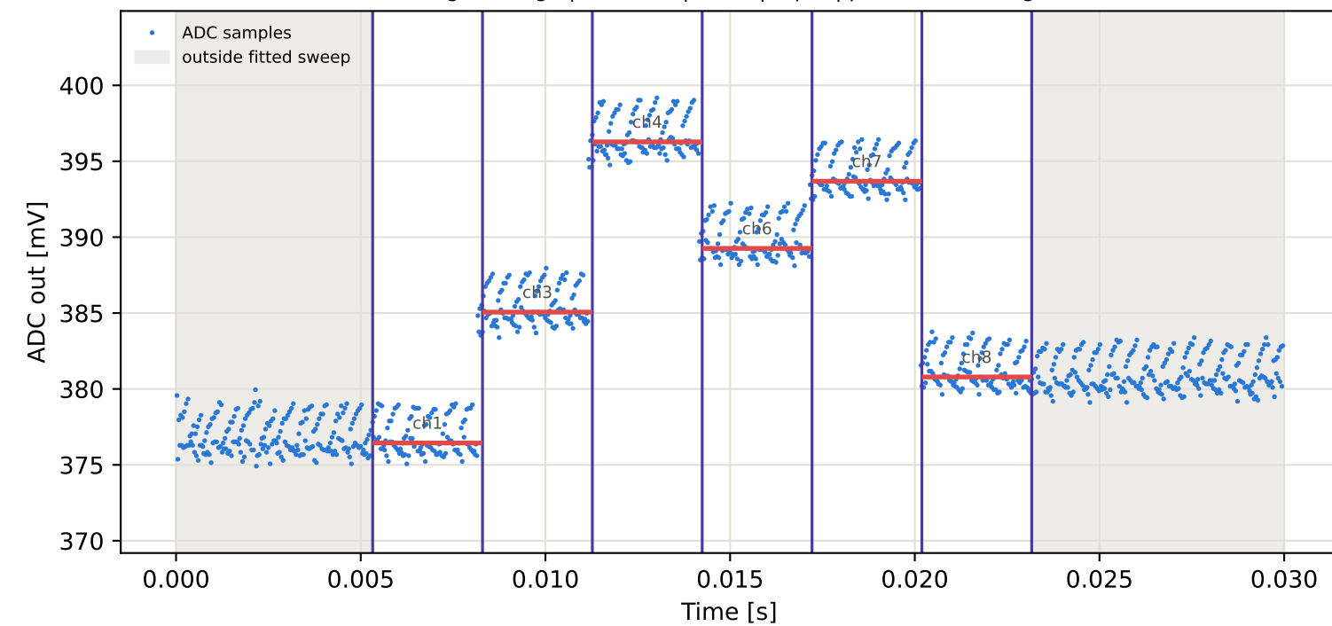
Tag7 &lt;- Tag10 | 845 MHz | run 0 | rep 1 | phase 36.41 deg
