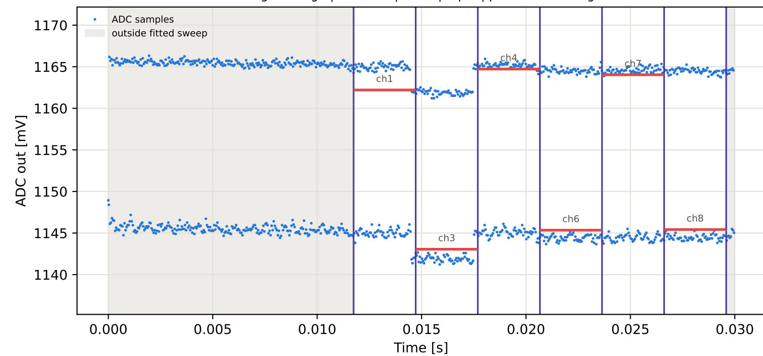
Tag8 &lt;- Tag4 | 925 MHz | run 0 | rep 1 | phase 4.06 deg
