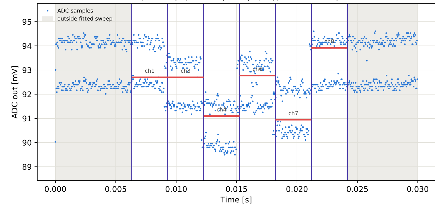
Tag10 &lt;- Tag4 | 825 MHz | run 0 | rep 1 | phase 114.05 deg
