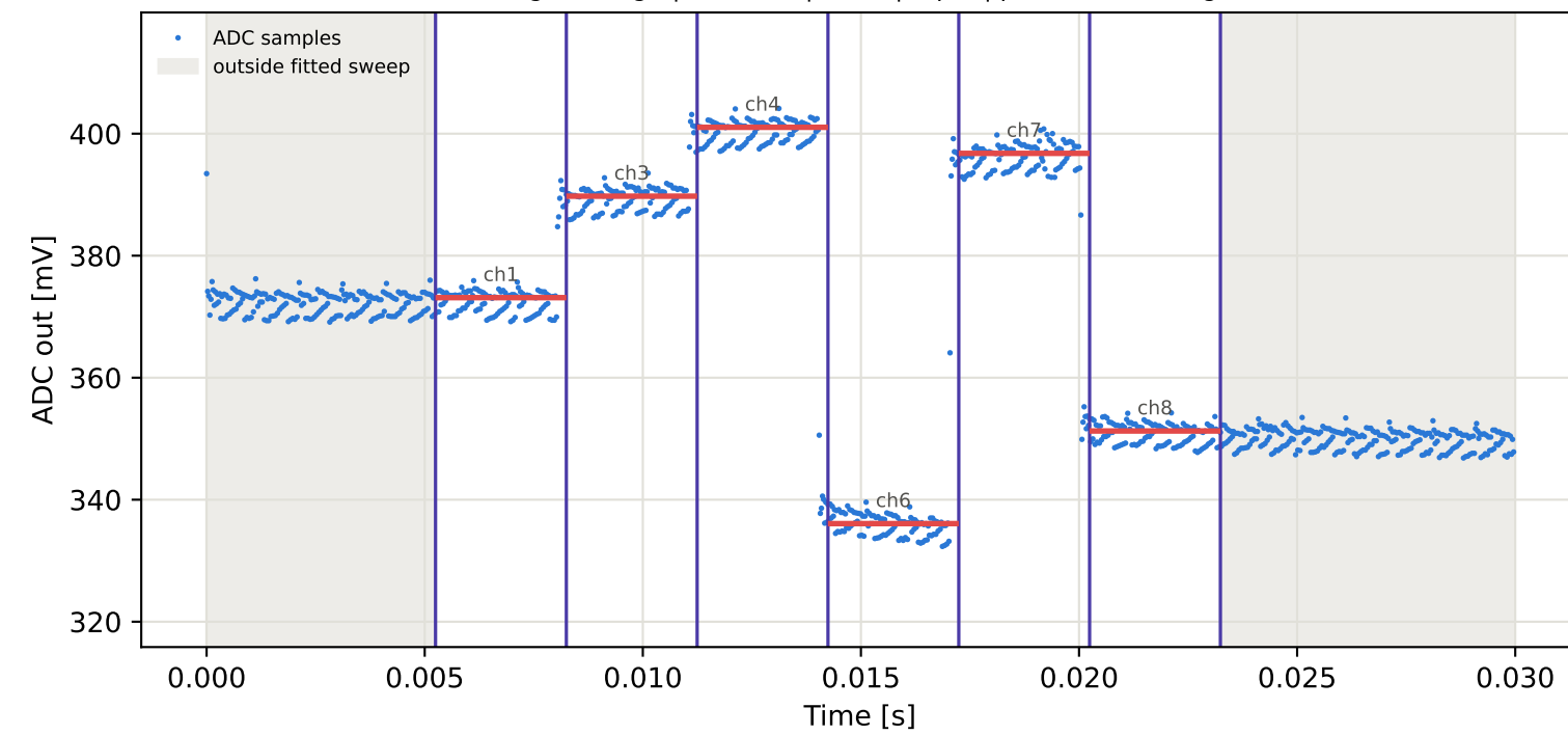
Tag9 &lt;- Tag5 | 965 MHz | run 0 | rep 1 | phase 26.42 deg
