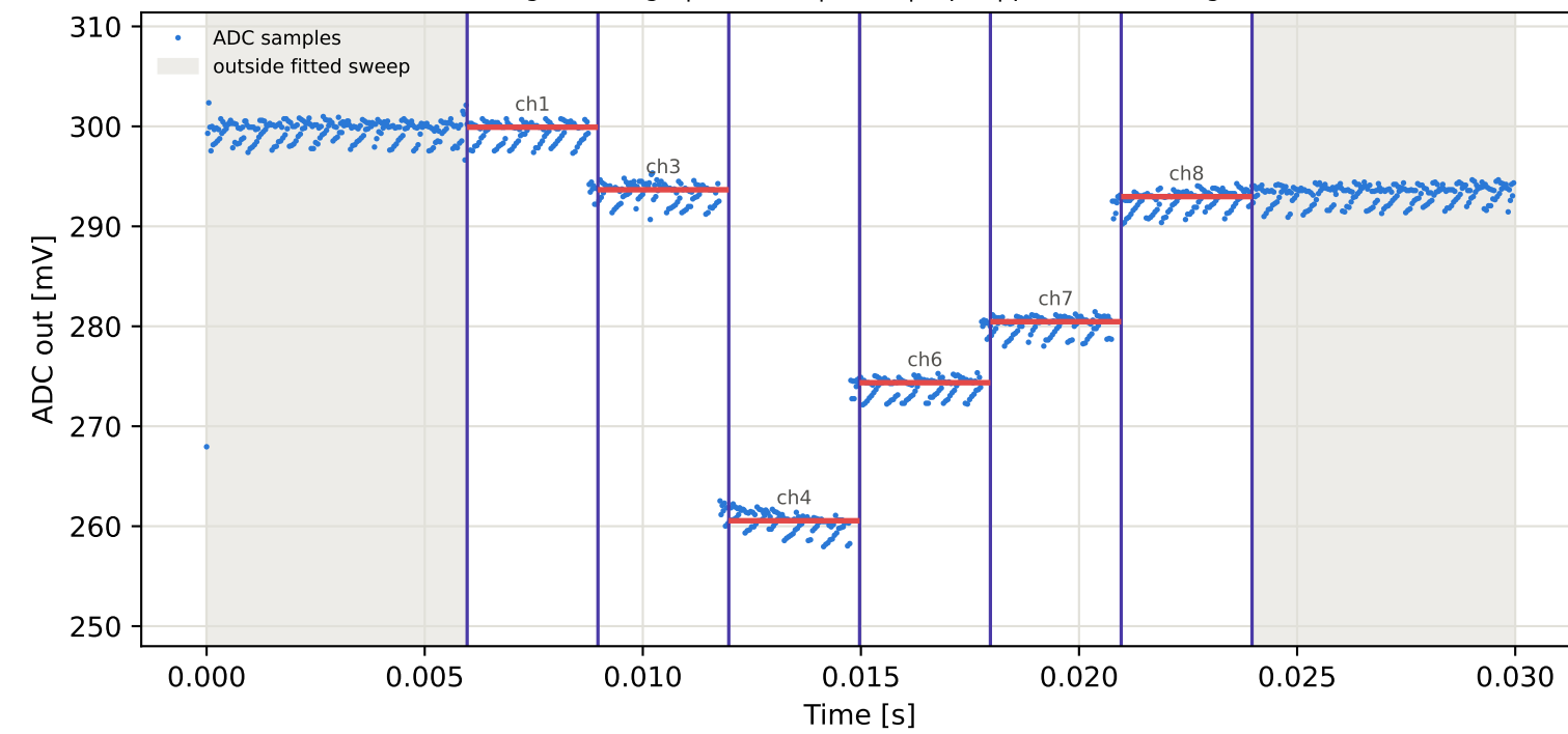
Tag10 &lt;- Tag8 | 975 MHz | run 0 | rep 1 | phase 80.72 deg
