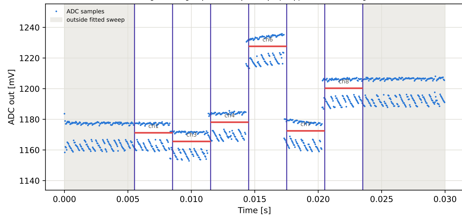
Tag16 &lt;- Tag15 | 925 MHz | run 0 | rep 1 | phase -170.05 deg
