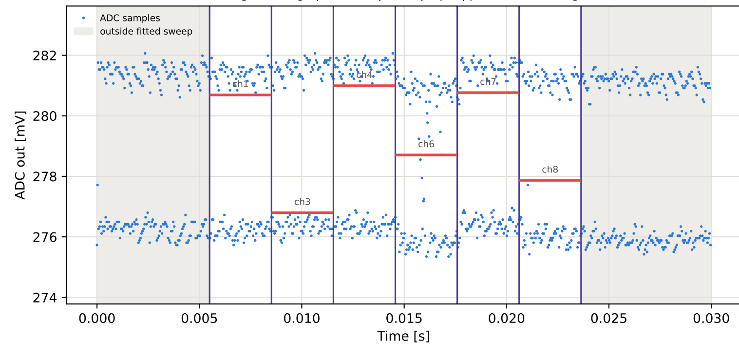
Tag10 &lt;- Tag4 | 965 MHz | run 0 | rep 1 | phase 96.75 deg
