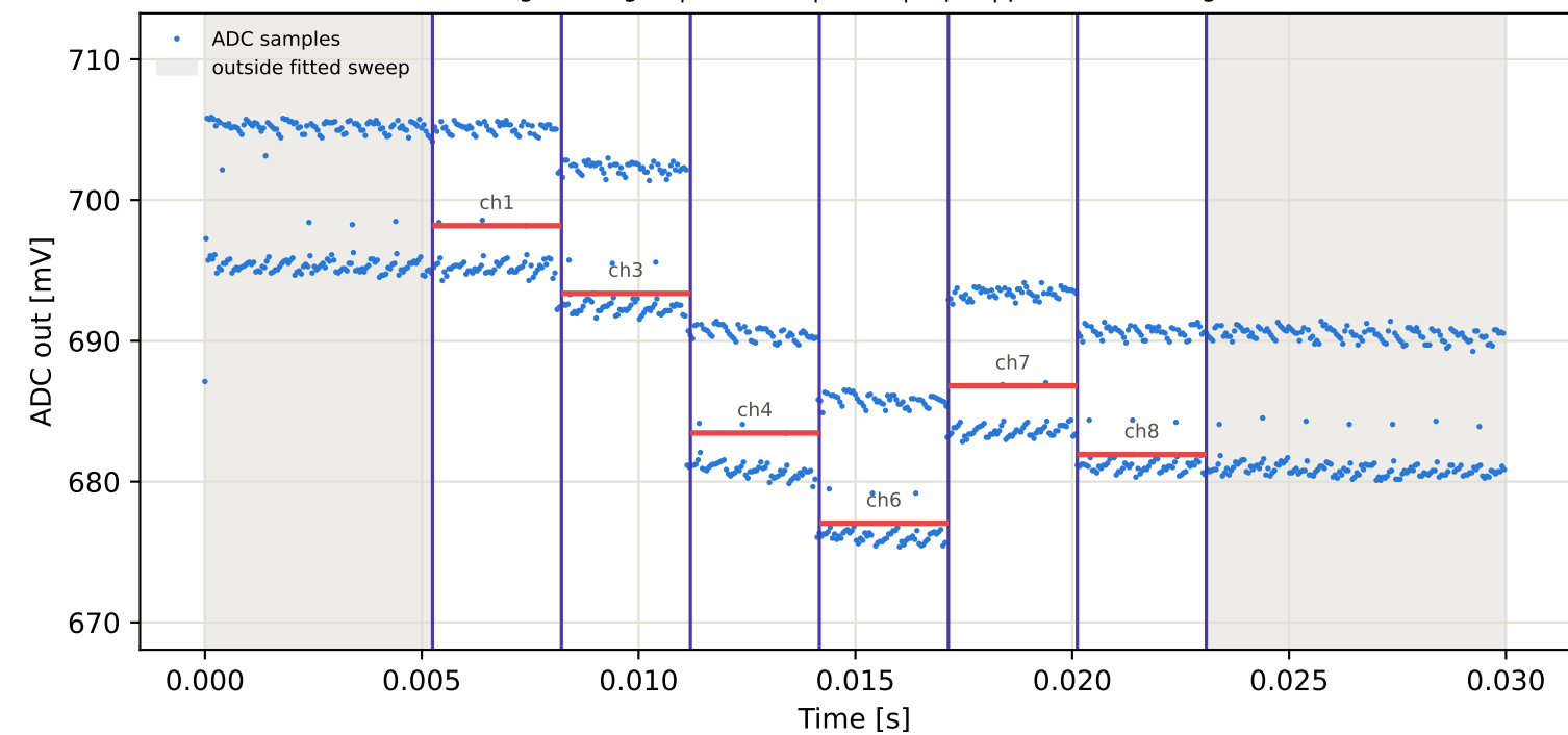
Tag7 &lt;- Tag15 | 865 MHz | run 0 | rep 1 | phase 41.35 deg
