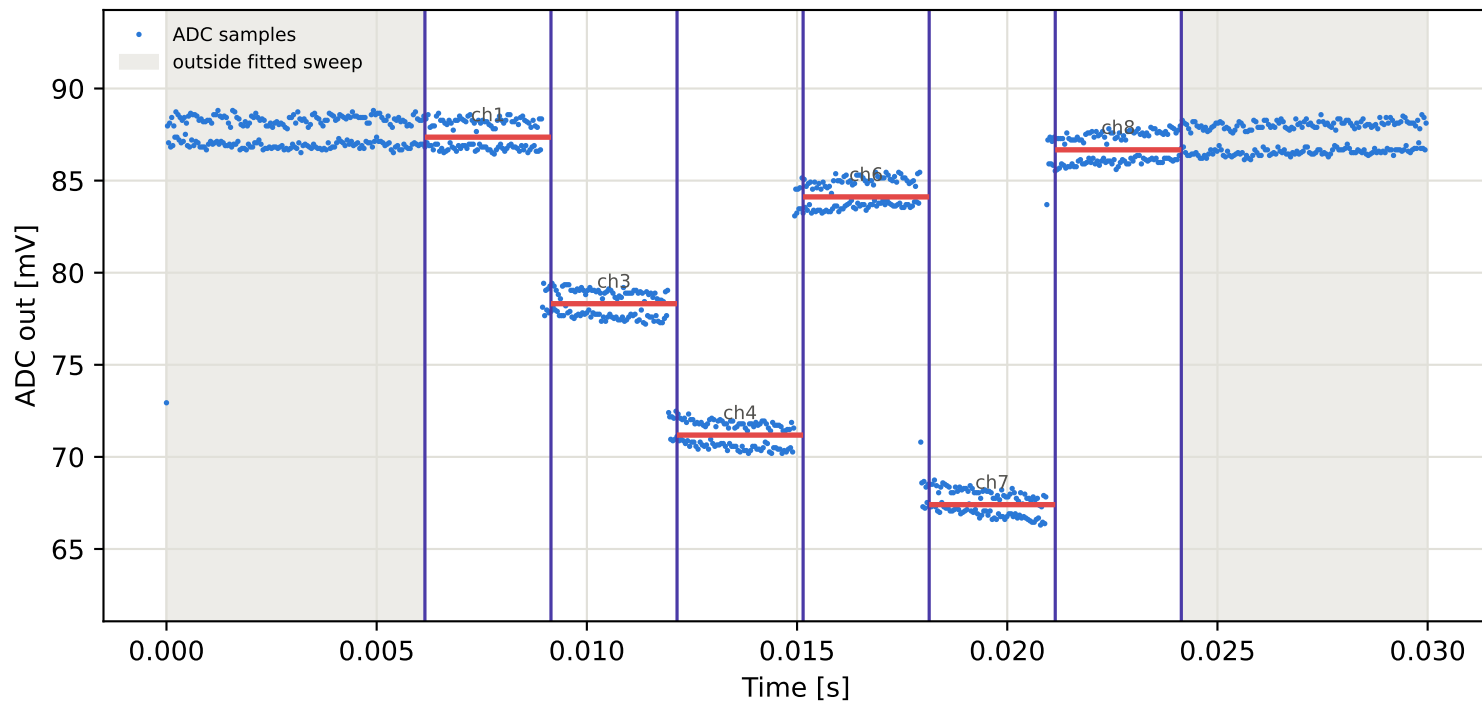
Tag2 &lt;- Tag1 | 785 MHz | run 0 | rep 1 | phase -55.23 deg
