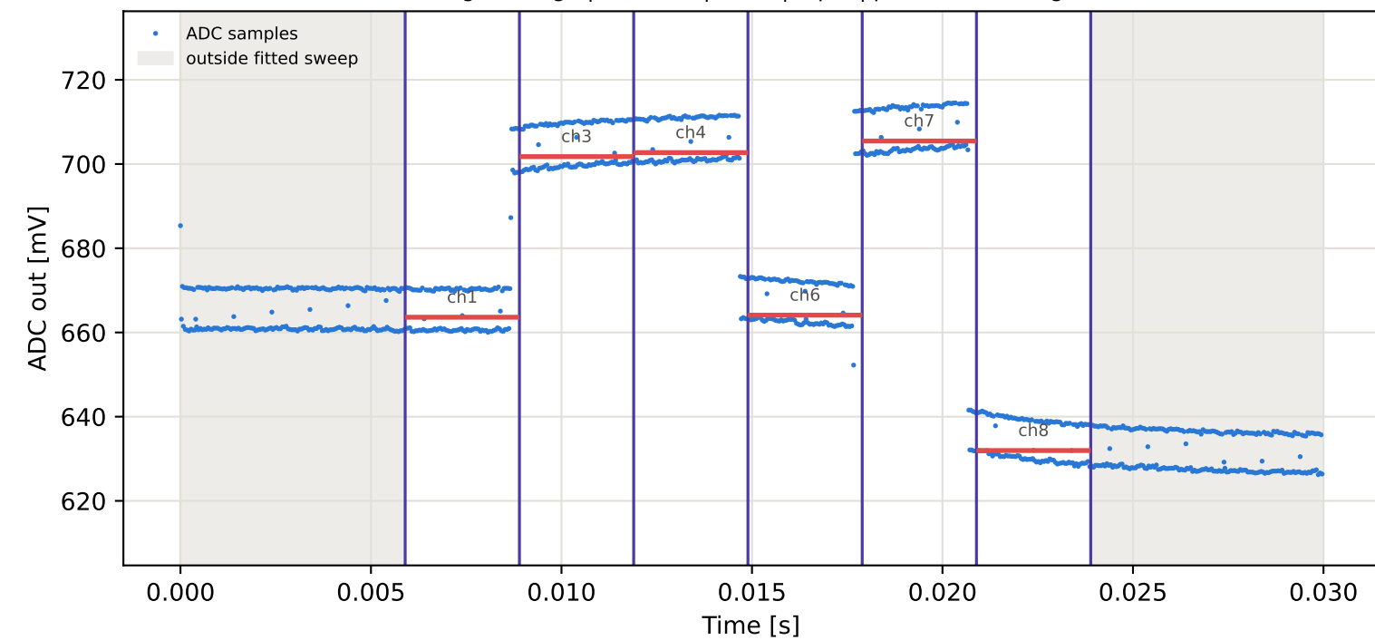
Tag7 &lt;- Tag5 | 865 MHz | run 0 | rep 1 | phase -165.85 deg
