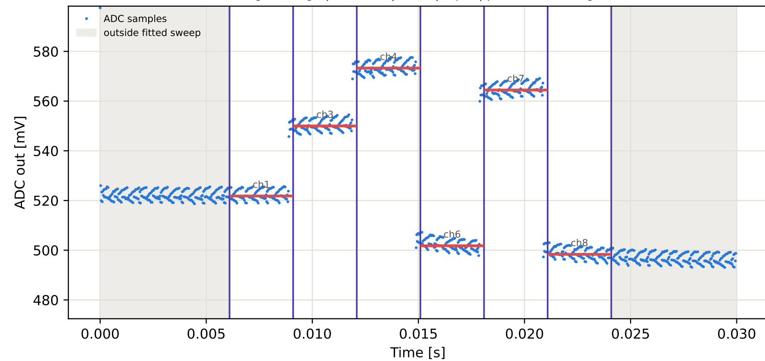
Tag8 &lt;- Tag10 | 955 MHz | run 0 | rep 1 | phase 33.69 deg
