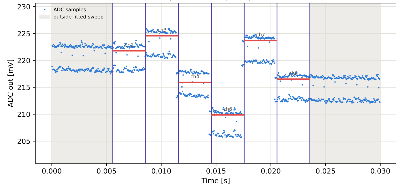
Tag7 &lt;- Tag1 | 995 MHz | run 0 | rep 1 | phase 60.70 deg
