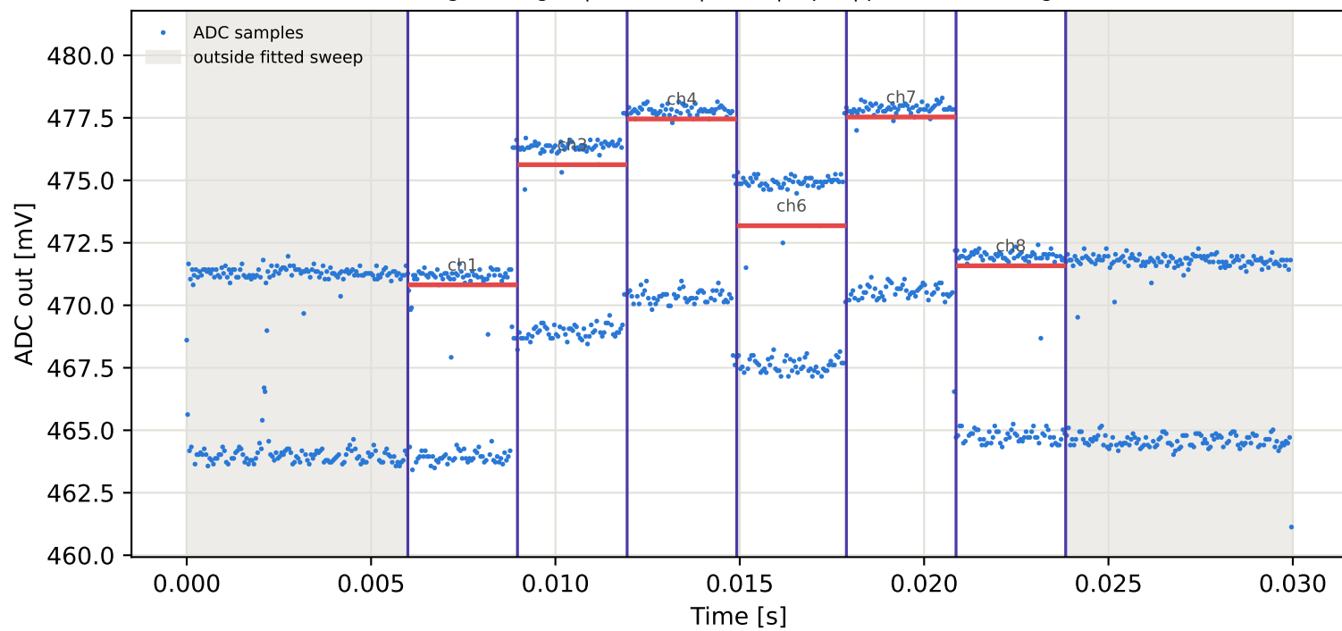
Tag4 &lt;- Tag16 | 855 MHz | run 0 | rep 1 | phase -56.27 deg
