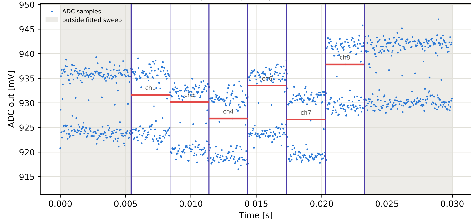
Tag15 &lt;- Tag4 | 885 MHz | run 0 | rep 1 | phase 131.37 deg
