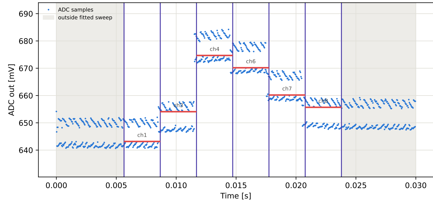
Tag16 &lt;- Tag7 | 965 MHz | run 0 | rep 1 | phase -14.71 deg
