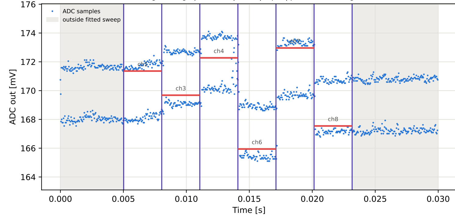
Tag1 &lt;- Tag4 | 995 MHz | run 0 | rep 1 | phase 97.19 deg
