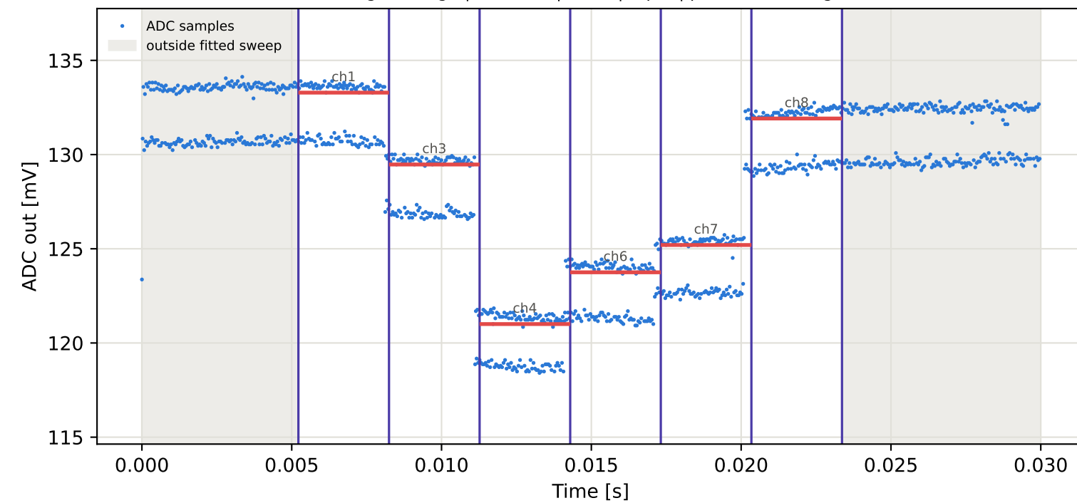
Tag3 &lt;- Tag10 | 945 MHz | run 0 | rep 1 | phase 7.63 deg
