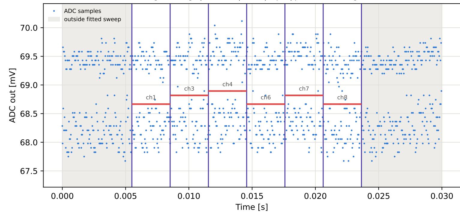
Tag16 &lt;- Tag4 | 775 MHz | run 0 | rep 1 | phase -138.56 deg
