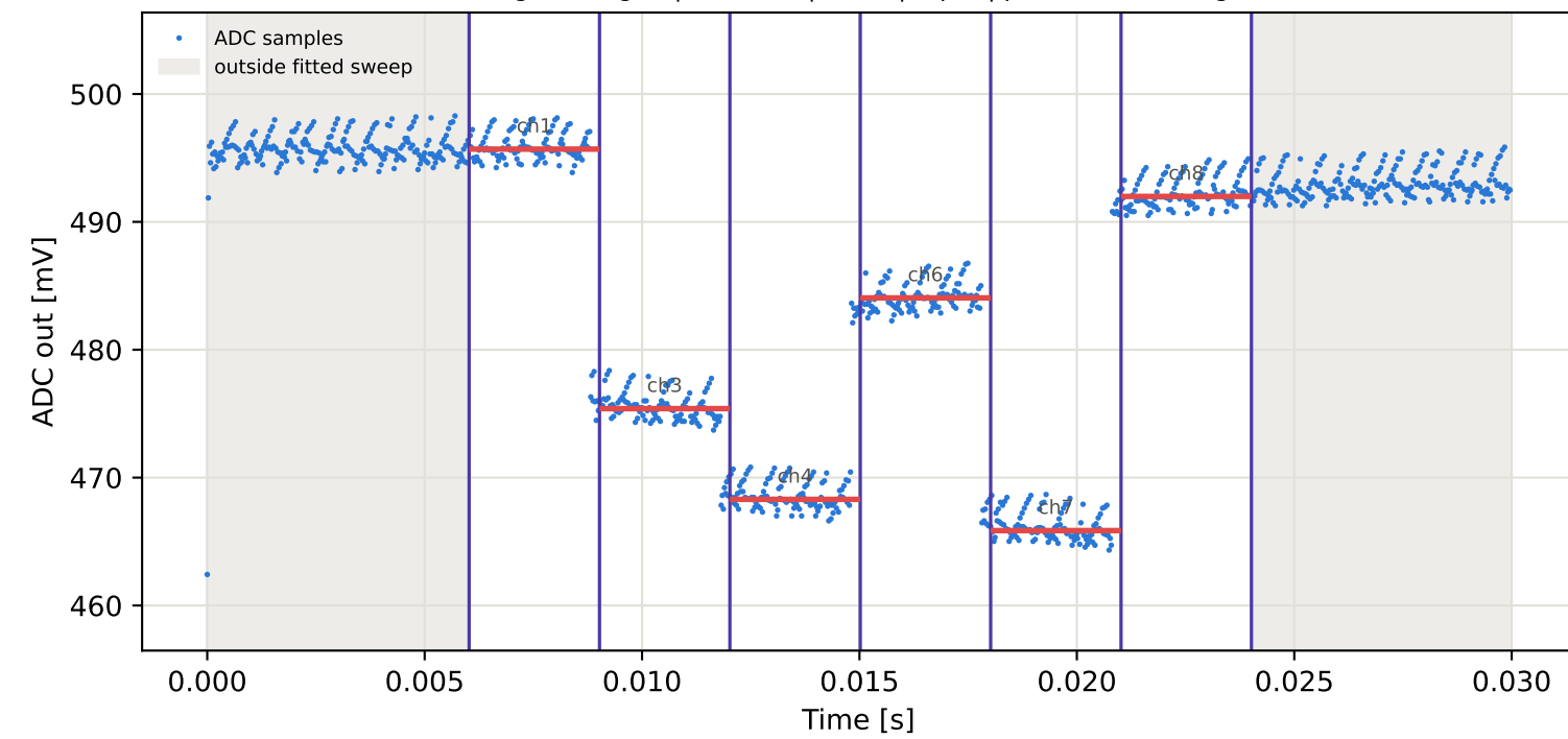
Tag7 &lt;- Tag3 | 835 MHz | run 0 | rep 1 | phase -116.48 deg
