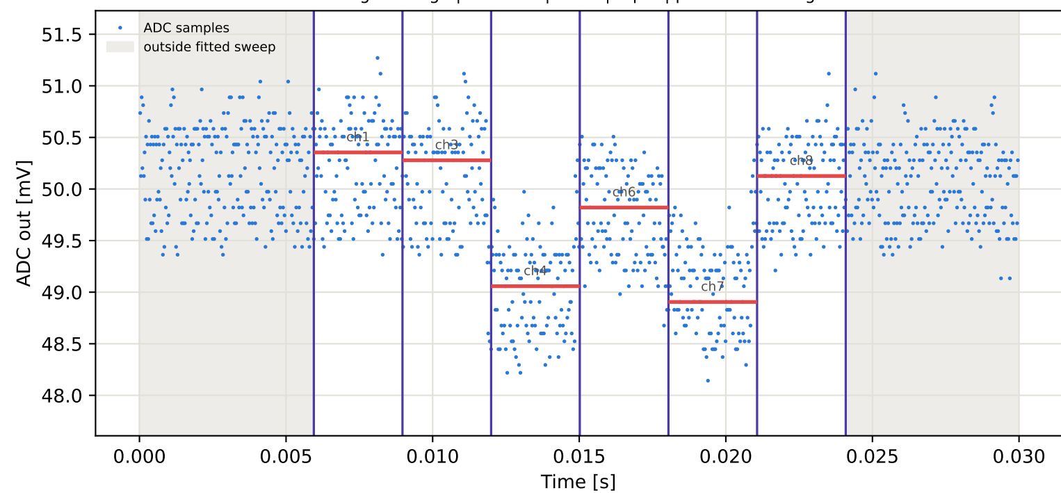
Tag10 &lt;- Tag1 | 775 MHz | run 0 | rep 1 | phase -98.12 deg
