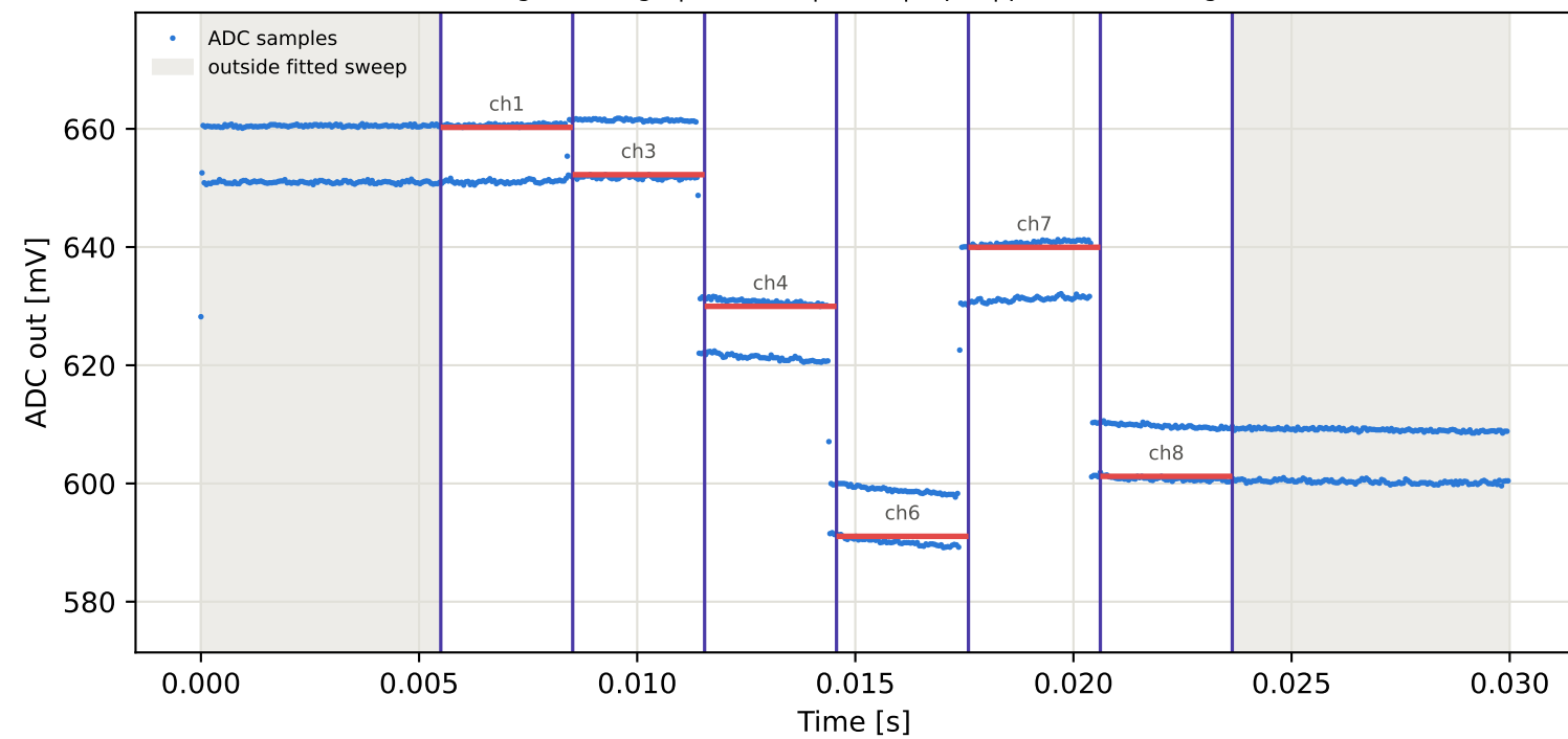
Tag16 &lt;- Tag1 | 865 MHz | run 0 | rep 1 | phase 94.05 deg
