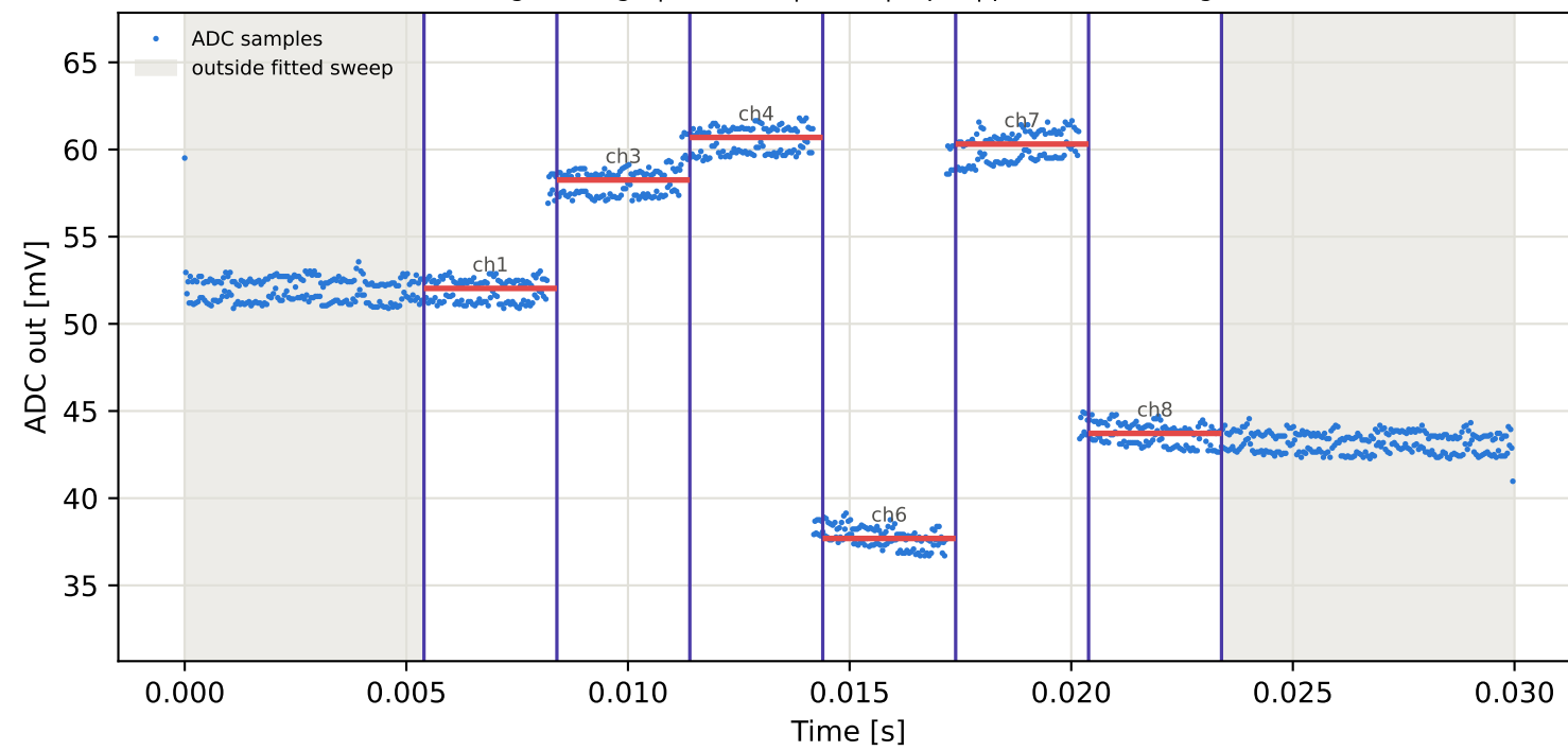
Tag1 &lt;- Tag7 | 955 MHz | run 0 | rep 1 | phase -110.49 deg
