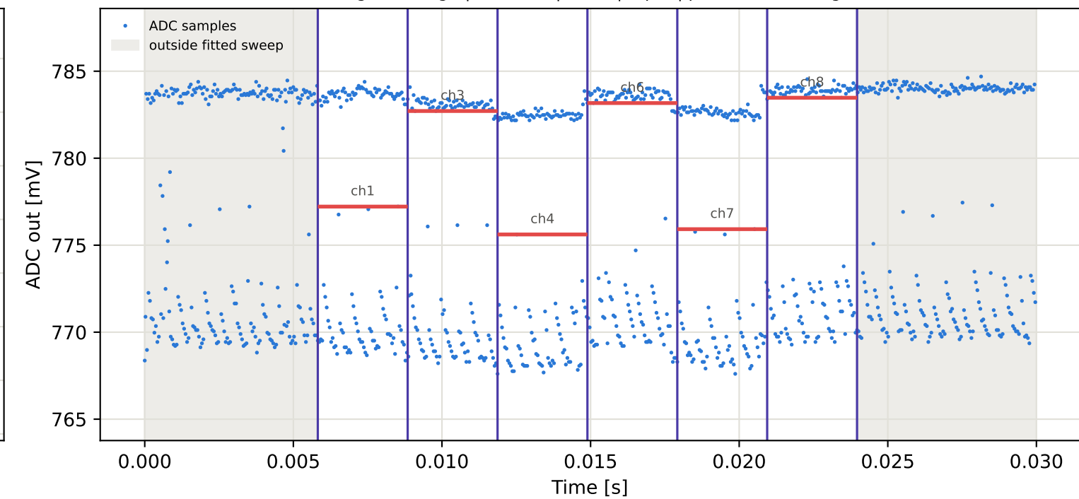
Tag15 &lt;- Tag4 | 945 MHz | run 0 | rep 1 | phase -125.13 deg
