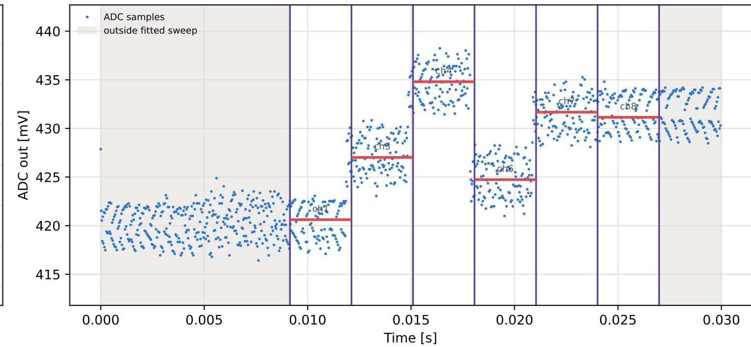
Tag9 &lt;- Tag15 | 875 MHz | run 0 | rep 1 | phase -153.14 deg
