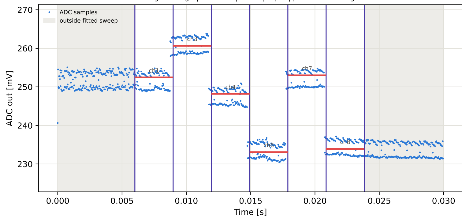
Tag9 &lt;- Tag8 | 845 MHz | run 0 | rep 1 | phase -42.13 deg
