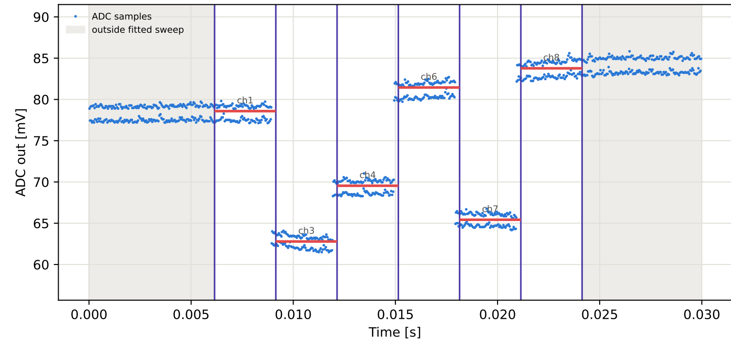
Tag9 &lt;- Tag16 | 835 MHz | run 0 | rep 1 | phase -92.73 deg
