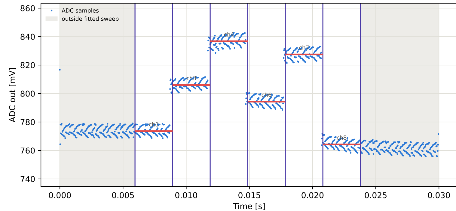
Tag9 &lt;- Tag7 | 925 MHz | run 0 | rep 1 | phase -86.57 deg
