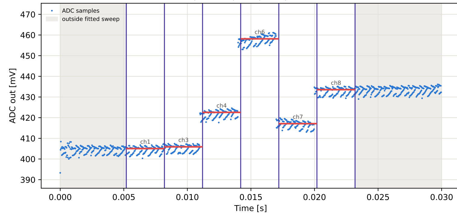
Tag6 &lt;- Tag4 | 895 MHz | run 0 | rep 1 | phase -157.61 deg
