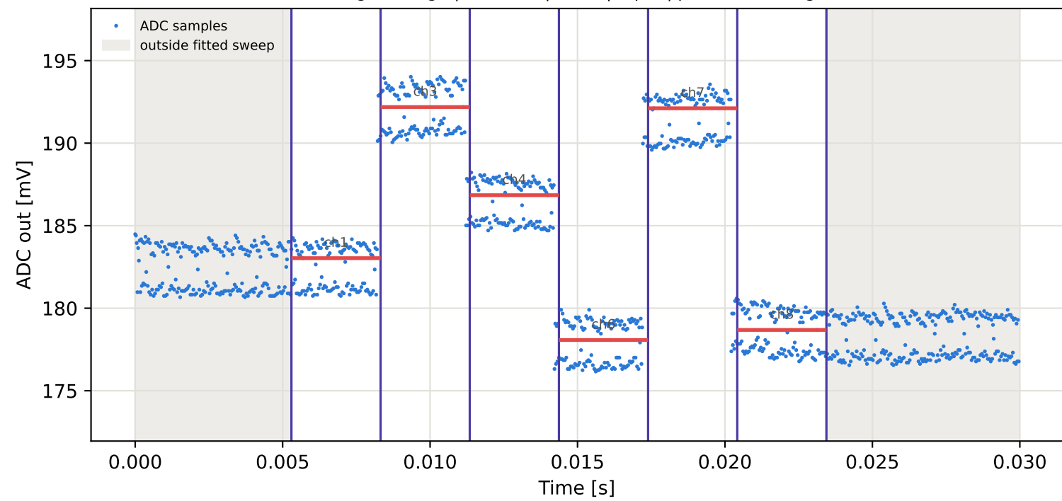
Tag4 &lt;- Tag15 | 825 MHz | run 0 | rep 1 | phase -145.98 deg
