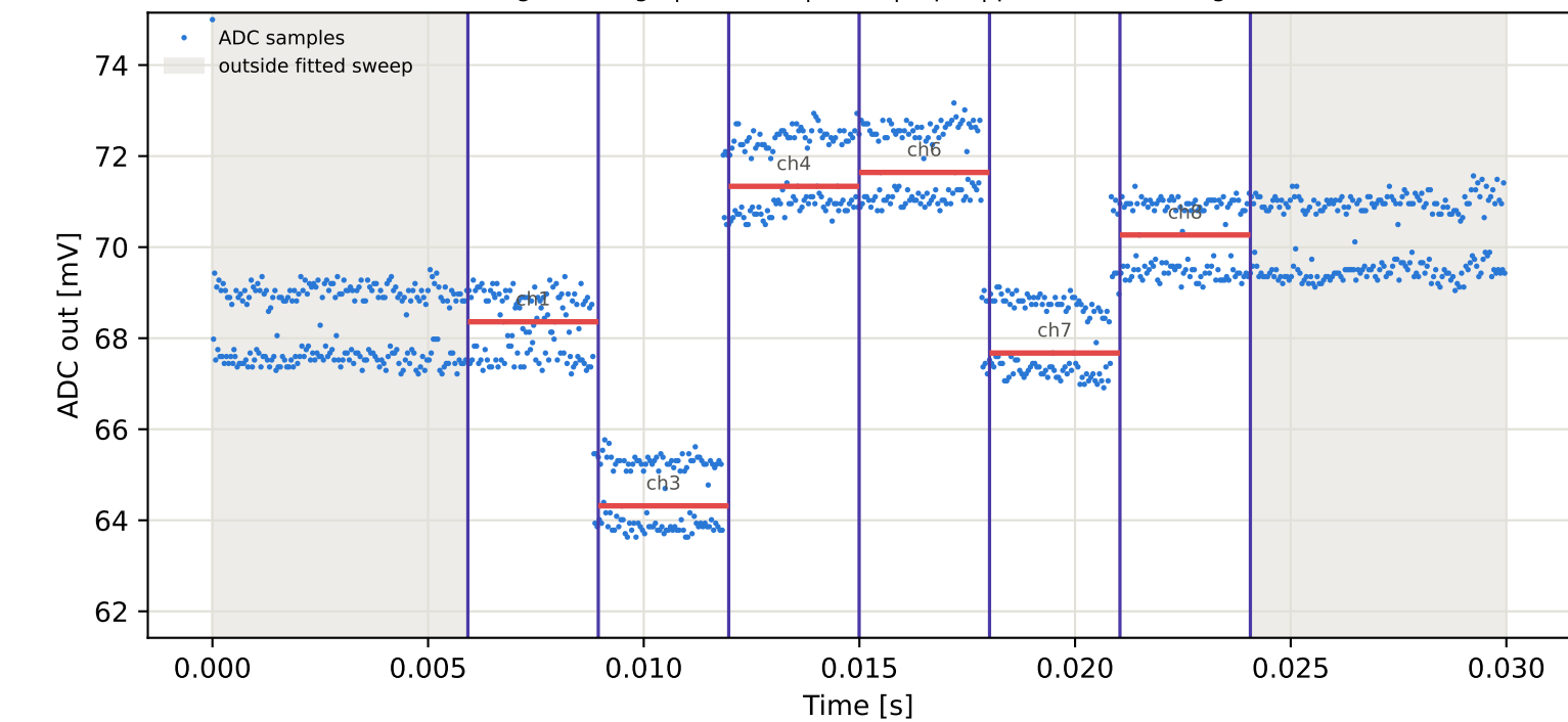
Tag16 &lt;- Tag6 | 775 MHz | run 0 | rep 1 | phase -34.05 deg
