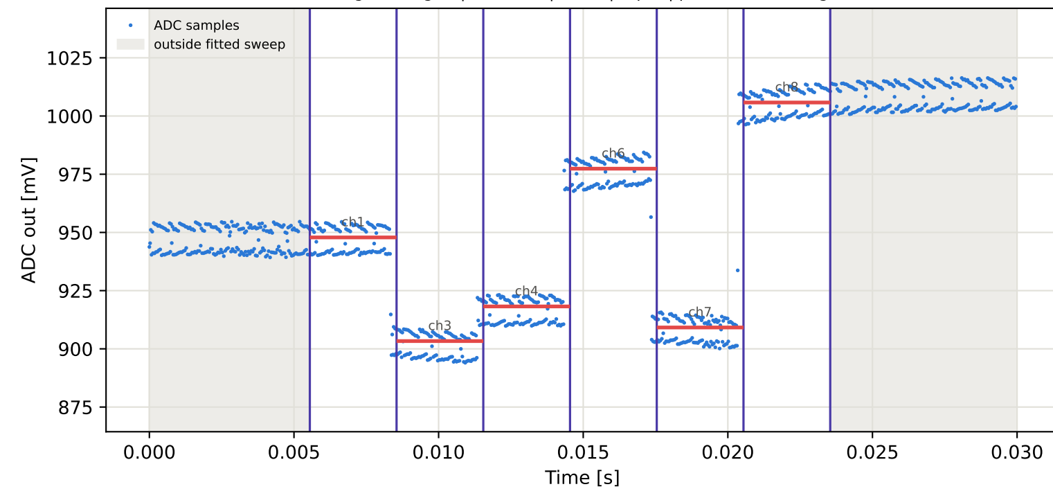
Tag7 &lt;- Tag3 | 875 MHz | run 0 | rep 1 | phase -28.47 deg
