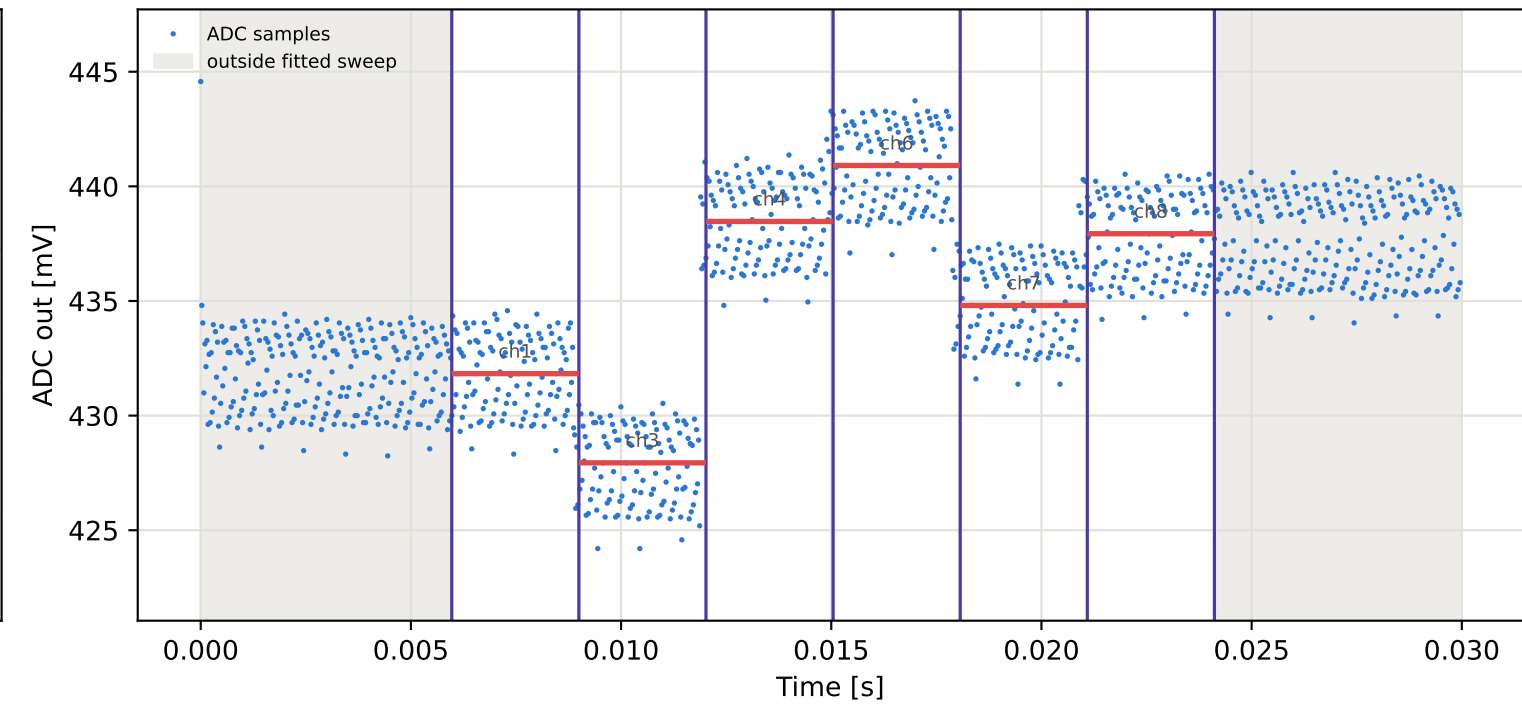
Tag3 &lt;- Tag2 | 835 MHz | run 0 | rep 1 | phase -146.12 deg
