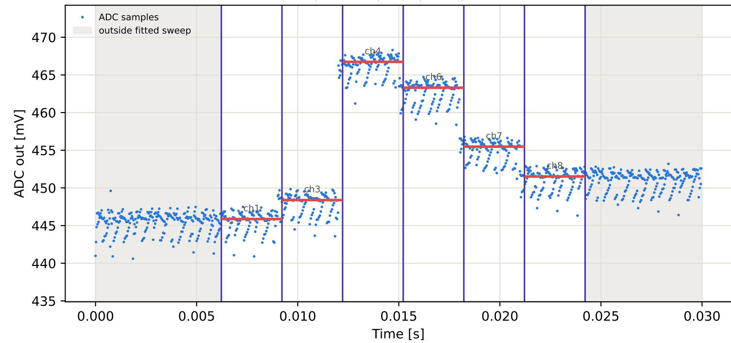
Tag16 &lt;- Tag15 | 995 MHz | run 0 | rep 1 | phase -133.07 deg
