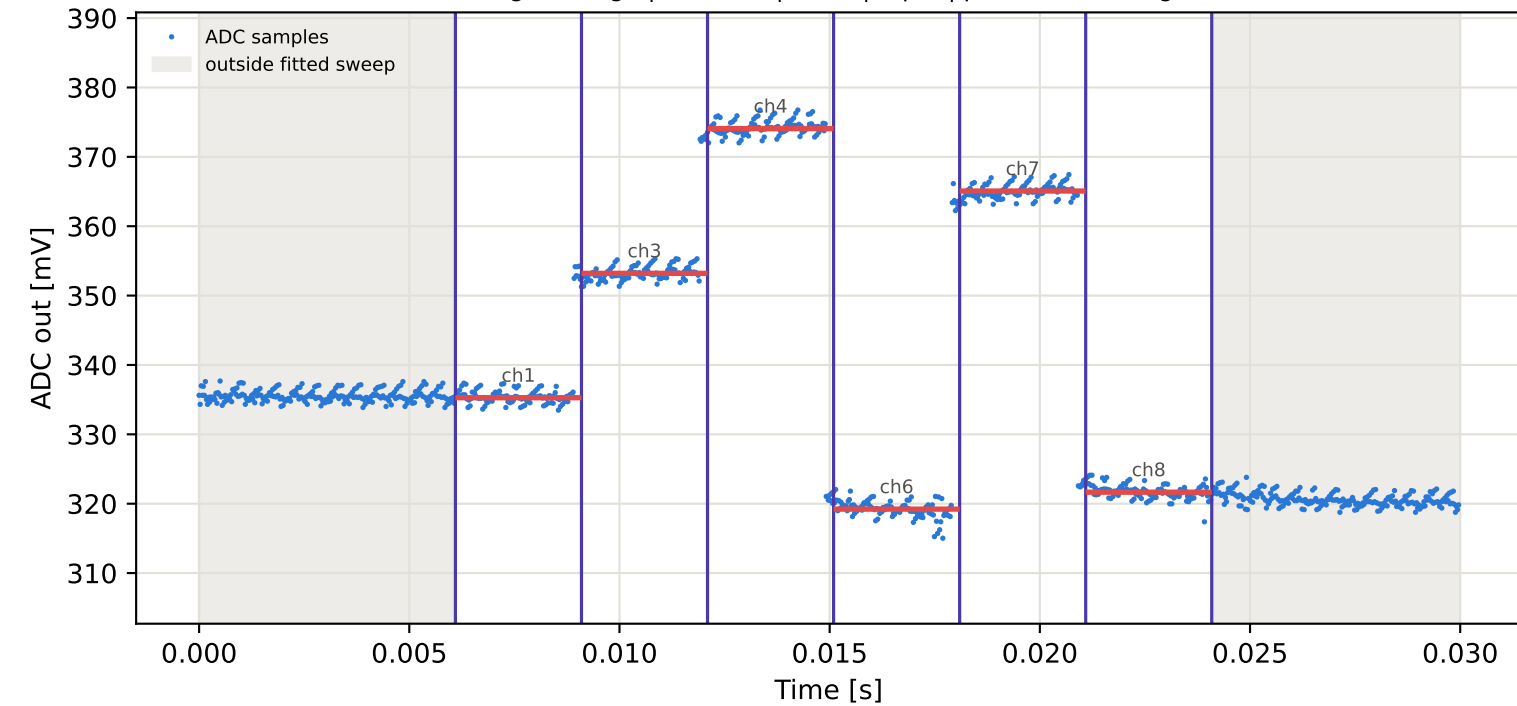
Tag6 &lt;- Tag1 | 965 MHz | run 0 | rep 1 | phase 144.08 deg
