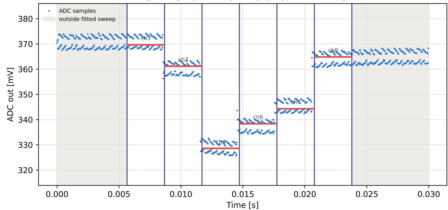
Tag5 &lt;- Tag2 | 965 MHz | run 0 | rep 1 | phase -109.84 deg
