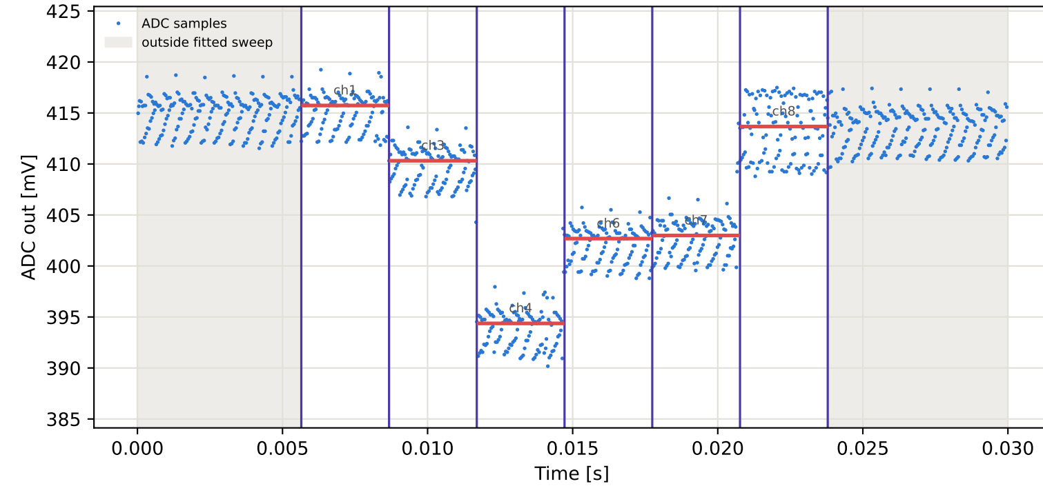
Tag15 &lt;- Tag1 | 955 MHz | run 0 | rep 1 | phase 148.70 deg
