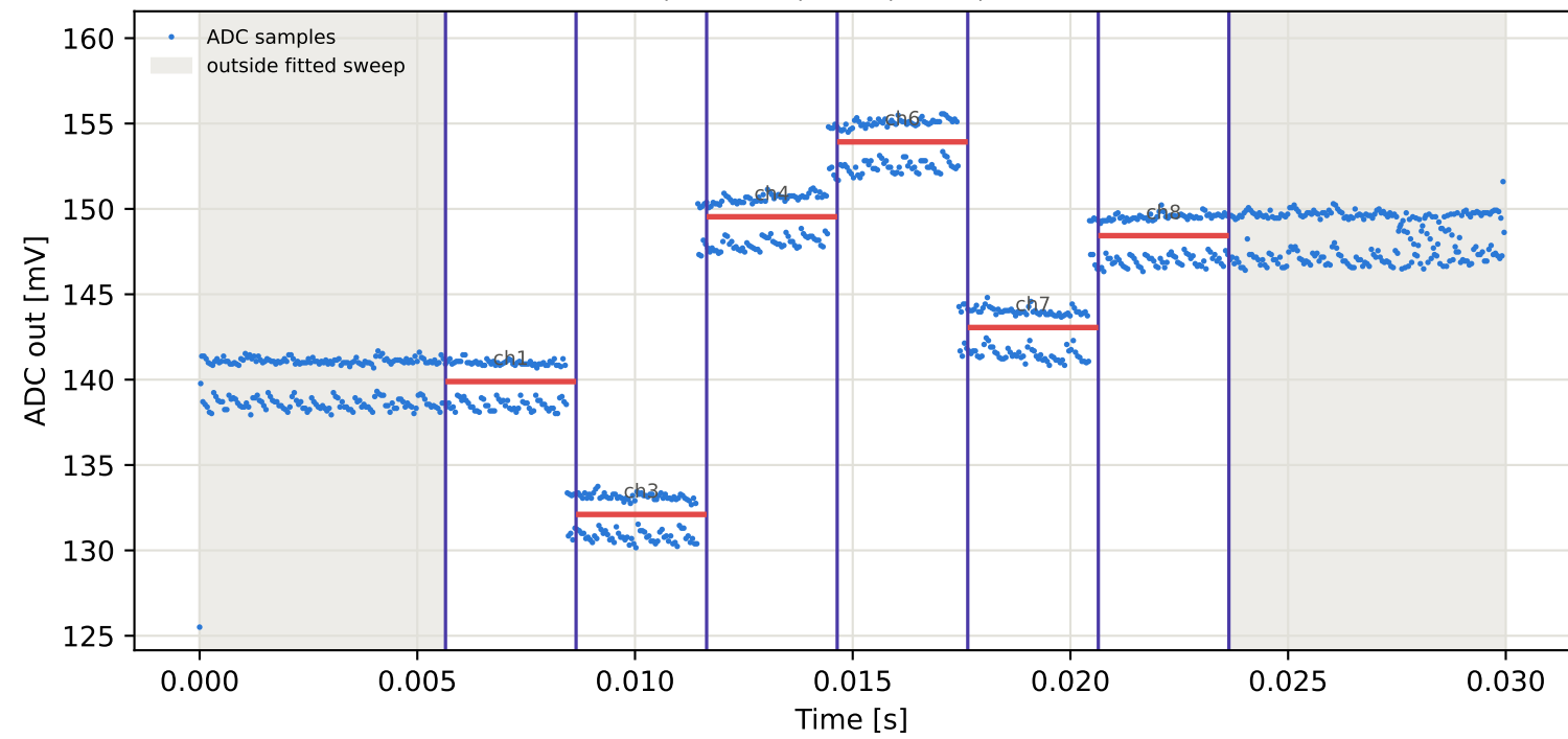
Tag15 &lt;- Tag5 | 805 MHz | run 0 | rep 1 | phase -140.36 deg
