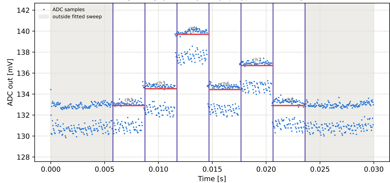
Tag3 &lt;- Tag15 | 995 MHz | run 0 | rep 1 | phase 44.15 deg
