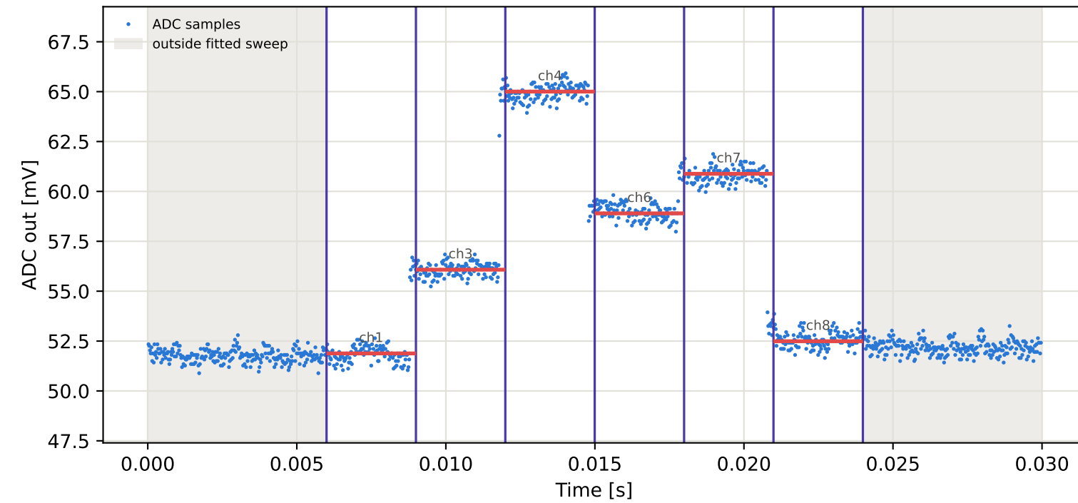
Tag1 &lt;- Tag9 | 955 MHz | run 0 | rep 1 | phase -0.44 deg
