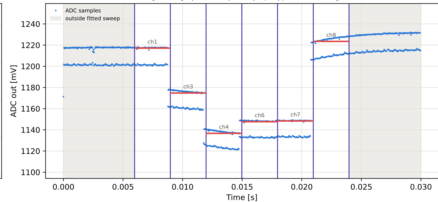
Tag8 &lt;- Tag7 | 895 MHz | run 0 | rep 1 | phase -130.19 deg
