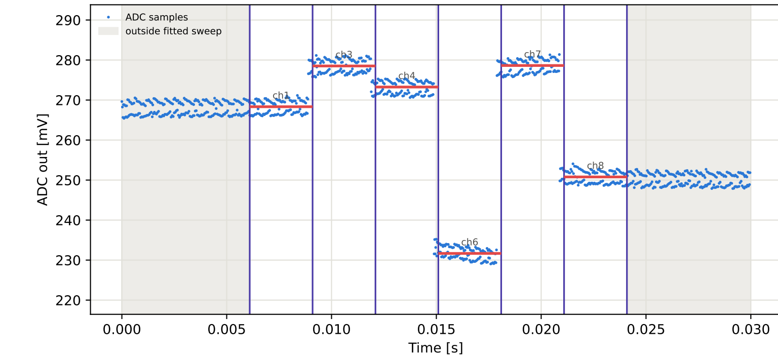
Tag9 &lt;- Tag16 | 975 MHz | run 0 | rep 1 | phase 127.79 deg
