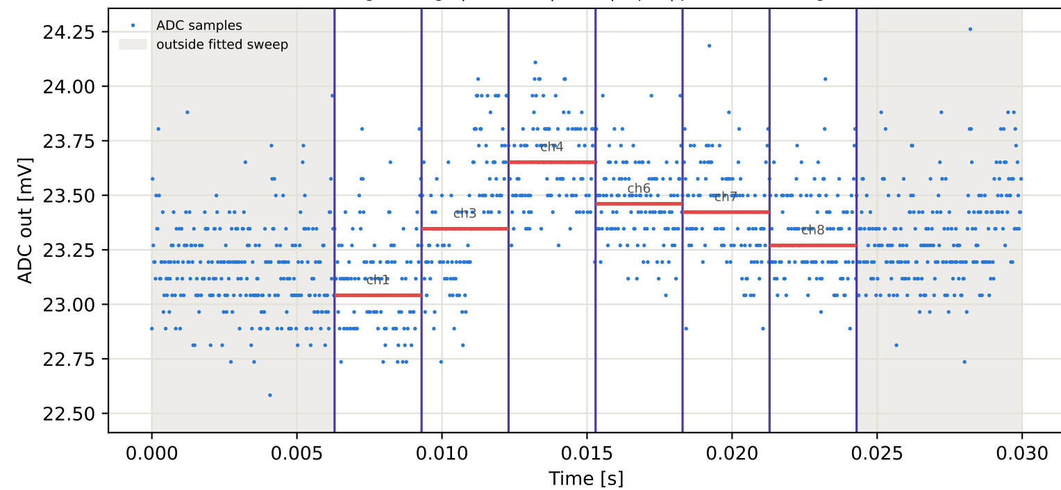
Tag3 &lt;- Tag15 | 785 MHz | run 0 | rep 1 | phase 137.17 deg
