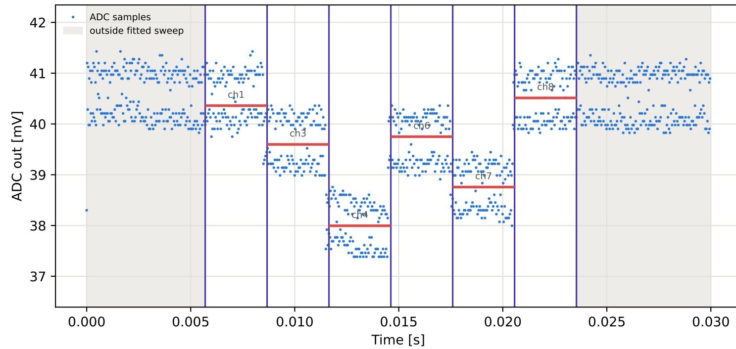
Tag3 &lt;- Tag10 | 985 MHz | run 0 | rep 1 | phase 94.17 deg
