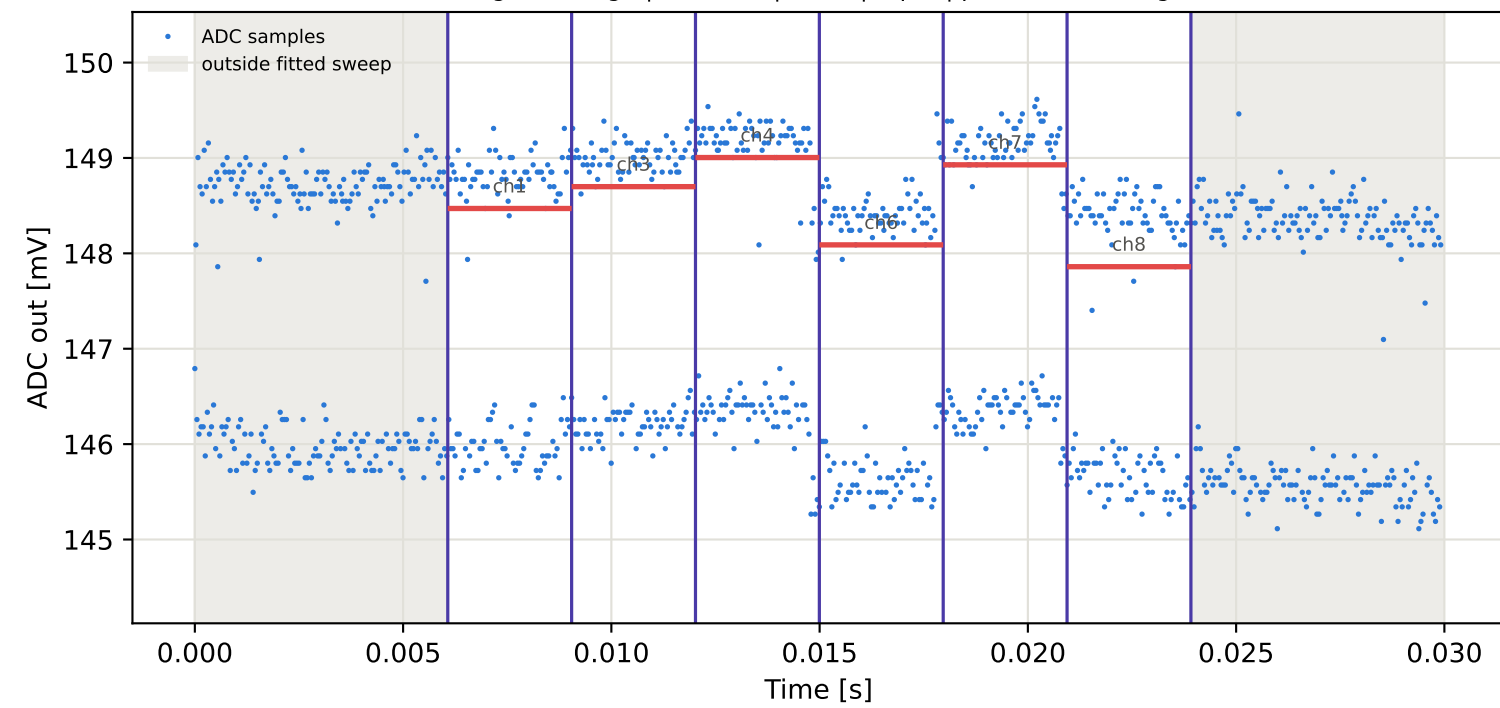
Tag15 &lt;- Tag4 | 805 MHz | run 0 | rep 1 | phase -90.66 deg
