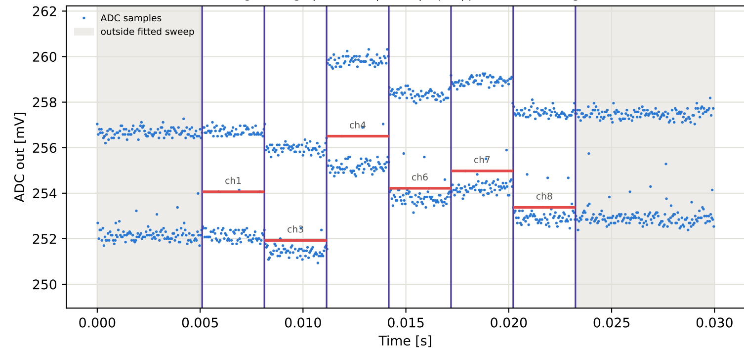
Tag8 &lt;- Tag5 | 785 MHz | run 0 | rep 1 | phase 124.58 deg
