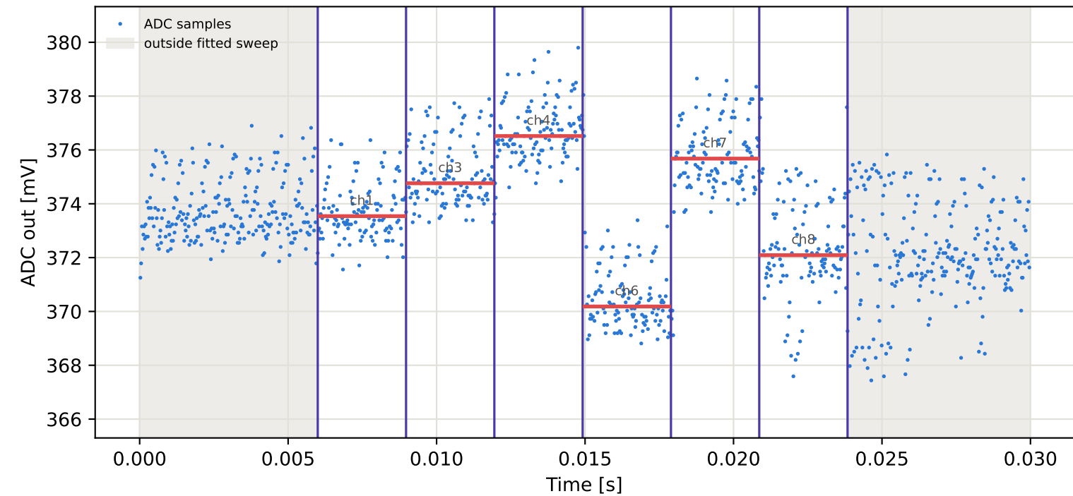
Tag5 &lt;- Tag4 | 985 MHz | run 0 | rep 1 | phase -143.56 deg
