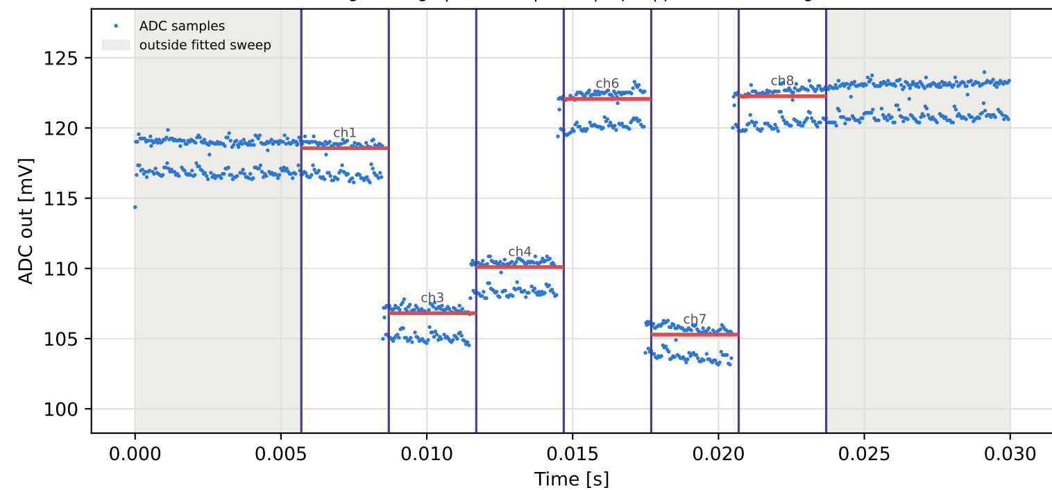
Tag6 &lt;- Tag5 | 805 MHz | run 0 | rep 1 | phase 158.38 deg
