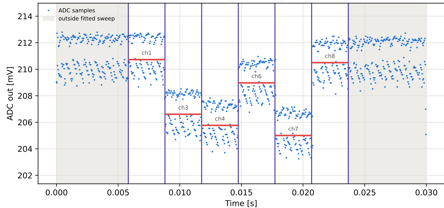
Tag16 &lt;- Tag10 | 825 MHz | run 0 | rep 1 | phase 119.86 deg
