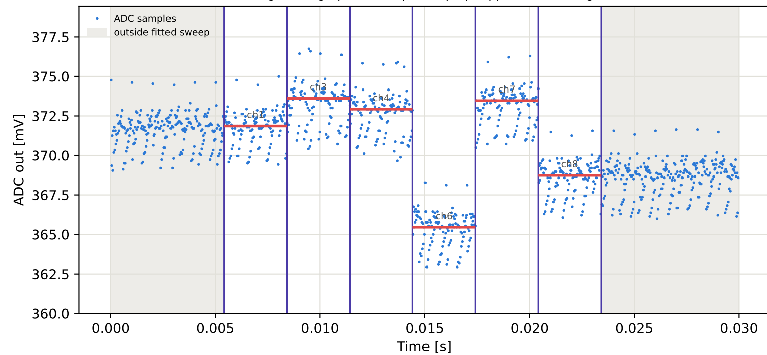
Tag4 &lt;- Tag8 | 945 MHz | run 0 | rep 1 | phase -15.11 deg
