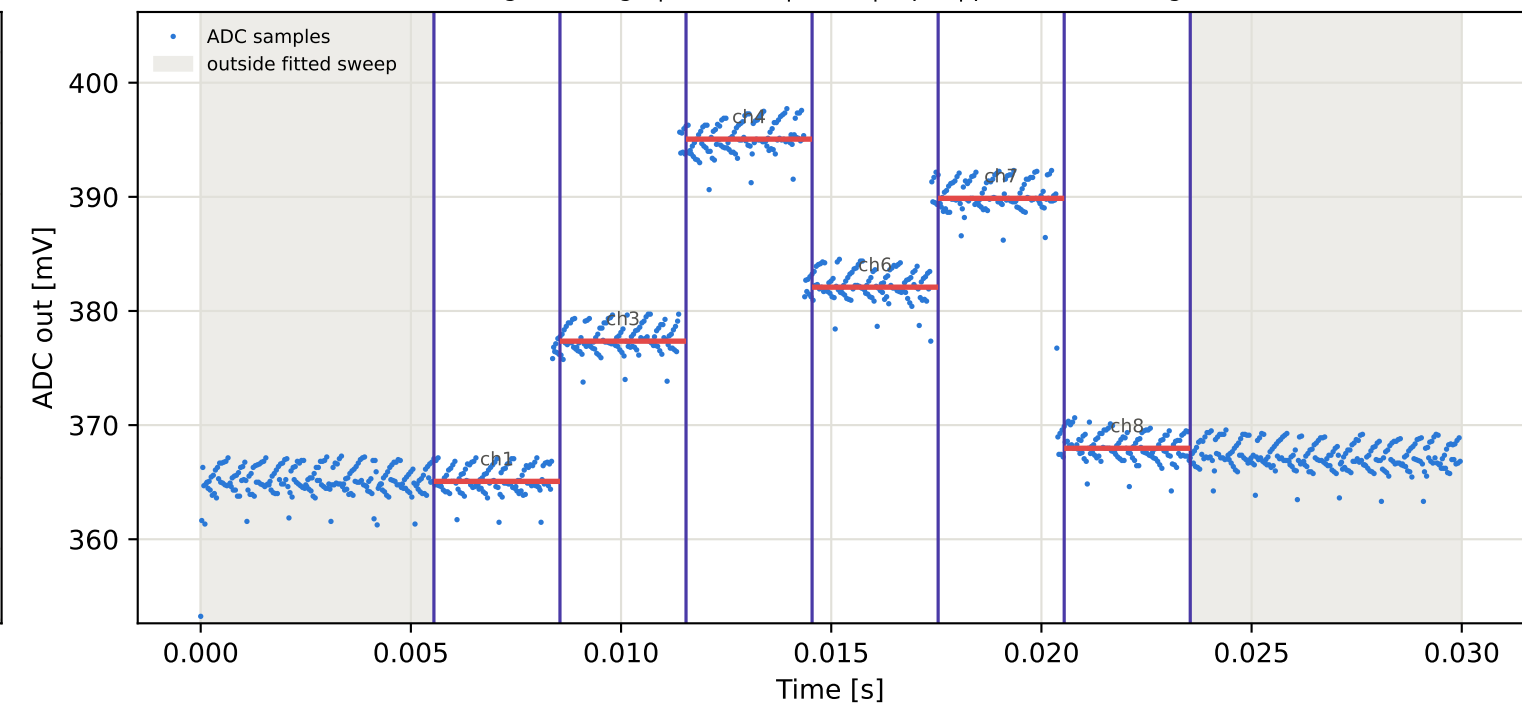
Tag10 &lt;- Tag9 | 865 MHz | run 0 | rep 1 | phase -113.67 deg
