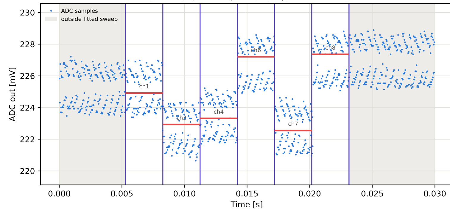
Tag3 &lt;- Tag10 | 835 MHz | run 0 | rep 1 | phase 78.86 deg
