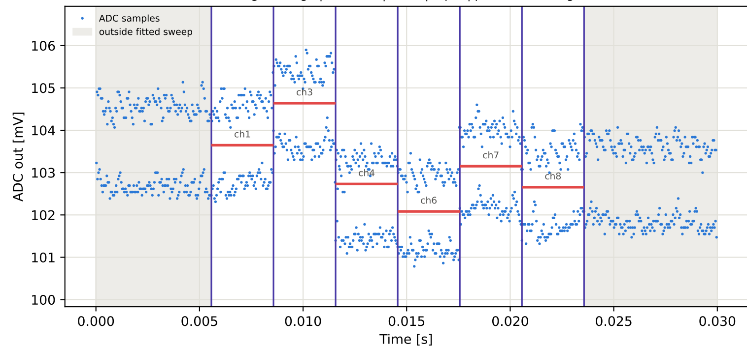
Tag7 &lt;- Tag6 | 775 MHz | run 0 | rep 1 | phase 40.88 deg
