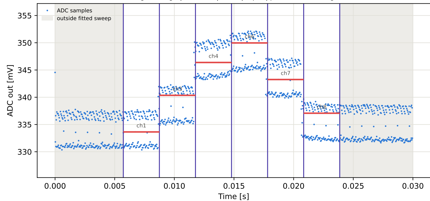
Tag10 &lt;- Tag1 | 925 MHz | run 0 | rep 1 | phase 178.01 deg
