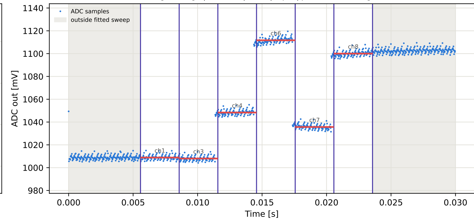
Tag3 &lt;- Tag7 | 875 MHz | run 0 | rep 1 | phase -168.79 deg
