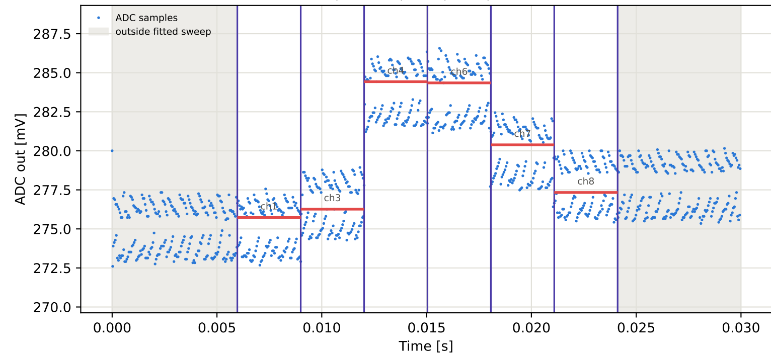
Tag10 &lt;- Tag1 | 965 MHz | run 0 | rep 1 | phase -132.78 deg
