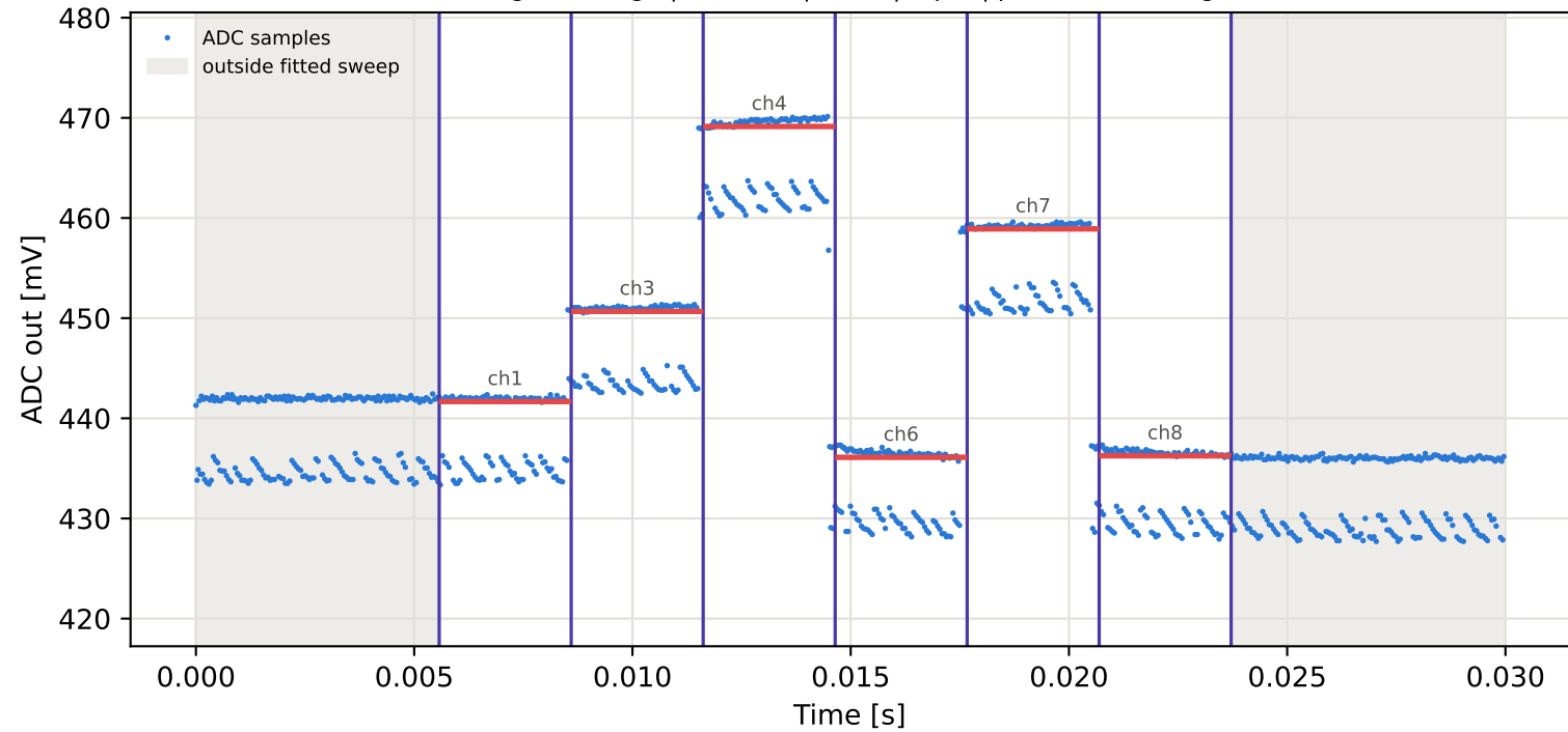
Tag16 &lt;- Tag5 | 995 MHz | run 0 | rep 1 | phase -56.79 deg
