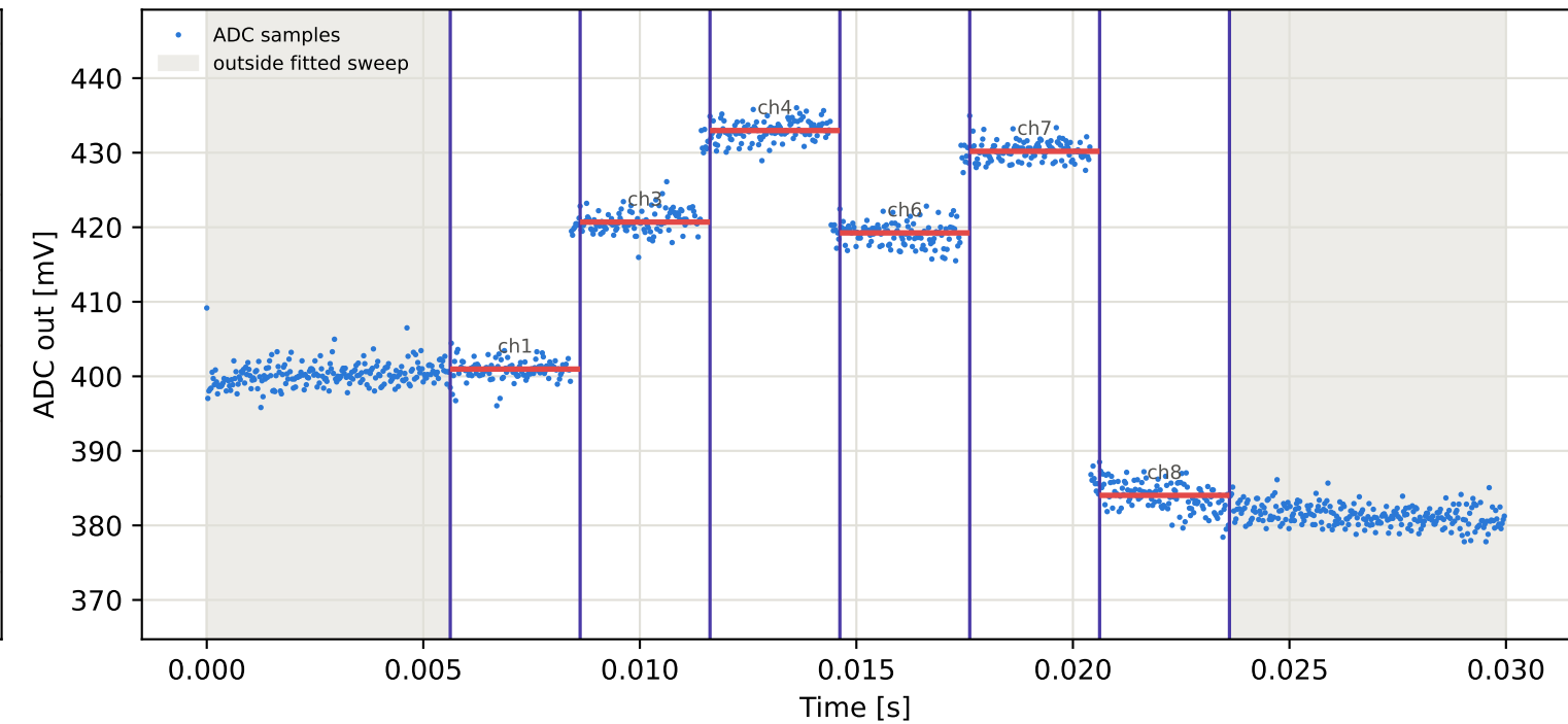
Tag1 &lt;- Tag4 | 885 MHz | run 0 | rep 1 | phase -57.08 deg
