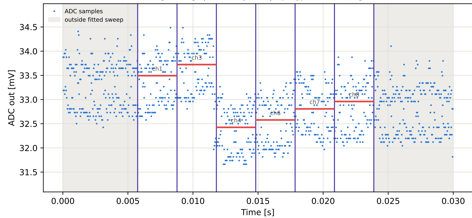
Tag1 &lt;- Tag8 | 795 MHz | run 0 | rep 1 | phase 119.56 deg
