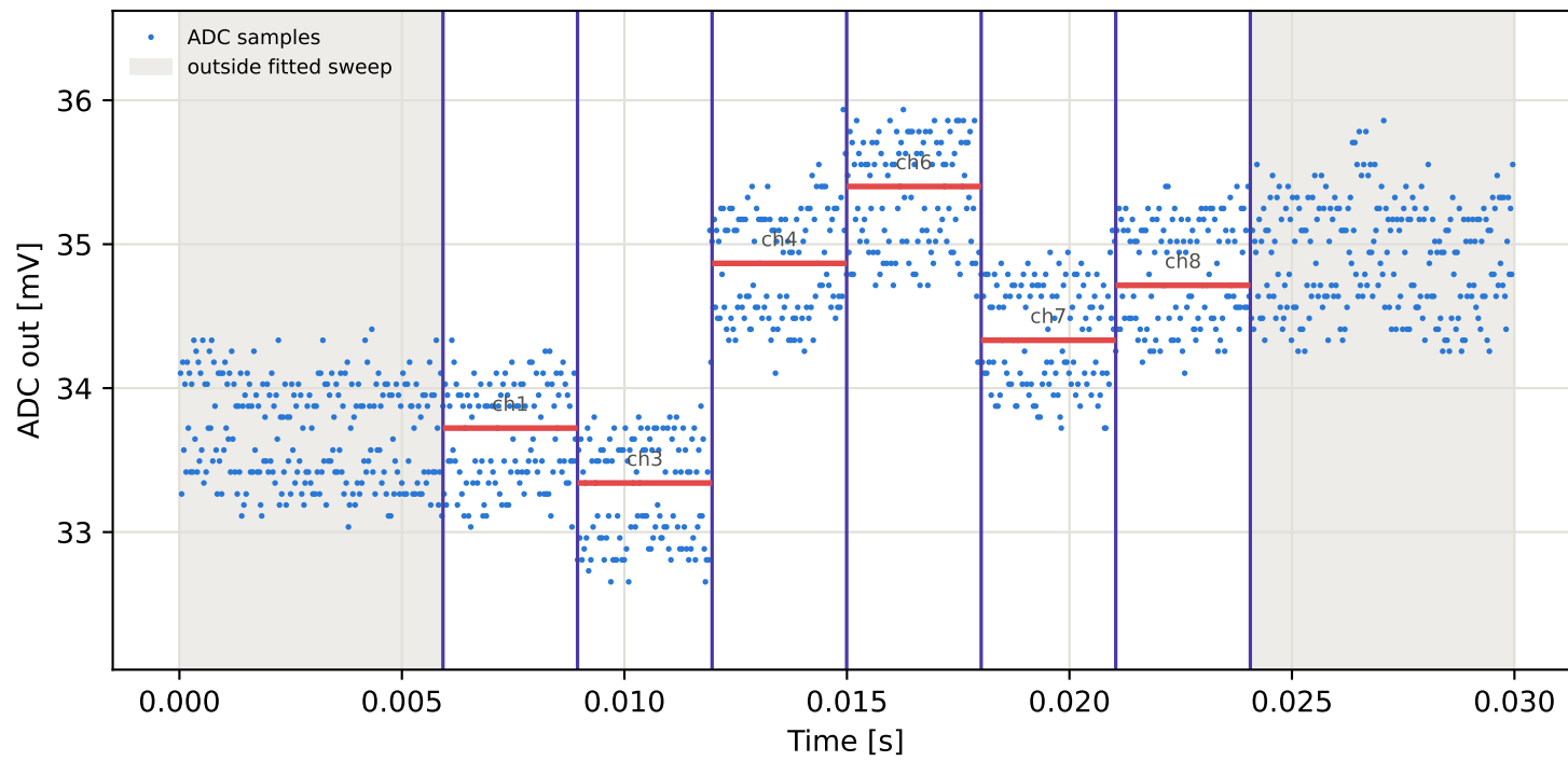
Tag3 &lt;- Tag10 | 805 MHz | run 0 | rep 1 | phase 78.39 deg
