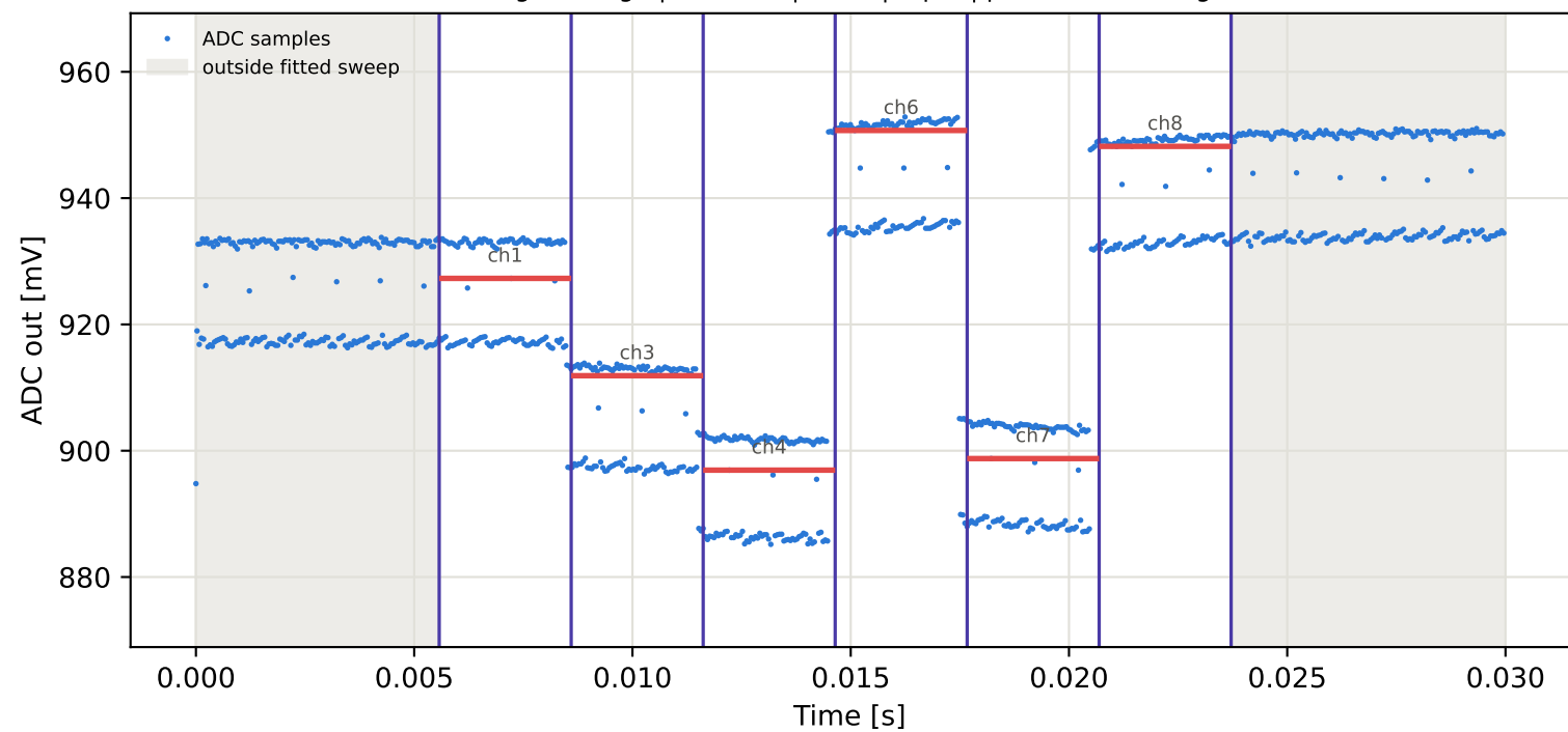
Tag8 &lt;- Tag7 | 985 MHz | run 0 | rep 1 | phase 132.46 deg
