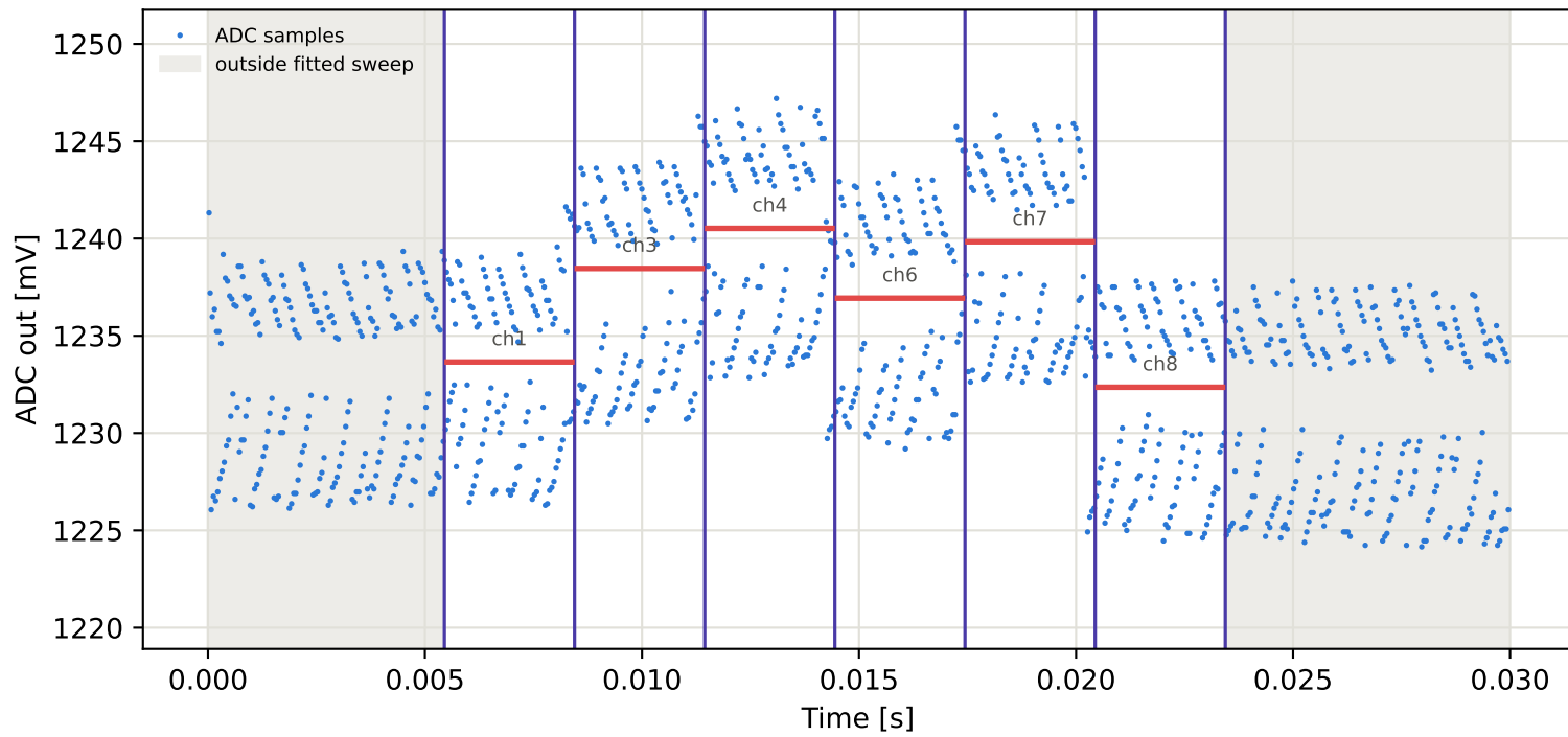
Tag16 &lt;- Tag15 | 895 MHz | run 0 | rep 1 | phase 102.90 deg
