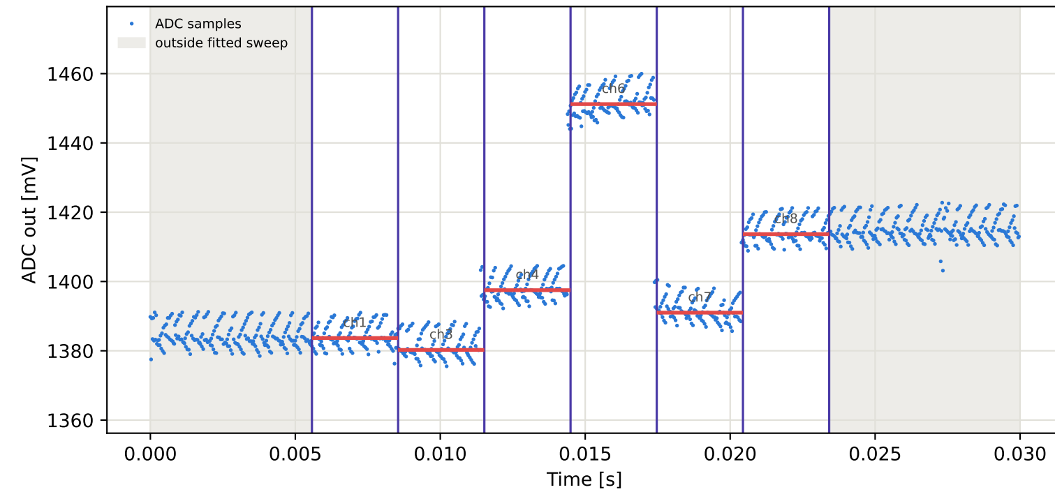
Tag15 &lt;- Tag5 | 915 MHz | run 0 | rep 1 | phase 73.51 deg
