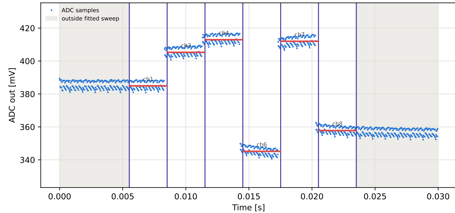
Tag3 &lt;- Tag2 | 955 MHz | run 0 | rep 1 | phase -1.21 deg
