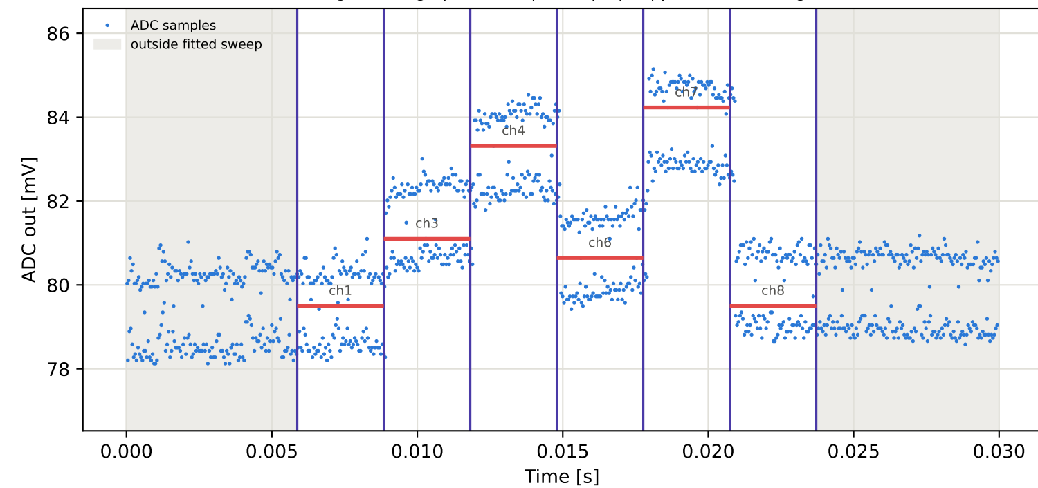
Tag16 &lt;- Tag1 | 795 MHz | run 0 | rep 1 | phase -95.54 deg
