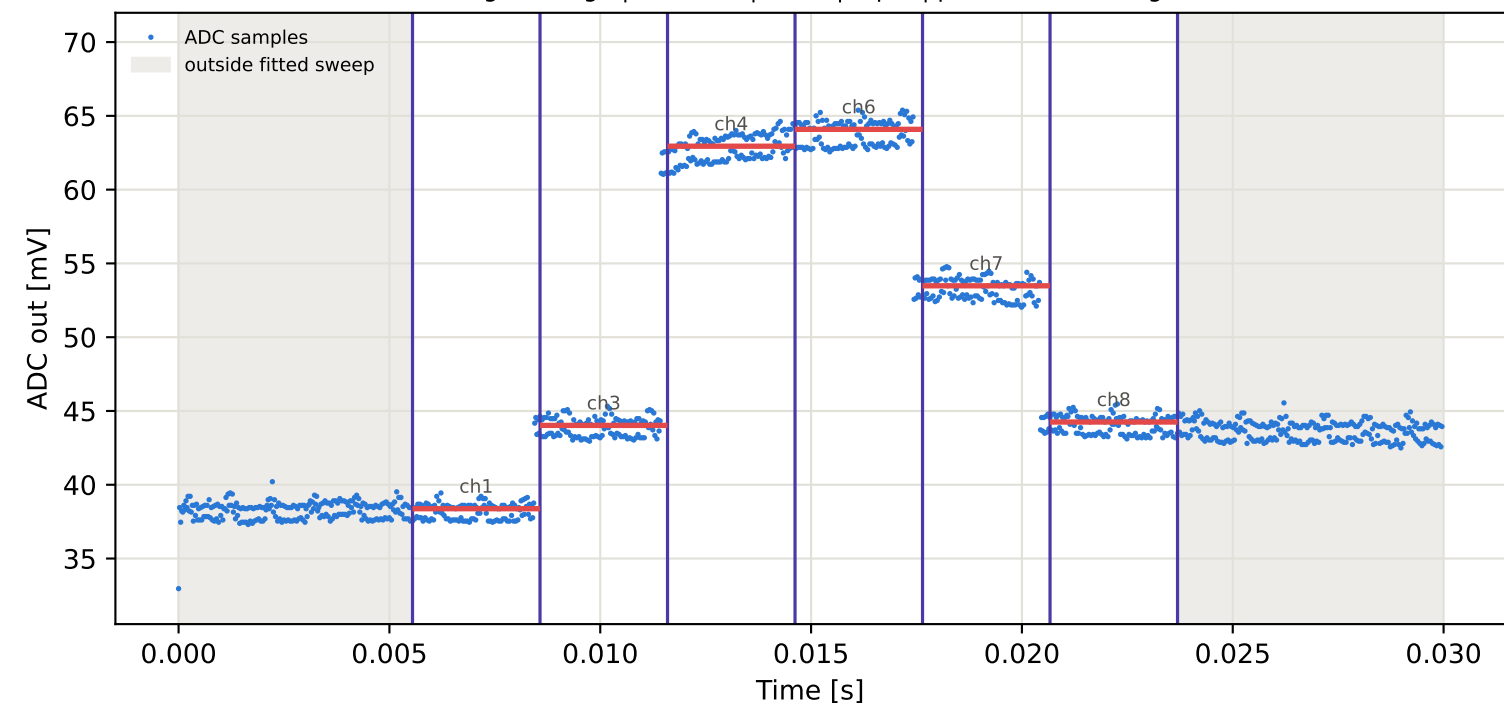
Tag6 &lt;- Tag5 | 945 MHz | run 0 | rep 1 | phase -131.08 deg
