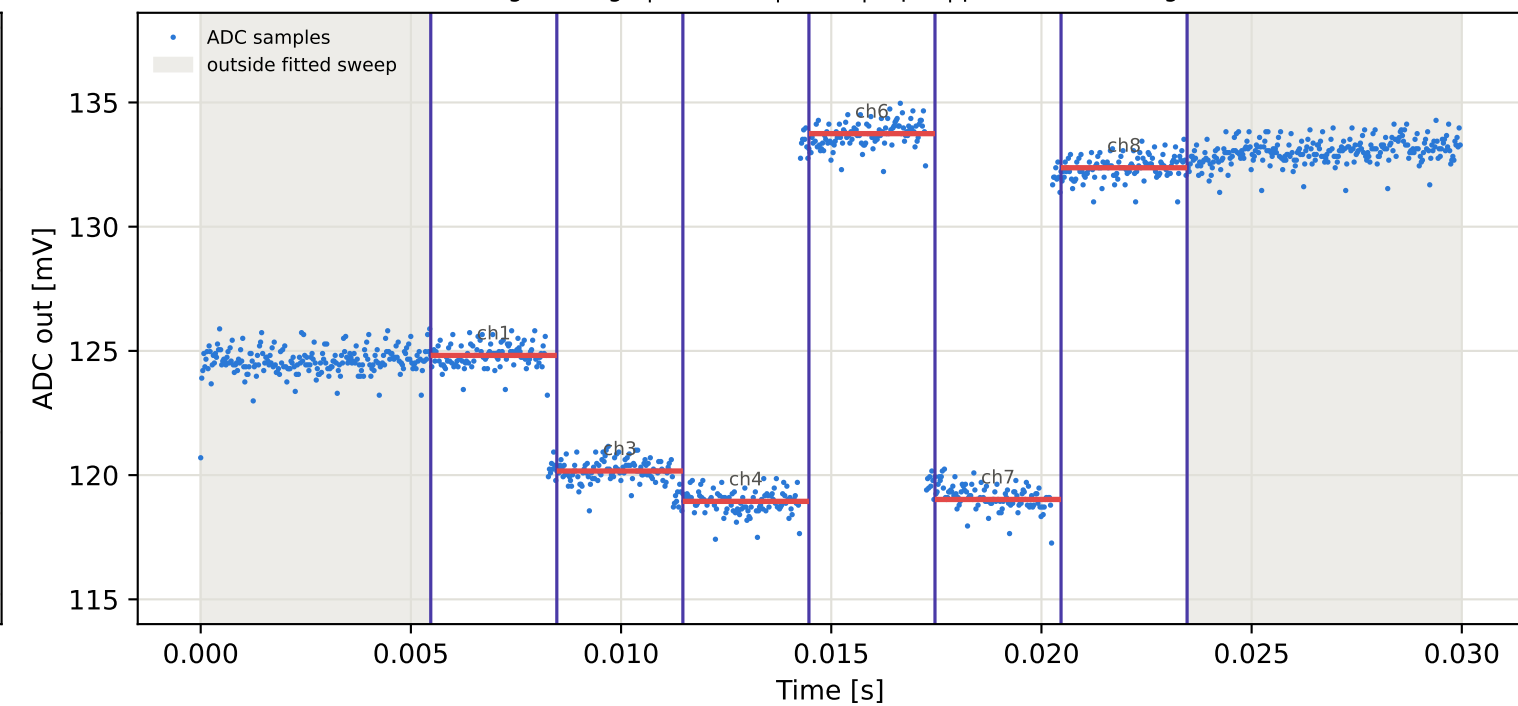
Tag1 &lt;- Tag4 | 915 MHz | run 0 | rep 1 | phase 154.80 deg
