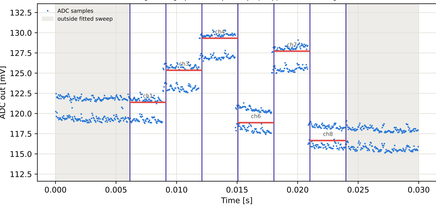
Tag6 &lt;- Tag4 | 935 MHz | run 0 | rep 1 | phase -56.73 deg
