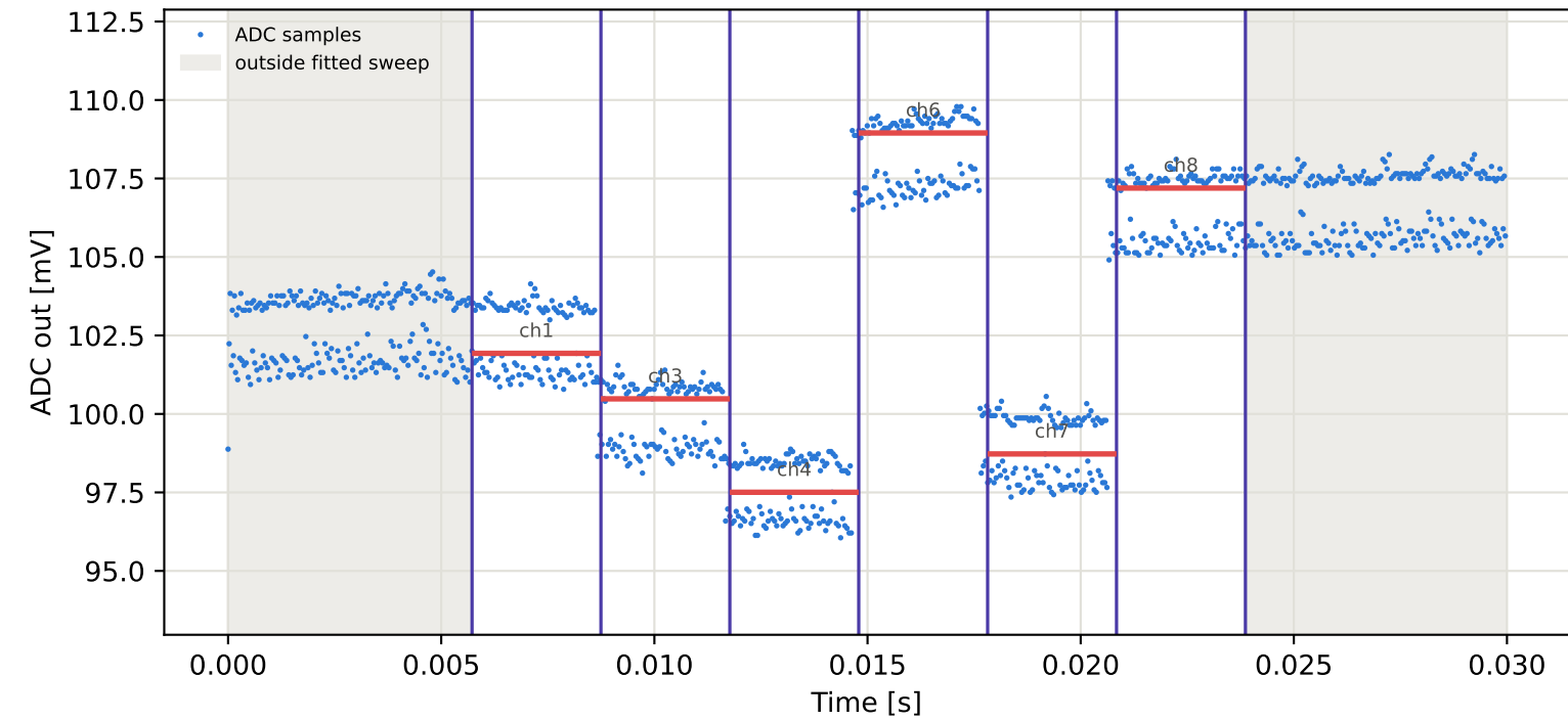
Tag1 &lt;- Tag4 | 945 MHz | run 0 | rep 1 | phase -31.93 deg
