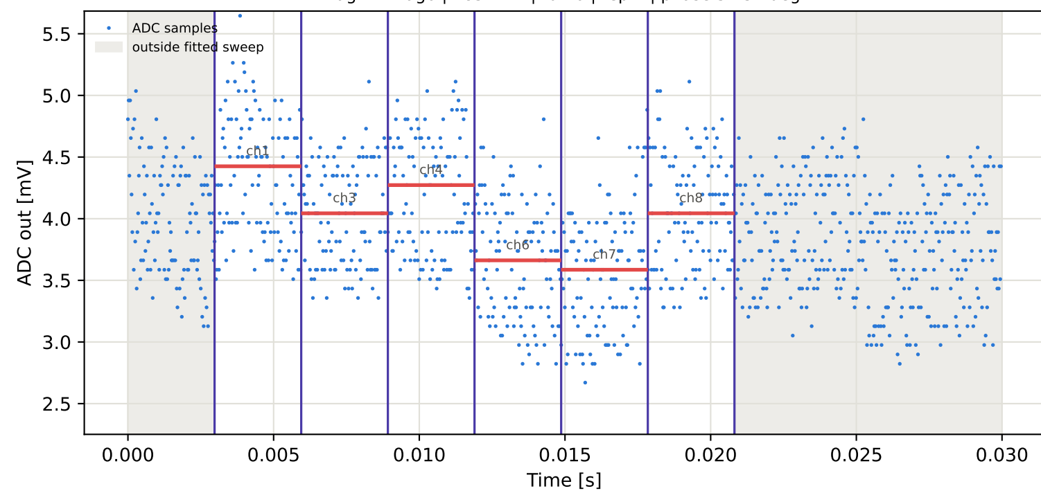
Tag1 &lt;- Tag8 | 785 MHz | run 0 | rep 1 | phase 13.68 deg
