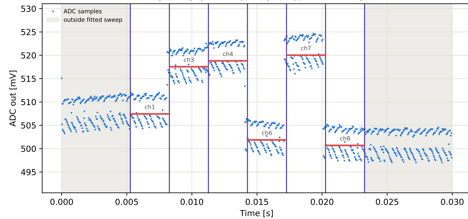
Tag6 &lt;- Tag9 | 855 MHz | run 0 | rep 1 | phase -104.97 deg
