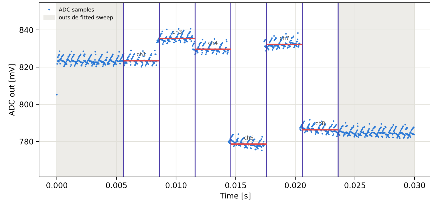
Tag7 &lt;- Tag5 | 895 MHz | run 0 | rep 1 | phase -112.78 deg
