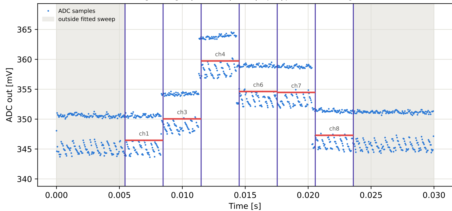
Tag4 &lt;- Tag16 | 955 MHz | run 0 | rep 1 | phase 107.76 deg
