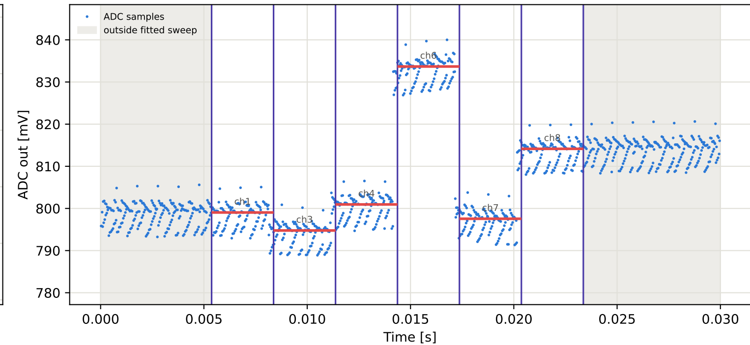
Tag9 &lt;- Tag8 | 925 MHz | run 0 | rep 1 | phase 103.87 deg
