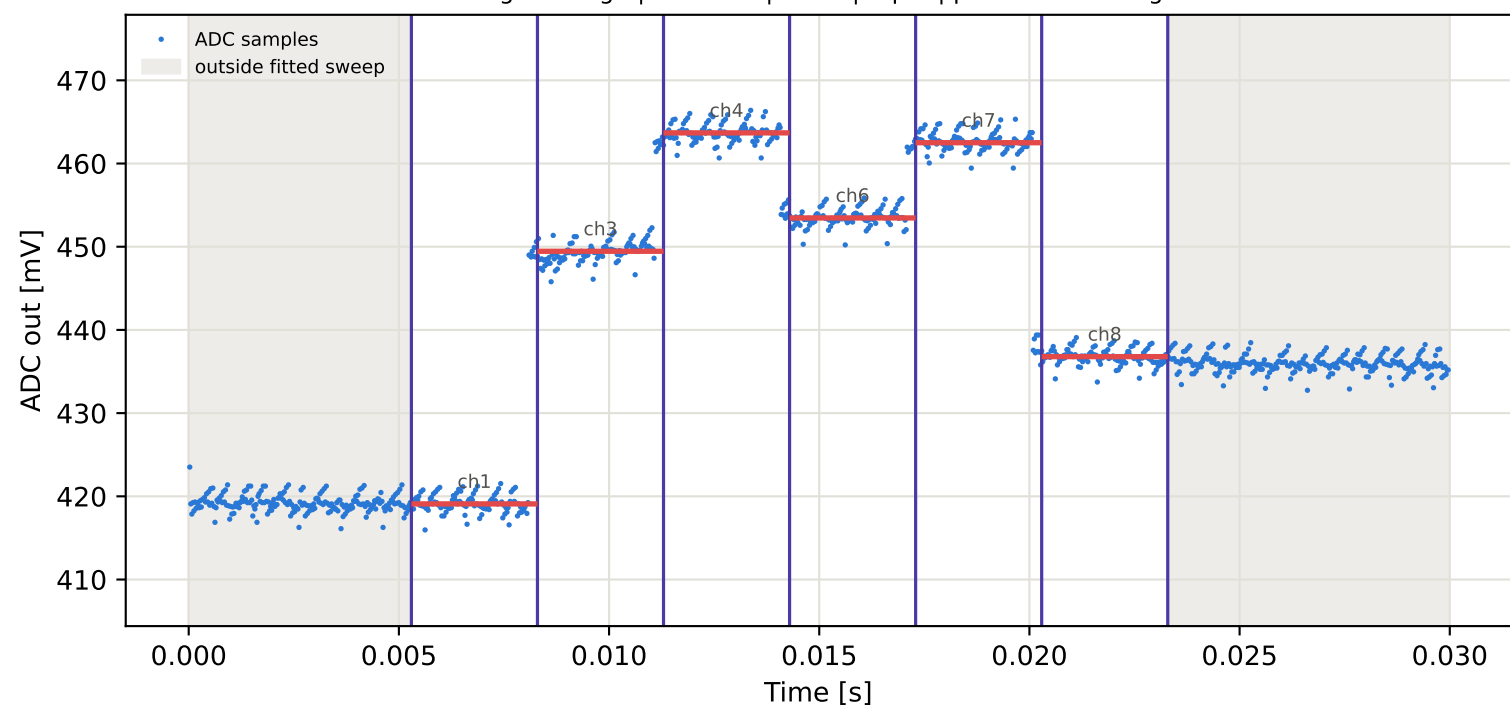
Tag5 &lt;- Tag4 | 845 MHz | run 0 | rep 1 | phase -96.70 deg
