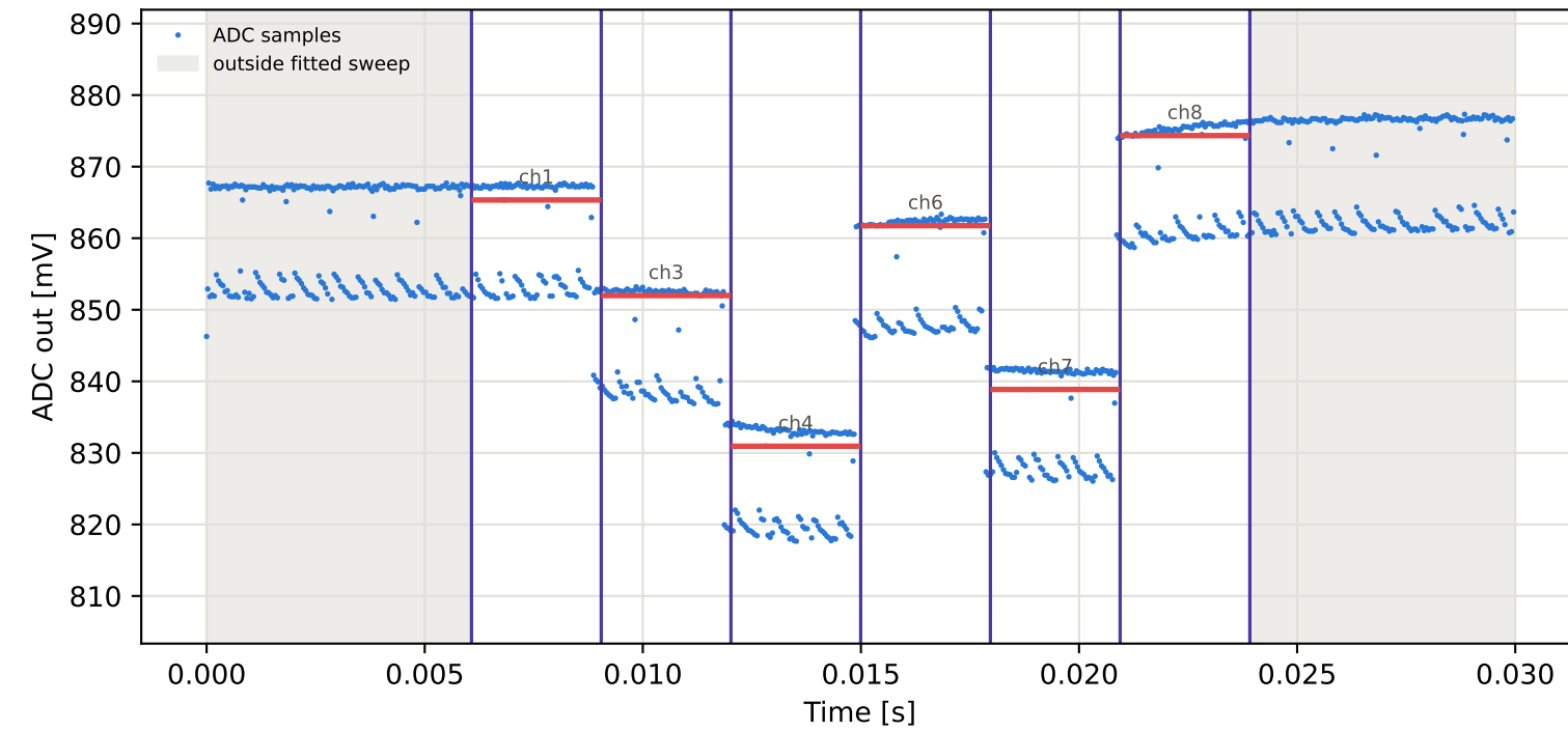
Tag7 &lt;- Tag5 | 935 MHz | run 0 | rep 1 | phase -0.12 deg
