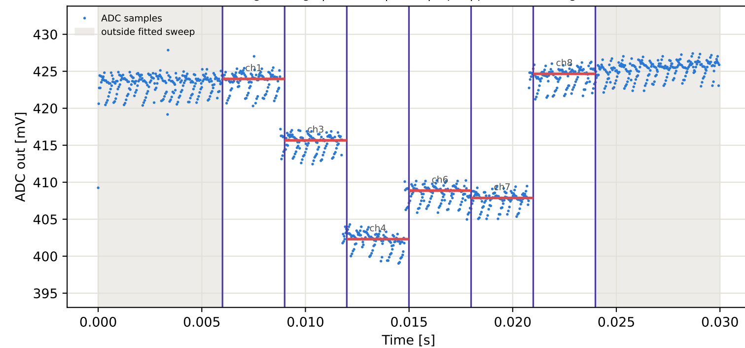
Tag7 &lt;- Tag5 | 925 MHz | run 0 | rep 1 | phase -50.02 deg
