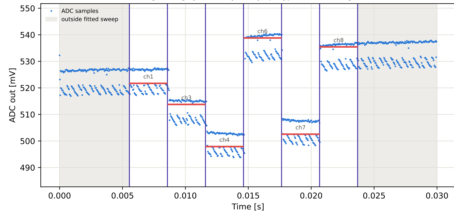
Tag5 &lt;- Tag8 | 975 MHz | run 0 | rep 1 | phase -53.18 deg
