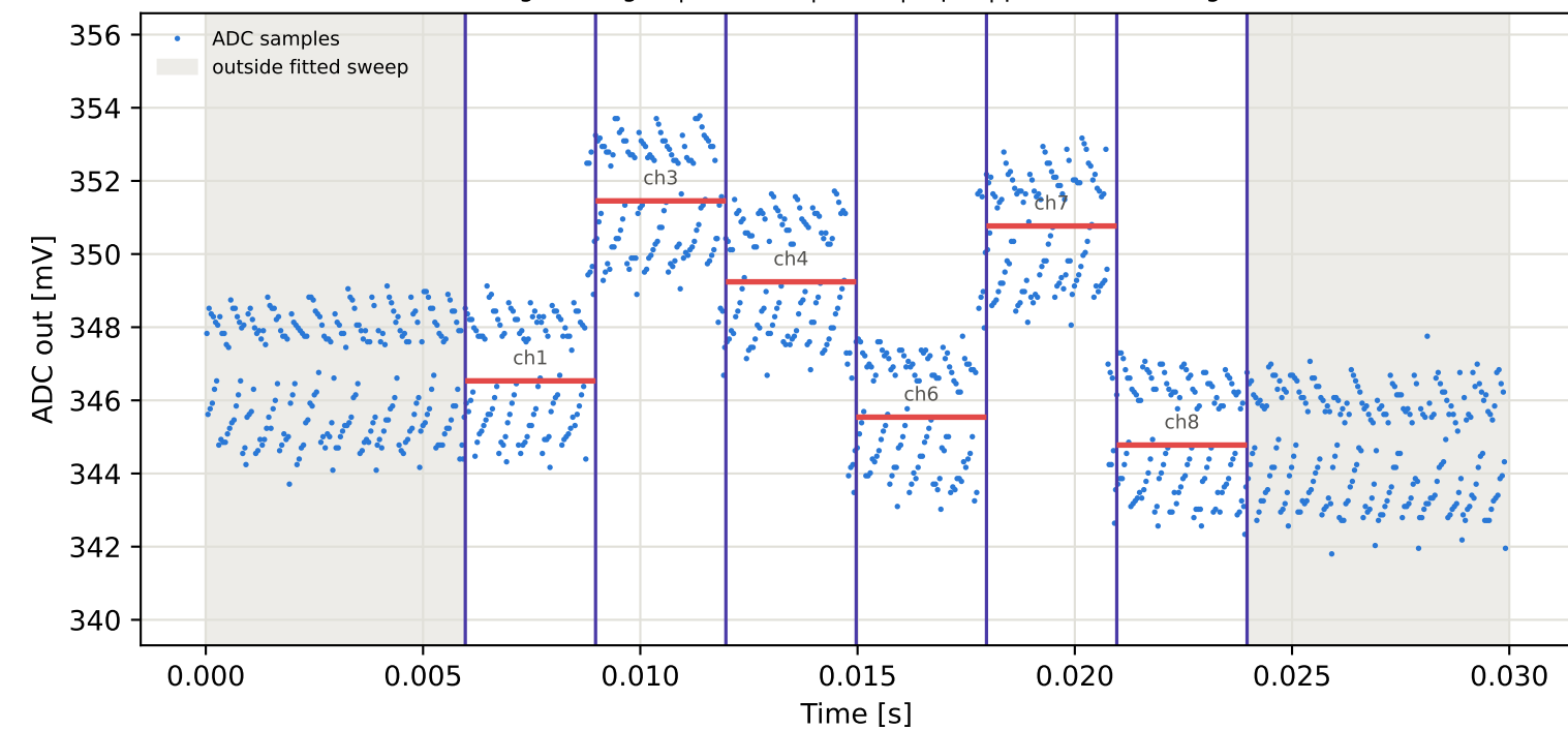
Tag7 &lt;- Tag10 | 825 MHz | run 0 | rep 1 | phase -16.30 deg
