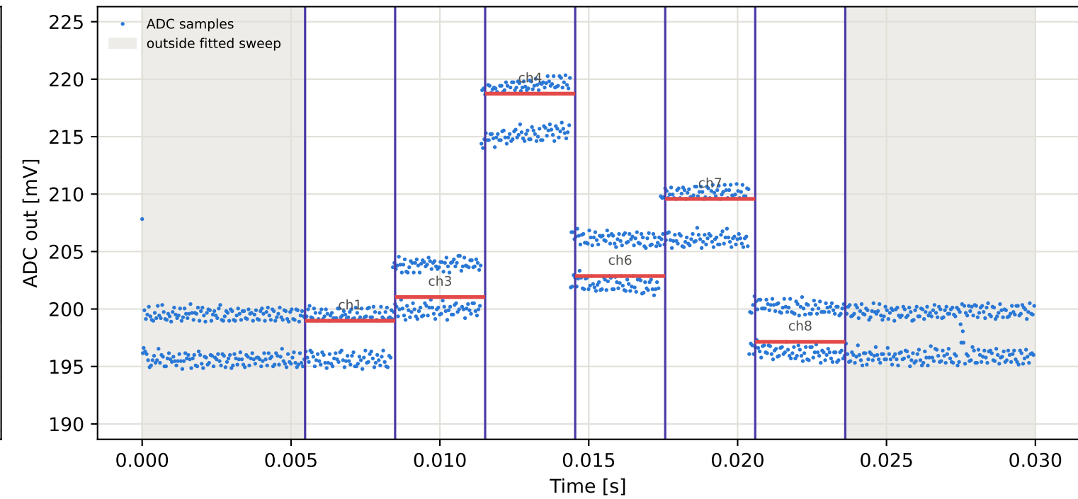
Tag10 &lt;- Tag5 | 985 MHz | run 0 | rep 1 | phase -50.87 deg
