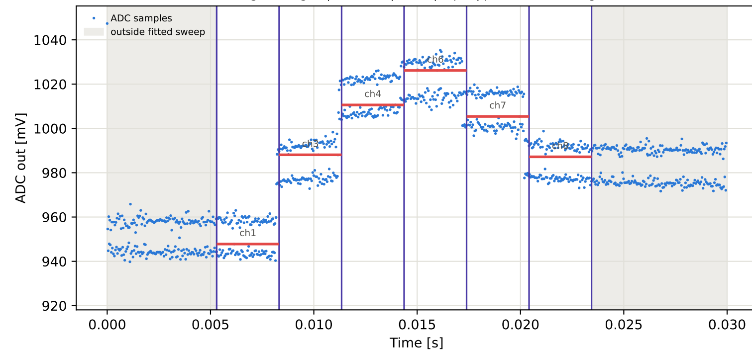
Tag6 &lt;- Tag2 | 885 MHz | run 0 | rep 1 | phase -145.07 deg
