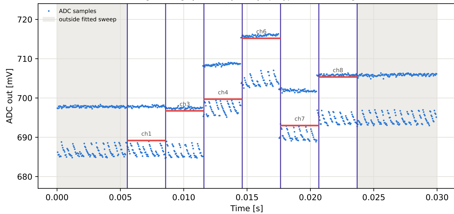
Tag2 &lt;- Tag10 | 975 MHz | run 0 | rep 1 | phase -160.24 deg
