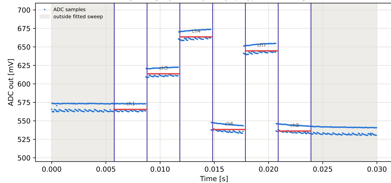
Tag7 &lt;- Tag3 | 985 MHz | run 0 | rep 1 | phase 160.45 deg
