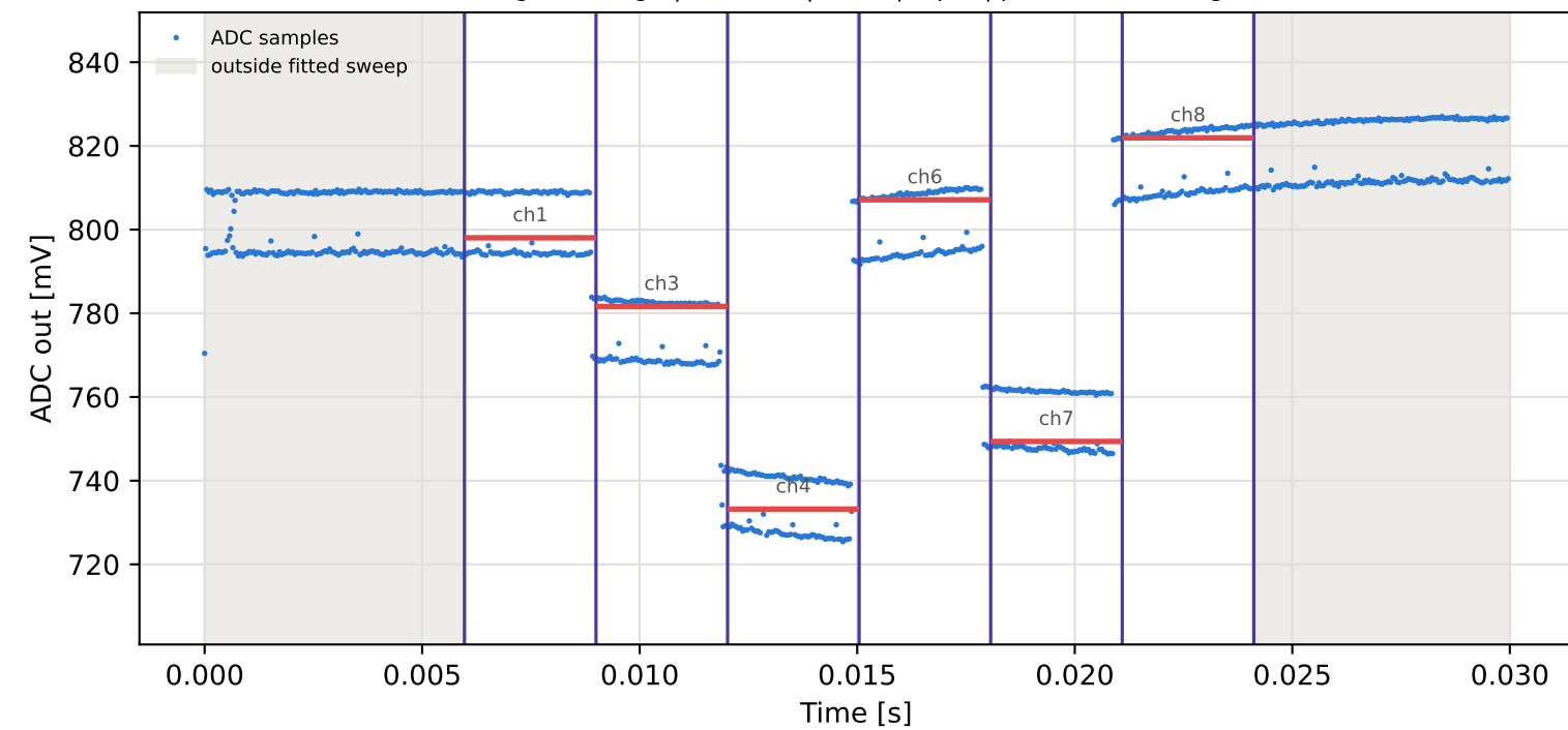
Tag16 &lt;- Tag1 | 945 MHz | run 0 | rep 1 | phase 58.67 deg
