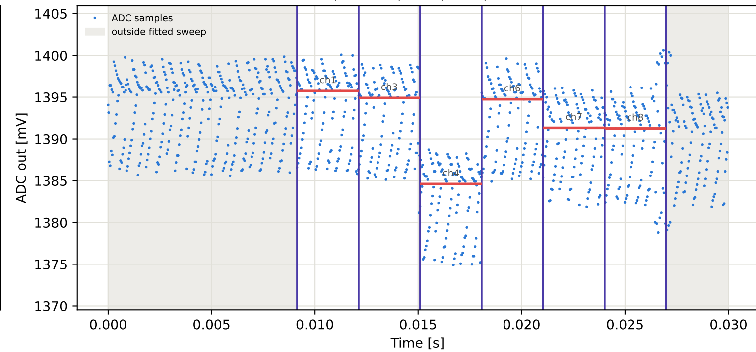
Tag15 &lt;- Tag4 | 915 MHz | run 0 | rep 1 | phase -153.21 deg
