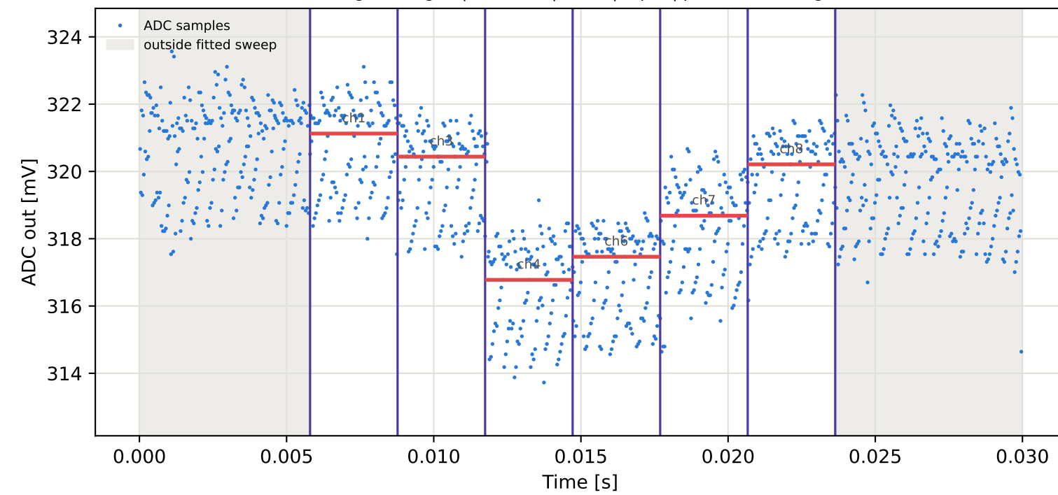
Tag6 &lt;- Tag2 | 975 MHz | run 0 | rep 1 | phase -106.14 deg
