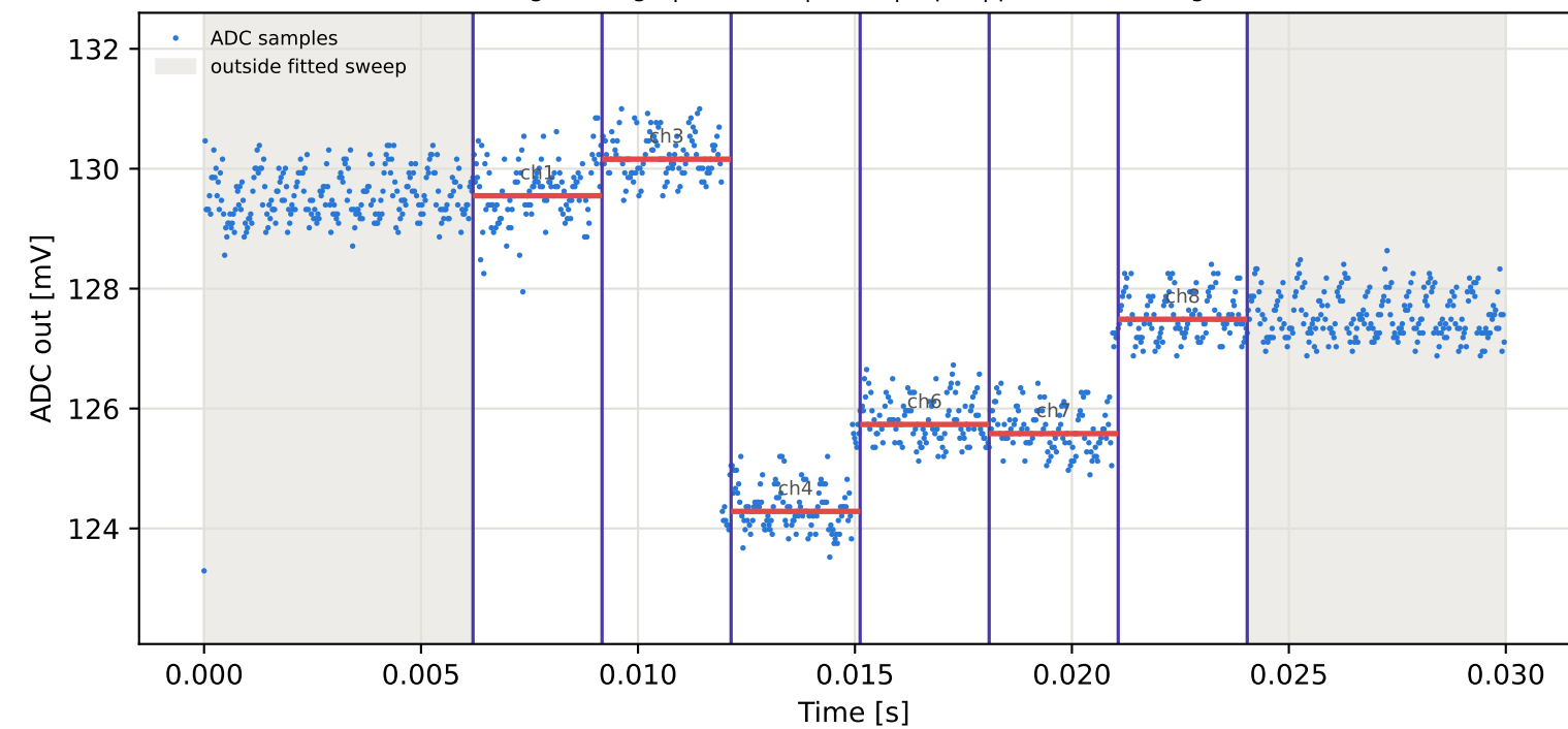
Tag5 &lt;- Tag1 | 795 MHz | run 0 | rep 1 | phase -37.27 deg
