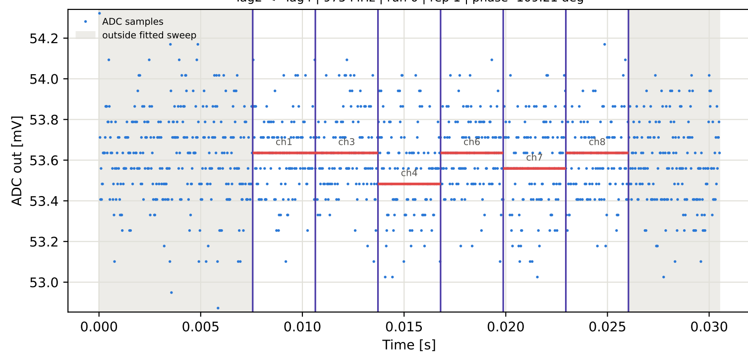
Tag2 &lt;- Tag6 | 975 MHz | run 0 | rep 1 | phase -106.31 deg
