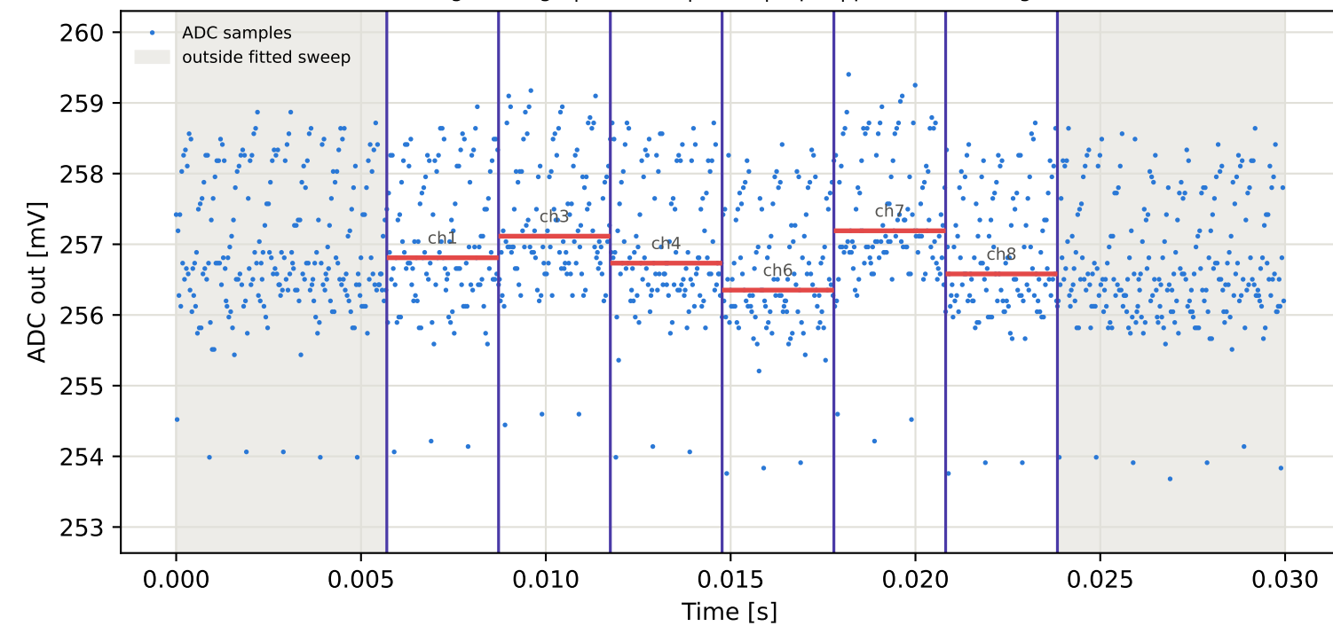
Tag8 &lt;- Tag6 | 785 MHz | run 0 | rep 1 | phase -142.50 deg
