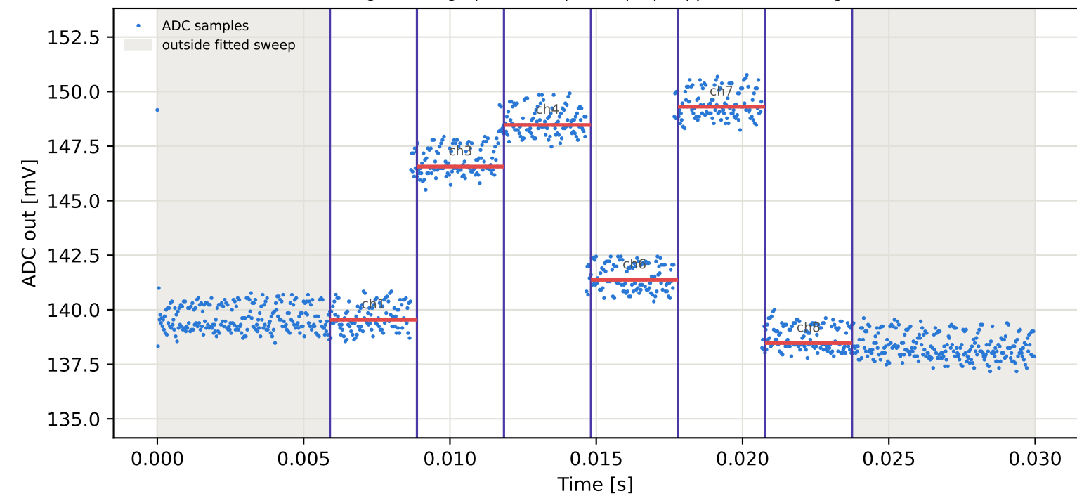
Tag15 &lt;- Tag9 | 805 MHz | run 0 | rep 1 | phase -58.54 deg
