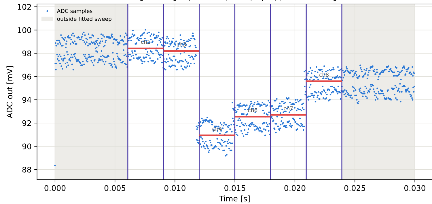
Tag10 &lt;- Tag2 | 825 MHz | run 0 | rep 1 | phase 108.88 deg
