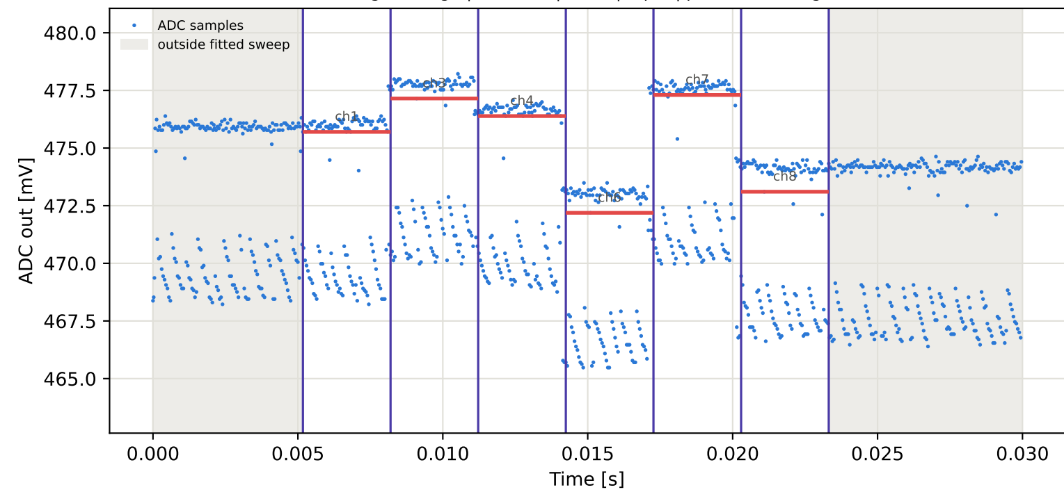
Tag7 &lt;- Tag4 | 835 MHz | run 0 | rep 1 | phase 69.12 deg
