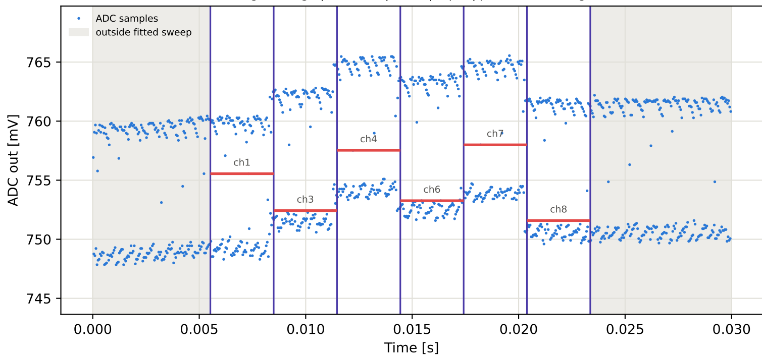
Tag9 &lt;- Tag10 | 835 MHz | run 0 | rep 1 | phase 162.33 deg
