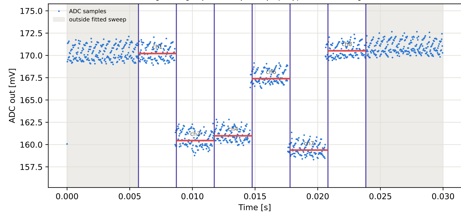
Tag2 &lt;- Tag16 | 845 MHz | run 0 | rep 1 | phase 127.52 deg
