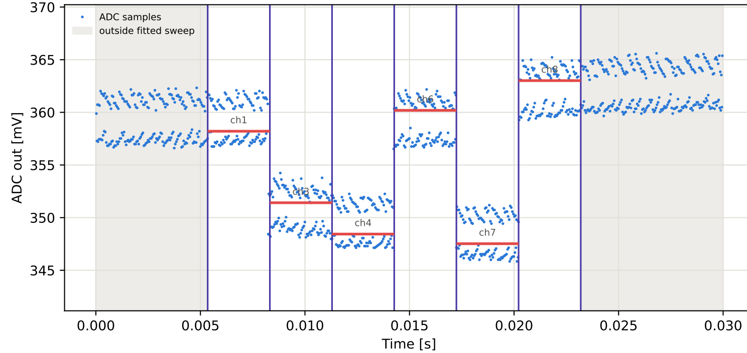
Tag16 &lt;- Tag10 | 855 MHz | run 0 | rep 1 | phase -79.27 deg
