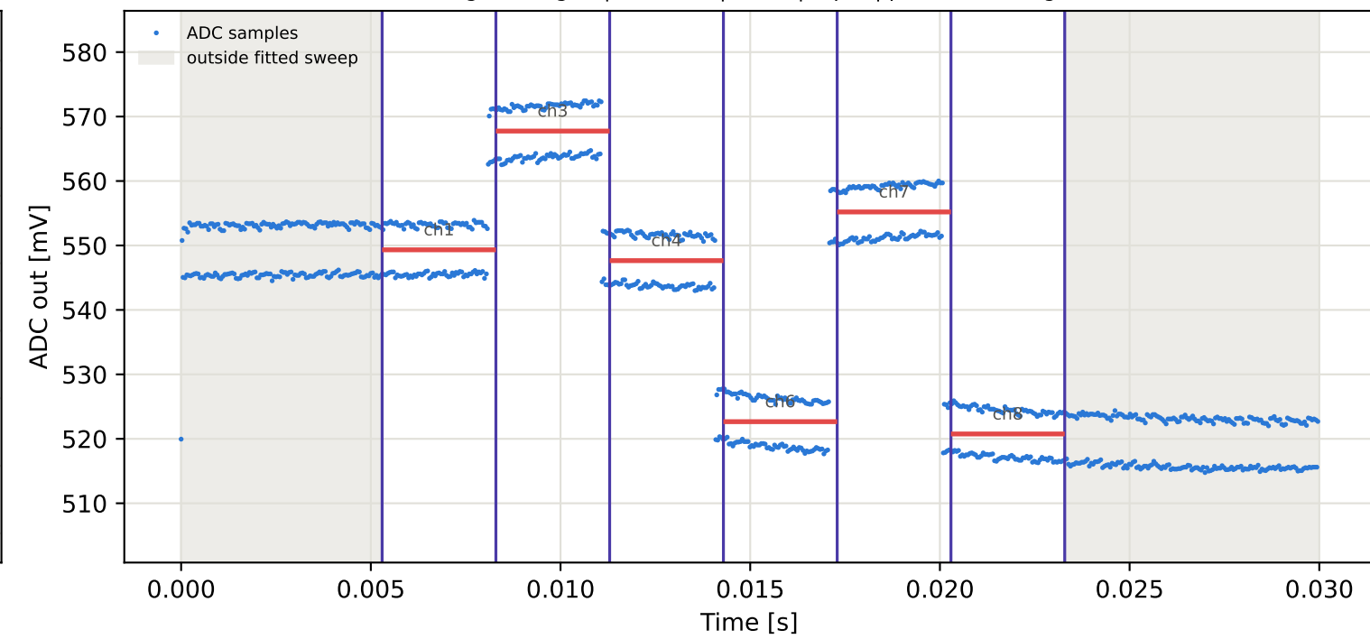
Tag5 &lt;- Tag2 | 865 MHz | run 0 | rep 1 | phase -133.48 deg
