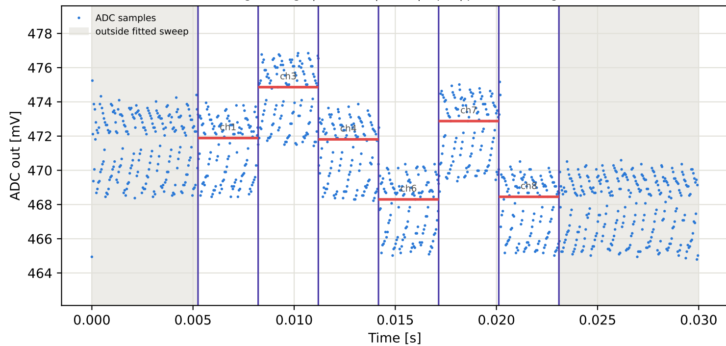
Tag4 &lt;- Tag15 | 855 MHz | run 0 | rep 1 | phase -119.18 deg
