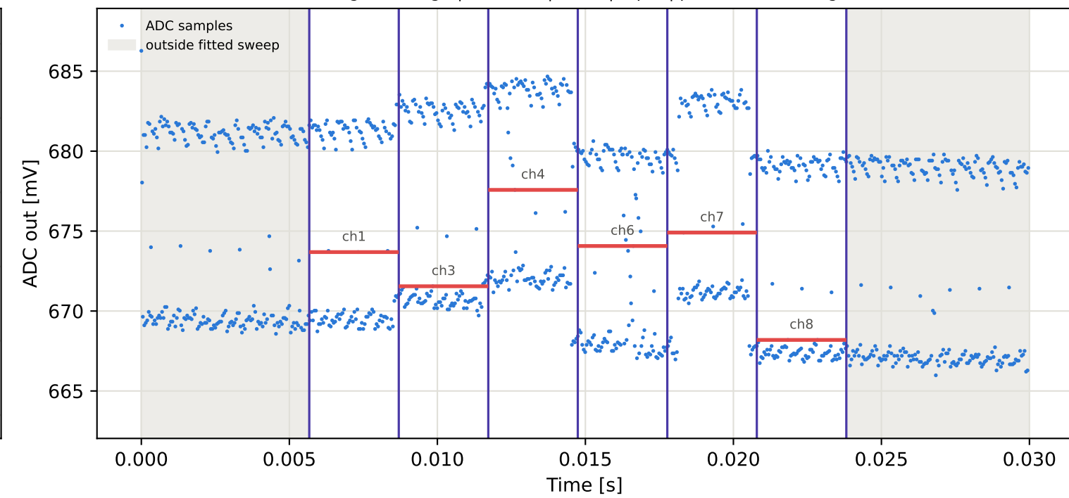
Tag15 &lt;- Tag4 | 935 MHz | run 0 | rep 1 | phase -141.42 deg
