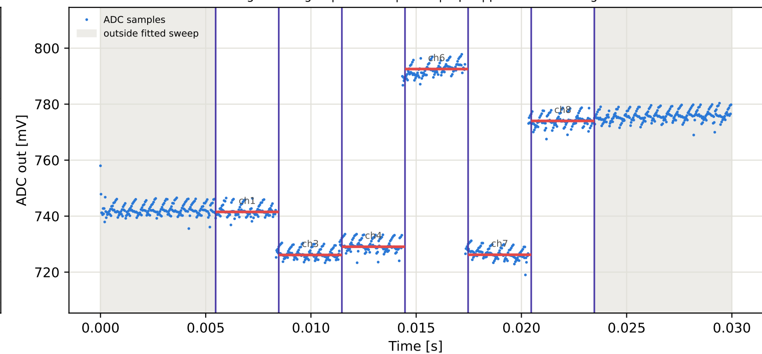
Tag16 &lt;- Tag15 | 935 MHz | run 0 | rep 1 | phase 170.32 deg
