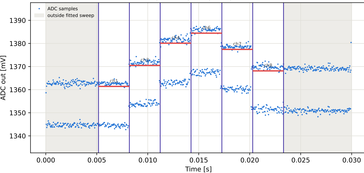
Tag16 &lt;- Tag10 | 885 MHz | run 0 | rep 1 | phase -122.53 deg
