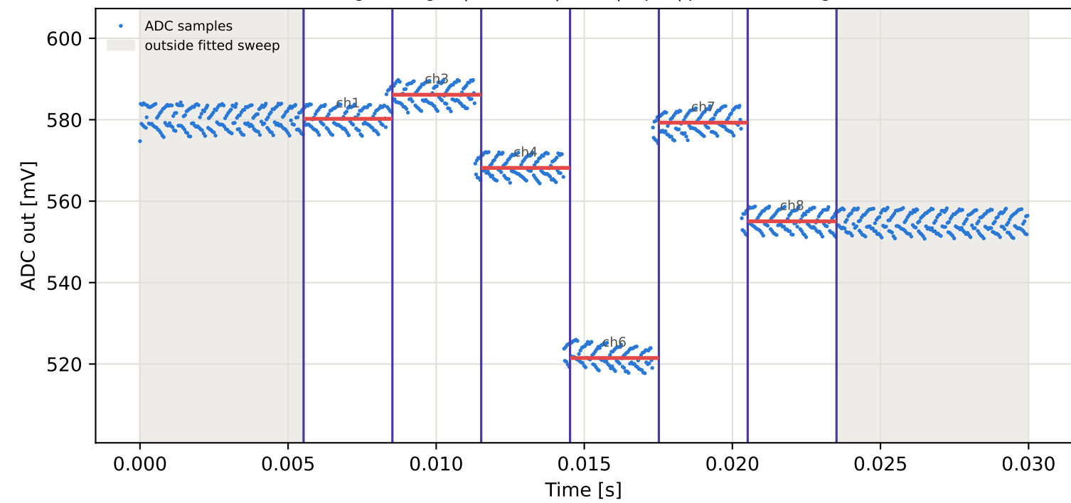
Tag5 &lt;- Tag2 | 955 MHz | run 0 | rep 1 | phase -175.43 deg
