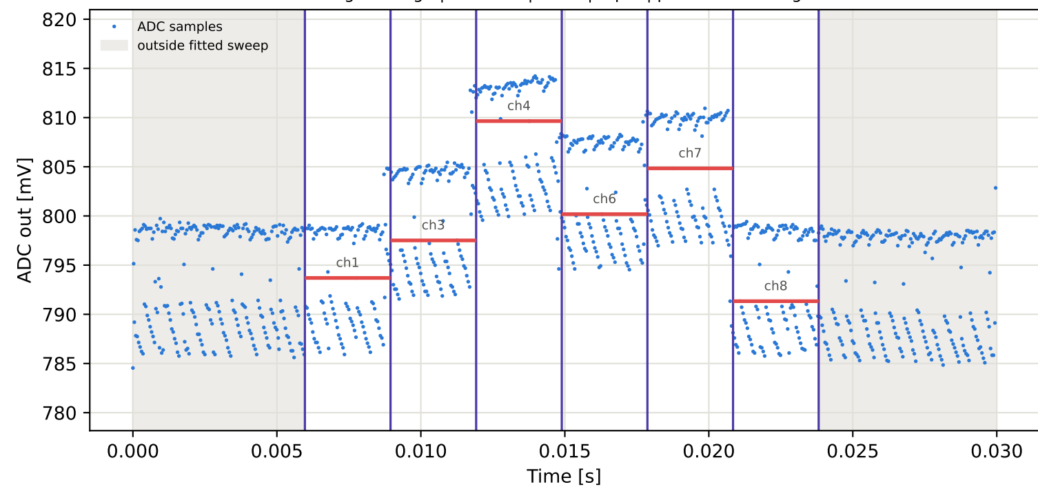
Tag9 &lt;- Tag15 | 925 MHz | run 0 | rep 1 | phase -76.07 deg
