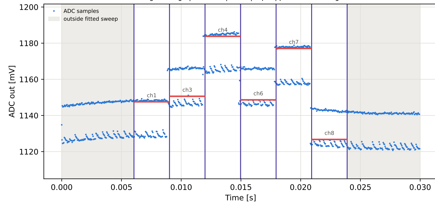
Tag9 &lt;- Tag10 | 925 MHz | run 0 | rep 1 | phase -124.12 deg
