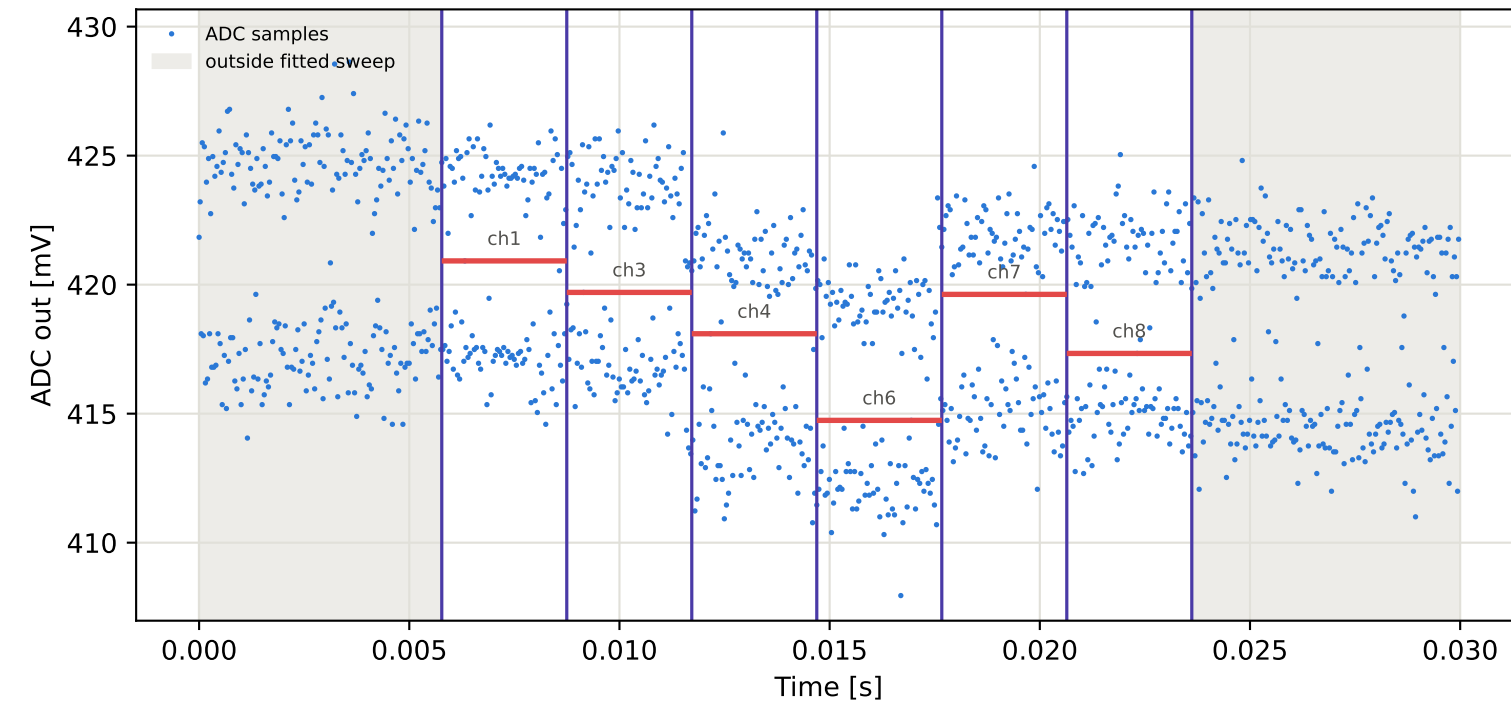
Tag1 &lt;- Tag9 | 885 MHz | run 0 | rep 1 | phase -173.35 deg
