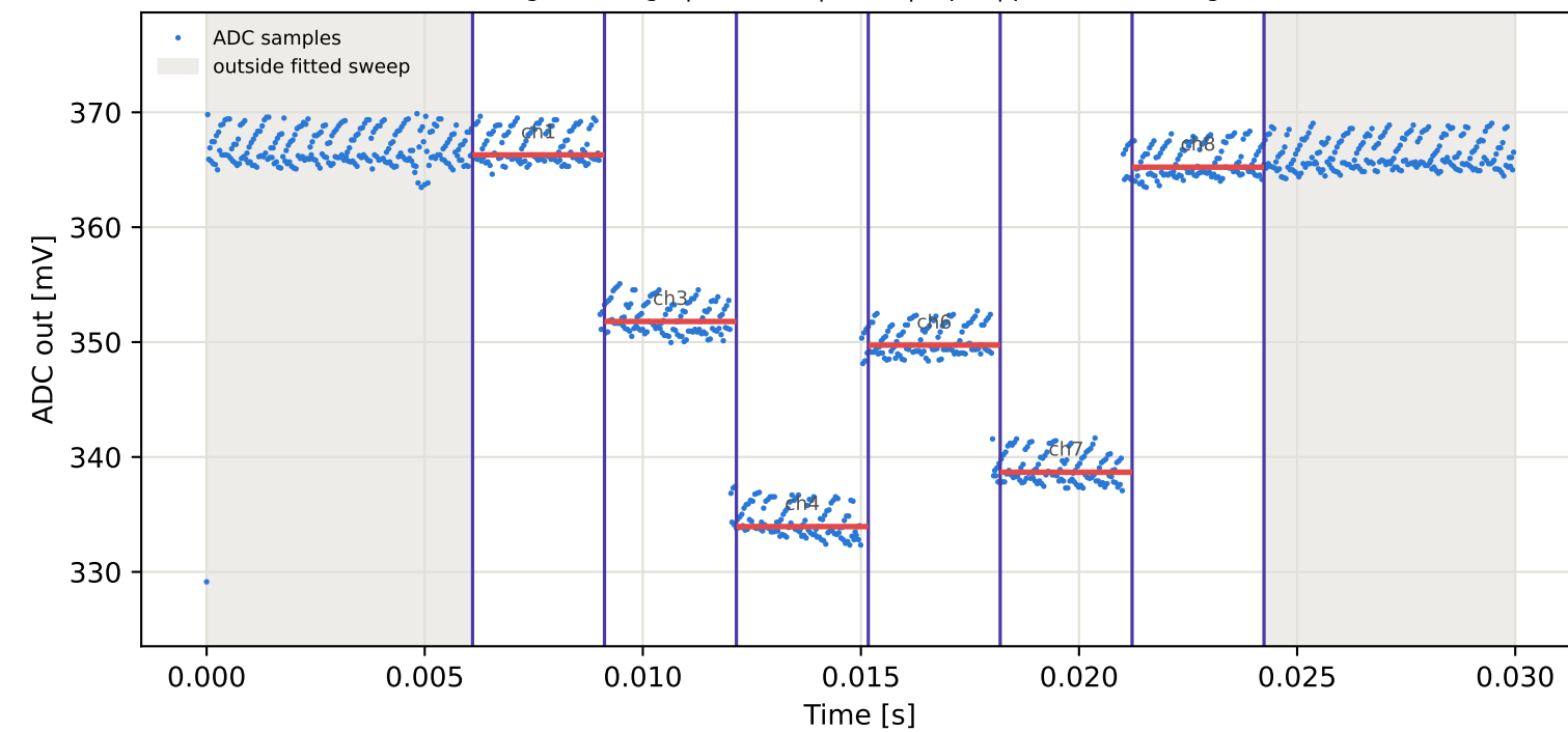
Tag15 &lt;- Tag9 | 845 MHz | run 0 | rep 1 | phase 81.11 deg
