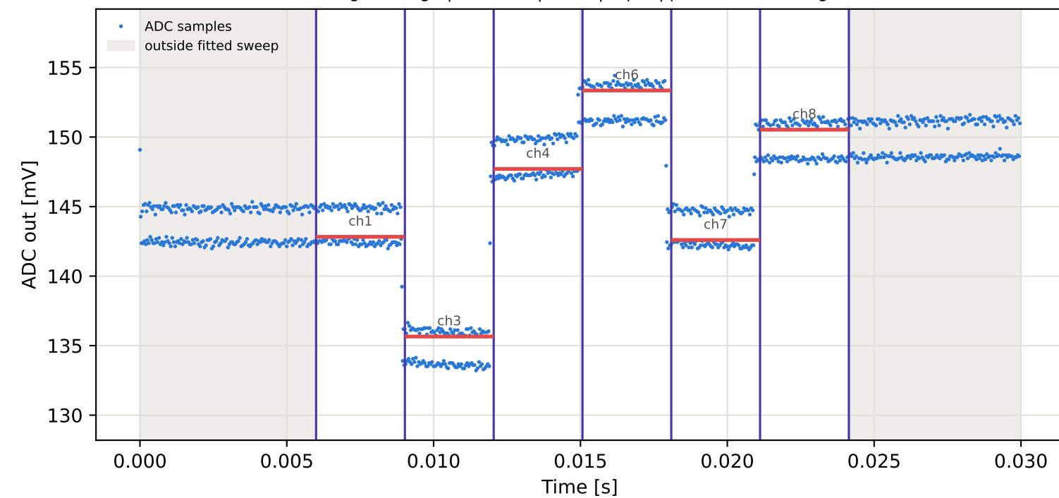
Tag3 &lt;- Tag8 | 805 MHz | run 0 | rep 1 | phase -149.94 deg
