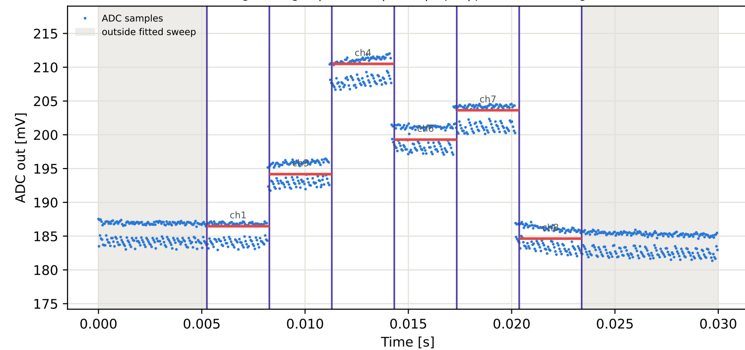
Tag1 &lt;- Tag3 | 935 MHz | run 0 | rep 1 | phase -85.28 deg
