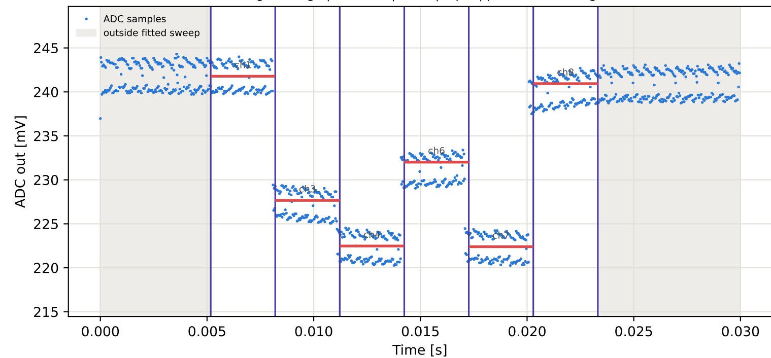
Tag2 &lt;- Tag8 | 855 MHz | run 0 | rep 1 | phase 101.34 deg
