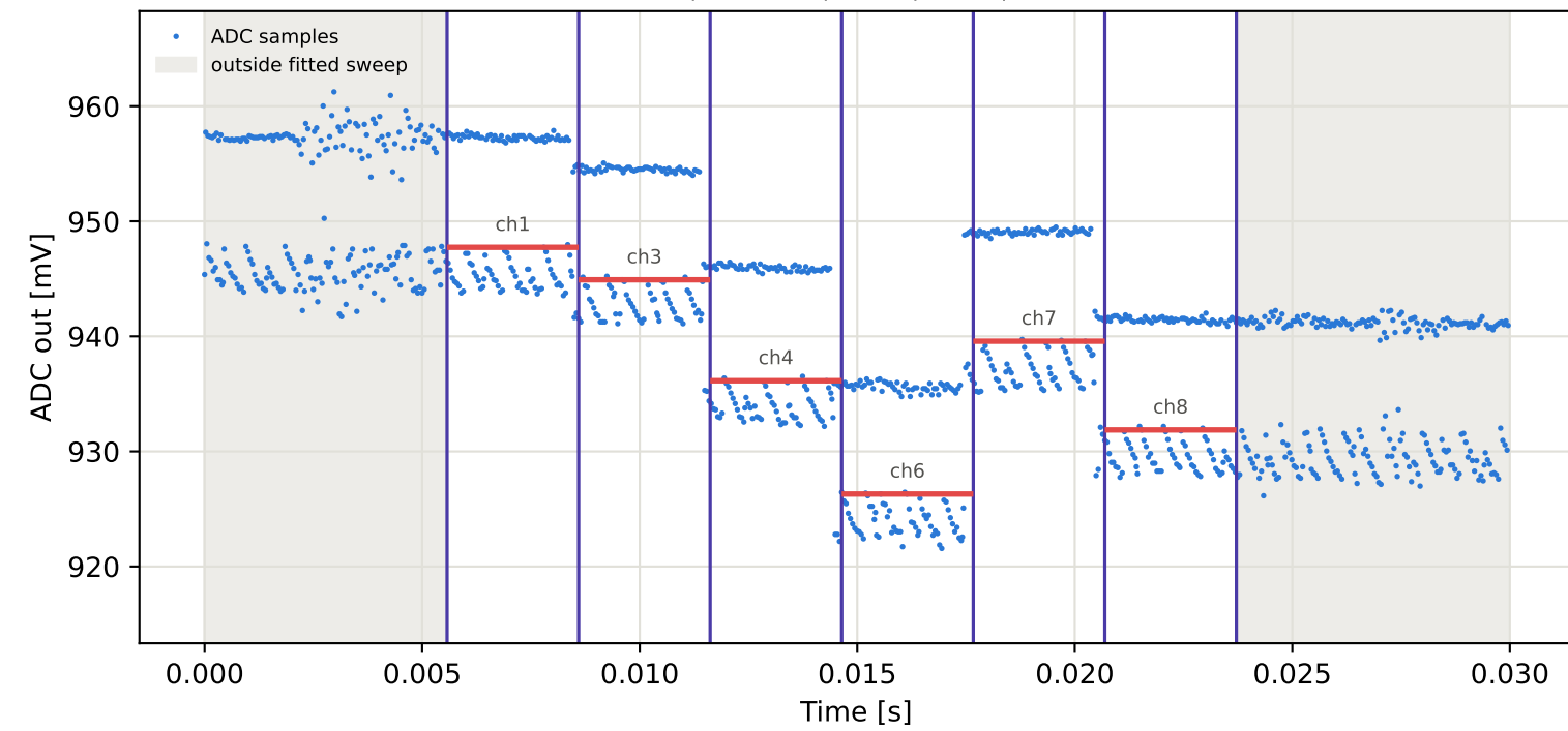
Tag15 &lt;- Tag10 | 875 MHz | run 0 | rep 1 | phase 31.62 deg
