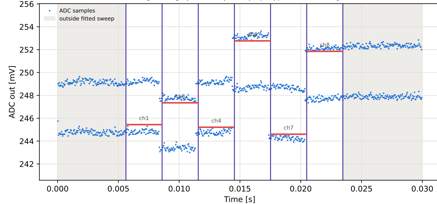
Tag1 &lt;- Tag9 | 865 MHz | run 0 | rep 1 | phase 159.99 deg
