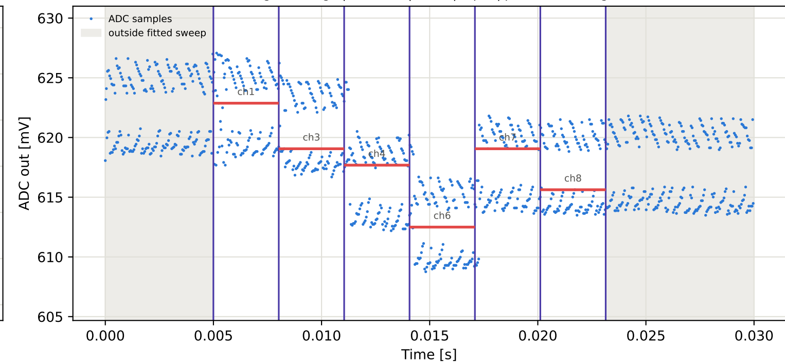
Tag15 &lt;- Tag4 | 865 MHz | run 0 | rep 1 | phase 85.22 deg
