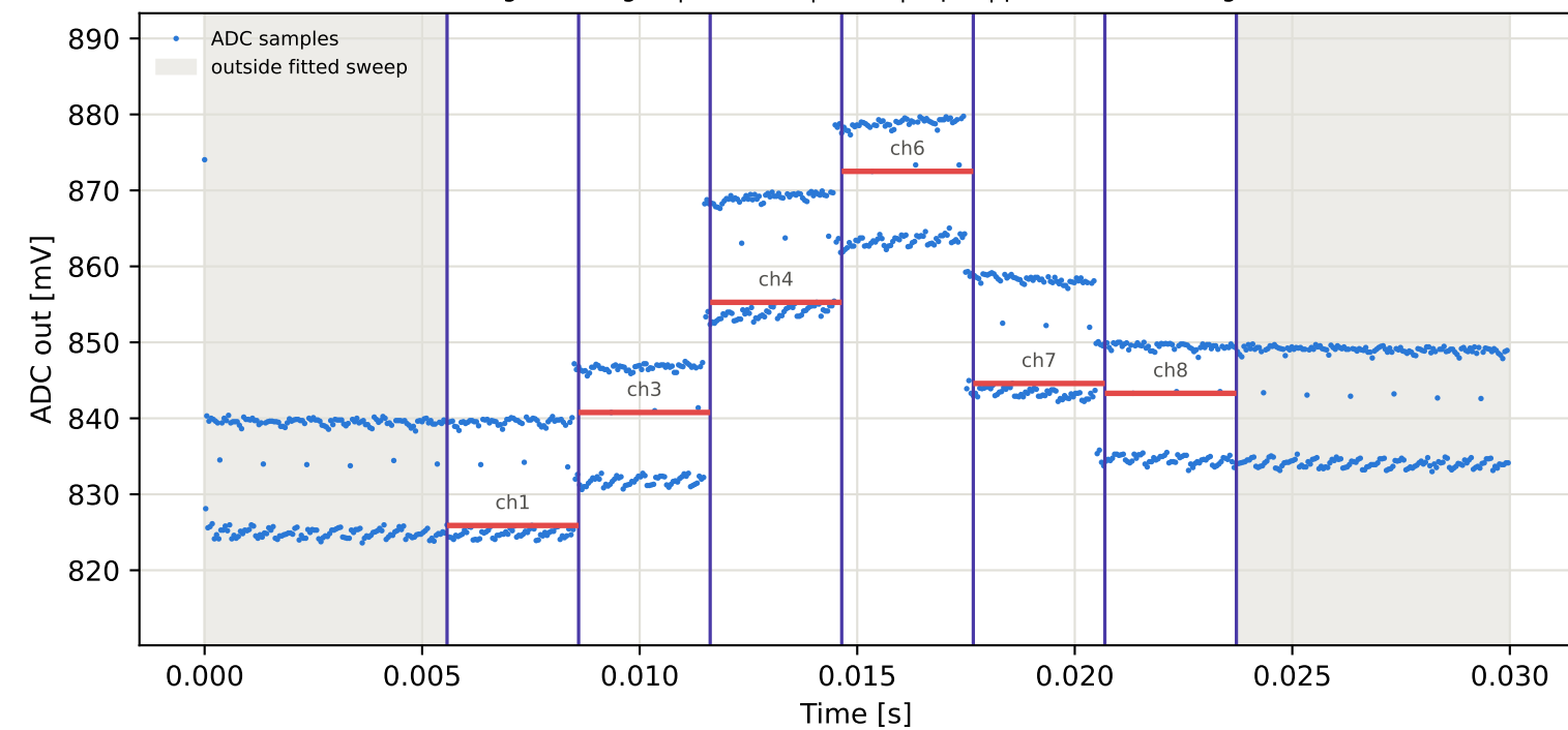
Tag16 &lt;- Tag15 | 945 MHz | run 0 | rep 1 | phase -142.03 deg
