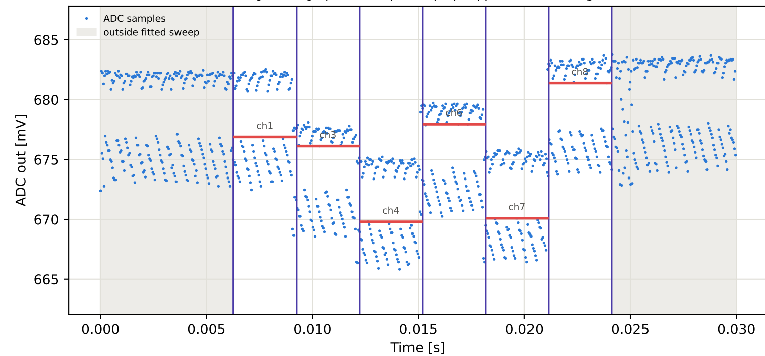
Tag8 &lt;- Tag4 | 855 MHz | run 0 | rep 1 | phase 72.55 deg
