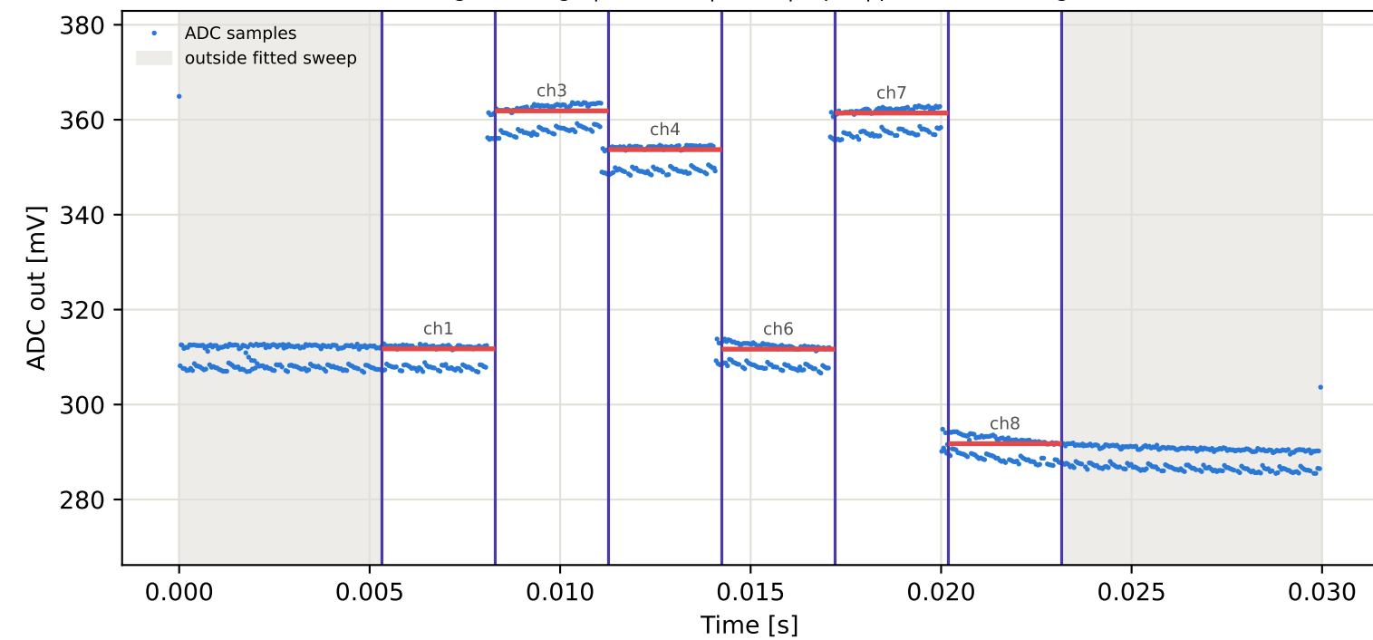
Tag16 &lt;- Tag1 | 845 MHz | run 0 | rep 1 | phase 94.44 deg
