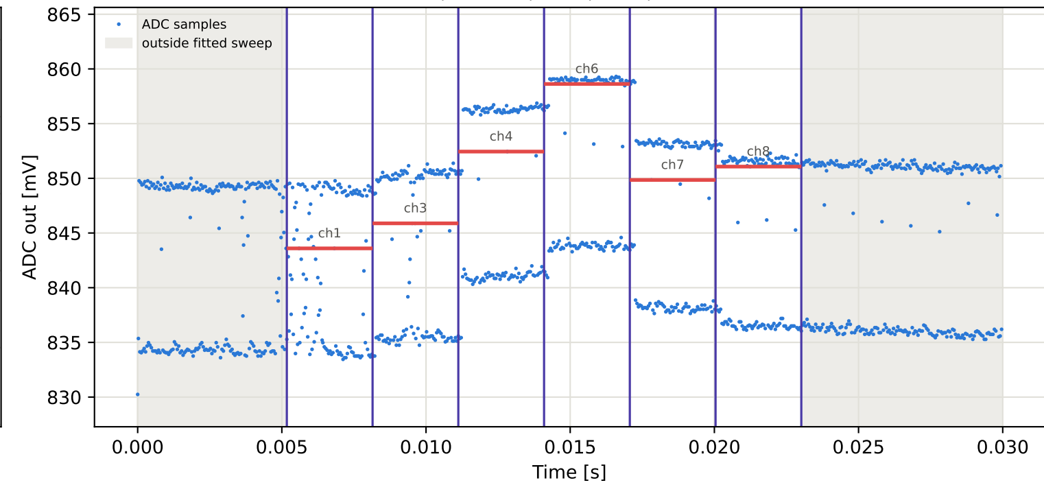
Tag7 &lt;- Tag6 | 935 MHz | run 0 | rep 1 | phase -147.53 deg
