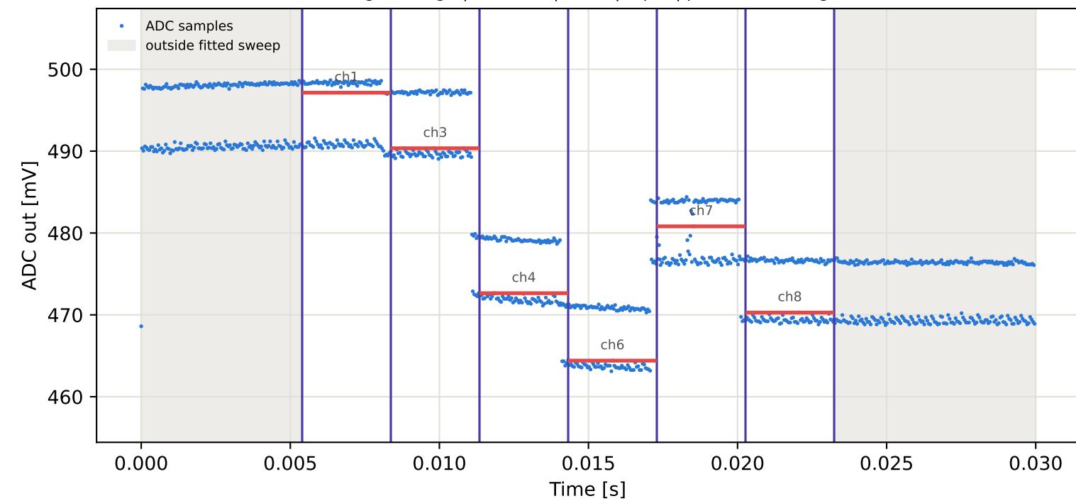
Tag3 &lt;- Tag6 | 845 MHz | run 0 | rep 1 | phase 103.34 deg
