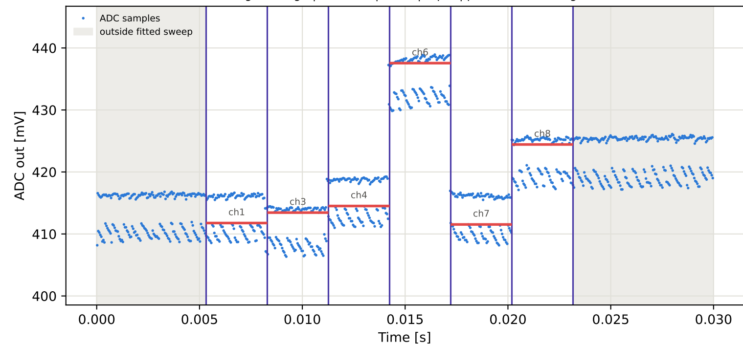
Tag7 &lt;- Tag6 | 925 MHz | run 0 | rep 1 | phase -175.84 deg
