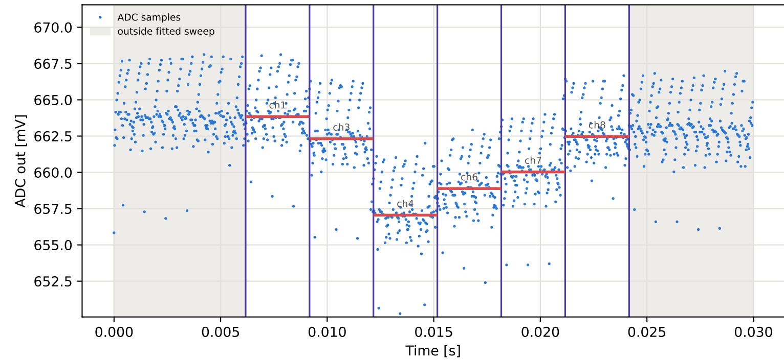
Tag16 &lt;- Tag15 | 965 MHz | run 0 | rep 1 | phase -58.25 deg
