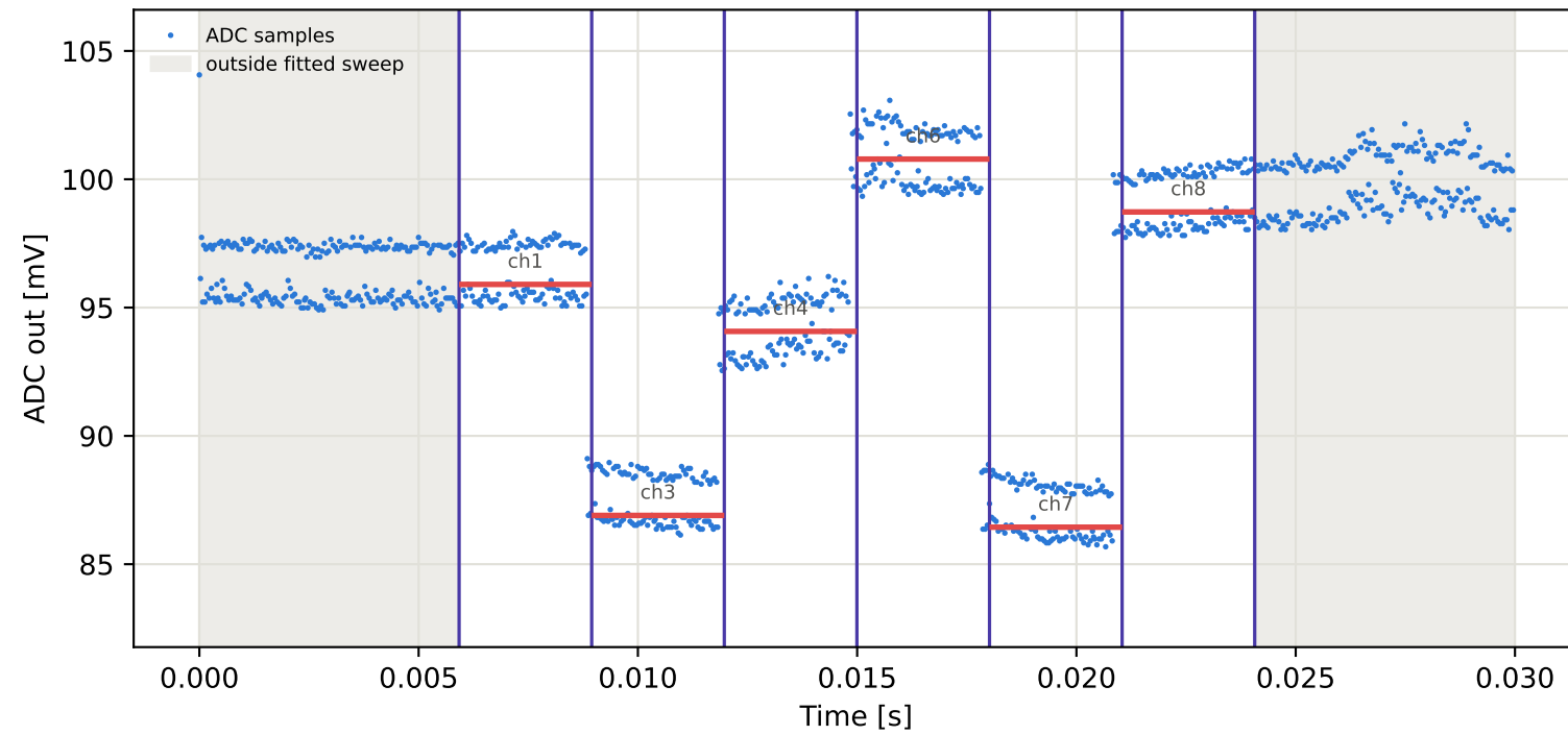
Tag6 &lt;- Tag1 | 775 MHz | run 0 | rep 1 | phase -44.66 deg
