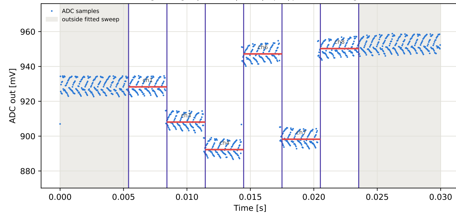
Tag5 &lt;- Tag16 | 925 MHz | run 0 | rep 1 | phase 80.94 deg
