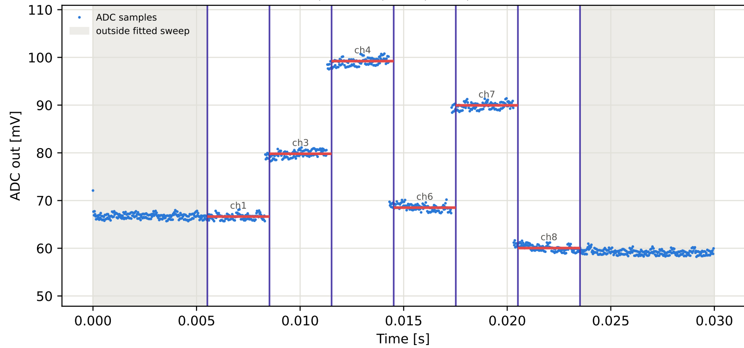
Tag6 &lt;- Tag10 | 955 MHz | run 0 | rep 1 | phase -78.40 deg
