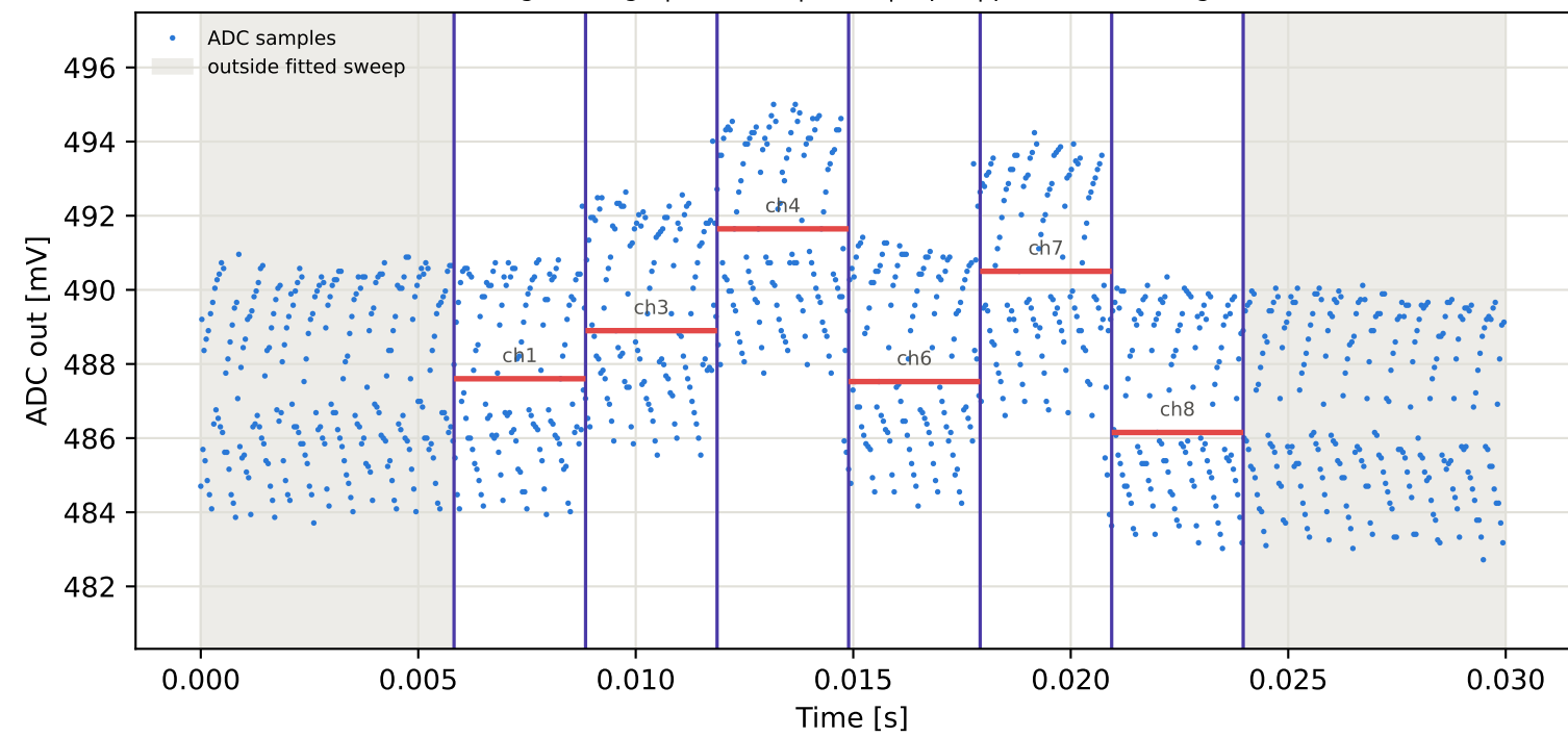
Tag9 &lt;- Tag15 | 955 MHz | run 0 | rep 1 | phase -45.73 deg
