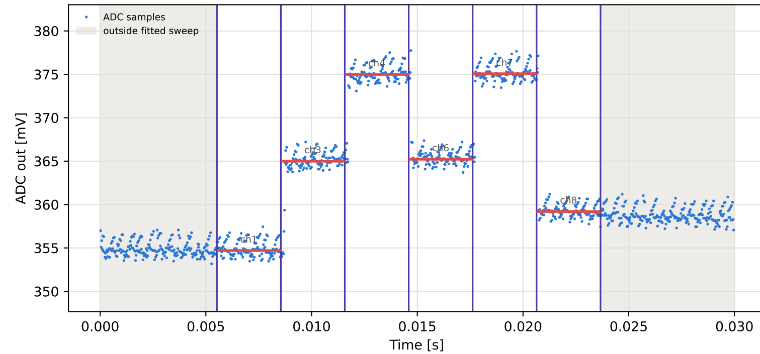
Tag5 &lt;- Tag3 | 825 MHz | run 0 | rep 1 | phase -84.94 deg
