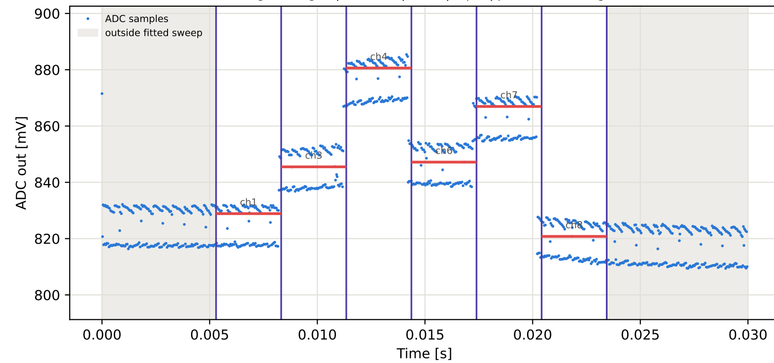
Tag7 &lt;- Tag3 | 935 MHz | run 0 | rep 1 | phase 98.98 deg
