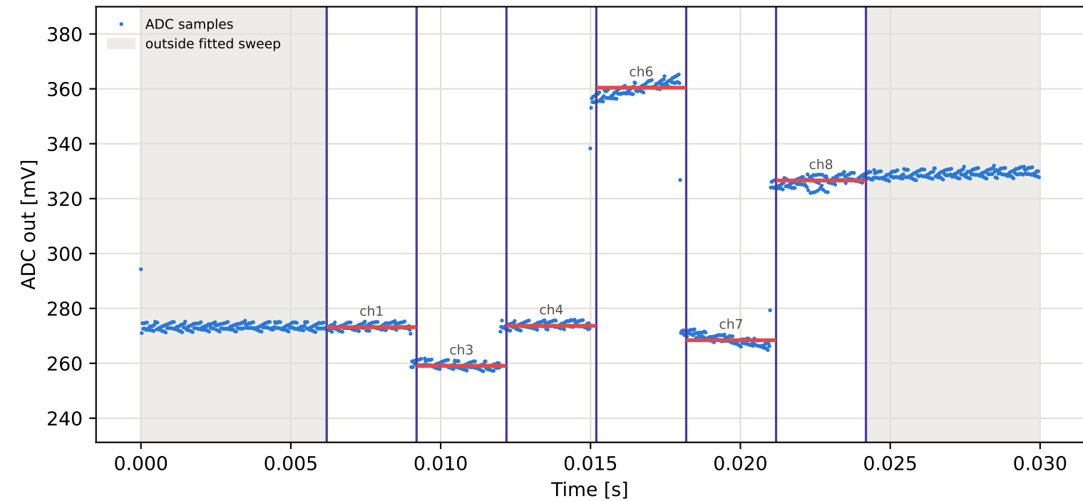
Tag10 &lt;- Tag5 | 905 MHz | run 0 | rep 1 | phase 154.04 deg
