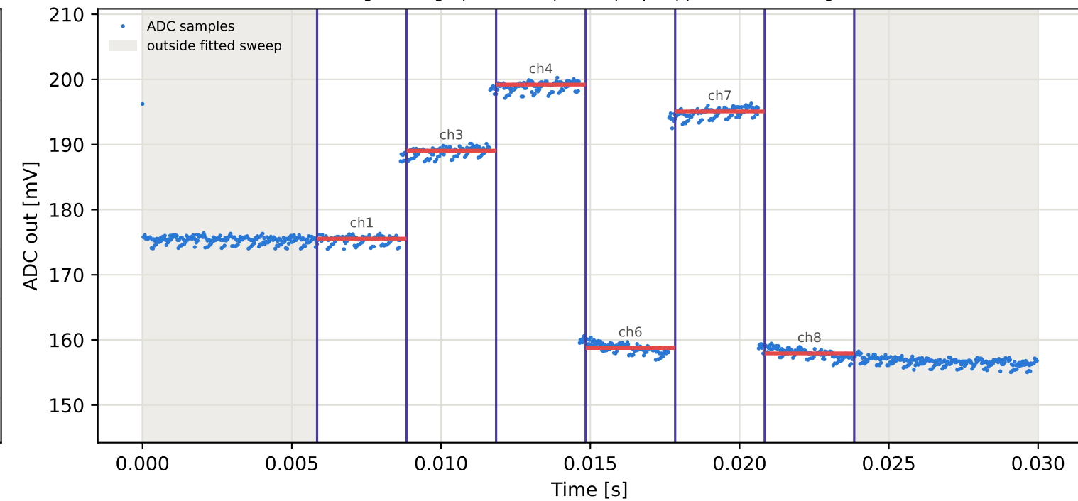
Tag5 &lt;- Tag1 | 925 MHz | run 0 | rep 1 | phase -154.19 deg
