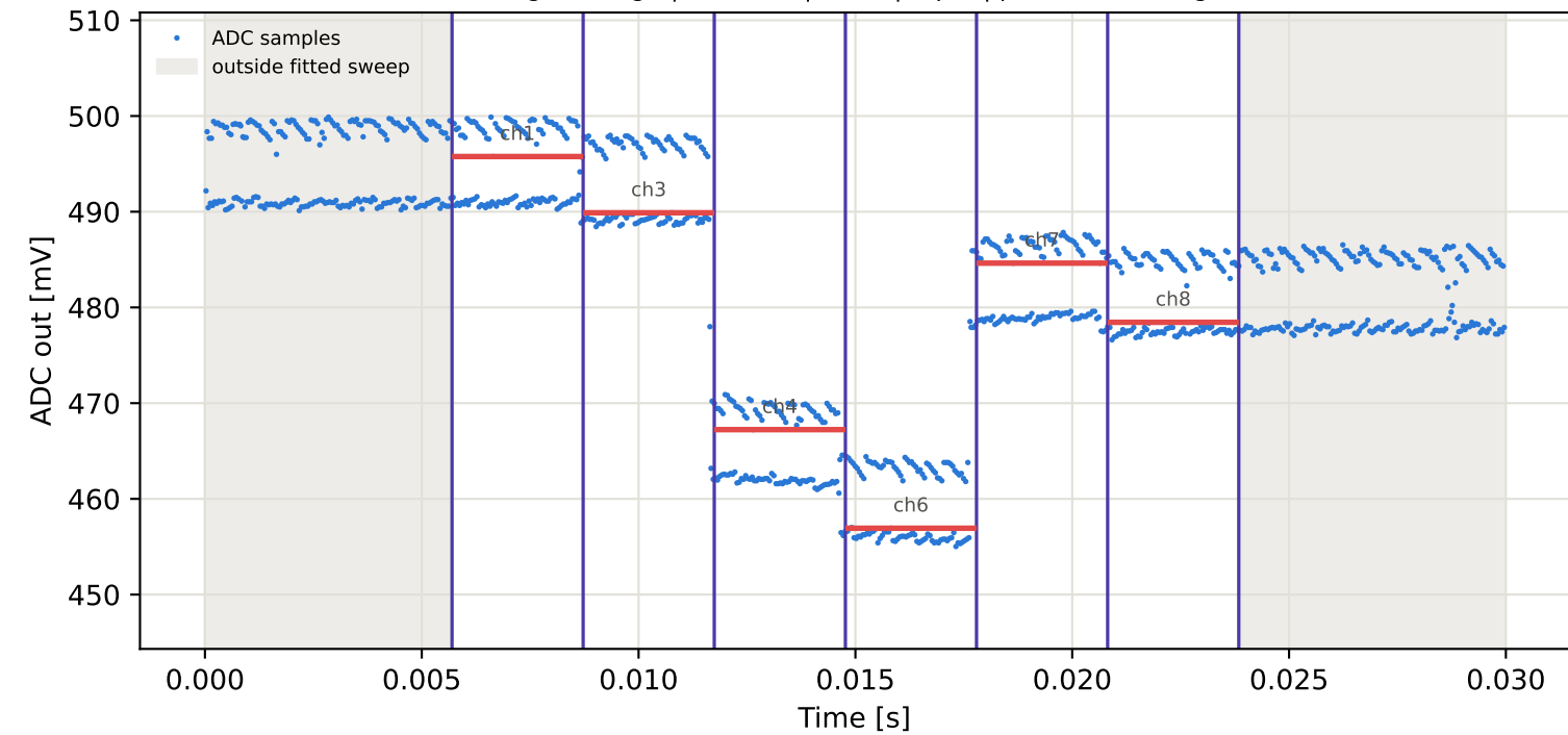
Tag8 &lt;- Tag10 | 995 MHz | run 0 | rep 1 | phase 121.57 deg
