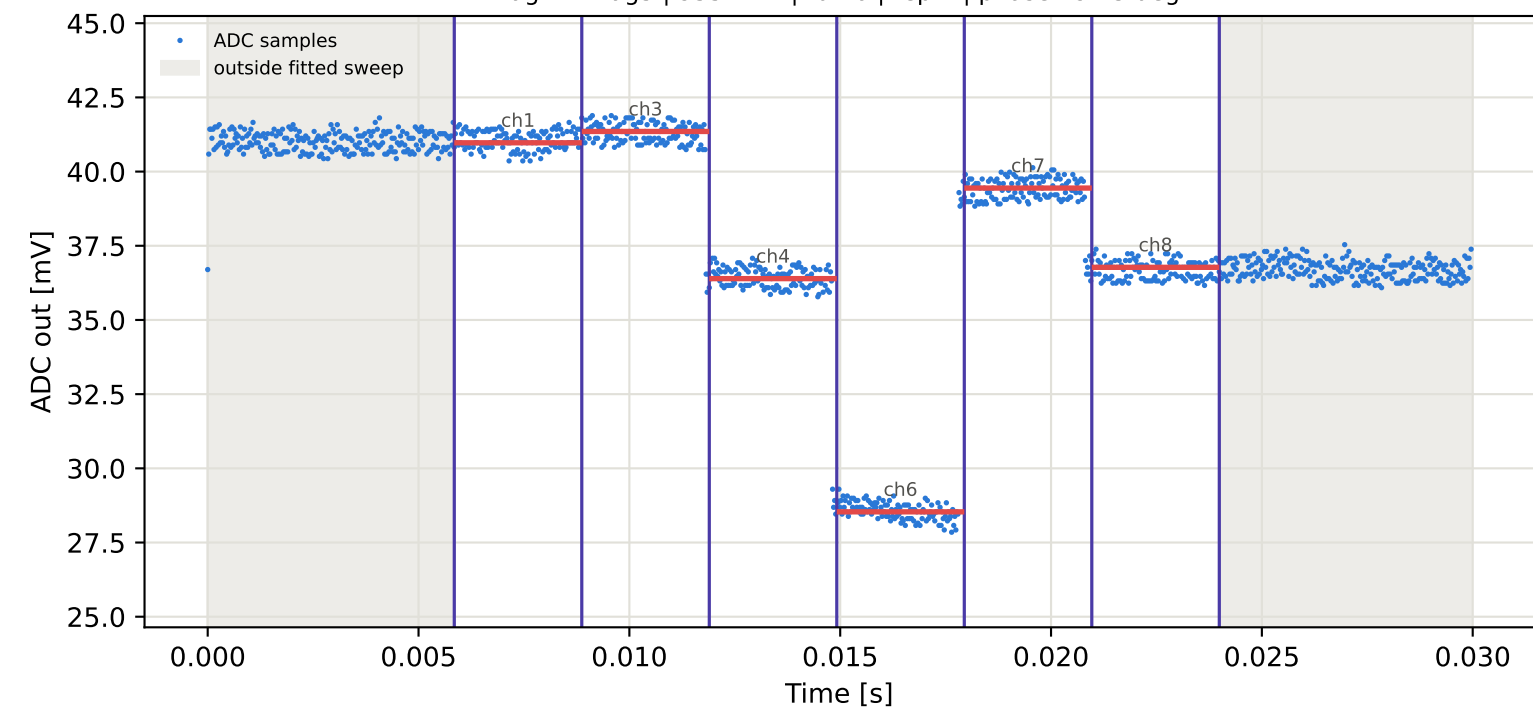
Tag2 &lt;- Tag5 | 955 MHz | run 0 | rep 1 | phase 50.56 deg
