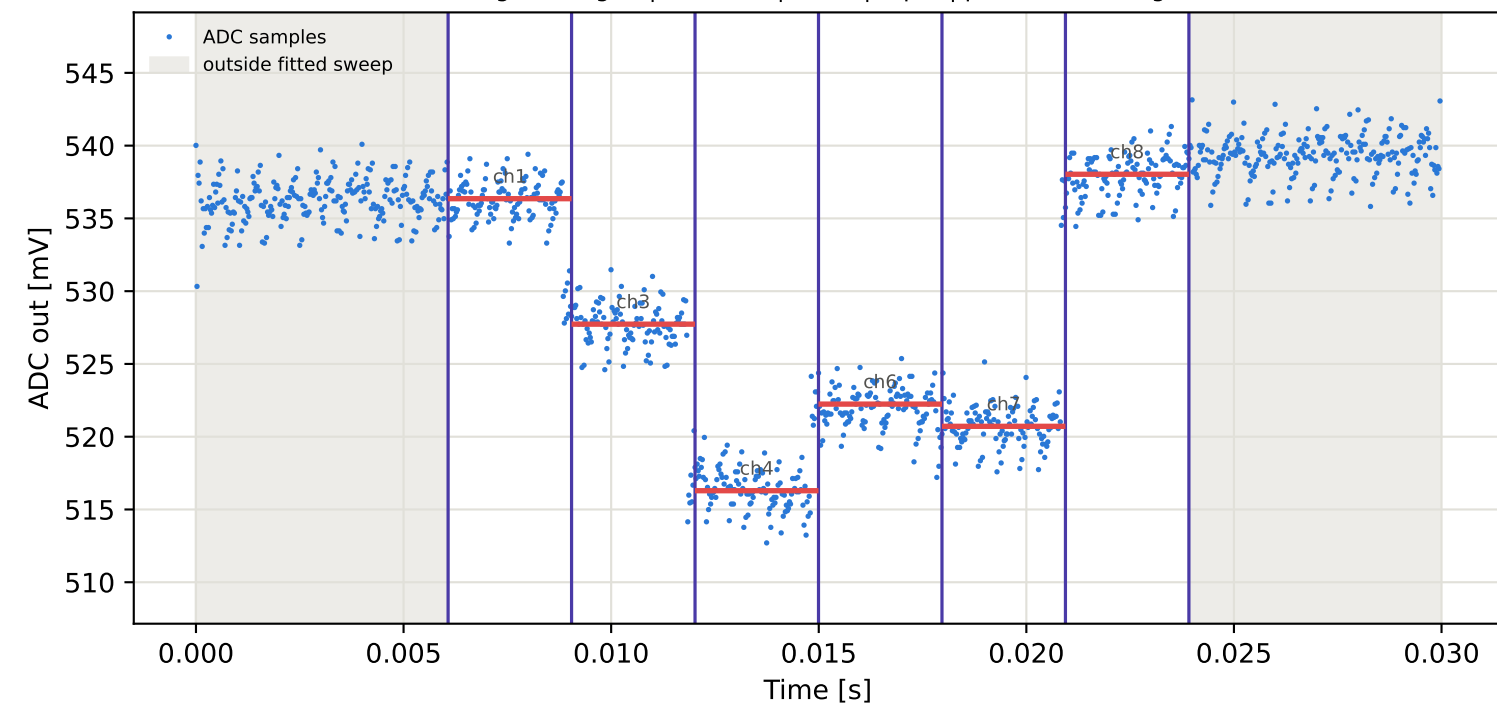
Tag2 &lt;- Tag16 | 915 MHz | run 0 | rep 1 | phase 68.83 deg
