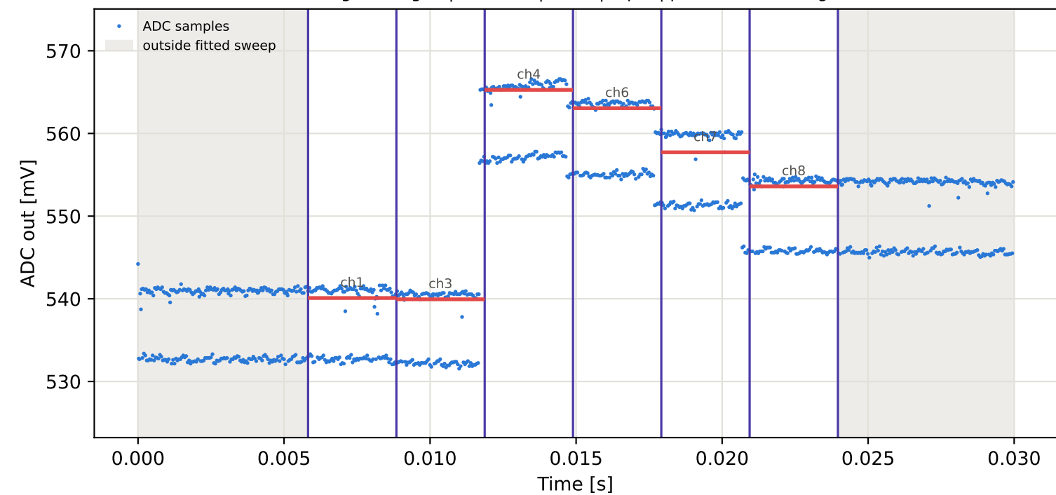
Tag8 &lt;- Tag16 | 825 MHz | run 0 | rep 1 | phase -121.40 deg
