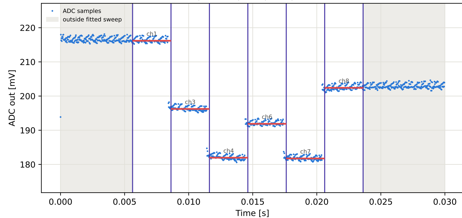
Tag4 &lt;- Tag3 | 835 MHz | run 0 | rep 1 | phase 83.93 deg
