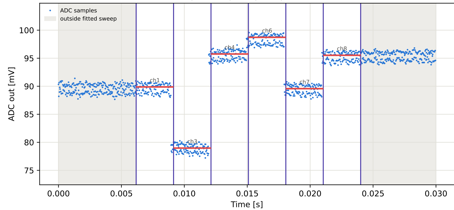
Tag5 &lt;- Tag4 | 795 MHz | run 0 | rep 1 | phase -142.83 deg
