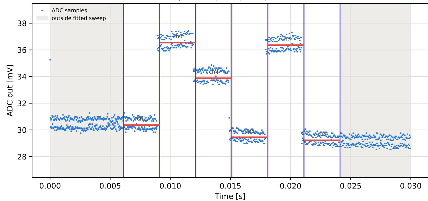
Tag2 &lt;- Tag6 | 805 MHz | run 0 | rep 1 | phase -97.66 deg
