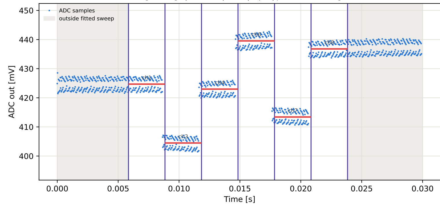
Tag3 &lt;- Tag7 | 825 MHz | run 0 | rep 1 | phase 90.54 deg
