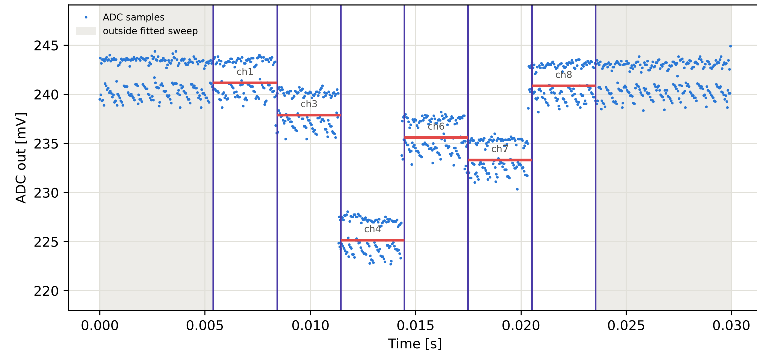
Tag15 &lt;- Tag5 | 985 MHz | run 0 | rep 1 | phase -122.53 deg
