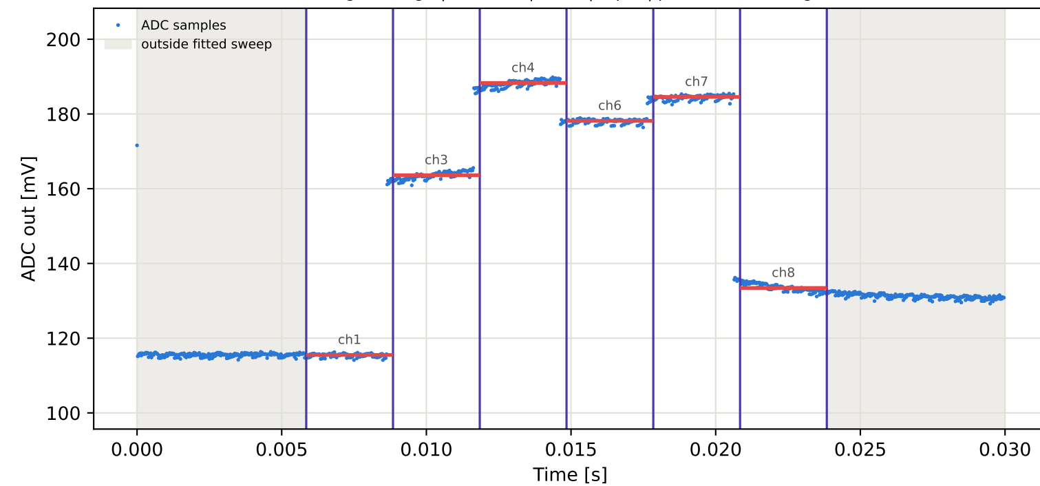
Tag9 &lt;- Tag5 | 865 MHz | run 0 | rep 1 | phase -142.28 deg
