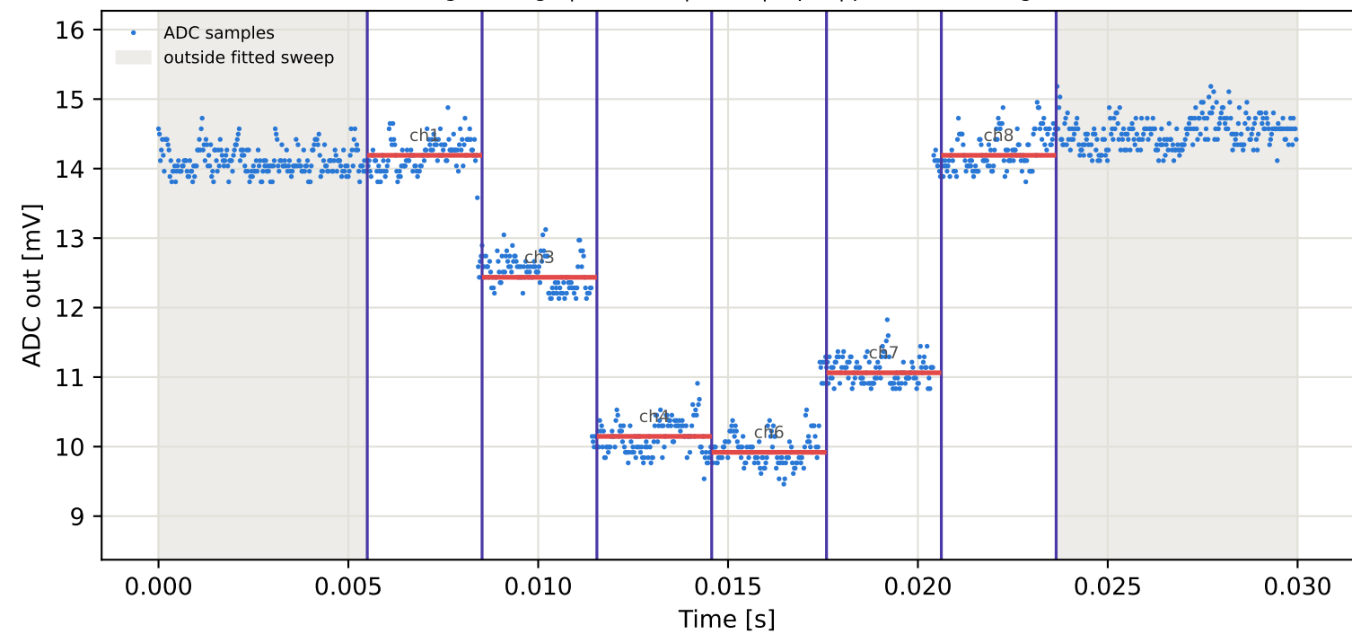
Tag1 &lt;- Tag8 | 905 MHz | run 0 | rep 1 | phase -25.52 deg
