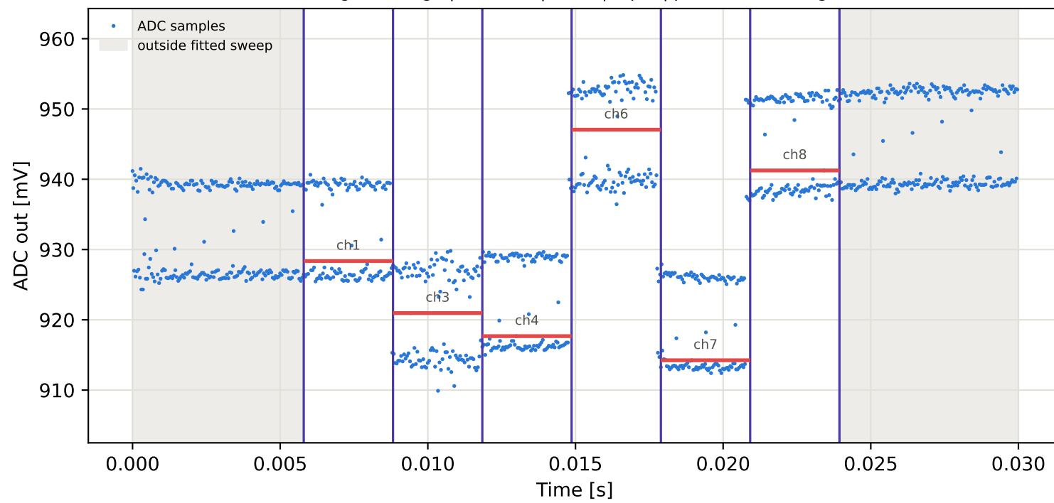
Tag15 &lt;- Tag9 | 875 MHz | run 0 | rep 1 | phase 152.85 deg
