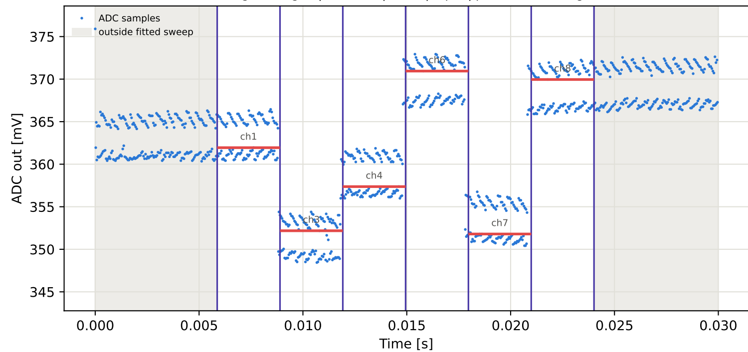
Tag6 &lt;- Tag2 | 825 MHz | run 0 | rep 1 | phase 70.91 deg
