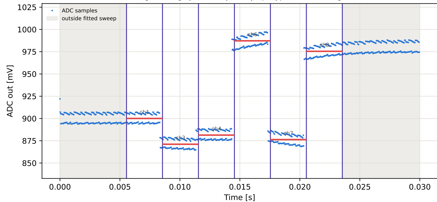
Tag10 &lt;- Tag5 | 895 MHz | run 0 | rep 1 | phase 170.49 deg
