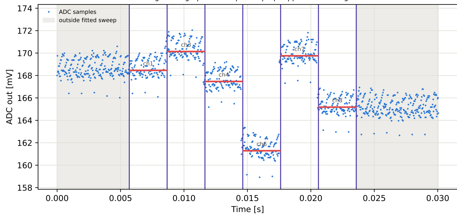
Tag5 &lt;- Tag1 | 995 MHz | run 0 | rep 1 | phase 2.05 deg
