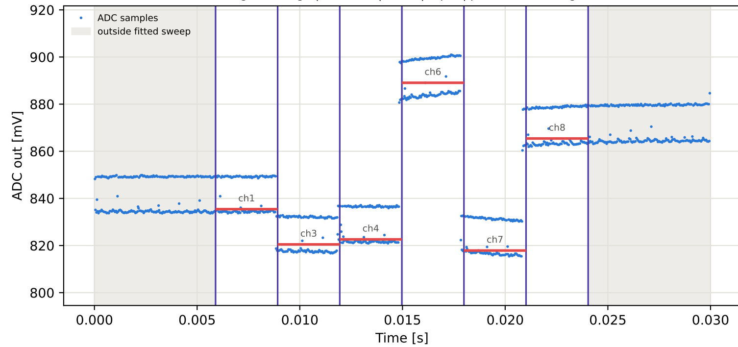
Tag2 &lt;- Tag10 | 955 MHz | run 0 | rep 1 | phase 132.54 deg
