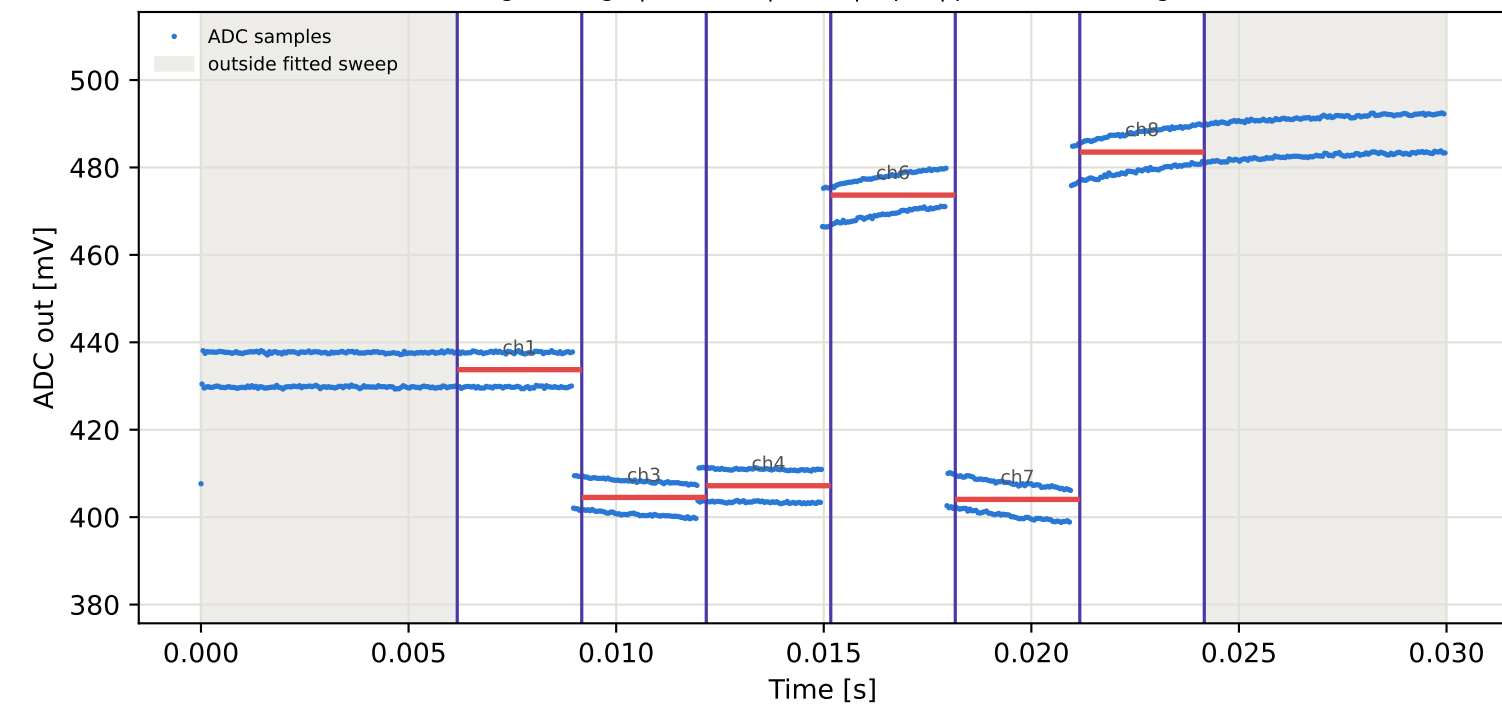
Tag8 &lt;- Tag10 | 905 MHz | run 0 | rep 1 | phase 153.13 deg
