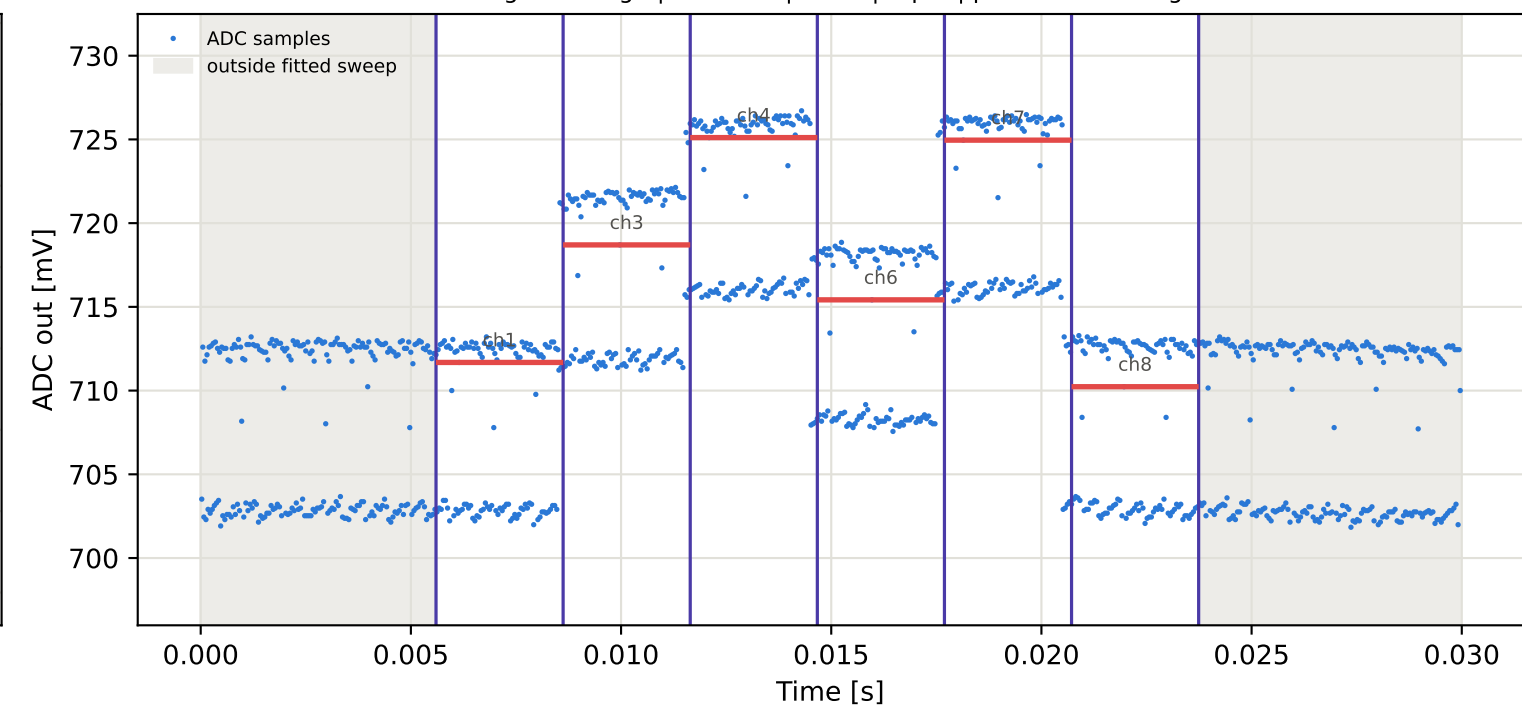
Tag2 &lt;- Tag10 | 865 MHz | run 0 | rep 1 | phase 68.28 deg
