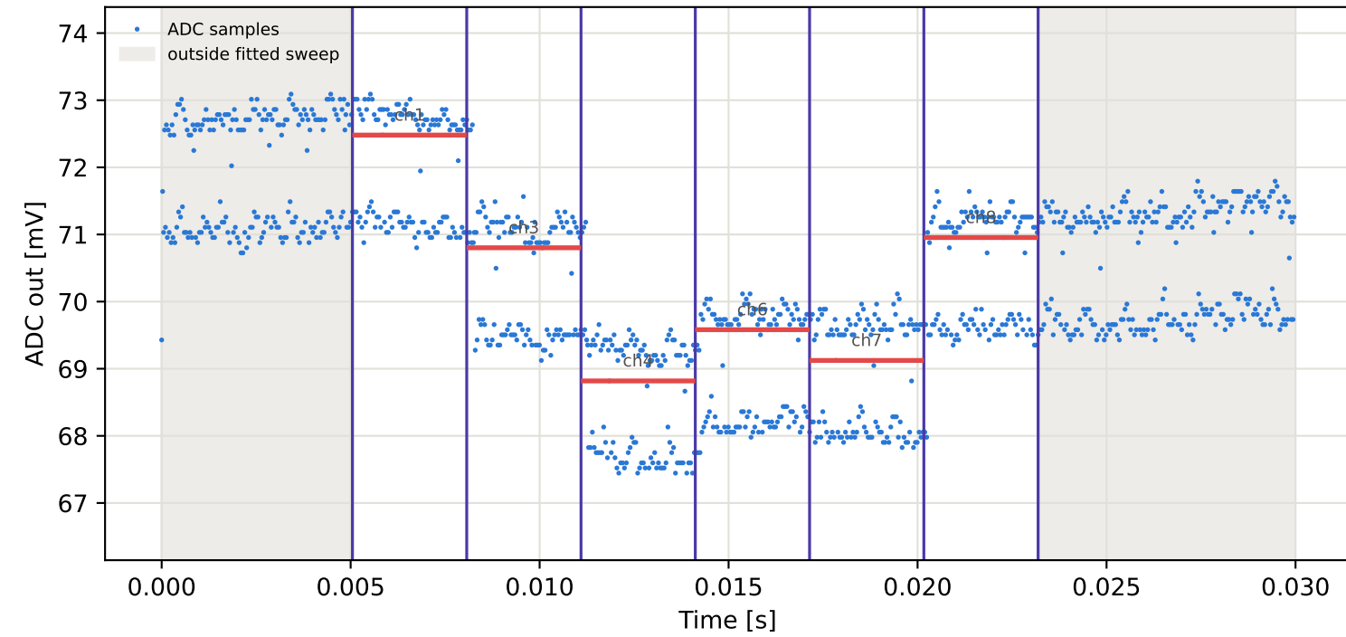
Tag10 &lt;- Tag1 | 855 MHz | run 0 | rep 1 | phase 74.12 deg
