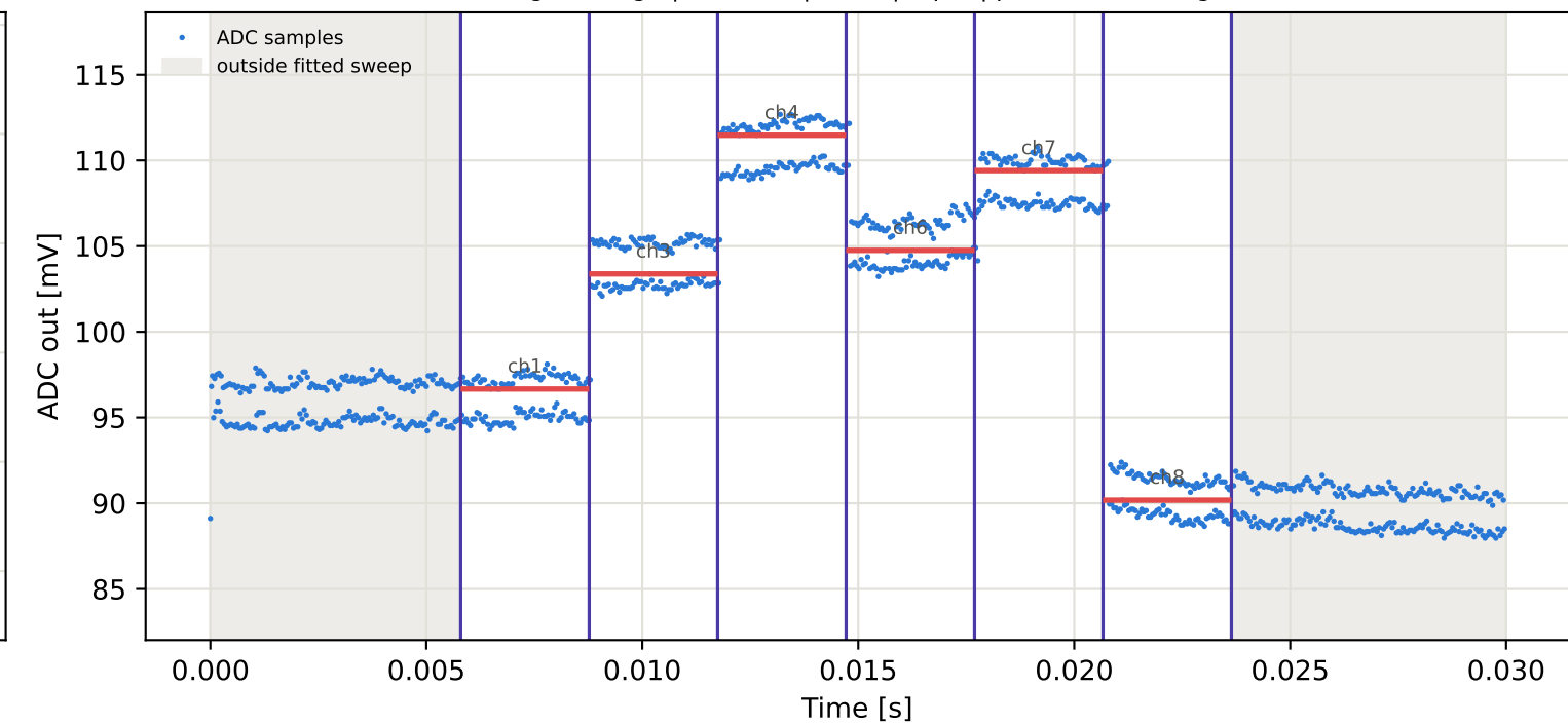
Tag7 &lt;- Tag1 | 905 MHz | run 0 | rep 1 | phase -163.99 deg
