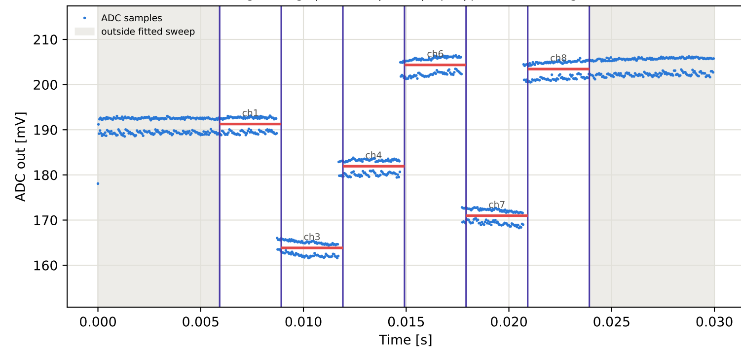
Tag4 &lt;- Tag7 | 825 MHz | run 0 | rep 1 | phase -3.79 deg
