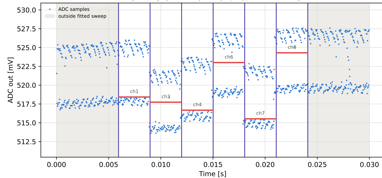
Tag5 &lt;- Tag8 | 835 MHz | run 0 | rep 1 | phase -100.06 deg
