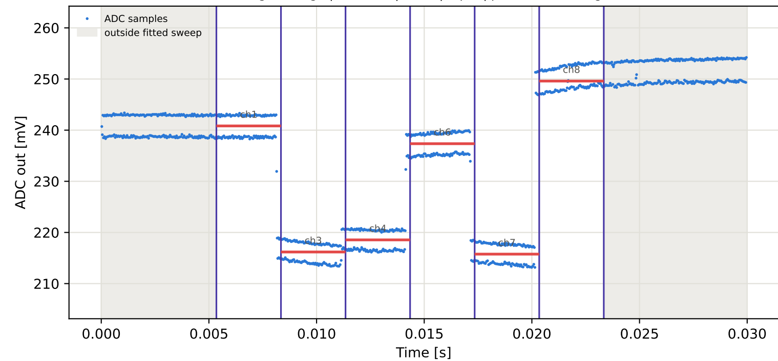
Tag2 &lt;- Tag6 | 855 MHz | run 0 | rep 1 | phase 16.33 deg
