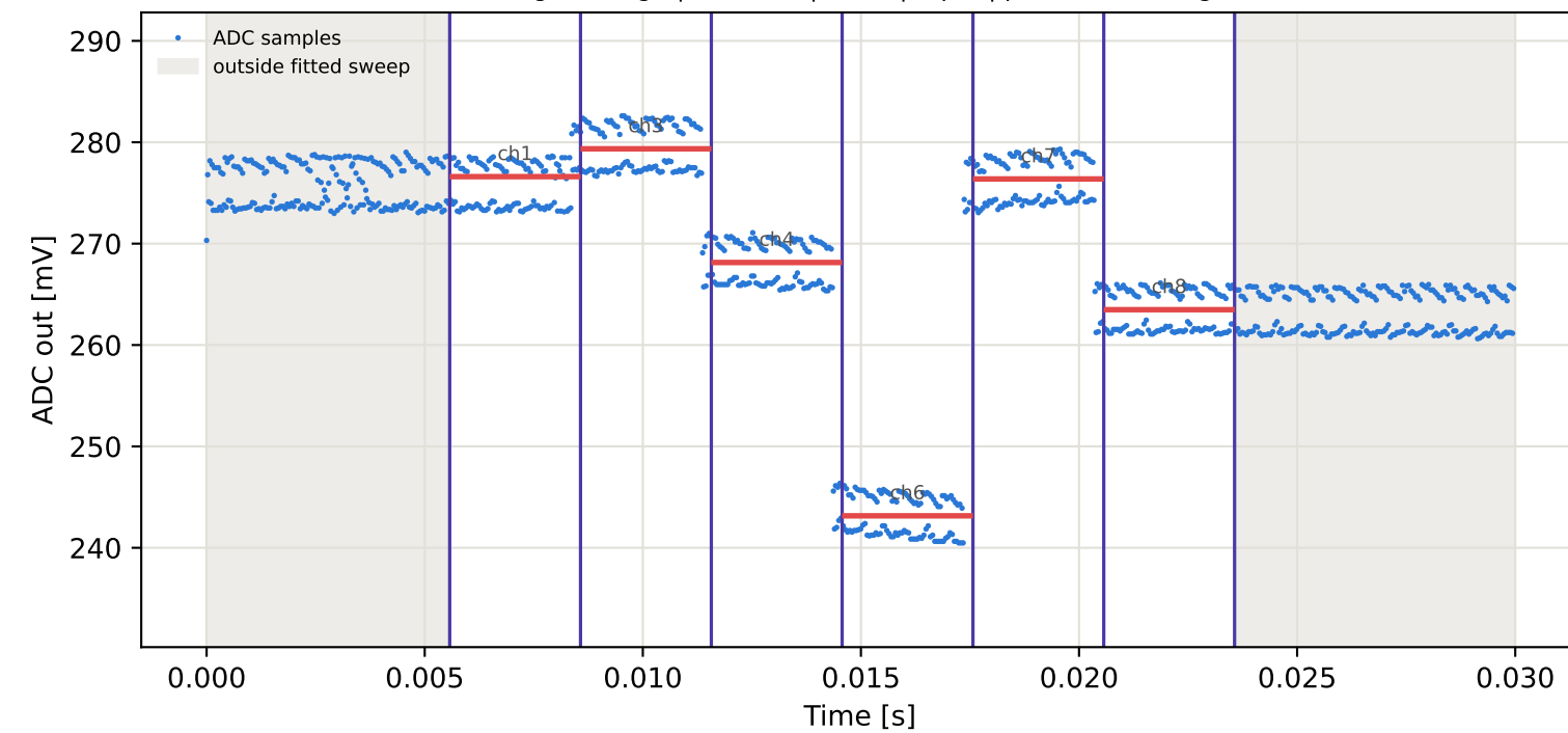
Tag9 &lt;- Tag5 | 975 MHz | run 0 | rep 1 | phase 26.69 deg
