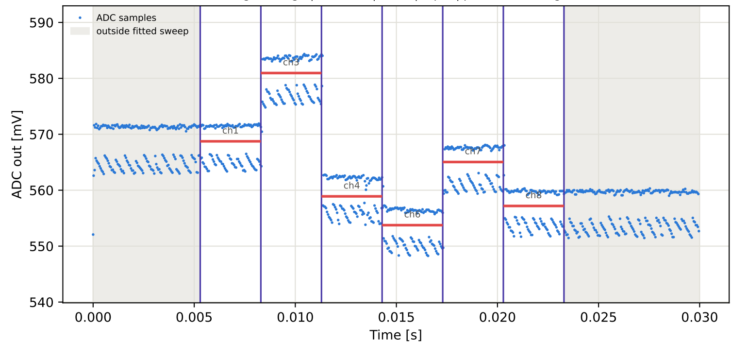
Tag8 &lt;- Tag5 | 825 MHz | run 0 | rep 1 | phase -65.23 deg
