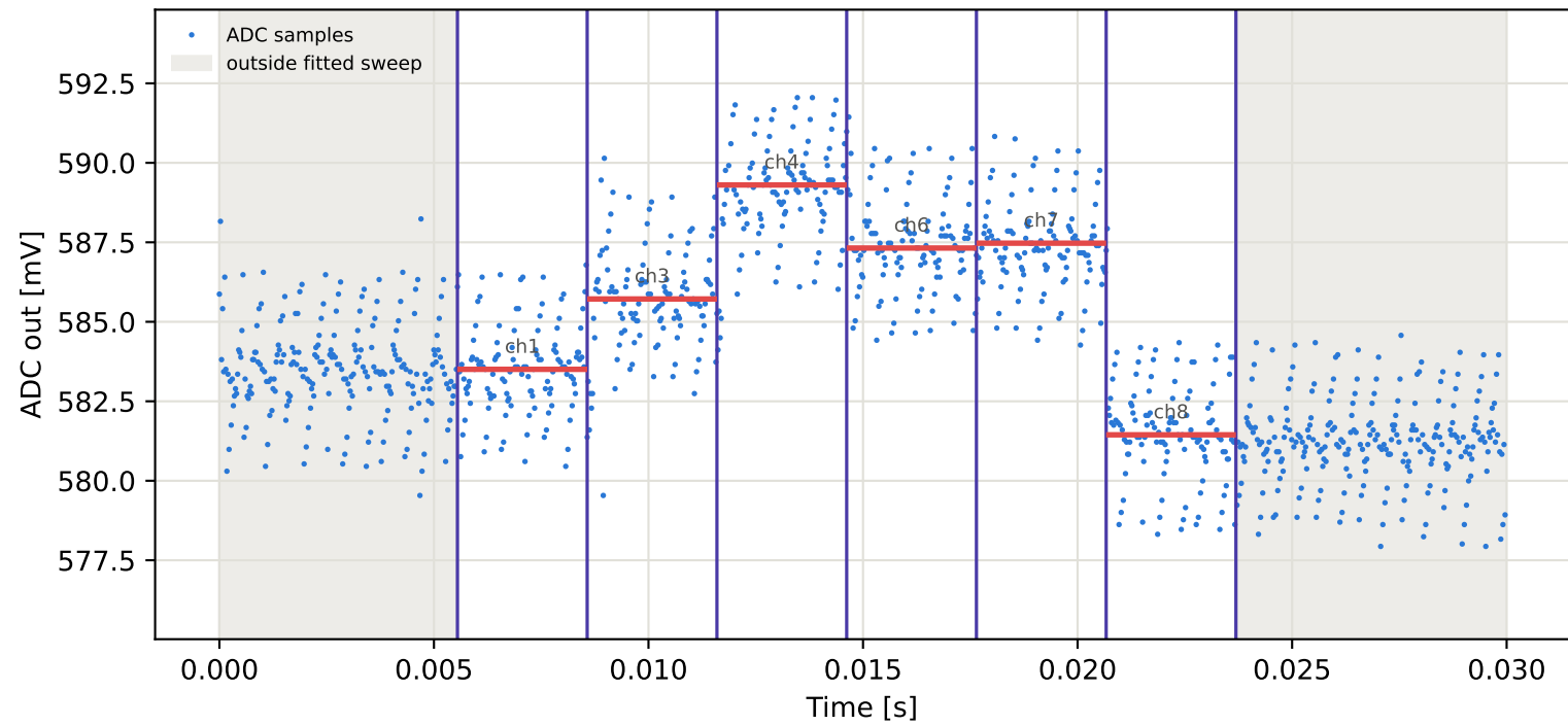
Tag10 &lt;- Tag4 | 945 MHz | run 0 | rep 1 | phase -5.67 deg
