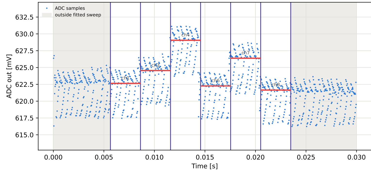
Tag7 &lt;- Tag6 | 985 MHz | run 0 | rep 1 | phase -43.11 deg
