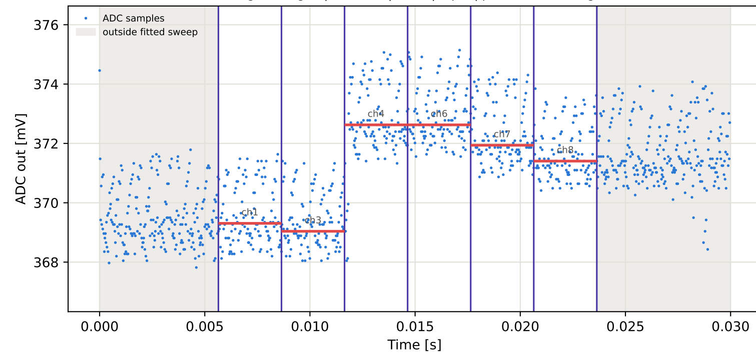
Tag5 &lt;- Tag16 | 825 MHz | run 0 | rep 1 | phase -84.30 deg
