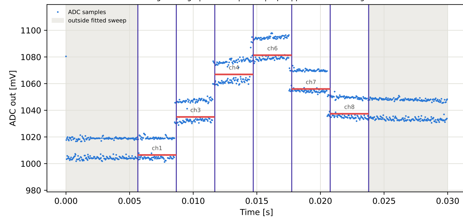
Tag3 &lt;- Tag8 | 885 MHz | run 0 | rep 1 | phase -127.96 deg
