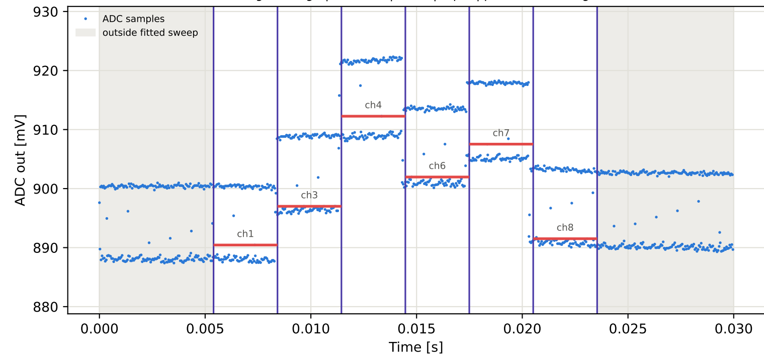
Tag8 &lt;- Tag7 | 865 MHz | run 0 | rep 1 | phase -99.74 deg
