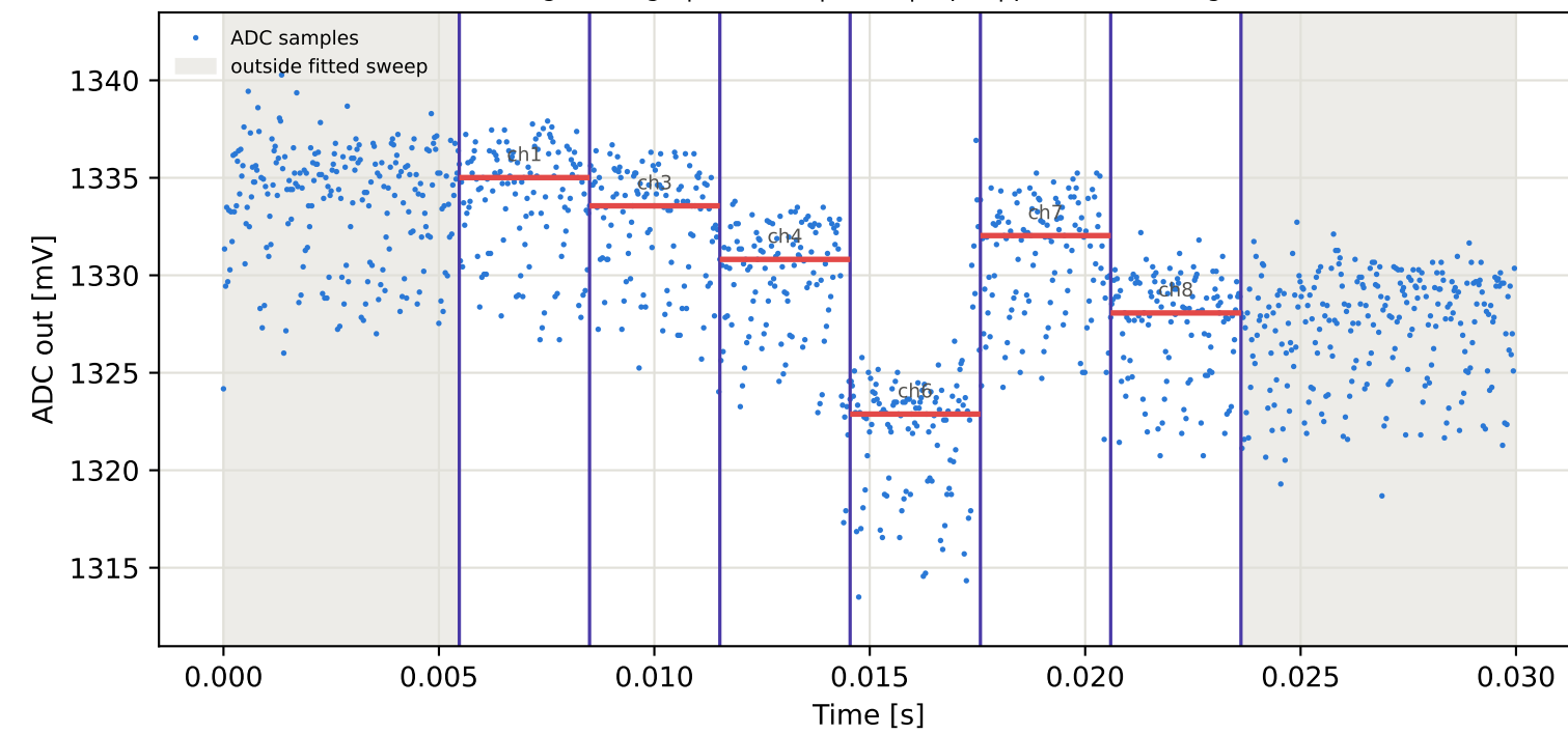
Tag8 &lt;- Tag4 | 885 MHz | run 0 | rep 1 | phase -155.82 deg
