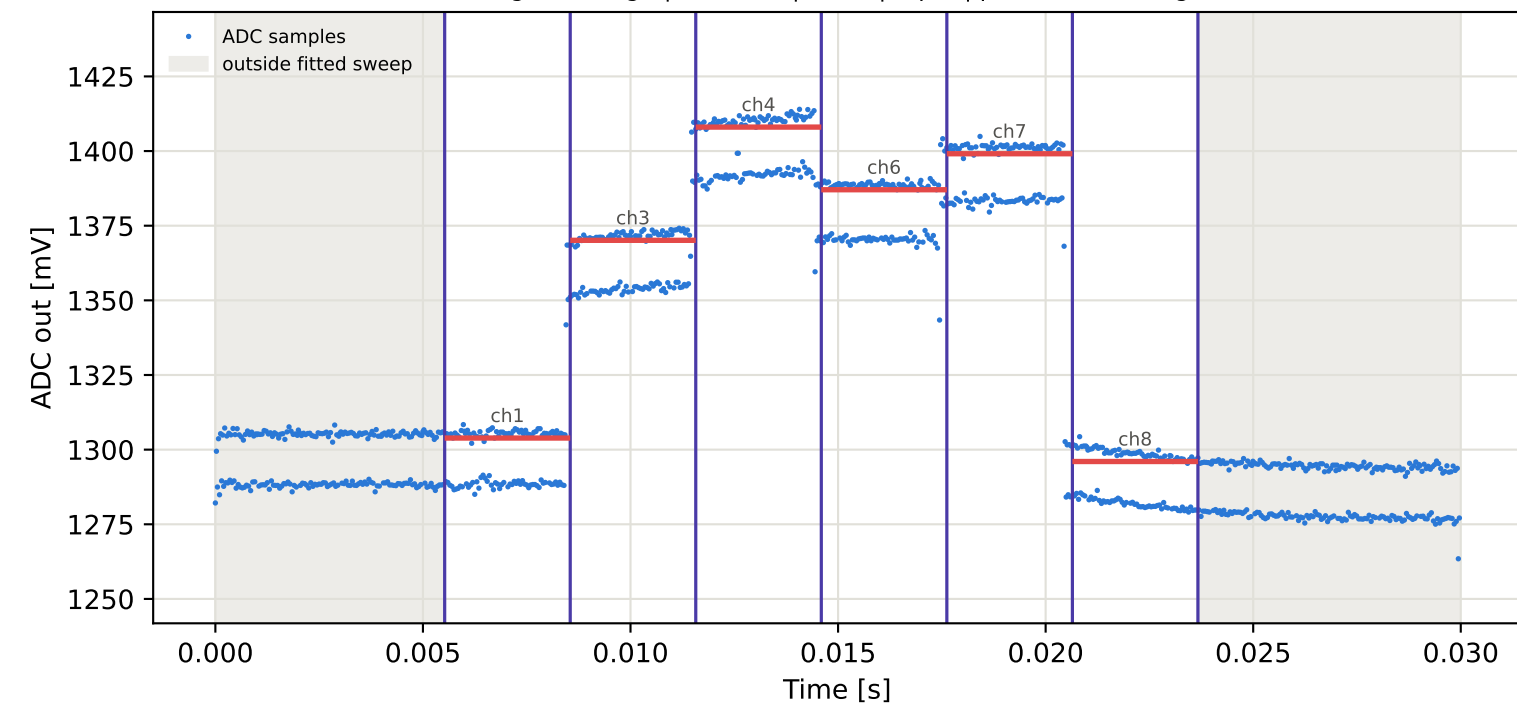
Tag2 &lt;- Tag1 | 885 MHz | run 0 | rep 1 | phase 175.67 deg
