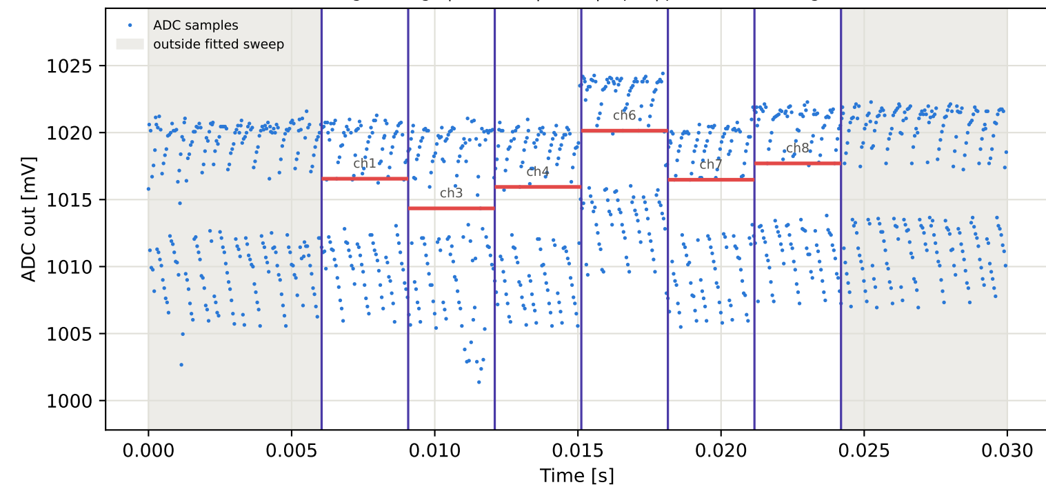
Tag8 &lt;- Tag4 | 975 MHz | run 0 | rep 1 | phase -170.72 deg
