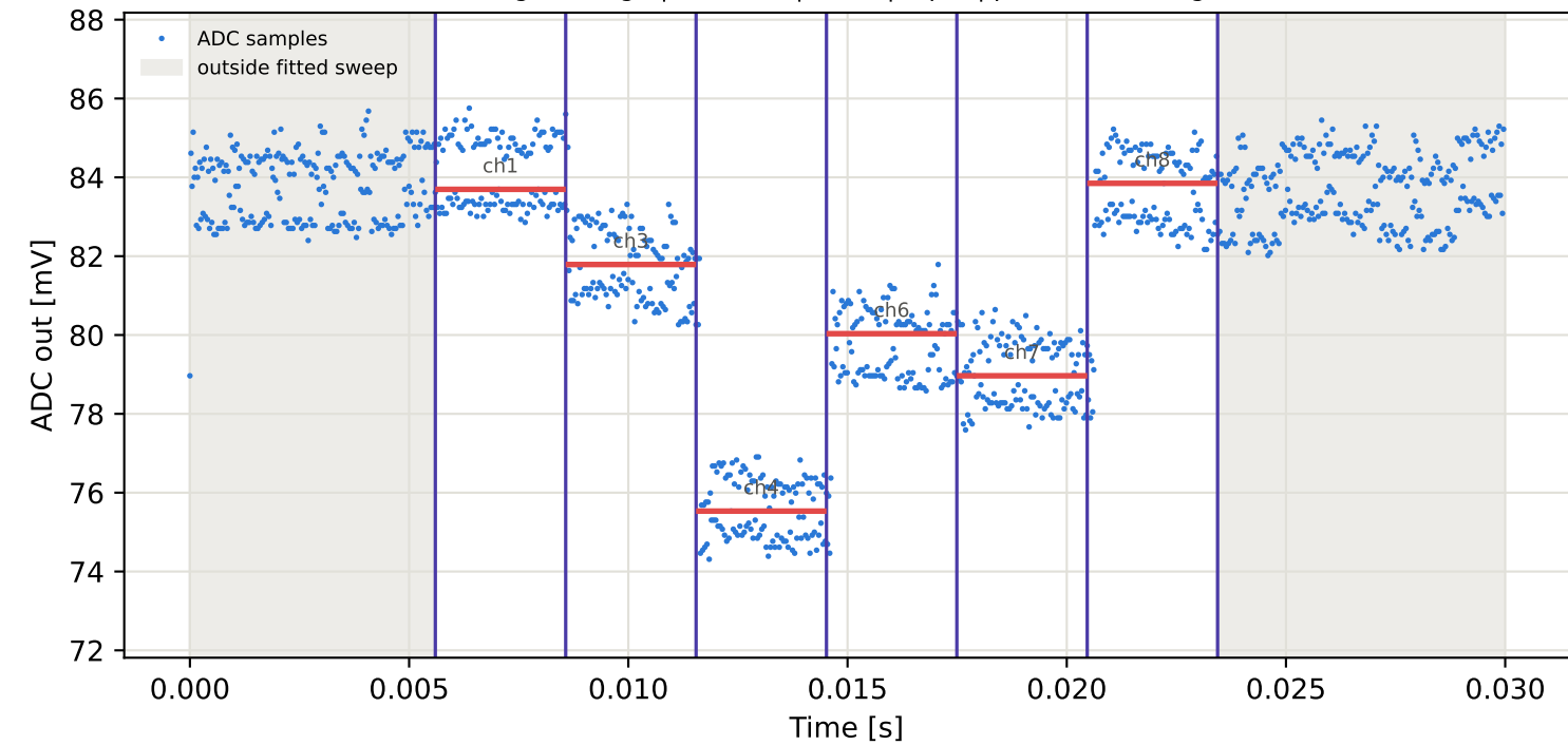
Tag7 &lt;- Tag1 | 955 MHz | run 0 | rep 1 | phase -173.45 deg
