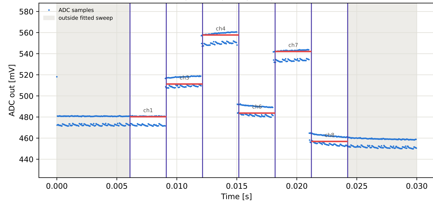
Tag9 &lt;- Tag7 | 945 MHz | run 0 | rep 1 | phase -78.48 deg
