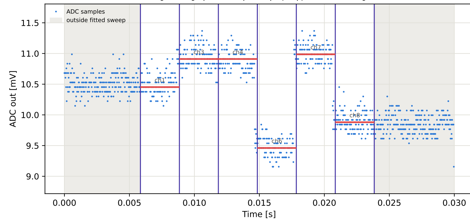
Tag2 &lt;- Tag7 | 995 MHz | run 0 | rep 1 | phase -22.53 deg
