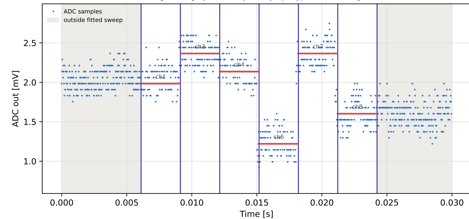
Tag2 &lt;- Tag15 | 965 MHz | run 0 | rep 1 | phase -174.17 deg
