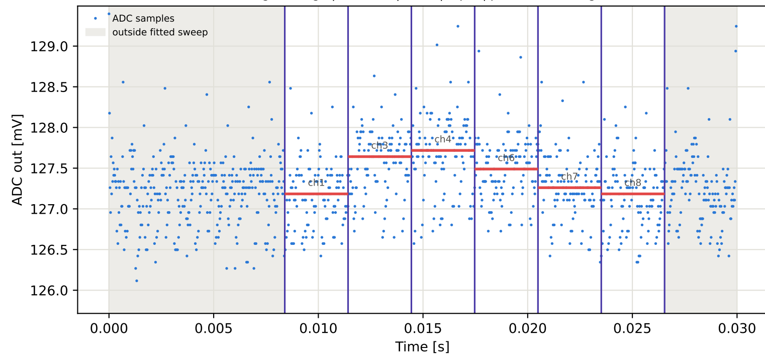
Tag7 &lt;- Tag4 | 805 MHz | run 0 | rep 1 | phase -52.99 deg
