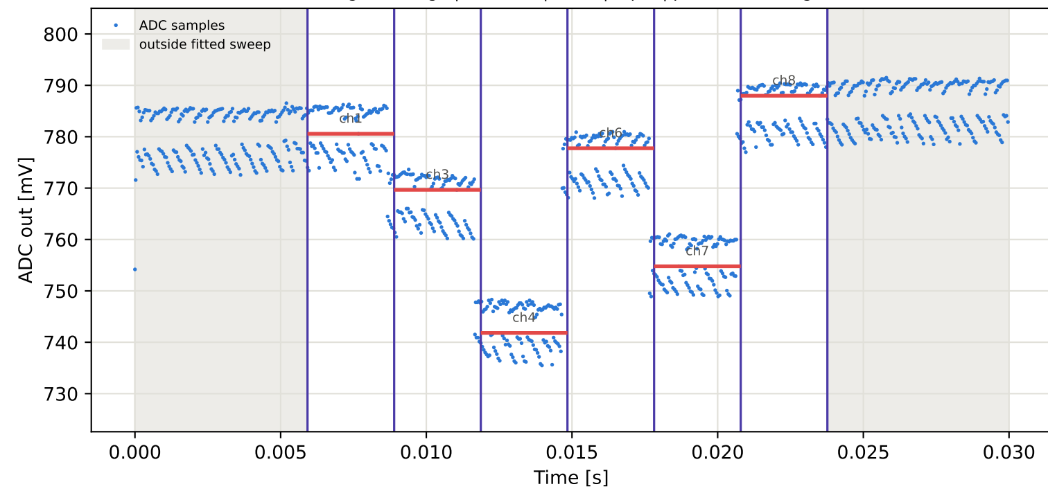
Tag16 &lt;- Tag1 | 955 MHz | run 0 | rep 1 | phase -19.66 deg
