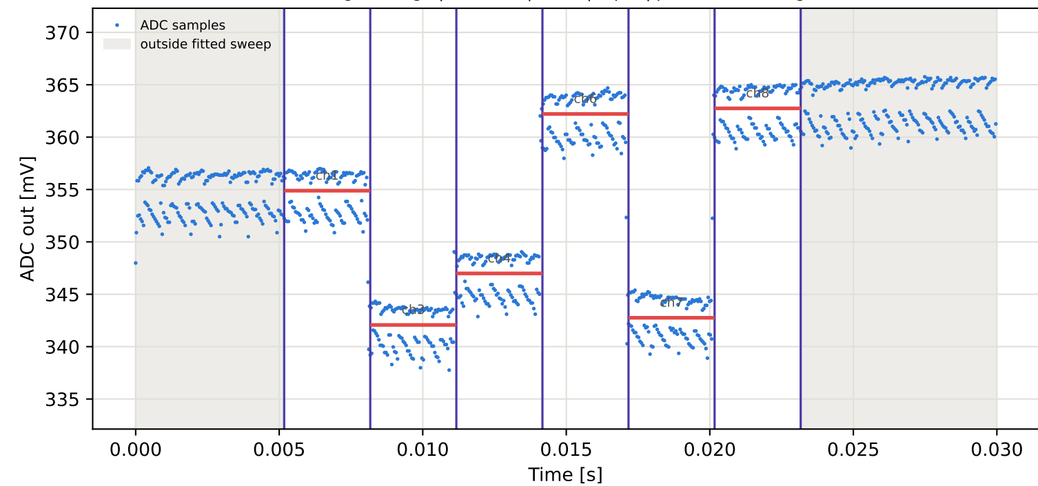
Tag8 &lt;- Tag10 | 825 MHz | run 0 | rep 1 | phase -149.37 deg
