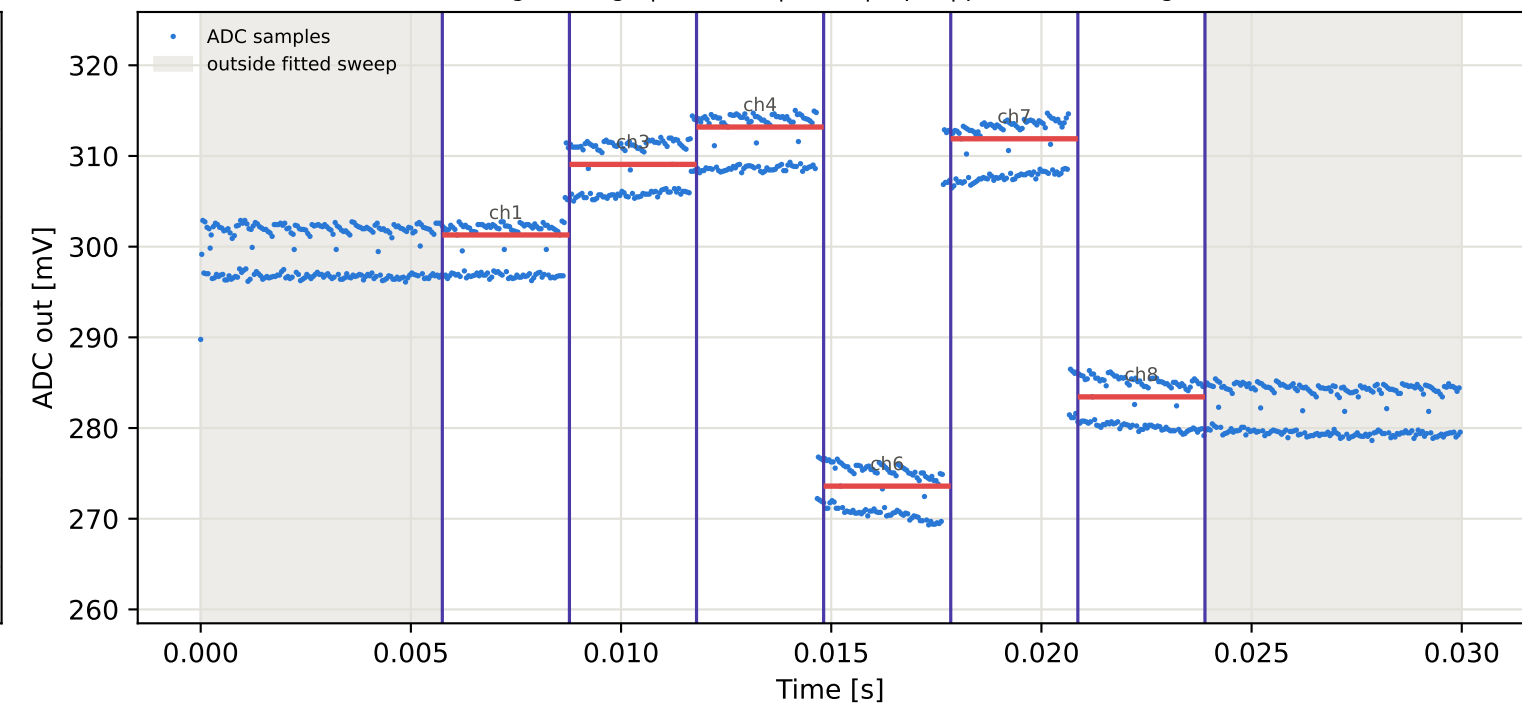
Tag7 &lt;- Tag1 | 925 MHz | run 0 | rep 1 | phase 168.03 deg
