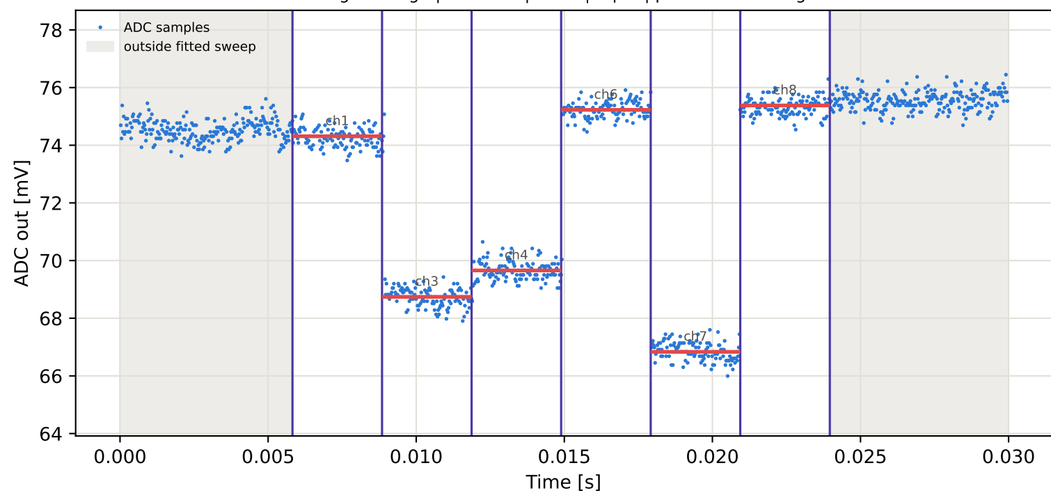
Tag9 &lt;- Tag8 | 785 MHz | run 0 | rep 1 | phase 154.08 deg
