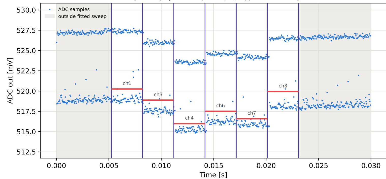
Tag6 &lt;- Tag10 | 835 MHz | run 0 | rep 1 | phase 83.85 deg
