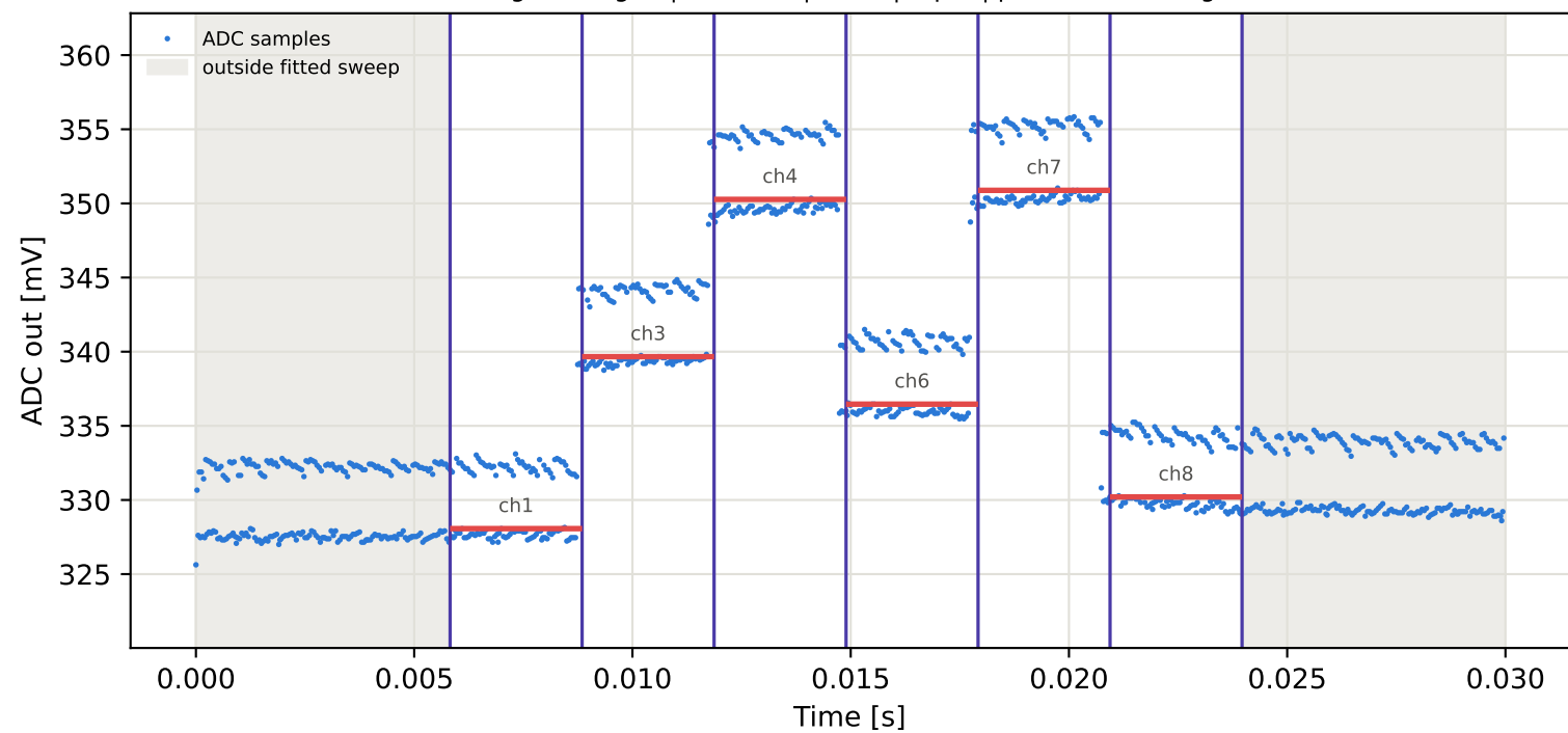
Tag7 &lt;- Tag15 | 825 MHz | run 0 | rep 1 | phase -74.49 deg
