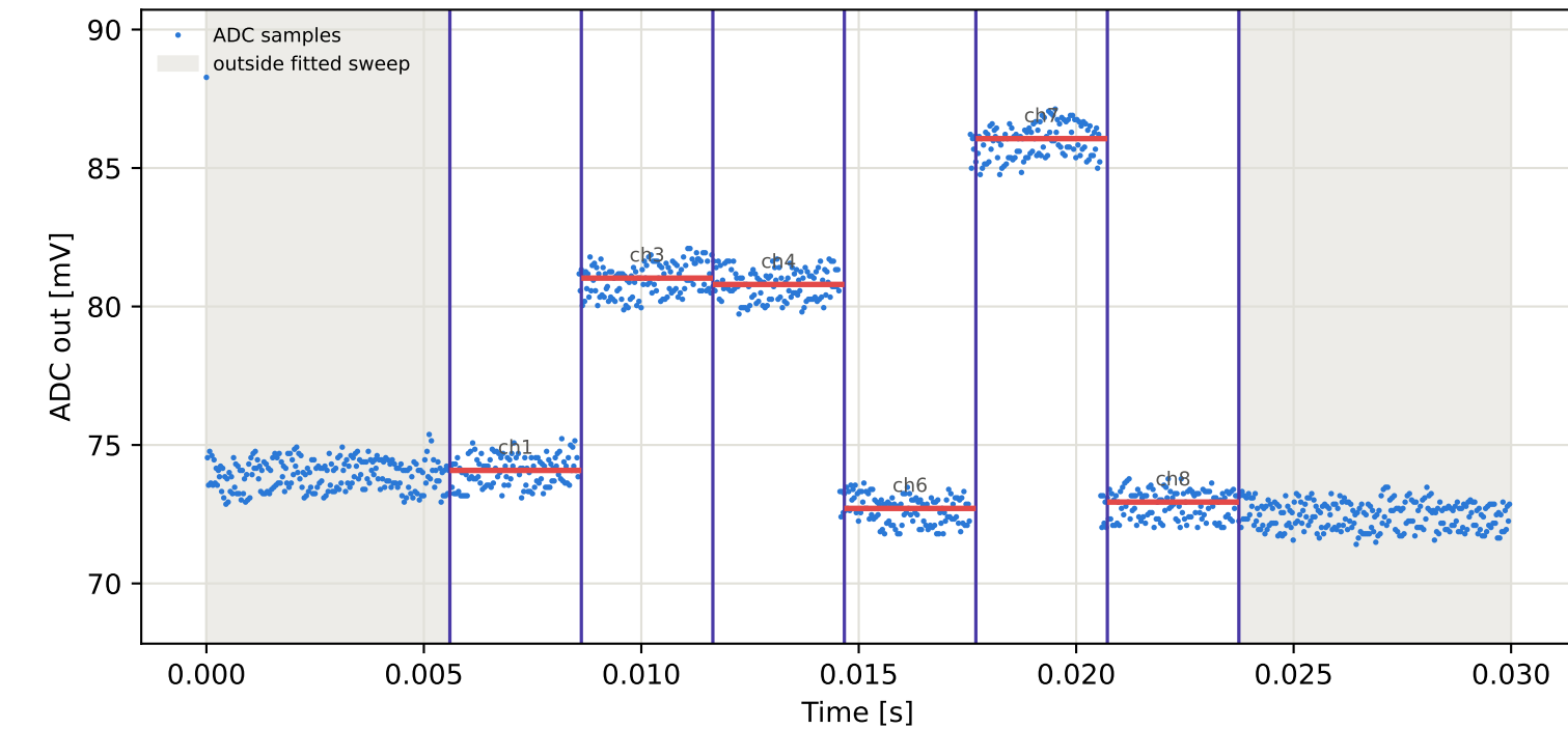
Tag9 &lt;- Tag16 | 775 MHz | run 0 | rep 1 | phase -135.47 deg
