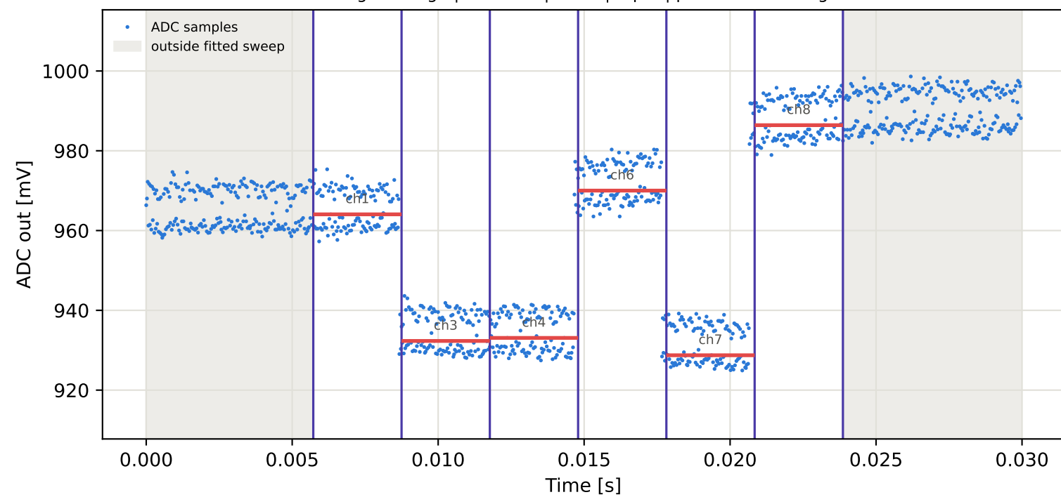
Tag8 &lt;- Tag10 | 885 MHz | run 0 | rep 1 | phase 7.69 deg
