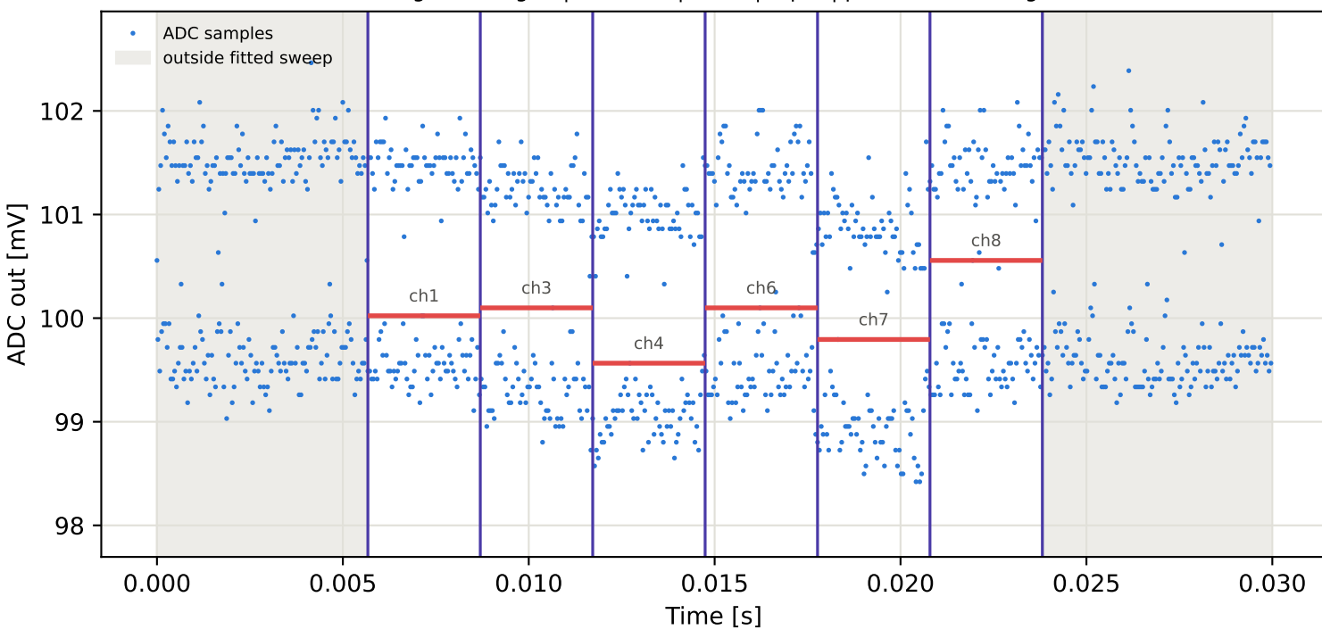
Tag15 &lt;- Tag10 | 785 MHz | run 0 | rep 1 | phase 112.34 deg
