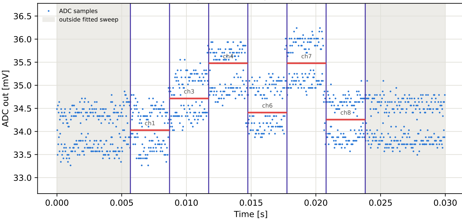
Tag2 &lt;- Tag15 | 805 MHz | run 0 | rep 1 | phase -68.76 deg
