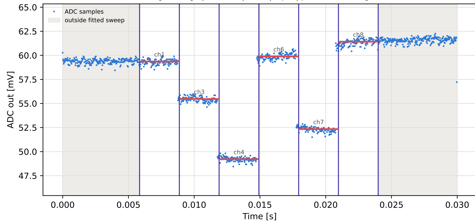
Tag2 &lt;- Tag7 | 975 MHz | run 0 | rep 1 | phase 81.48 deg
