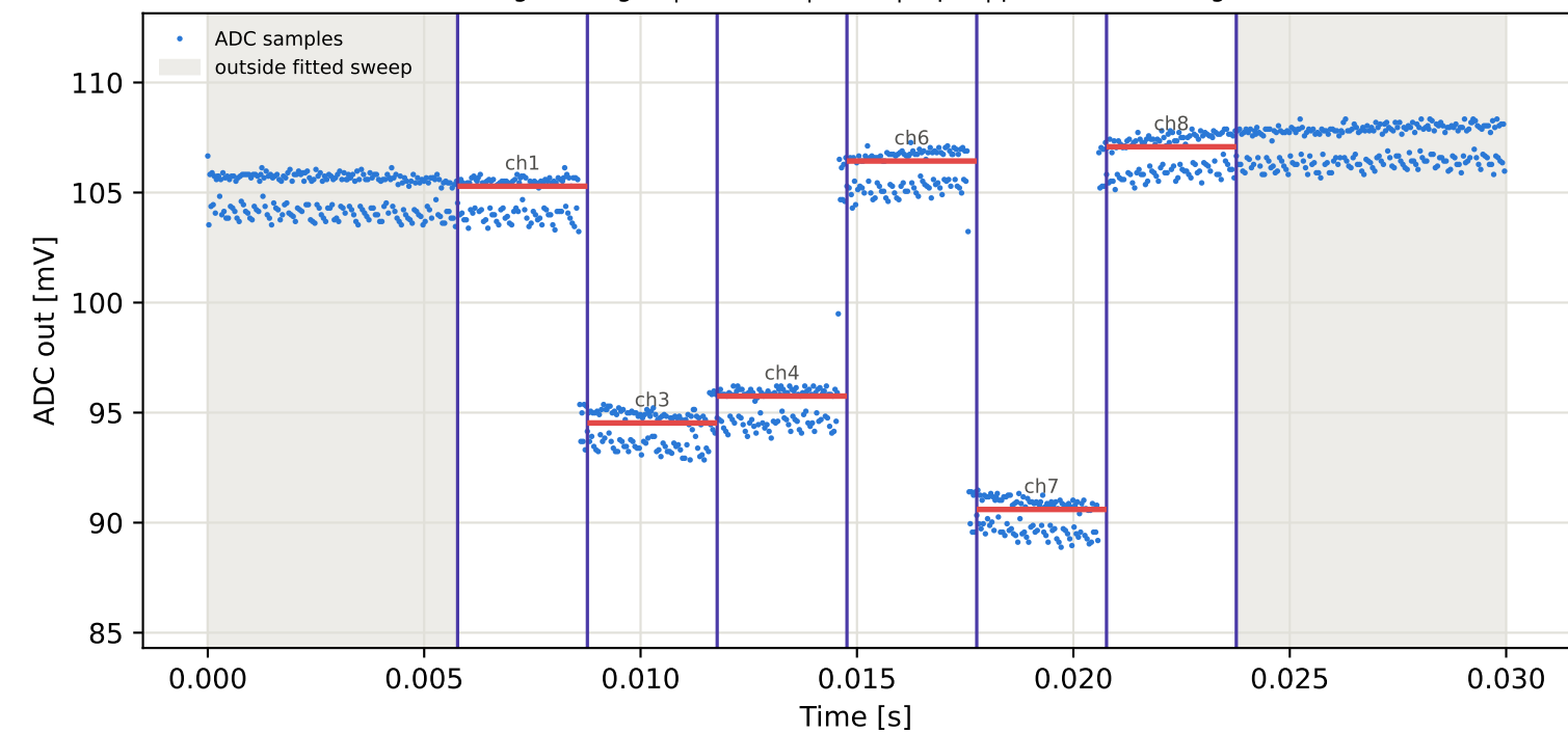
Tag3 &lt;- Tag16 | 795 MHz | run 0 | rep 1 | phase 148.43 deg
