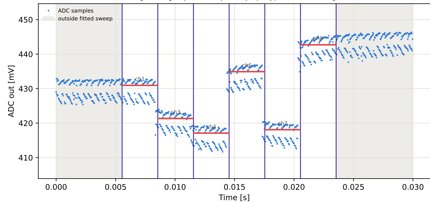
Tag2 &lt;- Tag16 | 905 MHz | run 0 | rep 1 | phase 129.28 deg
