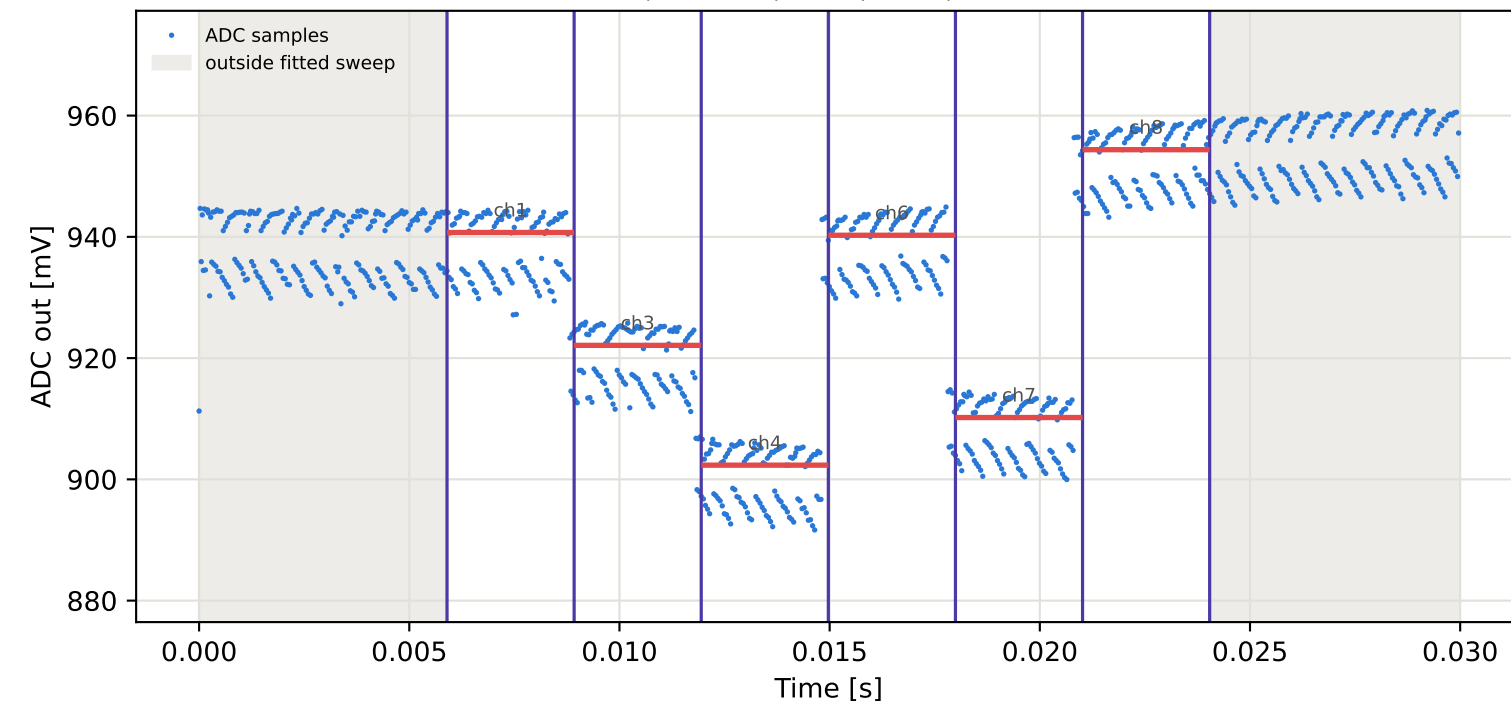
Tag5 &lt;- Tag3 | 925 MHz | run 0 | rep 1 | phase 108.72 deg
