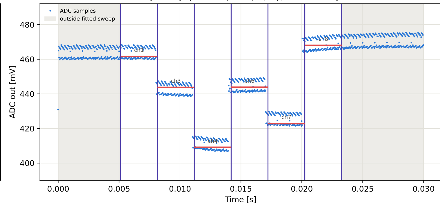
Tag3 &lt;- Tag9 | 945 MHz | run 0 | rep 1 | phase 85.47 deg
