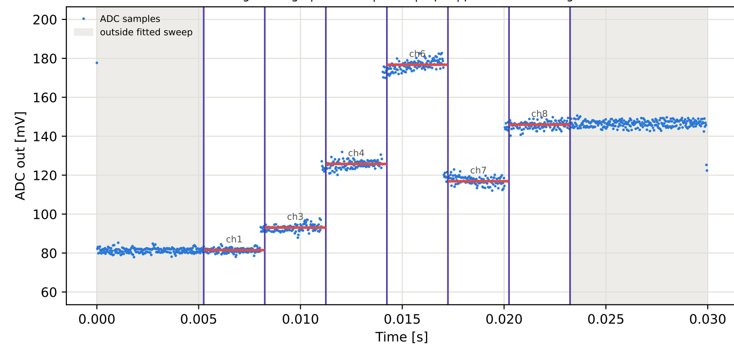
Tag4 &lt;- Tag7 | 885 MHz | run 0 | rep 1 | phase 158.96 deg
