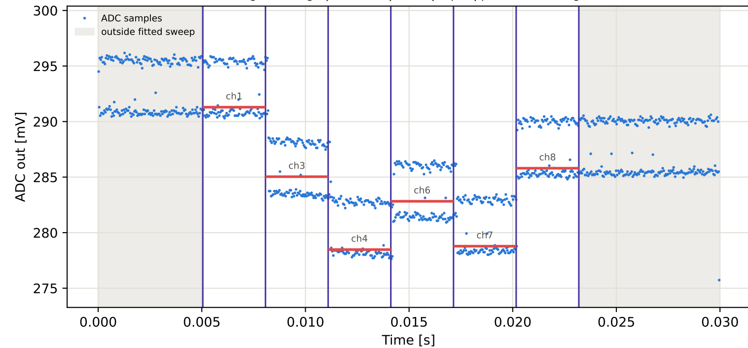
Tag16 &lt;- Tag6 | 835 MHz | run 0 | rep 1 | phase -94.81 deg
