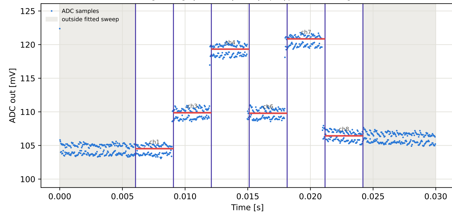
Tag8 &lt;- Tag1 | 785 MHz | run 0 | rep 1 | phase -37.55 deg
