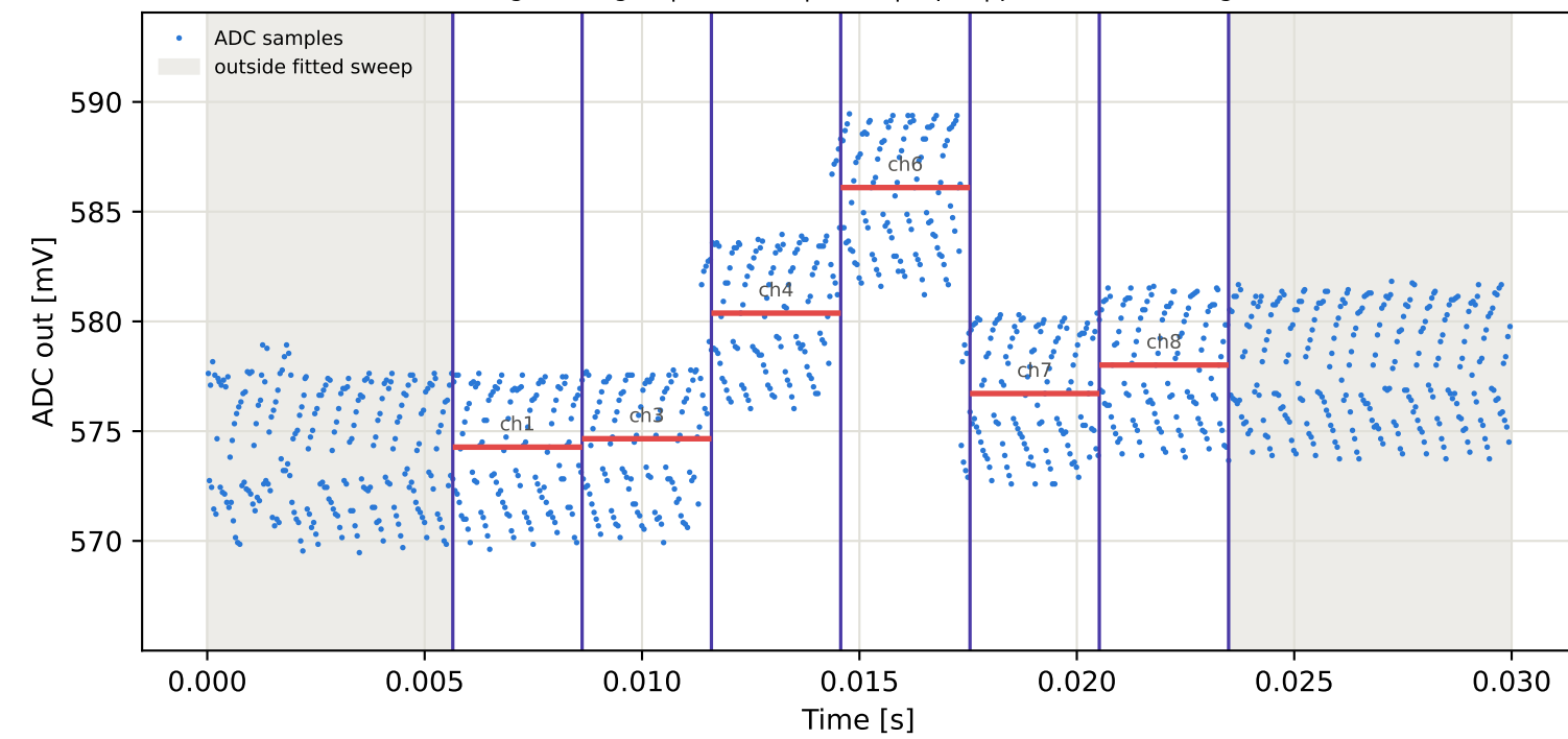
Tag5 &lt;- Tag16 | 955 MHz | run 0 | rep 1 | phase 79.51 deg
