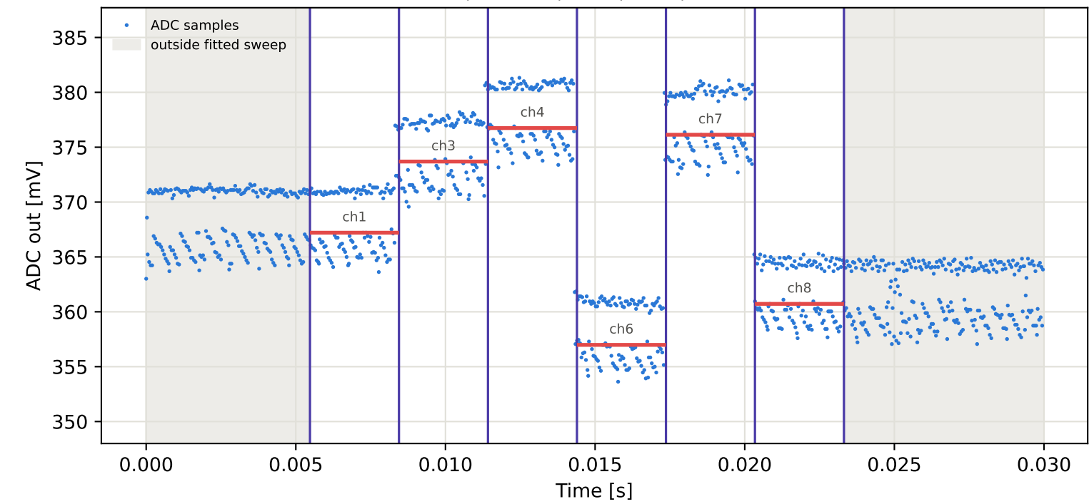
Tag5 &lt;- Tag1 | 985 MHz | run 0 | rep 1 | phase -37.33 deg
