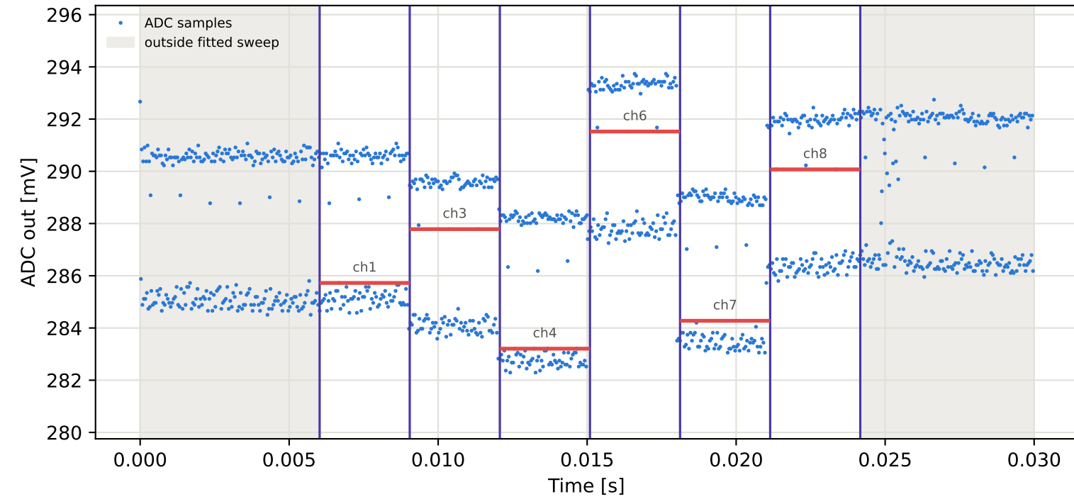
Tag3 &lt;- Tag2 | 985 MHz | run 0 | rep 1 | phase 132.23 deg
