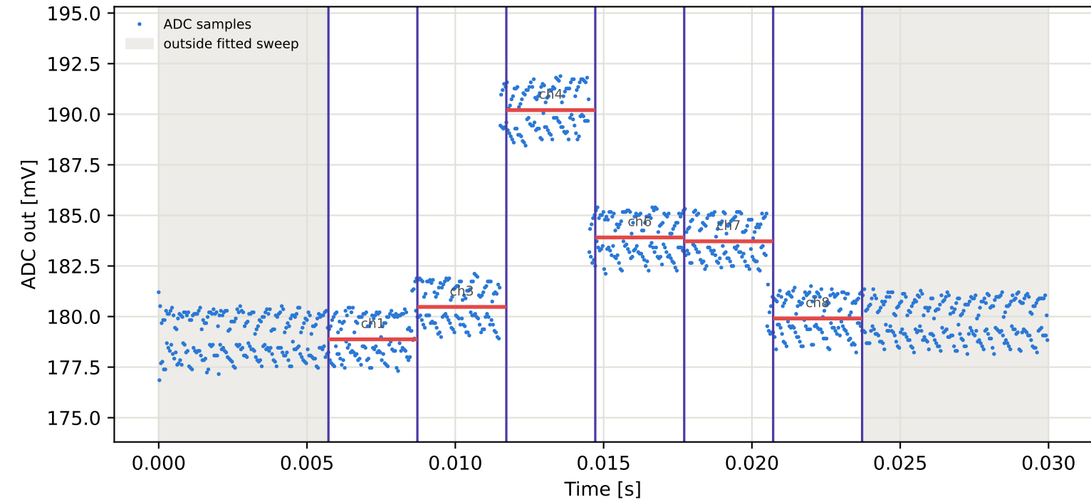
Tag10 &lt;- Tag5 | 995 MHz | run 0 | rep 1 | phase -39.82 deg
