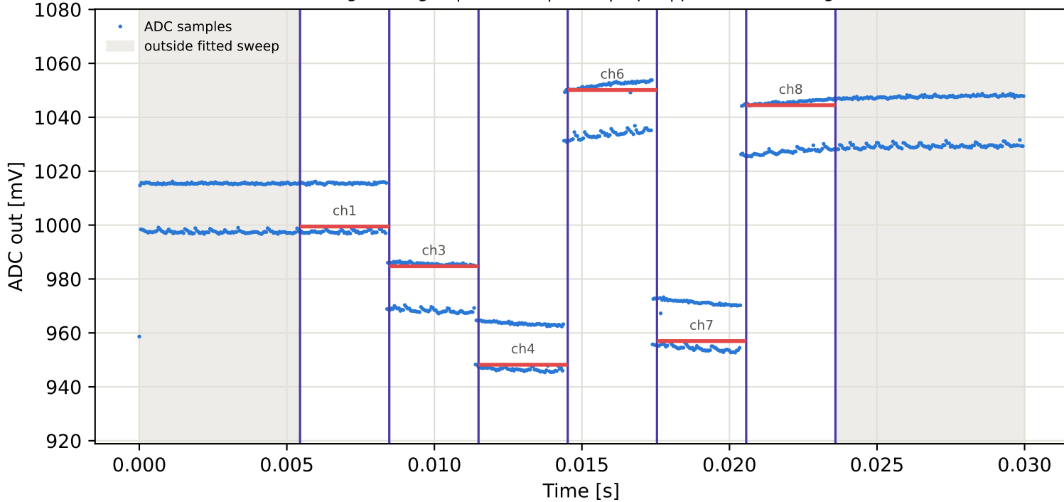
Tag8 &lt;- Tag16 | 945 MHz | run 0 | rep 1 | phase 134.77 deg
