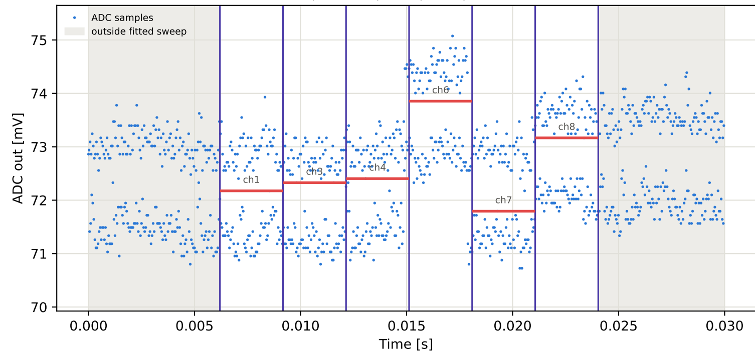
Tag9 &lt;- Tag2 | 795 MHz | run 0 | rep 1 | phase -170.96 deg
