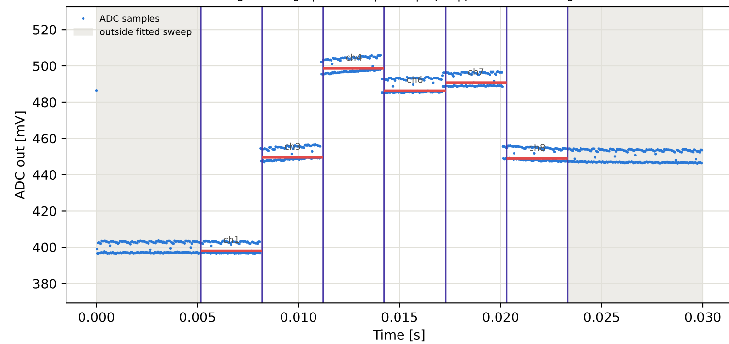
Tag2 &lt;- Tag1 | 845 MHz | run 0 | rep 1 | phase 133.17 deg
