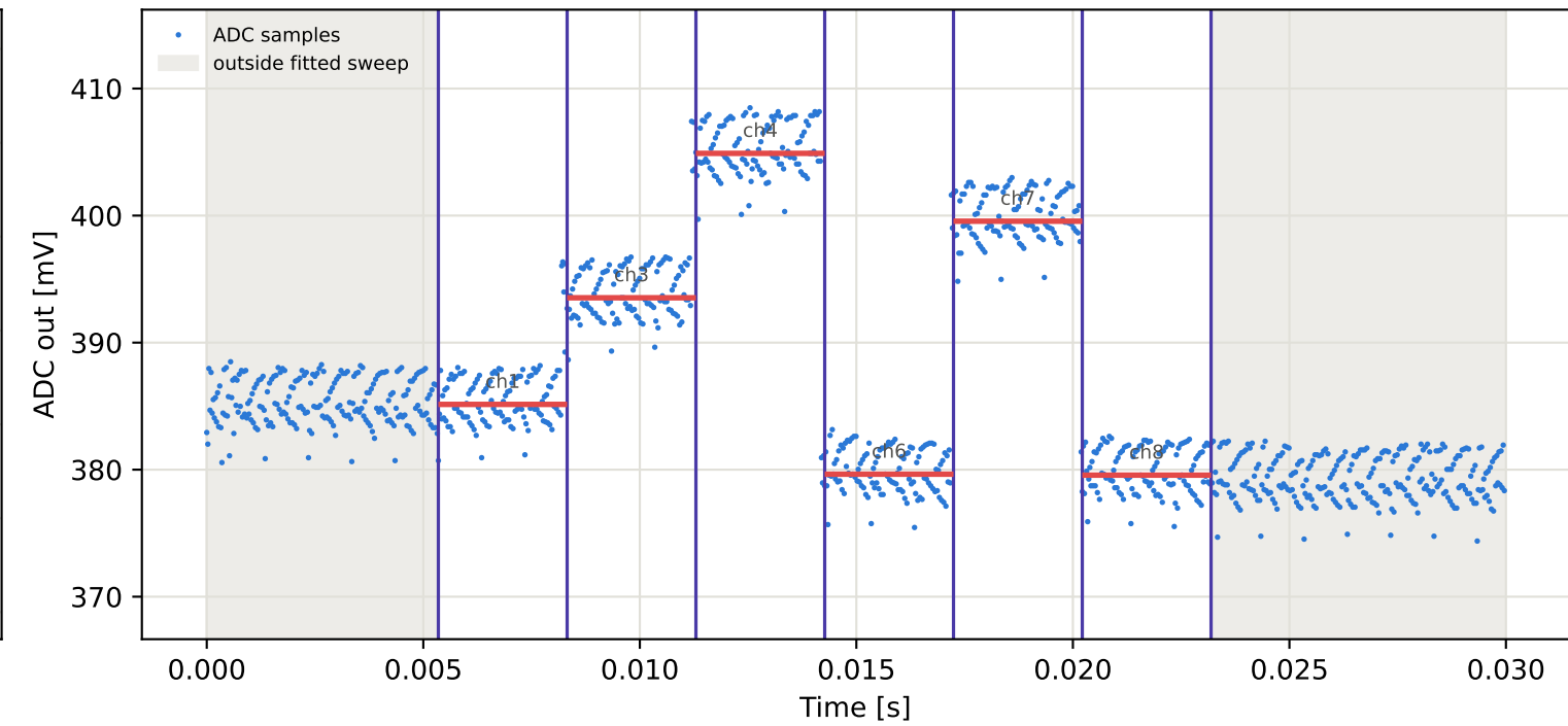
Tag5 &lt;- Tag1 | 975 MHz | run 0 | rep 1 | phase -47.15 deg
