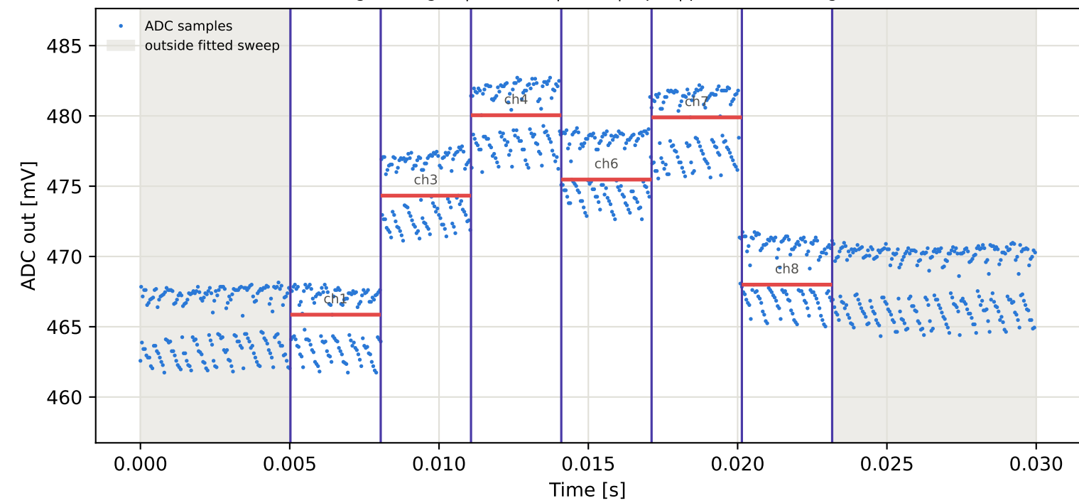
Tag4 &lt;- Tag16 | 865 MHz | run 0 | rep 1 | phase -8.95 deg
