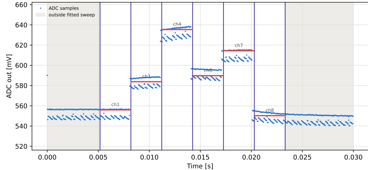
Tag15 &lt;- Tag10 | 945 MHz | run 0 | rep 1 | phase -15.52 deg
