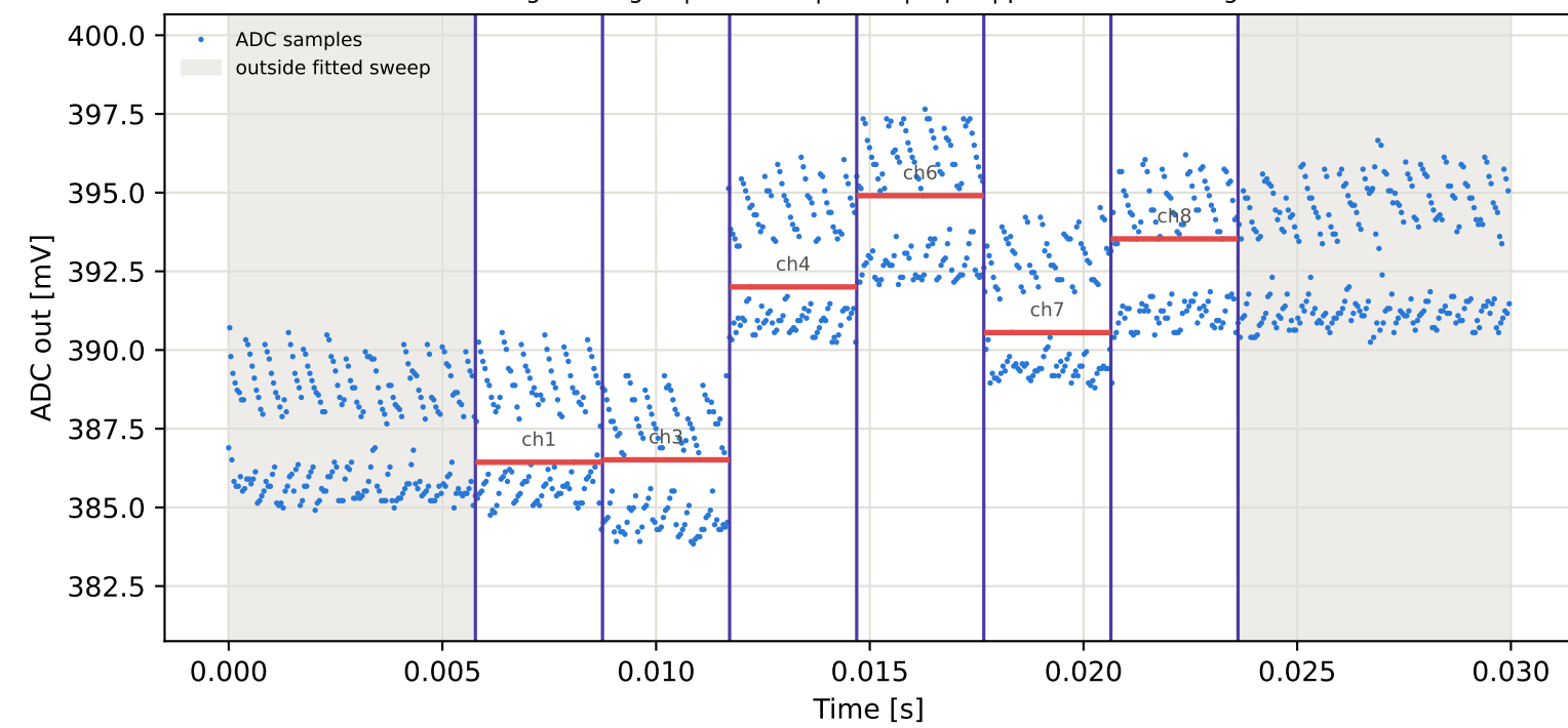
Tag6 &lt;- Tag3 | 845 MHz | run 0 | rep 1 | phase -135.64 deg
