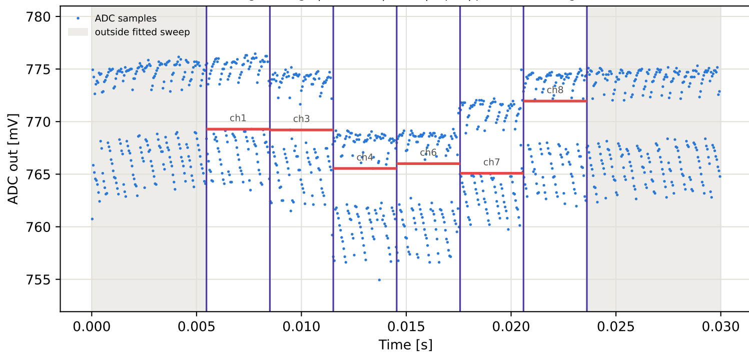
Tag5 &lt;- Tag8 | 945 MHz | run 0 | rep 1 | phase -65.38 deg
