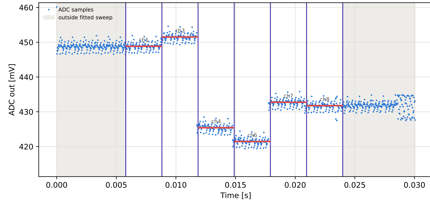
Tag3 &lt;- Tag8 | 825 MHz | run 0 | rep 1 | phase -134.53 deg
