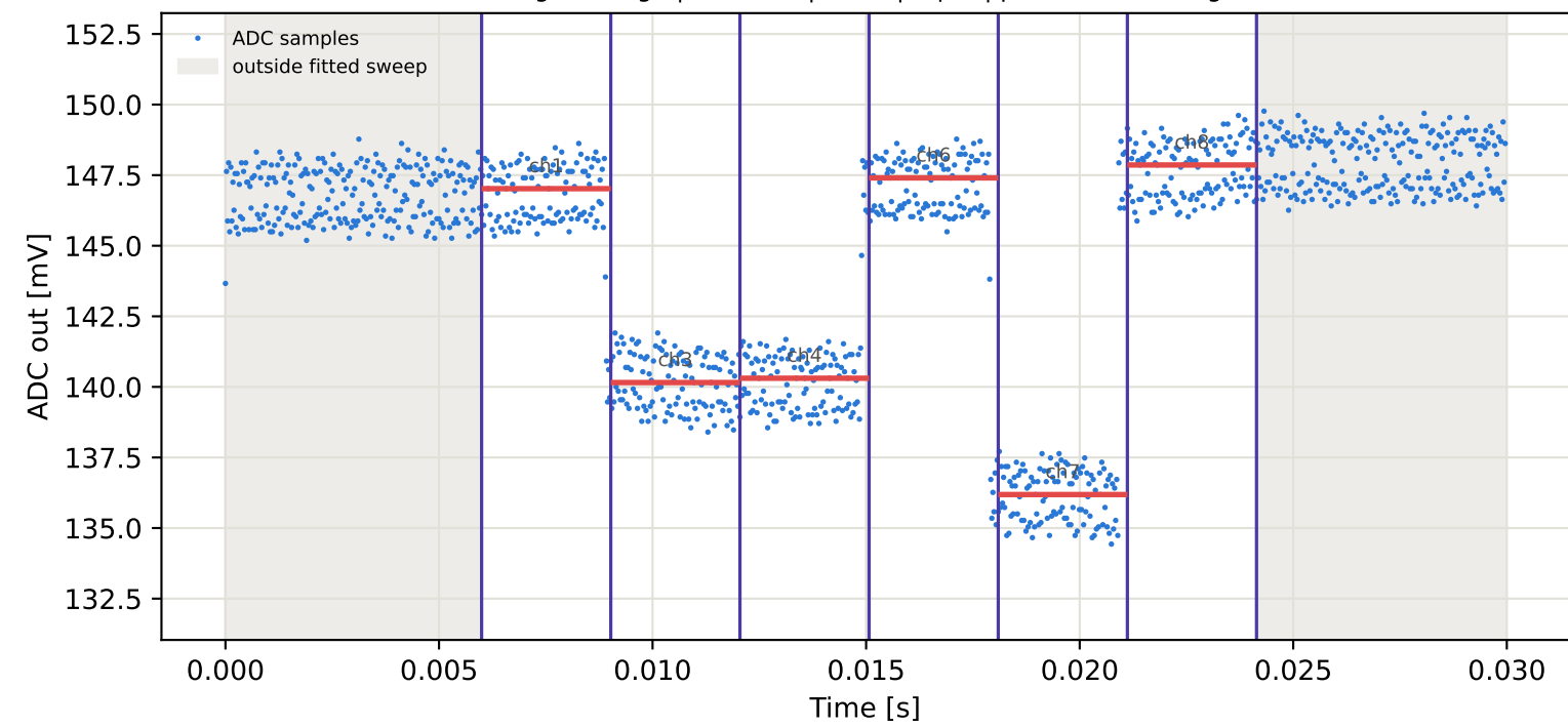
Tag5 &lt;- Tag4 | 785 MHz | run 0 | rep 1 | phase 146.23 deg
