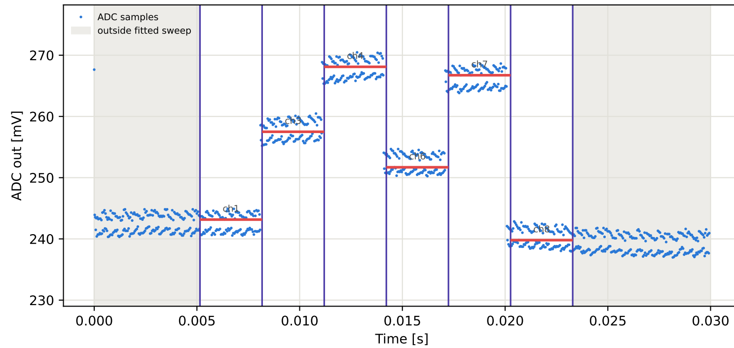
Tag6 &lt;- Tag9 | 835 MHz | run 0 | rep 1 | phase -158.44 deg
