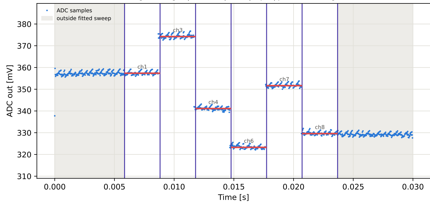
Tag15 &lt;- Tag3 | 845 MHz | run 0 | rep 1 | phase -10.85 deg
