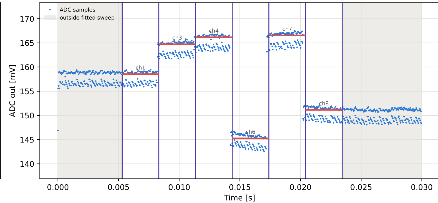
Tag10 &lt;- Tag1 | 975 MHz | run 0 | rep 1 | phase -79.29 deg
