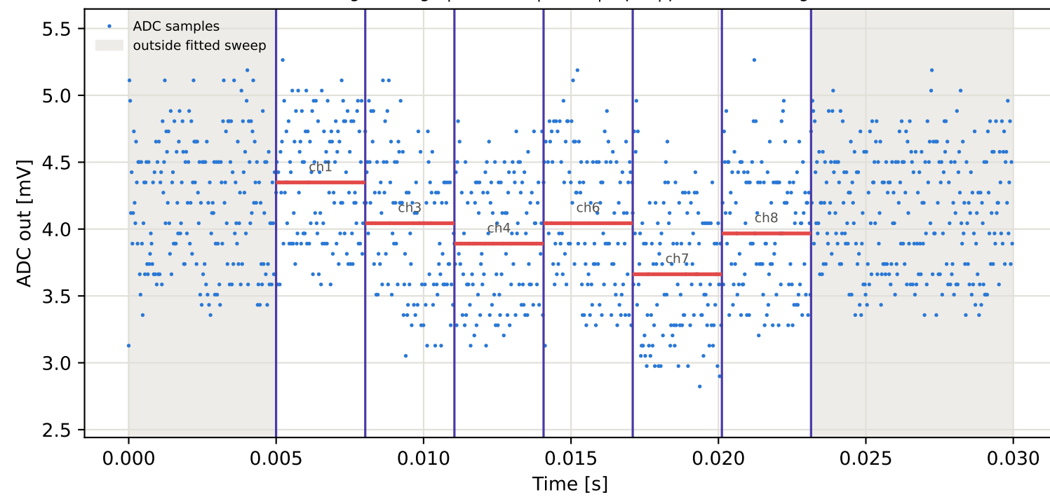
Tag1 &lt;- Tag3 | 785 MHz | run 0 | rep 1 | phase 99.73 deg
