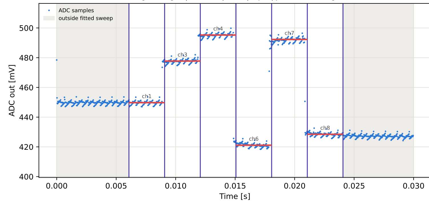
Tag7 &lt;- Tag3 | 995 MHz | run 0 | rep 1 | phase 150.98 deg
