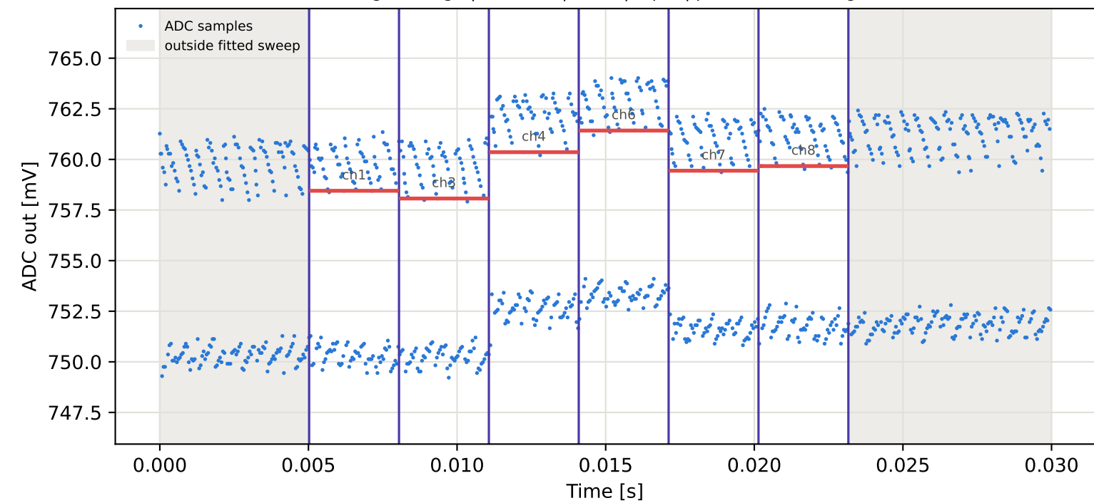
Tag8 &lt;- Tag4 | 835 MHz | run 0 | rep 1 | phase -46.62 deg
