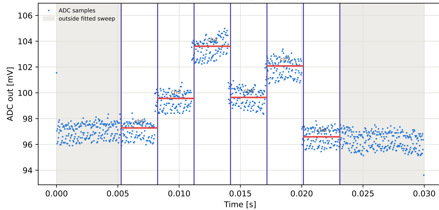
Tag1 &lt;- Tag9 | 945 MHz | run 0 | rep 1 | phase -95.12 deg
