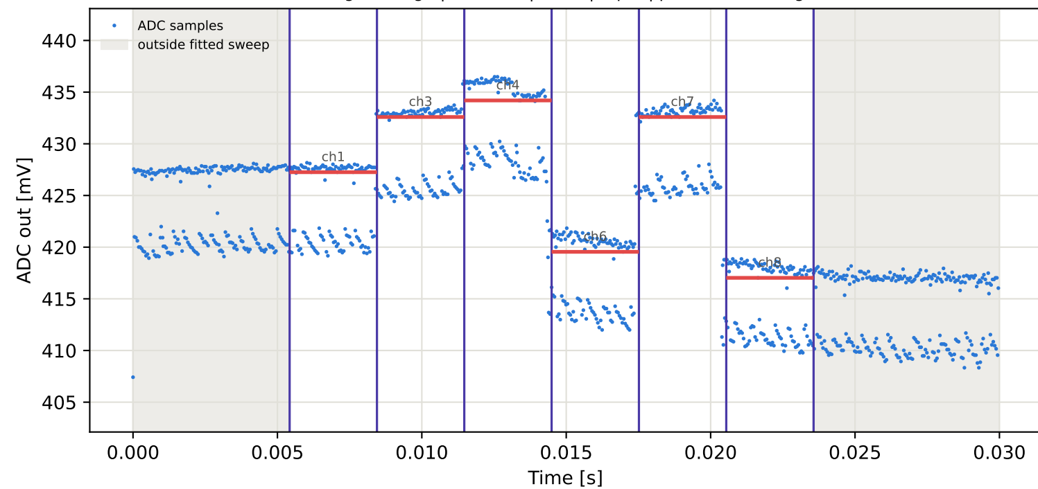
Tag2 &lt;- Tag8 | 905 MHz | run 0 | rep 1 | phase 133.84 deg
