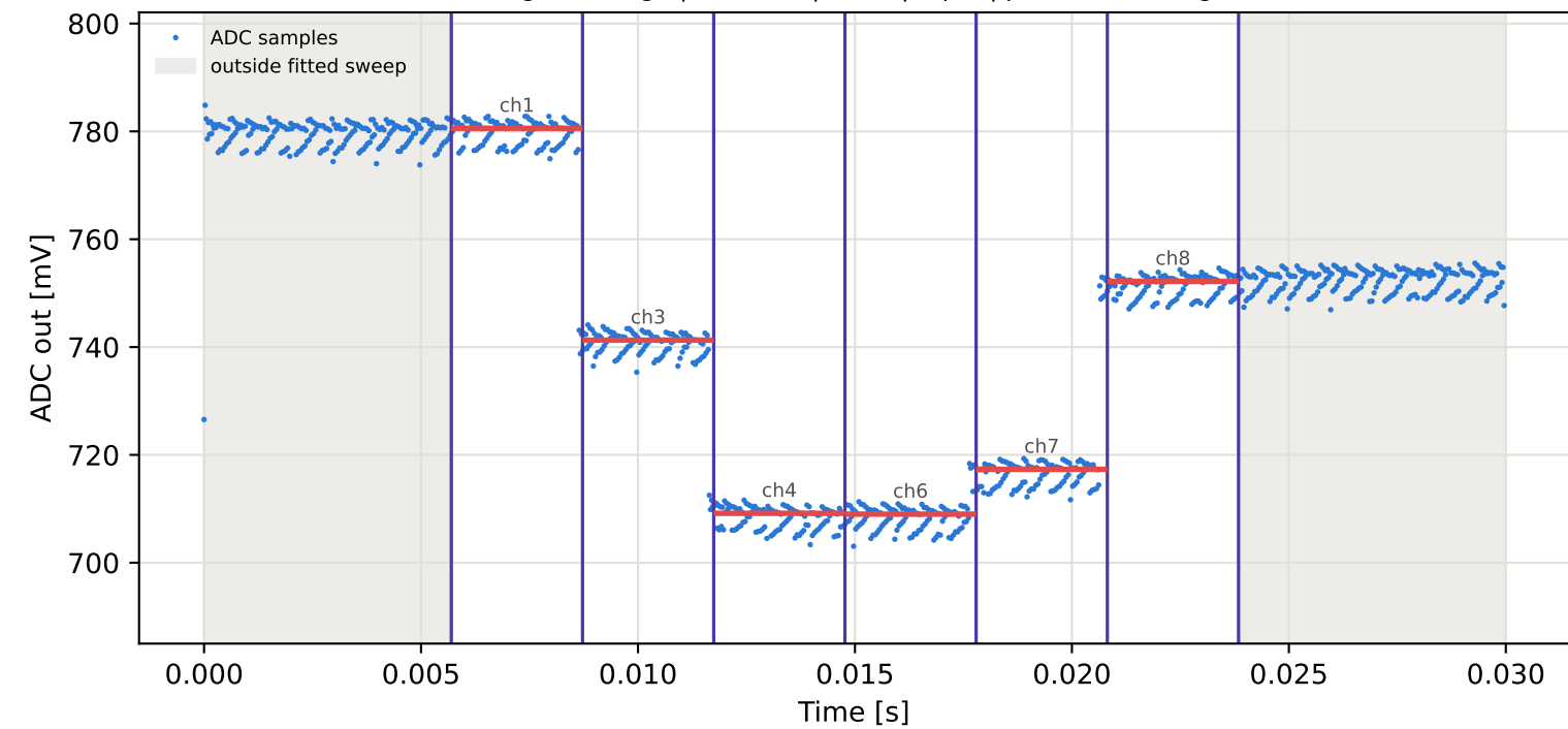
Tag16 &lt;- Tag5 | 865 MHz | run 0 | rep 1 | phase 27.85 deg
