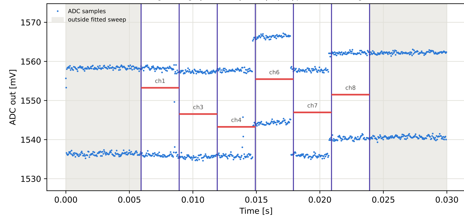
Tag8 &lt;- Tag4 | 905 MHz | run 0 | rep 1 | phase -22.75 deg
