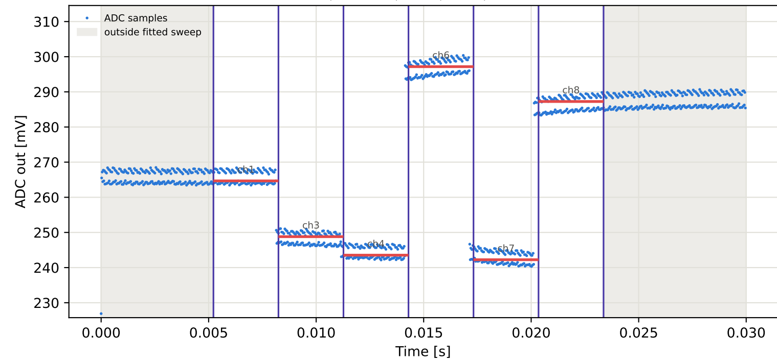
Tag3 &lt;- Tag9 | 965 MHz | run 0 | rep 1 | phase 150.90 deg
