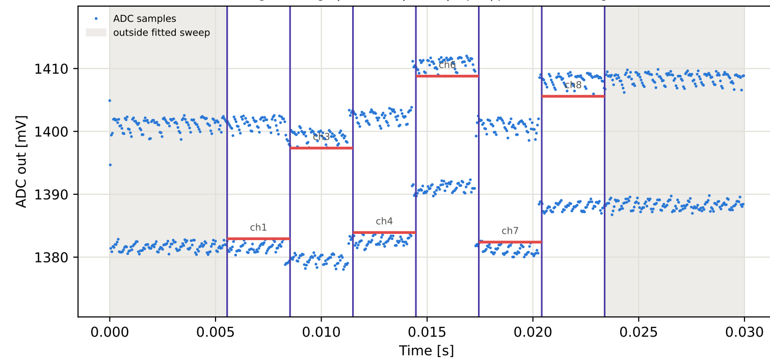
Tag15 &lt;- Tag9 | 915 MHz | run 0 | rep 1 | phase -94.98 deg
