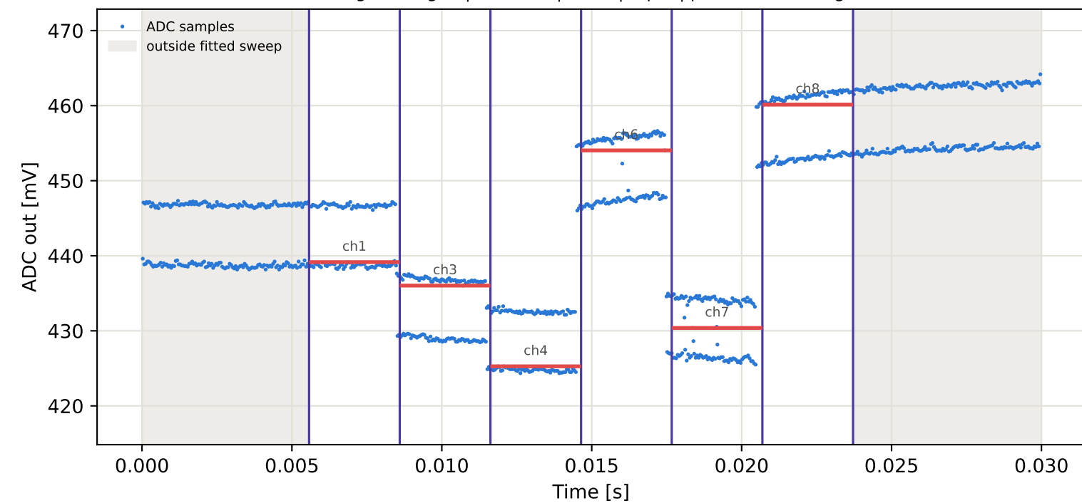
Tag7 &lt;- Tag10 | 905 MHz | run 0 | rep 1 | phase 137.71 deg
