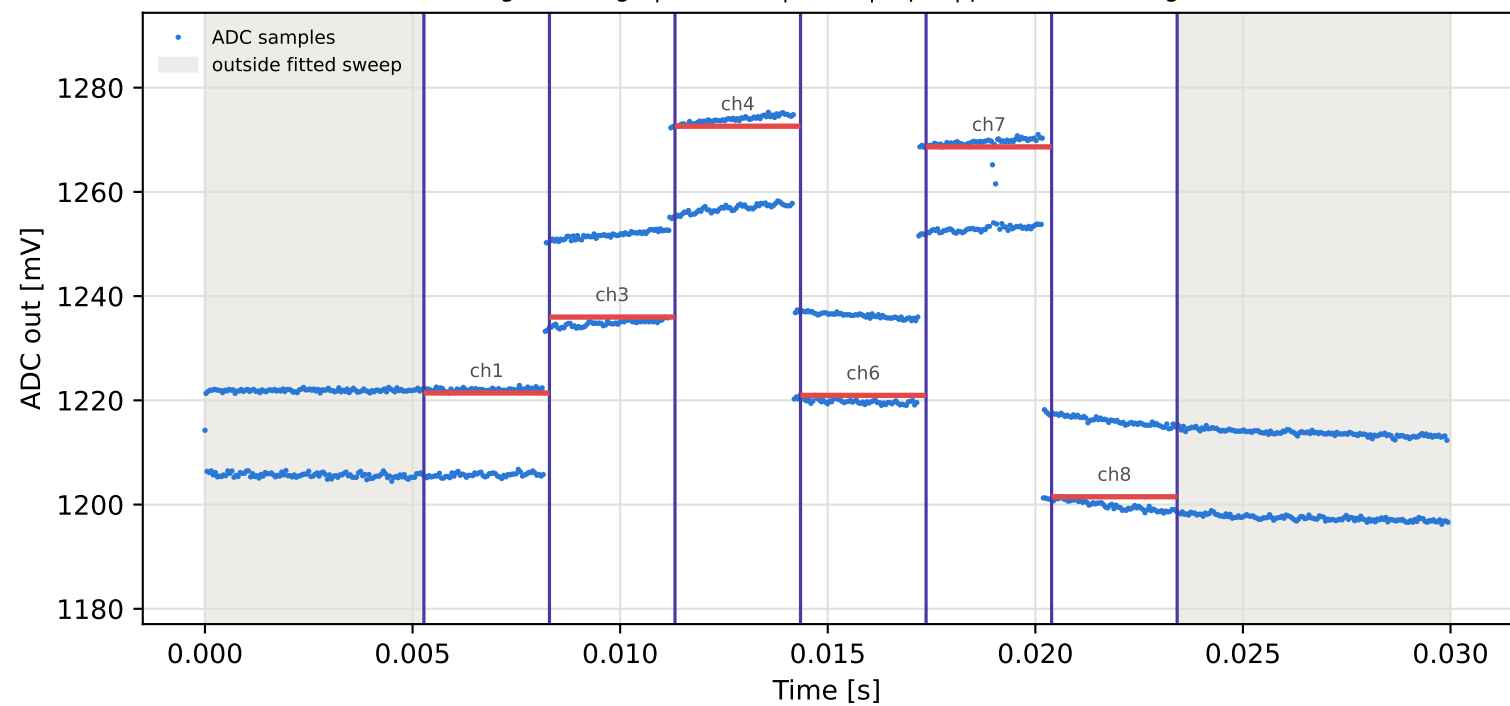
Tag16 &lt;- Tag7 | 895 MHz | run 0 | rep 1 | phase -74.03 deg
