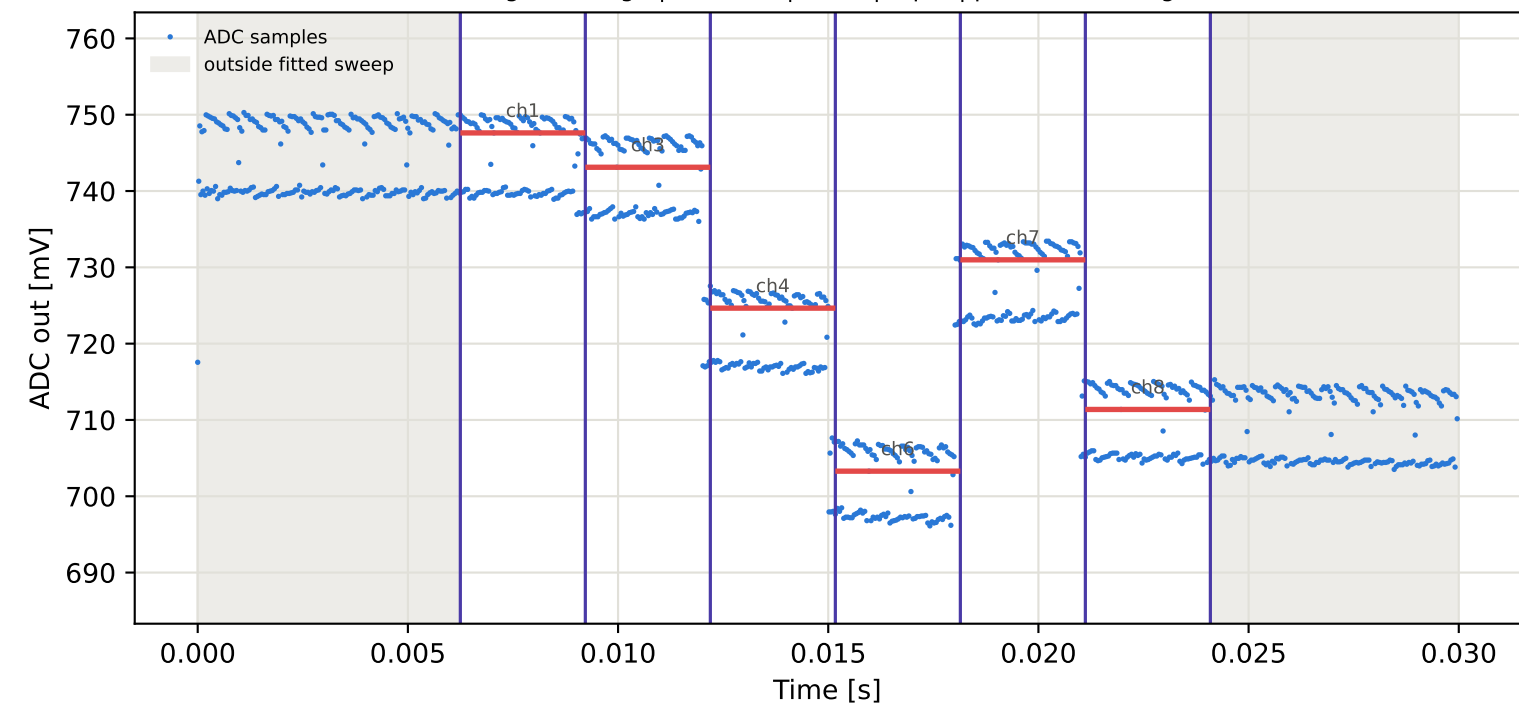
Tag16 &lt;- Tag7 | 865 MHz | run 0 | rep 1 | phase -121.92 deg
