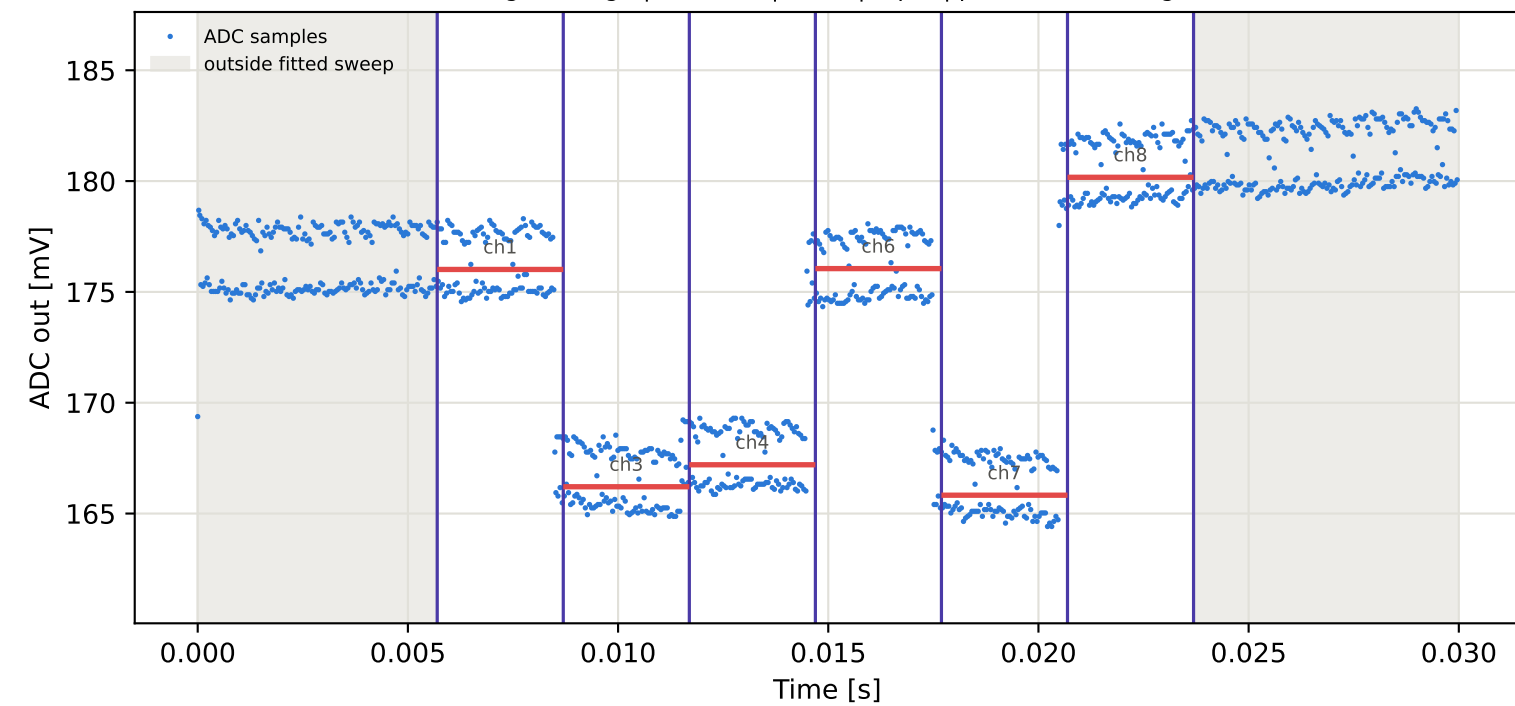
Tag9 &lt;- Tag15 | 865 MHz | run 0 | rep 1 | phase -158.78 deg
