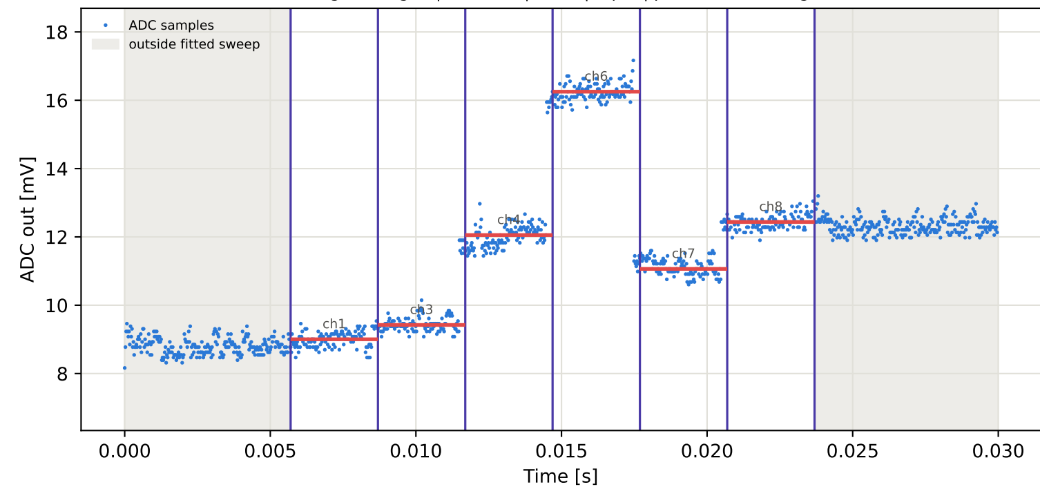
Tag1 &lt;- Tag2 | 905 MHz | run 0 | rep 1 | phase -168.62 deg
