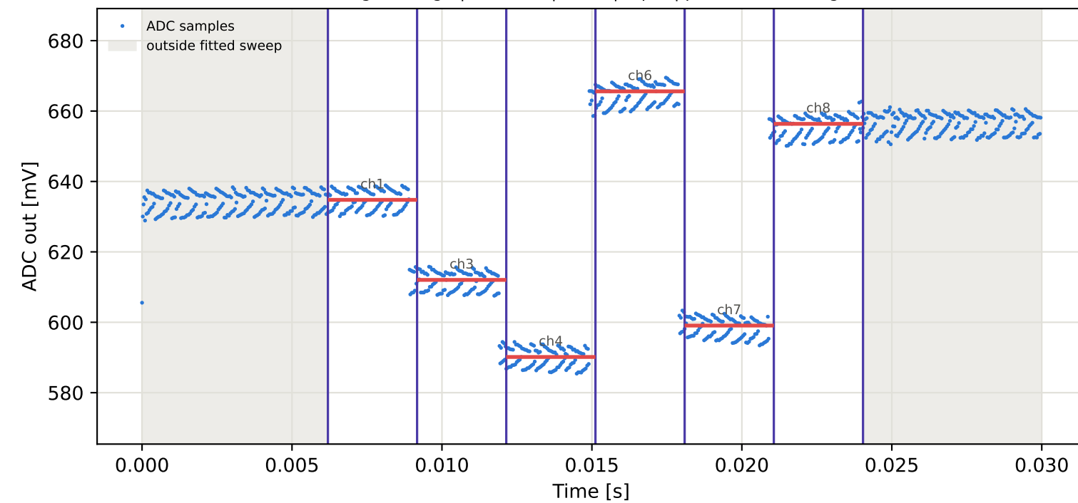
Tag8 &lt;- Tag1 | 965 MHz | run 0 | rep 1 | phase -106.68 deg
