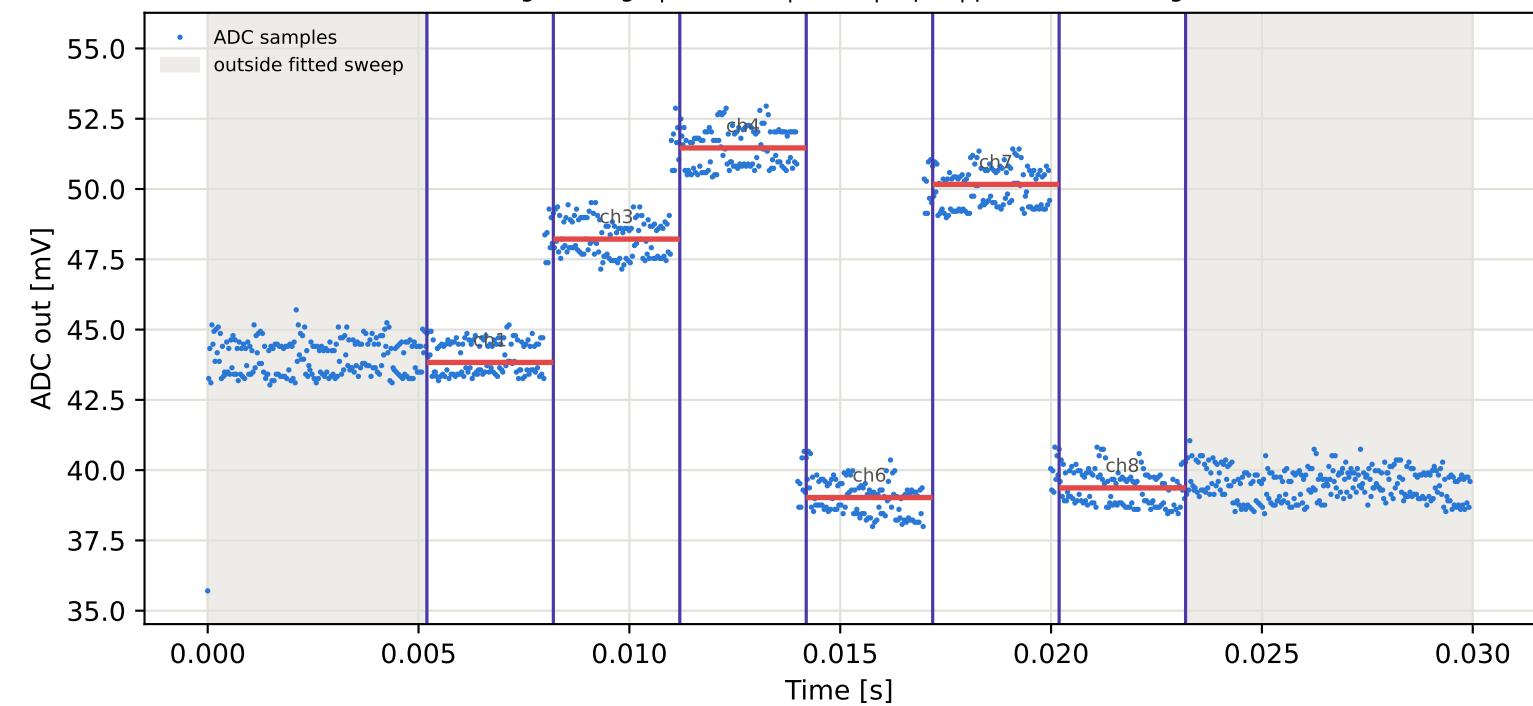
Tag6 &lt;- Tag4 | 945 MHz | run 0 | rep 1 | phase -44.24 deg
