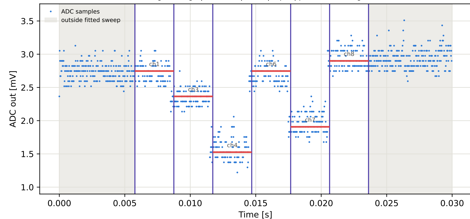
Tag2 &lt;- Tag7 | 965 MHz | run 0 | rep 1 | phase -14.05 deg
