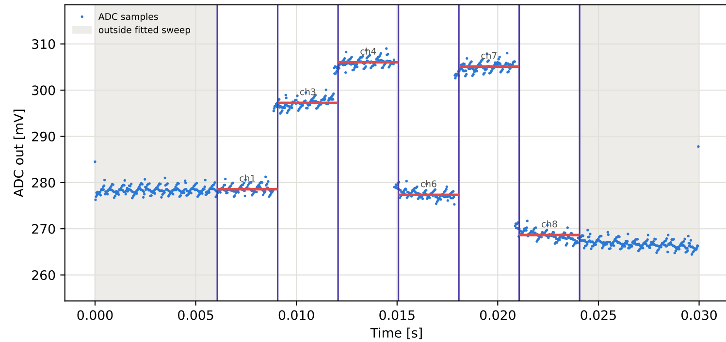
Tag10 &lt;- Tag9 | 905 MHz | run 0 | rep 1 | phase -130.00 deg
