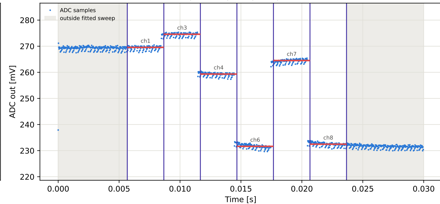
Tag1 &lt;- Tag4 | 865 MHz | run 0 | rep 1 | phase 12.68 deg
