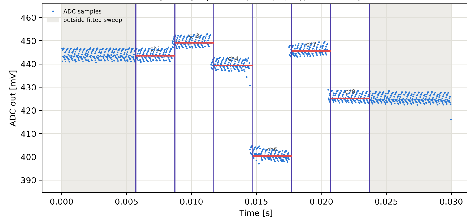
Tag3 &lt;- Tag16 | 945 MHz | run 0 | rep 1 | phase -104.98 deg
