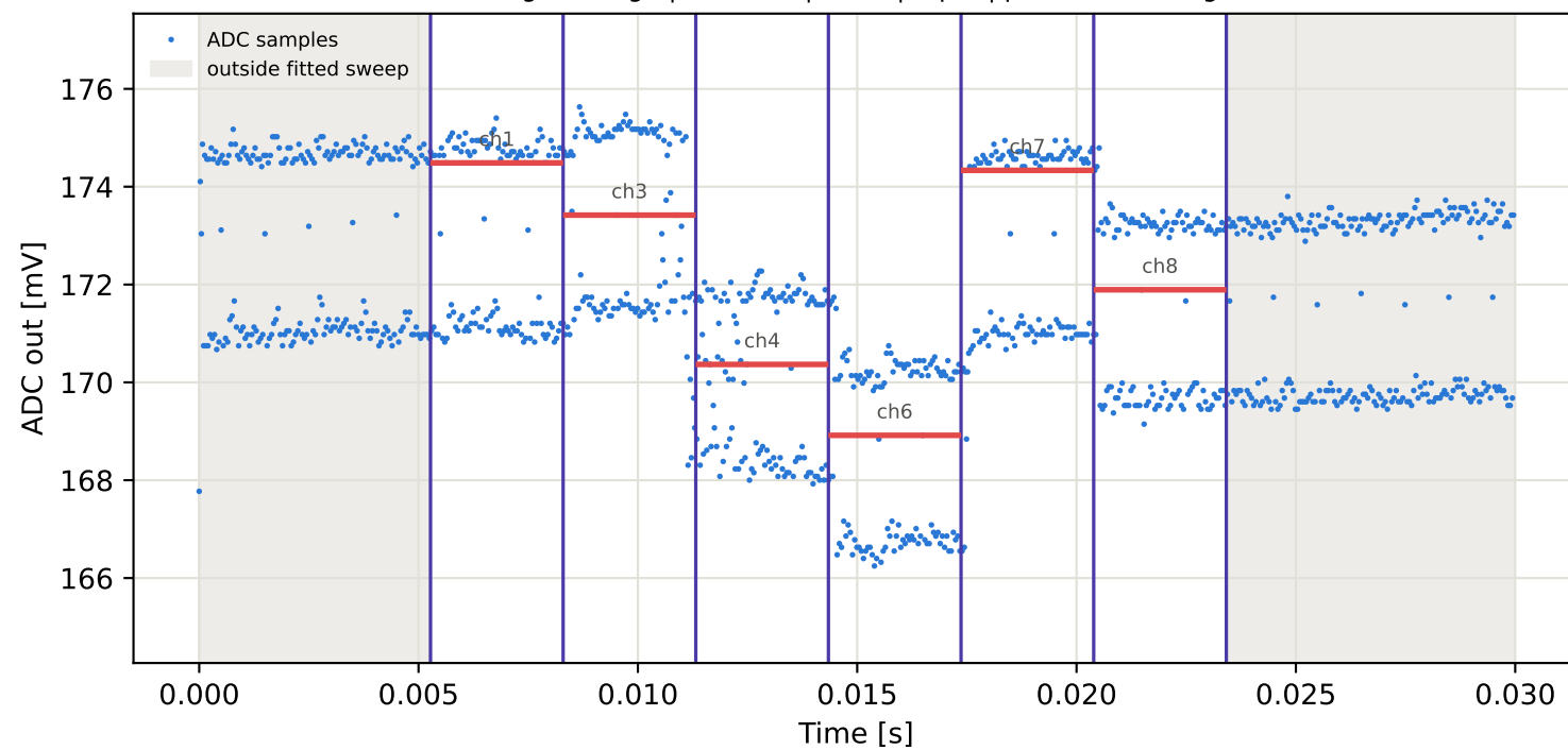
Tag1 &lt;- Tag3 | 995 MHz | run 0 | rep 1 | phase 24.74 deg
