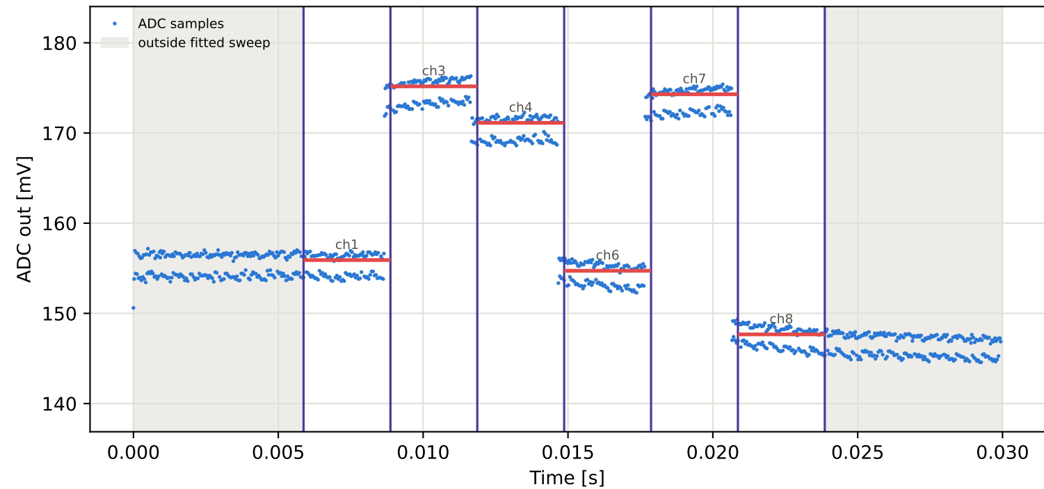
Tag2 &lt;- Tag8 | 845 MHz | run 0 | rep 1 | phase 66.17 deg
