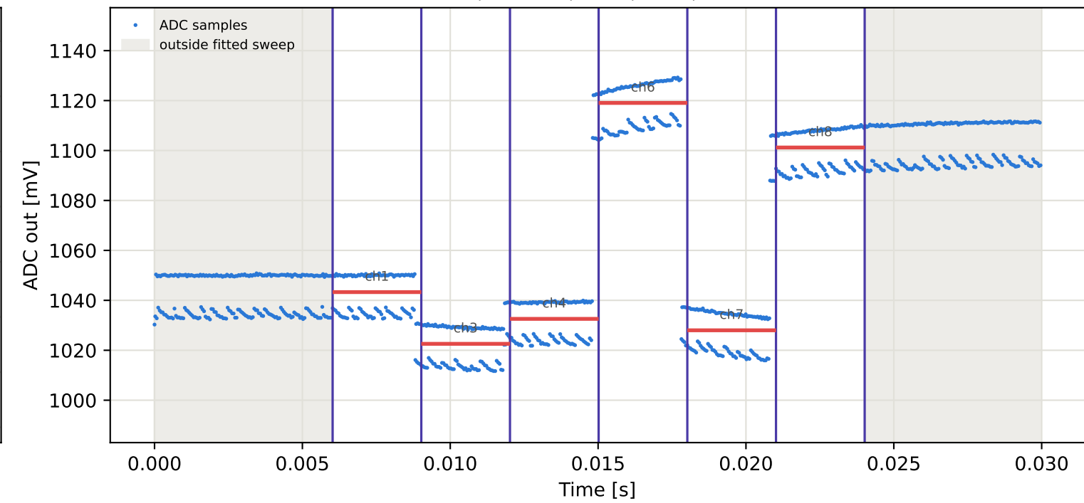
Tag16 &lt;- Tag15 | 915 MHz | run 0 | rep 1 | phase 174.91 deg
