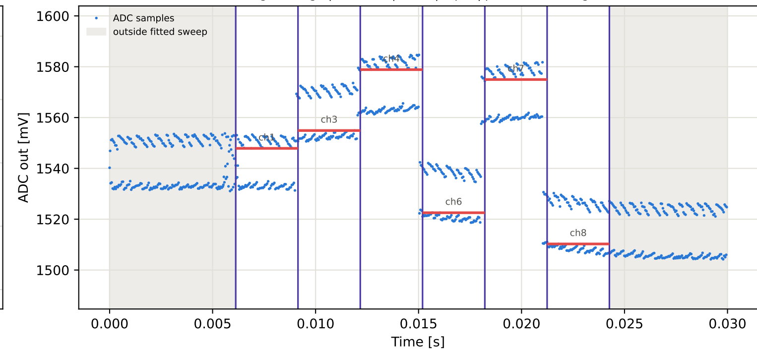
Tag8 &lt;- Tag5 | 905 MHz | run 0 | rep 1 | phase 109.57 deg
