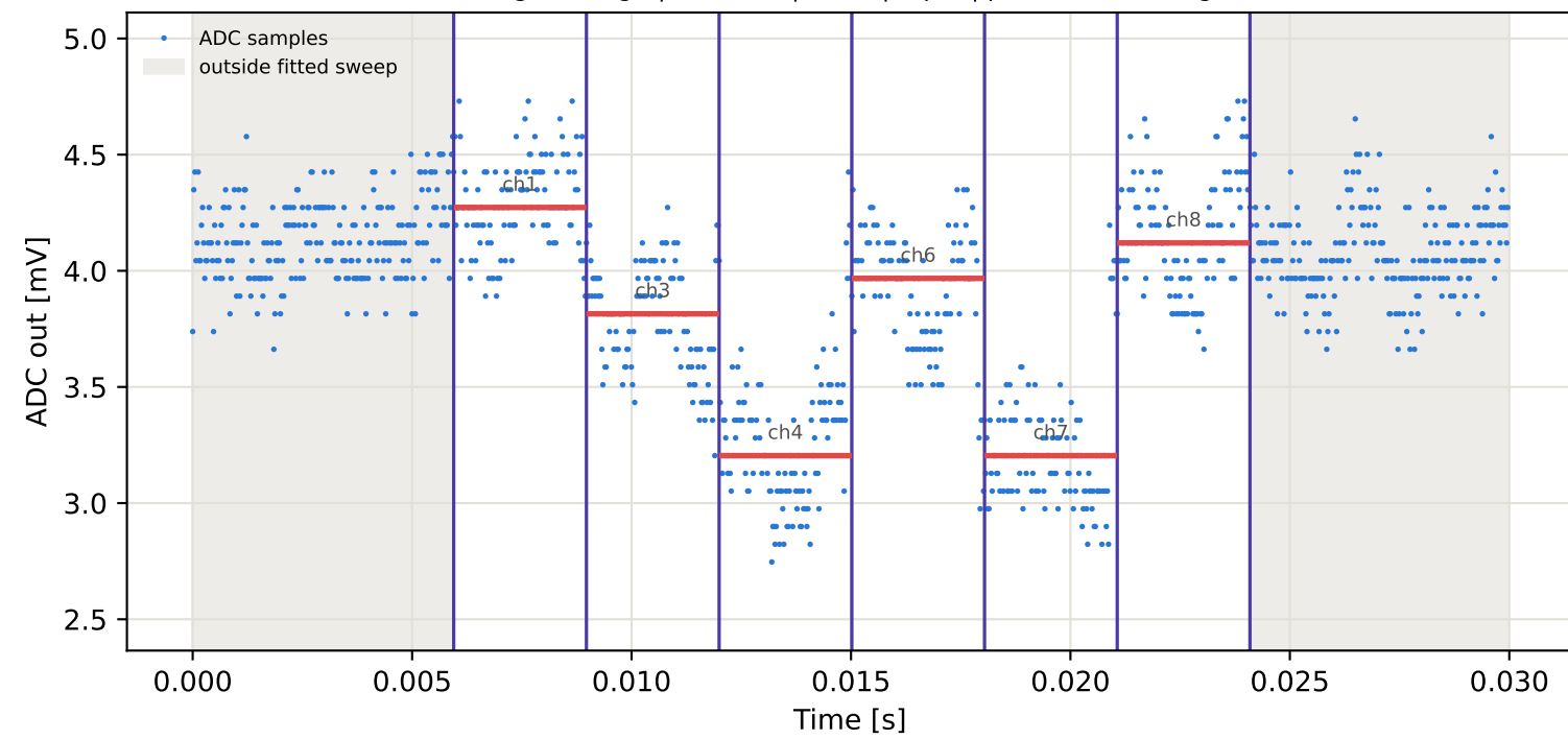
Tag2 &lt;- Tag6 | 785 MHz | run 0 | rep 1 | phase 108.55 deg
