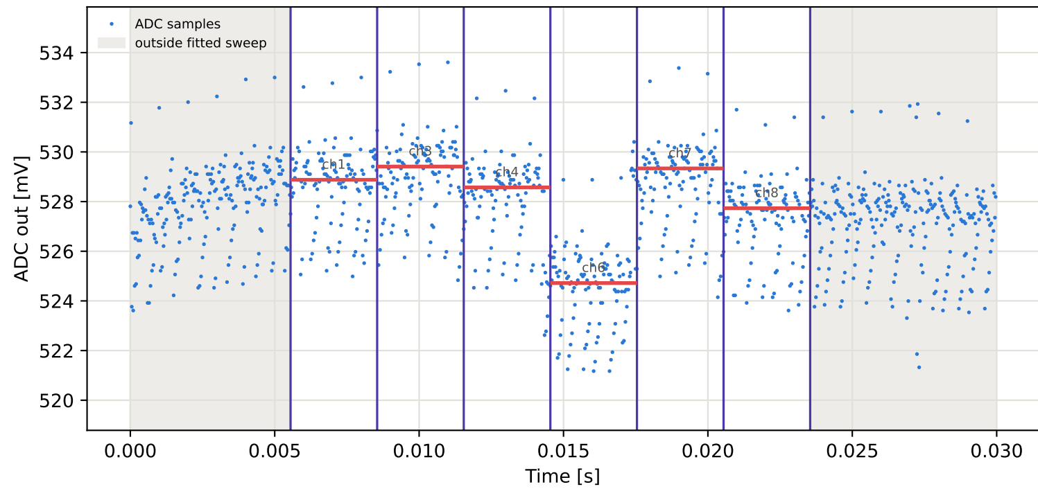
Tag2 &lt;- Tag5 | 915 MHz | run 0 | rep 1 | phase -89.75 deg
