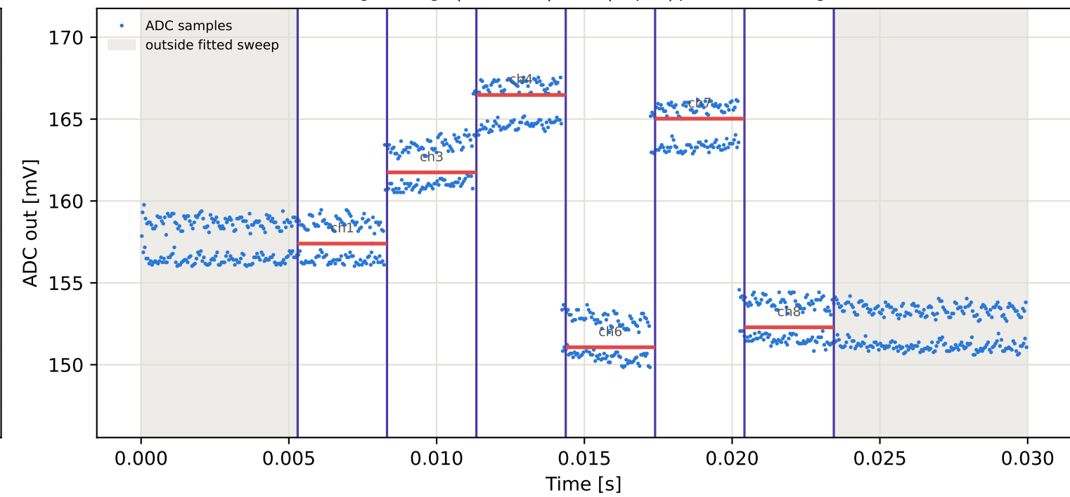
Tag4 &lt;- Tag8 | 935 MHz | run 0 | rep 1 | phase 16.90 deg
