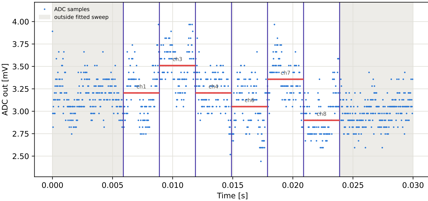
Tag2 &lt;- Tag7 | 785 MHz | run 0 | rep 1 | phase 6.23 deg
