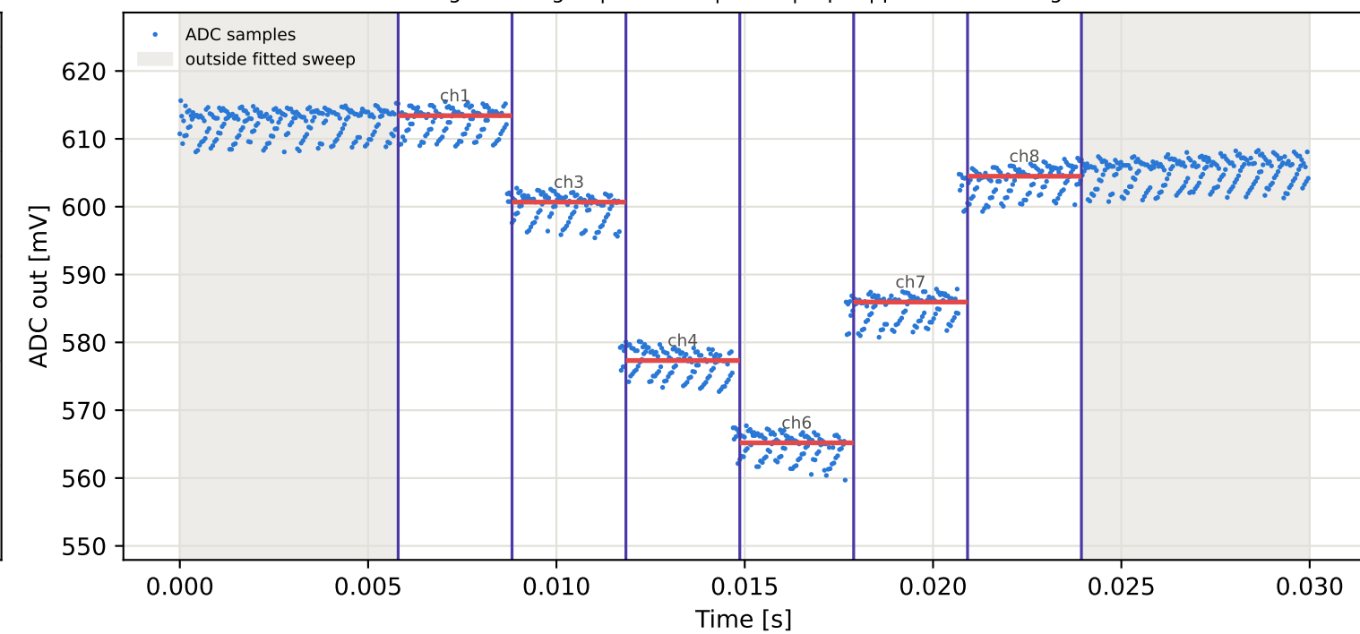
Tag10 &lt;- Tag3 | 915 MHz | run 0 | rep 1 | phase -139.38 deg
