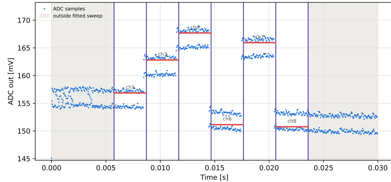
Tag1 &lt;- Tag9 | 975 MHz | run 0 | rep 1 | phase -38.21 deg
