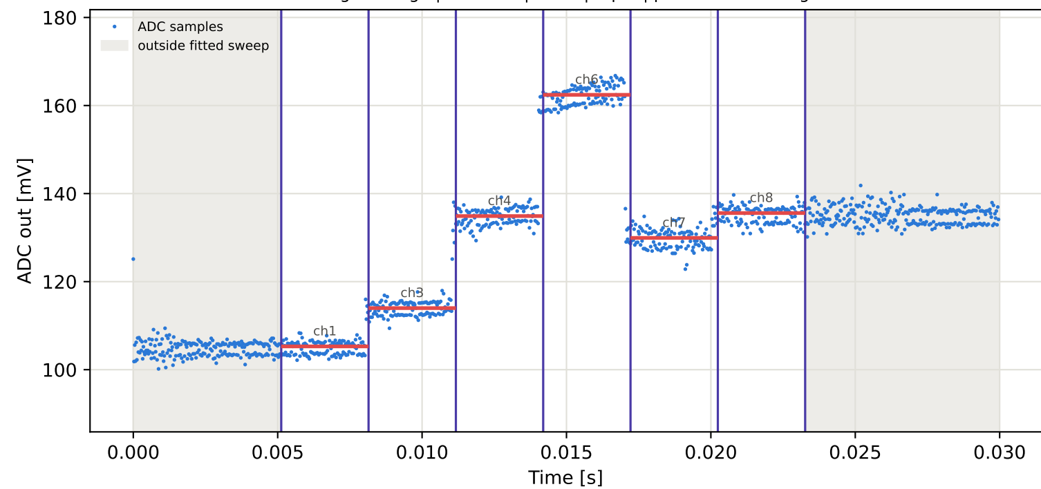
Tag4 &lt;- Tag8 | 885 MHz | run 0 | rep 1 | phase -101.44 deg
