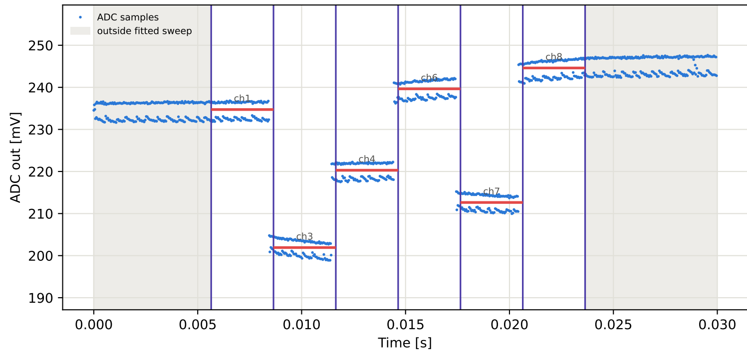
Tag2 &lt;- Tag5 | 835 MHz | run 0 | rep 1 | phase -106.80 deg
