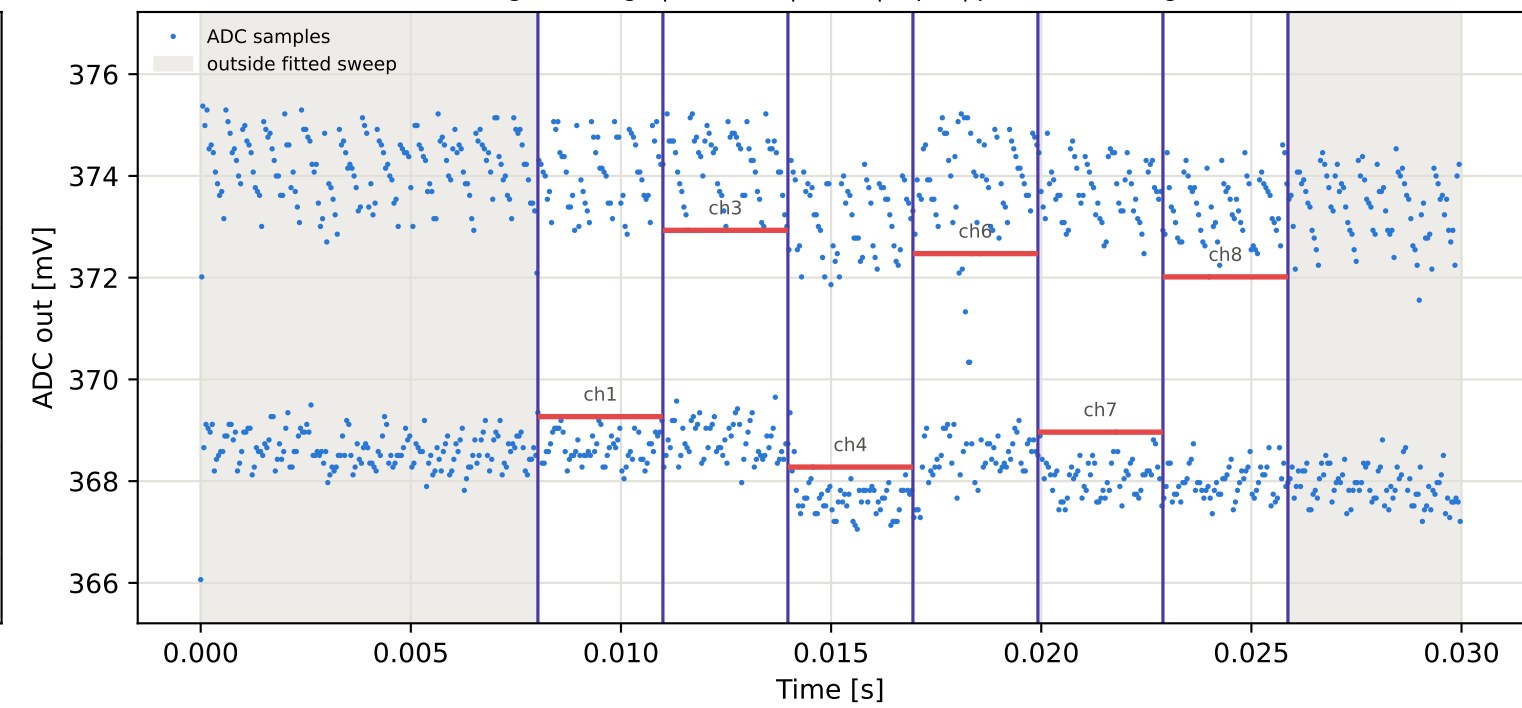
Tag15 &lt;- Tag4 | 995 MHz | run 0 | rep 1 | phase 146.96 deg
