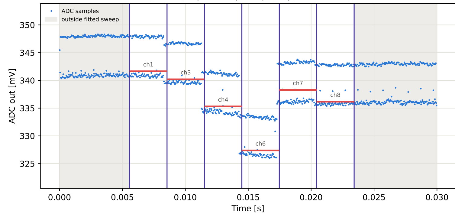
Tag1 &lt;- Tag2 | 925 MHz | run 0 | rep 1 | phase 178.85 deg
