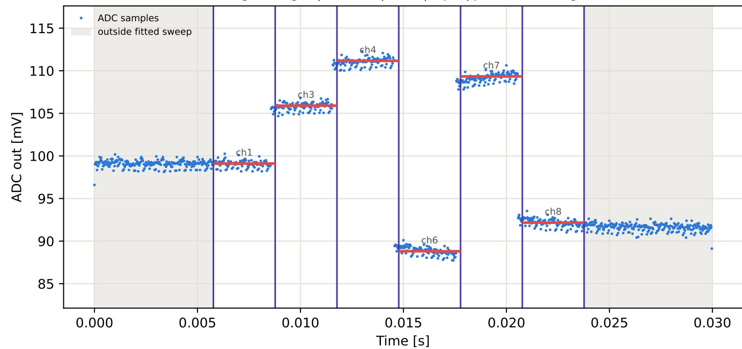
Tag1 &lt;- Tag16 | 965 MHz | run 0 | rep 1 | phase 15.82 deg
