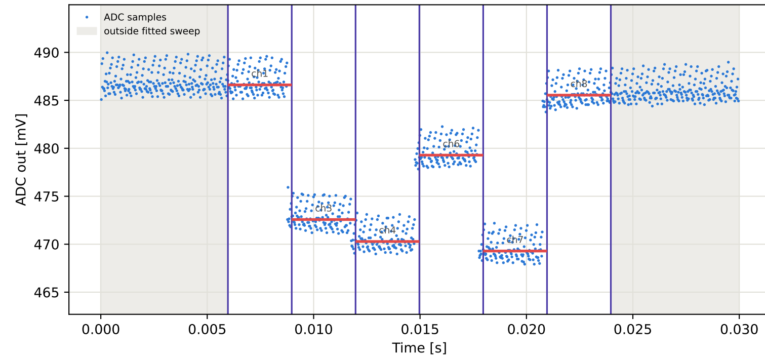
Tag3 &lt;- Tag16 | 845 MHz | run 0 | rep 1 | phase -165.92 deg
