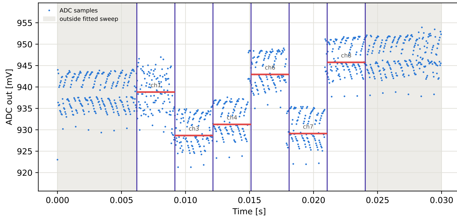
Tag16 &lt;- Tag10 | 875 MHz | run 0 | rep 1 | phase 162.07 deg
