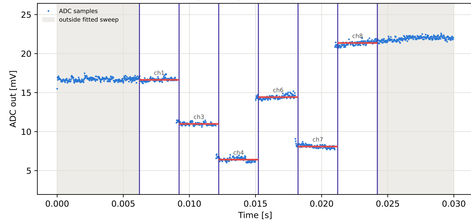
Tag1 &lt;- Tag3 | 905 MHz | run 0 | rep 1 | phase 103.36 deg
