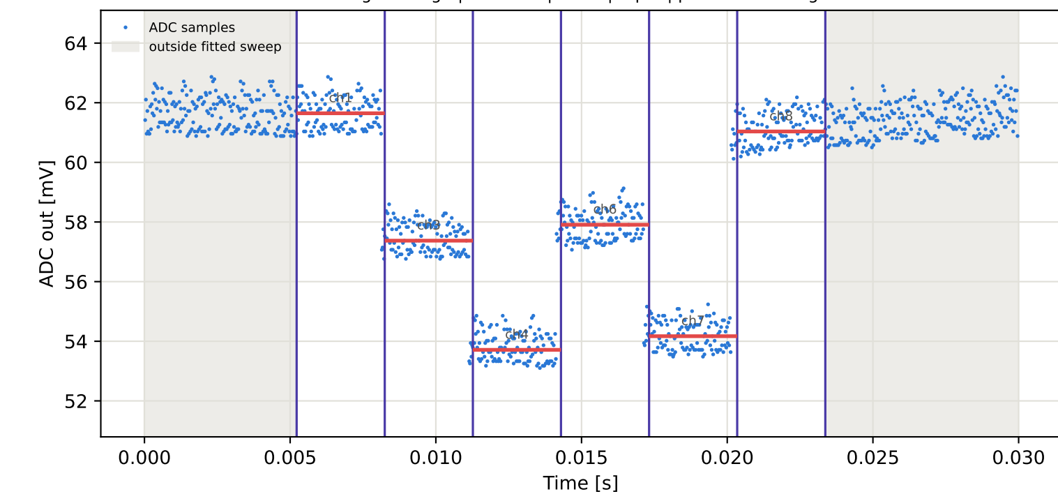
Tag1 &lt;- Tag9 | 845 MHz | run 0 | rep 1 | phase 97.81 deg
