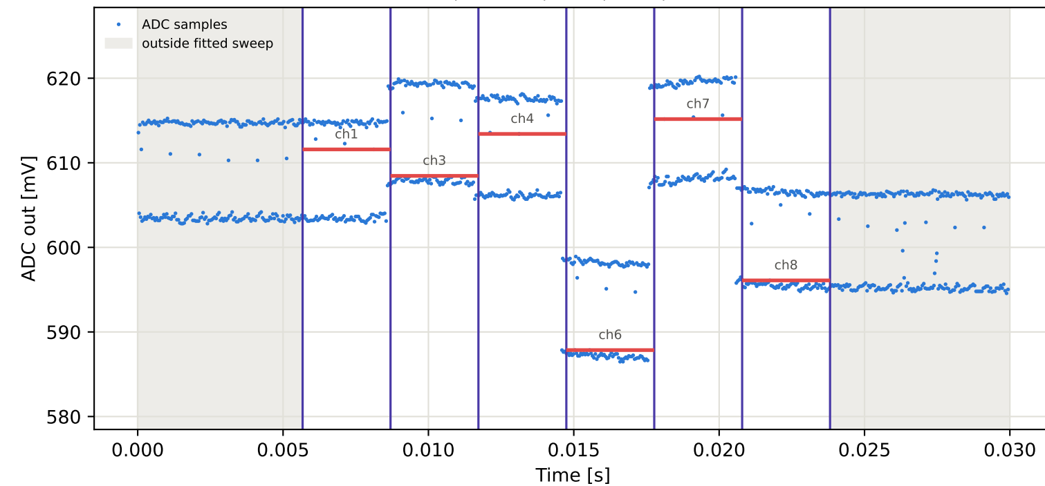
Tag7 &lt;- Tag10 | 965 MHz | run 0 | rep 1 | phase -14.02 deg
