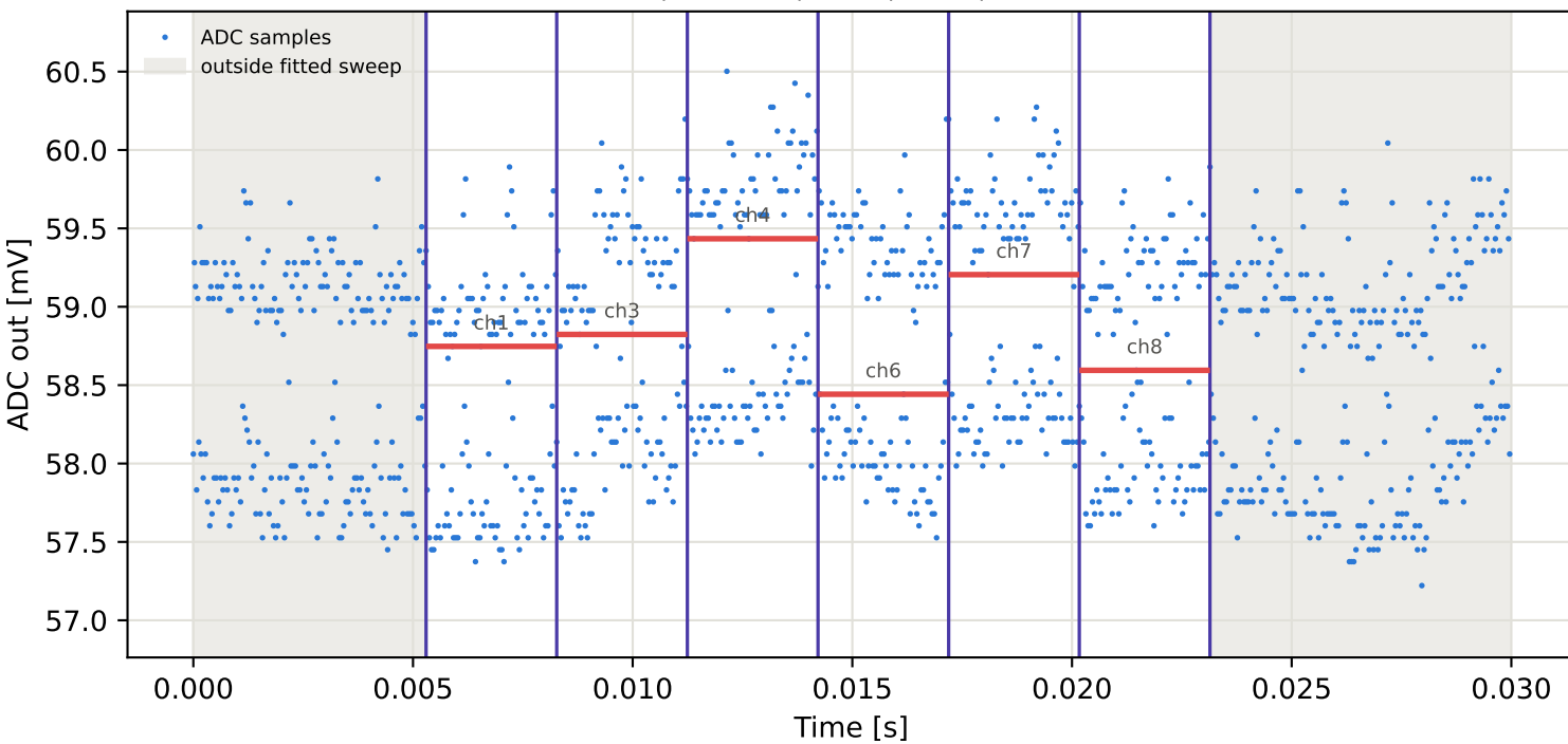
Tag6 &lt;- Tag1 | 785 MHz | run 0 | rep 1 | phase -47.69 deg
