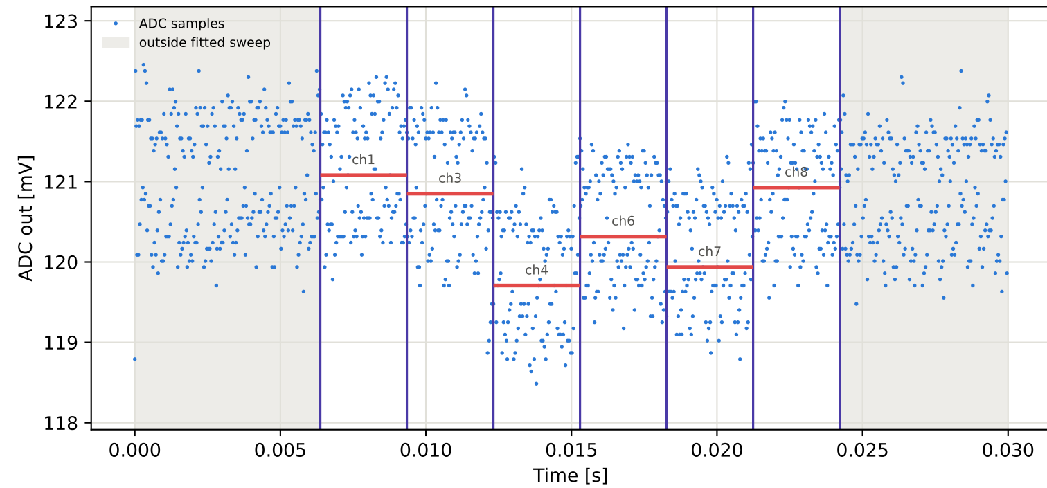
Tag7 &lt;- Tag15 | 795 MHz | run 0 | rep 1 | phase -137.70 deg
