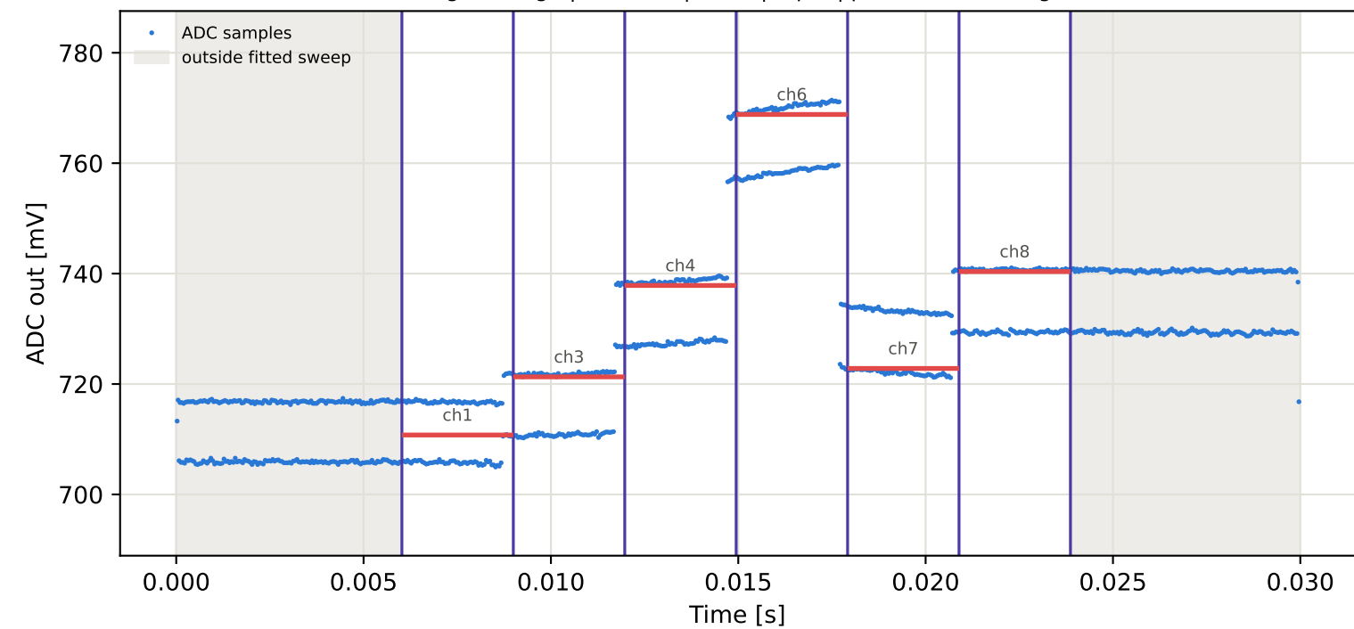
Tag9 &lt;- Tag8 | 895 MHz | run 0 | rep 1 | phase 23.74 deg
