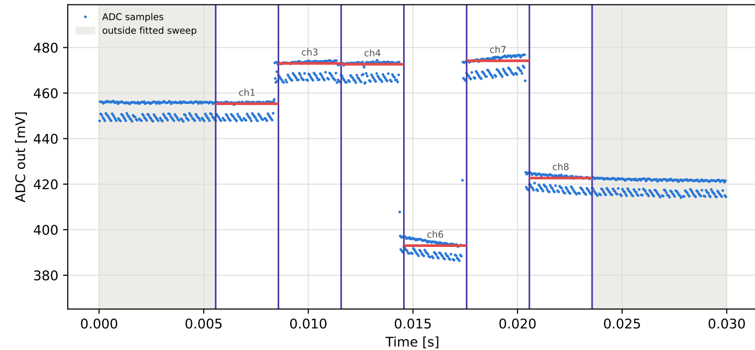
Tag3 &lt;- Tag16 | 935 MHz | run 0 | rep 1 | phase -84.45 deg
