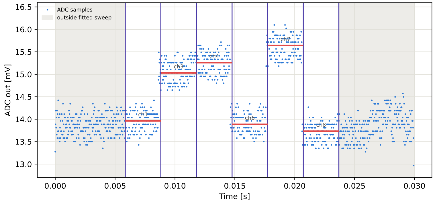
Tag2 &lt;- Tag8 | 795 MHz | run 0 | rep 1 | phase 146.79 deg
