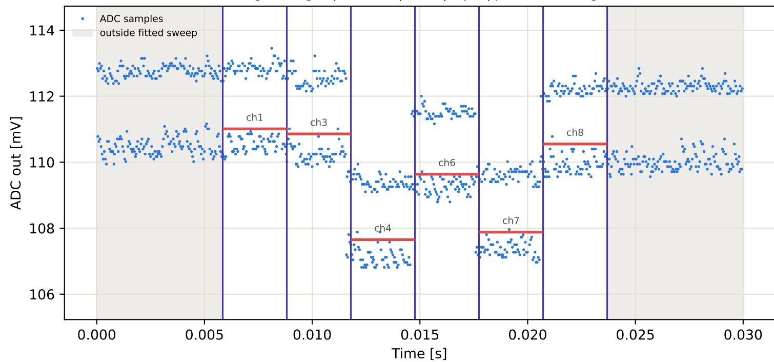
Tag4 &lt;- Tag16 | 775 MHz | run 0 | rep 1 | phase -148.21 deg
