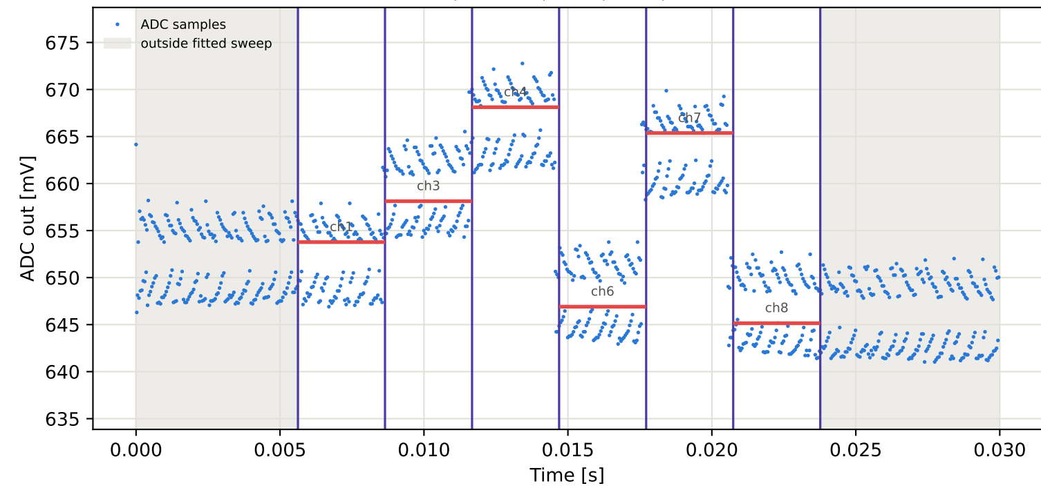
Tag16 &lt;- Tag15 | 965 MHz | run 0 | rep 1 | phase -58.25 deg
