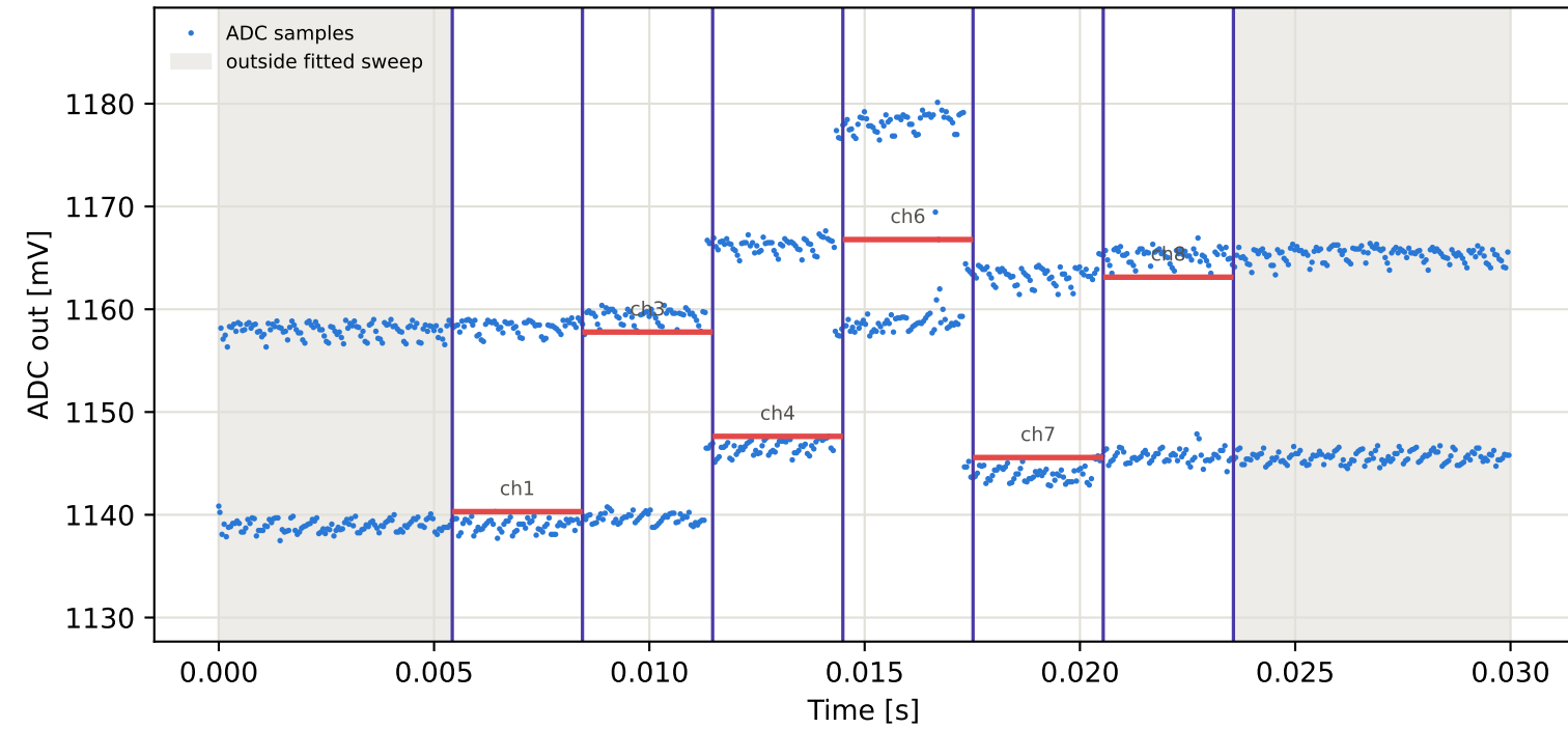
Tag8 &lt;- Tag16 | 925 MHz | run 0 | rep 1 | phase 124.27 deg
