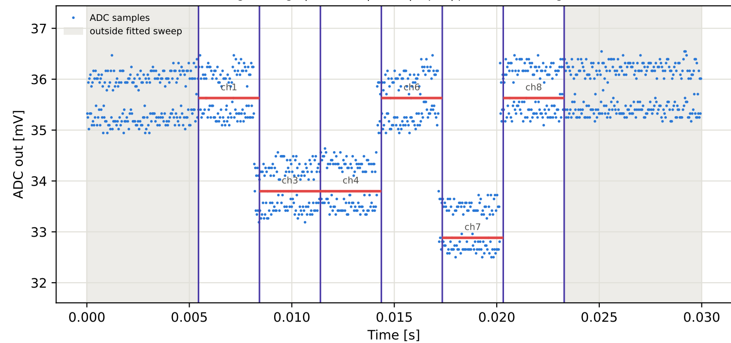
Tag2 &lt;- Tag5 | 805 MHz | run 0 | rep 1 | phase -116.04 deg
