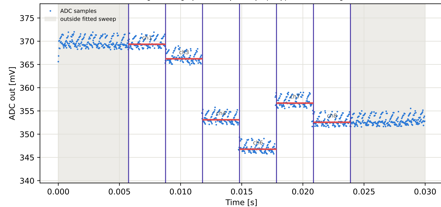
Tag15 &lt;- Tag5 | 855 MHz | run 0 | rep 1 | phase 41.33 deg
