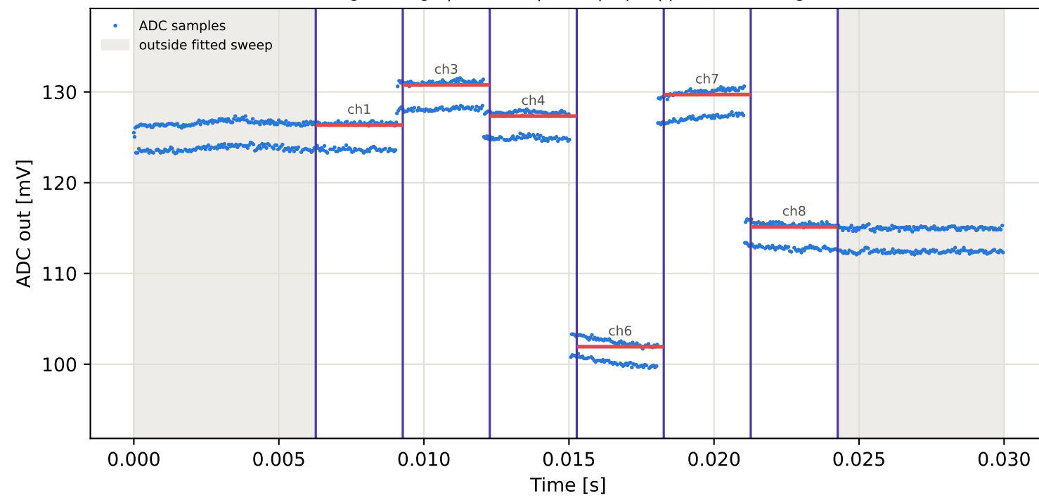
Tag2 &lt;- Tag5 | 945 MHz | run 0 | rep 1 | phase 39.09 deg
