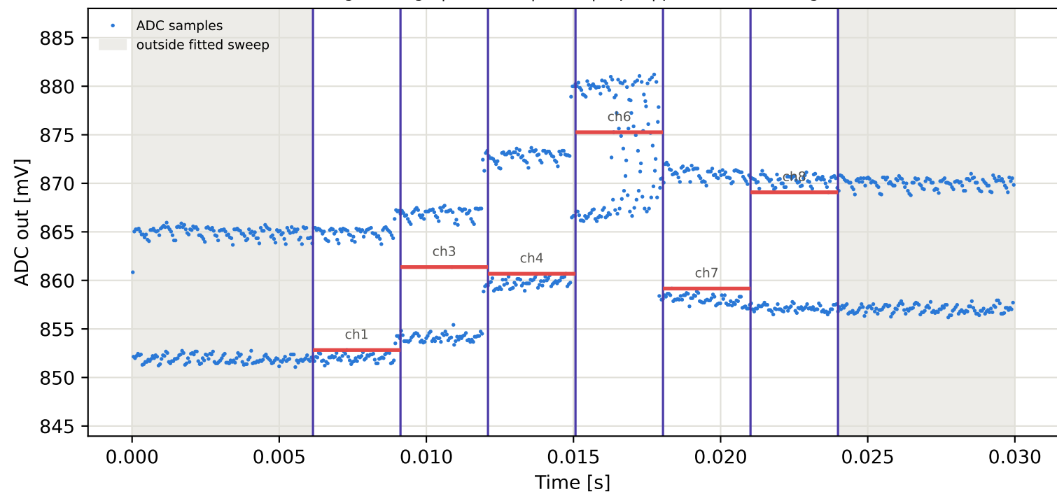
Tag9 &lt;- Tag6 | 905 MHz | run 0 | rep 1 | phase -166.19 deg
