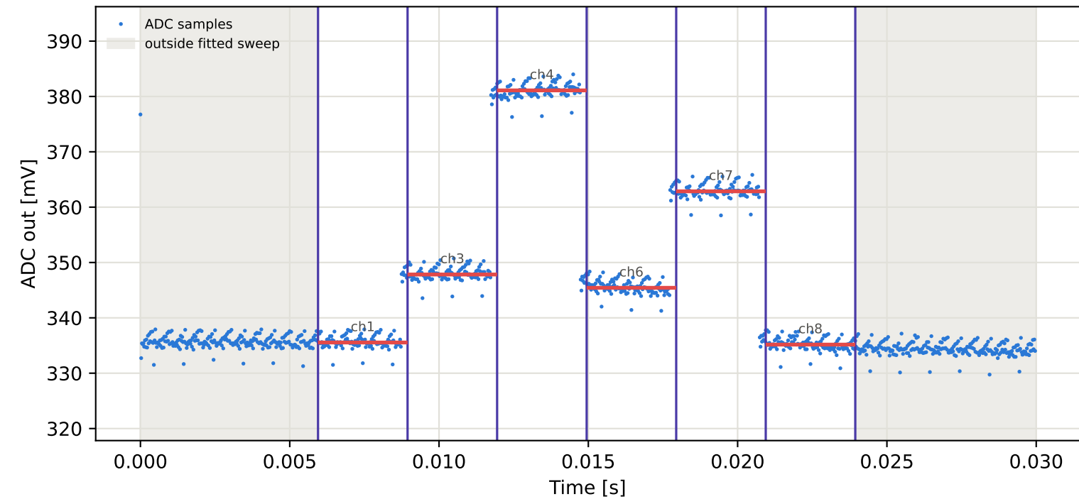
Tag9 &lt;- Tag8 | 985 MHz | run 0 | rep 1 | phase 7.99 deg
