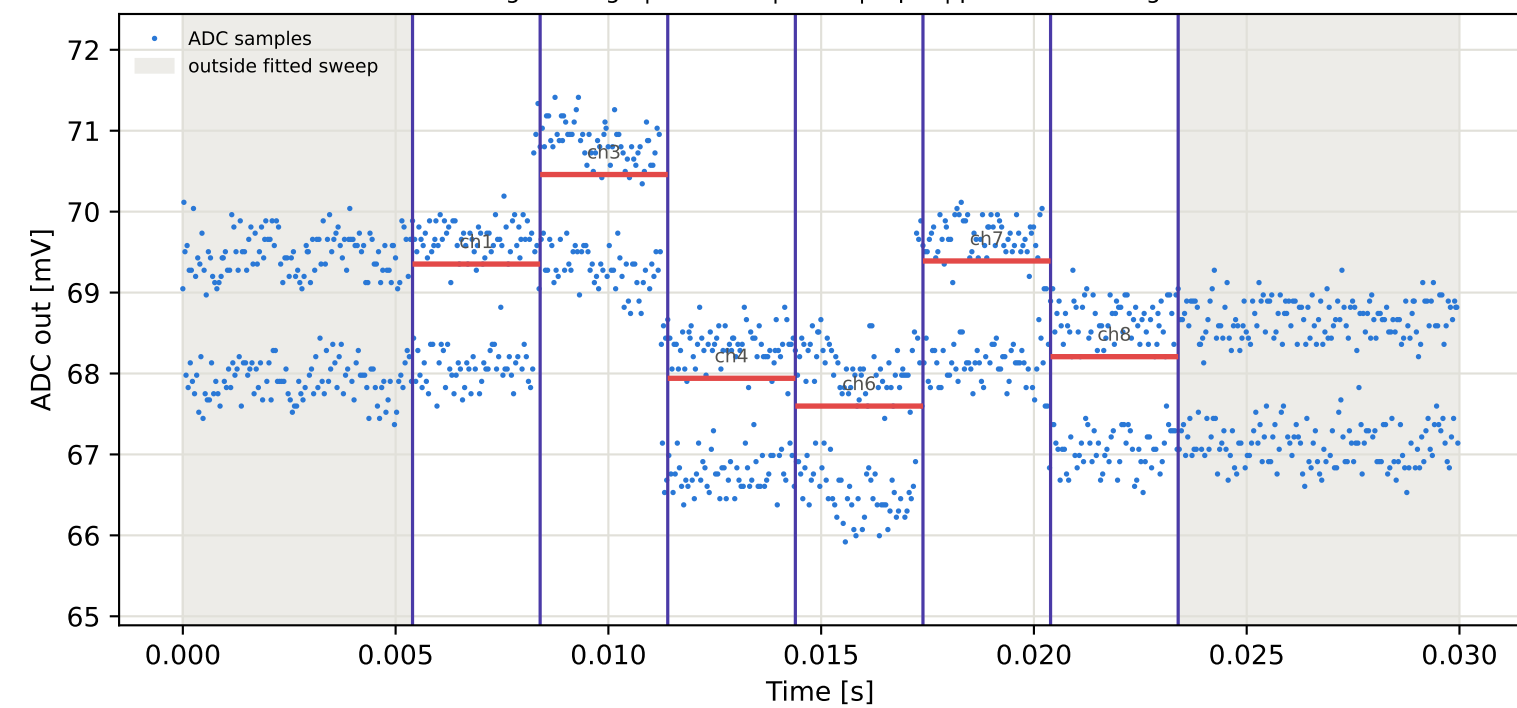
Tag9 &lt;- Tag5 | 785 MHz | run 0 | rep 1 | phase 38.12 deg
