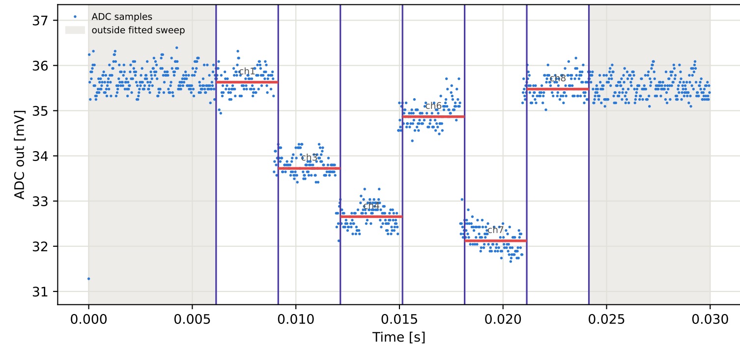
Tag10 &lt;- Tag1 | 795 MHz | run 0 | rep 1 | phase -68.30 deg
