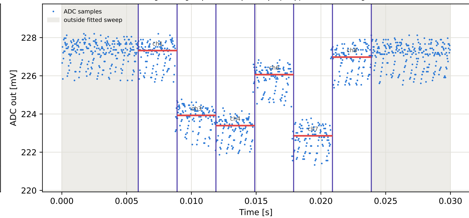
Tag2 &lt;- Tag16 | 835 MHz | run 0 | rep 1 | phase 120.55 deg
