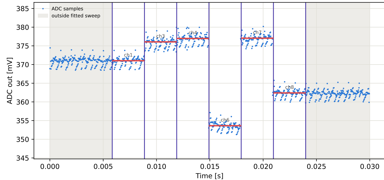
Tag5 &lt;- Tag1 | 945 MHz | run 0 | rep 1 | phase -55.46 deg
