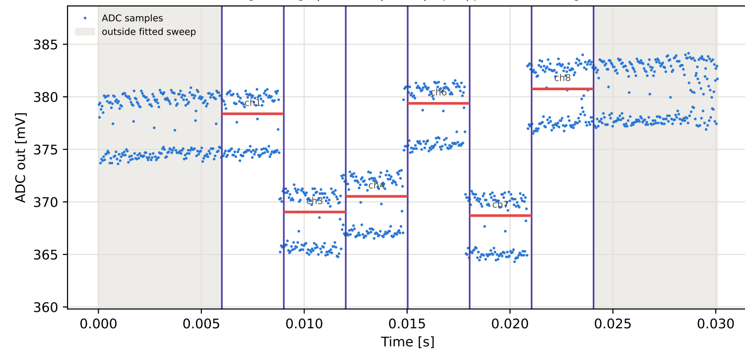
Tag5 &lt;- Tag8 | 825 MHz | run 0 | rep 1 | phase -127.26 deg
