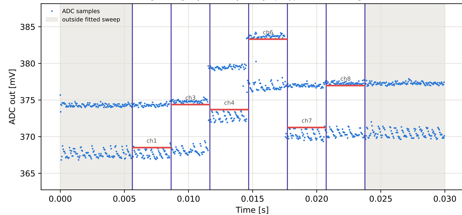
Tag4 &lt;- Tag16 | 945 MHz | run 0 | rep 1 | phase 47.81 deg
