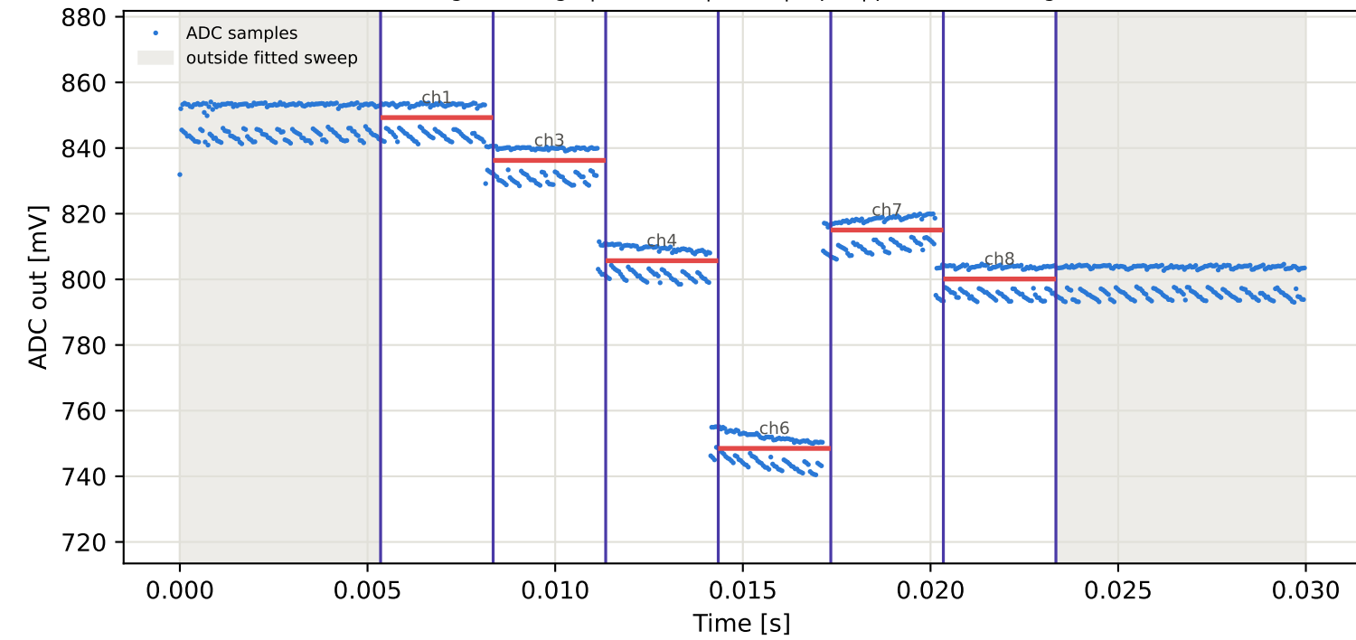
Tag16 &lt;- Tag1 | 895 MHz | run 0 | rep 1 | phase -80.73 deg
