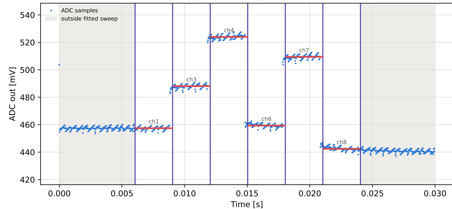
Tag9 &lt;- Tag7 | 955 MHz | run 0 | rep 1 | phase -76.70 deg
