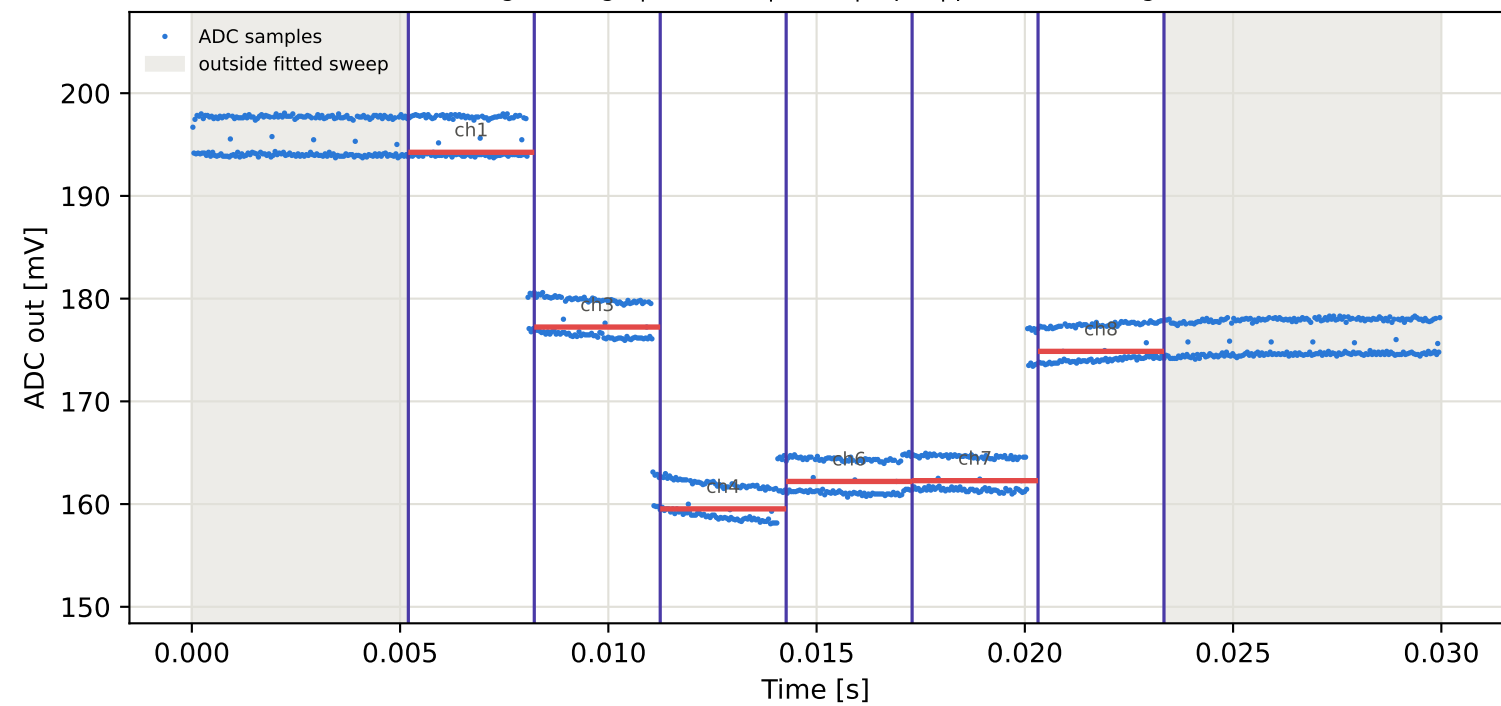
Tag2 &lt;- Tag6 | 845 MHz | run 0 | rep 1 | phase -34.91 deg
