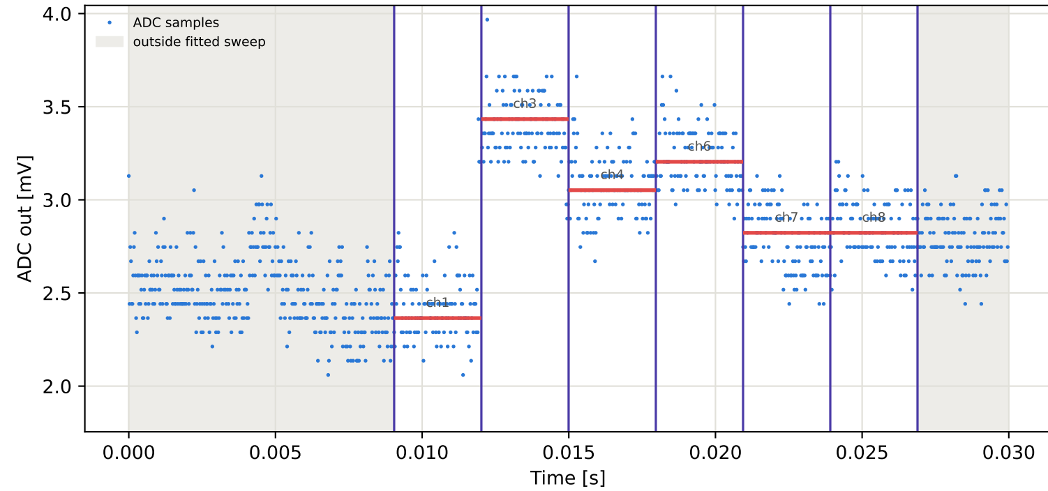
Tag2 &lt;- Tag8 | 785 MHz | run 0 | rep 1 | phase -101.18 deg
