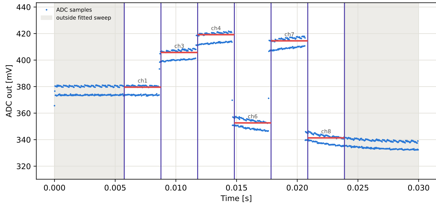
Tag4 &lt;- Tag3 | 915 MHz | run 0 | rep 1 | phase -151.93 deg
