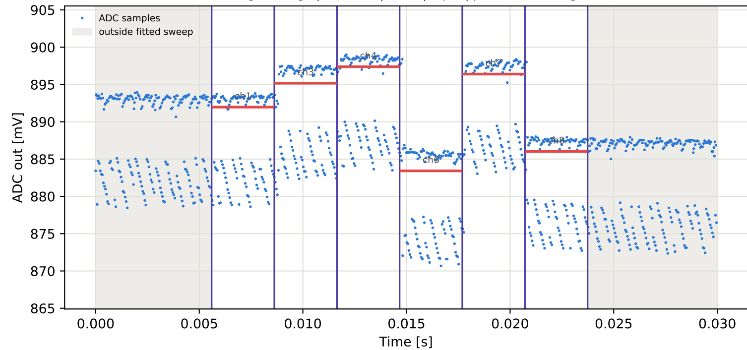
Tag9 &lt;- Tag15 | 935 MHz | run 0 | rep 1 | phase -95.48 deg
