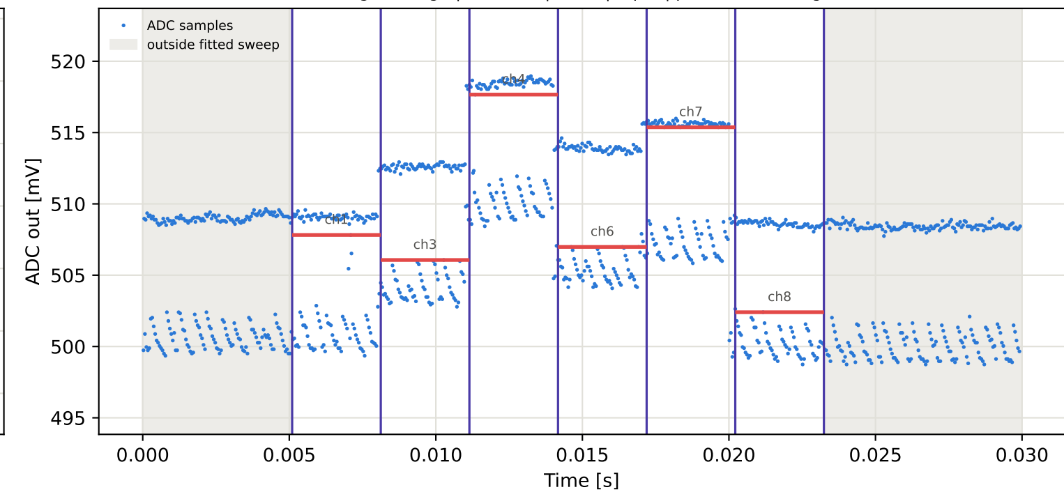
Tag9 &lt;- Tag6 | 945 MHz | run 0 | rep 1 | phase -167.57 deg
