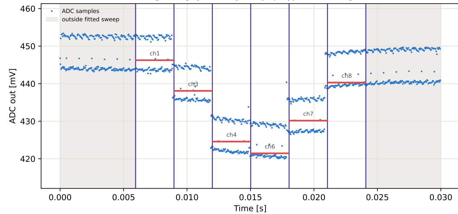
Tag3 &lt;- Tag10 | 925 MHz | run 0 | rep 1 | phase -53.62 deg
