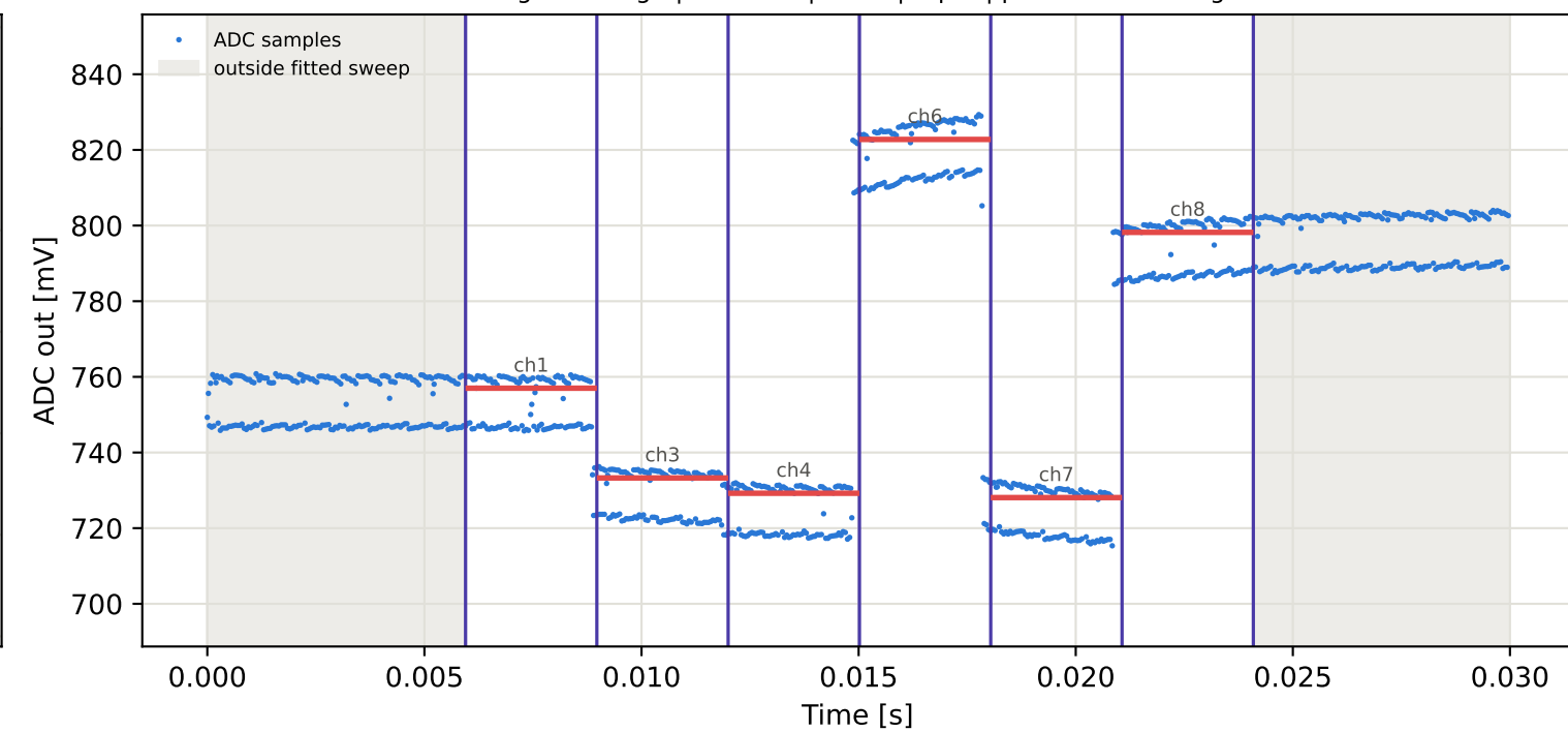
Tag16 &lt;- Tag5 | 935 MHz | run 0 | rep 1 | phase 162.24 deg
