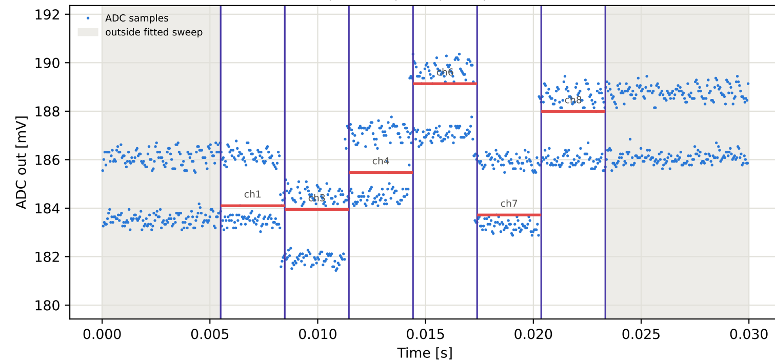
Tag4 &lt;- Tag9 | 835 MHz | run 0 | rep 1 | phase -166.46 deg
