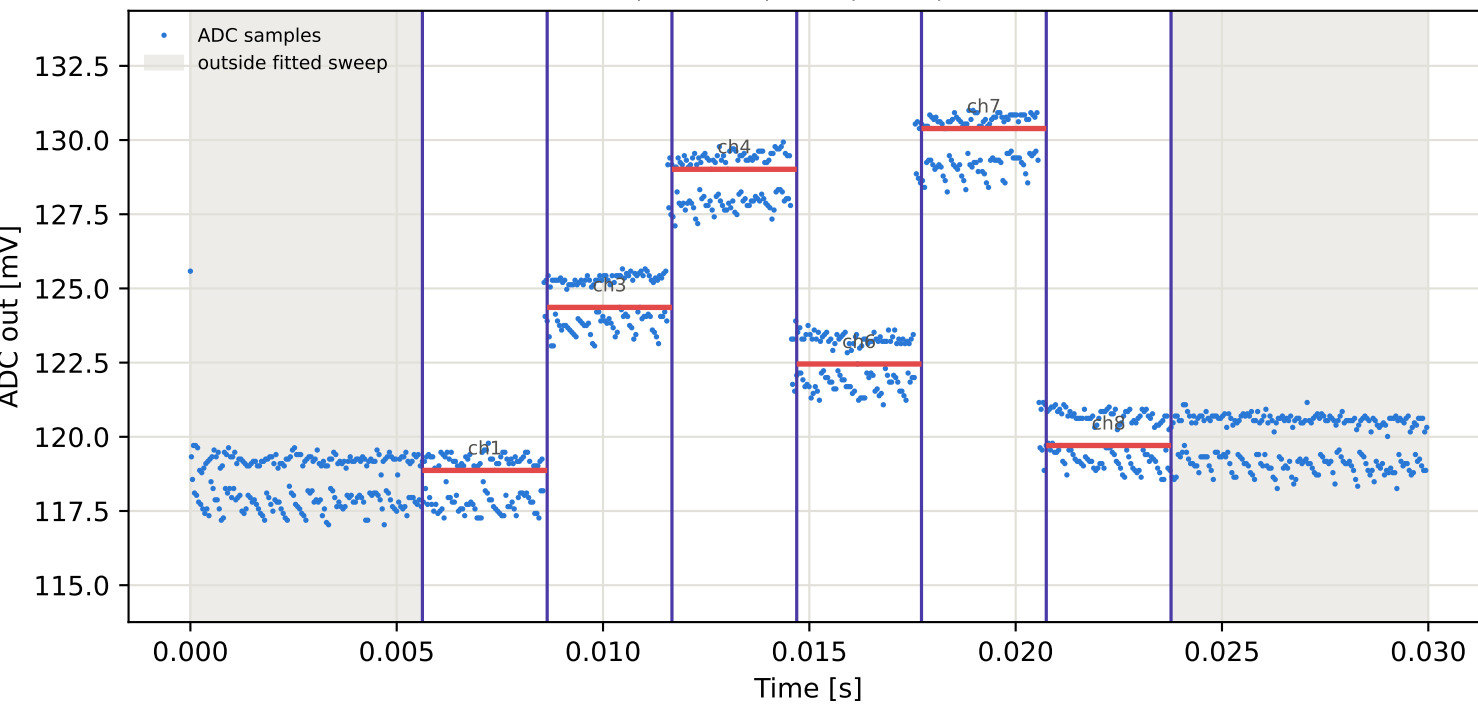
Tag7 &lt;- Tag10 | 805 MHz | run 0 | rep 1 | phase -69.01 deg
