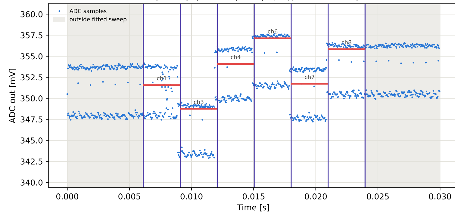
Tag8 &lt;- Tag6 | 805 MHz | run 0 | rep 1 | phase 72.03 deg
