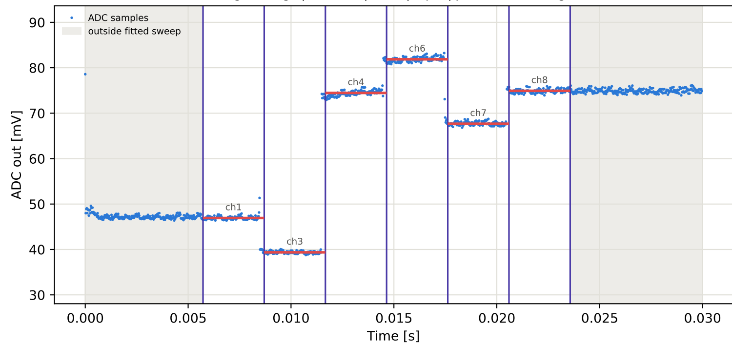
Tag9 &lt;- Tag5 | 835 MHz | run 0 | rep 1 | phase -134.01 deg
