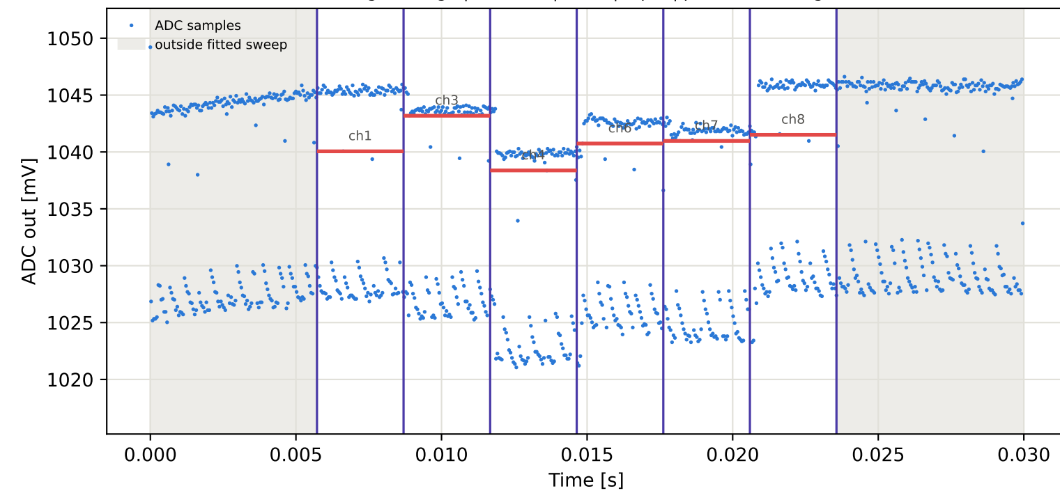
Tag9 &lt;- Tag10 | 955 MHz | run 0 | rep 1 | phase -48.87 deg
