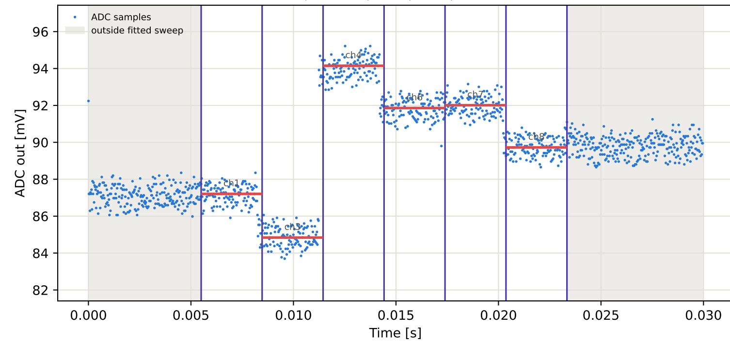
Tag5 &lt;- Tag3 | 795 MHz | run 0 | rep 1 | phase -115.00 deg
