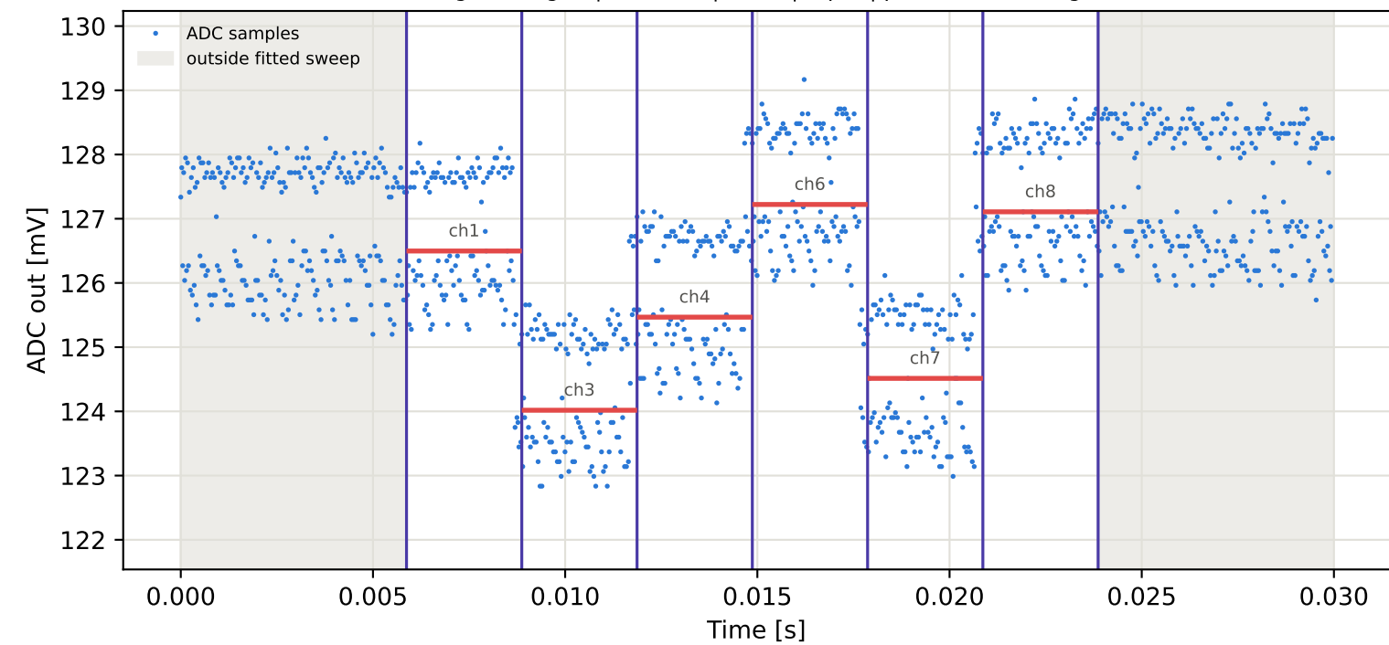
Tag4 &lt;- Tag16 | 795 MHz | run 0 | rep 1 | phase -101.57 deg
