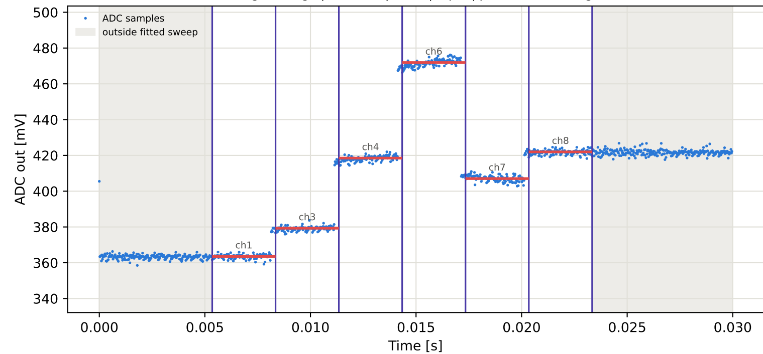
Tag1 &lt;- Tag8 | 885 MHz | run 0 | rep 1 | phase -163.02 deg
