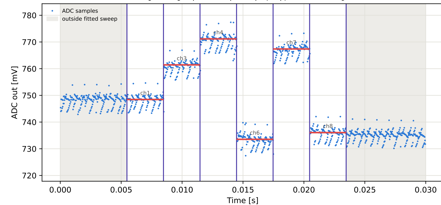
Tag7 &lt;- Tag10 | 945 MHz | run 0 | rep 1 | phase -43.42 deg
