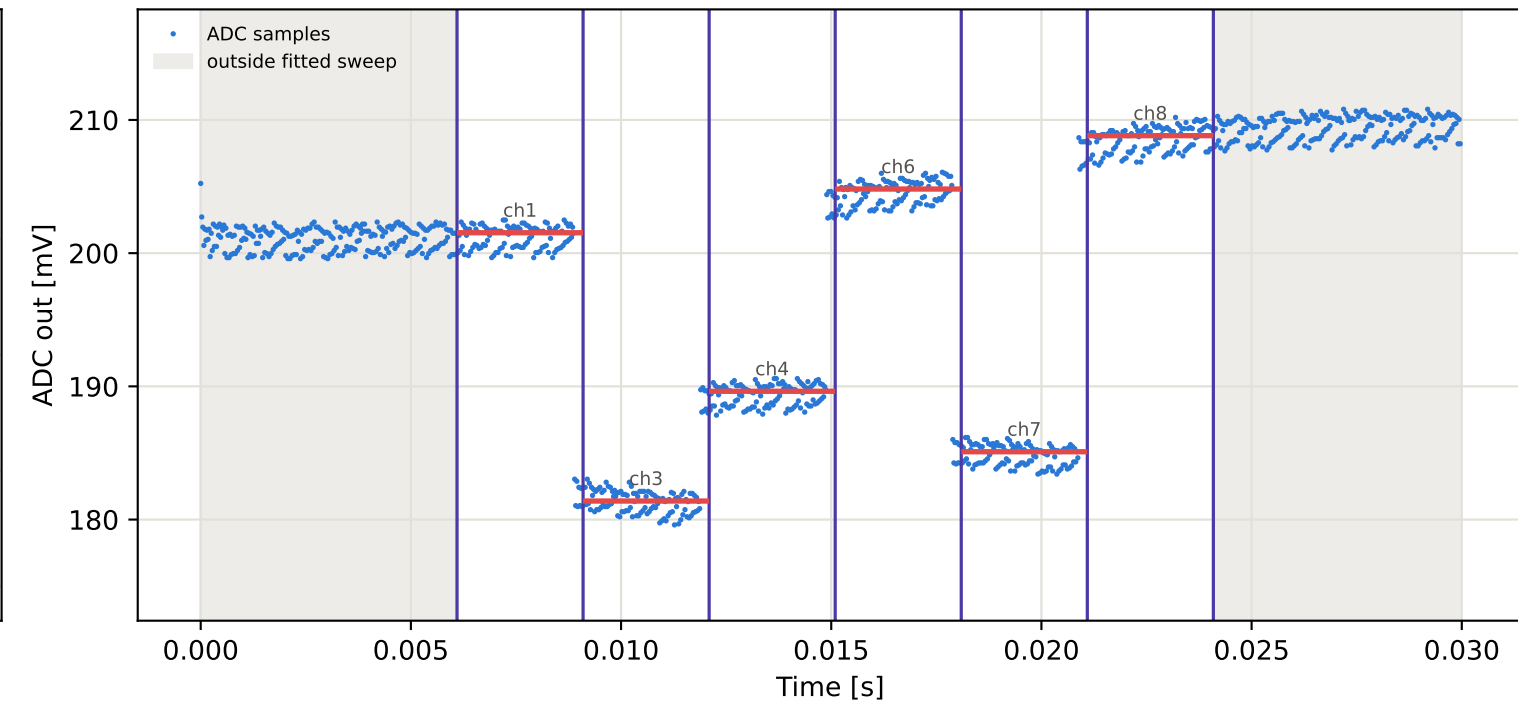
Tag9 &lt;- Tag2 | 855 MHz | run 0 | rep 1 | phase 120.98 deg
