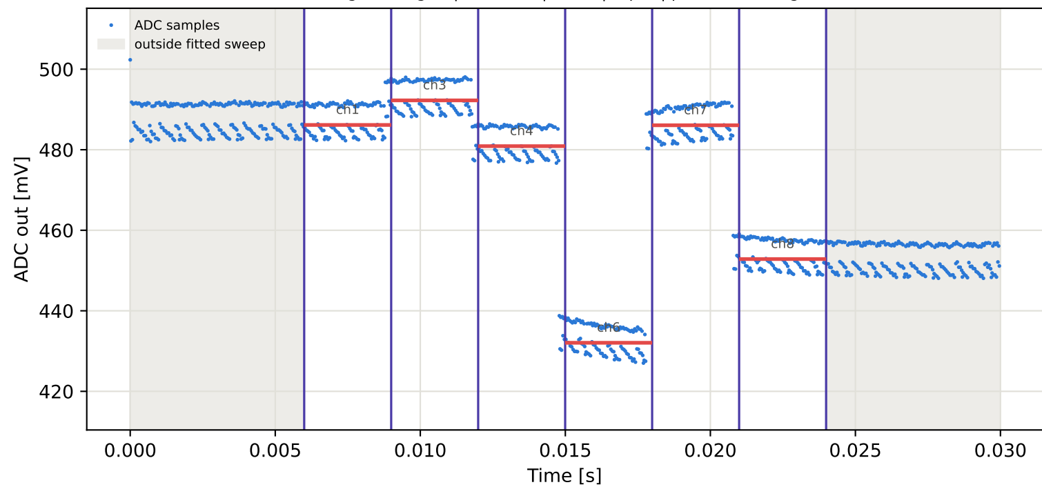
Tag5 &lt;- Tag2 | 915 MHz | run 0 | rep 1 | phase -166.04 deg
