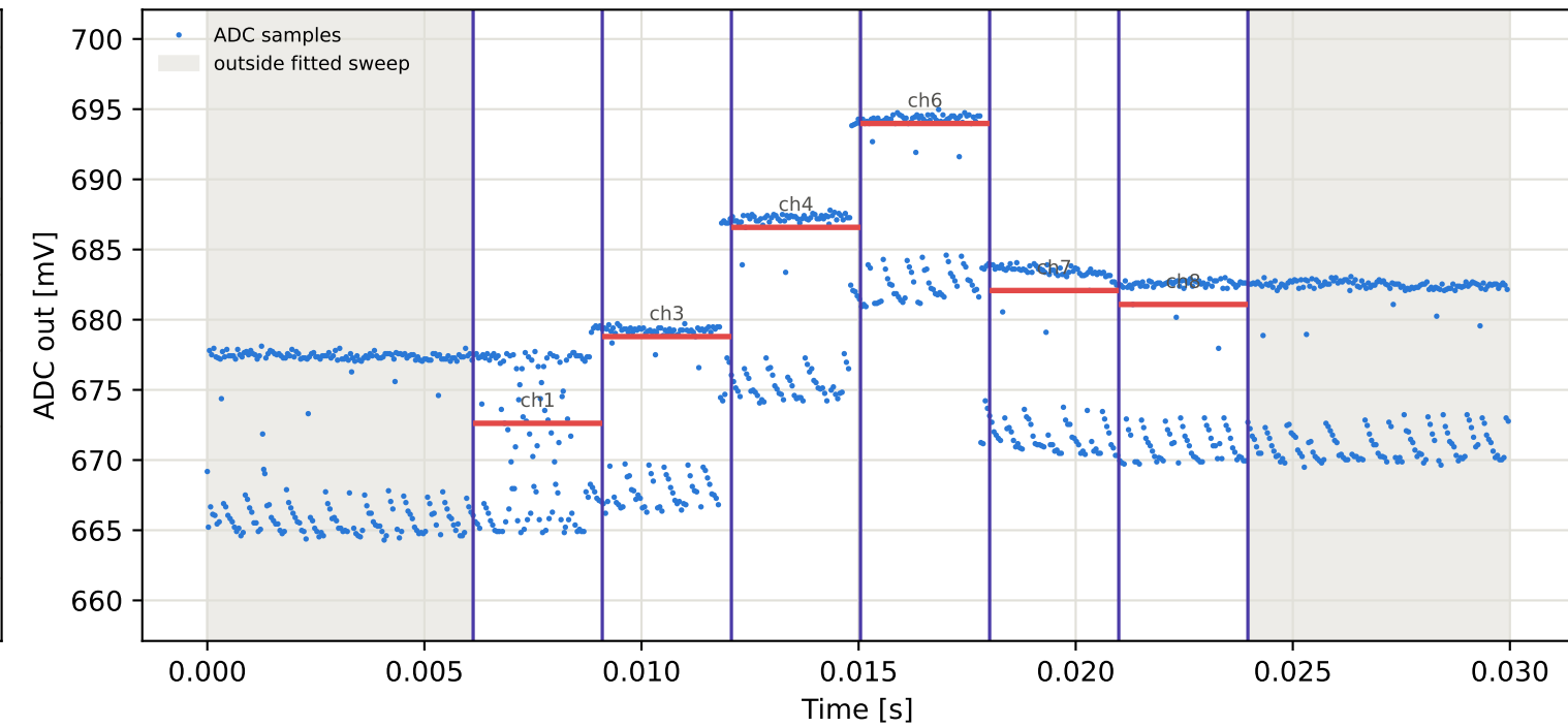
Tag15 &lt;- Tag6 | 935 MHz | run 0 | rep 1 | phase -115.08 deg
