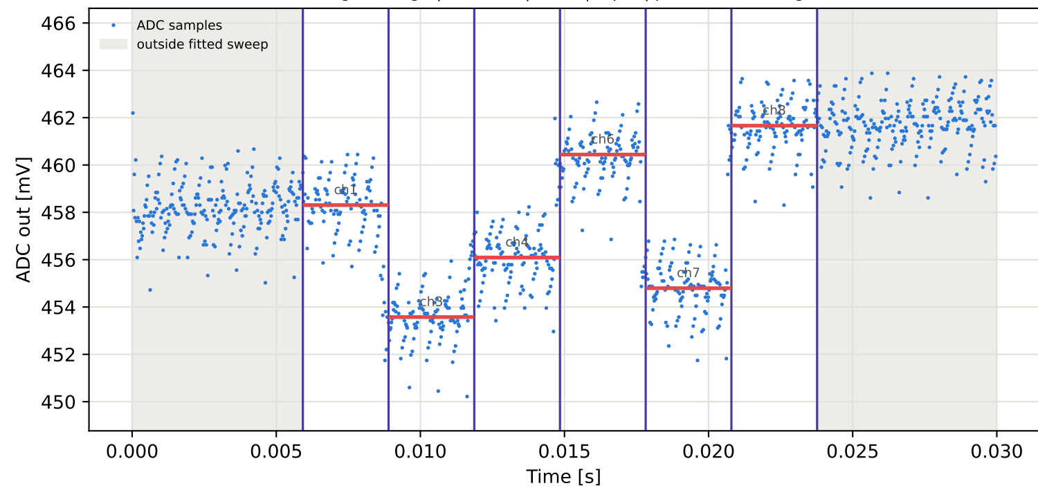
Tag5 &lt;- Tag8 | 845 MHz | run 0 | rep 1 | phase -86.29 deg
