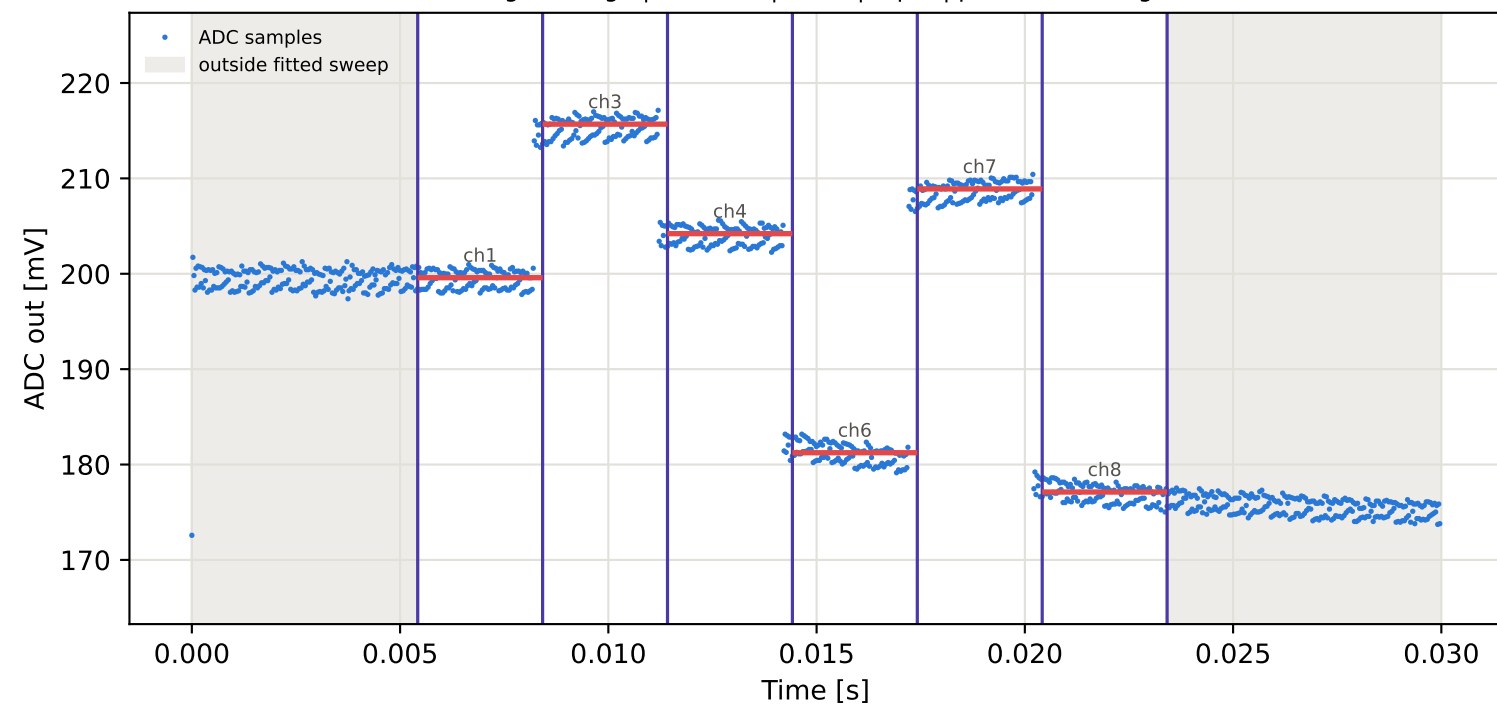
Tag9 &lt;- Tag8 | 855 MHz | run 0 | rep 1 | phase -3.83 deg
