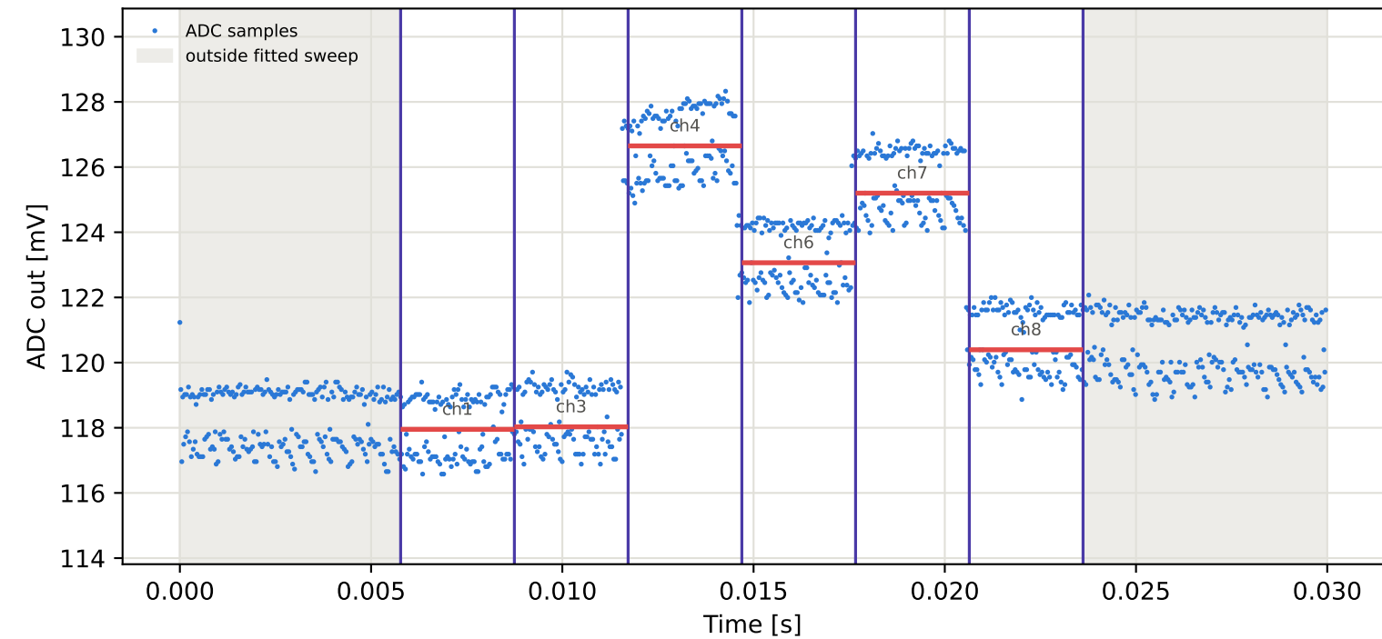
Tag4 &lt;- Tag3 | 795 MHz | run 0 | rep 1 | phase 56.11 deg
