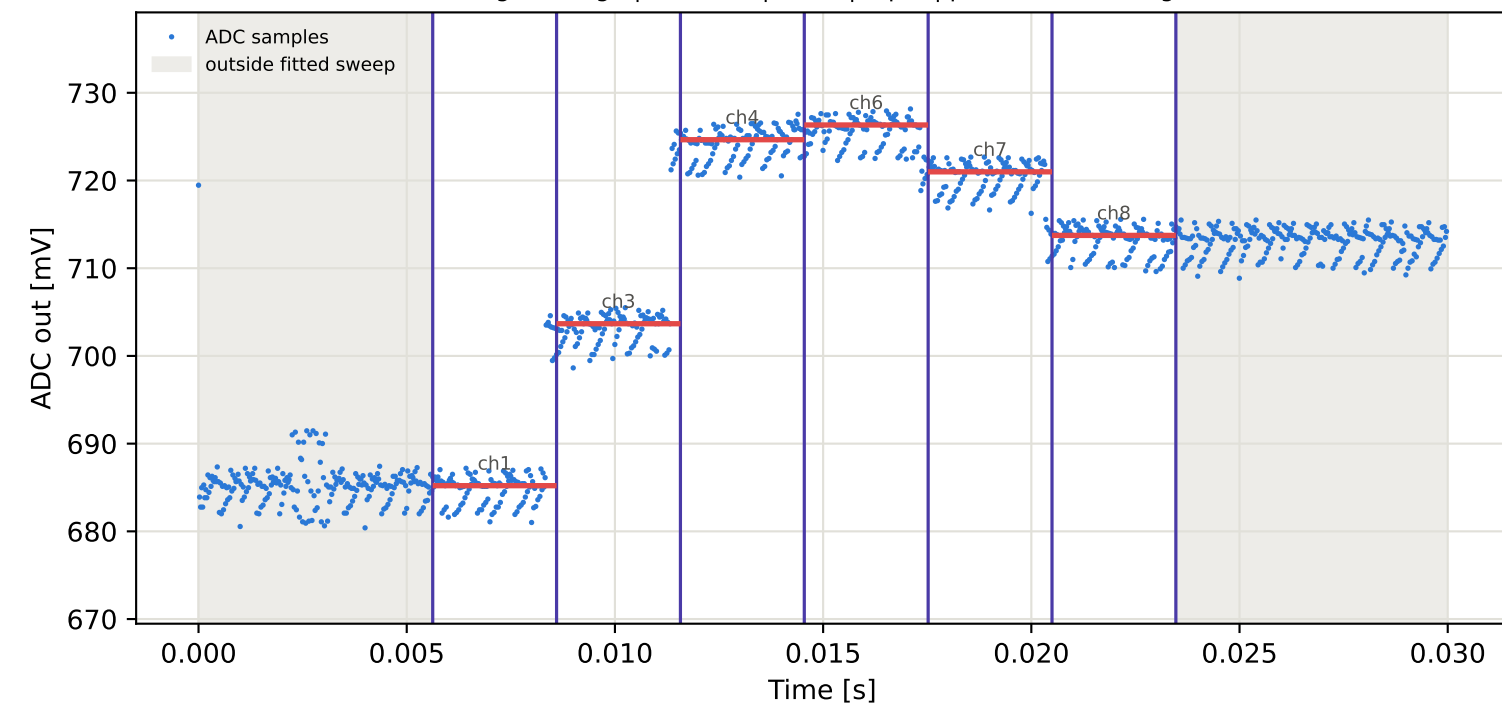
Tag7 &lt;- Tag5 | 845 MHz | run 0 | rep 1 | phase -132.51 deg
