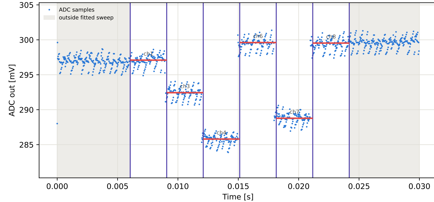
Tag9 &lt;- Tag7 | 995 MHz | run 0 | rep 1 | phase -10.43 deg
