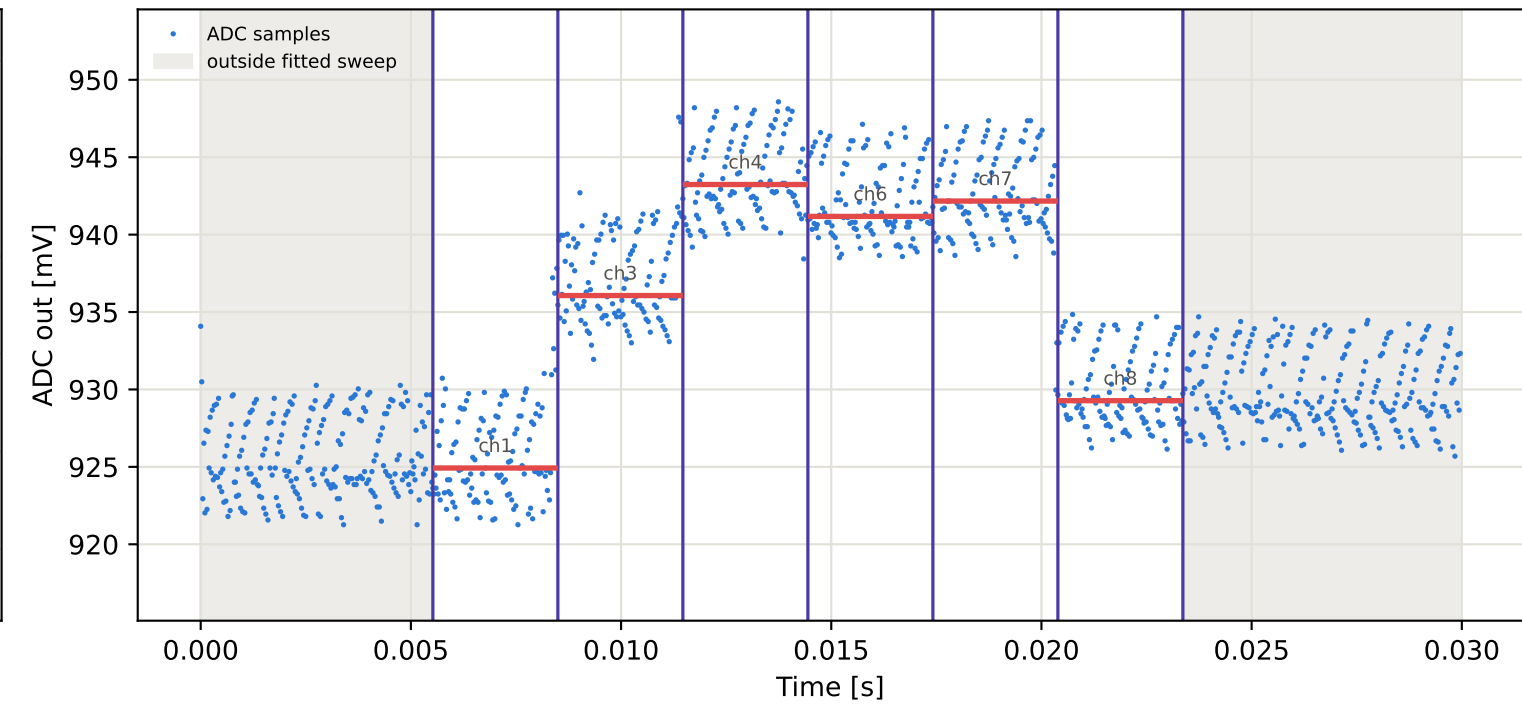
Tag8 &lt;- Tag7 | 875 MHz | run 0 | rep 1 | phase -112.83 deg
