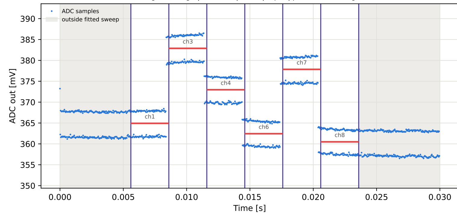
Tag15 &lt;- Tag5 | 825 MHz | run 0 | rep 1 | phase -46.48 deg
