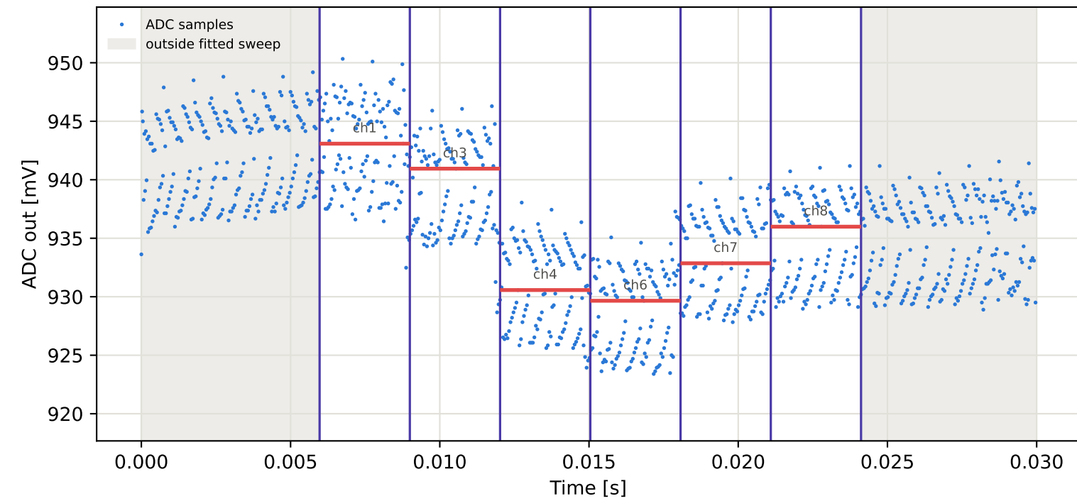
Tag9 &lt;- Tag10 | 875 MHz | run 0 | rep 1 | phase -158.66 deg
