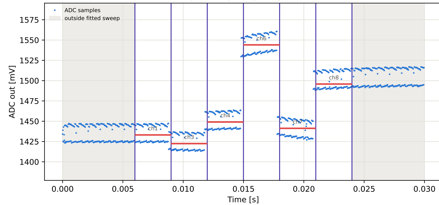
Tag8 &lt;- Tag15 | 915 MHz | run 0 | rep 1 | phase -168.42 deg
