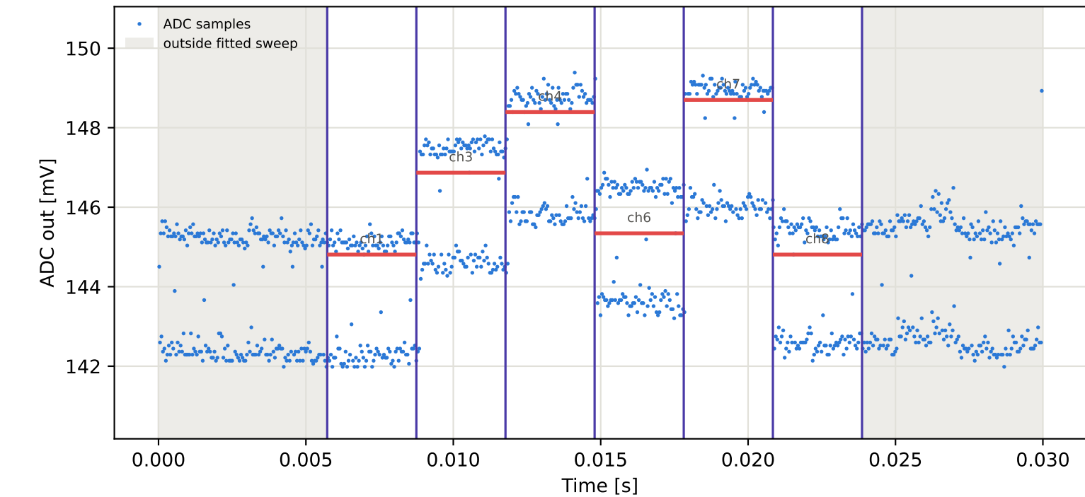
Tag16 &lt;- Tag10 | 805 MHz | run 0 | rep 1 | phase 86.07 deg
