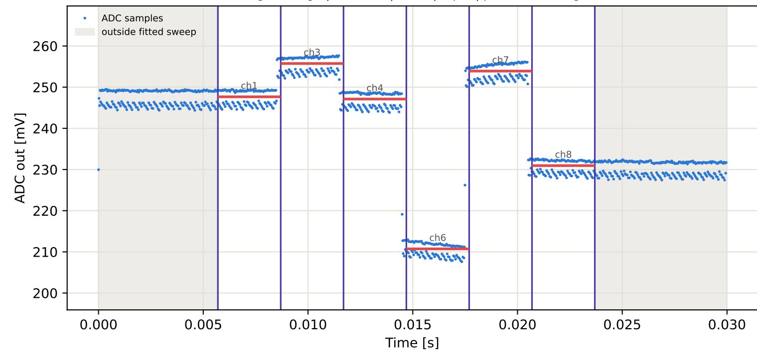
Tag3 &lt;- Tag7 | 965 MHz | run 0 | rep 1 | phase -114.45 deg
