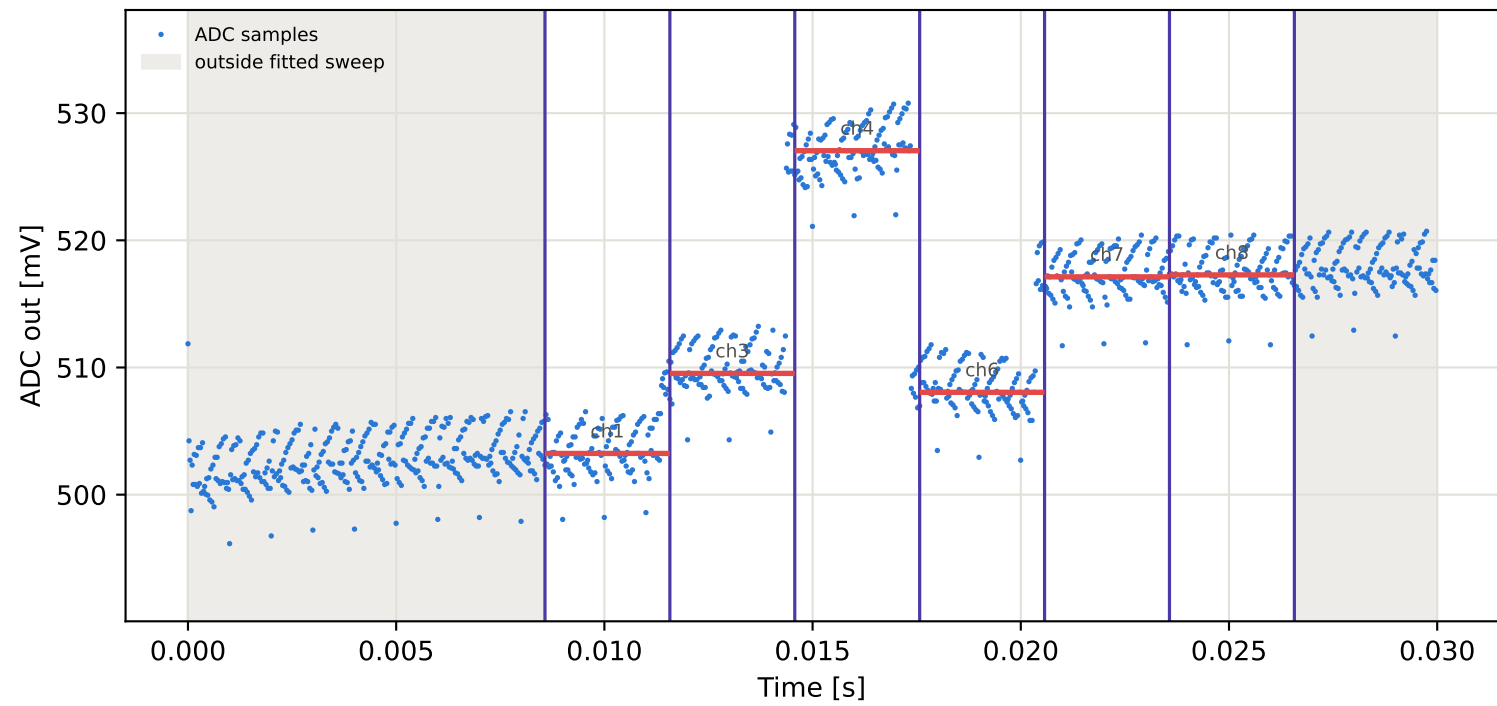
Tag2 &lt;- Tag5 | 895 MHz | run 0 | rep 1 | phase -109.31 deg
