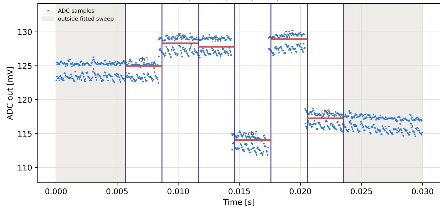
Tag6 &lt;- Tag2 | 935 MHz | run 0 | rep 1 | phase 141.66 deg
