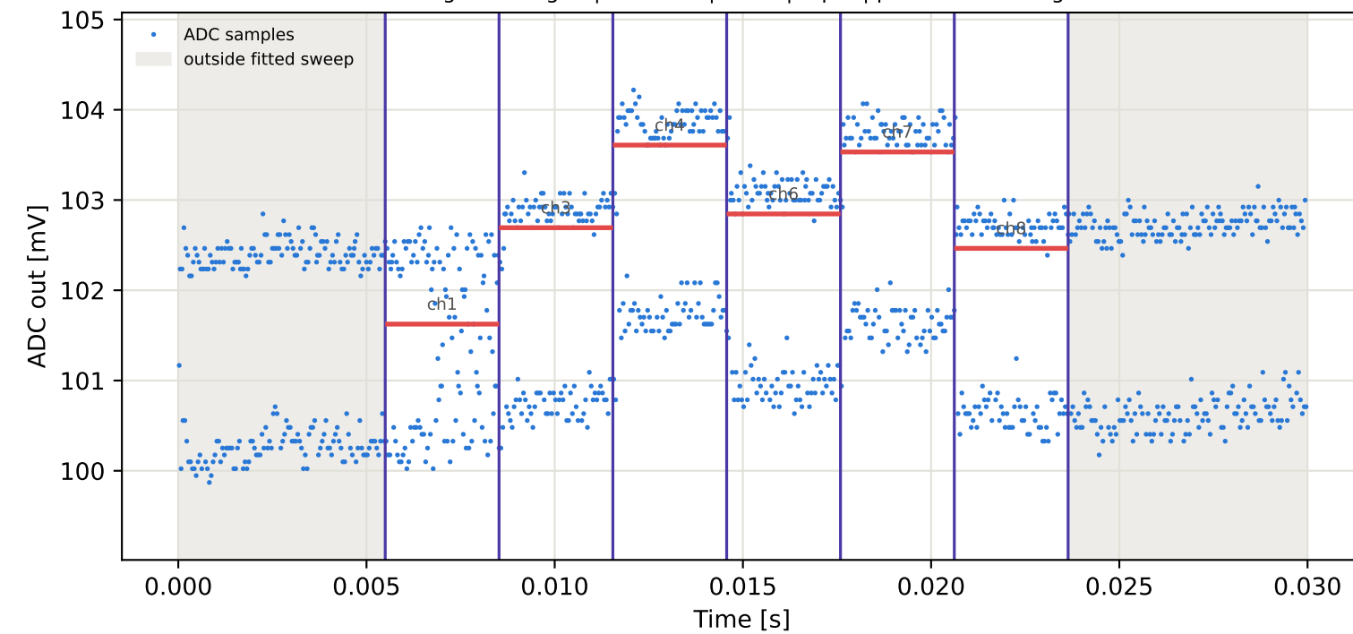
Tag10 &lt;- Tag2 | 795 MHz | run 0 | rep 1 | phase -8.34 deg
