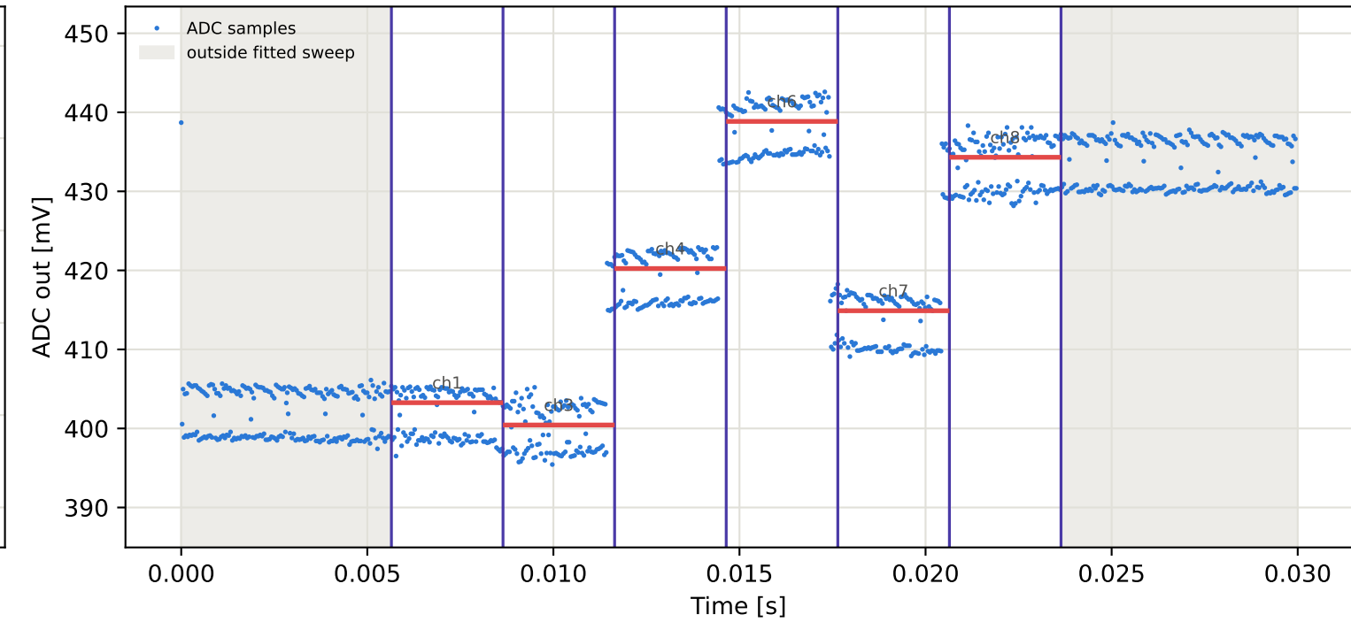
Tag9 &lt;- Tag2 | 875 MHz | run 0 | rep 1 | phase -108.28 deg
