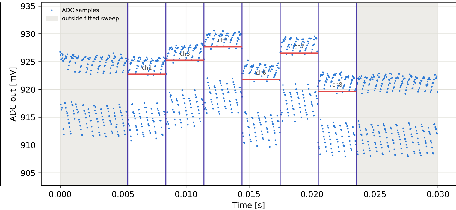
Tag5 &lt;- Tag4 | 925 MHz | run 0 | rep 1 | phase 70.99 deg
