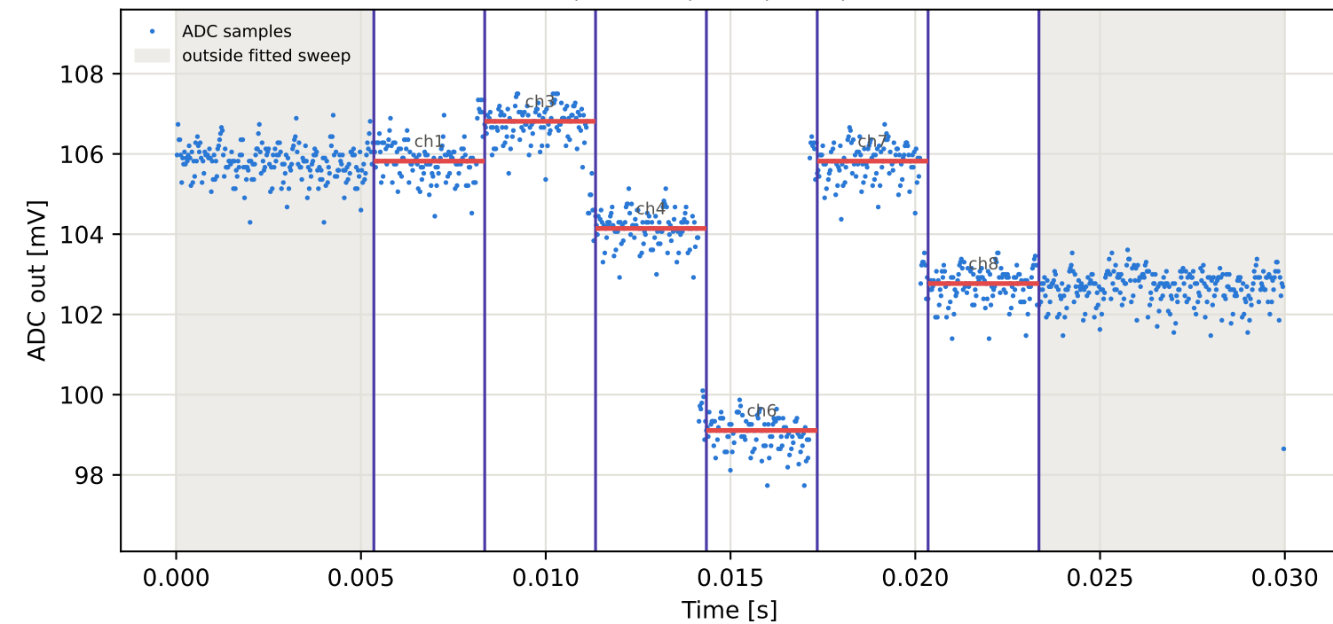
Tag1 &lt;- Tag9 | 965 MHz | run 0 | rep 1 | phase 11.75 deg
