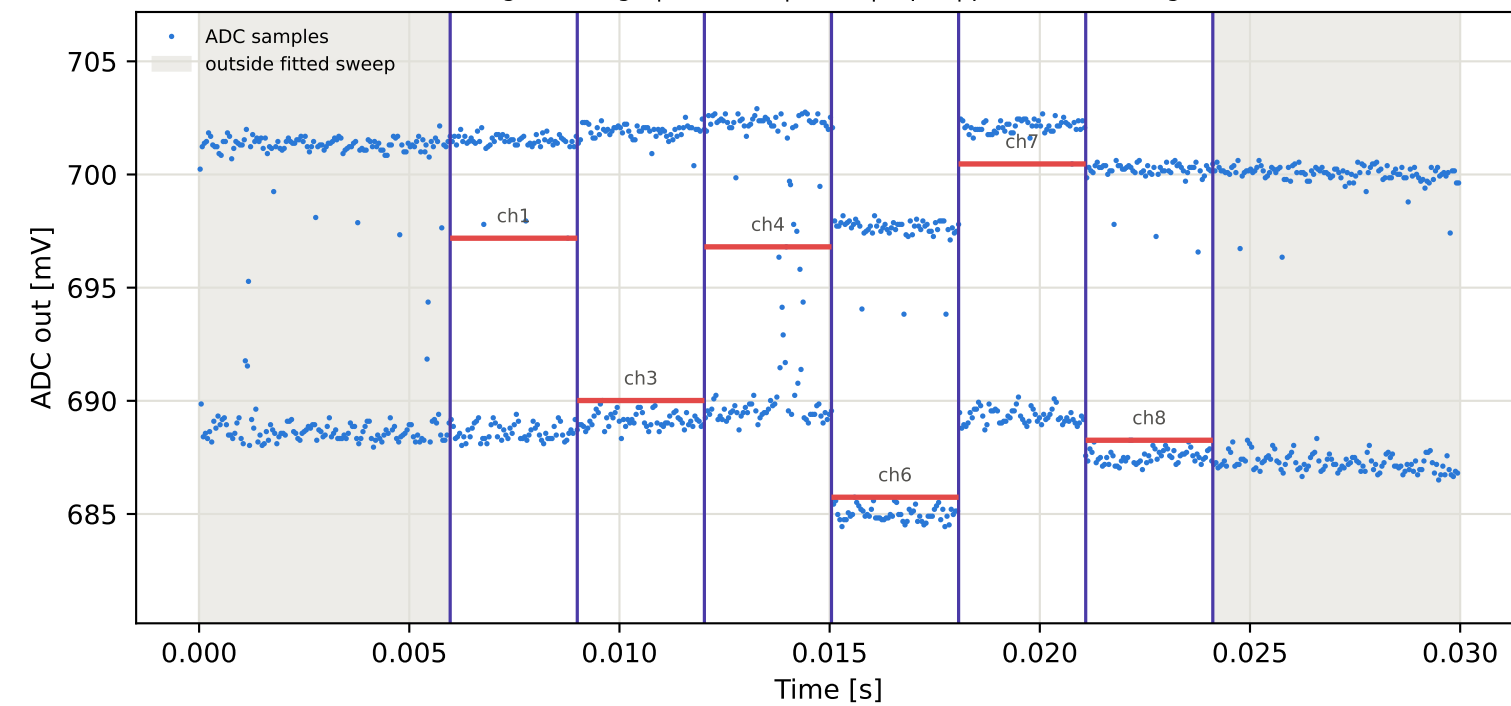
Tag16 &lt;- Tag4 | 975 MHz | run 0 | rep 1 | phase 90.98 deg
