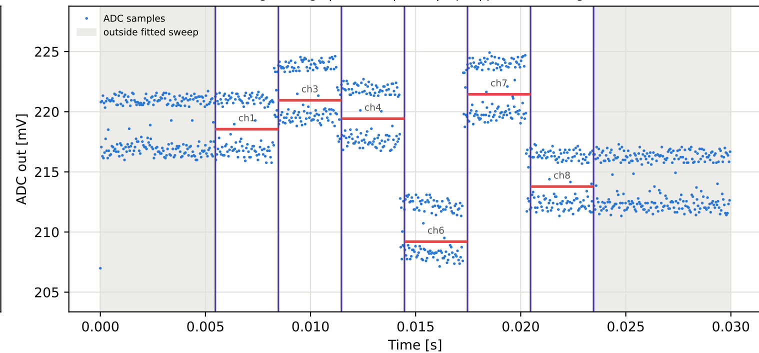
Tag10 &lt;- Tag1 | 985 MHz | run 0 | rep 1 | phase -44.22 deg
