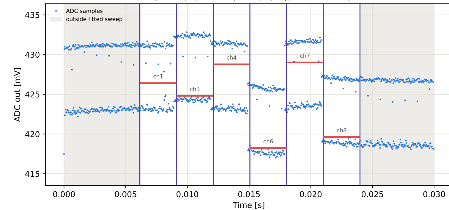
Tag2 &lt;- Tag15 | 905 MHz | run 0 | rep 1 | phase 36.77 deg
