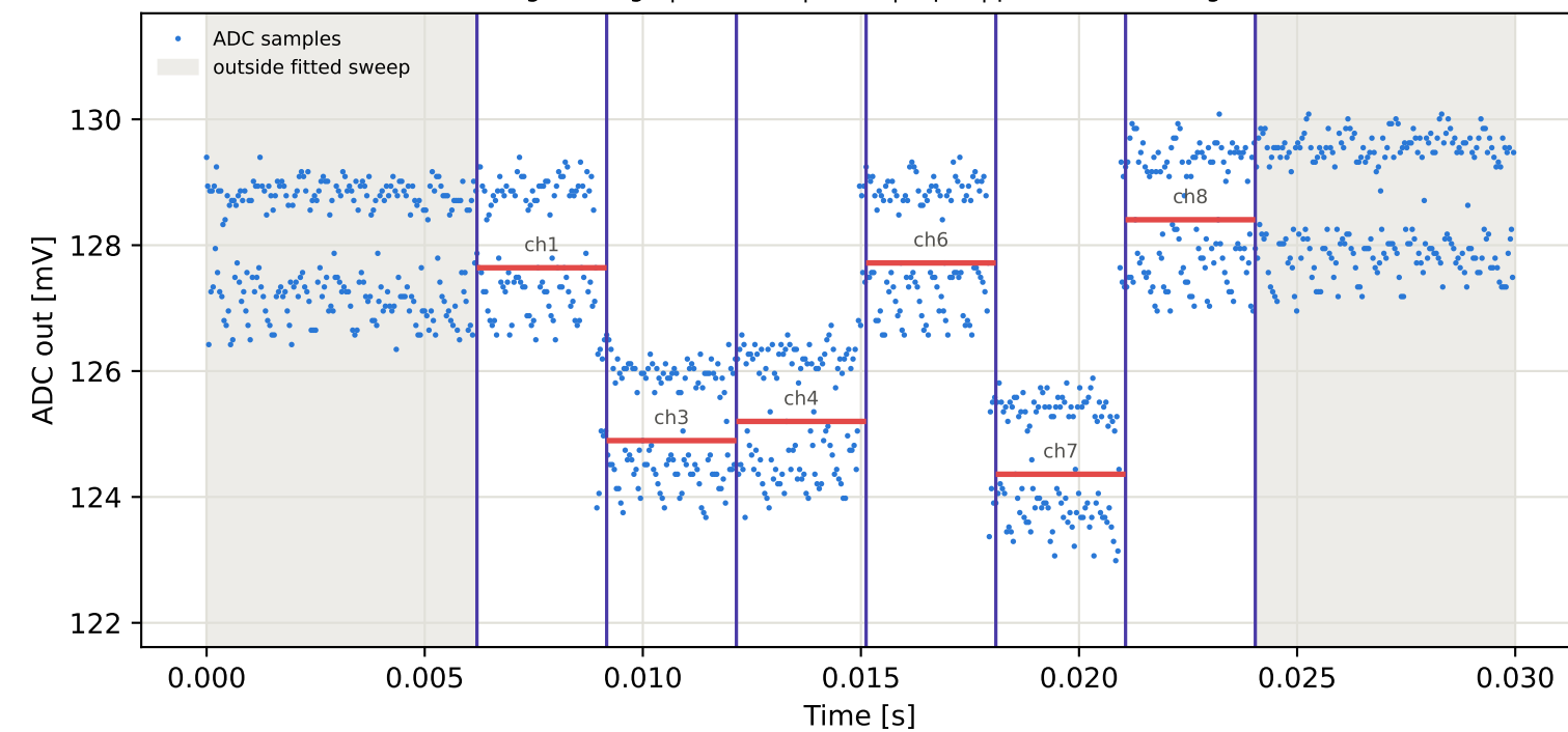
Tag4 &lt;- Tag9 | 795 MHz | run 0 | rep 1 | phase 146.83 deg
