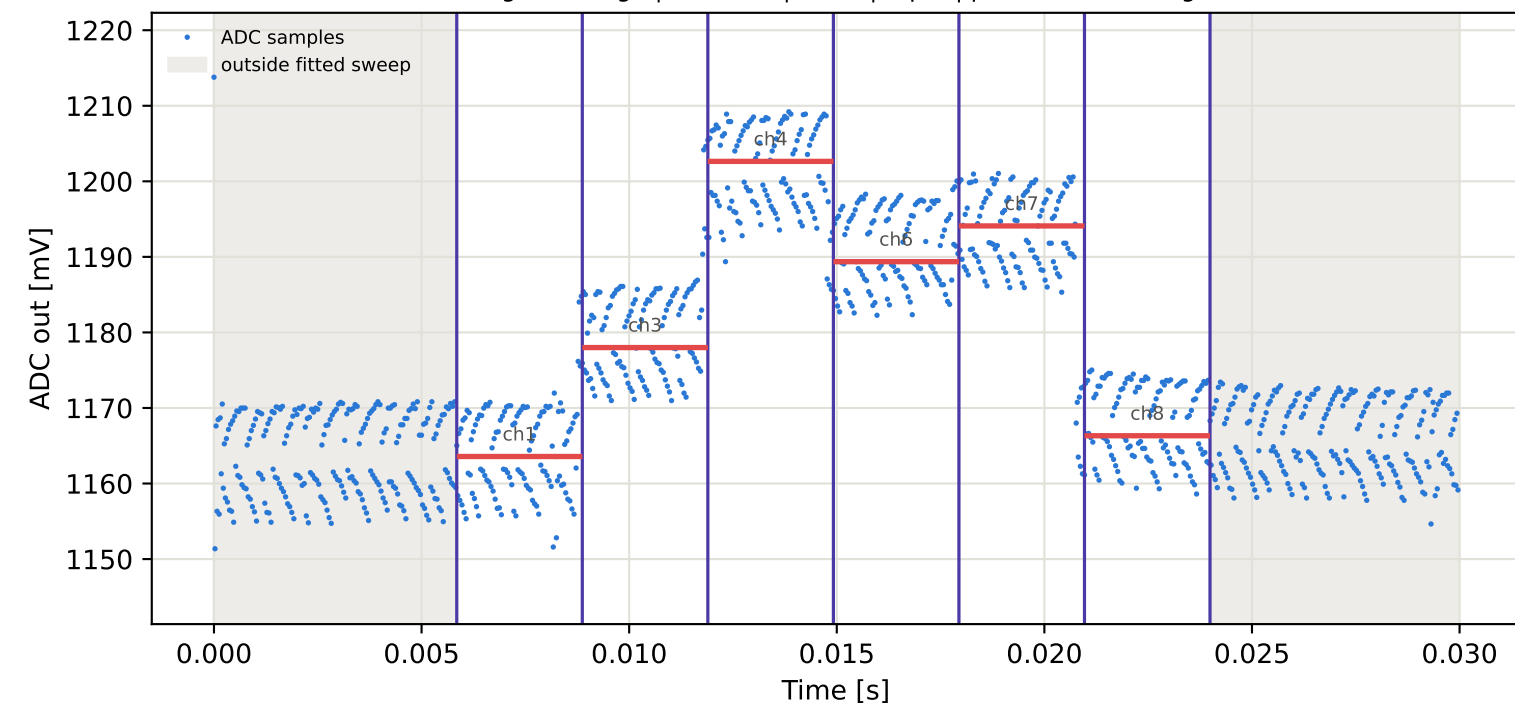
Tag16 &lt;- Tag7 | 925 MHz | run 0 | rep 1 | phase -109.95 deg
