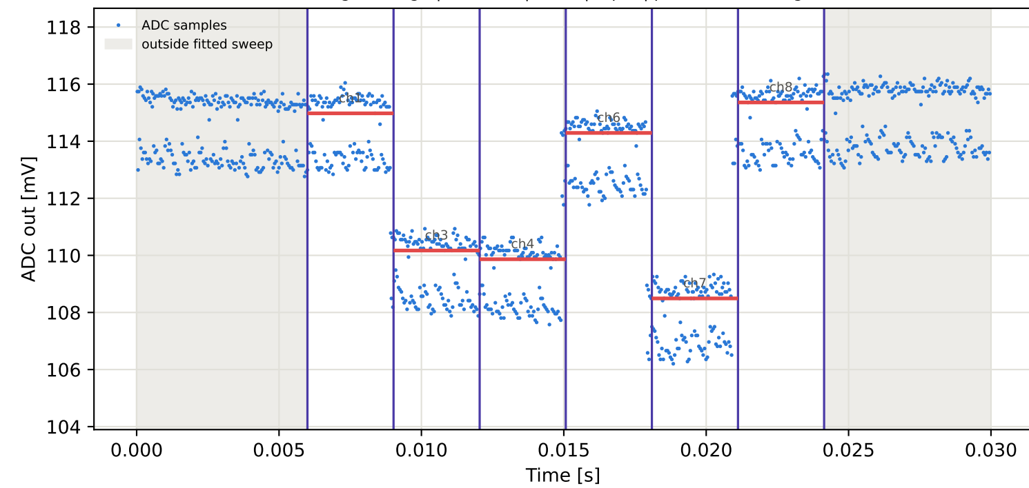
Tag7 &lt;- Tag1 | 805 MHz | run 0 | rep 1 | phase 118.95 deg
