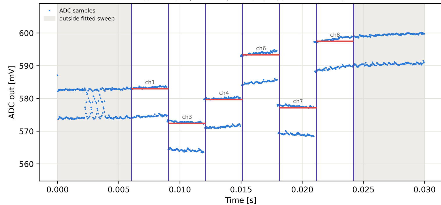
Tag6 &lt;- Tag3 | 865 MHz | run 0 | rep 1 | phase -108.37 deg
