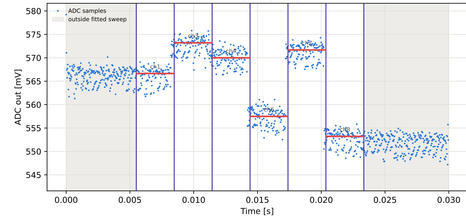
Tag2 &lt;- Tag15 | 885 MHz | run 0 | rep 1 | phase -13.10 deg
