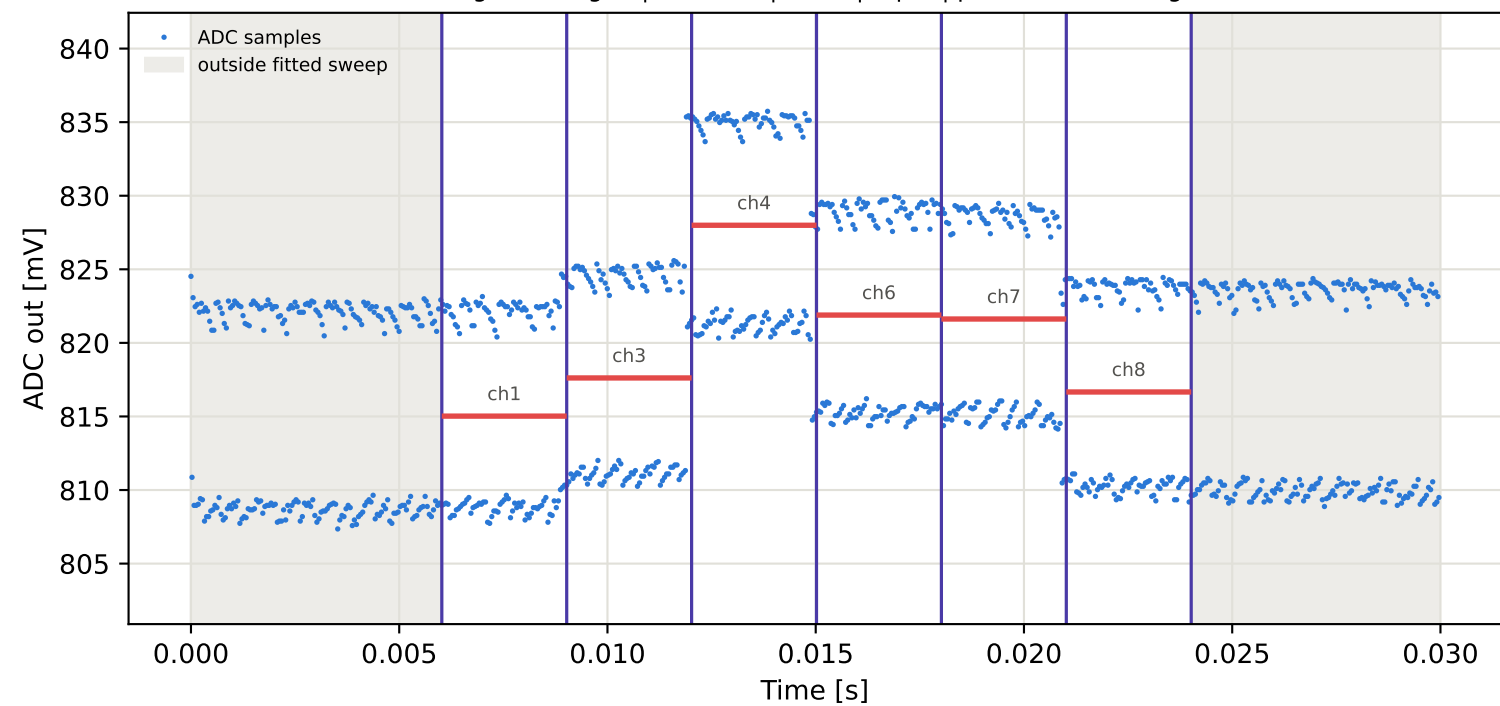
Tag16 &lt;- Tag10 | 985 MHz | run 0 | rep 1 | phase -118.32 deg
