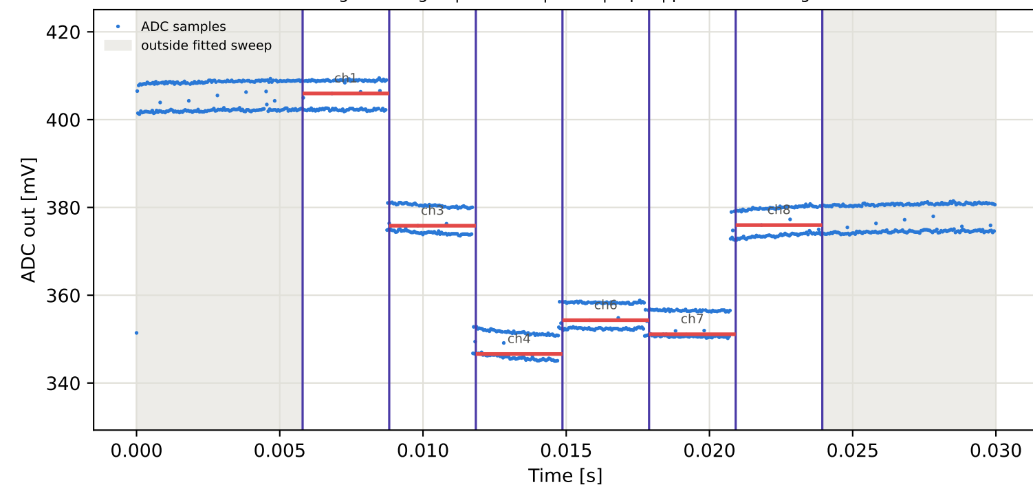
Tag15 &lt;- Tag3 | 855 MHz | run 0 | rep 1 | phase 23.68 deg
