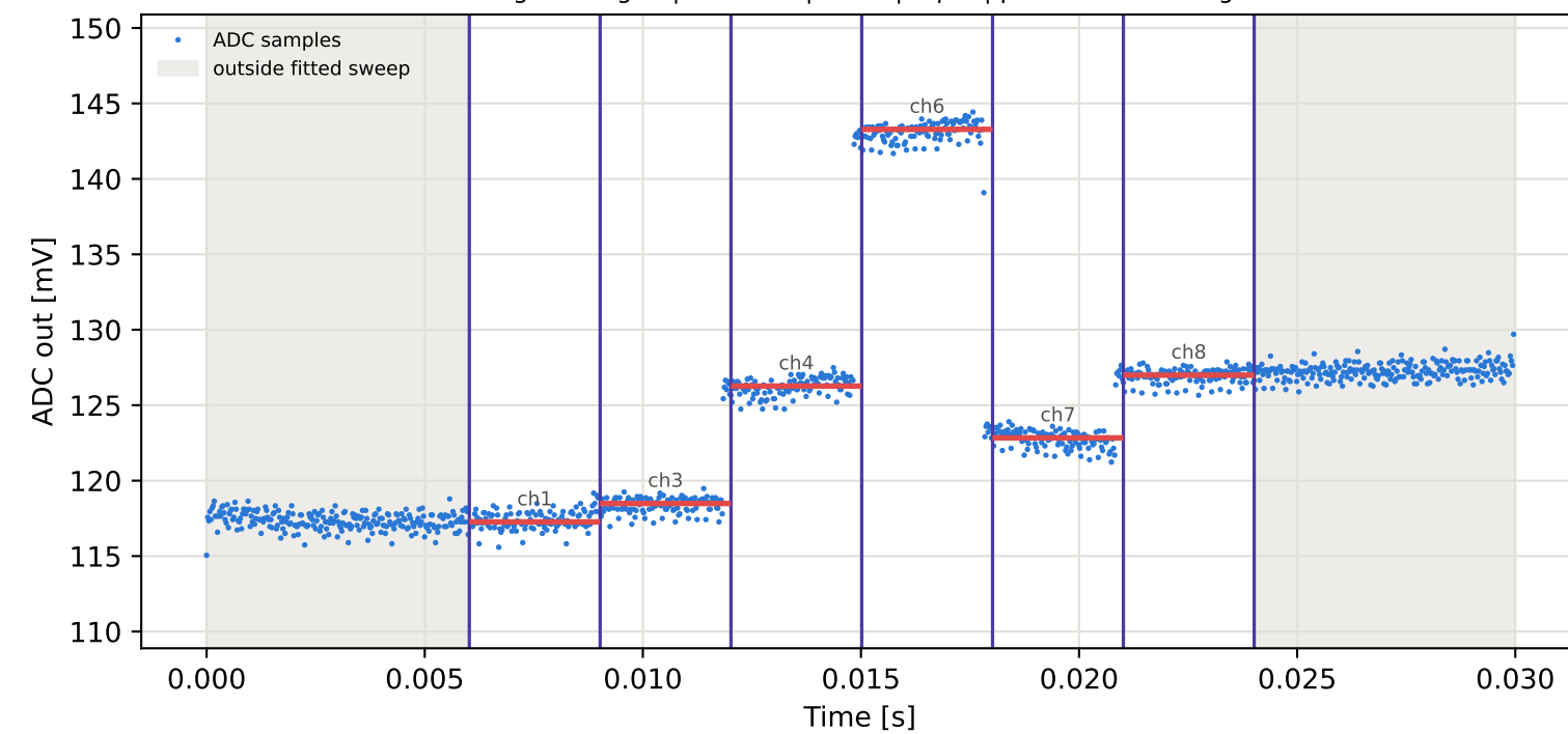
Tag1 &lt;- Tag16 | 915 MHz | run 0 | rep 1 | phase -49.65 deg
