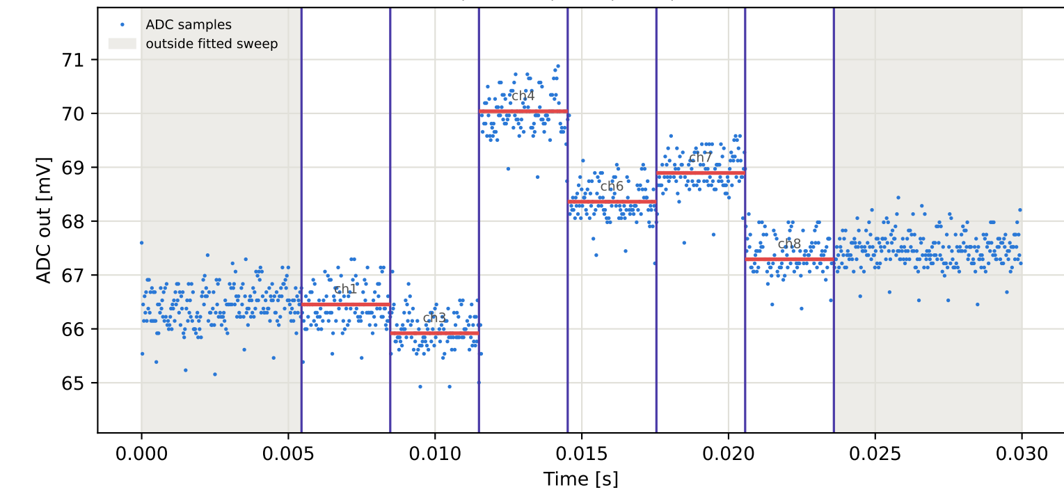
Tag16 &lt;- Tag15 | 775 MHz | run 0 | rep 1 | phase -101.81 deg
