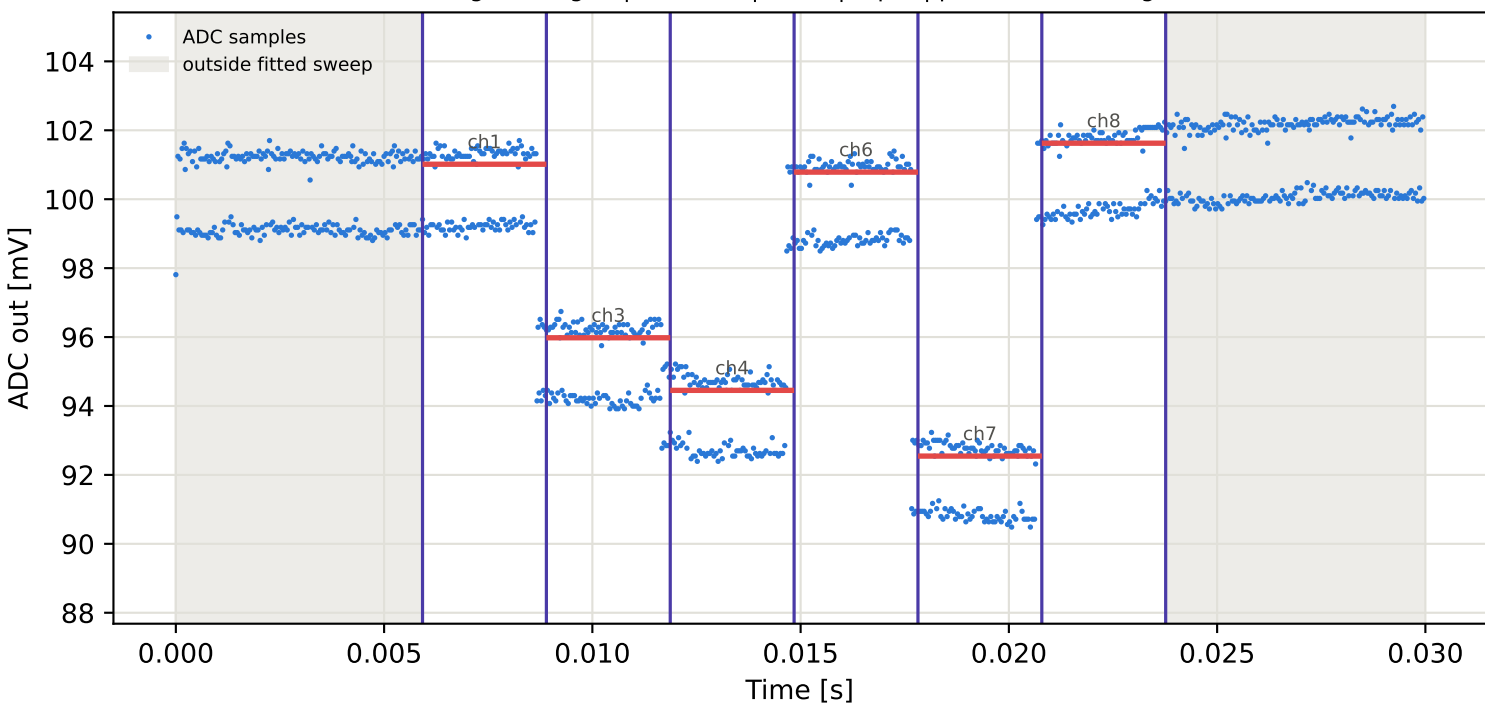
Tag3 &lt;- Tag2 | 795 MHz | run 0 | rep 1 | phase 52.21 deg
