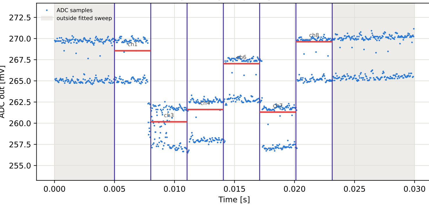
Tag6 &lt;- Tag4 | 835 MHz | run 0 | rep 1 | phase 138.19 deg
