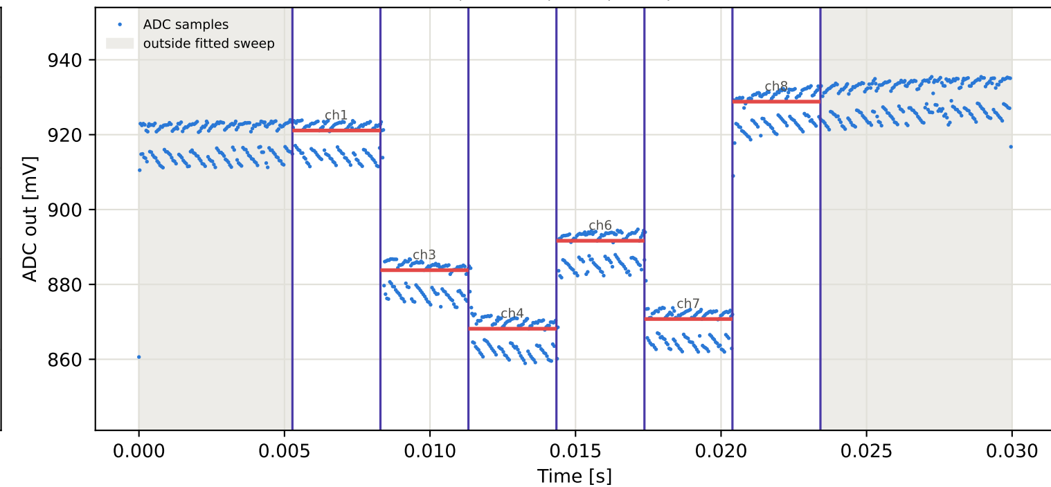
Tag6 &lt;- Tag10 | 875 MHz | run 0 | rep 1 | phase 98.41 deg
