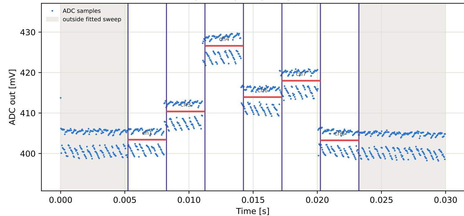
Tag4 &lt;- Tag3 | 965 MHz | run 0 | rep 1 | phase -108.31 deg
