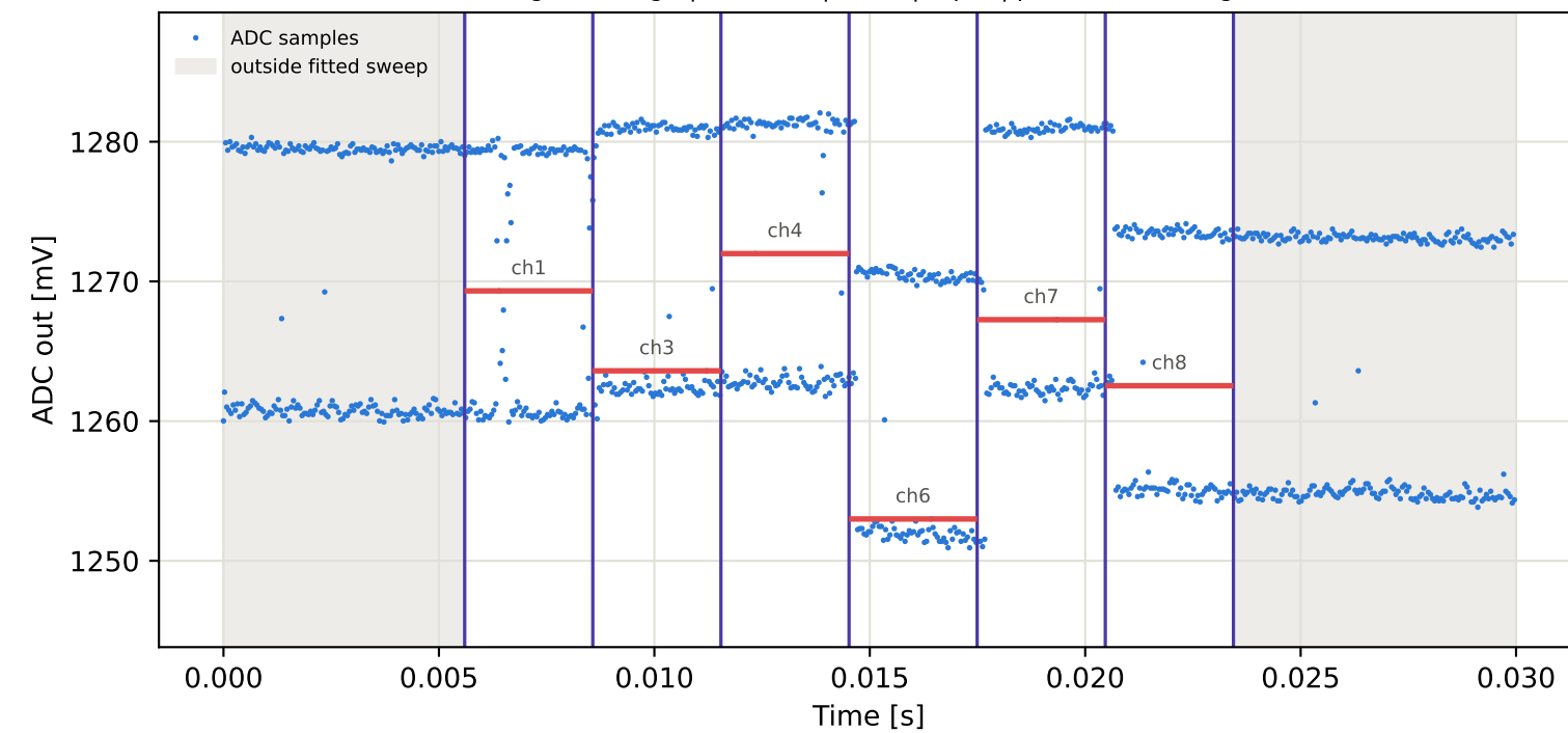
Tag16 &lt;- Tag4 | 905 MHz | run 0 | rep 1 | phase -165.36 deg
