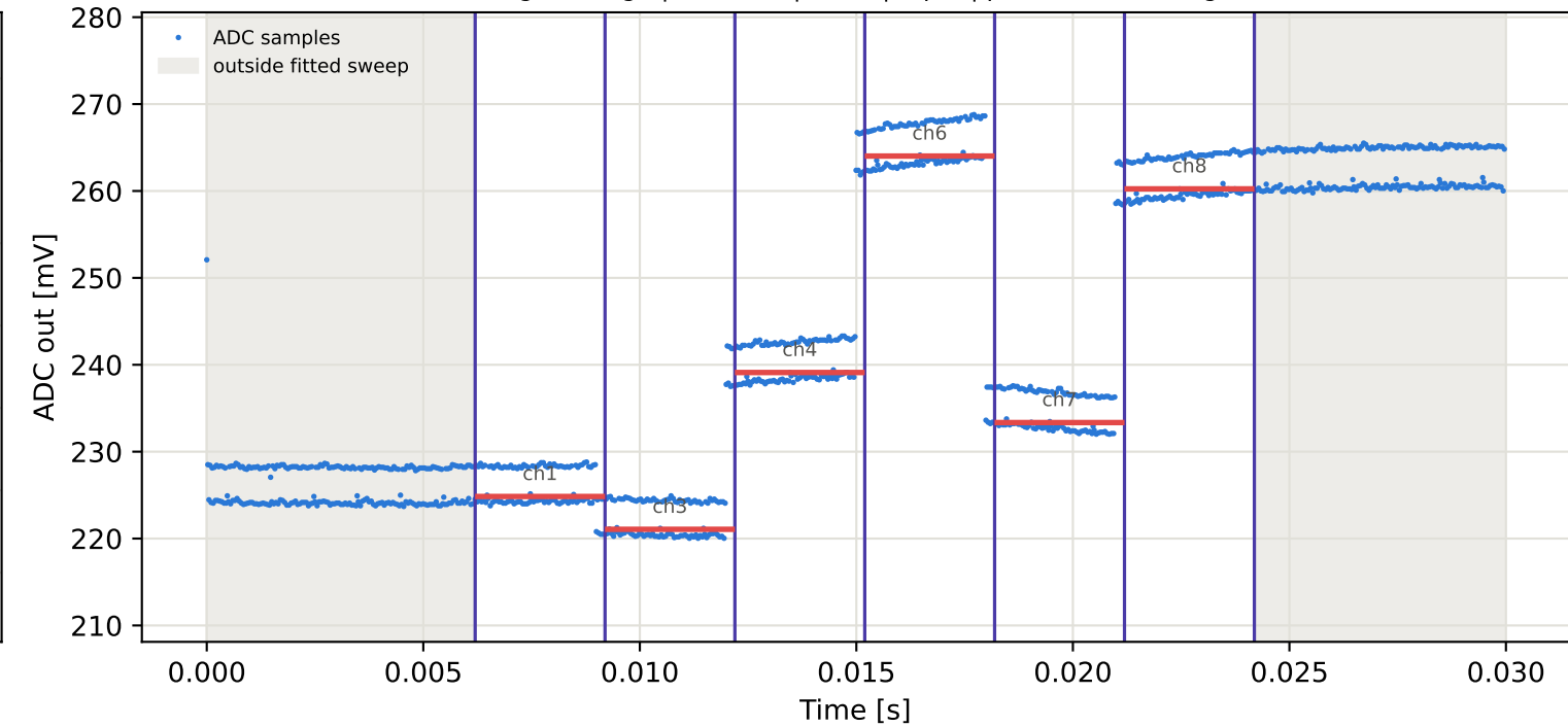
Tag1 &lt;- Tag8 | 865 MHz | run 0 | rep 1 | phase -96.24 deg
