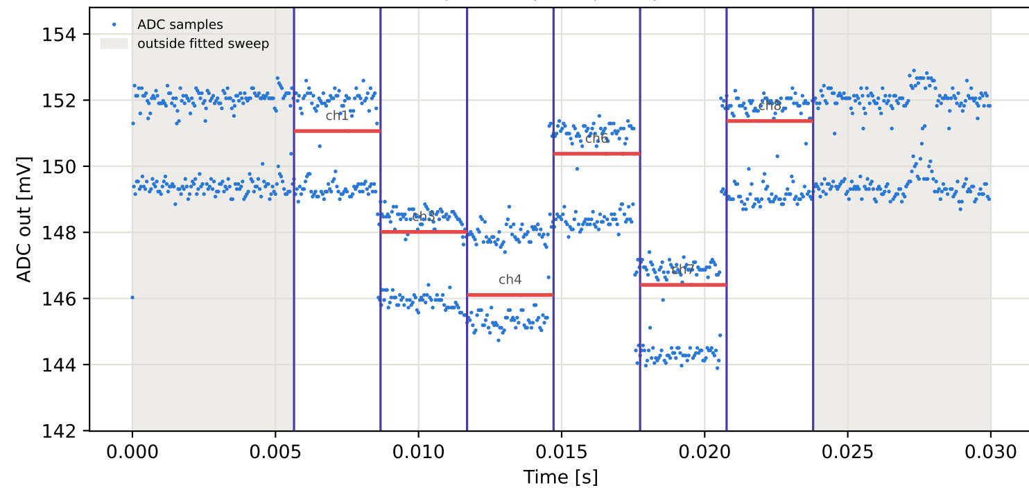
Tag15 &lt;- Tag10 | 805 MHz | run 0 | rep 1 | phase 122.85 deg
