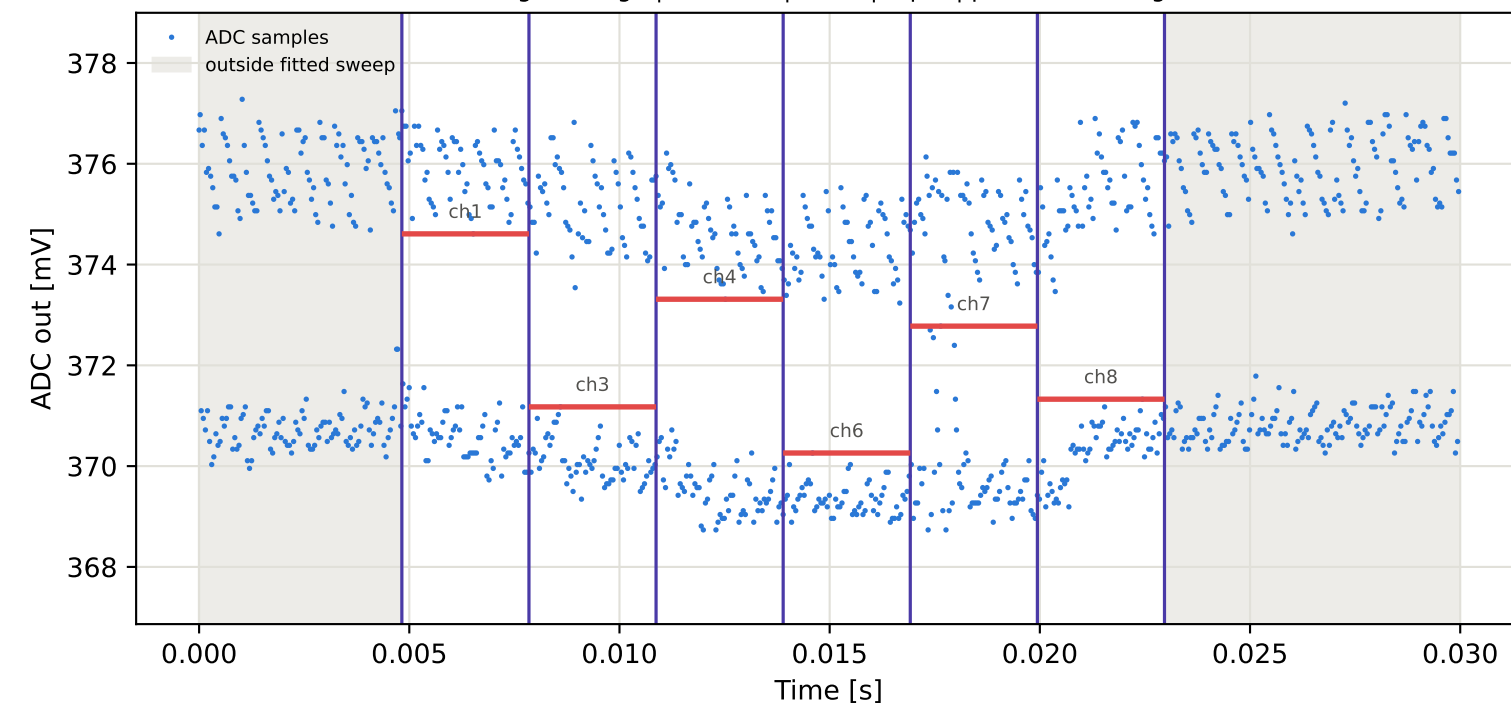
Tag4 &lt;- Tag2 | 945 MHz | run 0 | rep 1 | phase -1.23 deg
