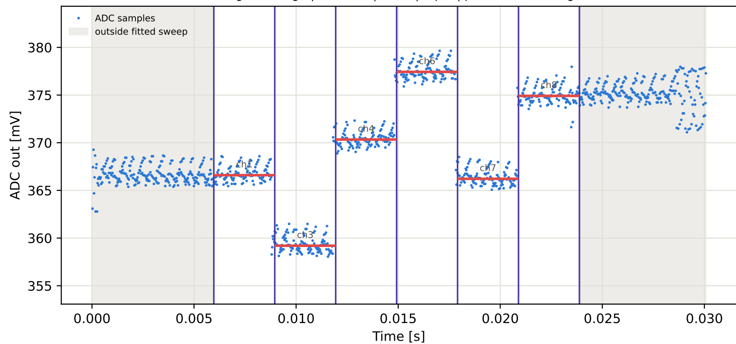
Tag15 &lt;- Tag6 | 825 MHz | run 0 | rep 1 | phase -156.86 deg
