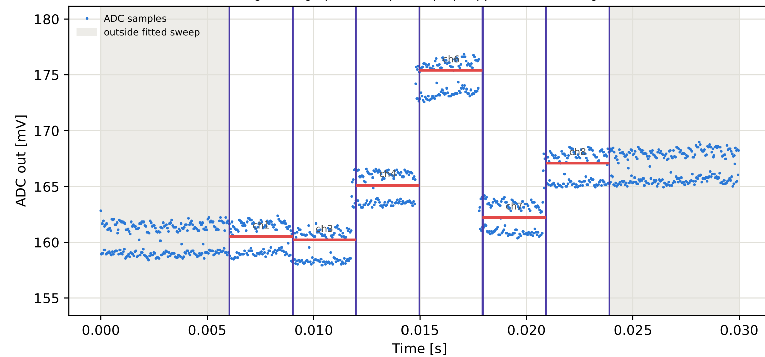
Tag4 &lt;- Tag15 | 935 MHz | run 0 | rep 1 | phase -20.14 deg
