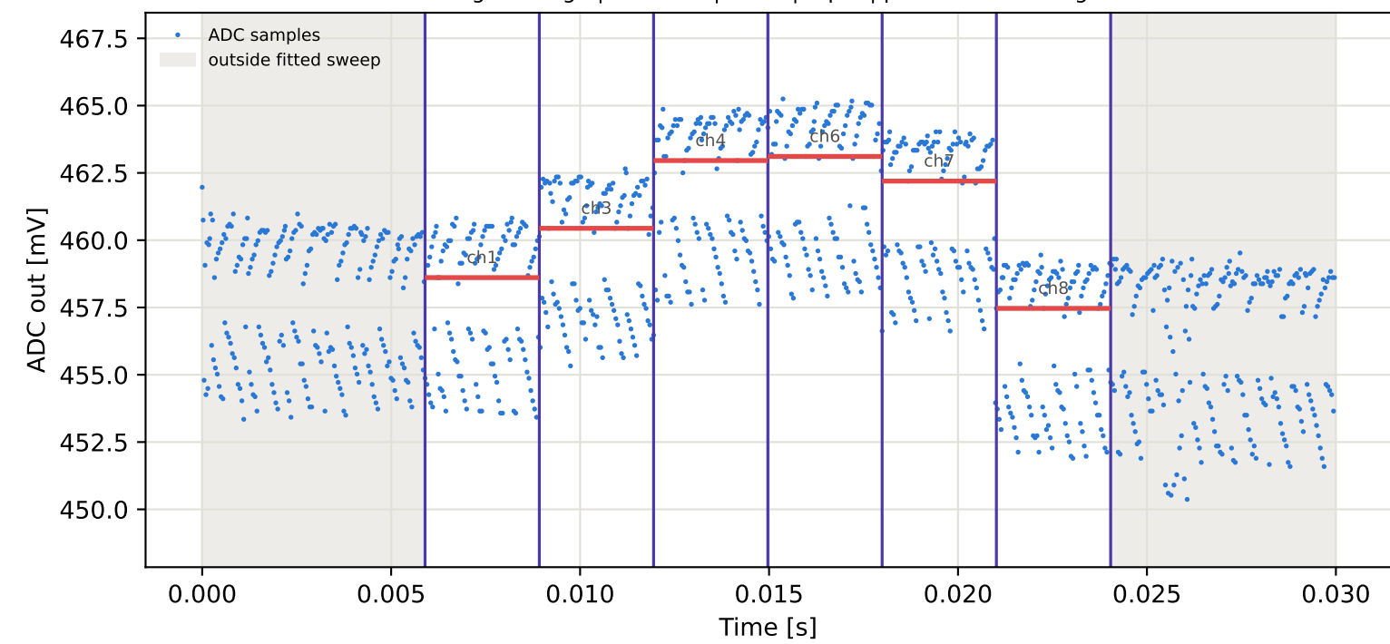
Tag7 &lt;- Tag4 | 915 MHz | run 0 | rep 1 | phase 16.09 deg
