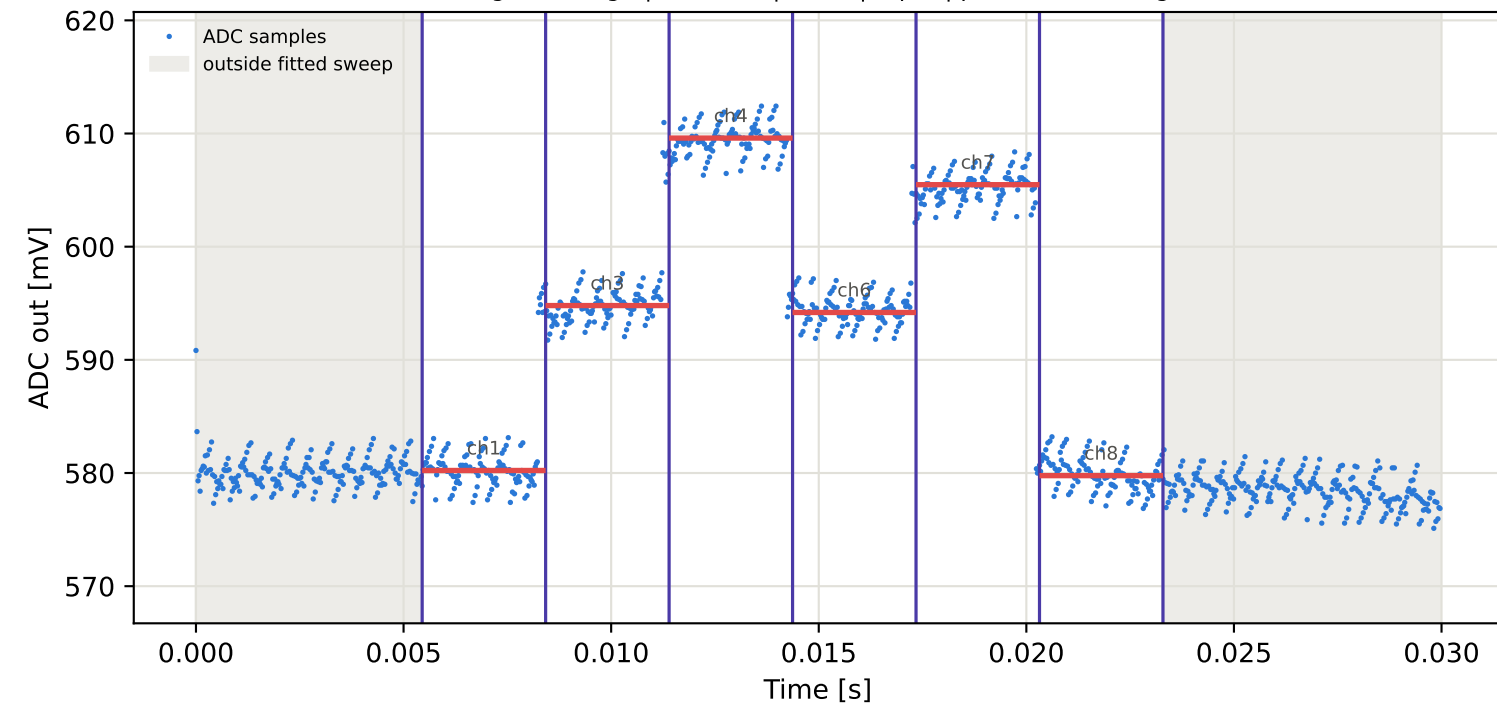
Tag10 &lt;- Tag9 | 915 MHz | run 0 | rep 1 | phase -103.41 deg
