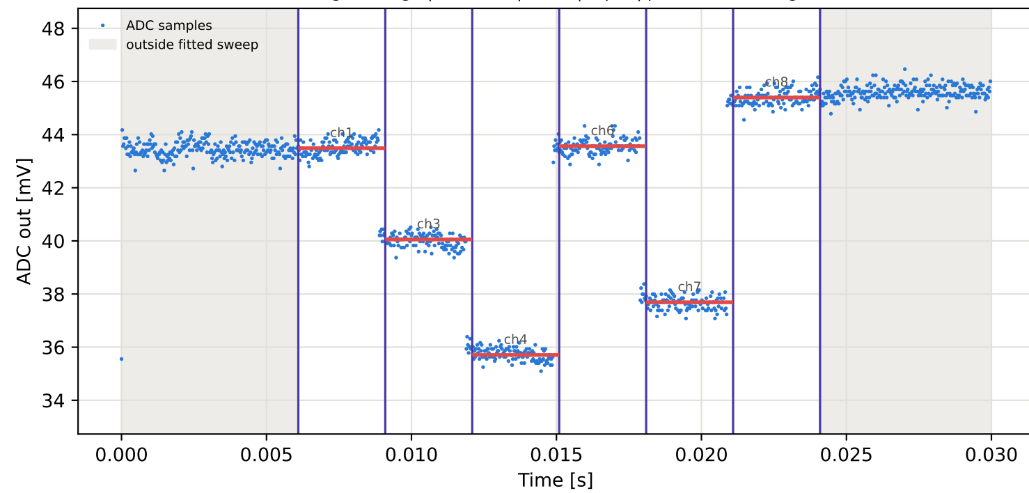
Tag3 &lt;- Tag10 | 955 MHz | run 0 | rep 1 | phase 11.29 deg
