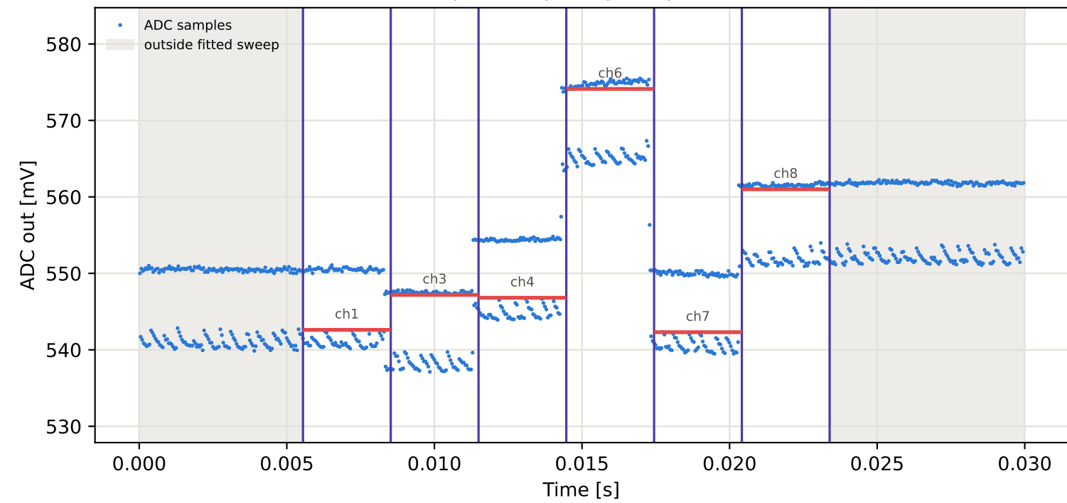
Tag7 &lt;- Tag15 | 955 MHz | run 0 | rep 1 | phase -178.21 deg
