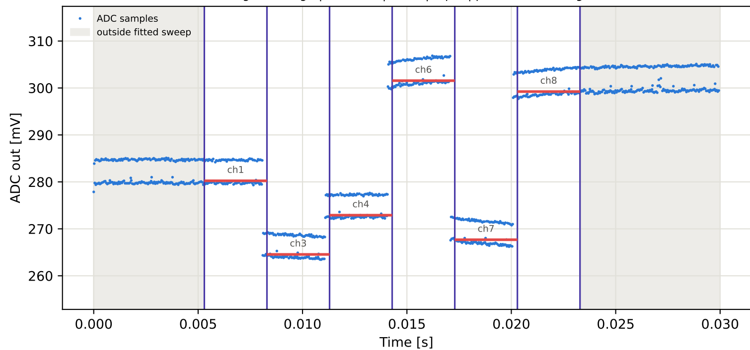
Tag16 &lt;- Tag7 | 835 MHz | run 0 | rep 1 | phase 174.60 deg
