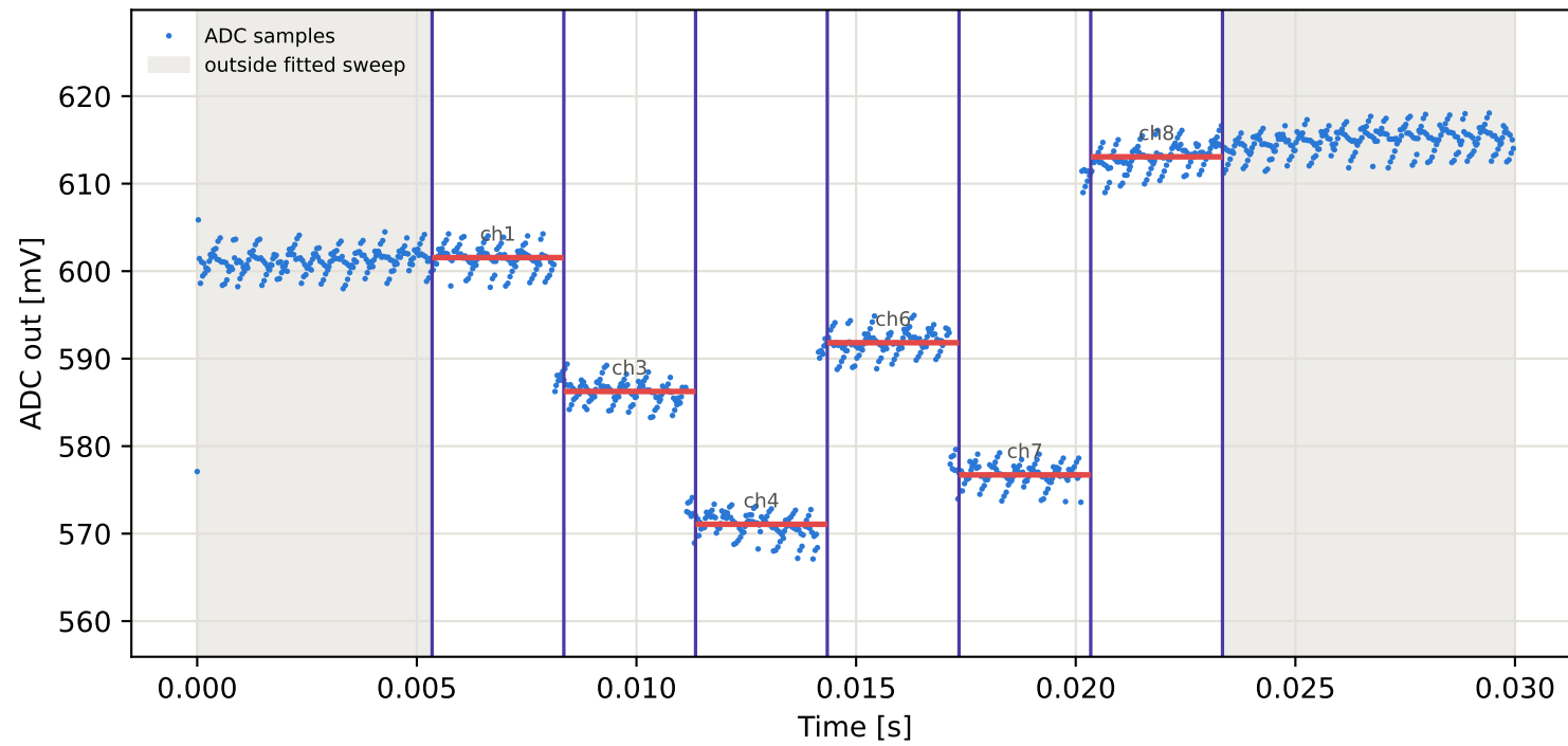
Tag15 &lt;- Tag1 | 915 MHz | run 0 | rep 1 | phase -117.62 deg
