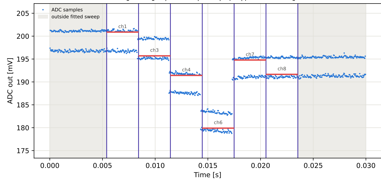
Tag1 &lt;- Tag2 | 935 MHz | run 0 | rep 1 | phase 122.79 deg
