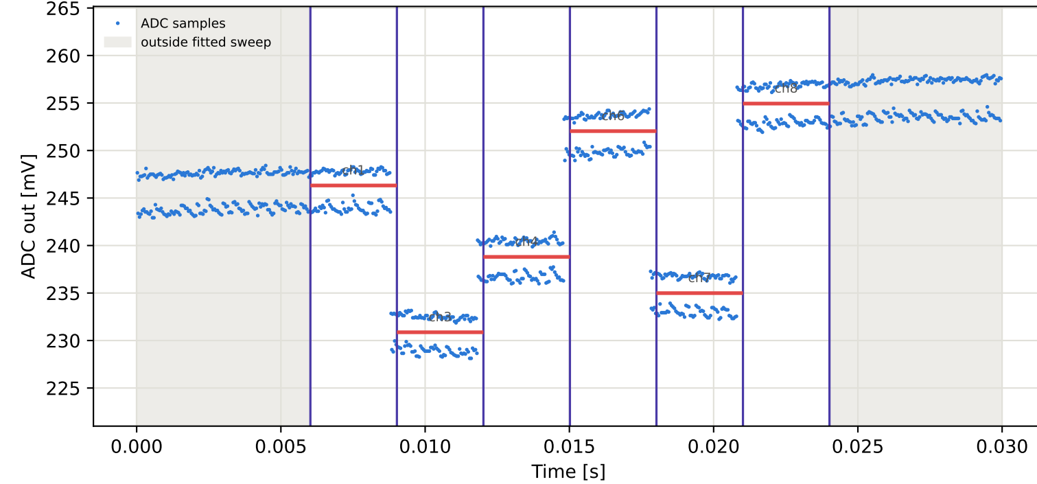
Tag9 &lt;- Tag16 | 845 MHz | run 0 | rep 1 | phase -89.64 deg
