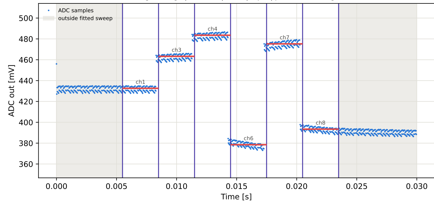
Tag3 &lt;- Tag7 | 935 MHz | run 0 | rep 1 | phase -141.02 deg
