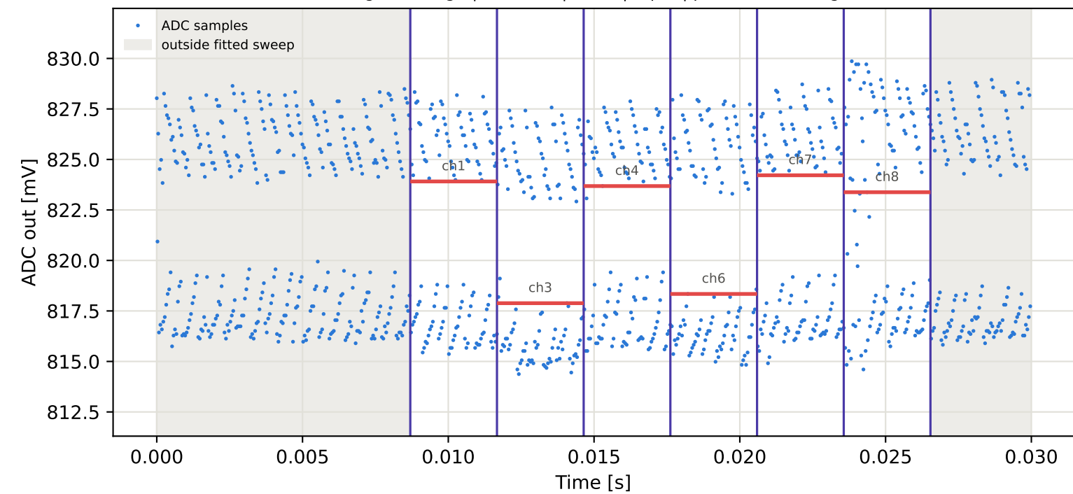
Tag16 &lt;- Tag4 | 985 MHz | run 0 | rep 1 | phase 145.56 deg
