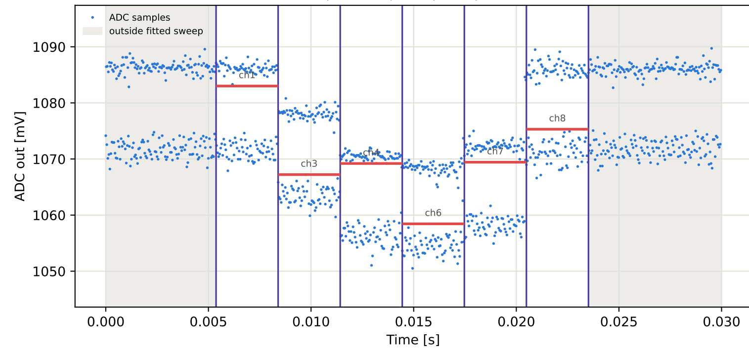
Tag3 &lt;- Tag2 | 885 MHz | run 0 | rep 1 | phase 48.16 deg
