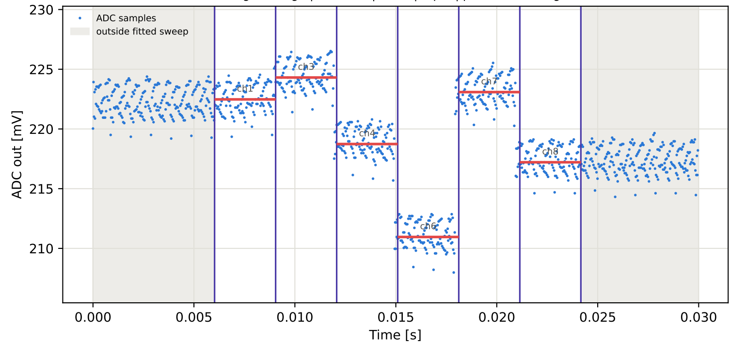
Tag6 &lt;- Tag5 | 995 MHz | run 0 | rep 1 | phase 10.73 deg
