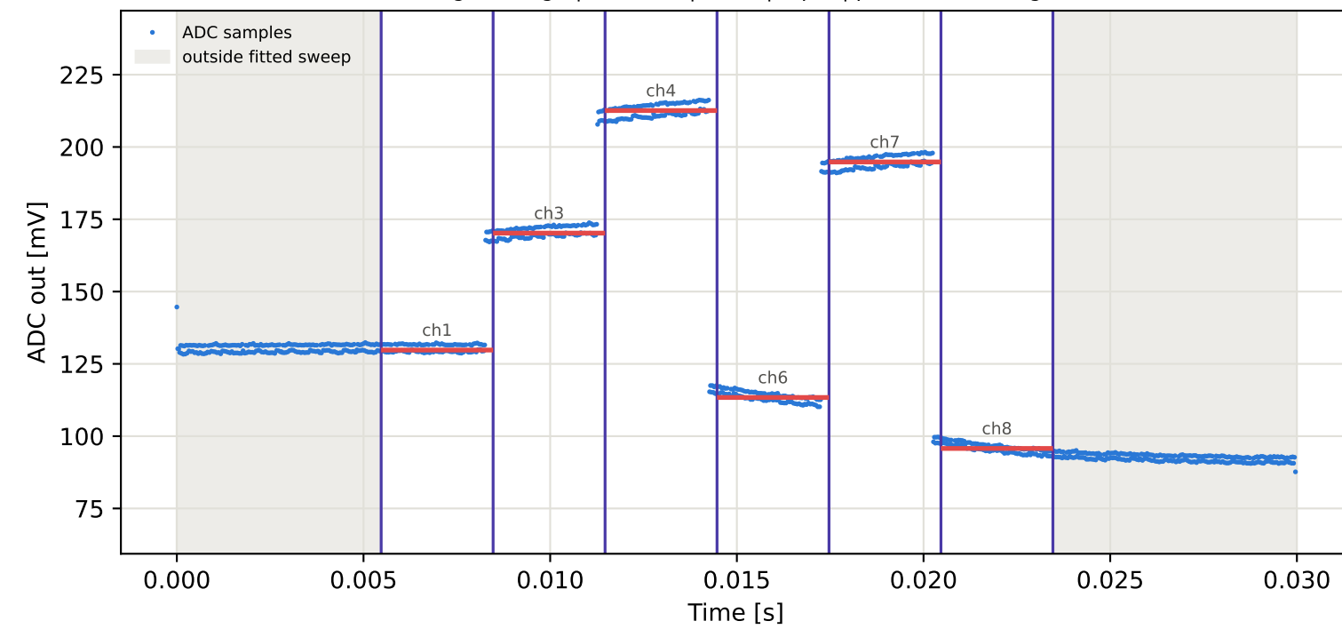
Tag4 &lt;- Tag7 | 935 MHz | run 0 | rep 1 | phase -106.22 deg
