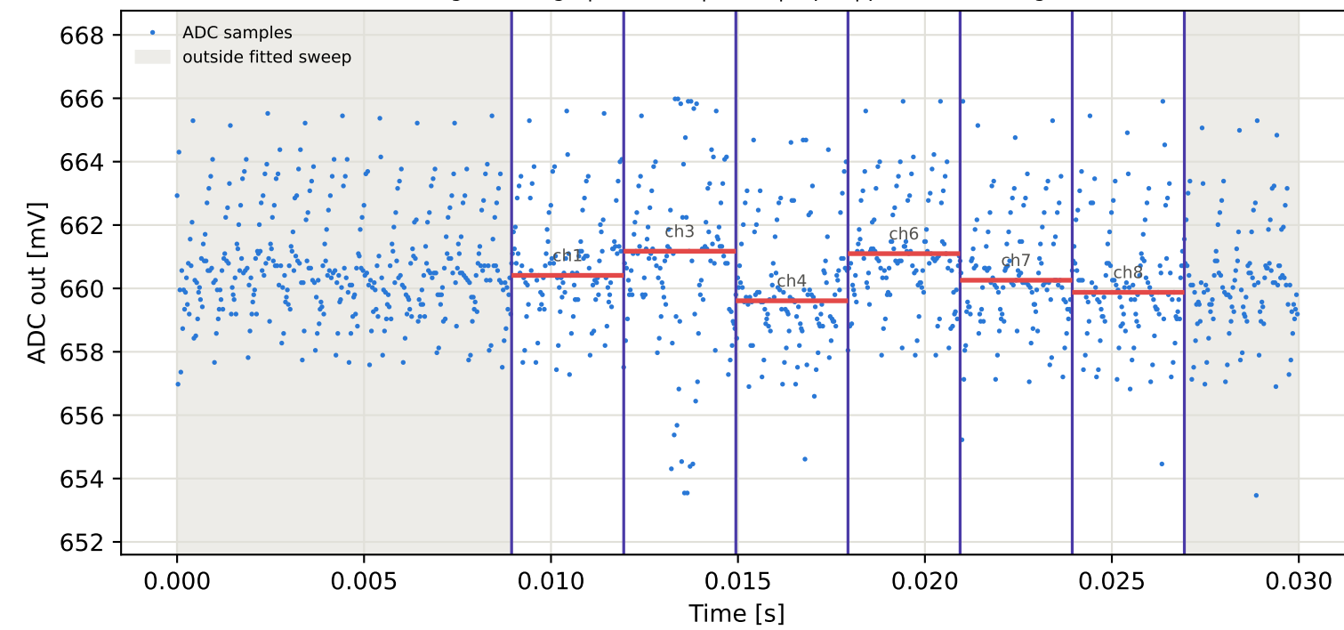
Tag16 &lt;- Tag4 | 965 MHz | run 0 | rep 1 | phase 29.03 deg
