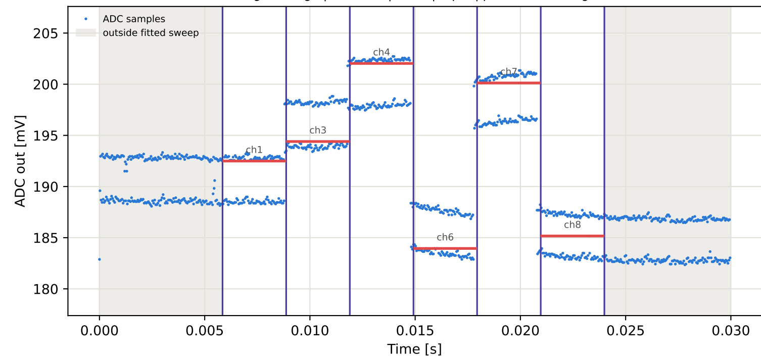
Tag1 &lt;- Tag4 | 935 MHz | run 0 | rep 1 | phase -47.41 deg
