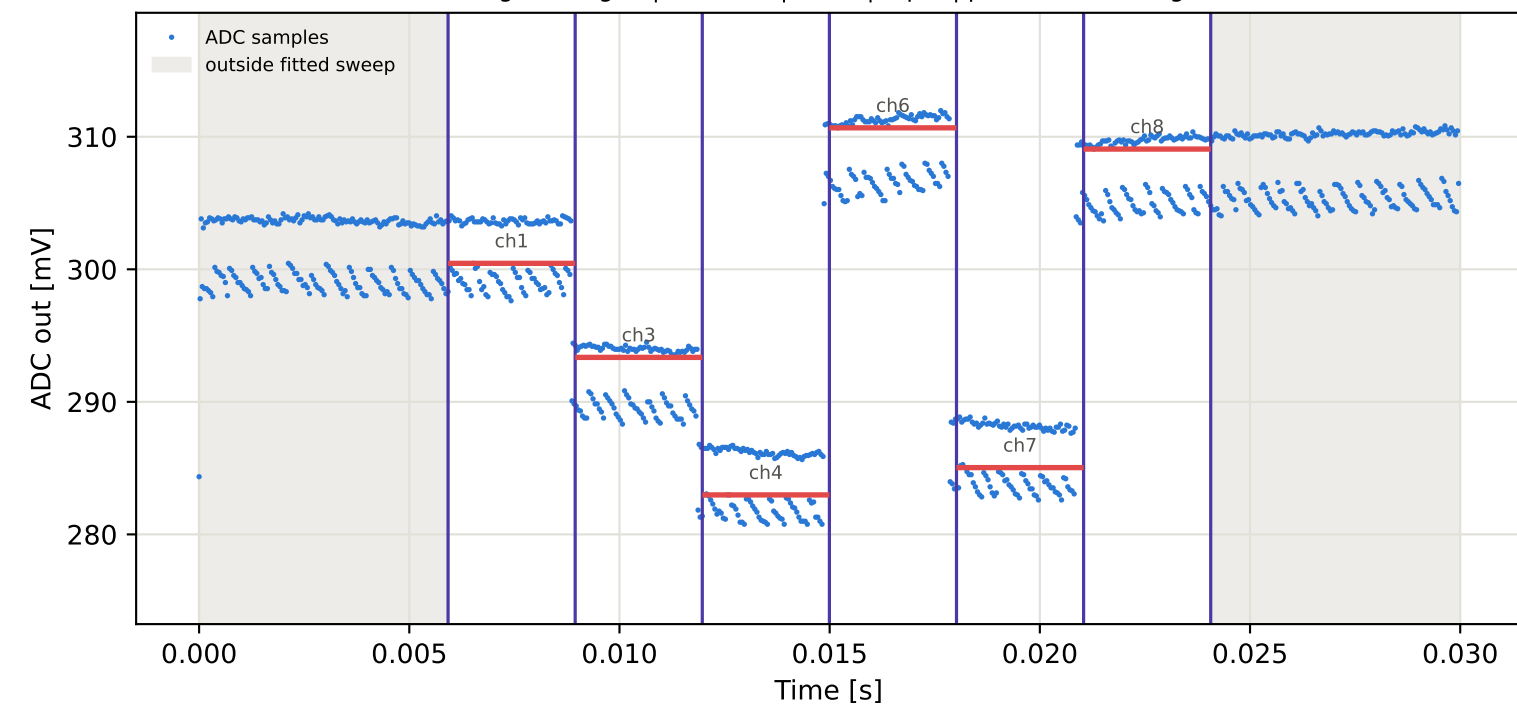
Tag9 &lt;- Tag16 | 995 MHz | run 0 | rep 1 | phase 123.39 deg
