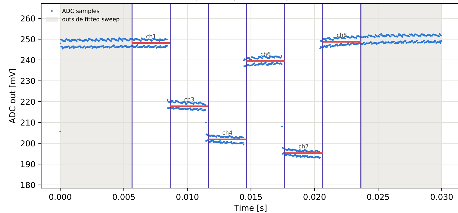
Tag4 &lt;- Tag7 | 805 MHz | run 0 | rep 1 | phase -45.37 deg
