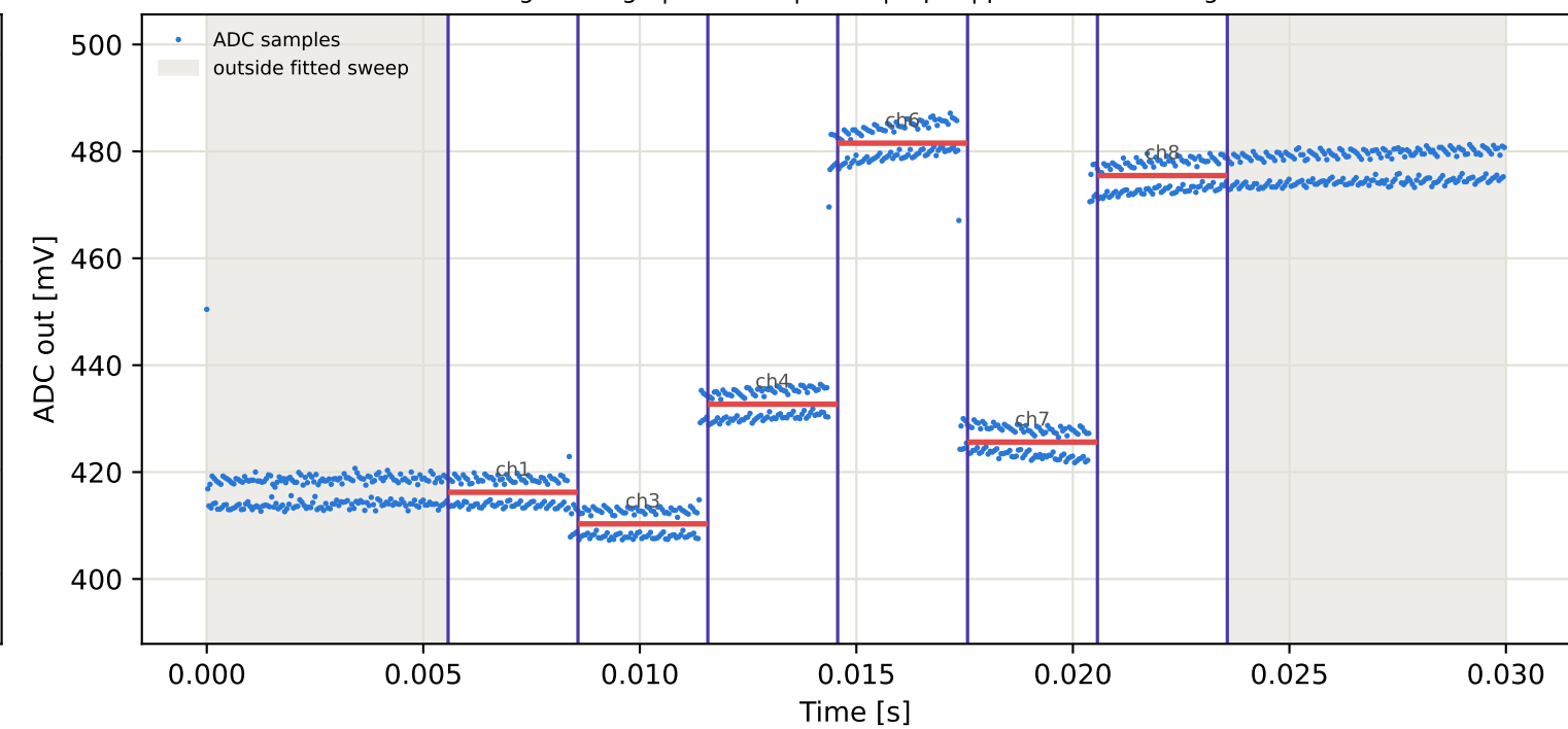
Tag1 &lt;- Tag8 | 875 MHz | run 0 | rep 1 | phase 170.39 deg
