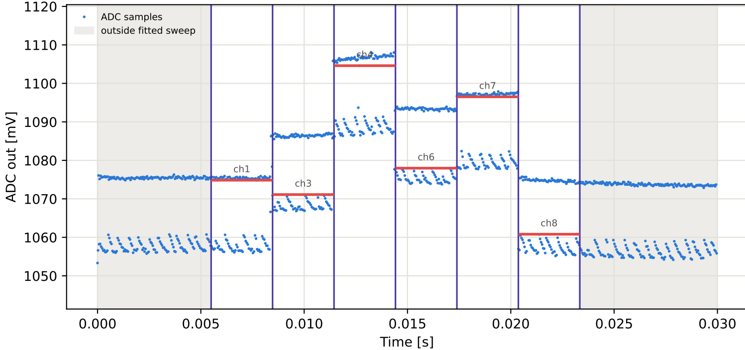
Tag8 &lt;- Tag16 | 935 MHz | run 0 | rep 1 | phase 136.78 deg
