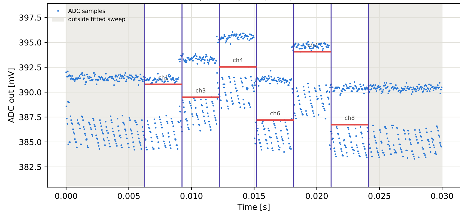
Tag9 &lt;- Tag15 | 965 MHz | run 0 | rep 1 | phase 0.05 deg
