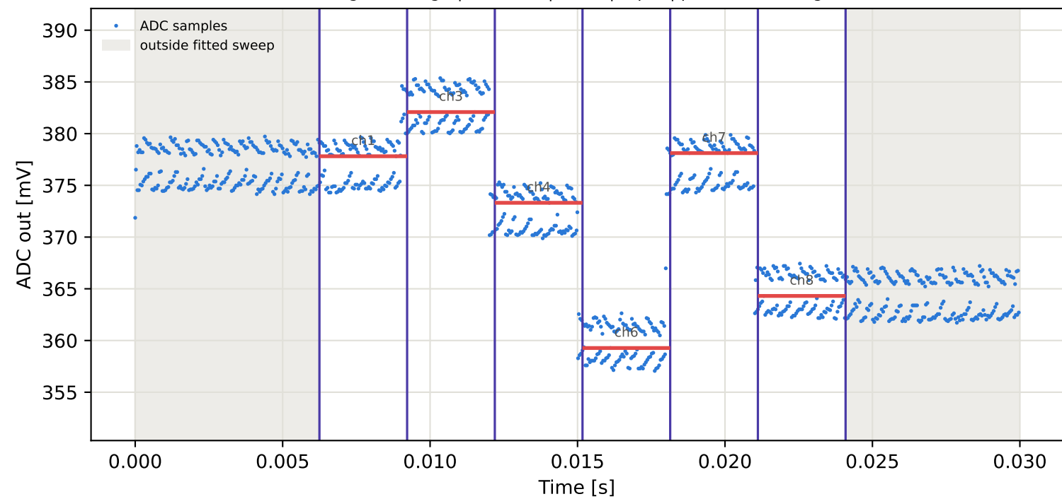
Tag15 &lt;- Tag9 | 825 MHz | run 0 | rep 1 | phase 63.33 deg
