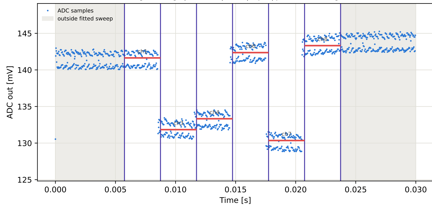
Tag10 &lt;- Tag8 | 805 MHz | run 0 | rep 1 | phase -105.88 deg
