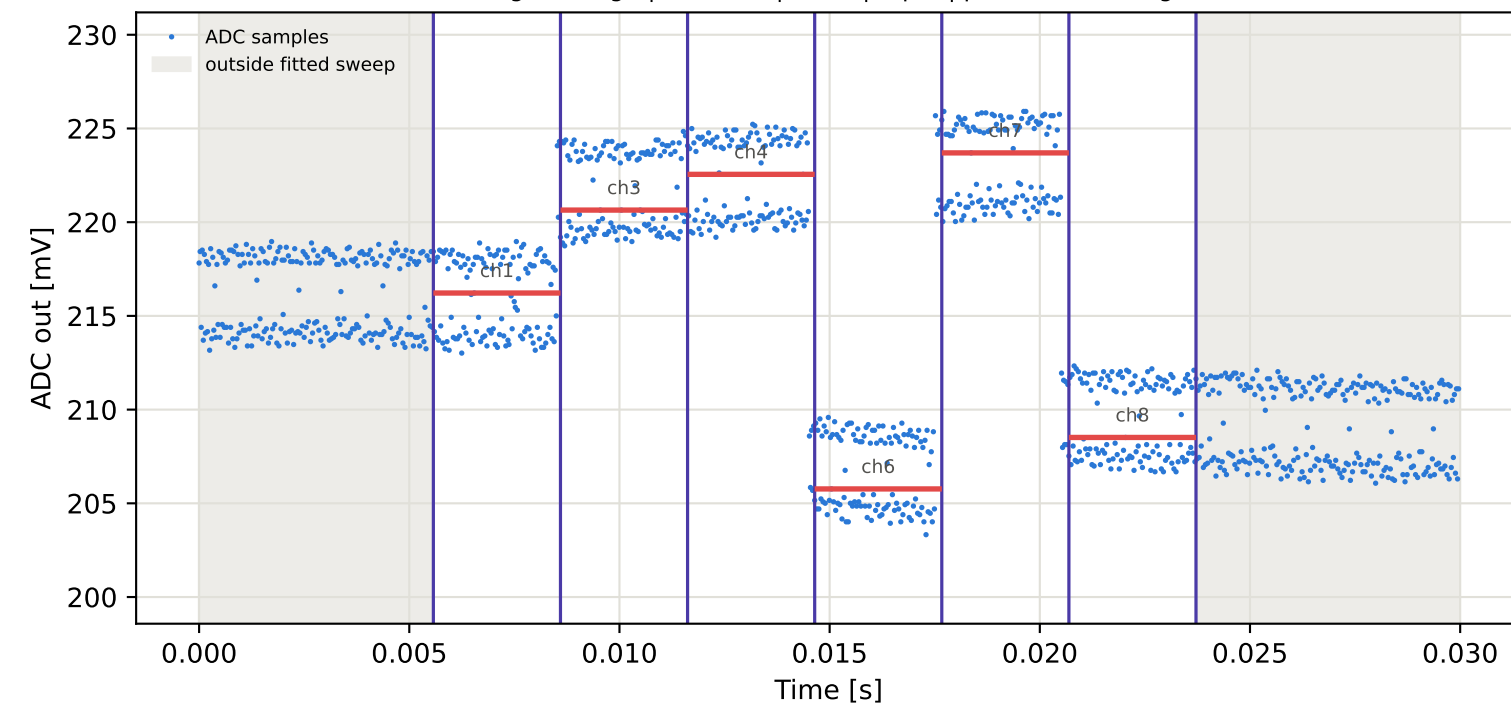
Tag1 &lt;- Tag9 | 985 MHz | run 0 | rep 1 | phase -1.33 deg
