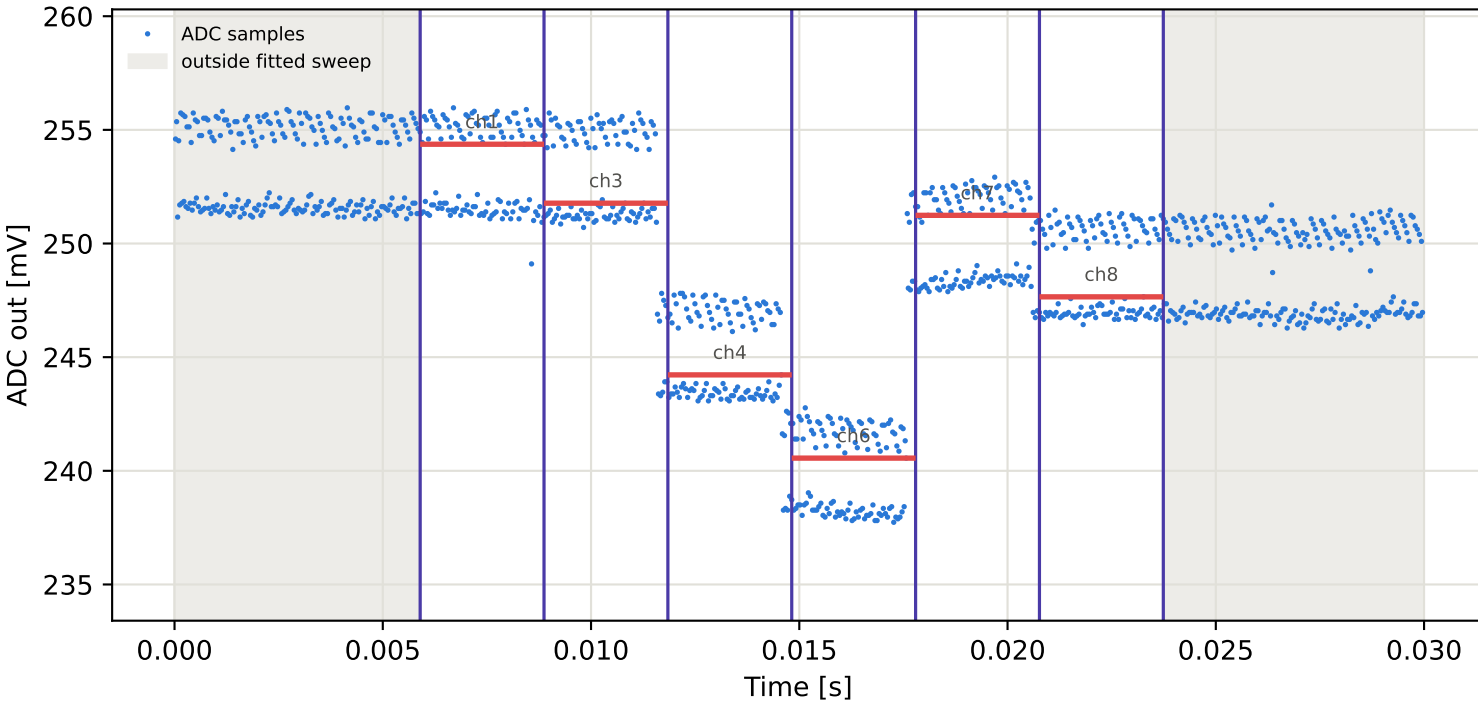
Tag3 &lt;- Tag16 | 965 MHz | run 0 | rep 1 | phase -68.14 deg
