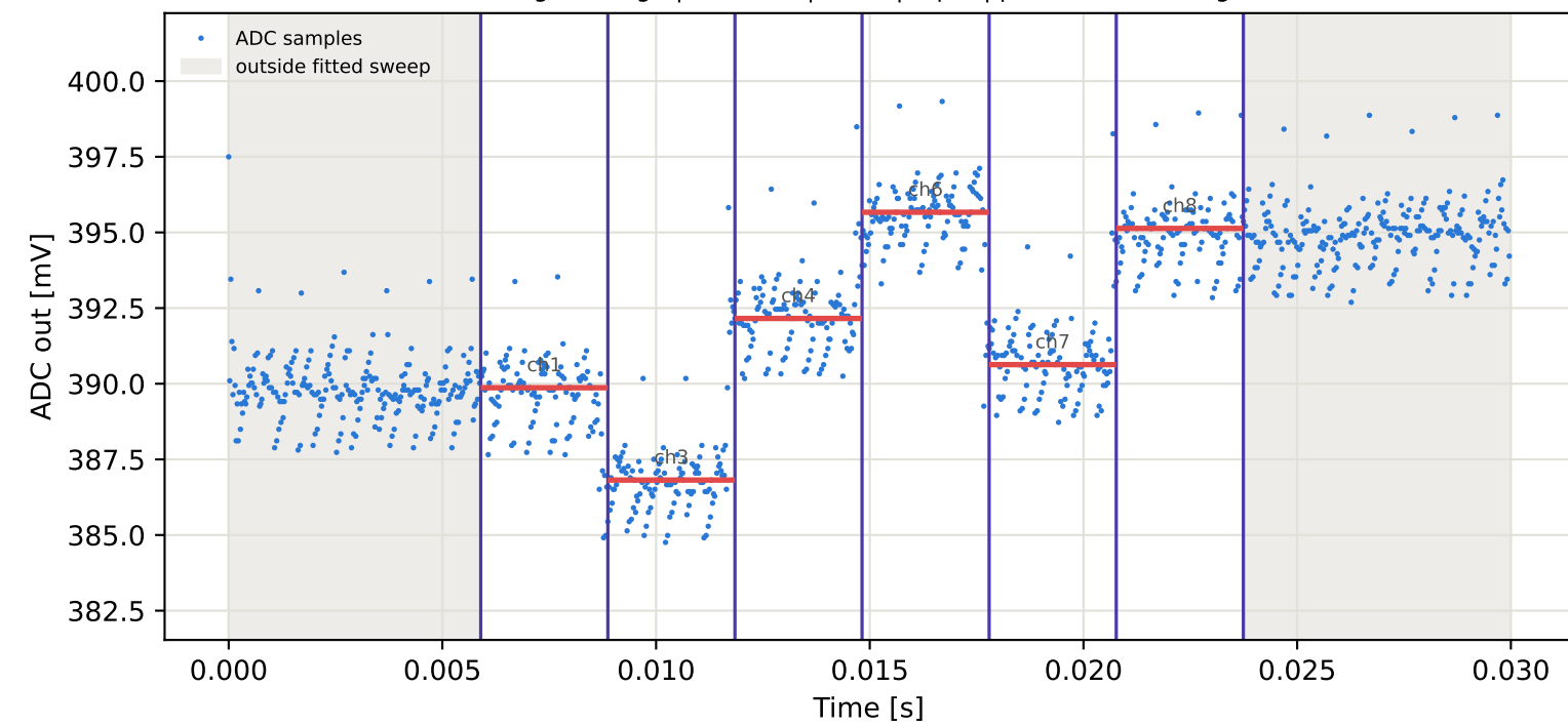
Tag6 &lt;- Tag5 | 845 MHz | run 0 | rep 1 | phase -157.39 deg
