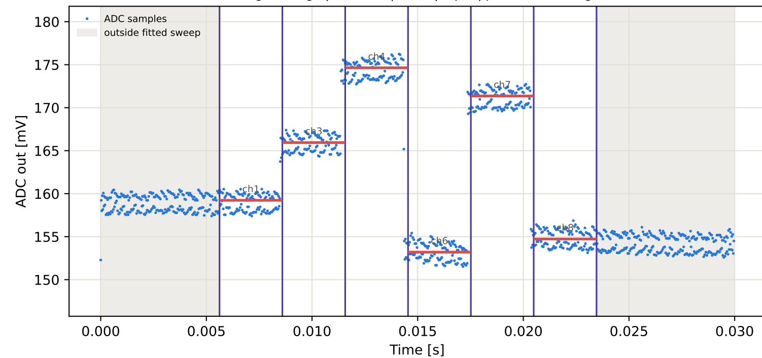
Tag6 &lt;- Tag1 | 995 MHz | run 0 | rep 1 | phase 168.99 deg
