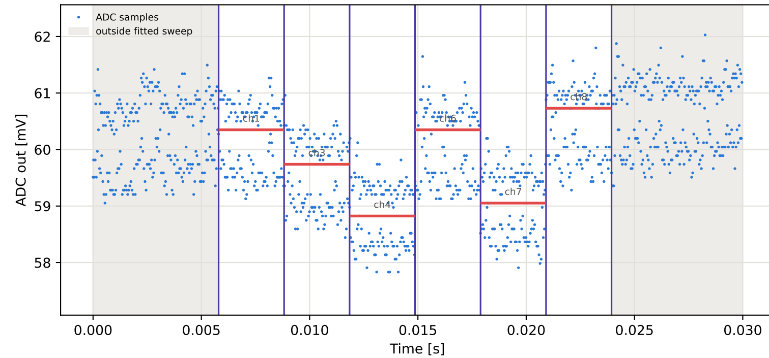
Tag6 &lt;- Tag4 | 785 MHz | run 0 | rep 1 | phase 77.66 deg
