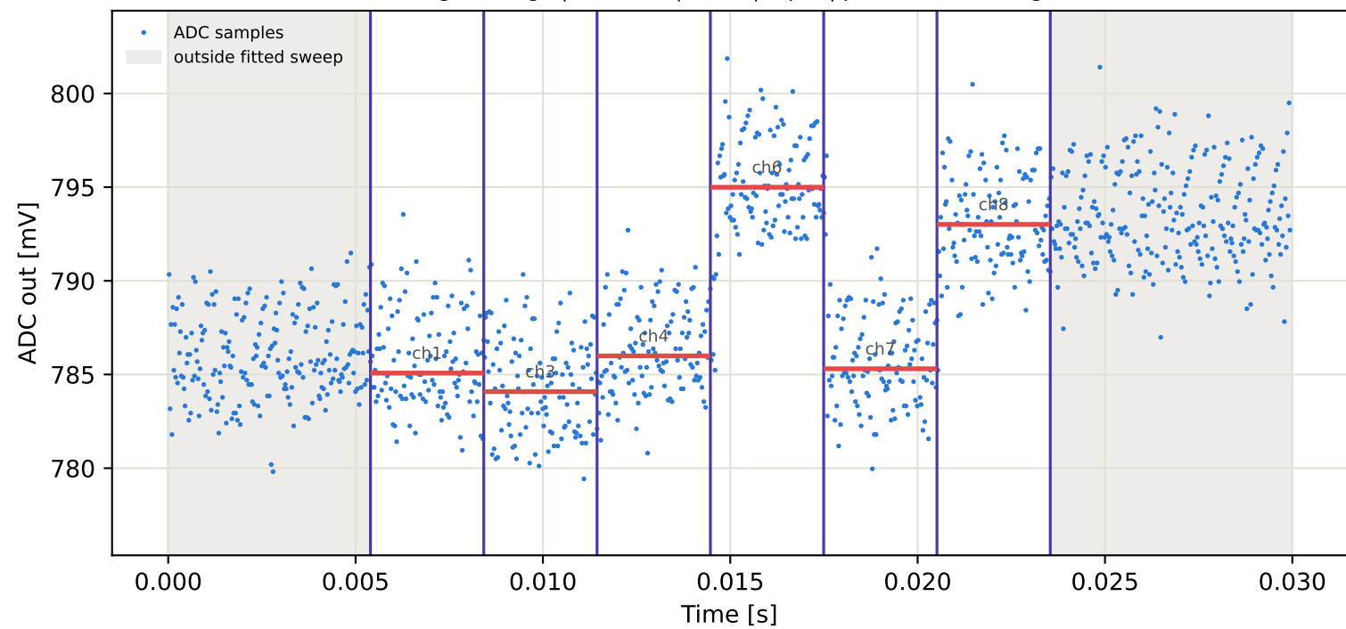
Tag9 &lt;- Tag6 | 885 MHz | run 0 | rep 1 | phase -173.50 deg
