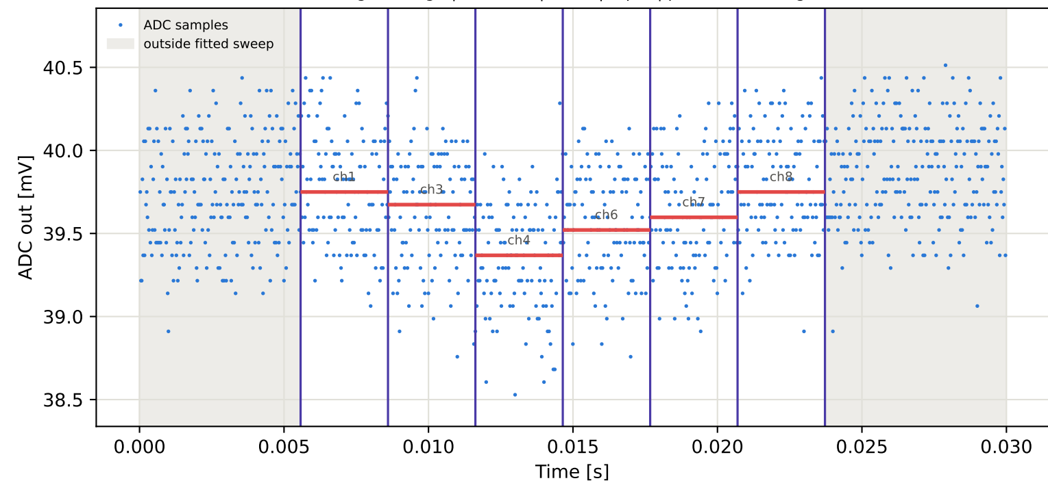
Tag2 &lt;- Tag6 | 985 MHz | run 0 | rep 1 | phase -126.01 deg
