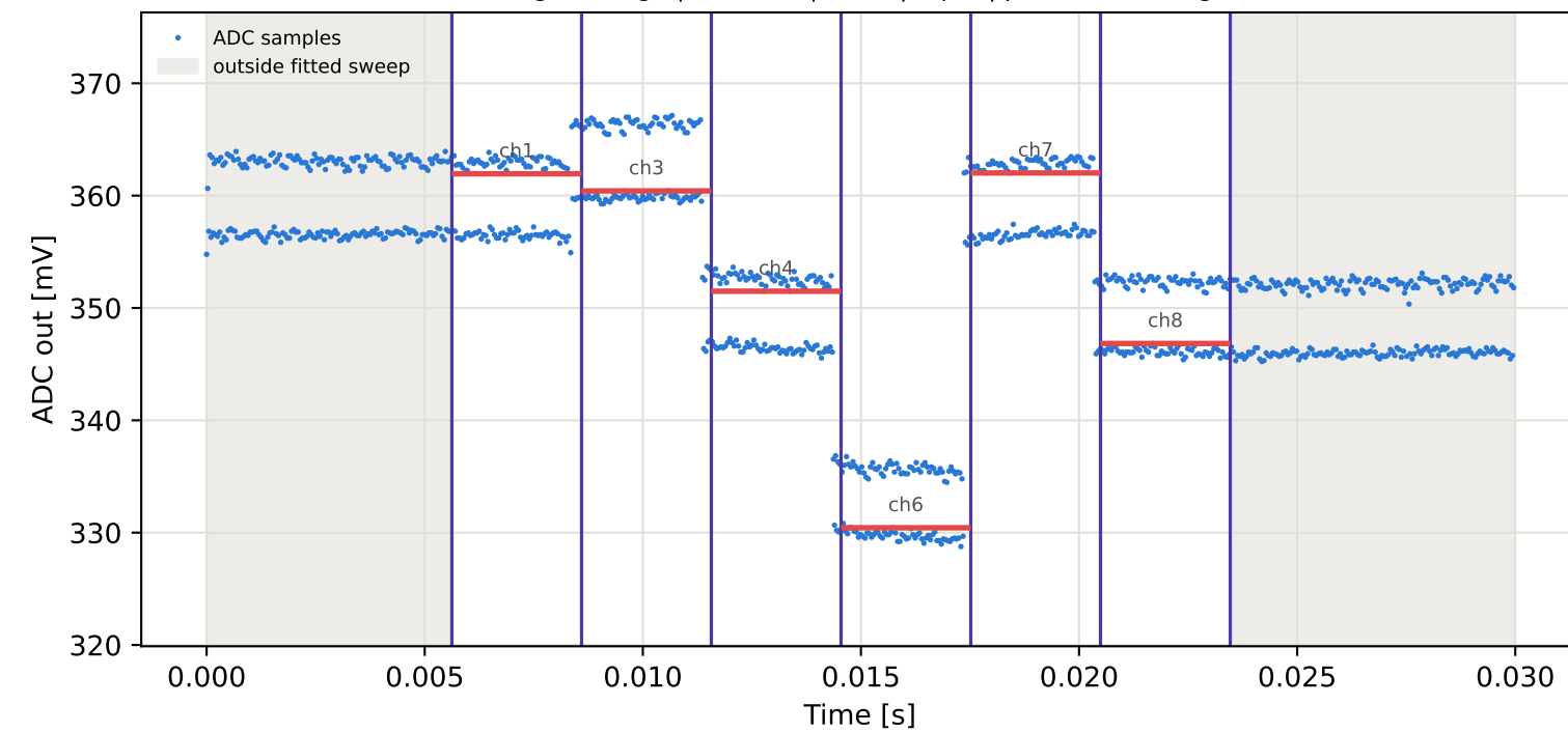
Tag9 &lt;- Tag5 | 985 MHz | run 0 | rep 1 | phase 79.74 deg
