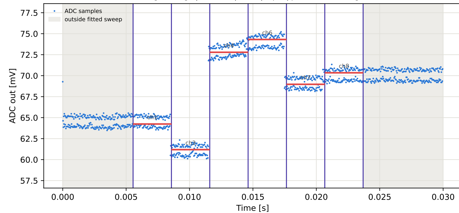
Tag1 &lt;- Tag7 | 805 MHz | run 0 | rep 1 | phase 118.54 deg
