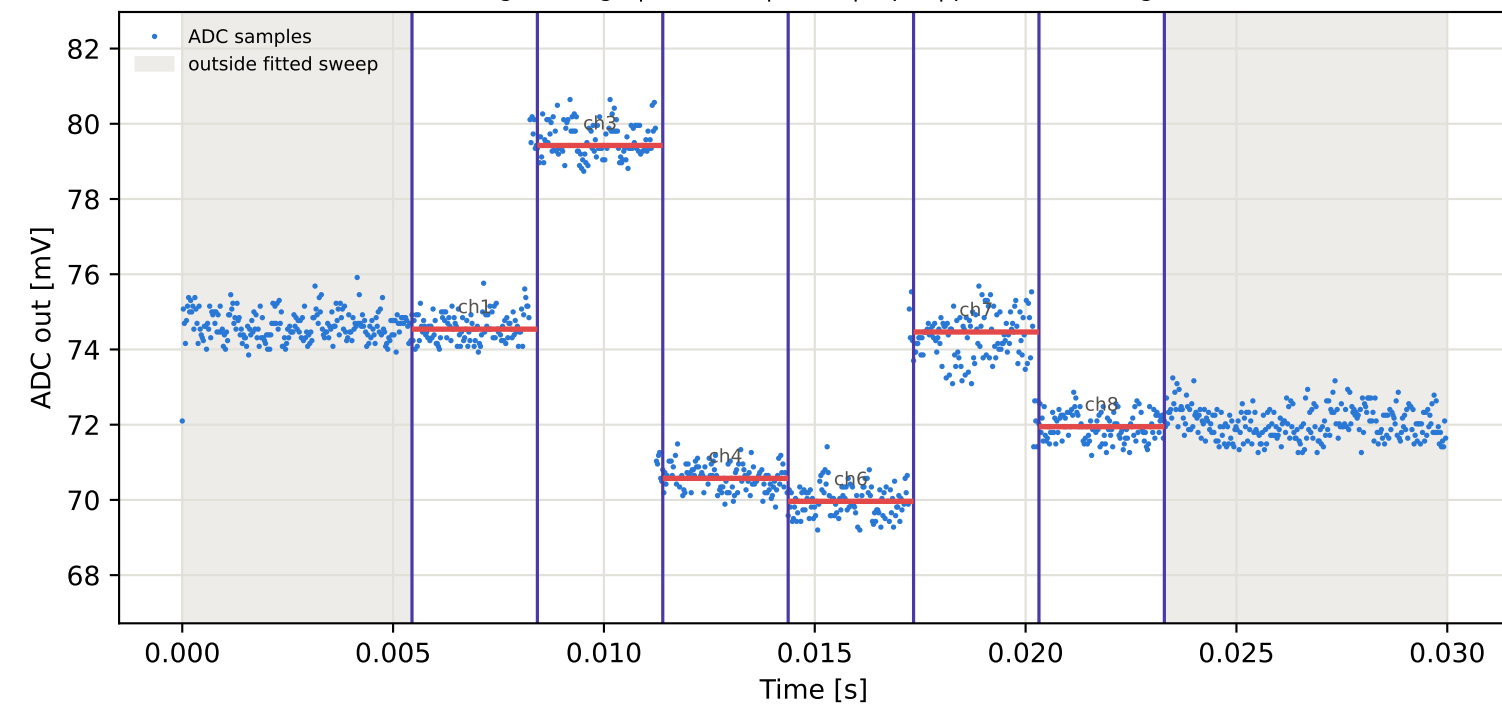
Tag9 &lt;- Tag5 | 795 MHz | run 0 | rep 1 | phase 53.80 deg
