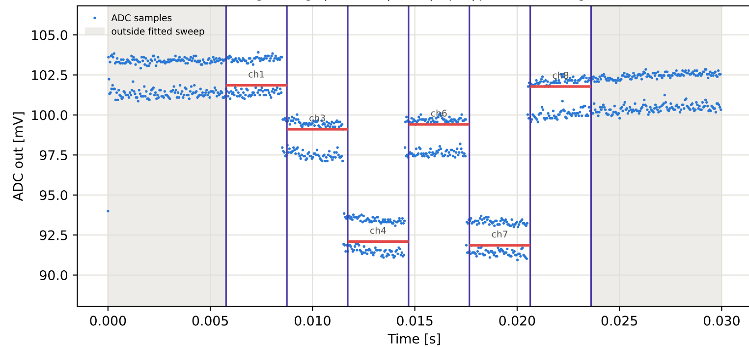
Tag3 &lt;- Tag7 | 795 MHz | run 0 | rep 1 | phase 150.34 deg
