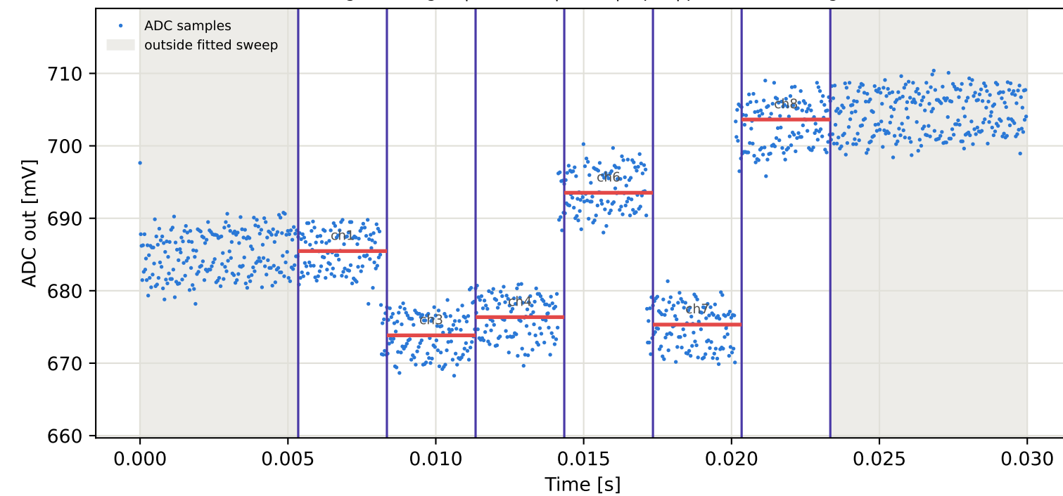
Tag10 &lt;- Tag2 | 885 MHz | run 0 | rep 1 | phase 3.81 deg
