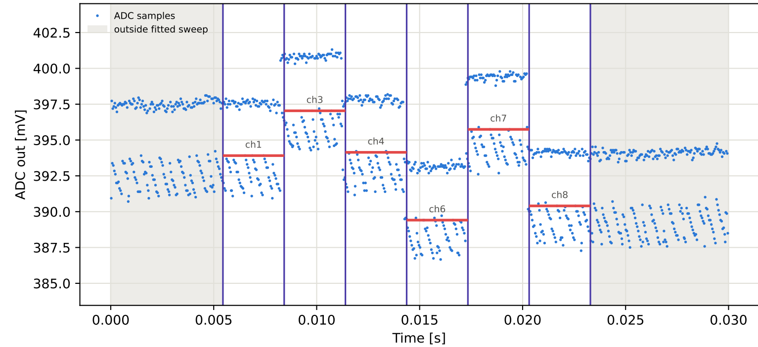
Tag16 &lt;- Tag10 | 835 MHz | run 0 | rep 1 | phase 173.92 deg
