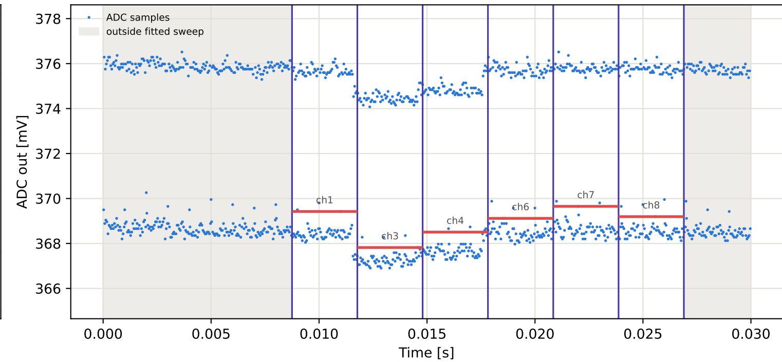
Tag15 &lt;- Tag6 | 995 MHz | run 0 | rep 1 | phase 71.20 deg
