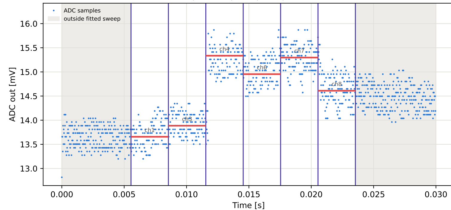
Tag2 &lt;- Tag7 | 795 MHz | run 0 | rep 1 | phase -108.19 deg
