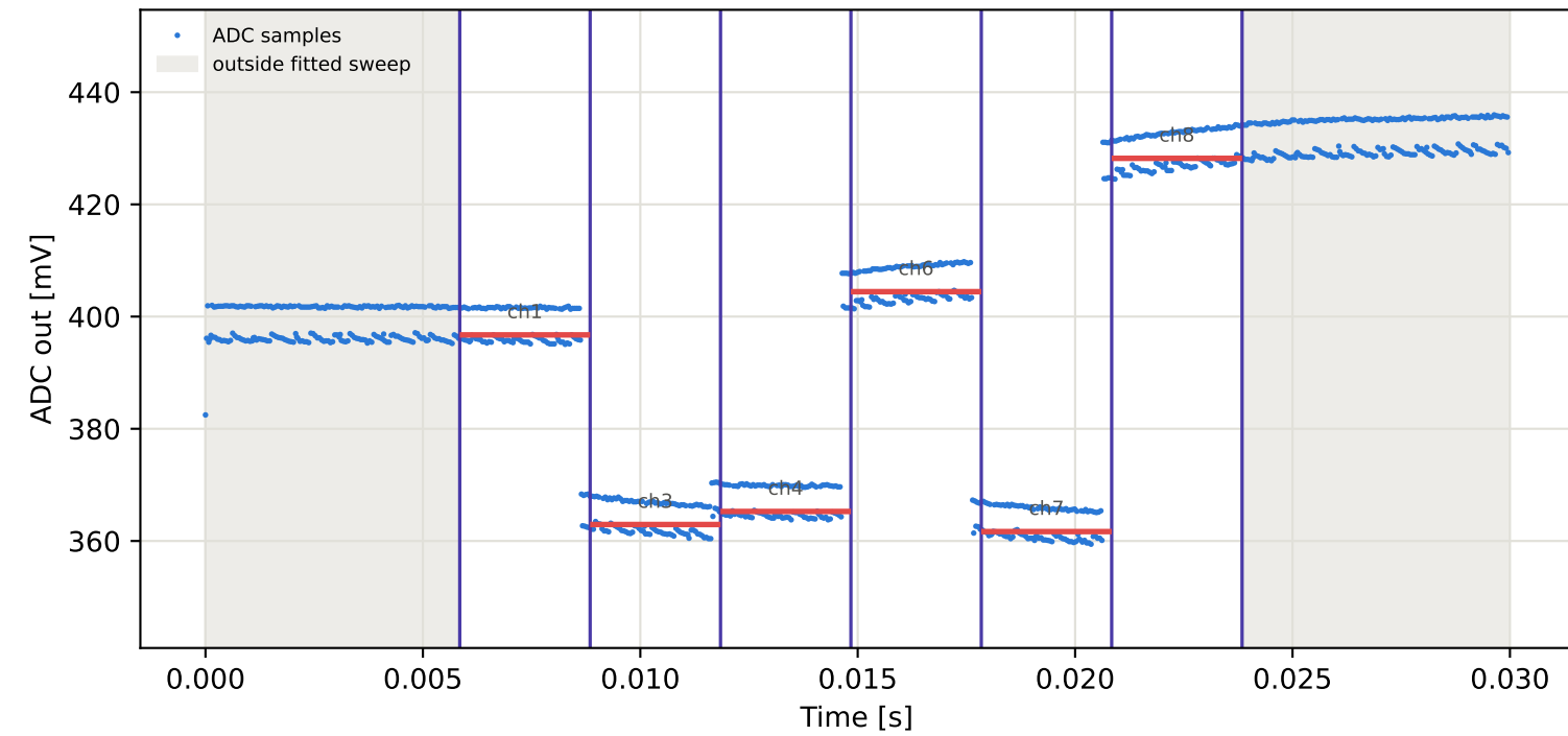
Tag10 &lt;- Tag5 | 865 MHz | run 0 | rep 1 | phase 74.13 deg
