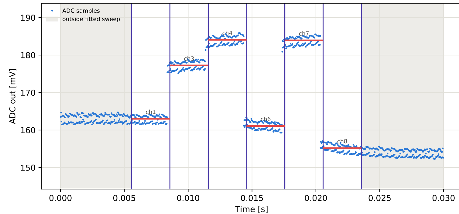
Tag9 &lt;- Tag7 | 865 MHz | run 0 | rep 1 | phase -53.91 deg
