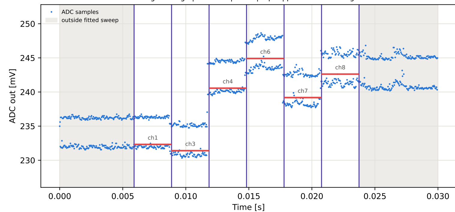
Tag9 &lt;- Tag7 | 845 MHz | run 0 | rep 1 | phase -85.84 deg
