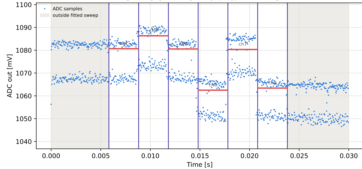
Tag3 &lt;- Tag15 | 885 MHz | run 0 | rep 1 | phase -152.86 deg
