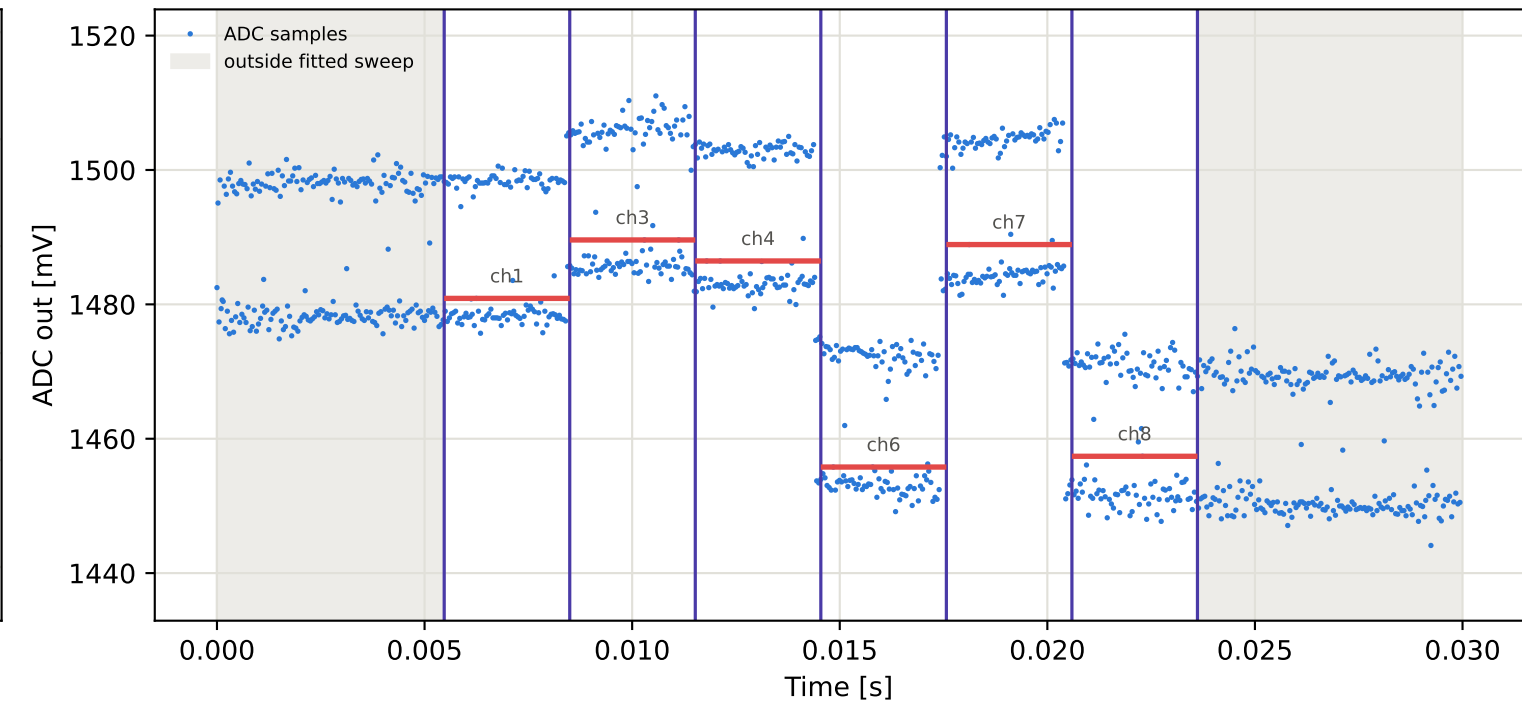
Tag5 &lt;- Tag4 | 885 MHz | run 0 | rep 1 | phase 11.61 deg
