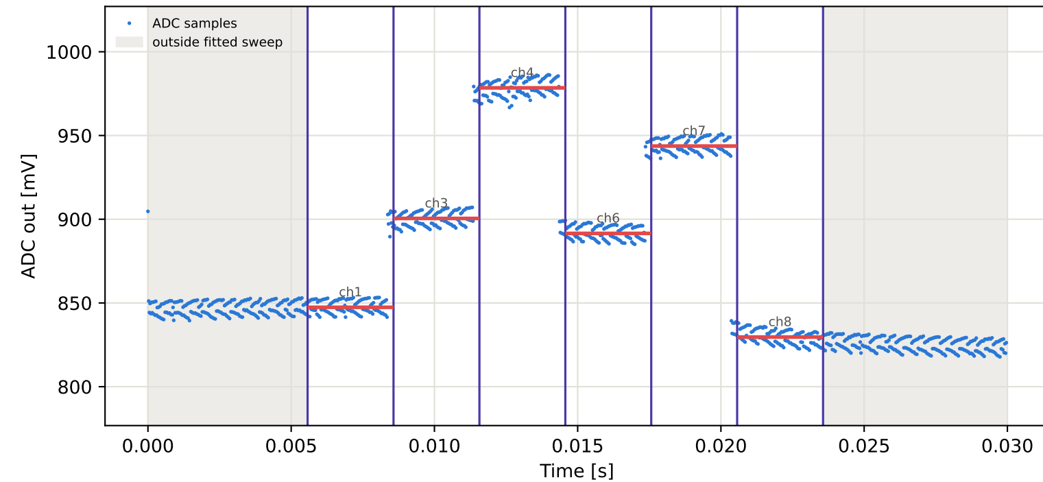
Tag9 &lt;- Tag16 | 935 MHz | run 0 | rep 1 | phase 72.14 deg
