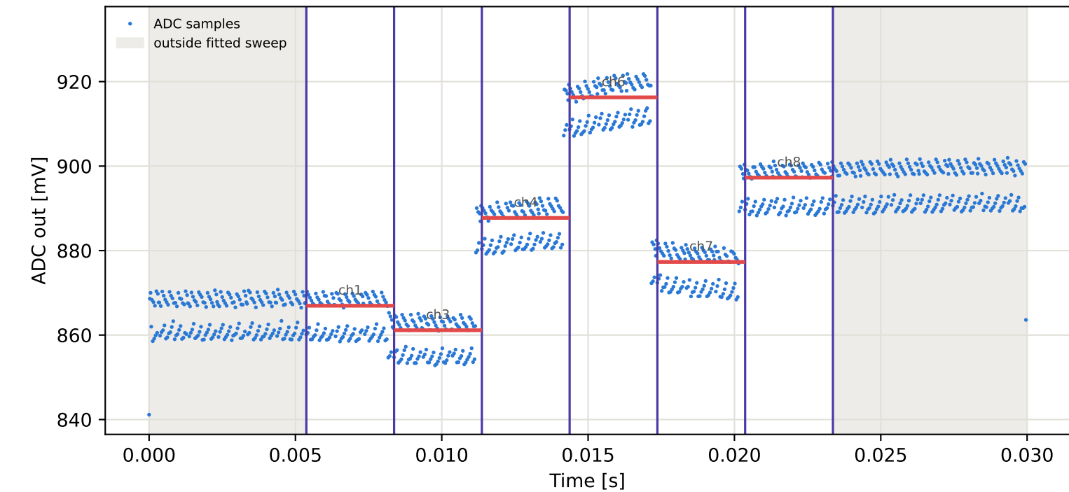
Tag3 &lt;- Tag9 | 895 MHz | run 0 | rep 1 | phase -4.42 deg
