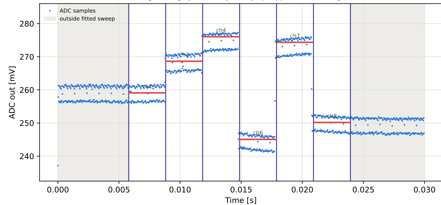
Tag3 &lt;- Tag8 | 975 MHz | run 0 | rep 1 | phase -47.55 deg
