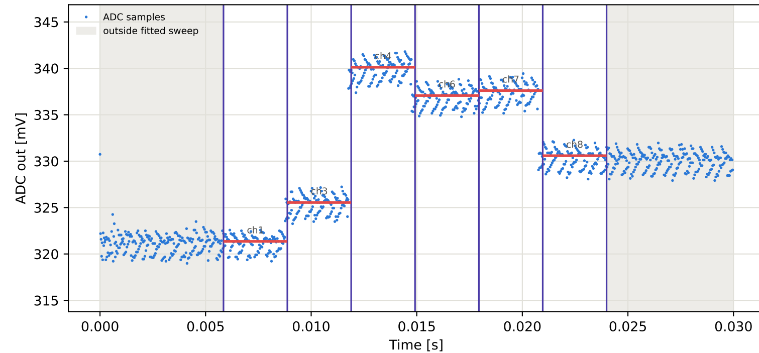
Tag4 &lt;- Tag2 | 845 MHz | run 0 | rep 1 | phase -123.03 deg
