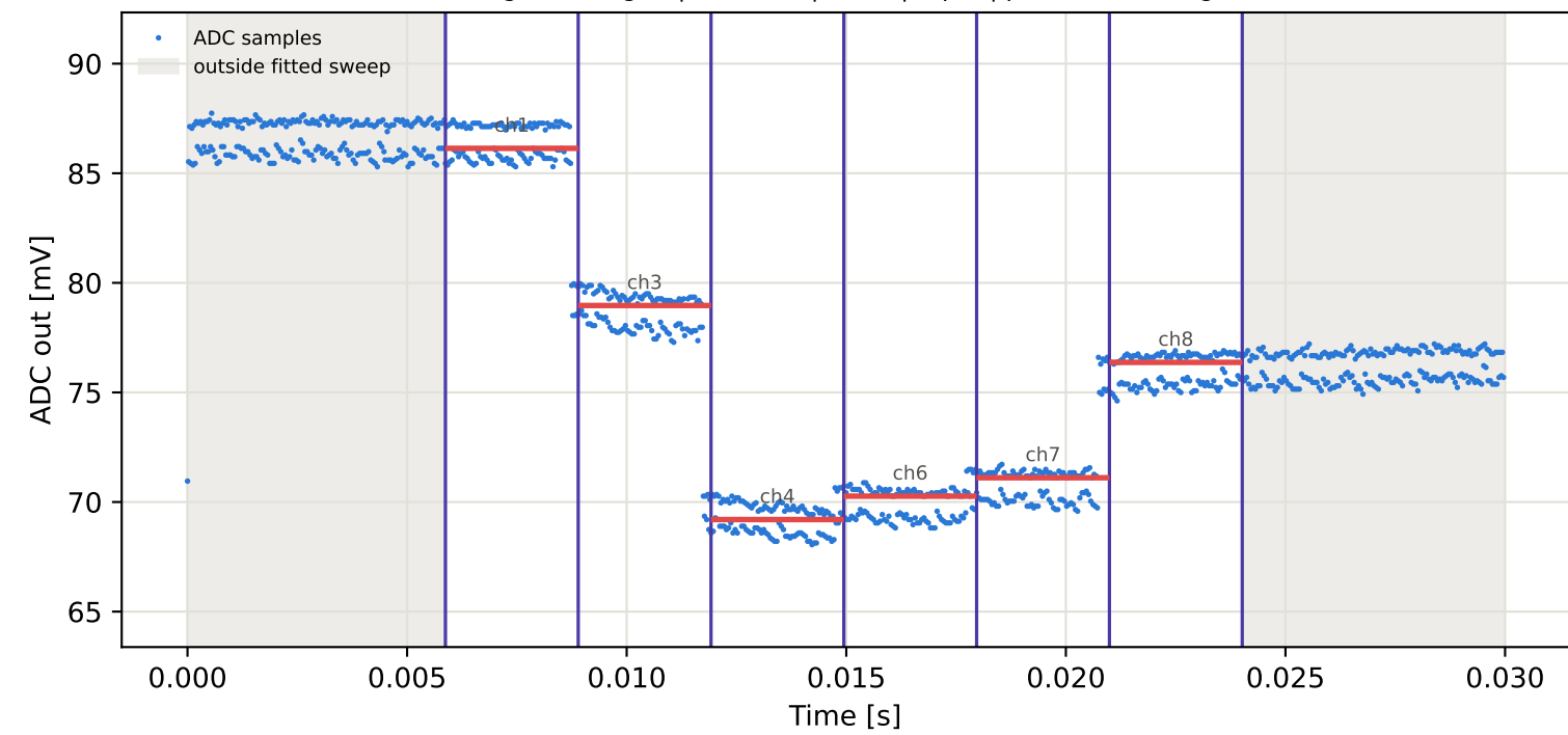
Tag10 &lt;- Tag3 | 855 MHz | run 0 | rep 1 | phase 87.05 deg
