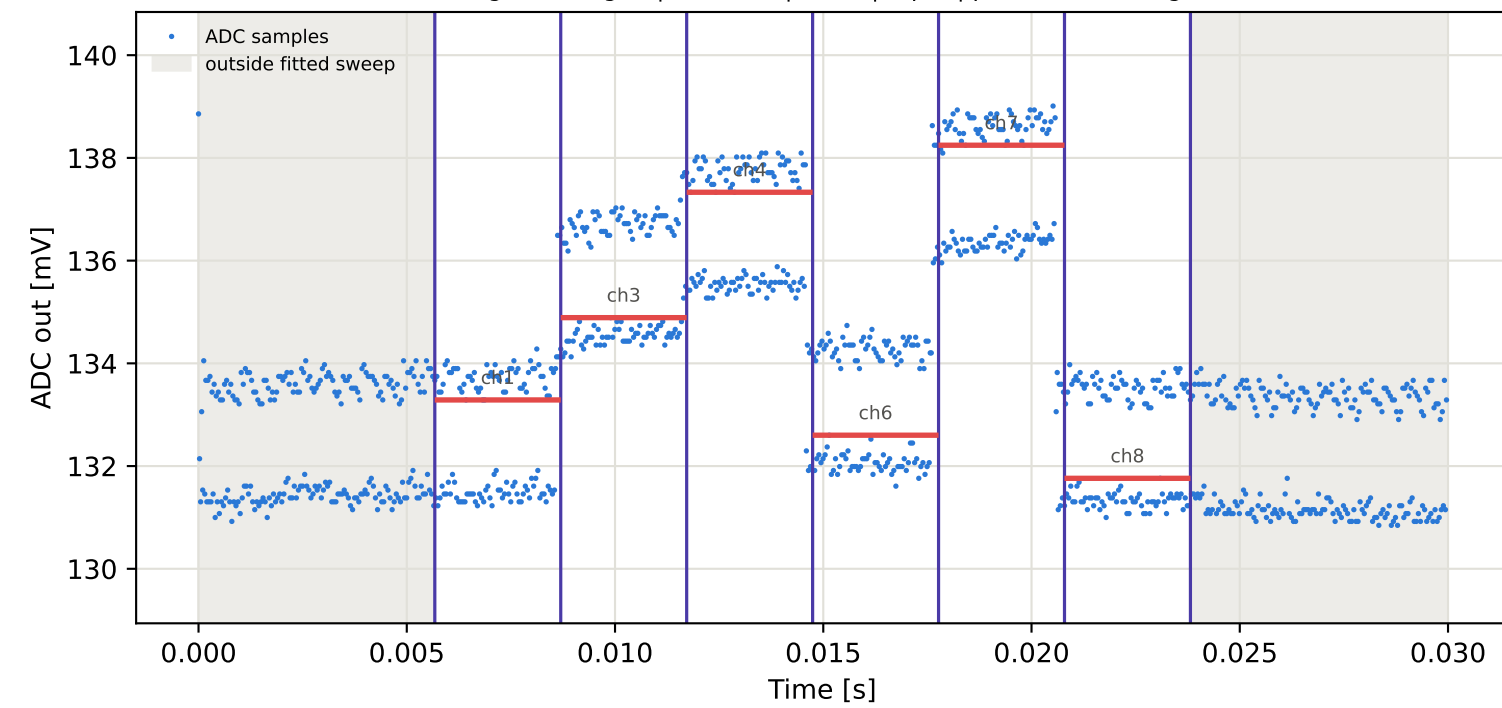
Tag10 &lt;- Tag2 | 805 MHz | run 0 | rep 1 | phase 101.90 deg
