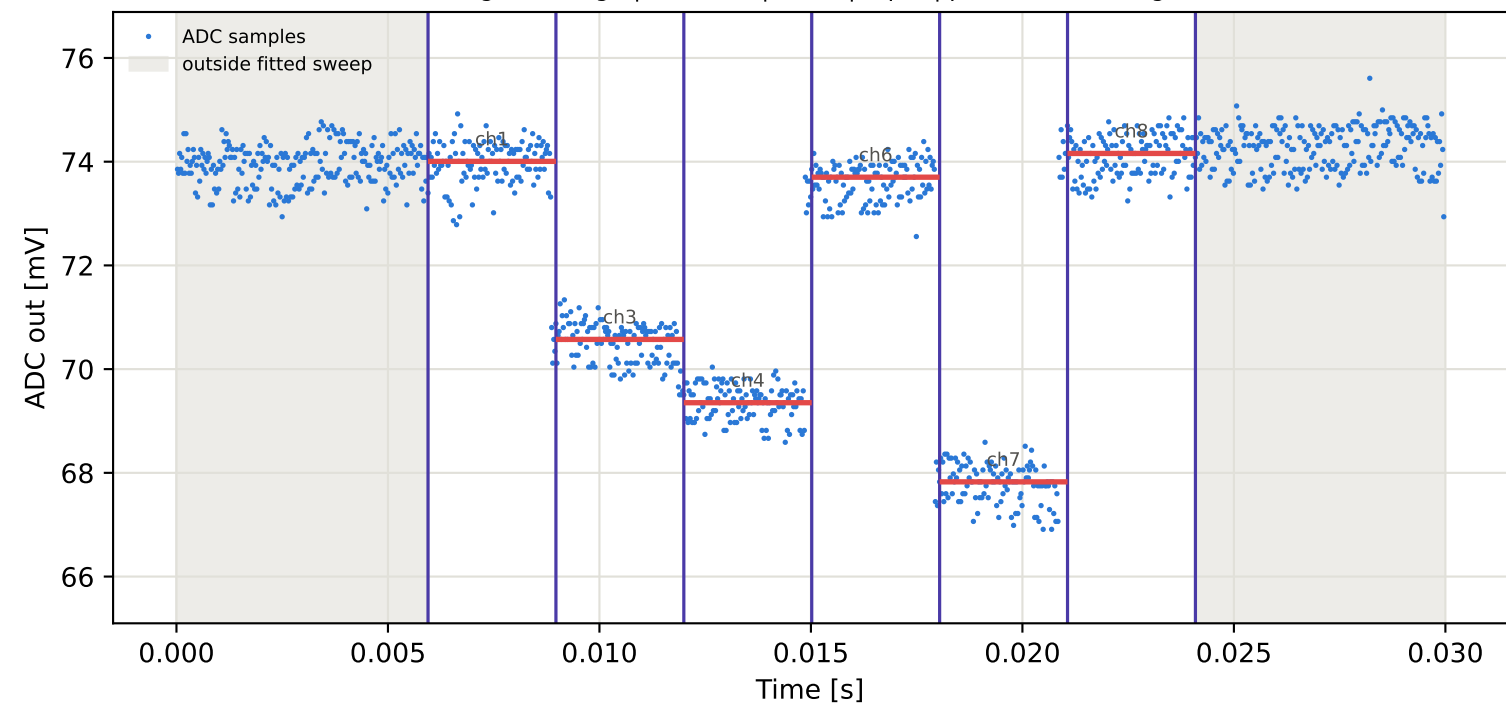
Tag2 &lt;- Tag10 | 775 MHz | run 0 | rep 1 | phase 51.27 deg
