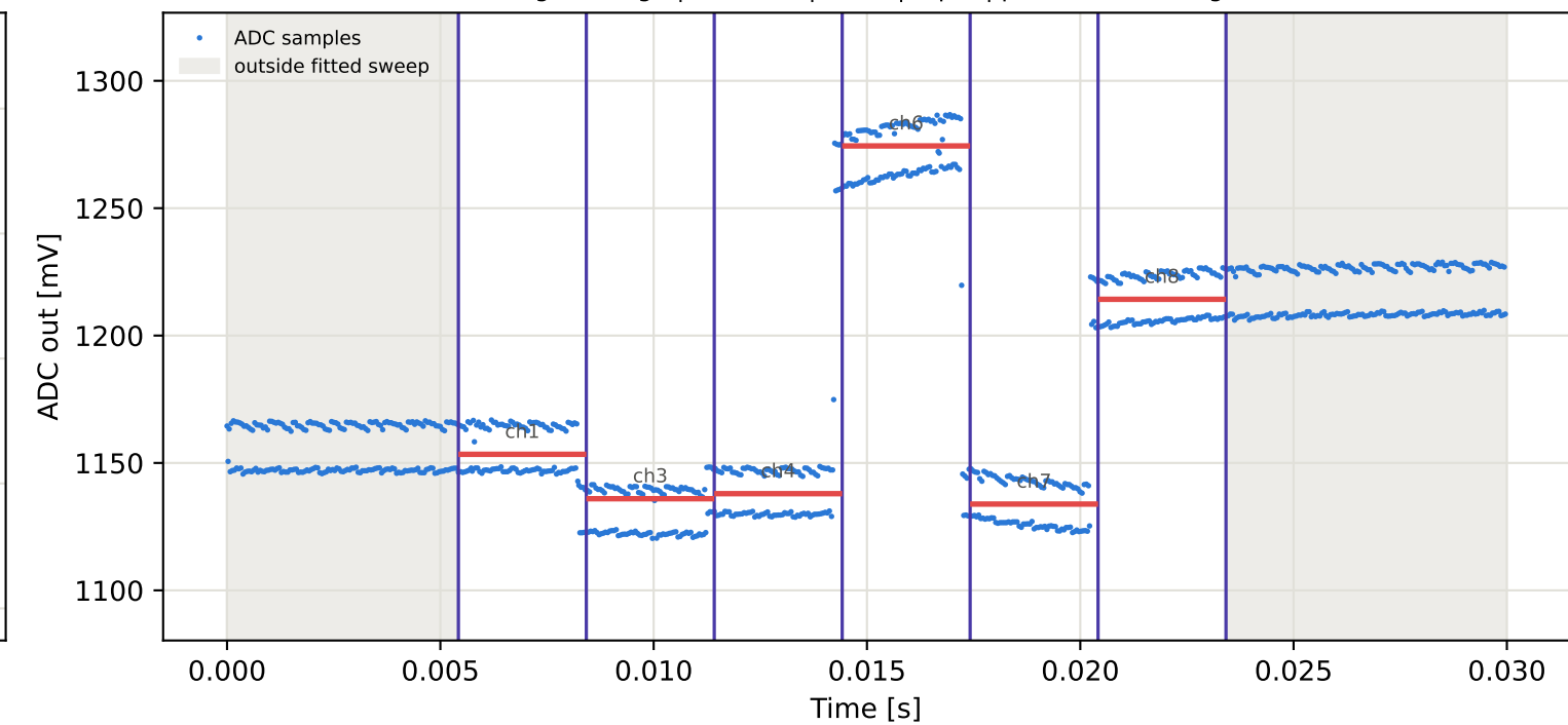
Tag8 &lt;- Tag7 | 925 MHz | run 0 | rep 1 | phase -52.50 deg
