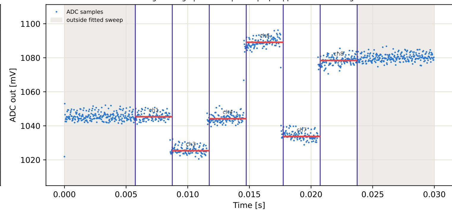
Tag3 &lt;- Tag9 | 885 MHz | run 0 | rep 1 | phase -11.11 deg
