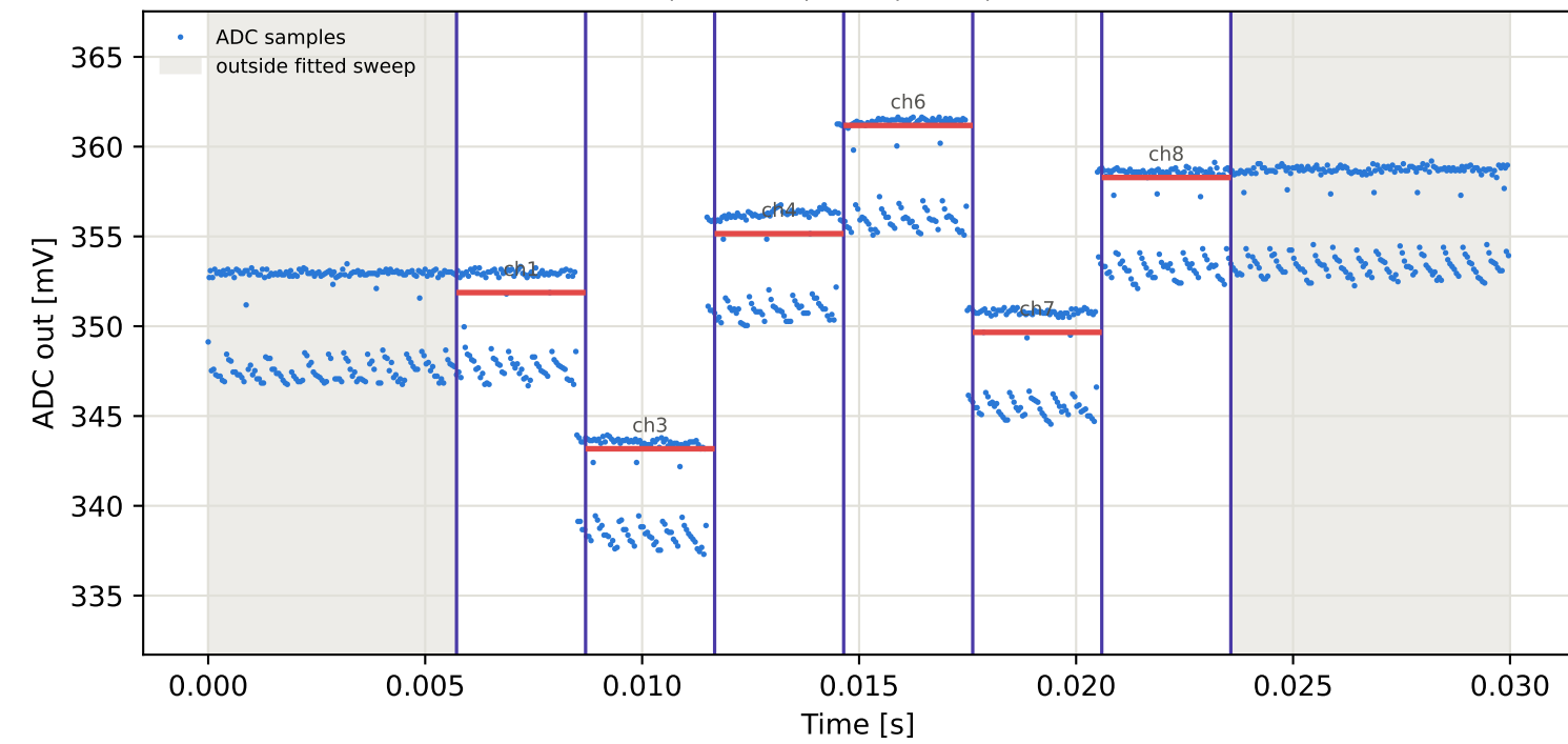
Tag8 &lt;- Tag16 | 805 MHz | run 0 | rep 1 | phase -155.89 deg
