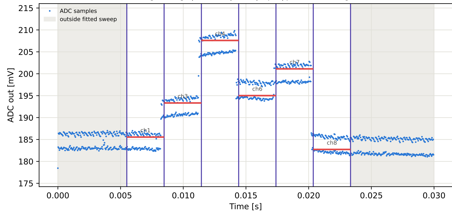
Tag1 &lt;- Tag8 | 935 MHz | run 0 | rep 1 | phase -117.07 deg
