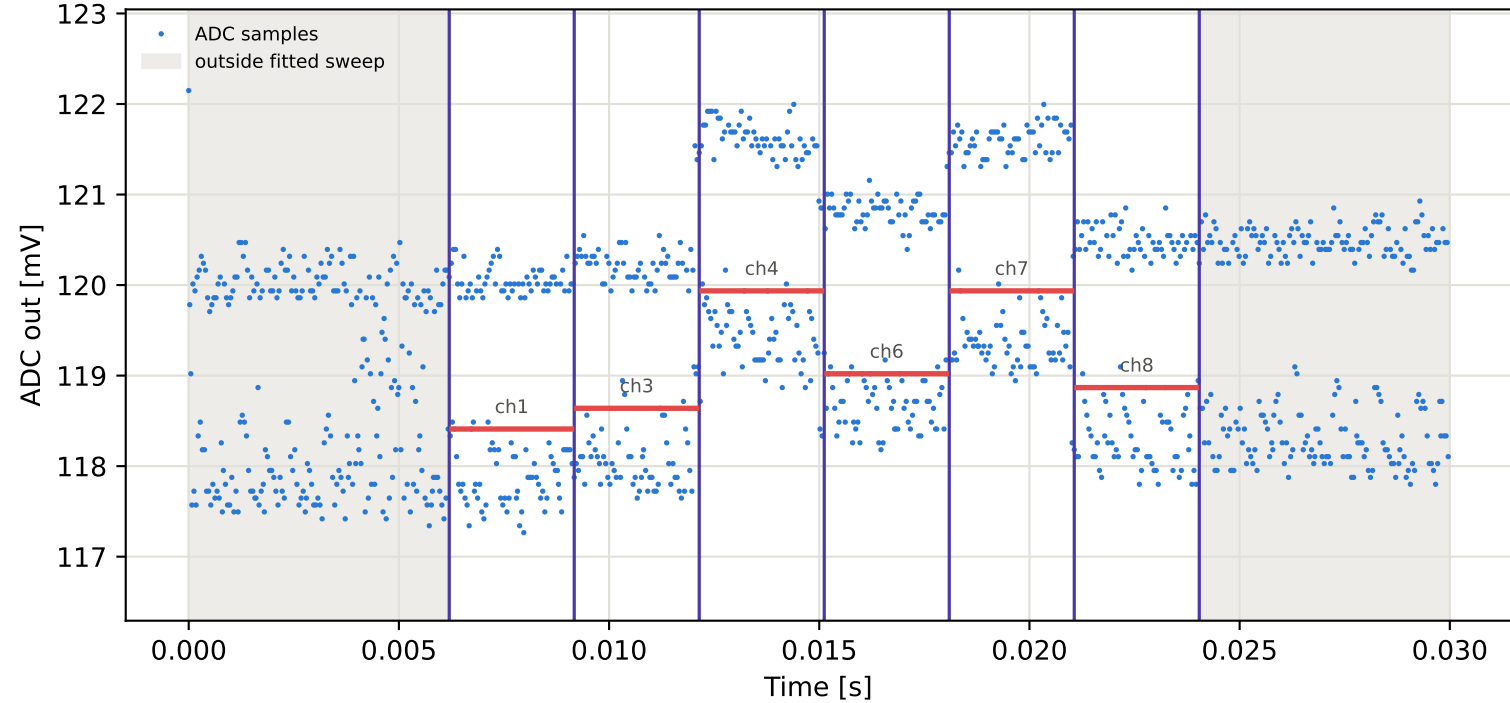
Tag7 &lt;- Tag6 | 795 MHz | run 0 | rep 1 | phase 135.39 deg
