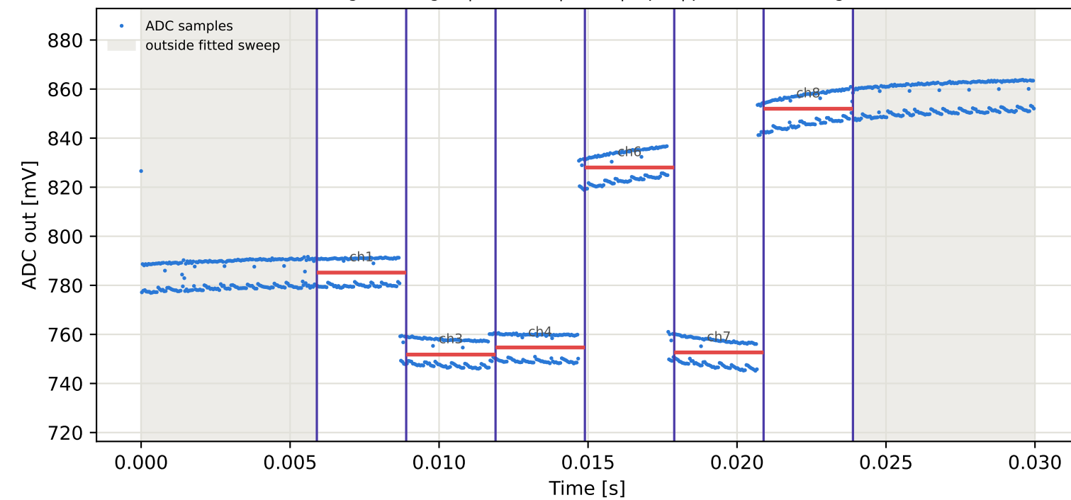
Tag15 &lt;- Tag3 | 895 MHz | run 0 | rep 1 | phase 160.40 deg
