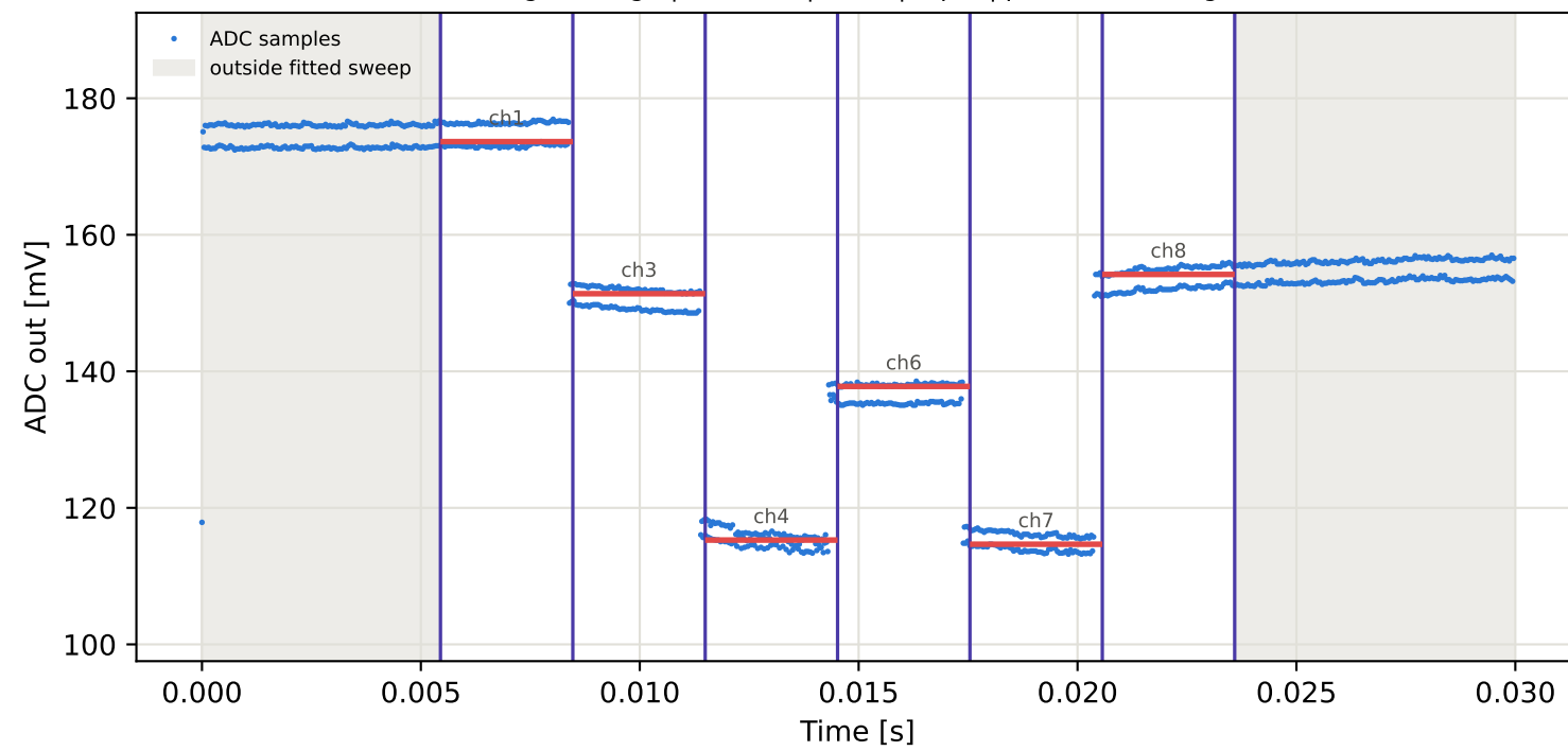
Tag9 &lt;- Tag5 | 825 MHz | run 0 | rep 1 | phase 105.77 deg
