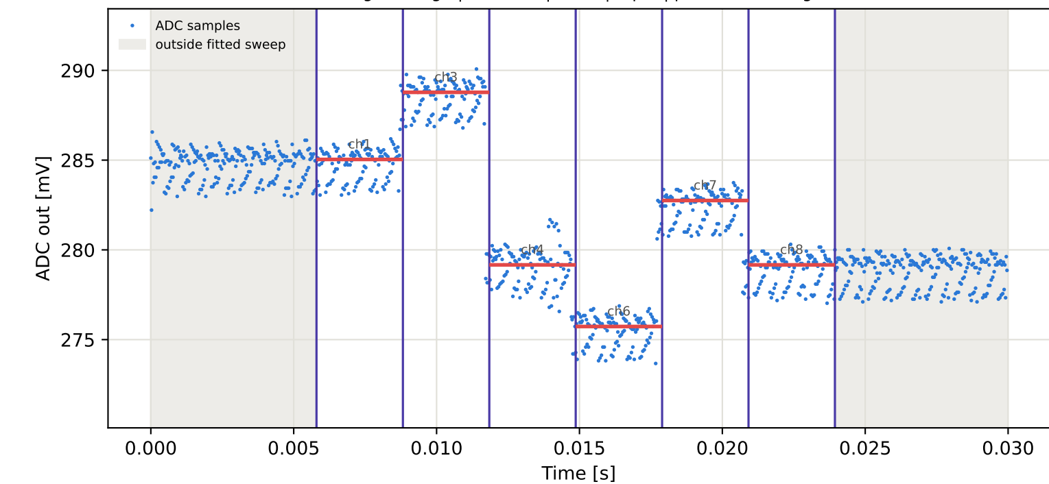
Tag8 &lt;- Tag7 | 795 MHz | run 0 | rep 1 | phase 39.57 deg
