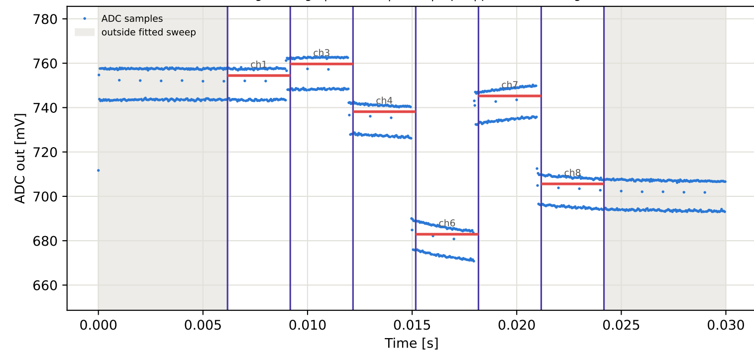
Tag3 &lt;- Tag9 | 905 MHz | run 0 | rep 1 | phase 12.48 deg
