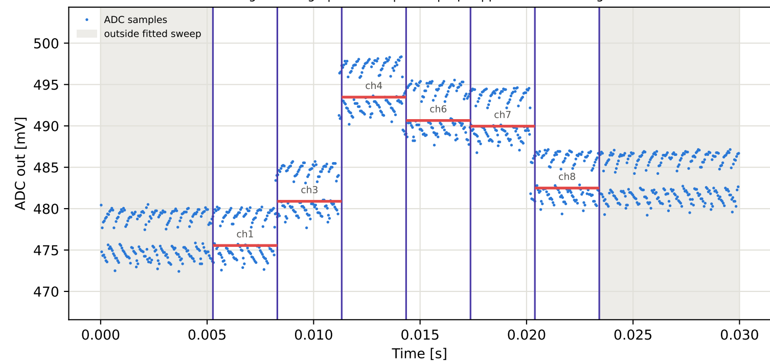
Tag2 &lt;- Tag10 | 845 MHz | run 0 | rep 1 | phase 13.53 deg
