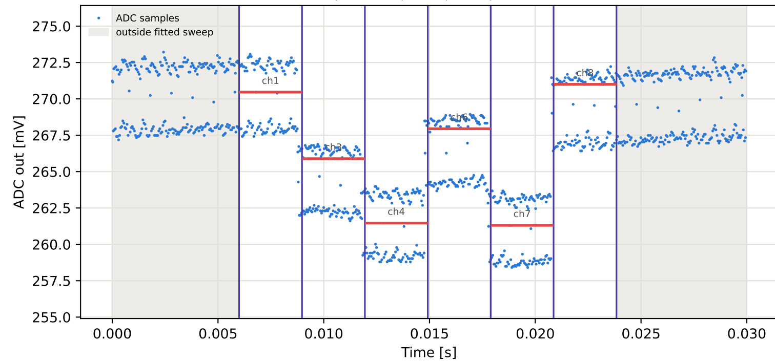
Tag6 &lt;- Tag5 | 835 MHz | run 0 | rep 1 | phase 107.24 deg
