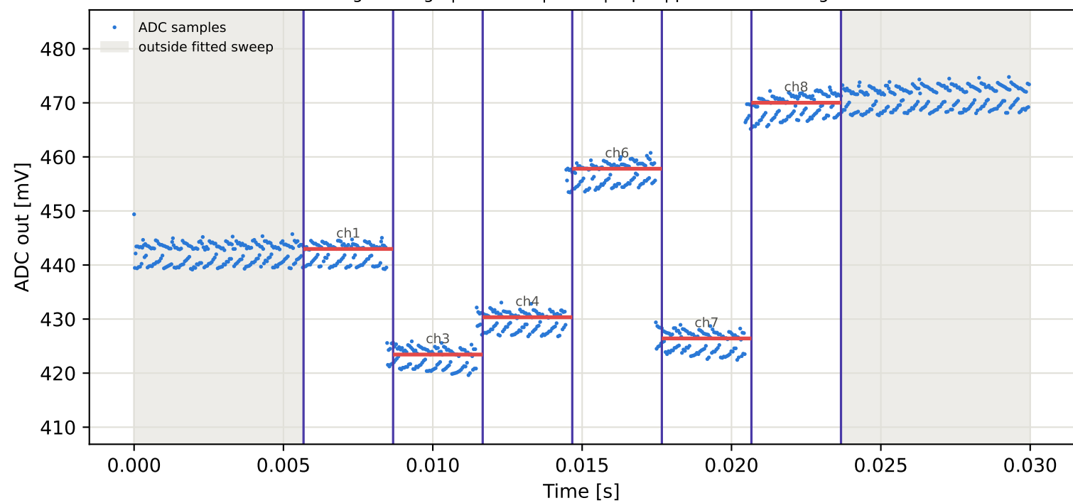
Tag2 &lt;- Tag6 | 865 MHz | run 0 | rep 1 | phase -58.83 deg
