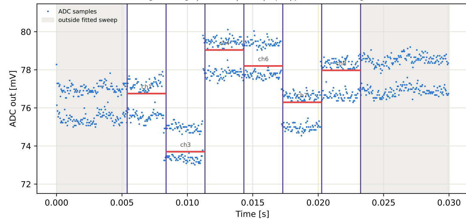
Tag15 &lt;- Tag5 | 775 MHz | run 0 | rep 1 | phase 166.74 deg
