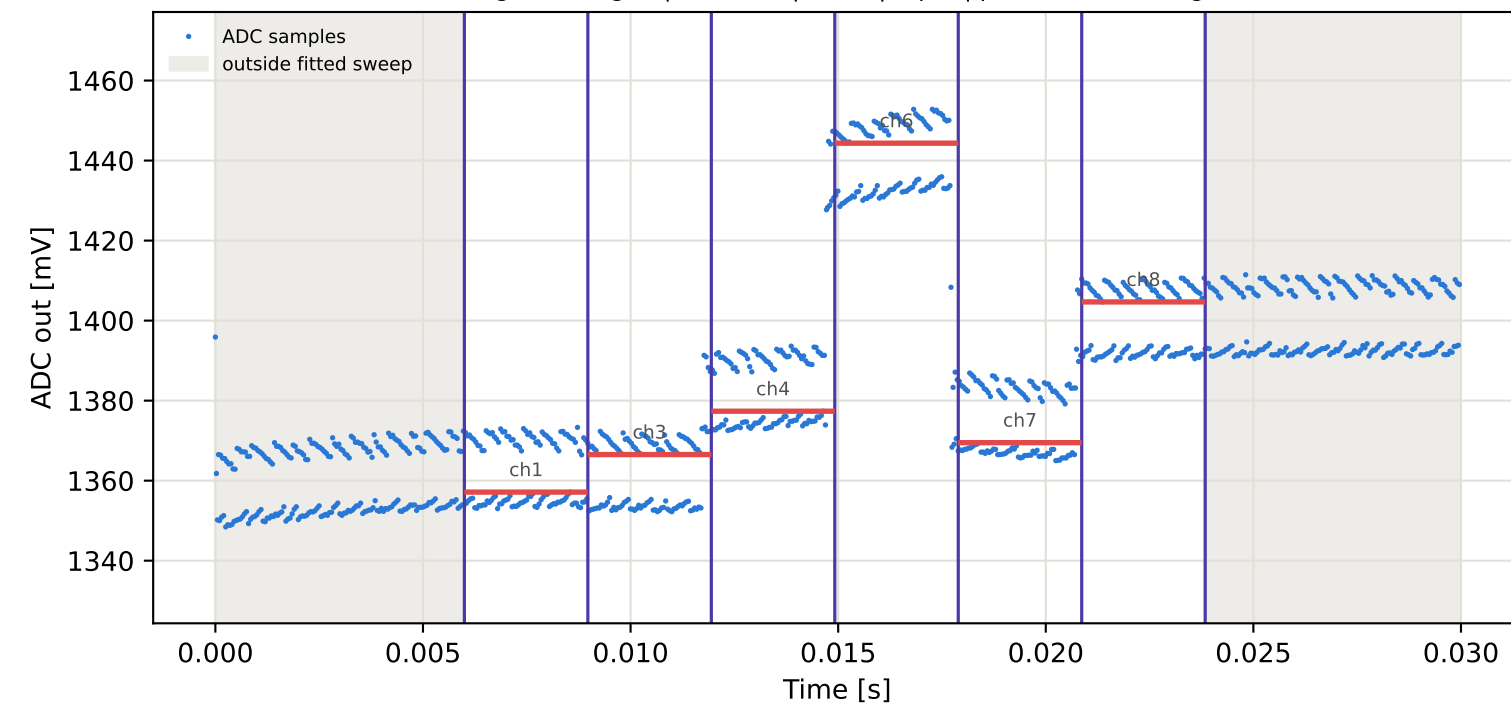
Tag15 &lt;- Tag3 | 915 MHz | run 0 | rep 1 | phase -165.75 deg
