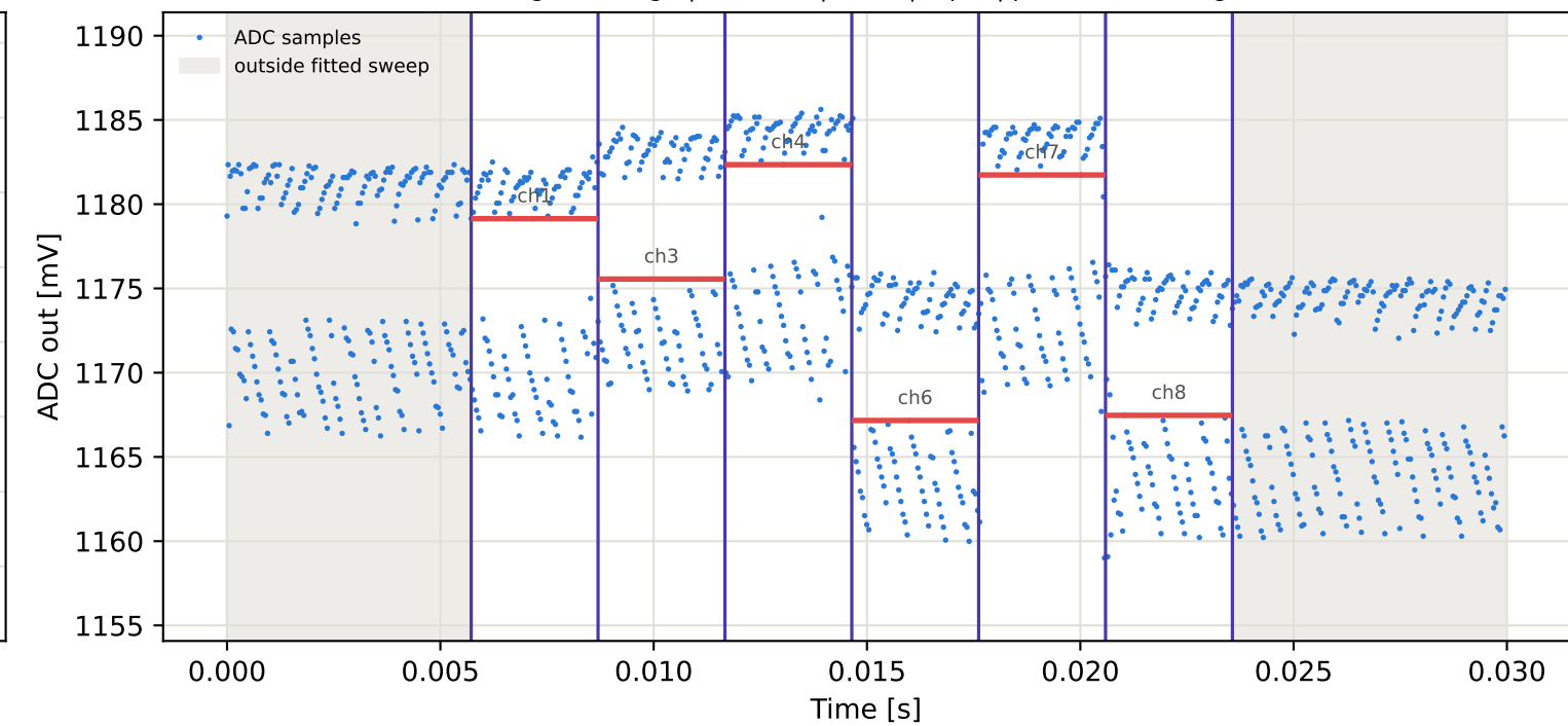
Tag15 &lt;- Tag4 | 905 MHz | run 0 | rep 1 | phase -92.33 deg
