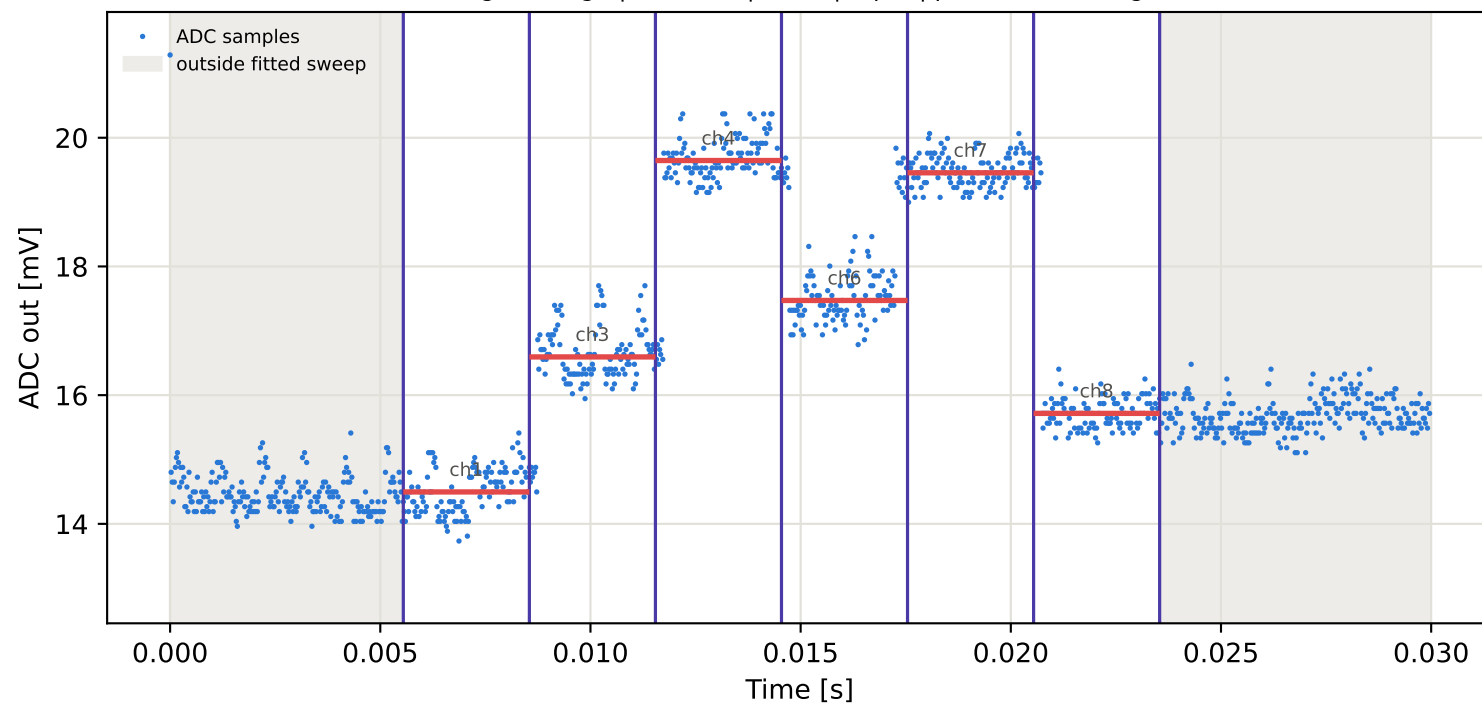
Tag6 &lt;- Tag9 | 795 MHz | run 0 | rep 1 | phase -76.76 deg
