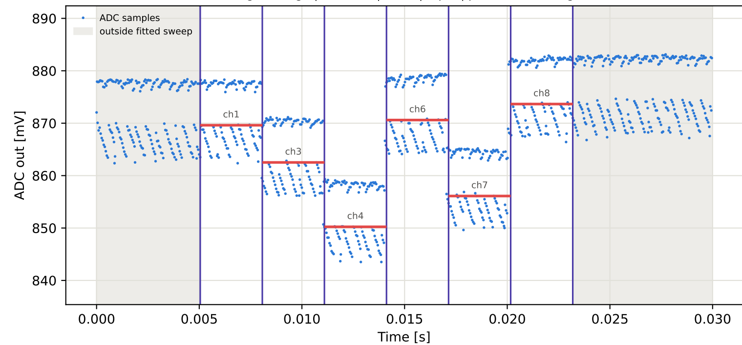
Tag8 &lt;- Tag5 | 965 MHz | run 0 | rep 1 | phase -32.97 deg
