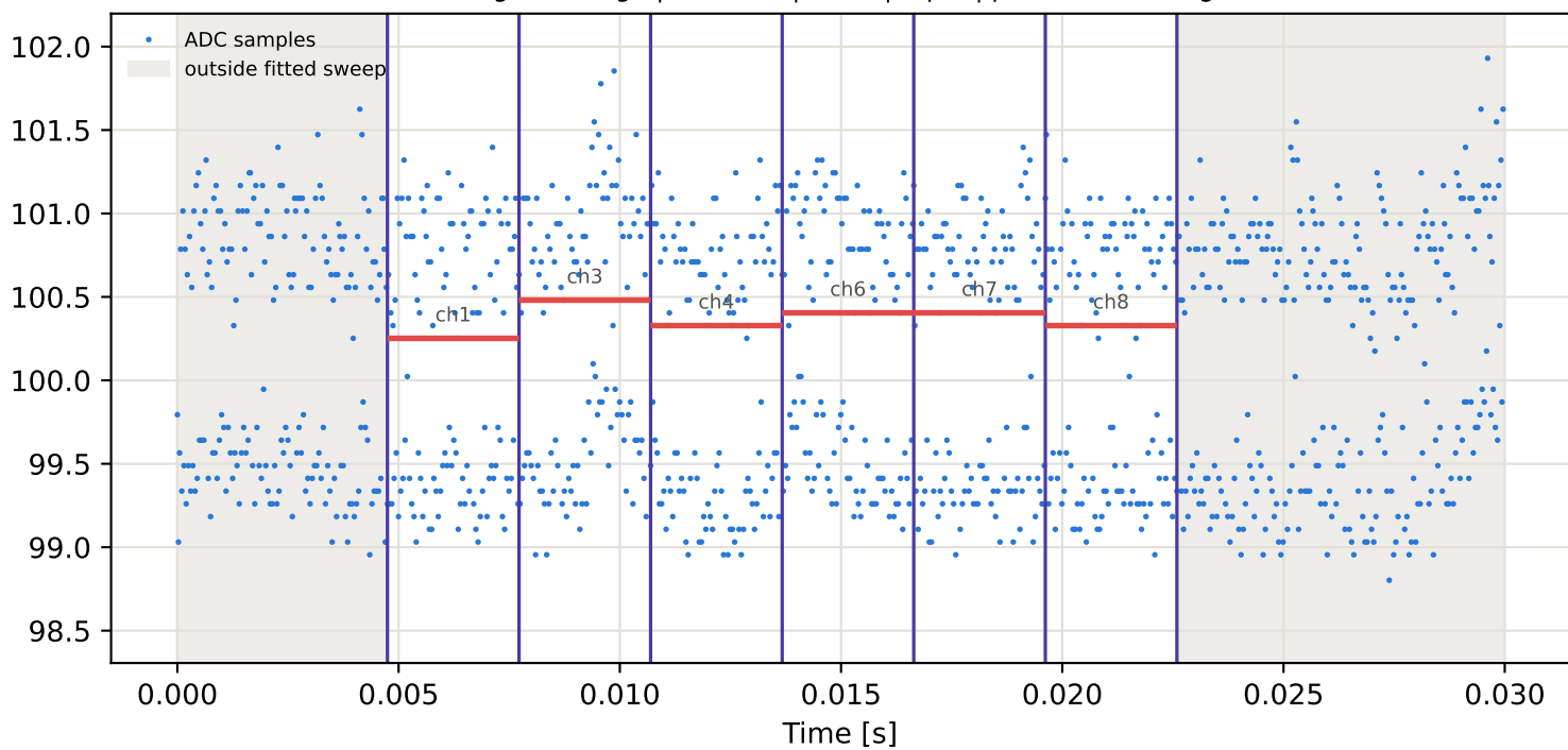
Tag15 &lt;- Tag1 | 785 MHz | run 0 | rep 1 | phase -44.79 deg
