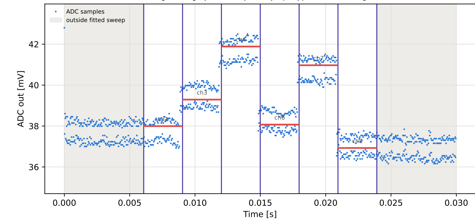
Tag2 &lt;- Tag7 | 955 MHz | run 0 | rep 1 | phase -81.19 deg
