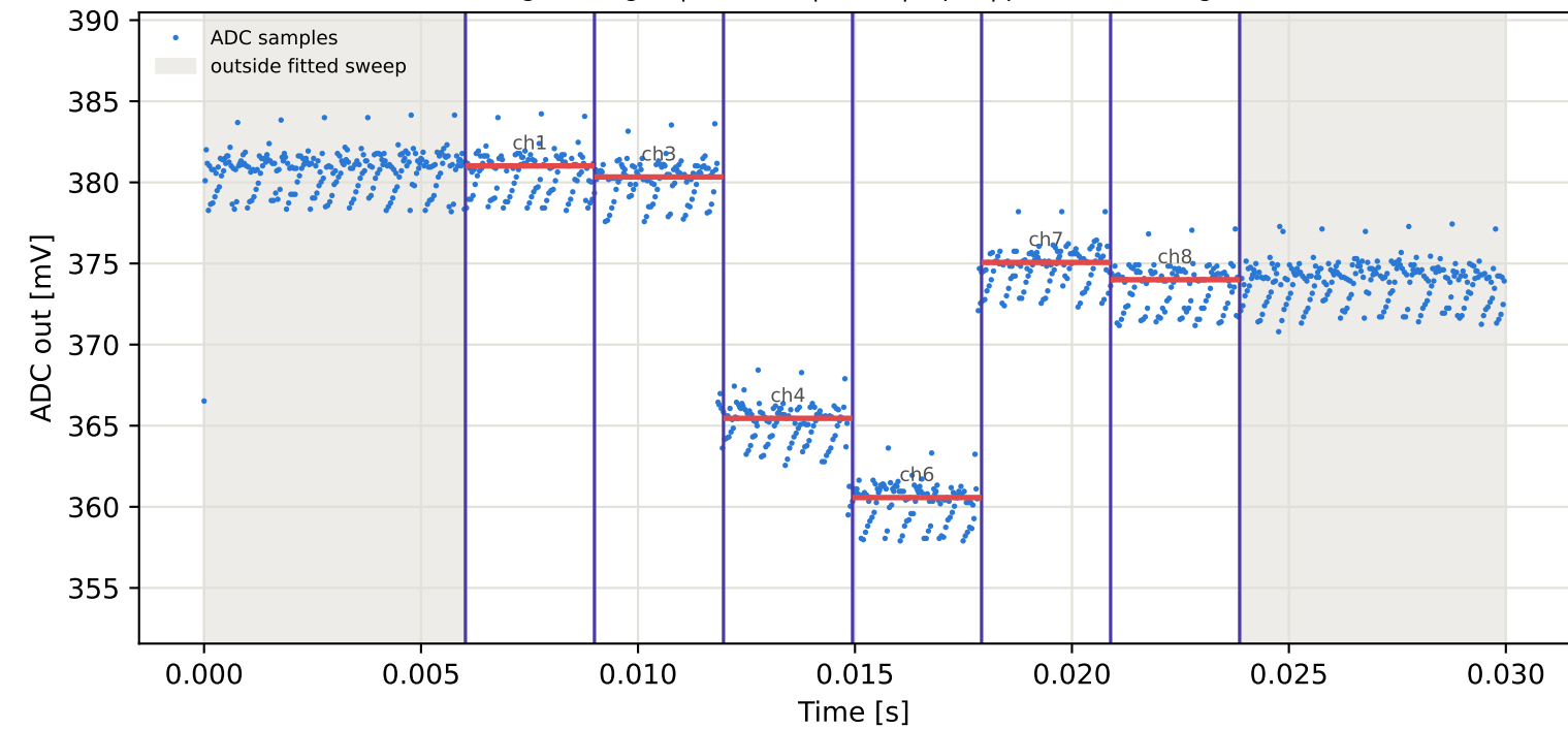
Tag5 &lt;- Tag2 | 985 MHz | run 0 | rep 1 | phase -40.48 deg
