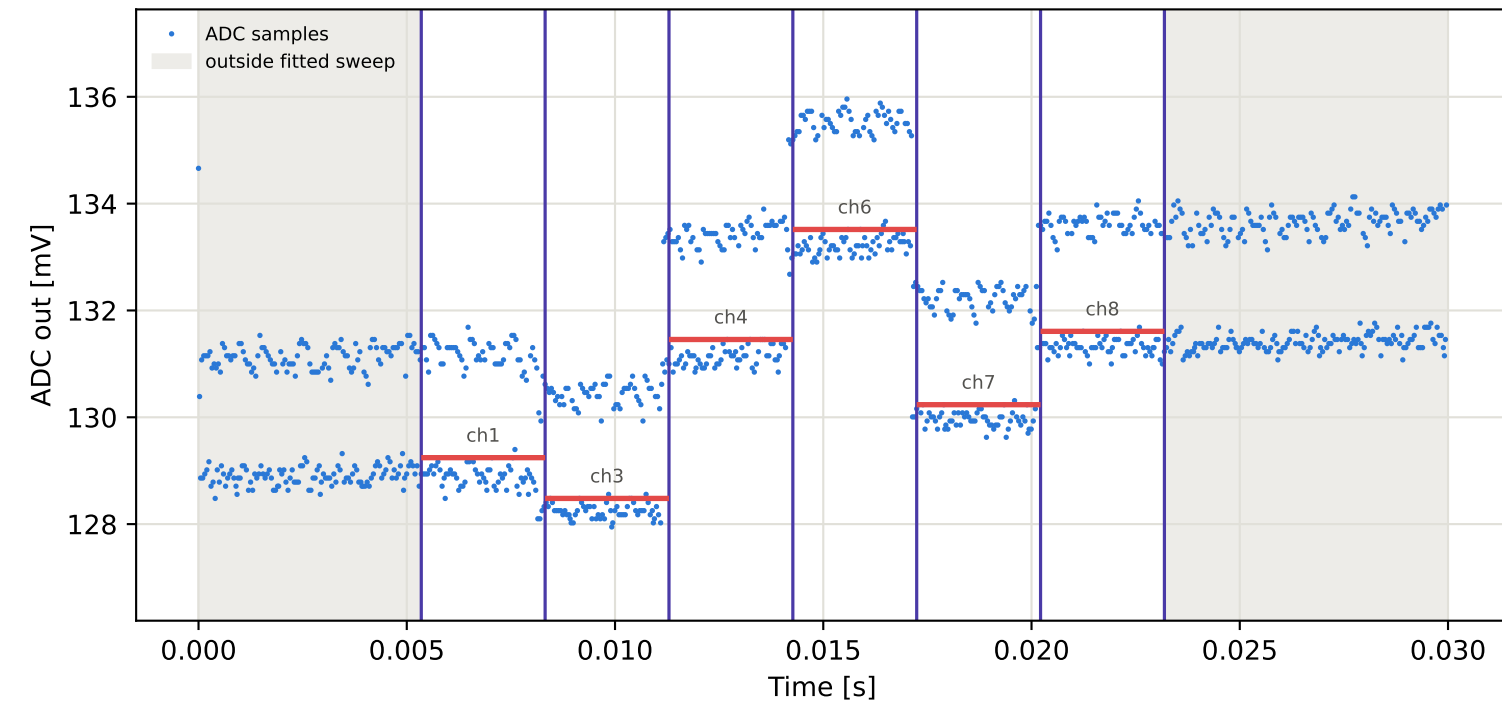
Tag10 &lt;- Tag4 | 835 MHz | run 0 | rep 1 | phase 96.59 deg
