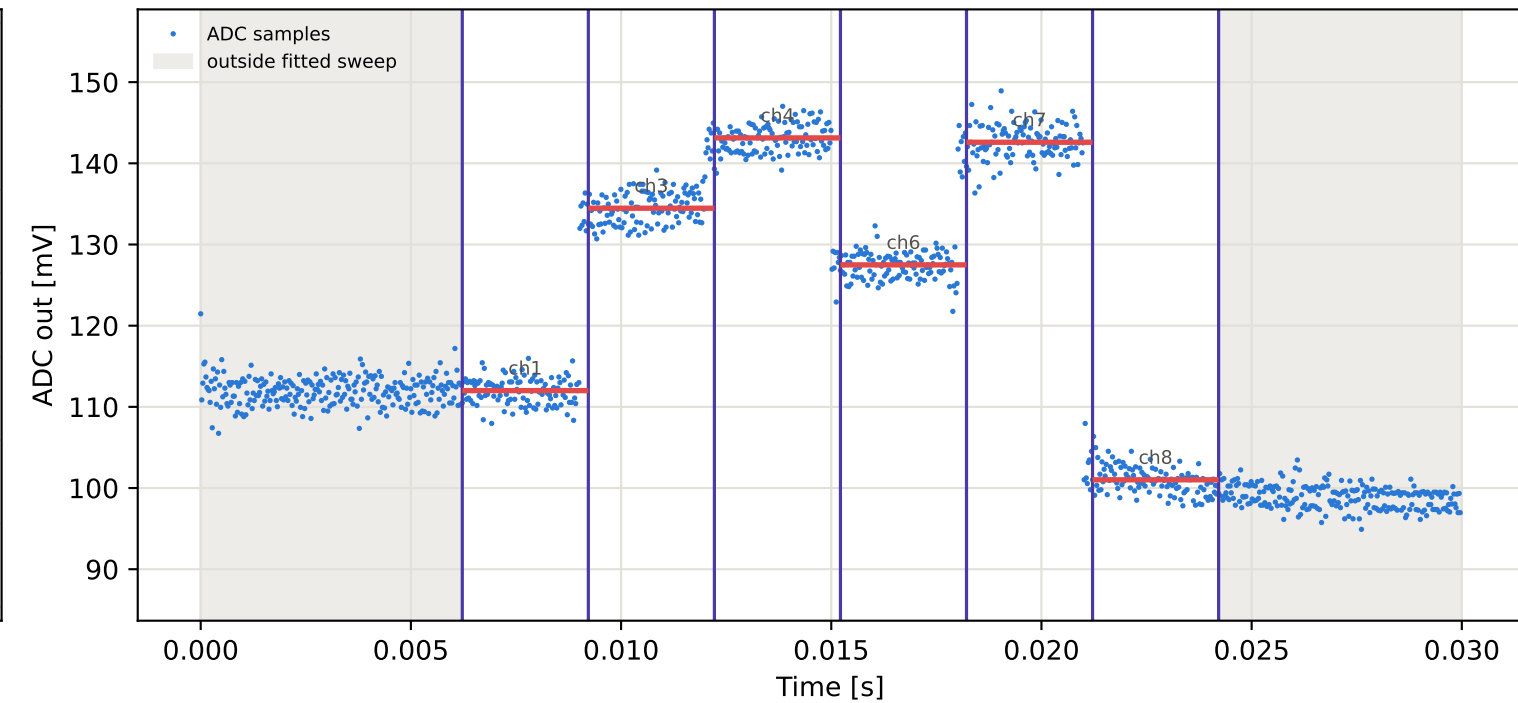
Tag4 &lt;- Tag3 | 885 MHz | run 0 | rep 1 | phase 173.43 deg
