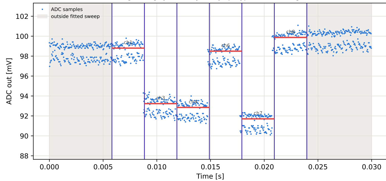
Tag5 &lt;- Tag9 | 795 MHz | run 0 | rep 1 | phase 73.30 deg
