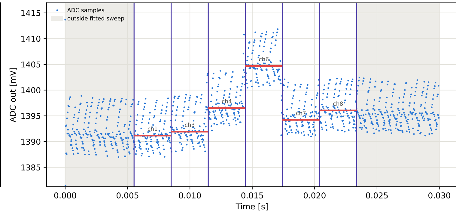
Tag15 &lt;- Tag6 | 915 MHz | run 0 | rep 1 | phase -73.60 deg
