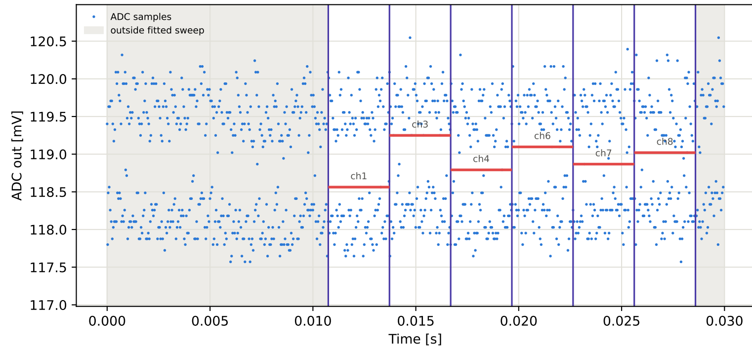
Tag7 &lt;- Tag15 | 785 MHz | run 0 | rep 1 | phase -145.41 deg
