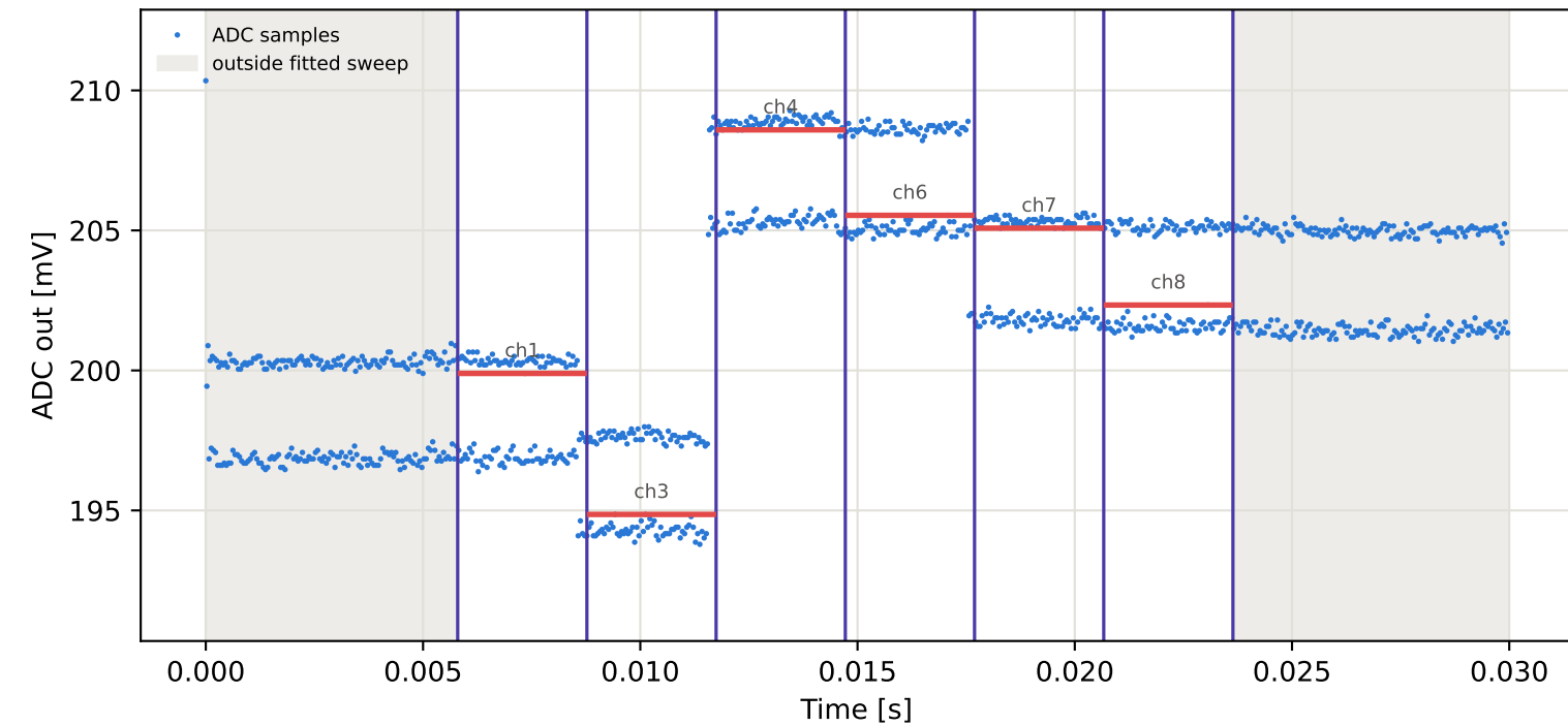
Tag4 &lt;- Tag2 | 805 MHz | run 0 | rep 1 | phase -34.94 deg
