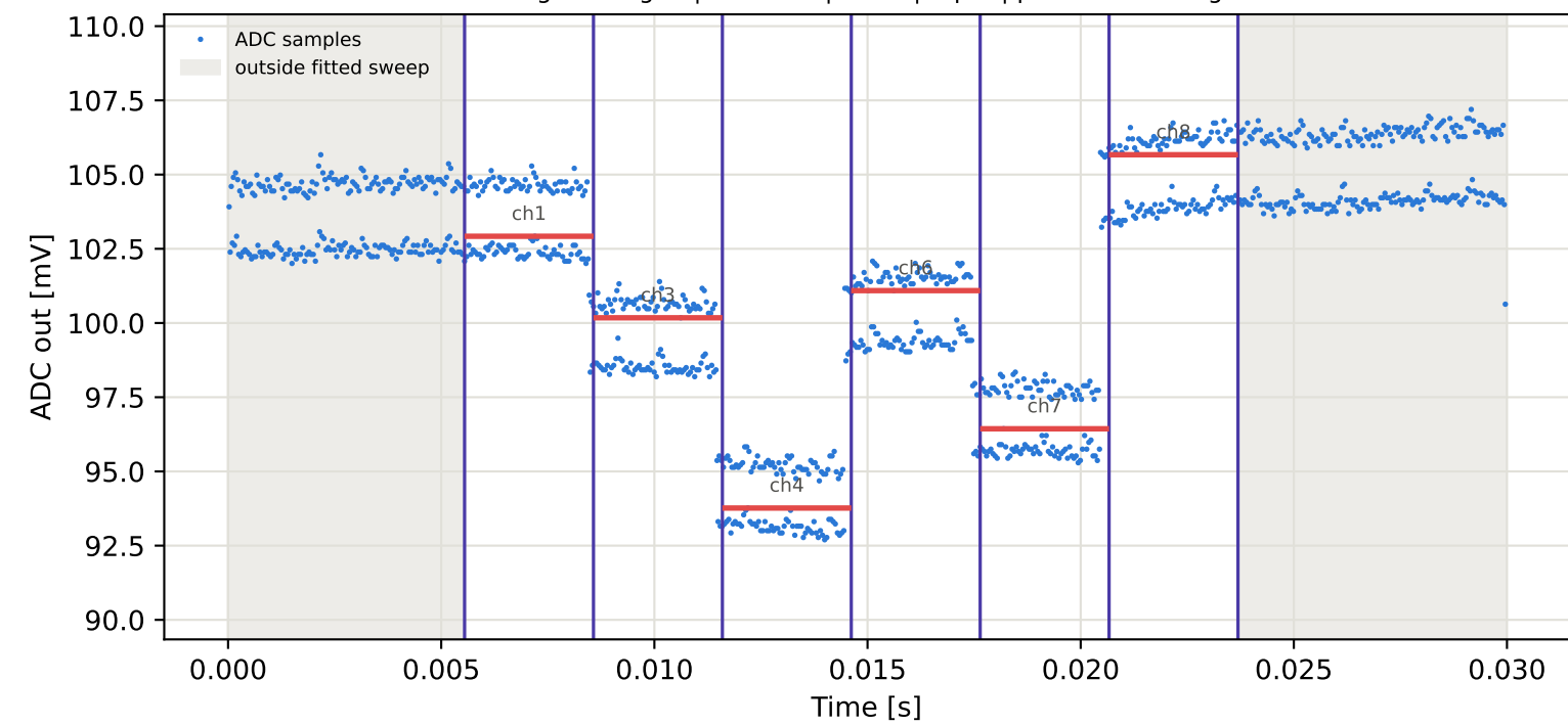
Tag1 &lt;- Tag2 | 945 MHz | run 0 | rep 1 | phase 145.89 deg
