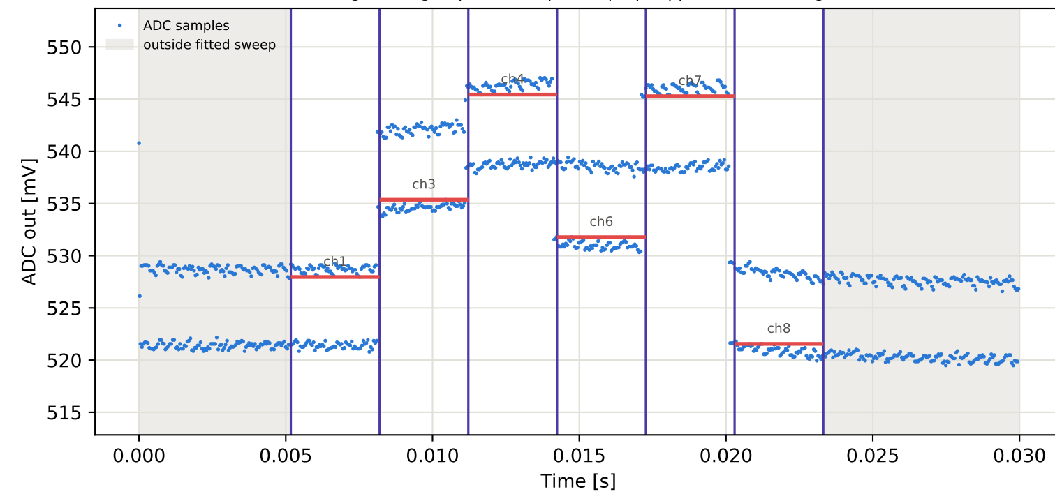
Tag5 &lt;- Tag16 | 865 MHz | run 0 | rep 1 | phase 13.66 deg
