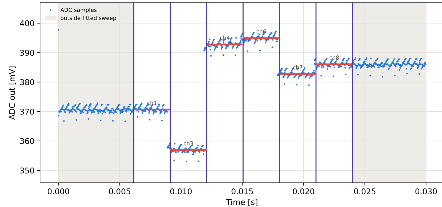
Tag6 &lt;- Tag1 | 805 MHz | run 0 | rep 1 | phase -118.17 deg
