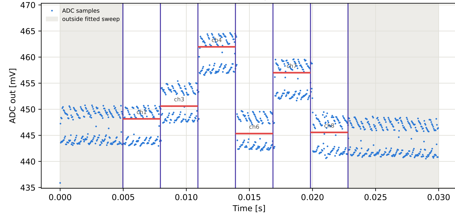
Tag16 &lt;- Tag10 | 995 MHz | run 0 | rep 1 | phase -80.47 deg
