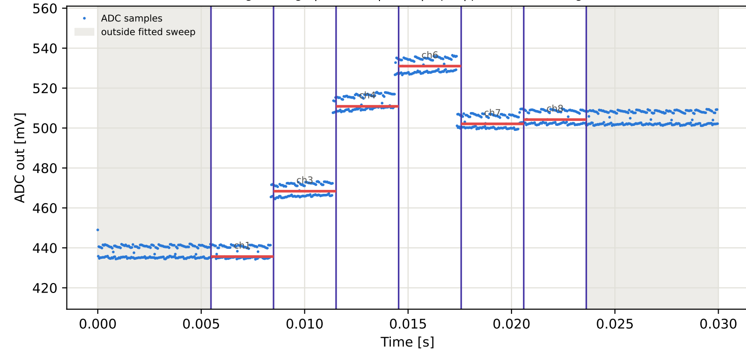
Tag6 &lt;- Tag5 | 855 MHz | run 0 | rep 1 | phase 96.52 deg
