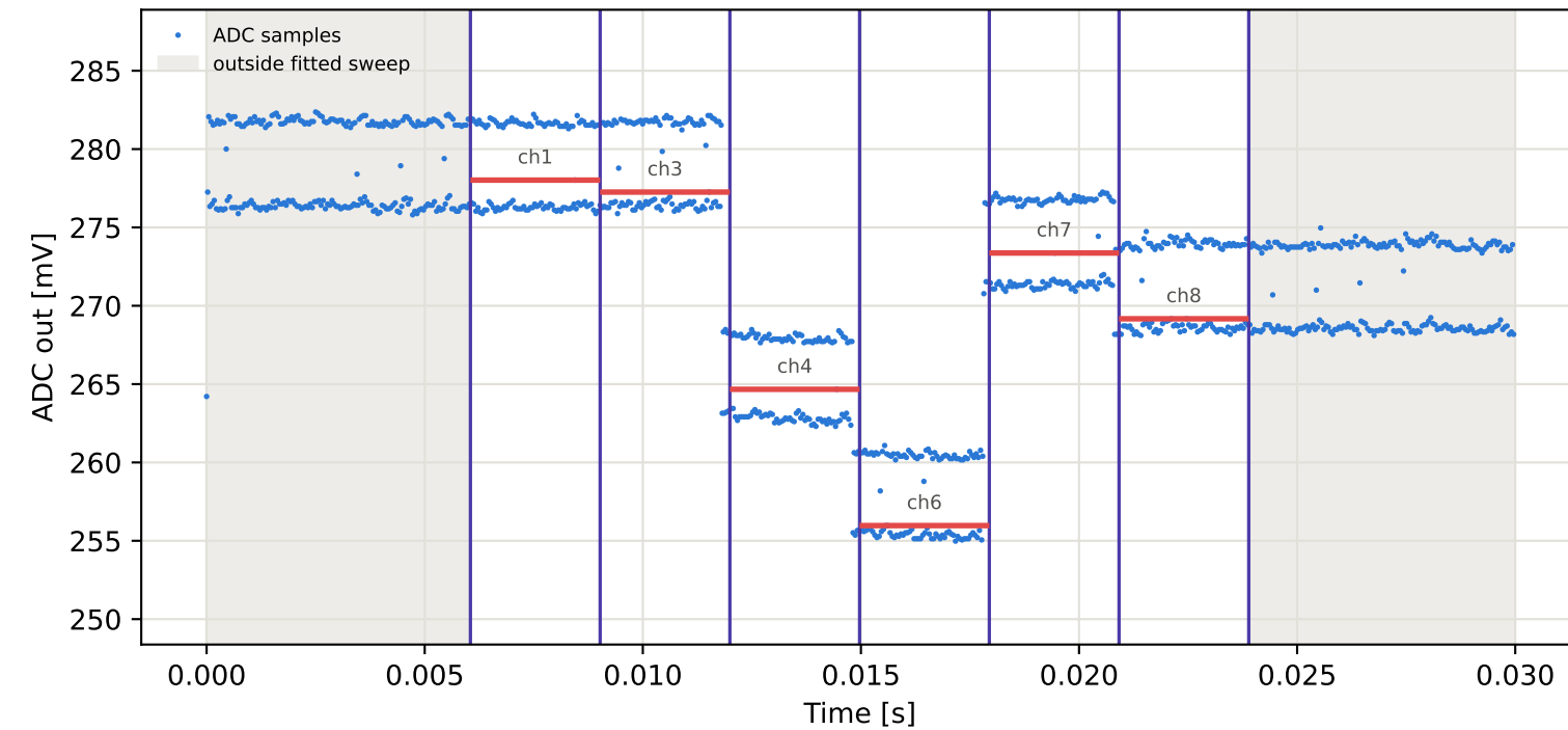
Tag9 &lt;- Tag7 | 975 MHz | run 0 | rep 1 | phase -39.16 deg
