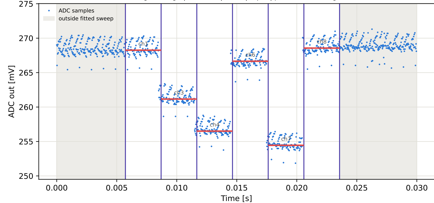
Tag8 &lt;- Tag7 | 785 MHz | run 0 | rep 1 | phase 0.97 deg
