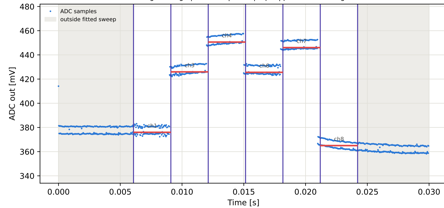
Tag9 &lt;- Tag5 | 875 MHz | run 0 | rep 1 | phase -120.91 deg
