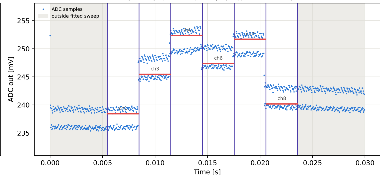
Tag10 &lt;- Tag1 | 865 MHz | run 0 | rep 1 | phase 134.10 deg
