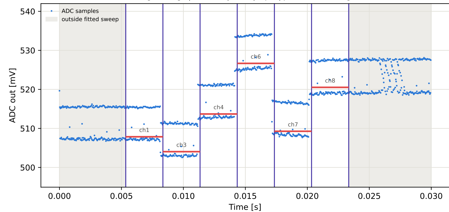
Tag5 &lt;- Tag9 | 835 MHz | run 0 | rep 1 | phase 82.95 deg
