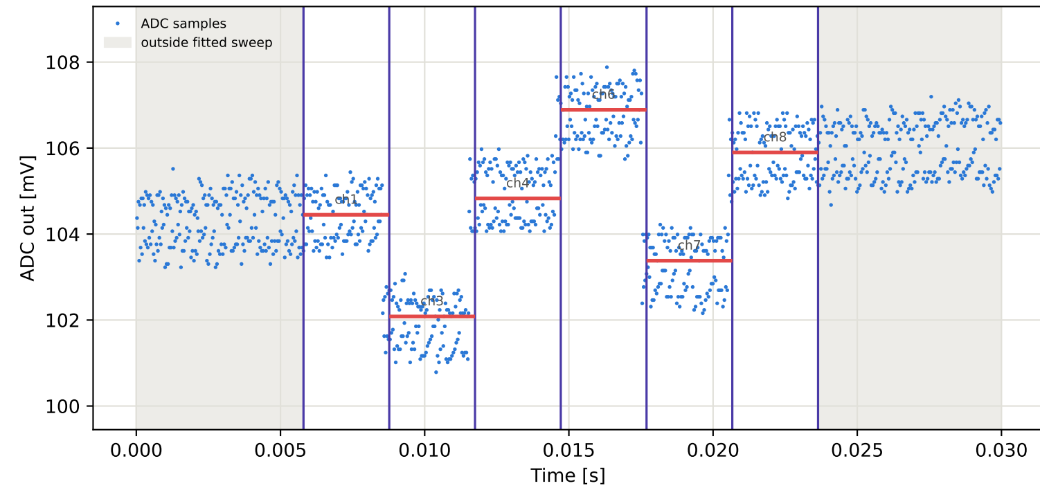
Tag16 &lt;- Tag7 | 795 MHz | run 0 | rep 1 | phase 60.21 deg
