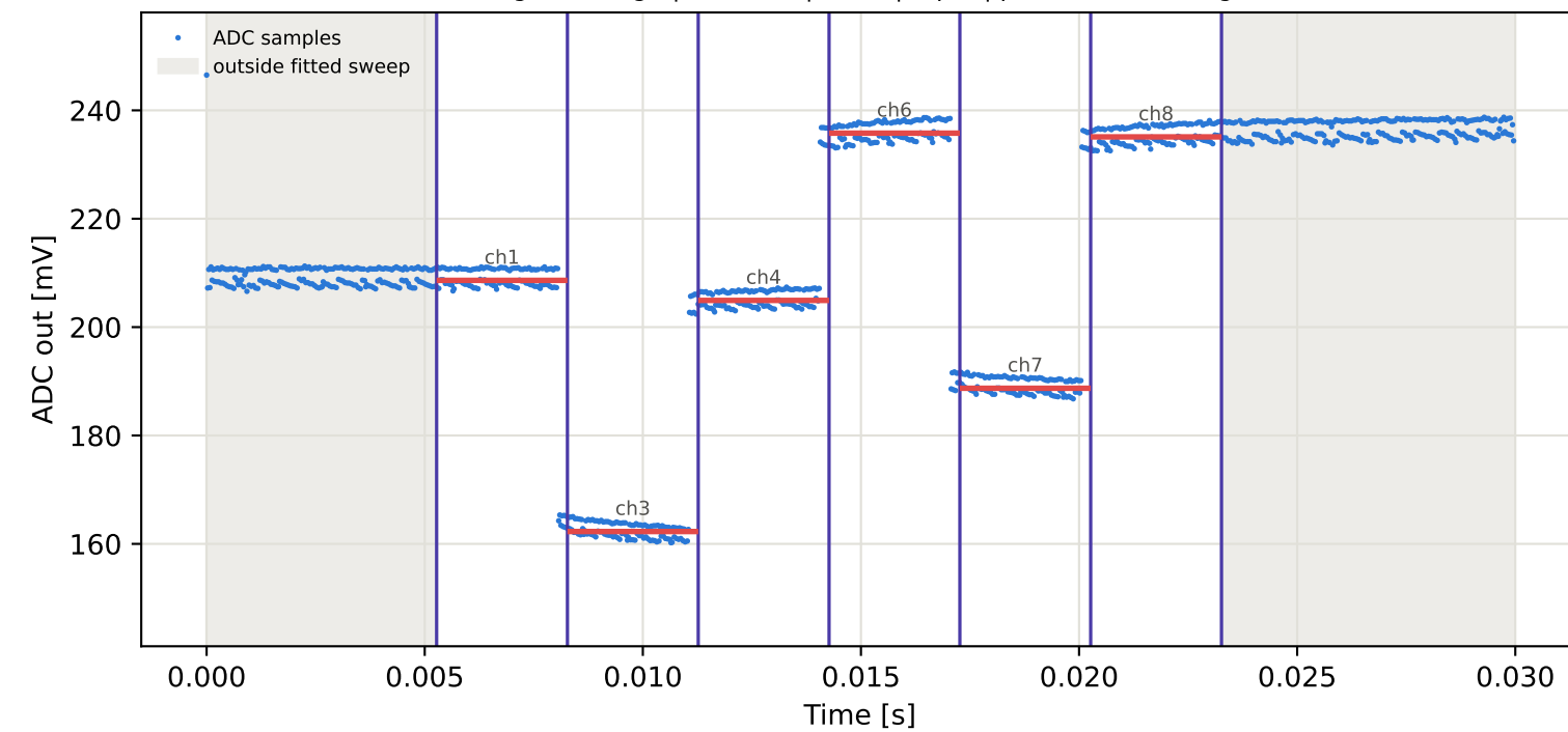
Tag2 &lt;- Tag1 | 825 MHz | run 0 | rep 1 | phase 92.65 deg
