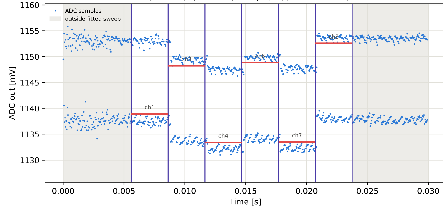
Tag16 &lt;- Tag6 | 875 MHz | run 0 | rep 1 | phase -16.45 deg
