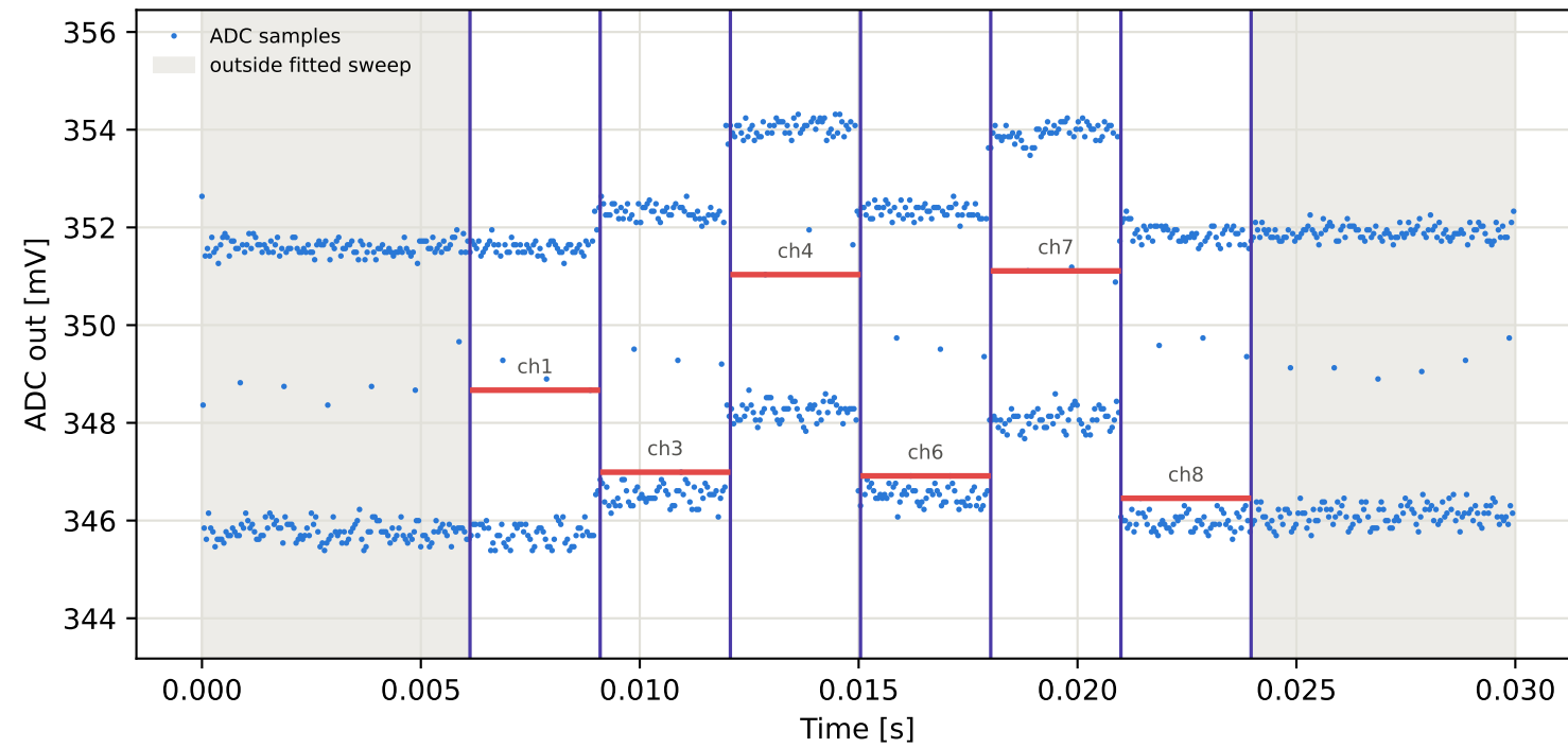
Tag8 &lt;- Tag15 | 805 MHz | run 0 | rep 1 | phase -61.37 deg
