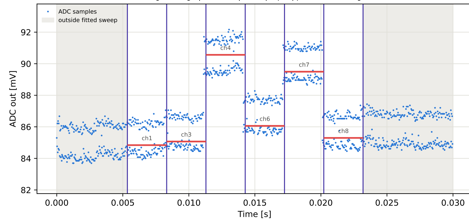
Tag5 &lt;- Tag3 | 775 MHz | run 0 | rep 1 | phase -81.72 deg
