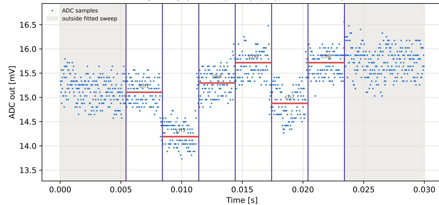
Tag2 &lt;- Tag5 | 795 MHz | run 0 | rep 1 | phase -104.44 deg
