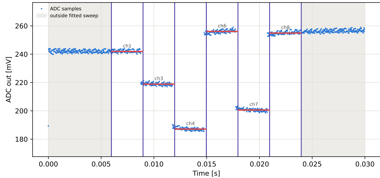
Tag10 &lt;- Tag8 | 985 MHz | run 0 | rep 1 | phase 23.23 deg
