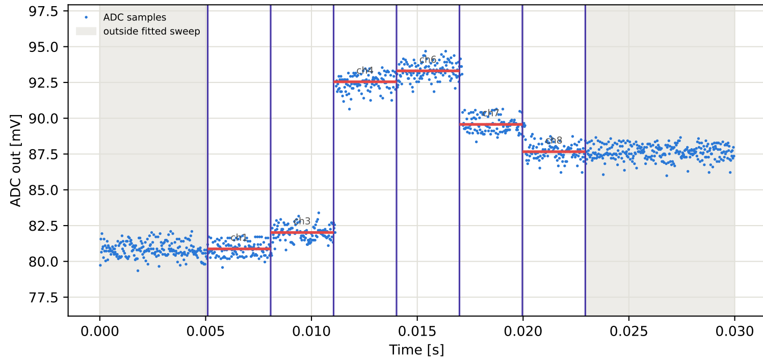
Tag15 &lt;- Tag10 | 825 MHz | run 0 | rep 1 | phase -66.61 deg
