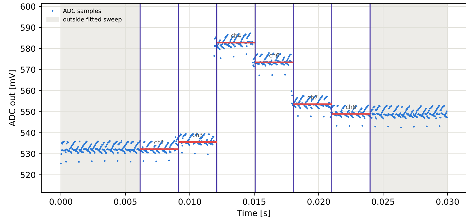
Tag8 &lt;- Tag16 | 995 MHz | run 0 | rep 1 | phase -135.99 deg
