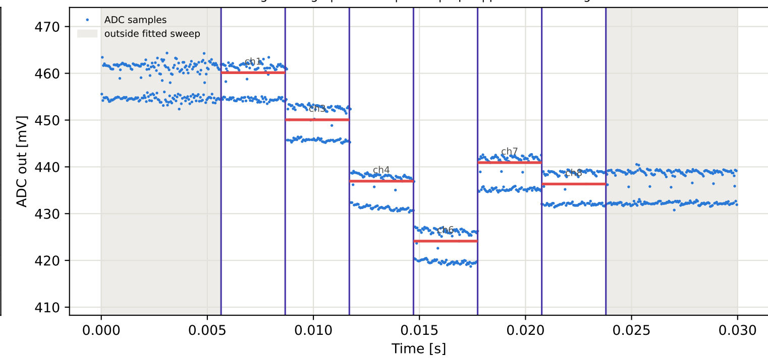
Tag9 &lt;- Tag8 | 875 MHz | run 0 | rep 1 | phase 39.34 deg
