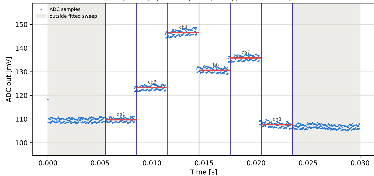
Tag6 &lt;- Tag5 | 935 MHz | run 0 | rep 1 | phase -106.28 deg
