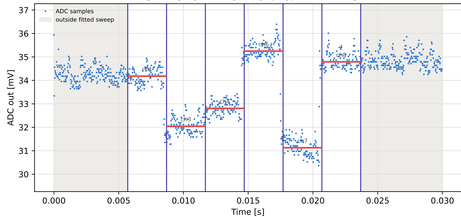
Tag6 &lt;- Tag3 | 775 MHz | run 0 | rep 1 | phase -125.89 deg
