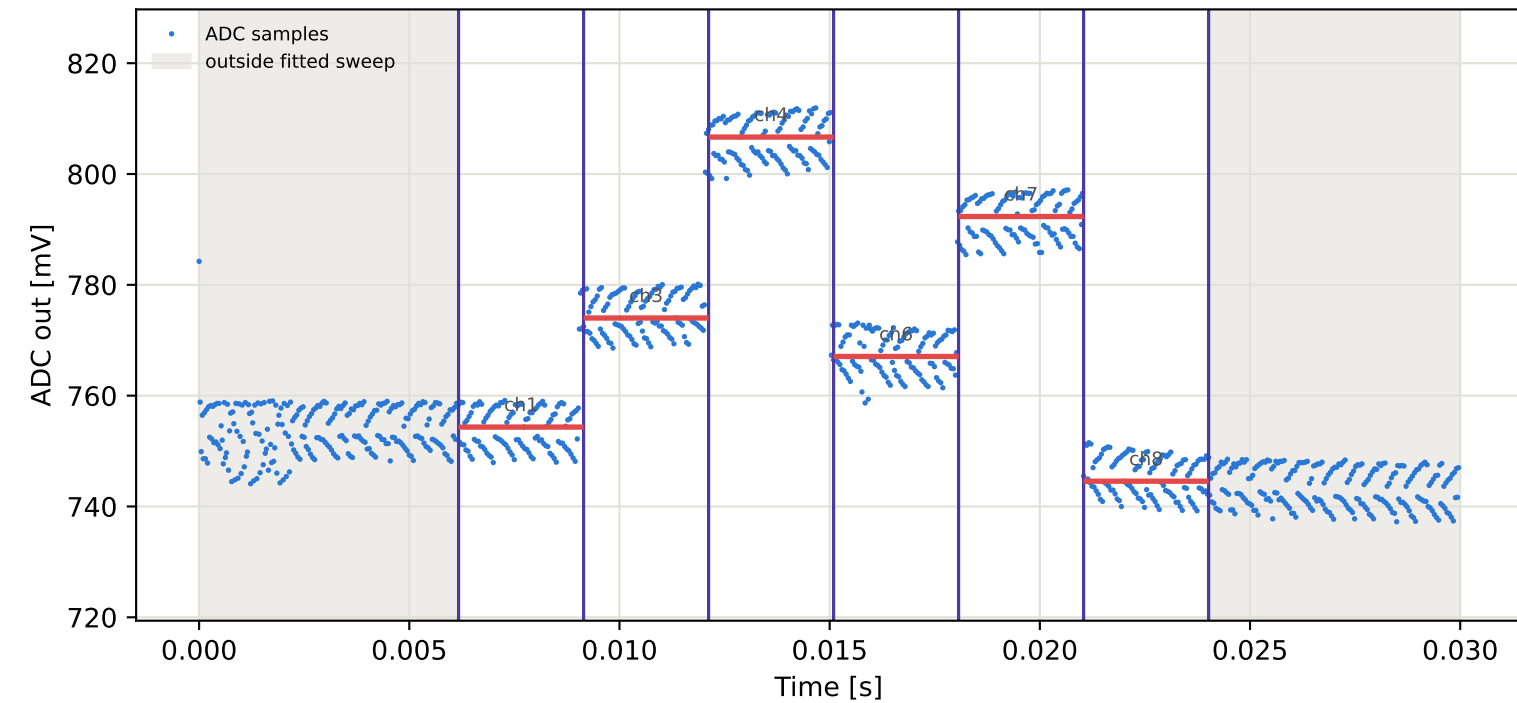
Tag15 &lt;- Tag5 | 945 MHz | run 0 | rep 1 | phase 167.41 deg
