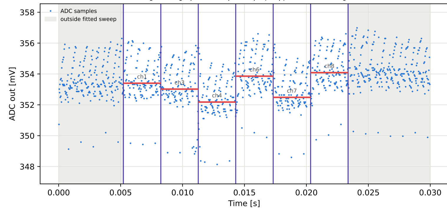
Tag4 &lt;- Tag2 | 955 MHz | run 0 | rep 1 | phase 115.39 deg
