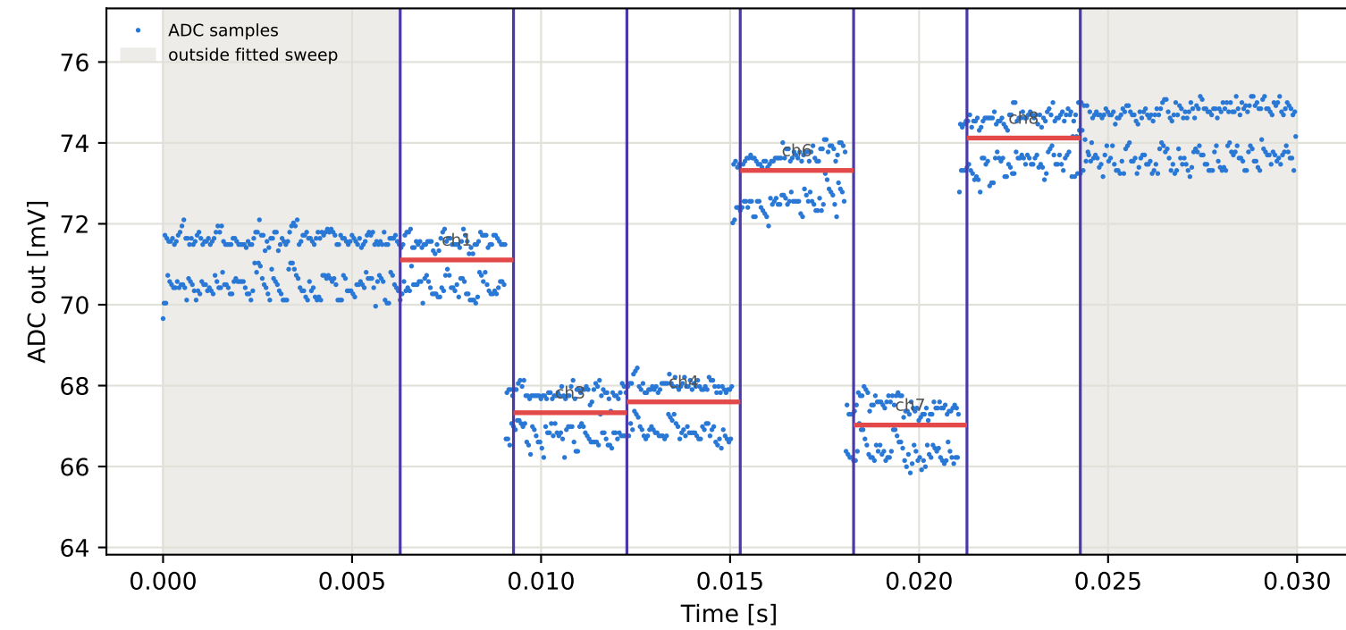
Tag10 &lt;- Tag4 | 855 MHz | run 0 | rep 1 | phase -89.29 deg
