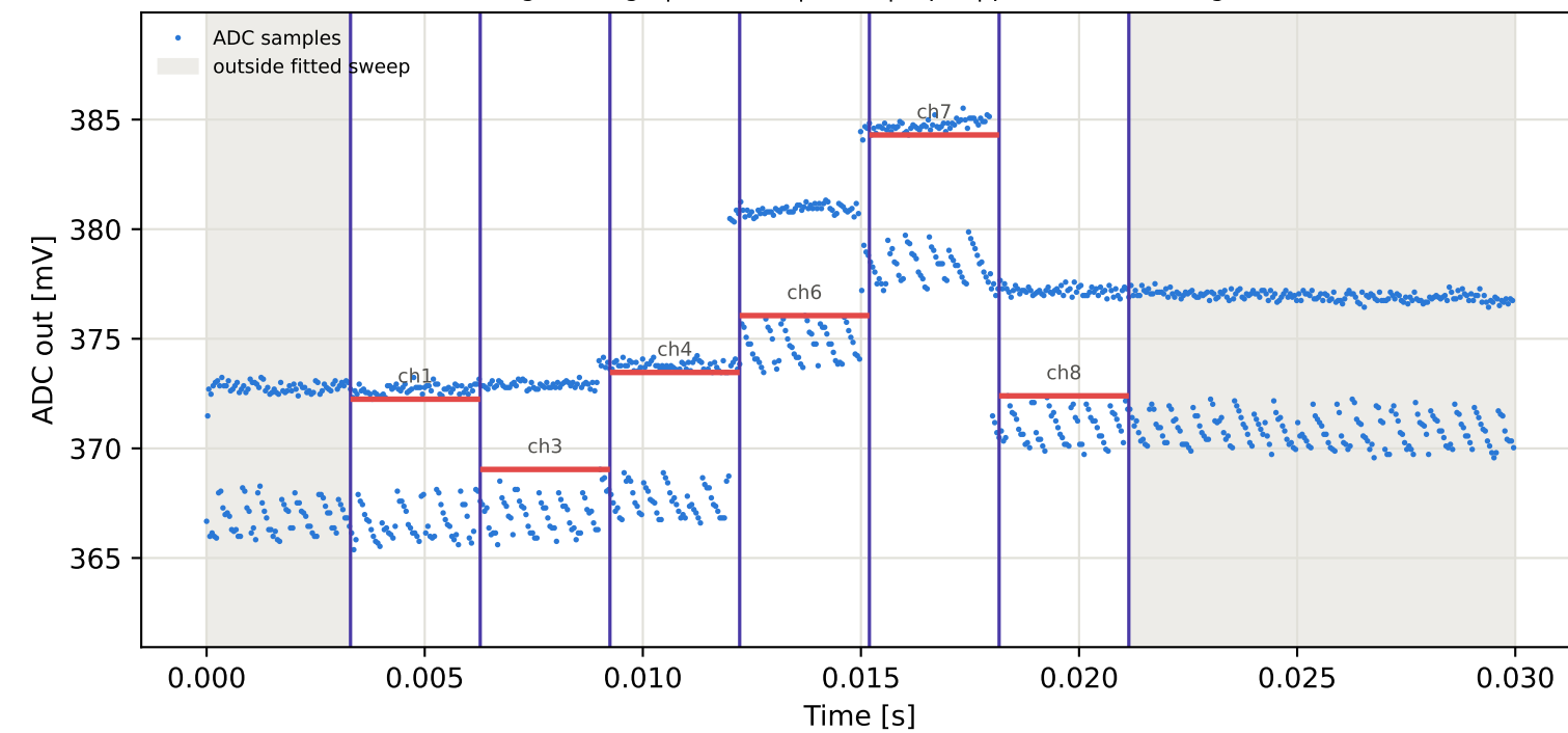
Tag4 &lt;- Tag15 | 945 MHz | run 0 | rep 1 | phase -30.77 deg
