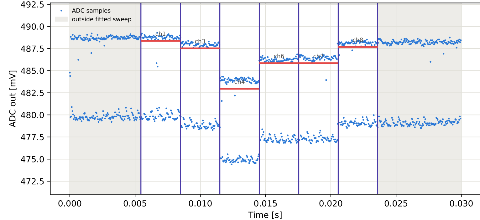
Tag7 &lt;- Tag15 | 995 MHz | run 0 | rep 1 | phase -99.12 deg
