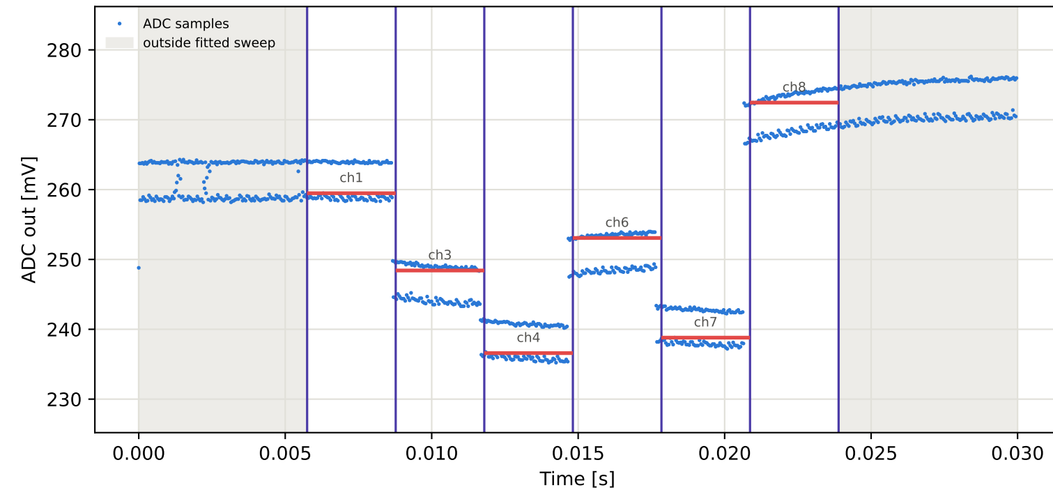
Tag1 &lt;- Tag3 | 895 MHz | run 0 | rep 1 | phase 161.41 deg
