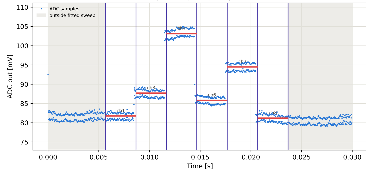
Tag4 &lt;- Tag15 | 995 MHz | run 0 | rep 1 | phase 4.49 deg
