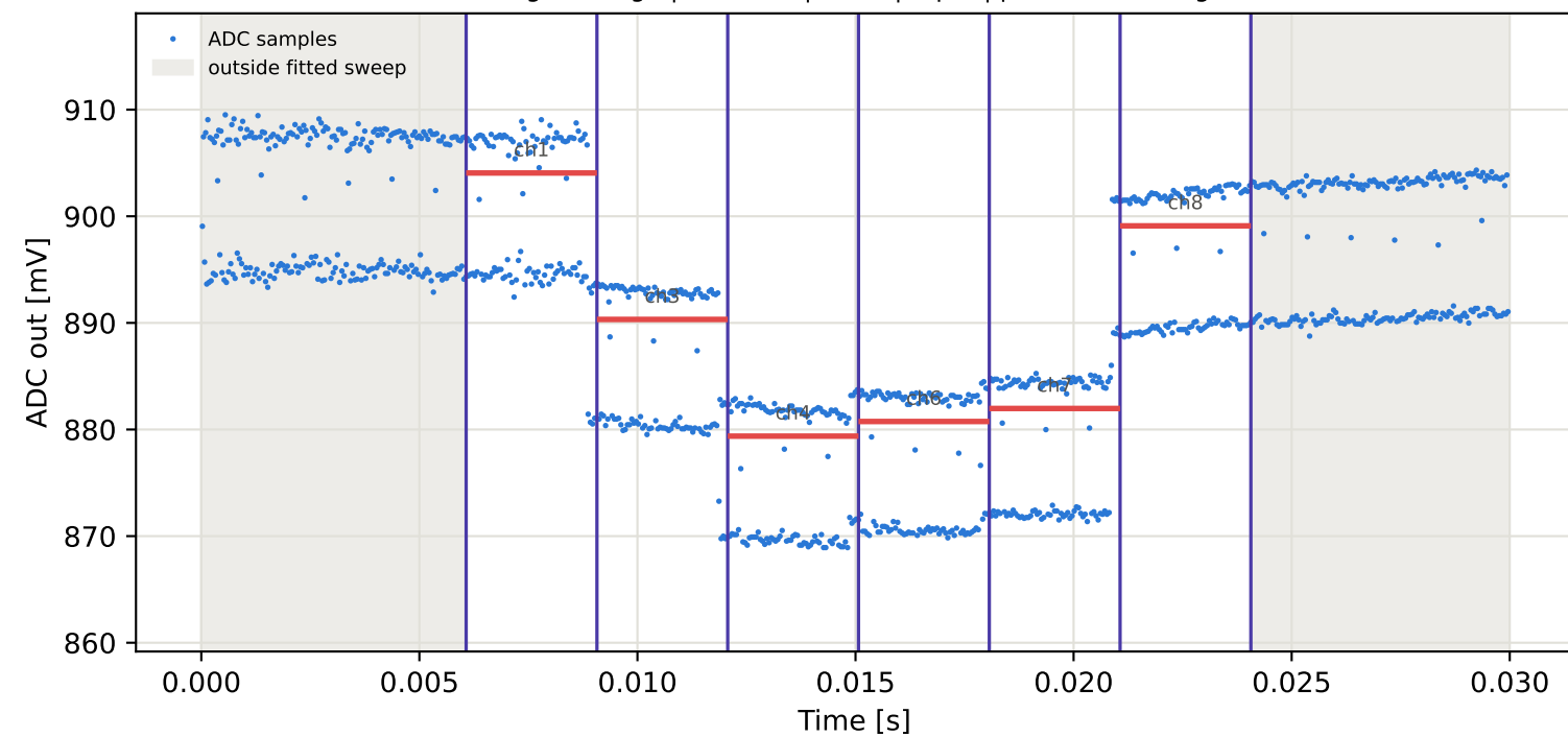
Tag5 &lt;- Tag4 | 875 MHz | run 0 | rep 1 | phase 70.60 deg
