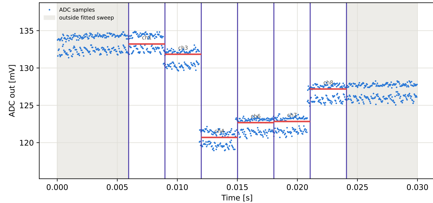
Tag9 &lt;- Tag16 | 825 MHz | run 0 | rep 1 | phase -57.19 deg
