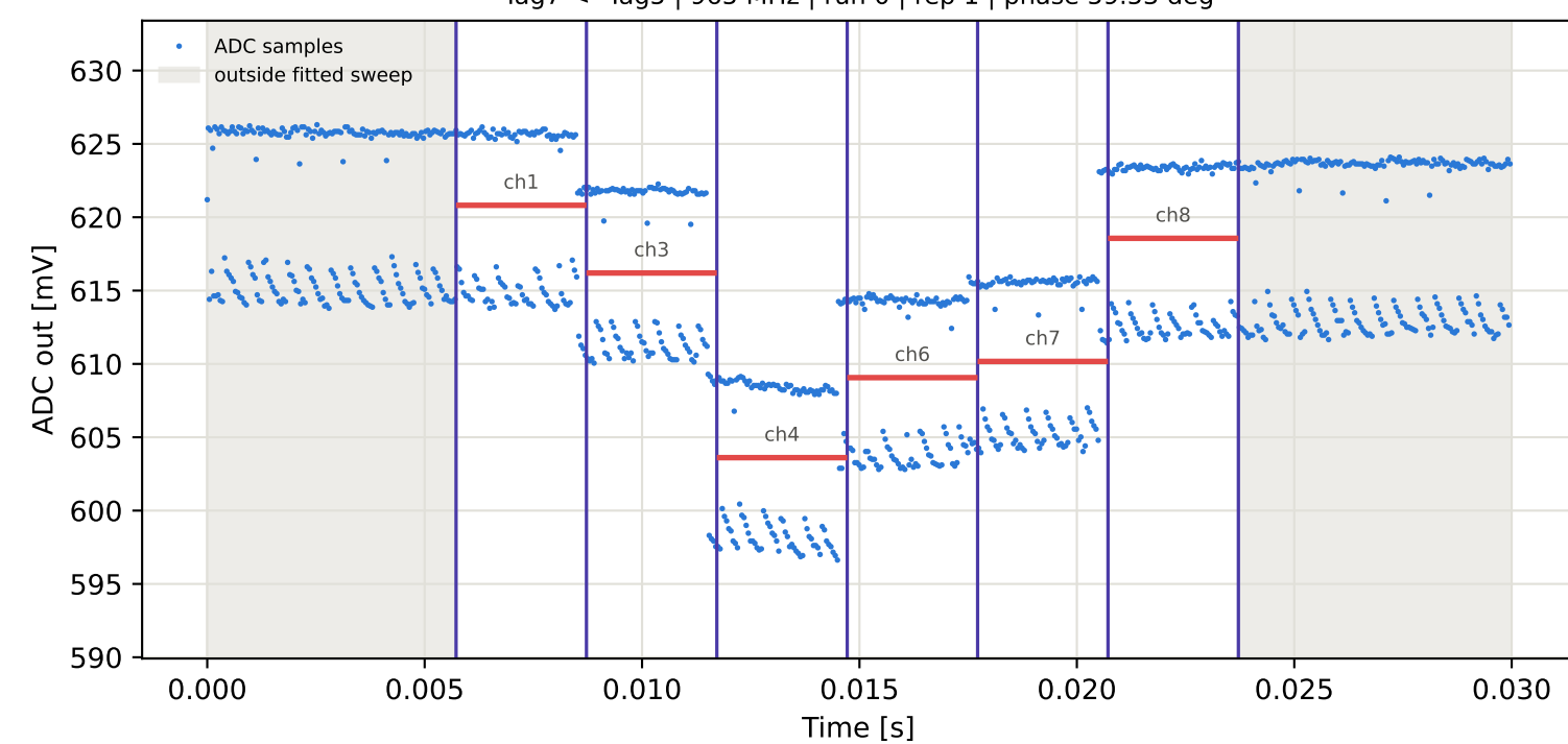
Tag7 &lt;- Tag5 | 965 MHz | run 0 | rep 1 | phase 59.53 deg
