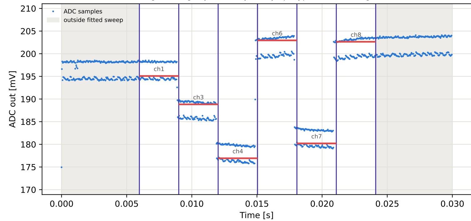
Tag10 &lt;- Tag3 | 995 MHz | run 0 | rep 1 | phase -120.86 deg
