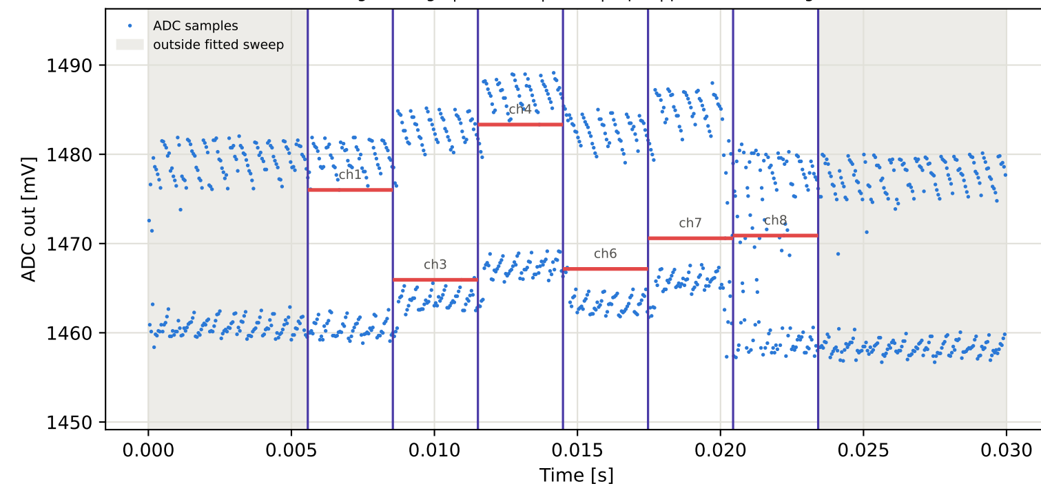
Tag8 &lt;- Tag6 | 915 MHz | run 0 | rep 1 | phase -97.14 deg
