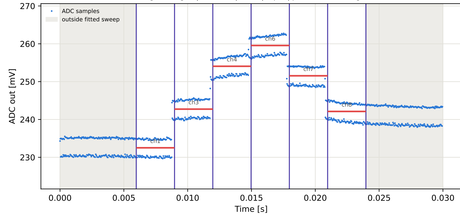
Tag1 &lt;- Tag2 | 895 MHz | run 0 | rep 1 | phase -126.43 deg
