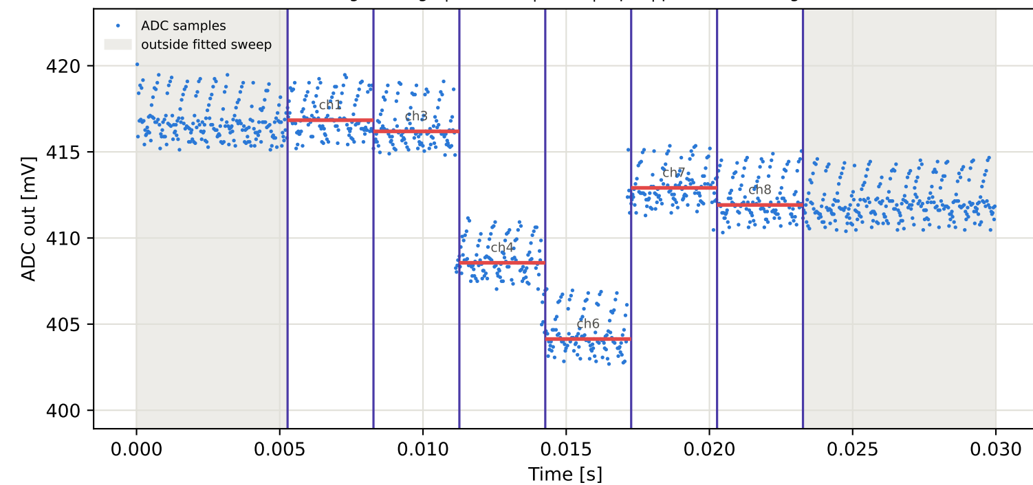
Tag4 &lt;- Tag9 | 965 MHz | run 0 | rep 1 | phase 32.33 deg
