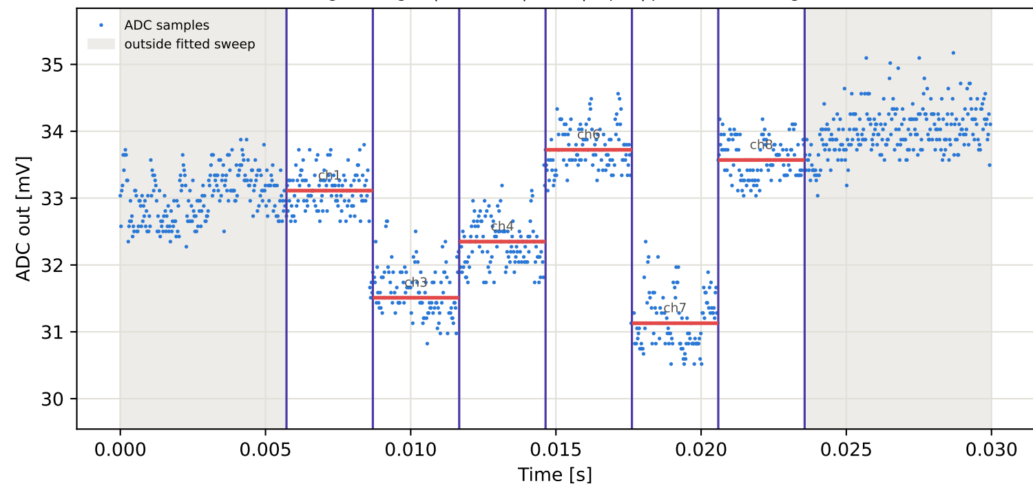
Tag6 &lt;- Tag2 | 775 MHz | run 0 | rep 1 | phase 54.69 deg
