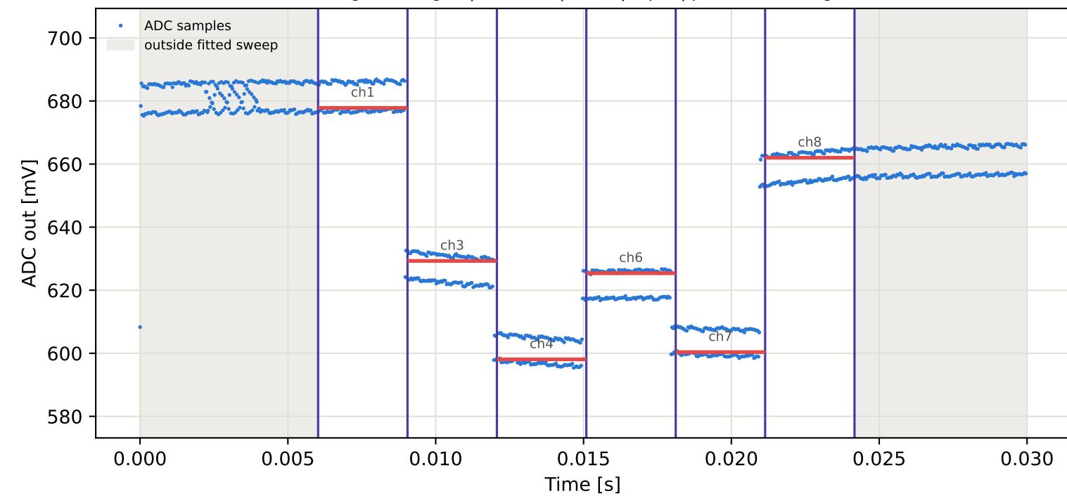
Tag15 &lt;- Tag3 | 865 MHz | run 0 | rep 1 | phase 66.26 deg
