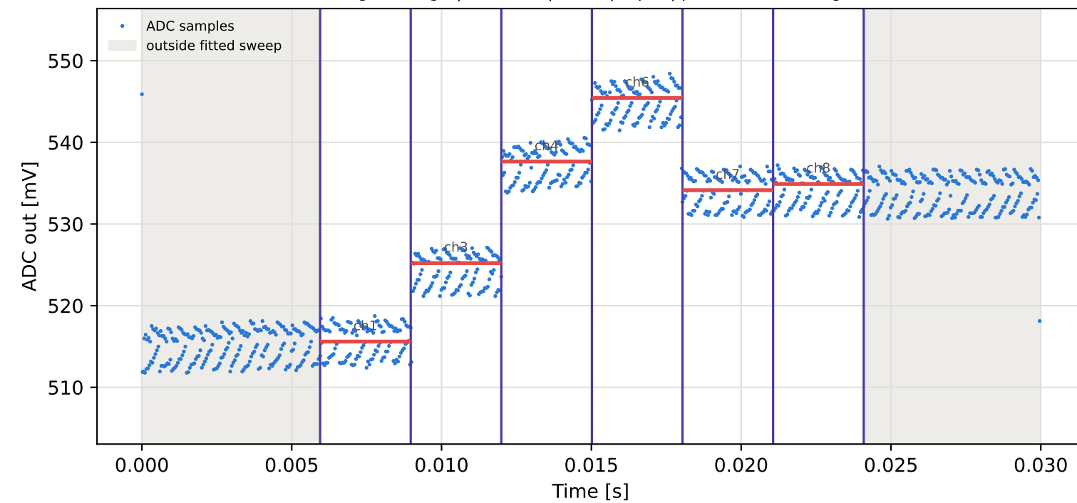
Tag5 &lt;- Tag8 | 865 MHz | run 0 | rep 1 | phase -168.68 deg
