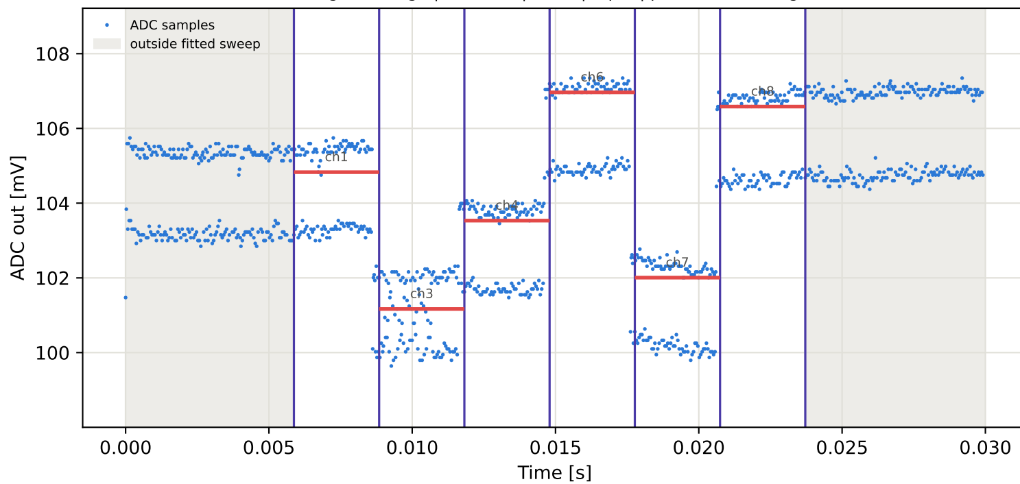
Tag10 &lt;- Tag8 | 795 MHz | run 0 | rep 1 | phase -115.02 deg
