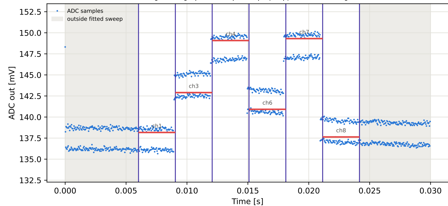
Tag3 &lt;- Tag9 | 805 MHz | run 0 | rep 1 | phase -68.87 deg
