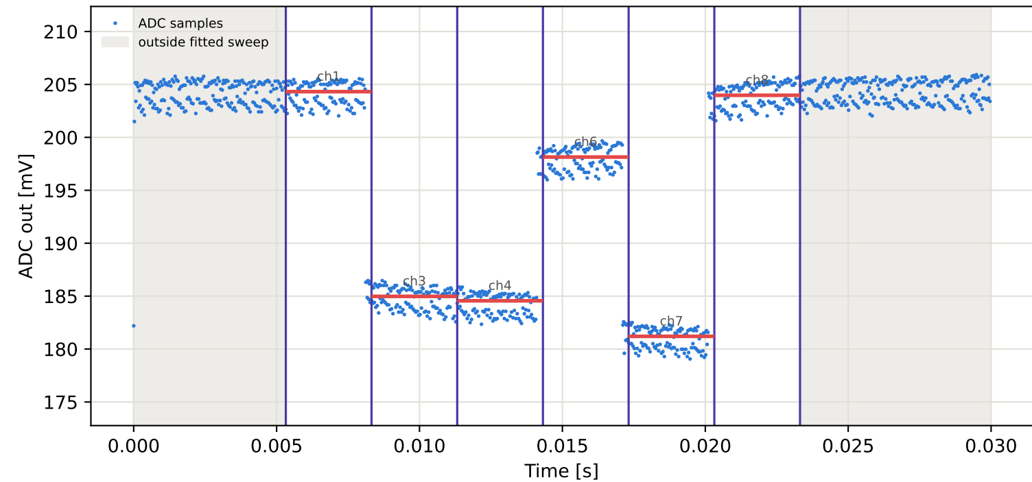
Tag5 &lt;- Tag1 | 825 MHz | run 0 | rep 1 | phase 8.52 deg
