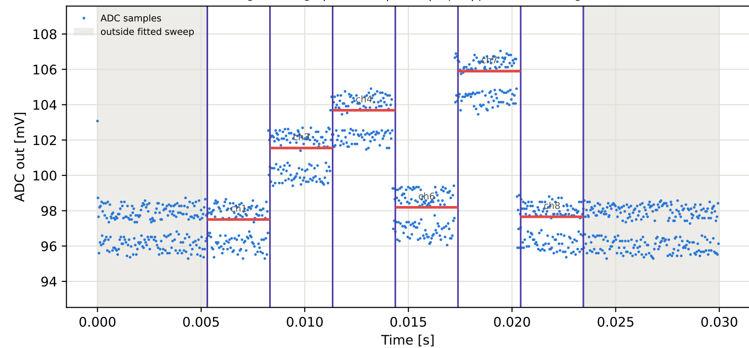
Tag10 &lt;- Tag5 | 795 MHz | run 0 | rep 1 | phase -74.00 deg
