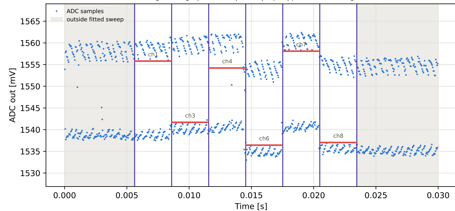
Tag8 &lt;- Tag6 | 905 MHz | run 0 | rep 1 | phase -29.37 deg
