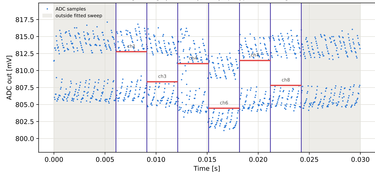
Tag7 &lt;- Tag4 | 895 MHz | run 0 | rep 1 | phase -119.92 deg
