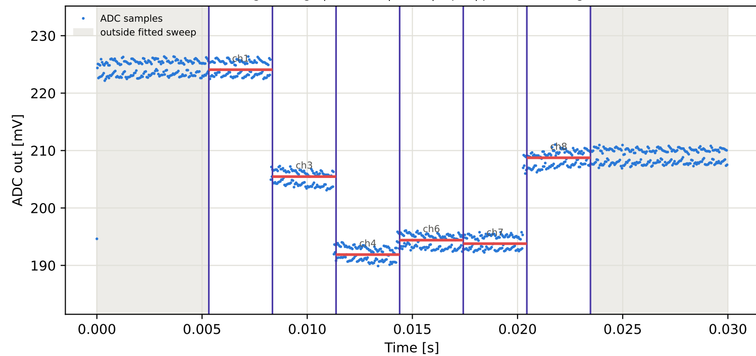
Tag9 &lt;- Tag6 | 855 MHz | run 0 | rep 1 | phase 44.39 deg
