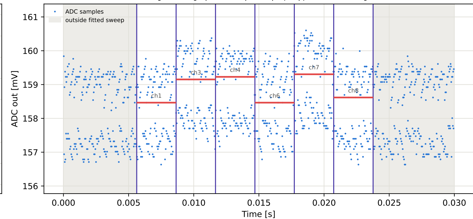
Tag10 &lt;- Tag5 | 845 MHz | run 0 | rep 1 | phase -44.19 deg
