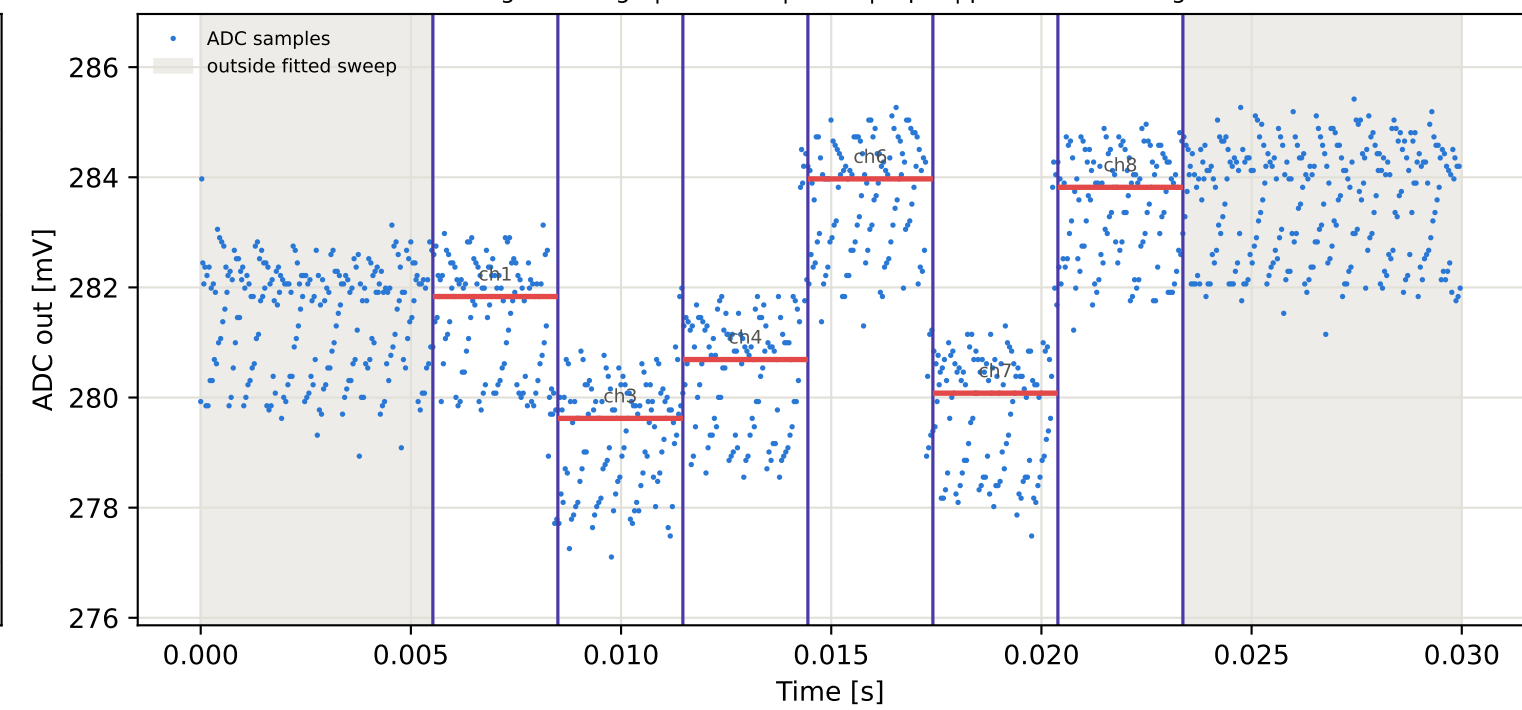
Tag2 &lt;- Tag10 | 835 MHz | run 0 | rep 1 | phase -130.12 deg
