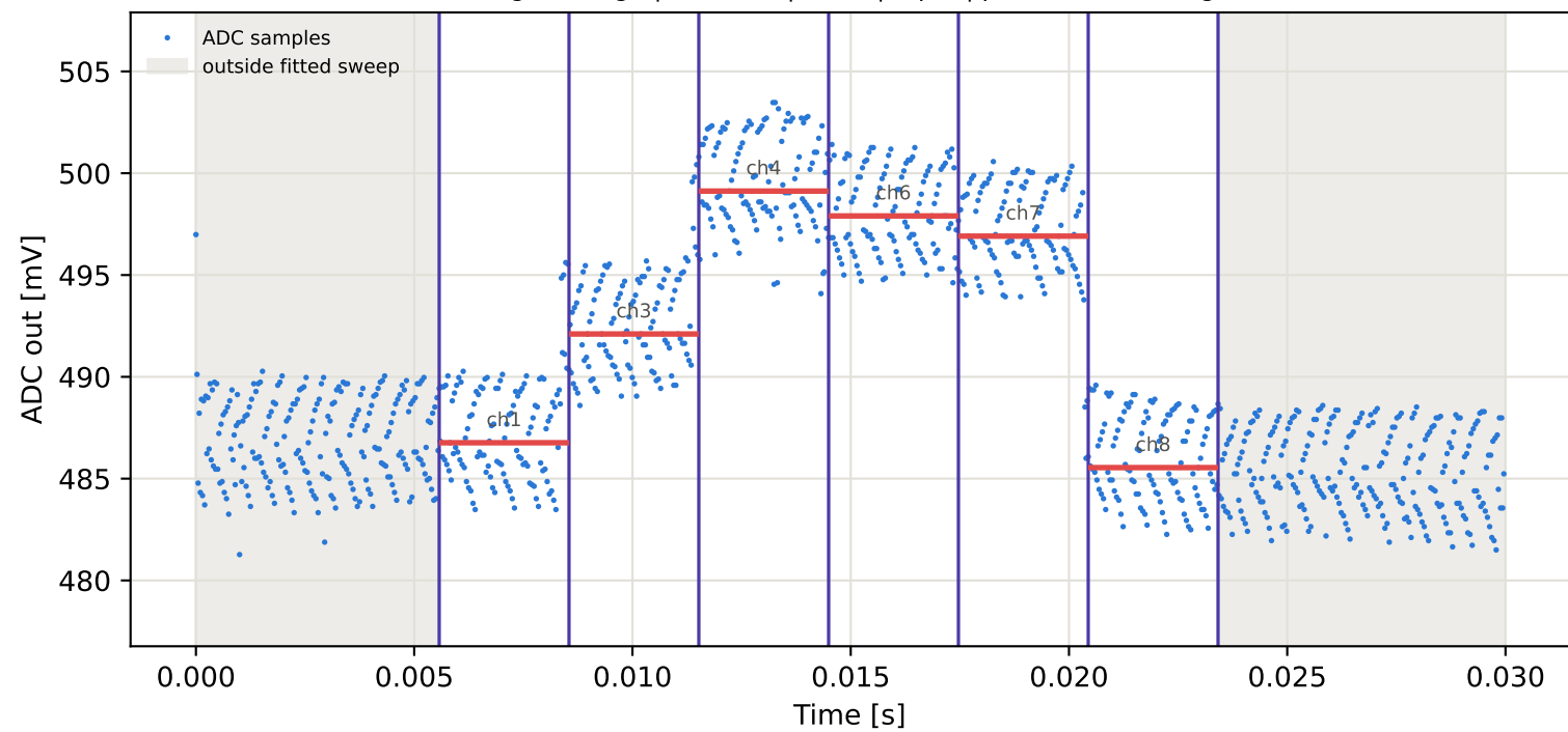
Tag4 &lt;- Tag8 | 905 MHz | run 0 | rep 1 | phase -99.33 deg
