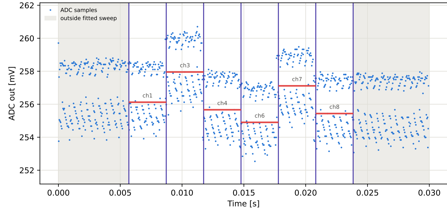
Tag8 &lt;- Tag16 | 785 MHz | run 0 | rep 1 | phase 154.64 deg
