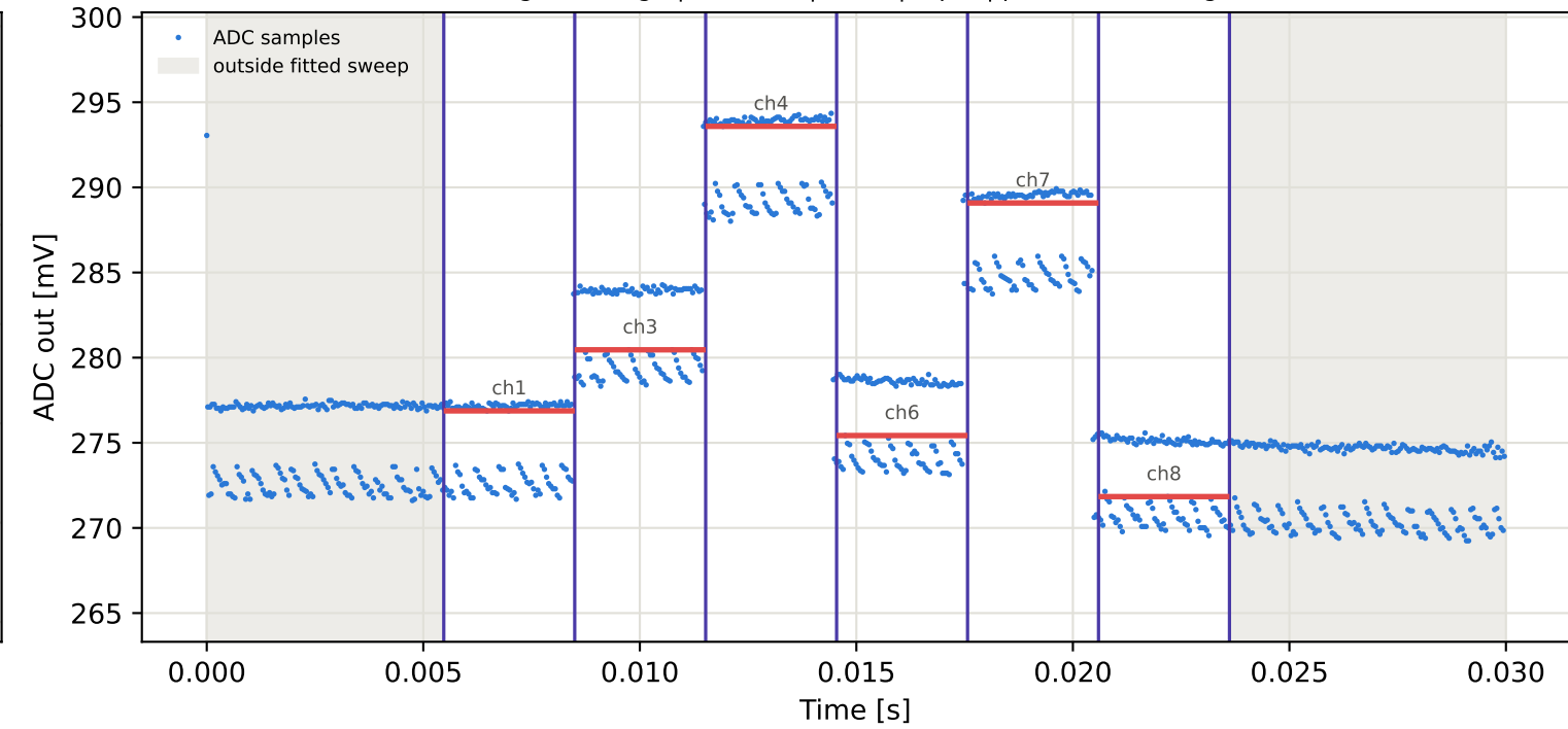
Tag10 &lt;- Tag9 | 975 MHz | run 0 | rep 1 | phase -82.62 deg
