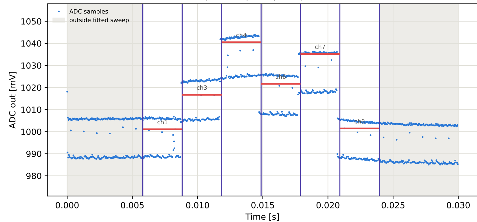
Tag10 &lt;- Tag9 | 925 MHz | run 0 | rep 1 | phase -112.04 deg
