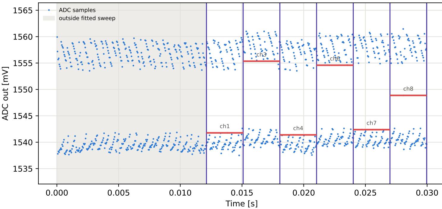
Tag8 &lt;- Tag15 | 905 MHz | run 0 | rep 1 | phase 152.17 deg
