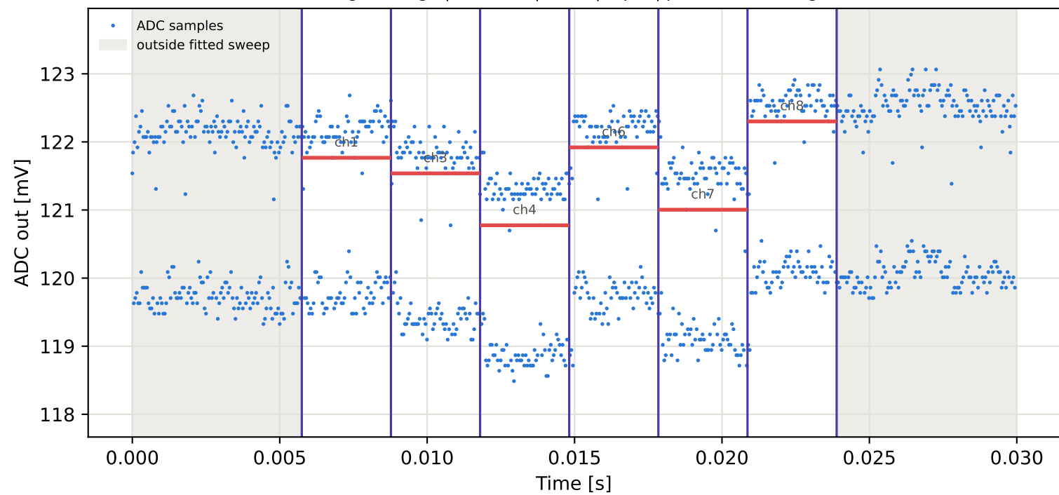
Tag7 &lt;- Tag4 | 795 MHz | run 0 | rep 1 | phase -87.96 deg
