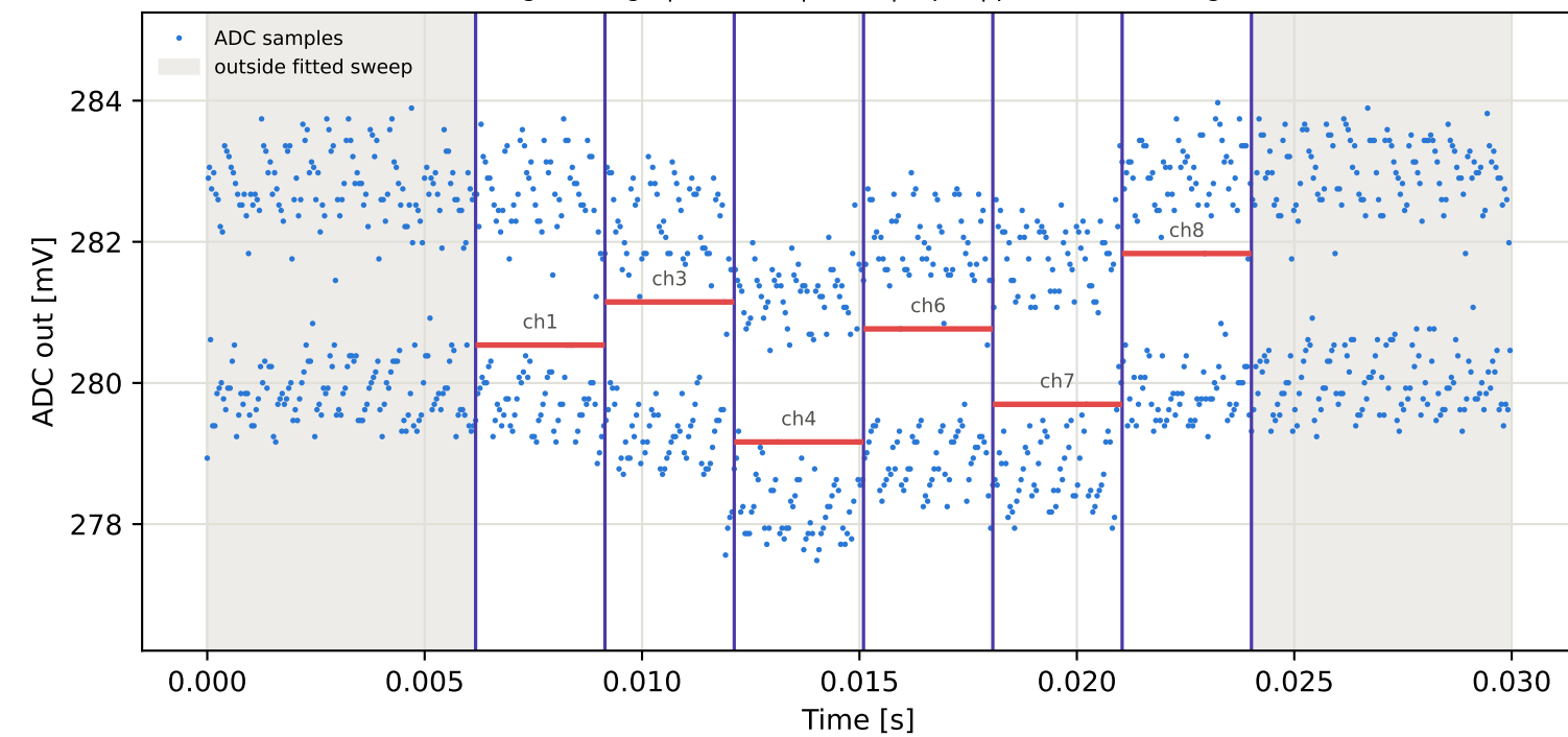
Tag8 &lt;- Tag4 | 795 MHz | run 0 | rep 1 | phase 117.65 deg
