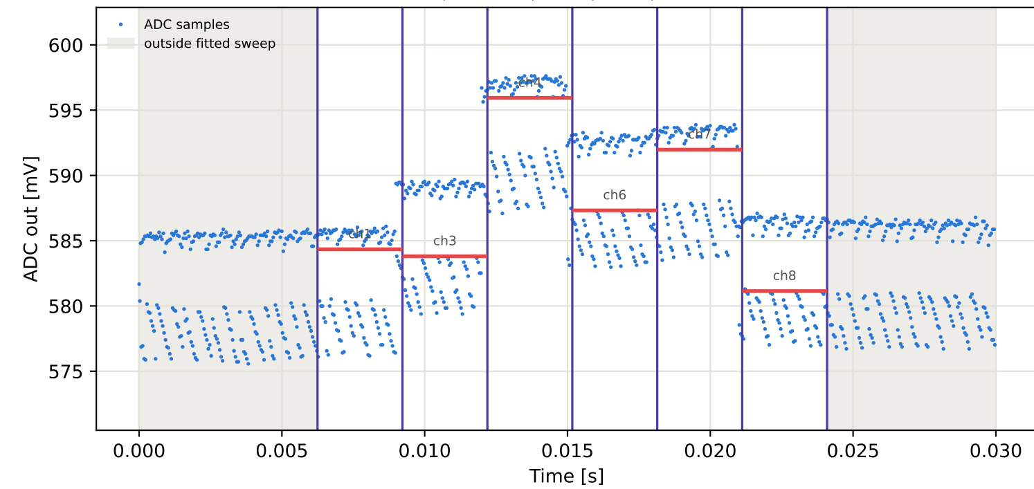
Tag10 &lt;- Tag1 | 945 MHz | run 0 | rep 1 | phase -101.92 deg
