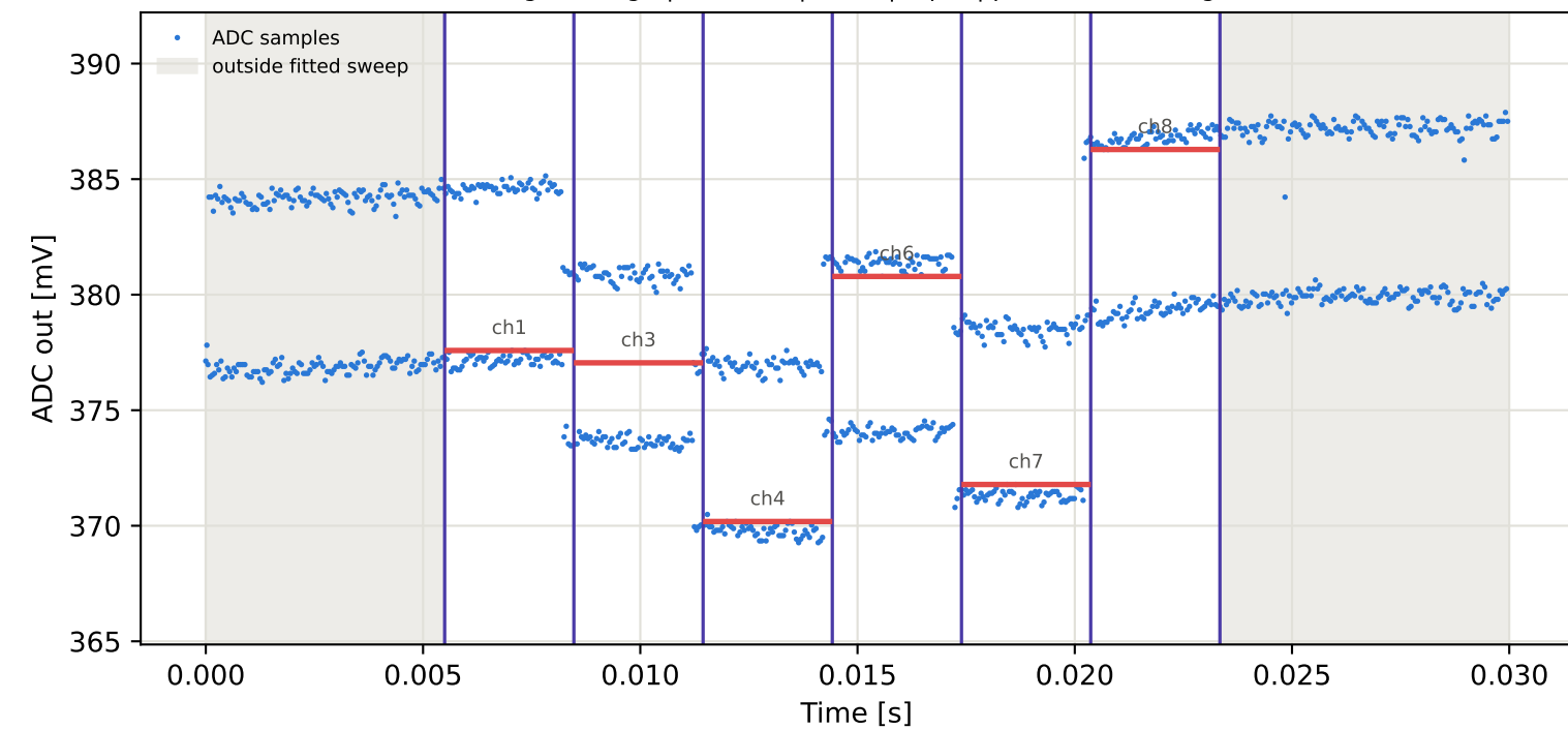
Tag4 &lt;- Tag15 | 915 MHz | run 0 | rep 1 | phase -97.44 deg
