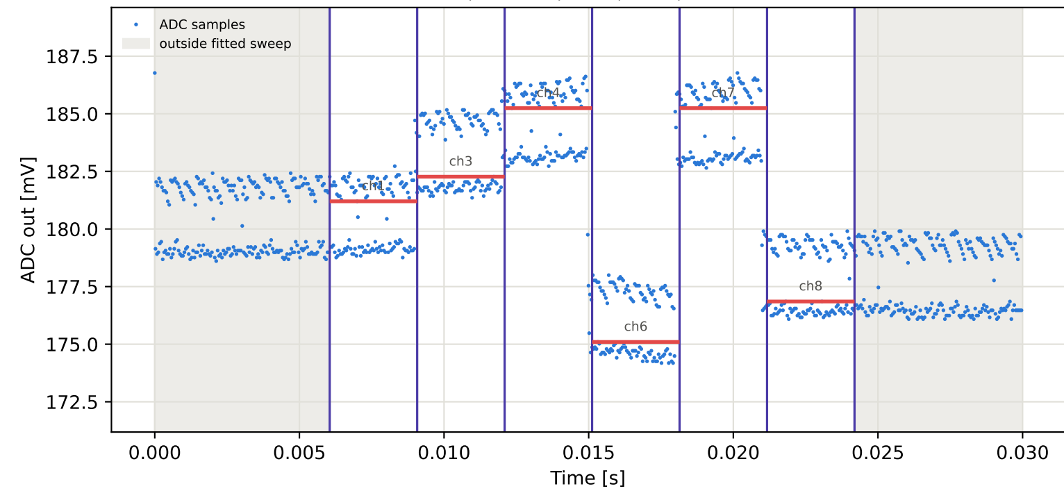
Tag10 &lt;- Tag5 | 995 MHz | run 0 | rep 1 | phase -39.82 deg
