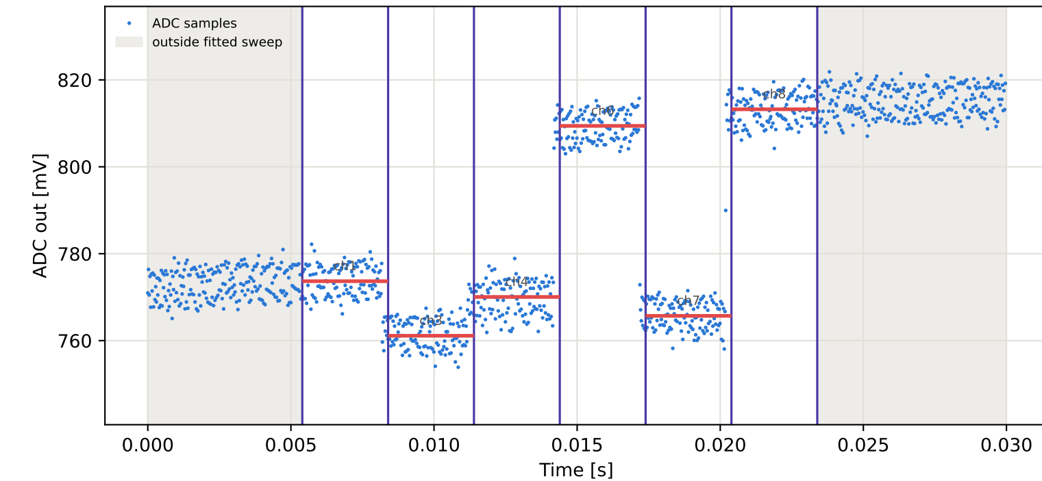
Tag9 &lt;- Tag16 | 885 MHz | run 0 | rep 1 | phase 31.42 deg
