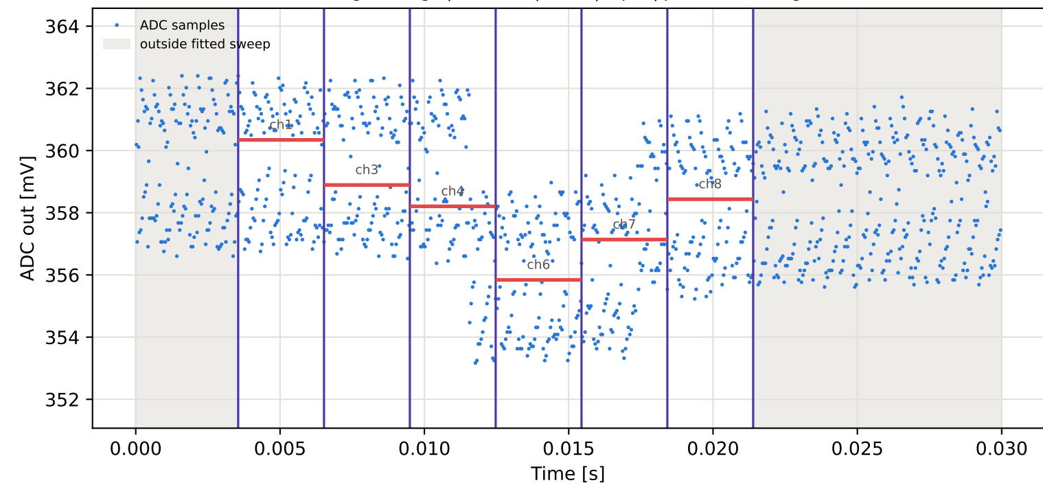
Tag9 &lt;- Tag6 | 985 MHz | run 0 | rep 1 | phase -100.84 deg
