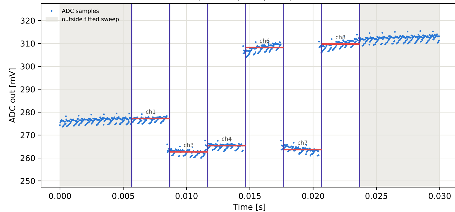
Tag10 &lt;- Tag2 | 905 MHz | run 0 | rep 1 | phase 34.03 deg
