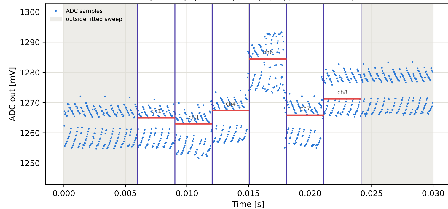
Tag16 &lt;- Tag6 | 905 MHz | run 0 | rep 1 | phase 46.85 deg
