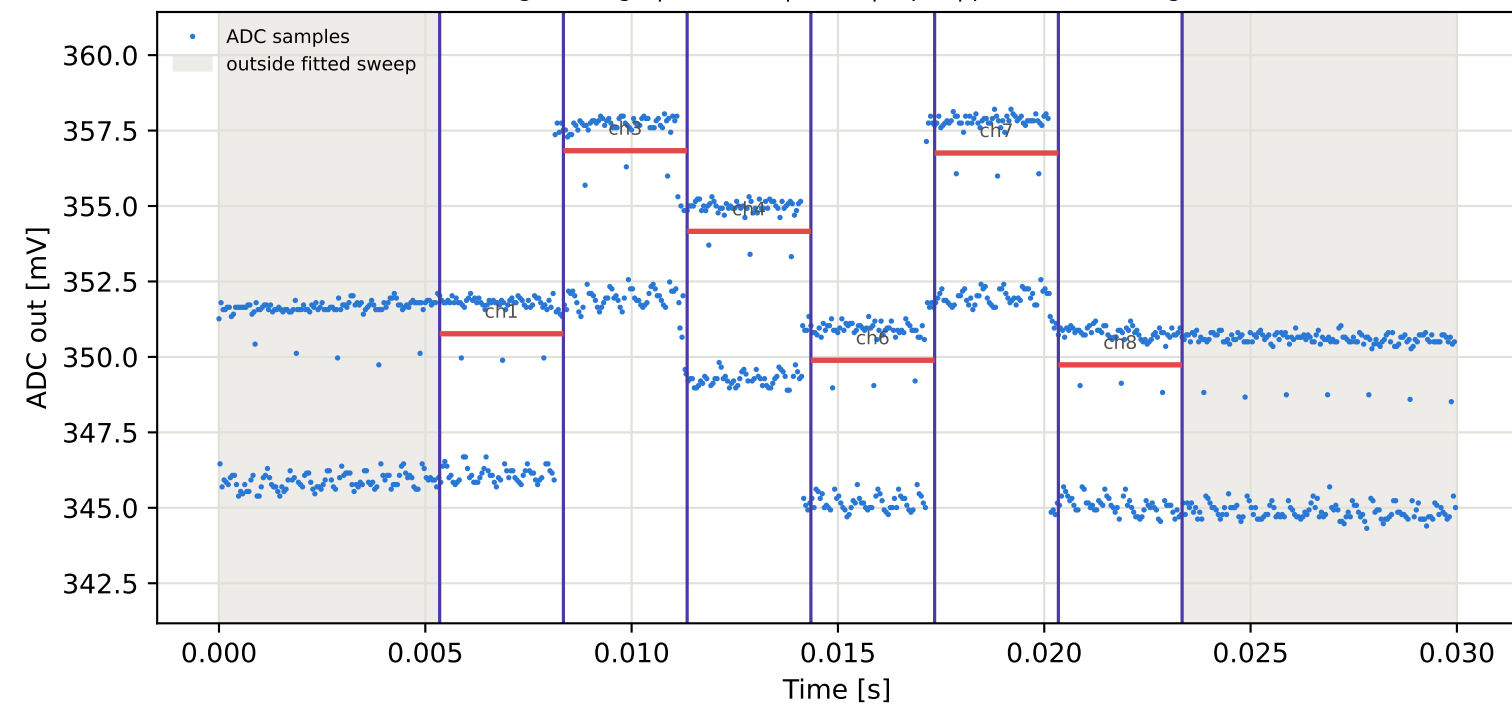
Tag8 &lt;- Tag5 | 805 MHz | run 0 | rep 1 | phase -152.96 deg
