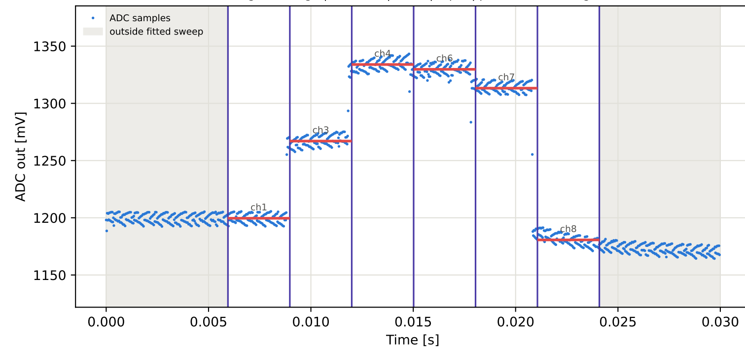
Tag2 &lt;- Tag1 | 905 MHz | run 0 | rep 1 | phase -27.90 deg
