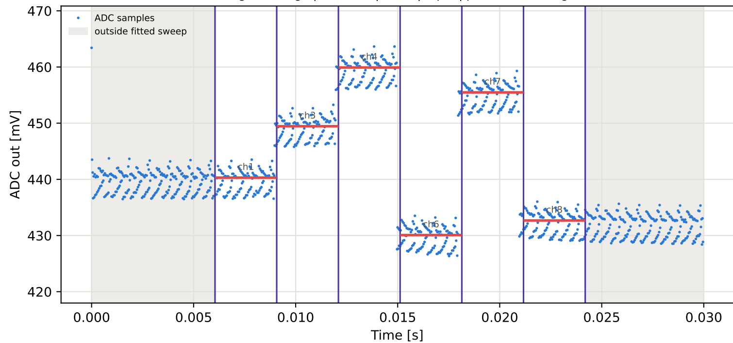
Tag16 &lt;- Tag7 | 995 MHz | run 0 | rep 1 | phase 42.25 deg
