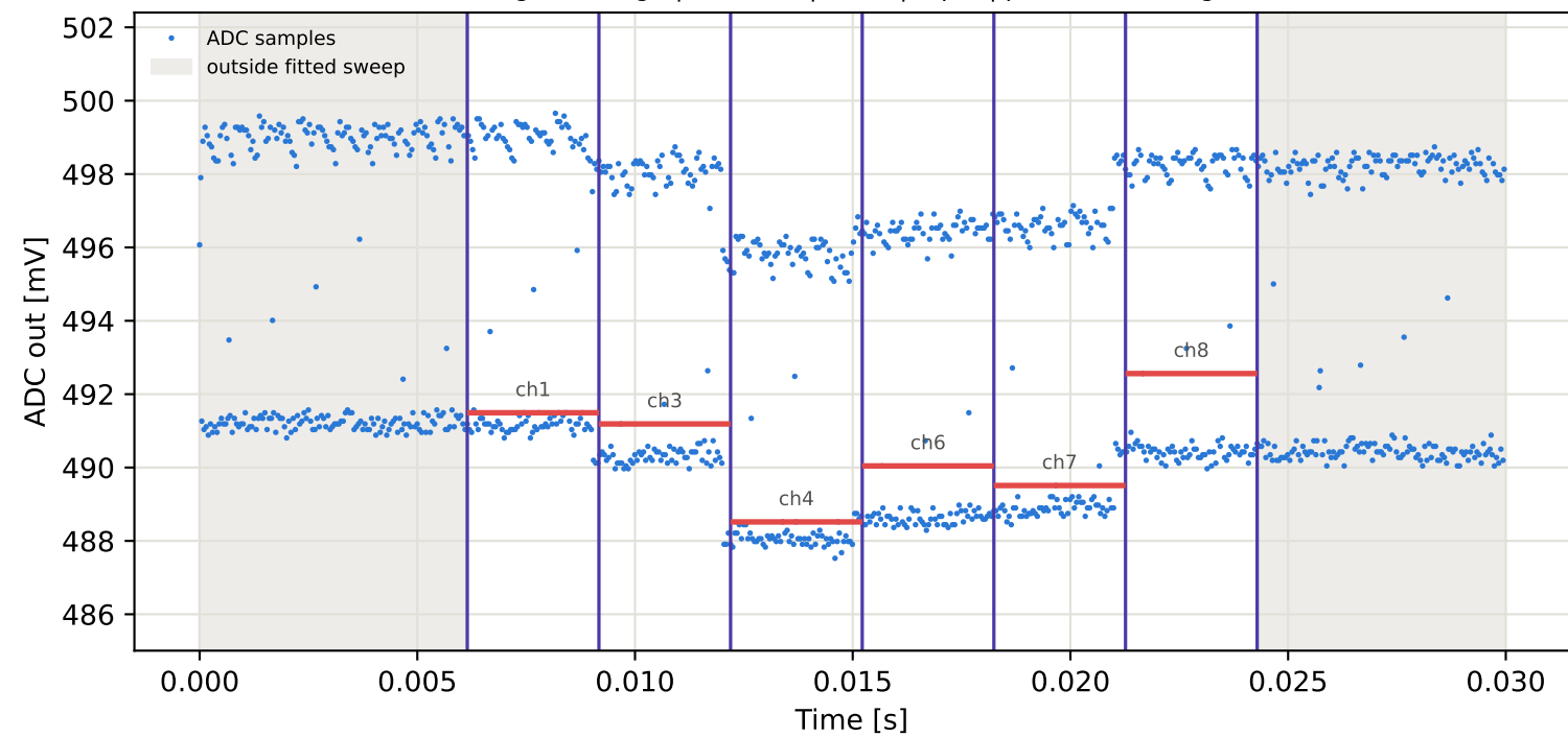
Tag16 &lt;- Tag4 | 845 MHz | run 0 | rep 1 | phase 128.58 deg
