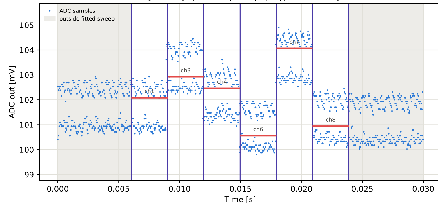
Tag10 &lt;- Tag4 | 775 MHz | run 0 | rep 1 | phase -5.65 deg
