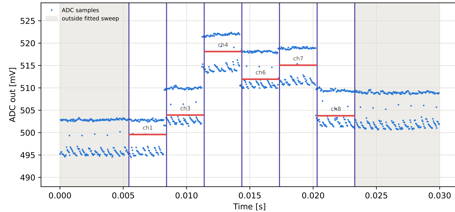
Tag7 &lt;- Tag10 | 855 MHz | run 0 | rep 1 | phase -15.35 deg
