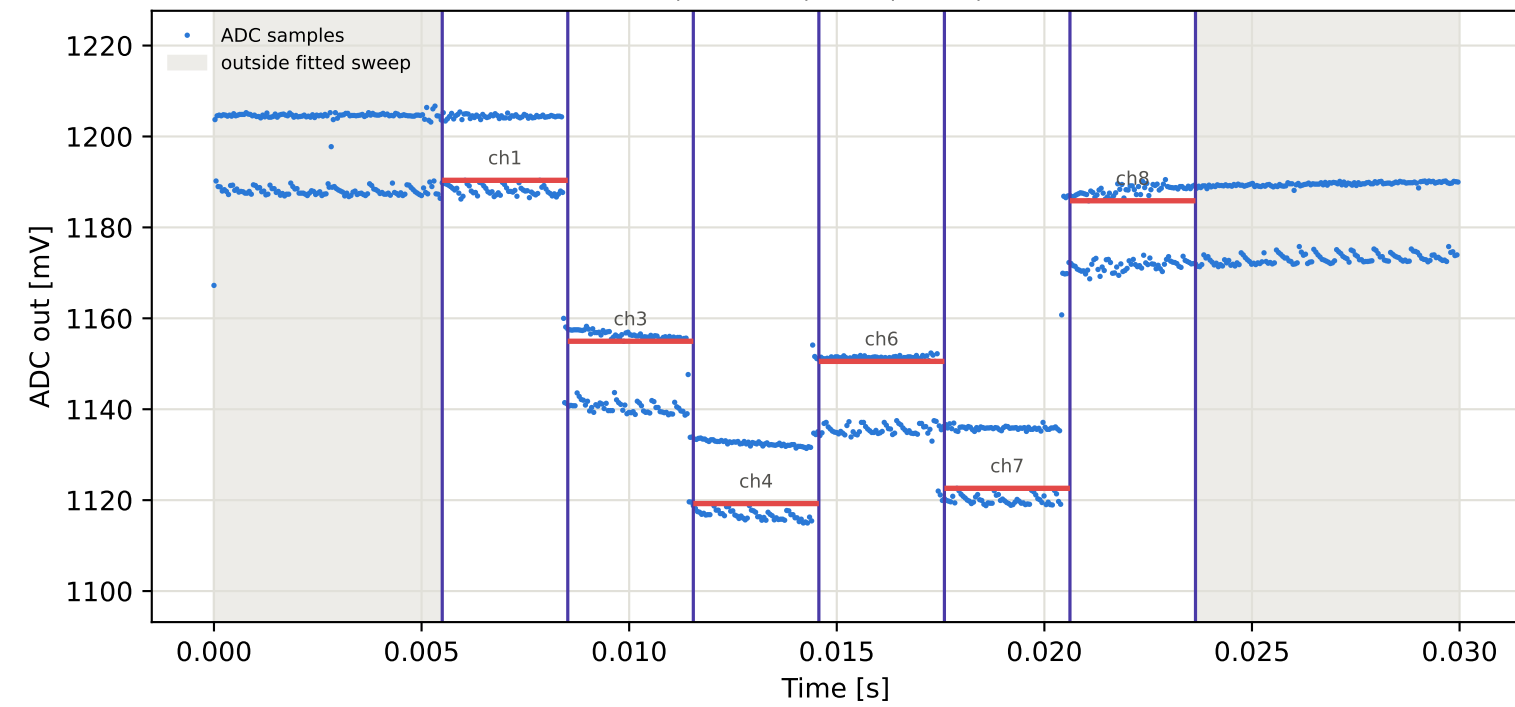
Tag16 &lt;- Tag15 | 875 MHz | run 0 | rep 1 | phase 89.46 deg
