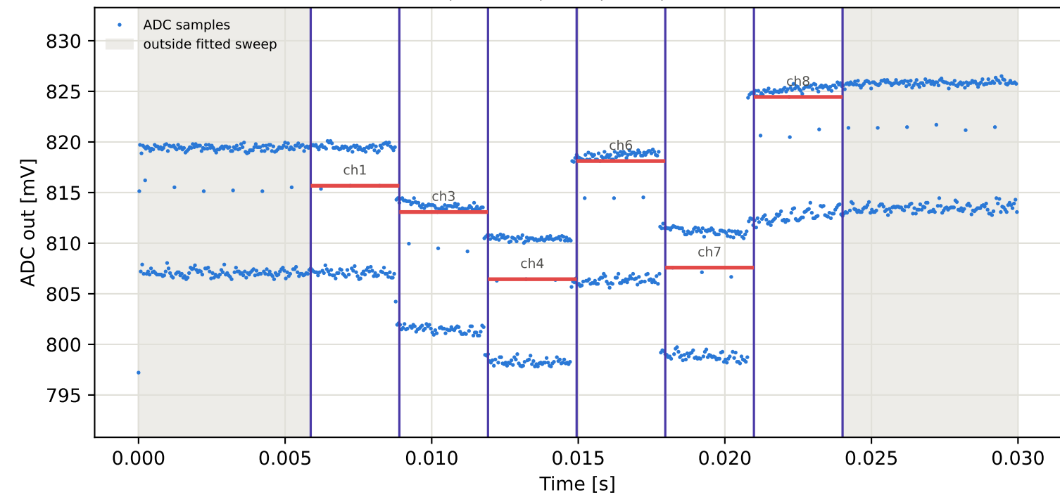
Tag7 &lt;- Tag6 | 895 MHz | run 0 | rep 1 | phase 117.34 deg
