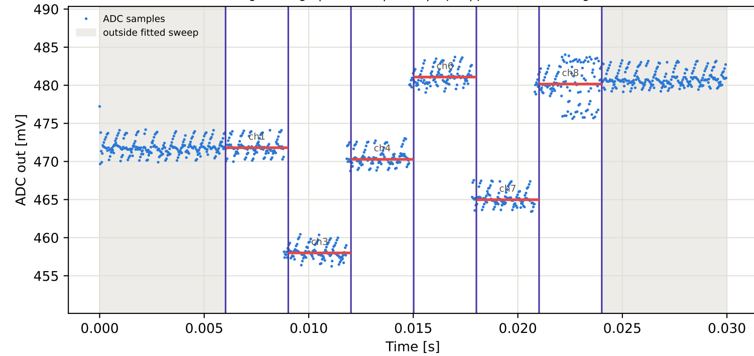
Tag7 &lt;- Tag5 | 835 MHz | run 0 | rep 1 | phase -173.10 deg
