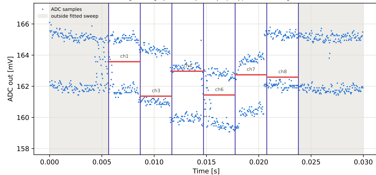
Tag4 &lt;- Tag2 | 935 MHz | run 0 | rep 1 | phase -0.46 deg
