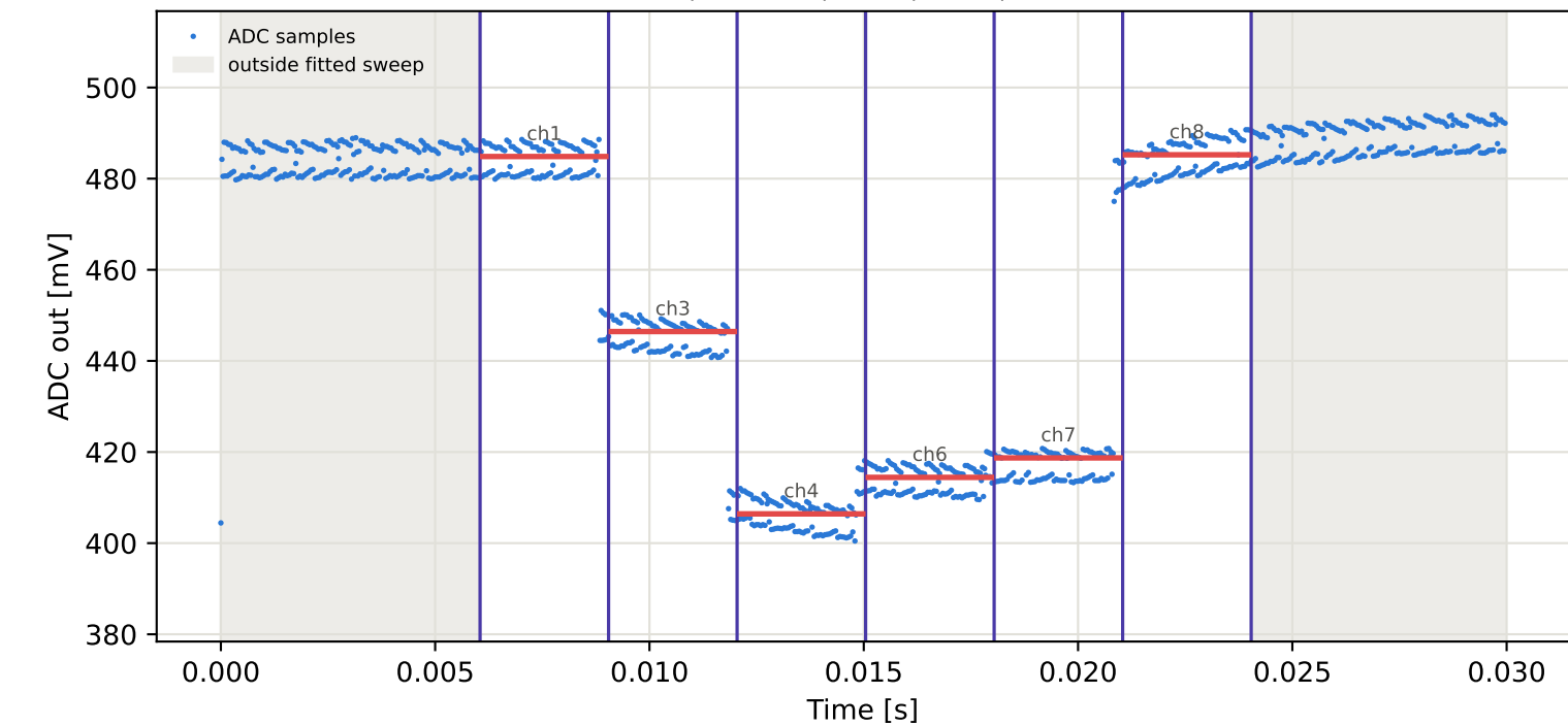
Tag6 &lt;- Tag10 | 895 MHz | run 0 | rep 1 | phase 72.13 deg
