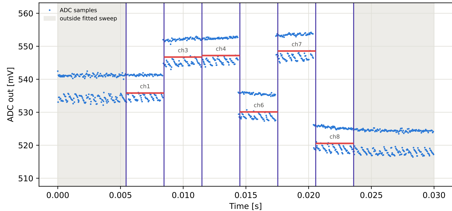
Tag2 &lt;- Tag8 | 875 MHz | run 0 | rep 1 | phase 130.25 deg
