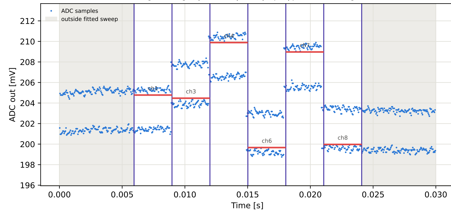
Tag10 &lt;- Tag2 | 985 MHz | run 0 | rep 1 | phase 90.71 deg
