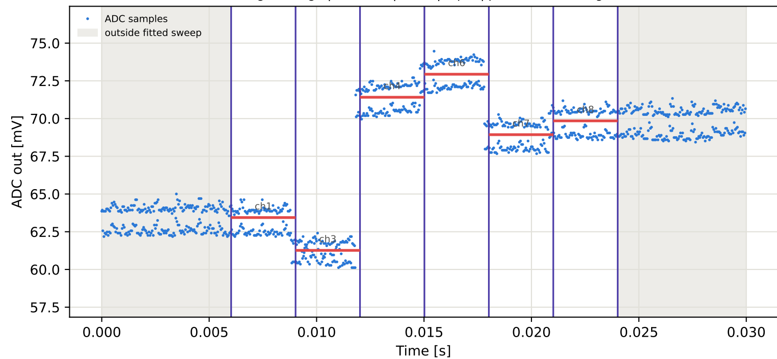
Tag9 &lt;- Tag7 | 835 MHz | run 0 | rep 1 | phase -88.55 deg
