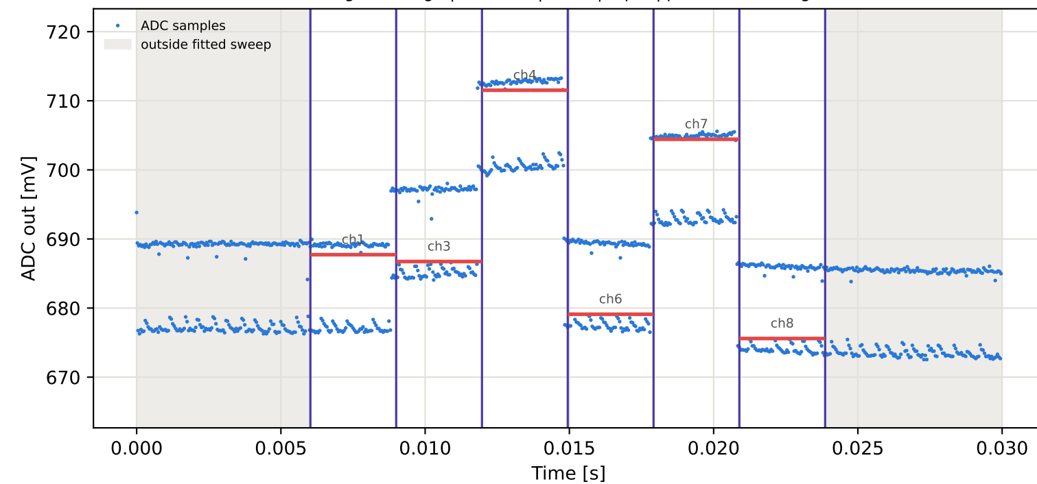
Tag16 &lt;- Tag6 | 975 MHz | run 0 | rep 1 | phase -78.88 deg
