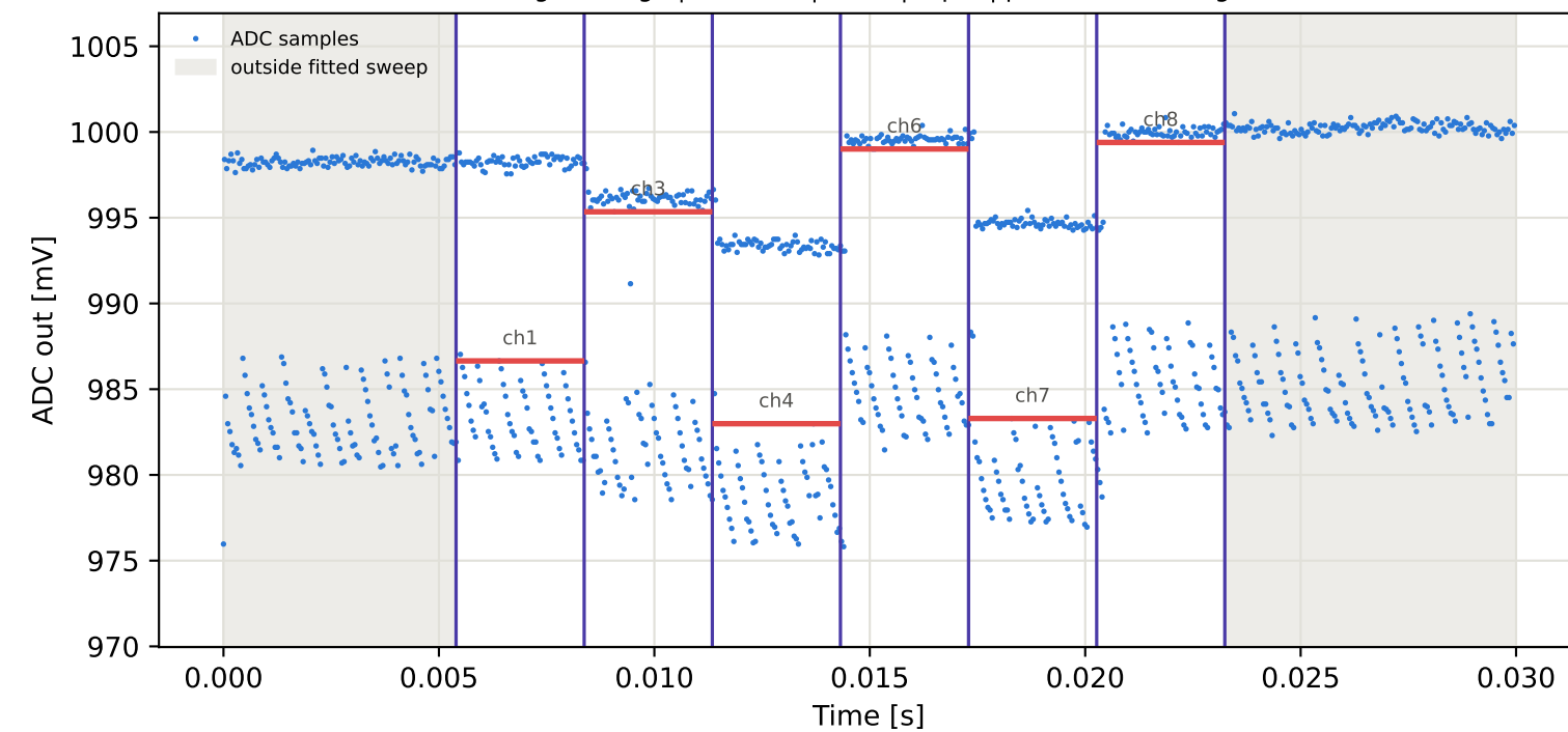
Tag8 &lt;- Tag6 | 945 MHz | run 0 | rep 1 | phase 127.54 deg
