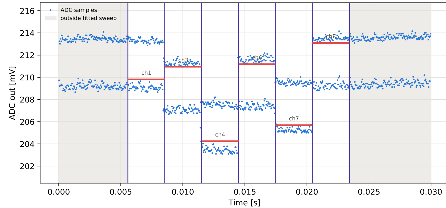
Tag16 &lt;- Tag10 | 975 MHz | run 0 | rep 1 | phase -105.70 deg
