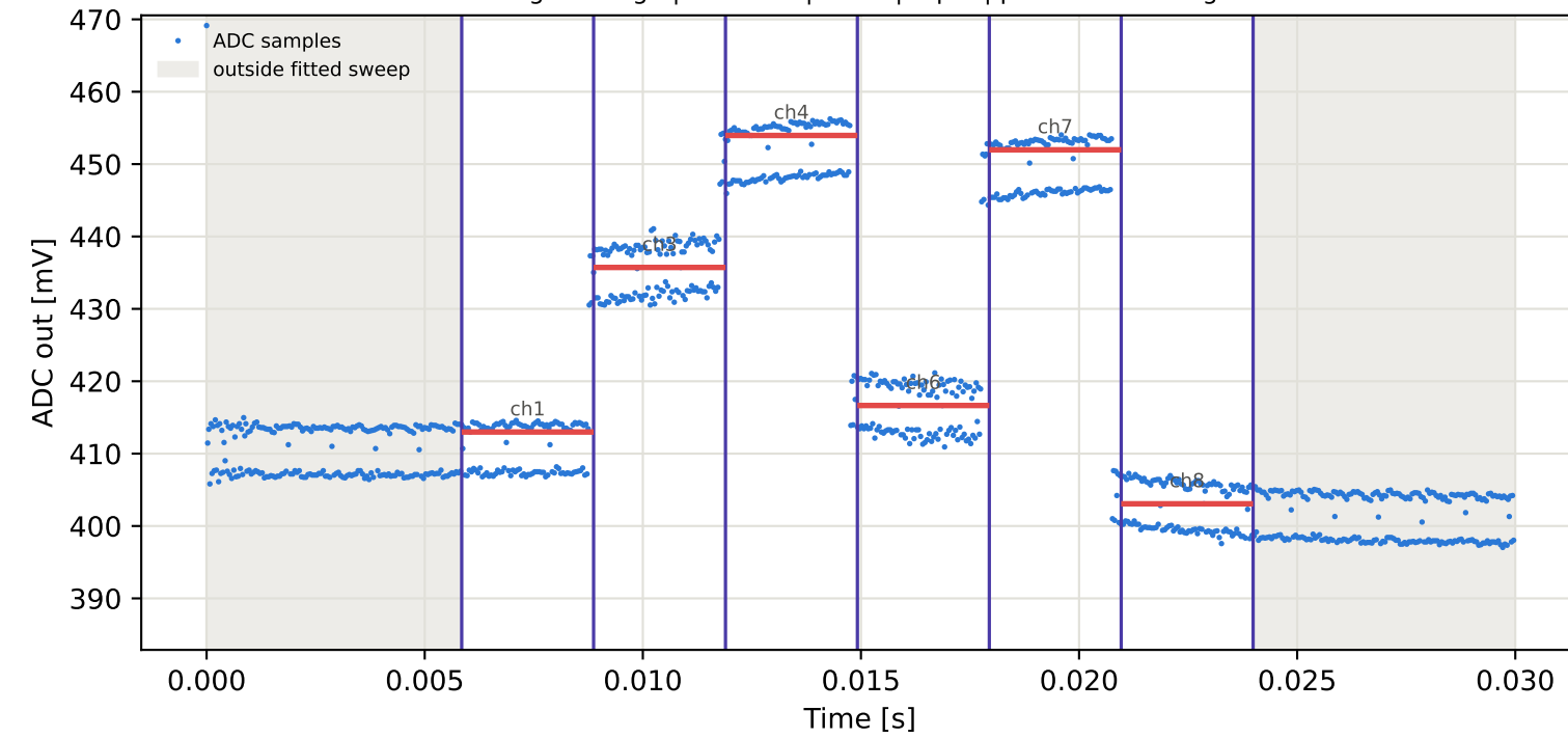
Tag9 &lt;- Tag7 | 875 MHz | run 0 | rep 1 | phase -67.12 deg
