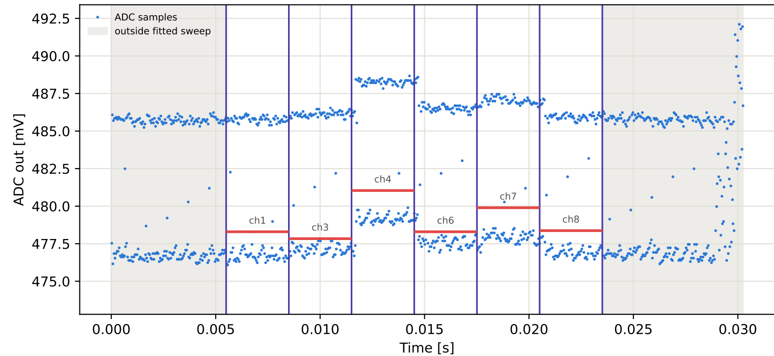
Tag7 &lt;- Tag6 | 995 MHz | run 0 | rep 1 | phase 5.85 deg
