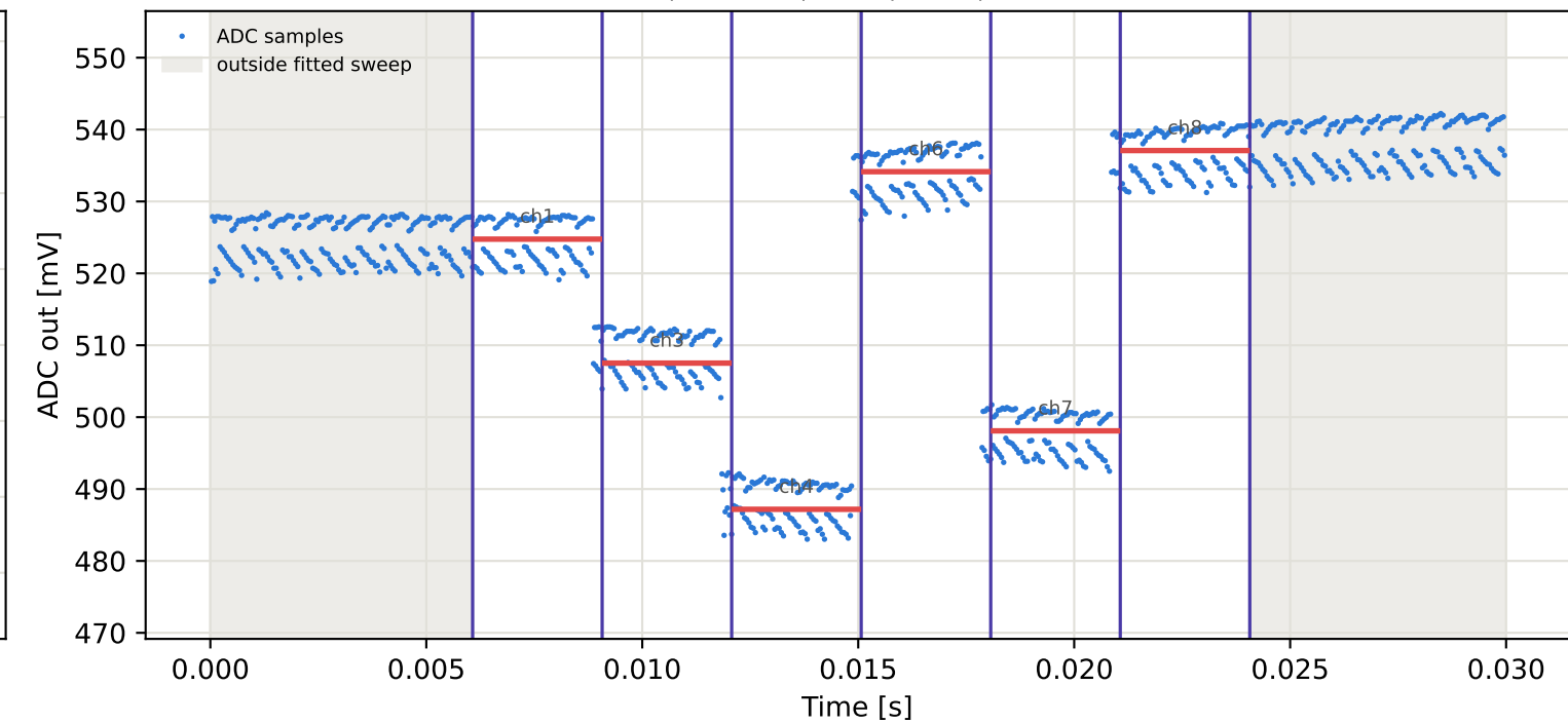
Tag9 &lt;- Tag8 | 945 MHz | run 0 | rep 1 | phase 116.55 deg
