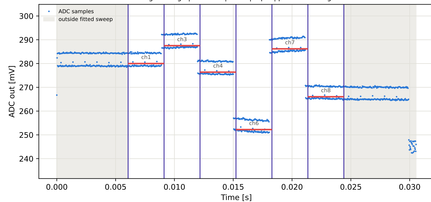
Tag3 &lt;- Tag8 | 985 MHz | run 0 | rep 1 | phase -39.91 deg
