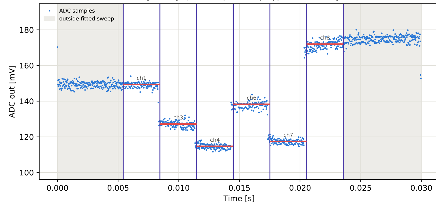
Tag4 &lt;- Tag2 | 885 MHz | run 0 | rep 1 | phase 104.40 deg
