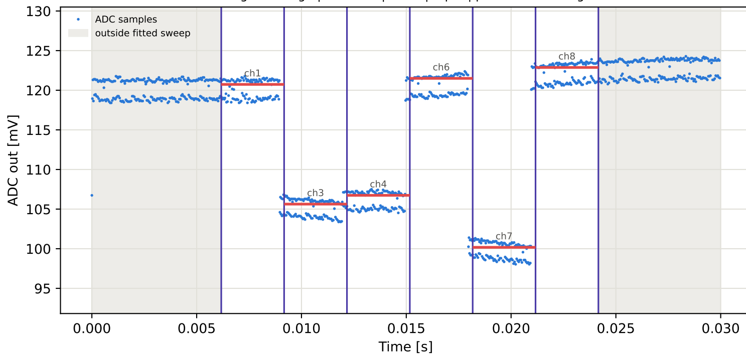
Tag2 &lt;- Tag1 | 795 MHz | run 0 | rep 1 | phase -37.02 deg
