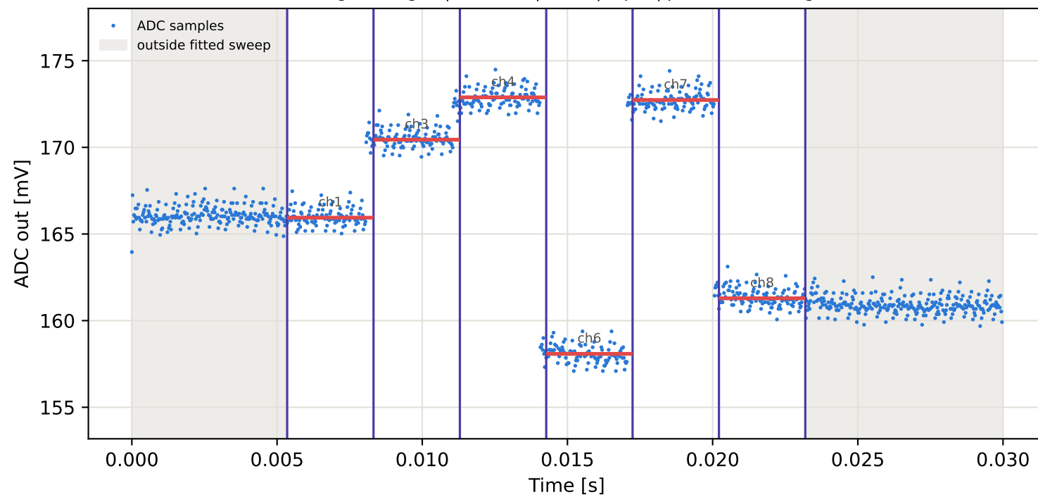
Tag1 &lt;- Tag16 | 995 MHz | run 0 | rep 1 | phase 22.48 deg
