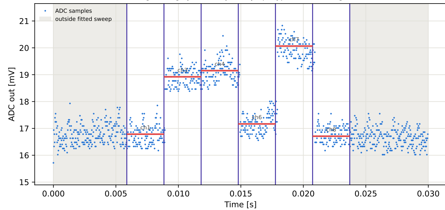
Tag7 &lt;- Tag1 | 795 MHz | run 0 | rep 1 | phase 86.17 deg
