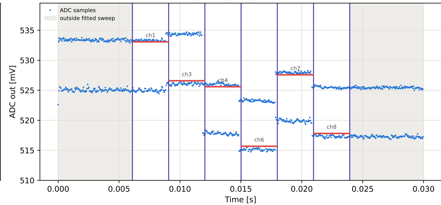
Tag7 &lt;- Tag15 | 855 MHz | run 0 | rep 1 | phase 21.57 deg
