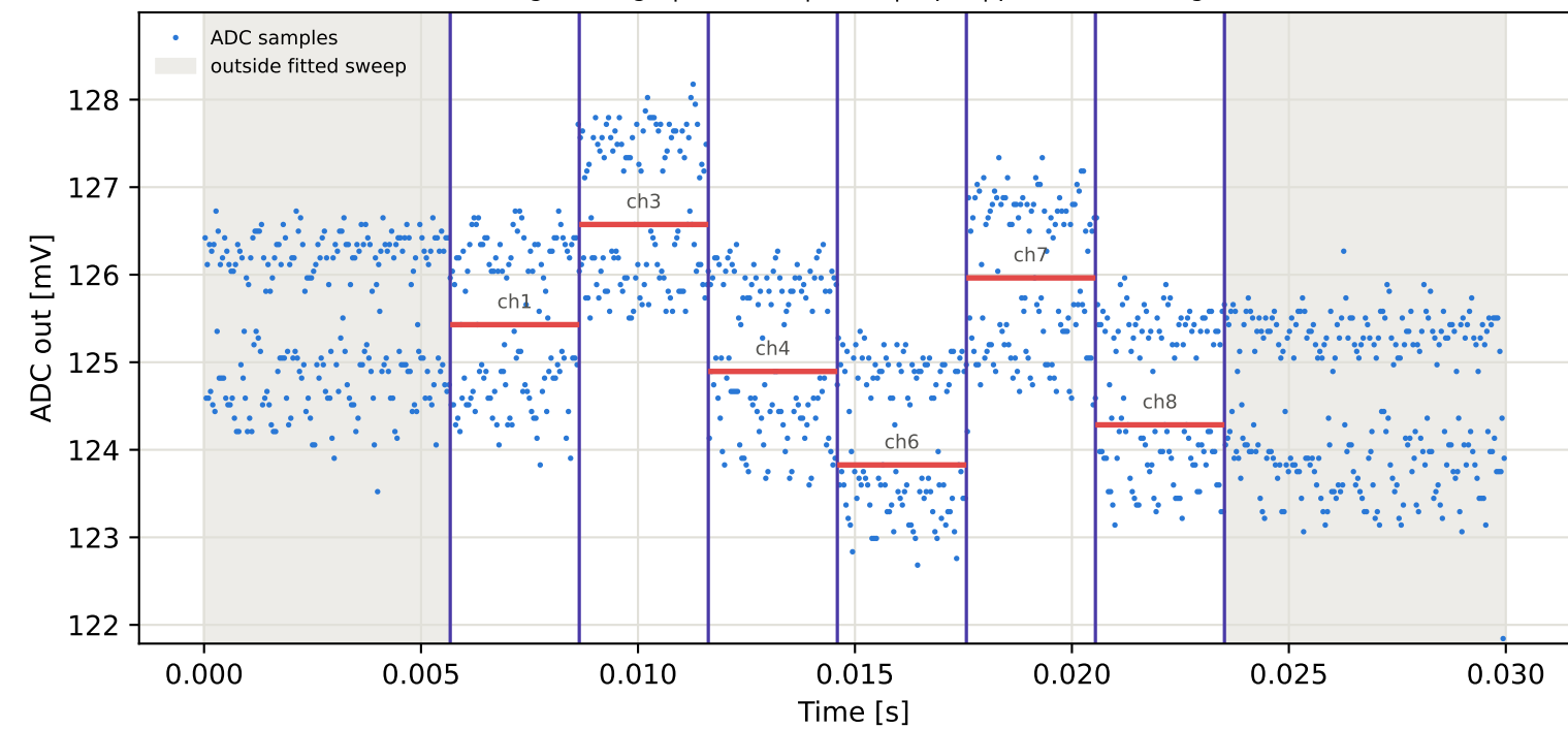
Tag4 &lt;- Tag8 | 795 MHz | run 0 | rep 1 | phase 67.82 deg
