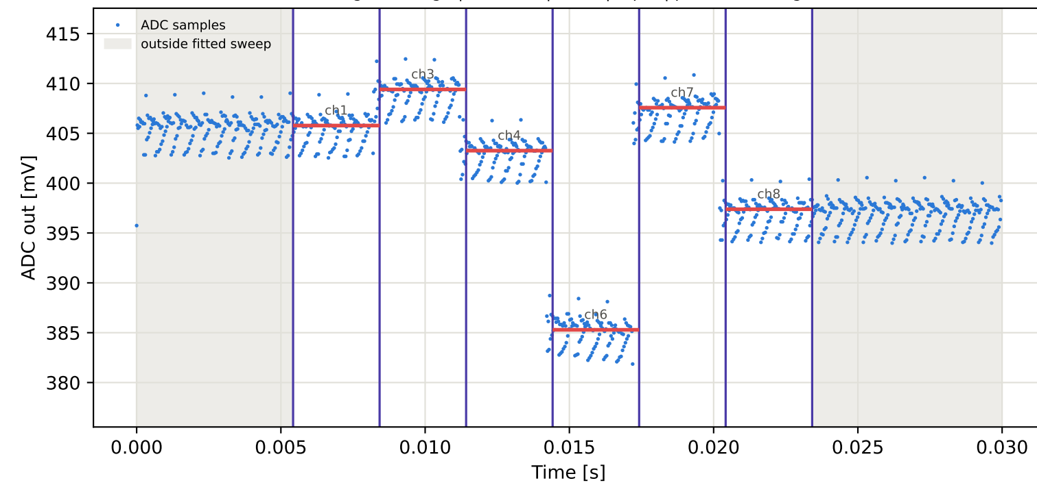
Tag10 &lt;- Tag8 | 955 MHz | run 0 | rep 1 | phase 62.77 deg
