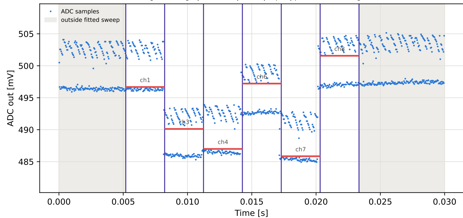
Tag16 &lt;- Tag6 | 845 MHz | run 0 | rep 1 | phase -74.71 deg
