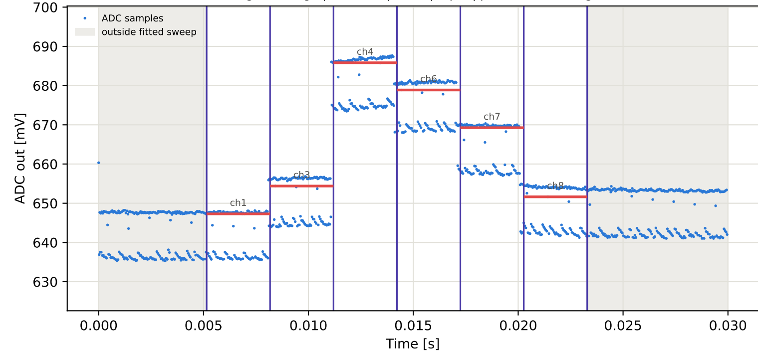
Tag16 &lt;- Tag5 | 965 MHz | run 0 | rep 1 | phase -130.63 deg
