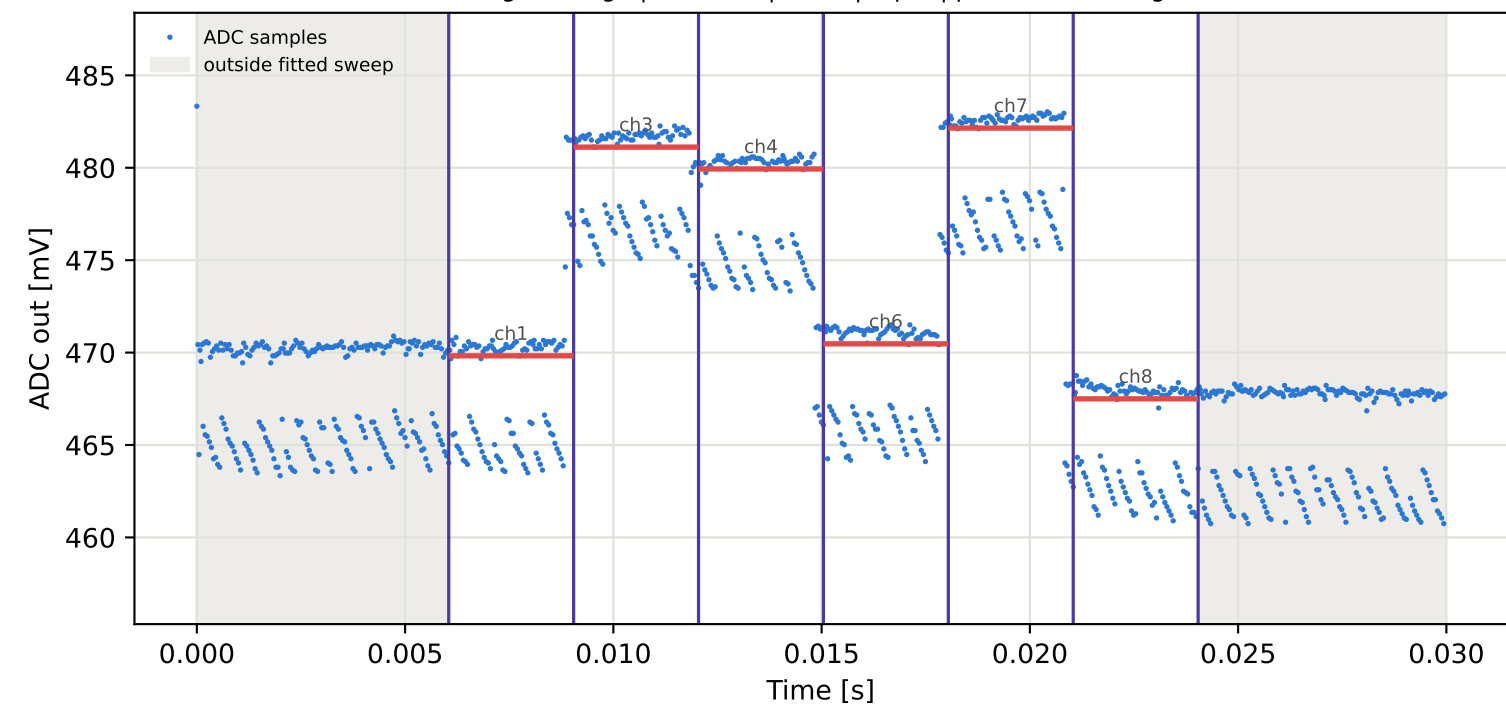
Tag7 &lt;- Tag6 | 835 MHz | run 0 | rep 1 | phase -40.69 deg
