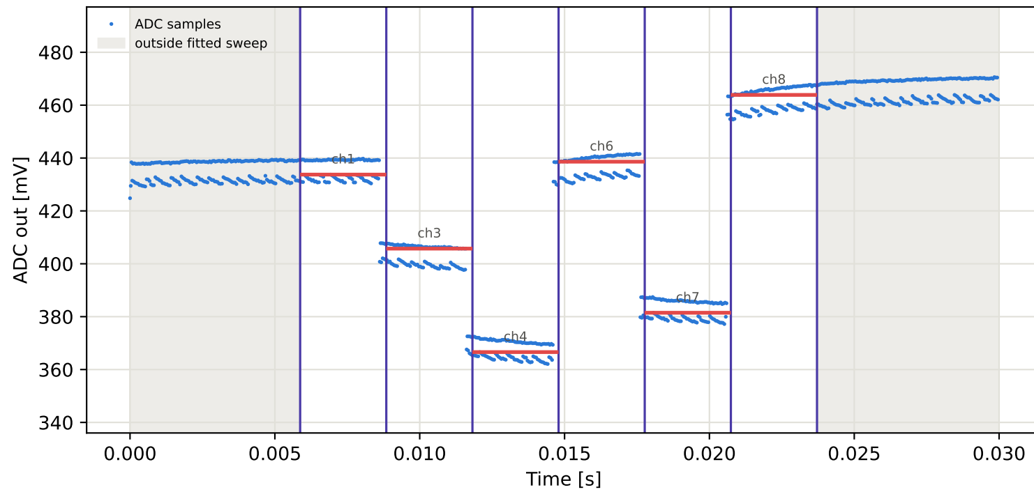
Tag8 &lt;- Tag1 | 925 MHz | run 0 | rep 1 | phase 28.06 deg
