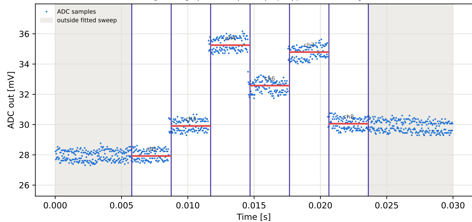
Tag2 &lt;- Tag8 | 805 MHz | run 0 | rep 1 | phase 156.56 deg
