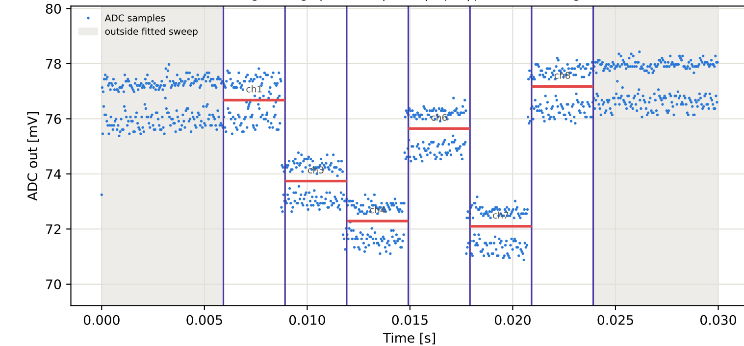
Tag1 &lt;- Tag9 | 805 MHz | run 0 | rep 1 | phase 132.85 deg
