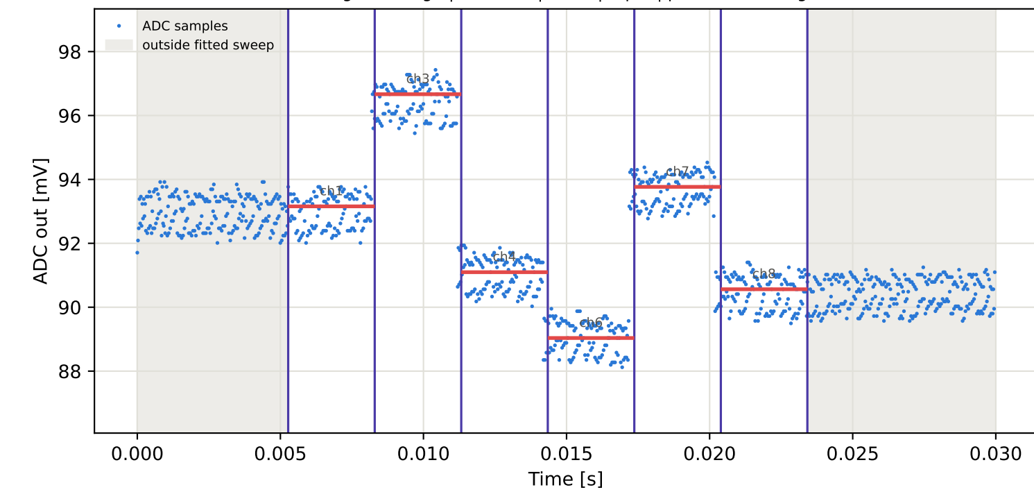
Tag10 &lt;- Tag1 | 825 MHz | run 0 | rep 1 | phase 27.86 deg
