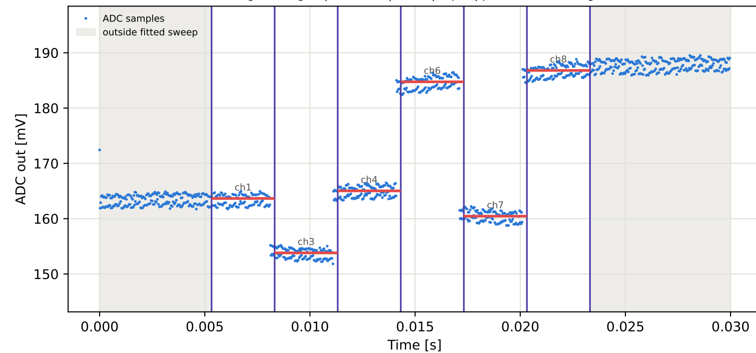
Tag9 &lt;- Tag16 | 865 MHz | run 0 | rep 1 | phase 1.96 deg
