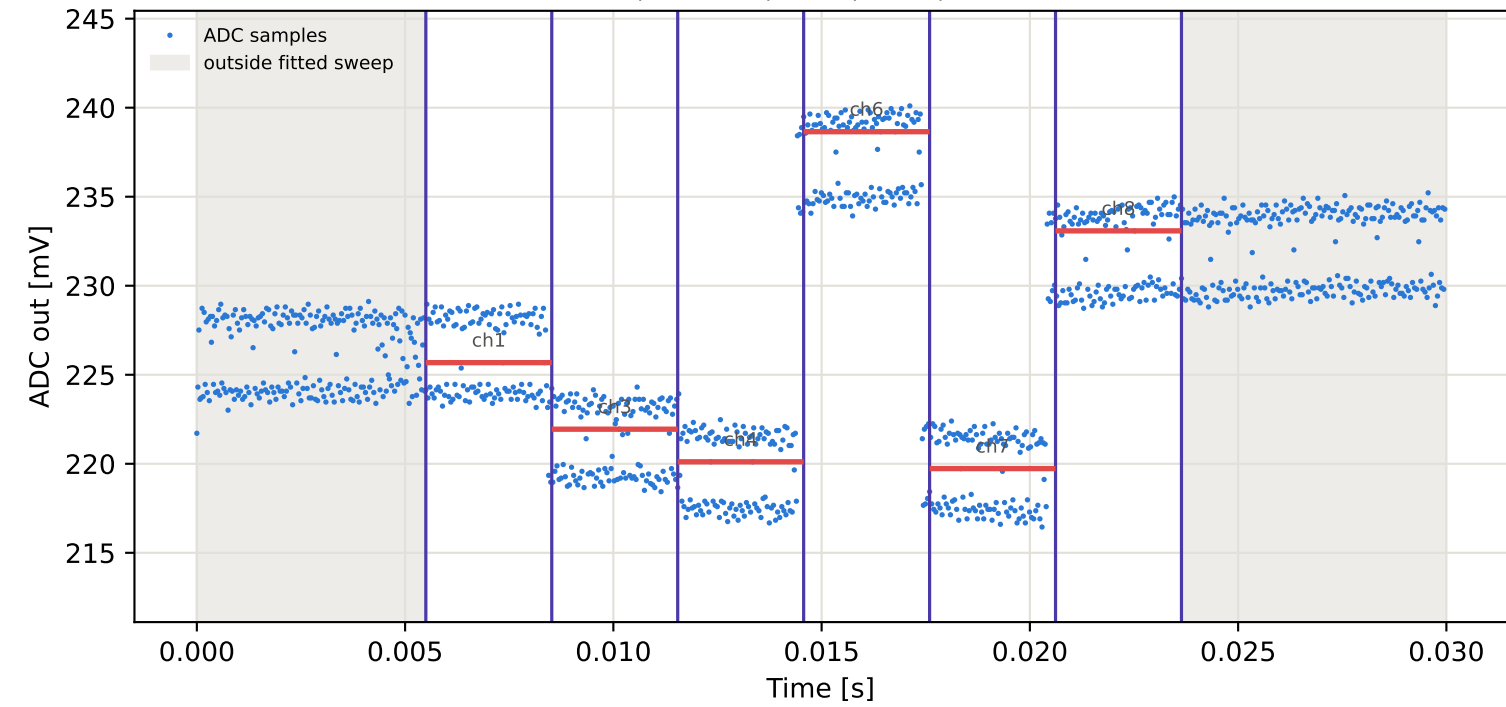
Tag1 &lt;- Tag4 | 985 MHz | run 0 | rep 1 | phase 155.97 deg
