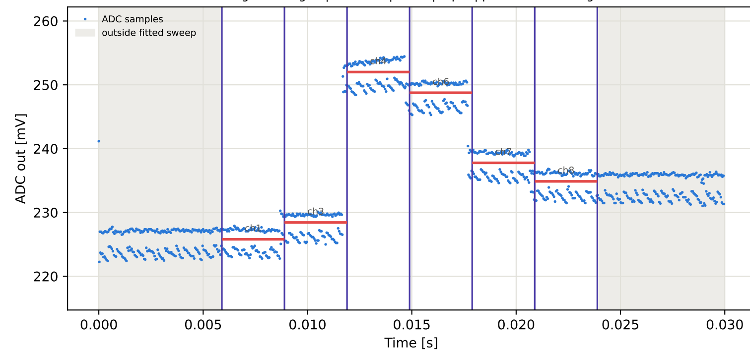
Tag15 &lt;- Tag3 | 985 MHz | run 0 | rep 1 | phase 68.16 deg
