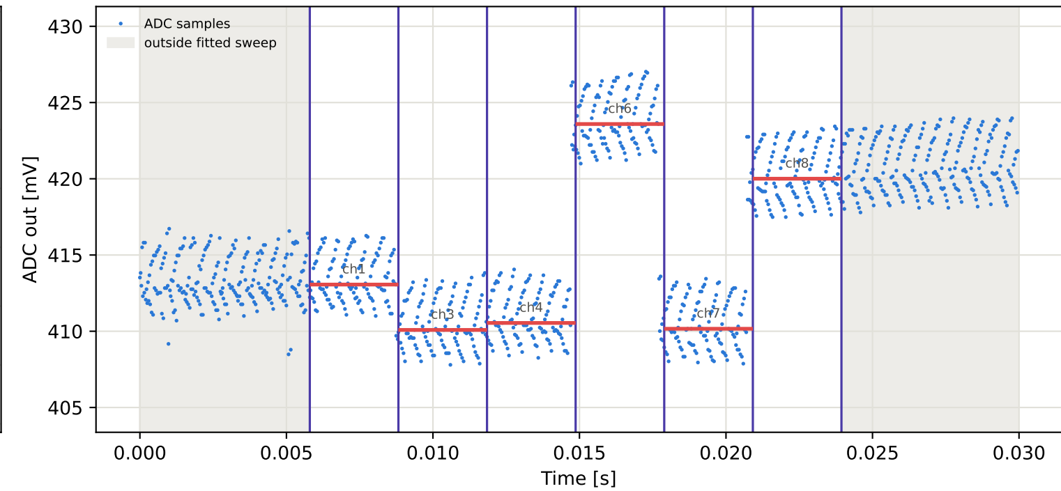
Tag7 &lt;- Tag15 | 925 MHz | run 0 | rep 1 | phase 159.28 deg
