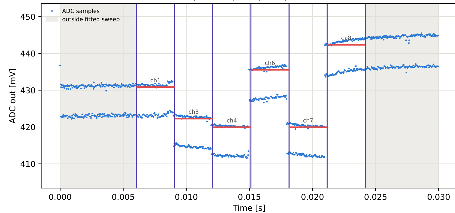
Tag3 &lt;- Tag10 | 905 MHz | run 0 | rep 1 | phase -122.64 deg
