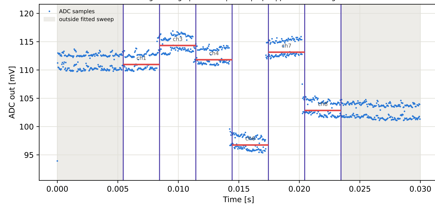
Tag6 &lt;- Tag4 | 915 MHz | run 0 | rep 1 | phase -0.15 deg
