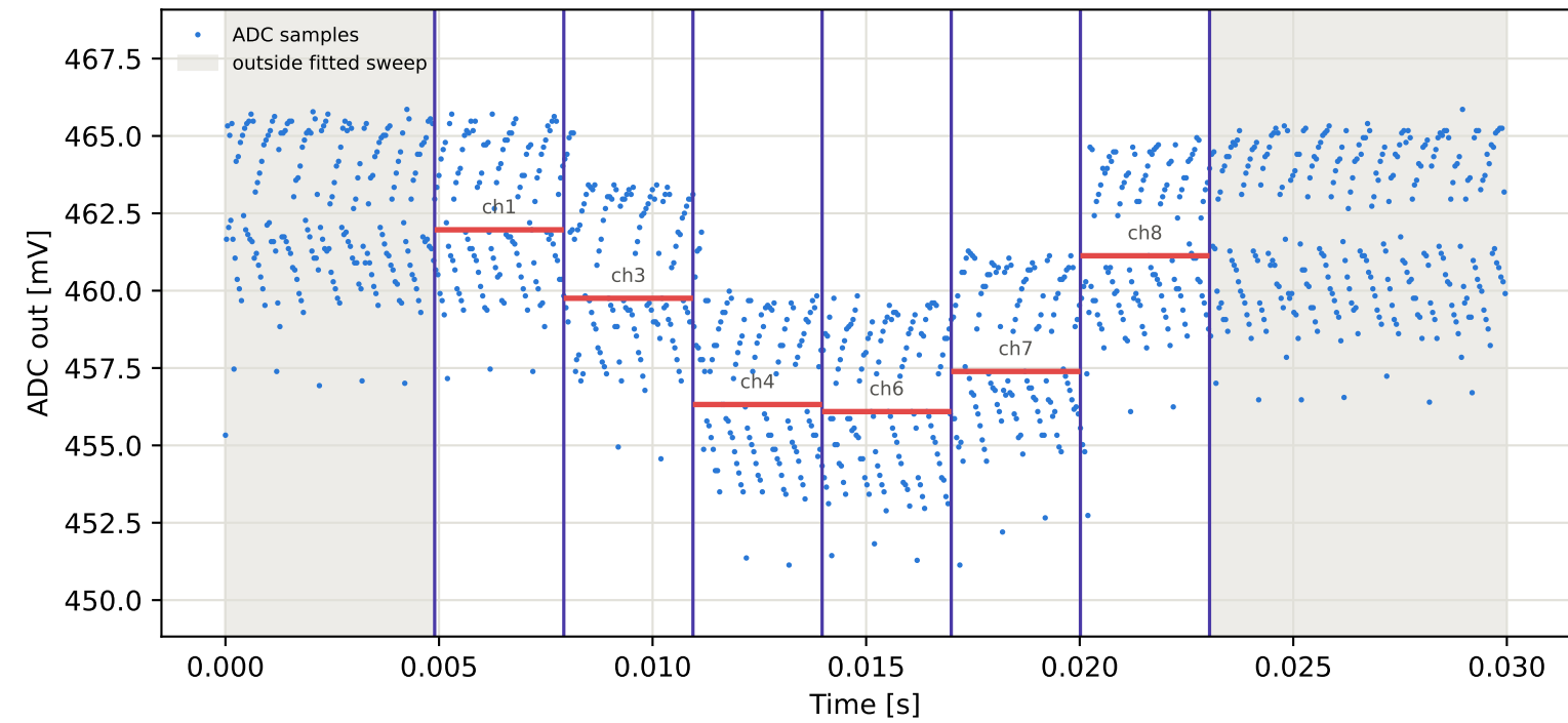
Tag7 &lt;- Tag15 | 915 MHz | run 0 | rep 1 | phase 135.82 deg
