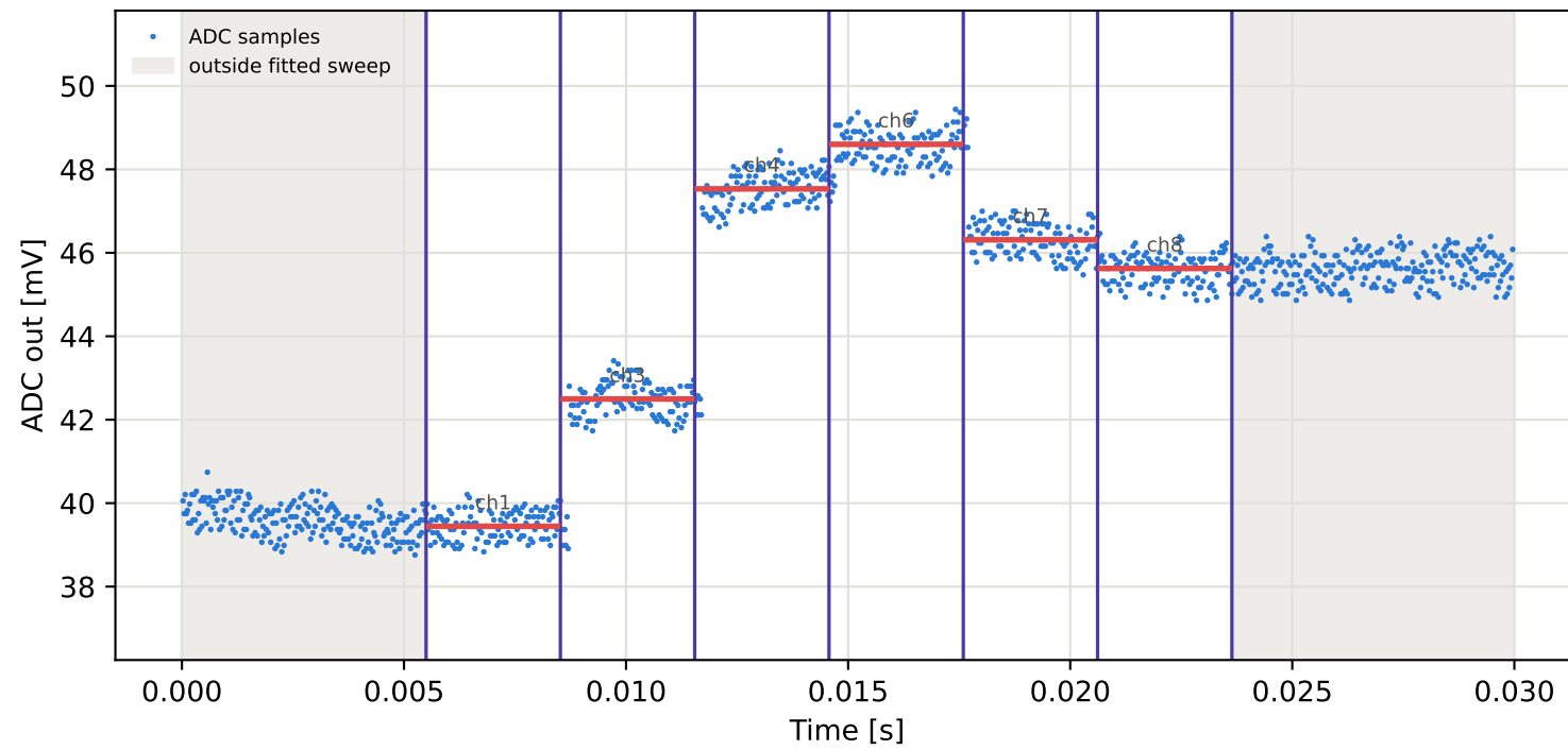
Tag1 &lt;- Tag7 | 855 MHz | run 0 | rep 1 | phase 128.69 deg
