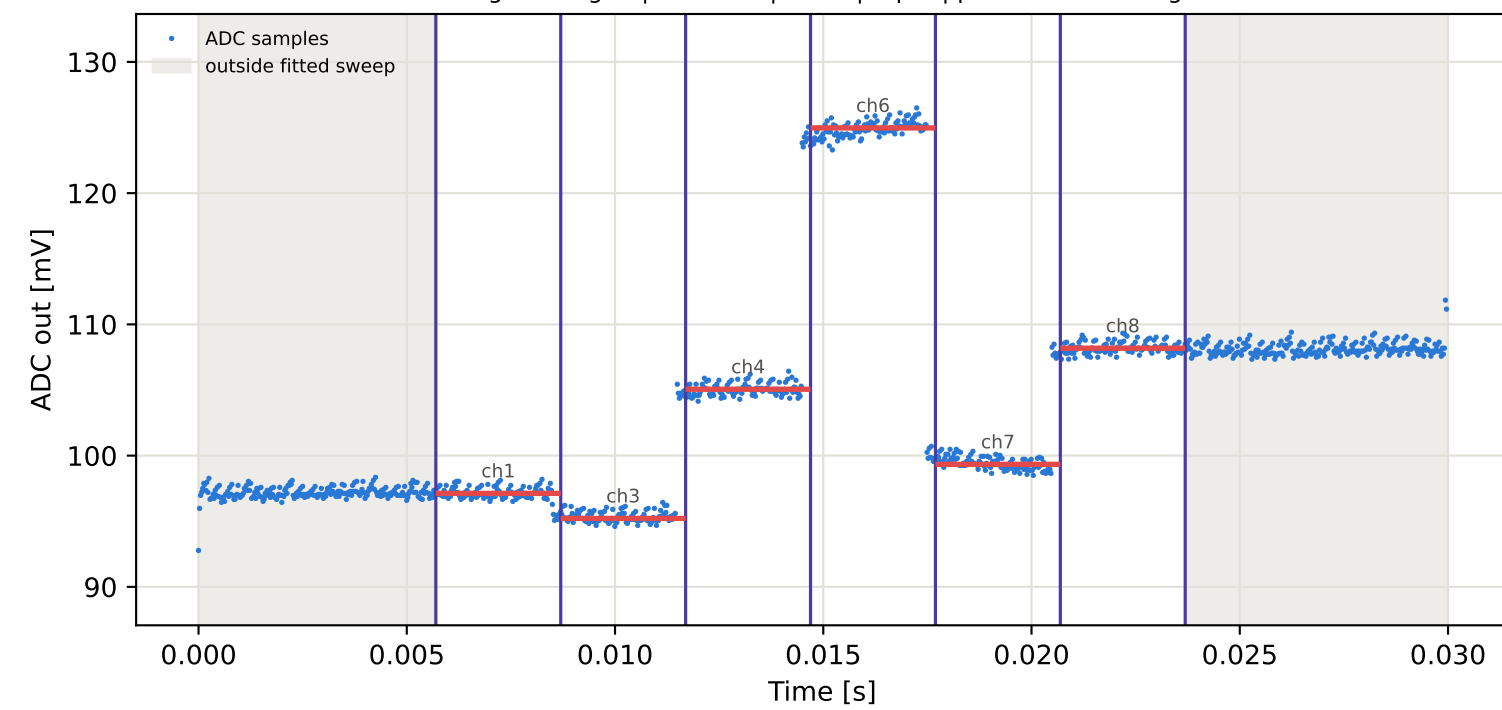
Tag1 &lt;- Tag16 | 945 MHz | run 0 | rep 1 | phase -101.00 deg
