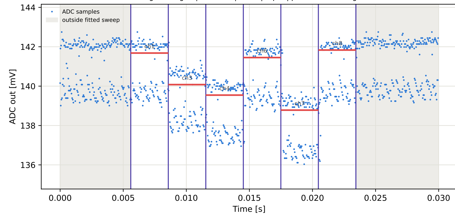
Tag5 &lt;- Tag16 | 785 MHz | run 0 | rep 1 | phase -88.62 deg
