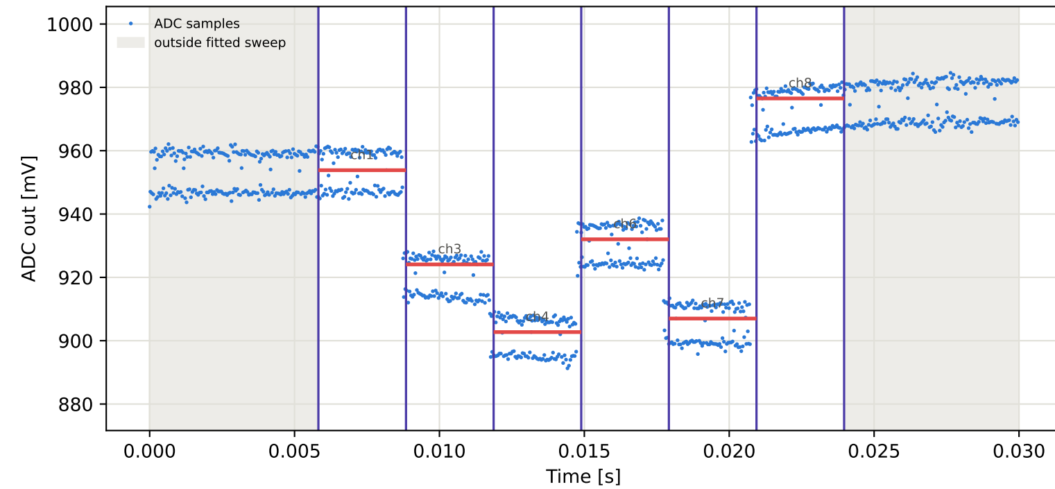
Tag15 &lt;- Tag5 | 885 MHz | run 0 | rep 1 | phase 24.50 deg
