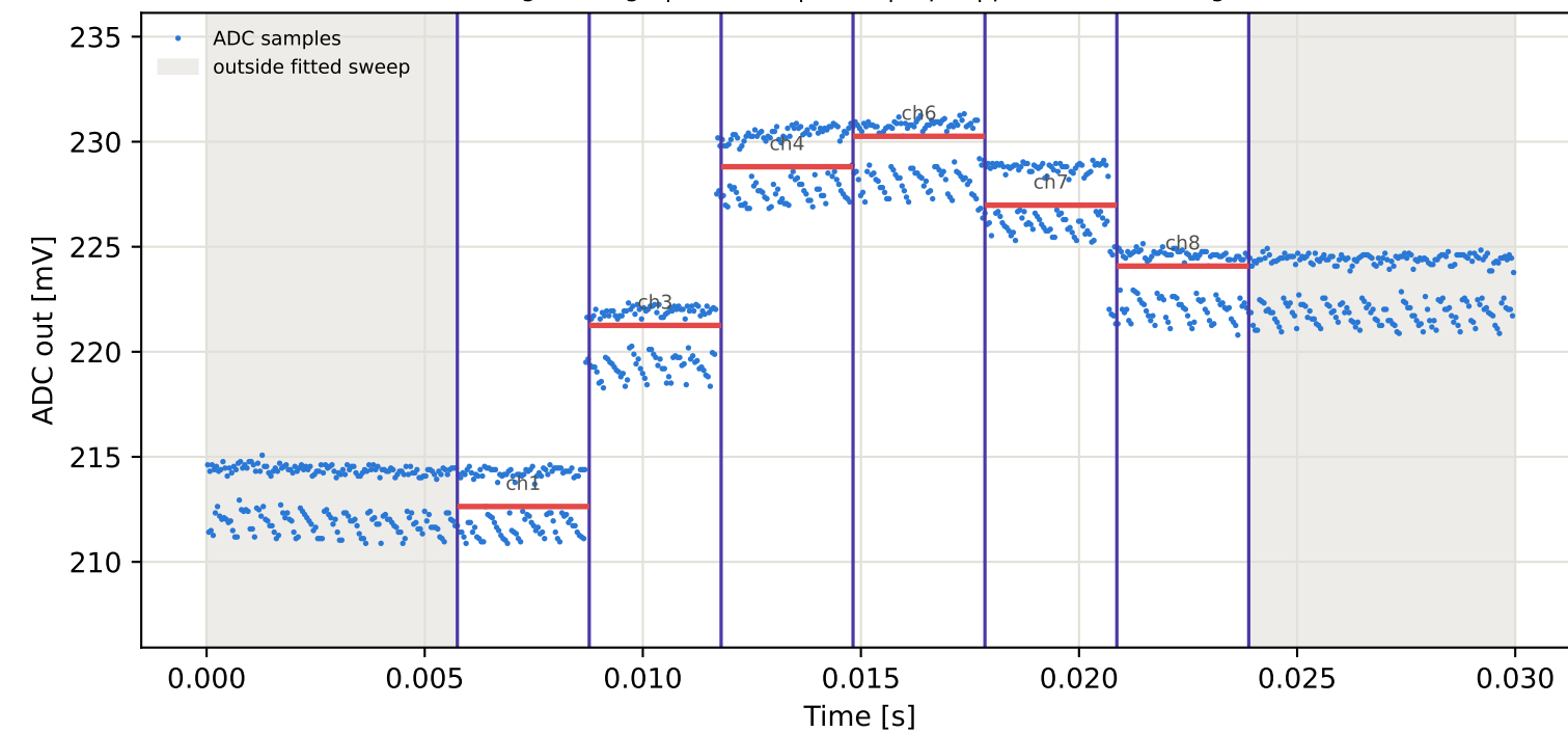
Tag2 &lt;- Tag7 | 855 MHz | run 0 | rep 1 | phase -39.46 deg
