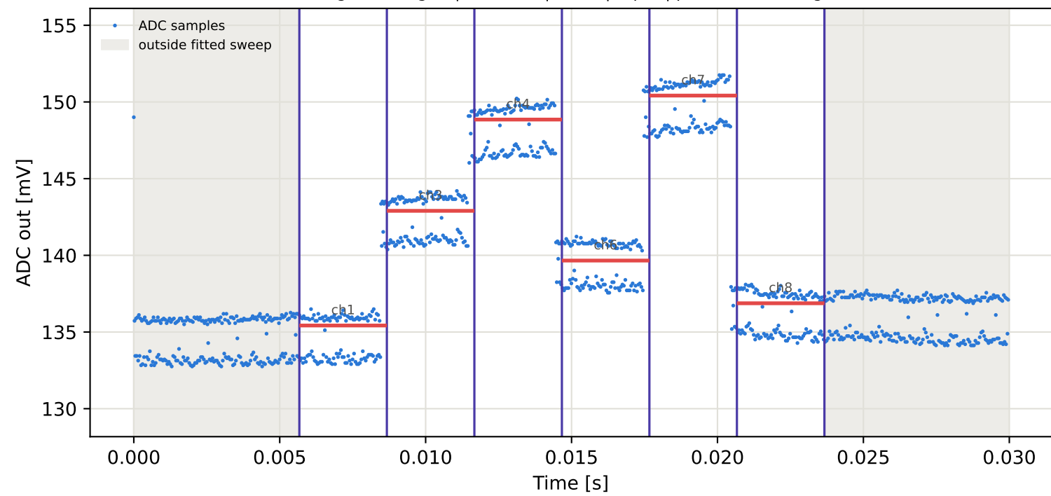
Tag15 &lt;- Tag3 | 805 MHz | run 0 | rep 1 | phase -87.08 deg
