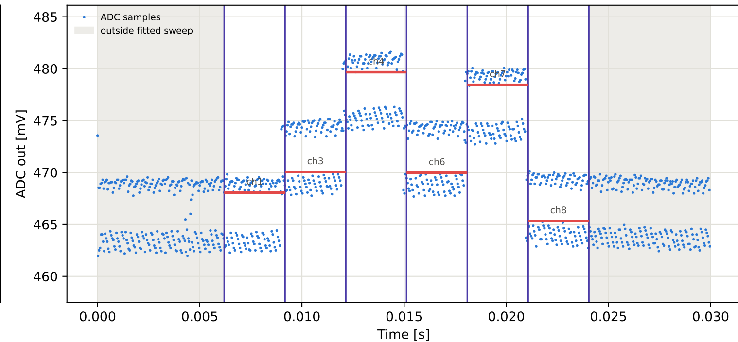
Tag3 &lt;- Tag2 | 845 MHz | run 0 | rep 1 | phase -80.94 deg
