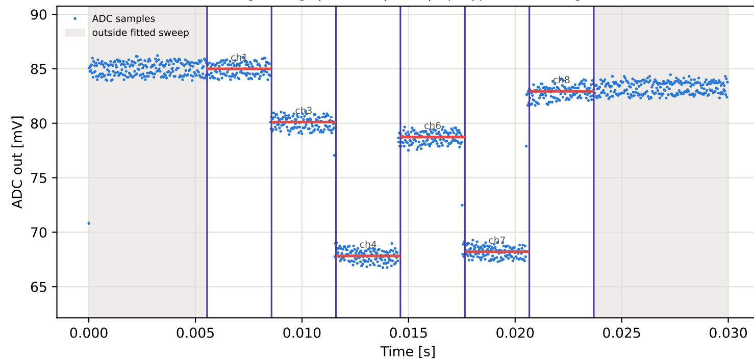
Tag4 &lt;- Tag7 | 785 MHz | run 0 | rep 1 | phase 86.40 deg
