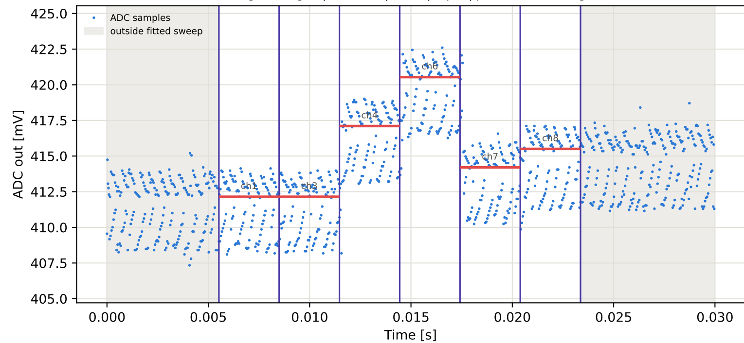
Tag4 &lt;- Tag16 | 965 MHz | run 0 | rep 1 | phase 85.16 deg
