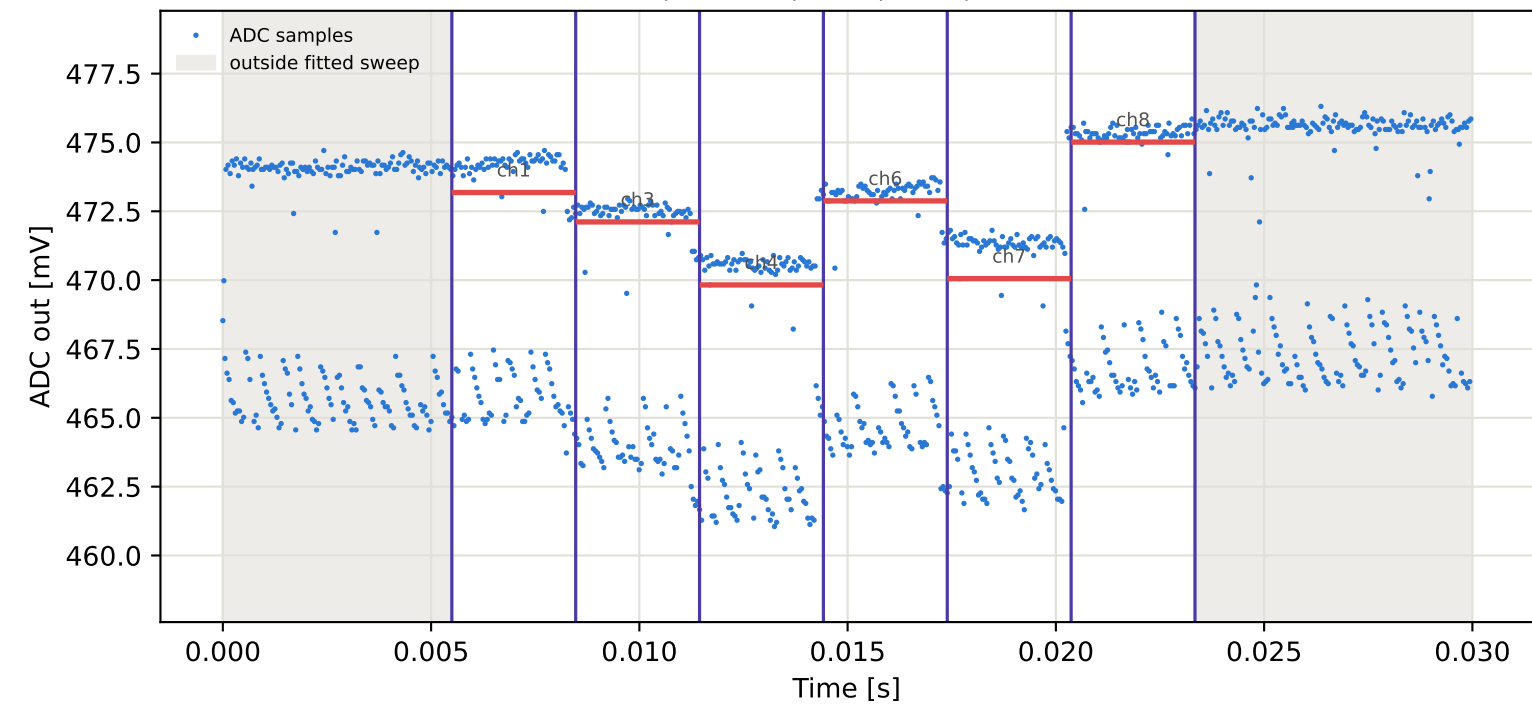
Tag5 &lt;- Tag1 | 915 MHz | run 0 | rep 1 | phase 104.24 deg
