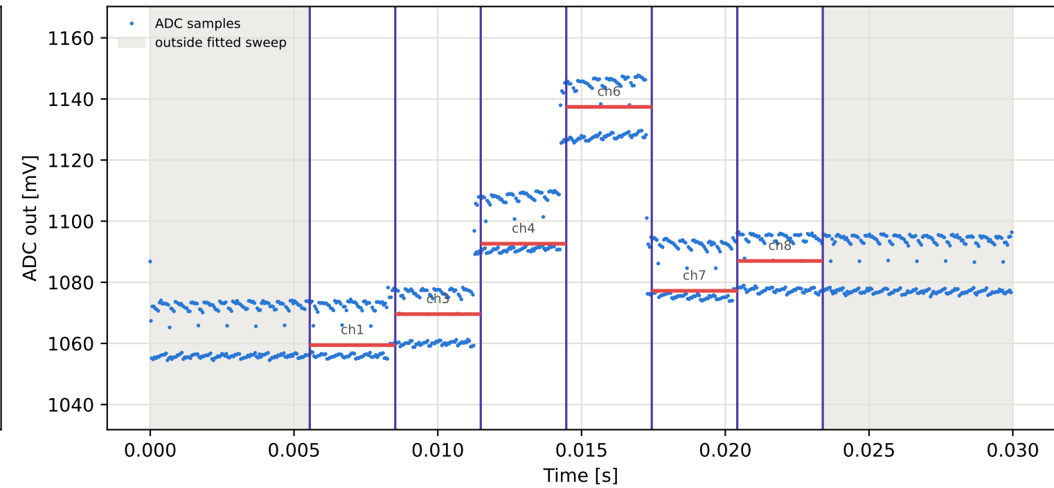
Tag8 &lt;- Tag7 | 935 MHz | run 0 | rep 1 | phase -29.77 deg
