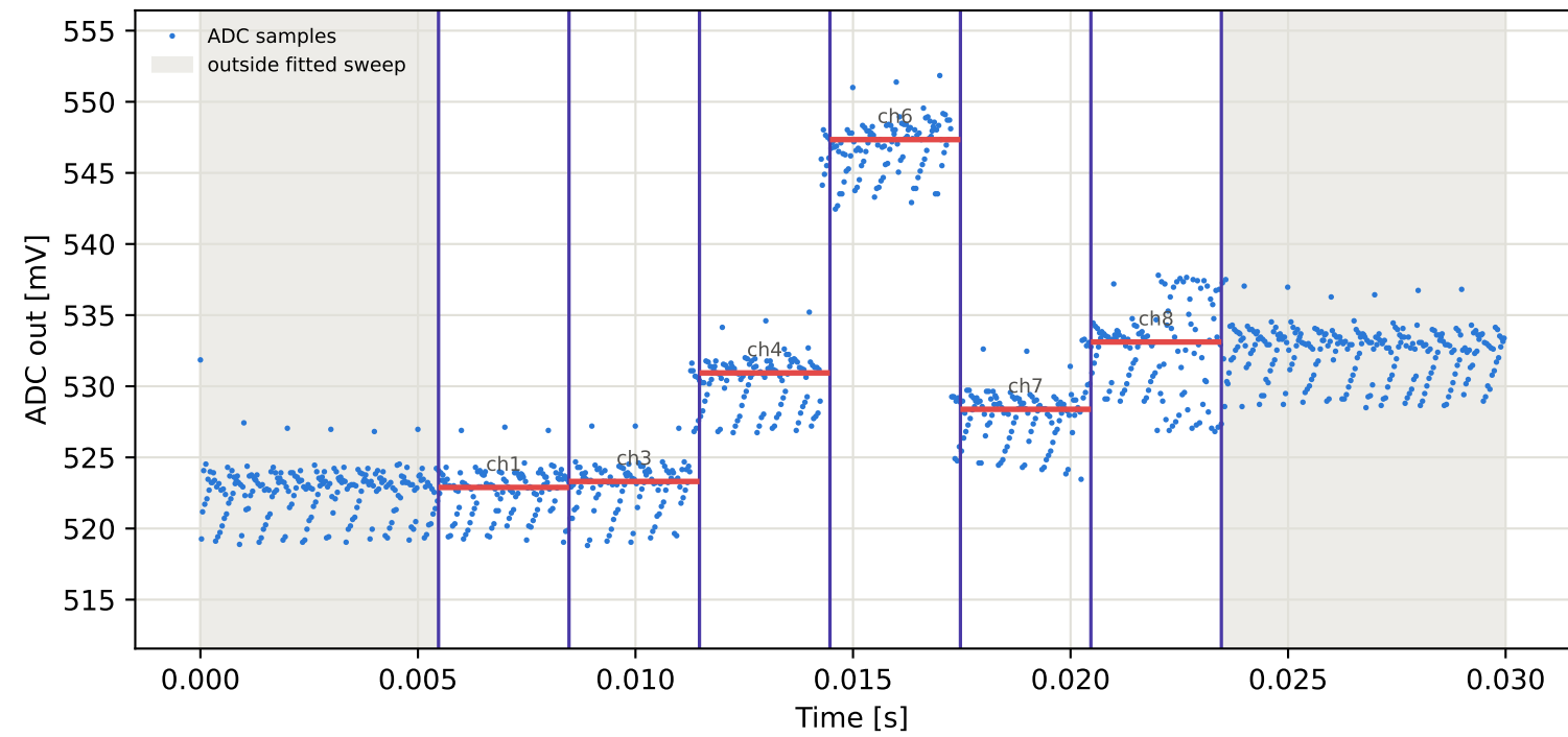
Tag2 &lt;- Tag6 | 915 MHz | run 0 | rep 1 | phase -135.75 deg
