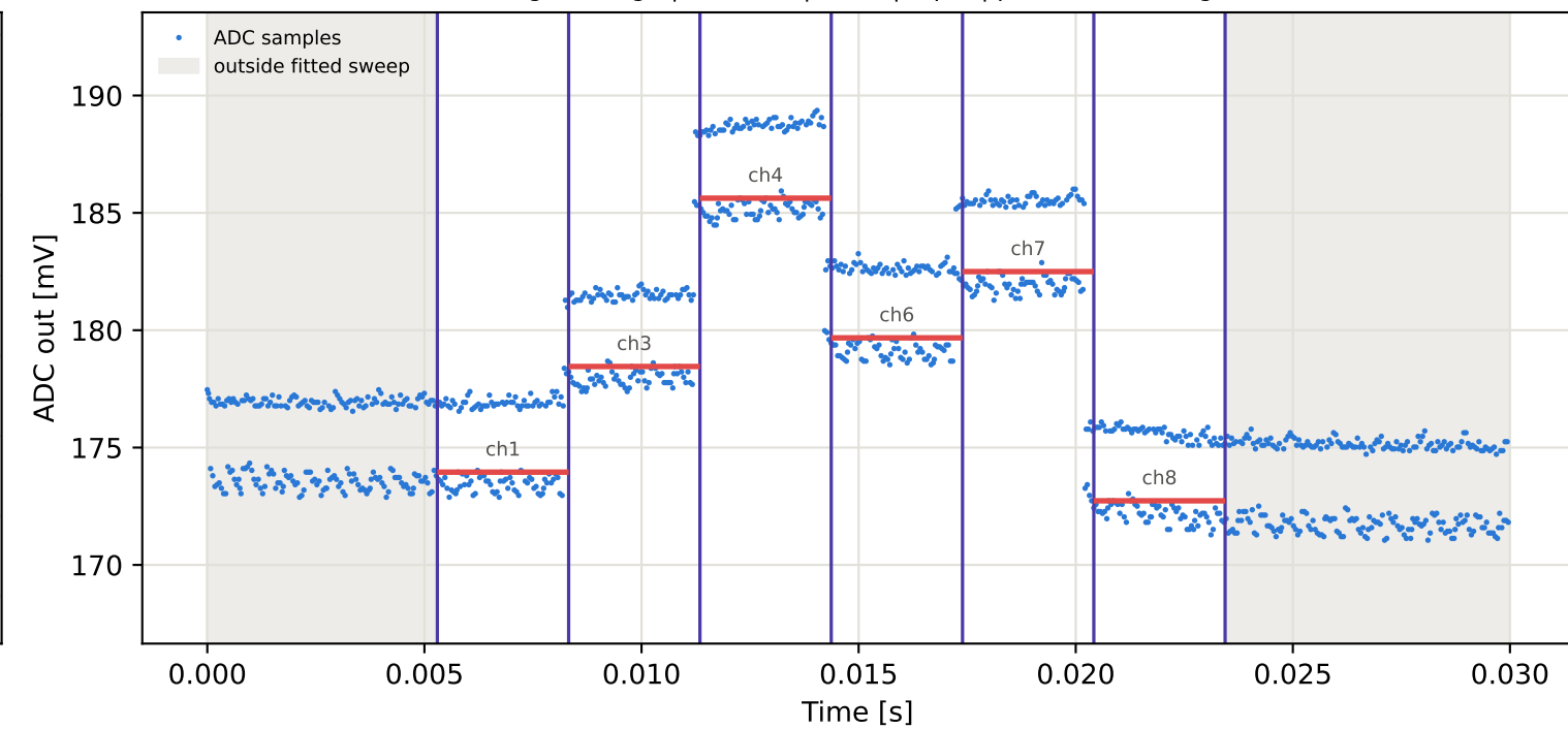
Tag4 &lt;- Tag8 | 925 MHz | run 0 | rep 1 | phase -41.94 deg
