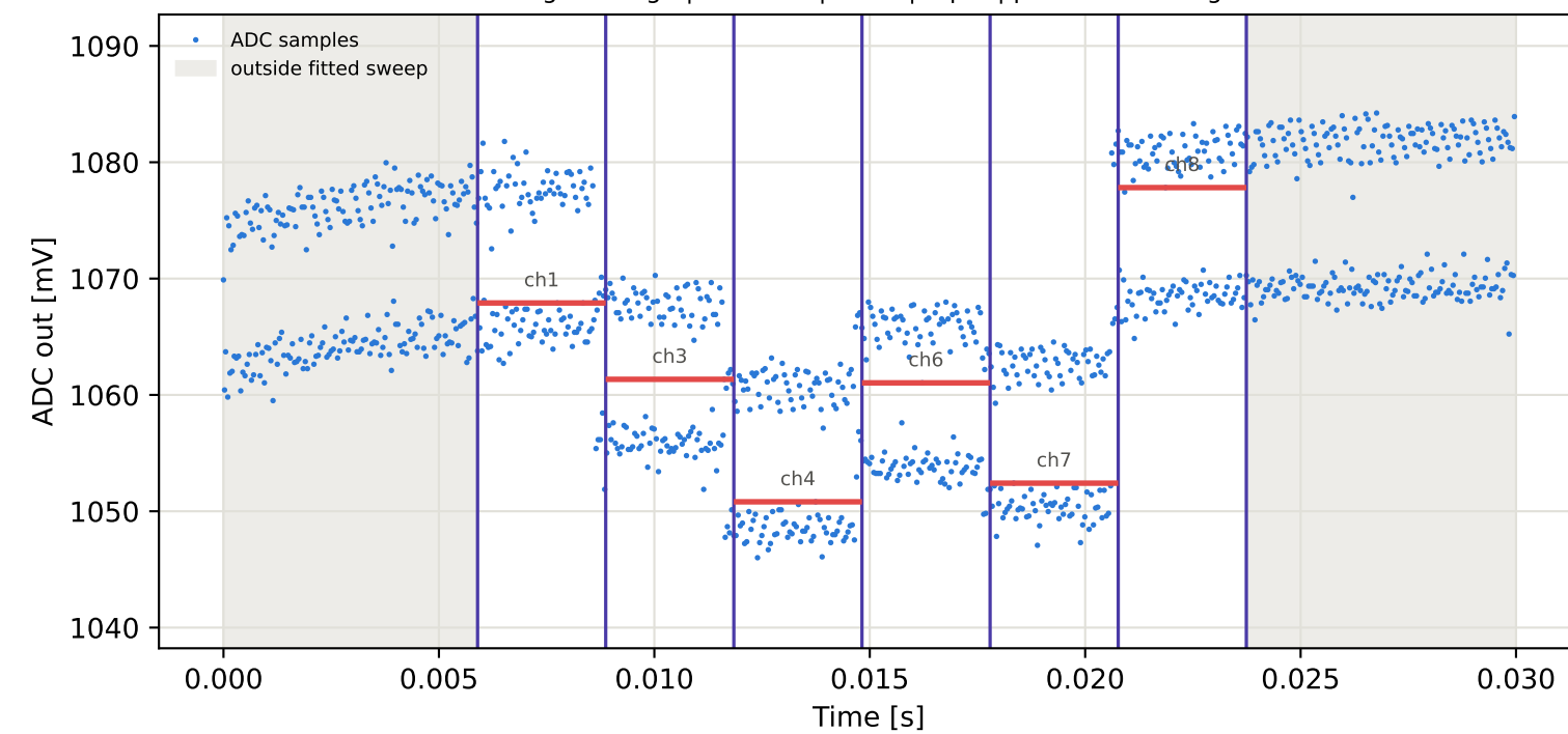
Tag3 &lt;- Tag6 | 885 MHz | run 0 | rep 1 | phase -123.17 deg
