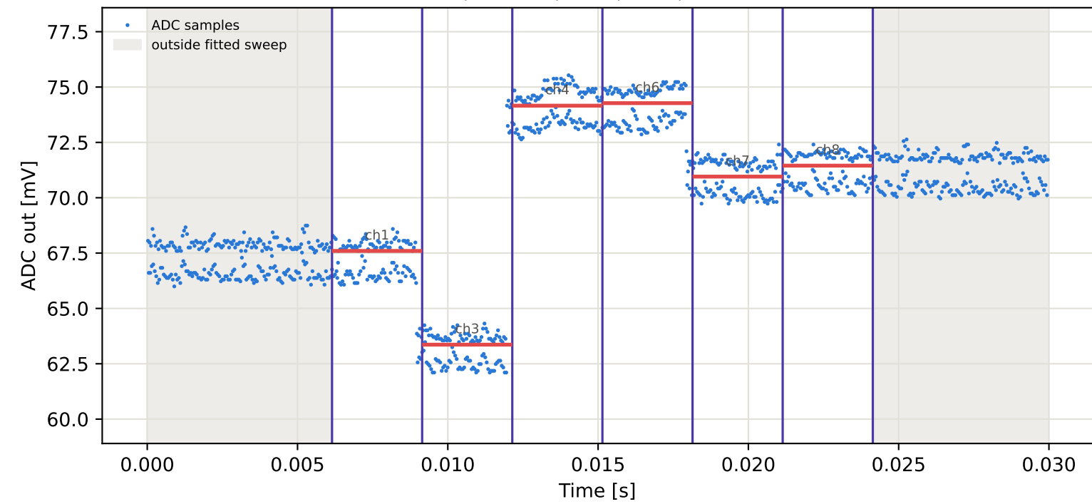
Tag9 &lt;- Tag8 | 795 MHz | run 0 | rep 1 | phase -128.62 deg
