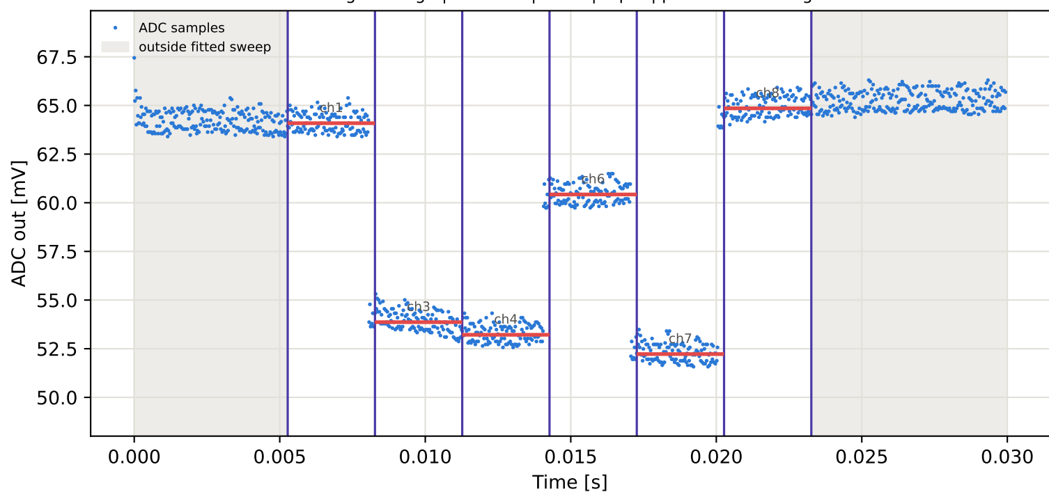
Tag10 &lt;- Tag1 | 845 MHz | run 0 | rep 1 | phase 86.13 deg
