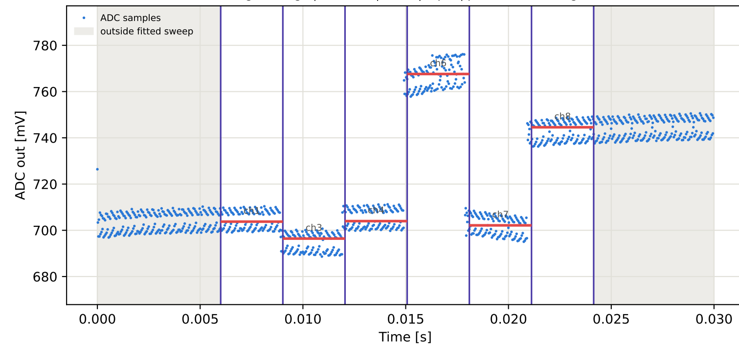
Tag3 &lt;- Tag6 | 905 MHz | run 0 | rep 1 | phase -88.16 deg
