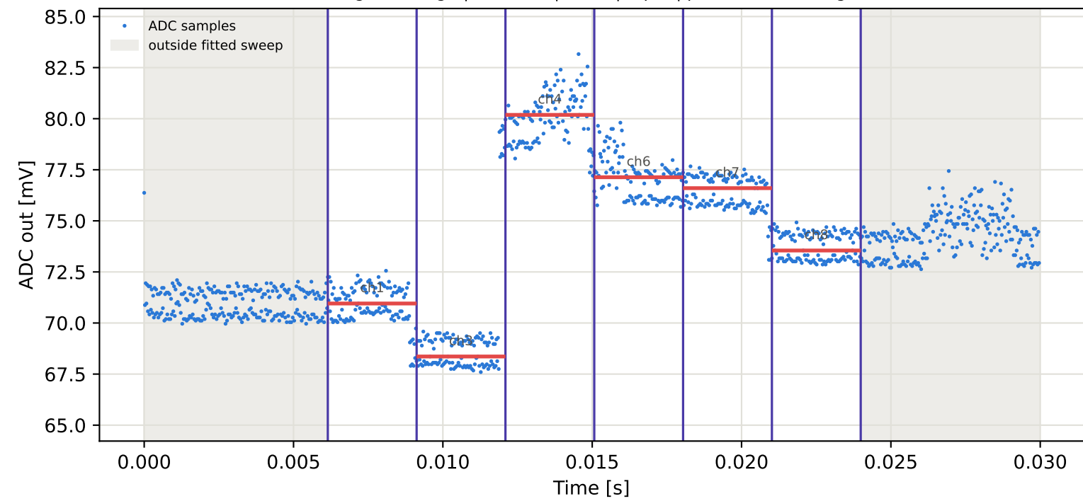
Tag16 &lt;- Tag1 | 775 MHz | run 0 | rep 1 | phase -110.87 deg
