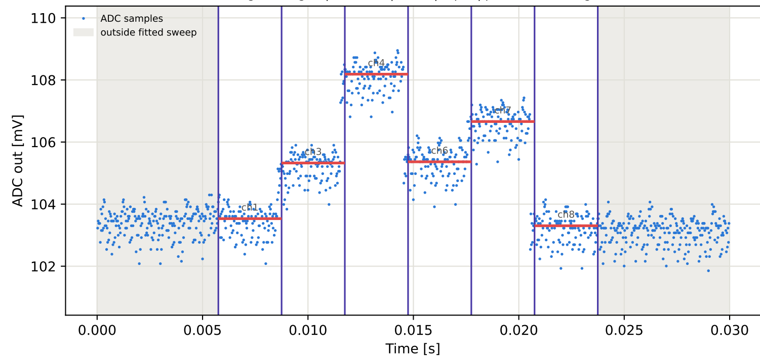
Tag1 &lt;- Tag2 | 965 MHz | run 0 | rep 1 | phase -94.51 deg
