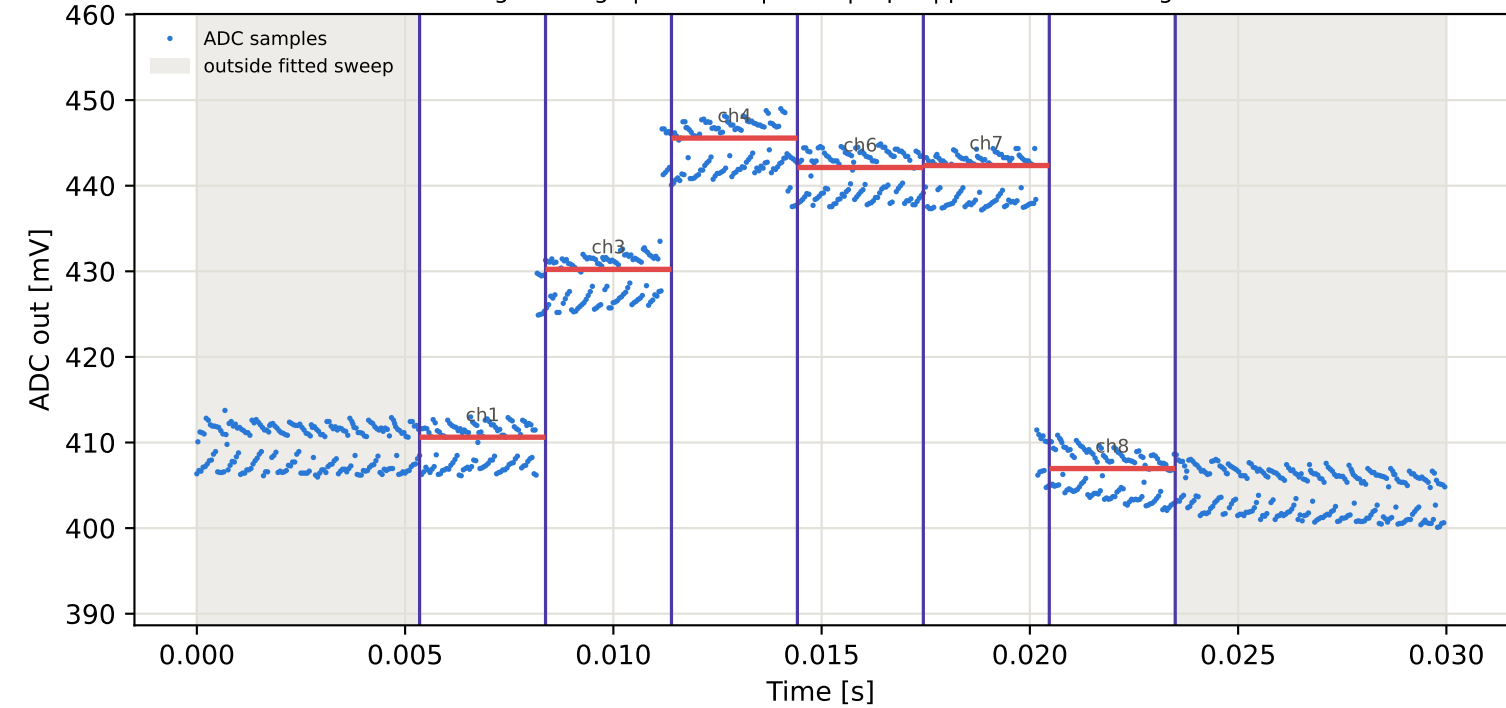
Tag7 &lt;- Tag1 | 895 MHz | run 0 | rep 1 | phase 86.57 deg
