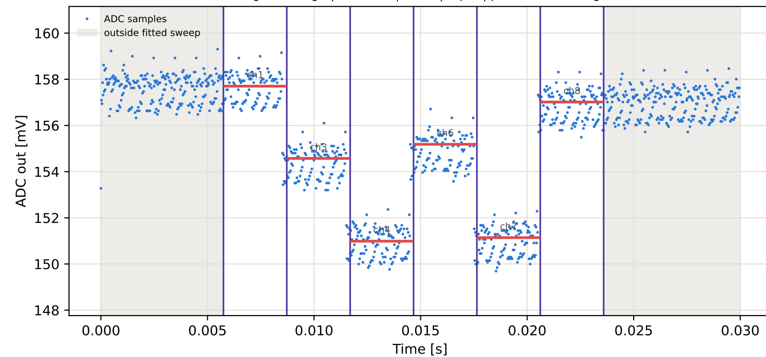
Tag16 &lt;- Tag6 | 805 MHz | run 0 | rep 1 | phase 103.50 deg
