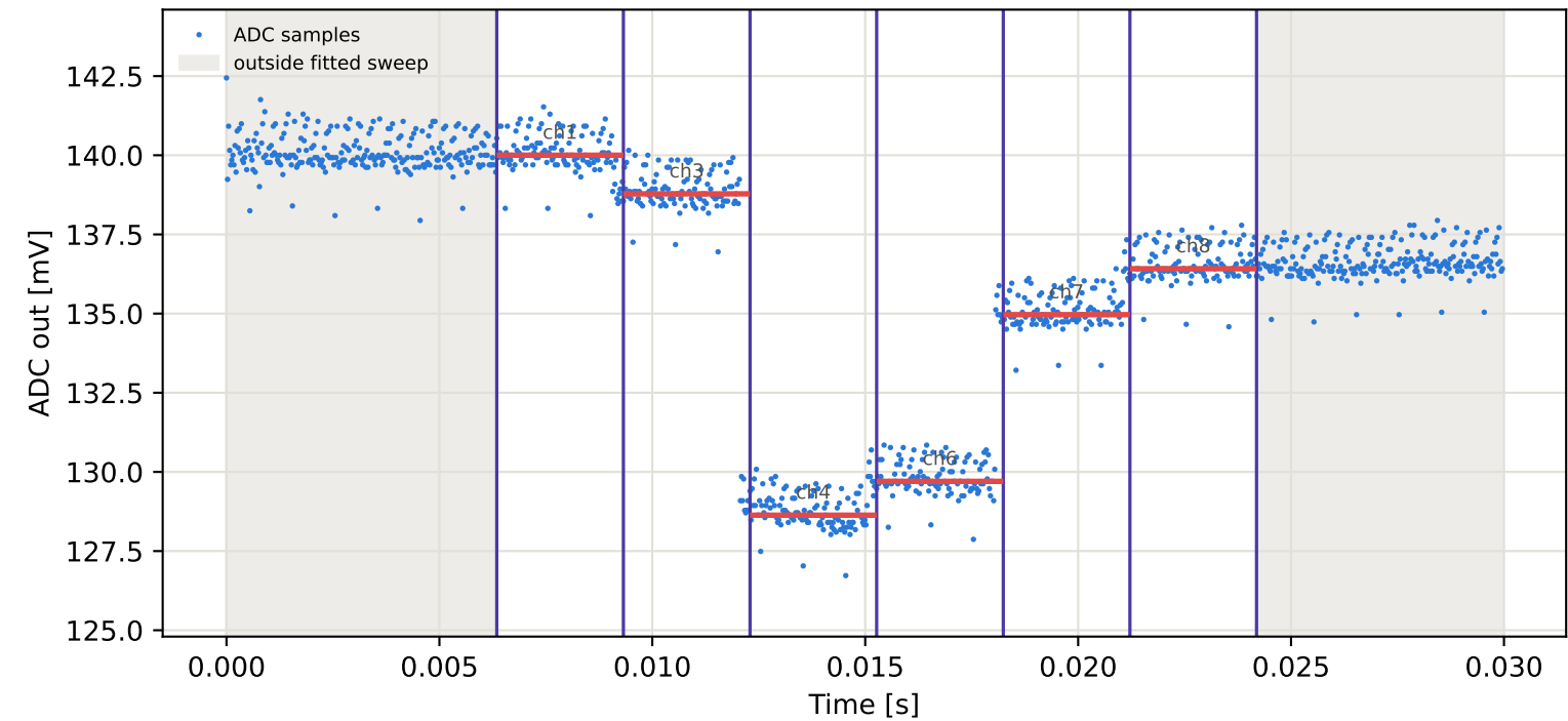
Tag3 &lt;- Tag2 | 995 MHz | run 0 | rep 1 | phase -133.04 deg
