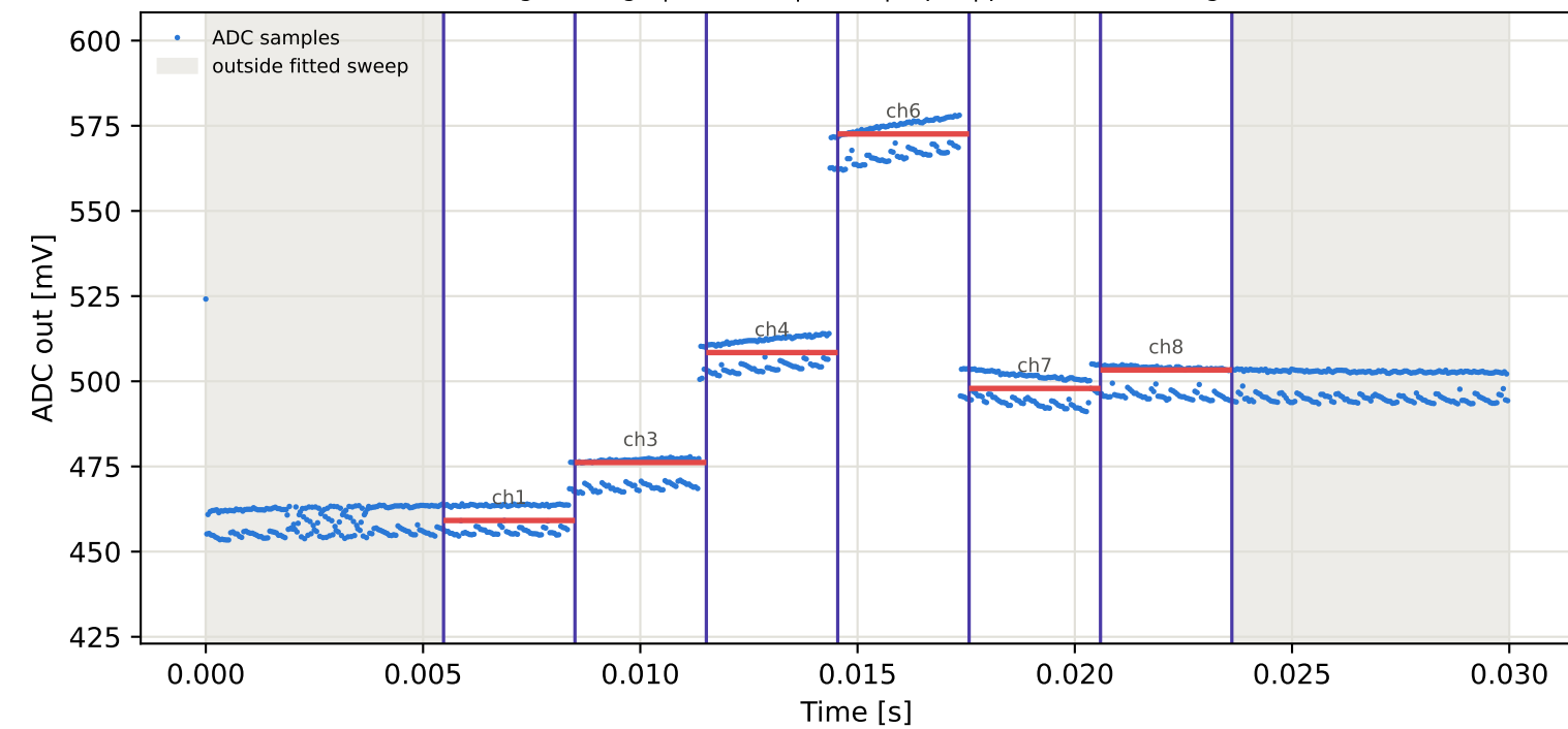
Tag4 &lt;- Tag7 | 905 MHz | run 0 | rep 1 | phase -157.32 deg
