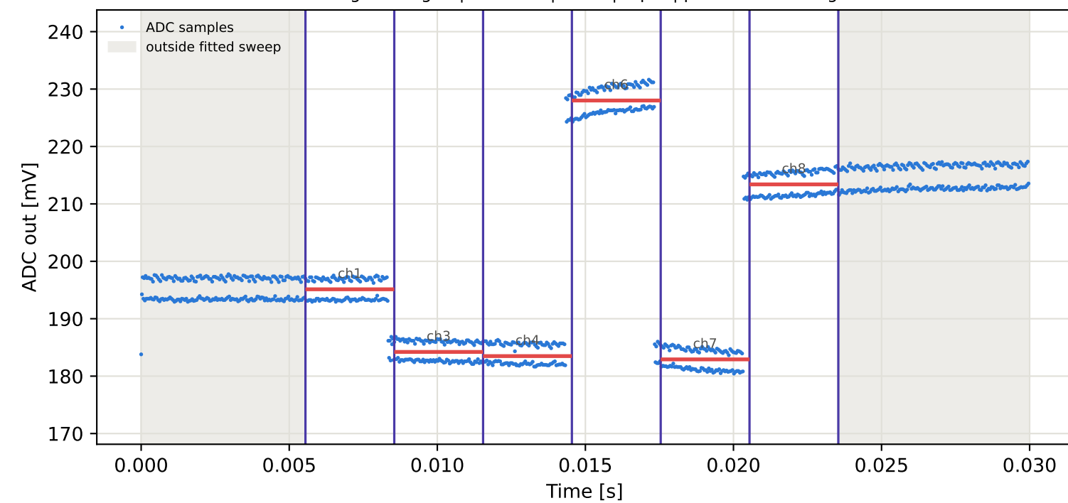
Tag1 &lt;- Tag16 | 935 MHz | run 0 | rep 1 | phase -104.08 deg
