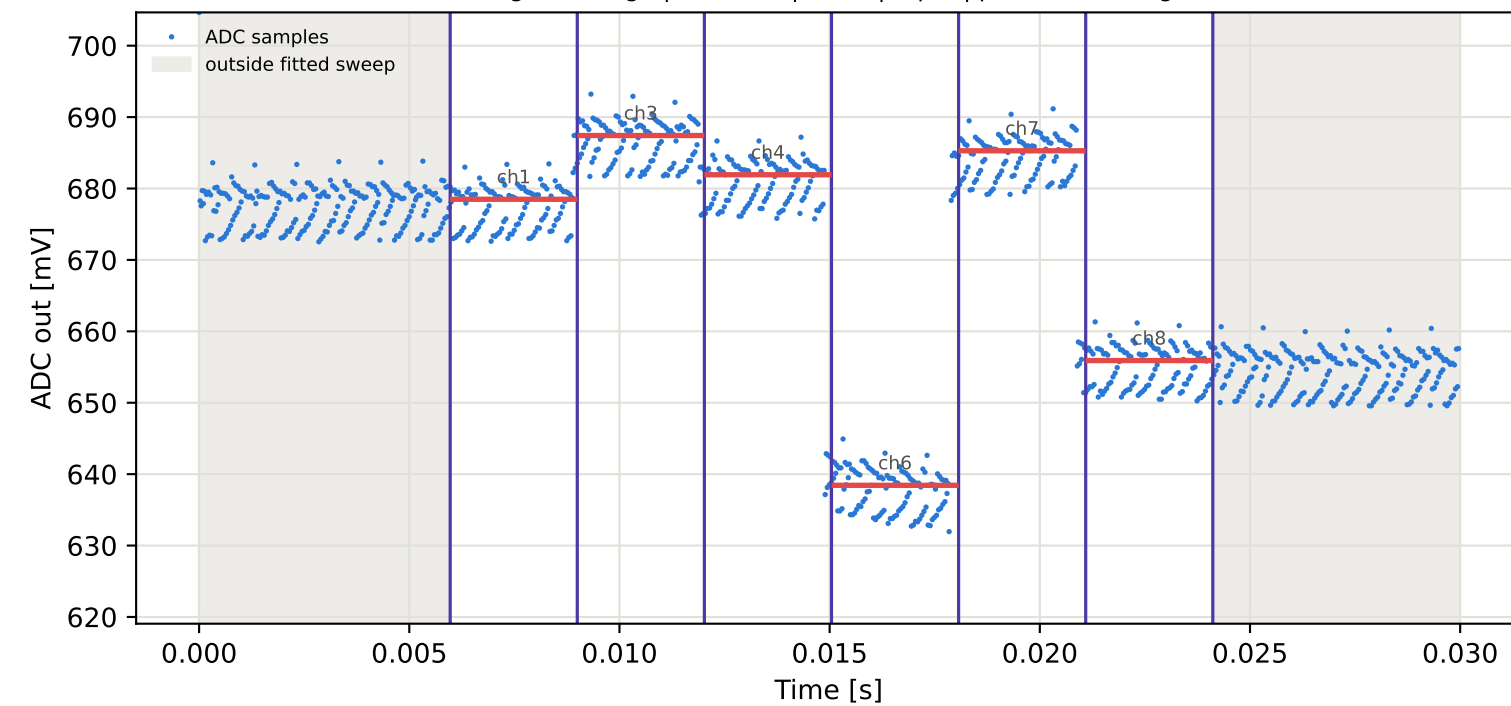
Tag16 &lt;- Tag10 | 935 MHz | run 0 | rep 1 | phase 68.67 deg
