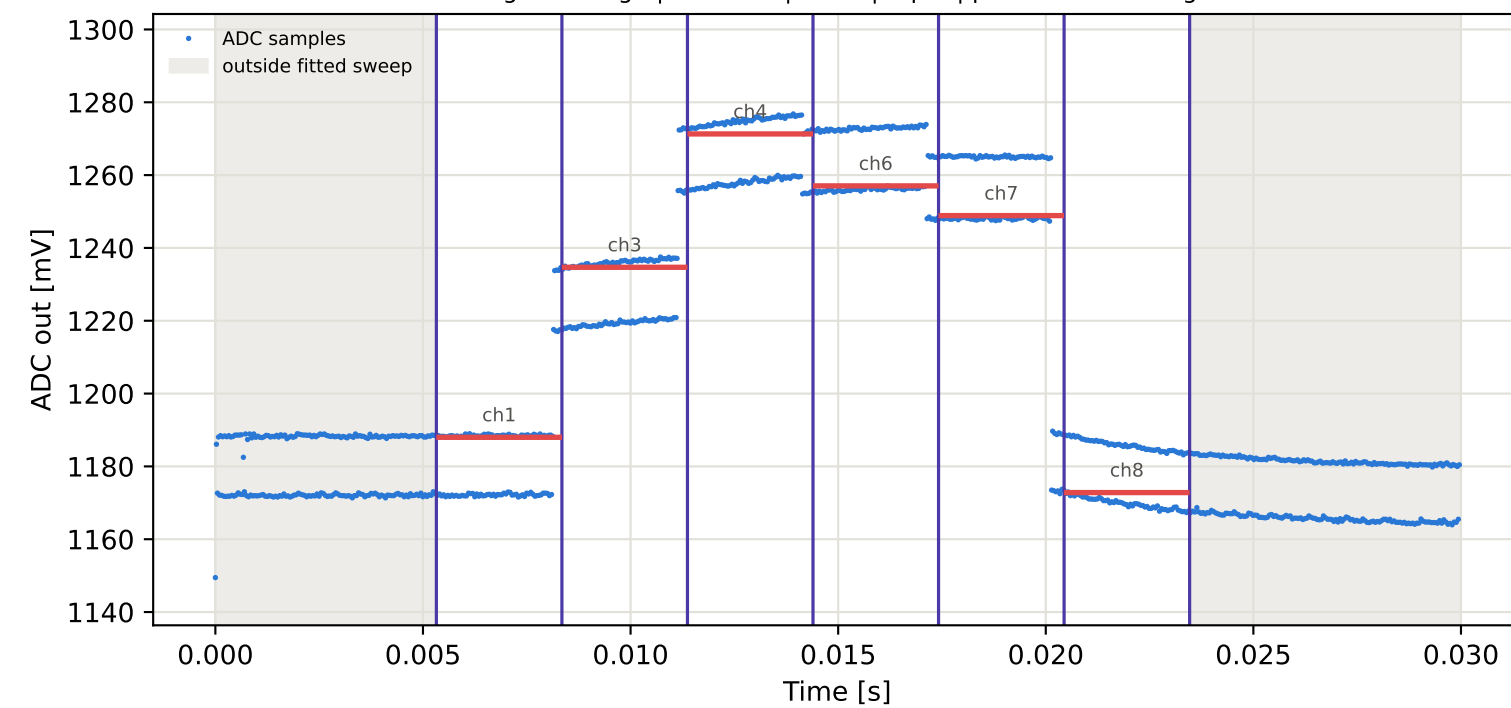
Tag2 &lt;- Tag1 | 895 MHz | run 0 | rep 1 | phase -130.00 deg
