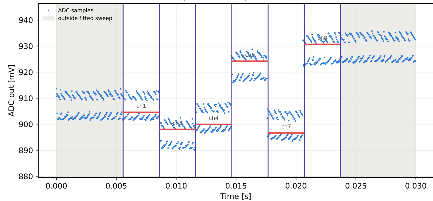
Tag8 &lt;- Tag5 | 865 MHz | run 0 | rep 1 | phase -113.06 deg
