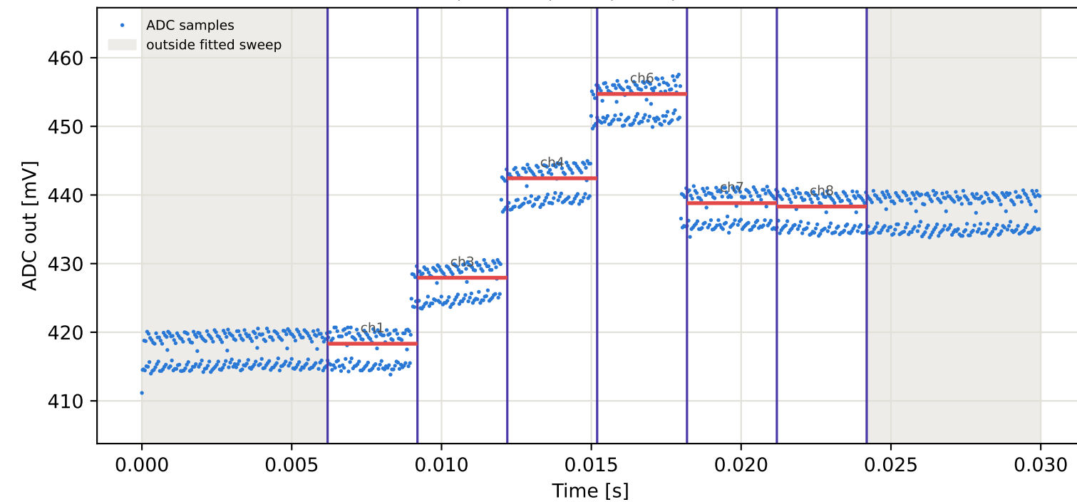
Tag1 &lt;- Tag3 | 875 MHz | run 0 | rep 1 | phase -137.30 deg
