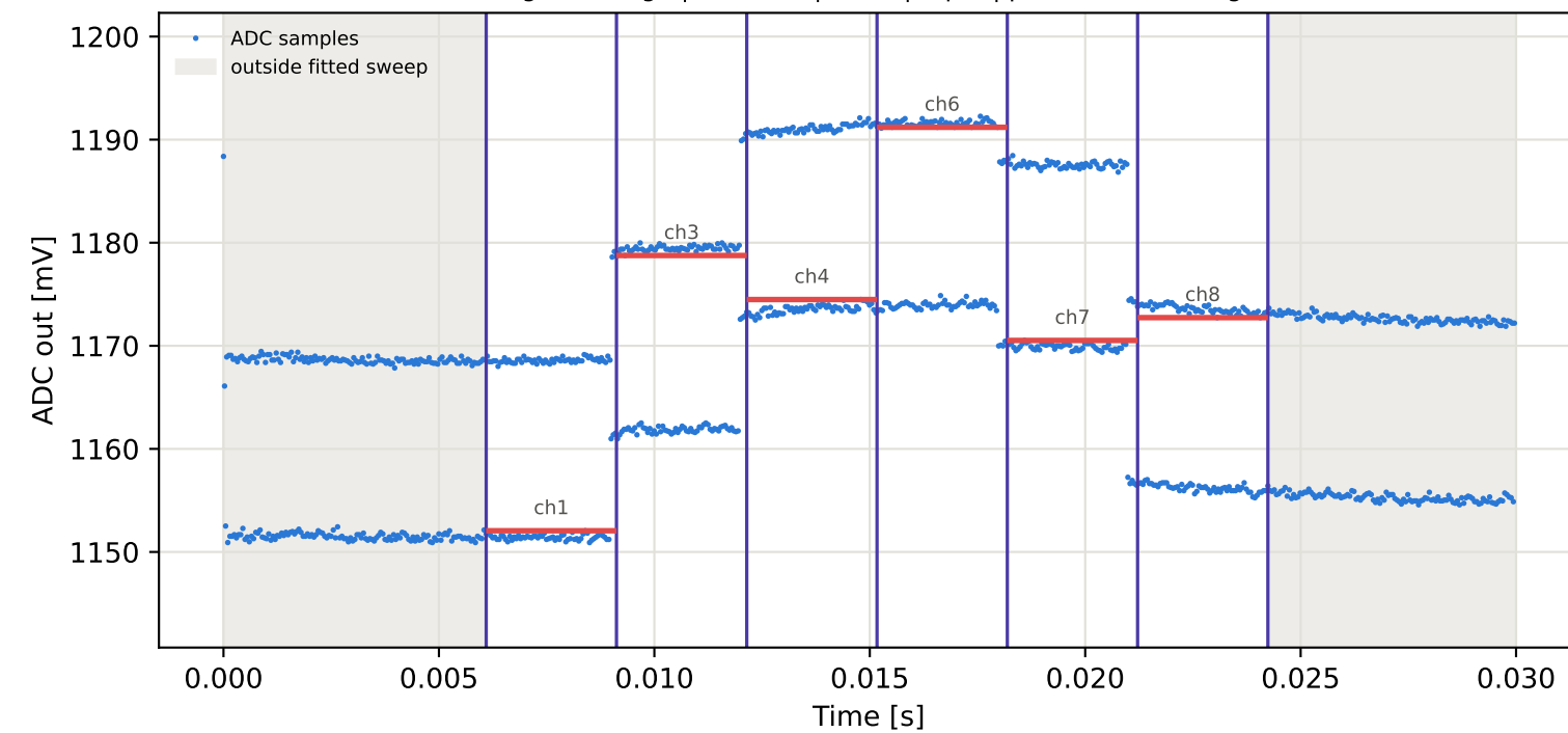
Tag16 &lt;- Tag10 | 905 MHz | run 0 | rep 1 | phase -34.35 deg
