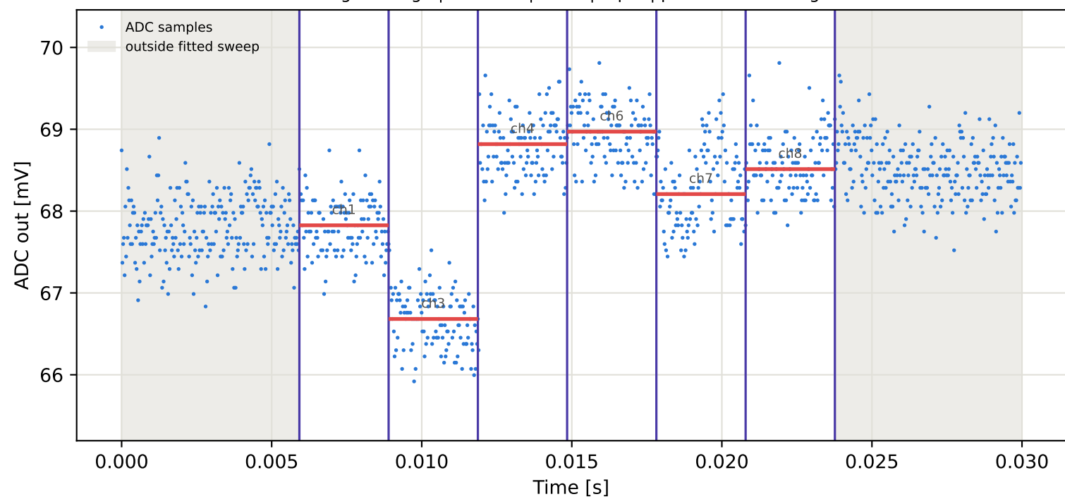
Tag9 &lt;- Tag6 | 785 MHz | run 0 | rep 1 | phase -112.02 deg
