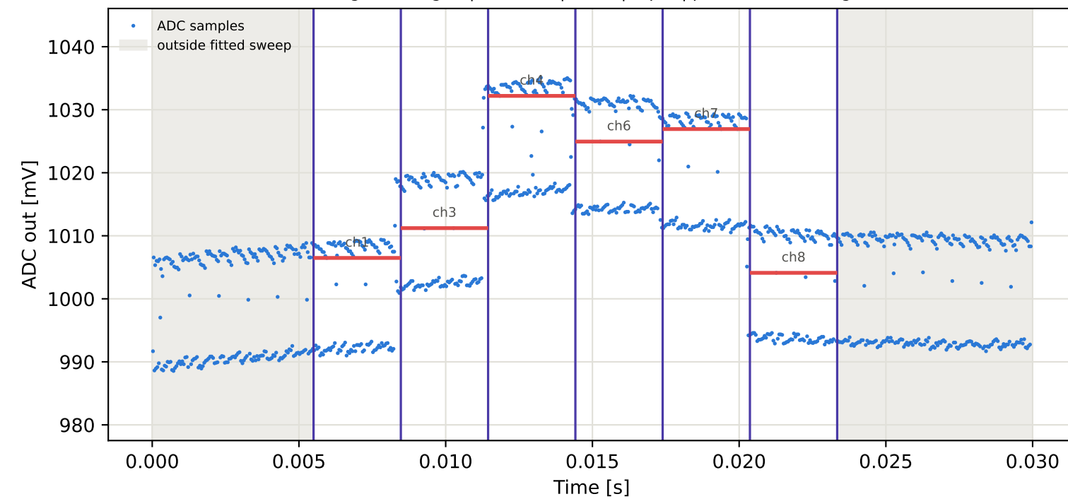
Tag10 &lt;- Tag2 | 925 MHz | run 0 | rep 1 | phase 173.43 deg
