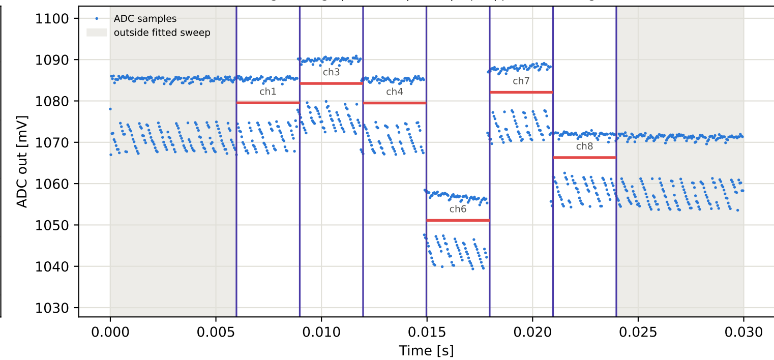
Tag8 &lt;- Tag5 | 935 MHz | run 0 | rep 1 | phase -154.51 deg
