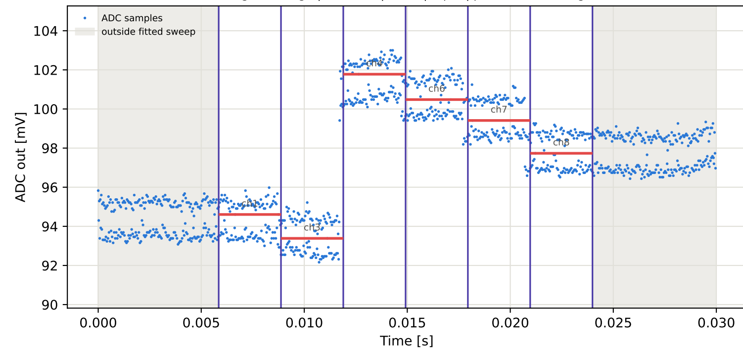
Tag15 &lt;- Tag9 | 785 MHz | run 0 | rep 1 | phase -113.91 deg
