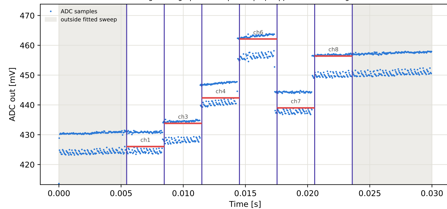
Tag1 &lt;- Tag7 | 875 MHz | run 0 | rep 1 | phase -151.59 deg
