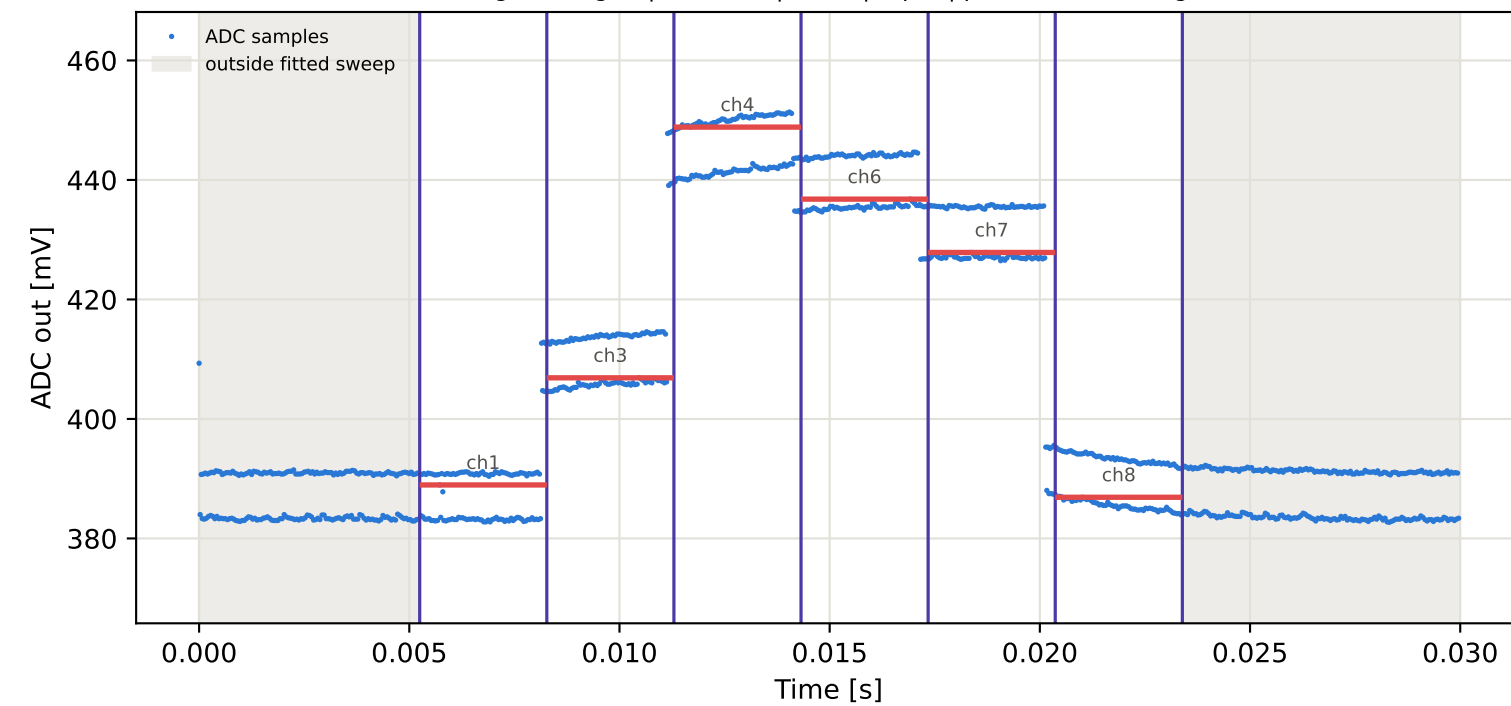
Tag7 &lt;- Tag3 | 925 MHz | run 0 | rep 1 | phase 70.42 deg
