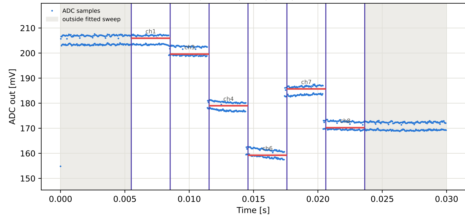
Tag9 &lt;- Tag8 | 865 MHz | run 0 | rep 1 | phase 32.94 deg
