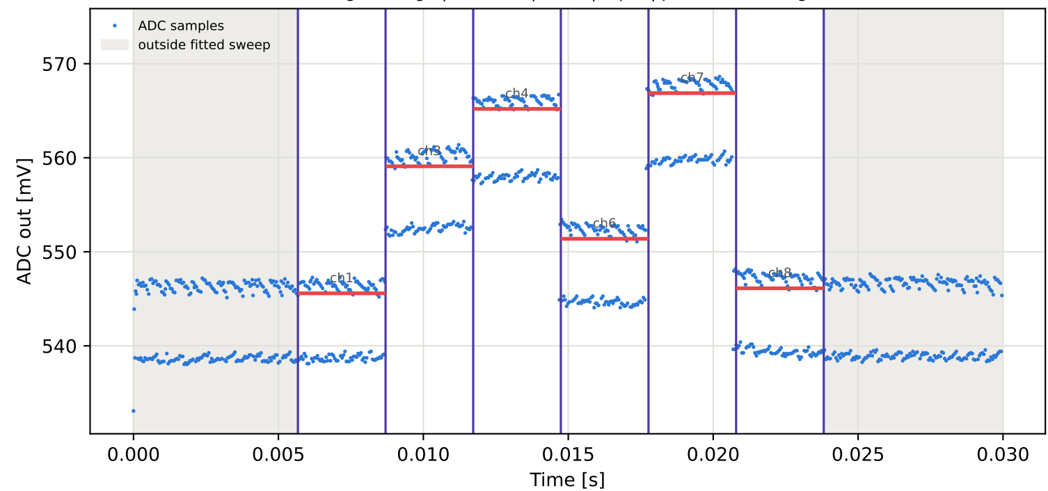
Tag8 &lt;- Tag7 | 825 MHz | run 0 | rep 1 | phase 123.96 deg
