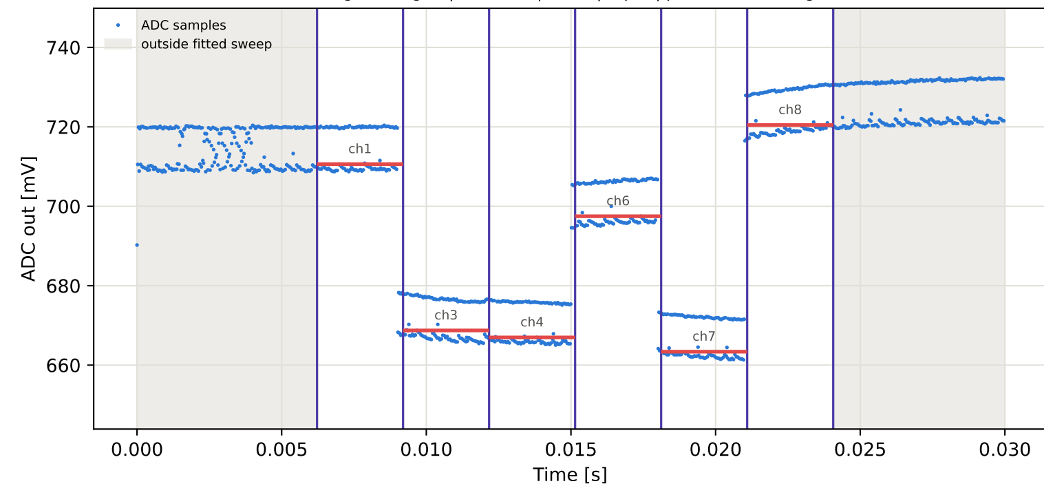
Tag7 &lt;- Tag3 | 865 MHz | run 0 | rep 1 | phase -48.71 deg
