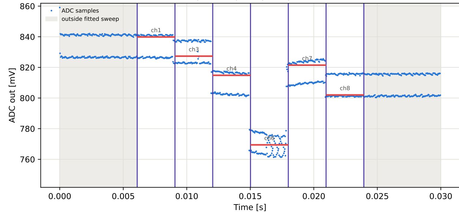
Tag5 &lt;- Tag4 | 905 MHz | run 0 | rep 1 | phase 21.97 deg
