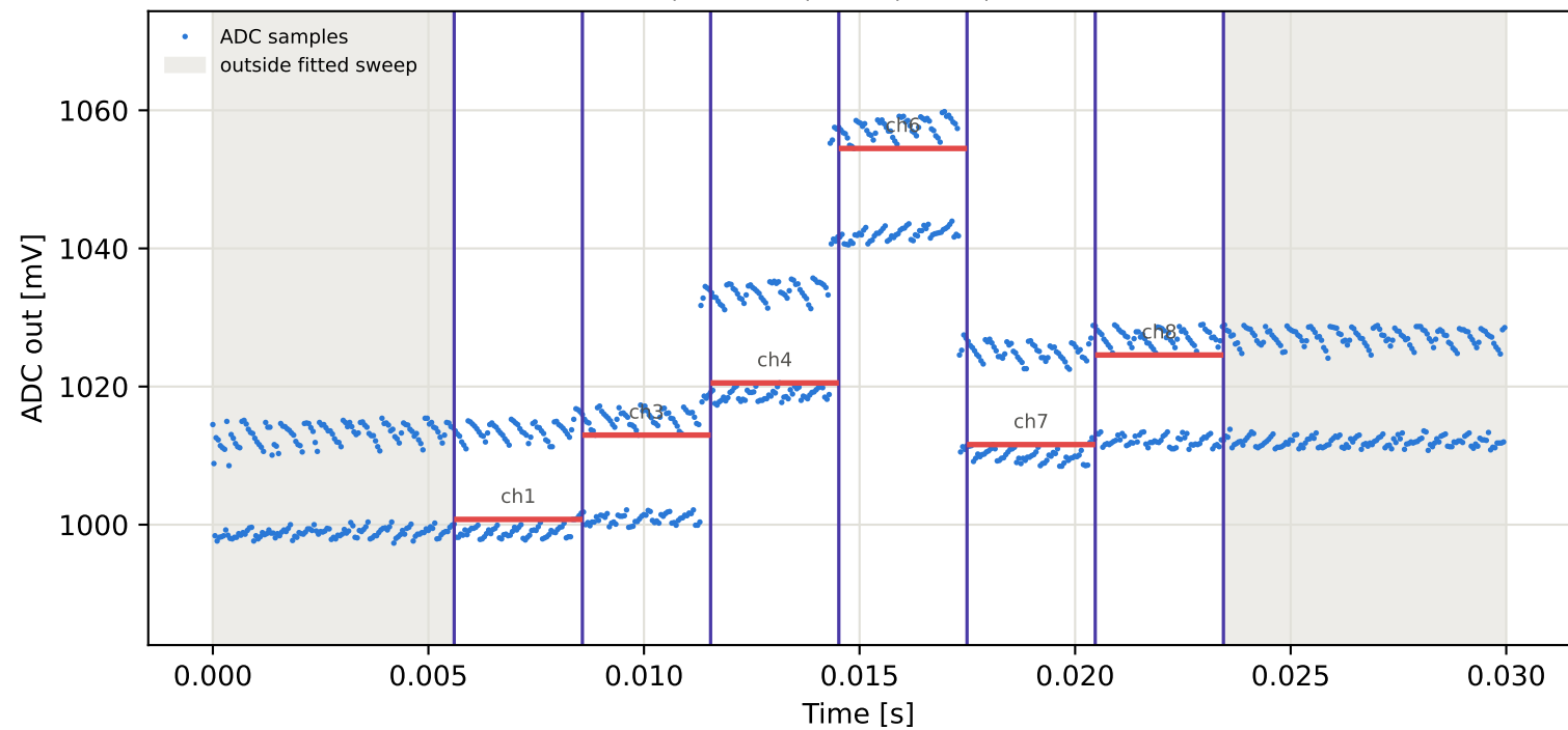
Tag10 &lt;- Tag5 | 935 MHz | run 0 | rep 1 | phase -160.08 deg
