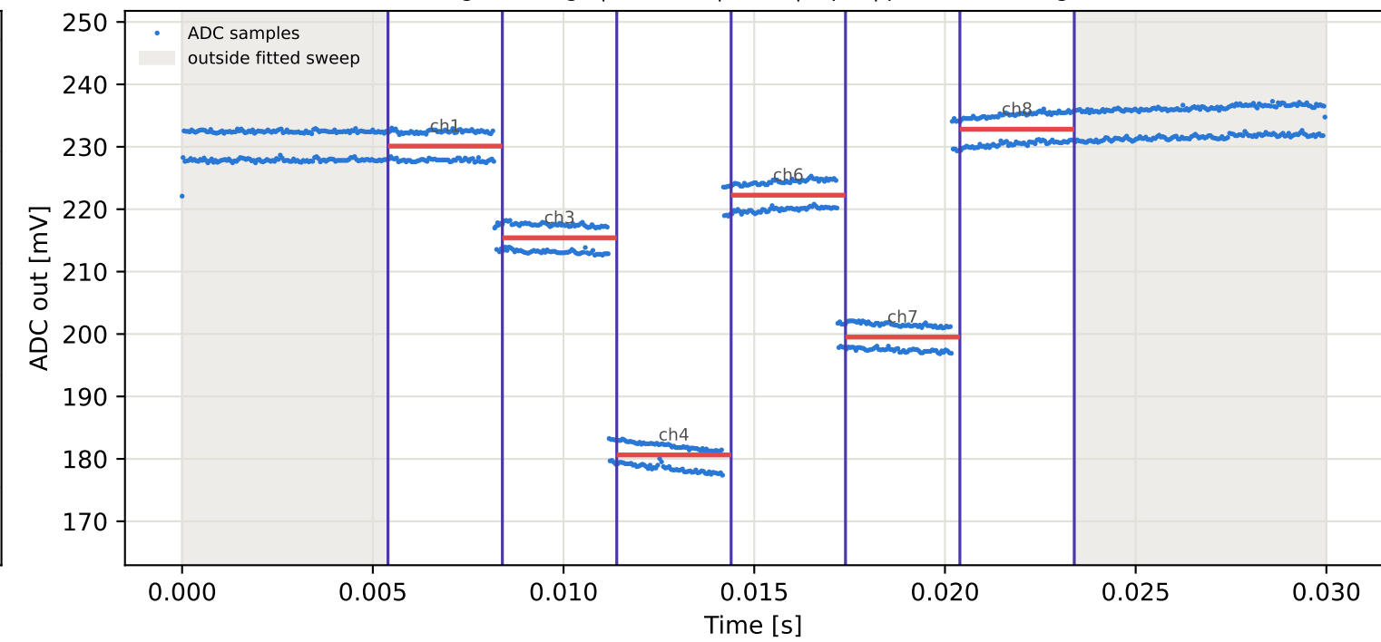
Tag16 &lt;- Tag1 | 975 MHz | run 0 | rep 1 | phase 125.67 deg
