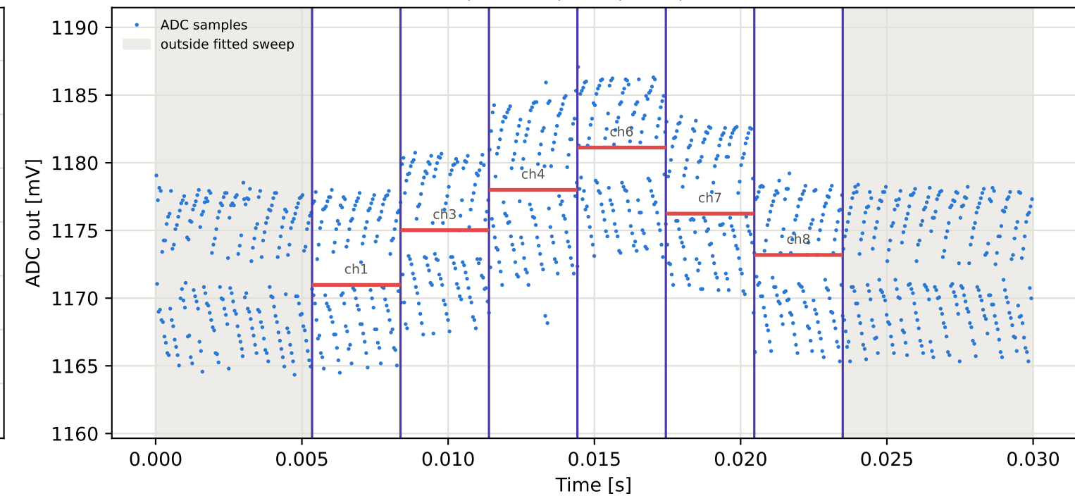
Tag15 &lt;- Tag6 | 905 MHz | run 0 | rep 1 | phase -131.32 deg
