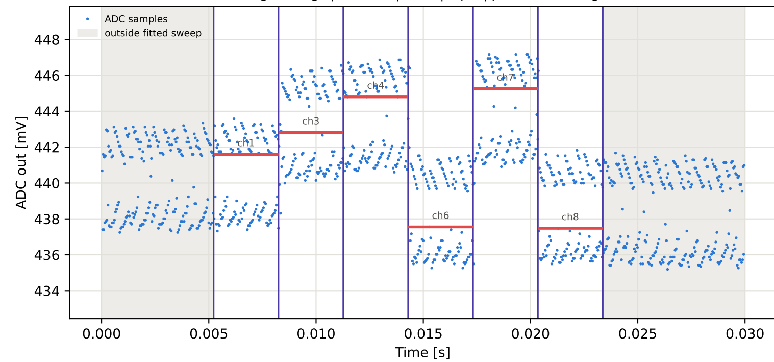
Tag2 &lt;- Tag7 | 865 MHz | run 0 | rep 1 | phase -33.55 deg
