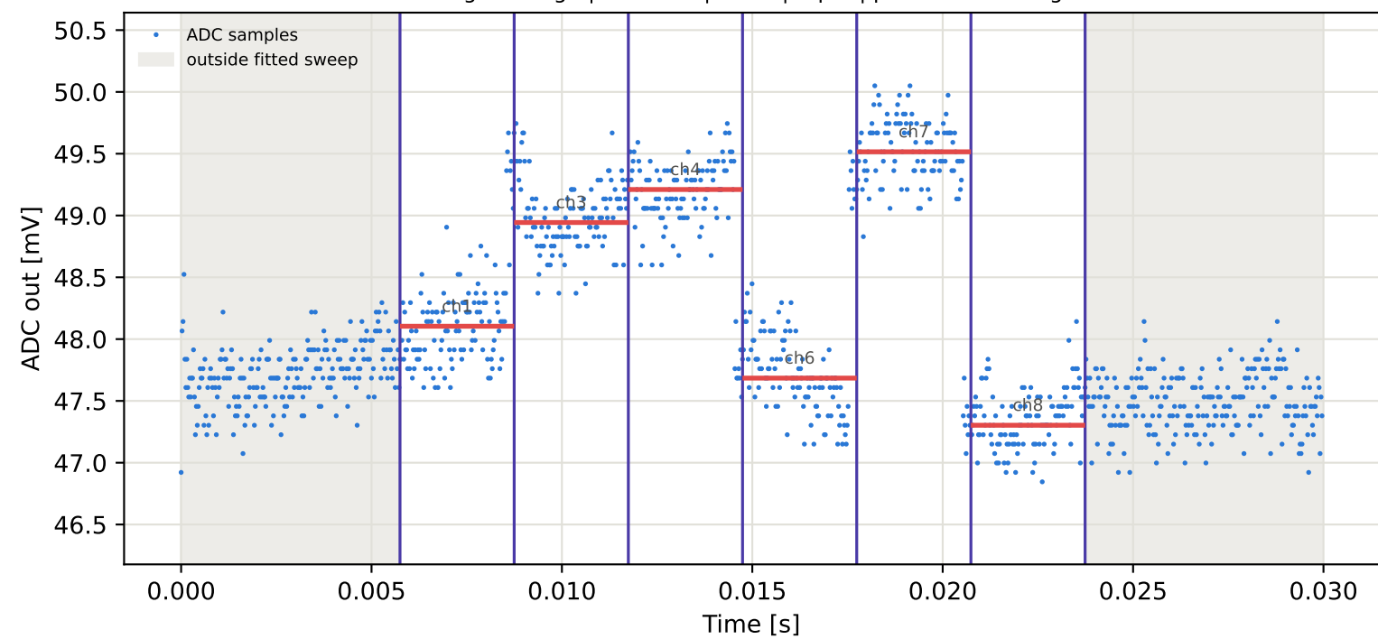
Tag1 &lt;- Tag8 | 775 MHz | run 0 | rep 1 | phase 93.94 deg
