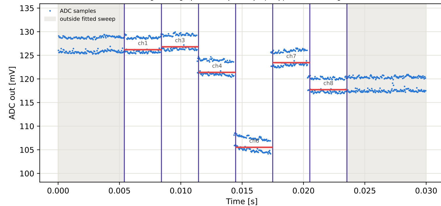
Tag1 &lt;- Tag3 | 915 MHz | run 0 | rep 1 | phase 16.31 deg
