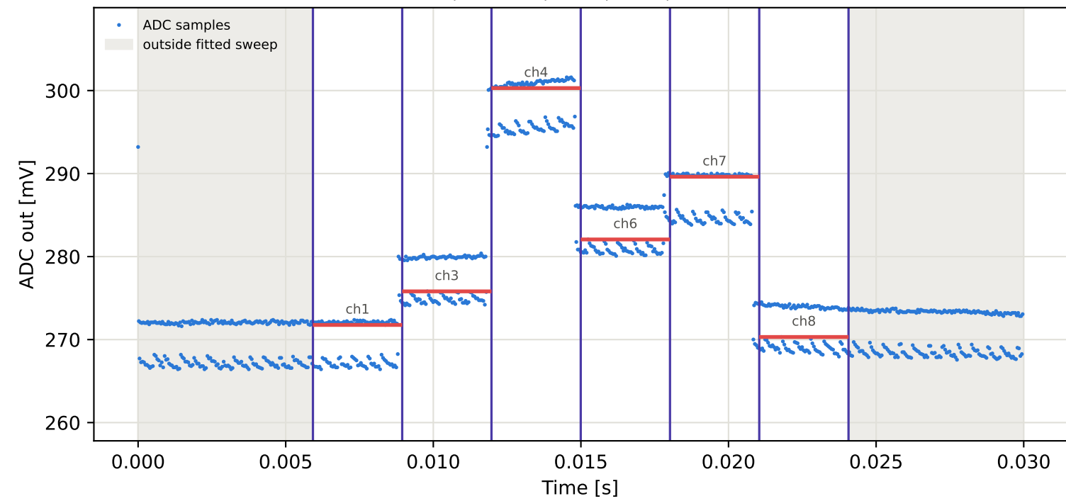
Tag10 &lt;- Tag5 | 975 MHz | run 0 | rep 1 | phase -109.61 deg
