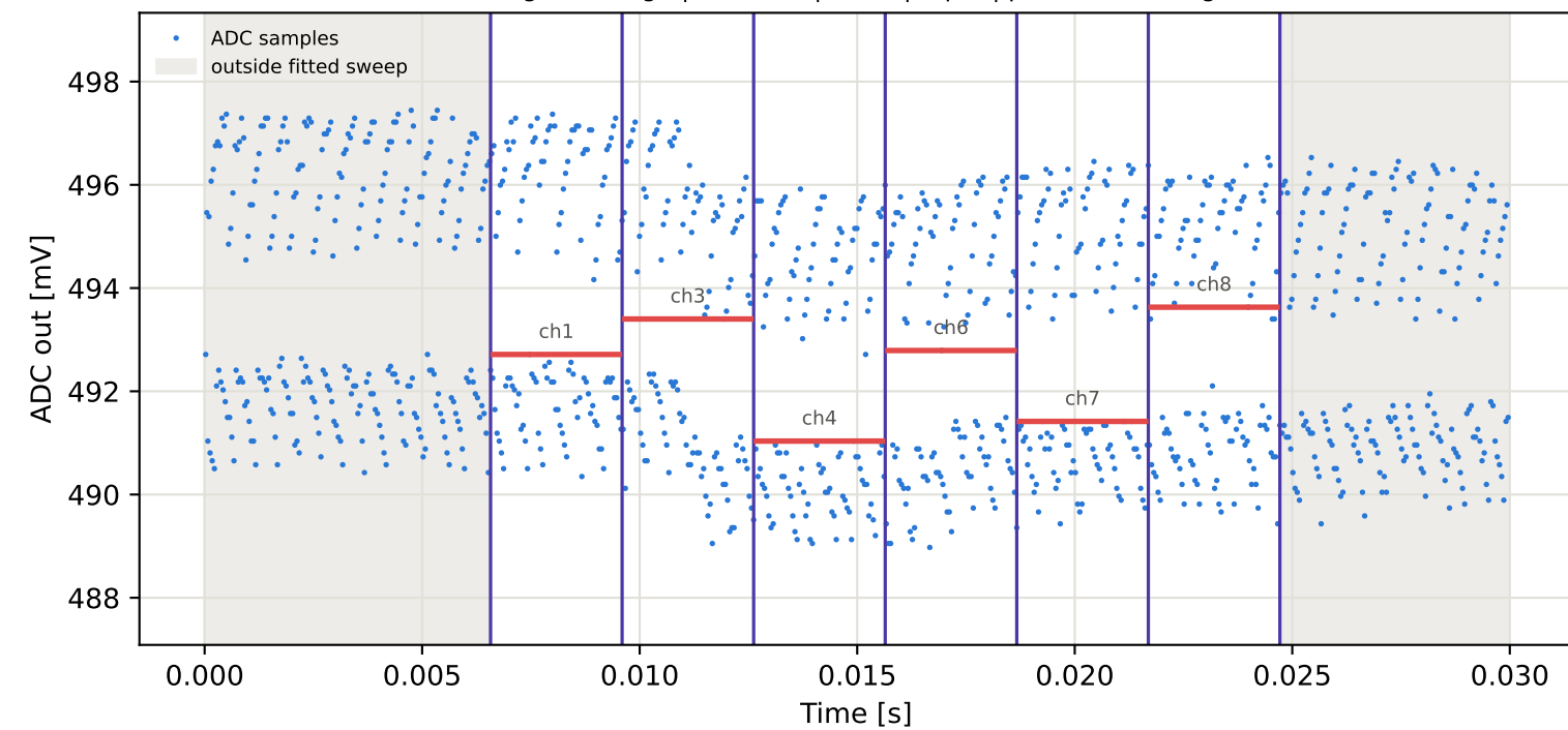
Tag16 &lt;- Tag15 | 845 MHz | run 0 | rep 1 | phase 53.54 deg
