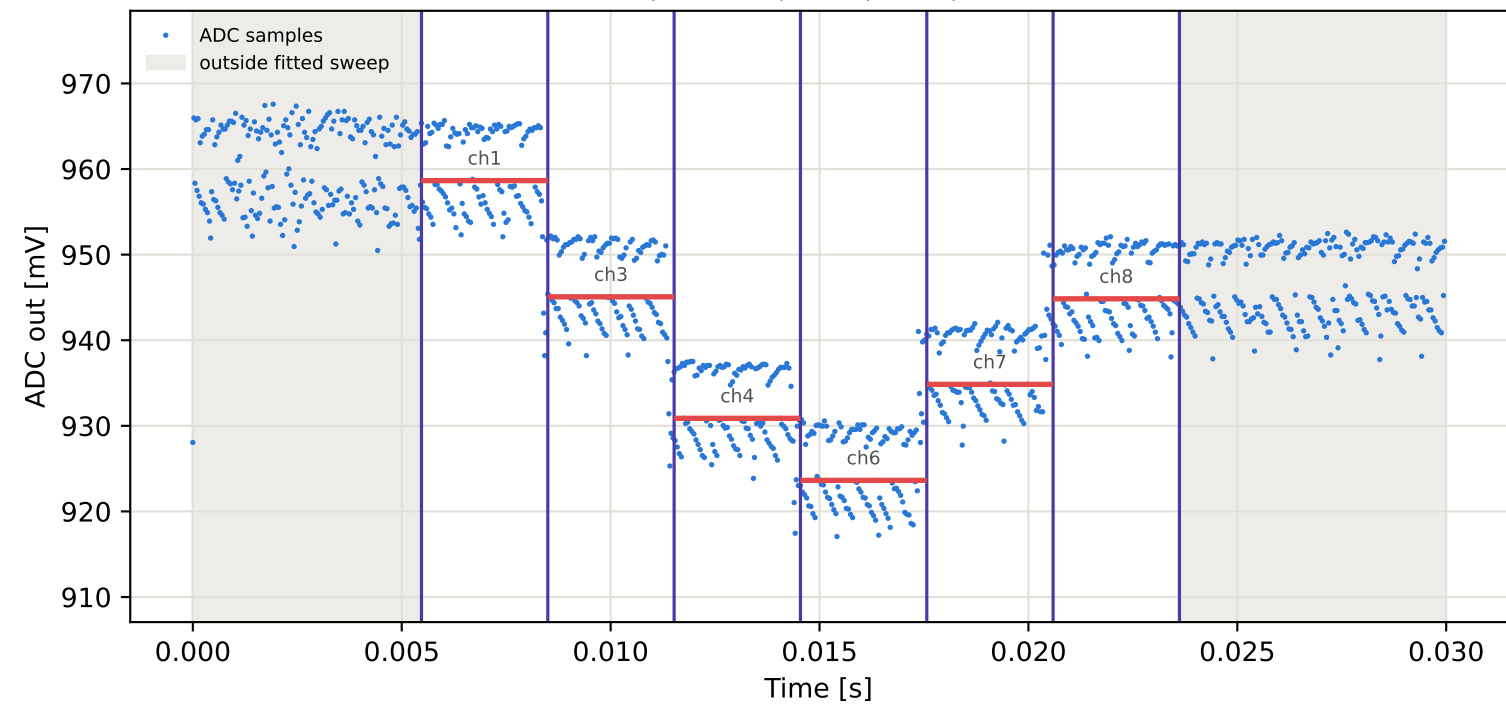
Tag15 &lt;- Tag6 | 875 MHz | run 0 | rep 1 | phase 53.81 deg
