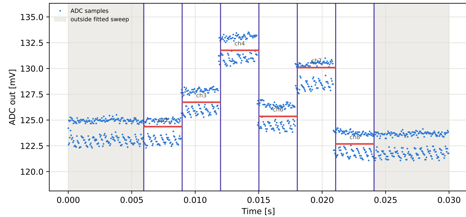
Tag2 &lt;- Tag8 | 945 MHz | run 0 | rep 1 | phase -85.96 deg
