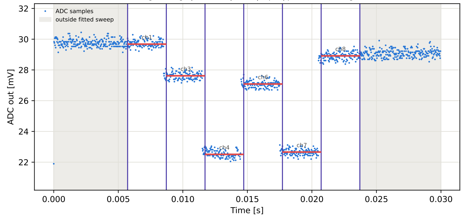
Tag3 &lt;- Tag7 | 785 MHz | run 0 | rep 1 | phase 121.02 deg
