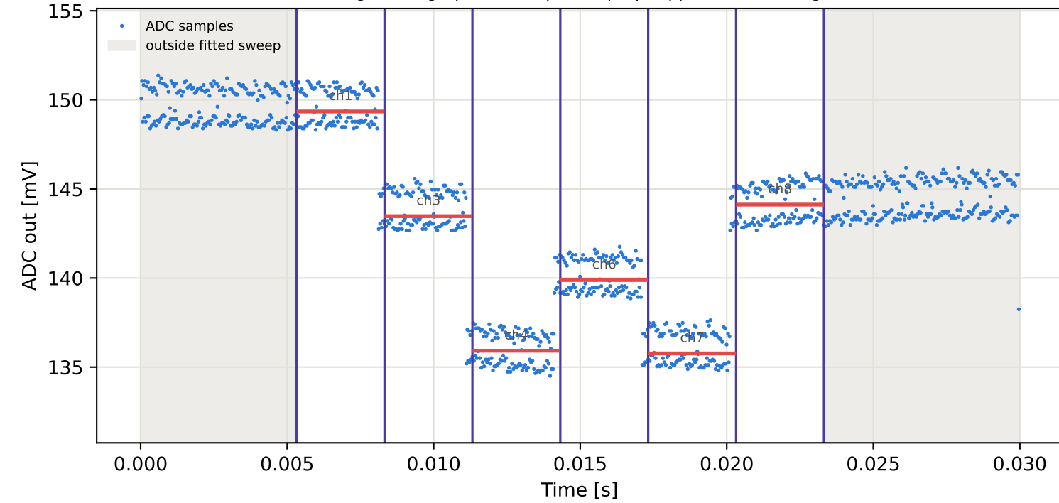
Tag2 &lt;- Tag6 | 825 MHz | run 0 | rep 1 | phase -9.37 deg
