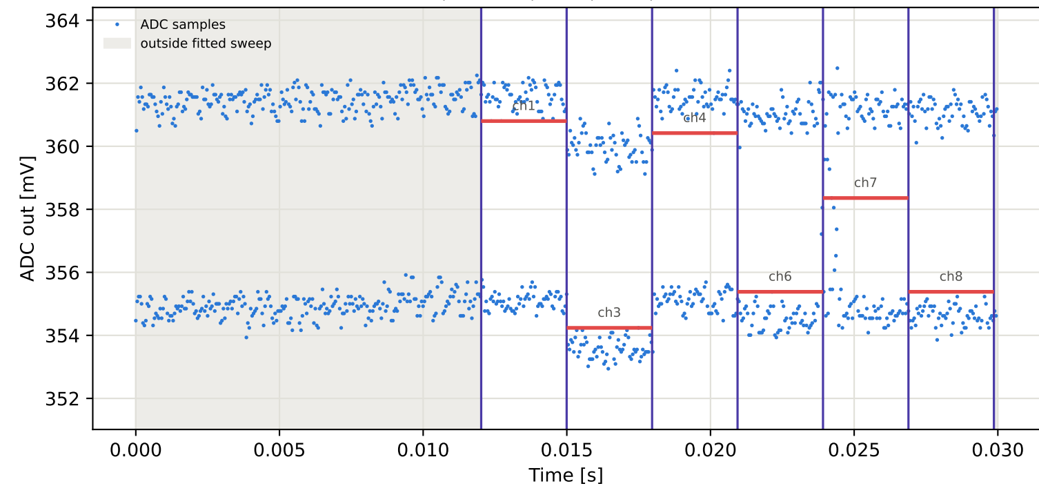
Tag9 &lt;- Tag2 | 985 MHz | run 0 | rep 1 | phase -79.04 deg
