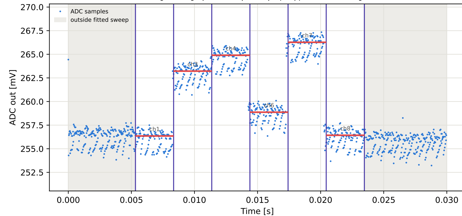
Tag6 &lt;- Tag1 | 835 MHz | run 0 | rep 1 | phase -60.00 deg
