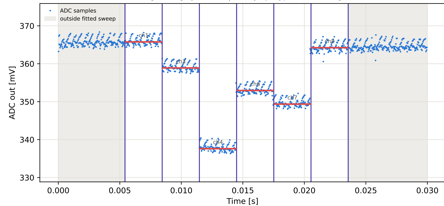
Tag5 &lt;- Tag8 | 965 MHz | run 0 | rep 1 | phase -57.25 deg
