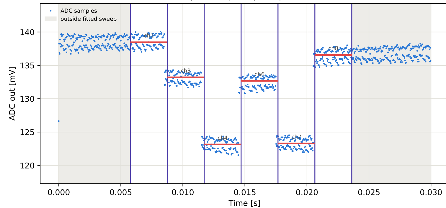
Tag4 &lt;- Tag7 | 795 MHz | run 0 | rep 1 | phase -79.37 deg
