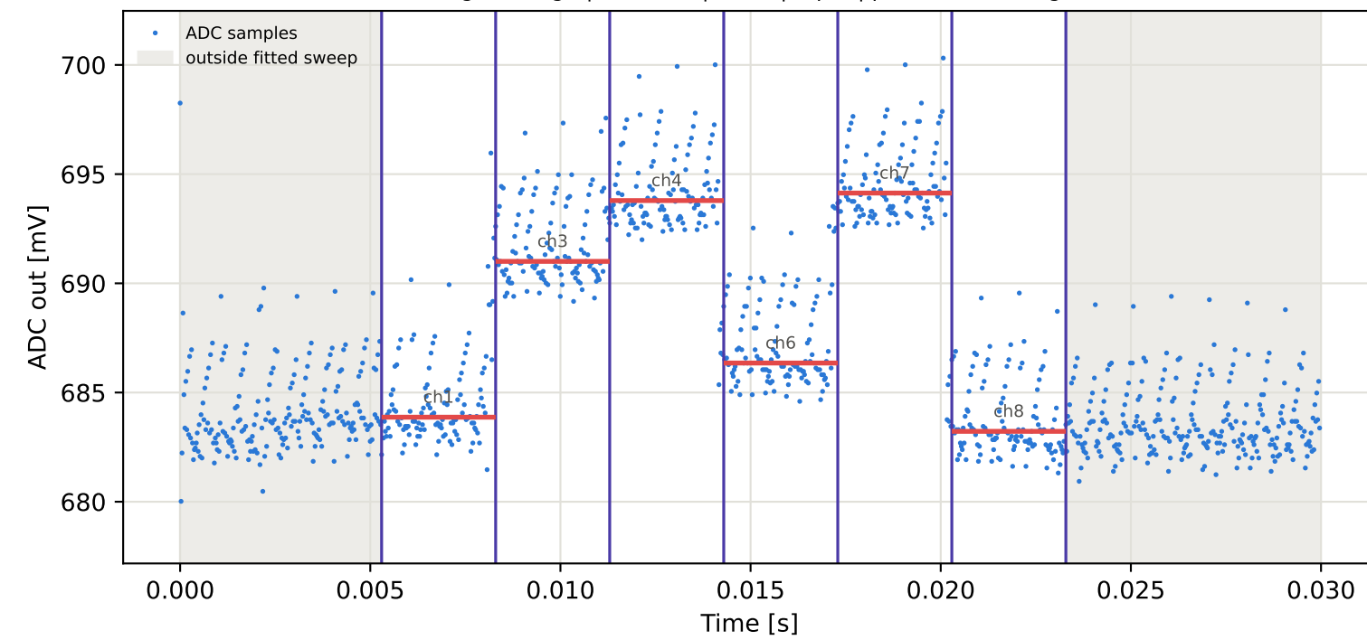
Tag9 &lt;- Tag10 | 845 MHz | run 0 | rep 1 | phase 167.59 deg
