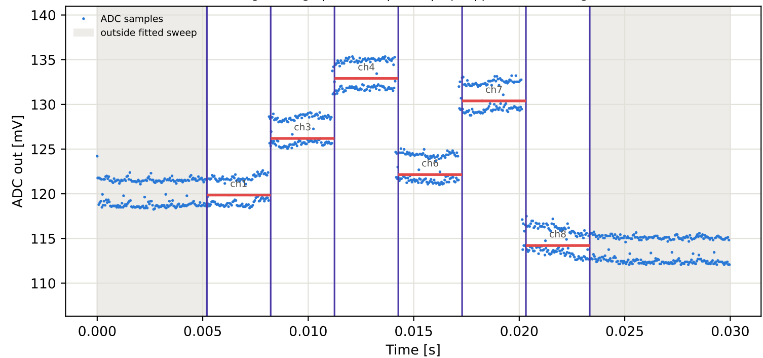
Tag10 &lt;- Tag1 | 915 MHz | run 0 | rep 1 | phase 149.74 deg
