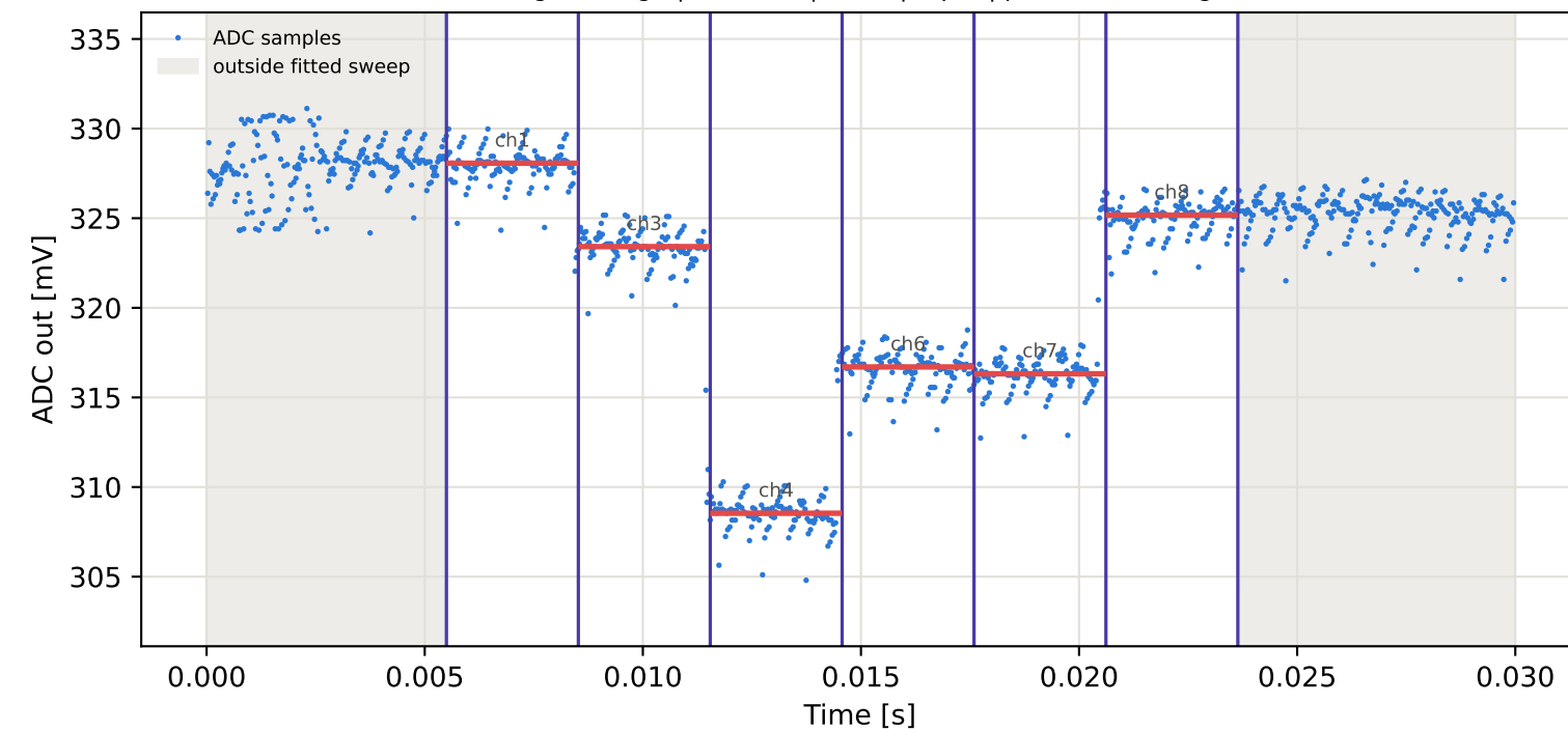
Tag6 &lt;- Tag9 | 975 MHz | run 0 | rep 1 | phase 23.82 deg
