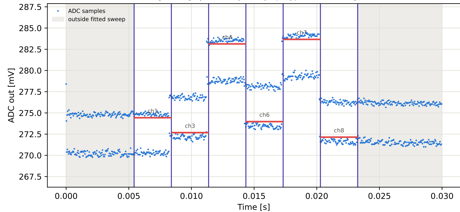
Tag8 &lt;- Tag5 | 795 MHz | run 0 | rep 1 | phase 135.73 deg
