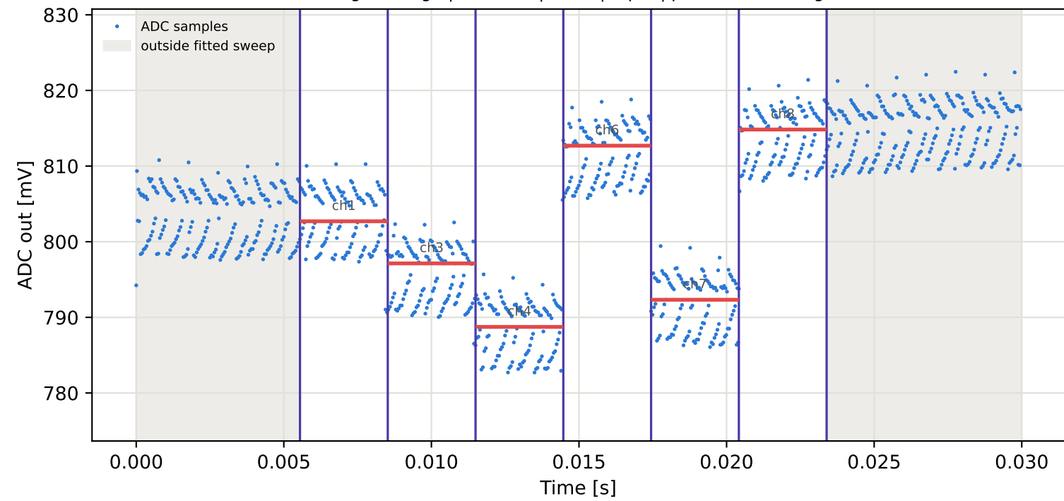
Tag9 &lt;- Tag2 | 925 MHz | run 0 | rep 1 | phase 131.09 deg
