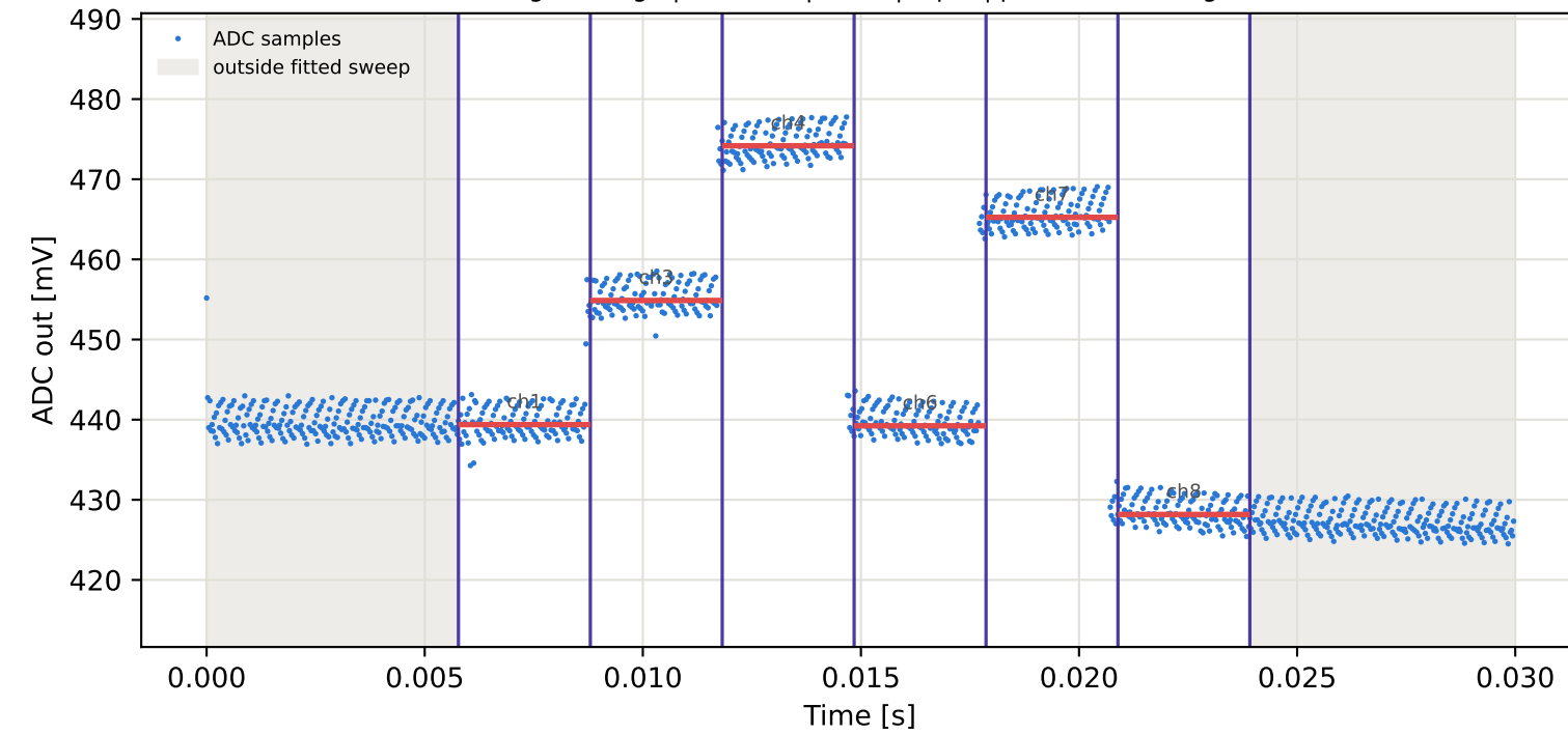
Tag3 &lt;- Tag8 | 935 MHz | run 0 | rep 1 | phase -73.59 deg
