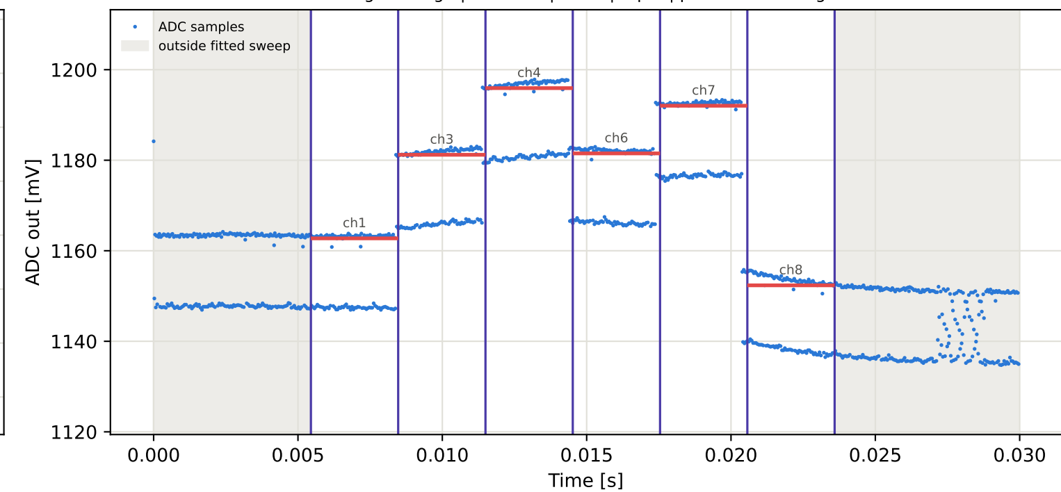
Tag8 &lt;- Tag5 | 895 MHz | run 0 | rep 1 | phase 73.17 deg
