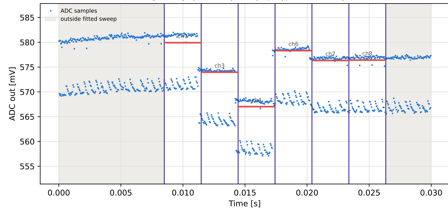
Tag5 &lt;- Tag8 | 955 MHz | run 0 | rep 1 | phase -70.04 deg
