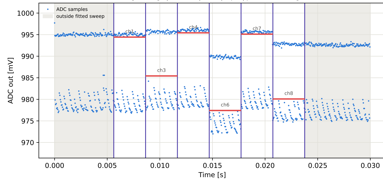
Tag8 &lt;- Tag4 | 945 MHz | run 0 | rep 1 | phase 90.76 deg
