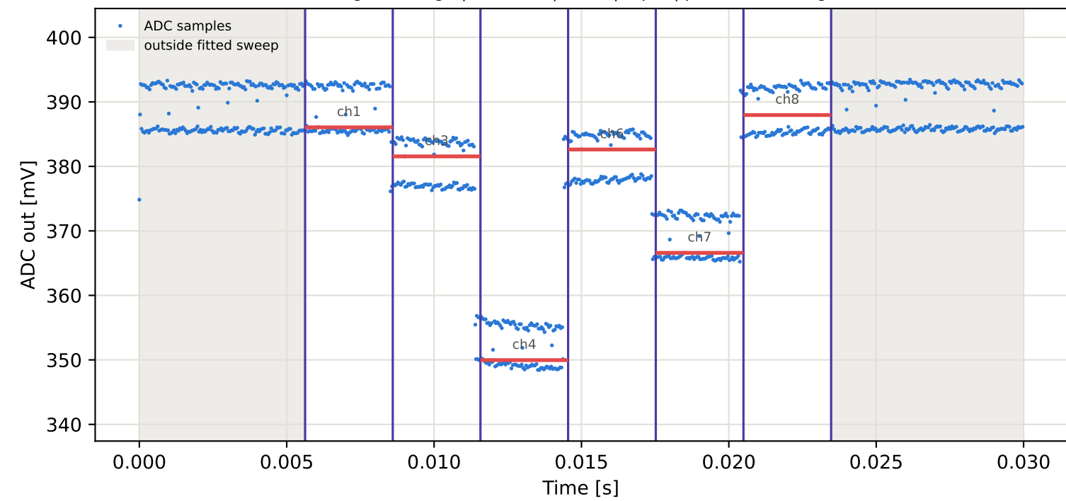
Tag16 &lt;- Tag1 | 995 MHz | run 0 | rep 1 | phase -161.44 deg
