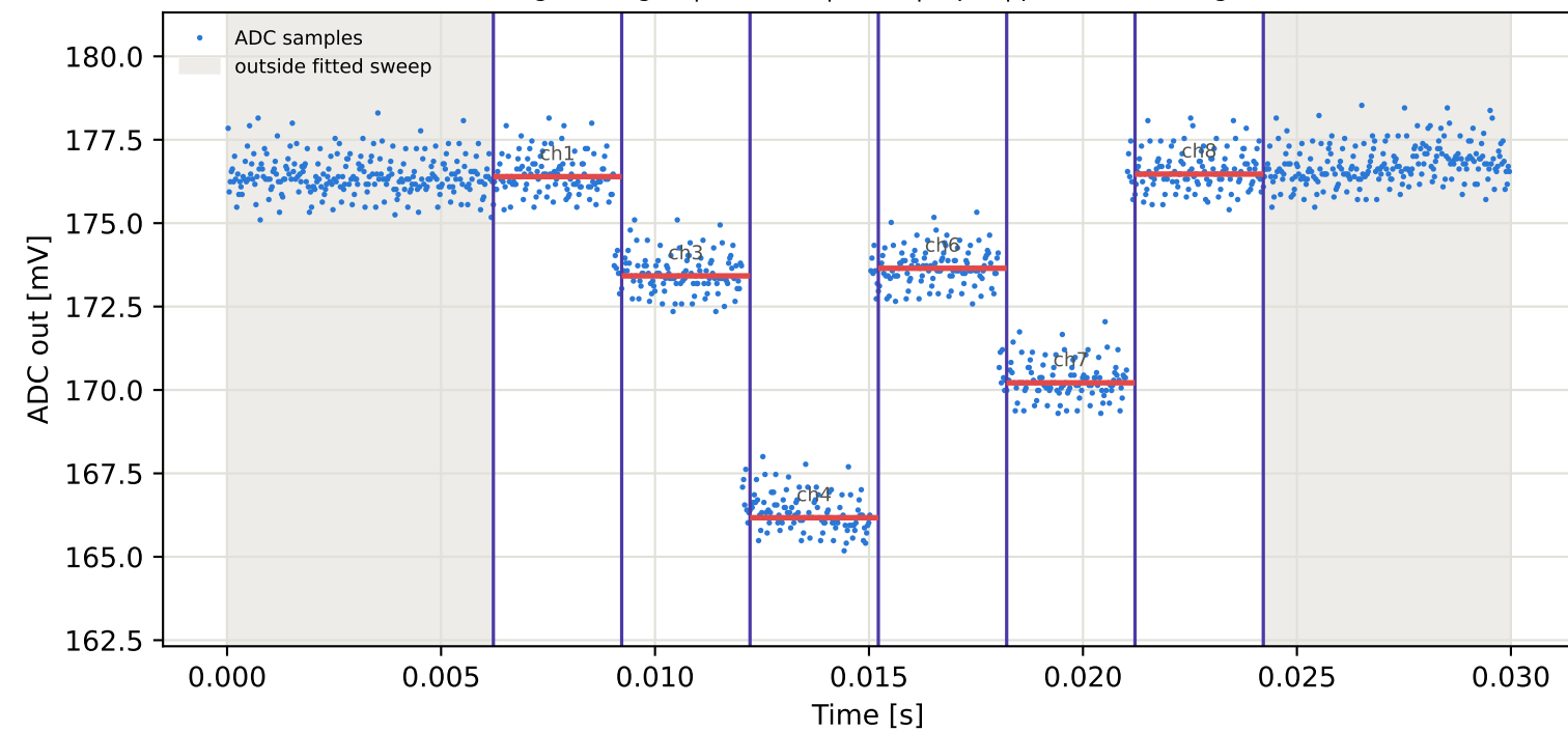
Tag1 &lt;- Tag2 | 995 MHz | run 0 | rep 1 | phase -30.65 deg
