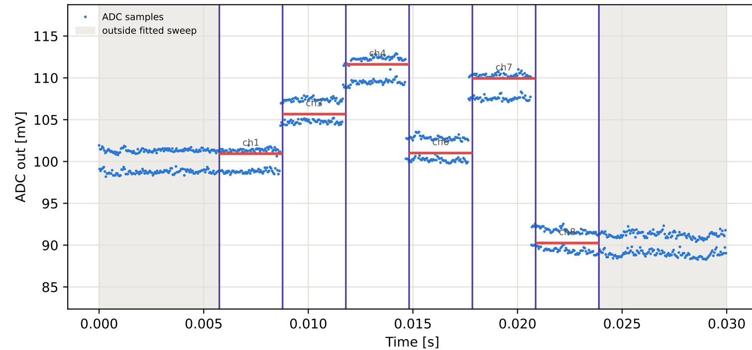
Tag6 &lt;- Tag4 | 905 MHz | run 0 | rep 1 | phase -116.19 deg
