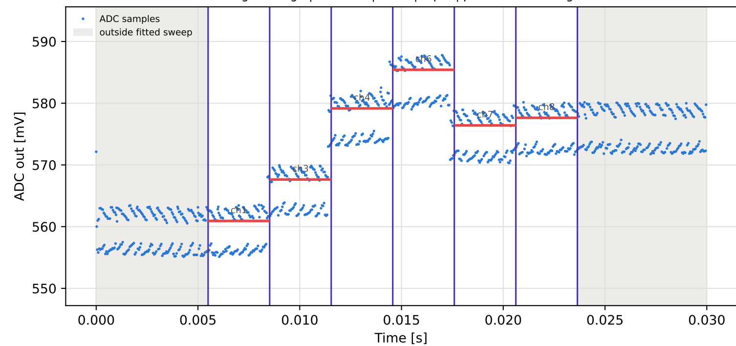
Tag7 &lt;- Tag1 | 865 MHz | run 0 | rep 1 | phase 3.47 deg
