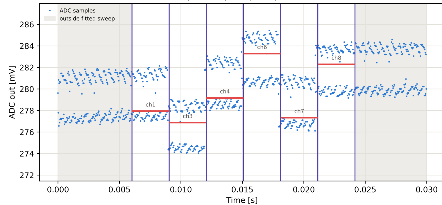
Tag9 &lt;- Tag10 | 795 MHz | run 0 | rep 1 | phase 37.58 deg
