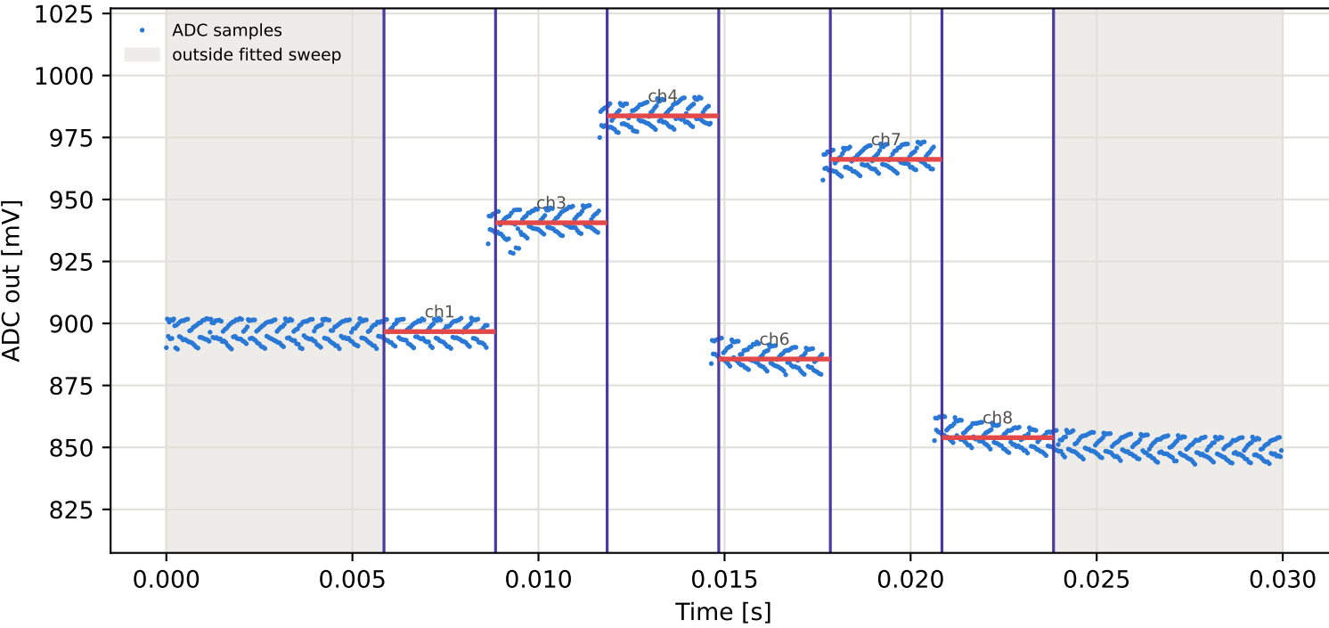
Tag6 &lt;- Tag1 | 925 MHz | run 0 | rep 1 | phase 55.95 deg
