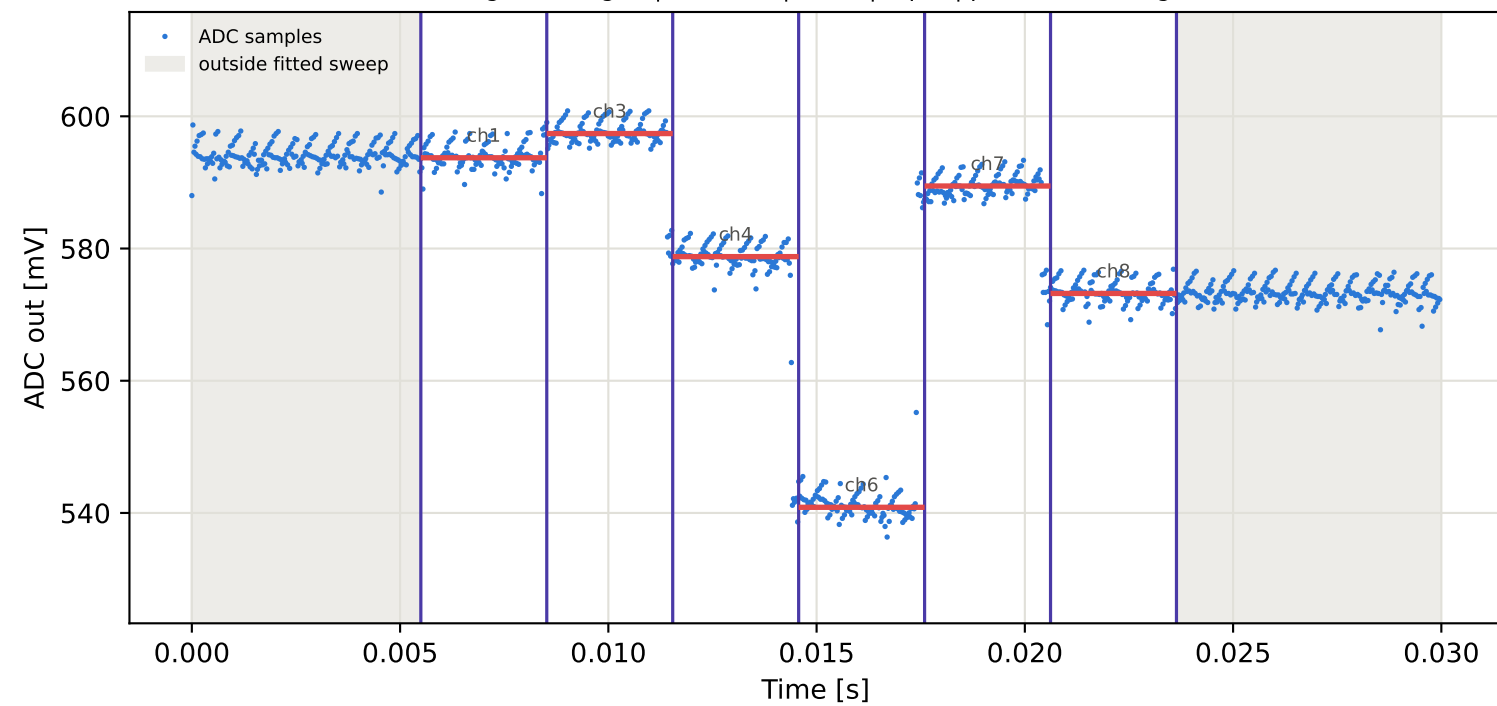
Tag10 &lt;- Tag3 | 945 MHz | run 0 | rep 1 | phase -165.93 deg
