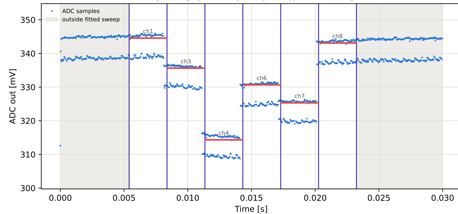
Tag6 &lt;- Tag9 | 965 MHz | run 0 | rep 1 | phase 70.80 deg
