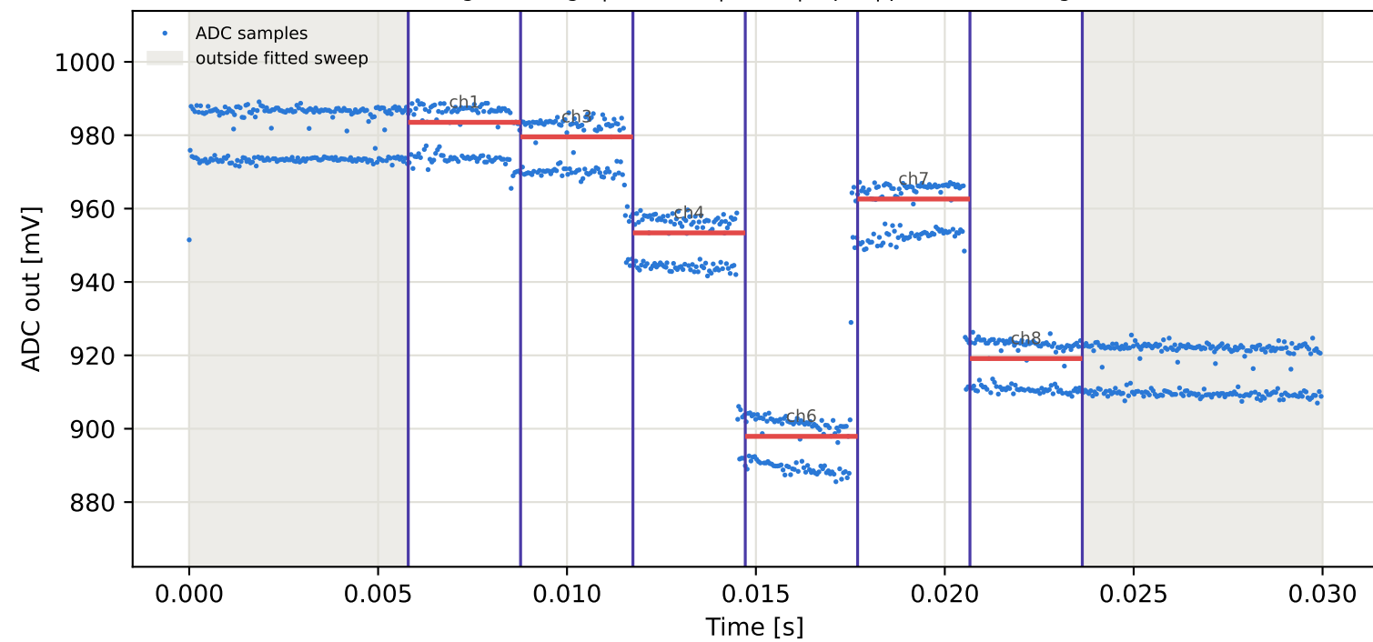
Tag16 &lt;- Tag1 | 885 MHz | run 0 | rep 1 | phase -141.94 deg
