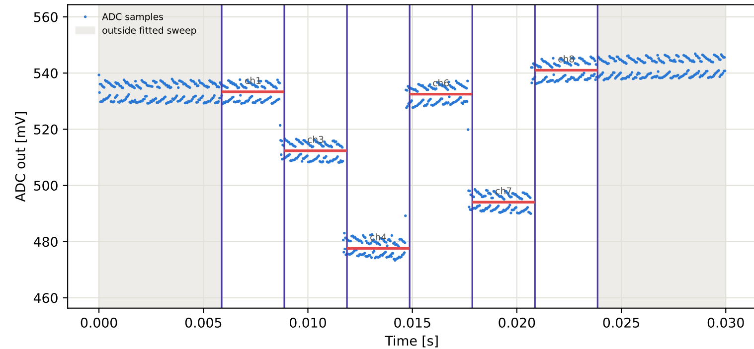
Tag5 &lt;- Tag3 | 975 MHz | run 0 | rep 1 | phase 165.20 deg
