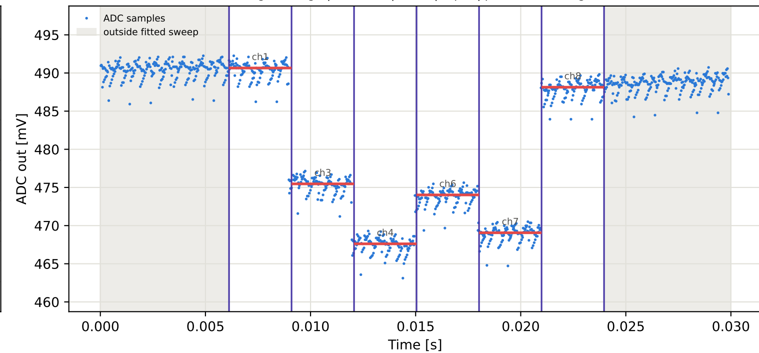
Tag4 &lt;- Tag8 | 865 MHz | run 0 | rep 1 | phase -157.38 deg
