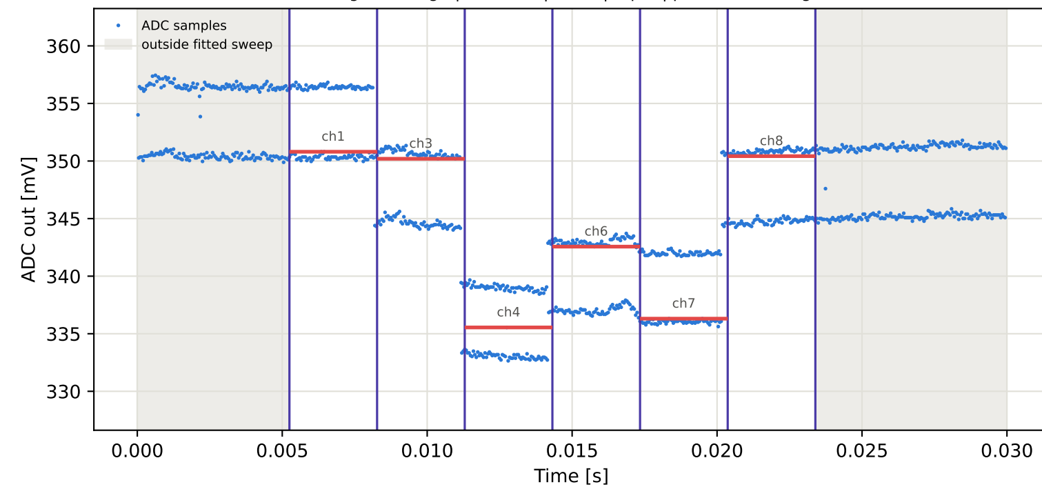
Tag16 &lt;- Tag10 | 845 MHz | run 0 | rep 1 | phase -124.19 deg
