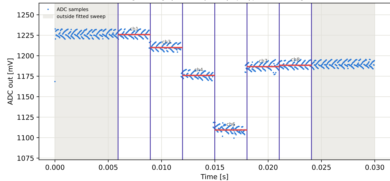
Tag16 &lt;- Tag1 | 905 MHz | run 0 | rep 1 | phase -10.47 deg
