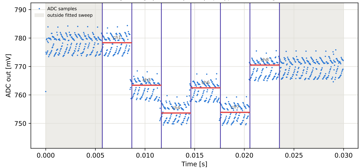
Tag8 &lt;- Tag5 | 835 MHz | run 0 | rep 1 | phase -32.67 deg
