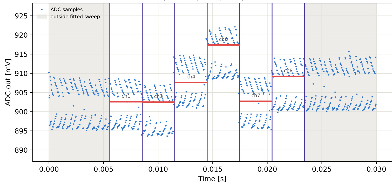
Tag8 &lt;- Tag5 | 985 MHz | run 0 | rep 1 | phase 24.86 deg
