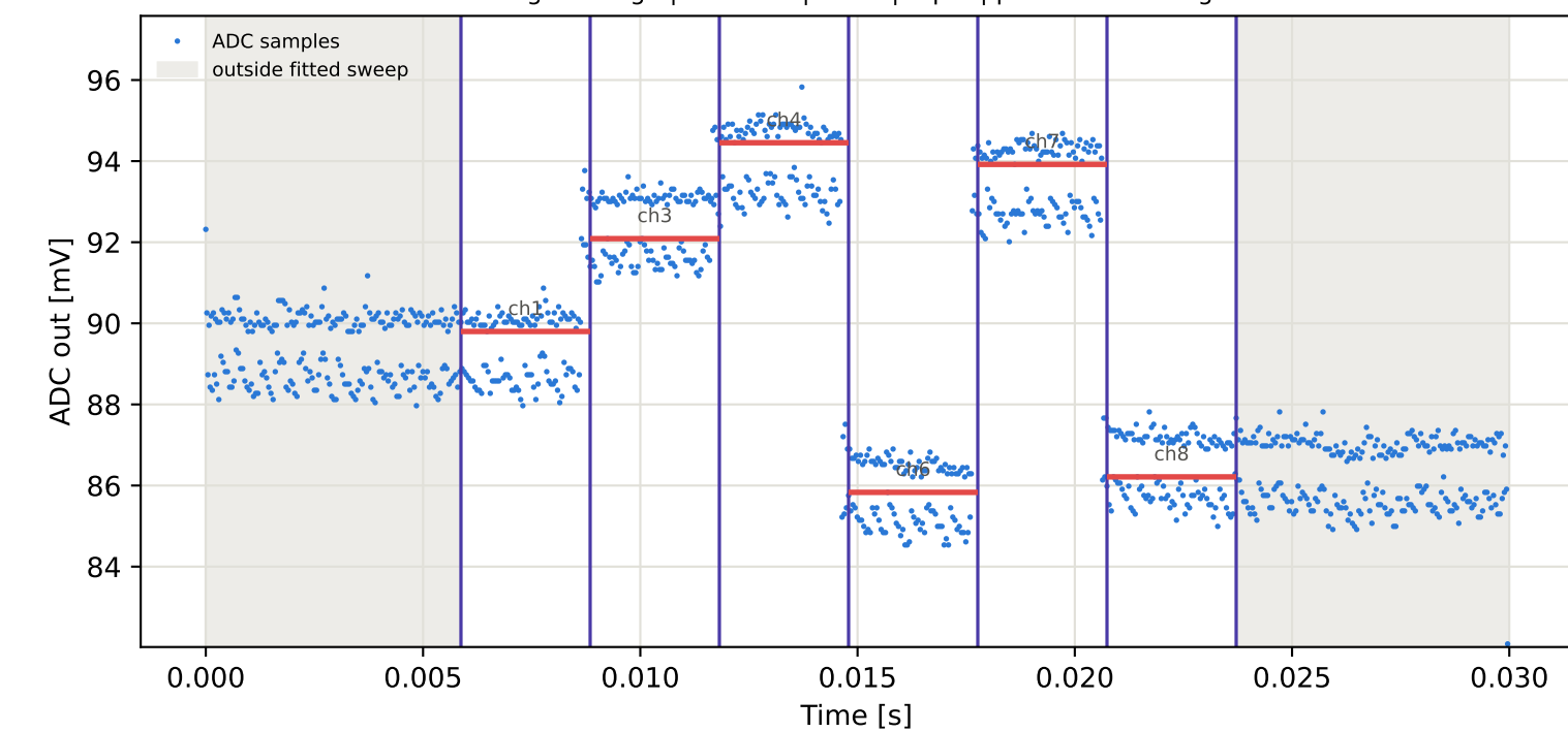
Tag4 &lt;- Tag9 | 995 MHz | run 0 | rep 1 | phase 119.05 deg
