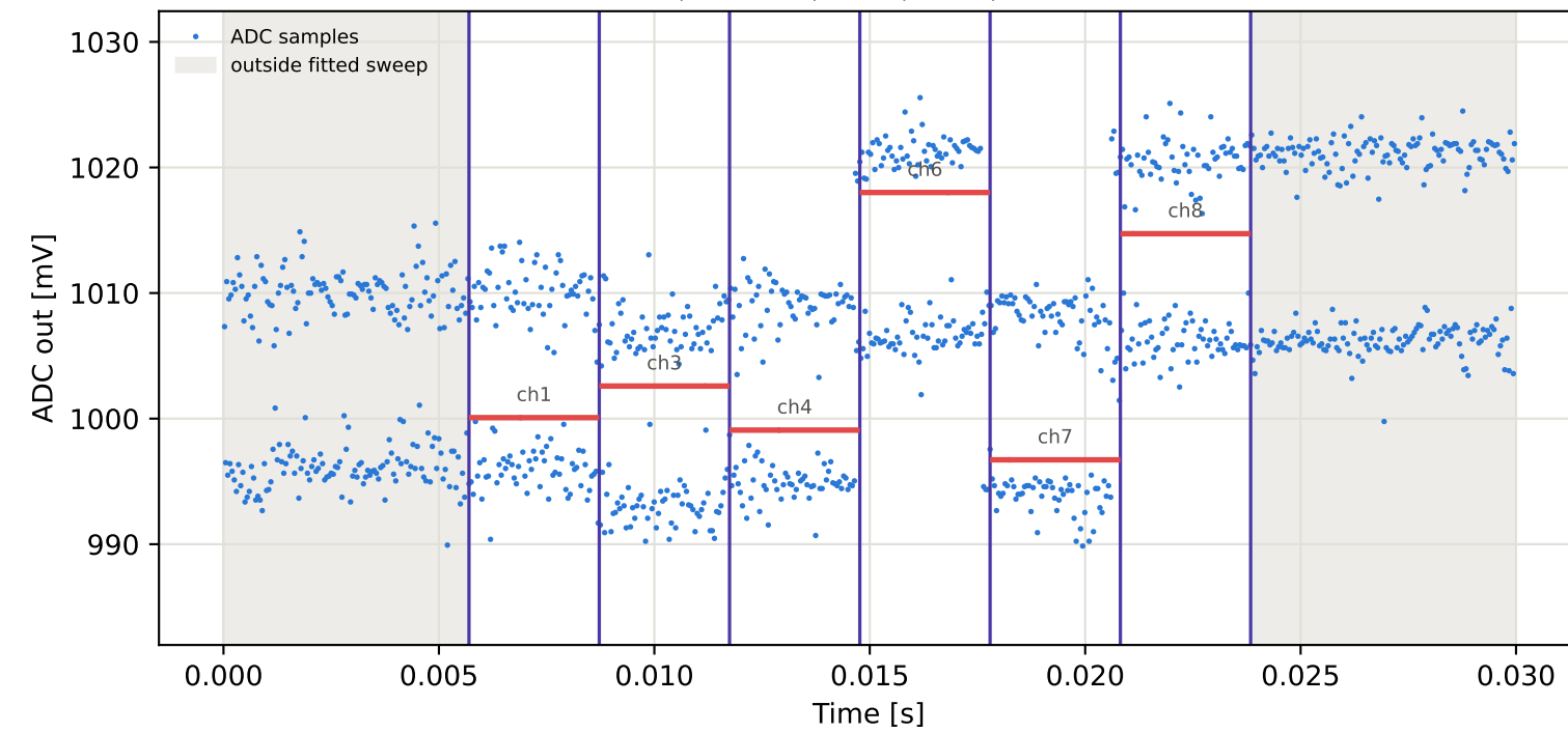
Tag6 &lt;- Tag4 | 885 MHz | run 0 | rep 1 | phase 168.64 deg
