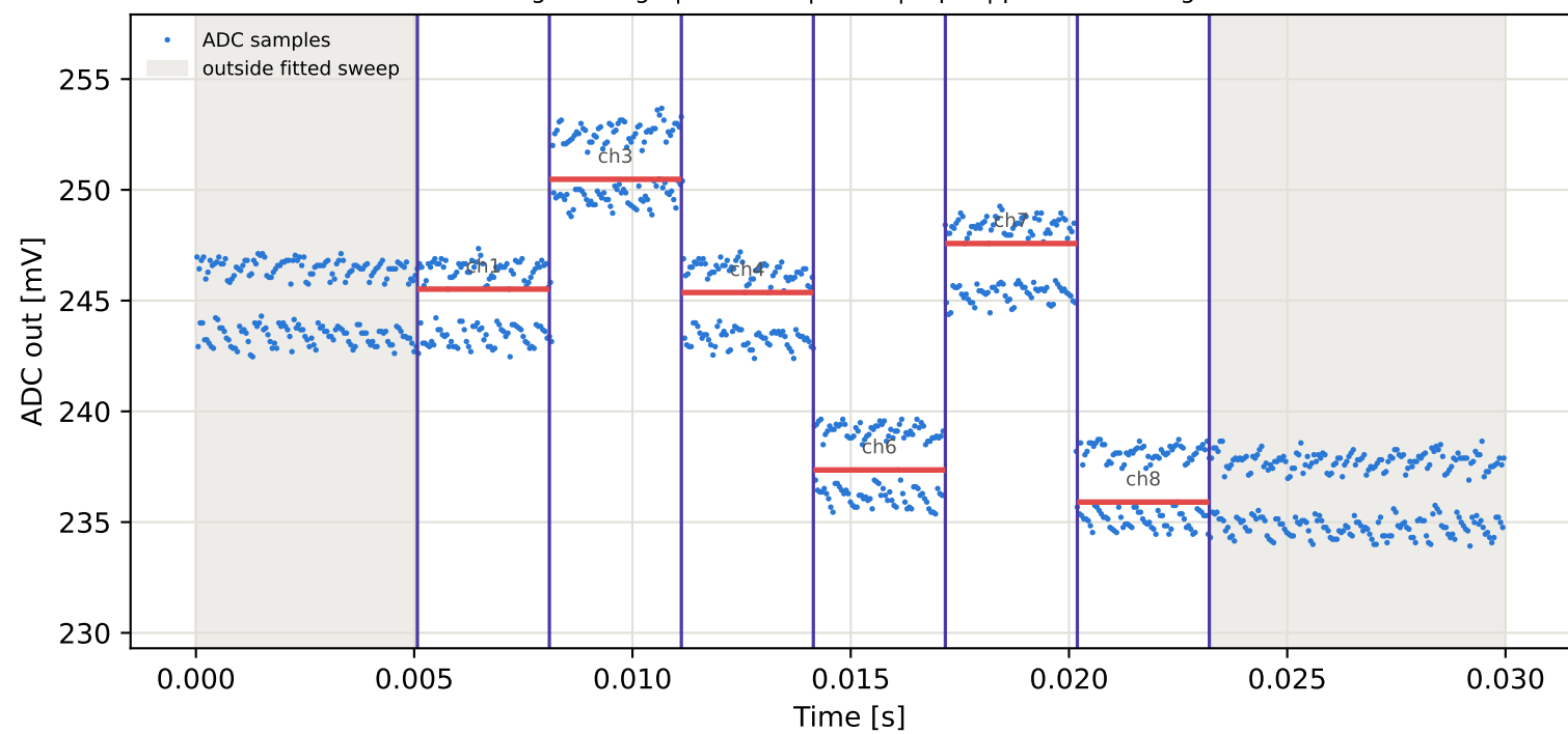
Tag9 &lt;- Tag6 | 845 MHz | run 0 | rep 1 | phase 12.86 deg
