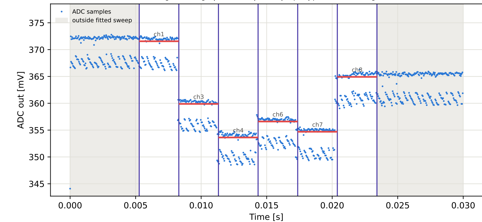
Tag15 &lt;- Tag6 | 855 MHz | run 0 | rep 1 | phase -23.08 deg
