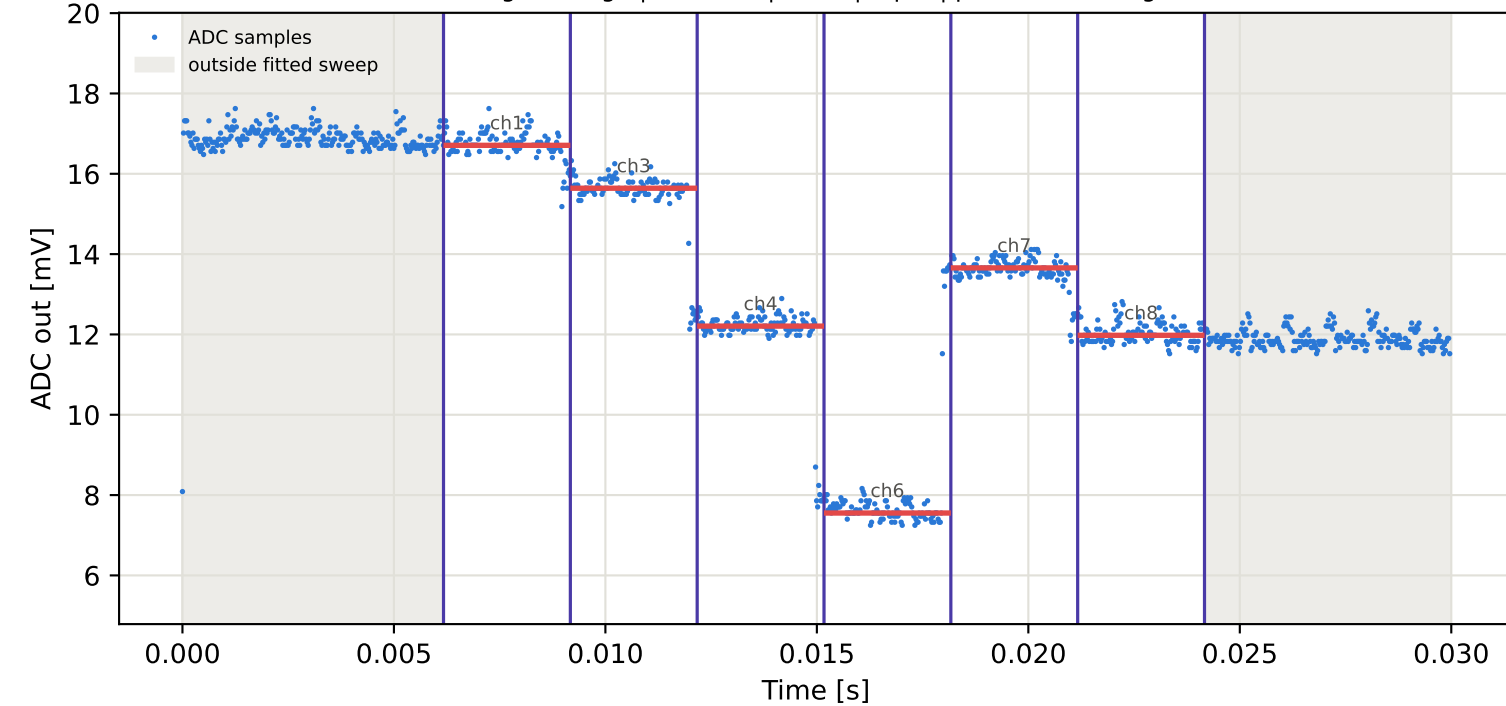
Tag1 &lt;- Tag9 | 905 MHz | run 0 | rep 1 | phase 28.87 deg
