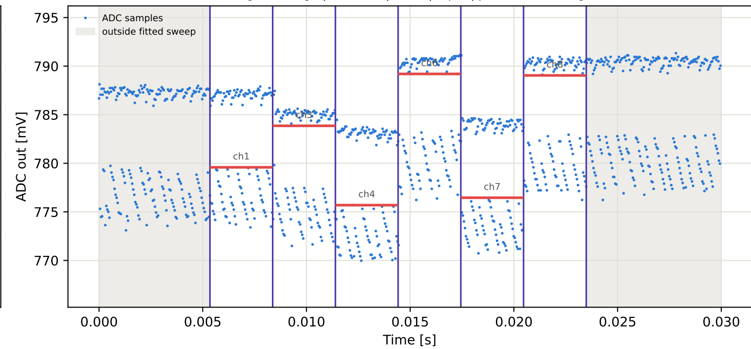
Tag15 &lt;- Tag4 | 925 MHz | run 0 | rep 1 | phase -176.91 deg
