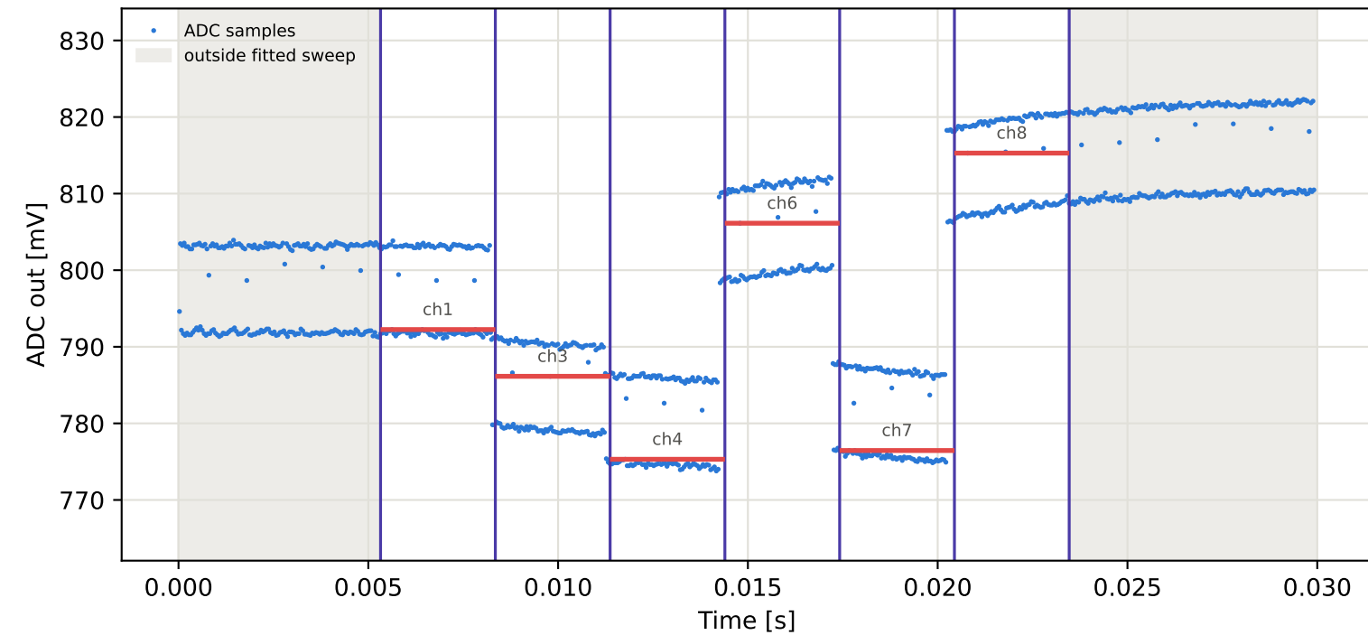
Tag15 &lt;- Tag6 | 895 MHz | run 0 | rep 1 | phase -158.81 deg
