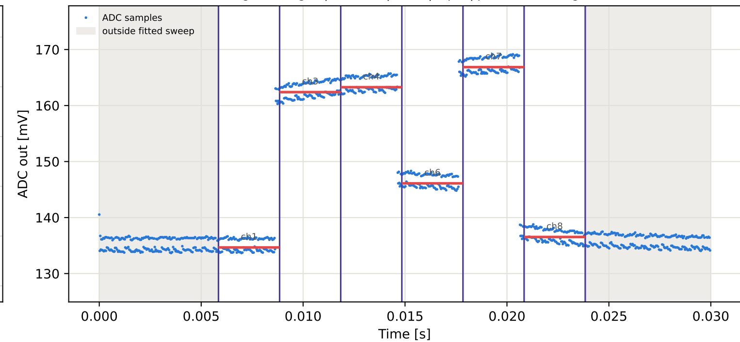
Tag10 &lt;- Tag3 | 845 MHz | run 0 | rep 1 | phase 21.35 deg
