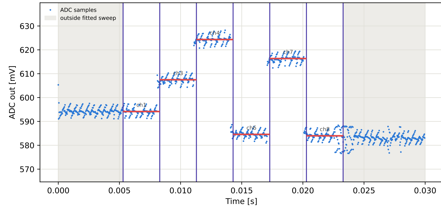
Tag15 &lt;- Tag5 | 965 MHz | run 0 | rep 1 | phase 172.96 deg
