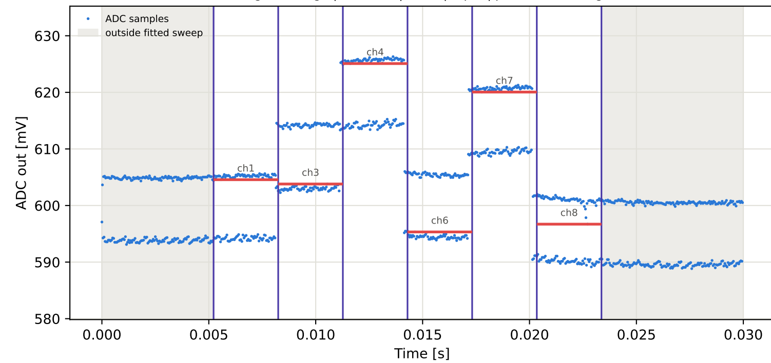
Tag15 &lt;- Tag9 | 965 MHz | run 0 | rep 1 | phase 91.78 deg
