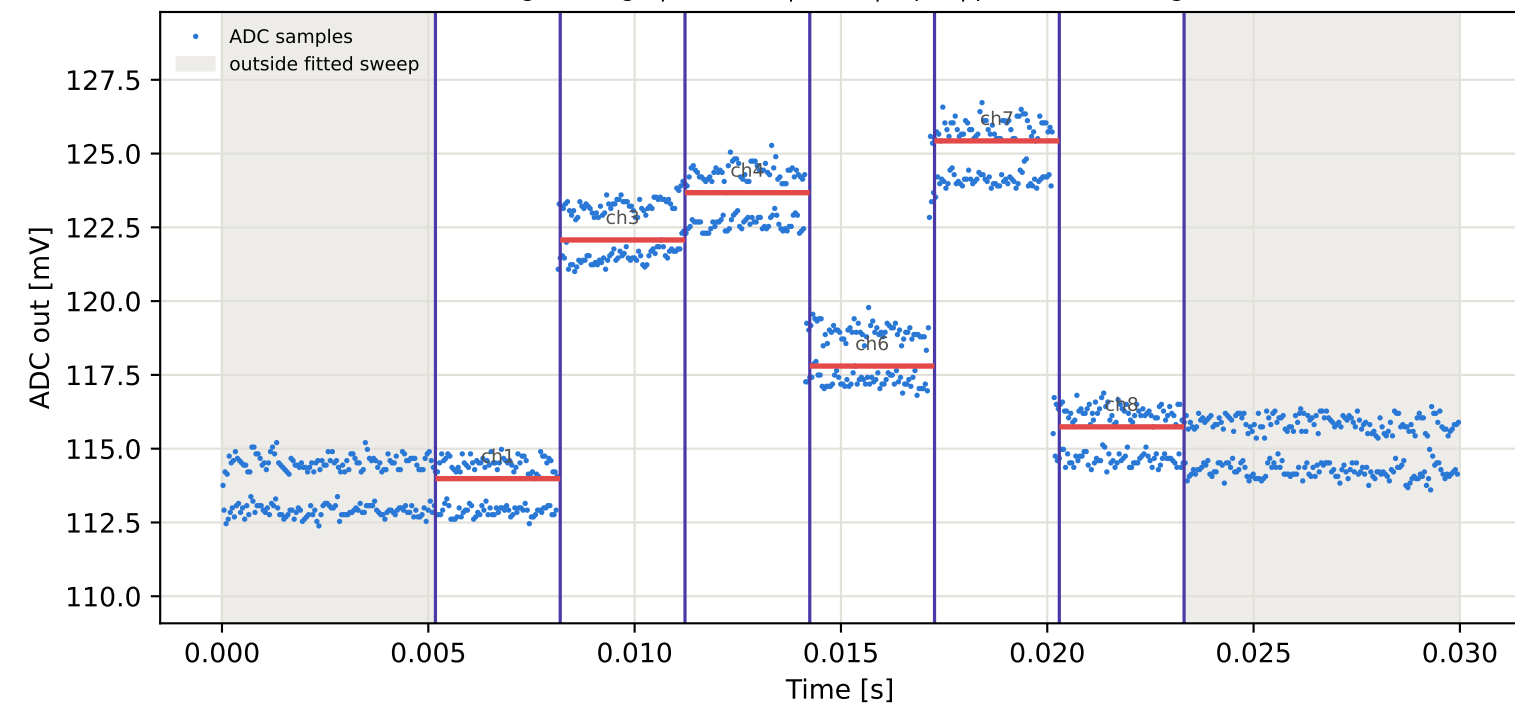
Tag9 &lt;- Tag6 | 825 MHz | run 0 | rep 1 | phase -83.47 deg
