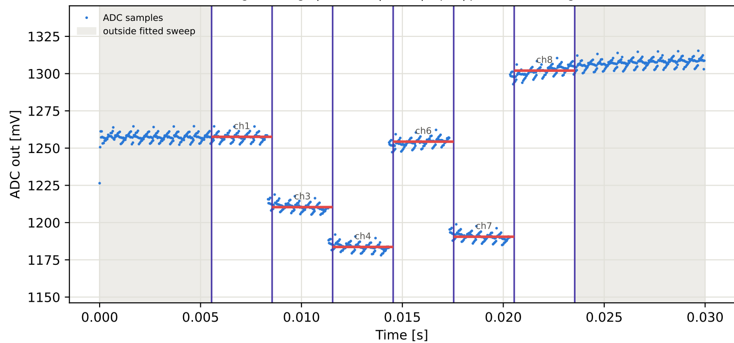
Tag16 &lt;- Tag5 | 895 MHz | run 0 | rep 1 | phase 102.47 deg
