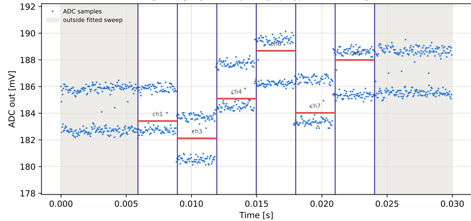
Tag4 &lt;- Tag16 | 825 MHz | run 0 | rep 1 | phase -64.14 deg
