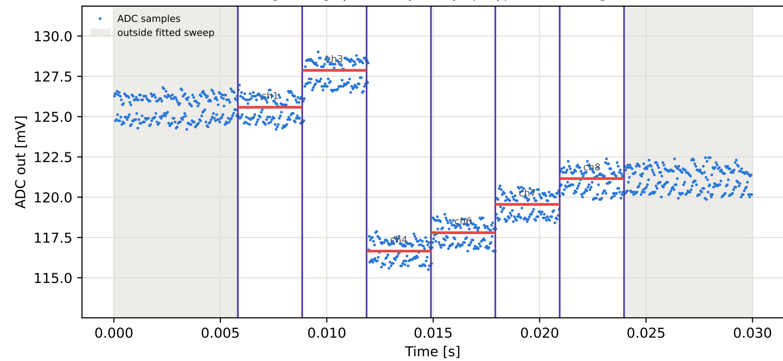
Tag8 &lt;- Tag10 | 785 MHz | run 0 | rep 1 | phase 25.92 deg
