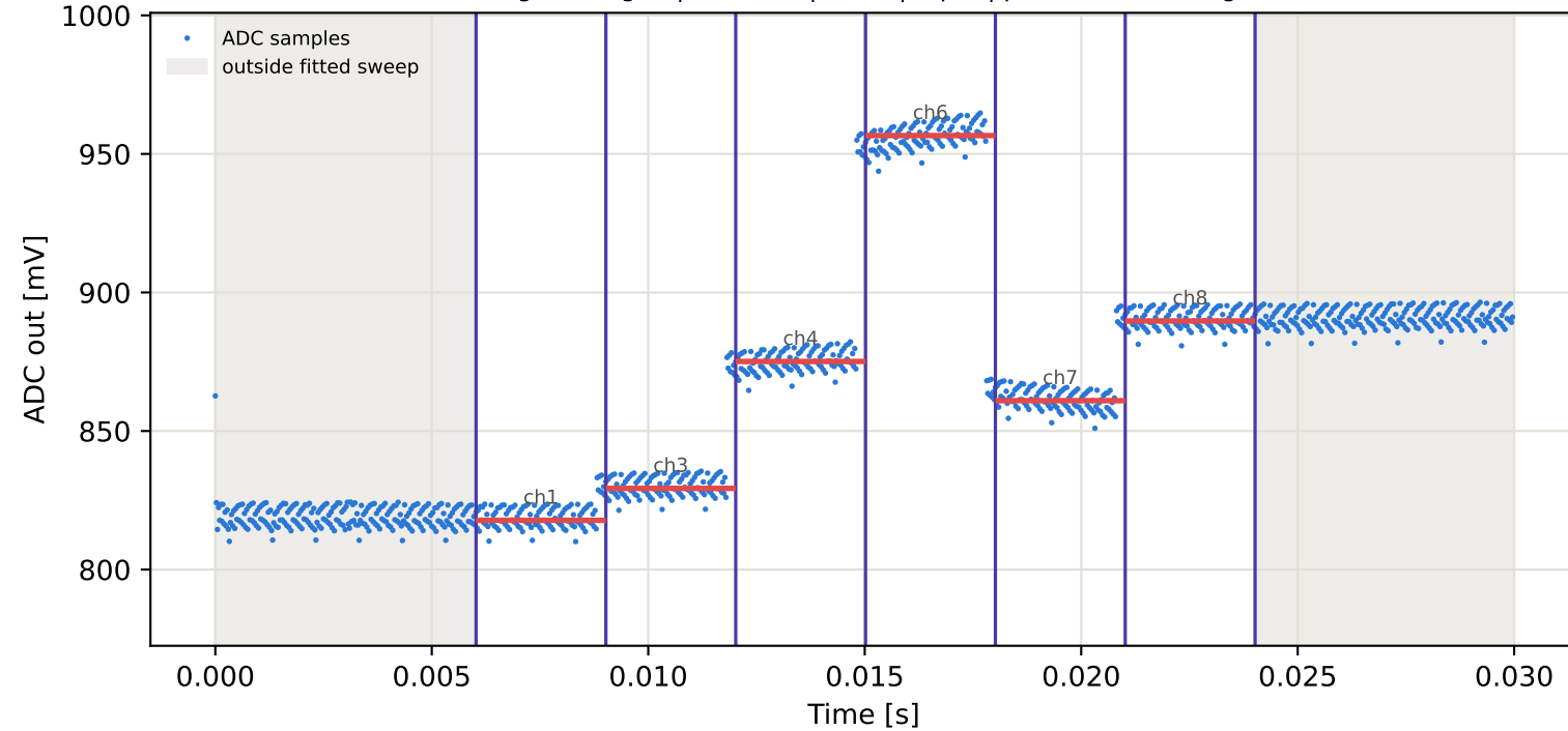
Tag3 &lt;- Tag16 | 895 MHz | run 0 | rep 1 | phase -145.01 deg
