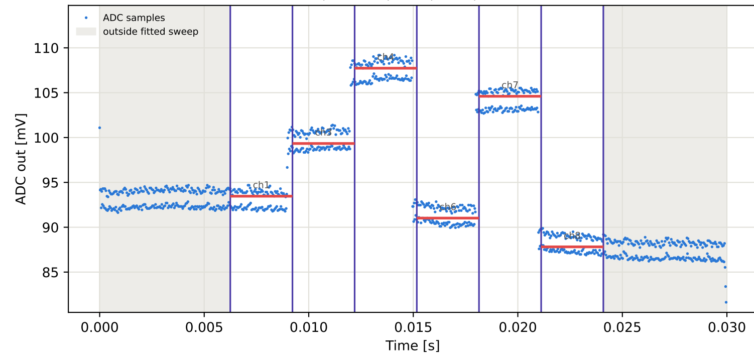
Tag1 &lt;- Tag3 | 945 MHz | run 0 | rep 1 | phase -67.42 deg
