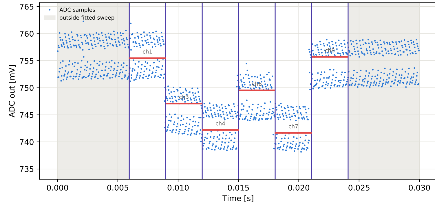
Tag3 &lt;- Tag16 | 855 MHz | run 0 | rep 1 | phase -159.66 deg
