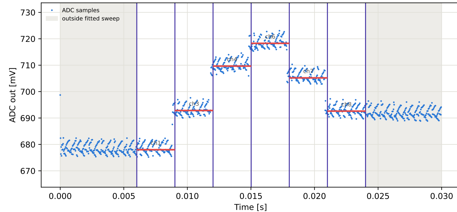
Tag4 &lt;- Tag2 | 895 MHz | run 0 | rep 1 | phase 179.16 deg
