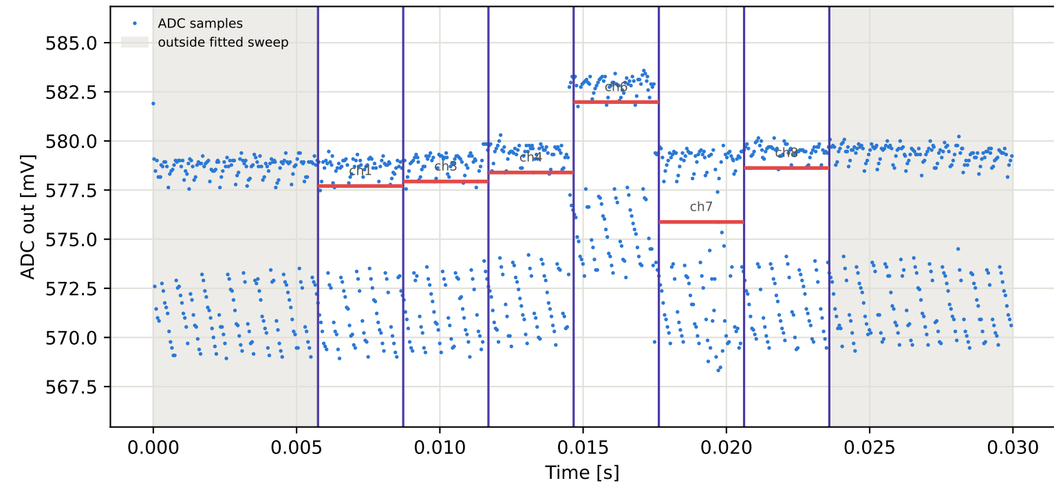
Tag5 &lt;- Tag4 | 955 MHz | run 0 | rep 1 | phase 81.27 deg
