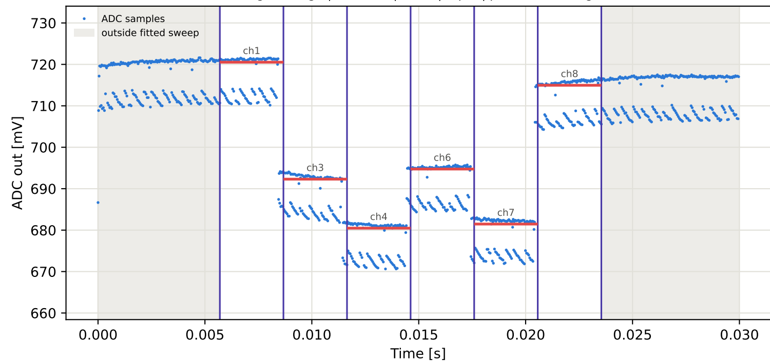
Tag8 &lt;- Tag1 | 865 MHz | run 0 | rep 1 | phase -132.92 deg
