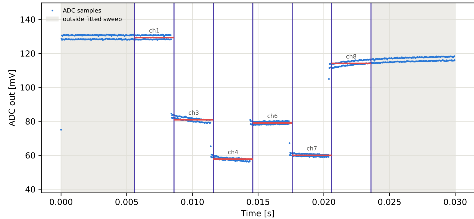
Tag10 &lt;- Tag5 | 855 MHz | run 0 | rep 1 | phase 76.51 deg
