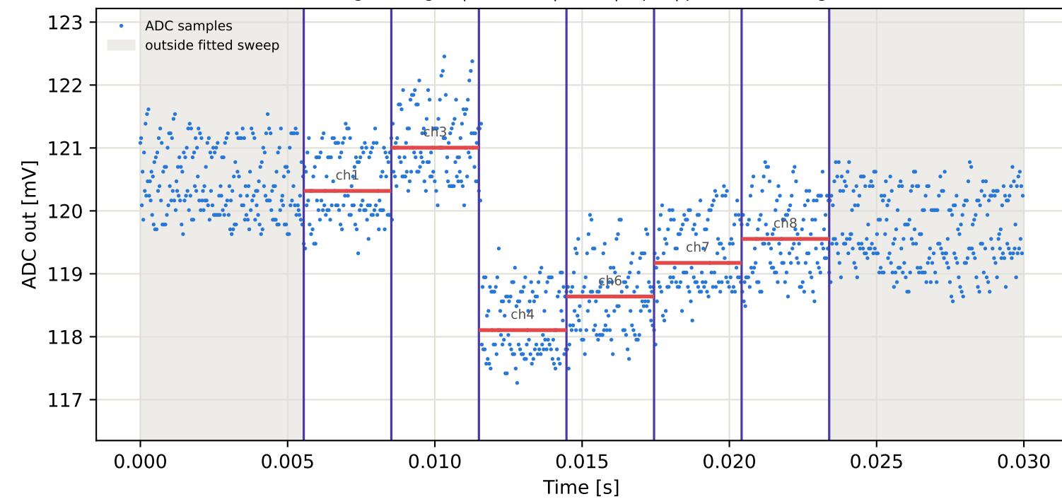
Tag7 &lt;- Tag3 | 785 MHz | run 0 | rep 1 | phase 138.24 deg
