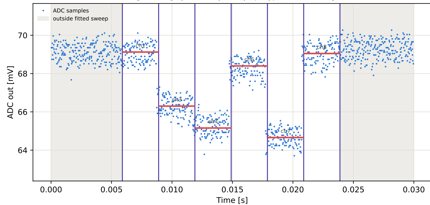
Tag10 &lt;- Tag9 | 785 MHz | run 0 | rep 1 | phase 168.50 deg
