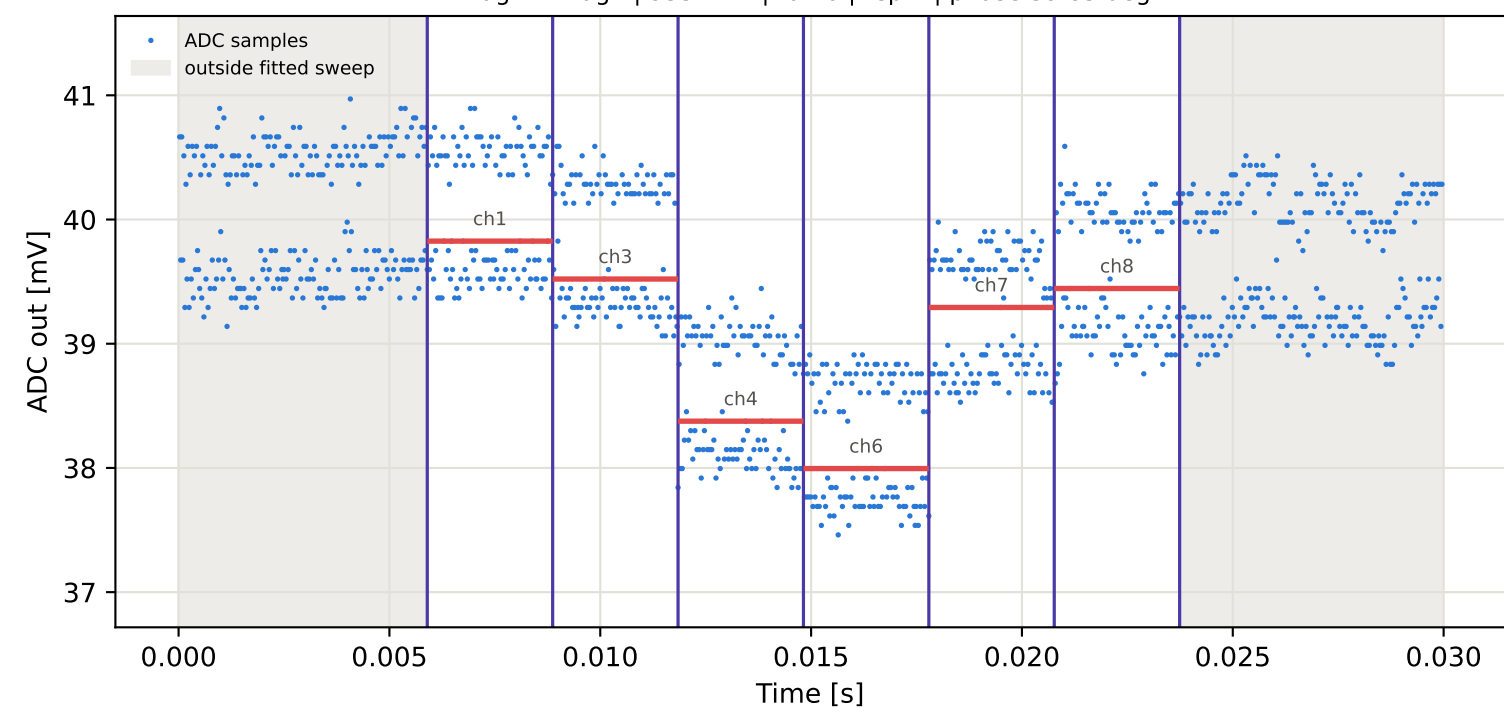
Tag2 &lt;- Tag6 | 955 MHz | run 0 | rep 1 | phase 167.27 deg
