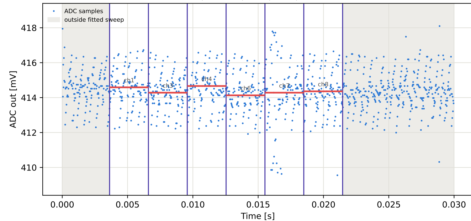
Tag4 &lt;- Tag2 | 965 MHz | run 0 | rep 1 | phase -47.19 deg
