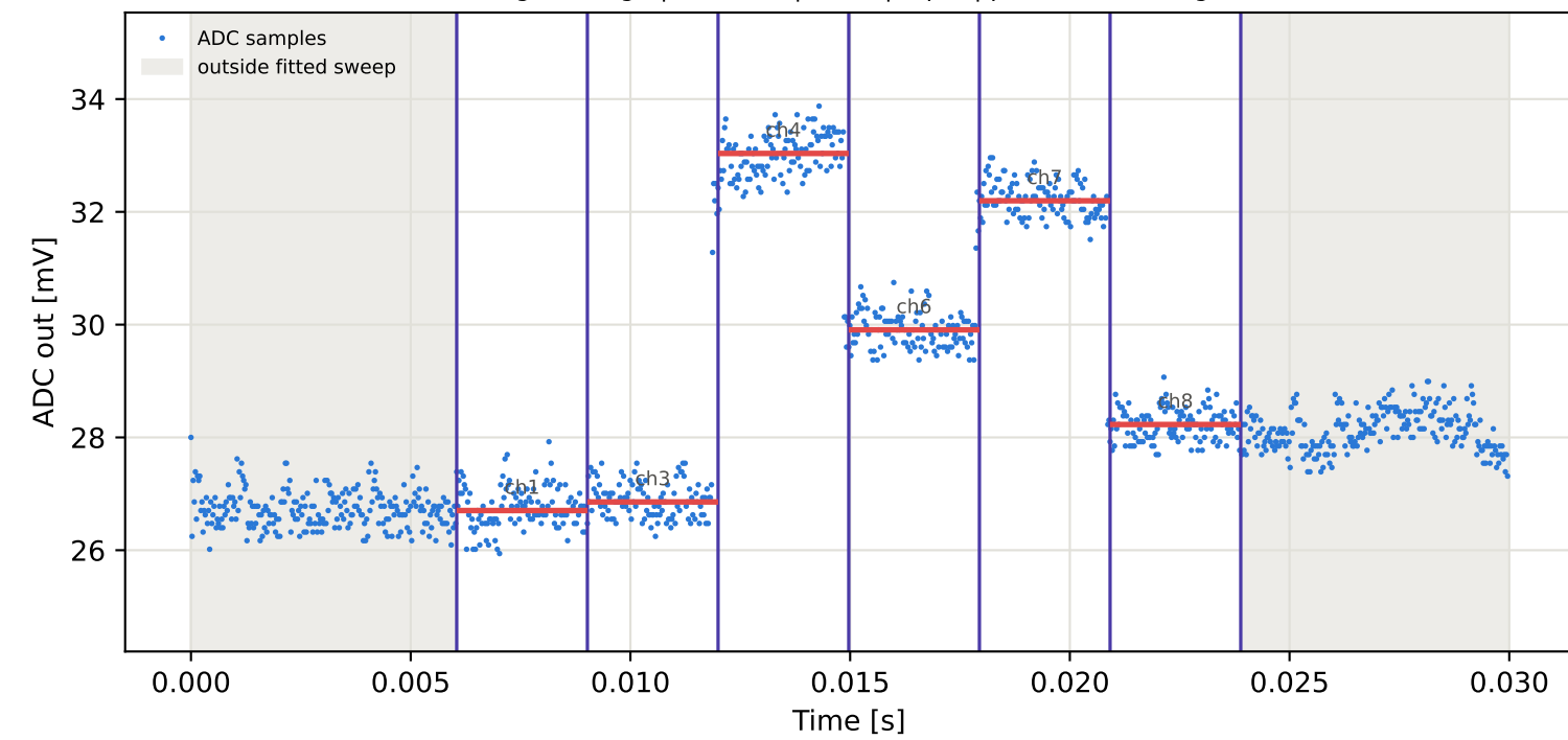
Tag7 &lt;- Tag1 | 775 MHz | run 0 | rep 1 | phase 75.84 deg
