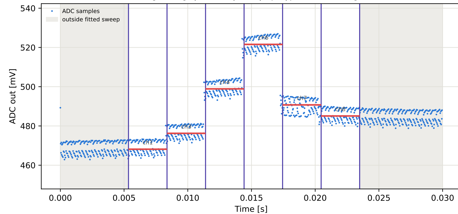
Tag3 &lt;- Tag6 | 915 MHz | run 0 | rep 1 | phase -131.52 deg
