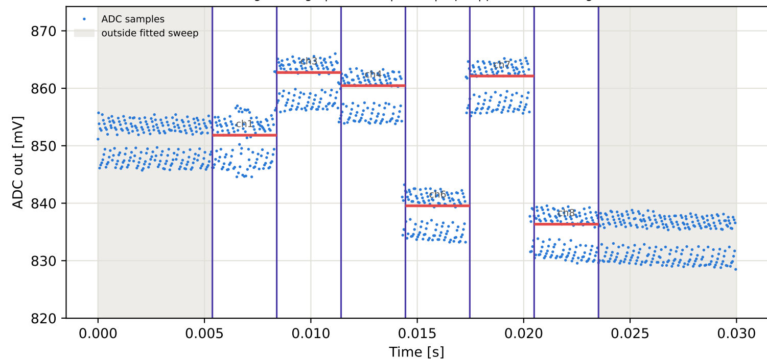
Tag3 &lt;- Tag2 | 865 MHz | run 0 | rep 1 | phase -20.96 deg
