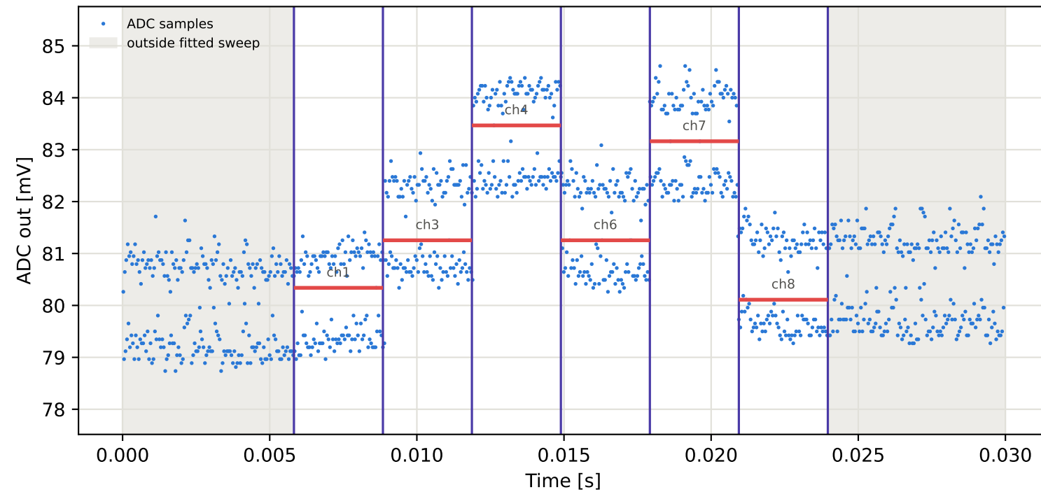
Tag16 &lt;- Tag10 | 795 MHz | run 0 | rep 1 | phase 42.09 deg
