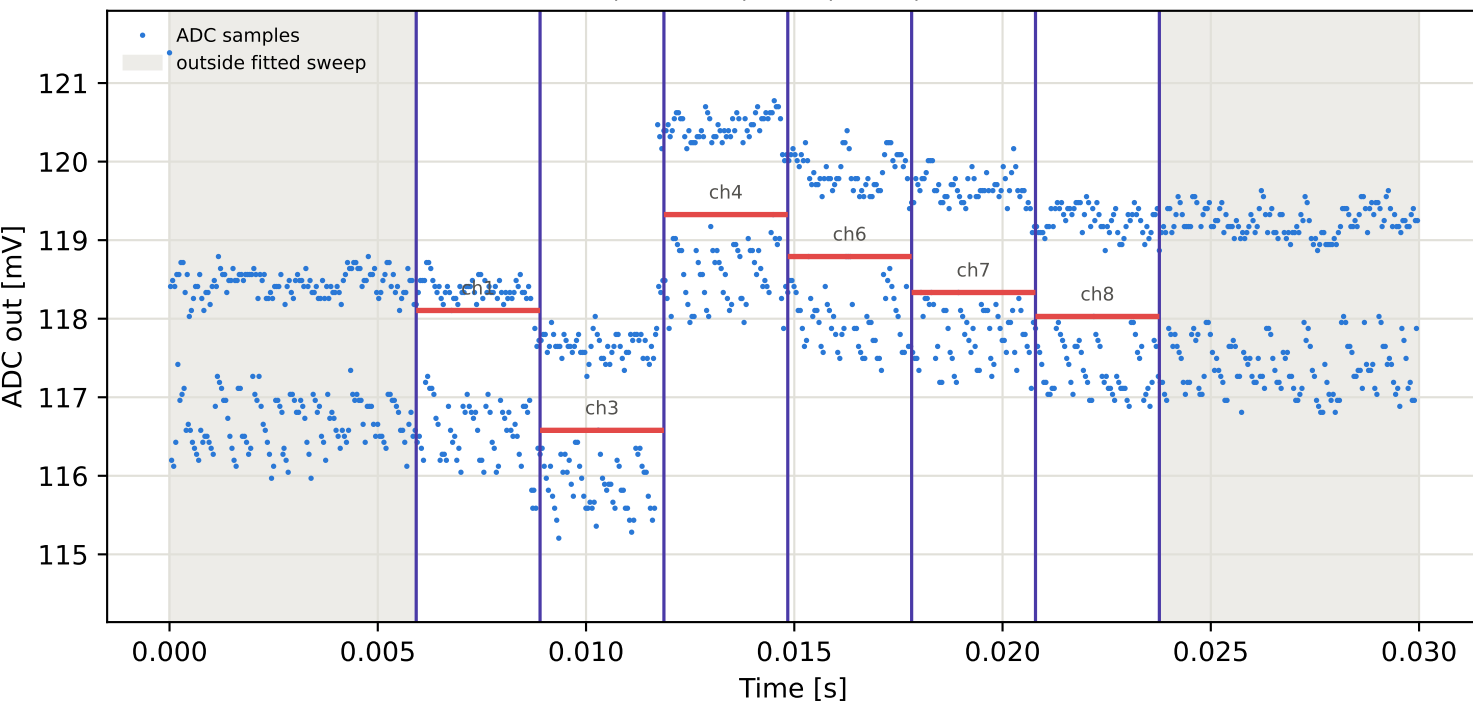
Tag7 &lt;- Tag10 | 785 MHz | run 0 | rep 1 | phase -120.12 deg
