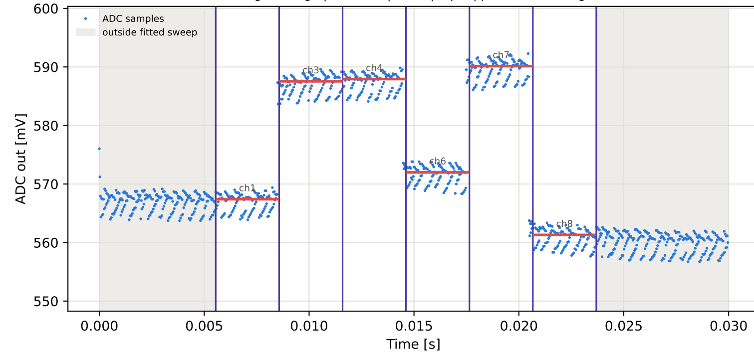
Tag6 &lt;- Tag1 | 865 MHz | run 0 | rep 1 | phase -54.33 deg
