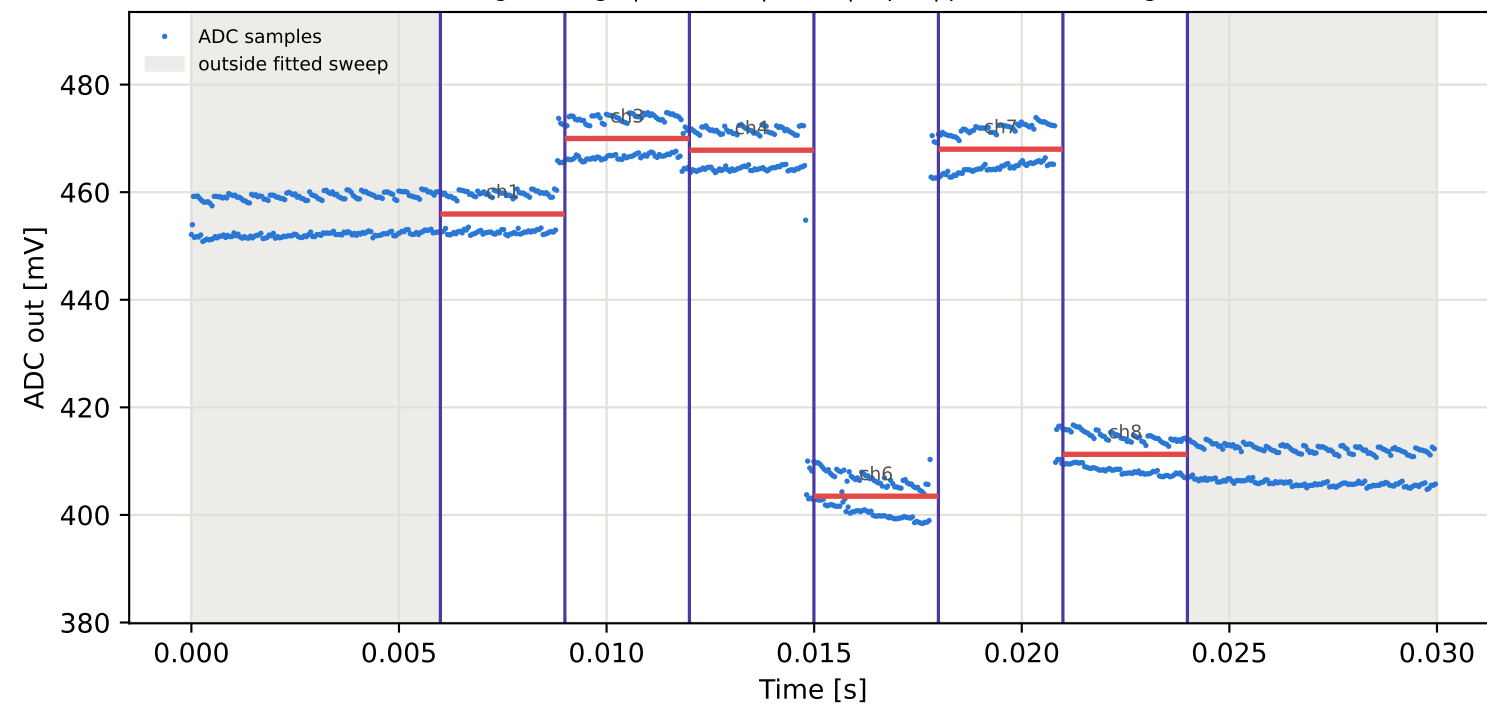
Tag8 &lt;- Tag1 | 905 MHz | run 0 | rep 1 | phase 128.98 deg
