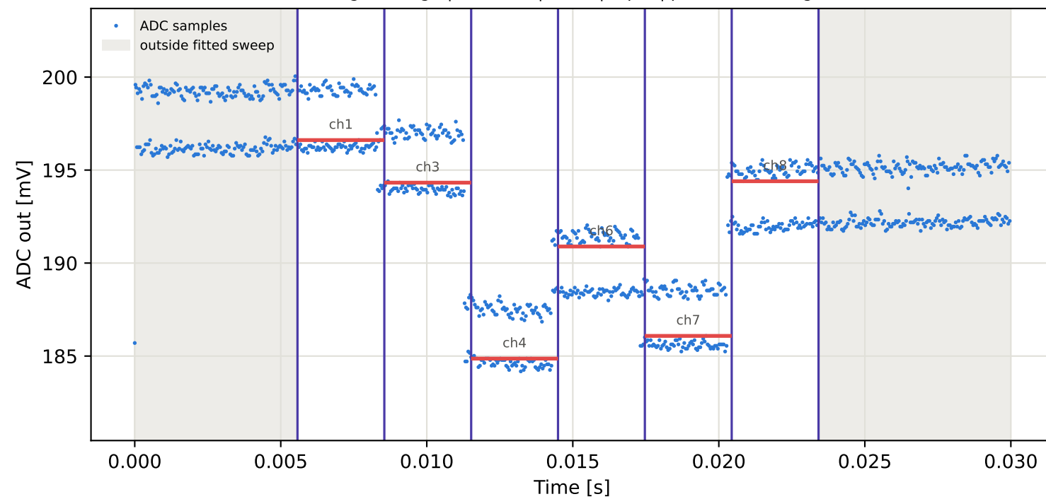
Tag4 &lt;- Tag15 | 835 MHz | run 0 | rep 1 | phase -141.85 deg
