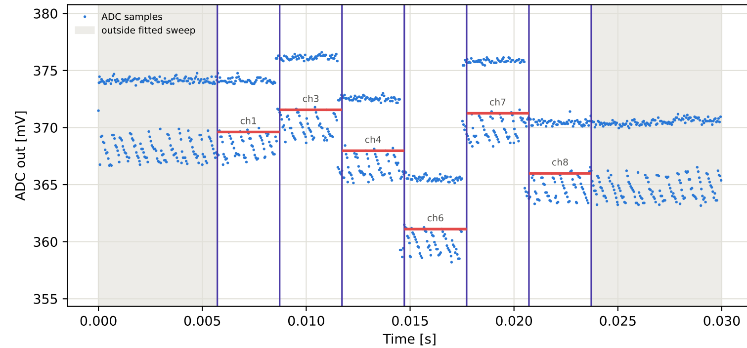
Tag15 &lt;- Tag5 | 995 MHz | run 0 | rep 1 | phase -77.02 deg
