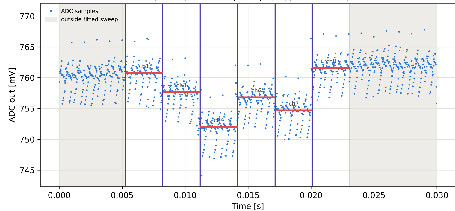
Tag7 &lt;- Tag6 | 945 MHz | run 0 | rep 1 | phase -92.25 deg
