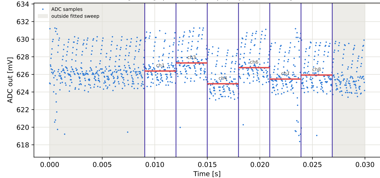
Tag7 &lt;- Tag4 | 985 MHz | run 0 | rep 1 | phase -84.31 deg
