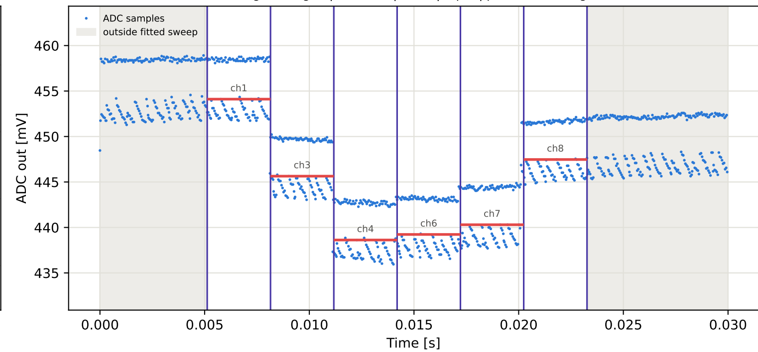
Tag2 &lt;- Tag16 | 865 MHz | run 0 | rep 1 | phase 115.94 deg
