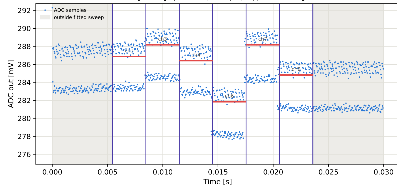
Tag3 &lt;- Tag6 | 985 MHz | run 0 | rep 1 | phase 2.78 deg
