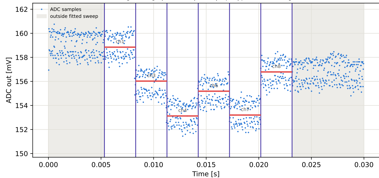
Tag10 &lt;- Tag1 | 835 MHz | run 0 | rep 1 | phase 66.09 deg
