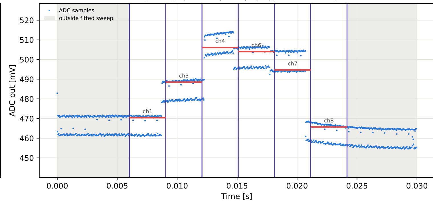
Tag3 &lt;- Tag7 | 915 MHz | run 0 | rep 1 | phase -173.82 deg
