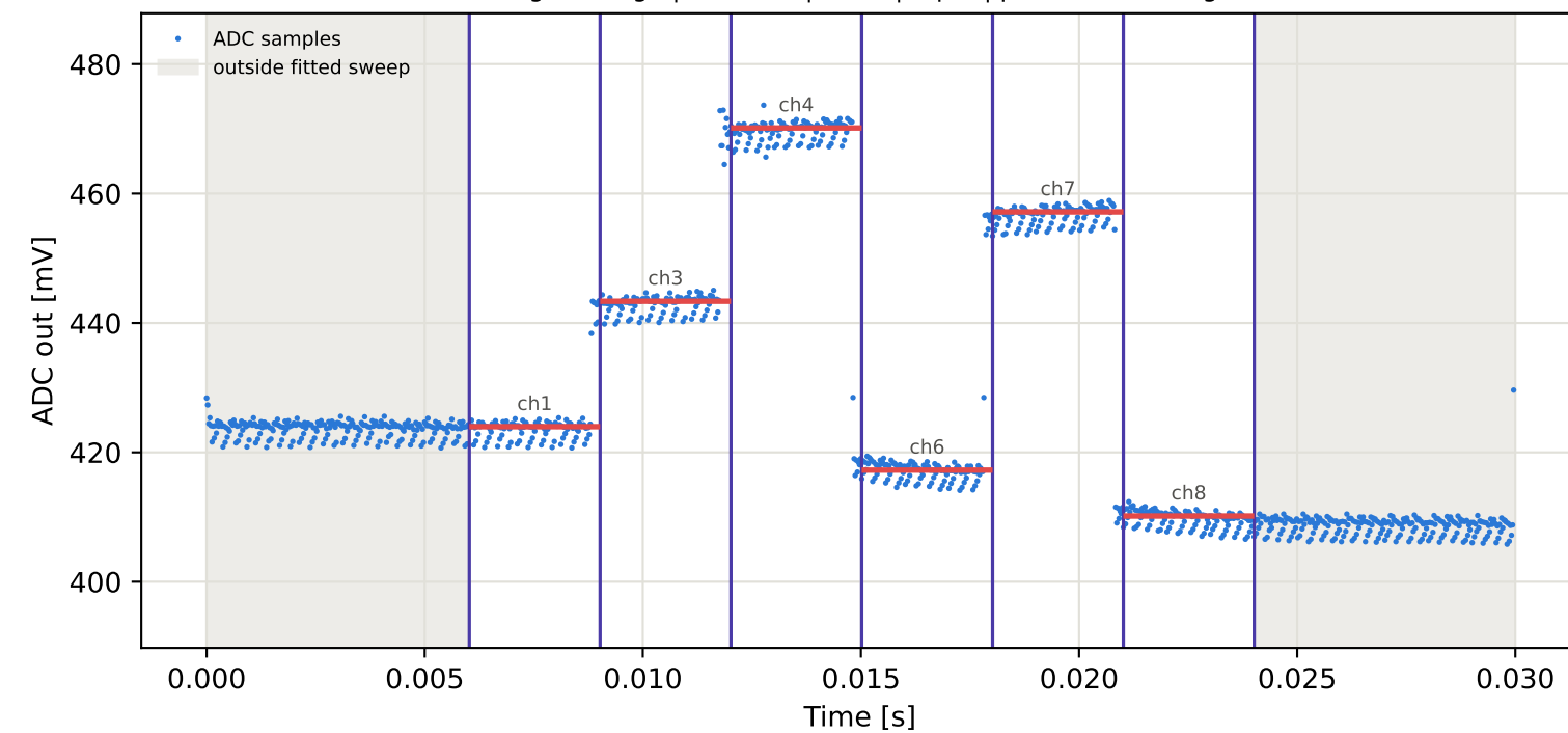
Tag3 &lt;- Tag8 | 945 MHz | run 0 | rep 1 | phase -69.11 deg
