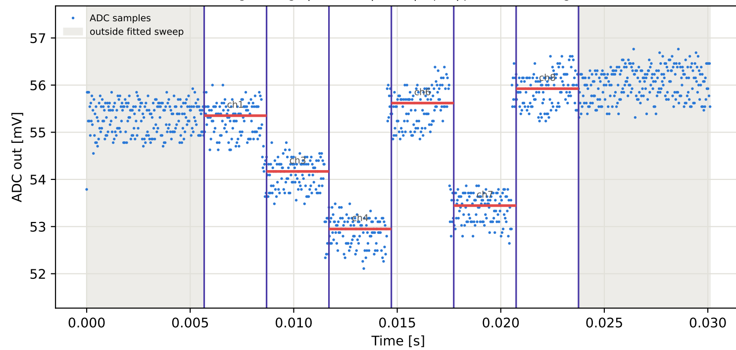
Tag3 &lt;- Tag10 | 975 MHz | run 0 | rep 1 | phase 62.20 deg
