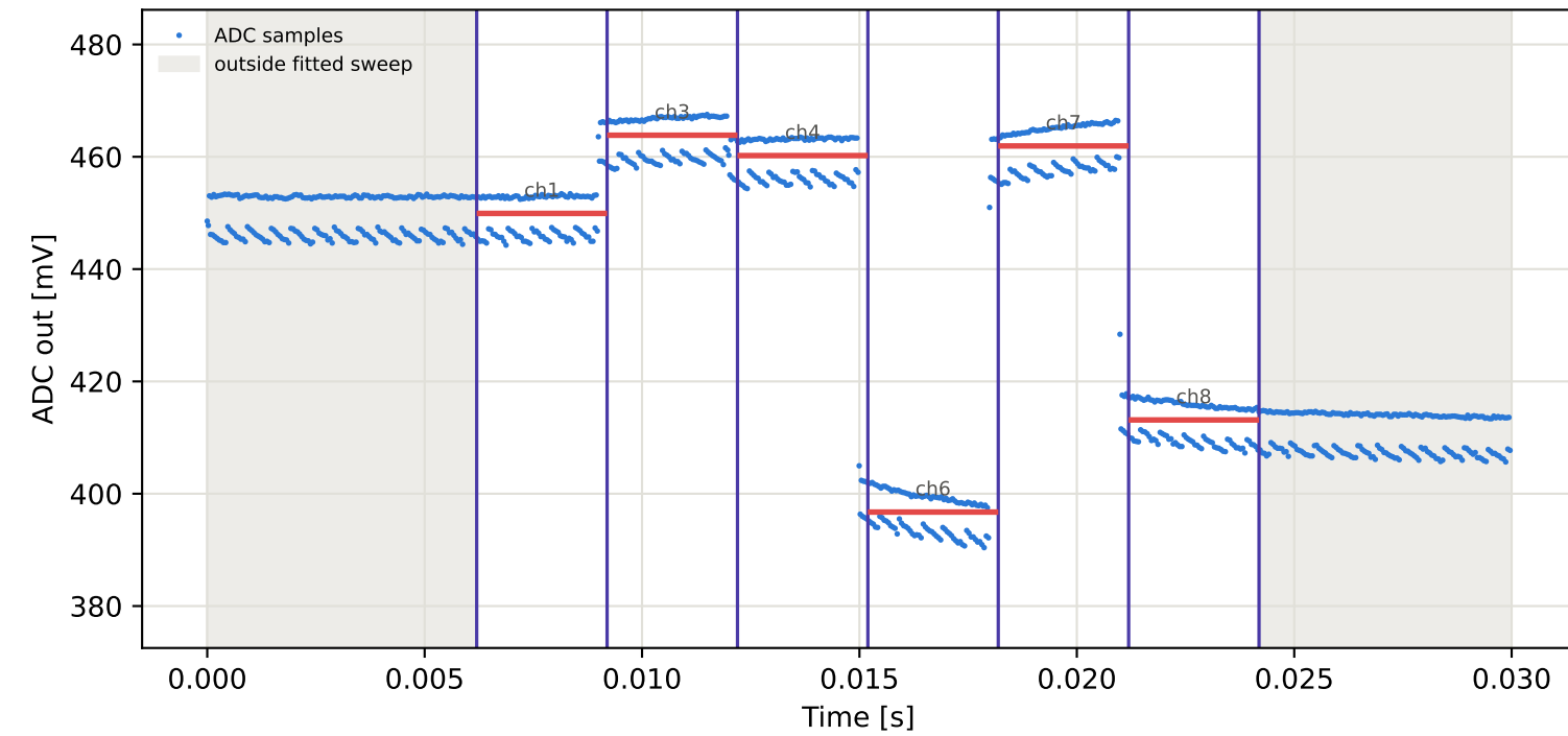
Tag7 &lt;- Tag5 | 905 MHz | run 0 | rep 1 | phase -26.44 deg
