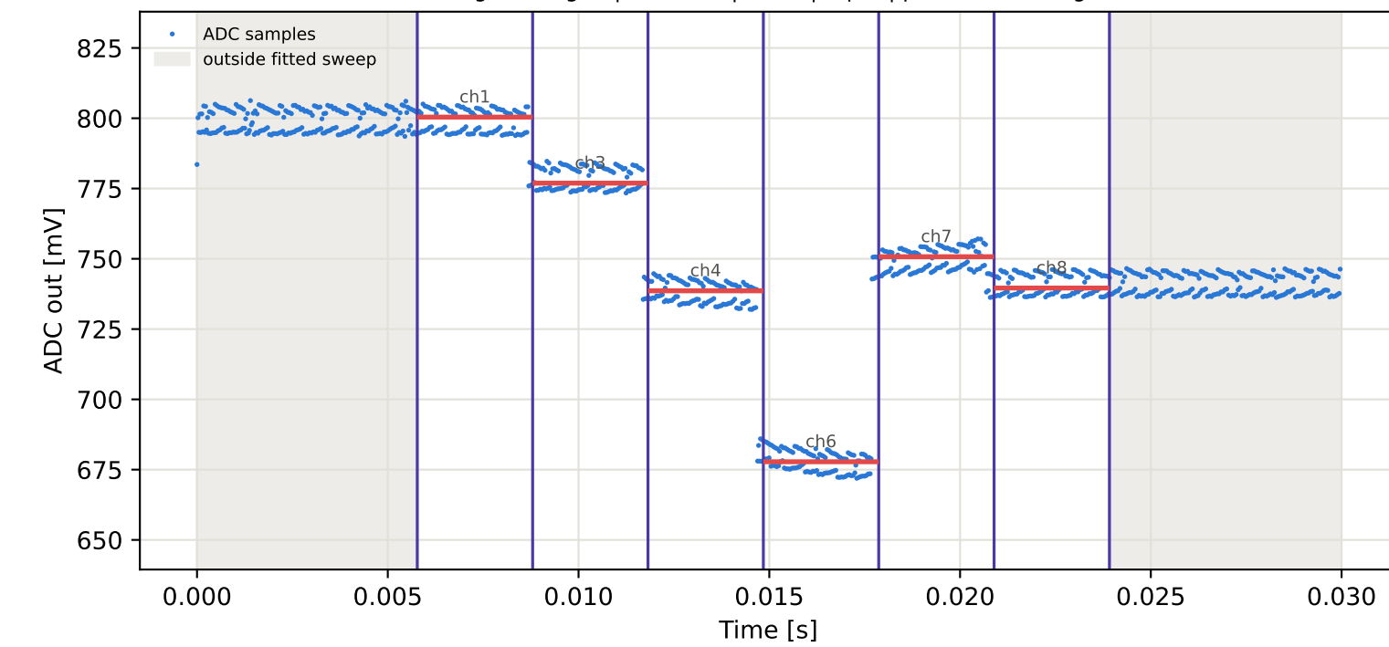
Tag9 &lt;- Tag16 | 895 MHz | run 0 | rep 1 | phase 33.33 deg
