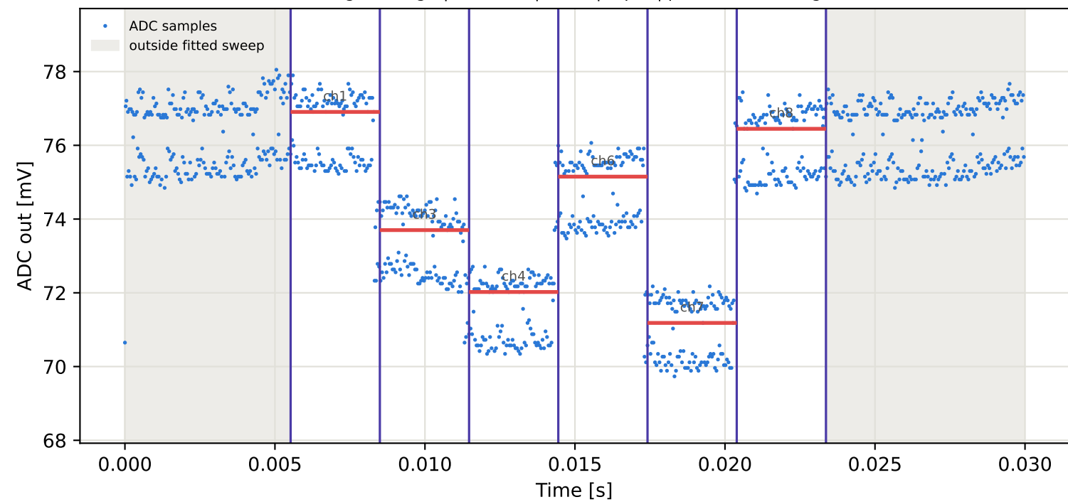
Tag9 &lt;- Tag15 | 835 MHz | run 0 | rep 1 | phase 108.10 deg
