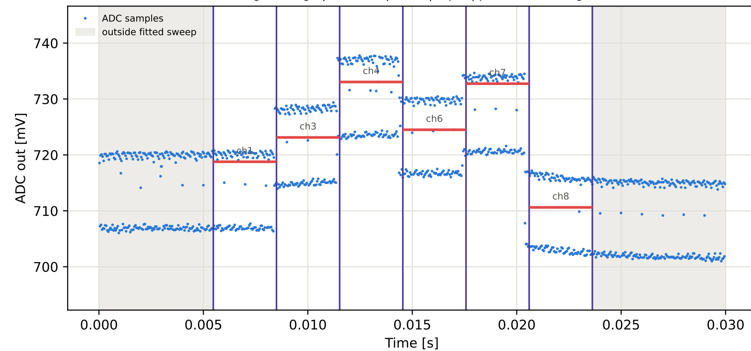
Tag3 &lt;- Tag8 | 905 MHz | run 0 | rep 1 | phase -124.01 deg
