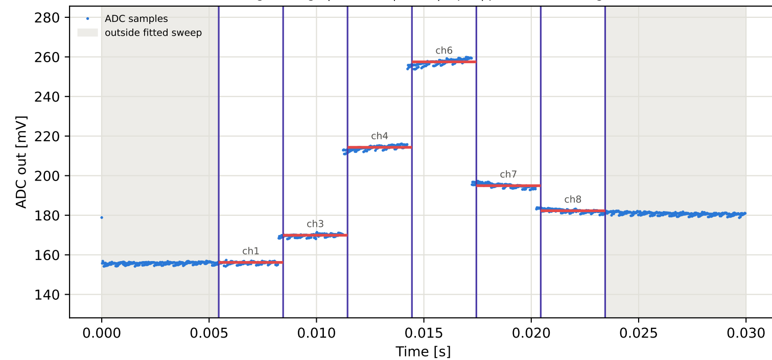
Tag4 &lt;- Tag7 | 925 MHz | run 0 | rep 1 | phase 176.32 deg
