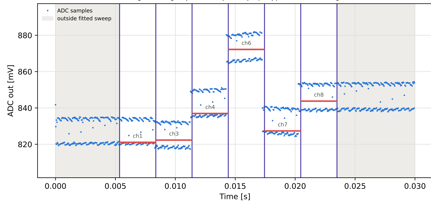
Tag16 &lt;- Tag15 | 955 MHz | run 0 | rep 1 | phase -162.48 deg
