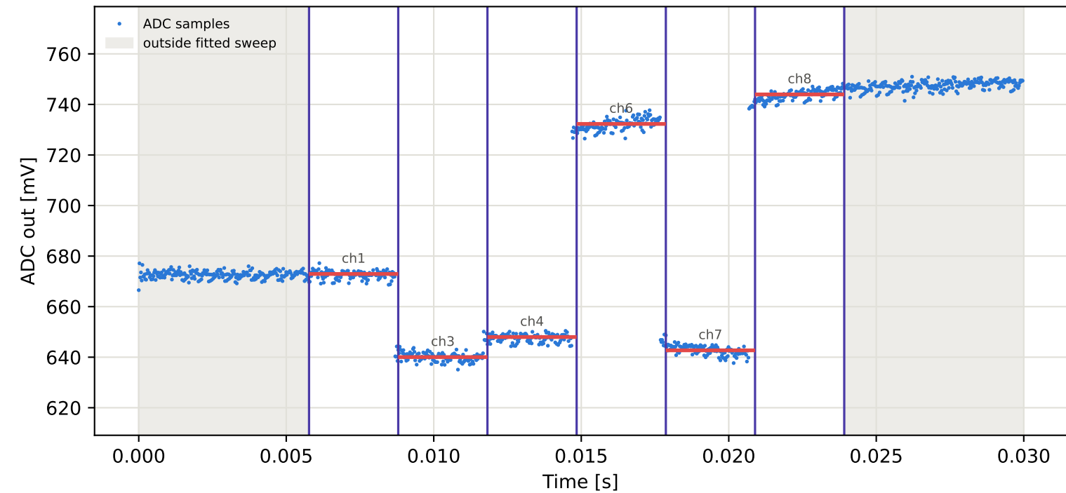
Tag10 &lt;- Tag5 | 885 MHz | run 0 | rep 1 | phase 117.24 deg
