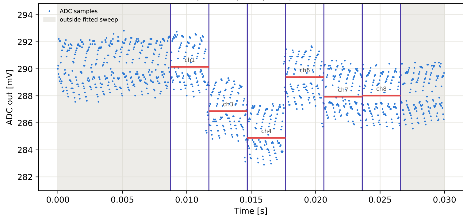
Tag9 &lt;- Tag15 | 995 MHz | run 0 | rep 1 | phase -8.51 deg
