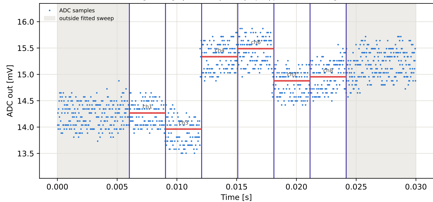
Tag3 &lt;- Tag10 | 795 MHz | run 0 | rep 1 | phase 67.18 deg
