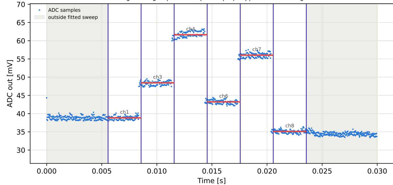
Tag6 &lt;- Tag3 | 945 MHz | run 0 | rep 1 | phase -30.07 deg
