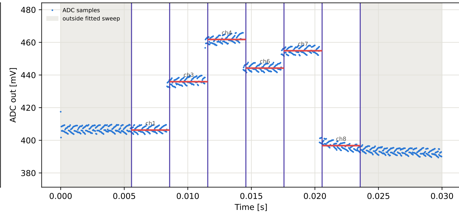
Tag6 &lt;- Tag5 | 895 MHz | run 0 | rep 1 | phase 144.71 deg
