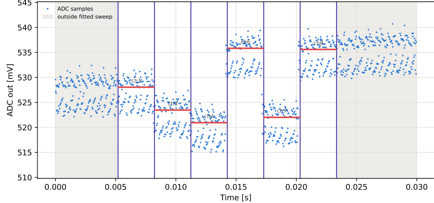
Tag2 &lt;- Tag8 | 915 MHz | run 0 | rep 1 | phase 147.27 deg
