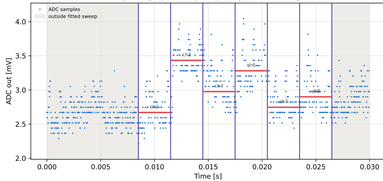
Tag1 &lt;- Tag16 | 785 MHz | run 0 | rep 1 | phase 138.54 deg
