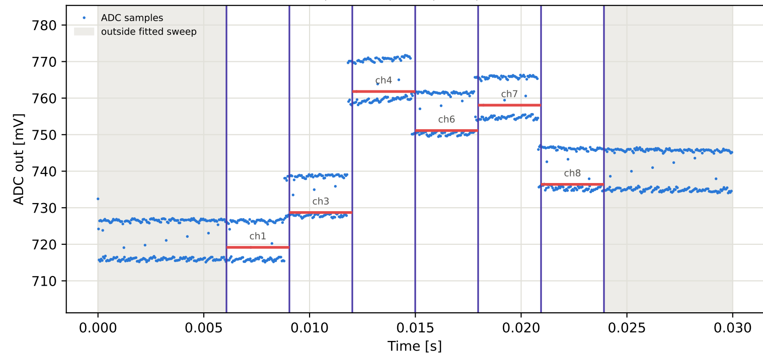
Tag8 &lt;- Tag16 | 835 MHz | run 0 | rep 1 | phase -107.51 deg
