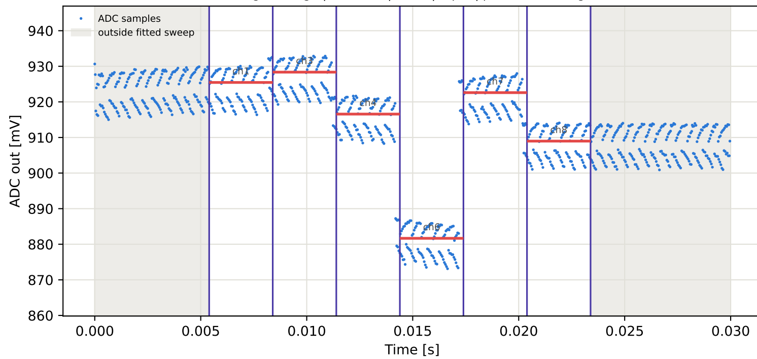
Tag5 &lt;- Tag8 | 925 MHz | run 0 | rep 1 | phase -64.03 deg
