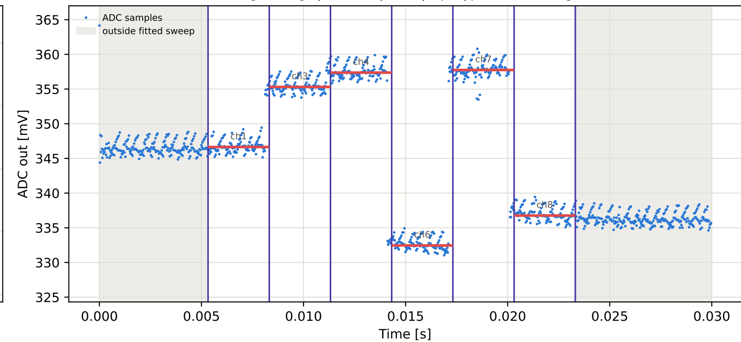
Tag5 &lt;- Tag9 | 965 MHz | run 0 | rep 1 | phase -20.81 deg
