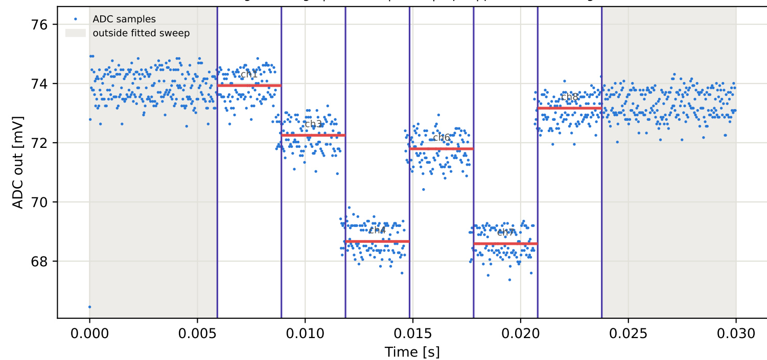
Tag16 &lt;- Tag7 | 775 MHz | run 0 | rep 1 | phase 100.24 deg
