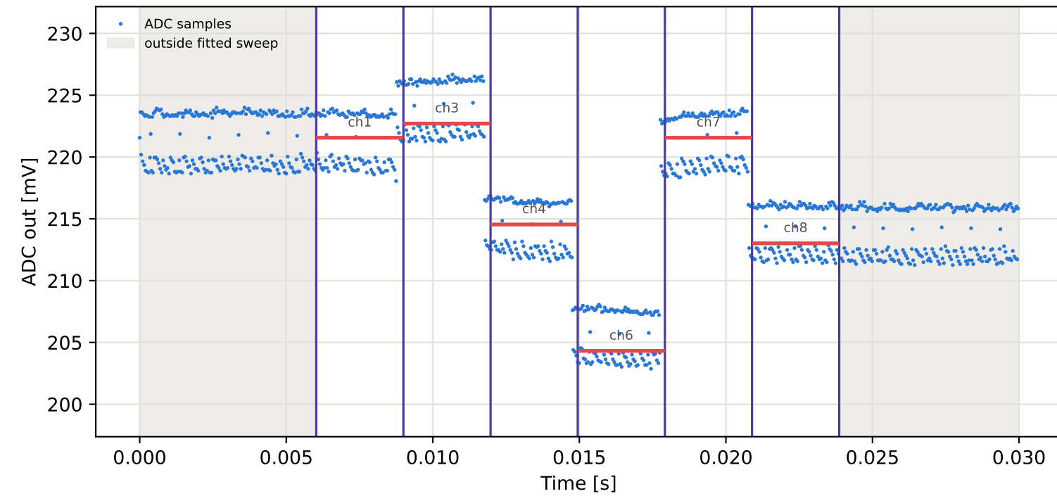
Tag1 &lt;- Tag3 | 985 MHz | run 0 | rep 1 | phase 52.47 deg
