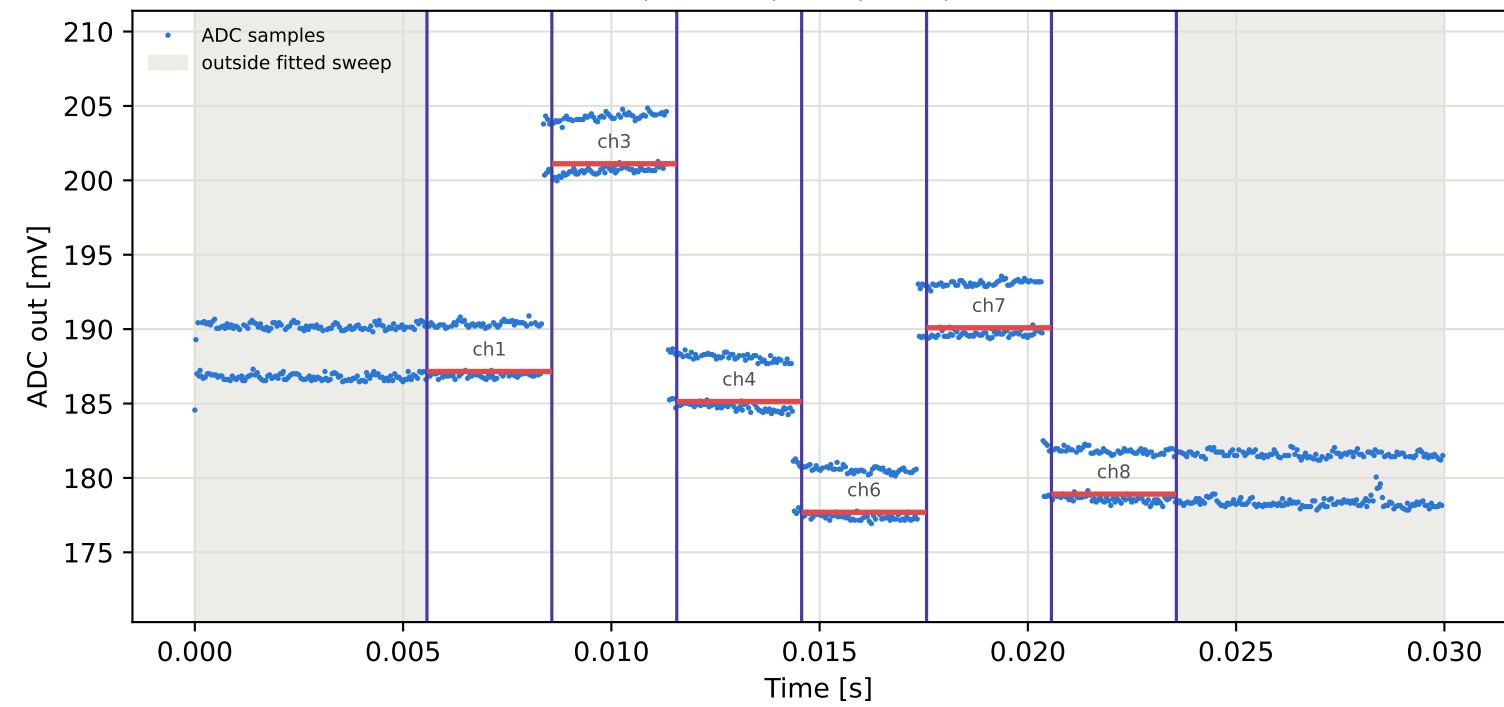
Tag4 &lt;- Tag3 | 825 MHz | run 0 | rep 1 | phase 19.94 deg
