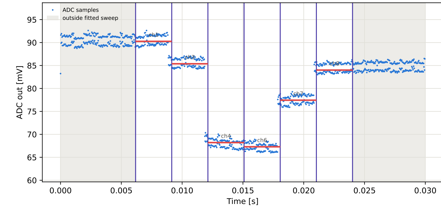
Tag7 &lt;- Tag10 | 955 MHz | run 0 | rep 1 | phase -30.10 deg
