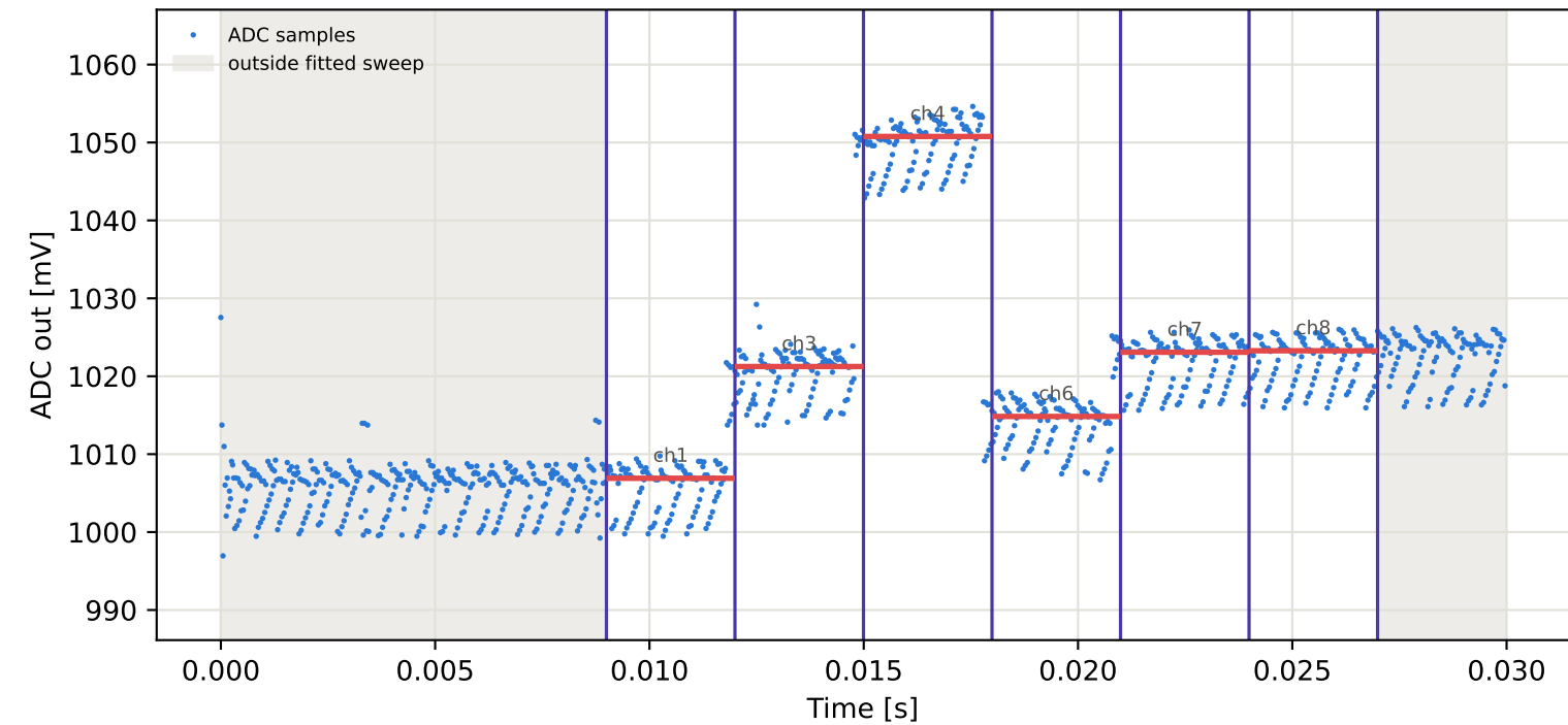
Tag10 &lt;- Tag5 | 925 MHz | run 0 | rep 1 | phase -158.78 deg
