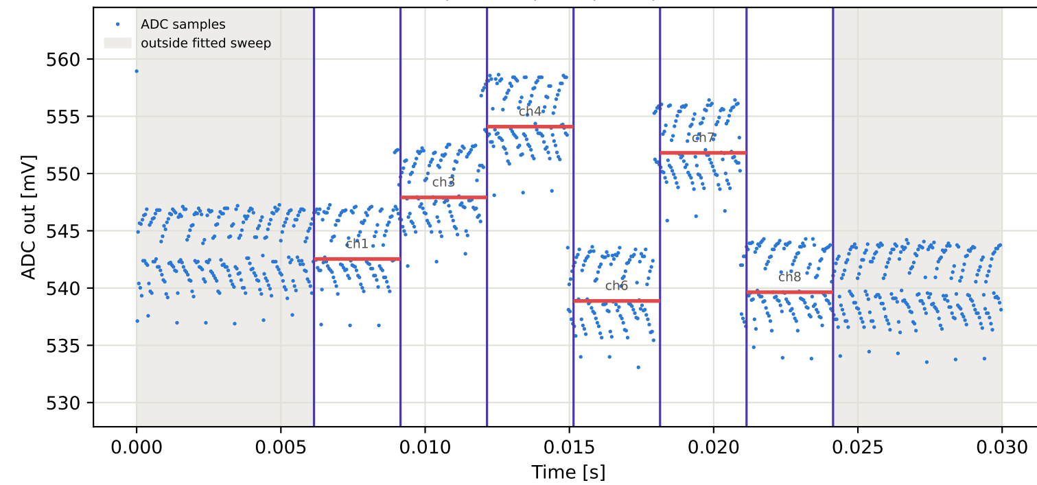
Tag8 &lt;- Tag6 | 995 MHz | run 0 | rep 1 | phase -64.18 deg
