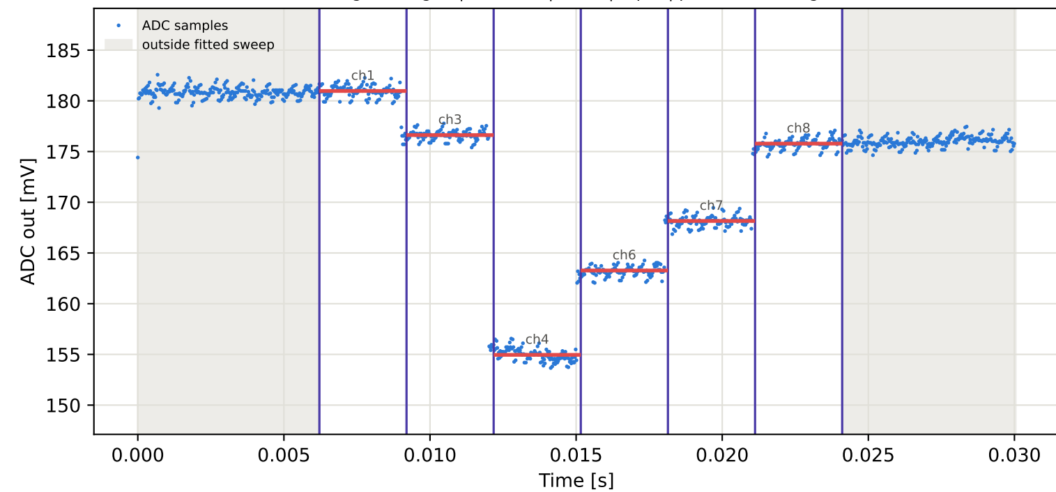
Tag5 &lt;- Tag2 | 995 MHz | run 0 | rep 1 | phase 78.46 deg
