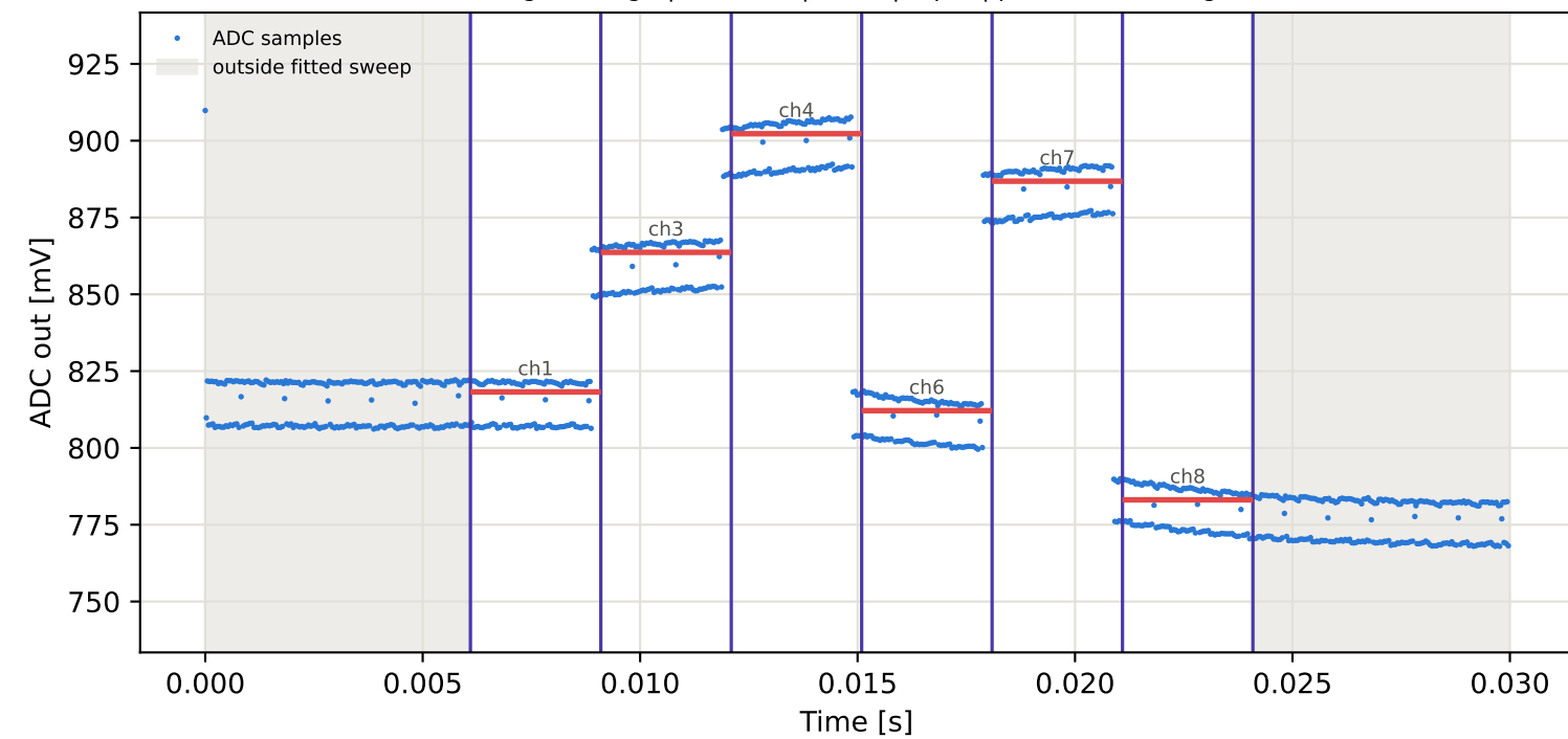
Tag8 &lt;- Tag10 | 935 MHz | run 0 | rep 1 | phase -94.17 deg
