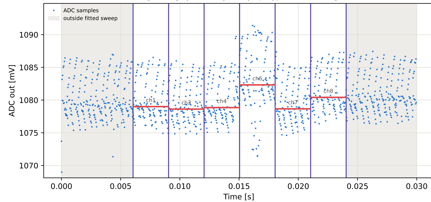
Tag8 &lt;- Tag4 | 935 MHz | run 0 | rep 1 | phase 51.80 deg
