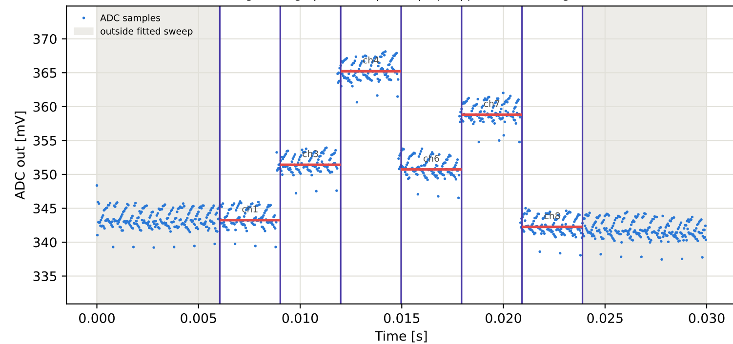
Tag4 &lt;- Tag9 | 955 MHz | run 0 | rep 1 | phase 92.61 deg
