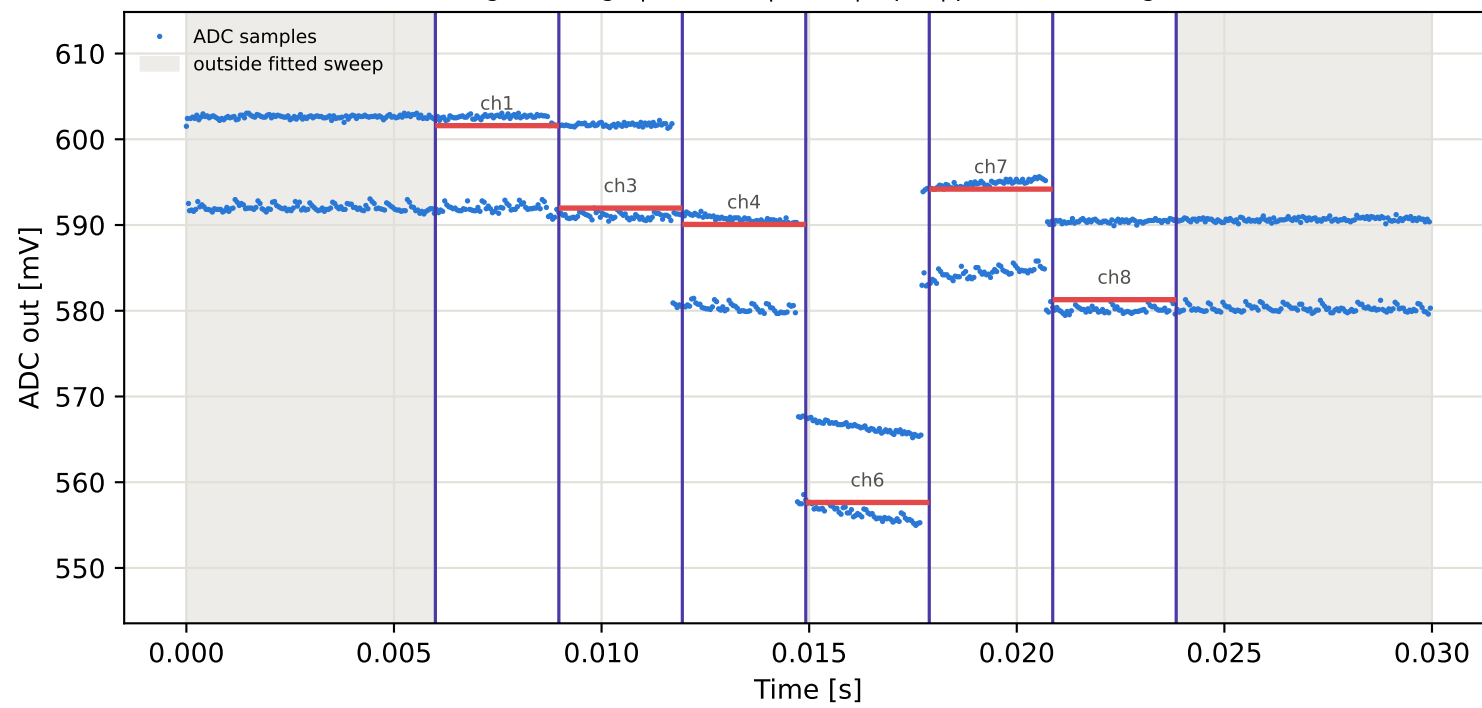
Tag10 &lt;- Tag8 | 915 MHz | run 0 | rep 1 | phase 96.40 deg
