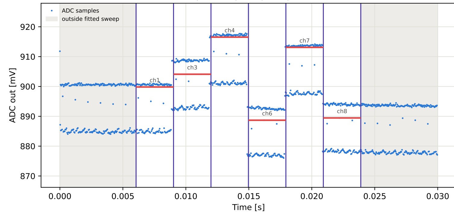
Tag8 &lt;- Tag15 | 985 MHz | run 0 | rep 1 | phase -55.58 deg
