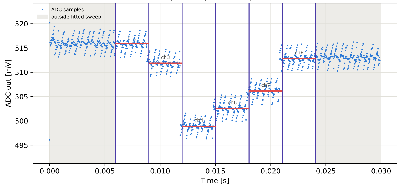
Tag5 &lt;- Tag2 | 975 MHz | run 0 | rep 1 | phase -106.13 deg
