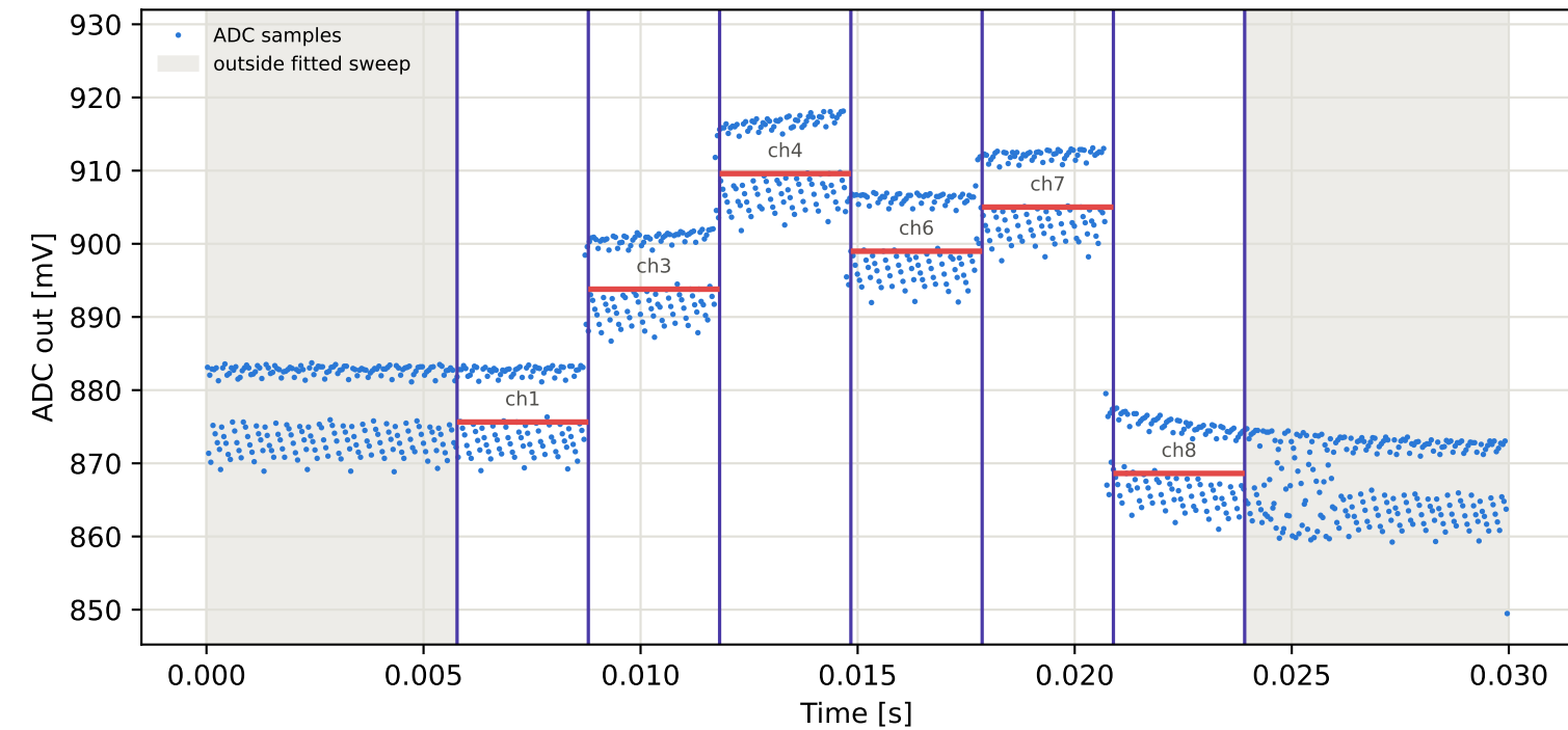
Tag3 &lt;- Tag8 | 895 MHz | run 0 | rep 1 | phase -145.22 deg
