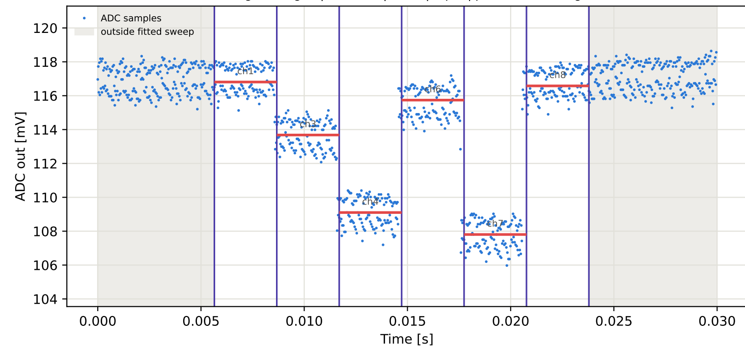
Tag4 &lt;- Tag2 | 775 MHz | run 0 | rep 1 | phase -87.84 deg
