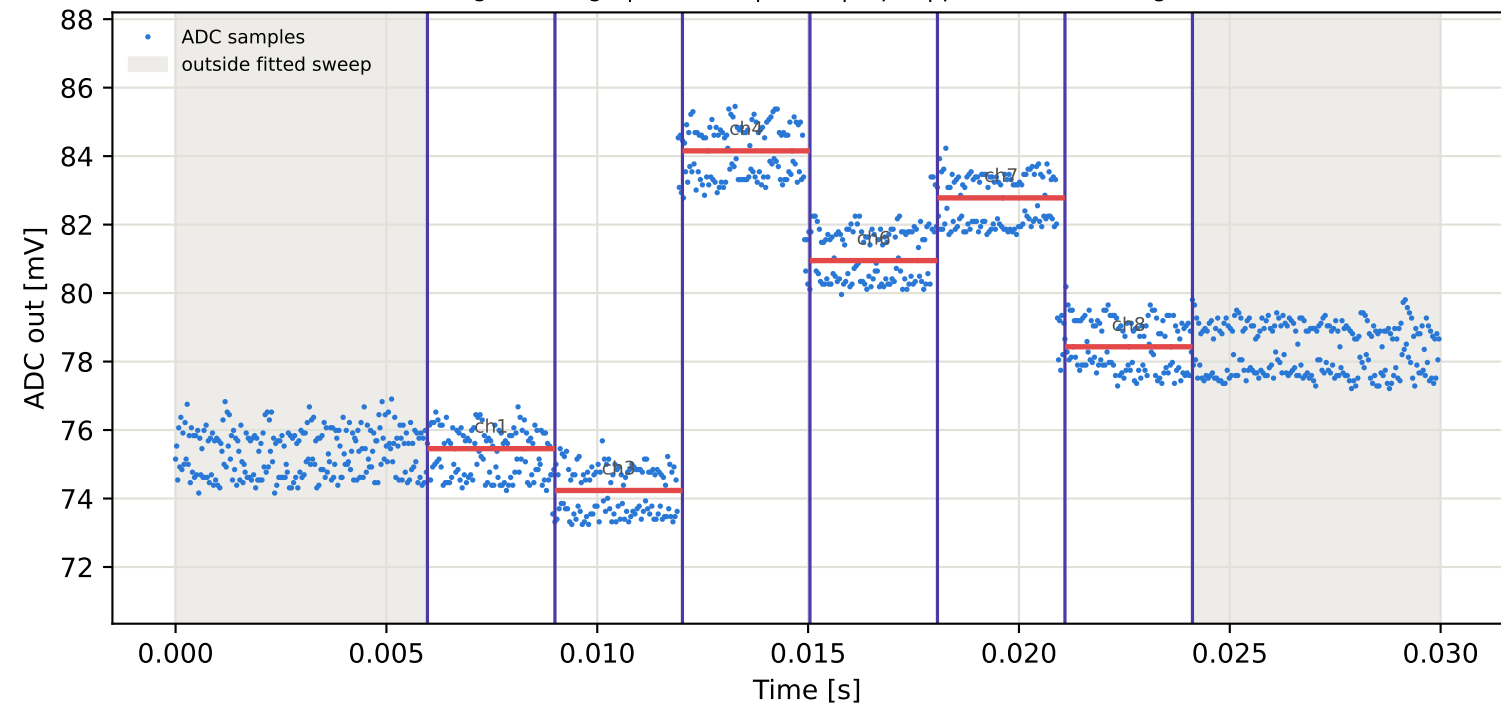
Tag15 &lt;- Tag6 | 795 MHz | run 0 | rep 1 | phase 13.27 deg
