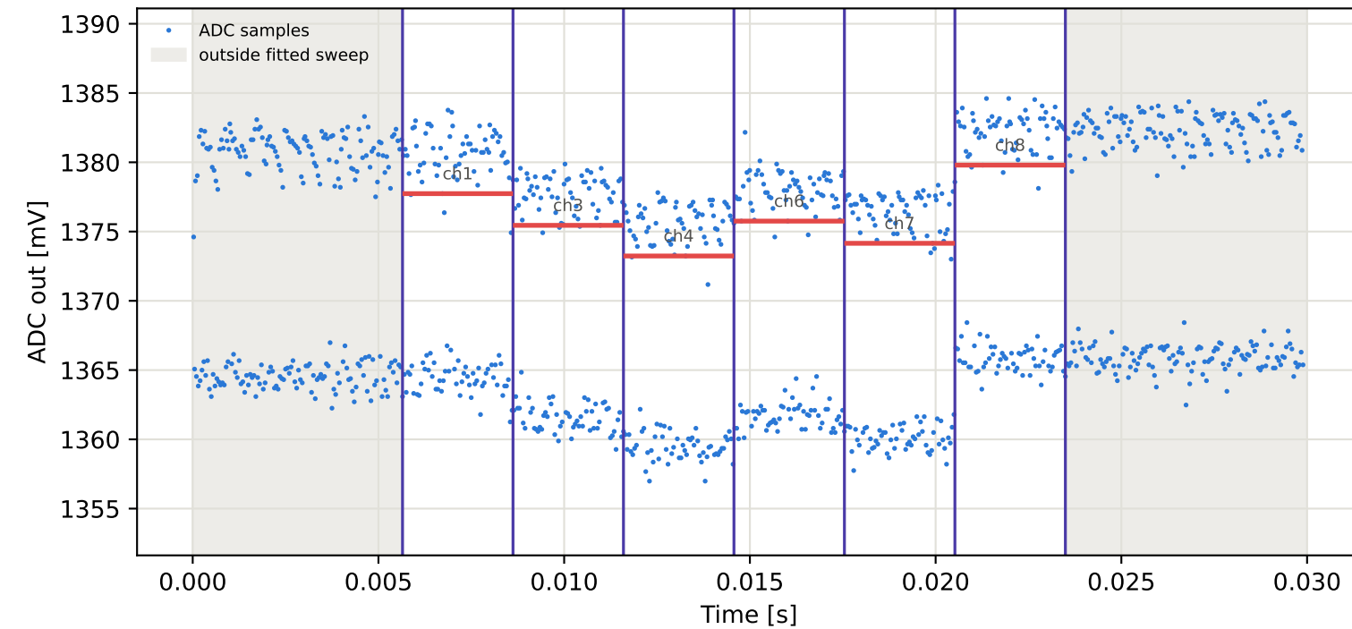
Tag16 &lt;- Tag6 | 885 MHz | run 0 | rep 1 | phase 52.19 deg
