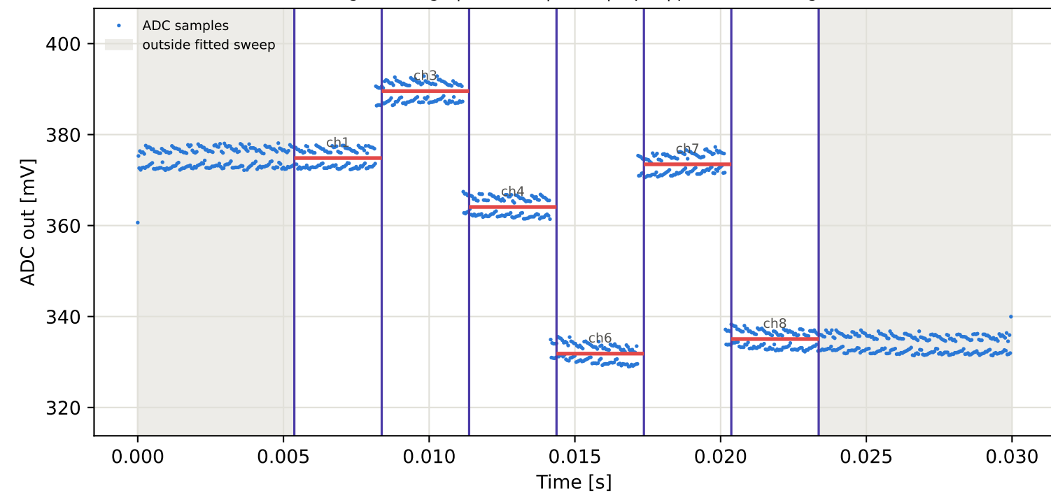
Tag16 &lt;- Tag1 | 855 MHz | run 0 | rep 1 | phase 13.49 deg
