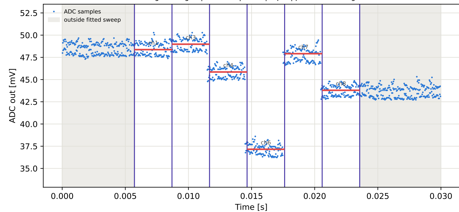
Tag6 &lt;- Tag2 | 945 MHz | run 0 | rep 1 | phase 170.61 deg
