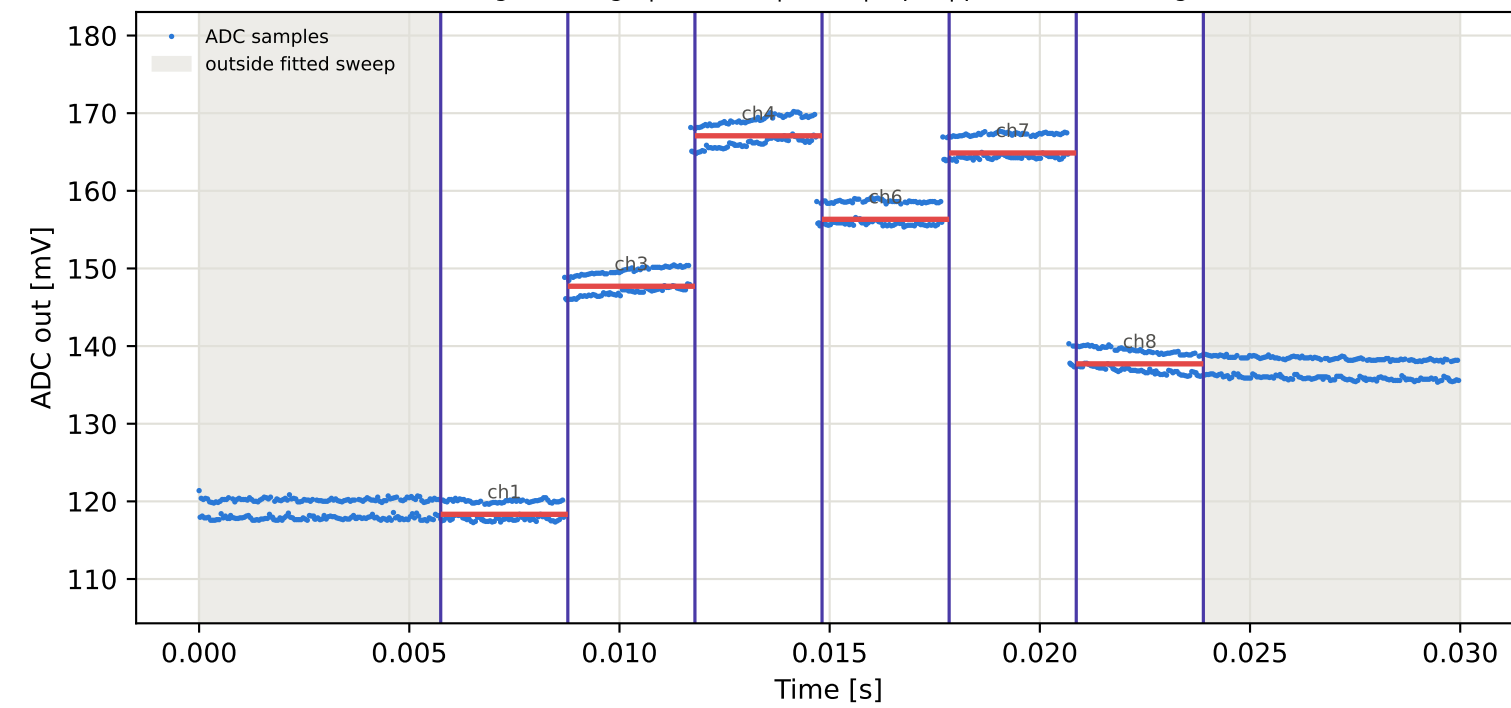
Tag10 &lt;- Tag8 | 845 MHz | run 0 | rep 1 | phase -25.14 deg
