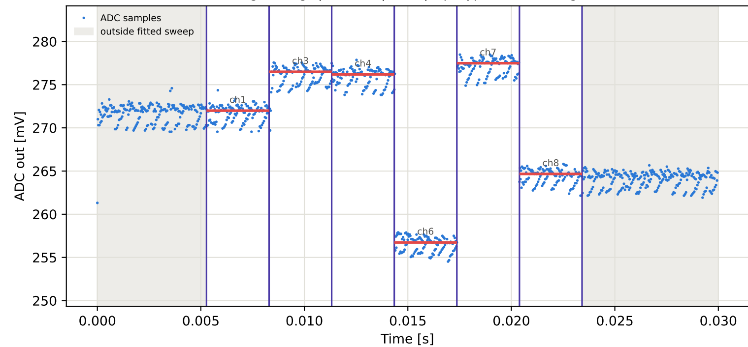
Tag9 &lt;- Tag6 | 975 MHz | run 0 | rep 1 | phase -125.72 deg
