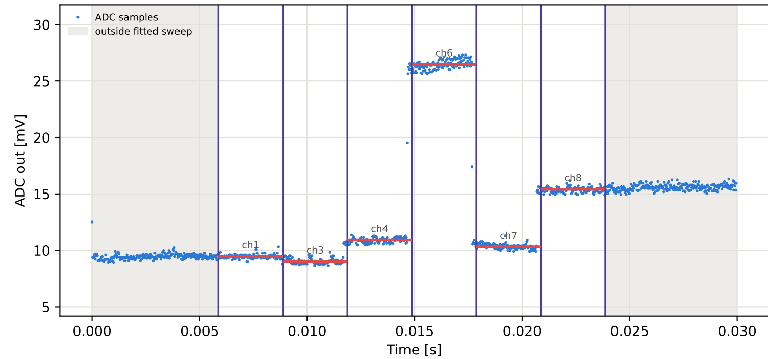
Tag1 &lt;- Tag4 | 905 MHz | run 0 | rep 1 | phase -155.74 deg
