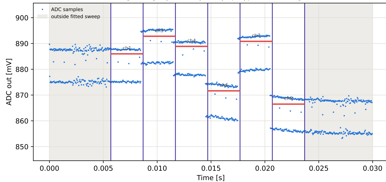
Tag5 &lt;- Tag16 | 875 MHz | run 0 | rep 1 | phase 35.92 deg
