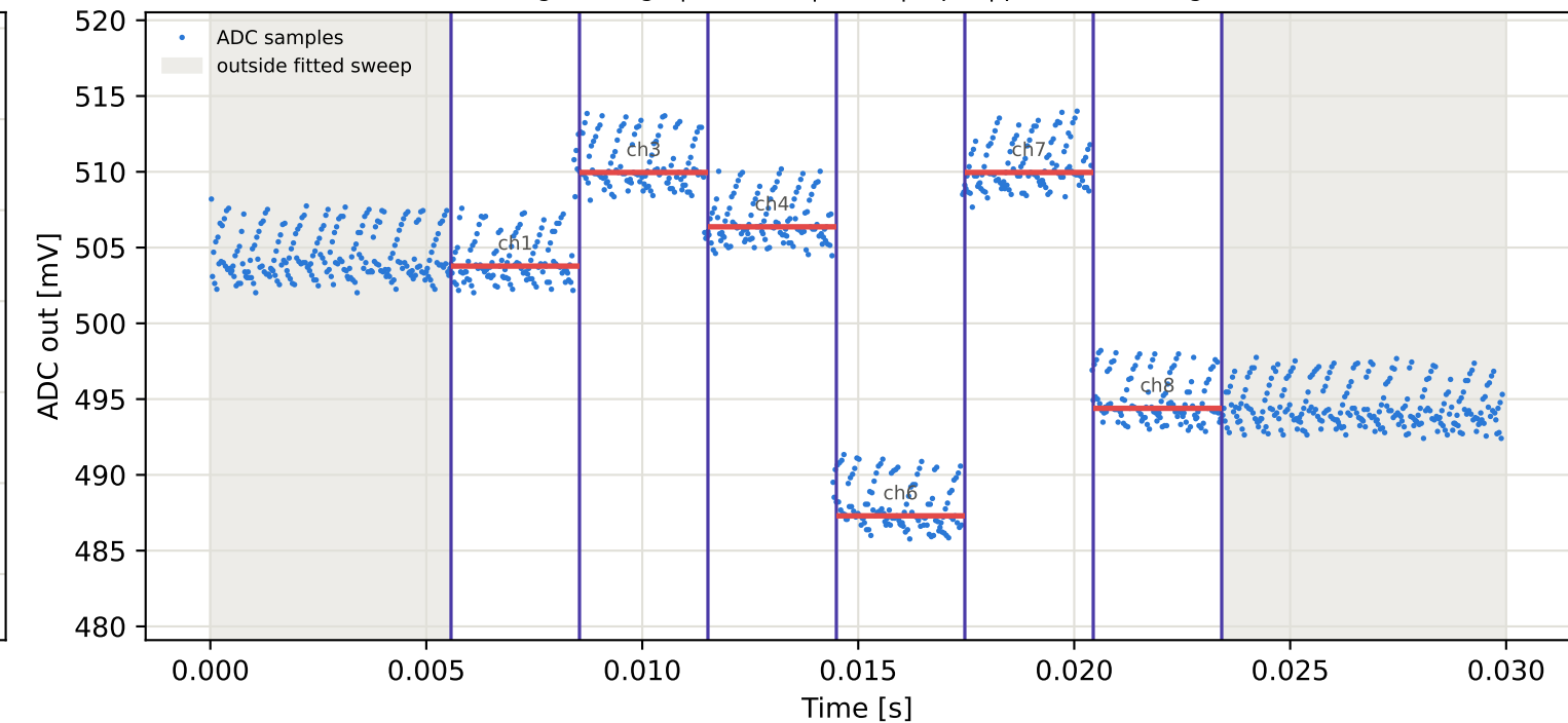
Tag5 &lt;- Tag9 | 975 MHz | run 0 | rep 1 | phase -21.66 deg
