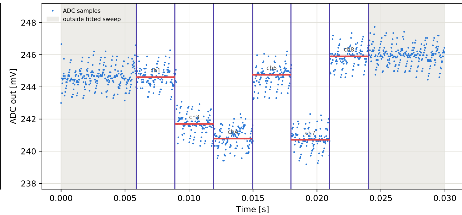
Tag9 &lt;- Tag2 | 845 MHz | run 0 | rep 1 | phase 128.88 deg
