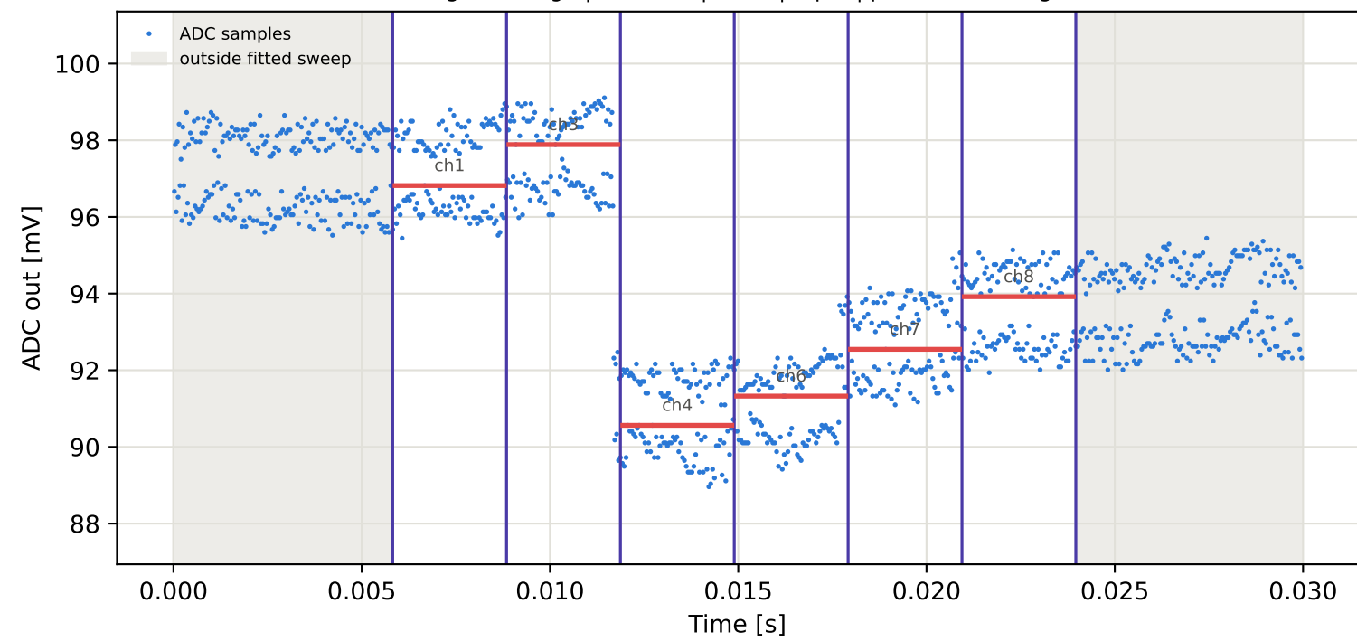
Tag10 &lt;- Tag5 | 825 MHz | run 0 | rep 1 | phase 57.80 deg
