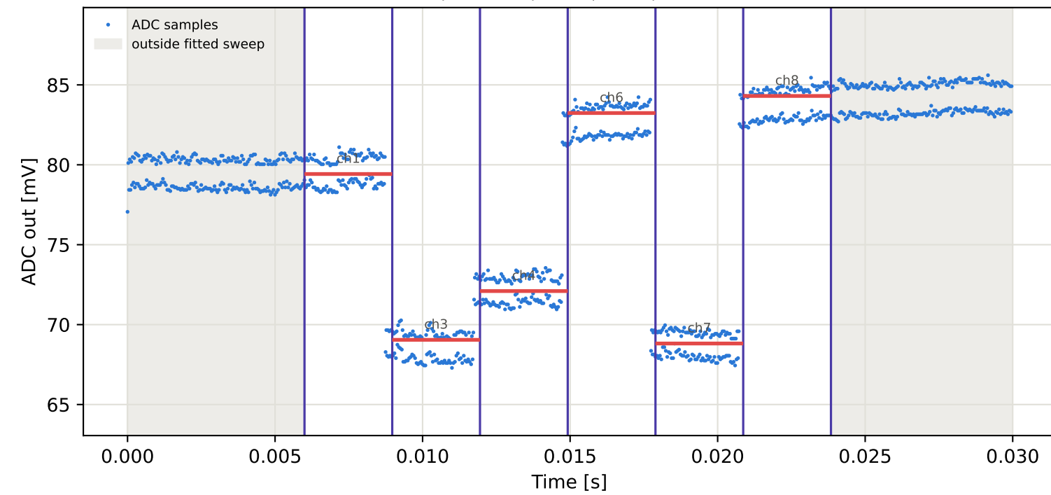
Tag9 &lt;- Tag7 | 795 MHz | run 0 | rep 1 | phase 160.90 deg
