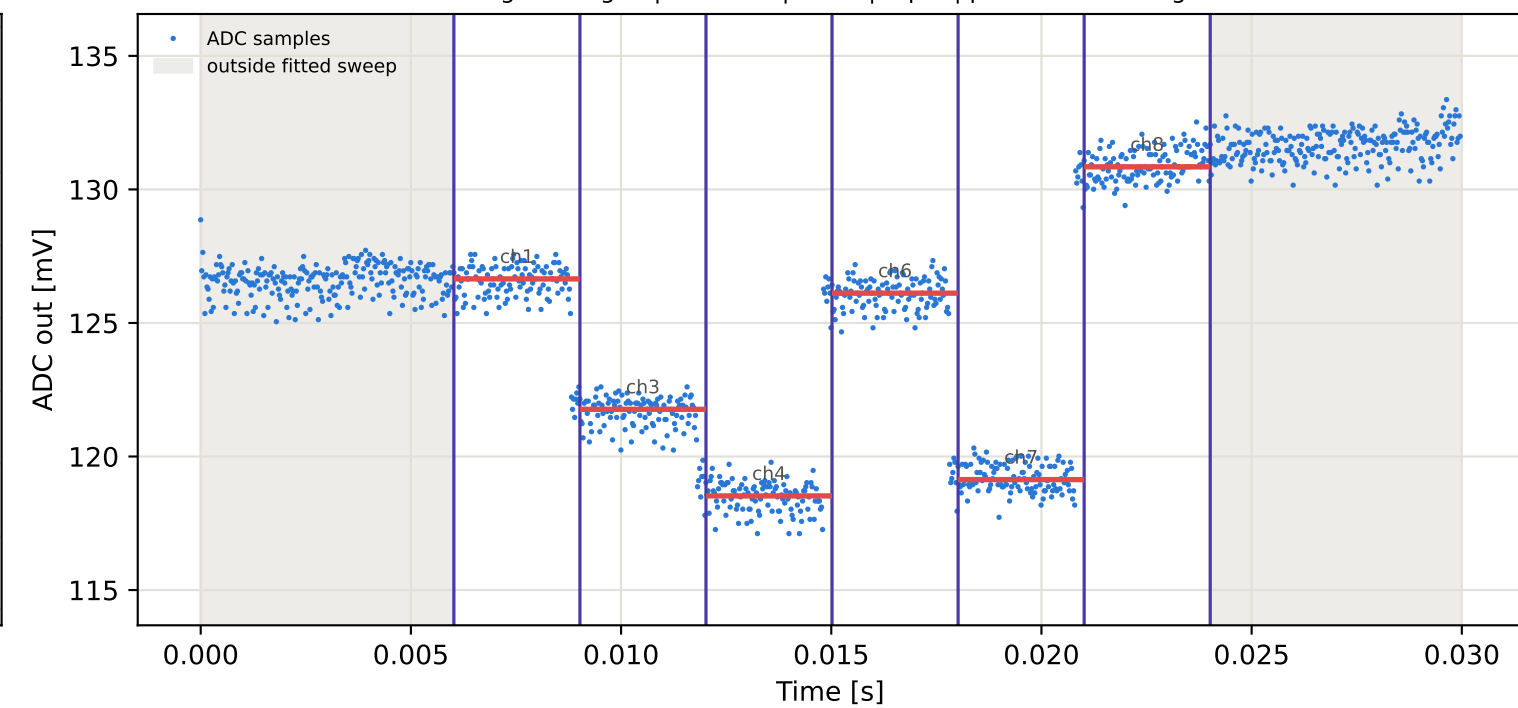
Tag1 &lt;- Tag2 | 915 MHz | run 0 | rep 1 | phase 175.19 deg
