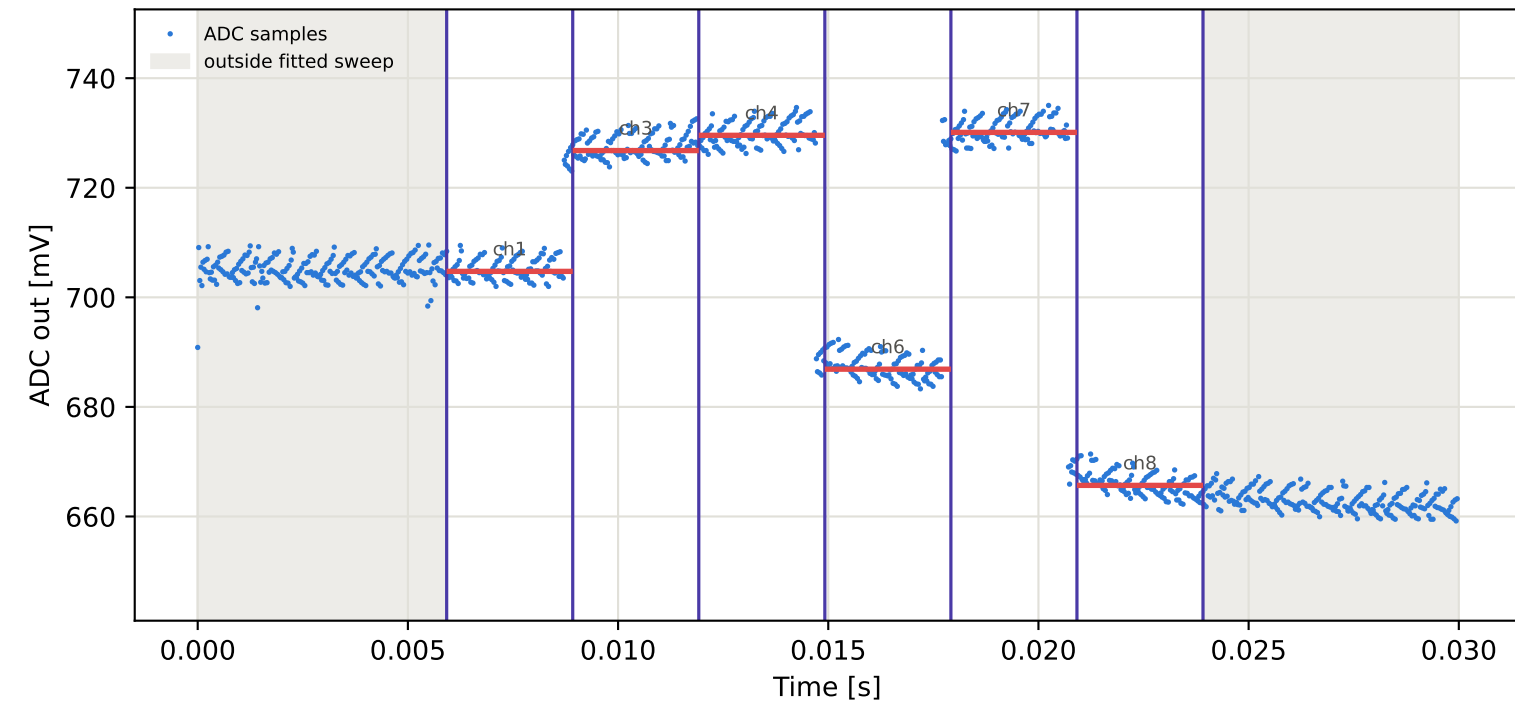
Tag4 &lt;- Tag3 | 895 MHz | run 0 | rep 1 | phase -164.61 deg
