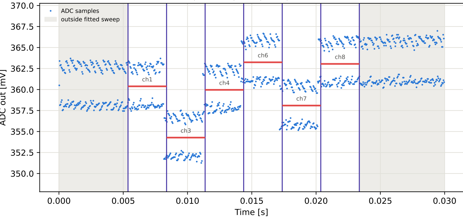
Tag6 &lt;- Tag4 | 825 MHz | run 0 | rep 1 | phase -166.58 deg
