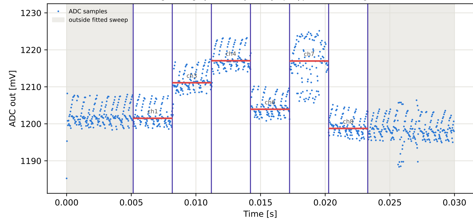
Tag5 &lt;- Tag9 | 895 MHz | run 0 | rep 1 | phase -170.33 deg
