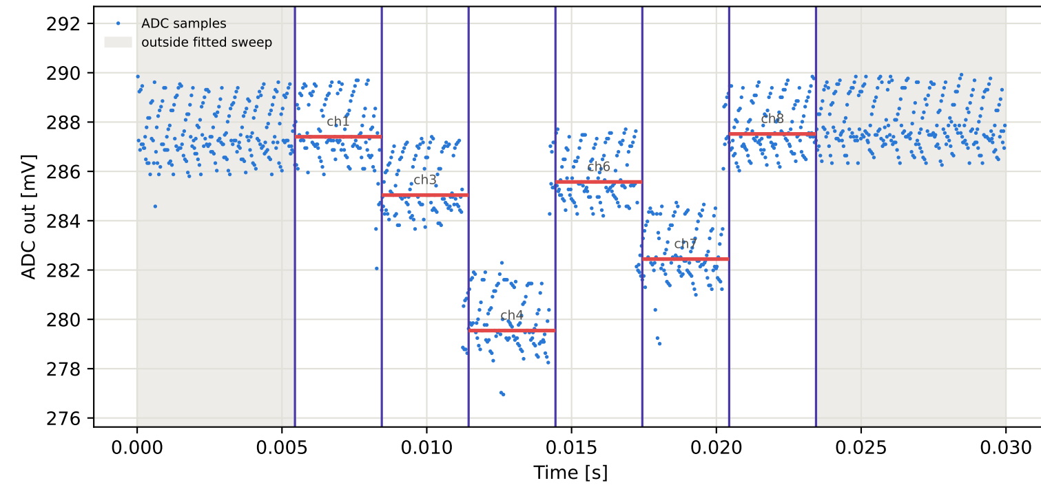
Tag15 &lt;- Tag1 | 975 MHz | run 0 | rep 1 | phase 77.09 deg
