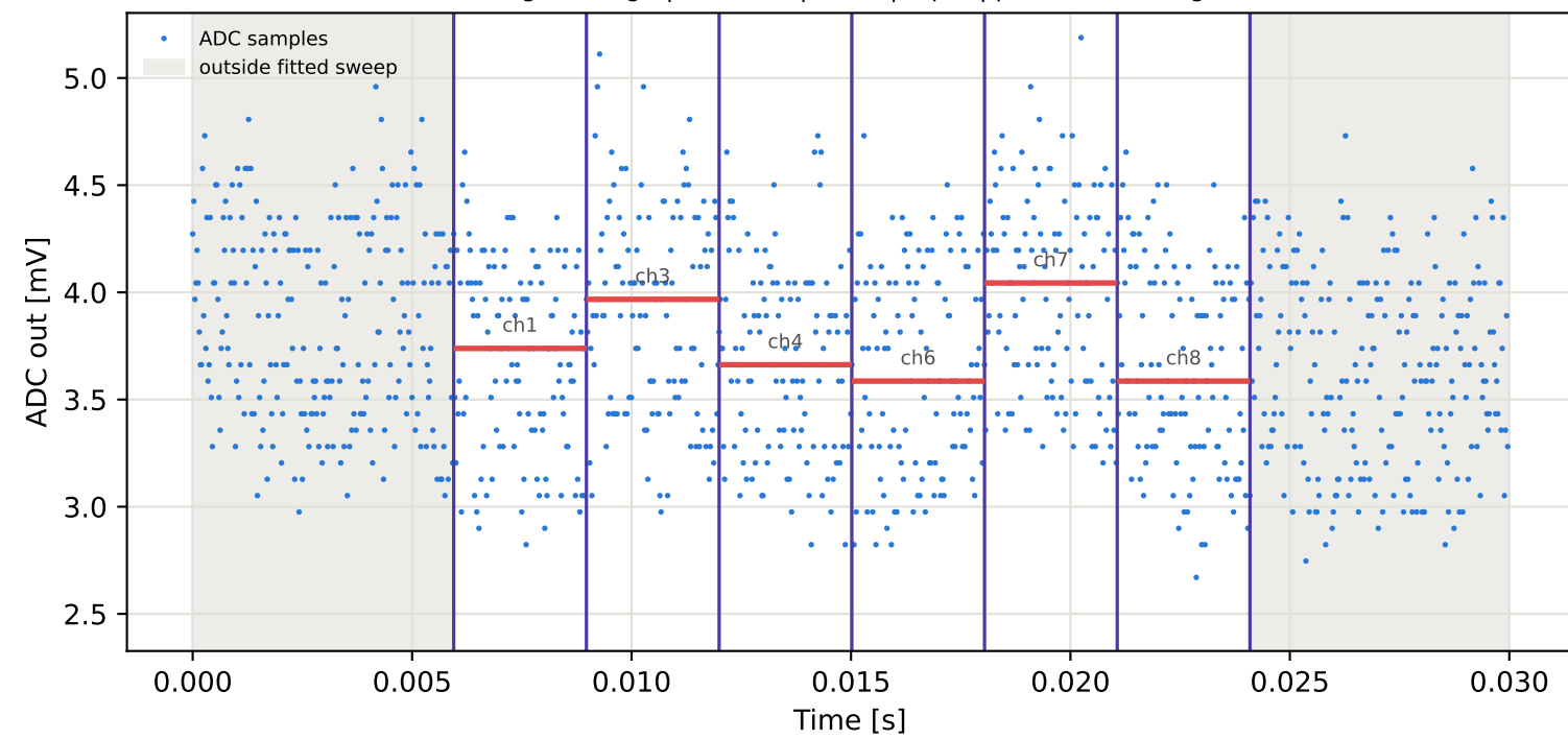
Tag10 &lt;- Tag1 | 785 MHz | run 0 | rep 1 | phase -84.06 deg
