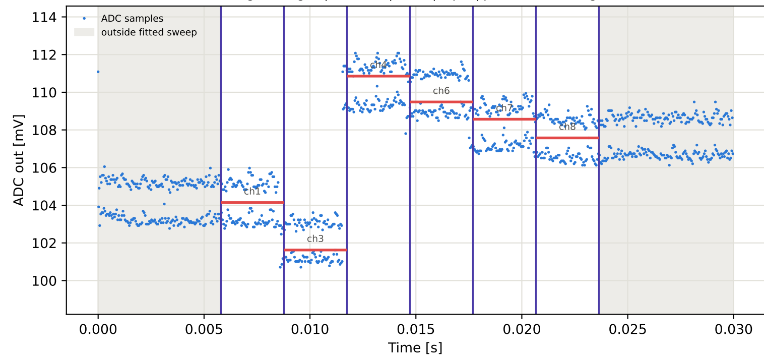
Tag6 &lt;- Tag3 | 805 MHz | run 0 | rep 1 | phase -171.09 deg
