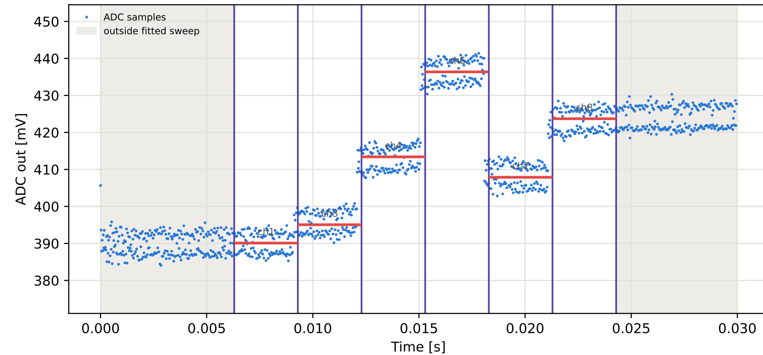
Tag1 &lt;- Tag3 | 885 MHz | run 0 | rep 1 | phase -137.88 deg
