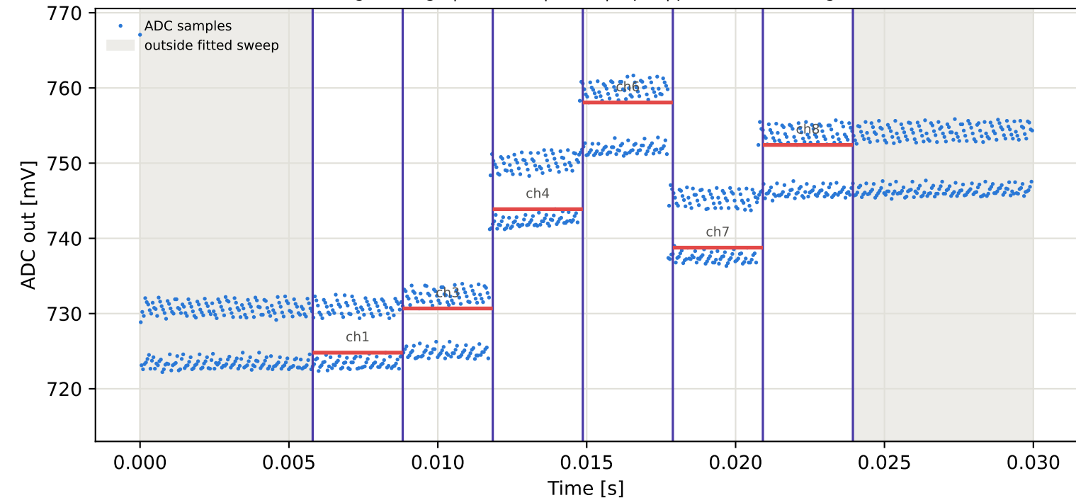
Tag3 &lt;- Tag7 | 855 MHz | run 0 | rep 1 | phase 157.92 deg
