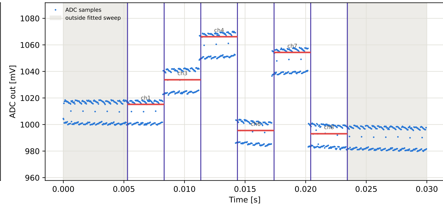
Tag8 &lt;- Tag7 | 955 MHz | run 0 | rep 1 | phase 49.17 deg
