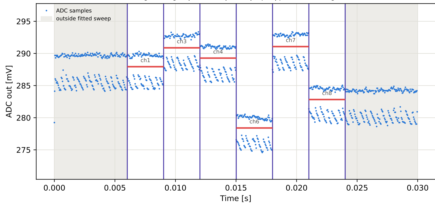
Tag9 &lt;- Tag2 | 995 MHz | run 0 | rep 1 | phase 118.52 deg
