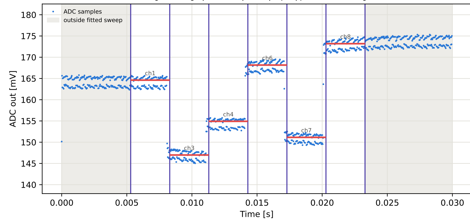
Tag10 &lt;- Tag4 | 845 MHz | run 0 | rep 1 | phase 161.08 deg
