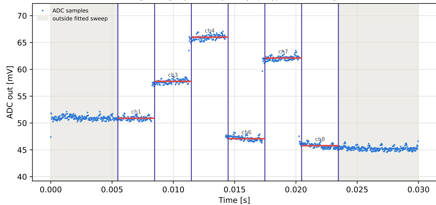
Tag1 &lt;- Tag16 | 955 MHz | run 0 | rep 1 | phase -3.08 deg
