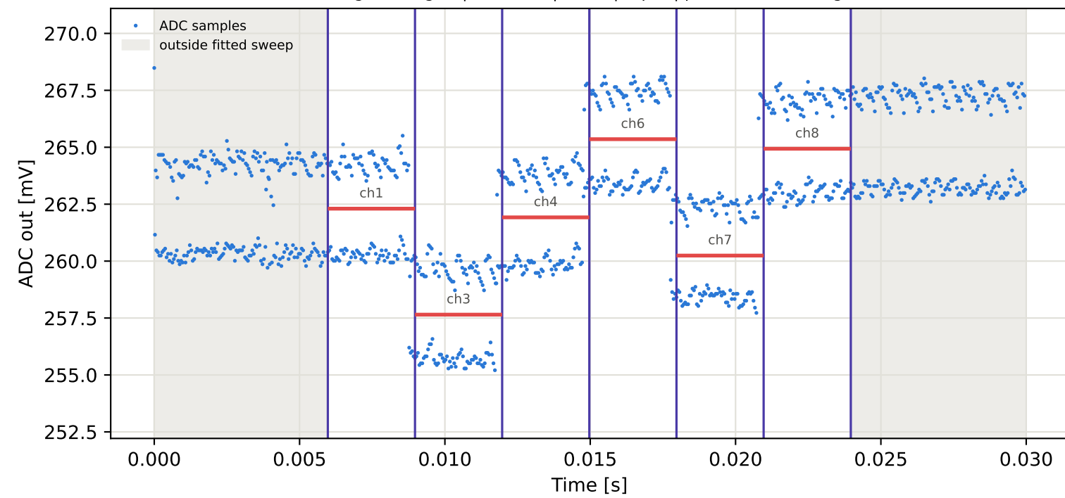
Tag6 &lt;- Tag3 | 835 MHz | run 0 | rep 1 | phase -158.83 deg
