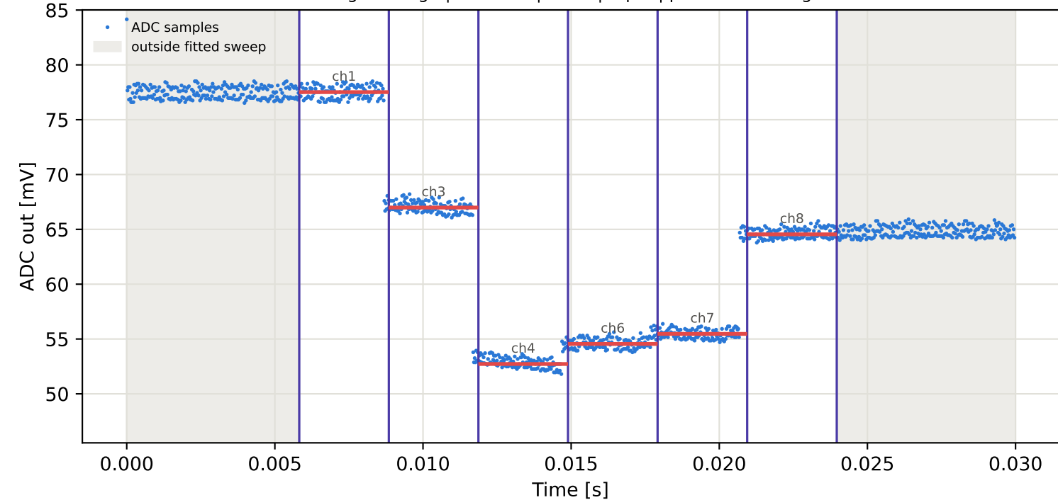
Tag1 &lt;- Tag8 | 845 MHz | run 0 | rep 1 | phase 121.37 deg
