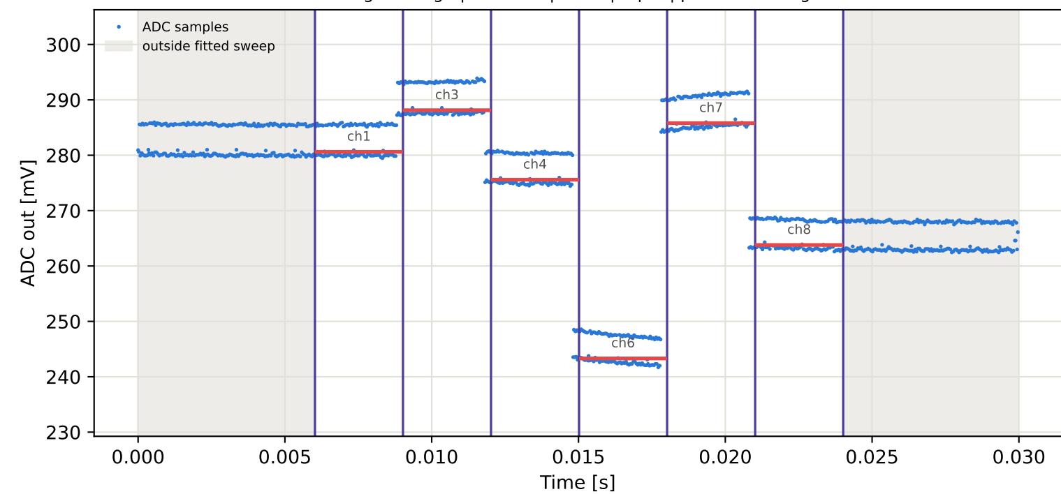
Tag3 &lt;- Tag7 | 985 MHz | run 0 | rep 1 | phase -107.65 deg
