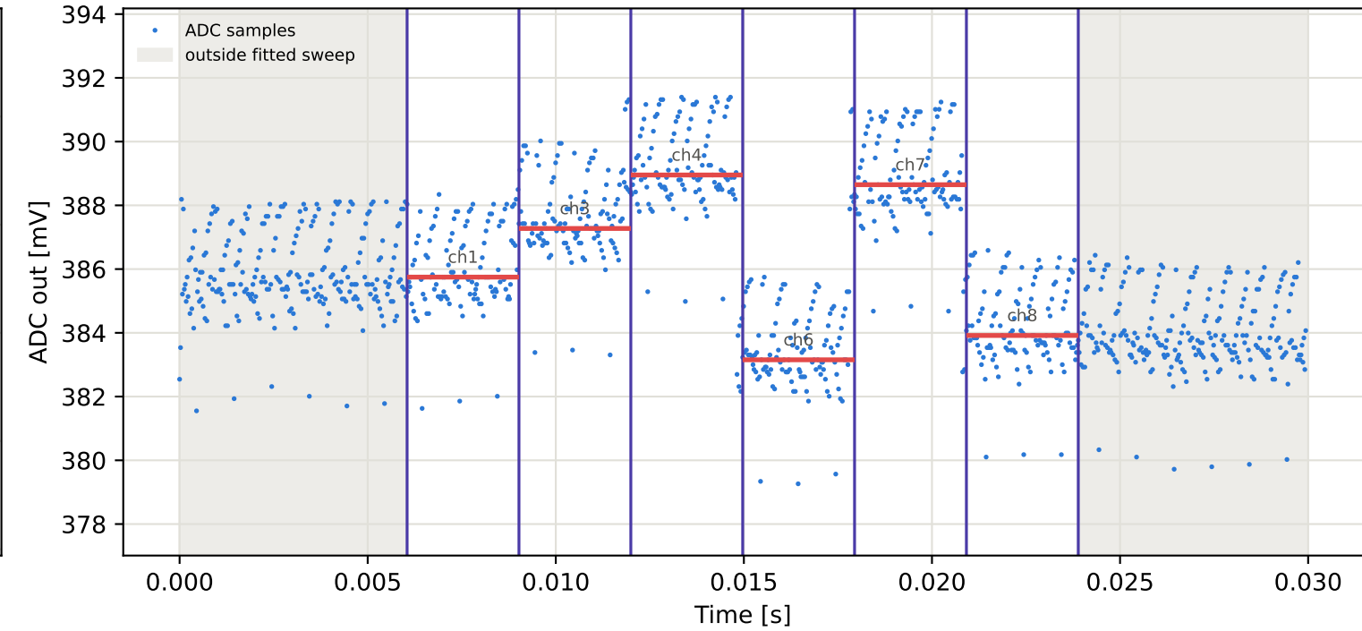
Tag5 &lt;- Tag4 | 805 MHz | run 0 | rep 1 | phase -121.37 deg
