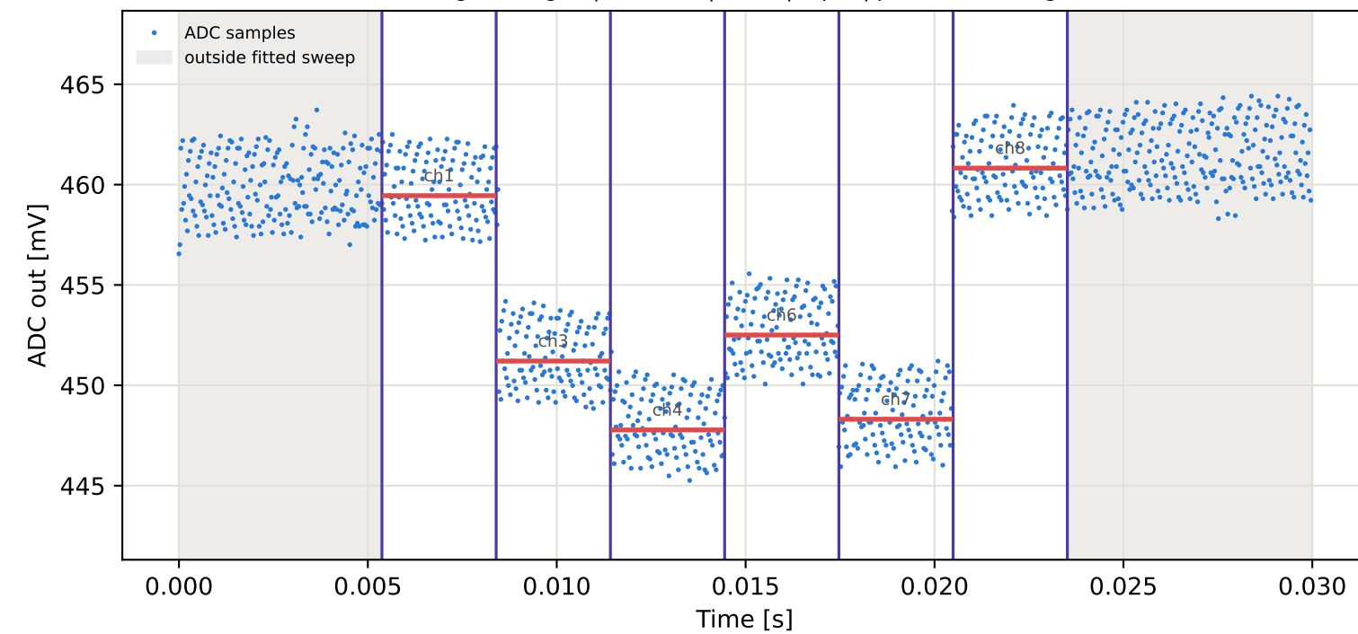
Tag1 &lt;- Tag16 | 875 MHz | run 0 | rep 1 | phase -160.45 deg
