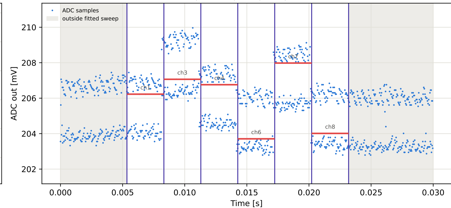
Tag4 &lt;- Tag3 | 805 MHz | run 0 | rep 1 | phase -7.98 deg
