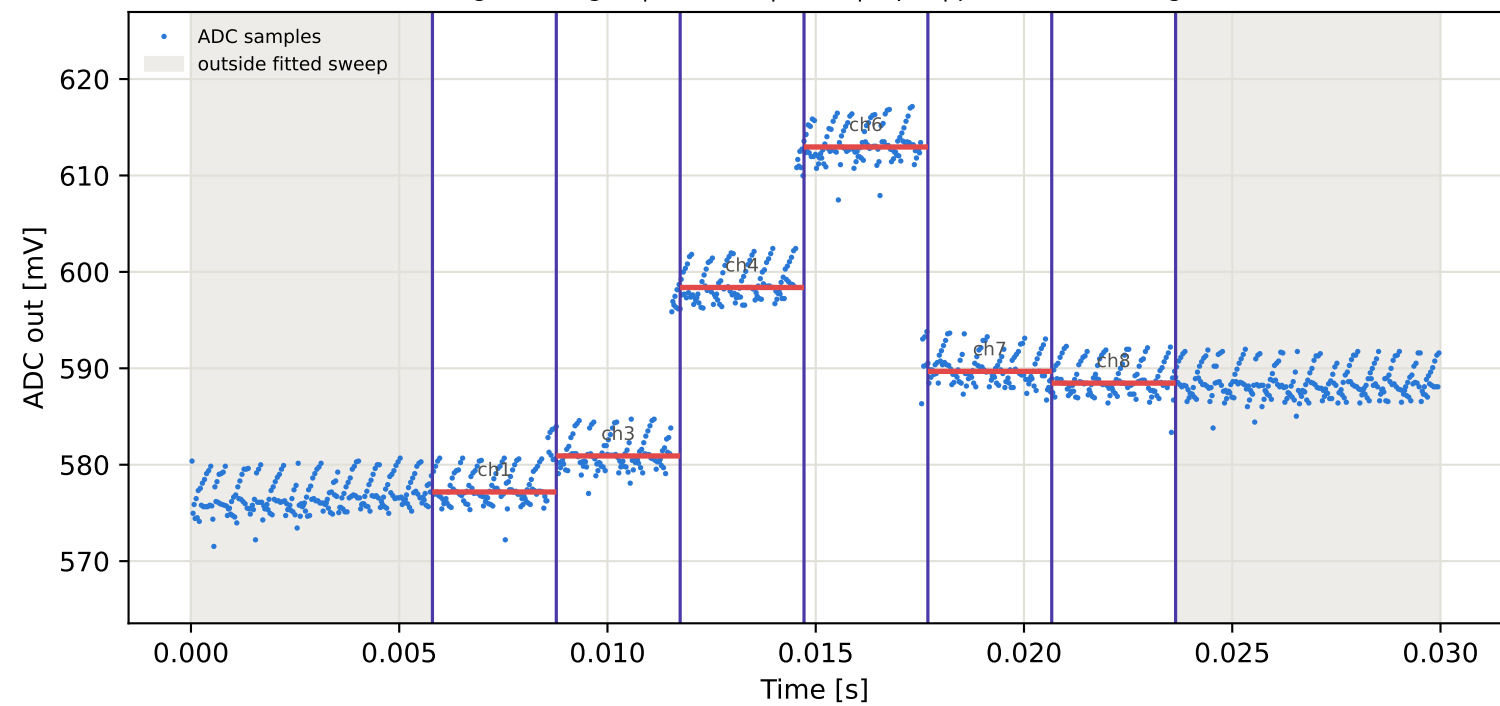
Tag10 &lt;- Tag2 | 945 MHz | run 0 | rep 1 | phase -107.79 deg
