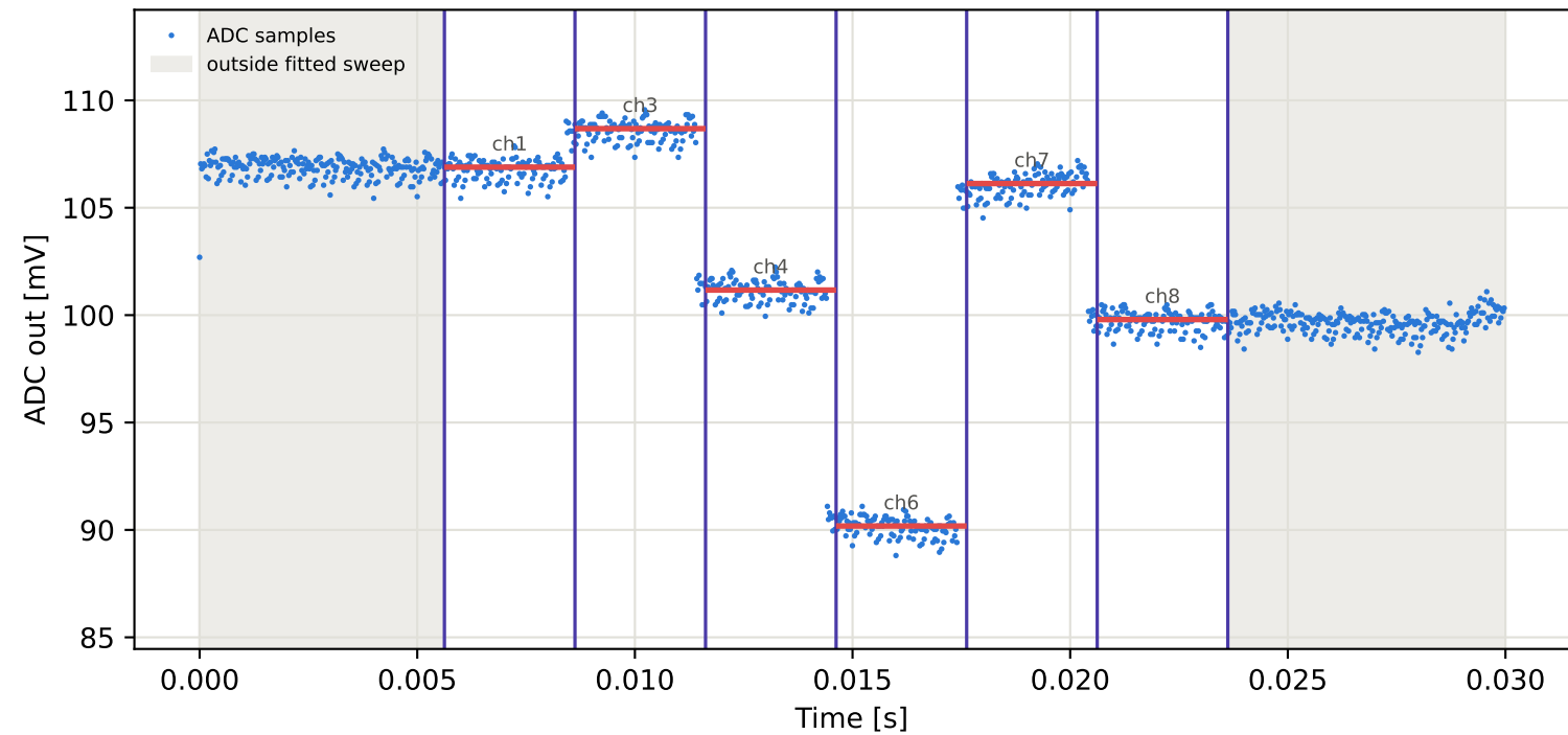
Tag1 &lt;- Tag3 | 965 MHz | run 0 | rep 1 | phase 22.27 deg
