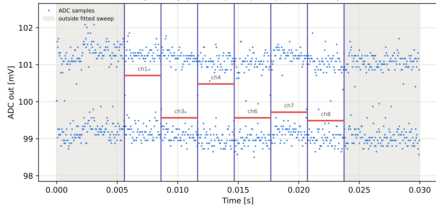
Tag15 &lt;- Tag4 | 785 MHz | run 0 | rep 1 | phase 179.37 deg
