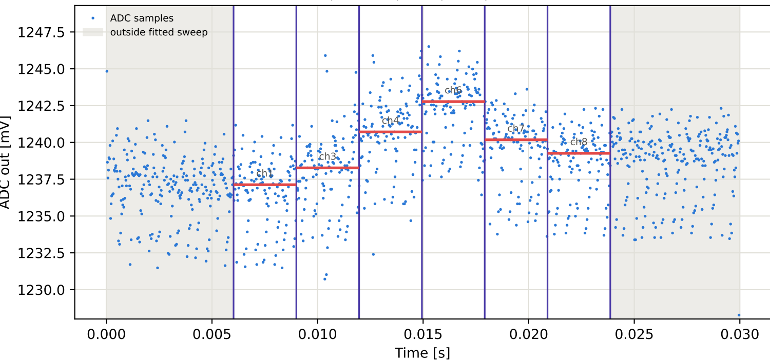
Tag10 &lt;- Tag4 | 885 MHz | run 0 | rep 1 | phase -135.45 deg
