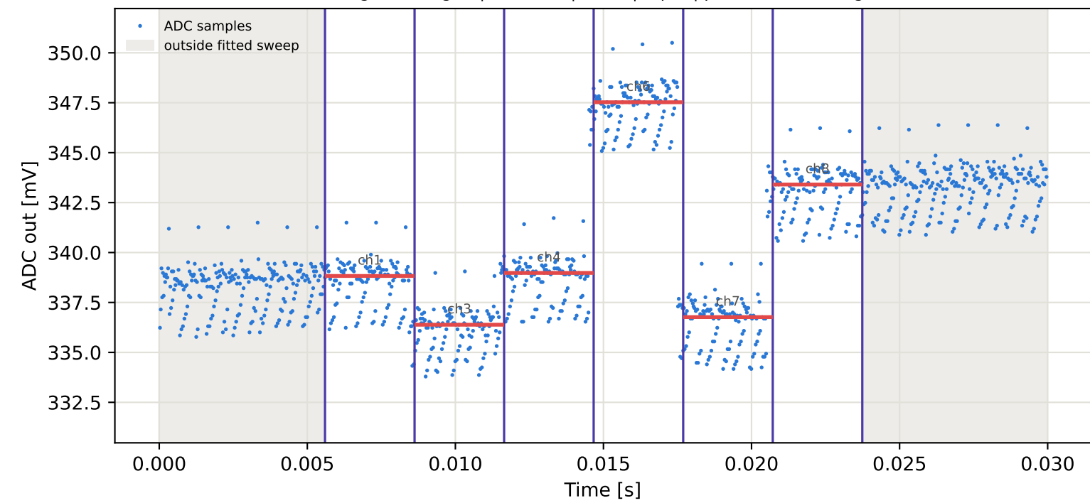
Tag10 &lt;- Tag2 | 975 MHz | run 0 | rep 1 | phase -117.19 deg
