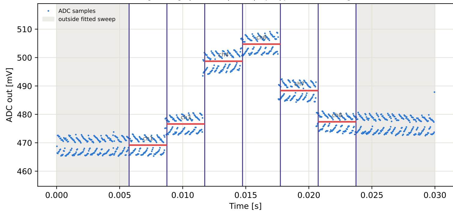
Tag4 &lt;- Tag8 | 935 MHz | run 0 | rep 1 | phase -2.59 deg
