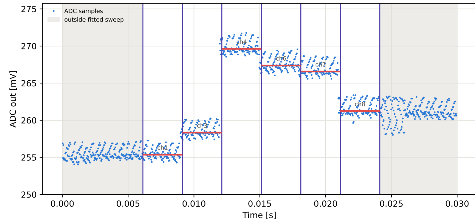
Tag4 &lt;- Tag9 | 835 MHz | run 0 | rep 1 | phase -113.39 deg
