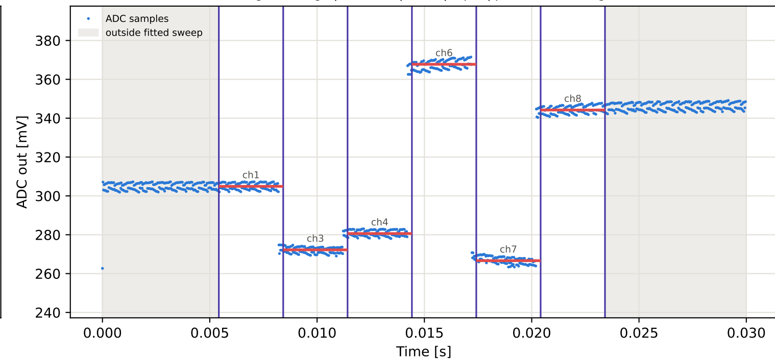
Tag2 &lt;- Tag10 | 985 MHz | run 0 | rep 1 | phase -102.35 deg
