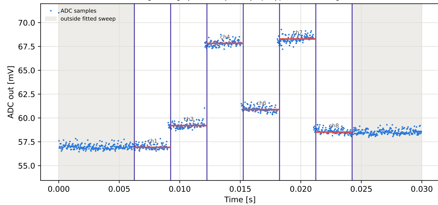
Tag1 &lt;- Tag4 | 785 MHz | run 0 | rep 1 | phase -81.11 deg
