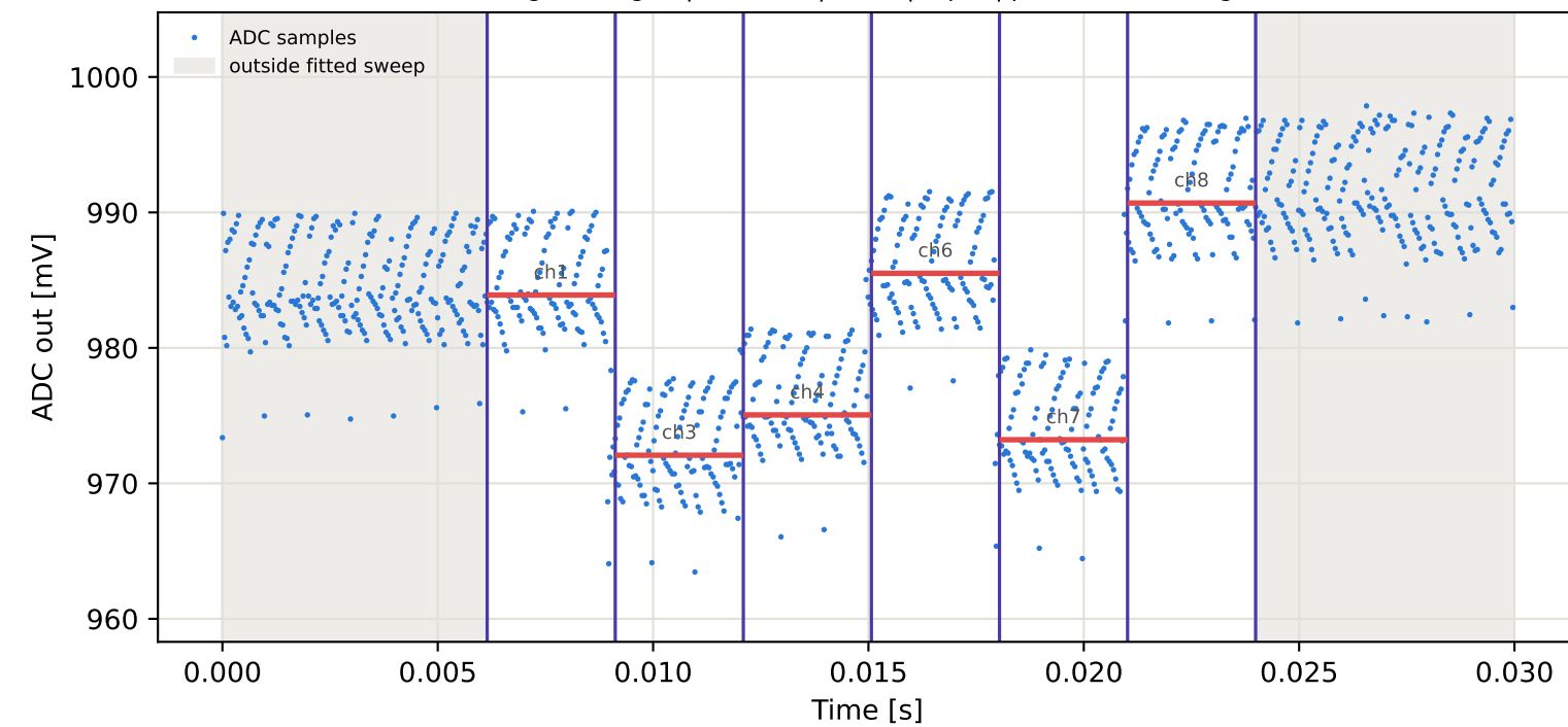
Tag7 &lt;- Tag3 | 865 MHz | run 0 | rep 1 | phase -132.26 deg
