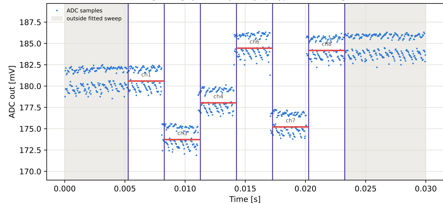
Tag9 &lt;- Tag10 | 795 MHz | run 0 | rep 1 | phase -55.94 deg
