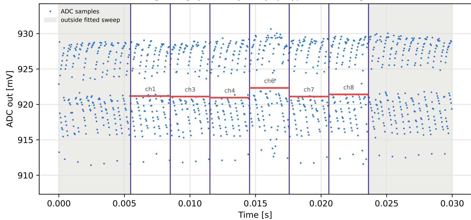
Tag7 &lt;- Tag4 | 965 MHz | run 0 | rep 1 | phase -143.70 deg
