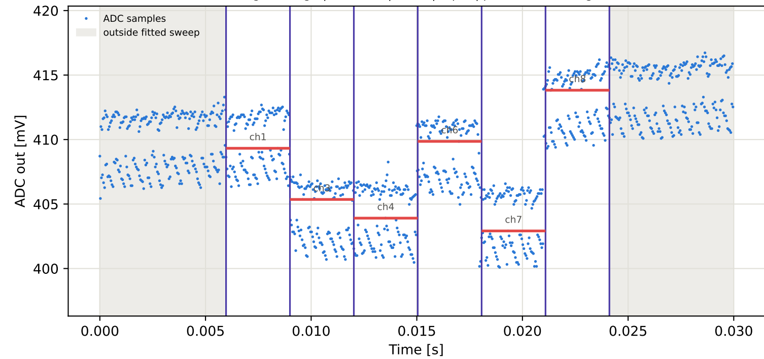
Tag2 &lt;- Tag6 | 865 MHz | run 0 | rep 1 | phase -72.30 deg
