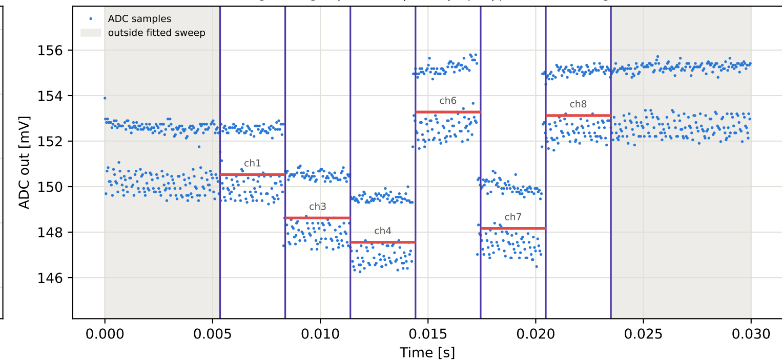
Tag1 &lt;- Tag2 | 925 MHz | run 0 | rep 1 | phase -33.93 deg
