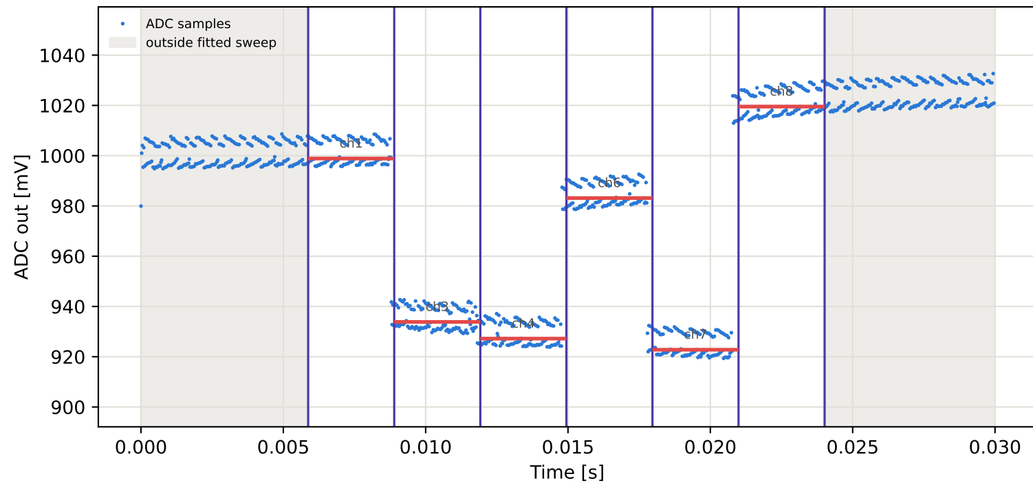
Tag2 &lt;- Tag10 | 875 MHz | run 0 | rep 1 | phase 50.73 deg
