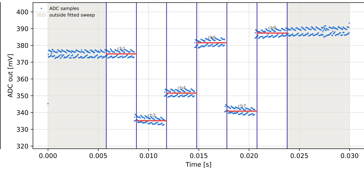
Tag6 &lt;- Tag10 | 825 MHz | run 0 | rep 1 | phase 161.81 deg
