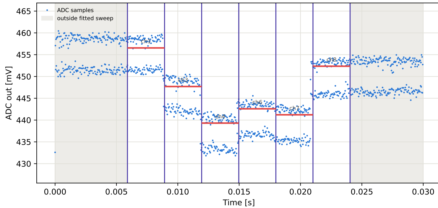
Tag15 &lt;- Tag9 | 885 MHz | run 0 | rep 1 | phase -9.32 deg
