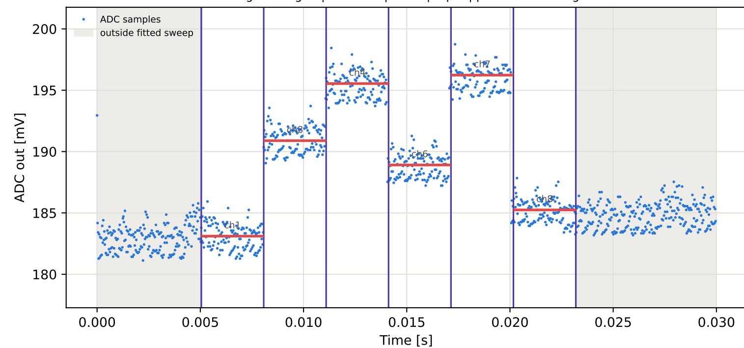
Tag2 &lt;- Tag16 | 835 MHz | run 0 | rep 1 | phase -77.28 deg
