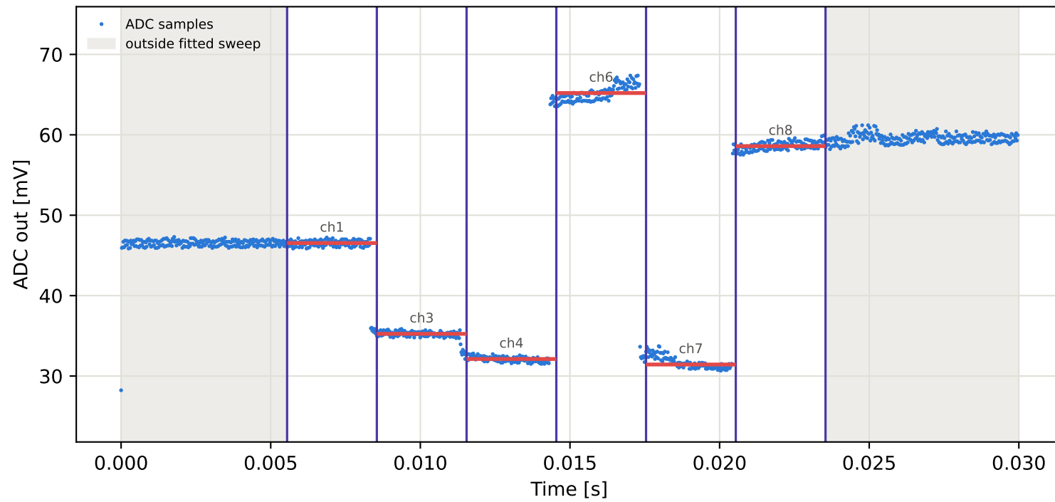
Tag16 &lt;- Tag10 | 965 MHz | run 0 | rep 1 | phase 30.94 deg
