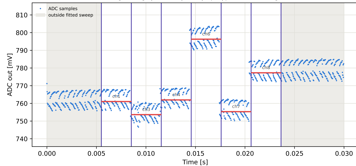
Tag8 &lt;- Tag1 | 955 MHz | run 0 | rep 1 | phase -106.04 deg
