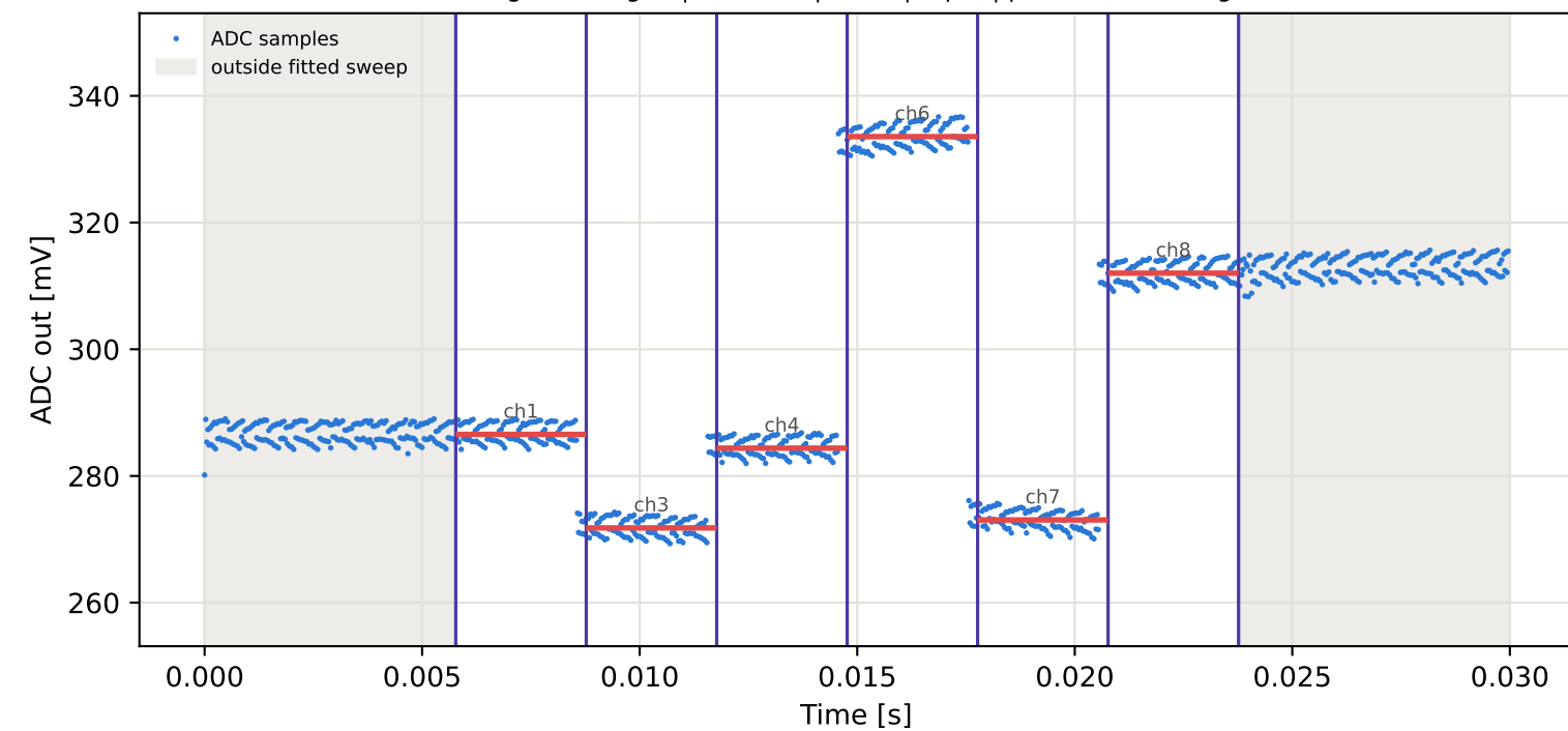
Tag16 &lt;- Tag15 | 985 MHz | run 0 | rep 1 | phase 176.68 deg
