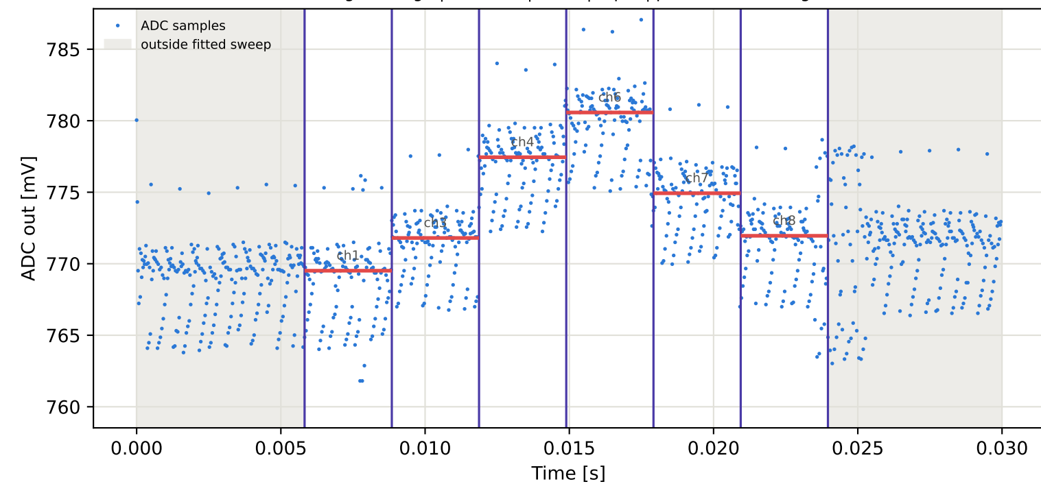
Tag8 &lt;- Tag6 | 925 MHz | run 0 | rep 1 | phase -135.50 deg
