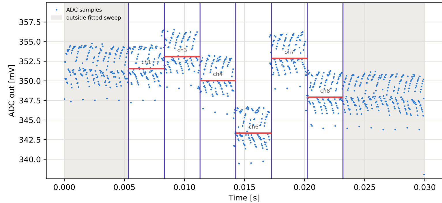
Tag15 &lt;- Tag6 | 985 MHz | run 0 | rep 1 | phase -155.82 deg
