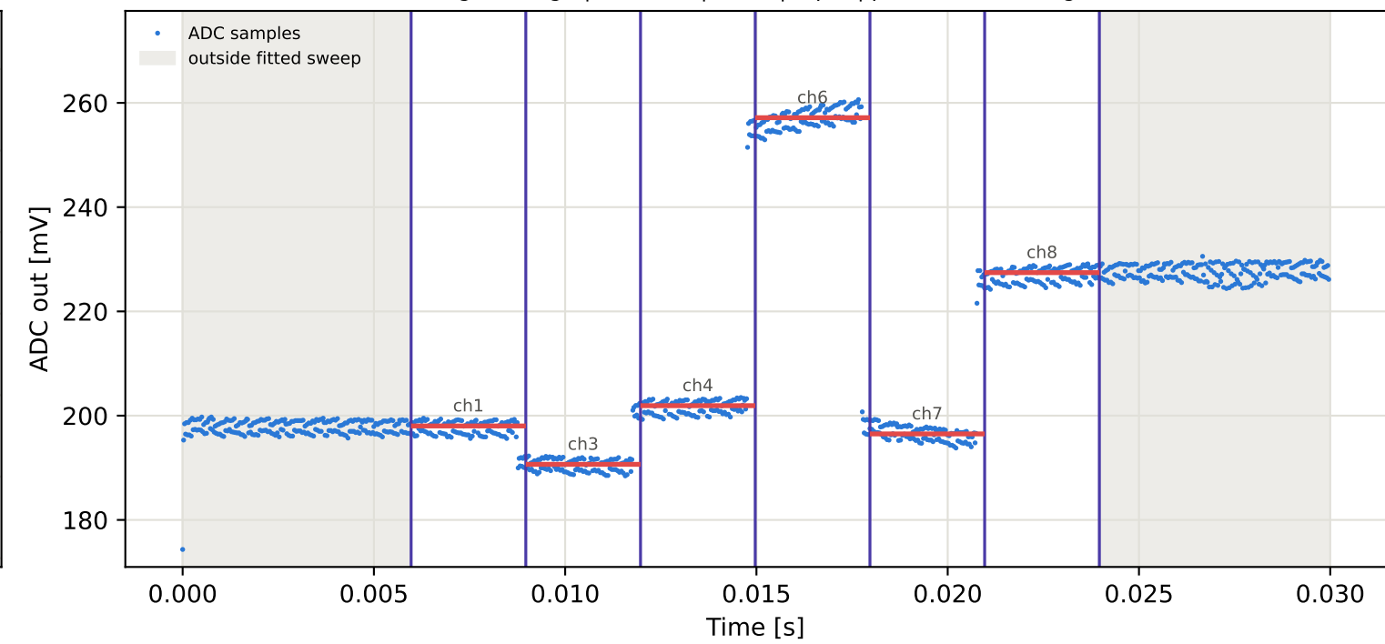
Tag4 &lt;- Tag8 | 915 MHz | run 0 | rep 1 | phase -18.43 deg
