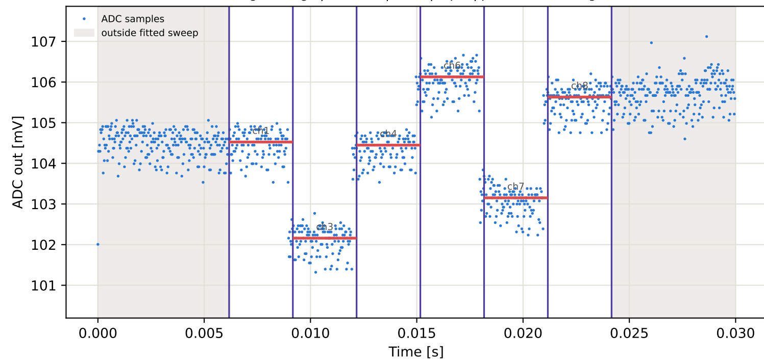
Tag10 &lt;- Tag1 | 795 MHz | run 0 | rep 1 | phase 156.94 deg
