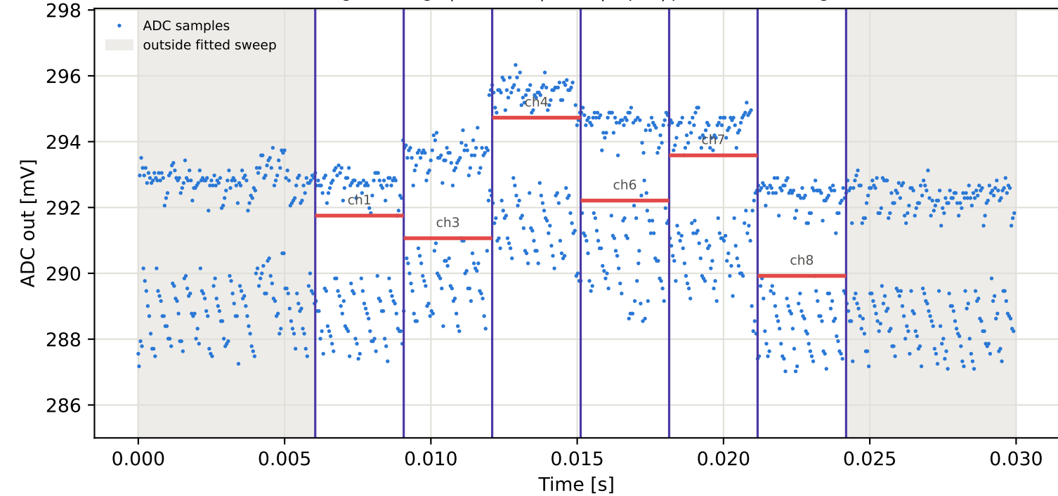
Tag15 &lt;- Tag4 | 945 MHz | run 0 | rep 1 | phase -97.76 deg
