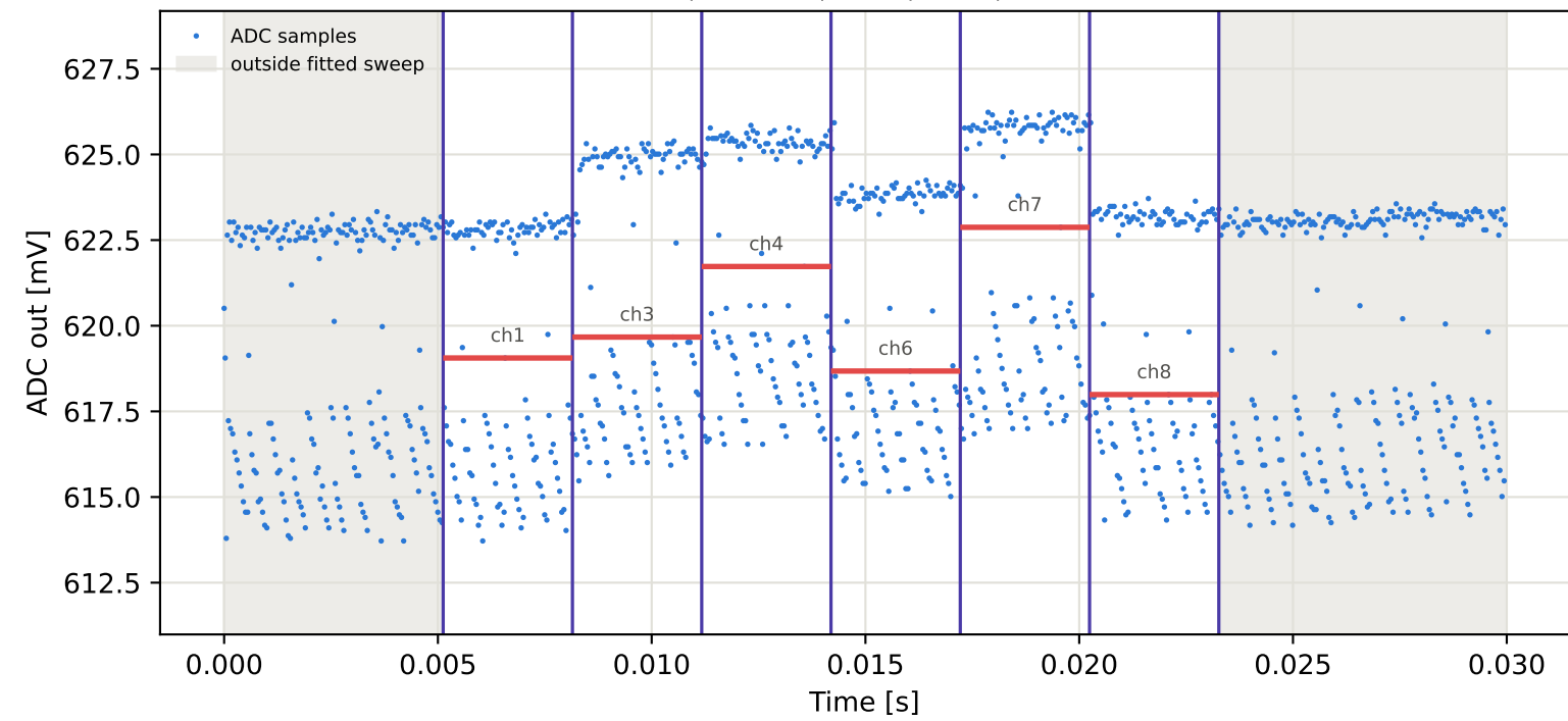
Tag10 &lt;- Tag1 | 855 MHz | run 0 | rep 1 | phase -60.75 deg
