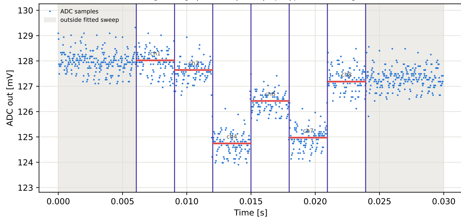
Tag5 &lt;- Tag1 | 785 MHz | run 0 | rep 1 | phase 130.94 deg
