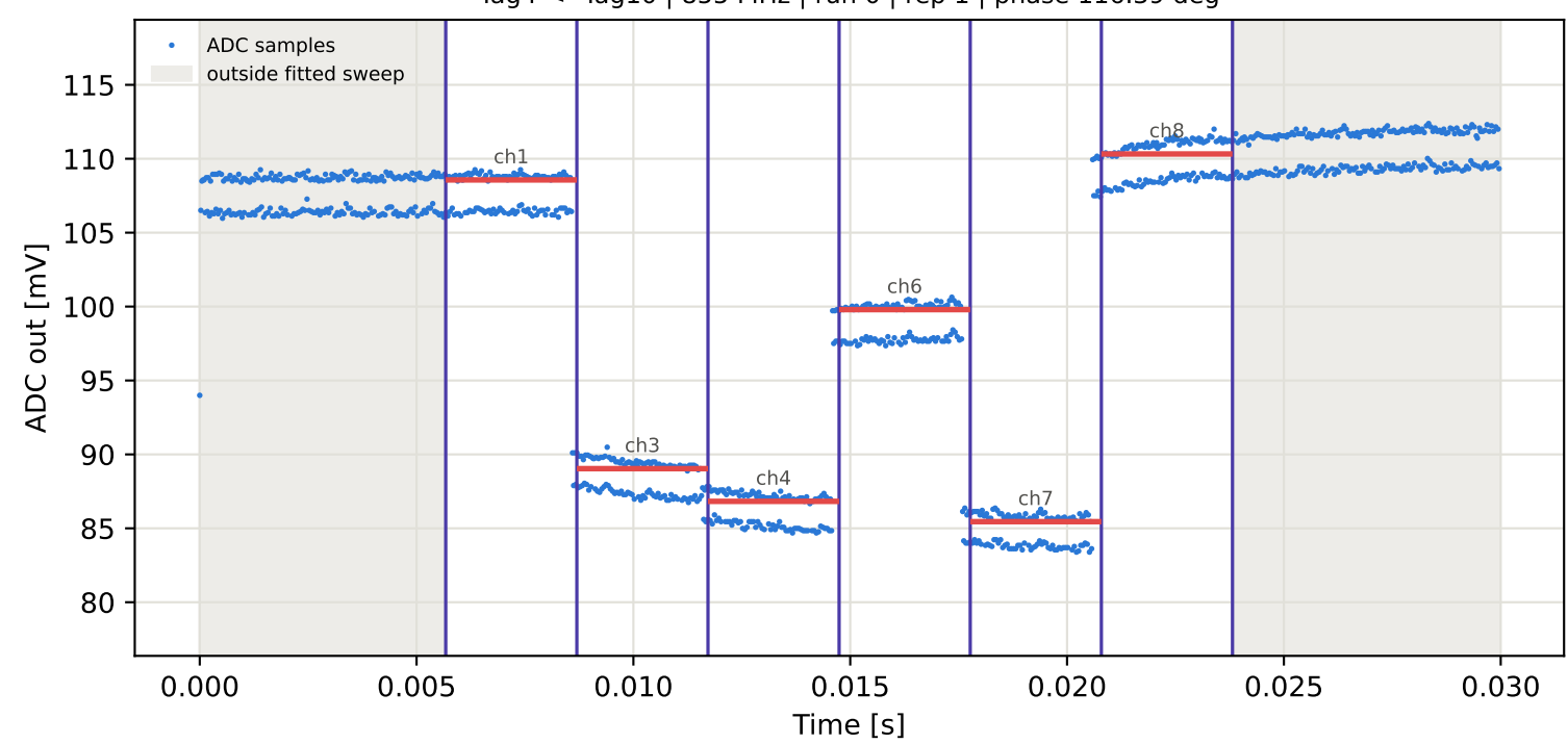
Tag4 &lt;- Tag16 | 855 MHz | run 0 | rep 1 | phase 155.01 deg
