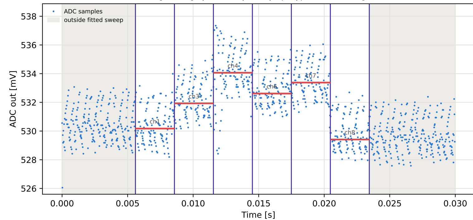
Tag8 &lt;- Tag4 | 845 MHz | run 0 | rep 1 | phase 86.91 deg
