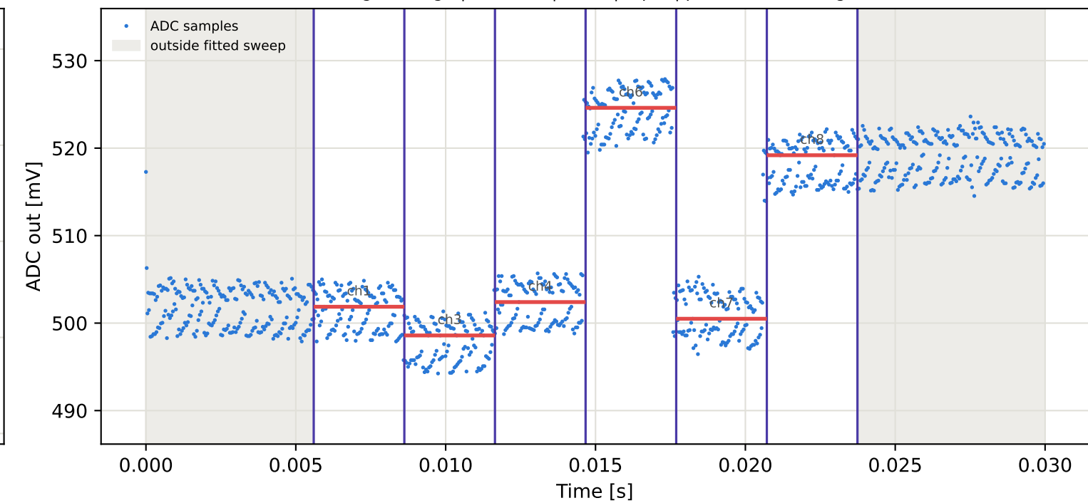
Tag2 &lt;- Tag6 | 895 MHz | run 0 | rep 1 | phase -148.94 deg
