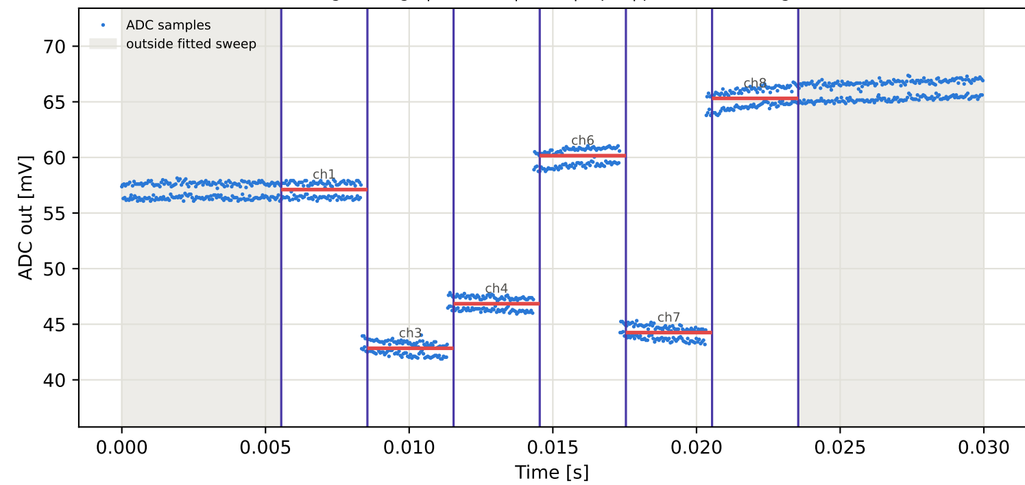
Tag1 &lt;- Tag8 | 855 MHz | run 0 | rep 1 | phase -87.64 deg
