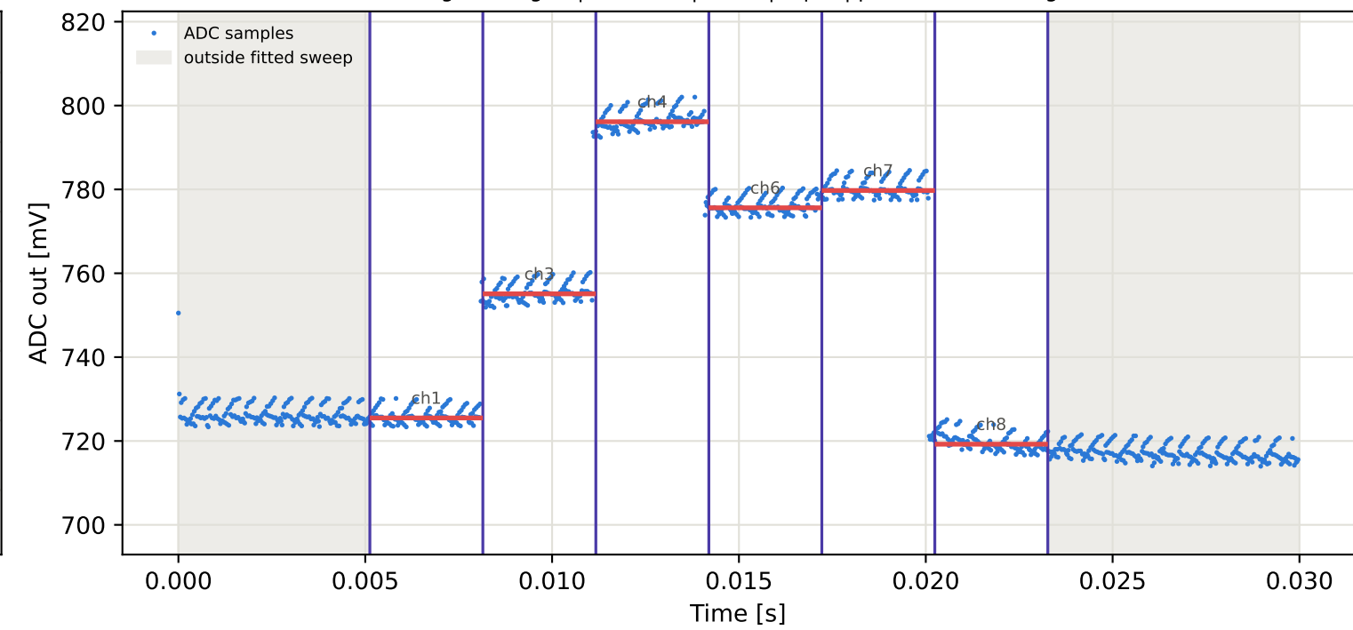
Tag6 &lt;- Tag10 | 915 MHz | run 0 | rep 1 | phase -104.64 deg
