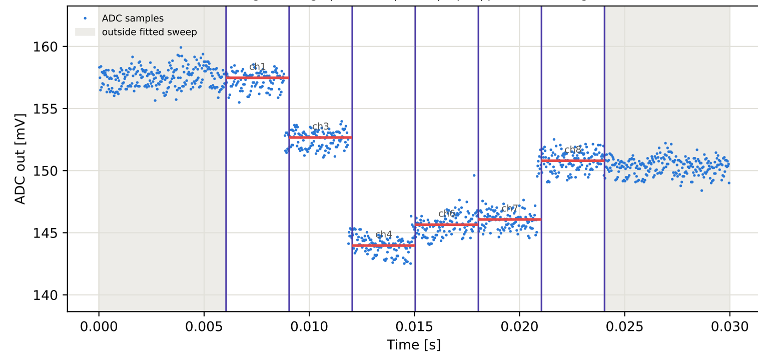
Tag16 &lt;- Tag1 | 835 MHz | run 0 | rep 1 | phase -36.47 deg
