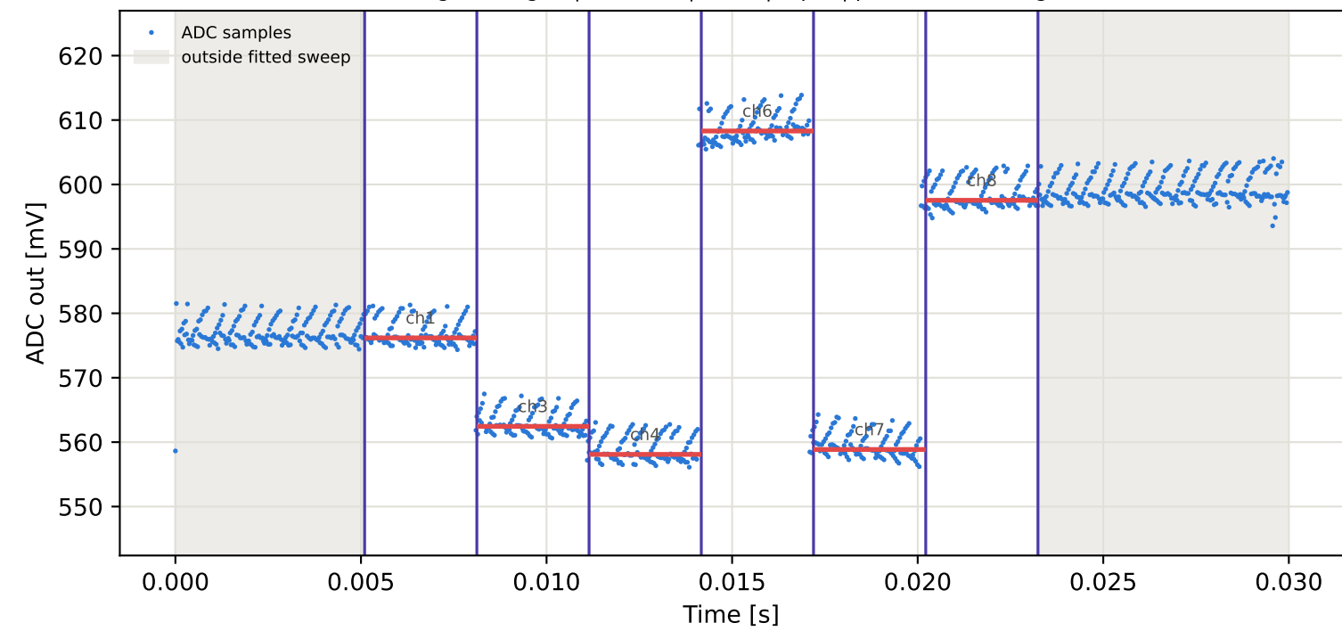
Tag5 &lt;- Tag2 | 935 MHz | run 0 | rep 1 | phase -38.39 deg
