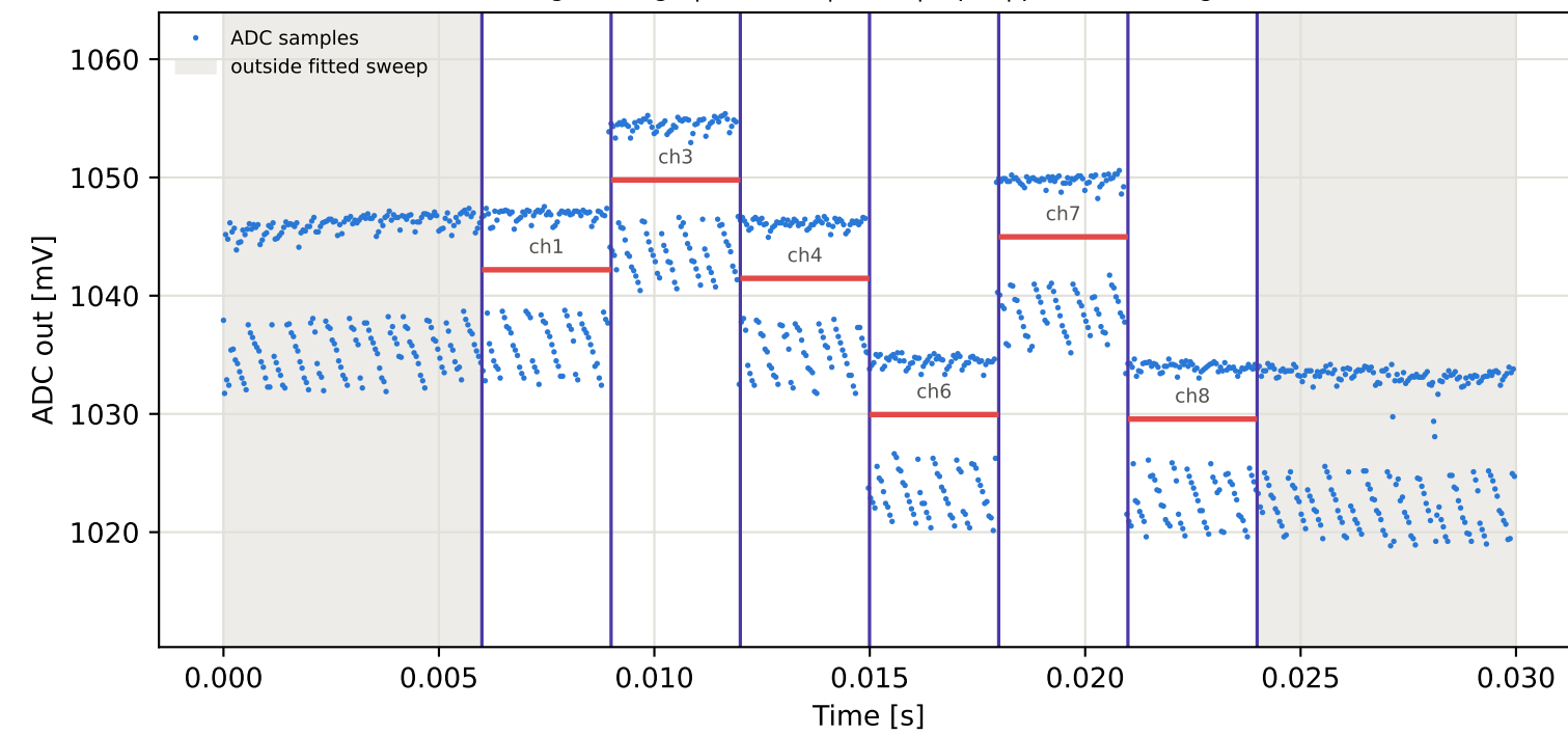
Tag8 &lt;- Tag1 | 855 MHz | run 0 | rep 1 | phase 69.43 deg
