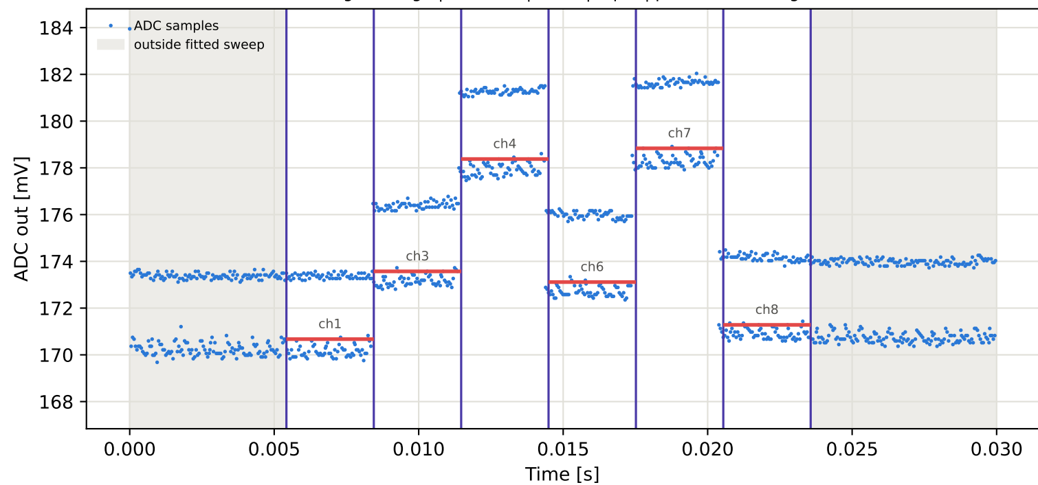
Tag7 &lt;- Tag6 | 775 MHz | run 0 | rep 1 | phase -71.70 deg
