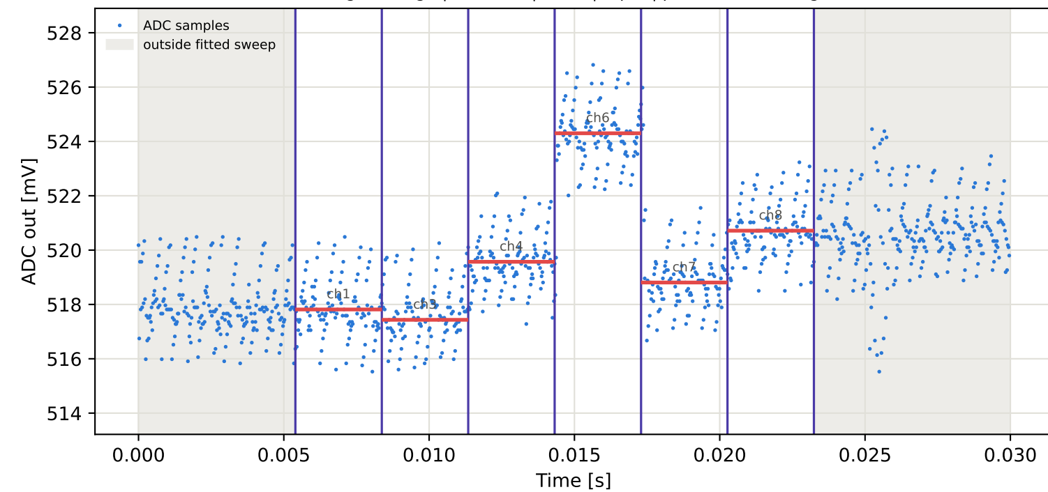
Tag8 &lt;- Tag4 | 835 MHz | run 0 | rep 1 | phase 68.98 deg
