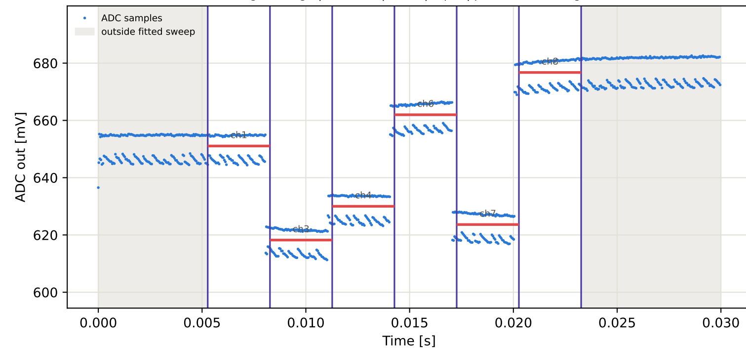
Tag9 &lt;- Tag5 | 855 MHz | run 0 | rep 1 | phase 178.89 deg
