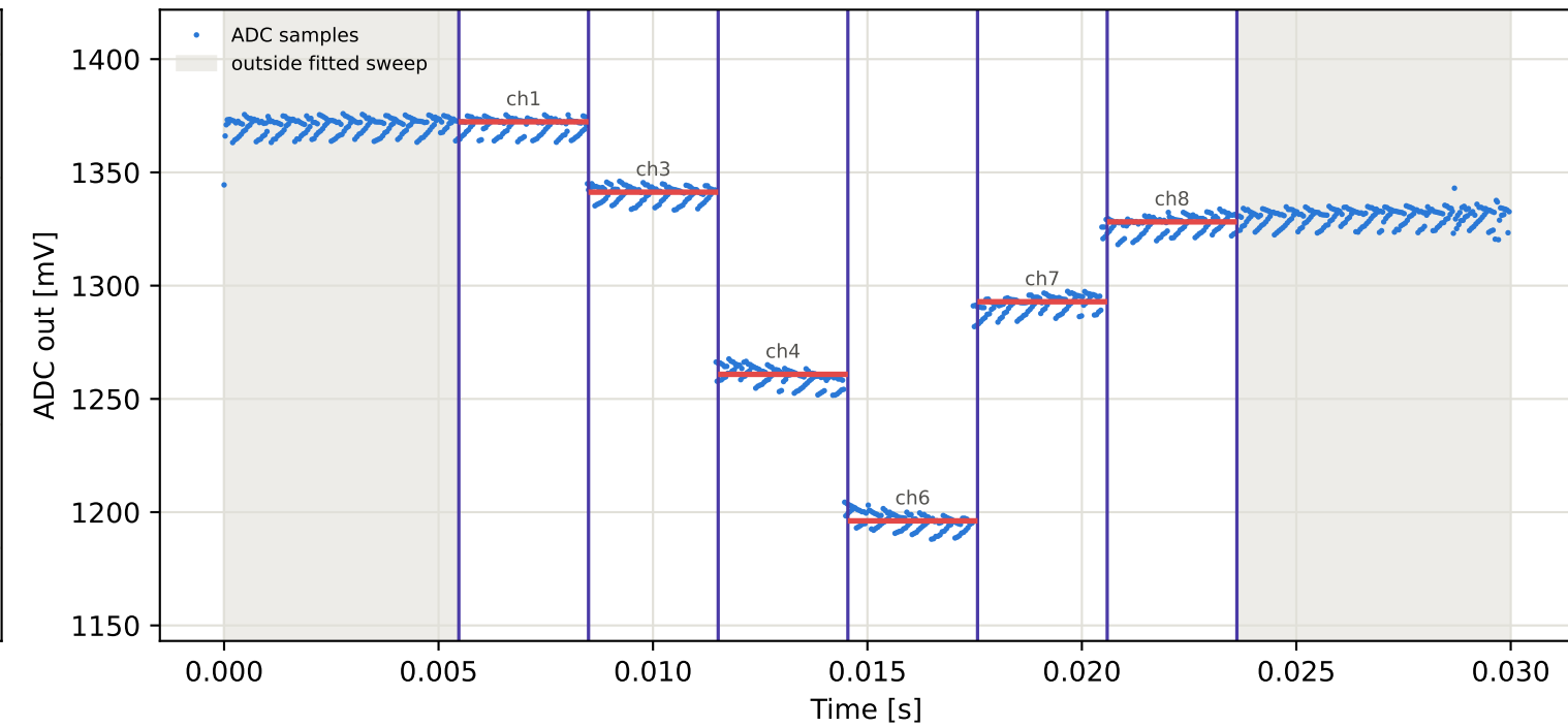
Tag10 &lt;- Tag5 | 915 MHz | run 0 | rep 1 | phase -122.57 deg
