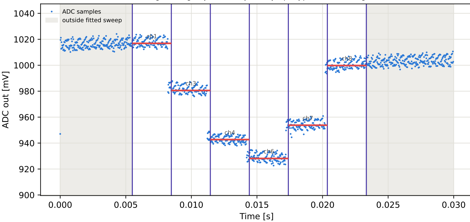
Tag9 &lt;- Tag16 | 885 MHz | run 0 | rep 1 | phase 78.76 deg
