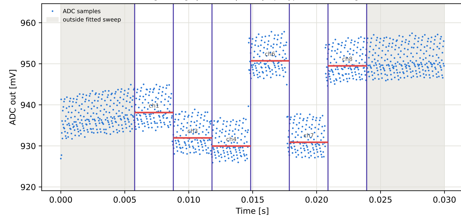
Tag3 &lt;- Tag6 | 915 MHz | run 0 | rep 1 | phase 93.34 deg
