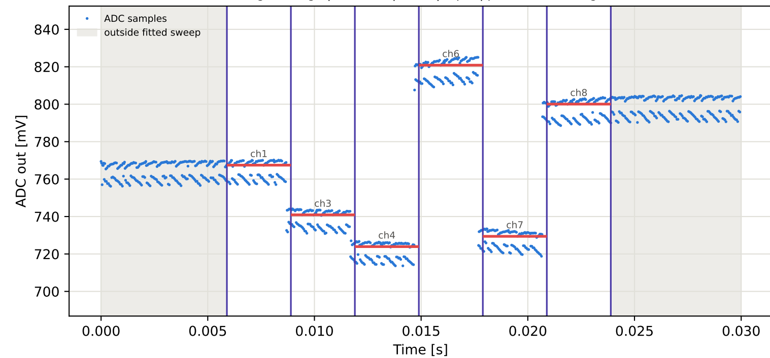
Tag8 &lt;- Tag1 | 945 MHz | run 0 | rep 1 | phase -99.12 deg
