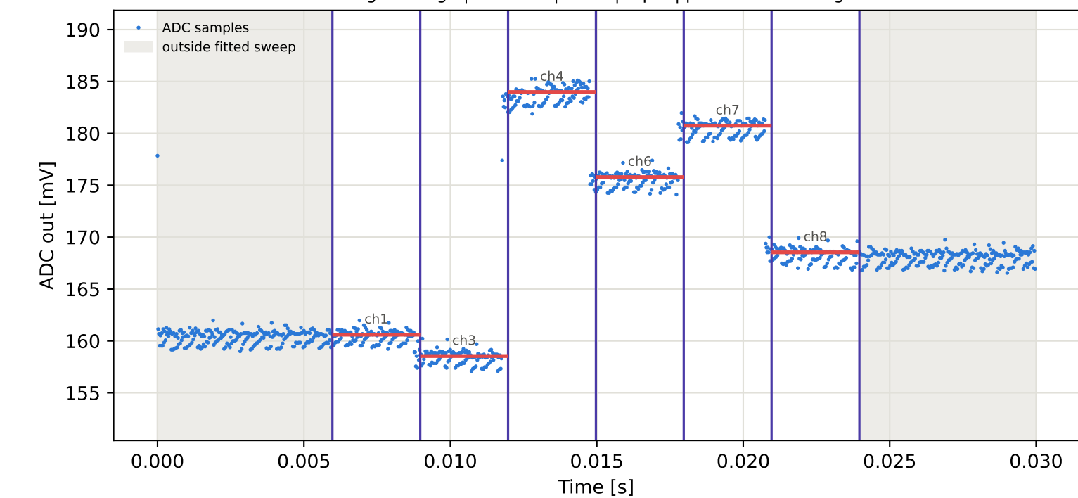
Tag9 &lt;- Tag7 | 775 MHz | run 0 | rep 1 | phase -104.70 deg
