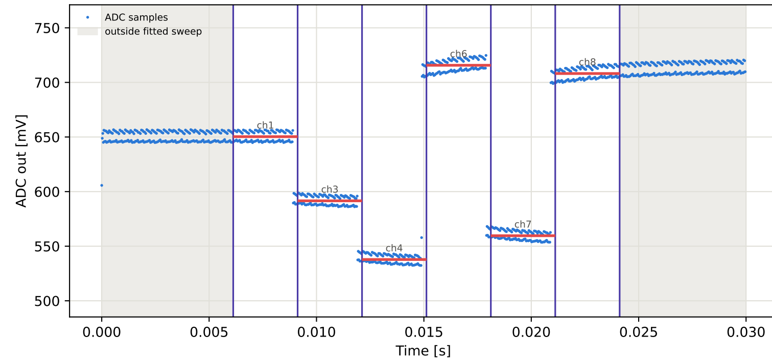
Tag3 &lt;- Tag16 | 935 MHz | run 0 | rep 1 | phase -119.54 deg
