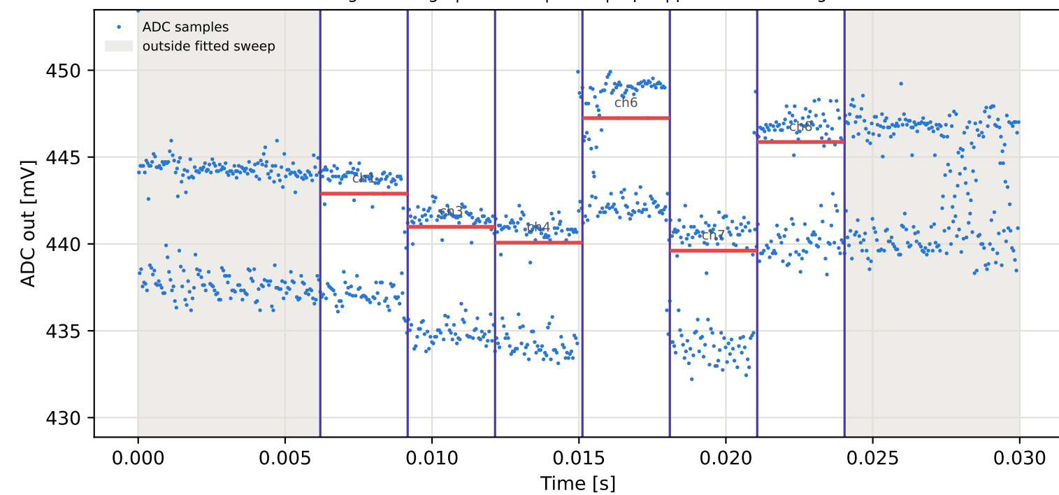
Tag15 &lt;- Tag4 | 885 MHz | run 0 | rep 1 | phase 96.82 deg
