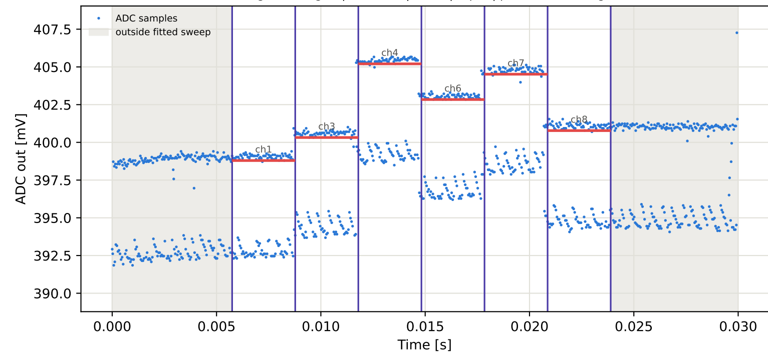
Tag10 &lt;- Tag2 | 825 MHz | run 0 | rep 1 | phase -111.52 deg
