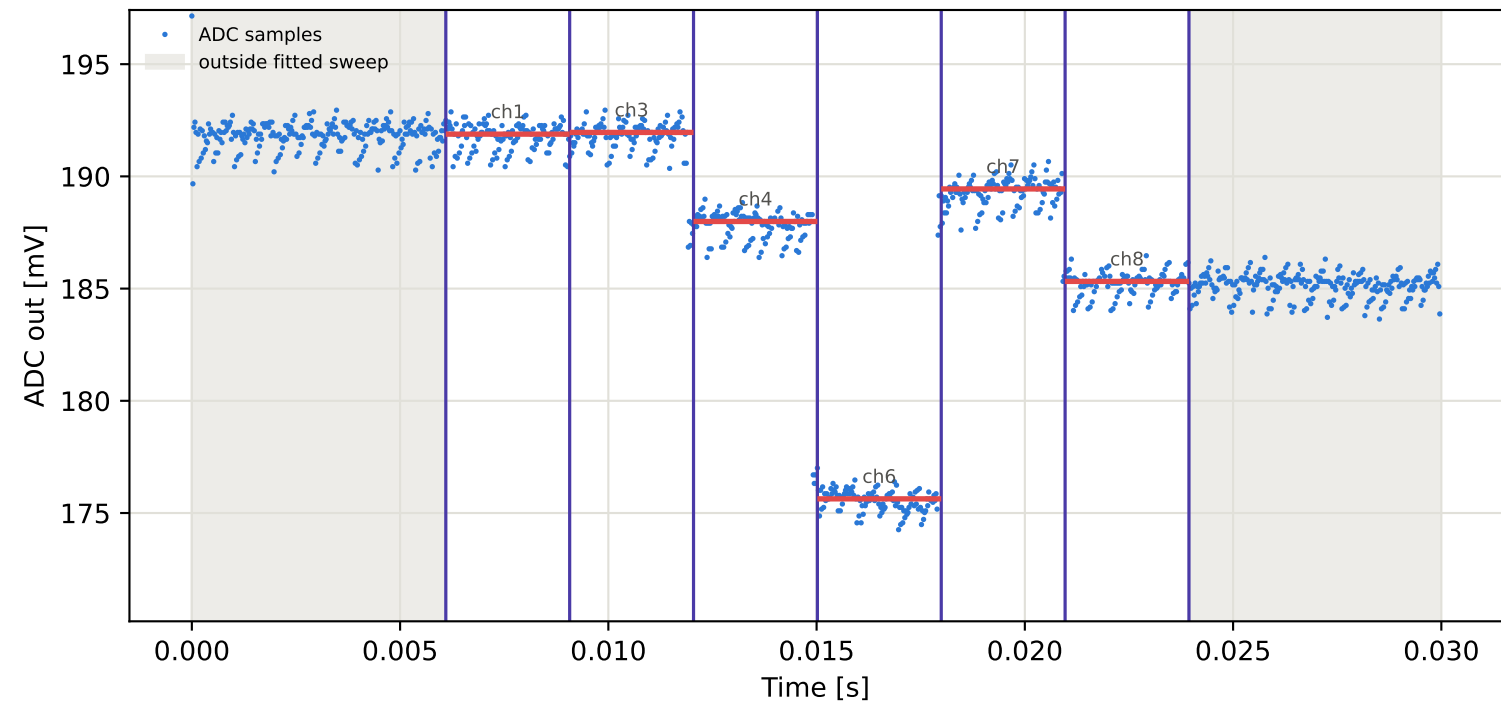
Tag4 &lt;- Tag16 | 905 MHz | run 0 | rep 1 | phase -83.71 deg
