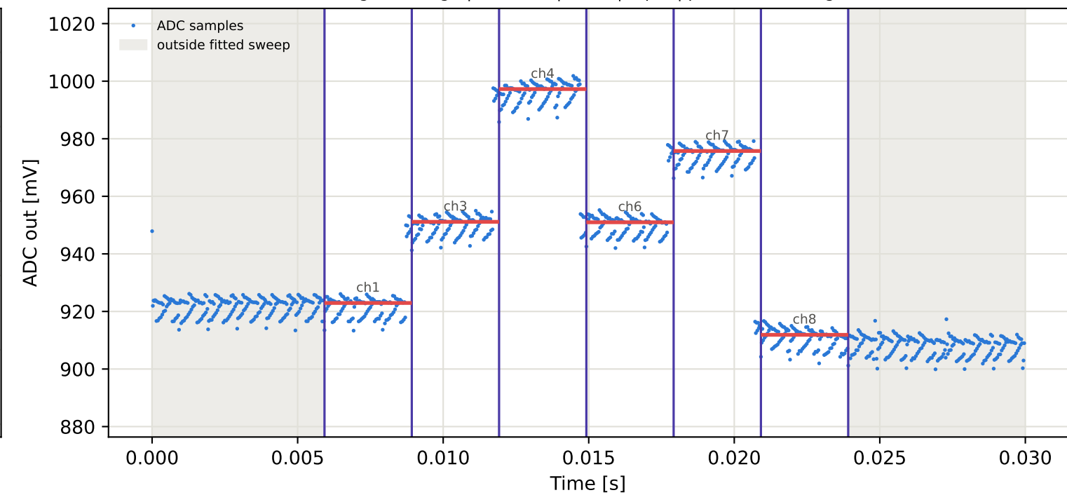
Tag10 &lt;- Tag9 | 935 MHz | run 0 | rep 1 | phase 92.34 deg
