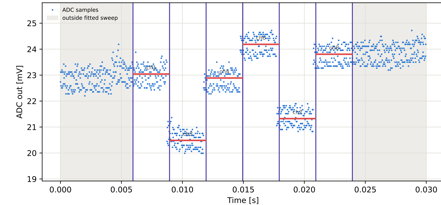
Tag1 &lt;- Tag9 | 775 MHz | run 0 | rep 1 | phase 124.87 deg
