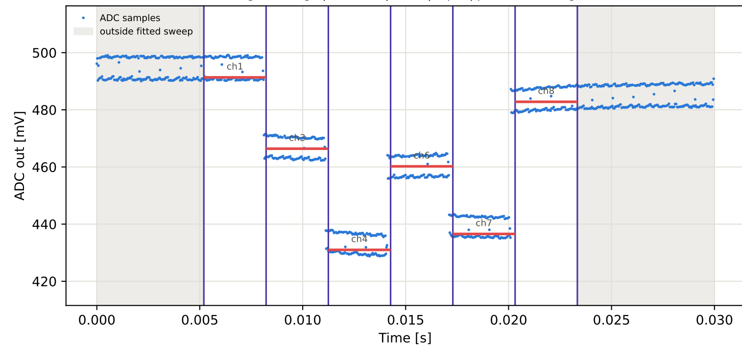
Tag2 &lt;- Tag10 | 845 MHz | run 0 | rep 1 | phase -163.81 deg
