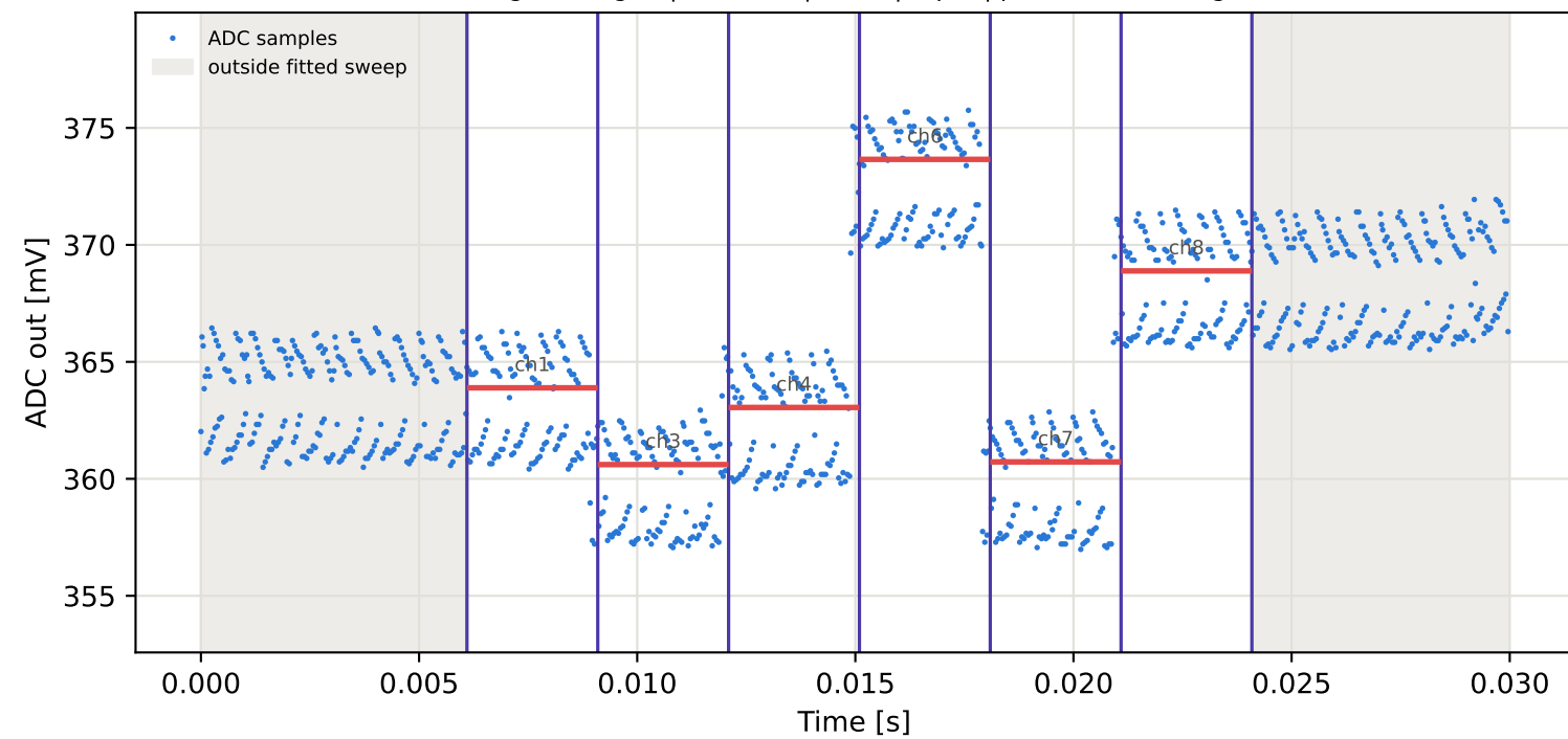
Tag6 &lt;- Tag3 | 985 MHz | run 0 | rep 1 | phase 177.45 deg
