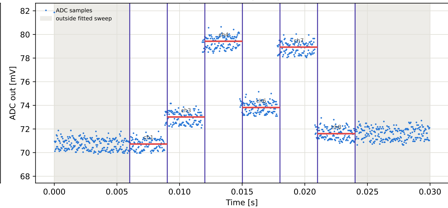
Tag6 &lt;- Tag5 | 775 MHz | run 0 | rep 1 | phase -79.49 deg
