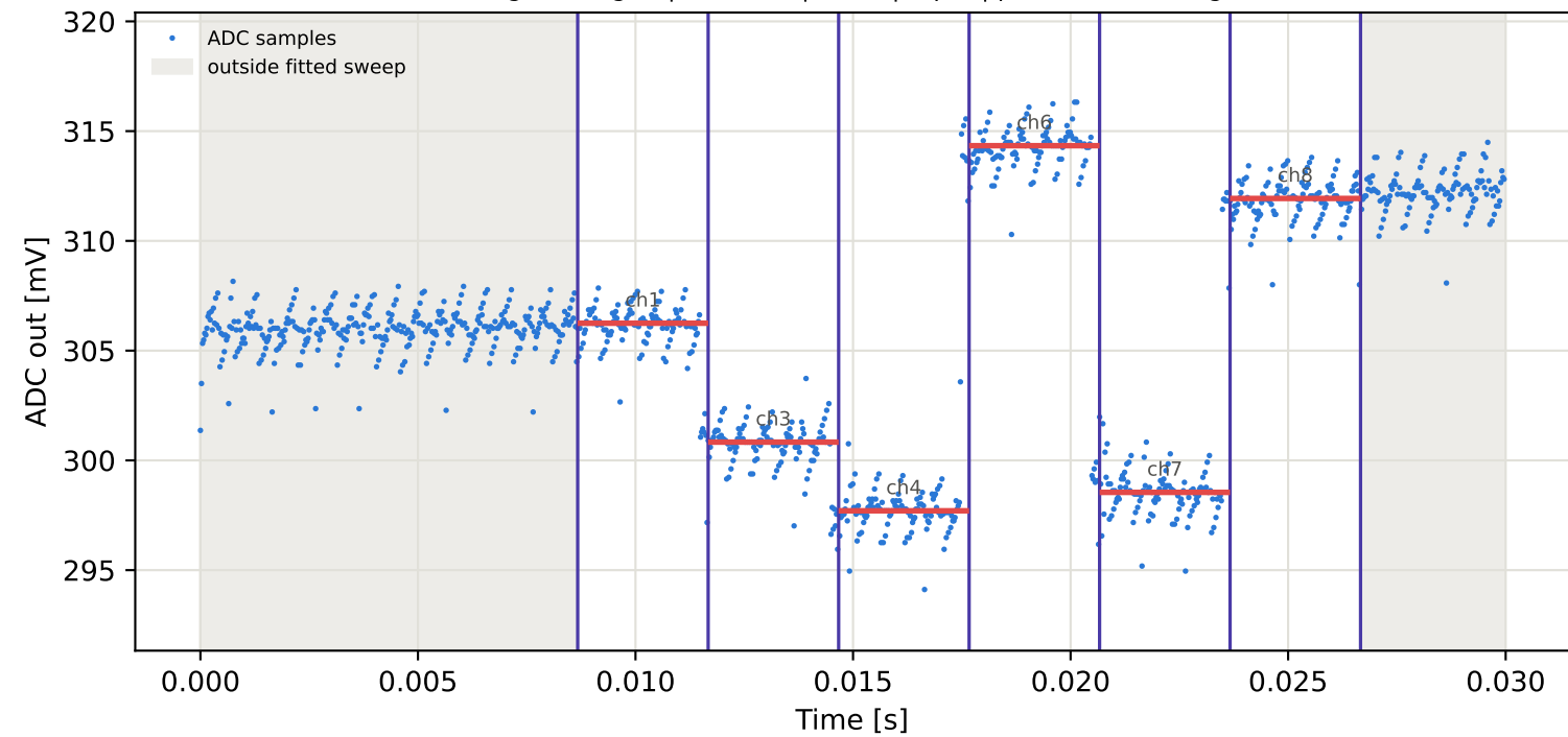
Tag6 &lt;- Tag3 | 955 MHz | run 0 | rep 1 | phase 136.70 deg
