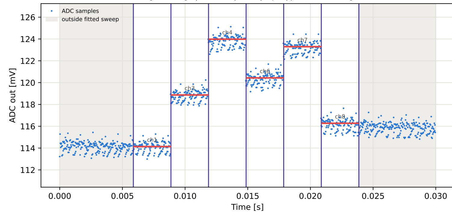
Tag15 &lt;- Tag9 | 805 MHz | run 0 | rep 1 | phase -109.78 deg
