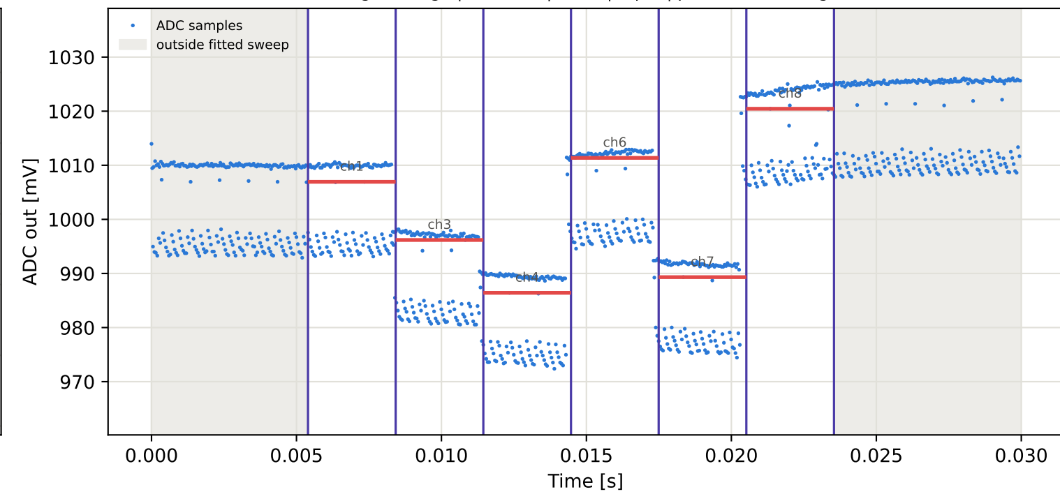
Tag3 &lt;- Tag7 | 905 MHz | run 0 | rep 1 | phase -84.19 deg
