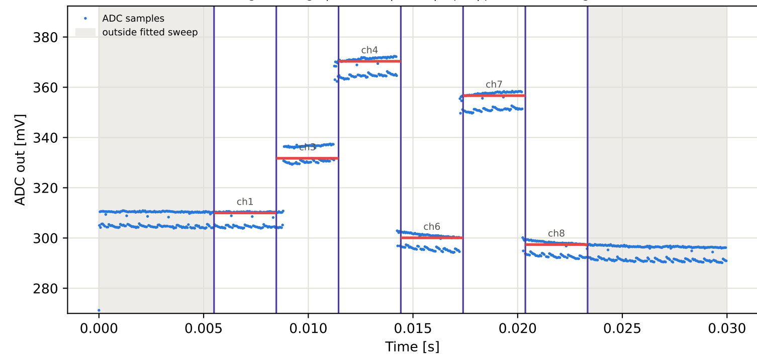
Tag10 &lt;- Tag9 | 975 MHz | run 0 | rep 1 | phase 171.63 deg
