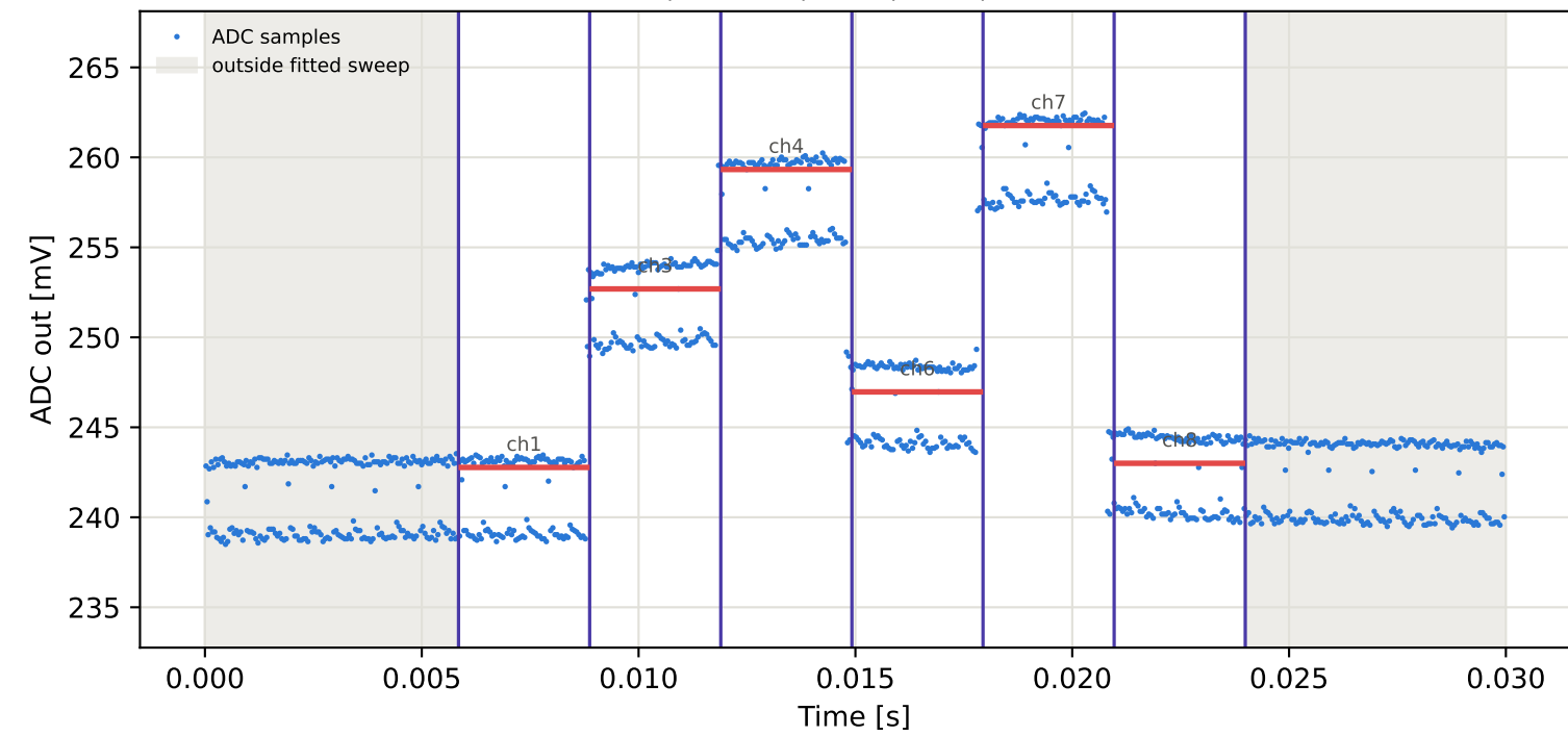
Tag9 &lt;- Tag8 | 805 MHz | run 0 | rep 1 | phase -63.70 deg
