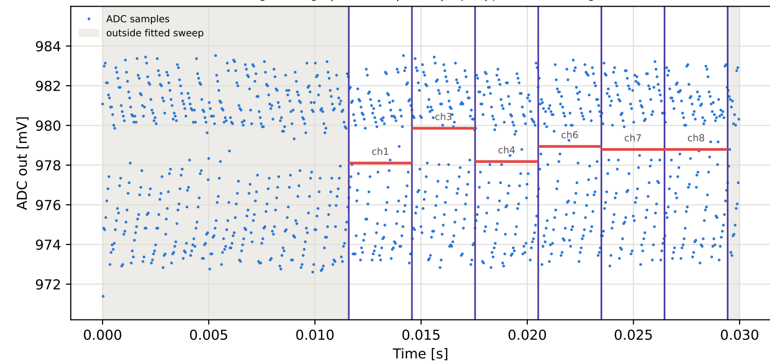
Tag7 &lt;- Tag15 | 865 MHz | run 0 | rep 1 | phase -14.58 deg
