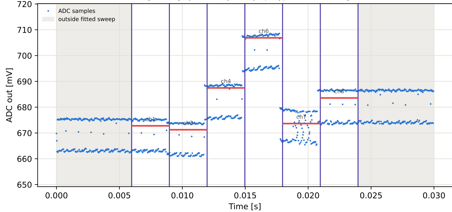
Tag8 &lt;- Tag5 | 975 MHz | run 0 | rep 1 | phase -55.50 deg
