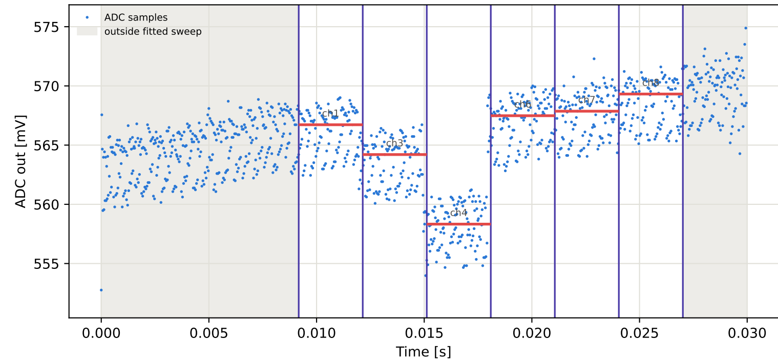
Tag5 &lt;- Tag4 | 875 MHz | run 0 | rep 1 | phase -176.71 deg
