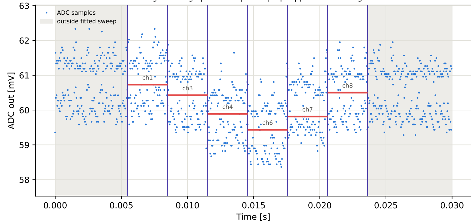
Tag15 &lt;- Tag4 | 845 MHz | run 0 | rep 1 | phase -106.80 deg
