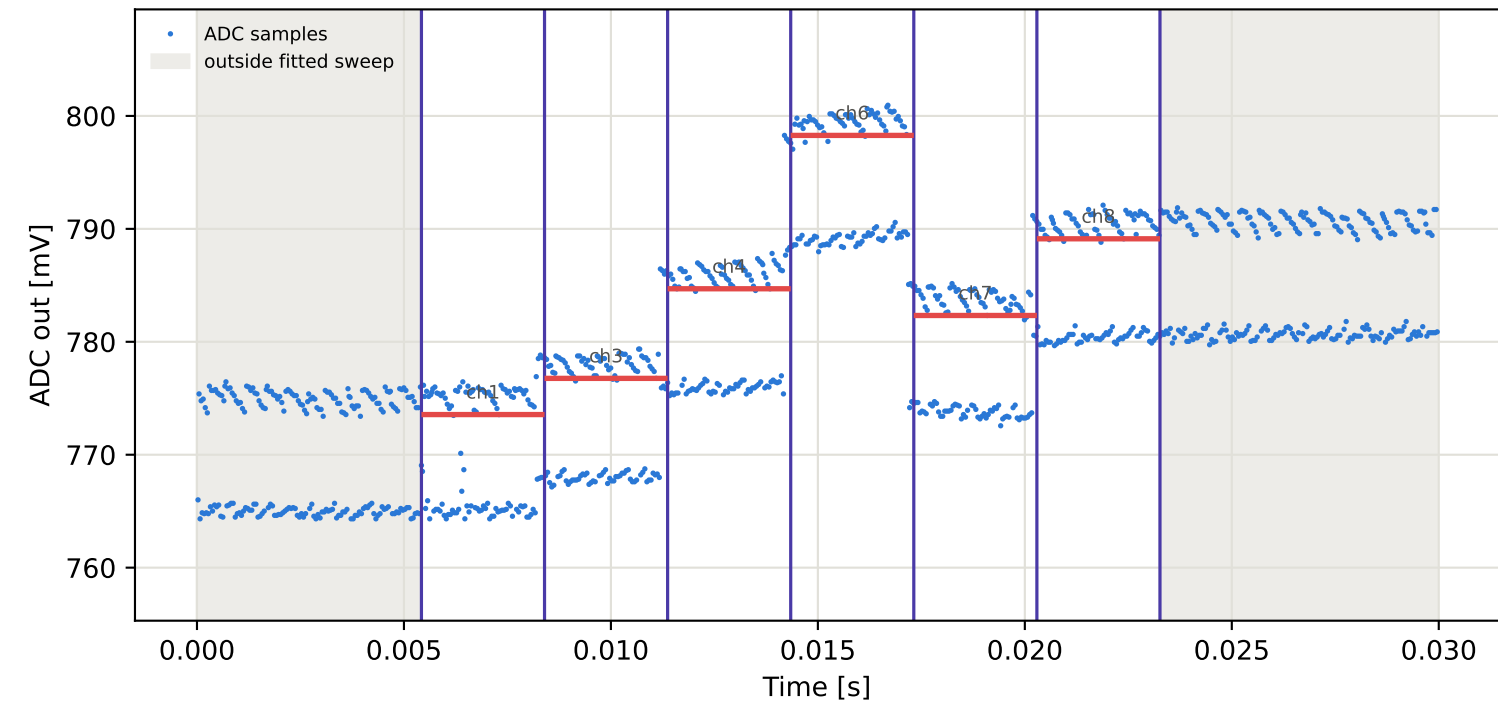
Tag9 &lt;- Tag2 | 895 MHz | run 0 | rep 1 | phase 121.45 deg
