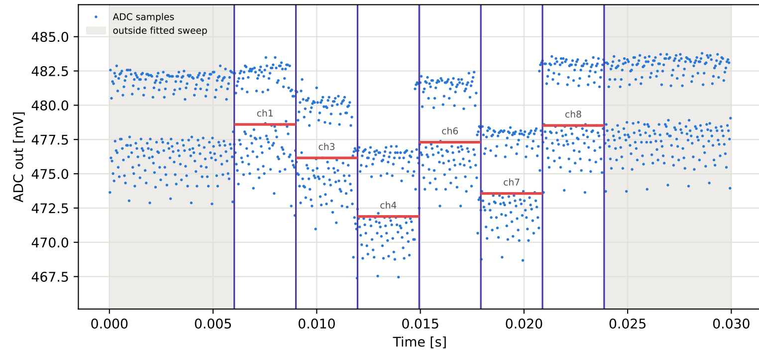
Tag3 &lt;- Tag2 | 965 MHz | run 0 | rep 1 | phase 117.14 deg
