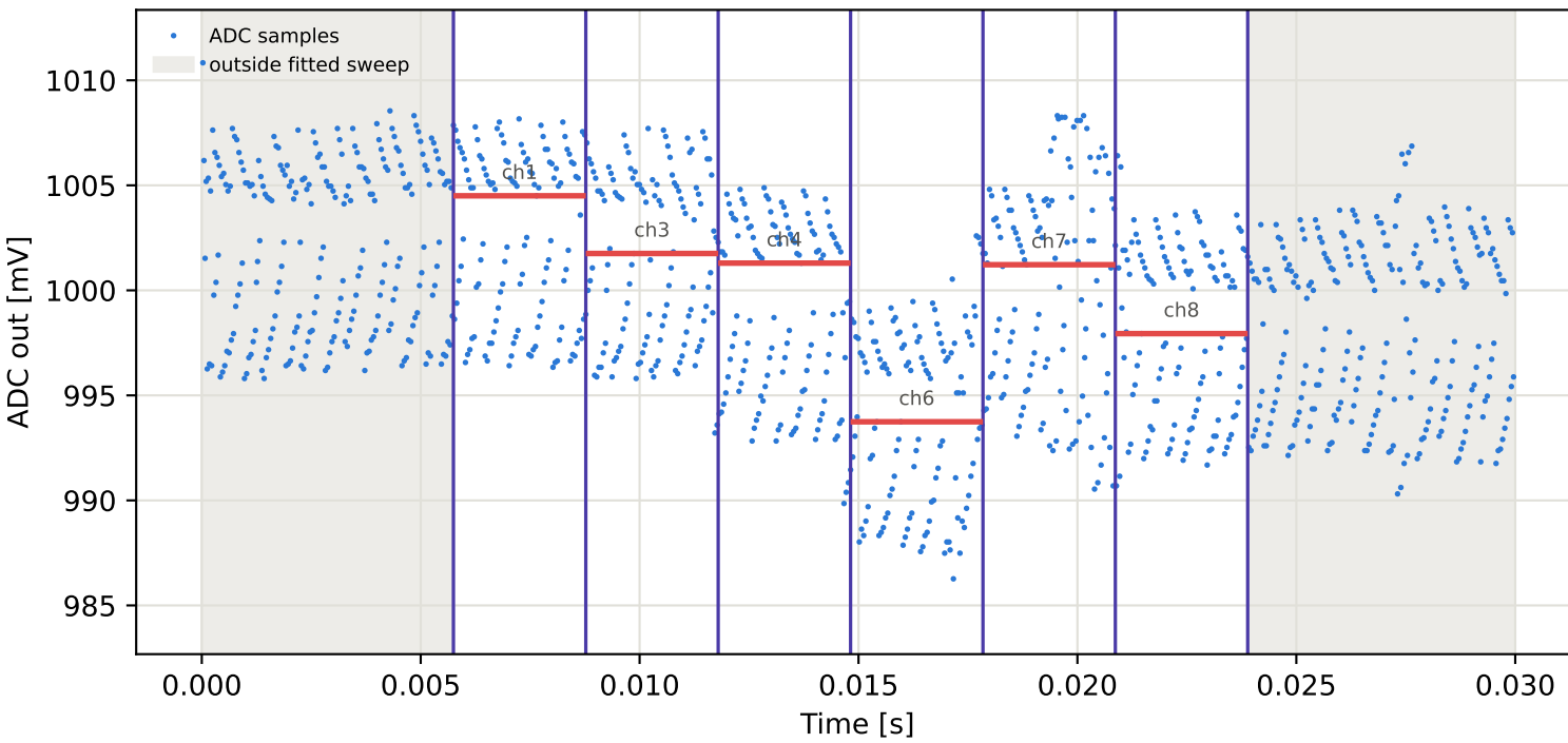
Tag8 &lt;- Tag15 | 905 MHz | run 0 | rep 1 | phase 107.48 deg
