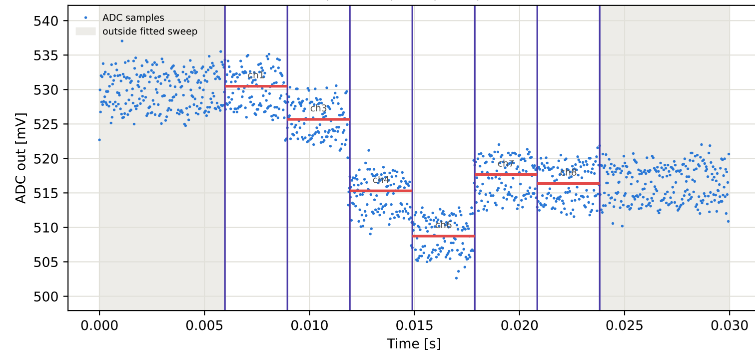
Tag2 &lt;- Tag7 | 885 MHz | run 0 | rep 1 | phase 40.92 deg
