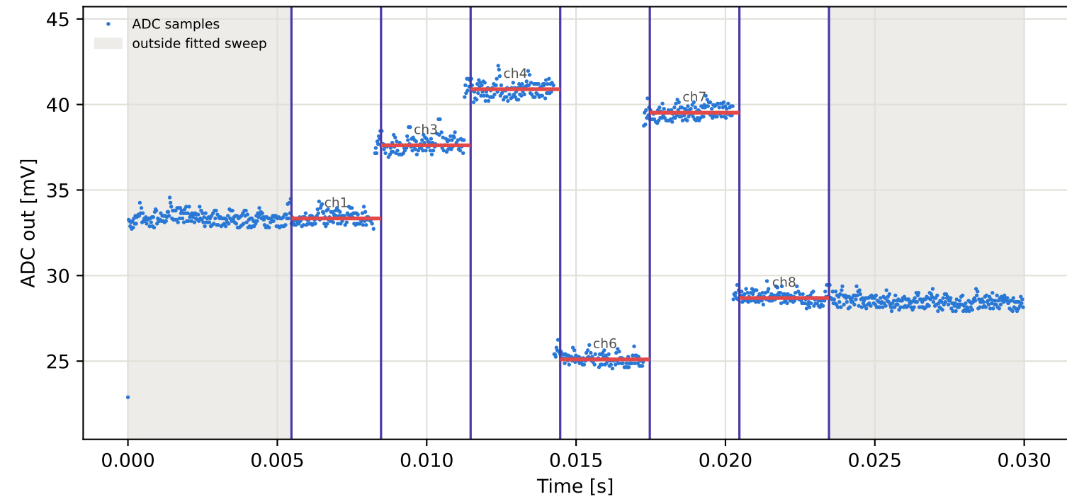
Tag15 &lt;- Tag6 | 965 MHz | run 0 | rep 1 | phase 138.05 deg
