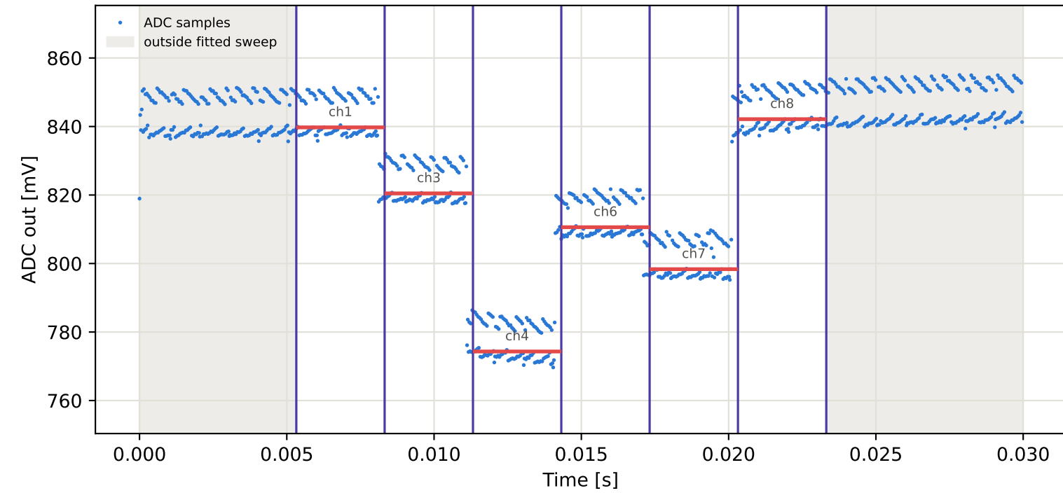
Tag9 &lt;- Tag7 | 945 MHz | run 0 | rep 1 | phase 73.45 deg
