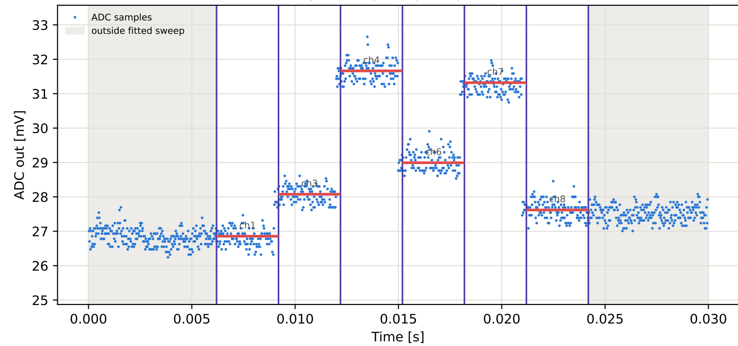
Tag6 &lt;- Tag5 | 785 MHz | run 0 | rep 1 | phase -86.15 deg
