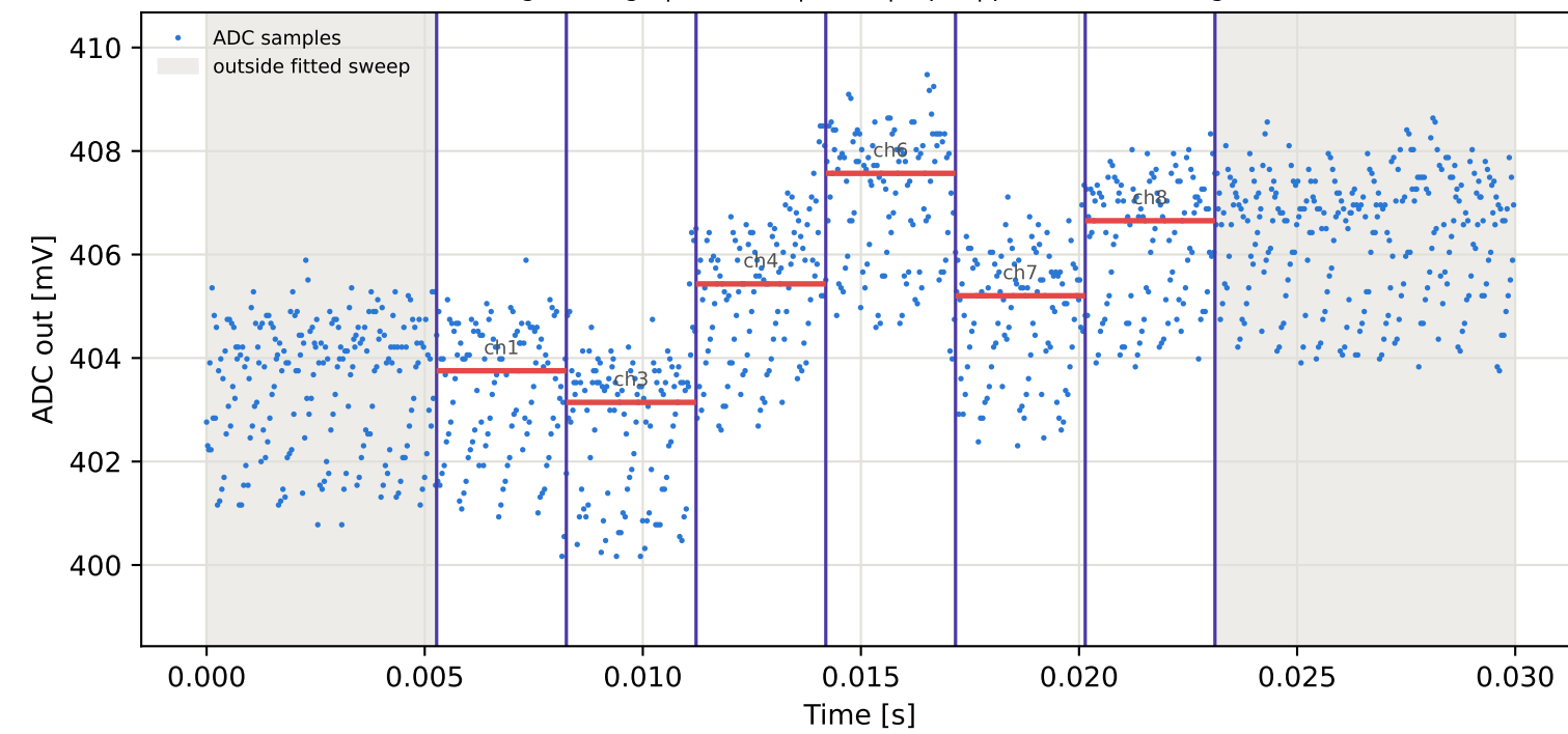
Tag3 &lt;- Tag10 | 865 MHz | run 0 | rep 1 | phase 42.37 deg
