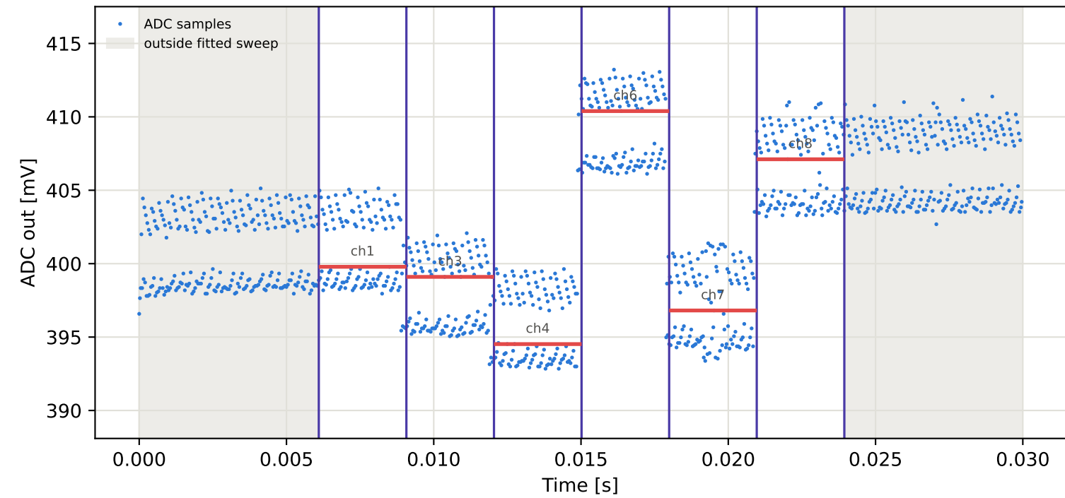
Tag1 &lt;- Tag4 | 995 MHz | run 0 | rep 1 | phase -162.97 deg
