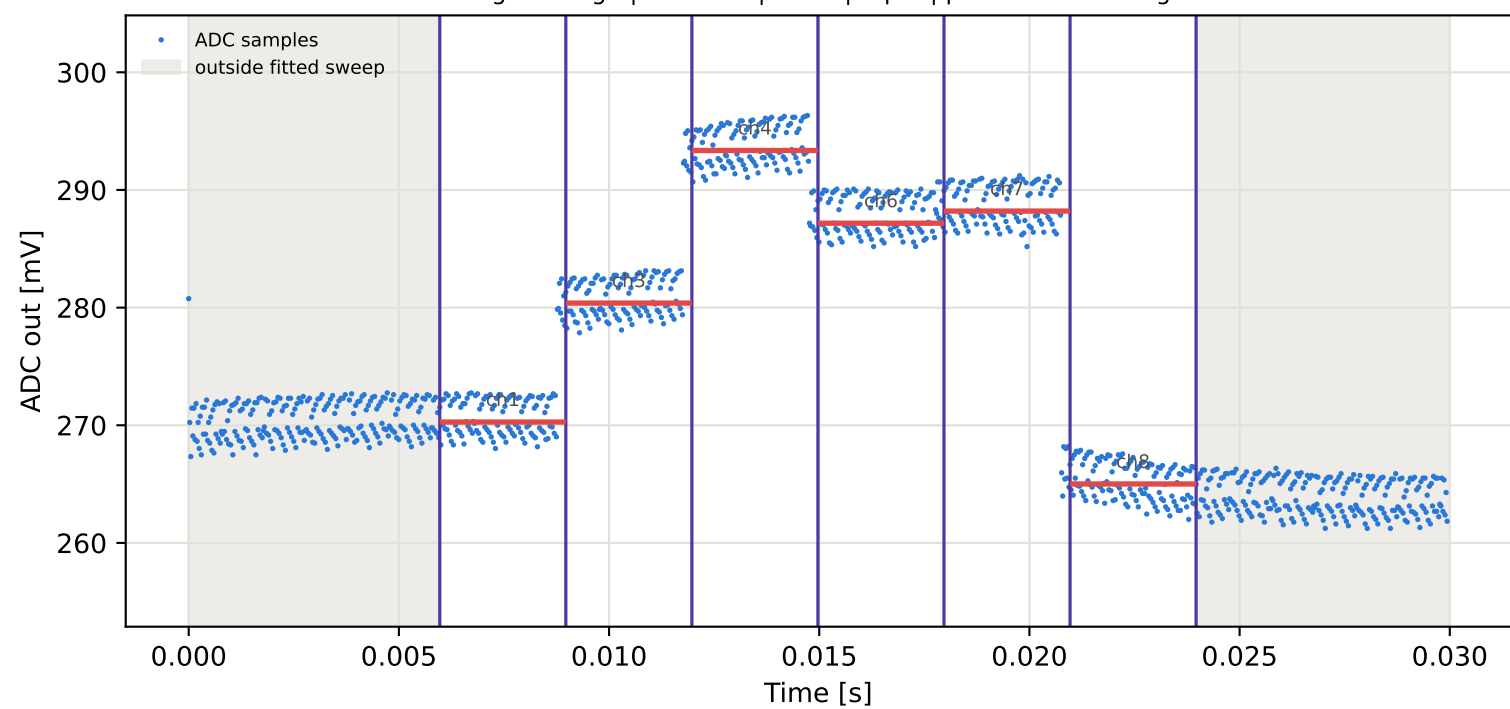
Tag1 &lt;- Tag4 | 915 MHz | run 0 | rep 1 | phase 150.28 deg
