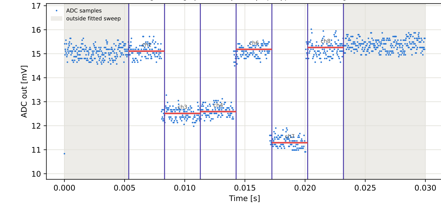
Tag16 &lt;- Tag6 | 795 MHz | run 0 | rep 1 | phase -82.01 deg
