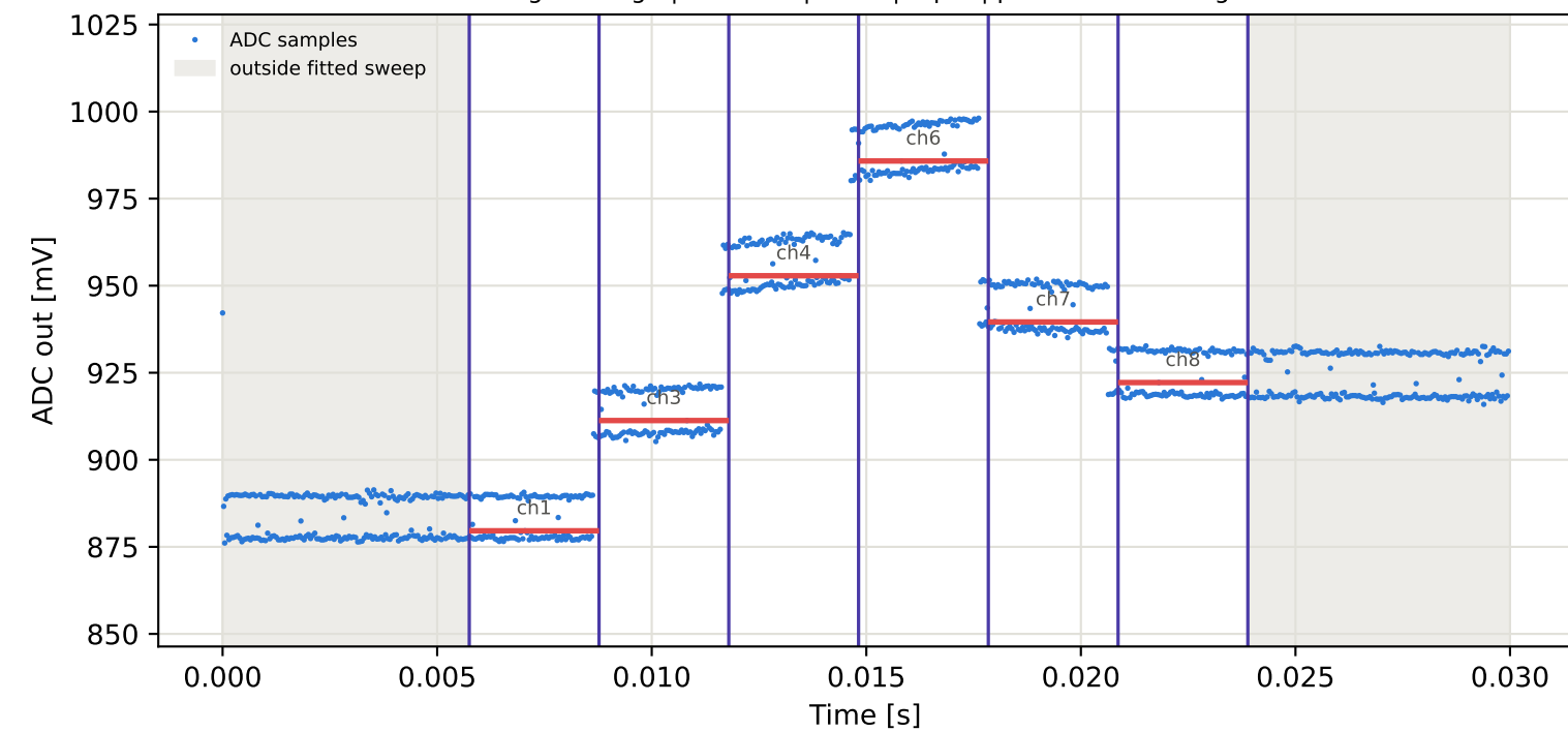
Tag9 &lt;- Tag5 | 885 MHz | run 0 | rep 1 | phase 162.78 deg
