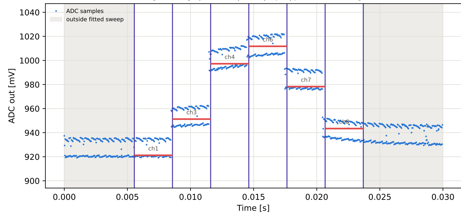
Tag16 &lt;- Tag5 | 915 MHz | run 0 | rep 1 | phase -175.92 deg
