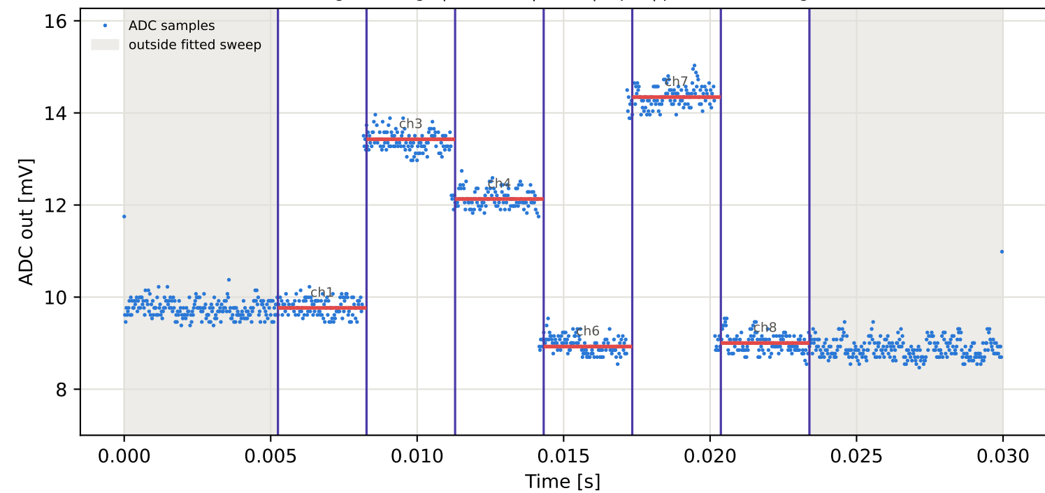
Tag16 &lt;- Tag5 | 795 MHz | run 0 | rep 1 | phase -119.32 deg
