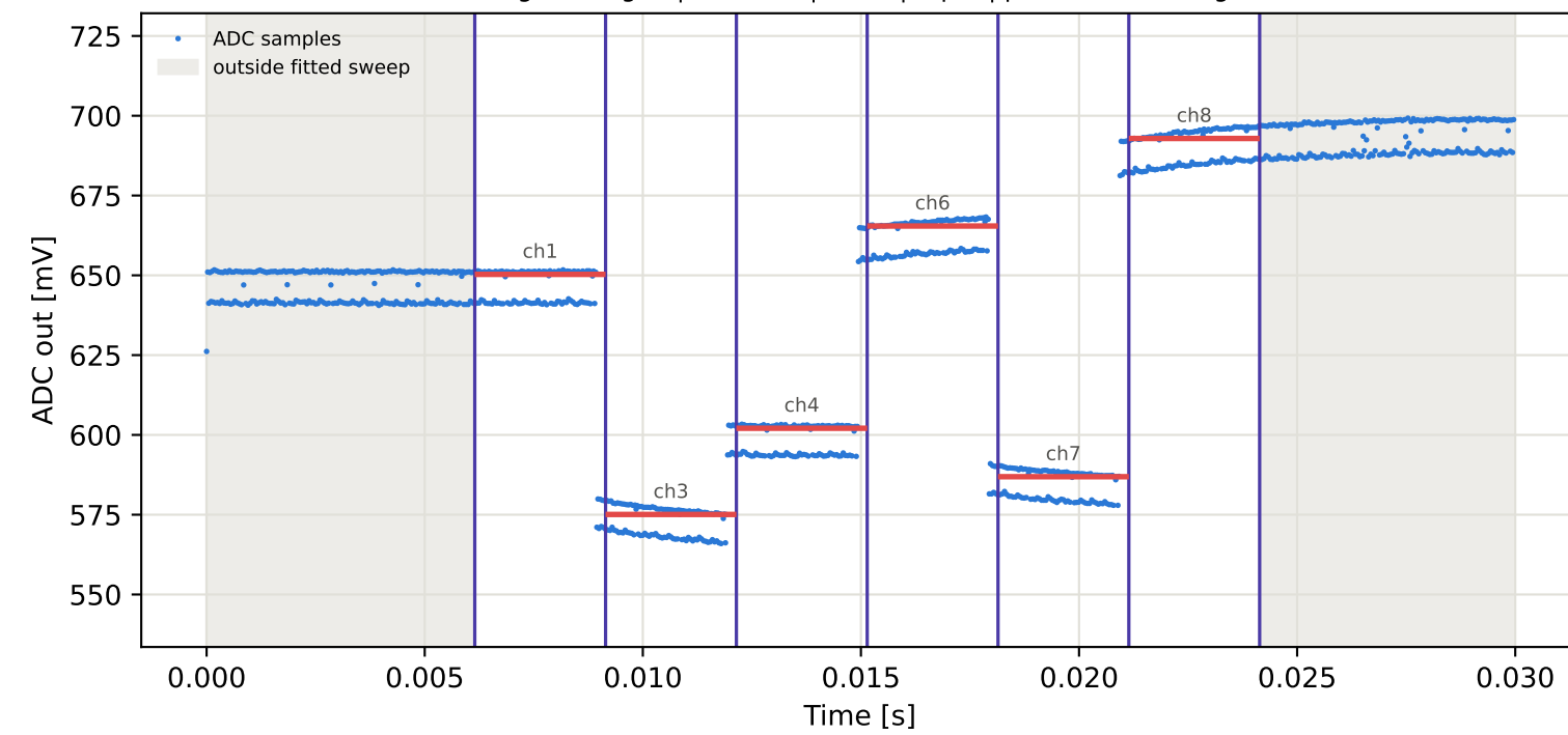
Tag3 &lt;- Tag16 | 865 MHz | run 0 | rep 1 | phase 152.17 deg
