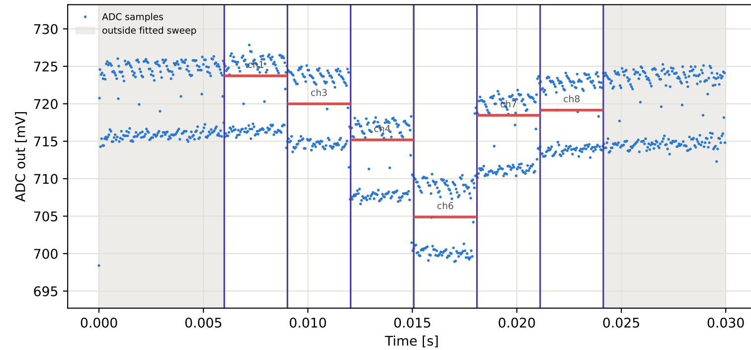
Tag6 &lt;- Tag4 | 875 MHz | run 0 | rep 1 | phase -16.32 deg
