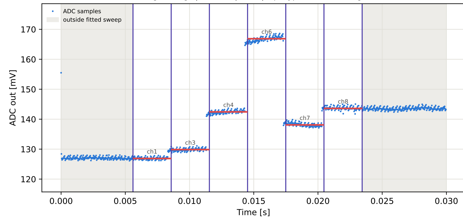
Tag1 &lt;- Tag7 | 905 MHz | run 0 | rep 1 | phase -1.33 deg
