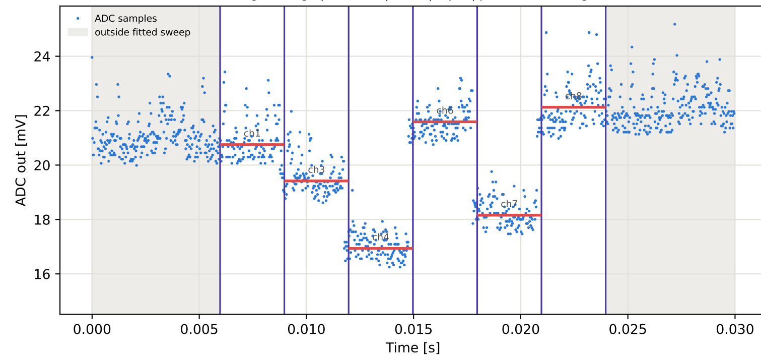
Tag2 &lt;- Tag5 | 975 MHz | run 0 | rep 1 | phase -99.10 deg
