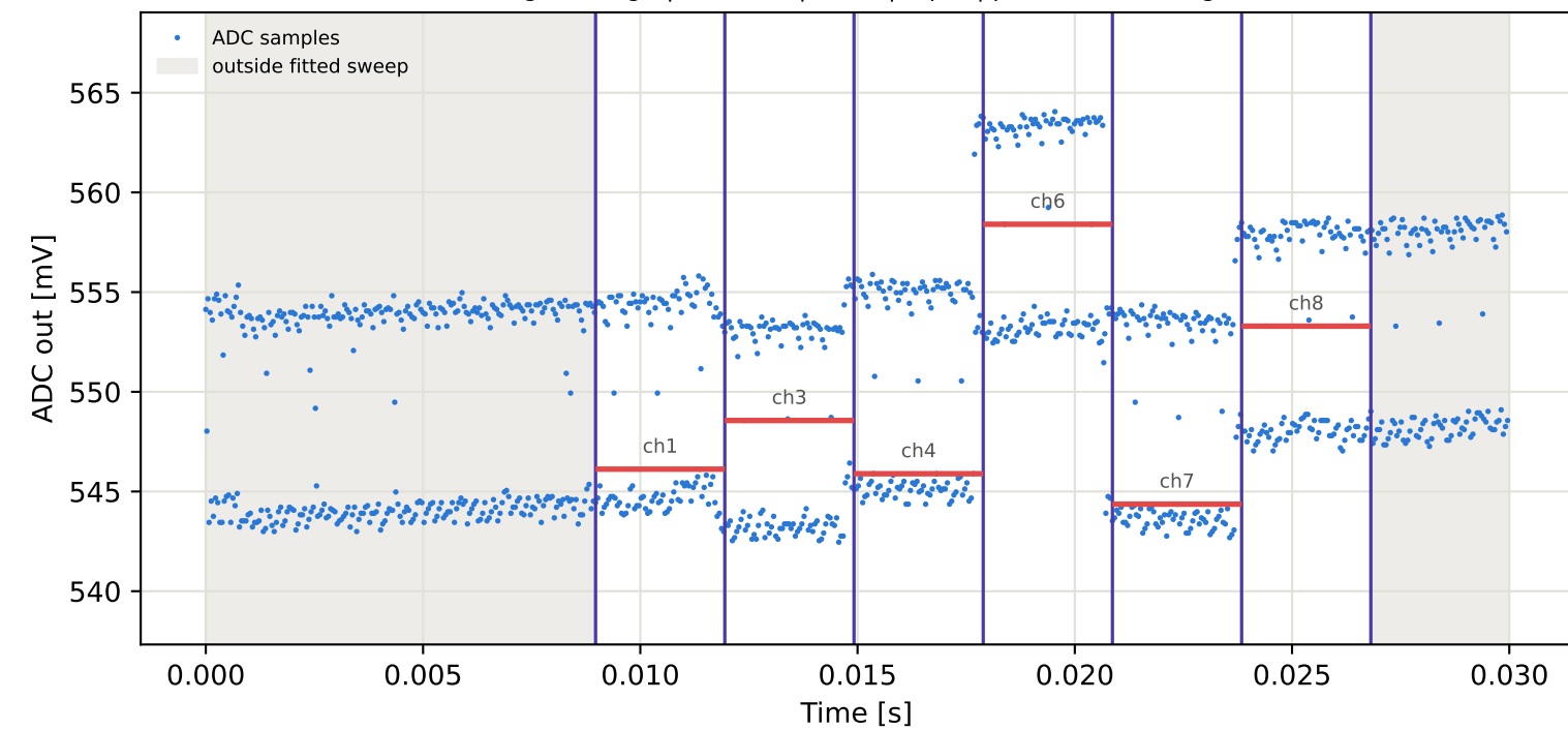
Tag3 &lt;- Tag6 | 955 MHz | run 0 | rep 1 | phase 139.33 deg
