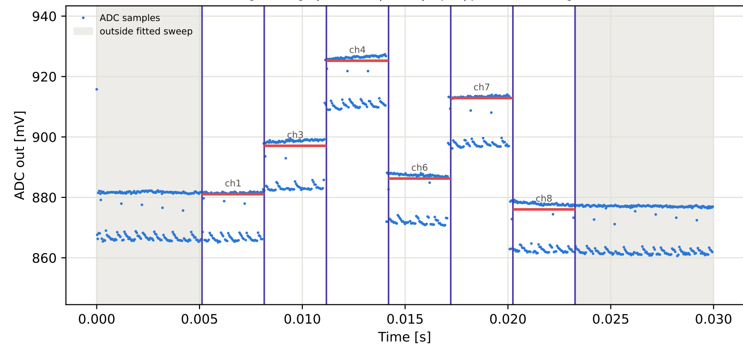
Tag8 &lt;- Tag10 | 995 MHz | run 0 | rep 1 | phase 66.39 deg
