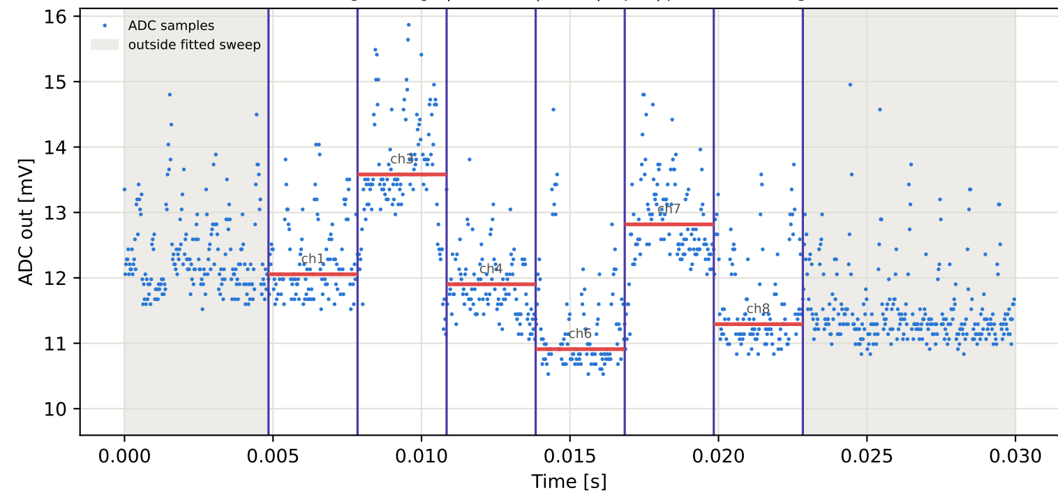
Tag2 &lt;- Tag6 | 795 MHz | run 0 | rep 1 | phase -133.18 deg
