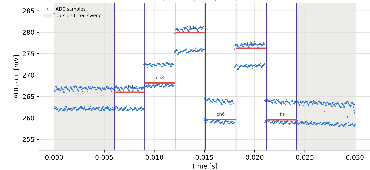
Tag16 &lt;- Tag6 | 995 MHz | run 0 | rep 1 | phase -69.39 deg
