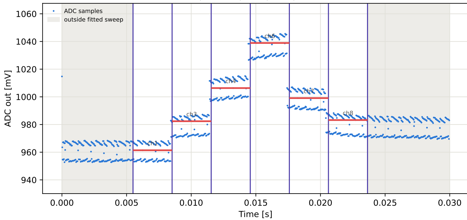
Tag8 &lt;- Tag16 | 905 MHz | run 0 | rep 1 | phase -137.06 deg
