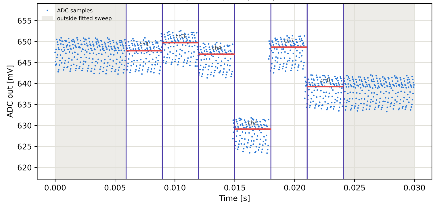
Tag3 &lt;- Tag15 | 925 MHz | run 0 | rep 1 | phase 21.20 deg
