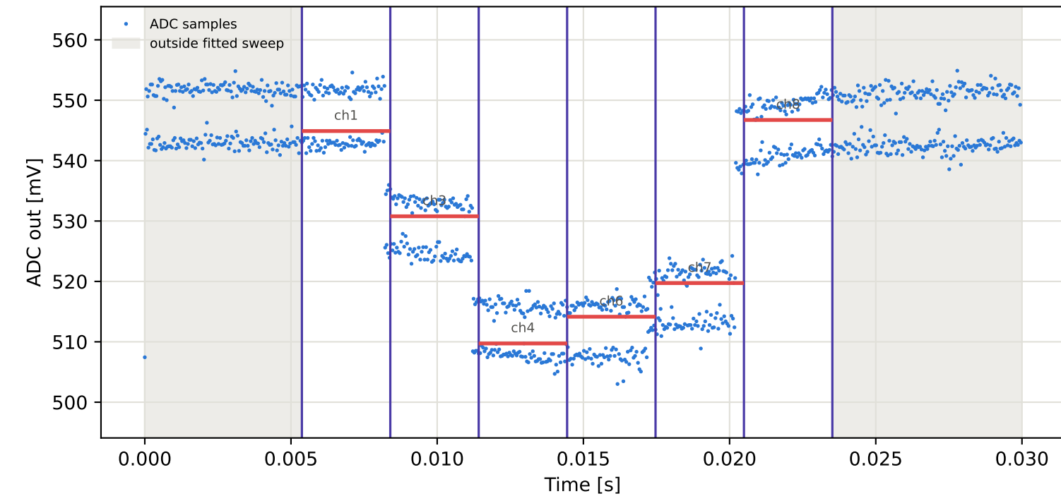
Tag2 &lt;- Tag16 | 885 MHz | run 0 | rep 1 | phase -8.17 deg
