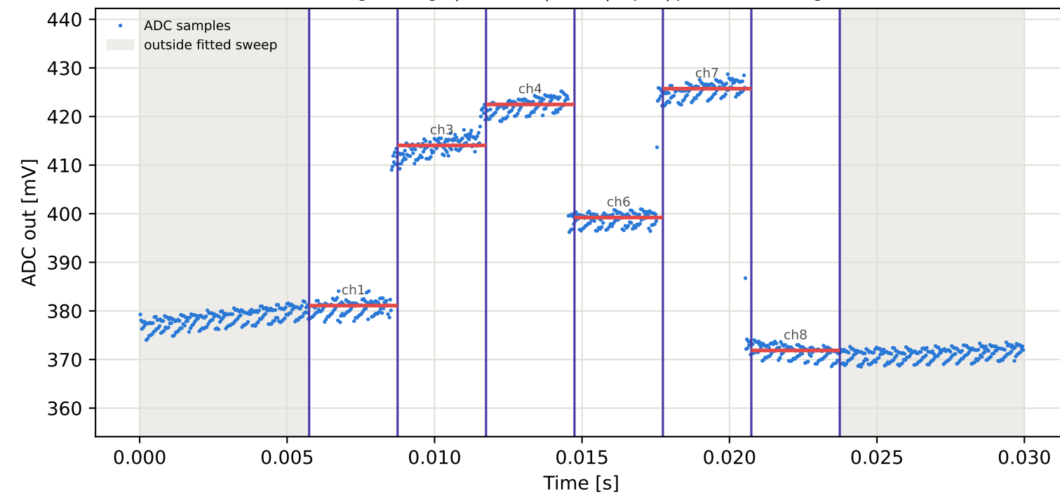
Tag4 &lt;- Tag7 | 875 MHz | run 0 | rep 1 | phase 36.27 deg
