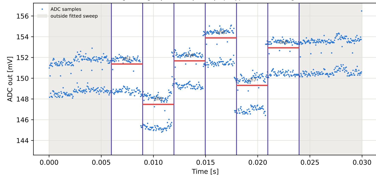
Tag3 &lt;- Tag2 | 795 MHz | run 0 | rep 1 | phase 148.87 deg
