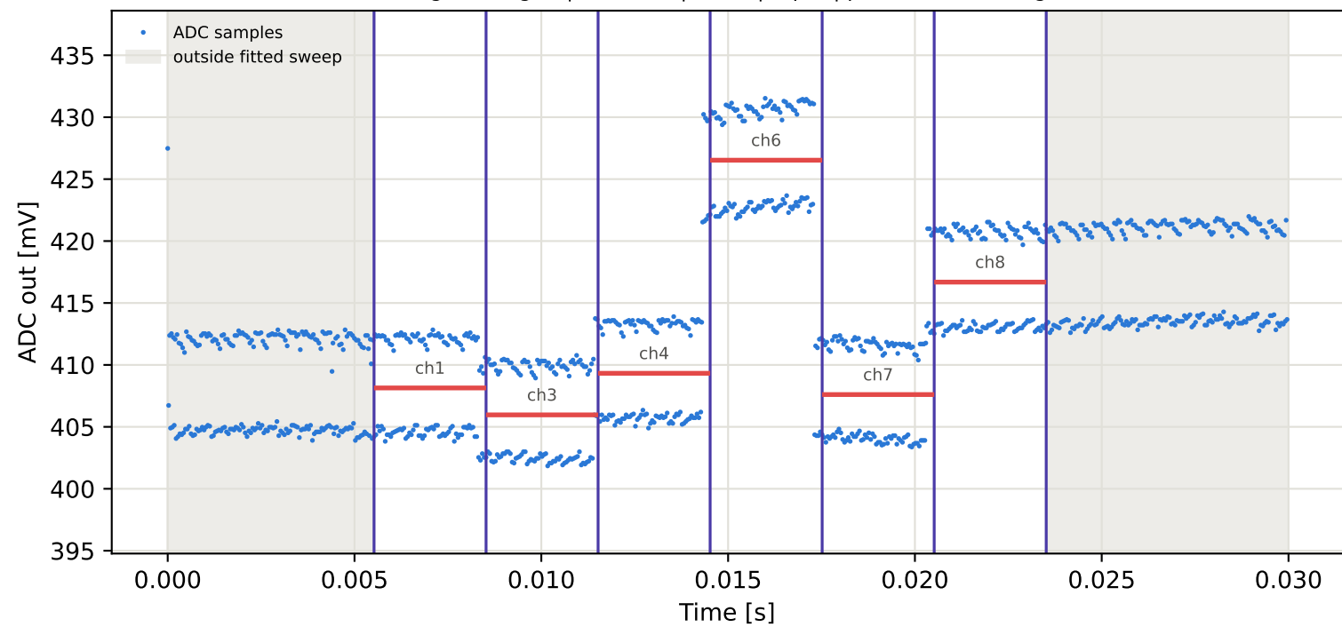
Tag5 &lt;- Tag2 | 925 MHz | run 0 | rep 1 | phase -59.15 deg
