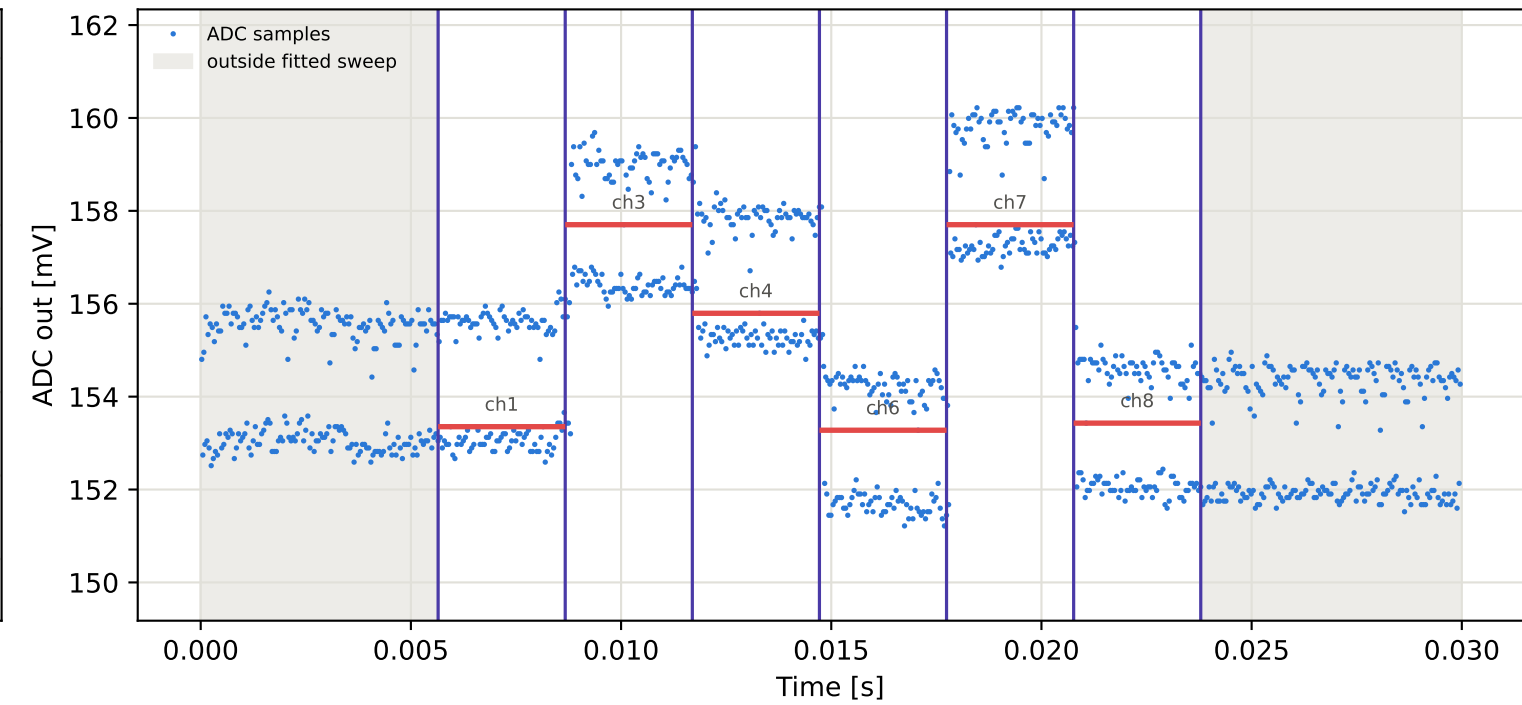
Tag9 &lt;- Tag2 | 785 MHz | run 0 | rep 1 | phase 131.41 deg
