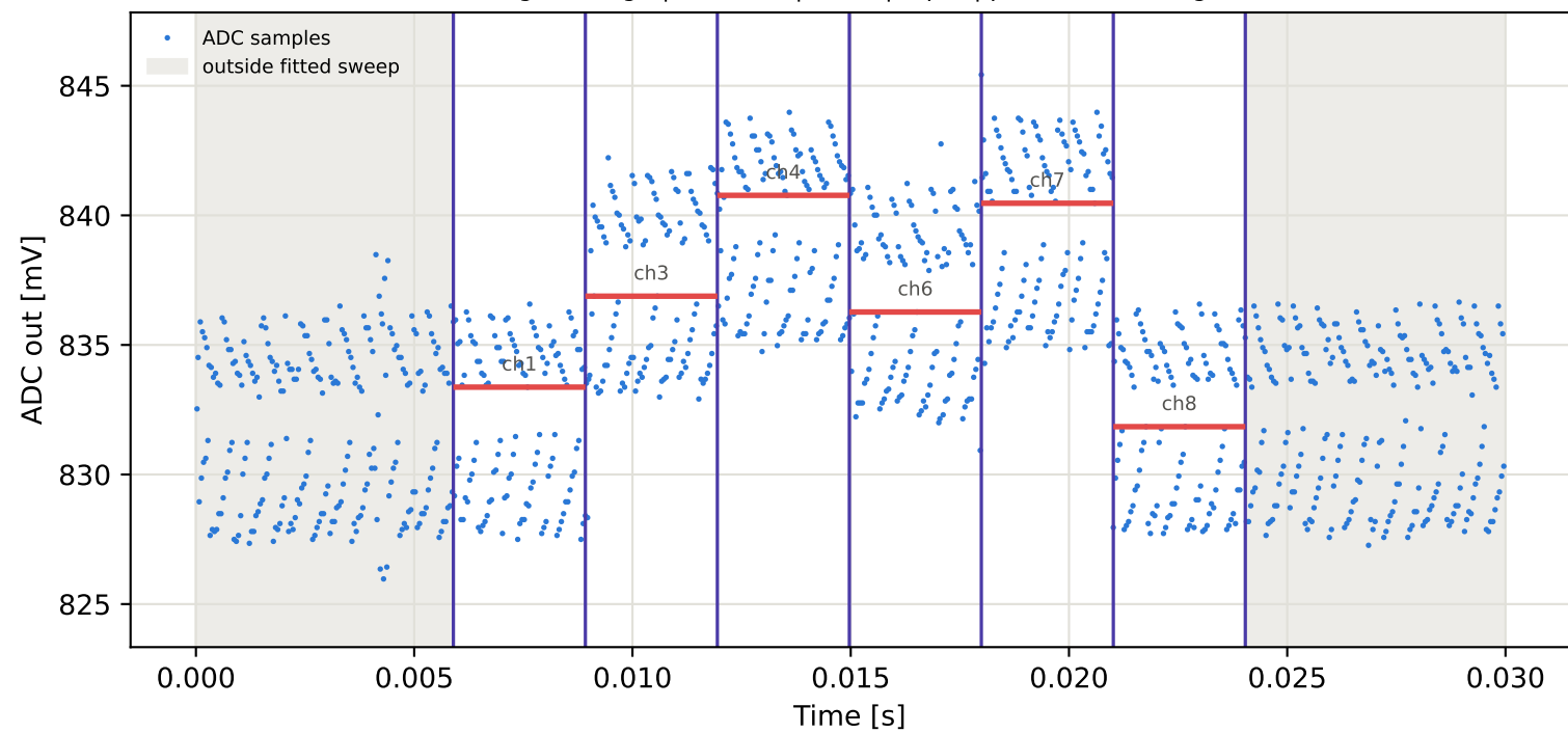
Tag9 &lt;- Tag6 | 865 MHz | run 0 | rep 1 | phase -151.92 deg
