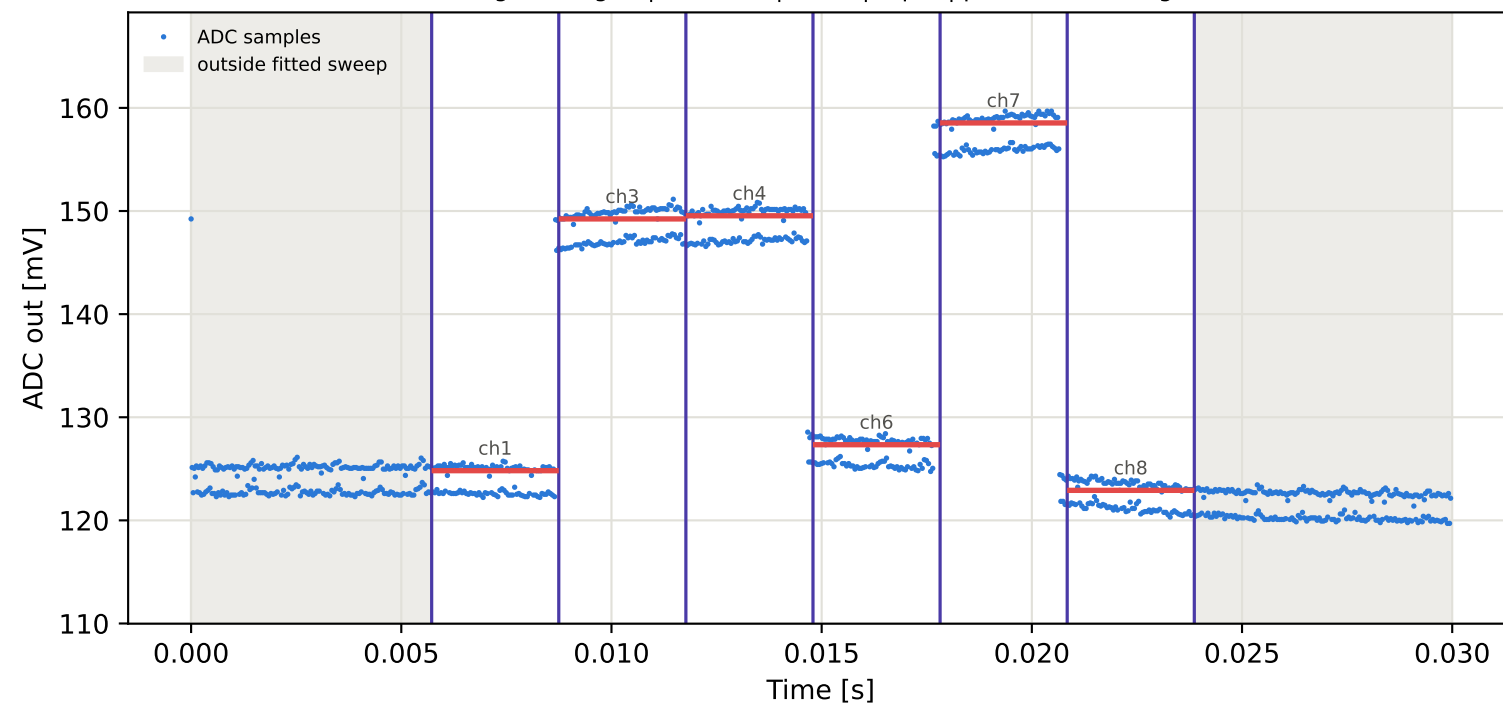
Tag3 &lt;- Tag16 | 795 MHz | run 0 | rep 1 | phase 129.35 deg
