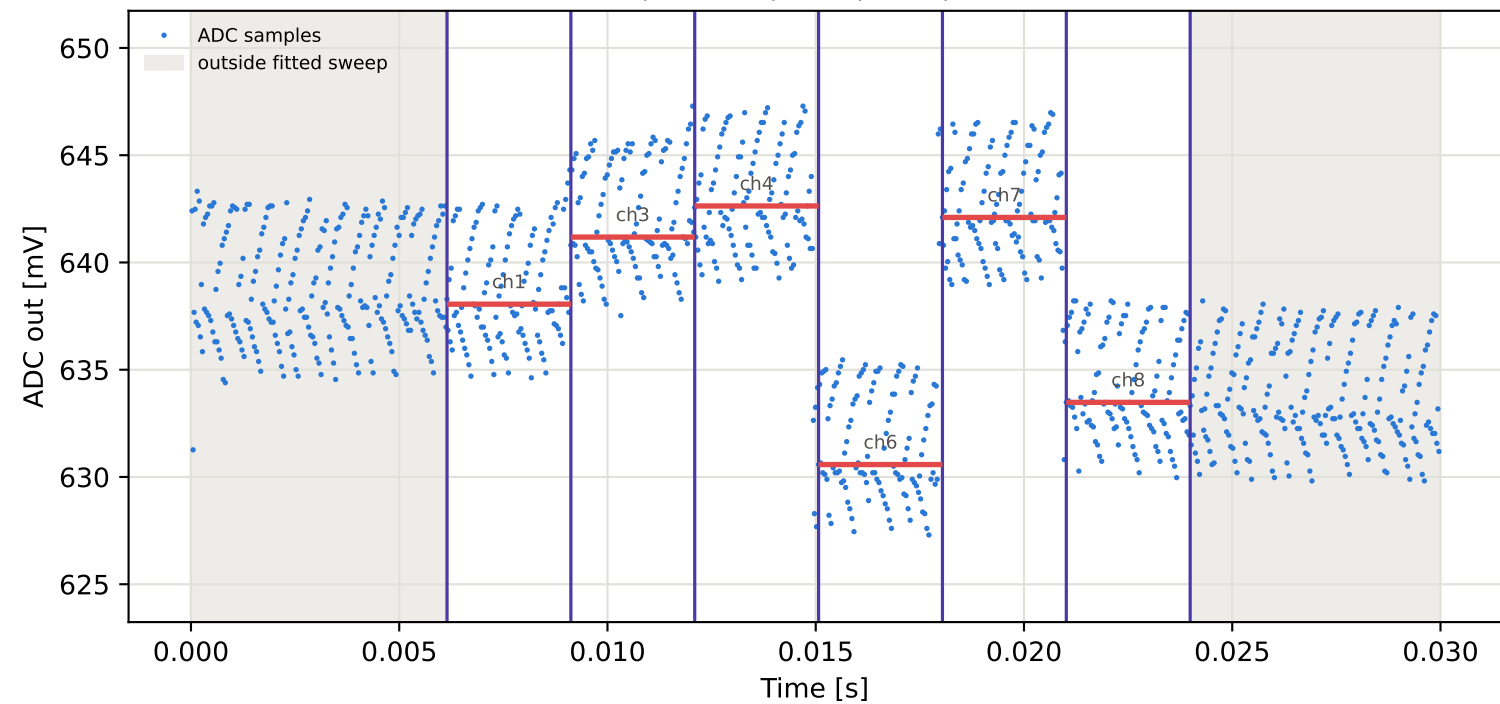
Tag10 &lt;- Tag4 | 945 MHz | run 0 | rep 1 | phase -25.61 deg
