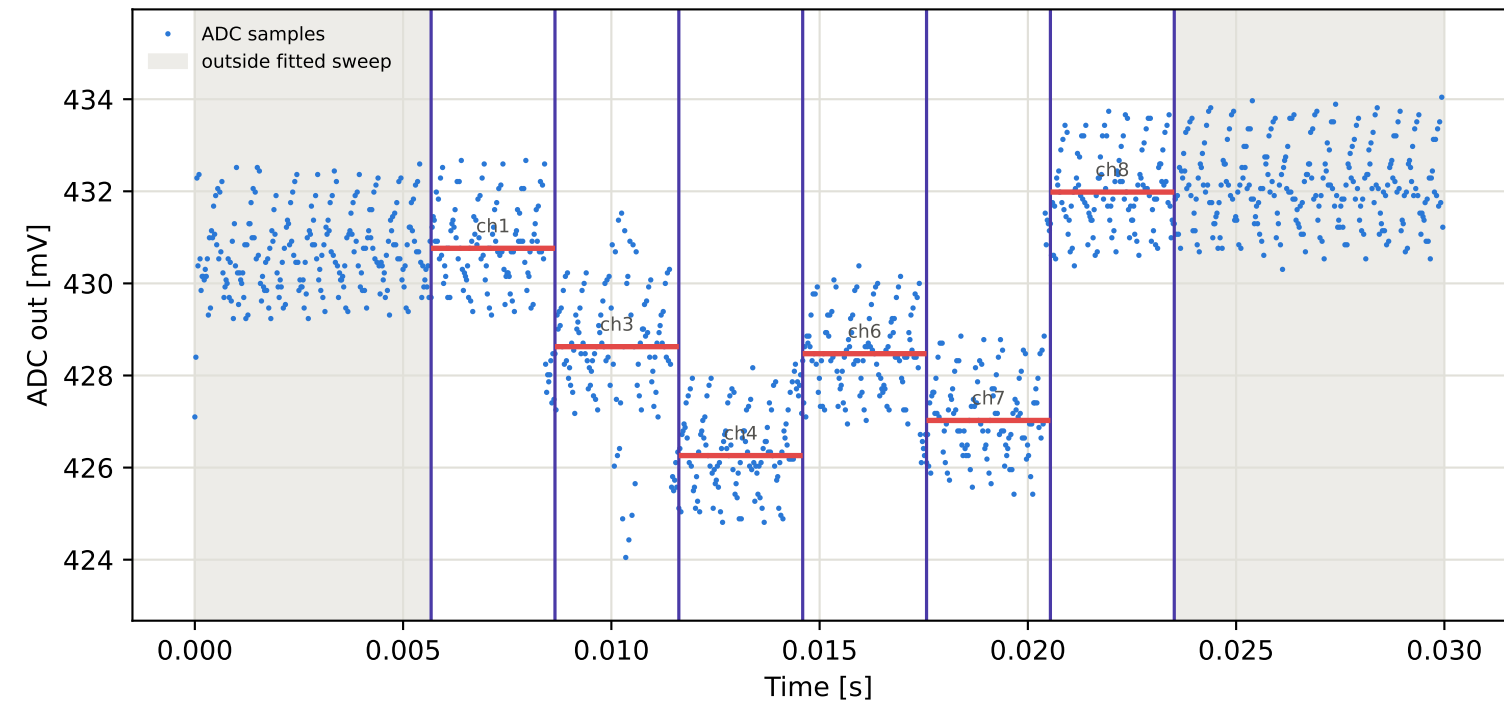
Tag5 &lt;- Tag4 | 845 MHz | run 0 | rep 1 | phase 164.21 deg
