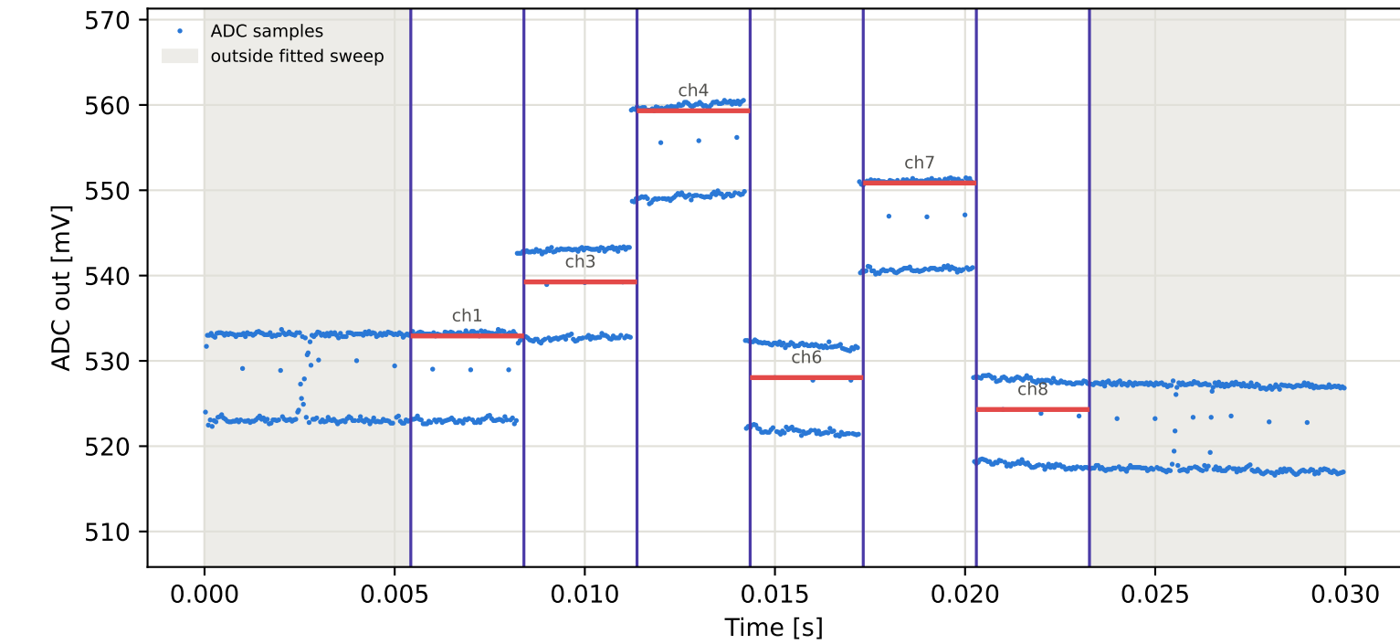
Tag16 &lt;- Tag6 | 965 MHz | run 0 | rep 1 | phase 177.29 deg
