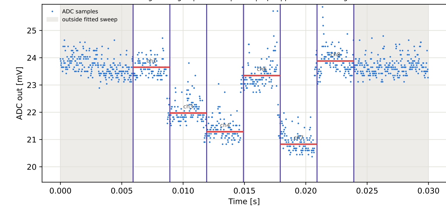
Tag2 &lt;- Tag15 | 805 MHz | run 0 | rep 1 | phase 128.59 deg
