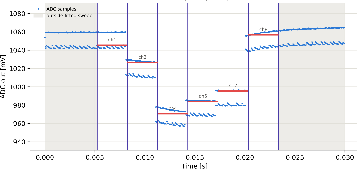
Tag7 &lt;- Tag10 | 915 MHz | run 0 | rep 1 | phase 66.74 deg
