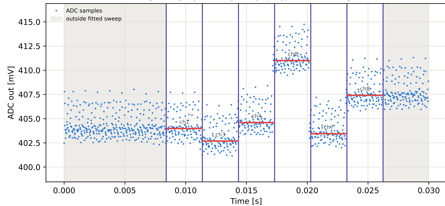
Tag1 &lt;- Tag2 | 955 MHz | run 0 | rep 1 | phase 132.84 deg
