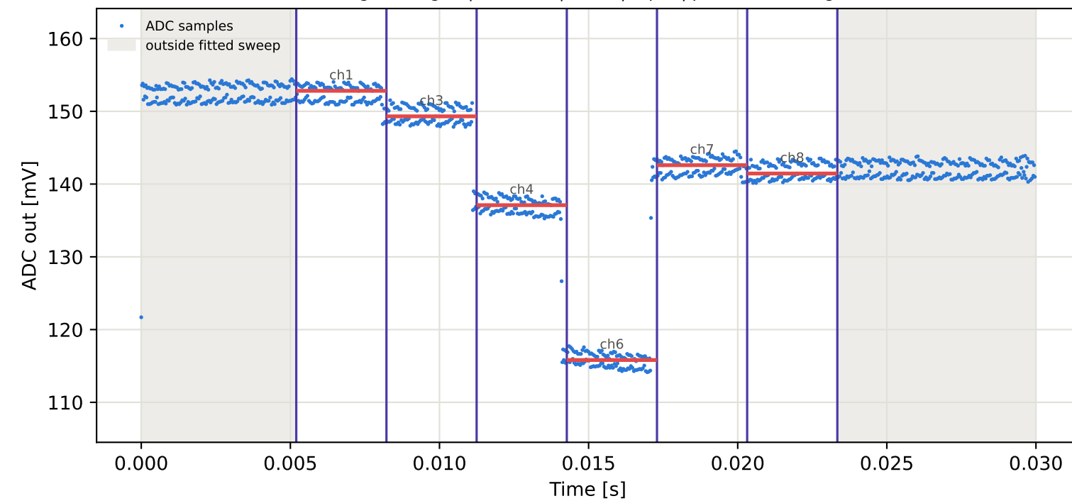
Tag5 &lt;- Tag16 | 915 MHz | run 0 | rep 1 | phase -94.24 deg
