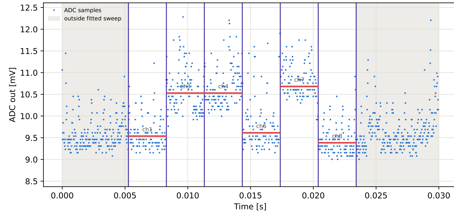
Tag2 &lt;- Tag15 | 775 MHz | run 0 | rep 1 | phase 97.49 deg
