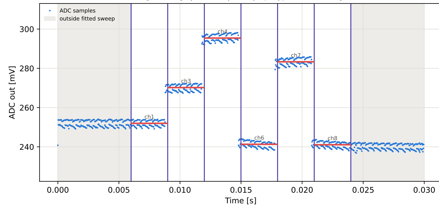
Tag2 &lt;- Tag1 | 985 MHz | run 0 | rep 1 | phase -152.76 deg
