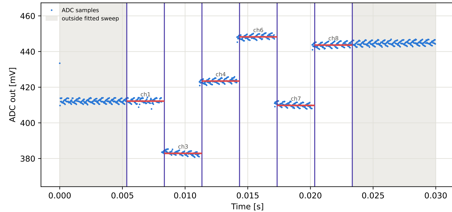
Tag5 &lt;- Tag3 | 845 MHz | run 0 | rep 1 | phase 106.42 deg
