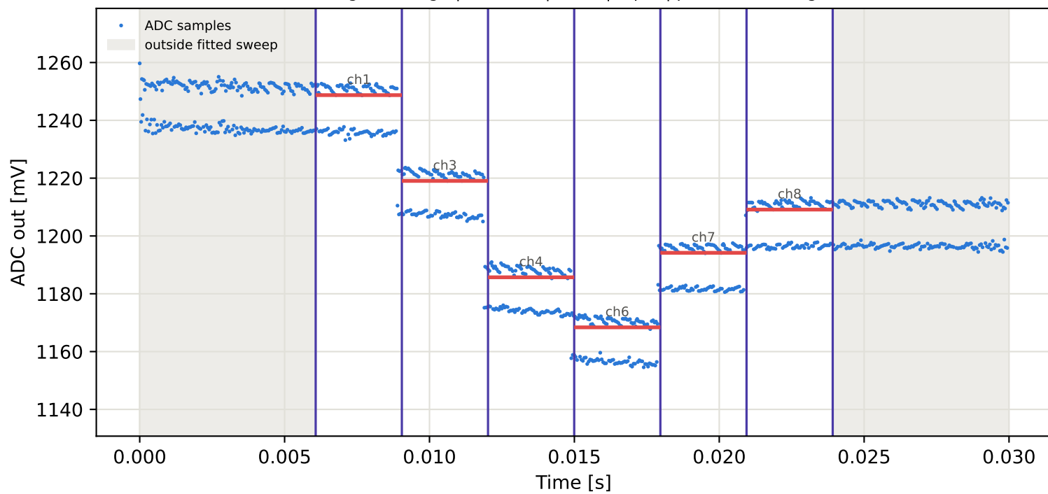
Tag10 &lt;- Tag8 | 875 MHz | run 0 | rep 1 | phase -153.20 deg
