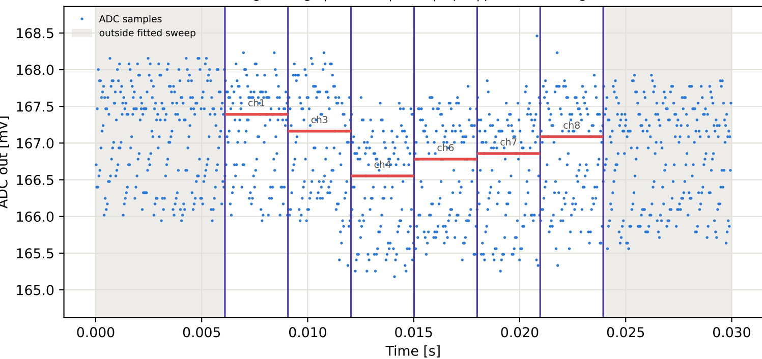
Tag8 &lt;- Tag6 | 785 MHz | run 0 | rep 1 | phase 73.73 deg
