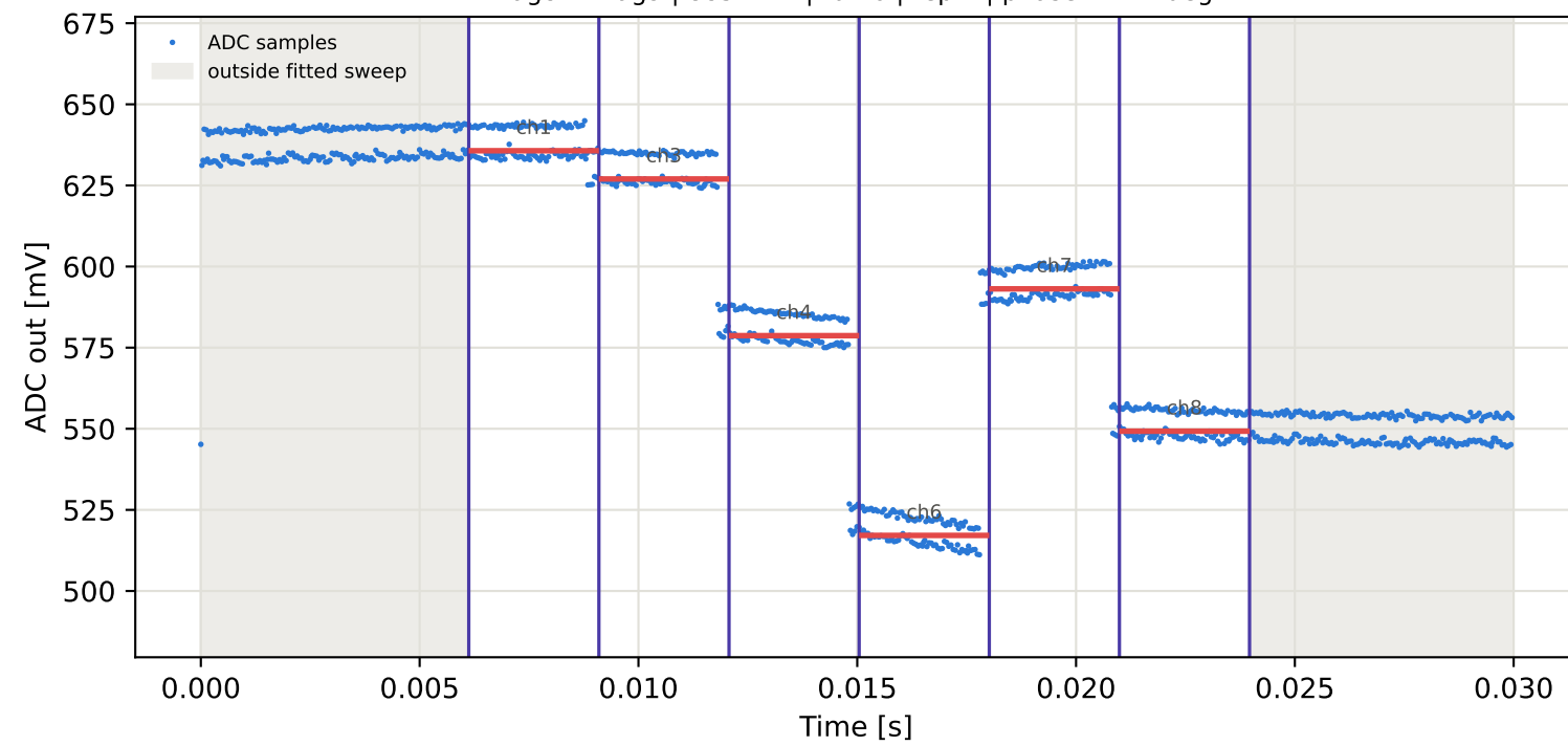
Tag9 &lt;- Tag10 | 885 MHz | run 0 | rep 1 | phase 60.33 deg
