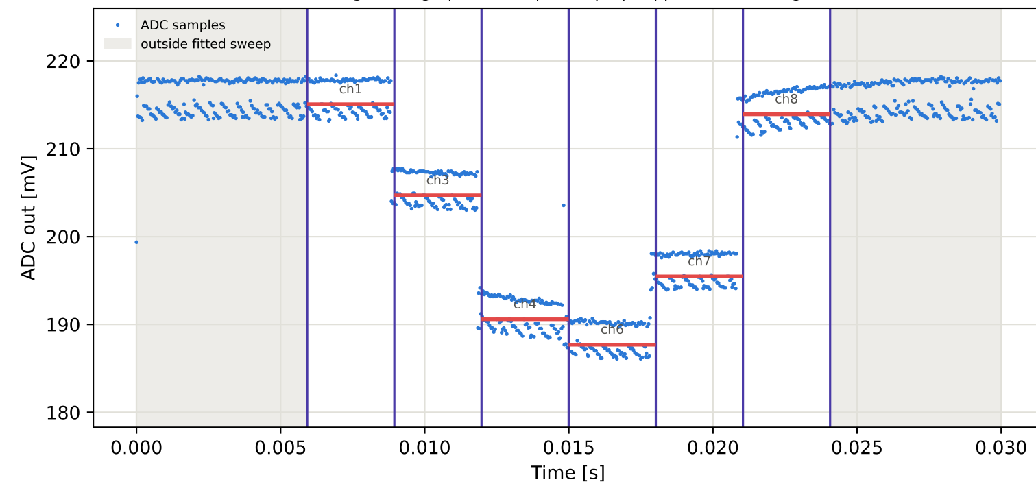
Tag4 &lt;- Tag15 | 915 MHz | run 0 | rep 1 | phase -132.56 deg
