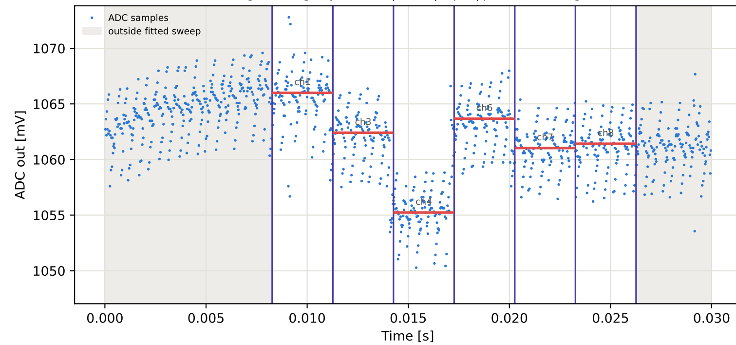
Tag10 &lt;- Tag2 | 905 MHz | run 0 | rep 1 | phase -82.30 deg
