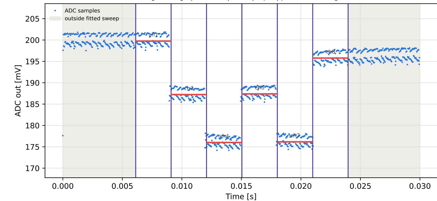
Tag8 &lt;- Tag7 | 795 MHz | run 0 | rep 1 | phase 98.35 deg
