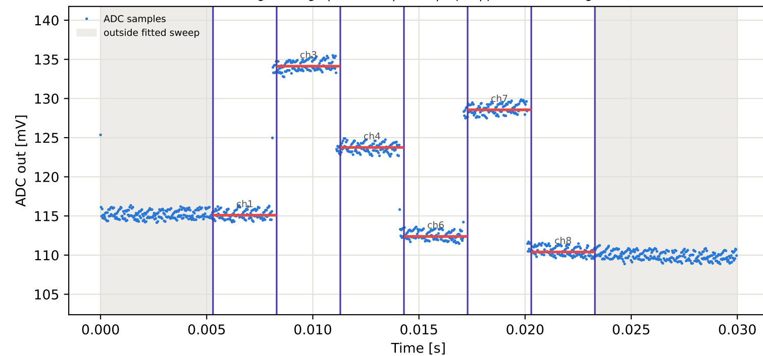
Tag5 &lt;- Tag3 | 825 MHz | run 0 | rep 1 | phase -12.08 deg
