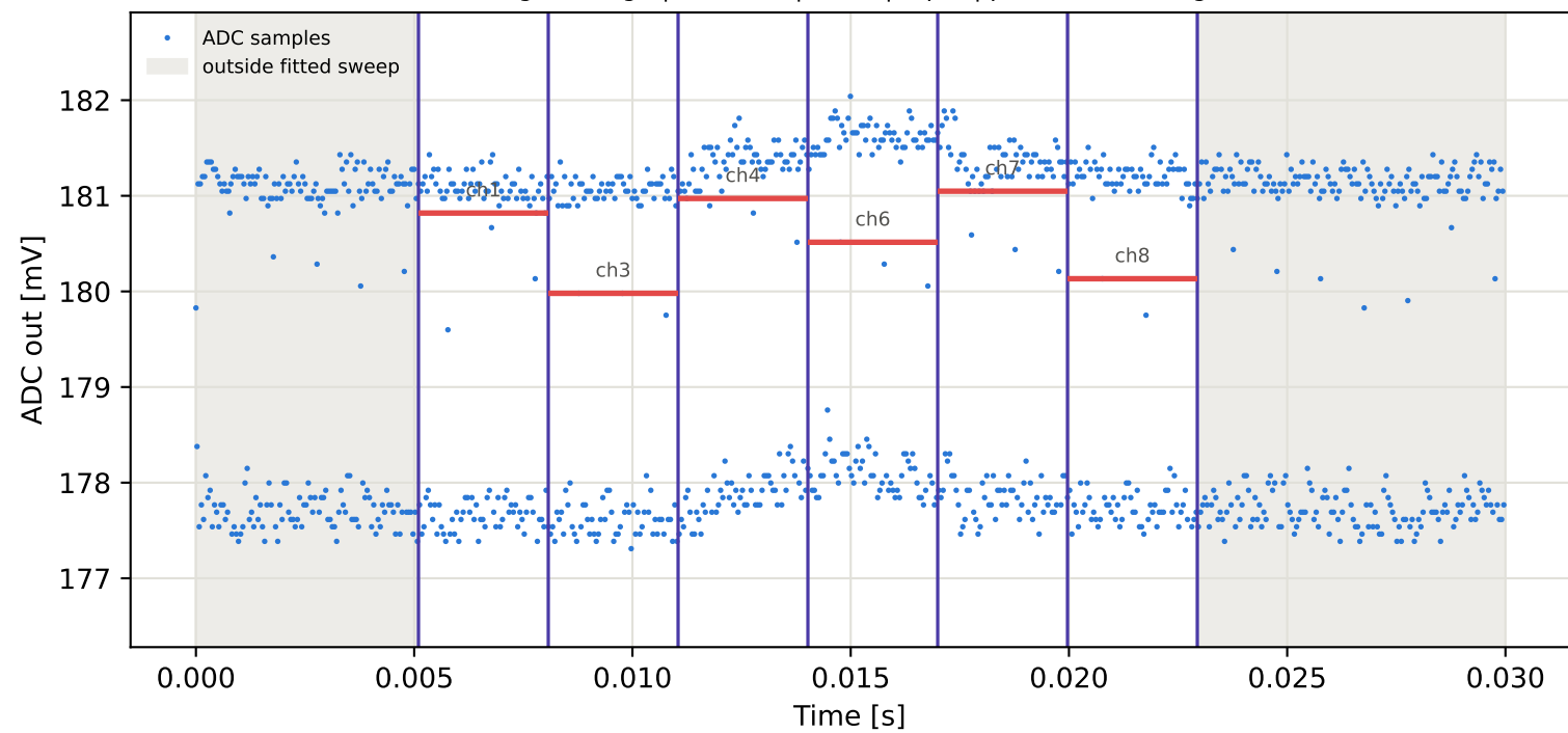
Tag7 &lt;- Tag4 | 775 MHz | run 0 | rep 1 | phase 112.51 deg
