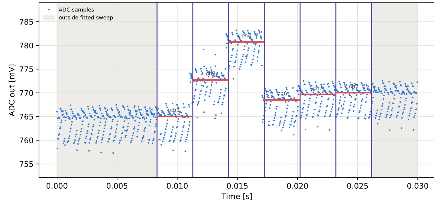
Tag8 &lt;- Tag15 | 945 MHz | run 0 | rep 1 | phase -159.88 deg
