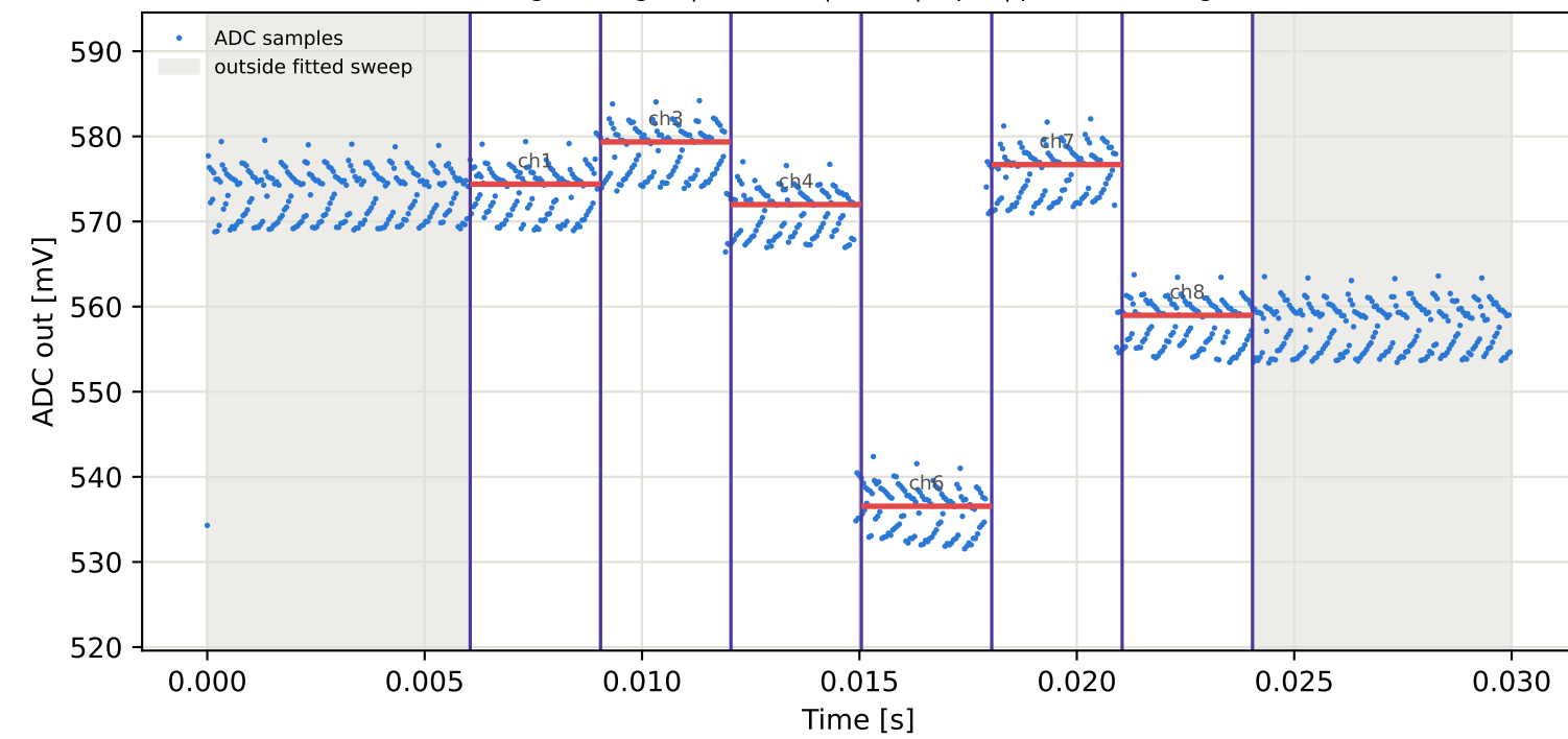
Tag5 &lt;- Tag16 | 935 MHz | run 0 | rep 1 | phase -82.48 deg
