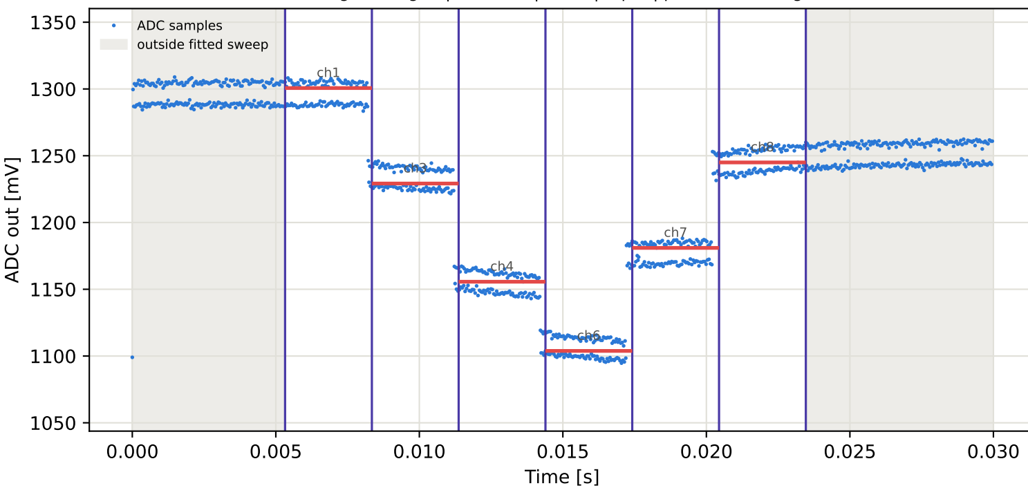
Tag3 &lt;- Tag16 | 885 MHz | run 0 | rep 1 | phase -150.63 deg
