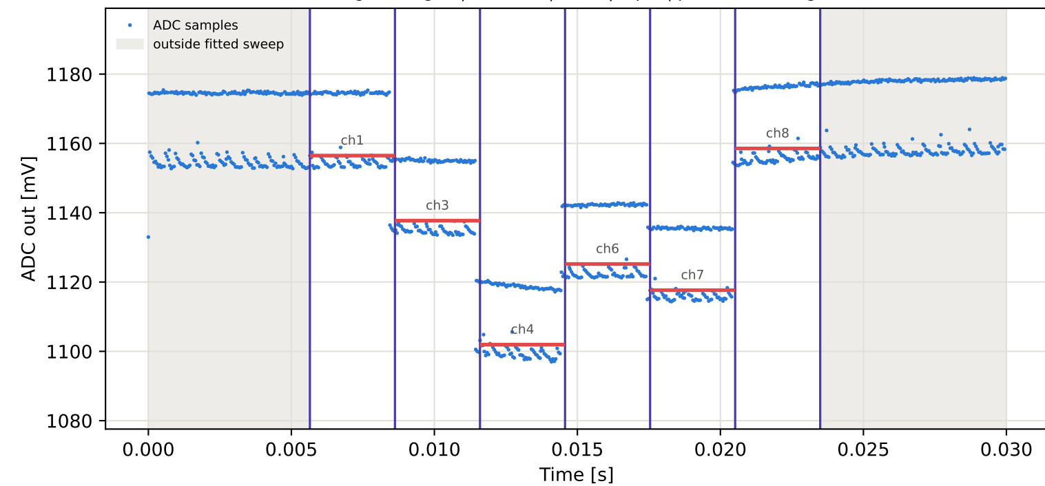
Tag7 &lt;- Tag3 | 935 MHz | run 0 | rep 1 | phase 166.22 deg
