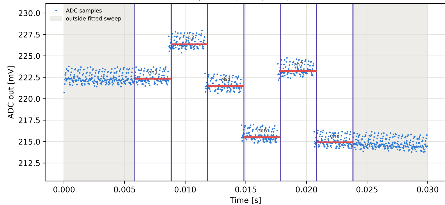
Tag1 &lt;- Tag2 | 865 MHz | run 0 | rep 1 | phase 173.70 deg
