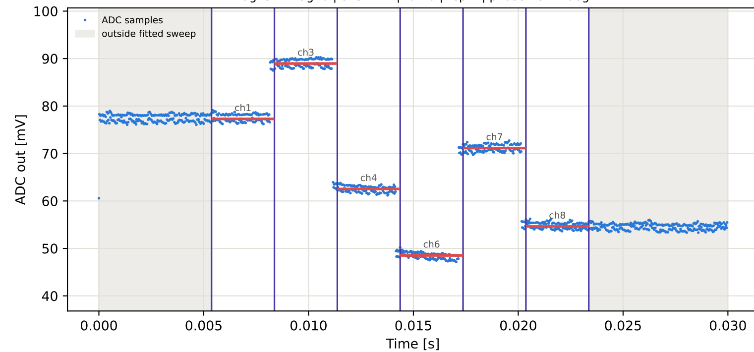
Tag15 &lt;- Tag3 | 845 MHz | run 0 | rep 1 | phase -44.59 deg
