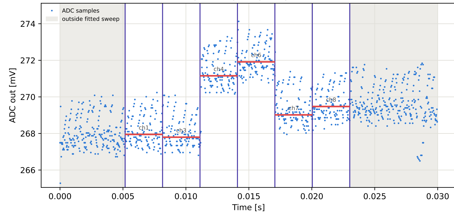
Tag15 &lt;- Tag1 | 975 MHz | run 0 | rep 1 | phase -146.00 deg
