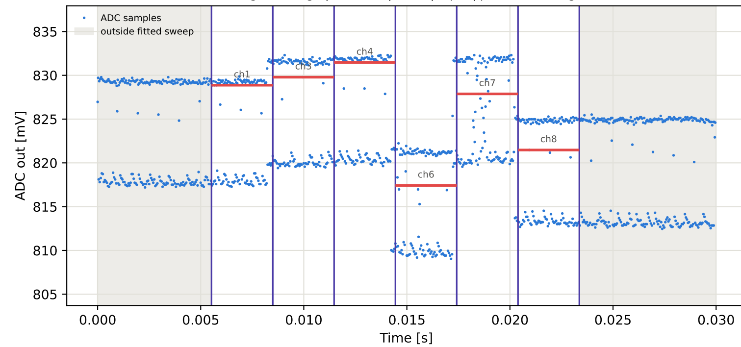
Tag16 &lt;- Tag4 | 865 MHz | run 0 | rep 1 | phase -72.19 deg
