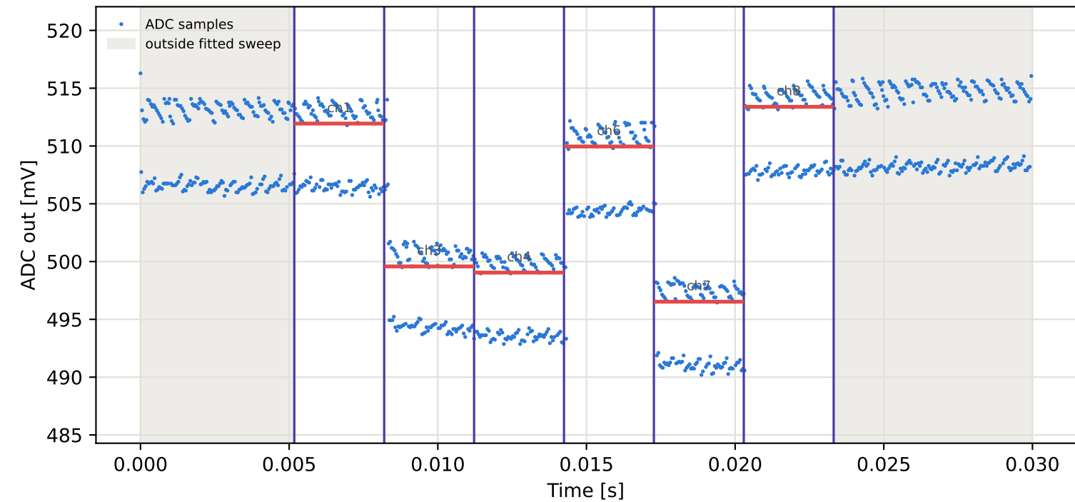
Tag9 &lt;- Tag8 | 825 MHz | run 0 | rep 1 | phase 25.50 deg
