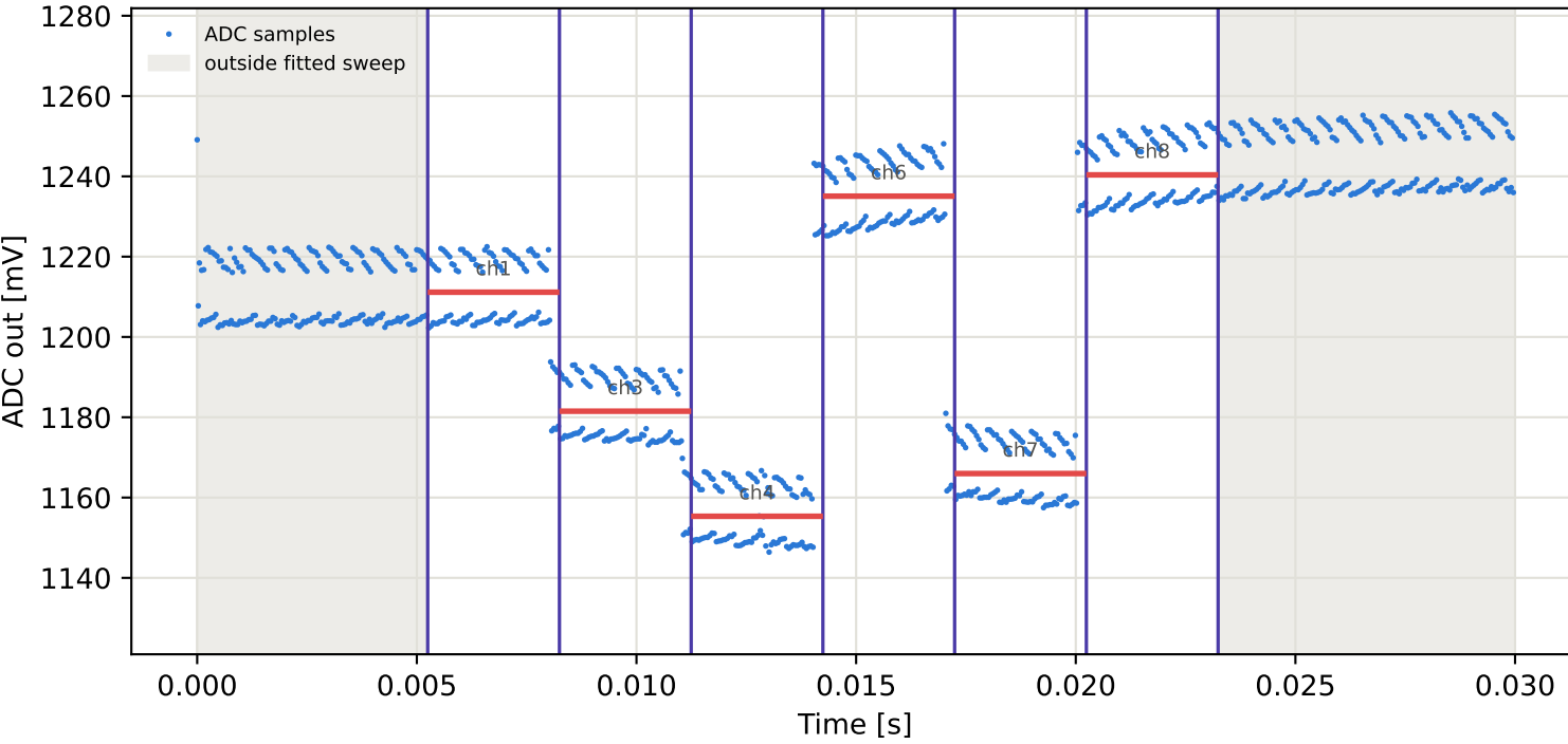
Tag7 &lt;- Tag10 | 925 MHz | run 0 | rep 1 | phase 129.71 deg
