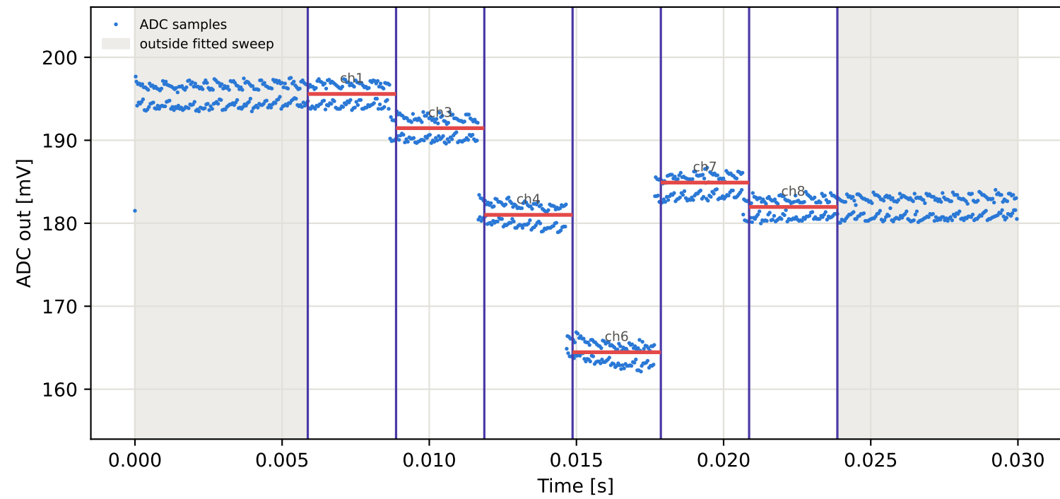
Tag4 &lt;- Tag15 | 905 MHz | run 0 | rep 1 | phase 173.25 deg
