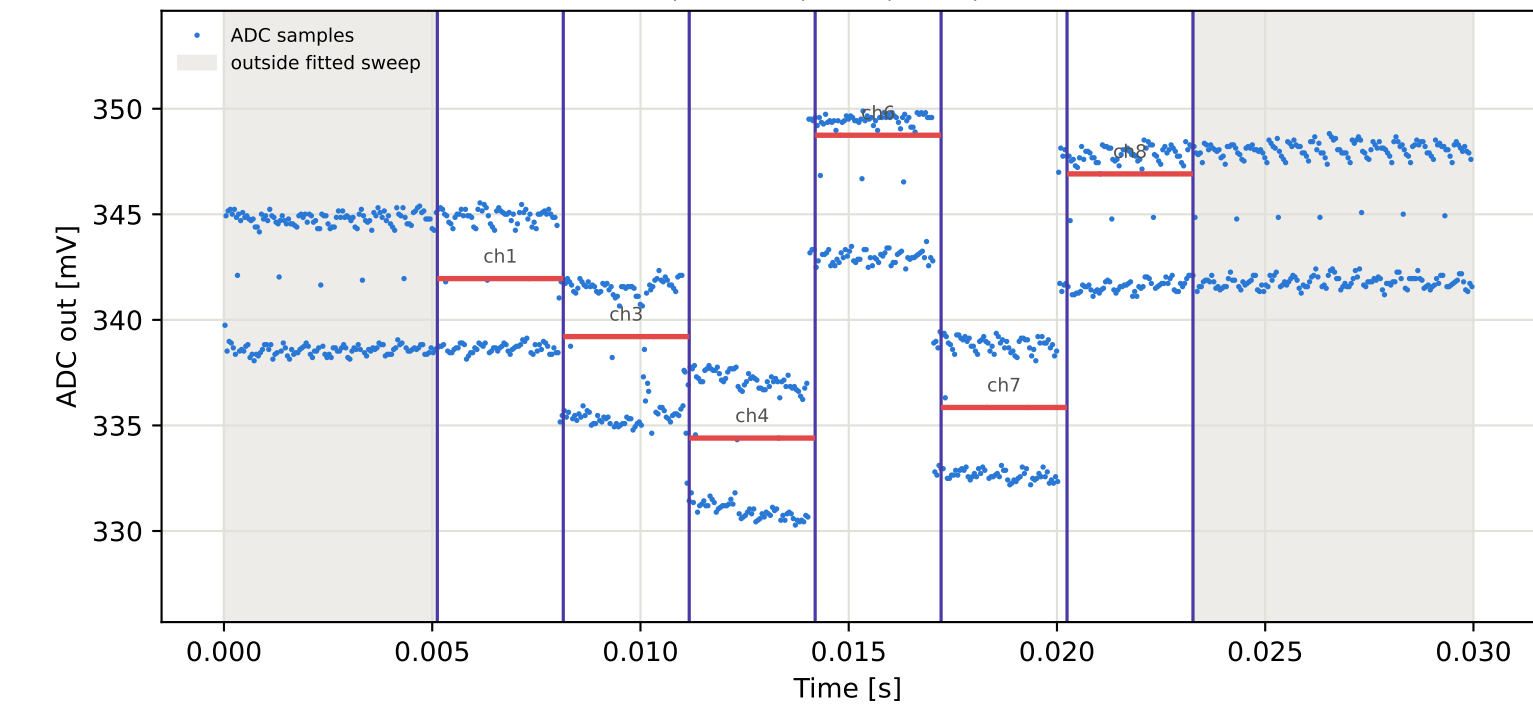
Tag10 &lt;- Tag4 | 975 MHz | run 0 | rep 1 | phase 133.43 deg
