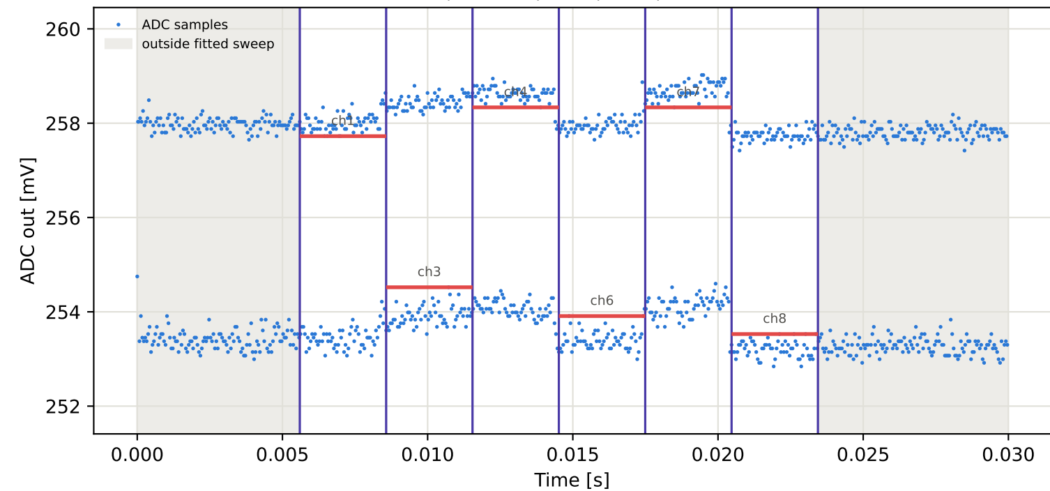
Tag9 &lt;- Tag2 | 805 MHz | run 0 | rep 1 | phase -42.00 deg
