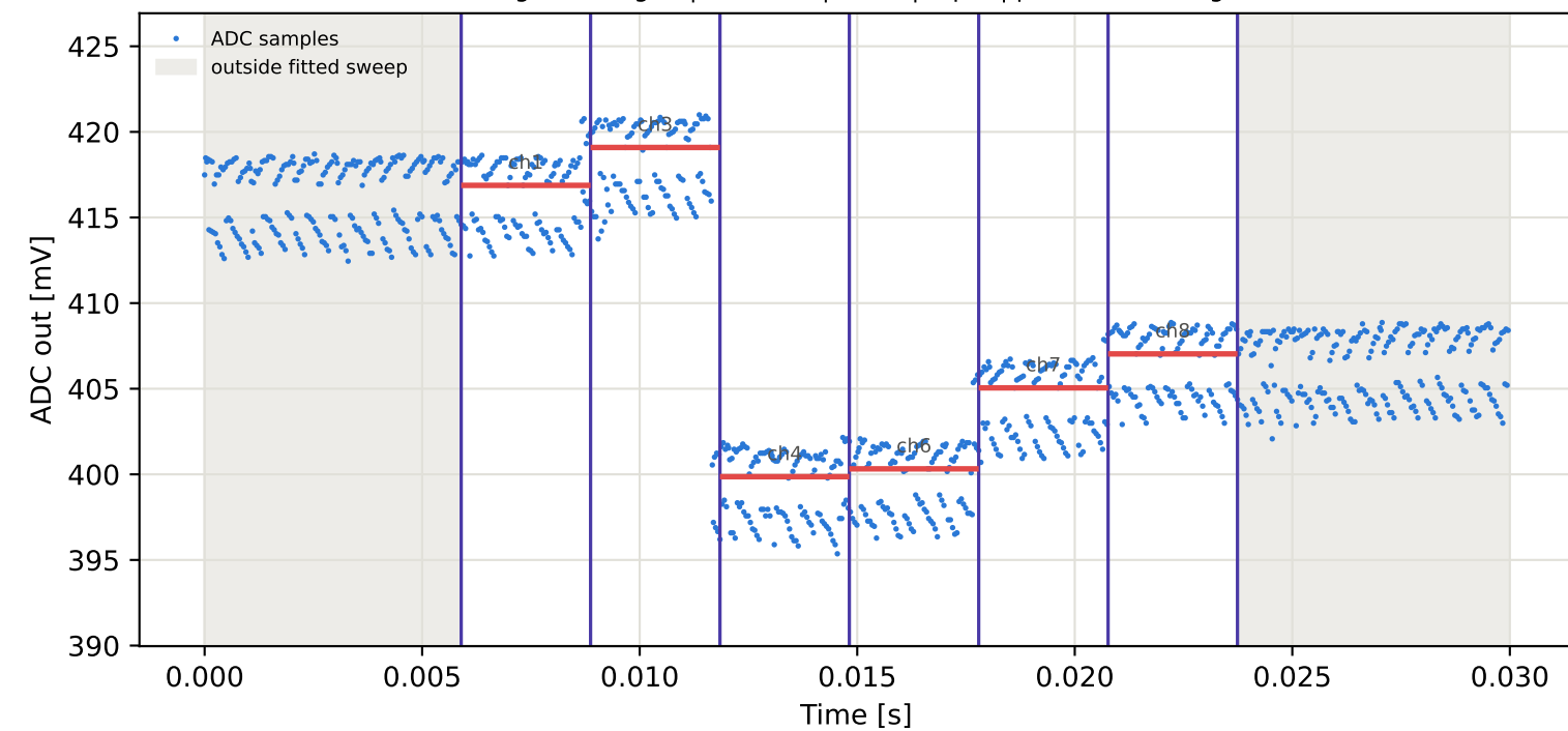
Tag16 &lt;- Tag15 | 835 MHz | run 0 | rep 1 | phase 55.95 deg
