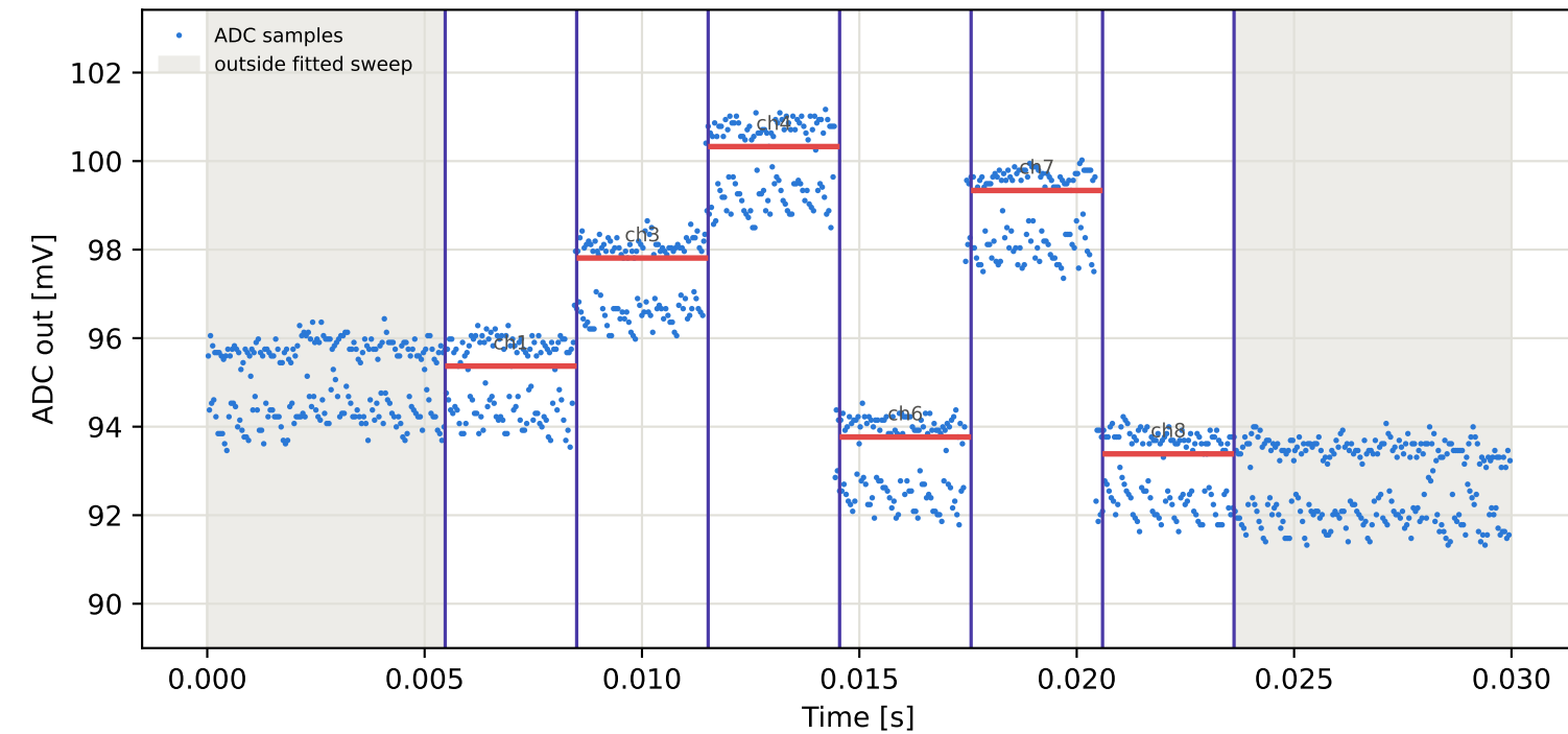
Tag4 &lt;- Tag2 | 995 MHz | run 0 | rep 1 | phase -71.95 deg
