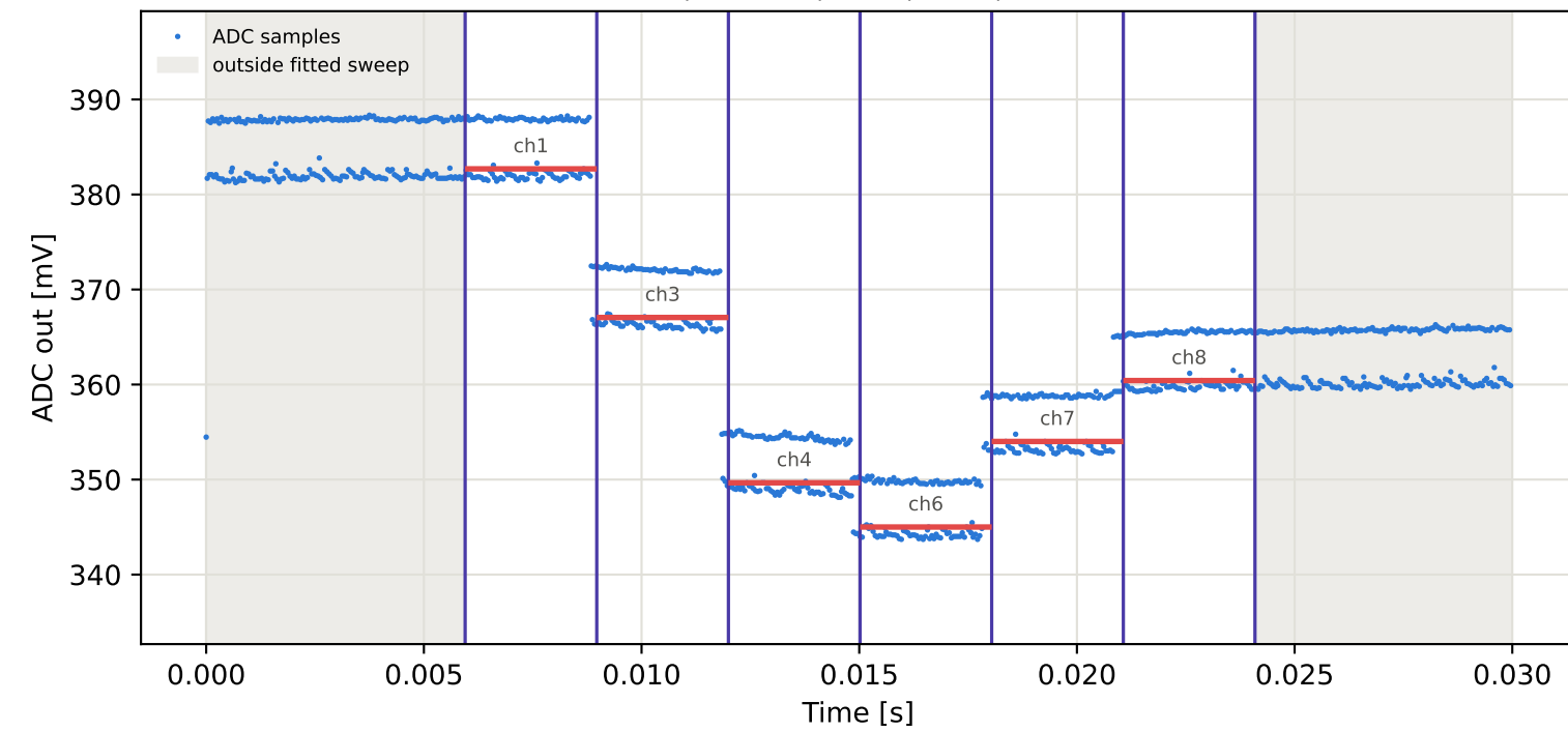
Tag15 &lt;- Tag5 | 865 MHz | run 0 | rep 1 | phase 54.54 deg
