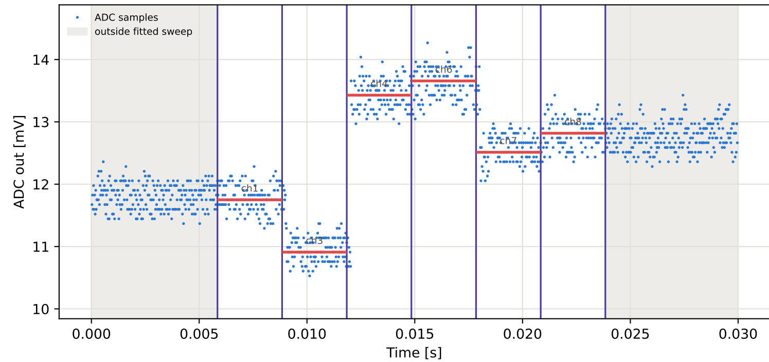
Tag16 &lt;- Tag7 | 785 MHz | run 0 | rep 1 | phase 89.85 deg
