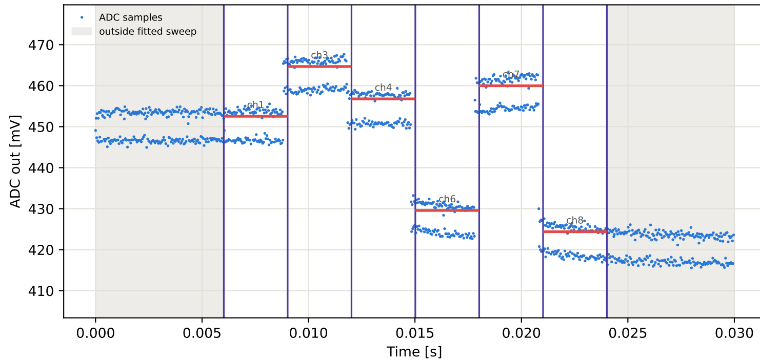
Tag16 &lt;- Tag10 | 885 MHz | run 0 | rep 1 | phase -102.35 deg
