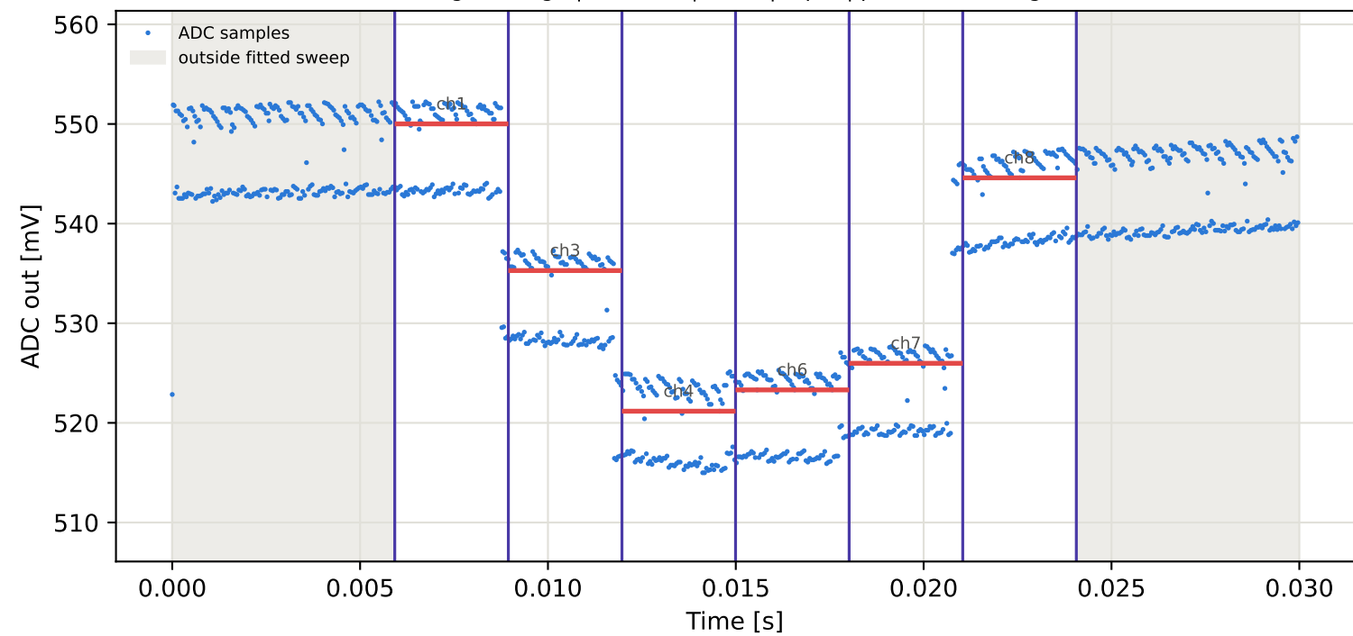
Tag4 &lt;- Tag15 | 895 MHz | run 0 | rep 1 | phase 157.33 deg
