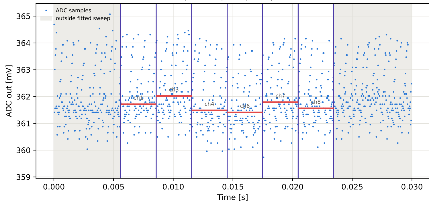
Tag6 &lt;- Tag2 | 985 MHz | run 0 | rep 1 | phase 13.59 deg
