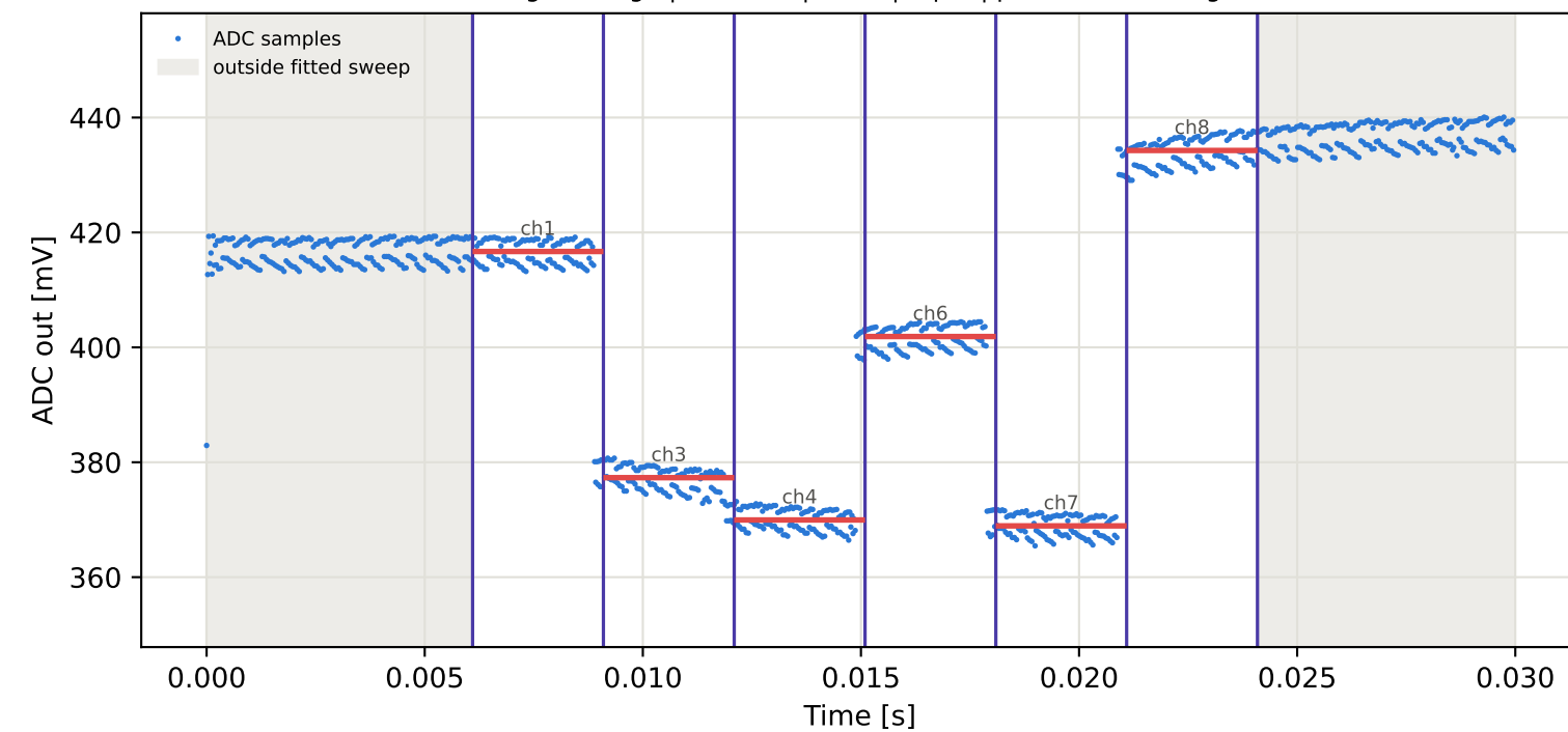
Tag5 &lt;- Tag3 | 865 MHz | run 0 | rep 1 | phase 115.56 deg
