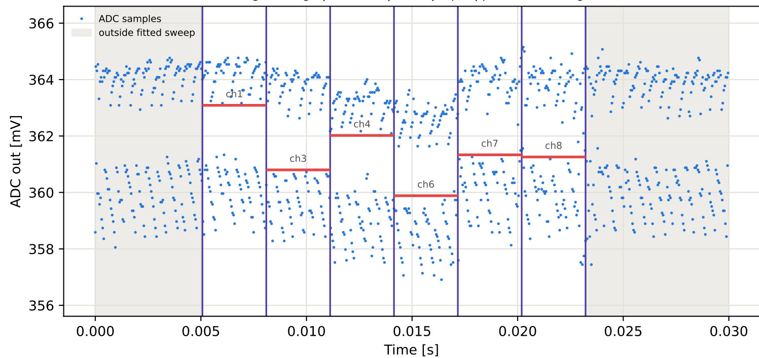
Tag6 &lt;- Tag4 | 985 MHz | run 0 | rep 1 | phase -150.58 deg
