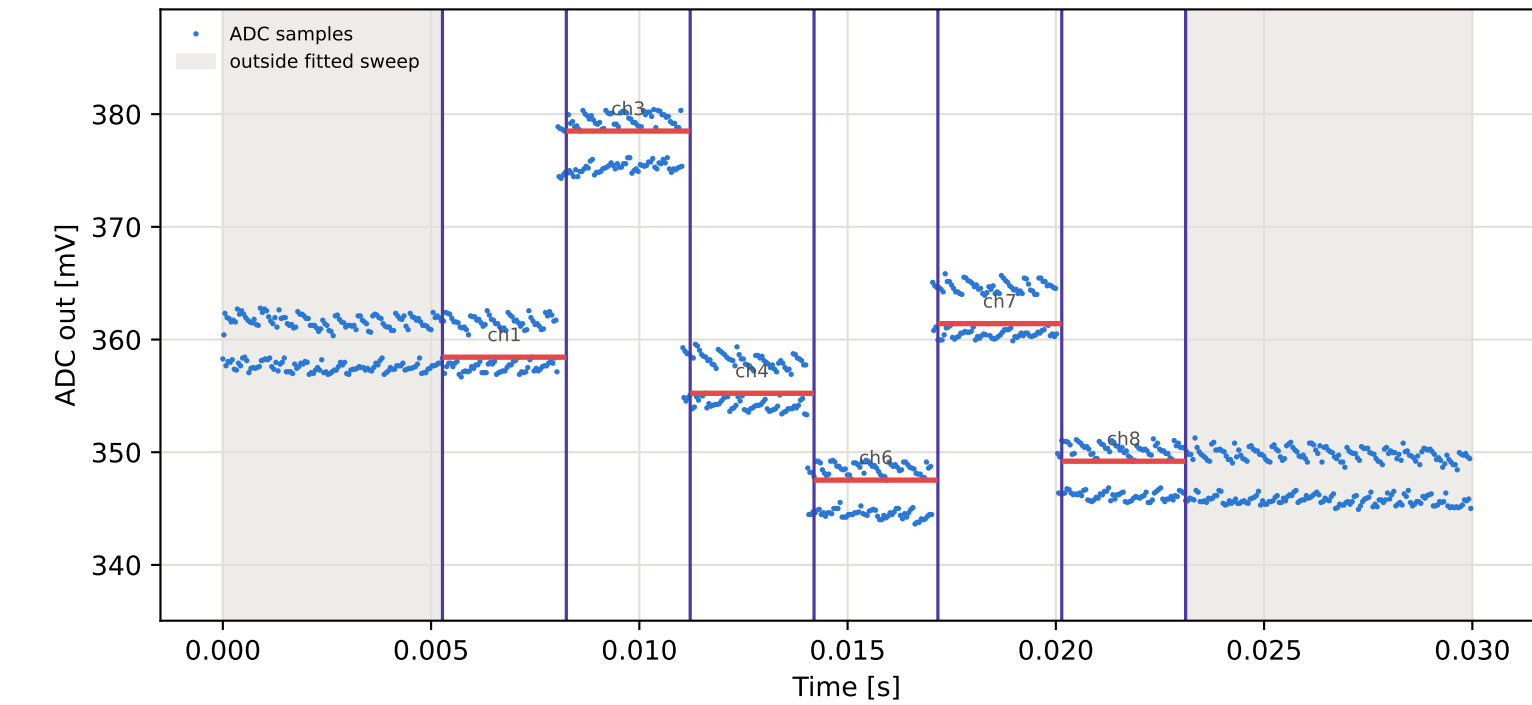
Tag6 &lt;- Tag5 | 825 MHz | run 0 | rep 1 | phase 97.82 deg
