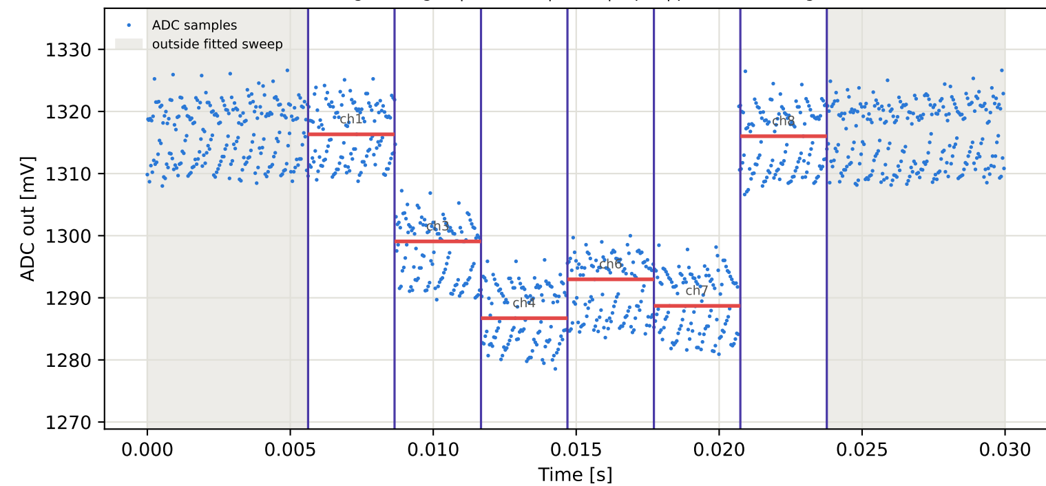
Tag6 &lt;- Tag3 | 885 MHz | run 0 | rep 1 | phase 117.12 deg
