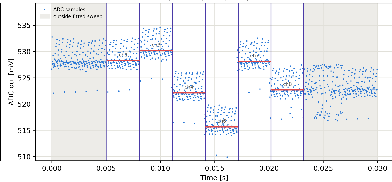
Tag1 &lt;- Tag8 | 985 MHz | run 0 | rep 1 | phase 54.29 deg
