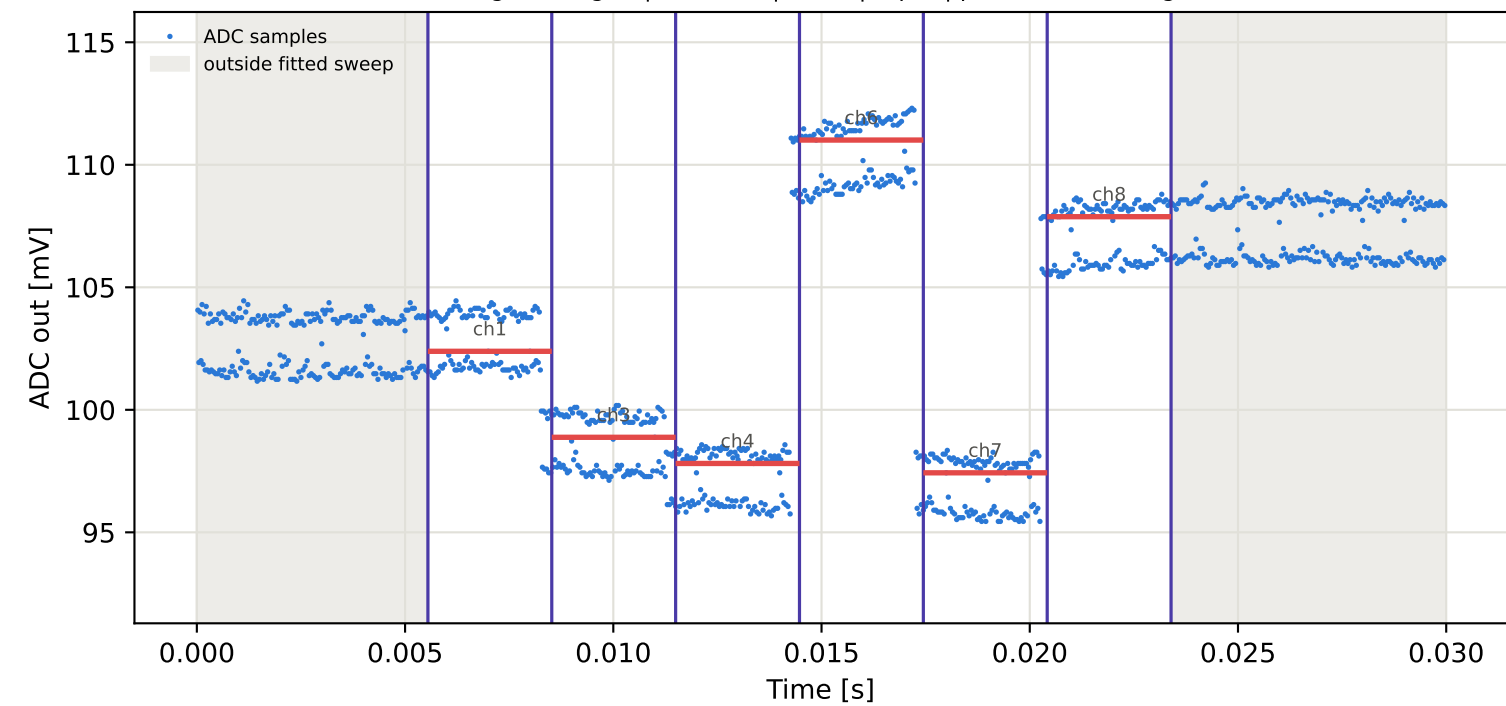
Tag4 &lt;- Tag16 | 995 MHz | run 0 | rep 1 | phase -75.63 deg
