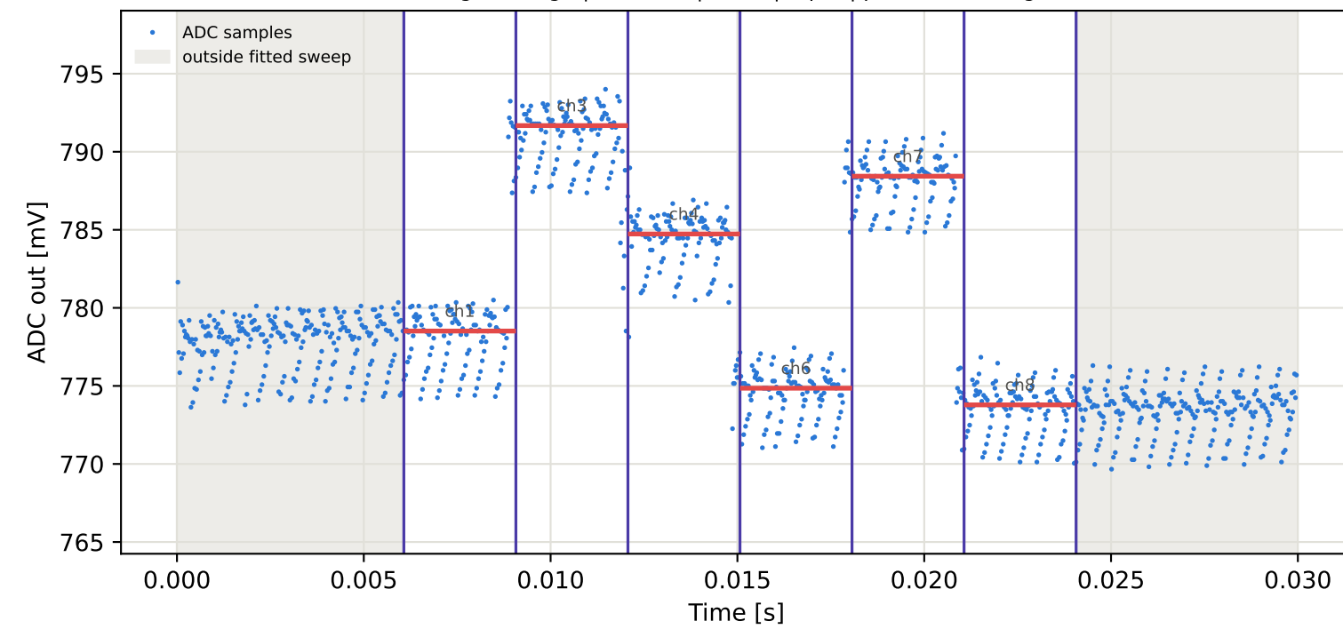
Tag8 &lt;- Tag1 | 825 MHz | run 0 | rep 1 | phase 140.90 deg
