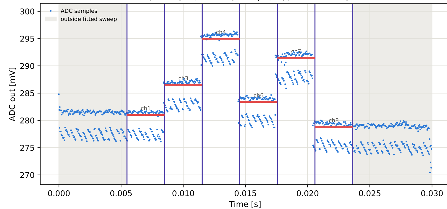
Tag4 &lt;- Tag2 | 955 MHz | run 0 | rep 1 | phase -68.85 deg
