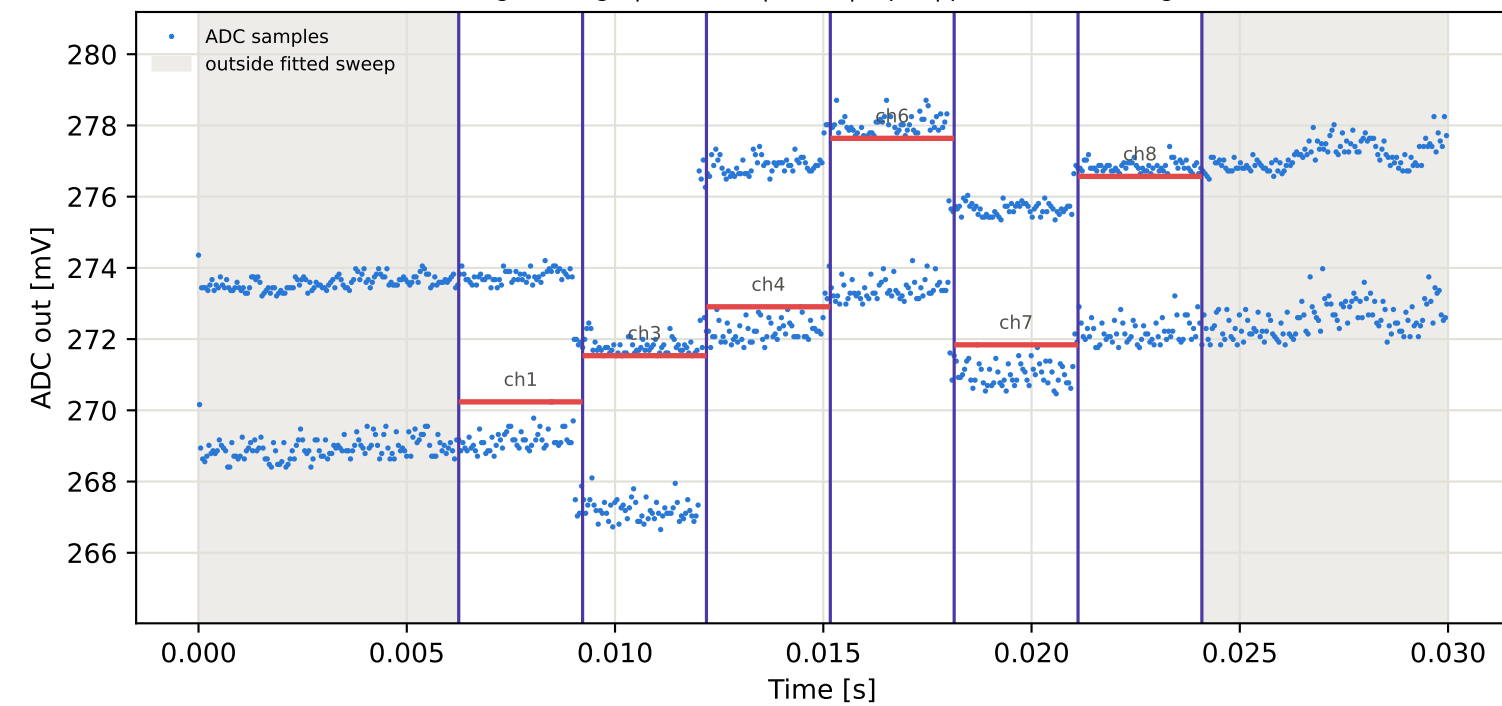
Tag3 &lt;- Tag6 | 825 MHz | run 0 | rep 1 | phase -123.92 deg
