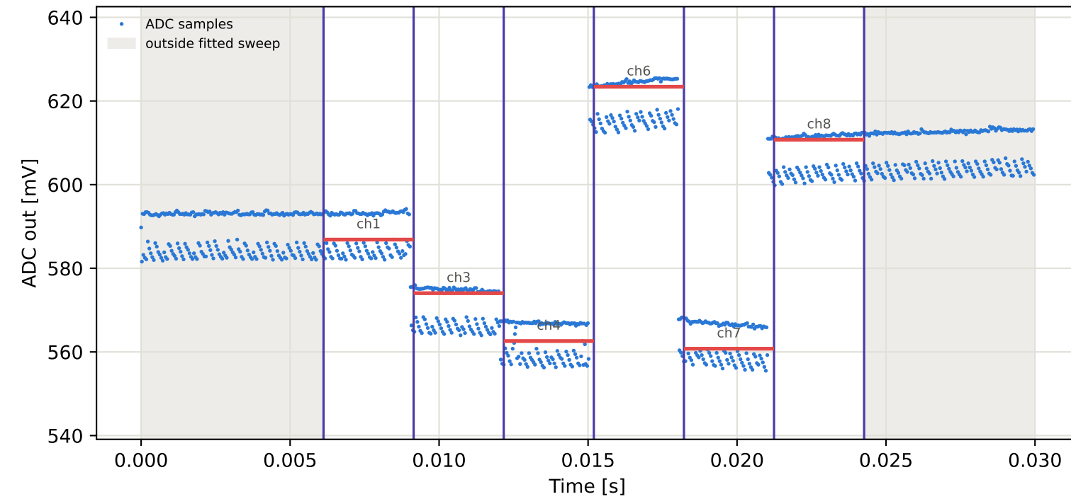
Tag3 &lt;- Tag8 | 975 MHz | run 0 | rep 1 | phase 111.44 deg
