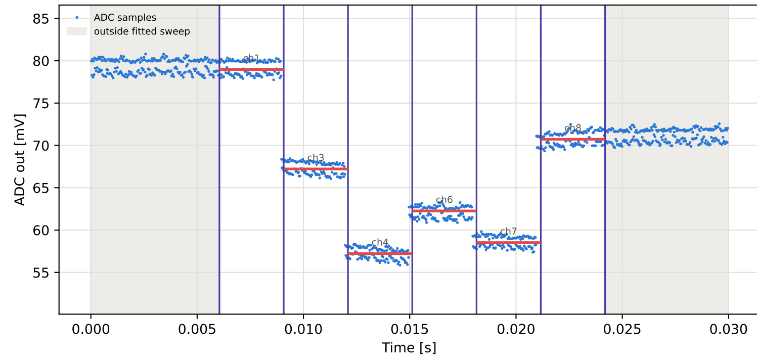
Tag16 &lt;- Tag1 | 845 MHz | run 0 | rep 1 | phase 15.16 deg
