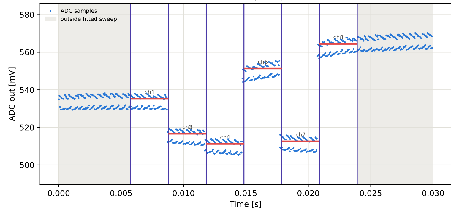
Tag4 &lt;- Tag8 | 895 MHz | run 0 | rep 1 | phase -91.04 deg
