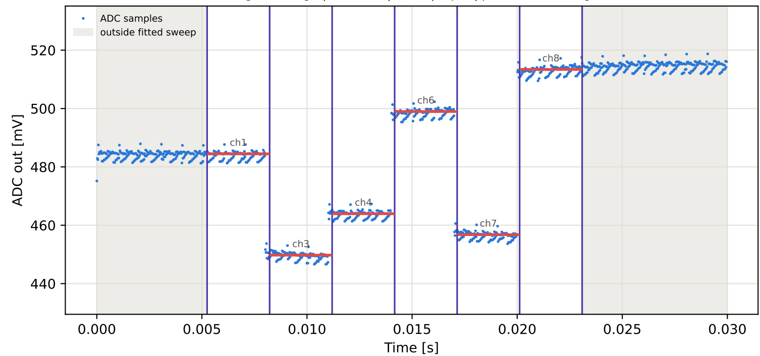
Tag16 &lt;- Tag5 | 855 MHz | run 0 | rep 1 | phase 98.13 deg
