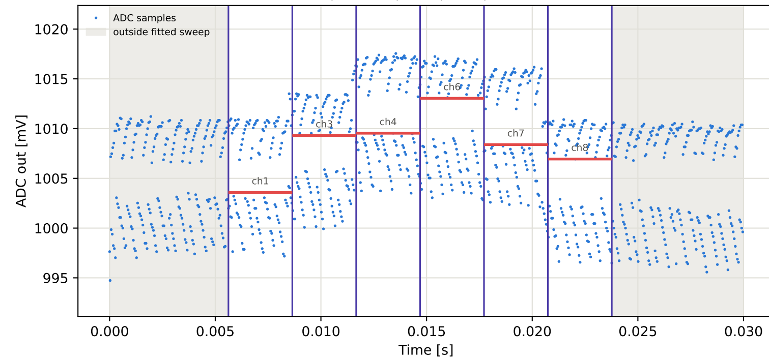
Tag7 &lt;- Tag5 | 915 MHz | run 0 | rep 1 | phase -135.29 deg
