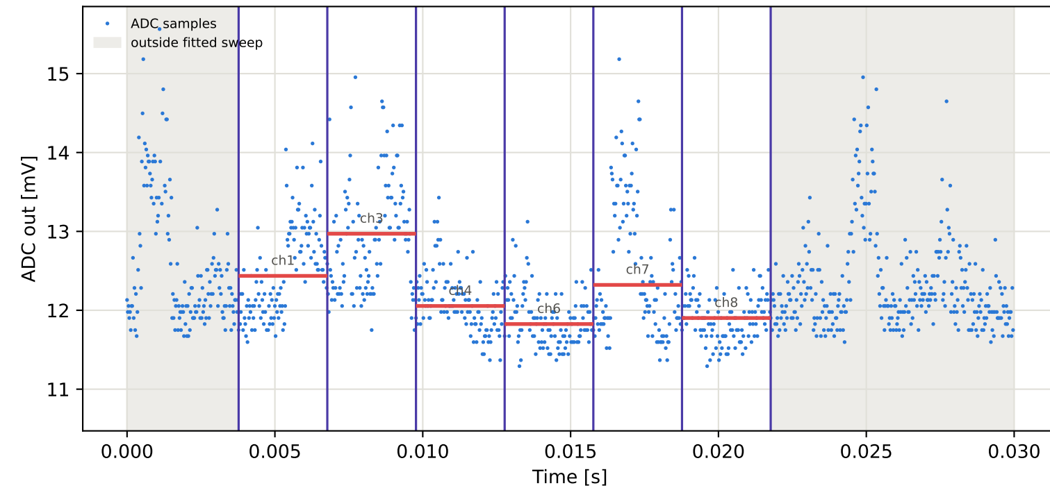
Tag2 &lt;- Tag7 | 795 MHz | run 0 | rep 1 | phase -30.80 deg
