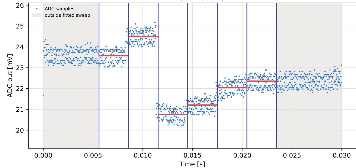
Tag1 &lt;- Tag8 | 775 MHz | run 0 | rep 1 | phase -135.48 deg
