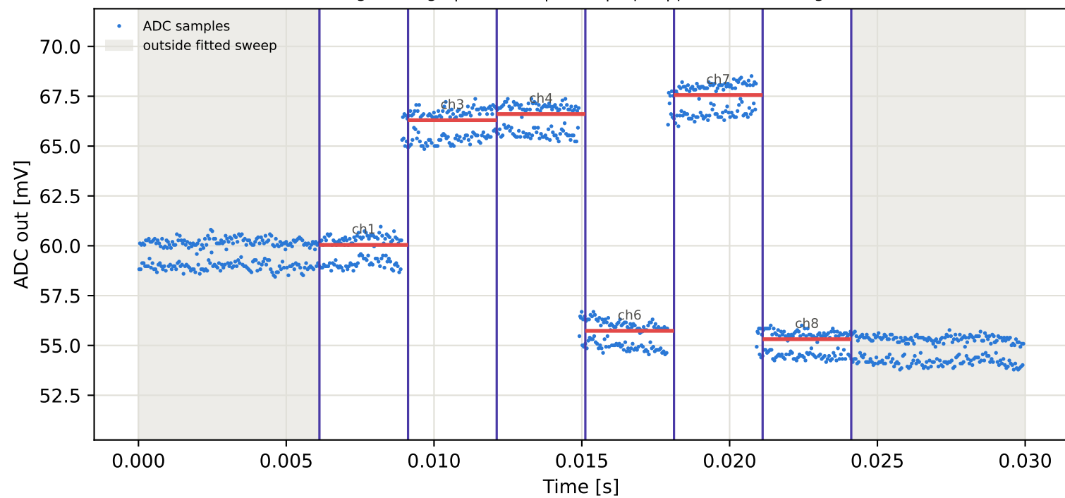
Tag4 &lt;- Tag9 | 825 MHz | run 0 | rep 1 | phase -141.84 deg
