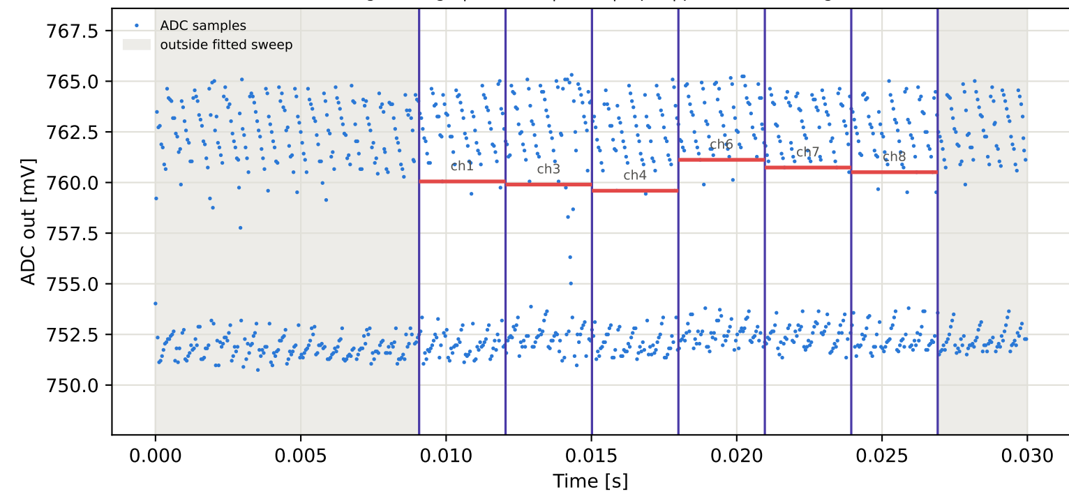
Tag7 &lt;- Tag4 | 955 MHz | run 0 | rep 1 | phase -171.43 deg
