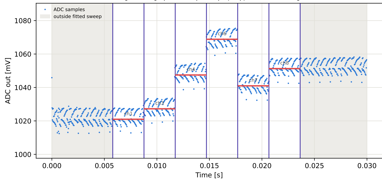
Tag16 &lt;- Tag7 | 895 MHz | run 0 | rep 1 | phase -148.30 deg
