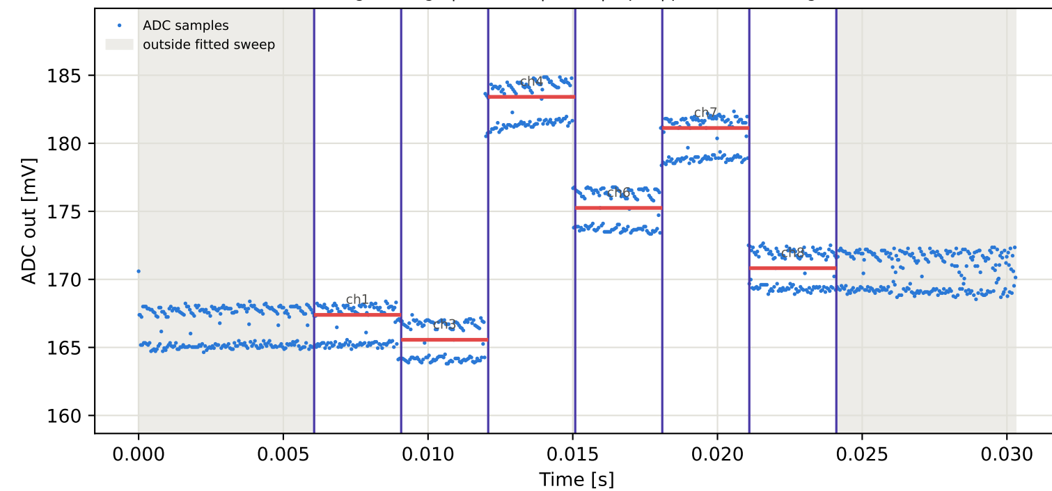
Tag8 &lt;- Tag1 | 775 MHz | run 0 | rep 1 | phase -64.91 deg
