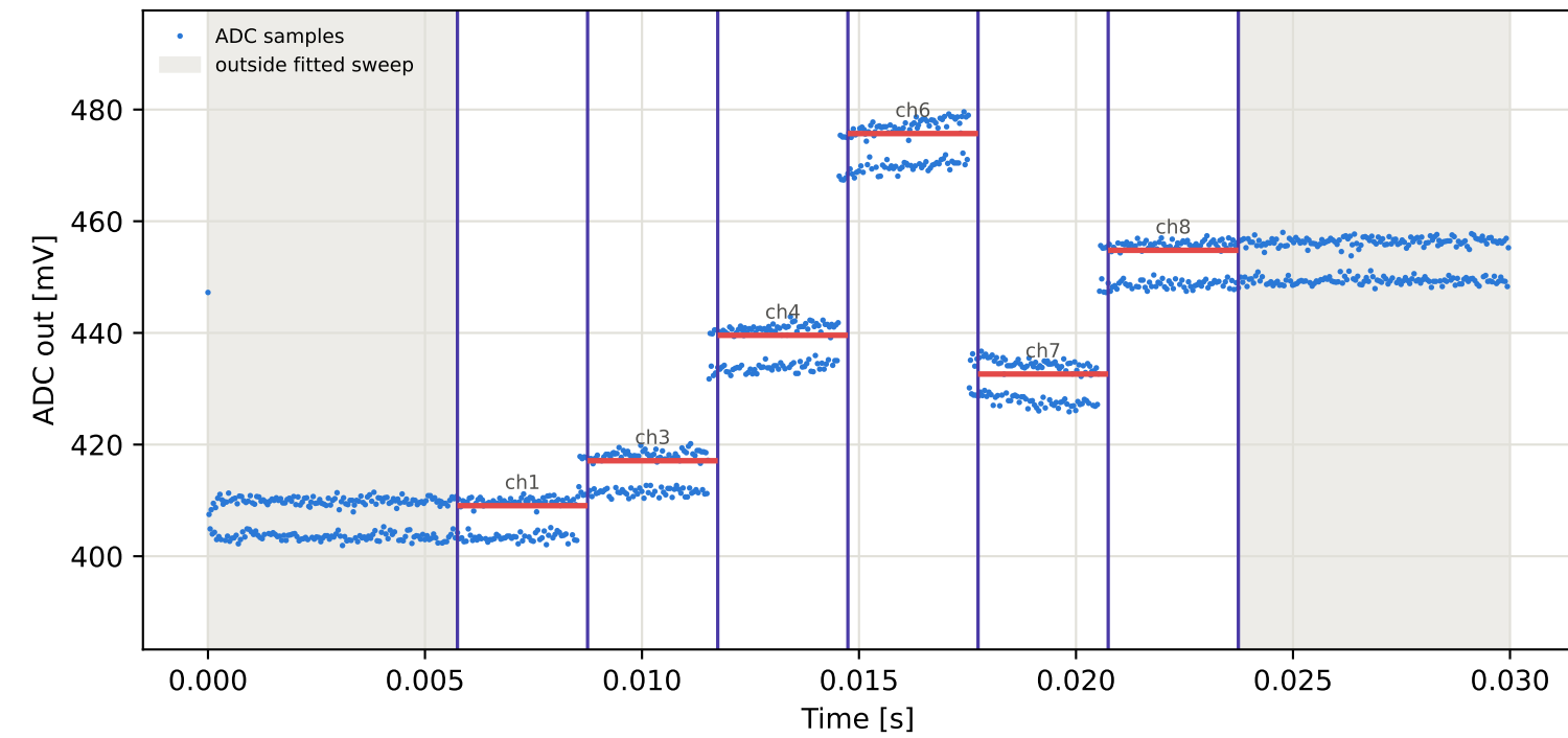
Tag16 &lt;- Tag1 | 885 MHz | run 0 | rep 1 | phase 132.36 deg
