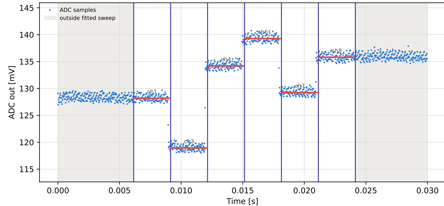
Tag3 &lt;- Tag9 | 785 MHz | run 0 | rep 1 | phase 150.63 deg
