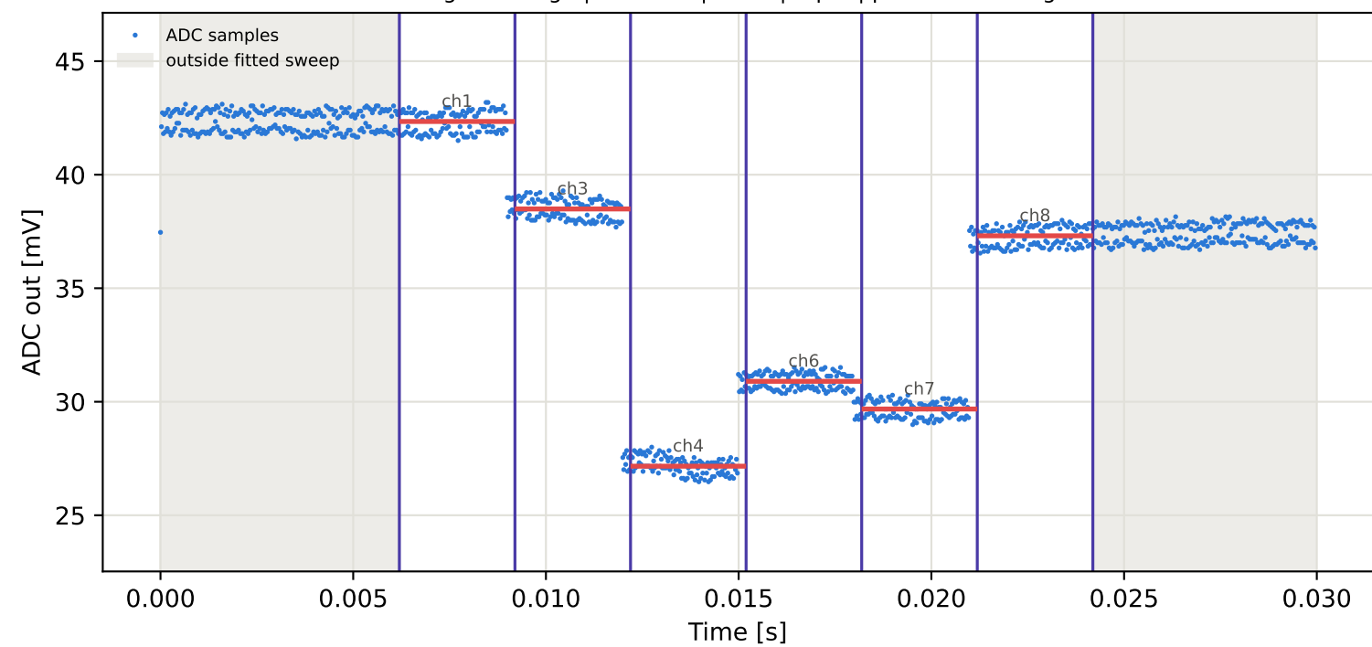
Tag2 &lt;- Tag10 | 805 MHz | run 0 | rep 1 | phase 134.33 deg
