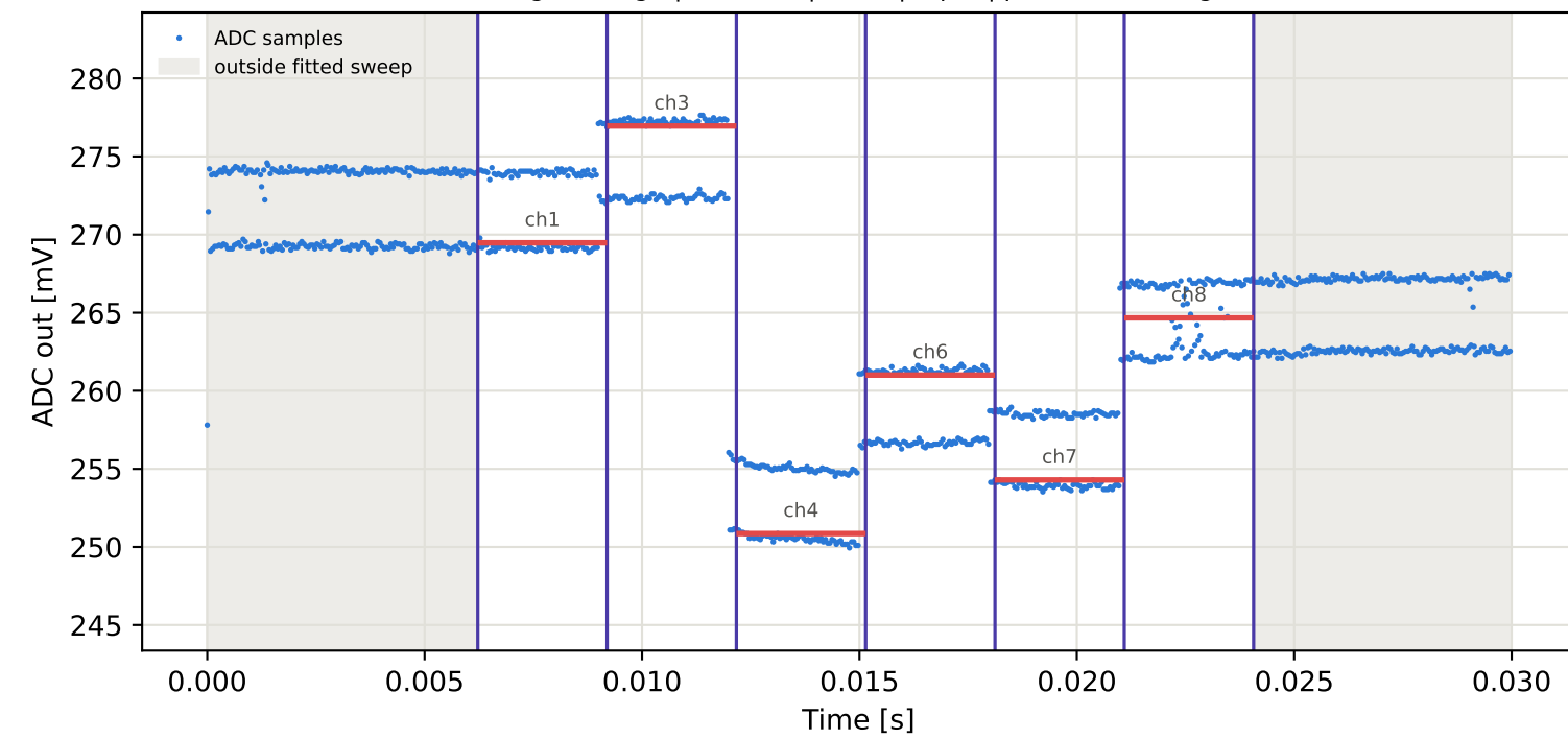
Tag9 &lt;- Tag5 | 805 MHz | run 0 | rep 1 | phase 24.99 deg
