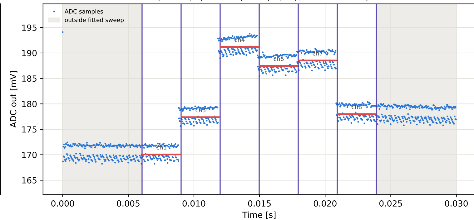
Tag3 &lt;- Tag9 | 805 MHz | run 0 | rep 1 | phase 179.29 deg
