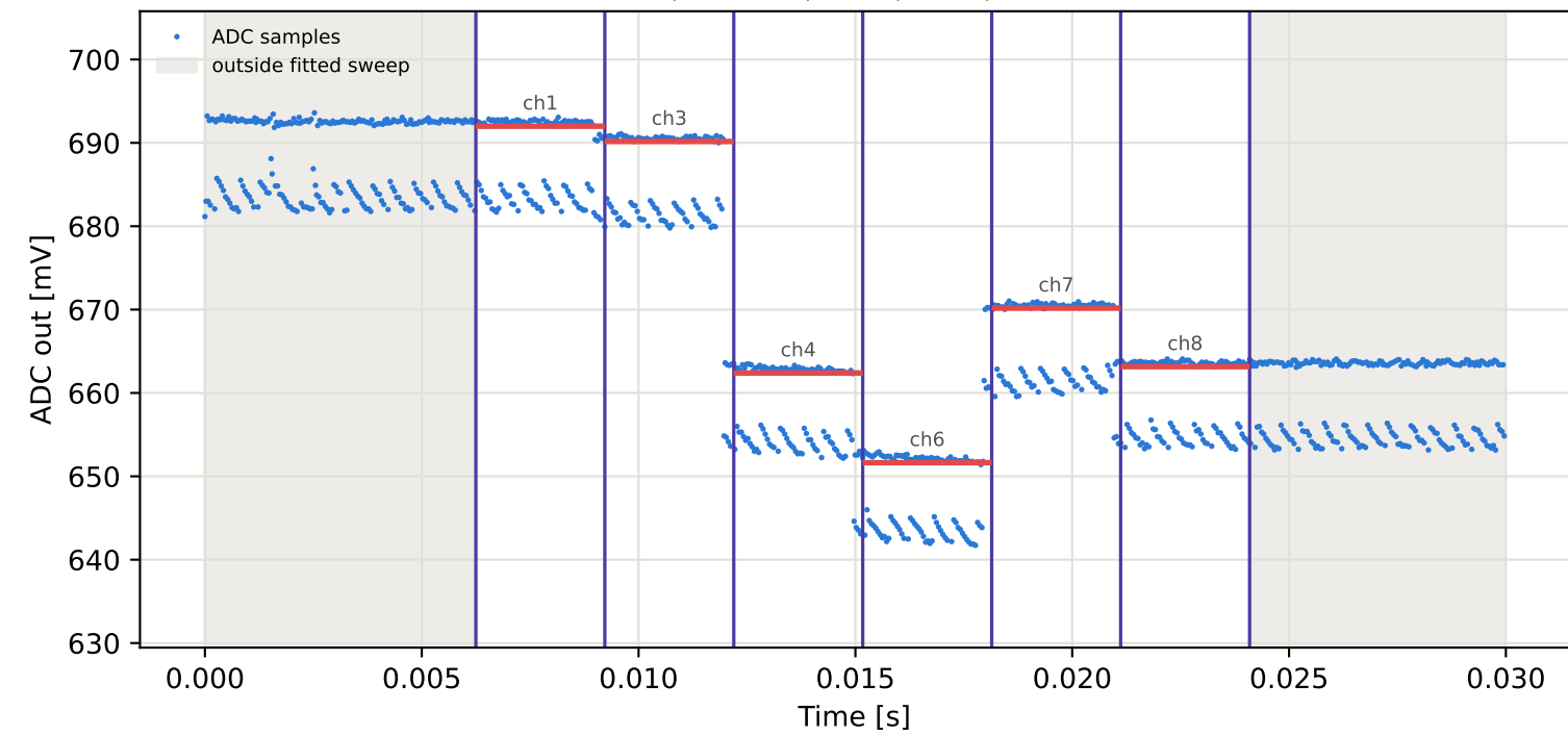
Tag9 &lt;- Tag8 | 845 MHz | run 0 | rep 1 | phase 42.96 deg
