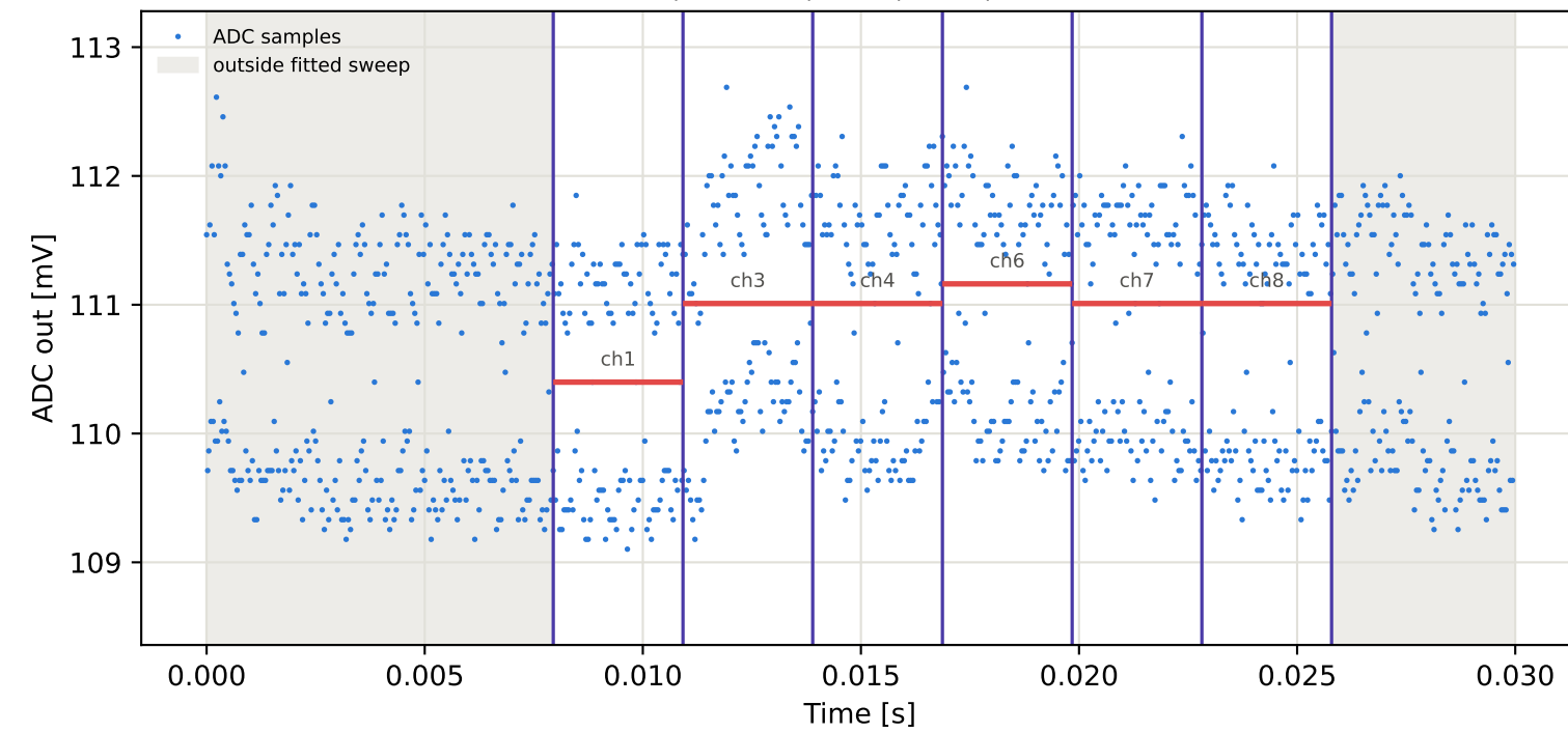
Tag15 &lt;- Tag1 | 785 MHz | run 0 | rep 1 | phase -114.63 deg
