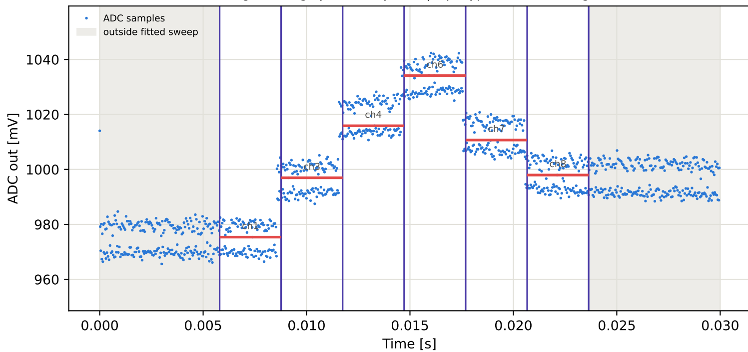
Tag2 &lt;- Tag1 | 885 MHz | run 0 | rep 1 | phase 22.01 deg
