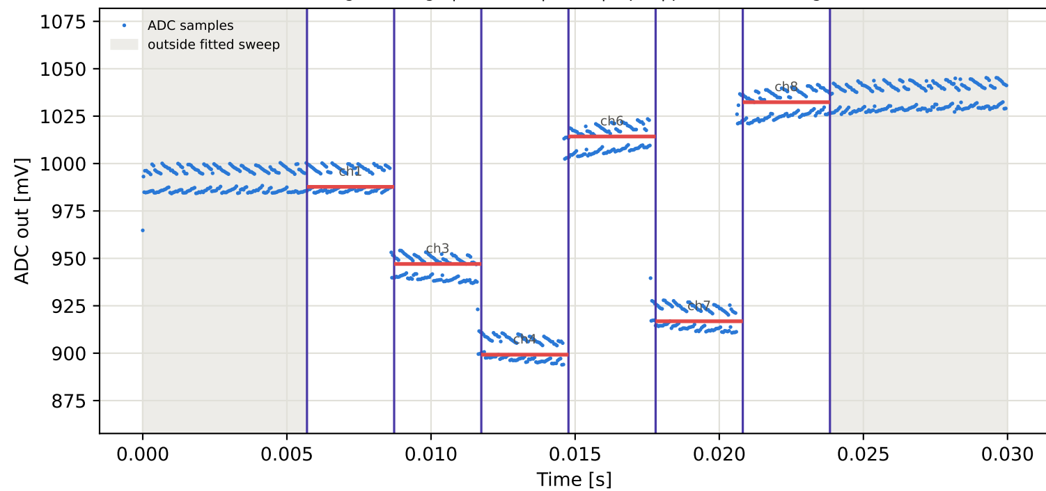
Tag2 &lt;- Tag10 | 935 MHz | run 0 | rep 1 | phase 34.87 deg
