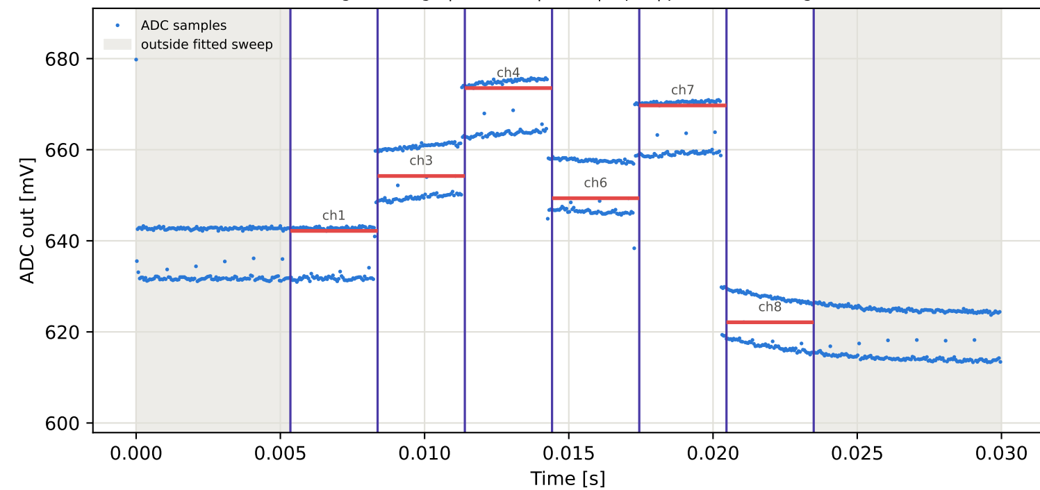
Tag16 &lt;- Tag1 | 905 MHz | run 0 | rep 1 | phase 92.58 deg
