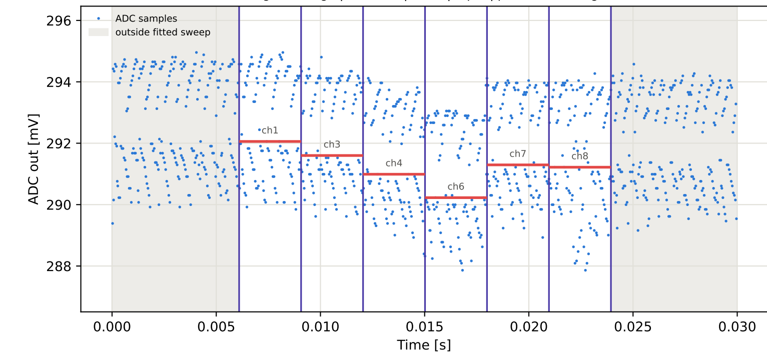
Tag10 &lt;- Tag4 | 995 MHz | run 0 | rep 1 | phase -131.14 deg
