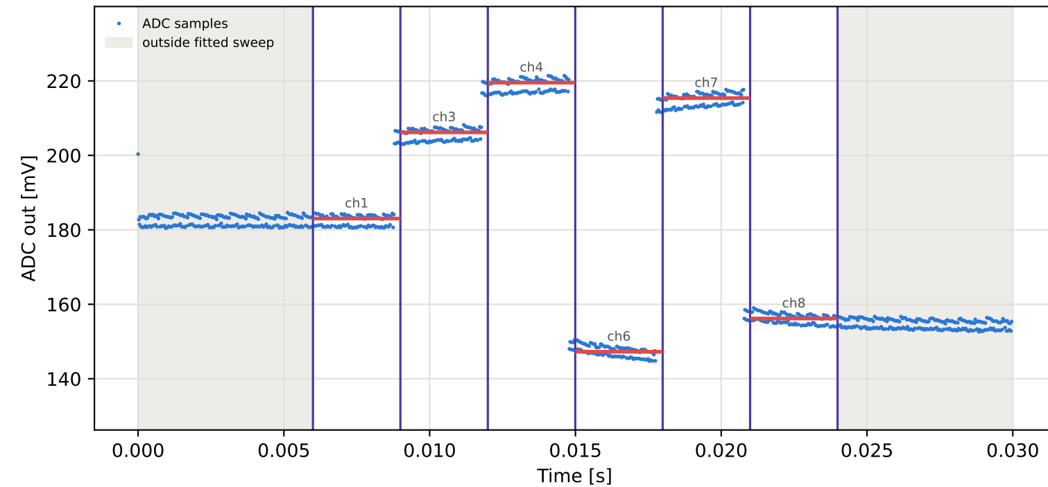
Tag5 &lt;- Tag3 | 945 MHz | run 0 | rep 1 | phase -154.72 deg
