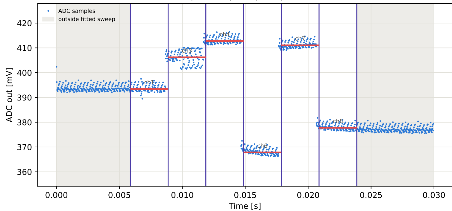
Tag1 &lt;- Tag8 | 955 MHz | run 0 | rep 1 | phase 31.34 deg
