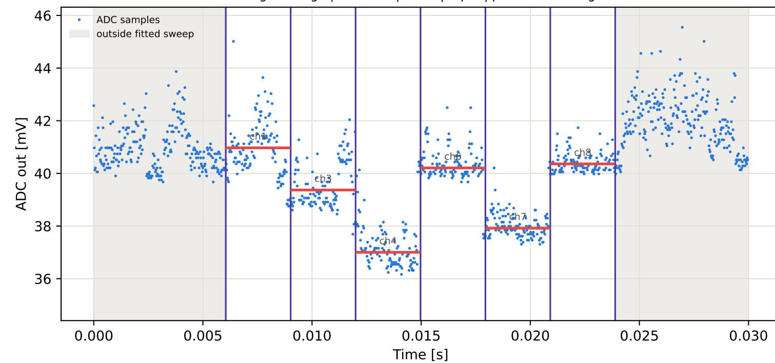
Tag2 &lt;- Tag5 | 985 MHz | run 0 | rep 1 | phase -93.79 deg
