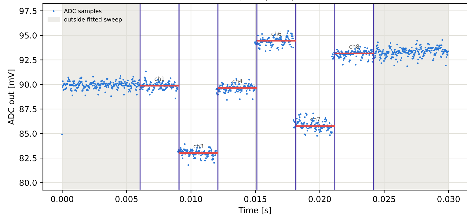
Tag16 &lt;- Tag1 | 795 MHz | run 0 | rep 1 | phase -179.42 deg
