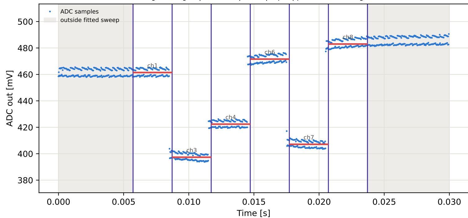
Tag6 &lt;- Tag10 | 835 MHz | run 0 | rep 1 | phase 159.62 deg
