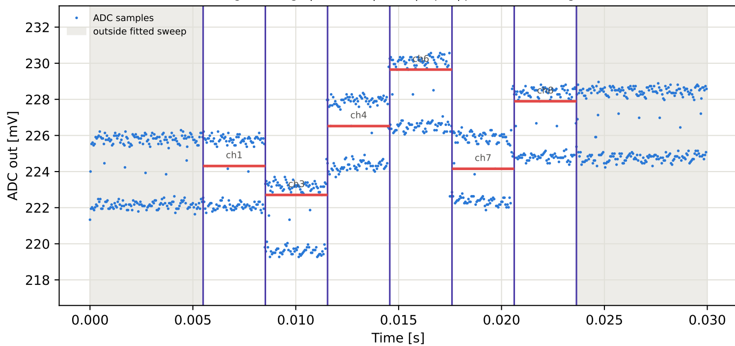
Tag10 &lt;- Tag8 | 795 MHz | run 0 | rep 1 | phase 92.90 deg
