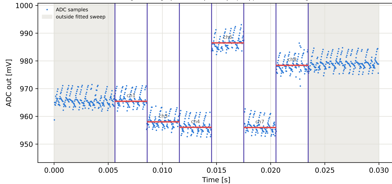
Tag16 &lt;- Tag6 | 935 MHz | run 0 | rep 1 | phase 126.00 deg
