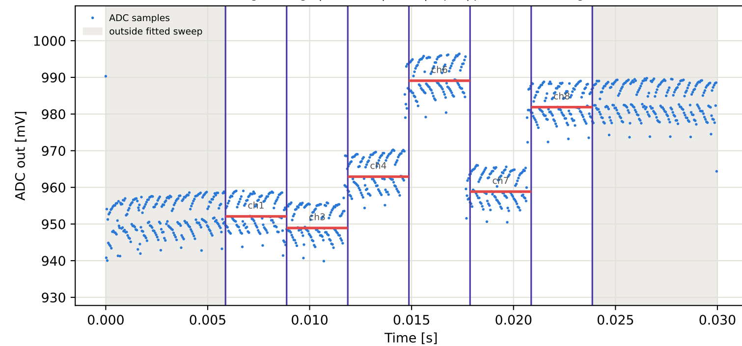
Tag6 &lt;- Tag9 | 895 MHz | run 0 | rep 1 | phase -6.08 deg
