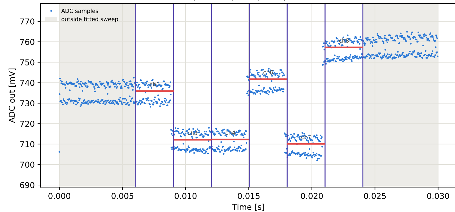
Tag8 &lt;- Tag10 | 885 MHz | run 0 | rep 1 | phase -144.61 deg
