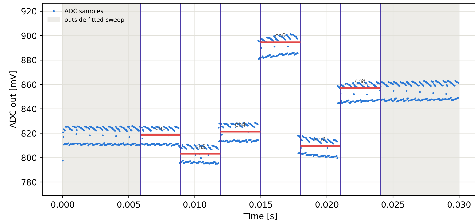
Tag9 &lt;- Tag16 | 945 MHz | run 0 | rep 1 | phase -178.39 deg
