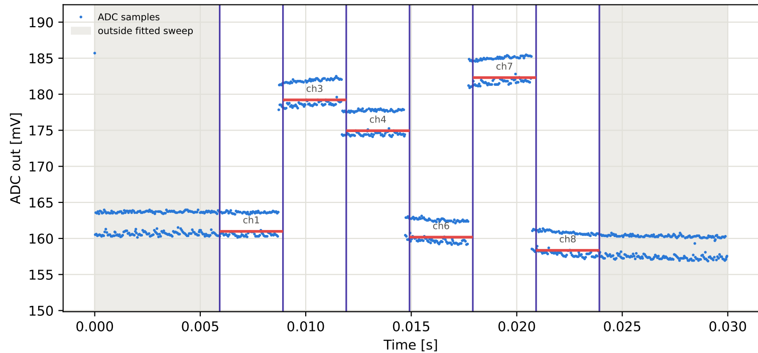
Tag8 &lt;- Tag16 | 795 MHz | run 0 | rep 1 | phase -11.47 deg
