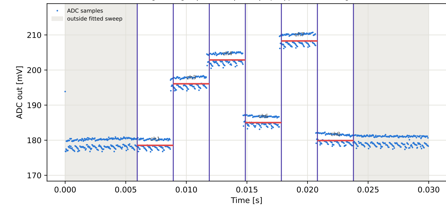
Tag9 &lt;- Tag16 | 795 MHz | run 0 | rep 1 | phase 21.66 deg
