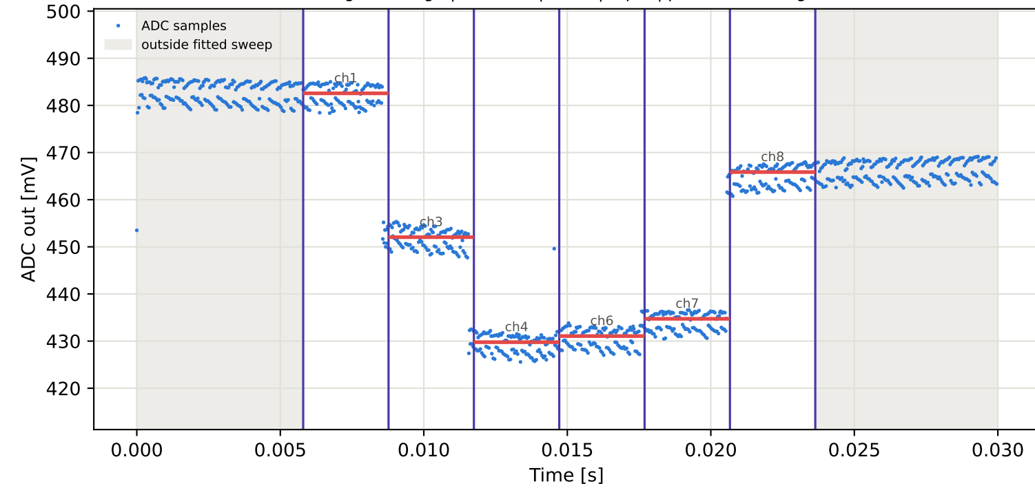
Tag15 &lt;- Tag5 | 875 MHz | run 0 | rep 1 | phase 67.38 deg
