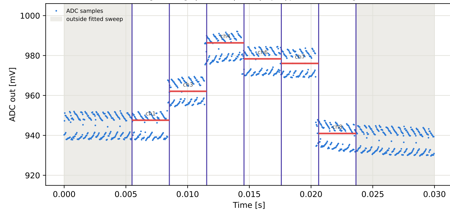
Tag2 &lt;- Tag1 | 915 MHz | run 0 | rep 1 | phase 36.90 deg
