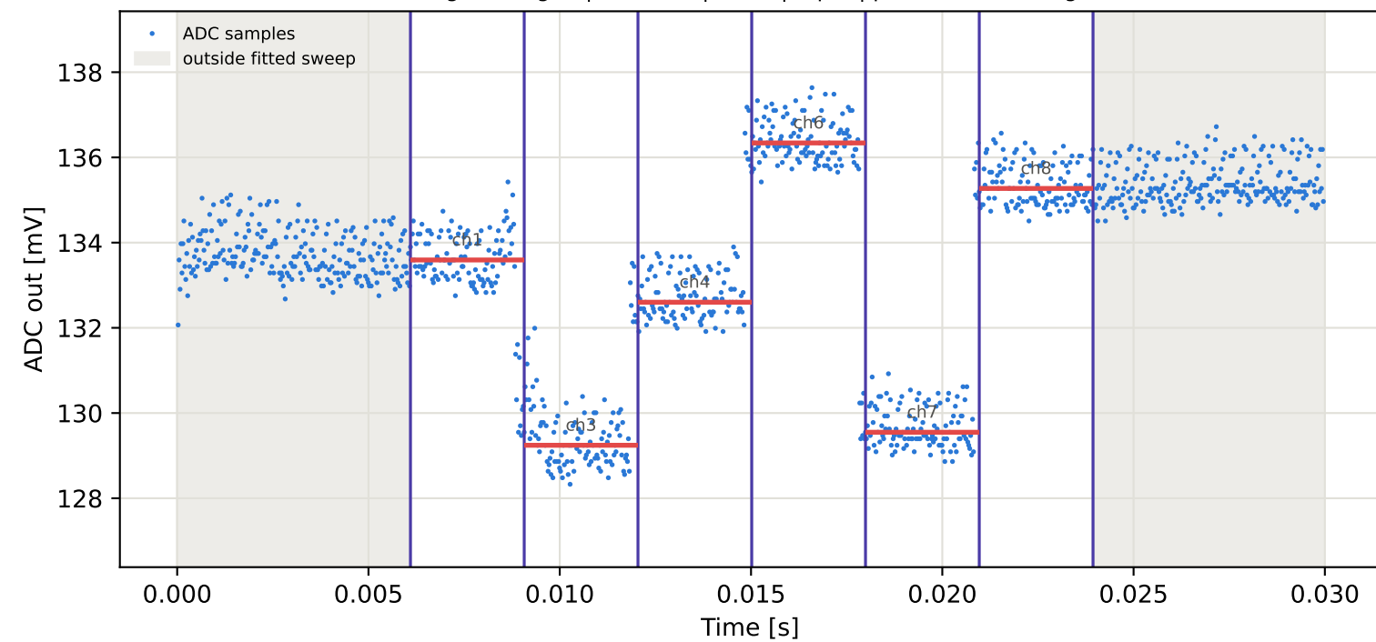
Tag3 &lt;- Tag2 | 785 MHz | run 0 | rep 1 | phase -123.55 deg
