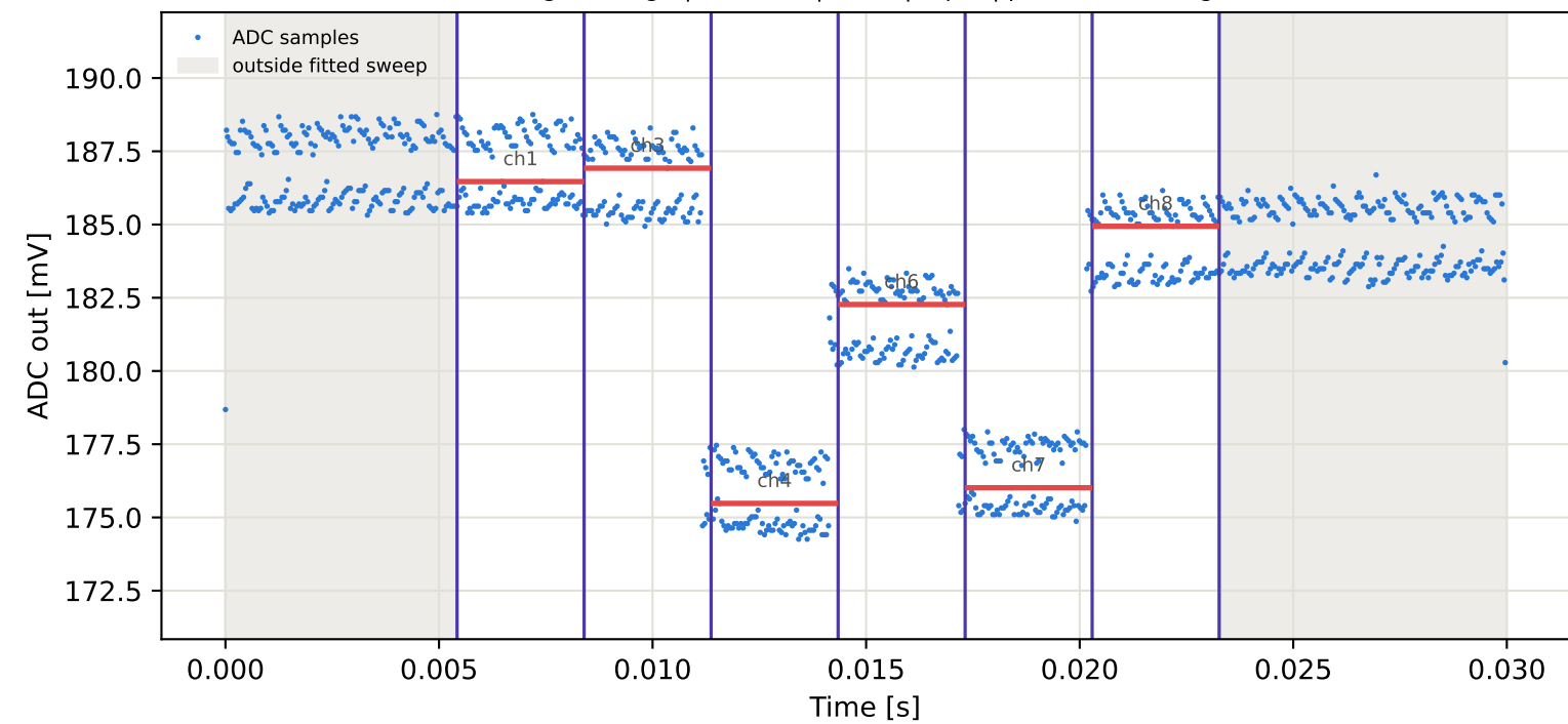
Tag8 &lt;- Tag5 | 795 MHz | run 0 | rep 1 | phase 123.94 deg
