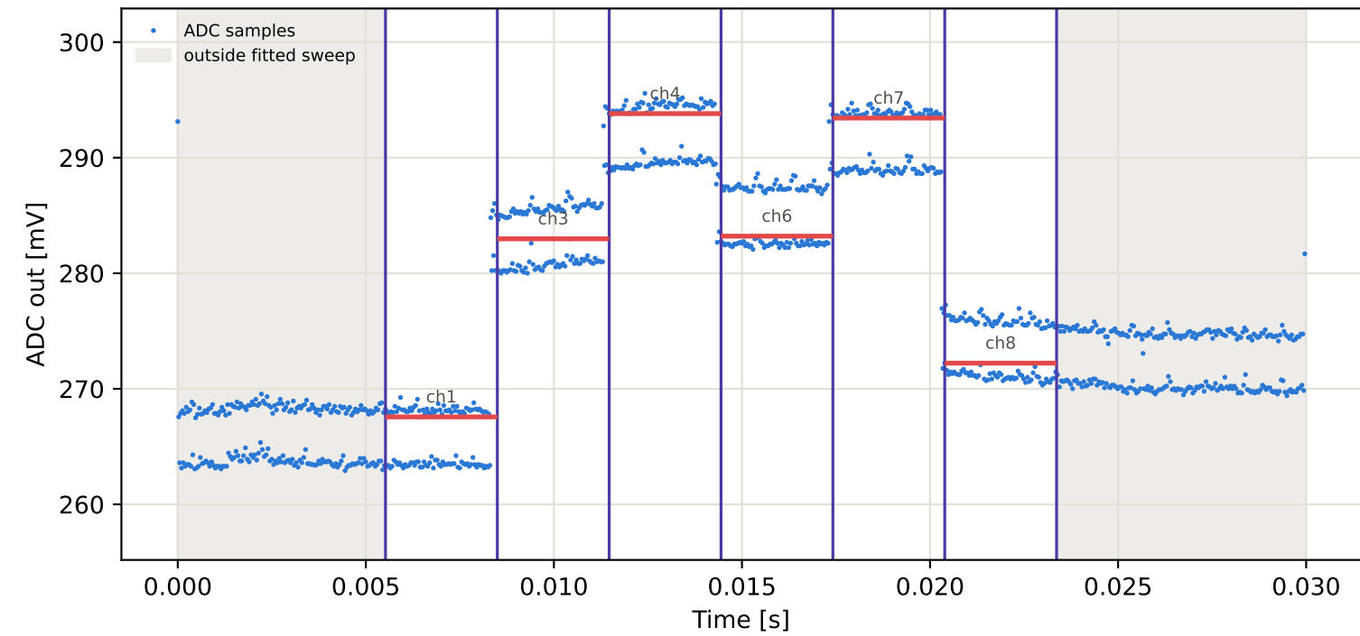
Tag2 &lt;- Tag8 | 855 MHz | run 0 | rep 1 | phase -69.86 deg
