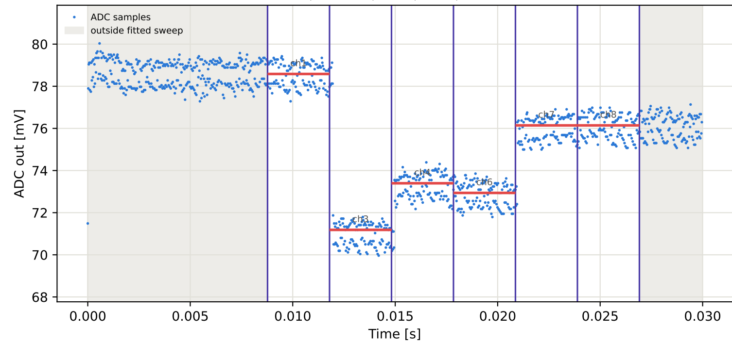
Tag6 &lt;- Tag5 | 795 MHz | run 0 | rep 1 | phase 82.14 deg
