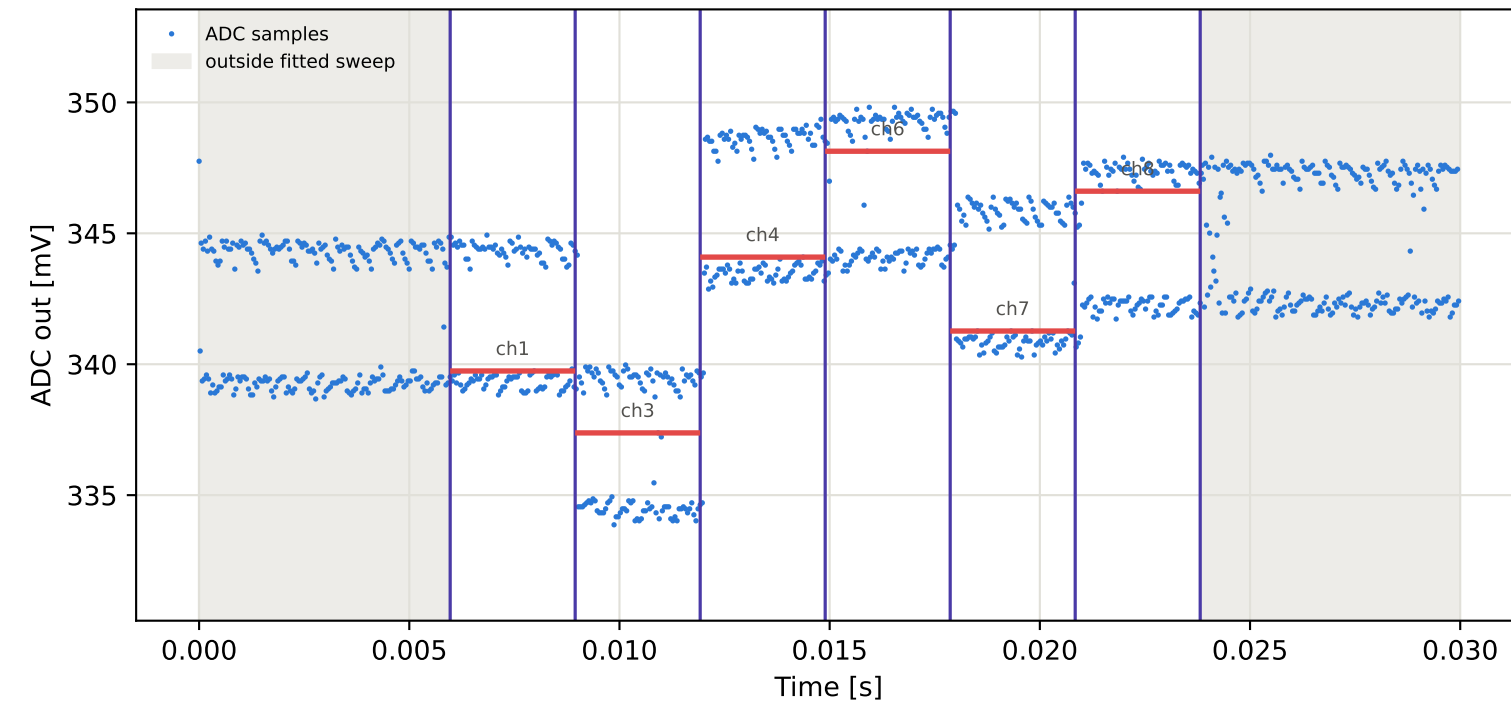
Tag7 &lt;- Tag5 | 805 MHz | run 0 | rep 1 | phase 155.95 deg
