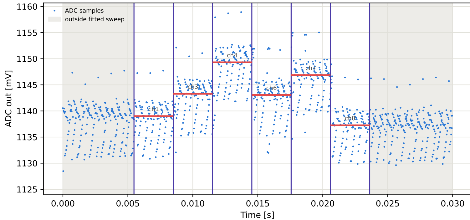
Tag7 &lt;- Tag15 | 935 MHz | run 0 | rep 1 | phase -147.30 deg
