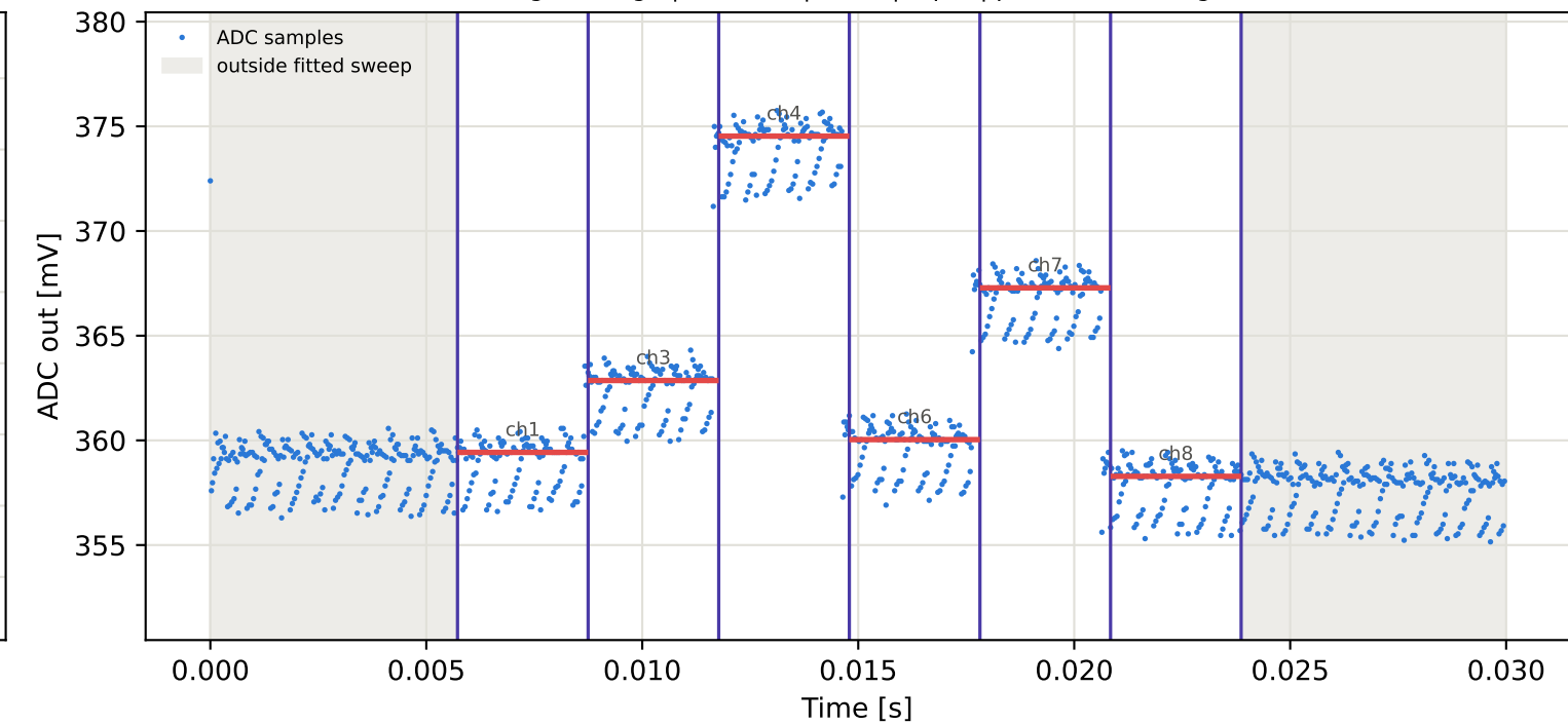
Tag8 &lt;- Tag5 | 995 MHz | run 0 | rep 1 | phase 80.16 deg
