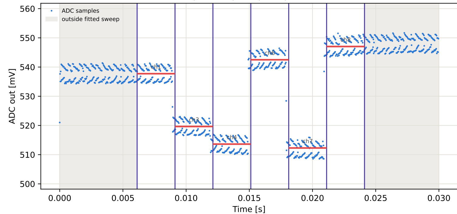
Tag8 &lt;- Tag7 | 835 MHz | run 0 | rep 1 | phase 135.80 deg
