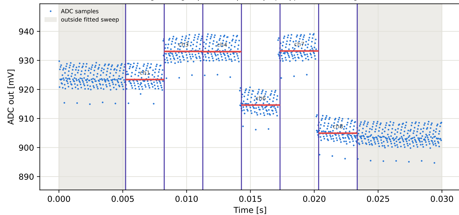
Tag3 &lt;- Tag2 | 895 MHz | run 0 | rep 1 | phase -140.34 deg
