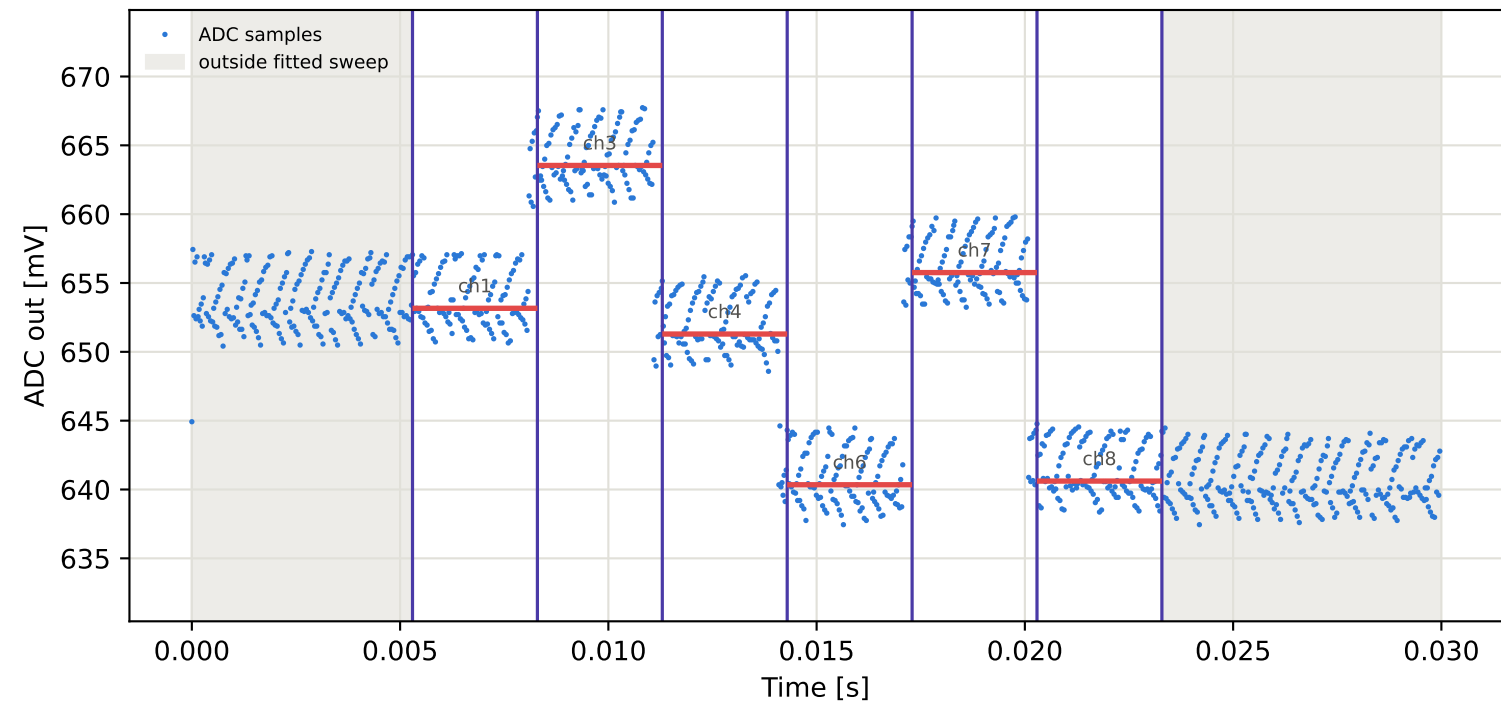
Tag6 &lt;- Tag3 | 855 MHz | run 0 | rep 1 | phase 44.73 deg
