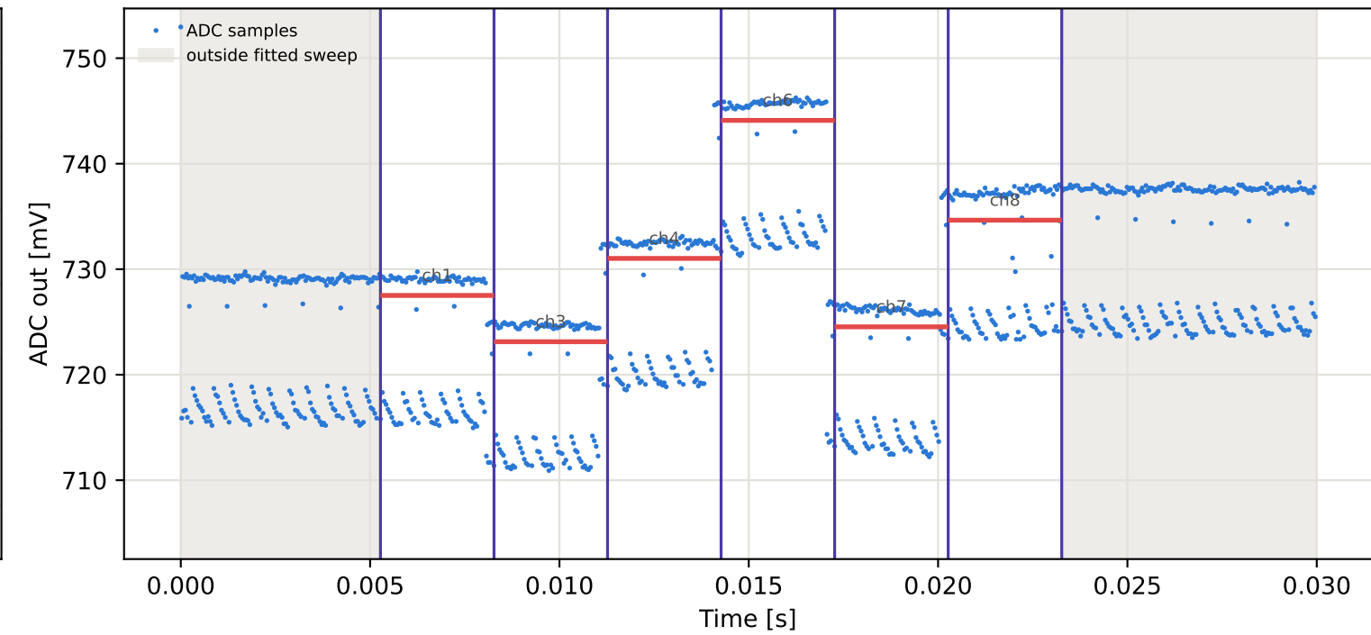
Tag9 &lt;- Tag8 | 985 MHz | run 0 | rep 1 | phase 178.47 deg
