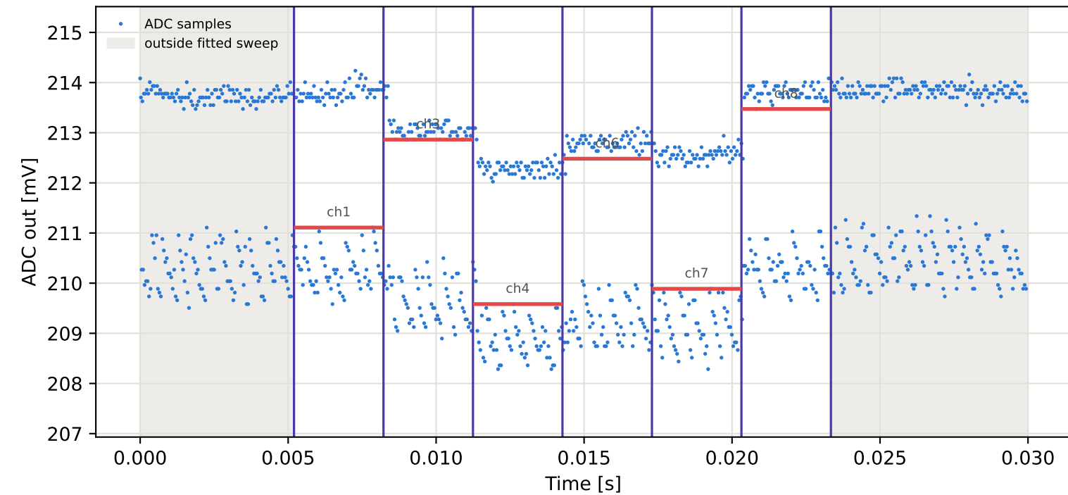
Tag10 &lt;- Tag4 | 805 MHz | run 0 | rep 1 | phase 34.27 deg
