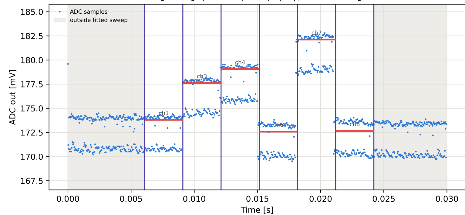
Tag9 &lt;- Tag5 | 775 MHz | run 0 | rep 1 | phase -46.00 deg
