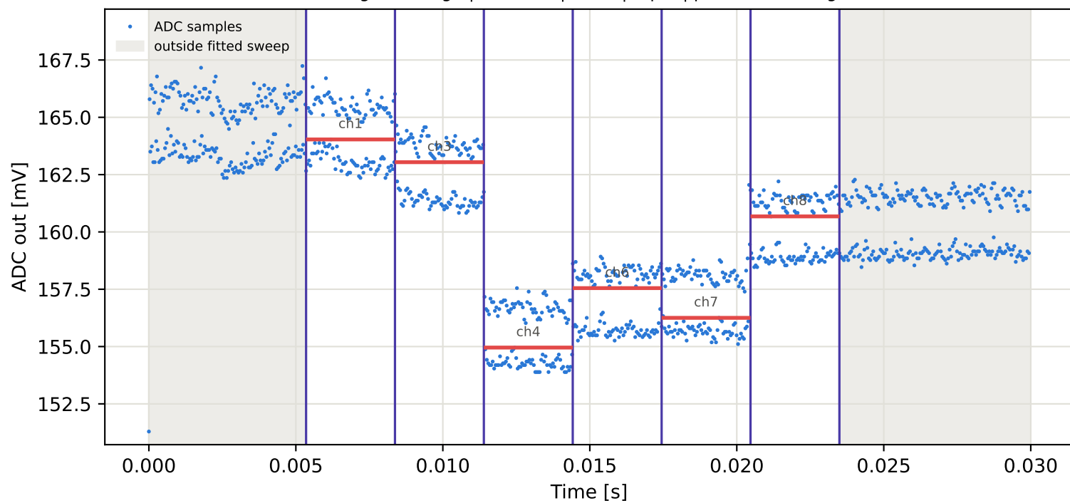
Tag15 &lt;- Tag6 | 825 MHz | run 0 | rep 1 | phase 71.03 deg
