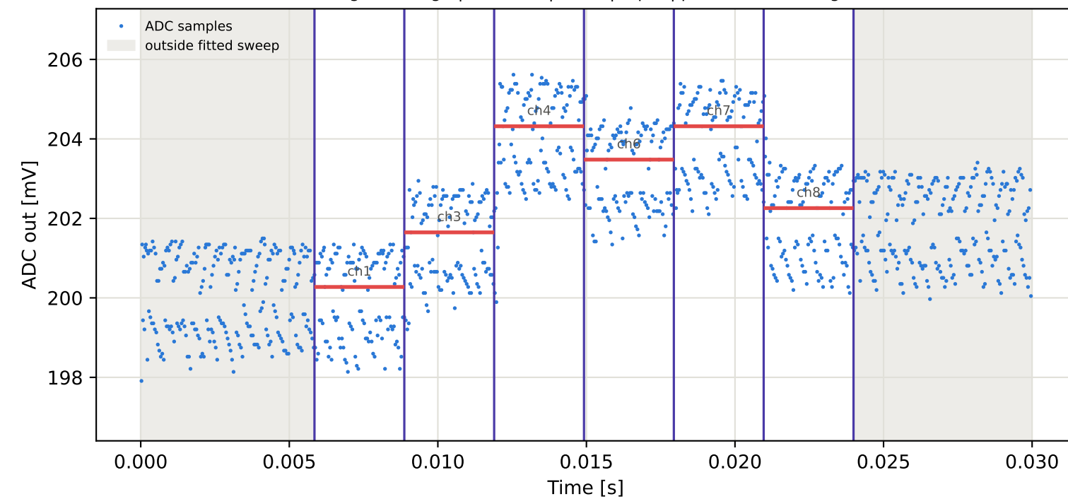
Tag16 &lt;- Tag6 | 825 MHz | run 0 | rep 1 | phase 165.89 deg
