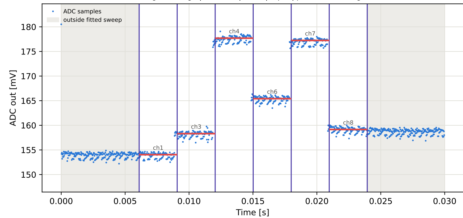
Tag15 &lt;- Tag10 | 775 MHz | run 0 | rep 1 | phase -32.51 deg
