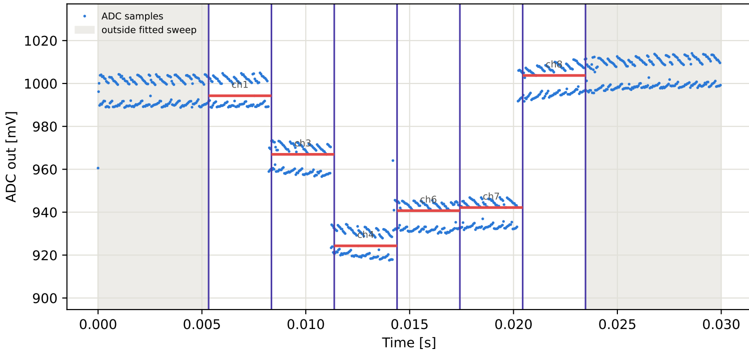
Tag16 &lt;- Tag15 | 915 MHz | run 0 | rep 1 | phase 72.60 deg
