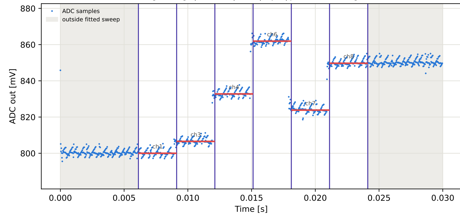
Tag9 &lt;- Tag5 | 865 MHz | run 0 | rep 1 | phase 167.90 deg
