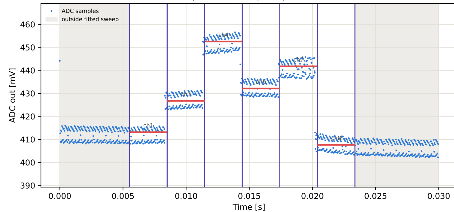
Tag1 &lt;- Tag7 | 935 MHz | run 0 | rep 1 | phase 20.84 deg
