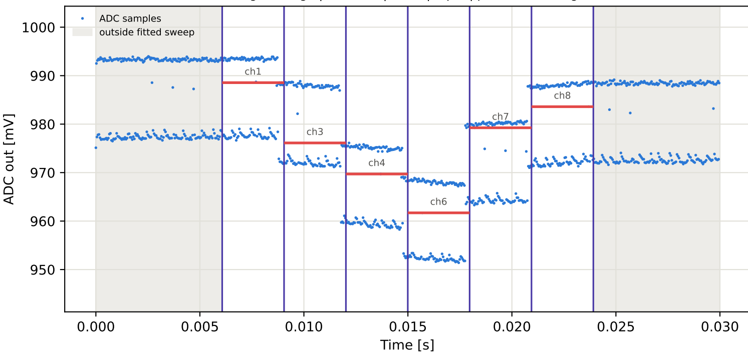
Tag6 &lt;- Tag4 | 895 MHz | run 0 | rep 1 | phase -22.98 deg
