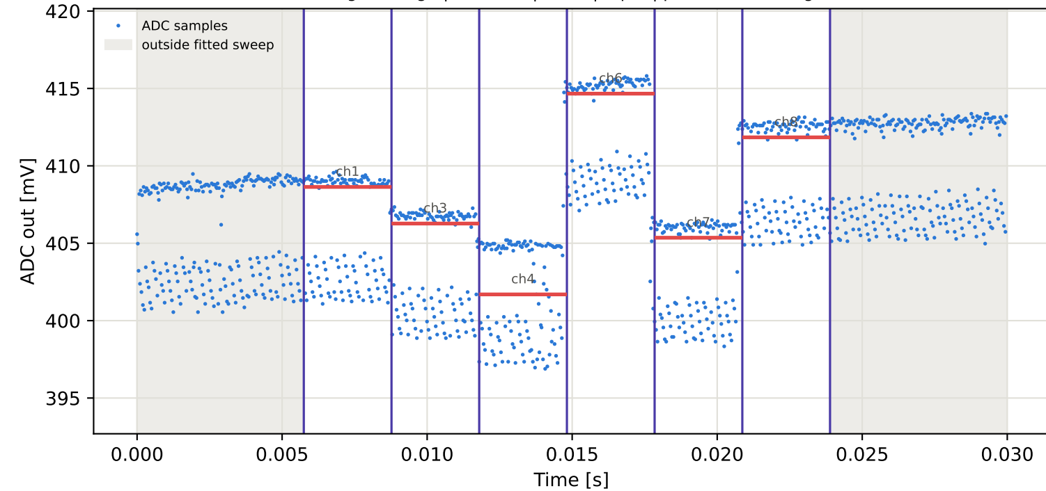
Tag1 &lt;- Tag4 | 955 MHz | run 0 | rep 1 | phase 142.13 deg
