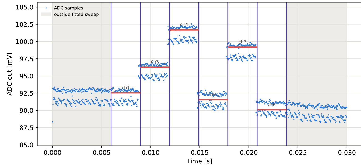
Tag4 &lt;- Tag3 | 995 MHz | run 0 | rep 1 | phase -29.95 deg
