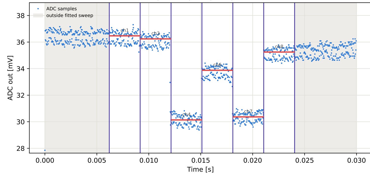
Tag6 &lt;- Tag4 | 785 MHz | run 0 | rep 1 | phase 90.54 deg
