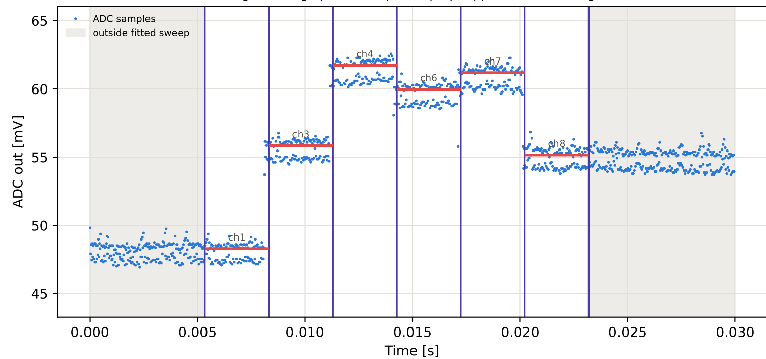
Tag15 &lt;- Tag6 | 845 MHz | run 0 | rep 1 | phase 4.94 deg
