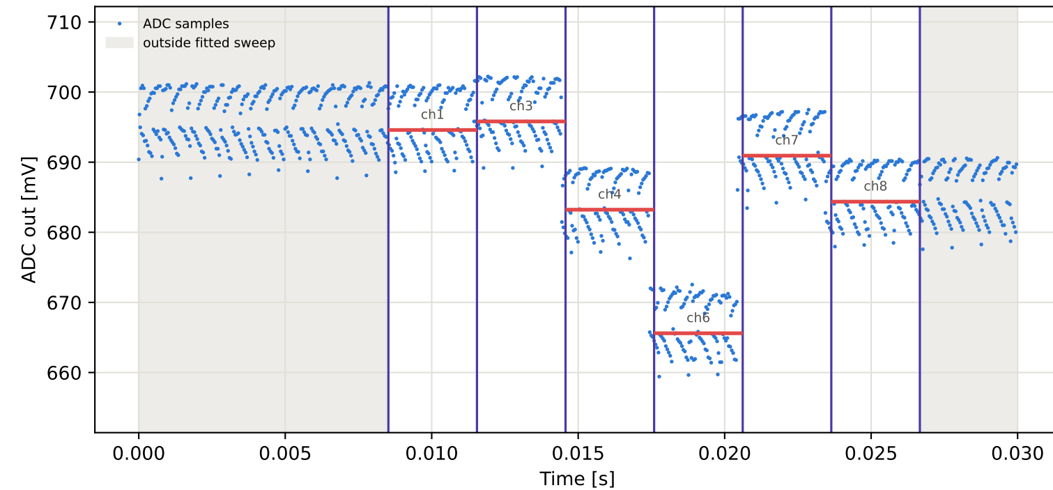
Tag9 &lt;- Tag7 | 955 MHz | run 0 | rep 1 | phase 86.04 deg
