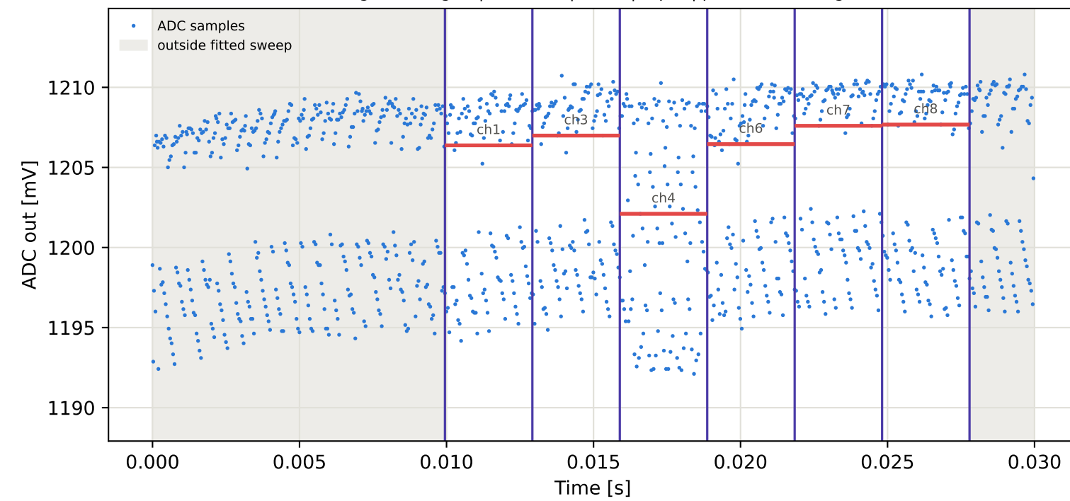
Tag10 &lt;- Tag2 | 875 MHz | run 0 | rep 1 | phase 11.50 deg
