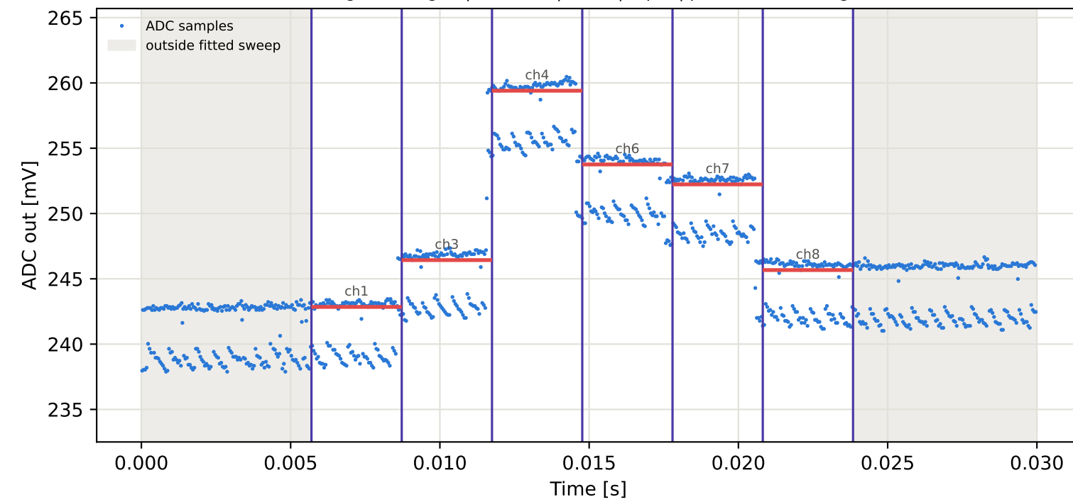
Tag10 &lt;- Tag2 | 985 MHz | run 0 | rep 1 | phase -62.50 deg
