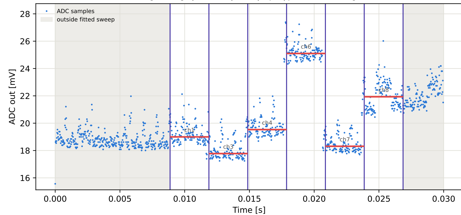
Tag2 &lt;- Tag6 | 955 MHz | run 0 | rep 1 | phase 126.11 deg
