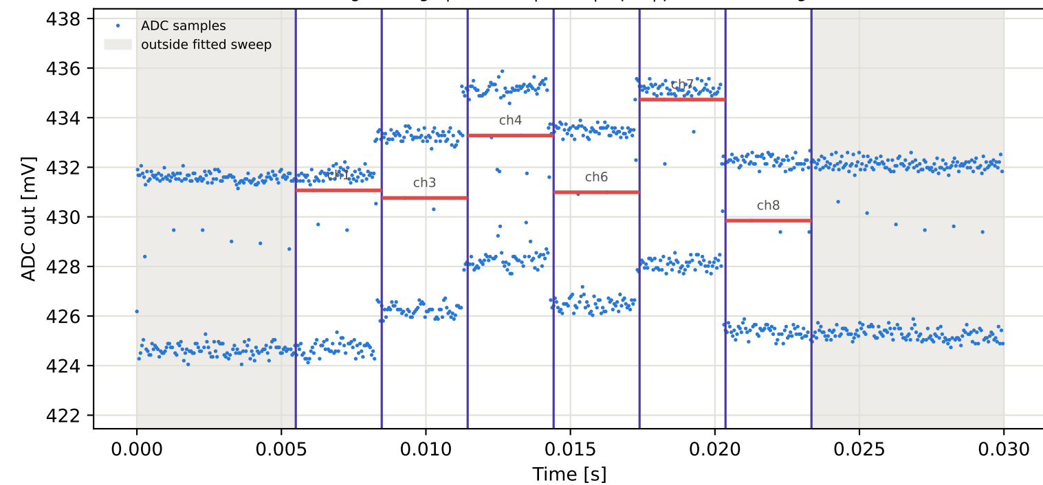
Tag6 &lt;- Tag1 | 835 MHz | run 0 | rep 1 | phase -69.82 deg
