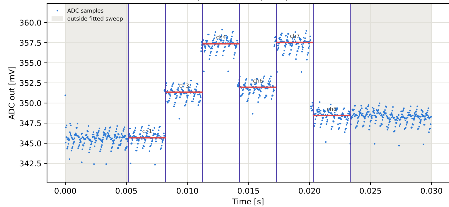
Tag6 &lt;- Tag3 | 825 MHz | run 0 | rep 1 | phase 23.84 deg
