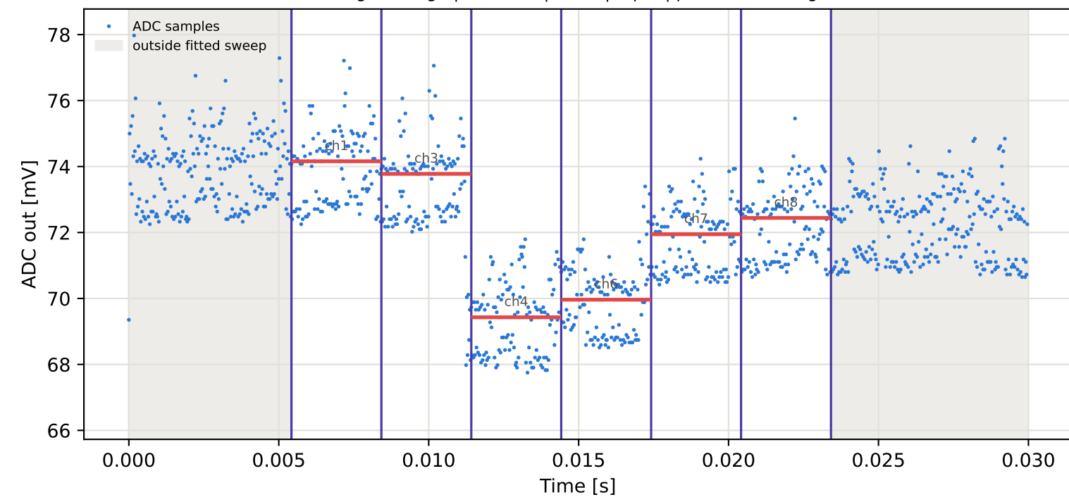
Tag2 &lt;- Tag7 | 995 MHz | run 0 | rep 1 | phase 41.46 deg
