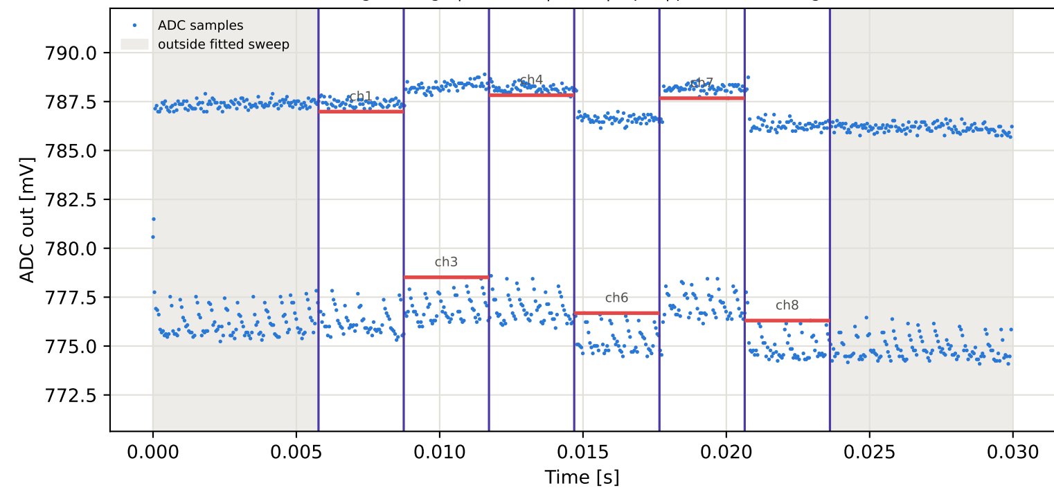
Tag9 &lt;- Tag15 | 895 MHz | run 0 | rep 1 | phase -151.44 deg
