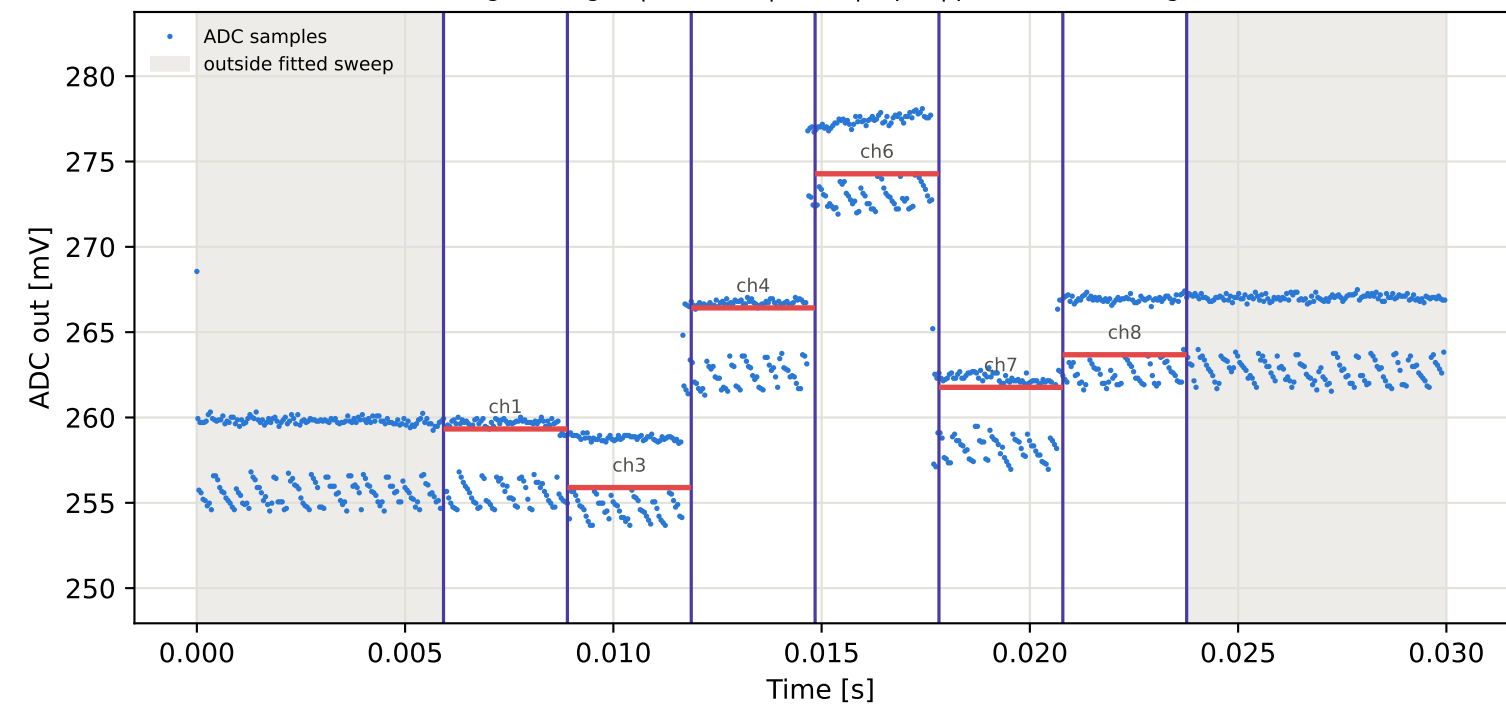
Tag5 &lt;- Tag2 | 955 MHz | run 0 | rep 1 | phase -58.30 deg
