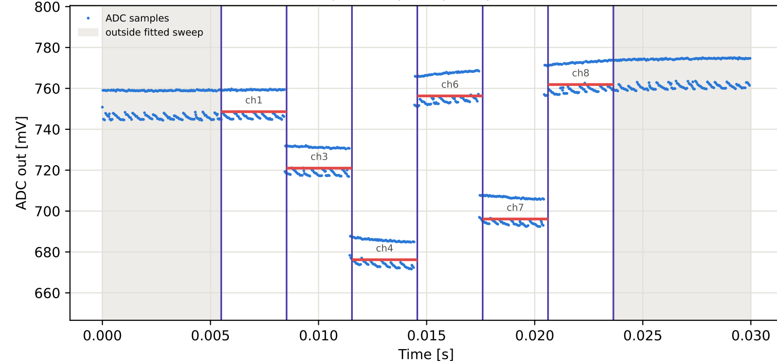
Tag9 &lt;- Tag7 | 965 MHz | run 0 | rep 1 | phase 104.14 deg
