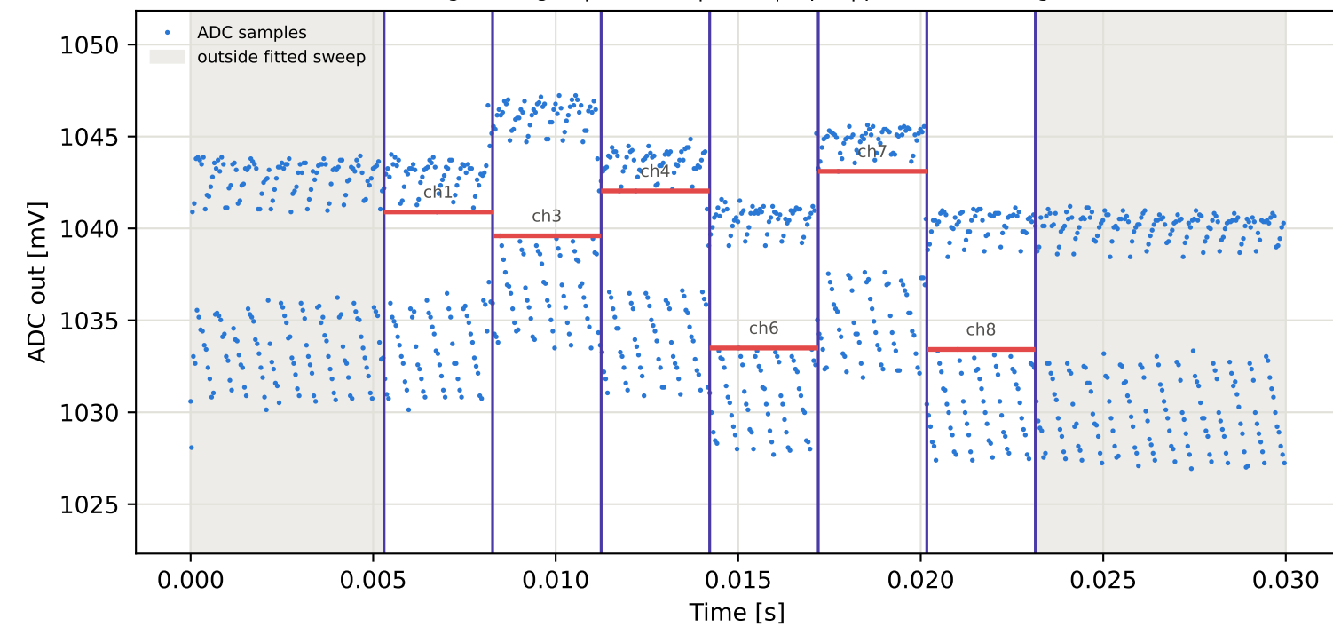
Tag7 &lt;- Tag3 | 855 MHz | run 0 | rep 1 | phase -107.58 deg
