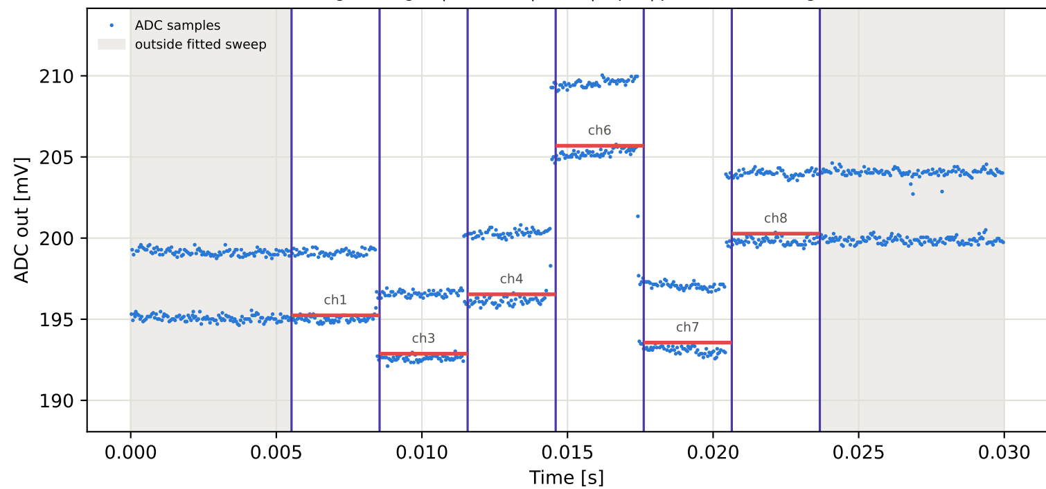
Tag4 &lt;- Tag16 | 985 MHz | run 0 | rep 1 | phase -37.42 deg
