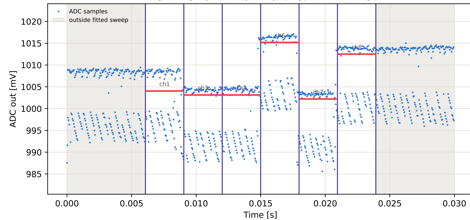
Tag7 &lt;- Tag3 | 975 MHz | run 0 | rep 1 | phase -75.19 deg
