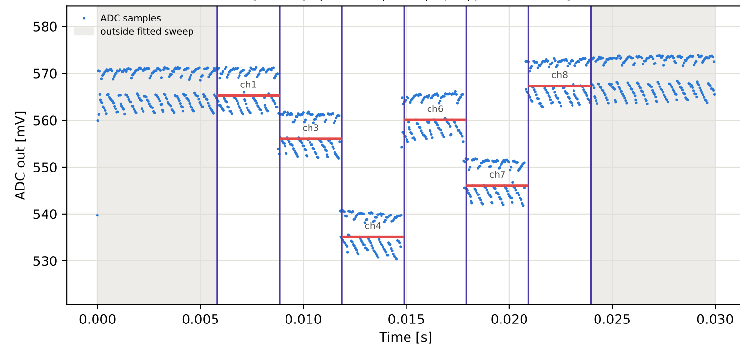
Tag9 &lt;- Tag7 | 975 MHz | run 0 | rep 1 | phase 87.01 deg
