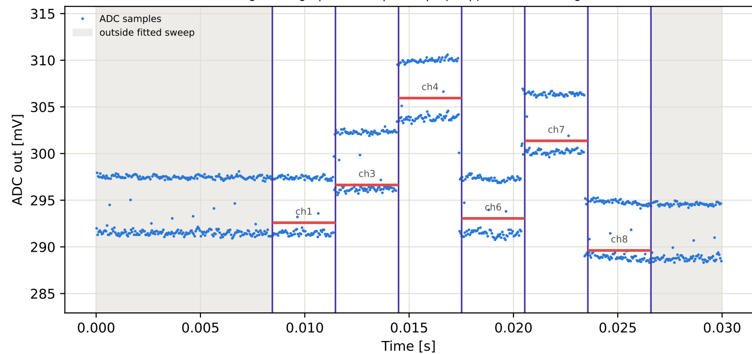
Tag6 &lt;- Tag5 | 955 MHz | run 0 | rep 1 | phase -84.90 deg
