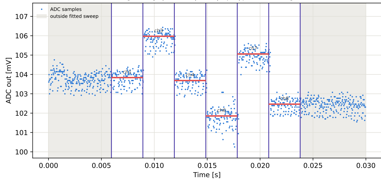
Tag1 &lt;- Tag7 | 795 MHz | run 0 | rep 1 | phase -131.77 deg
