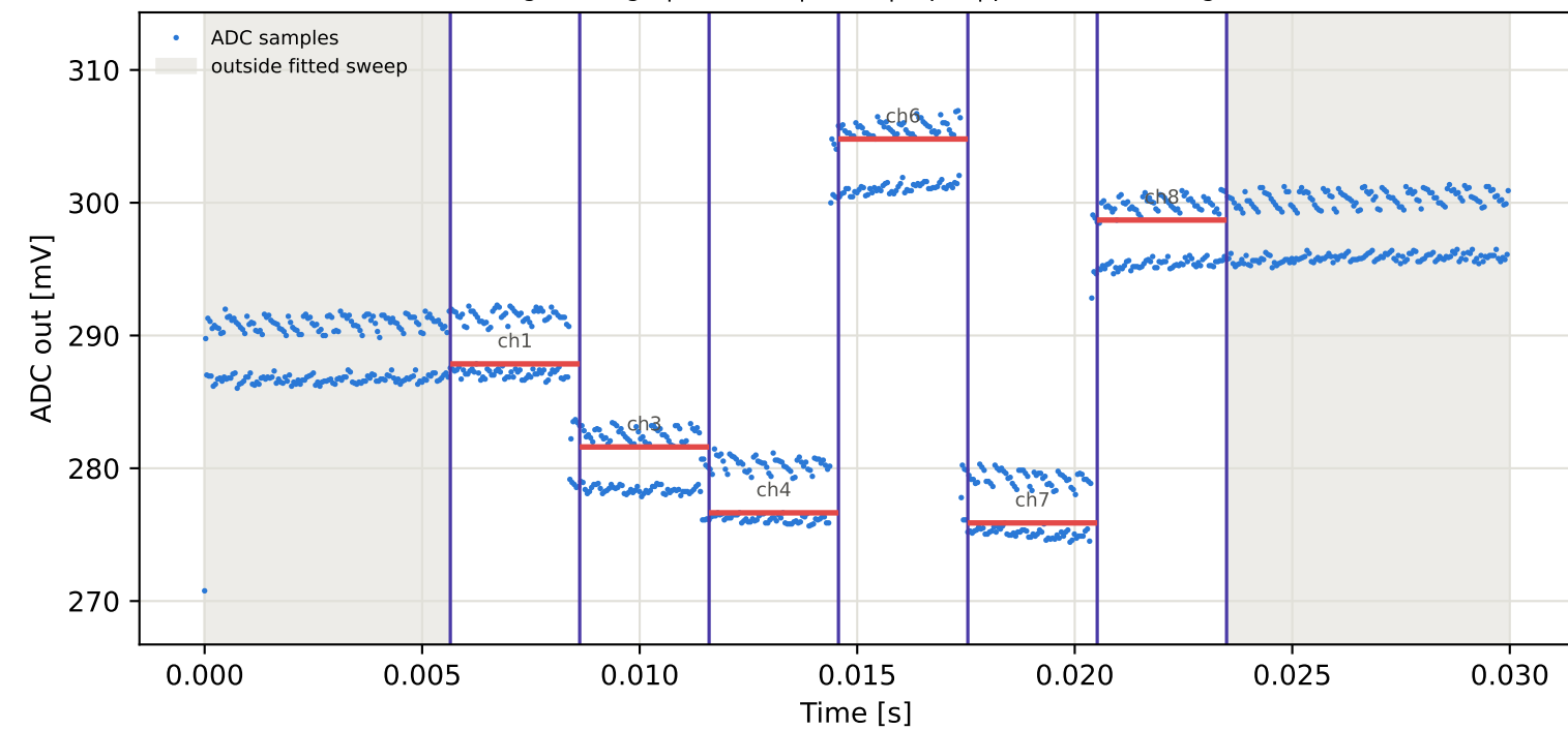
Tag5 &lt;- Tag9 | 965 MHz | run 0 | rep 1 | phase 16.91 deg
