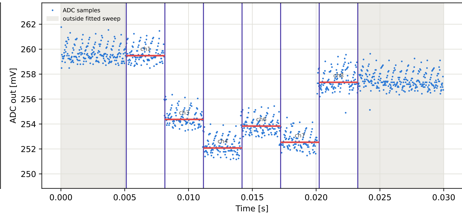
Tag15 &lt;- Tag6 | 855 MHz | run 0 | rep 1 | phase -168.04 deg
