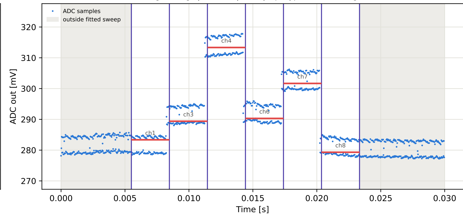
Tag4 &lt;- Tag8 | 965 MHz | run 0 | rep 1 | phase -35.97 deg
