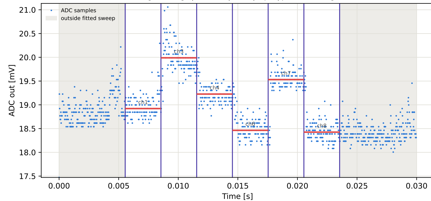
Tag15 &lt;- Tag9 | 775 MHz | run 0 | rep 1 | phase -139.77 deg
