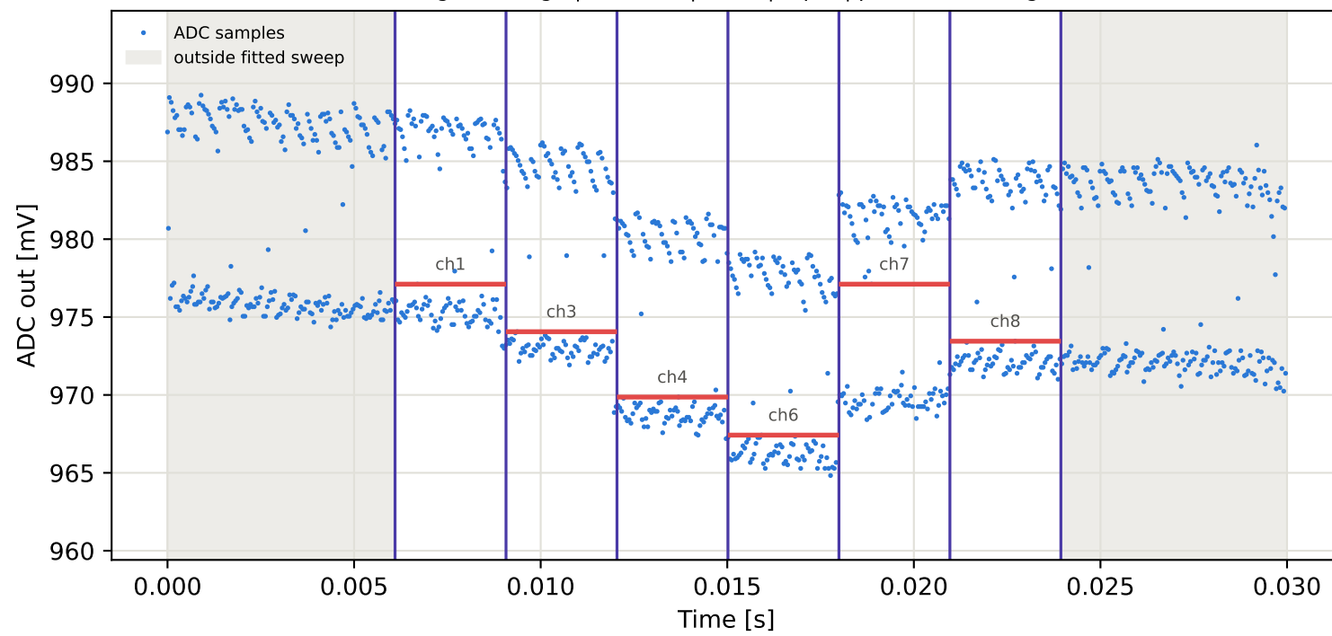
Tag16 &lt;- Tag4 | 875 MHz | run 0 | rep 1 | phase 0.88 deg
