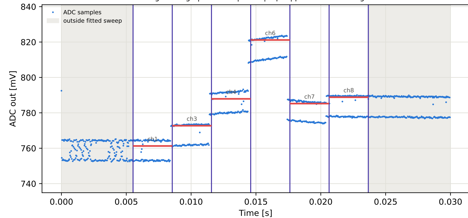
Tag9 &lt;- Tag7 | 895 MHz | run 0 | rep 1 | phase 45.24 deg
