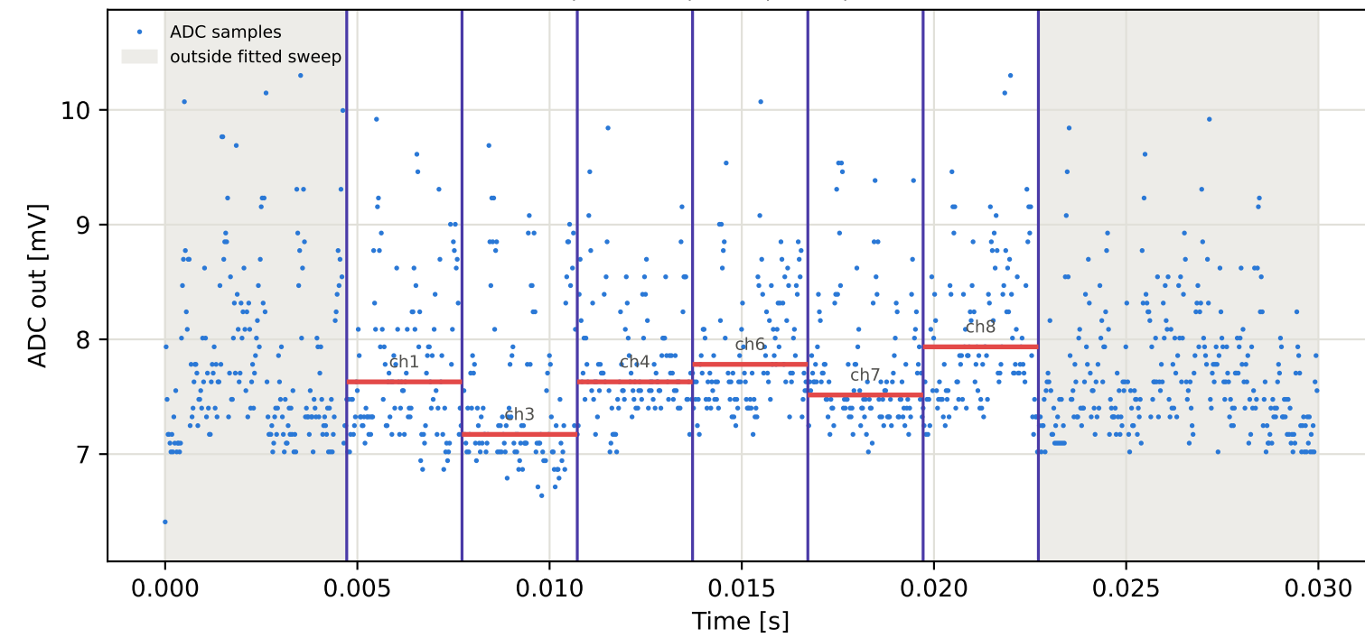
Tag2 &lt;- Tag7 | 785 MHz | run 0 | rep 1 | phase -164.19 deg
