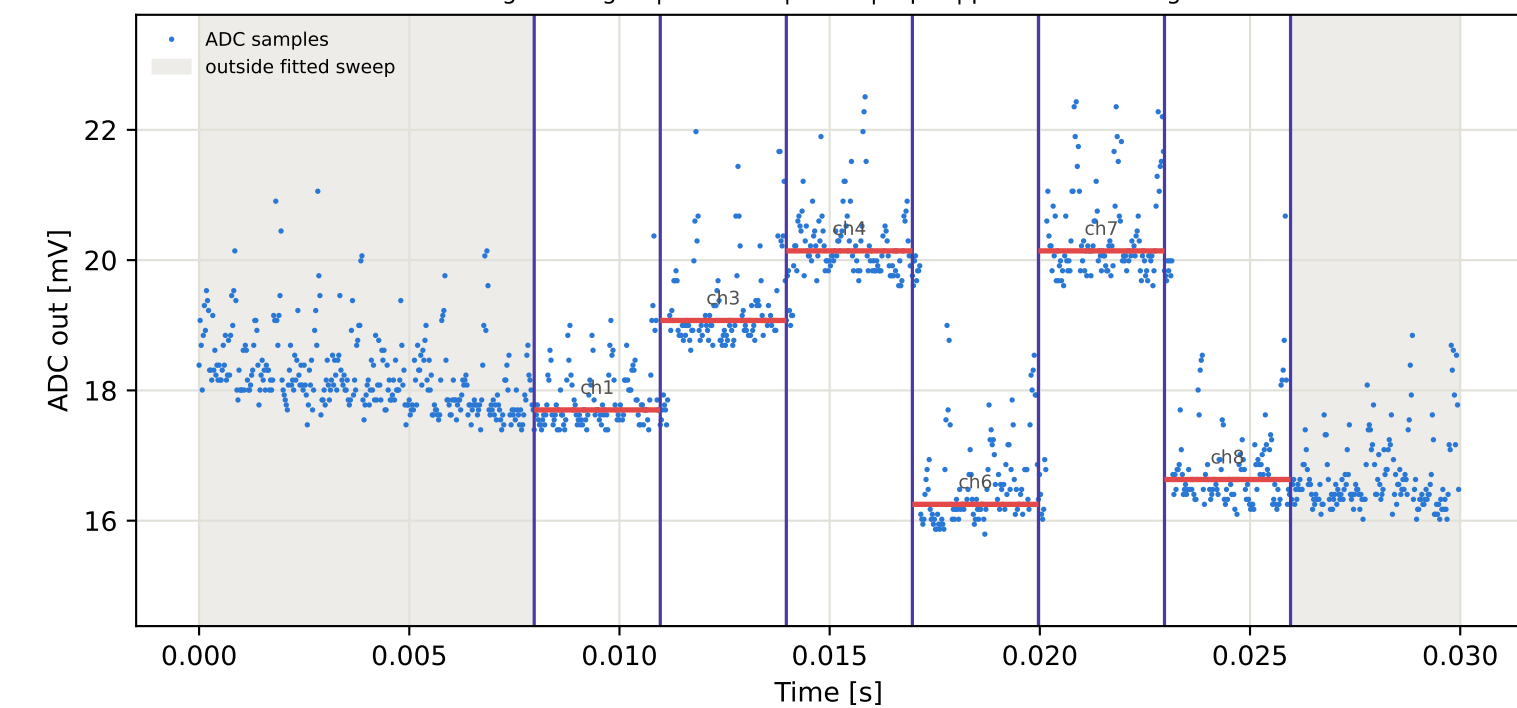
Tag2 &lt;- Tag15 | 955 MHz | run 0 | rep 1 | phase -43.60 deg
