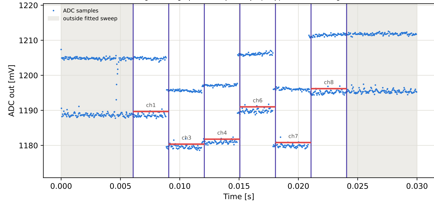
Tag10 &lt;- Tag5 | 865 MHz | run 0 | rep 1 | phase 142.12 deg
