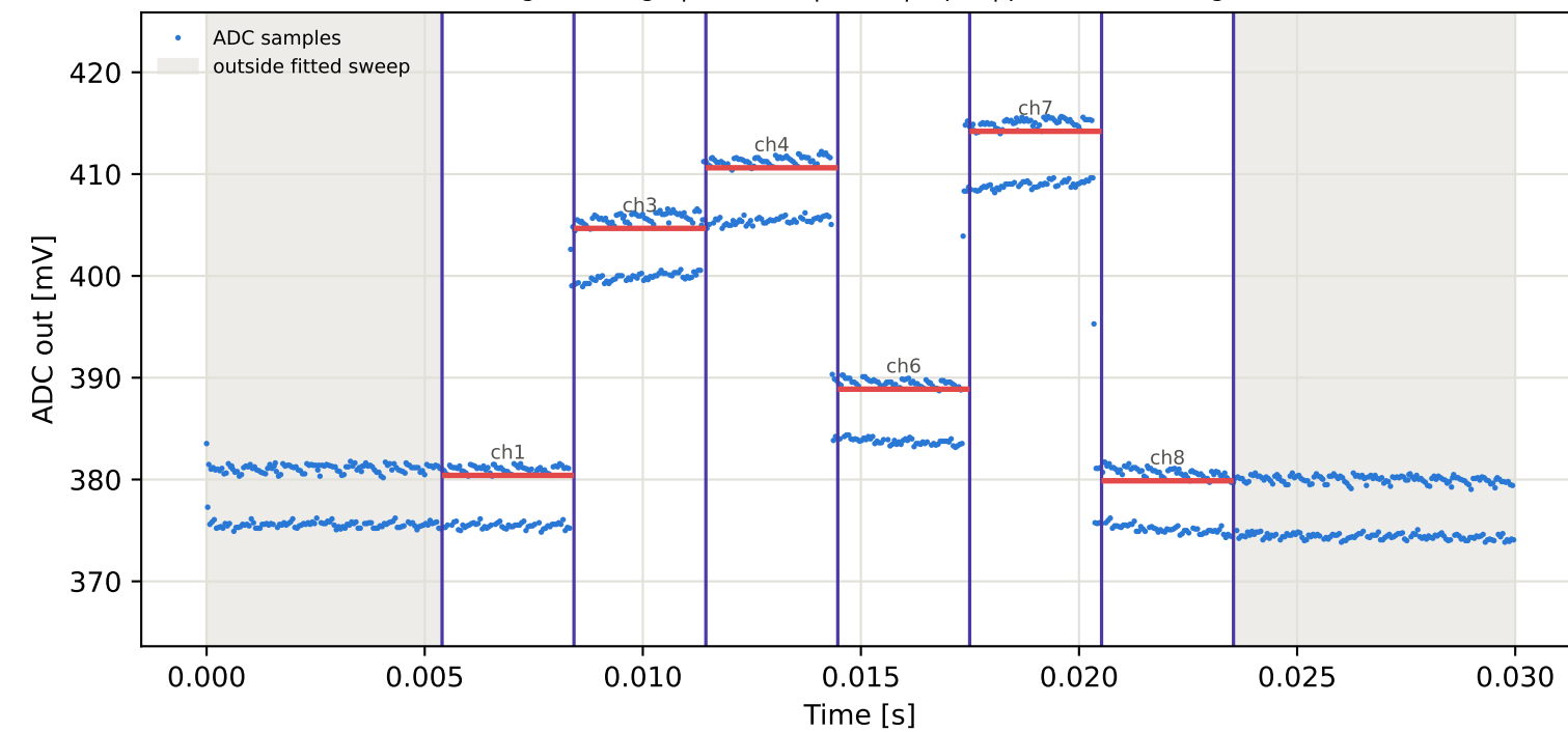
Tag10 &lt;- Tag8 | 825 MHz | run 0 | rep 1 | phase -146.06 deg
