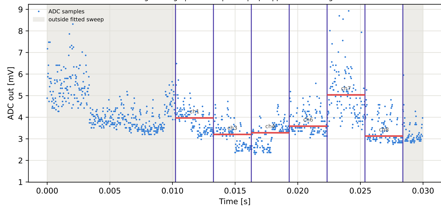
Tag2 &lt;- Tag8 | 965 MHz | run 0 | rep 1 | phase -9.49 deg
