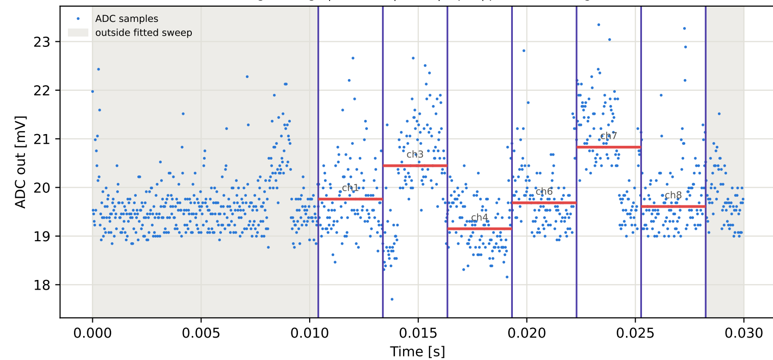
Tag2 &lt;- Tag6 | 975 MHz | run 0 | rep 1 | phase -91.28 deg
