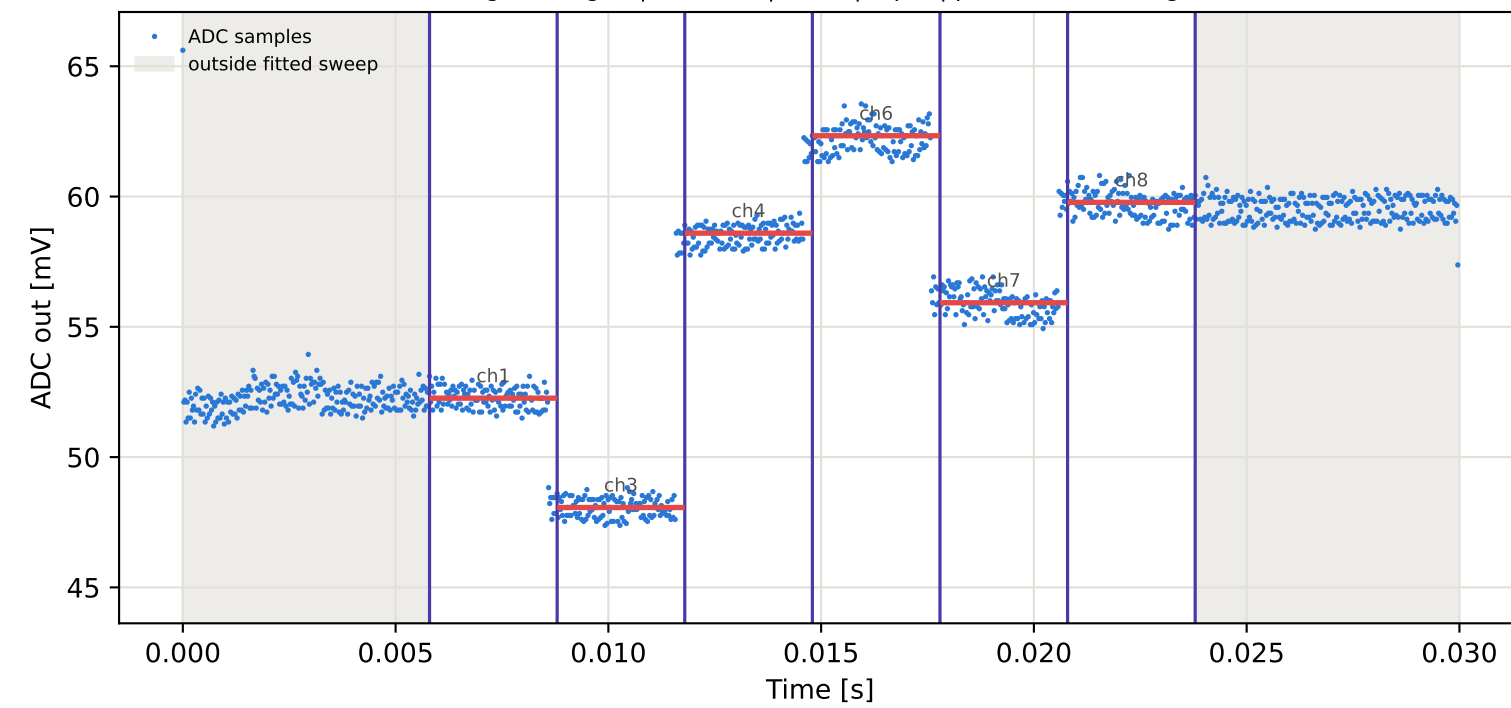
Tag1 &lt;- Tag16 | 825 MHz | run 0 | rep 1 | phase -159.19 deg
