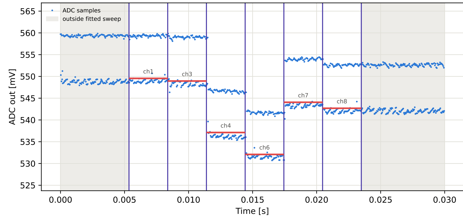
Tag9 &lt;- Tag2 | 975 MHz | run 0 | rep 1 | phase -95.42 deg
