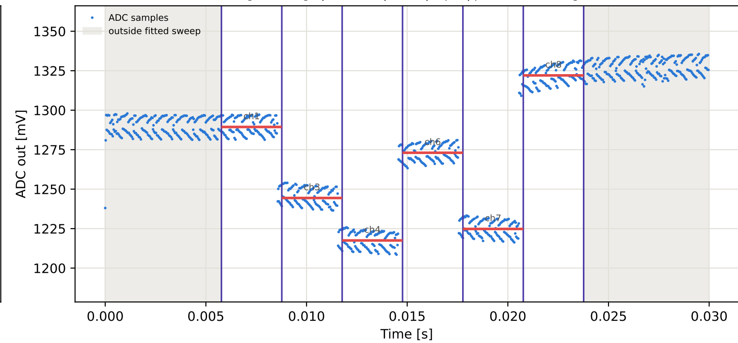
Tag2 &lt;- Tag10 | 905 MHz | run 0 | rep 1 | phase 78.76 deg
