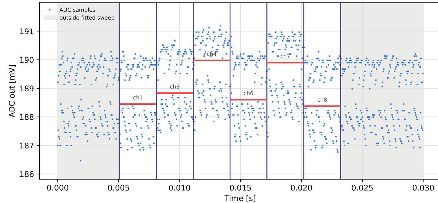
Tag8 &lt;- Tag15 | 775 MHz | run 0 | rep 1 | phase -178.57 deg
