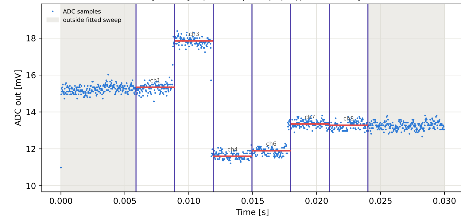
Tag16 &lt;- Tag10 | 785 MHz | run 0 | rep 1 | phase 55.63 deg
