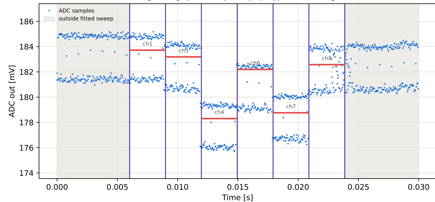
Tag7 &lt;- Tag5 | 775 MHz | run 0 | rep 1 | phase 97.36 deg
