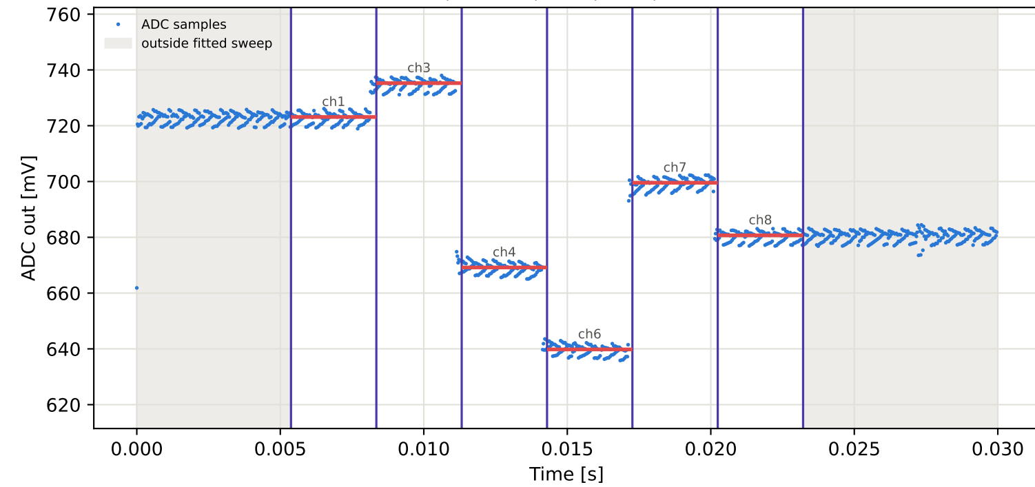
Tag9 &lt;- Tag7 | 845 MHz | run 0 | rep 1 | phase 38.53 deg
