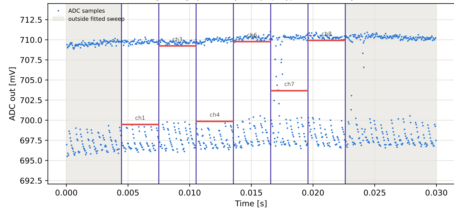
Tag8 &lt;- Tag4 | 965 MHz | run 0 | rep 1 | phase -67.57 deg
