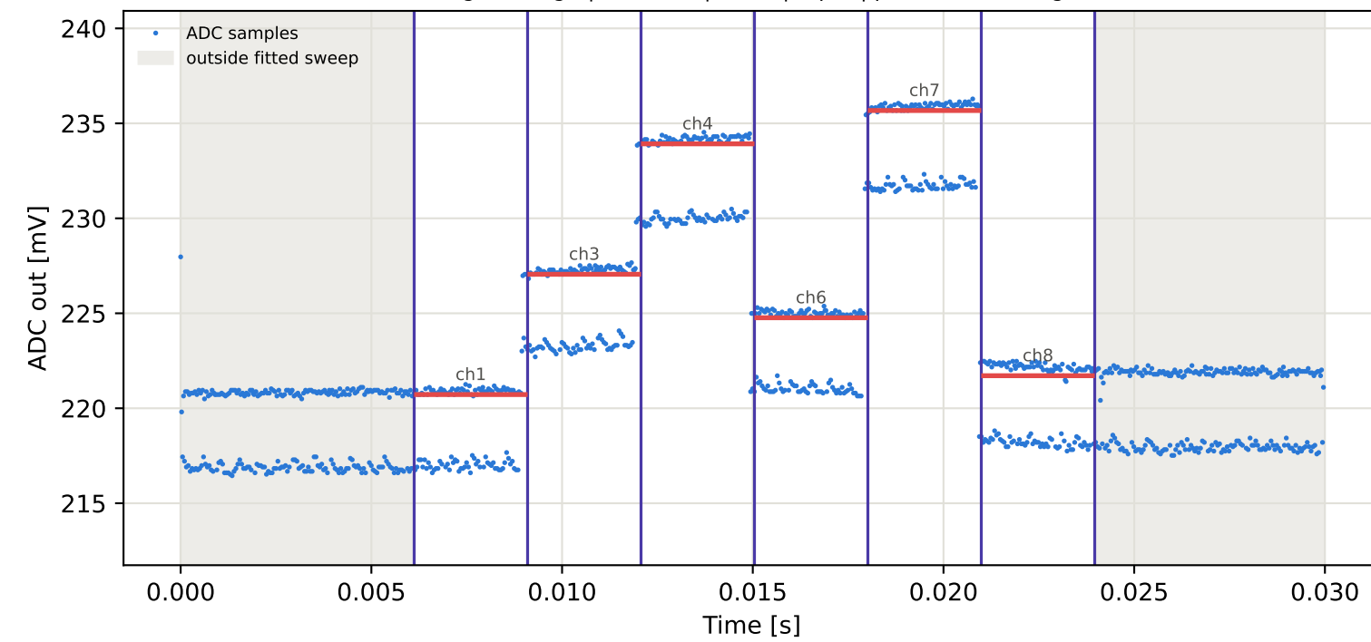
Tag8 &lt;- Tag1 | 785 MHz | run 0 | rep 1 | phase -35.71 deg
