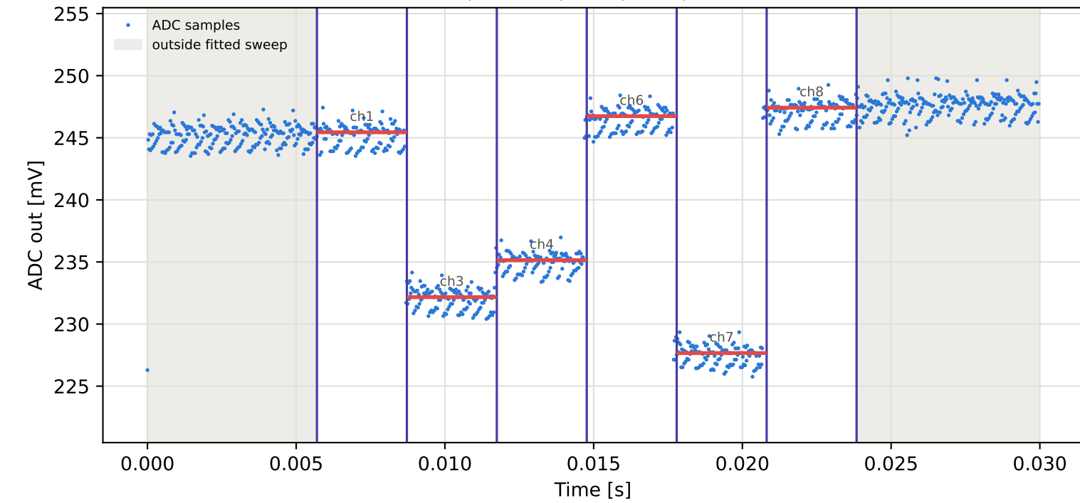
Tag7 &lt;- Tag10 | 785 MHz | run 0 | rep 1 | phase 154.58 deg
