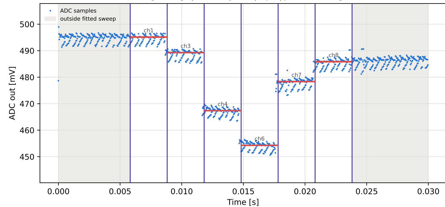
Tag4 &lt;- Tag15 | 935 MHz | run 0 | rep 1 | phase -145.95 deg
