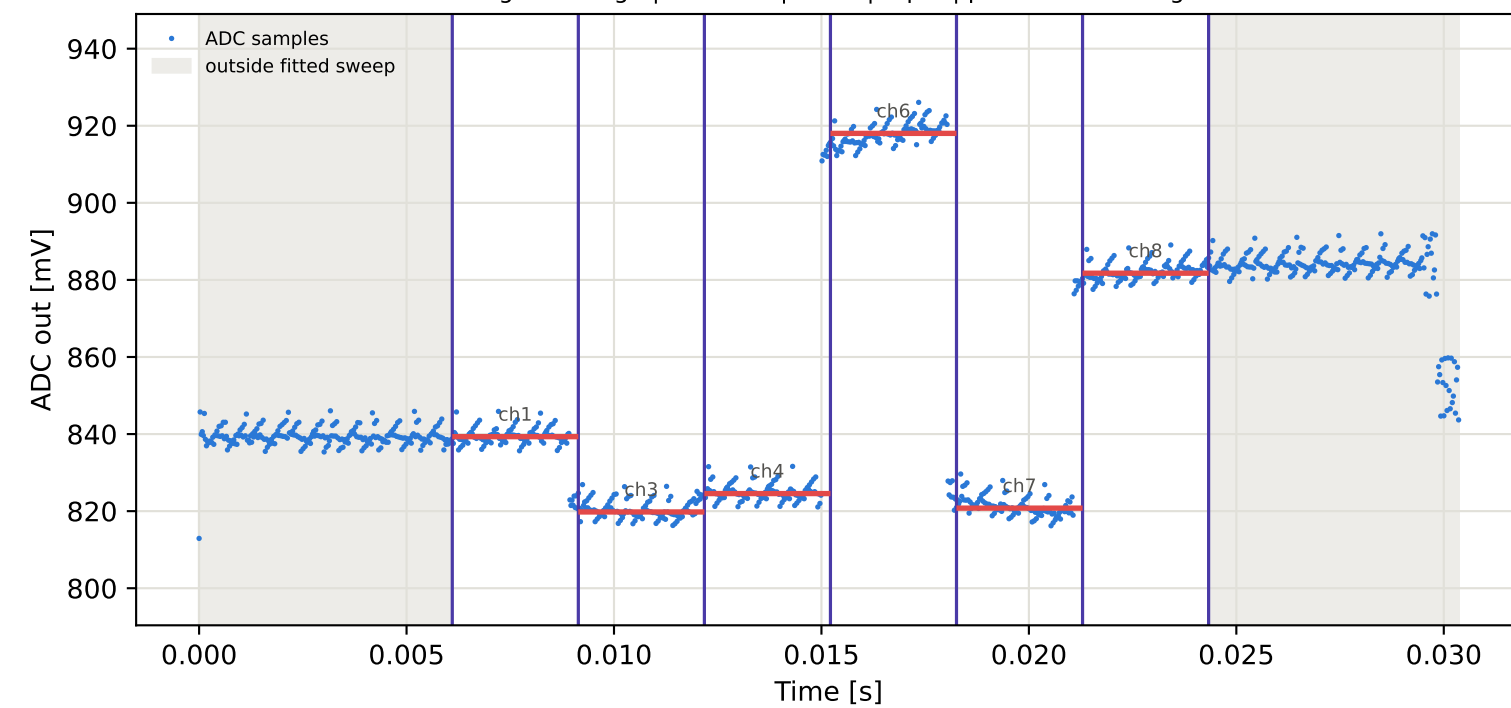
Tag10 &lt;- Tag8 | 925 MHz | run 0 | rep 1 | phase -145.17 deg
