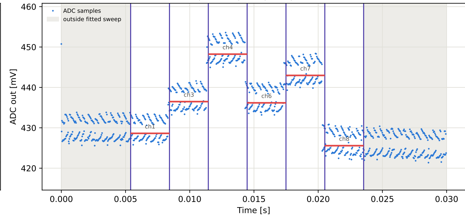
Tag6 &lt;- Tag5 | 935 MHz | run 0 | rep 1 | phase -95.72 deg
