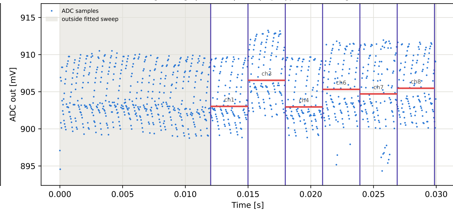
Tag7 &lt;- Tag4 | 995 MHz | run 0 | rep 1 | phase -55.43 deg
