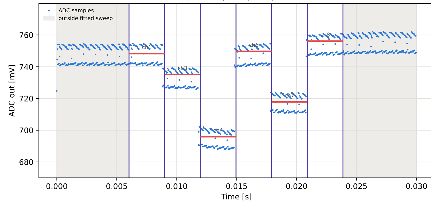
Tag9 &lt;- Tag5 | 985 MHz | run 0 | rep 1 | phase 118.92 deg
