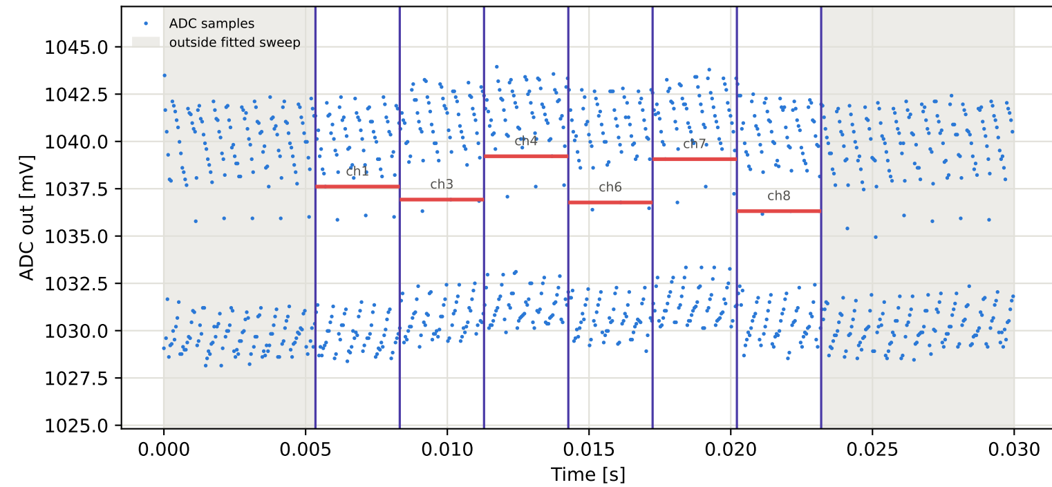
Tag7 &lt;- Tag15 | 855 MHz | run 0 | rep 1 | phase -101.39 deg
