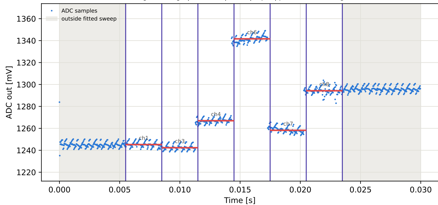
Tag16 &lt;- Tag7 | 905 MHz | run 0 | rep 1 | phase -163.98 deg
