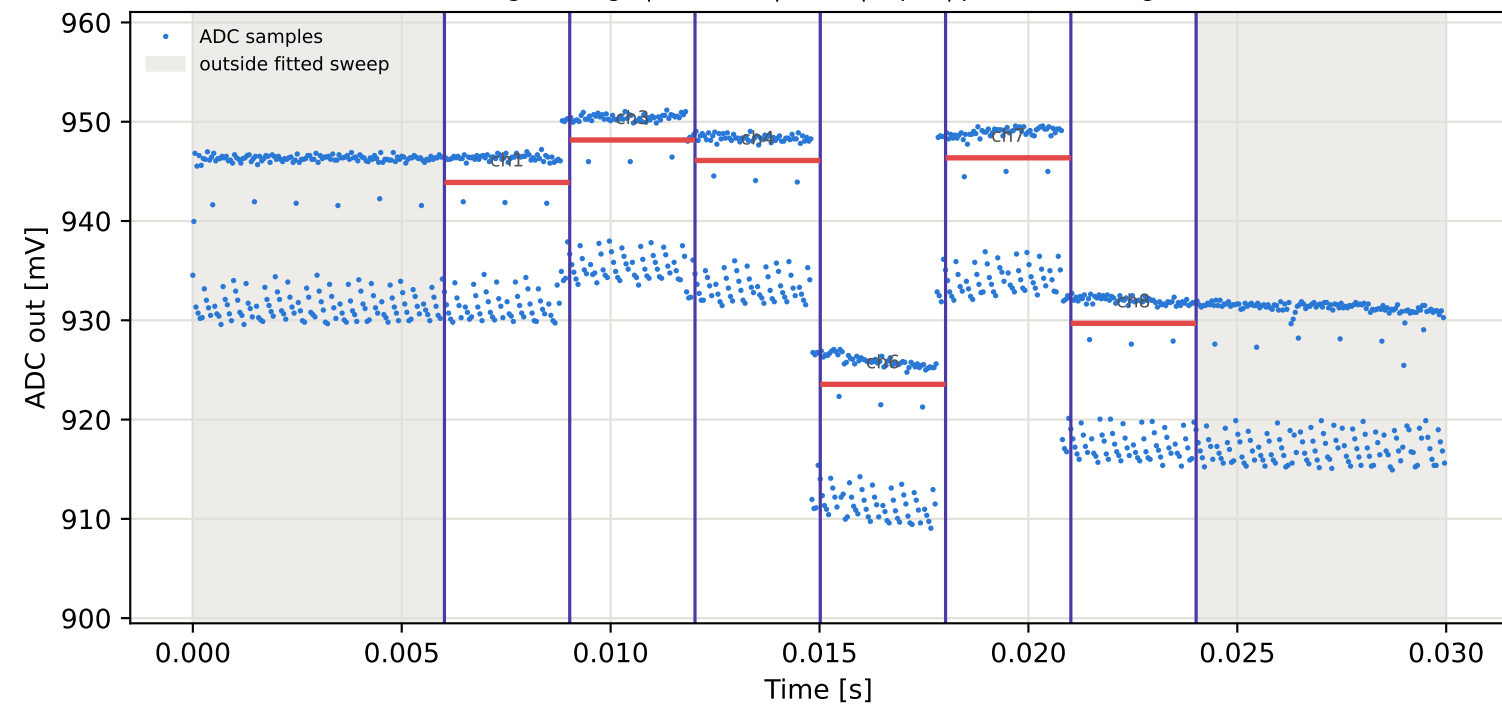
Tag3 &lt;- Tag15 | 915 MHz | run 0 | rep 1 | phase 13.91 deg
