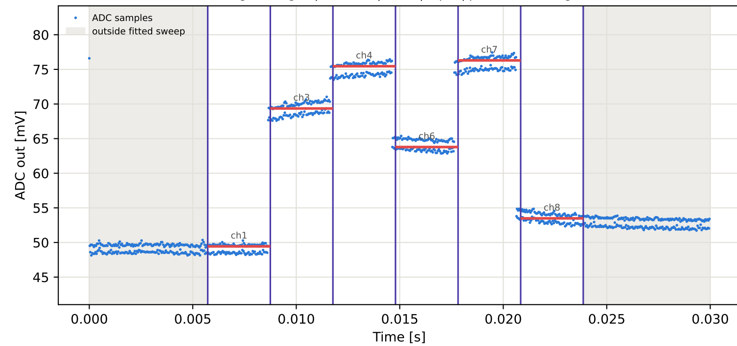
Tag1 &lt;- Tag16 | 845 MHz | run 0 | rep 1 | phase -87.78 deg
