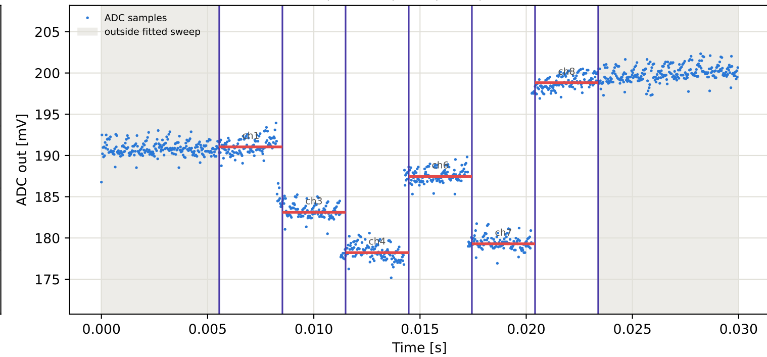
Tag2 &lt;- Tag8 | 905 MHz | run 0 | rep 1 | phase 105.62 deg
