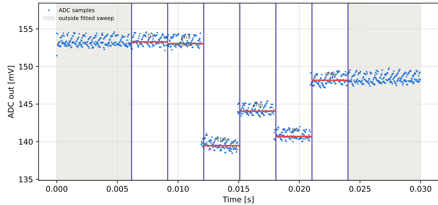
Tag5 &lt;- Tag4 | 805 MHz | run 0 | rep 1 | phase 74.51 deg
