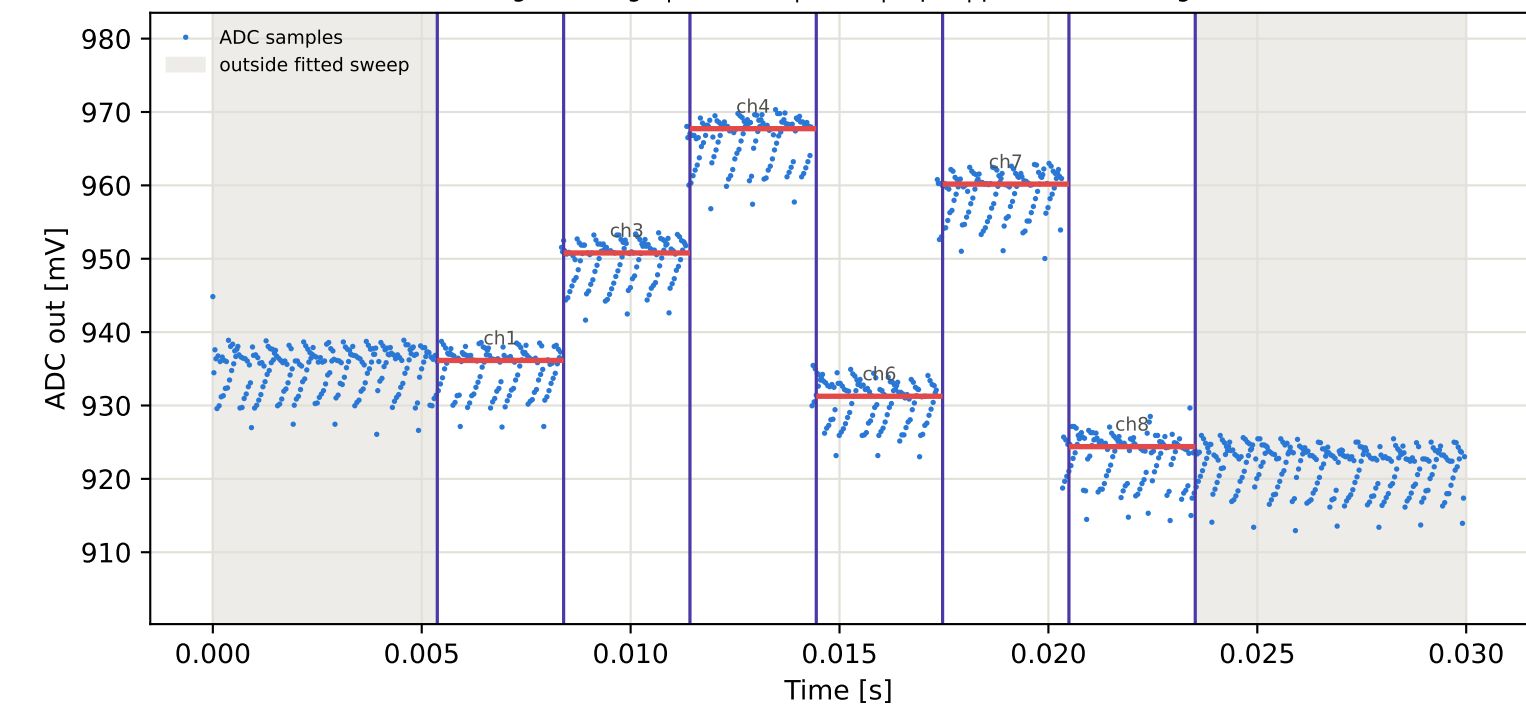
Tag10 &lt;- Tag5 | 935 MHz | run 0 | rep 1 | phase -66.39 deg
