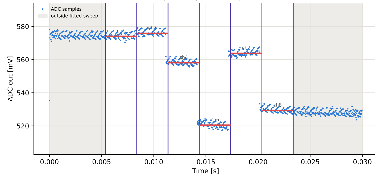
Tag5 &lt;- Tag16 | 875 MHz | run 0 | rep 1 | phase -131.91 deg
