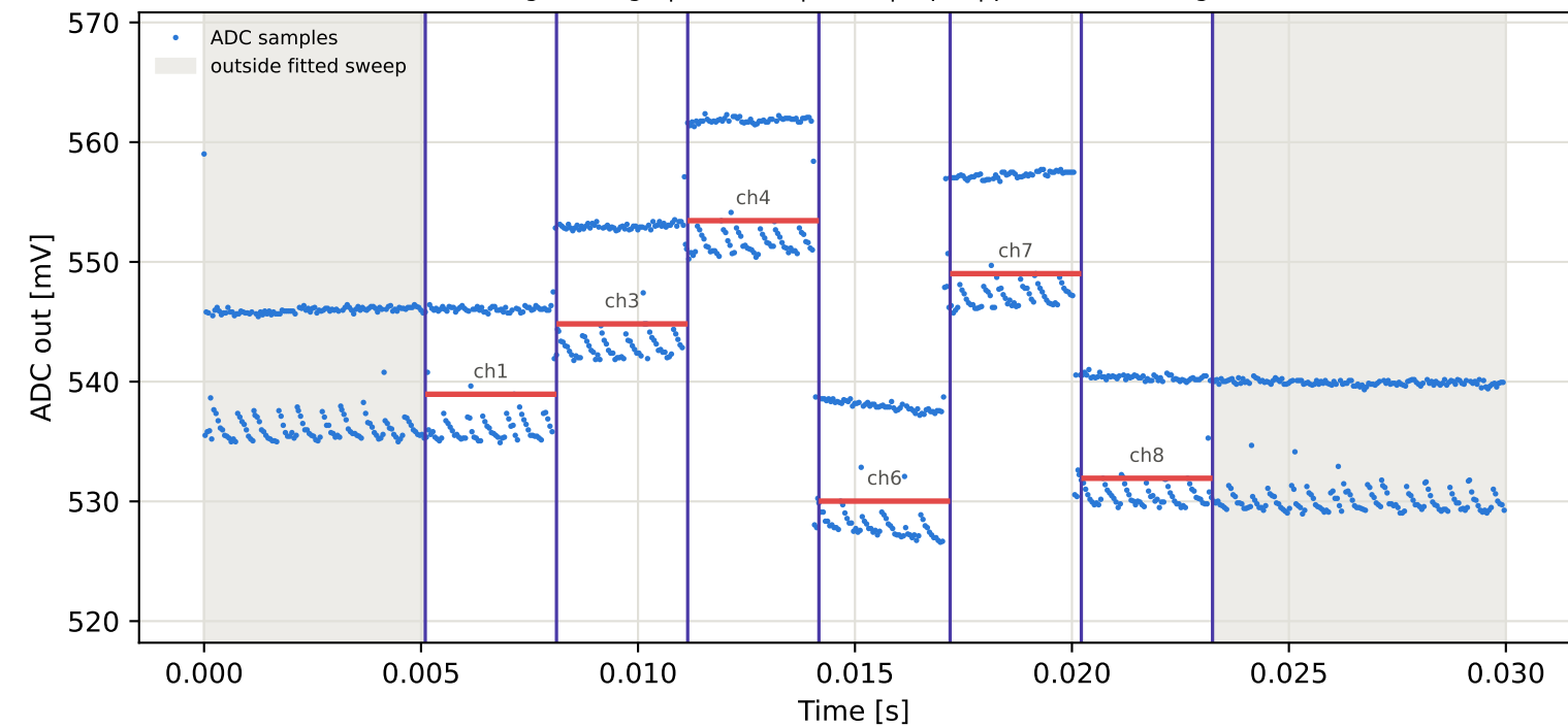
Tag9 &lt;- Tag6 | 975 MHz | run 0 | rep 1 | phase 117.65 deg
