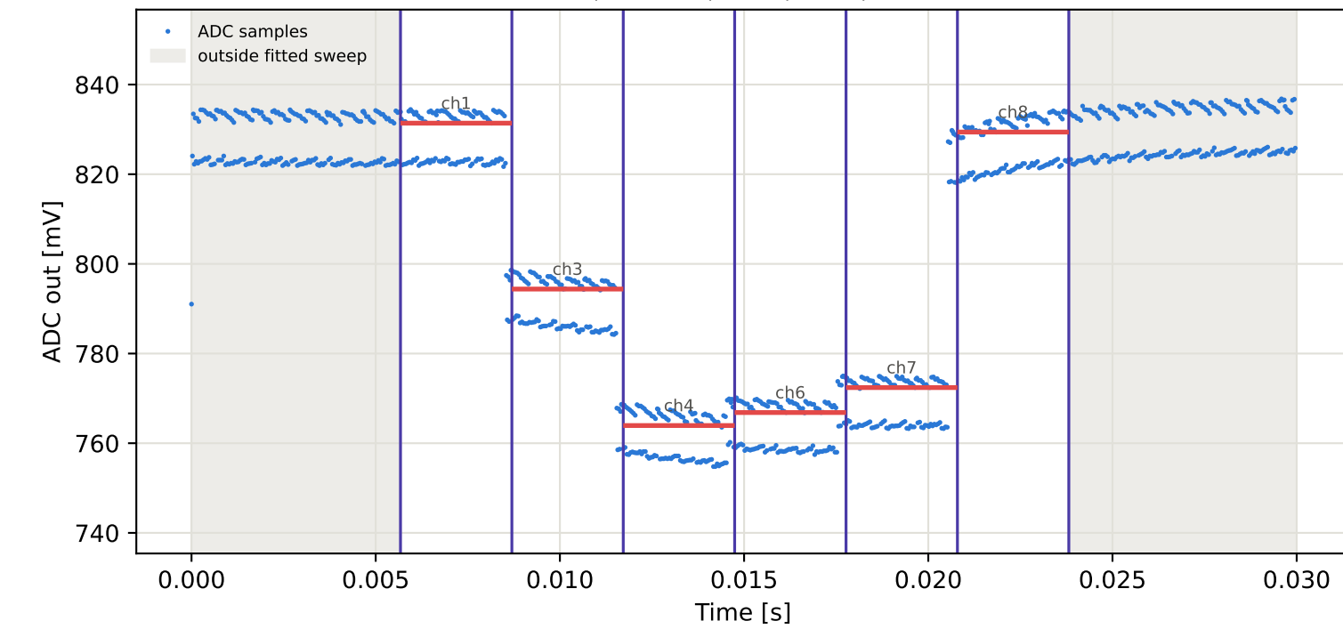
Tag9 &lt;- Tag16 | 895 MHz | run 0 | rep 1 | phase 70.88 deg
