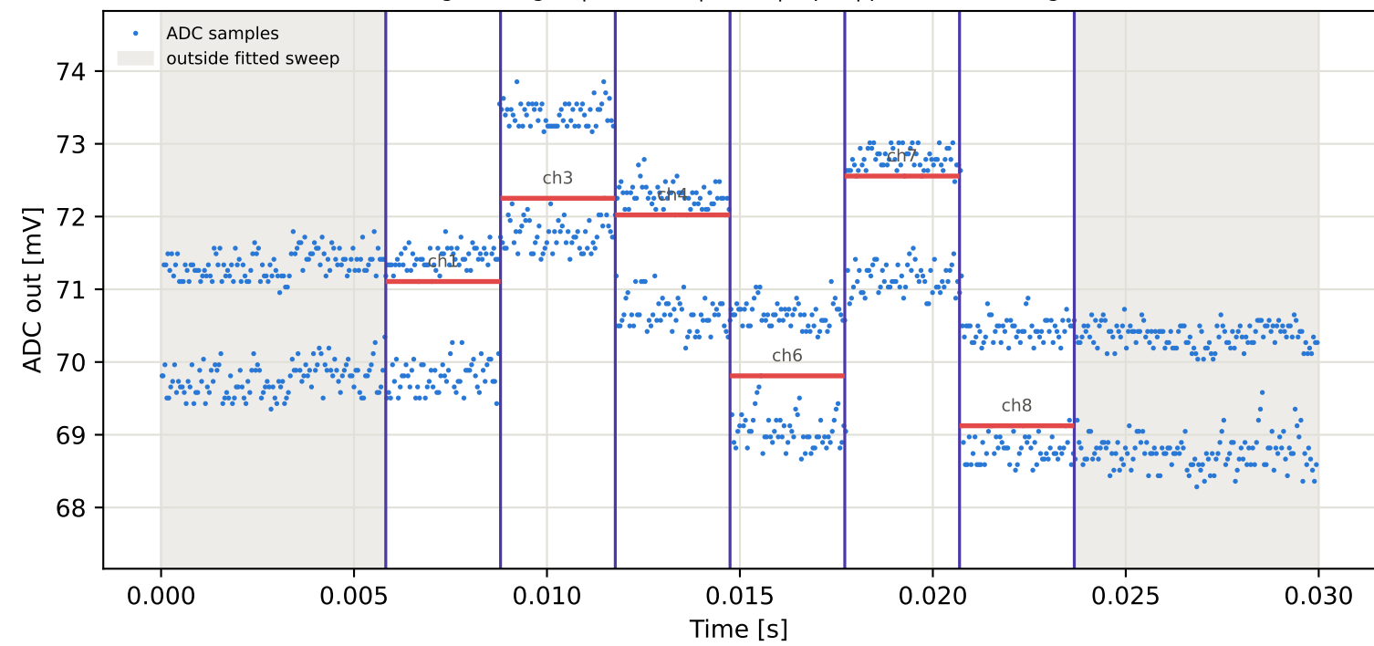
Tag1 &lt;- Tag2 | 845 MHz | run 0 | rep 1 | phase 34.04 deg
