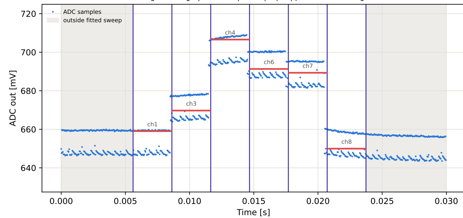
Tag2 &lt;- Tag1 | 925 MHz | run 0 | rep 1 | phase 65.08 deg
