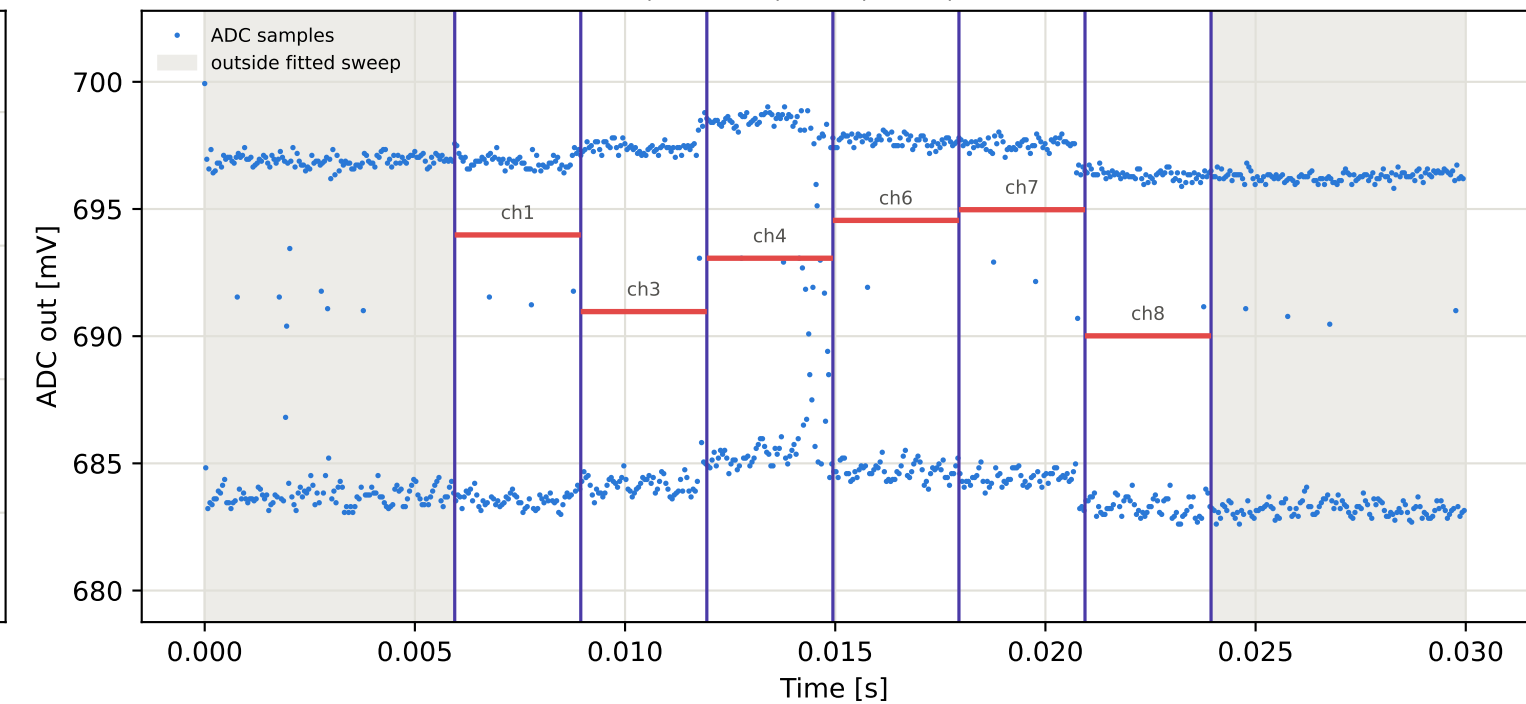
Tag9 &lt;- Tag2 | 955 MHz | run 0 | rep 1 | phase -123.63 deg
