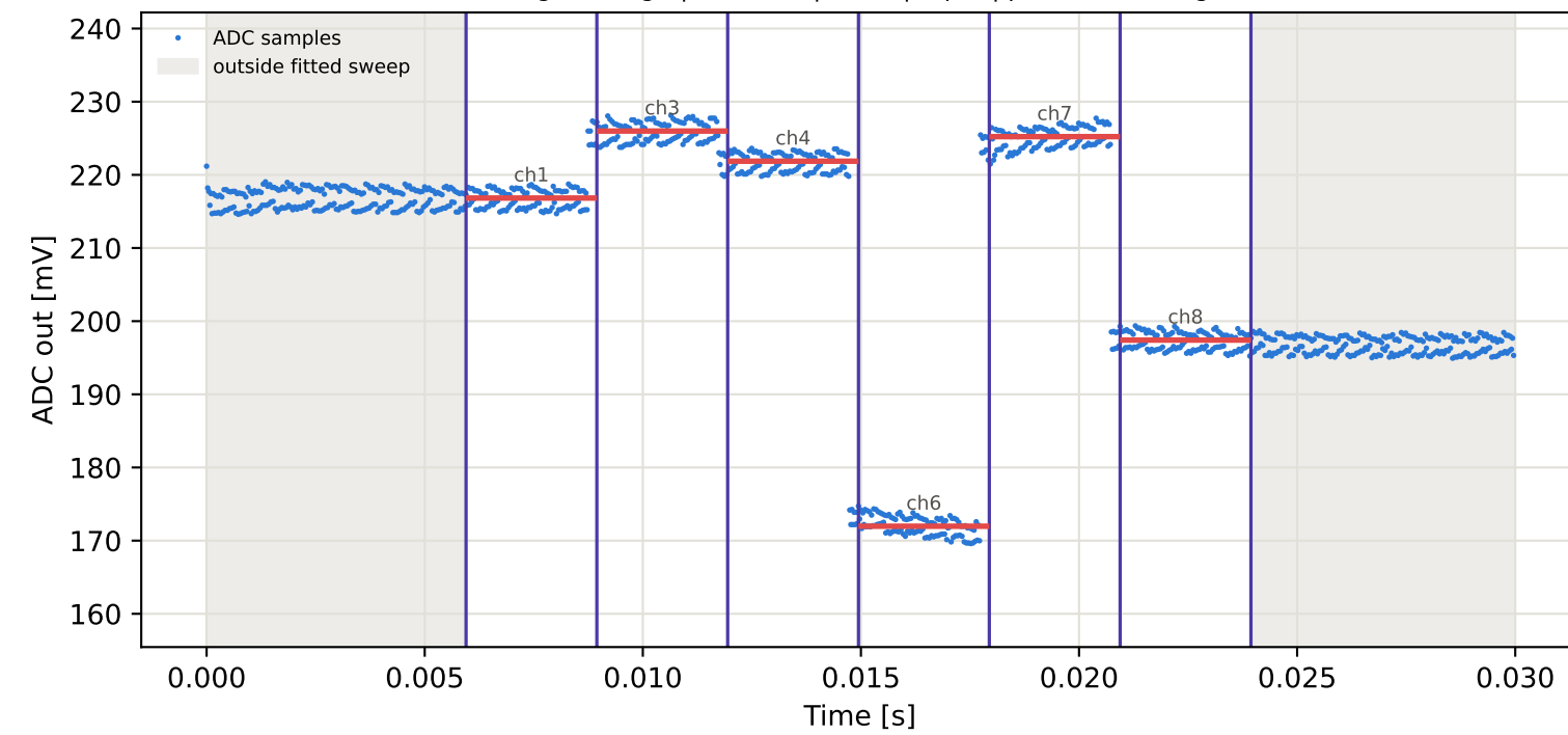
Tag4 &lt;- Tag7 | 945 MHz | run 0 | rep 1 | phase 106.13 deg
