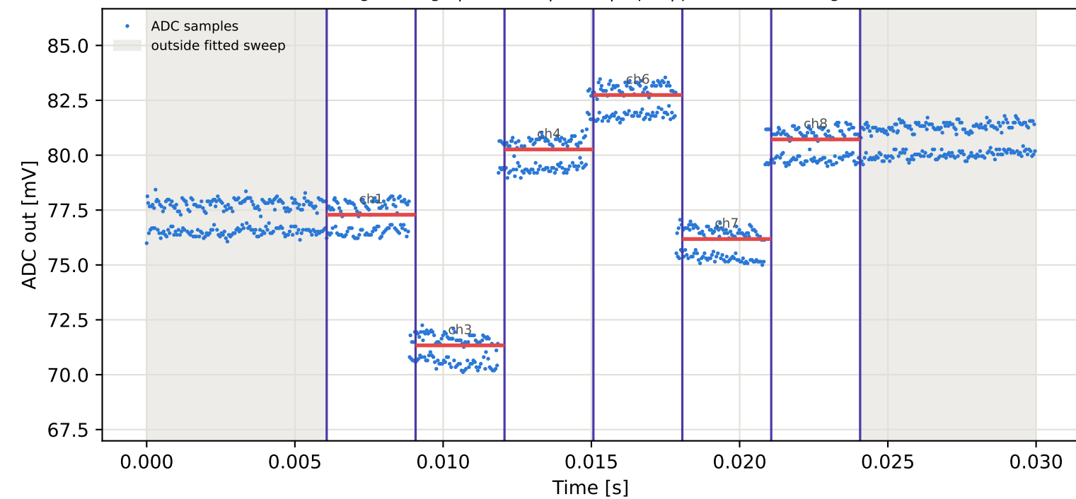
Tag7 &lt;- Tag10 | 775 MHz | run 0 | rep 1 | phase 117.65 deg
