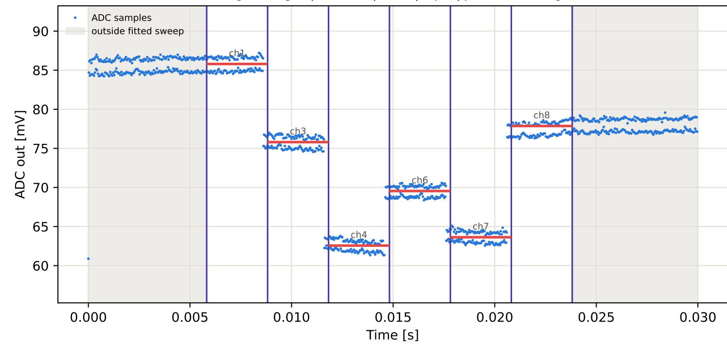
Tag4 &lt;- Tag16 | 825 MHz | run 0 | rep 1 | phase -127.82 deg
