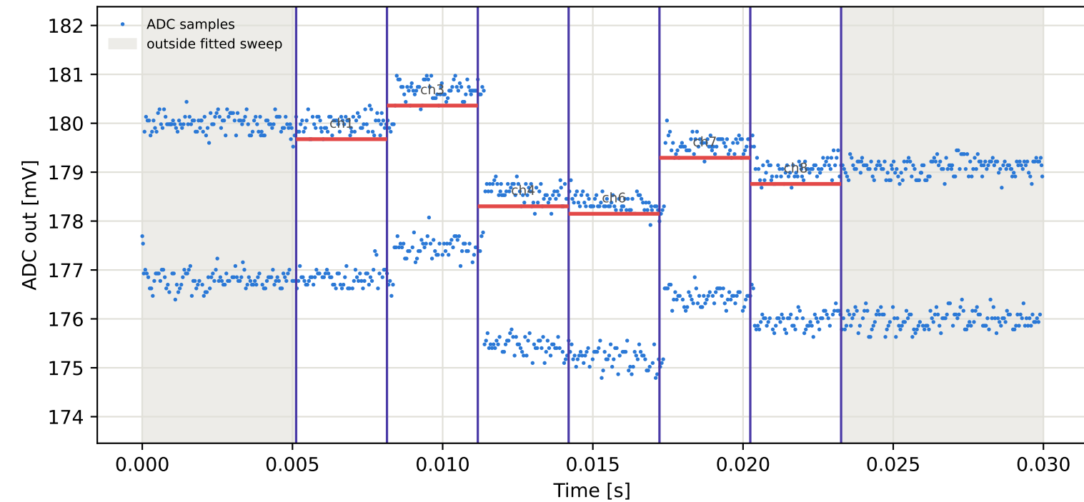
Tag8 &lt;- Tag15 | 795 MHz | run 0 | rep 1 | phase -81.72 deg
