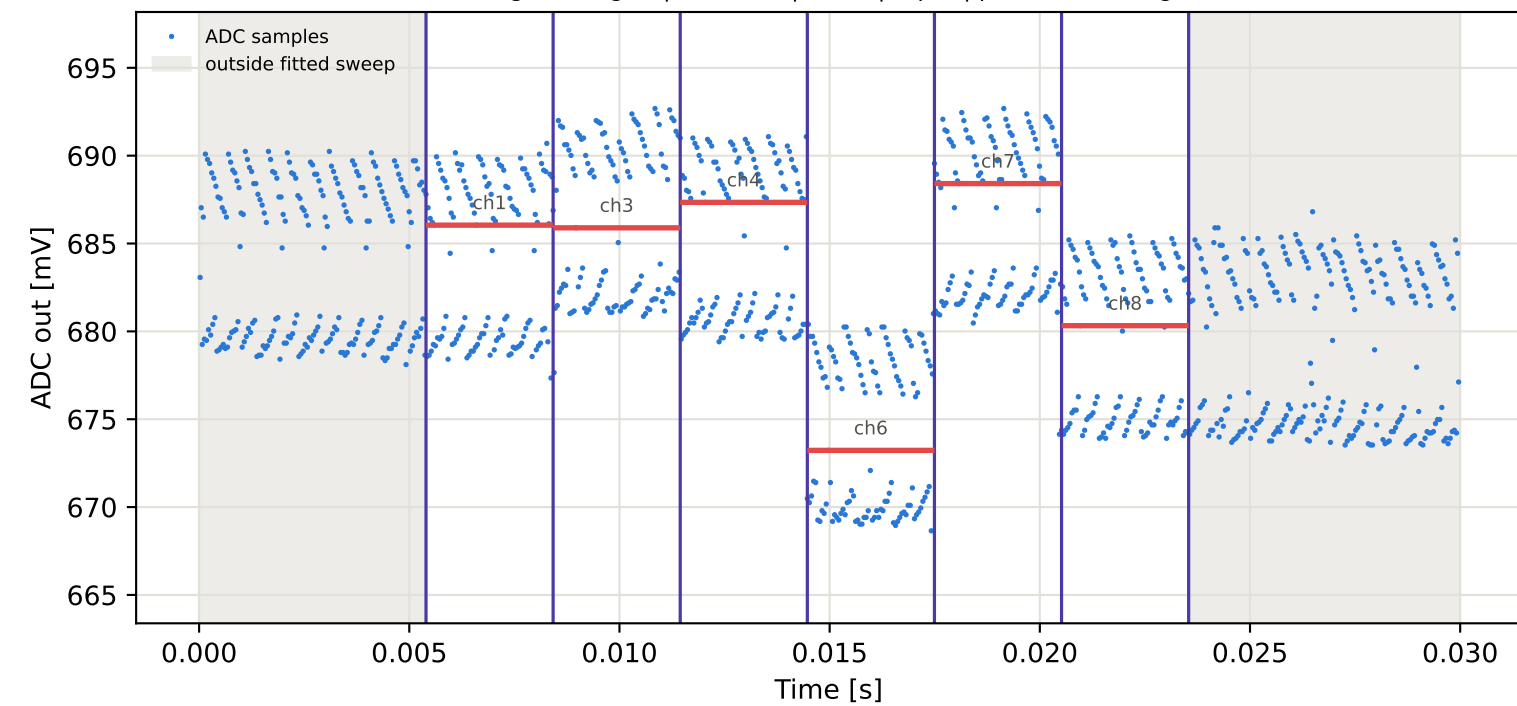
Tag6 &lt;- Tag2 | 945 MHz | run 0 | rep 1 | phase -14.34 deg
