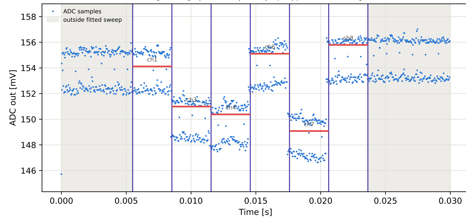
Tag3 &lt;- Tag8 | 795 MHz | run 0 | rep 1 | phase -52.10 deg
