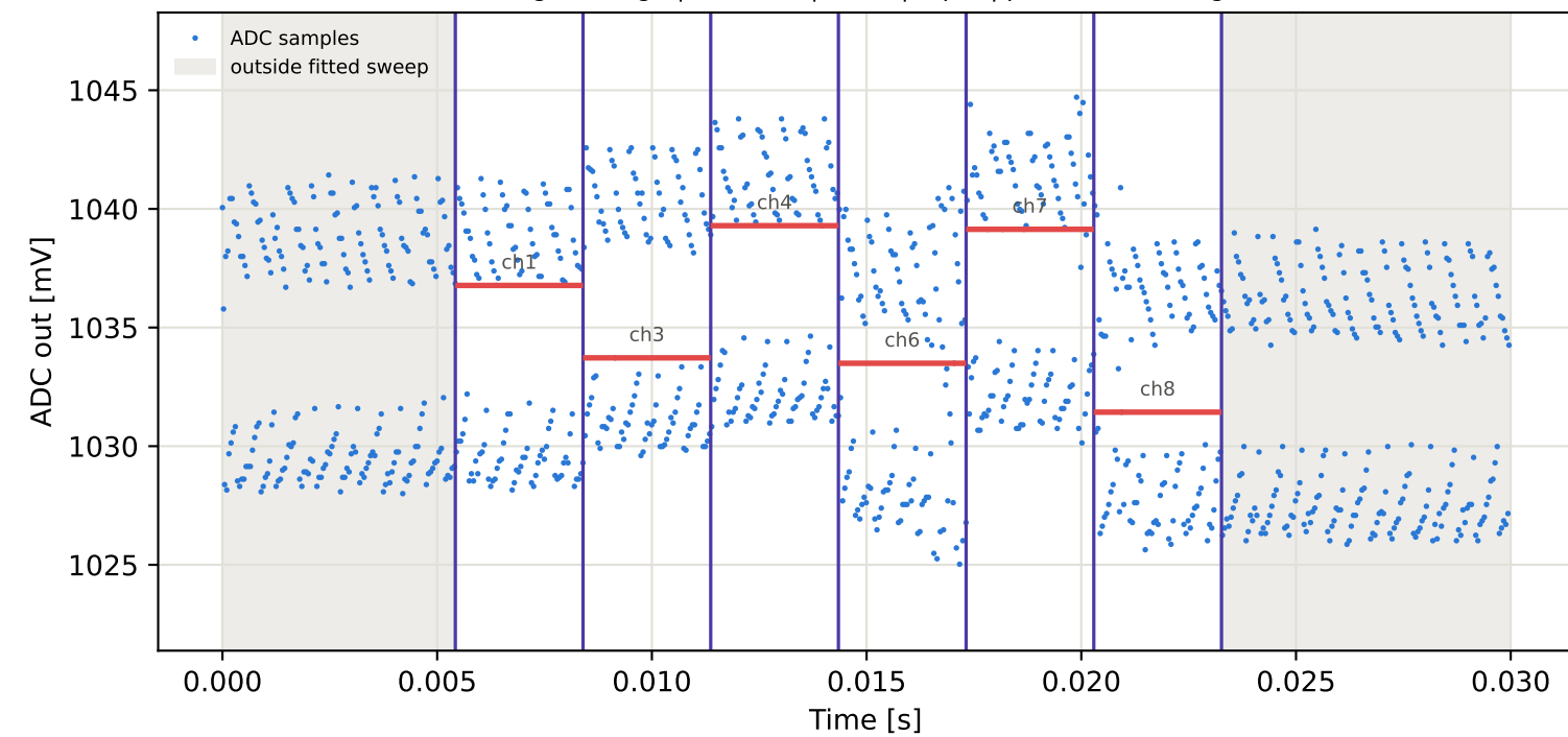
Tag7 &lt;- Tag4 | 855 MHz | run 0 | rep 1 | phase 135.72 deg
