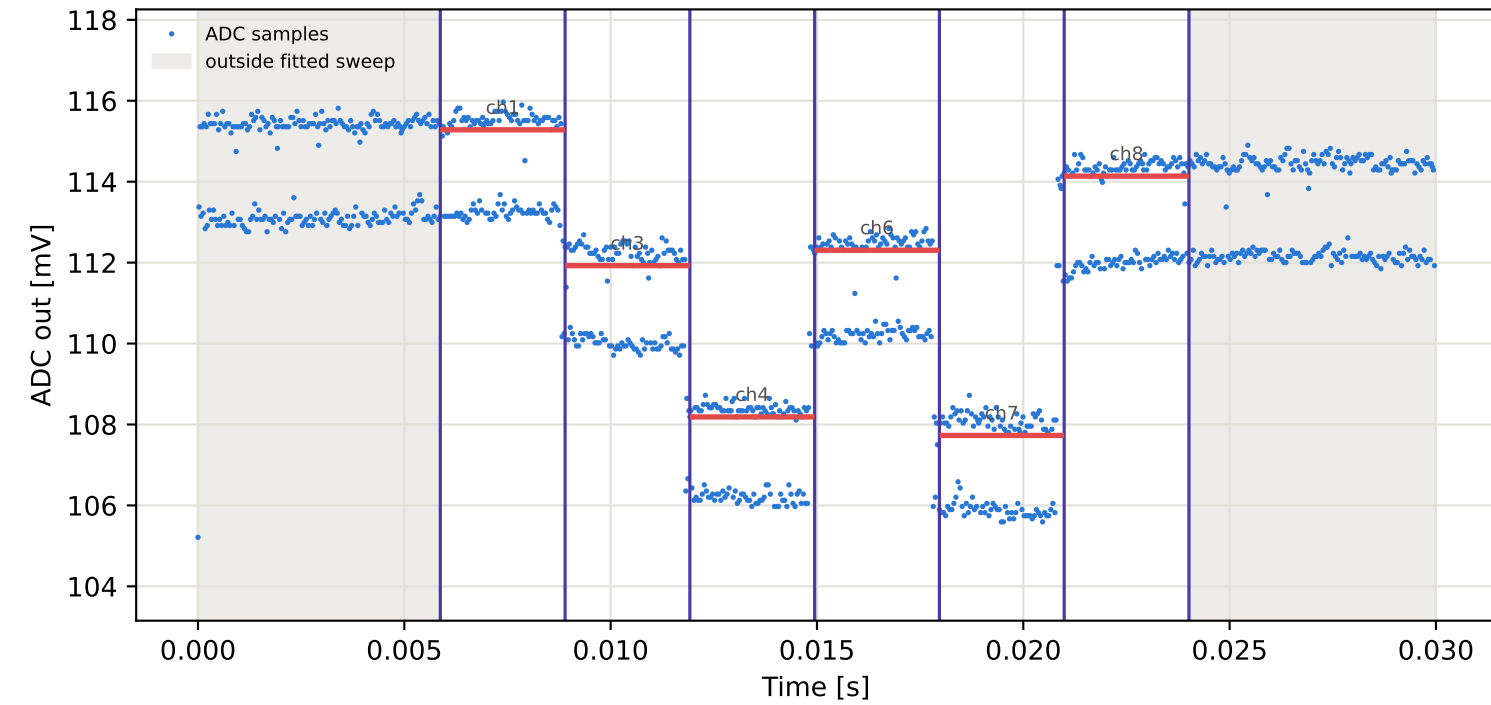
Tag5 &lt;- Tag1 | 805 MHz | run 0 | rep 1 | phase -147.10 deg
