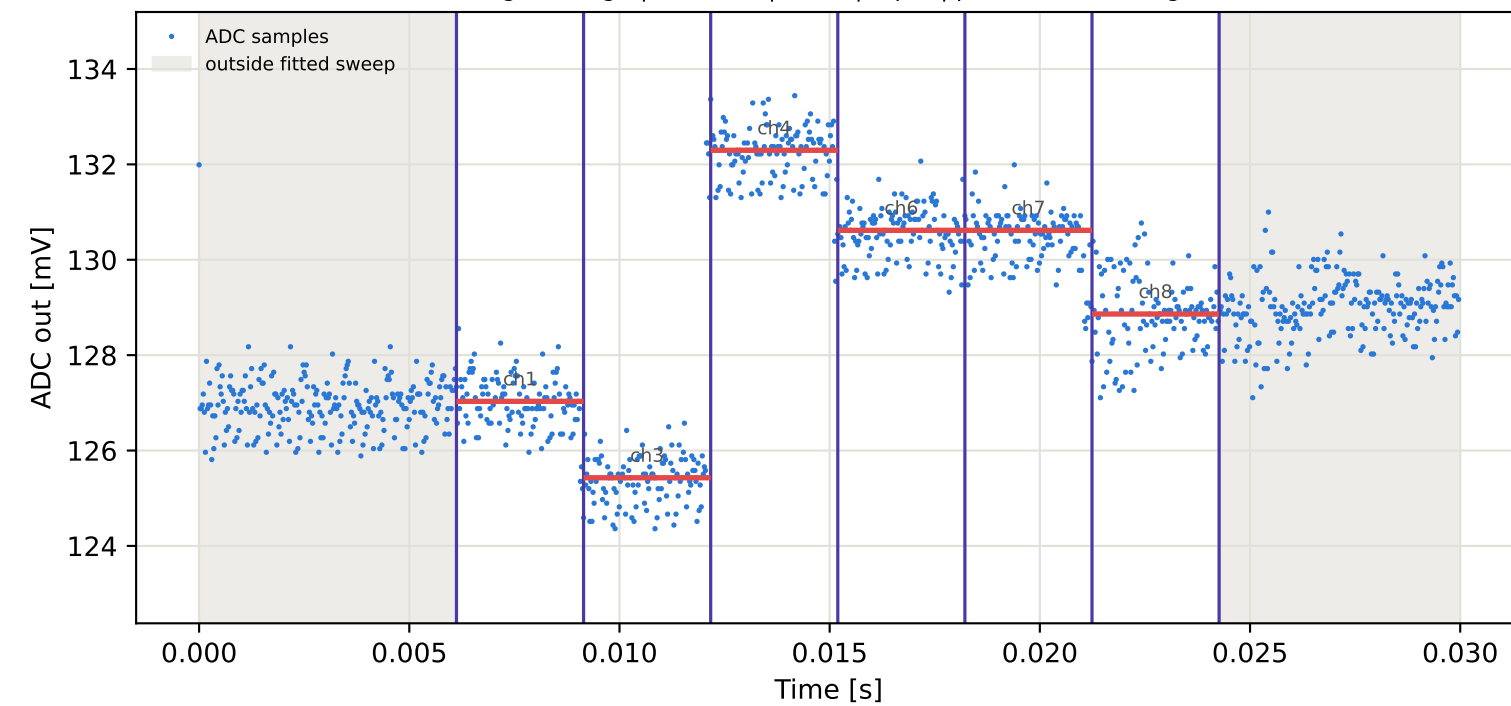
Tag3 &lt;- Tag6 | 785 MHz | run 0 | rep 1 | phase -102.22 deg
