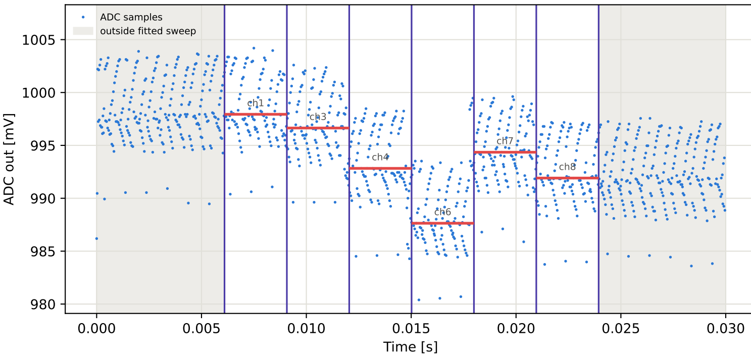
Tag8 &lt;- Tag15 | 895 MHz | run 0 | rep 1 | phase 54.58 deg
