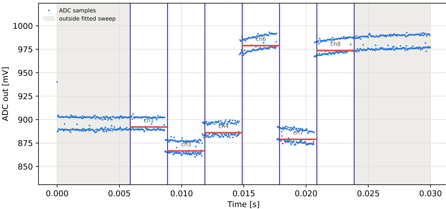
Tag5 &lt;- Tag3 | 885 MHz | run 0 | rep 1 | phase 175.70 deg
