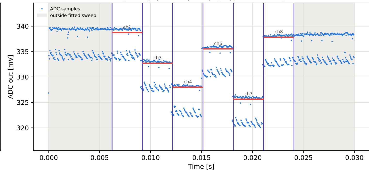
Tag8 &lt;- Tag5 | 805 MHz | run 0 | rep 1 | phase -167.66 deg
