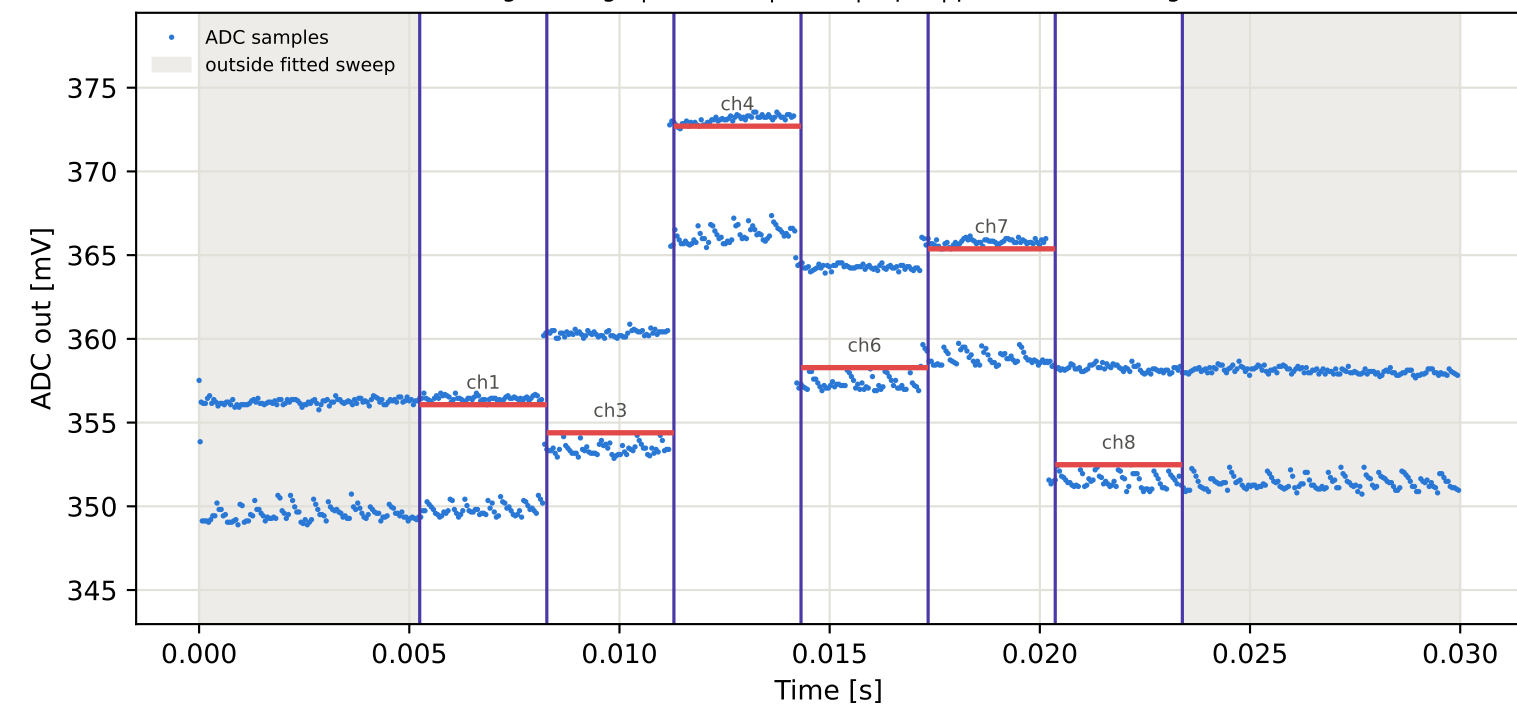
Tag6 &lt;- Tag1 | 985 MHz | run 0 | rep 1 | phase -105.10 deg
