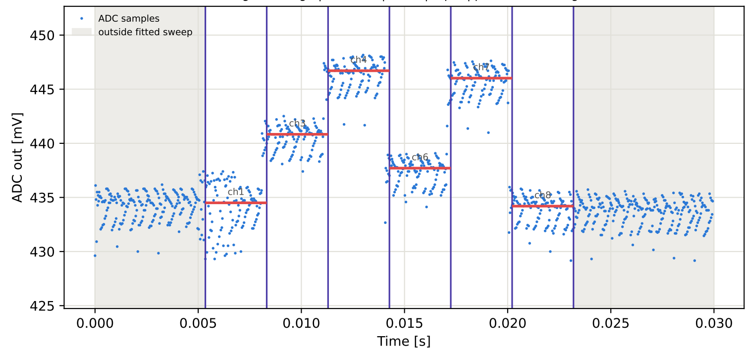
Tag16 &lt;- Tag7 | 845 MHz | run 0 | rep 1 | phase -74.39 deg
