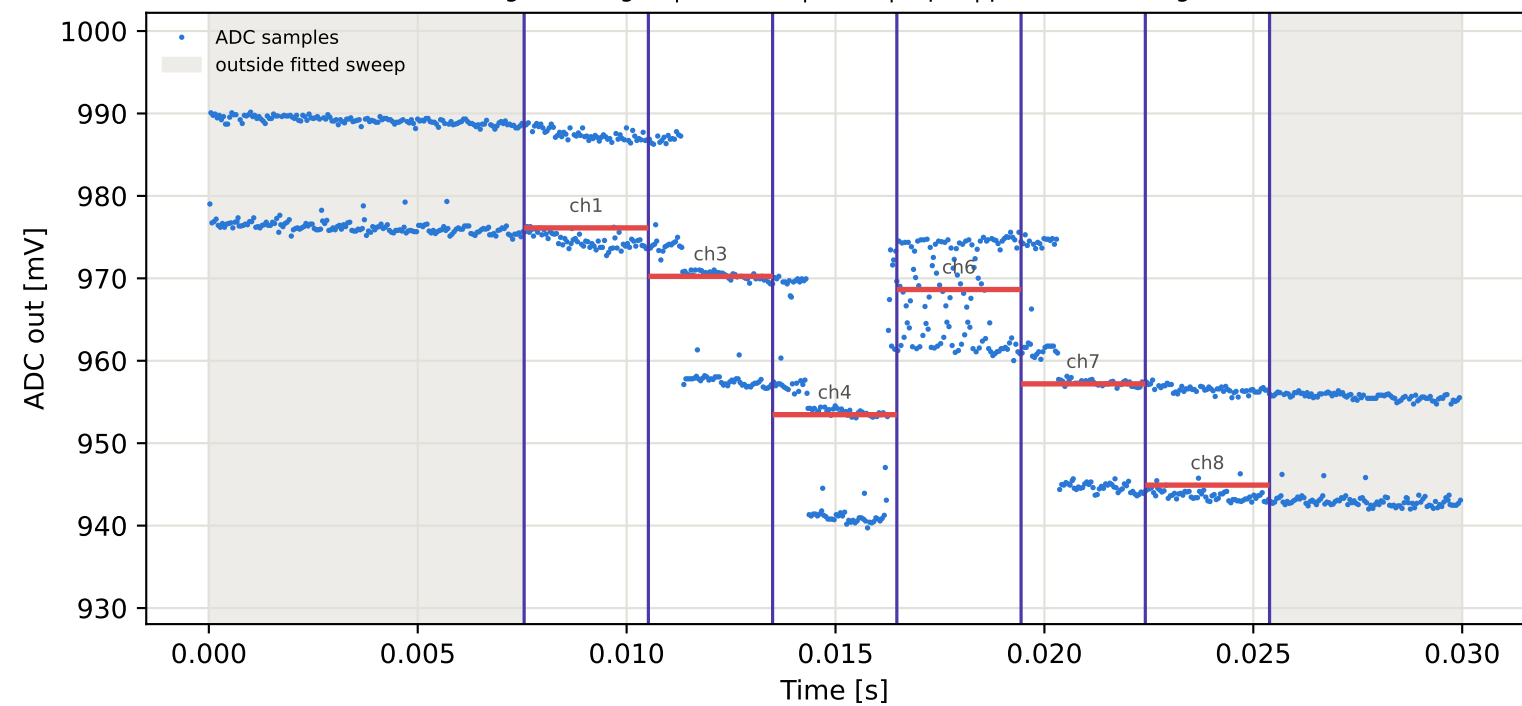
Tag16 &lt;- Tag15 | 875 MHz | run 0 | rep 1 | phase 67.60 deg
