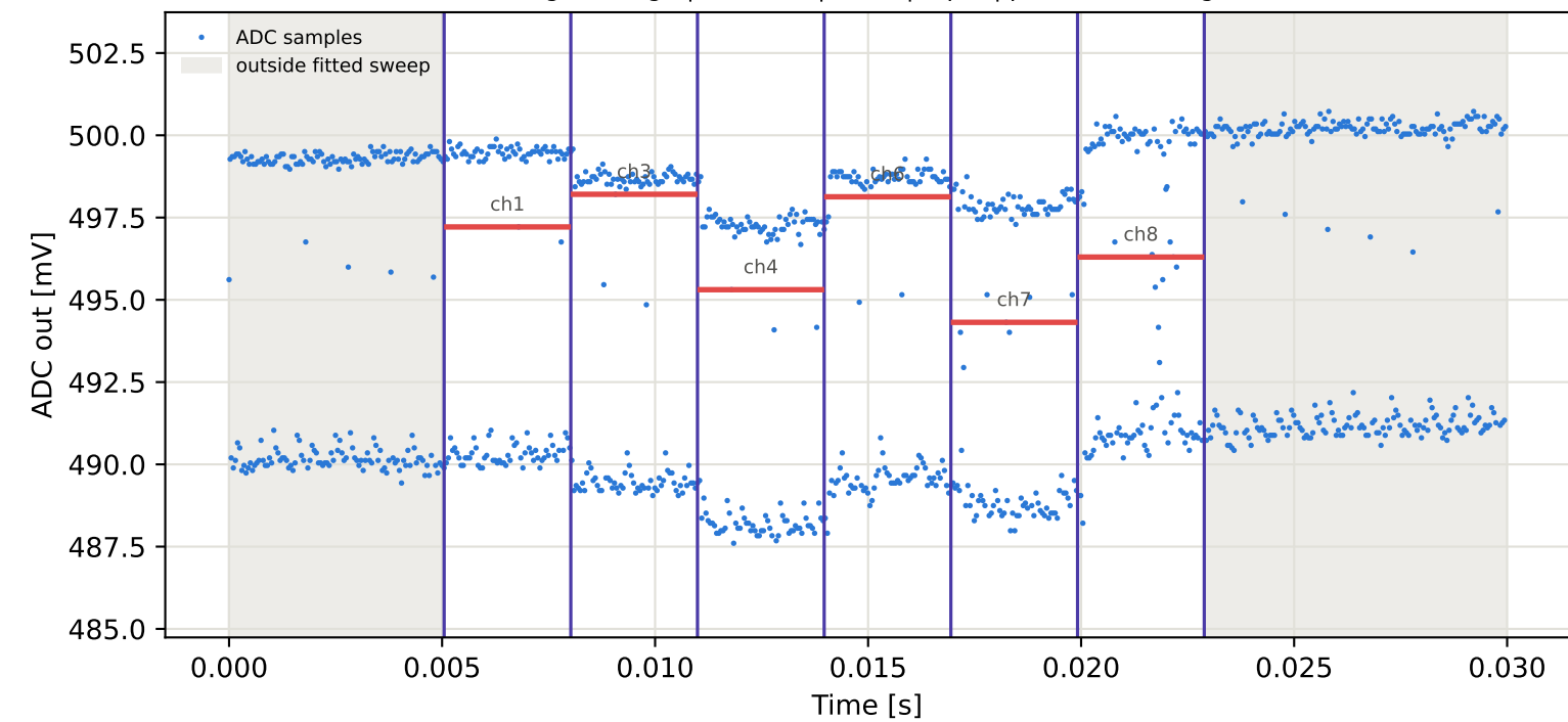
Tag8 &lt;- Tag4 | 985 MHz | run 0 | rep 1 | phase -29.55 deg
