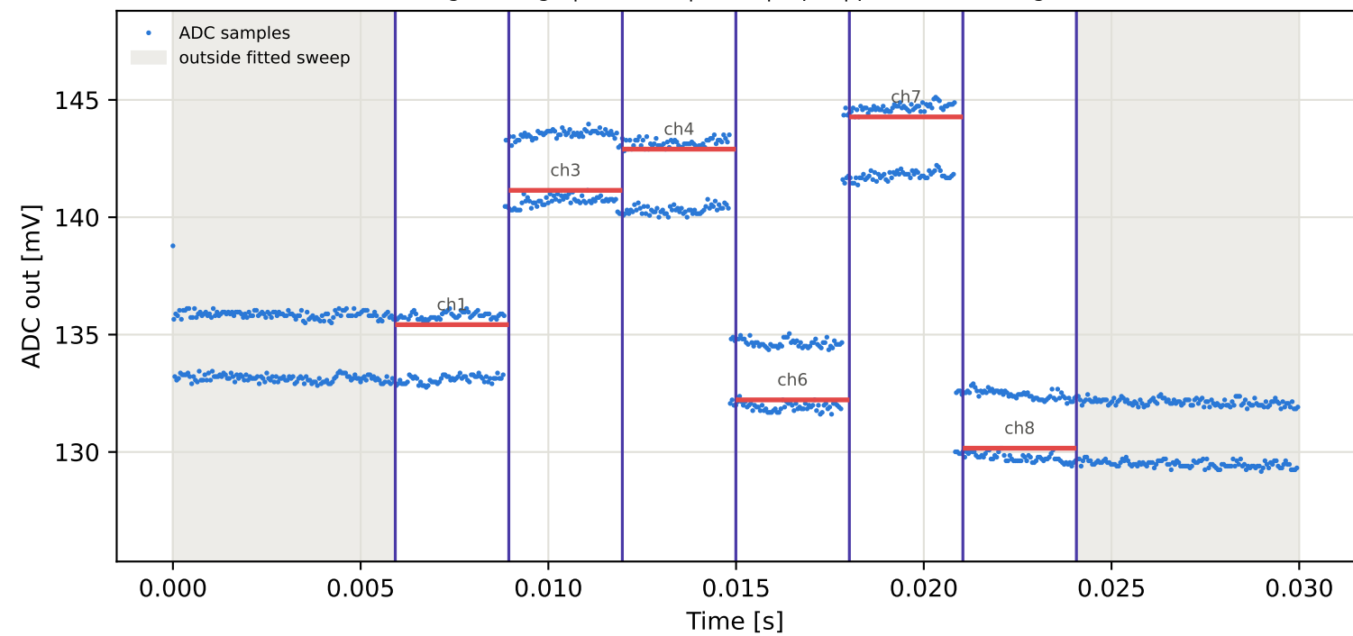
Tag5 &lt;- Tag9 | 805 MHz | run 0 | rep 1 | phase -102.88 deg
