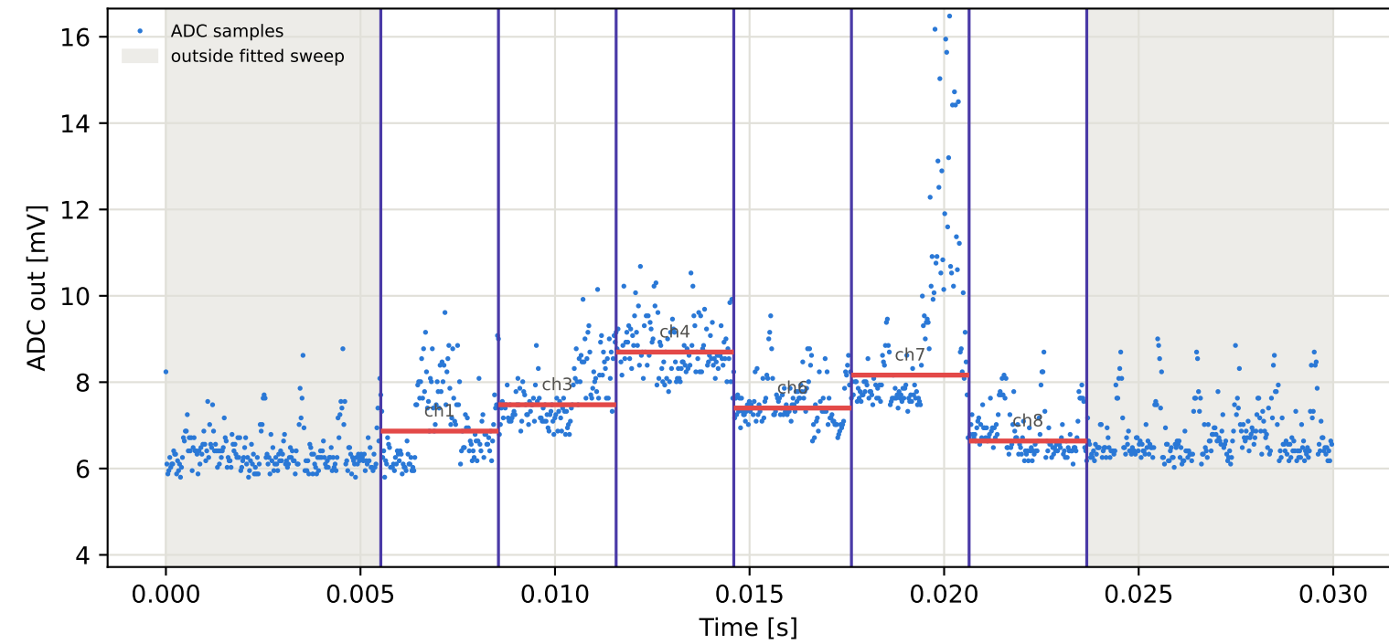
Tag2 &lt;- Tag8 | 785 MHz | run 0 | rep 1 | phase 46.15 deg
