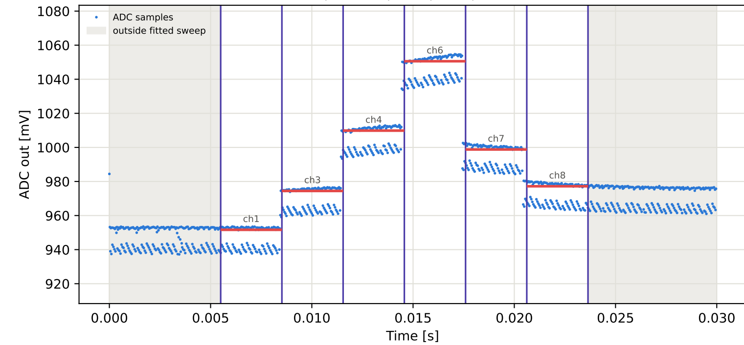
Tag3 &lt;- Tag16 | 905 MHz | run 0 | rep 1 | phase -136.87 deg
