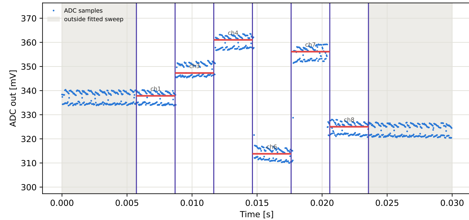
Tag15 &lt;- Tag5 | 985 MHz | run 0 | rep 1 | phase -48.79 deg
