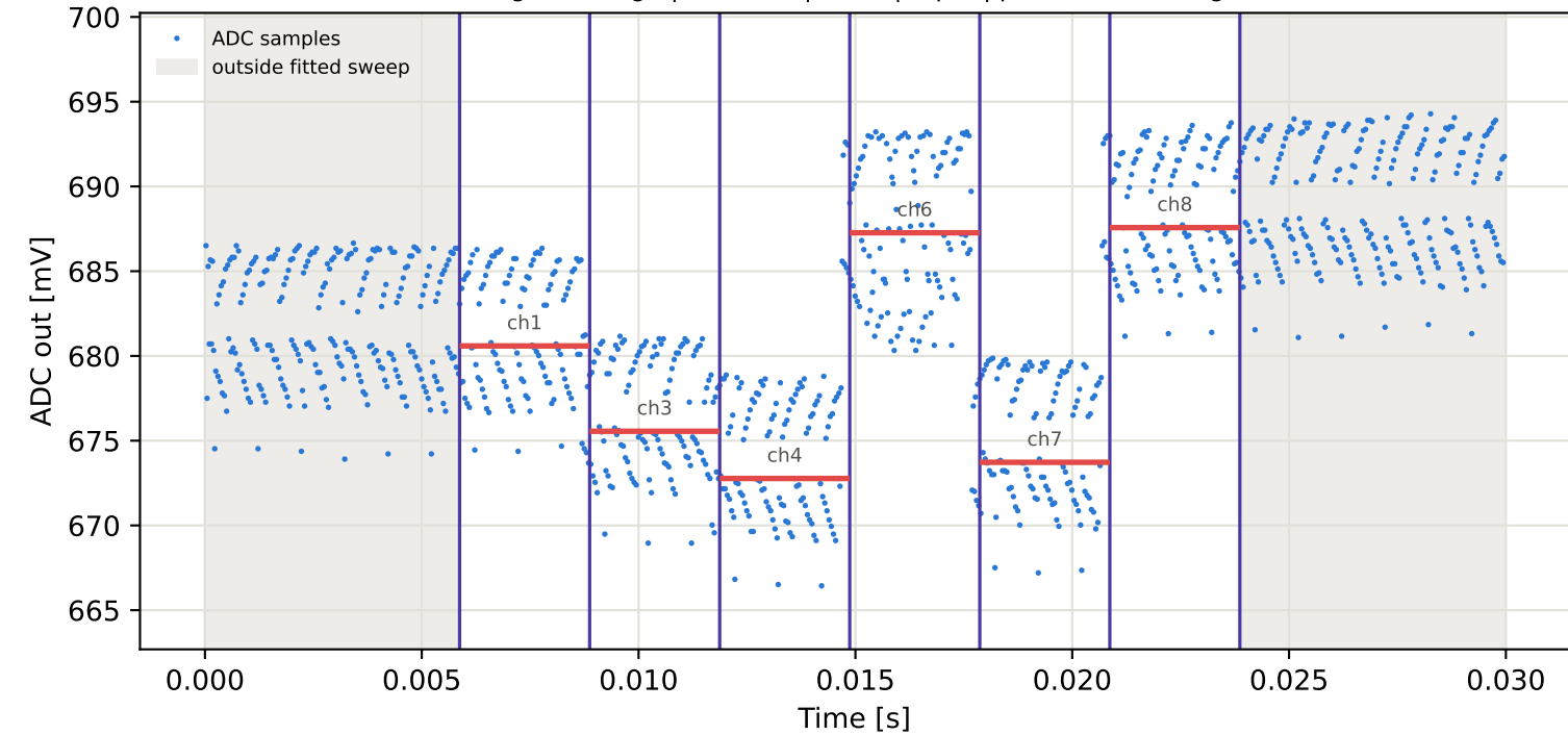
Tag15 &lt;- Tag6 | 915 MHz | run 0 | rep 1 | phase -28.48 deg
