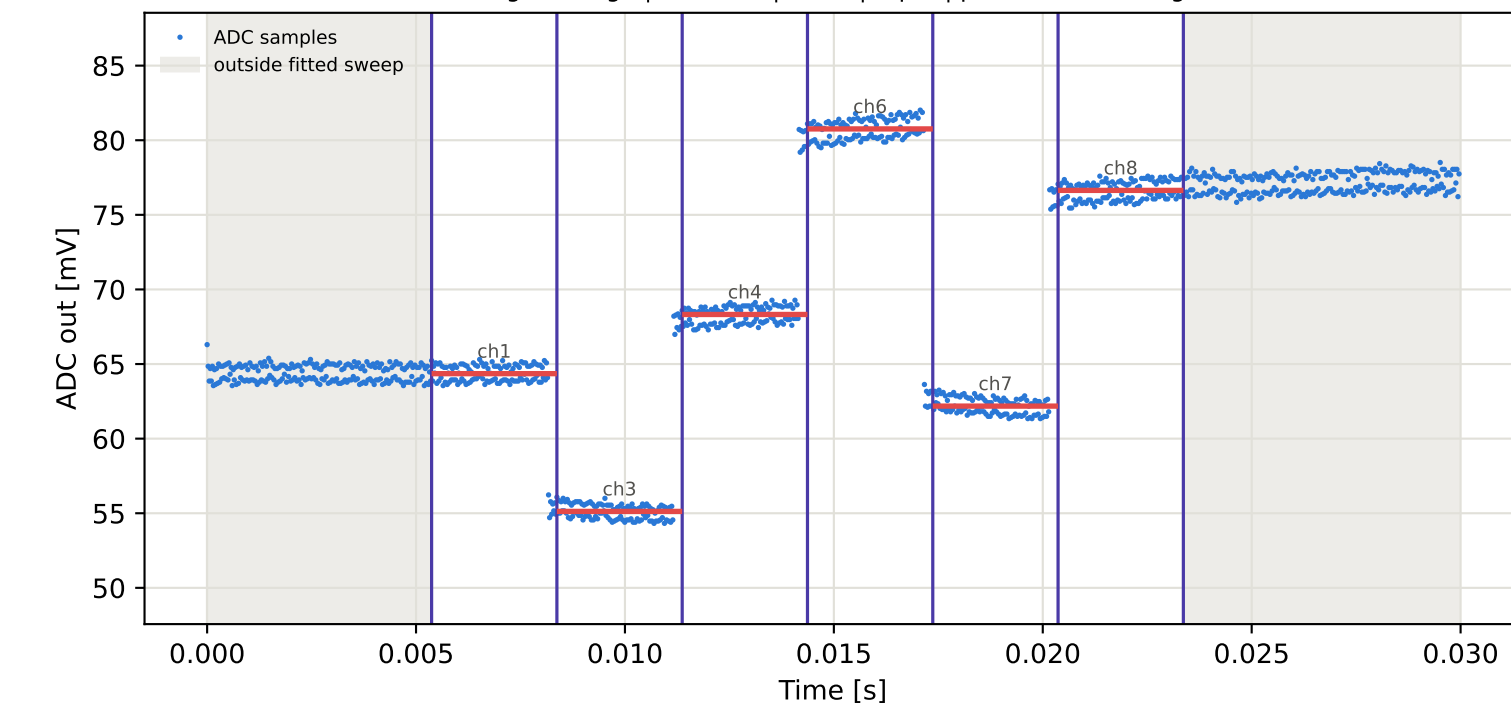
Tag1 &lt;- Tag9 | 845 MHz | run 0 | rep 1 | phase -162.74 deg
