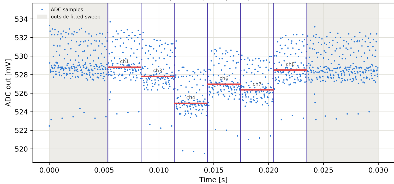
Tag1 &lt;- Tag2 | 985 MHz | run 0 | rep 1 | phase 120.11 deg
