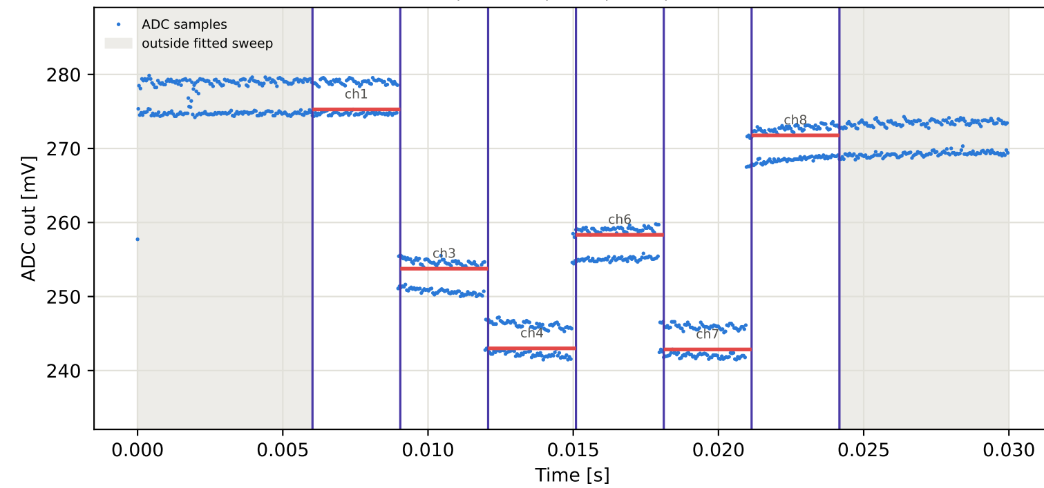
Tag15 &lt;- Tag5 | 855 MHz | run 0 | rep 1 | phase 97.26 deg
