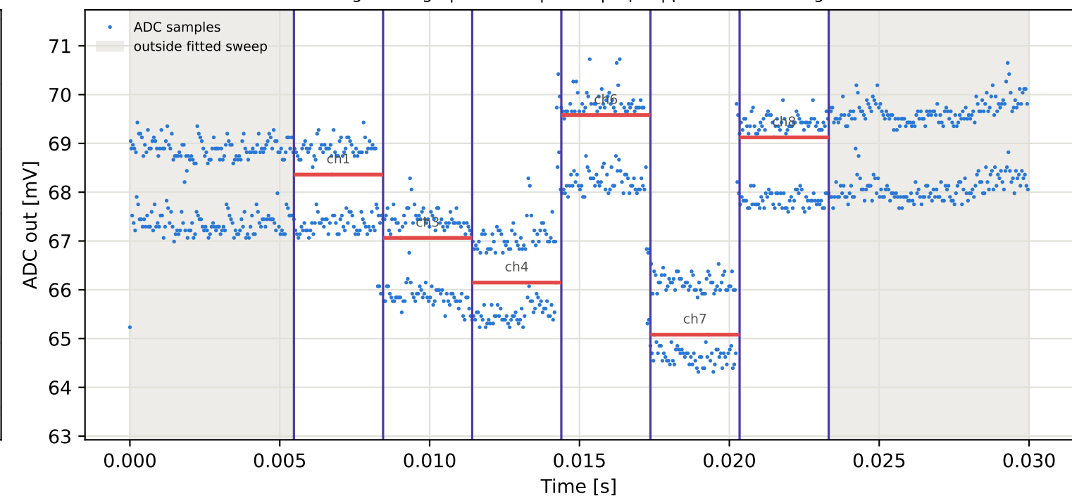
Tag3 &lt;- Tag15 | 775 MHz | run 0 | rep 1 | phase 179.79 deg
