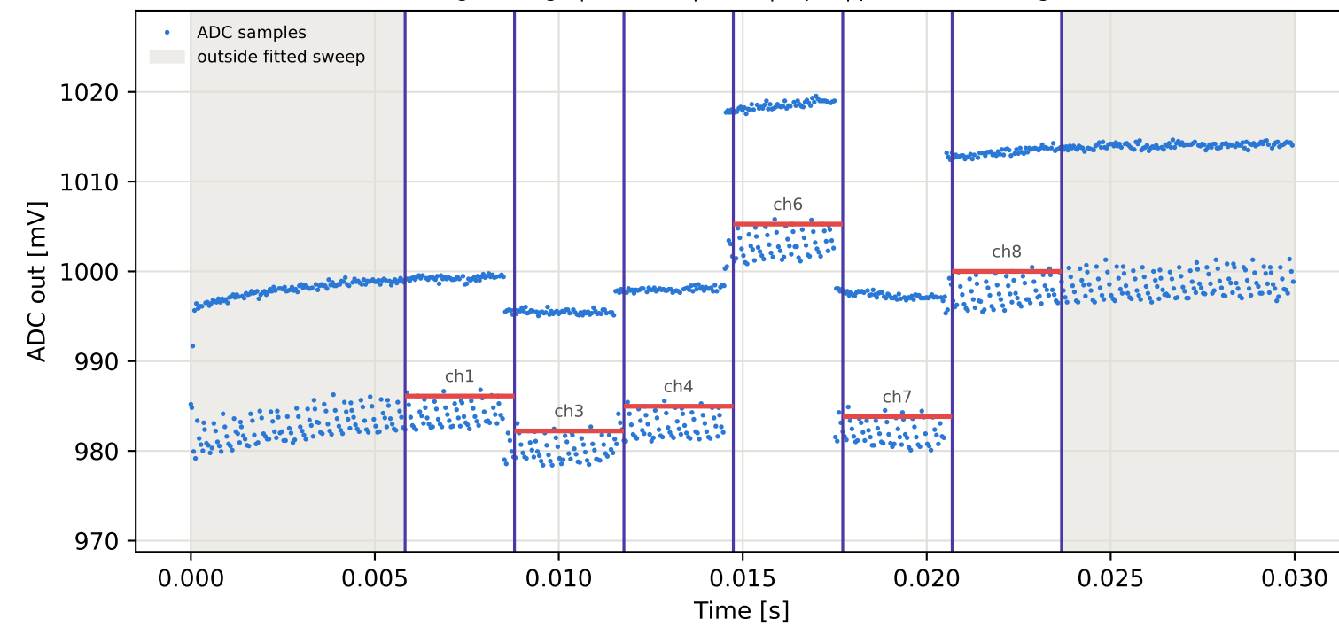
Tag3 &lt;- Tag6 | 905 MHz | run 0 | rep 1 | phase 62.61 deg
