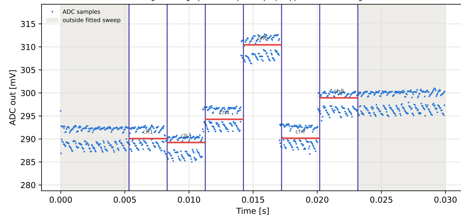
Tag15 &lt;- Tag9 | 945 MHz | run 0 | rep 1 | phase 57.78 deg
