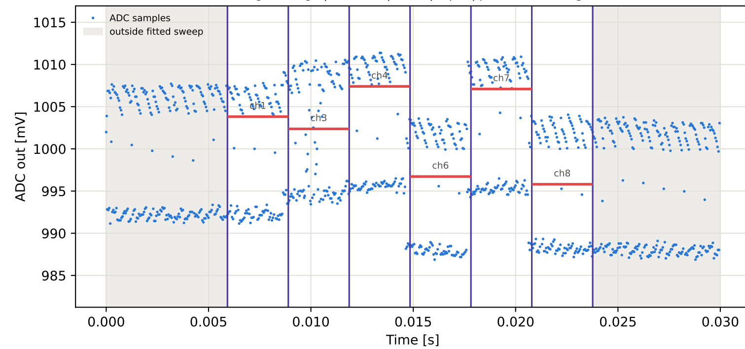
Tag8 &lt;- Tag4 | 905 MHz | run 0 | rep 1 | phase 95.17 deg
