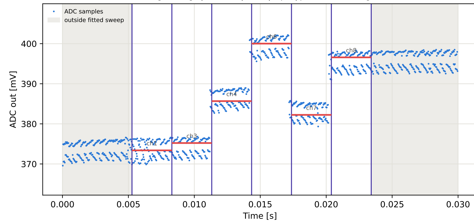
Tag5 &lt;- Tag8 | 865 MHz | run 0 | rep 1 | phase -97.28 deg
