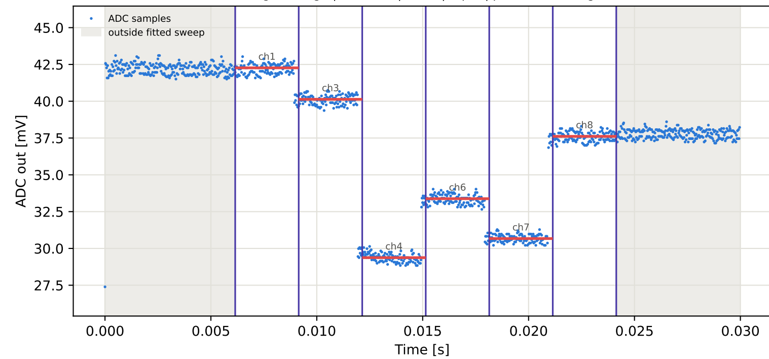
Tag6 &lt;- Tag9 | 785 MHz | run 0 | rep 1 | phase -131.48 deg
