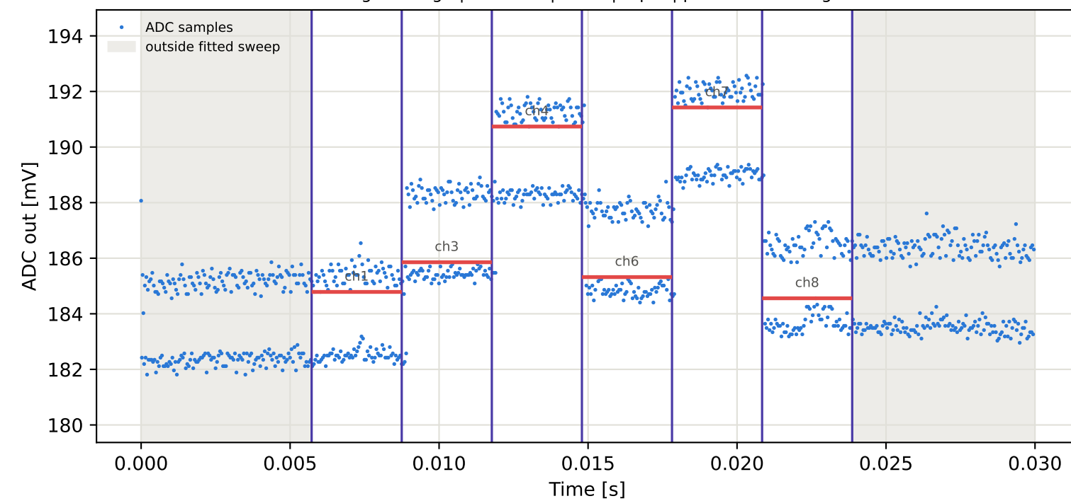
Tag3 &lt;- Tag6 | 805 MHz | run 0 | rep 1 | phase -169.58 deg
