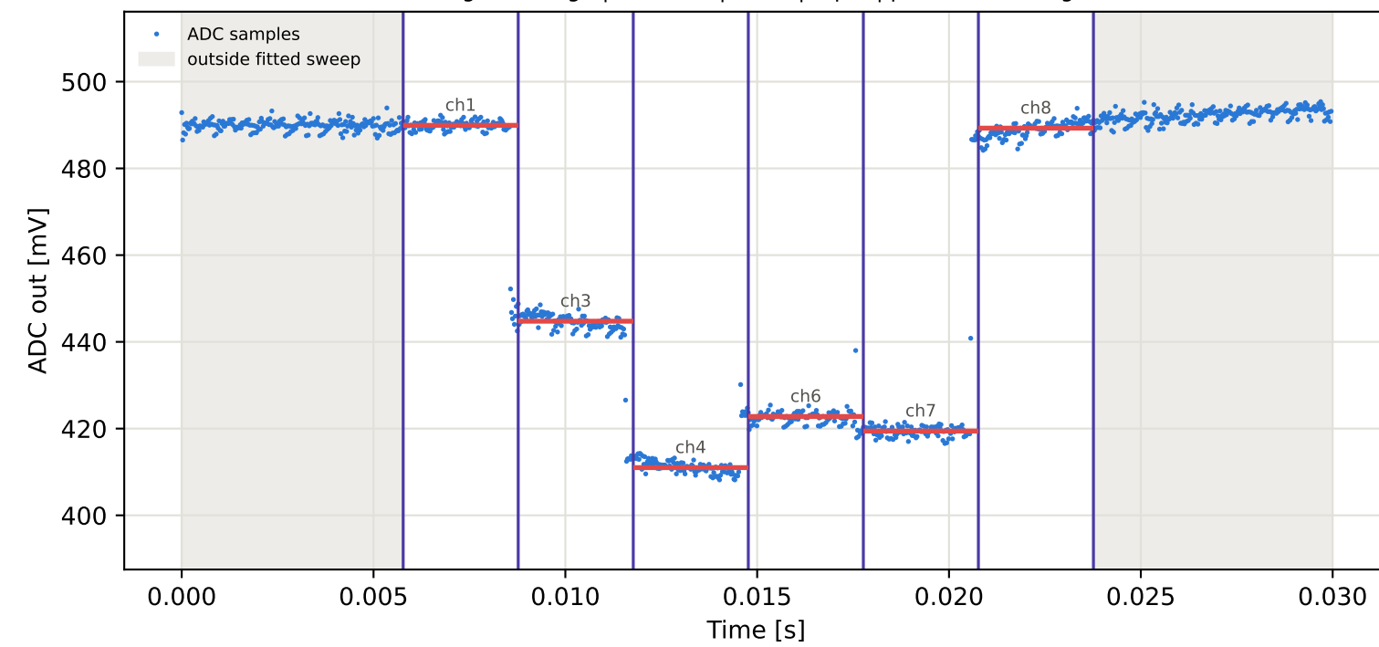
Tag15 &lt;- Tag5 | 885 MHz | run 0 | rep 1 | phase 75.13 deg
