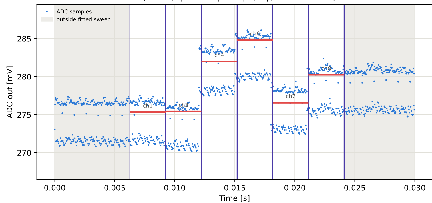
Tag3 &lt;- Tag15 | 995 MHz | run 0 | rep 1 | phase 174.13 deg
