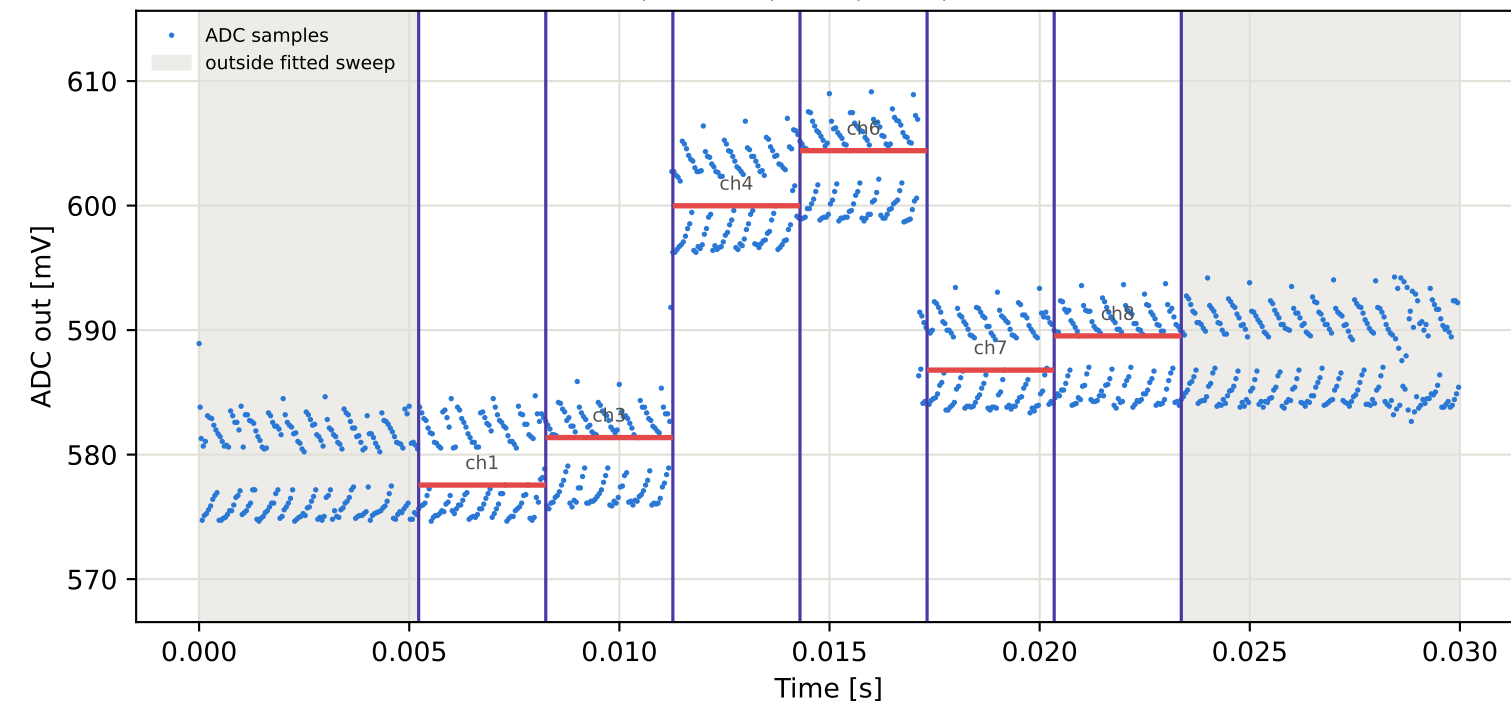
Tag6 &lt;- Tag1 | 975 MHz | run 0 | rep 1 | phase -143.96 deg
