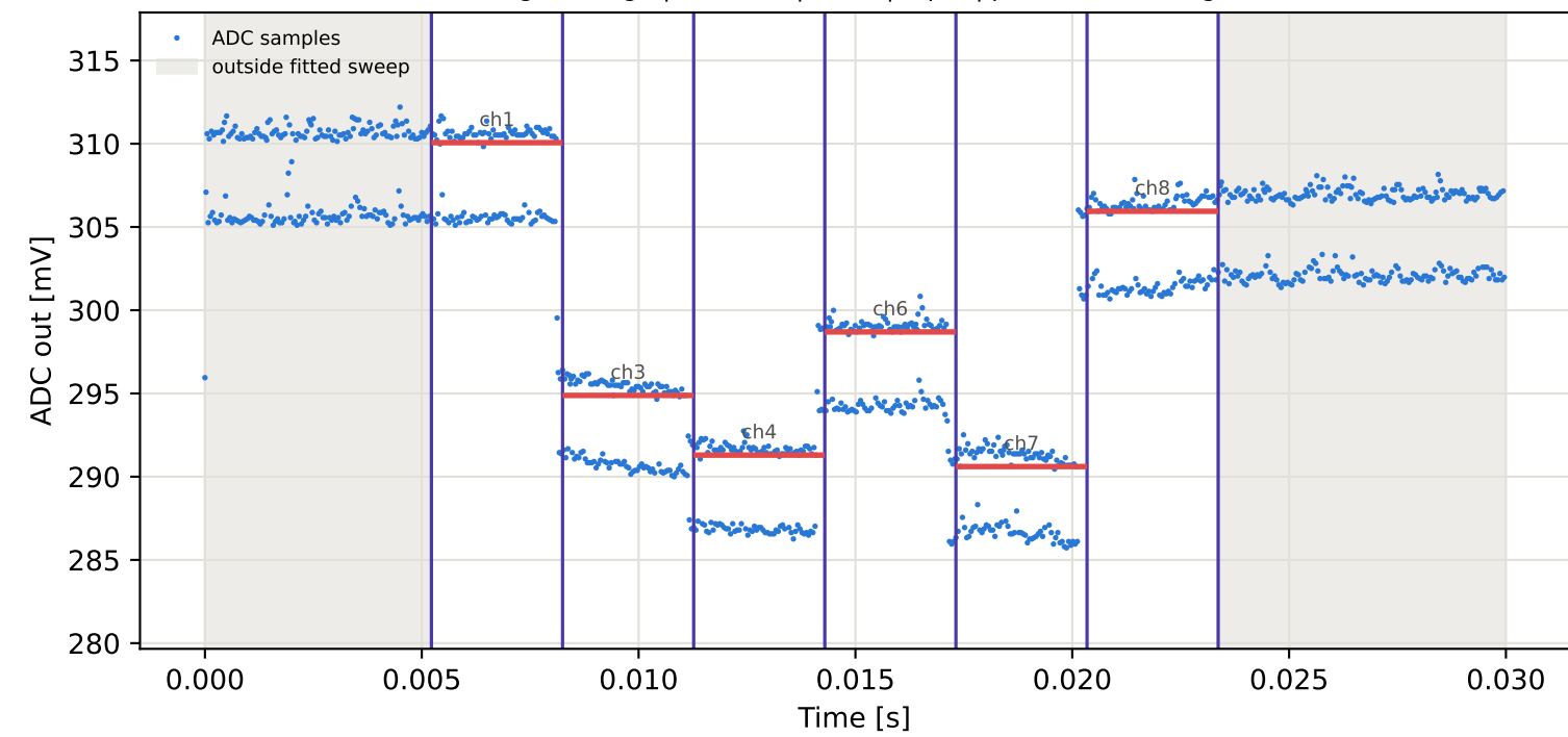
Tag2 &lt;- Tag6 | 845 MHz | run 0 | rep 1 | phase -93.15 deg
