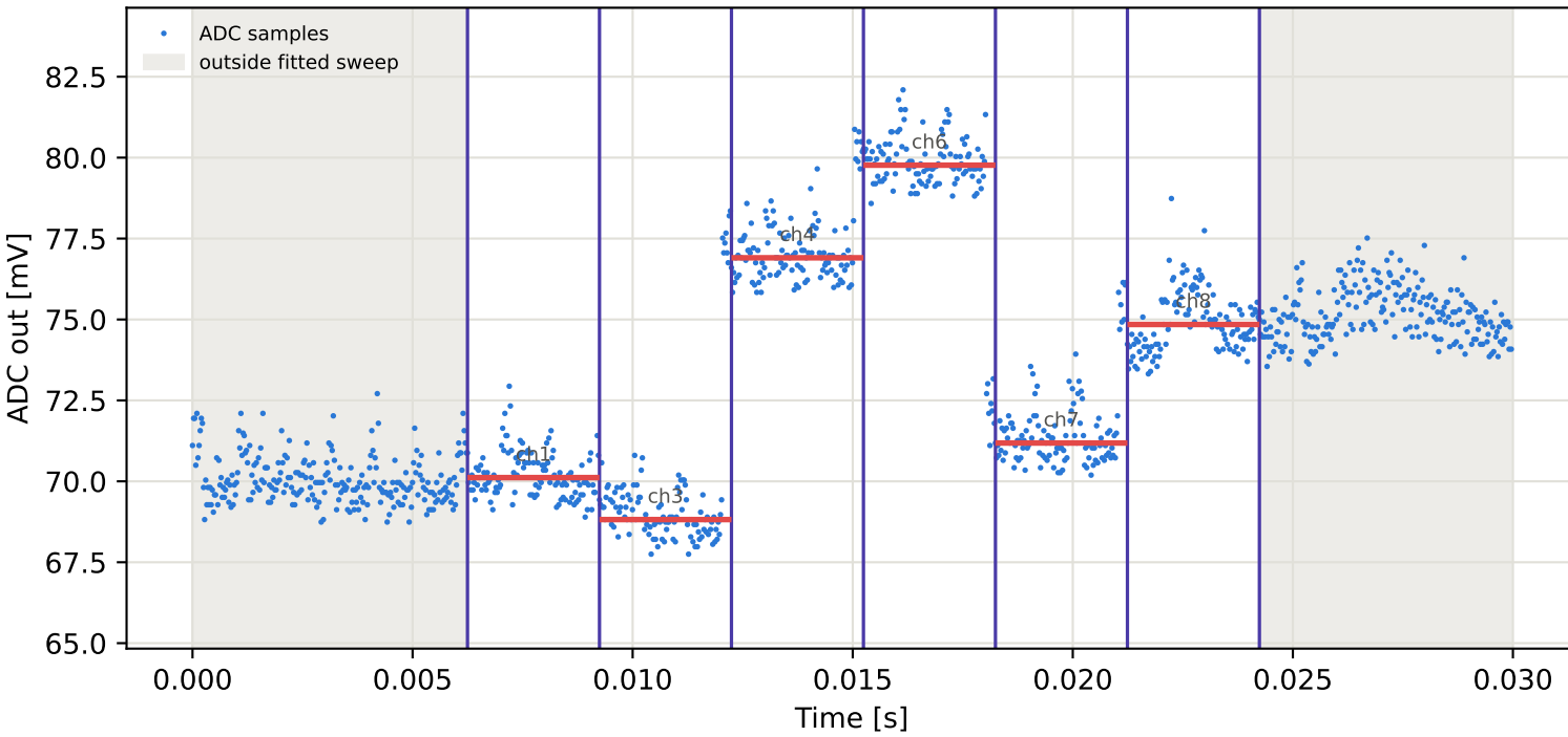
Tag2 &lt;- Tag15 | 995 MHz | run 0 | rep 1 | phase 14.64 deg
