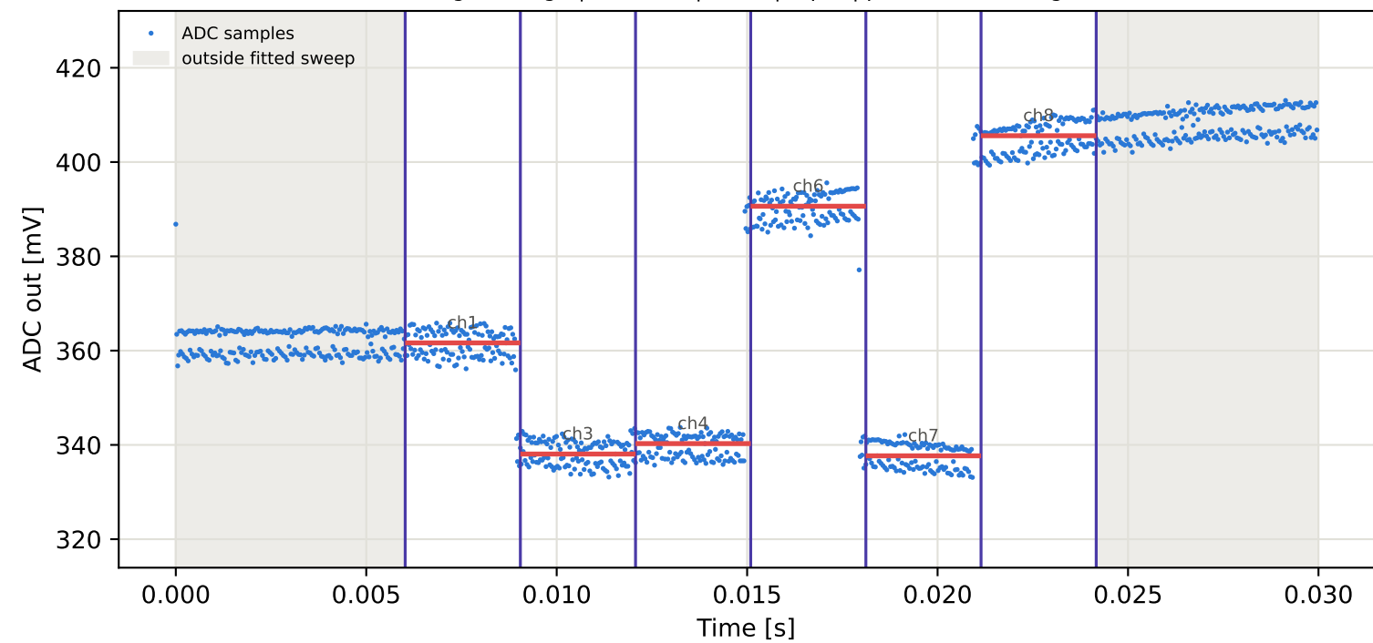
Tag1 &lt;- Tag8 | 885 MHz | run 0 | rep 1 | phase -145.65 deg
