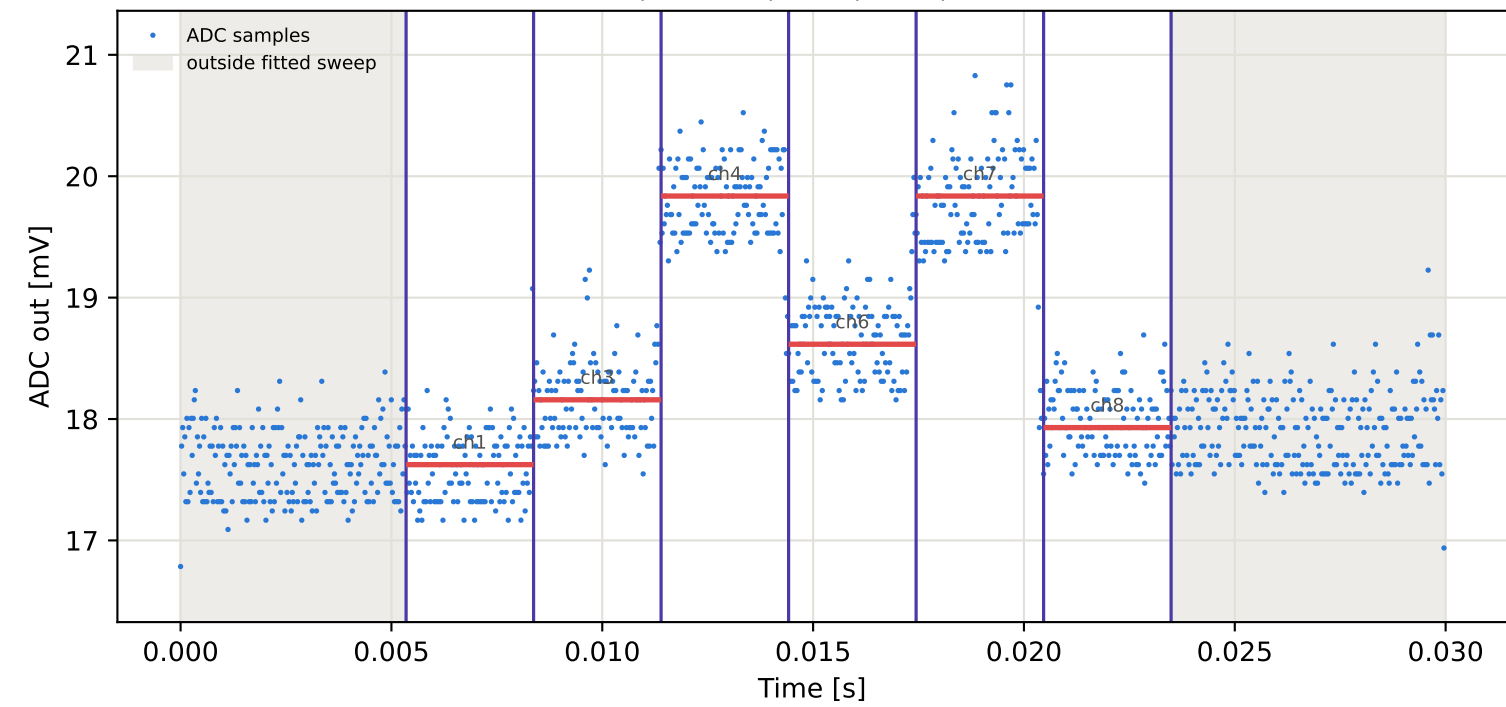
Tag15 &lt;- Tag6 | 775 MHz | run 0 | rep 1 | phase -83.64 deg
