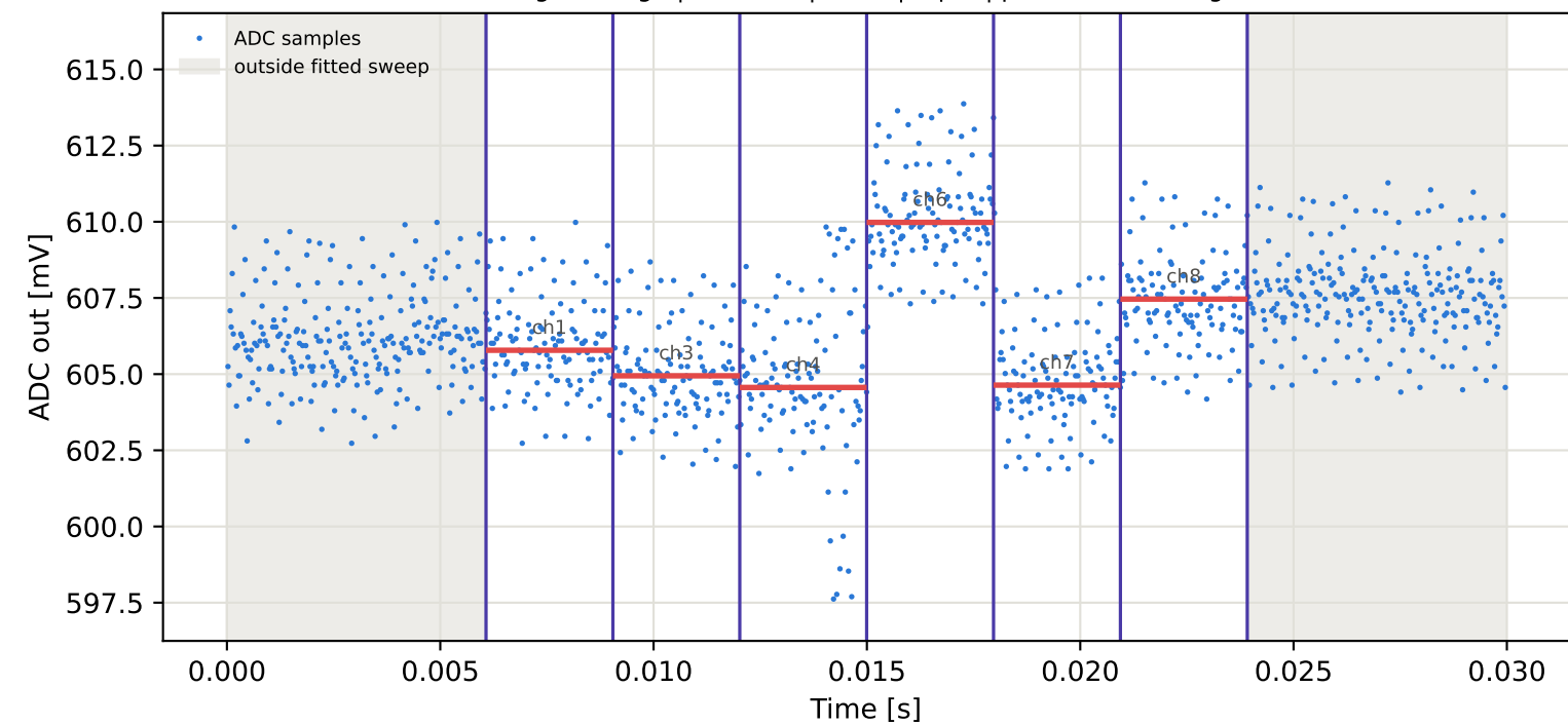
Tag3 &lt;- Tag2 | 945 MHz | run 0 | rep 1 | phase 166.93 deg
