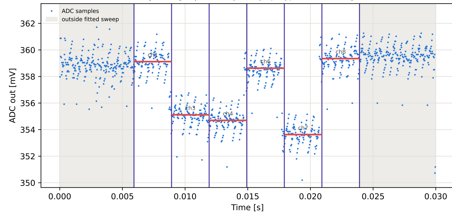
Tag6 &lt;- Tag2 | 825 MHz | run 0 | rep 1 | phase -139.35 deg
