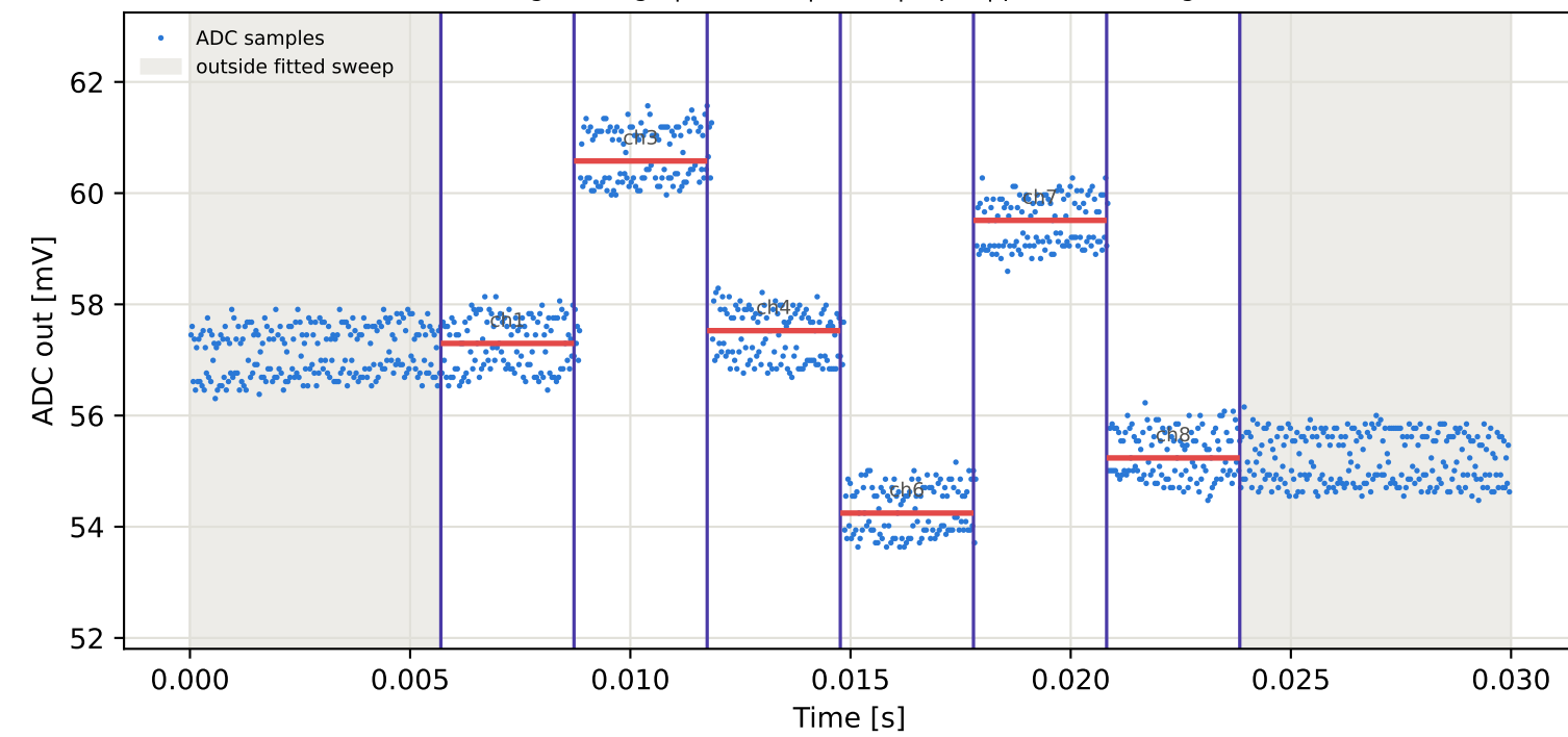
Tag1 &lt;- Tag7 | 805 MHz | run 0 | rep 1 | phase -96.09 deg
