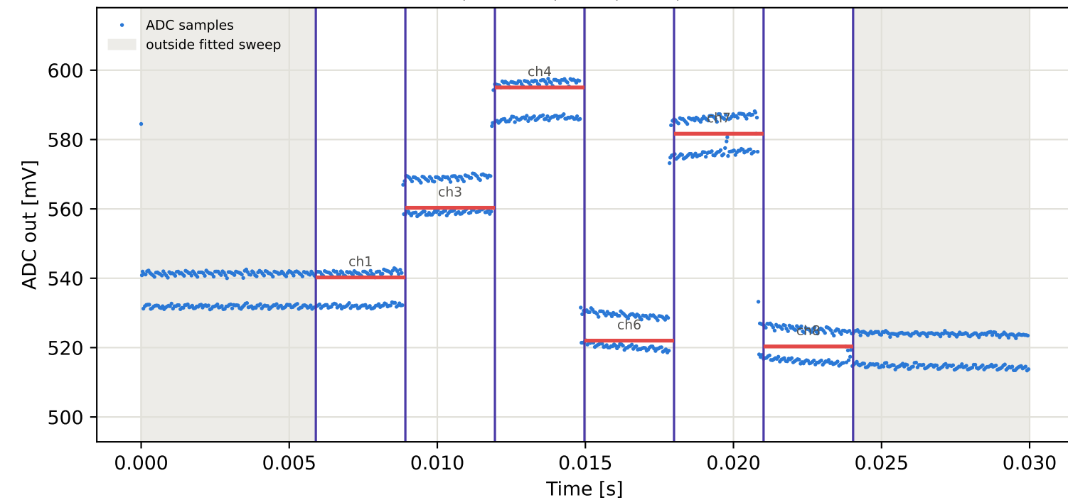
Tag3 &lt;- Tag16 | 975 MHz | run 0 | rep 1 | phase -64.98 deg
