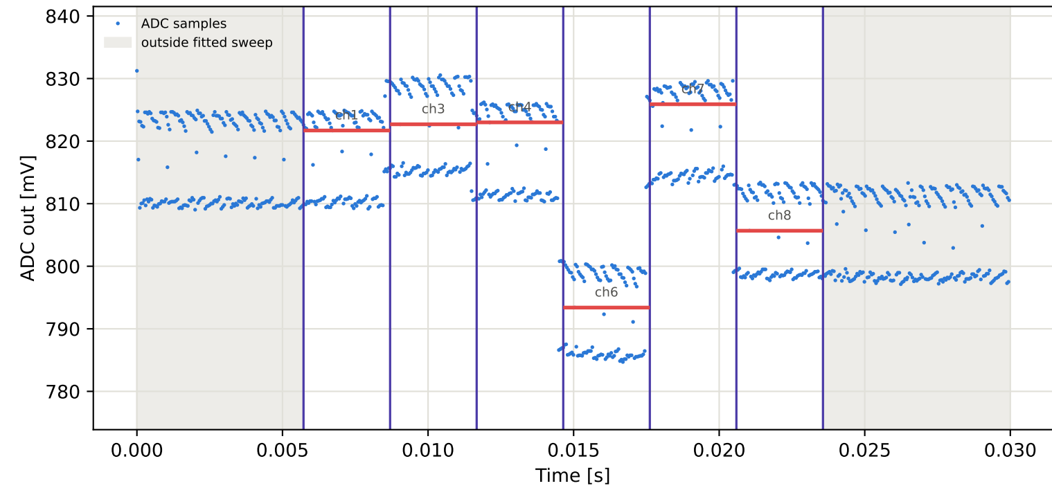
Tag9 &lt;- Tag2 | 945 MHz | run 0 | rep 1 | phase 115.71 deg
