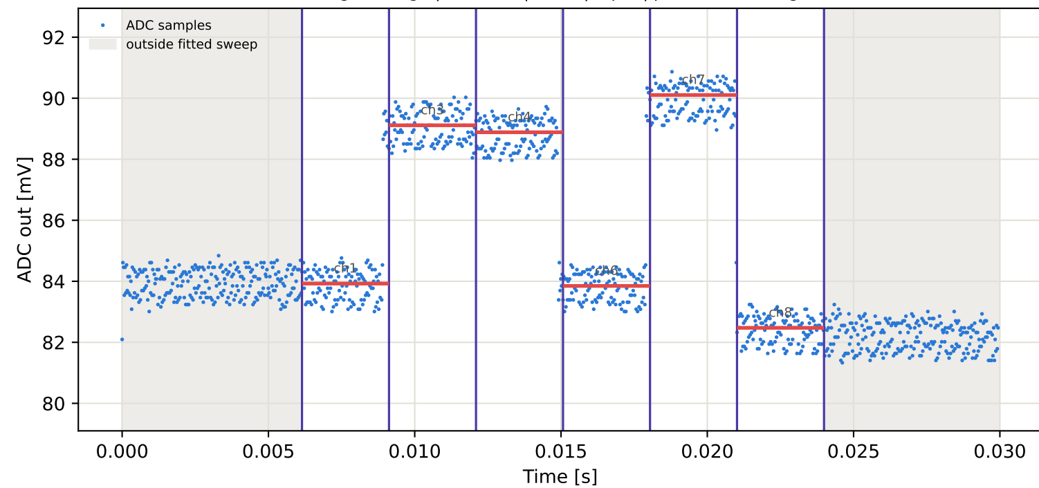
Tag5 &lt;- Tag9 | 795 MHz | run 0 | rep 1 | phase -130.18 deg
