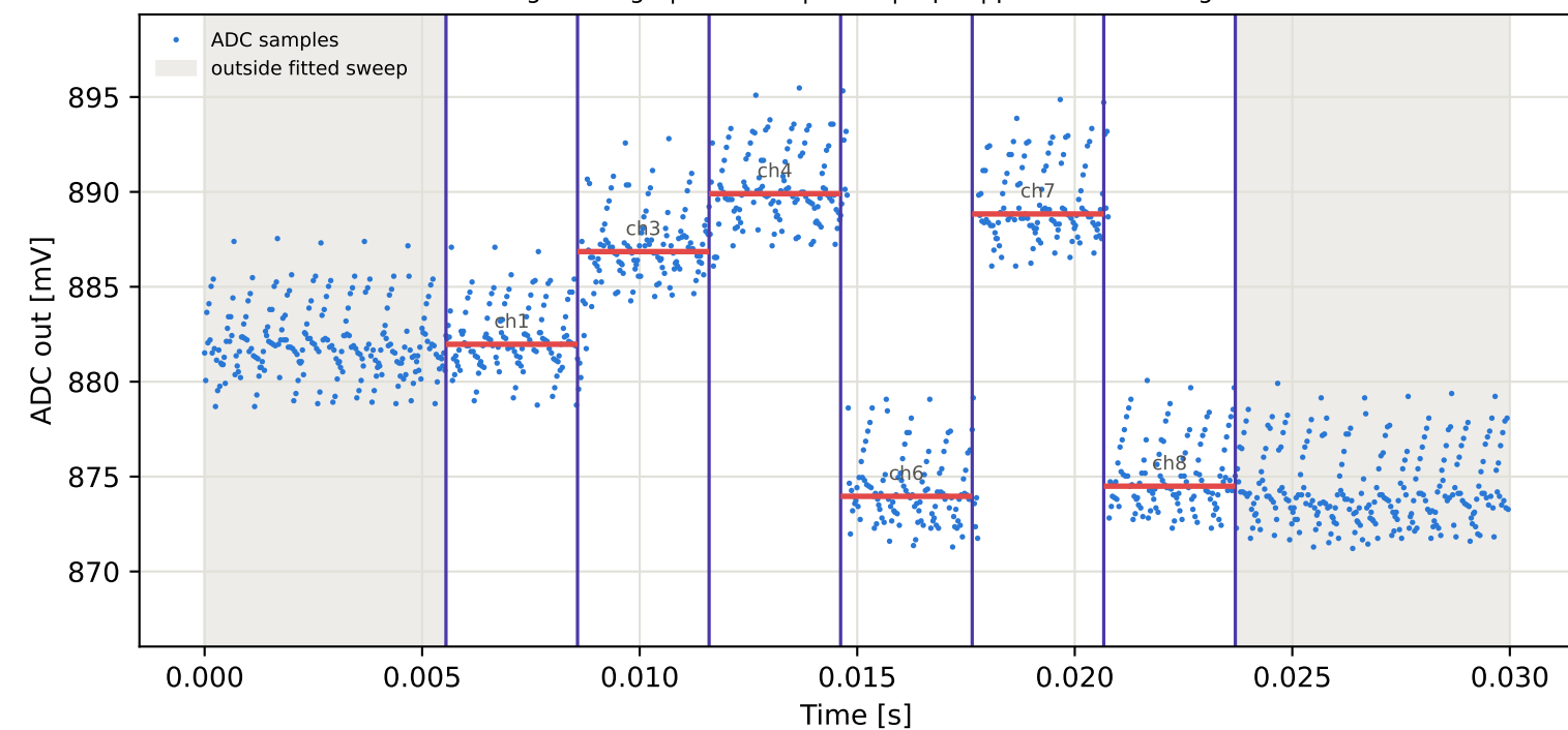
Tag7 &lt;- Tag4 | 895 MHz | run 0 | rep 1 | phase -98.85 deg
