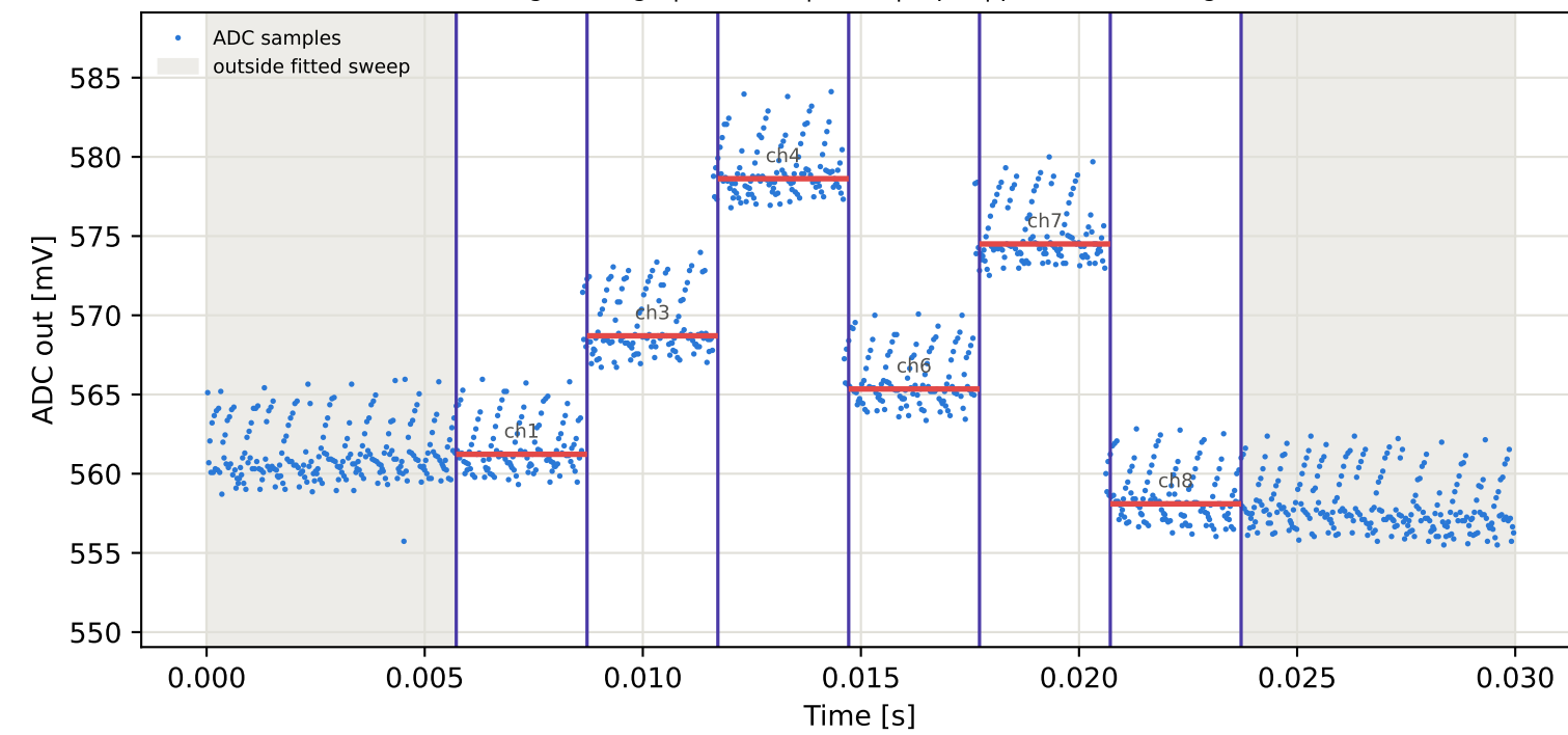
Tag5 &lt;- Tag8 | 935 MHz | run 0 | rep 1 | phase -157.65 deg
