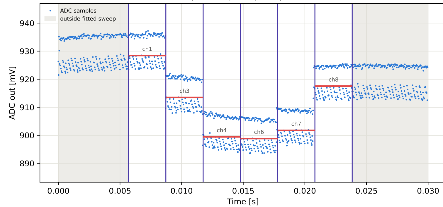
Tag3 &lt;- Tag6 | 875 MHz | run 0 | rep 1 | phase 0.73 deg
