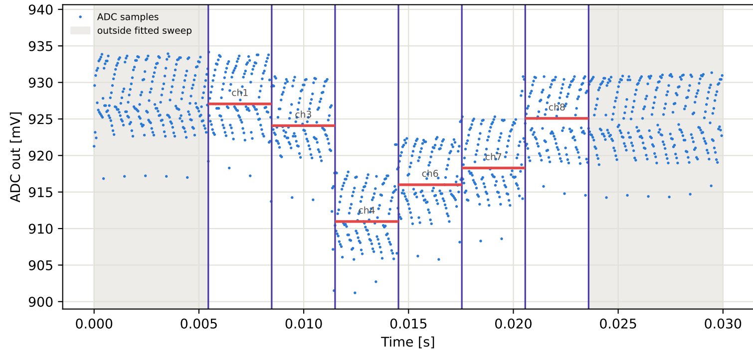
Tag7 &lt;- Tag15 | 965 MHz | run 0 | rep 1 | phase -126.95 deg
