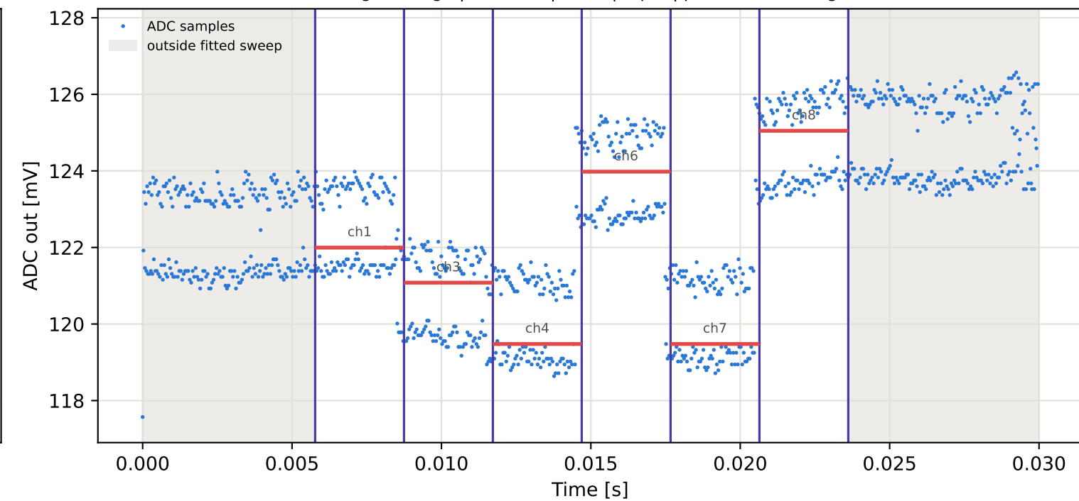
Tag5 &lt;- Tag4 | 825 MHz | run 0 | rep 1 | phase 23.65 deg
