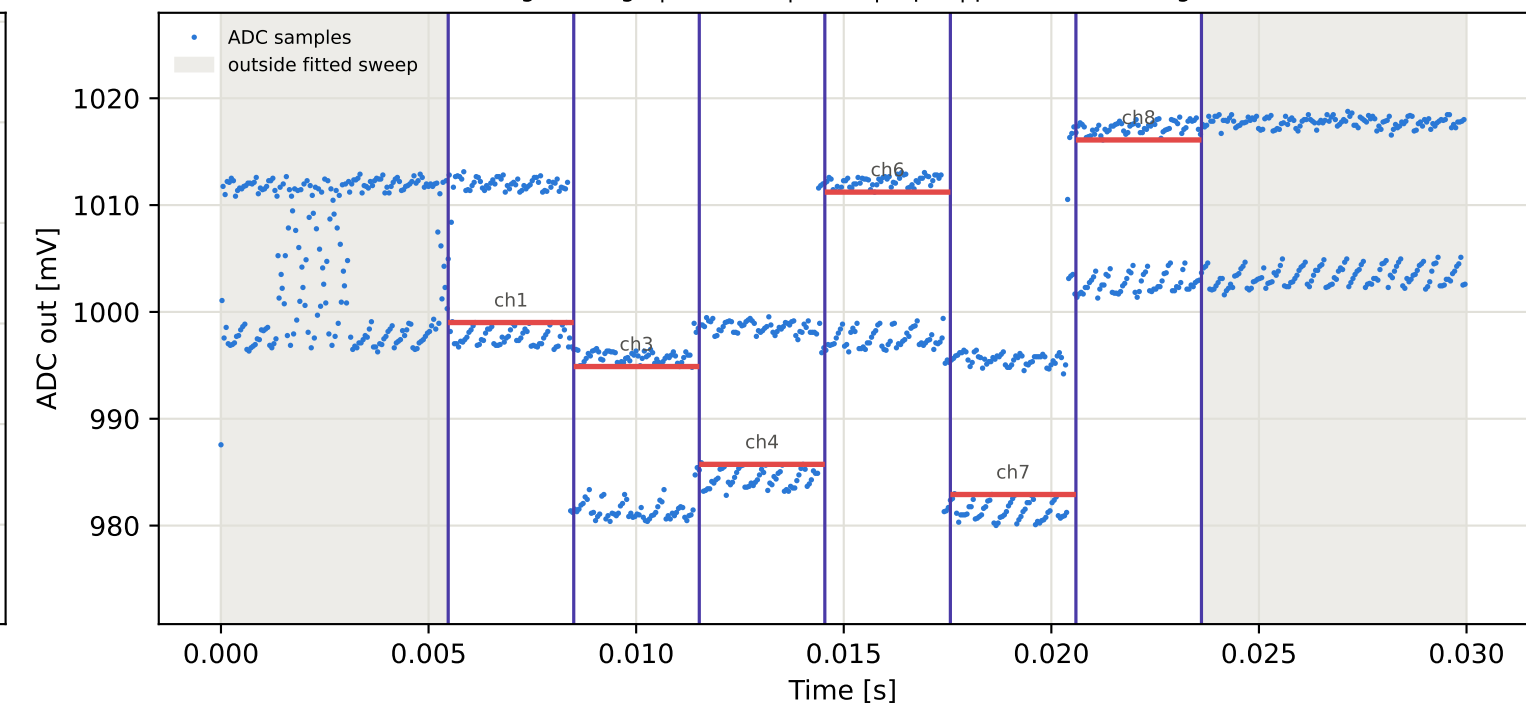
Tag7 &lt;- Tag6 | 845 MHz | run 0 | rep 1 | phase 140.62 deg
