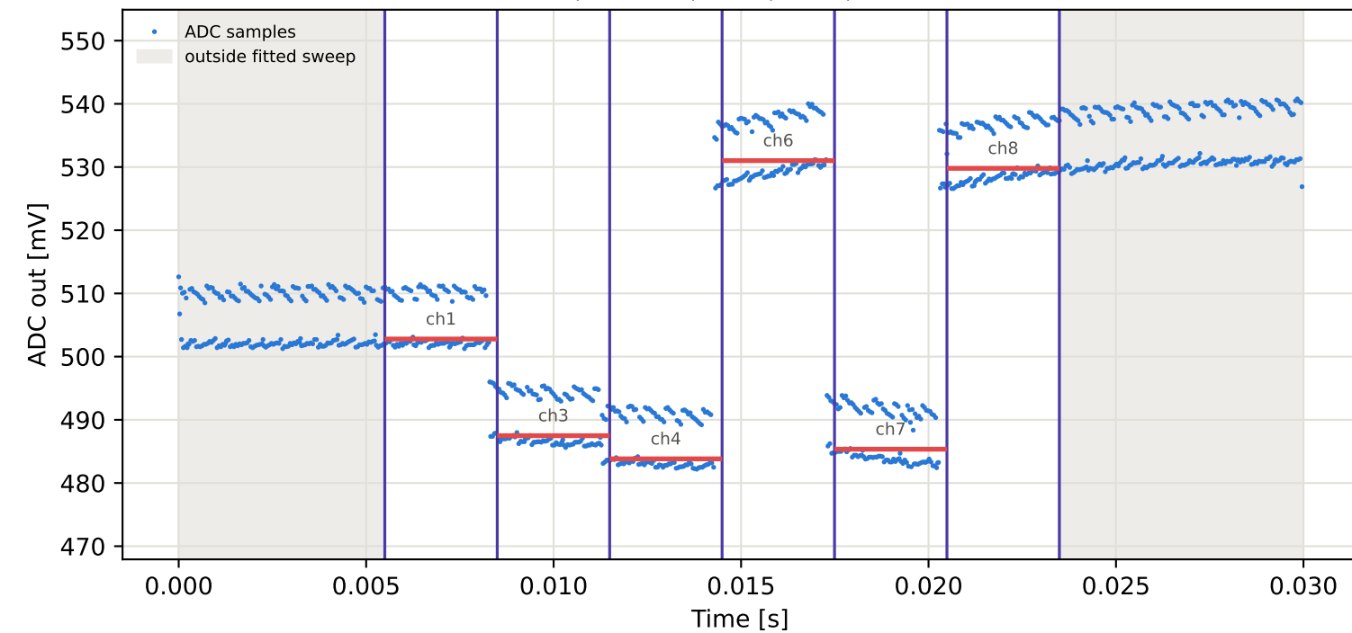
Tag5 &lt;- Tag3 | 905 MHz | run 0 | rep 1 | phase 153.97 deg
