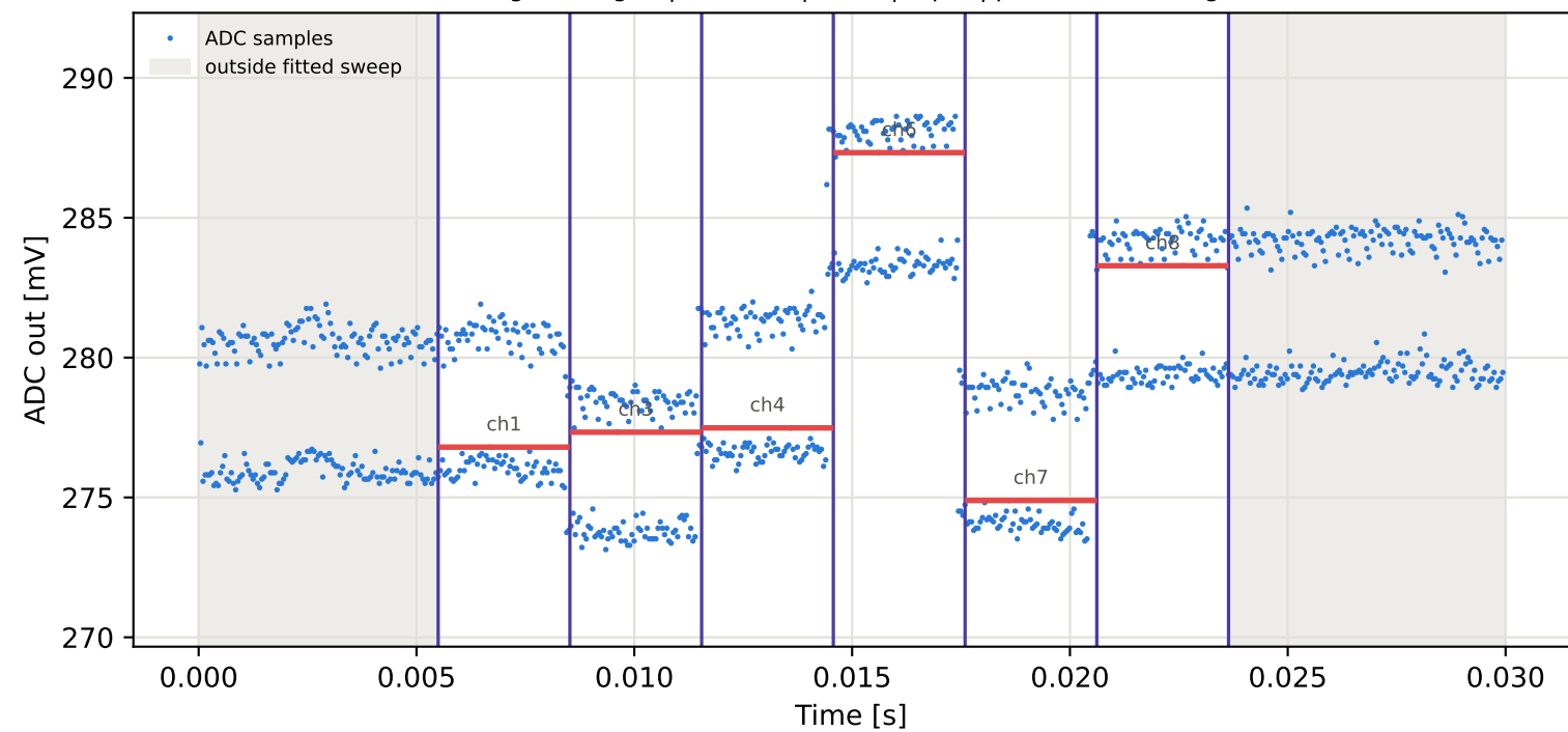
Tag3 &lt;- Tag2 | 995 MHz | run 0 | rep 1 | phase -169.42 deg
