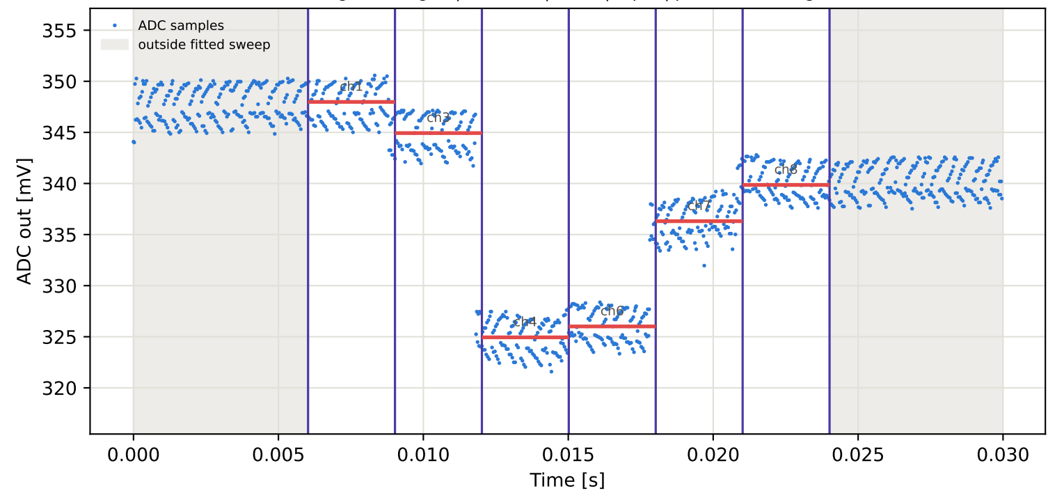
Tag10 &lt;- Tag3 | 975 MHz | run 0 | rep 1 | phase 174.18 deg
