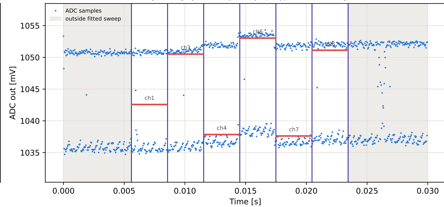
Tag7 &lt;- Tag4 | 835 MHz | run 0 | rep 1 | phase 8.83 deg
