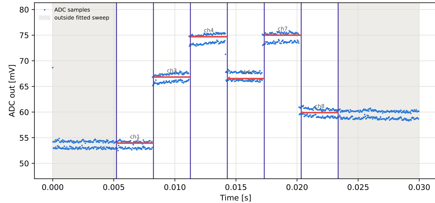
Tag1 &lt;- Tag3 | 845 MHz | run 0 | rep 1 | phase 123.73 deg
