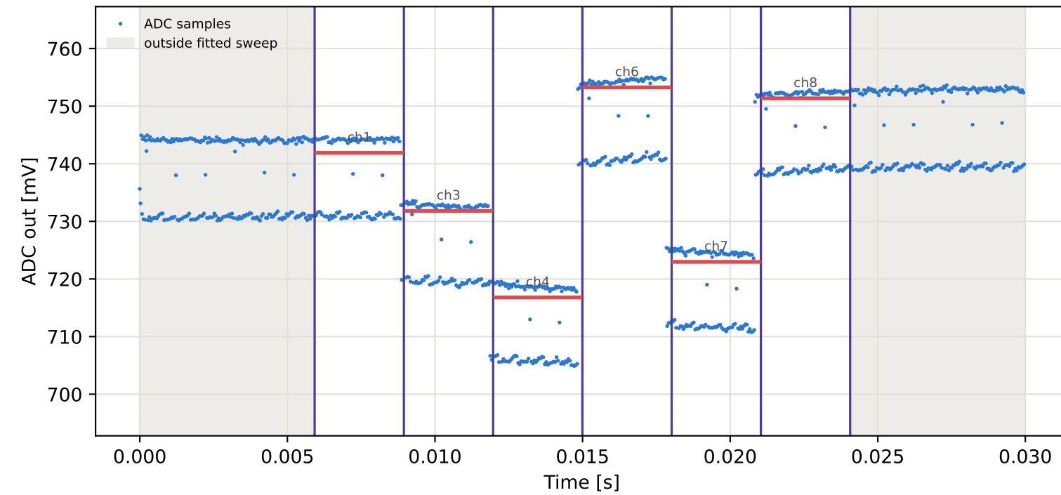
Tag9 &lt;- Tag7 | 985 MHz | run 0 | rep 1 | phase 117.86 deg
