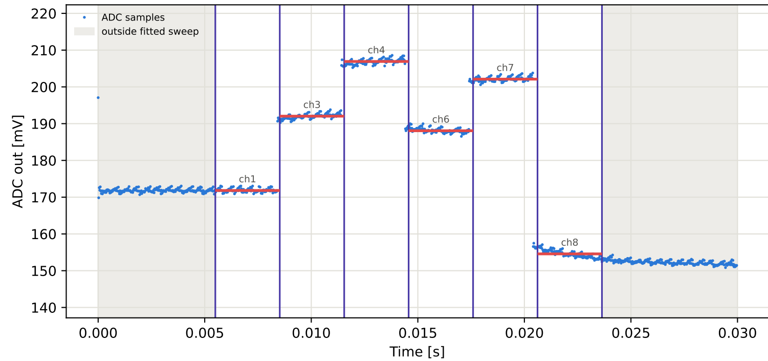
Tag4 &lt;- Tag3 | 905 MHz | run 0 | rep 1 | phase -13.52 deg
