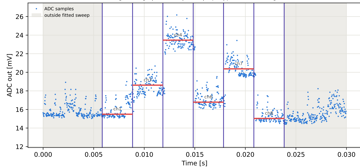
Tag2 &lt;- Tag8 | 975 MHz | run 0 | rep 1 | phase -108.14 deg
