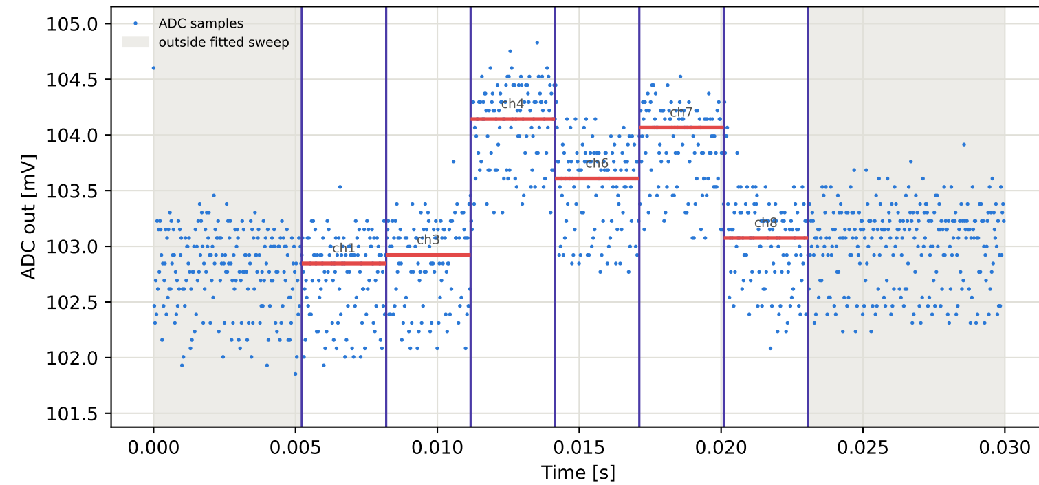
Tag1 &lt;- Tag3 | 795 MHz | run 0 | rep 1 | phase 140.36 deg
