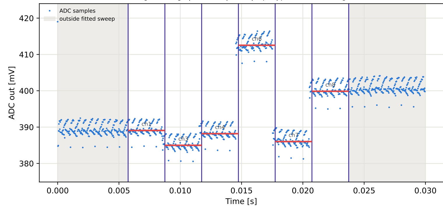
Tag15 &lt;- Tag6 | 935 MHz | run 0 | rep 1 | phase 82.49 deg
