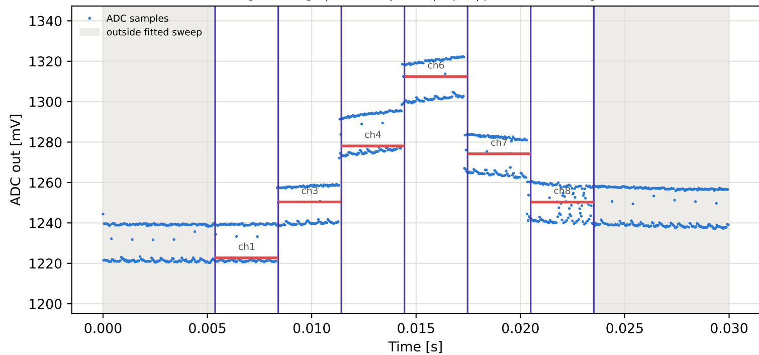
Tag16 &lt;- Tag5 | 905 MHz | run 0 | rep 1 | phase -164.82 deg
