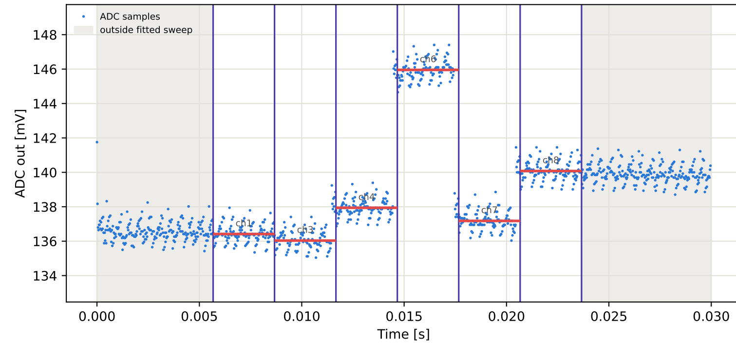
Tag6 &lt;- Tag1 | 915 MHz | run 0 | rep 1 | phase 26.55 deg
