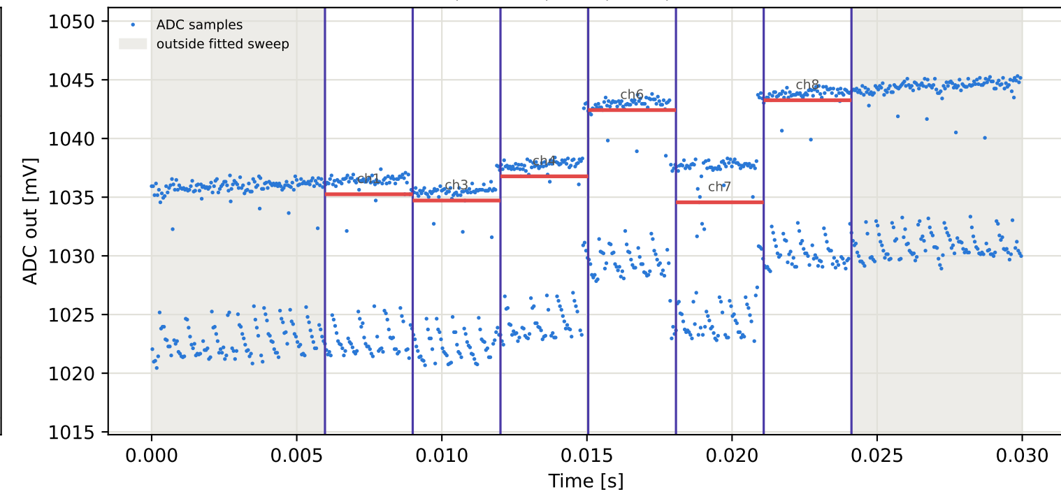
Tag7 &lt;- Tag6 | 875 MHz | run 0 | rep 1 | phase -178.24 deg
