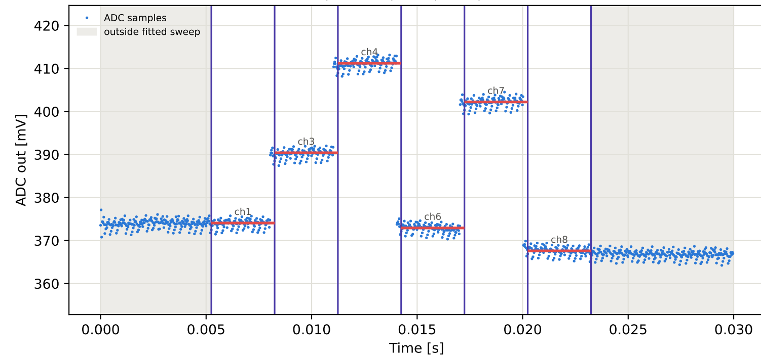
Tag1 &lt;- Tag9 | 995 MHz | run 0 | rep 1 | phase -77.16 deg
