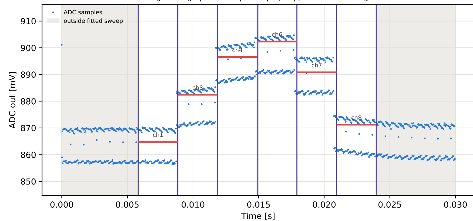
Tag7 &lt;- Tag6 | 895 MHz | run 0 | rep 1 | phase -121.01 deg
