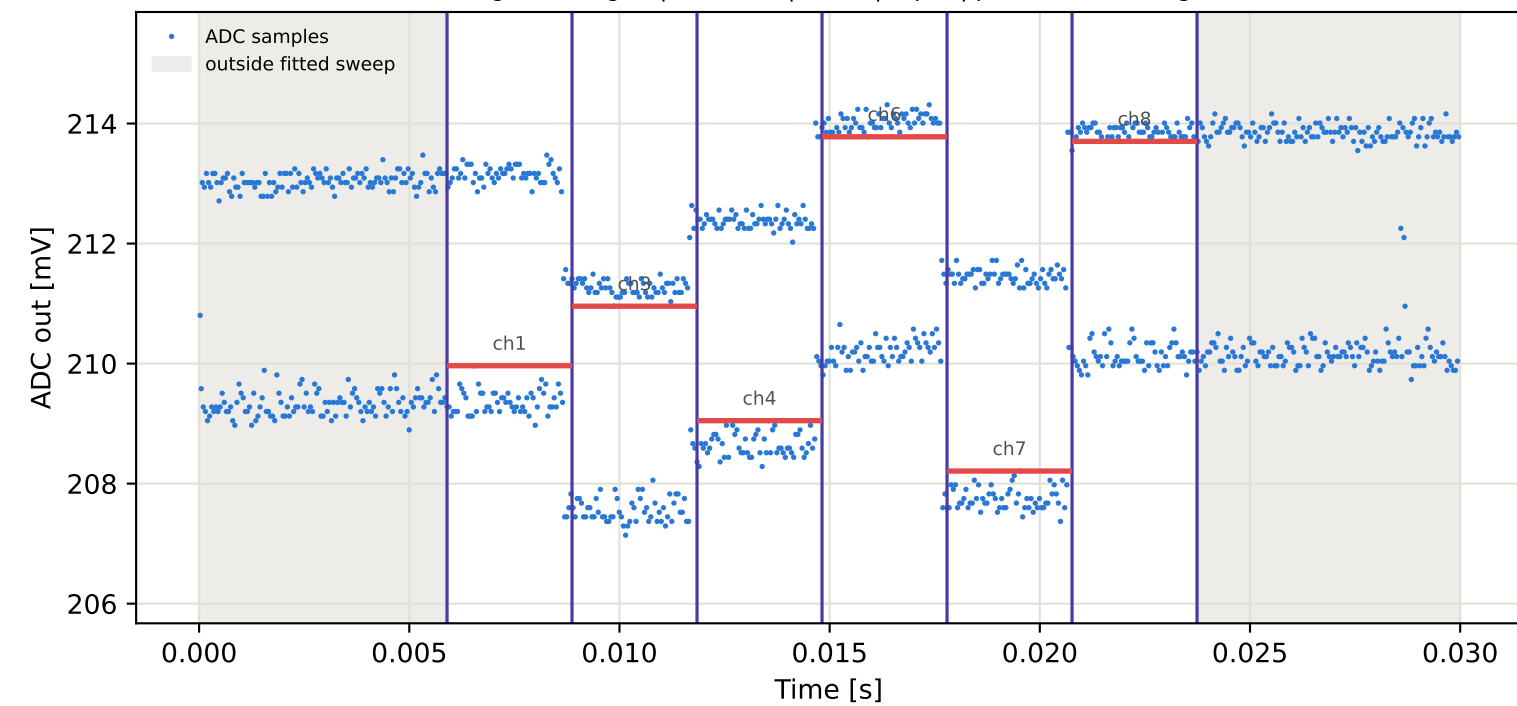
Tag10 &lt;- Tag2 | 805 MHz | run 0 | rep 1 | phase 111.34 deg
