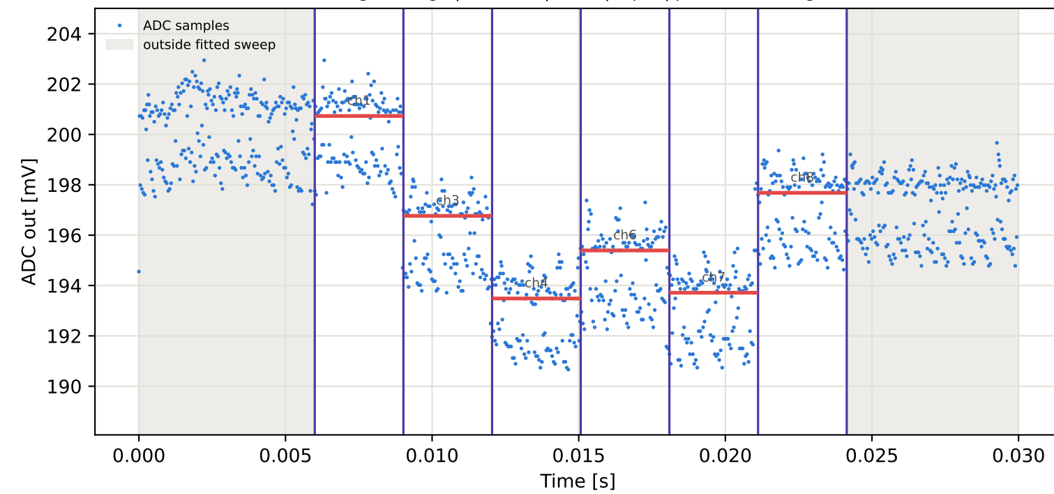
Tag2 &lt;- Tag5 | 835 MHz | run 0 | rep 1 | phase -50.63 deg
