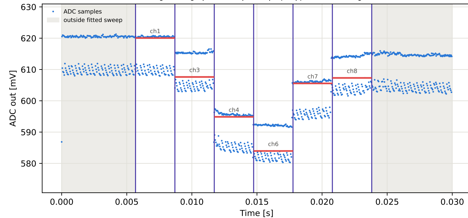
Tag3 &lt;- Tag8 | 945 MHz | run 0 | rep 1 | phase 38.38 deg
