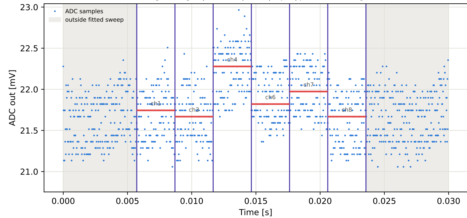
Tag1 &lt;- Tag2 | 775 MHz | run 0 | rep 1 | phase 3.25 deg
