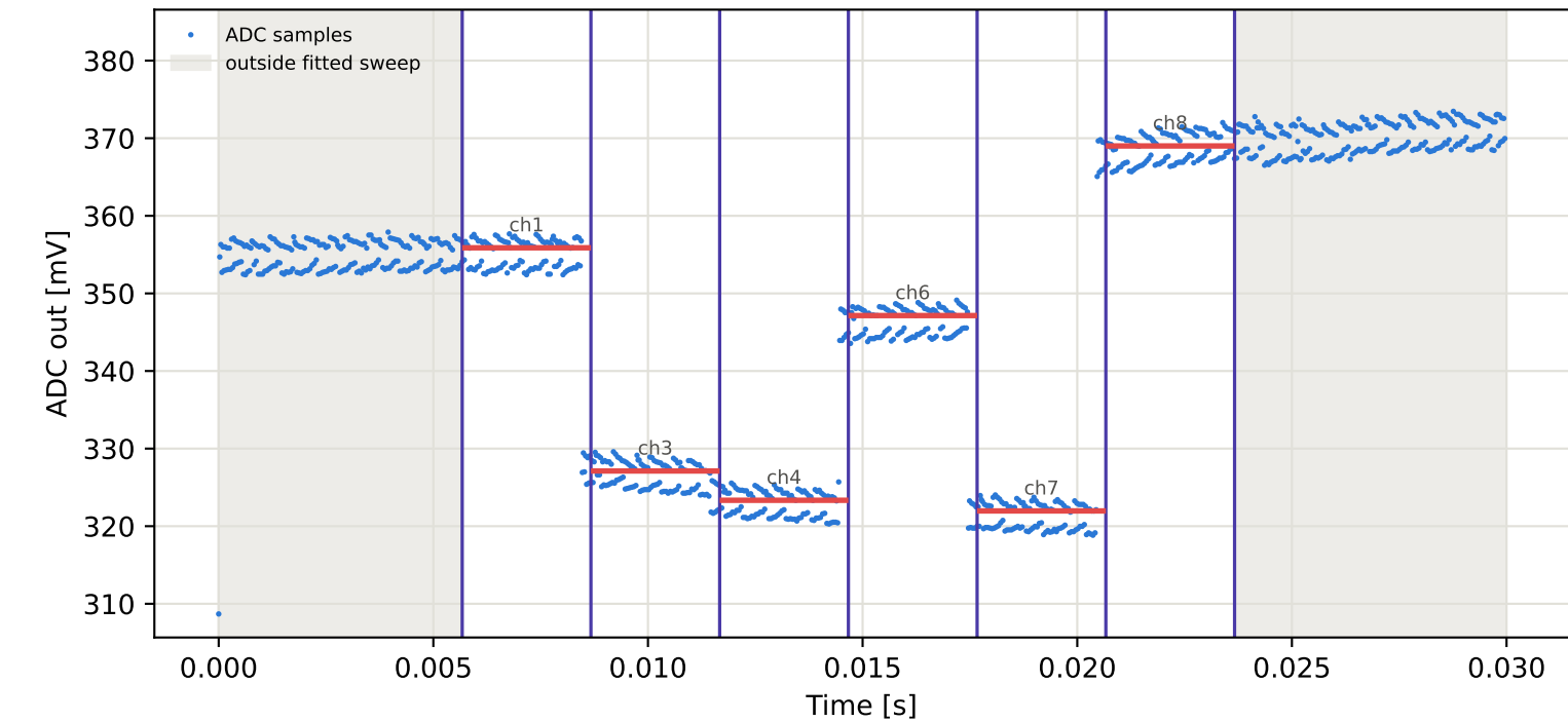
Tag8 &lt;- Tag16 | 865 MHz | run 0 | rep 1 | phase 87.80 deg
