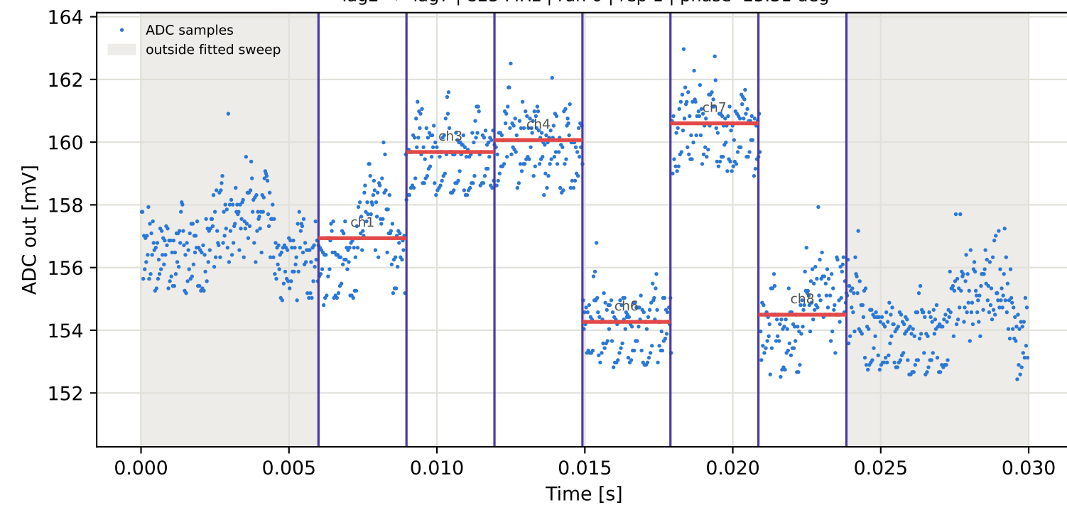
Tag2 &lt;- Tag7 | 825 MHz | run 0 | rep 1 | phase -25.31 deg
