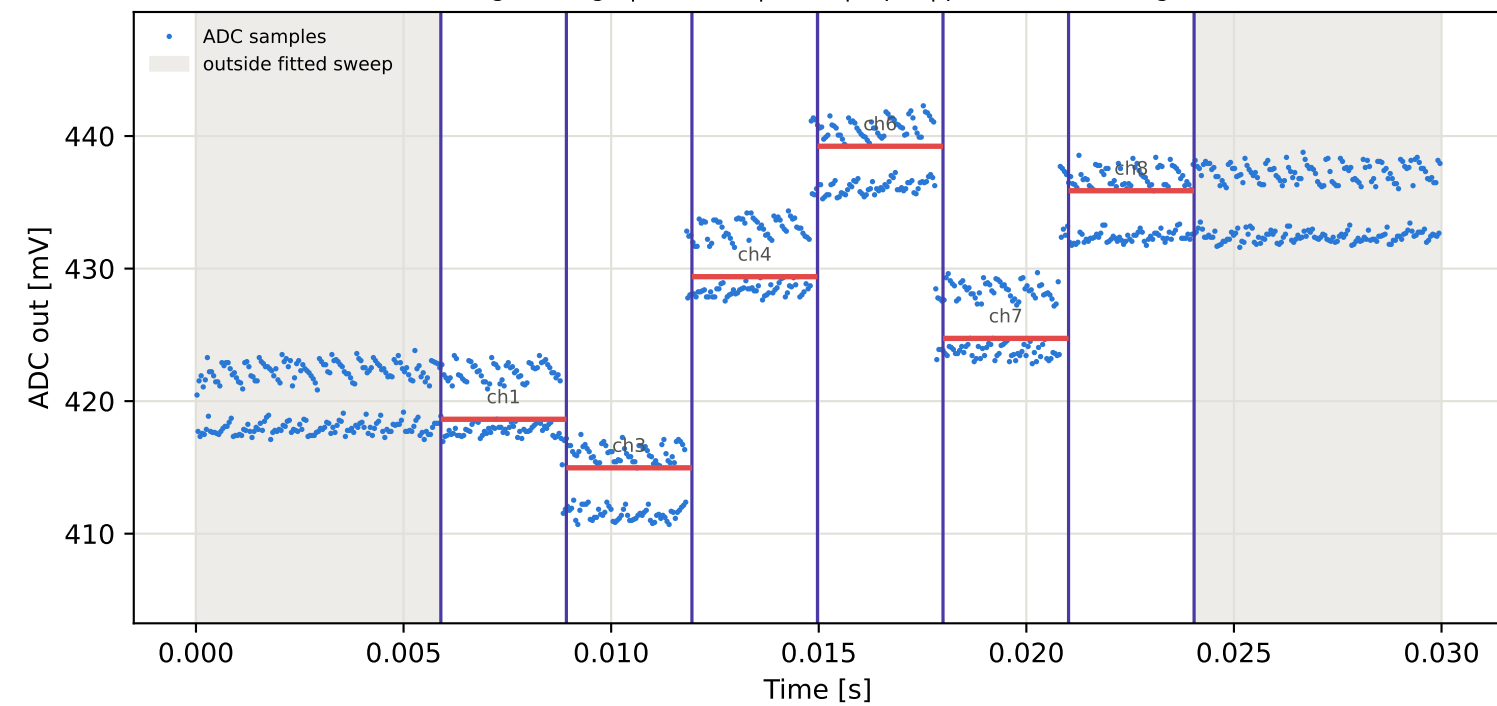
Tag7 &lt;- Tag1 | 835 MHz | run 0 | rep 1 | phase 157.86 deg
