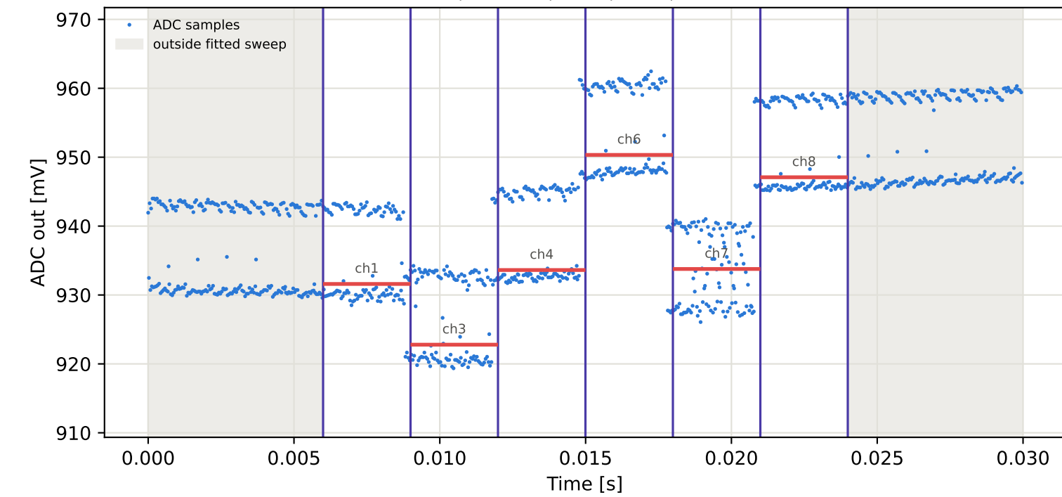
Tag16 &lt;- Tag7 | 875 MHz | run 0 | rep 1 | phase -168.00 deg
