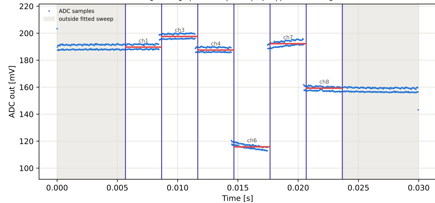
Tag4 &lt;- Tag7 | 925 MHz | run 0 | rep 1 | phase 122.39 deg
