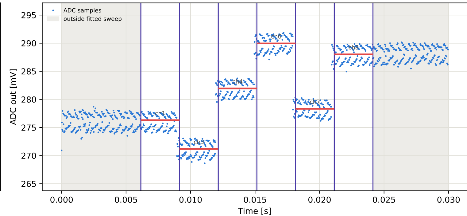
Tag5 &lt;- Tag1 | 845 MHz | run 0 | rep 1 | phase -77.05 deg
