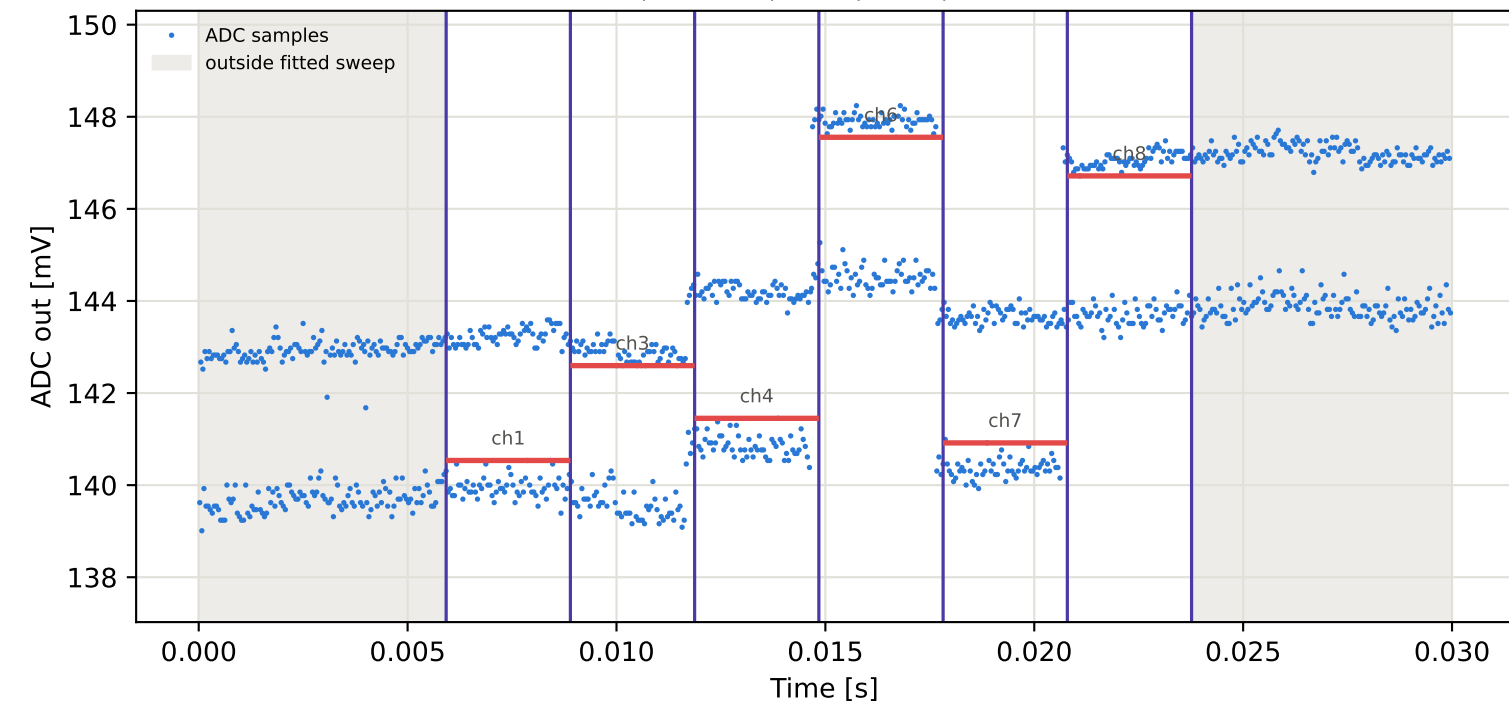
Tag1 &lt;- Tag9 | 895 MHz | run 0 | rep 1 | phase 176.06 deg
