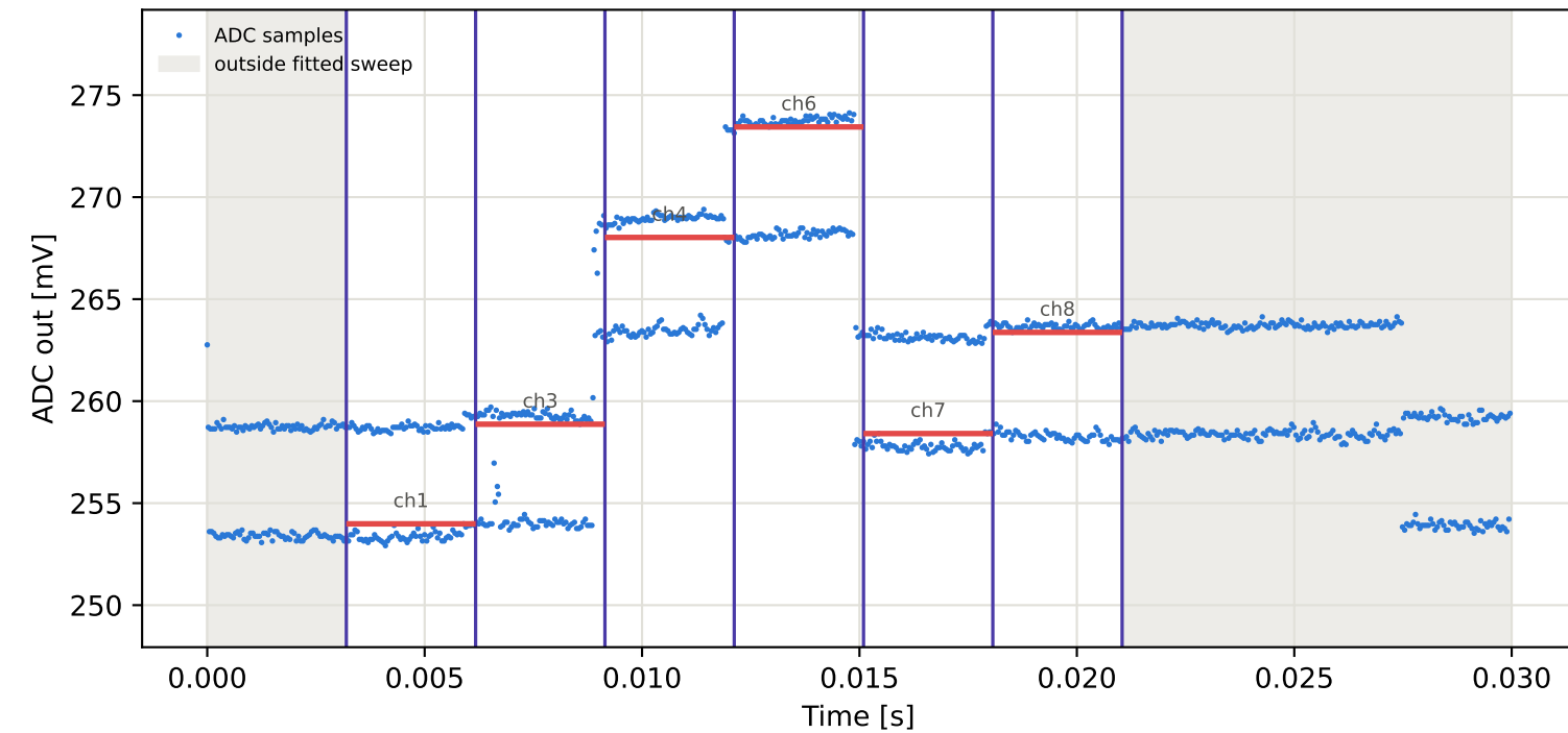
Tag6 &lt;- Tag1 | 955 MHz | run 0 | rep 1 | phase 127.15 deg
