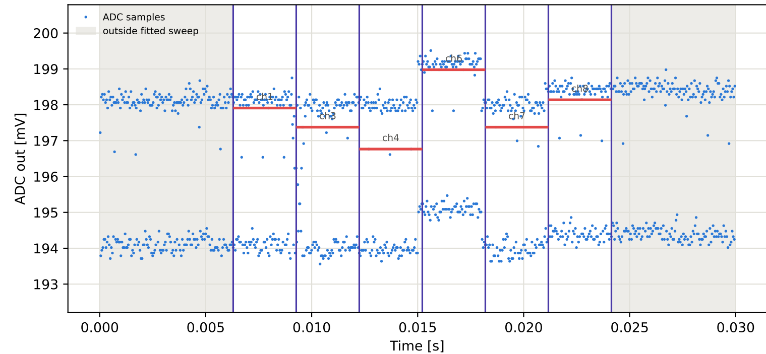
Tag5 &lt;- Tag4 | 945 MHz | run 0 | rep 1 | phase -94.32 deg
