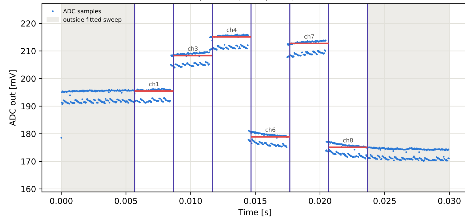
Tag4 &lt;- Tag7 | 915 MHz | run 0 | rep 1 | phase 27.81 deg
