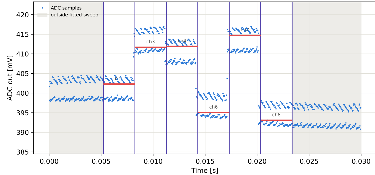
Tag6 &lt;- Tag10 | 855 MHz | run 0 | rep 1 | phase -161.58 deg
