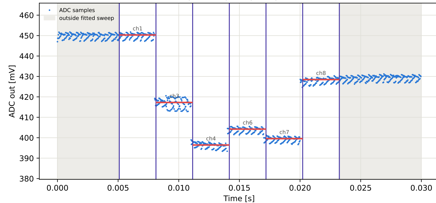
Tag5 &lt;- Tag3 | 855 MHz | run 0 | rep 1 | phase 74.36 deg
