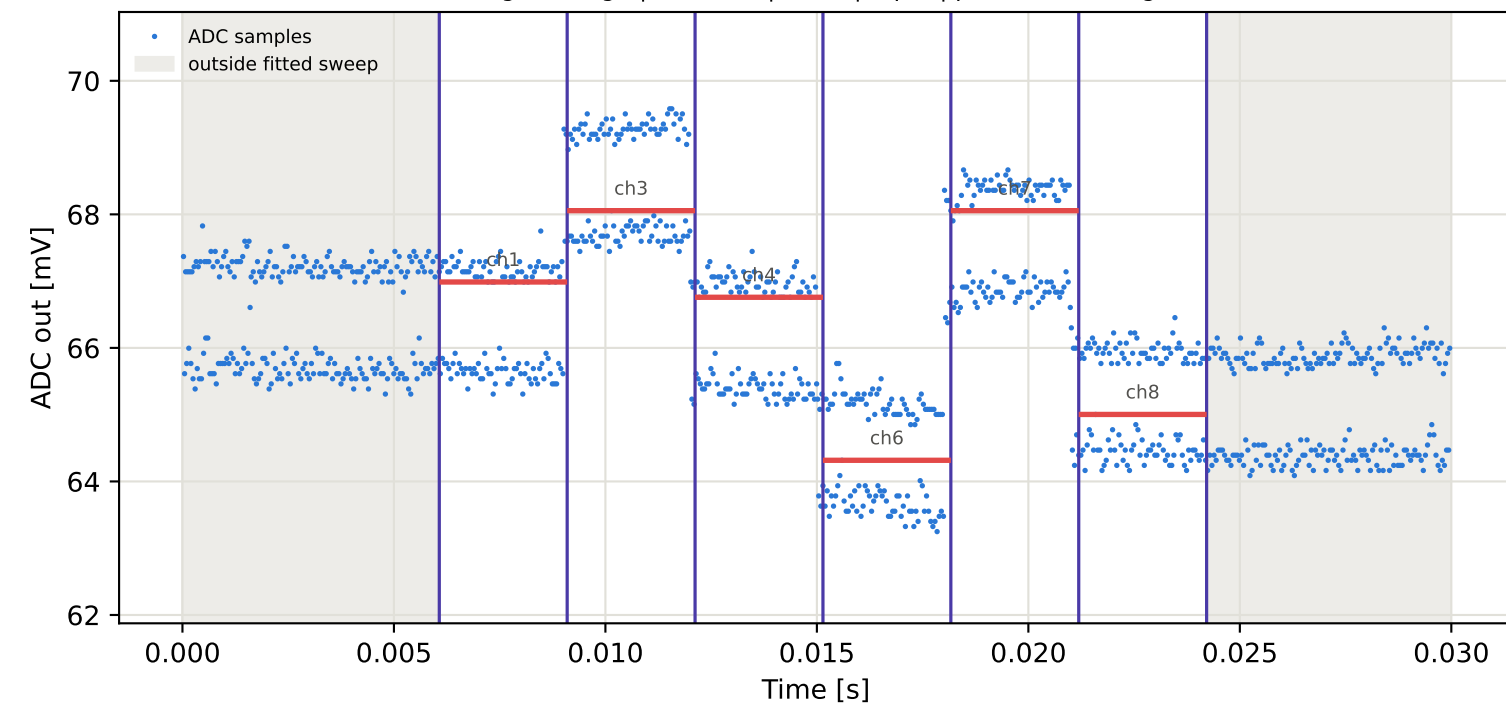
Tag1 &lt;- Tag7 | 785 MHz | run 0 | rep 1 | phase -147.87 deg
