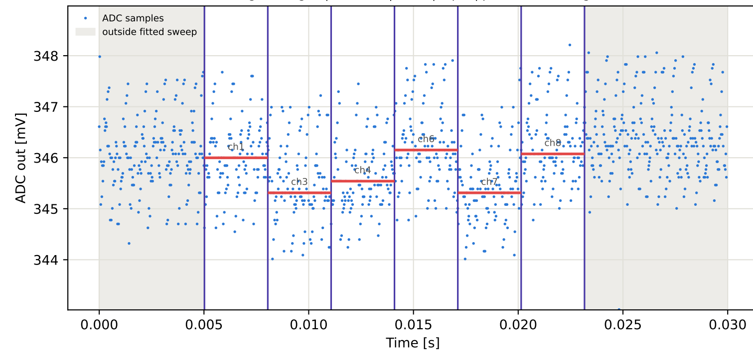
Tag7 &lt;- Tag3 | 805 MHz | run 0 | rep 1 | phase -149.86 deg
