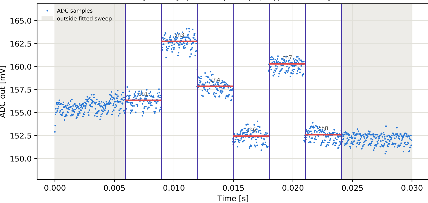
Tag15 &lt;- Tag5 | 825 MHz | run 0 | rep 1 | phase 1.43 deg
