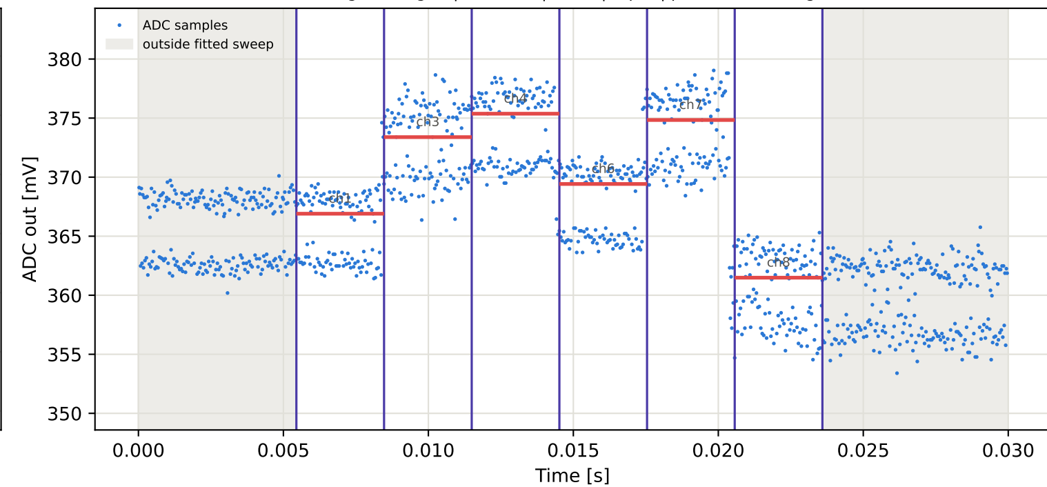
Tag1 &lt;- Tag2 | 885 MHz | run 0 | rep 1 | phase 0.54 deg
