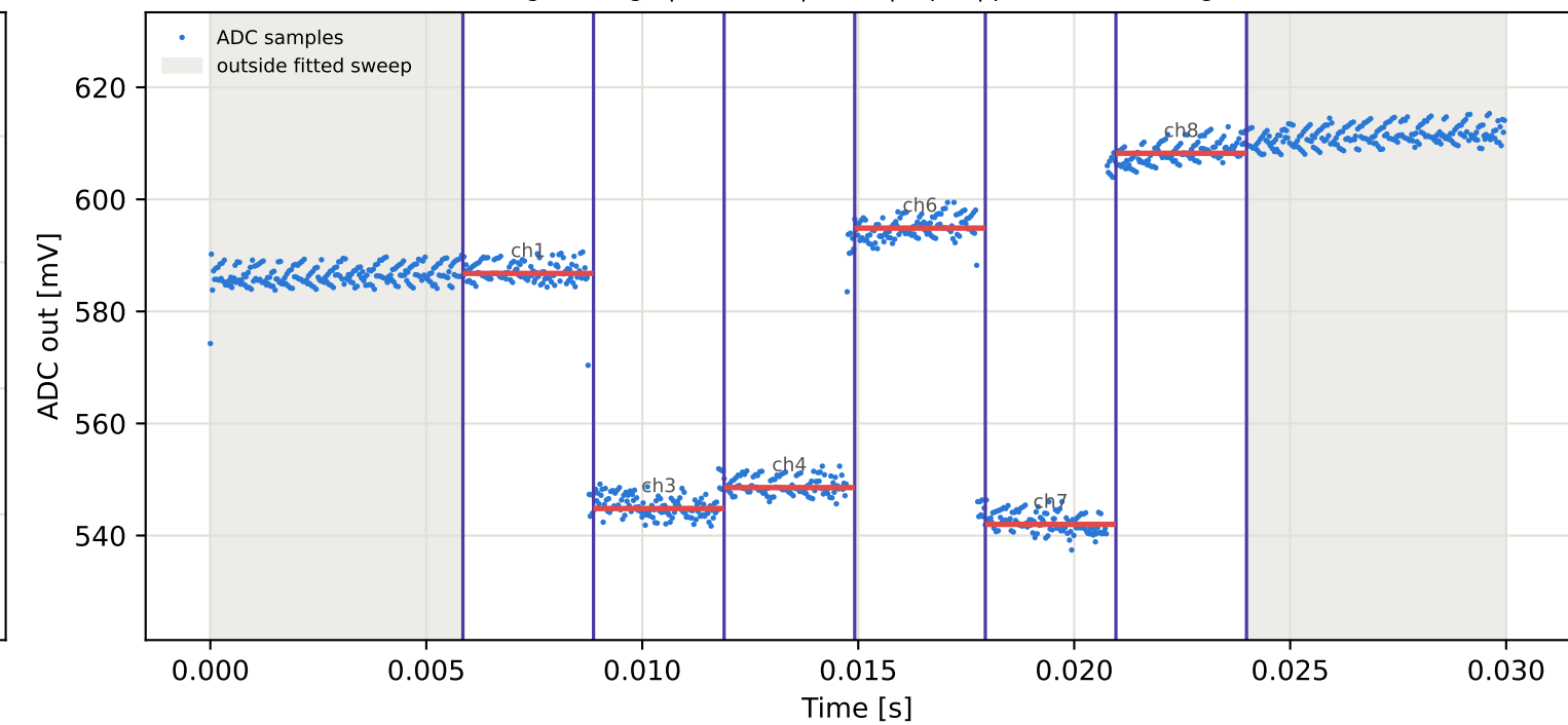
Tag5 &lt;- Tag9 | 875 MHz | run 0 | rep 1 | phase -12.66 deg
