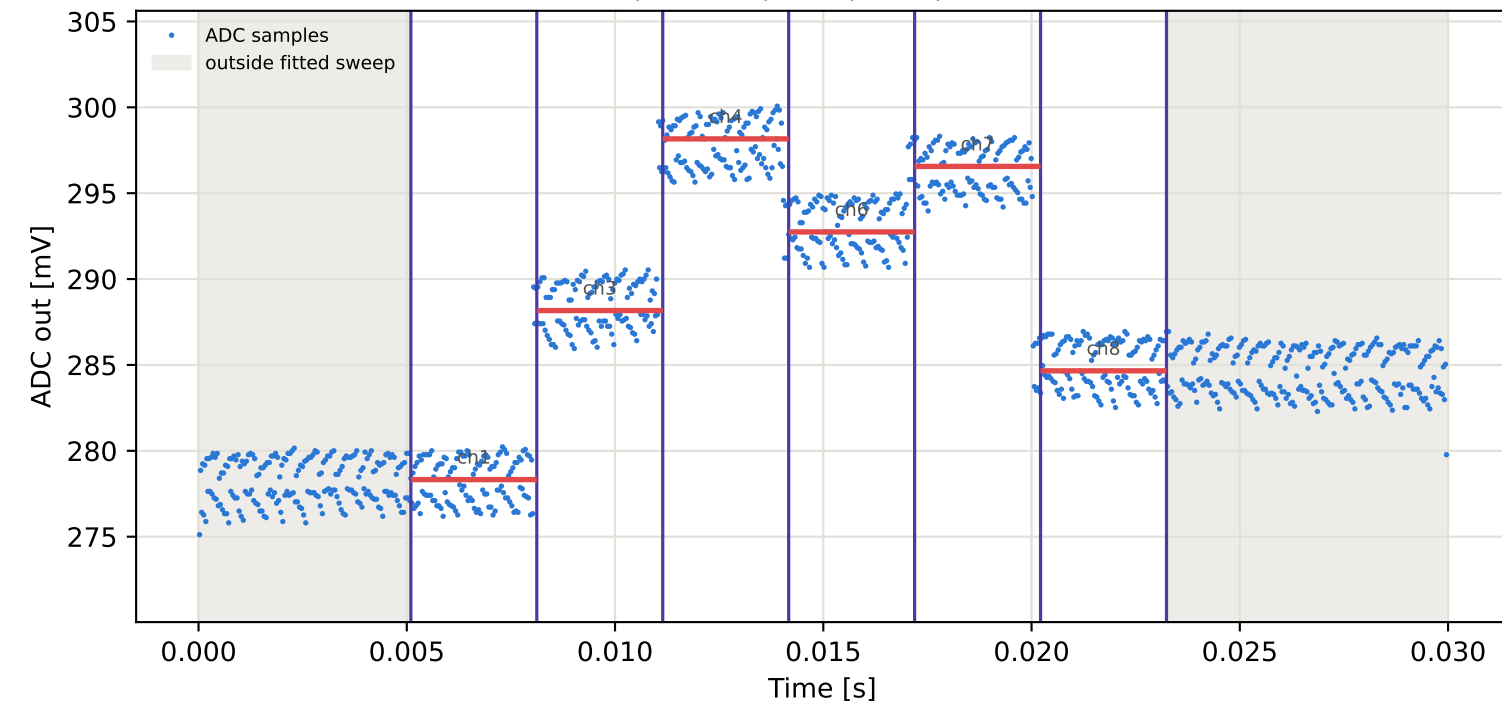
Tag4 &lt;- Tag9 | 865 MHz | run 0 | rep 1 | phase -101.57 deg
