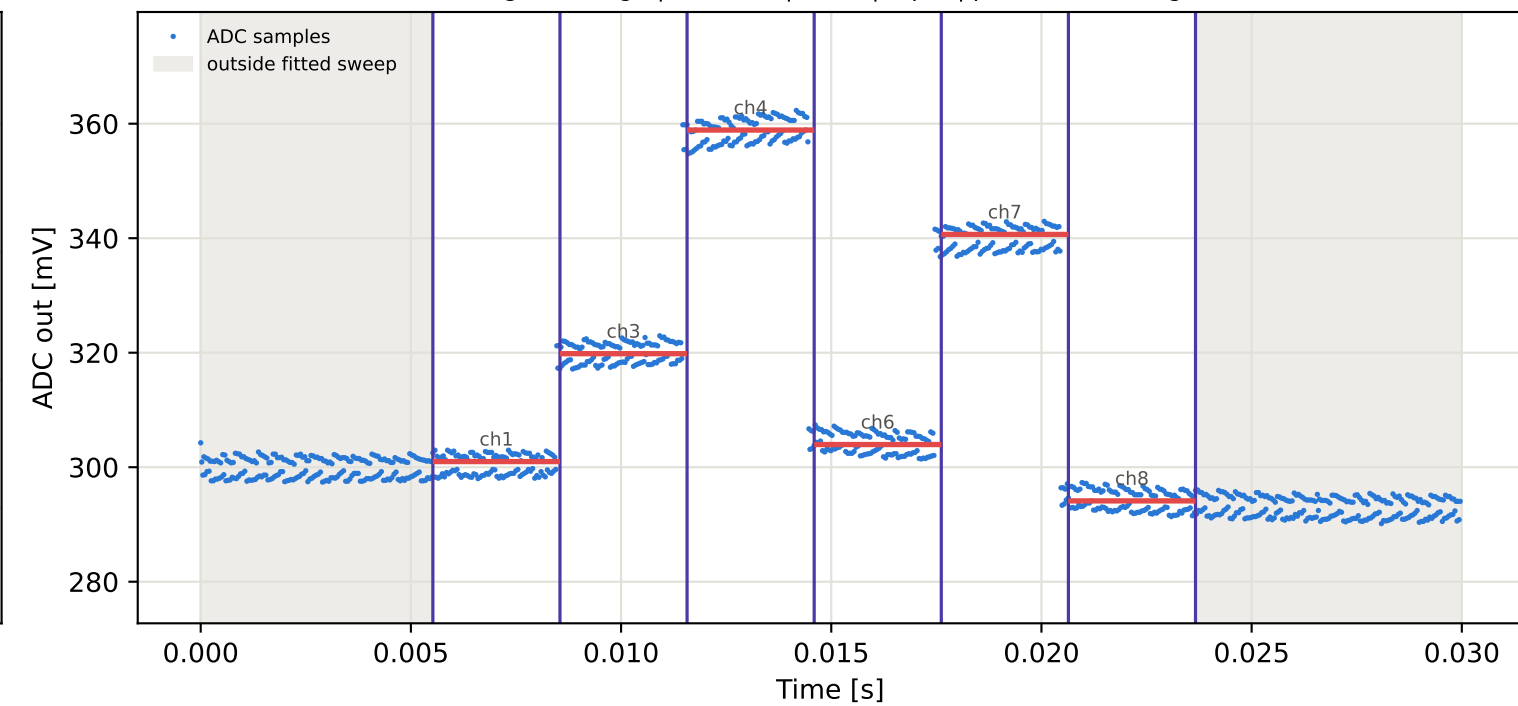
Tag10 &lt;- Tag9 | 965 MHz | run 0 | rep 1 | phase 124.25 deg
