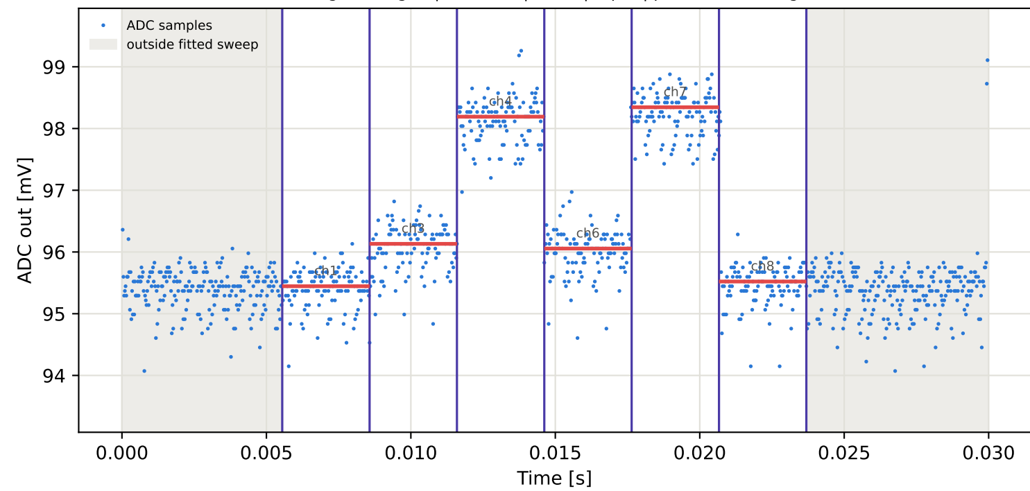
Tag5 &lt;- Tag2 | 775 MHz | run 0 | rep 1 | phase -153.68 deg
