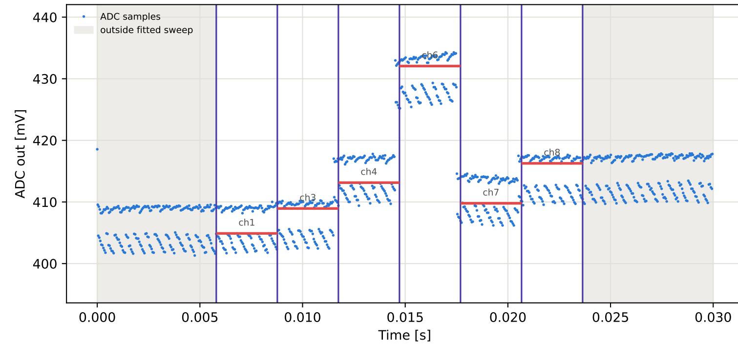
Tag6 &lt;- Tag1 | 925 MHz | run 0 | rep 1 | phase 80.84 deg
