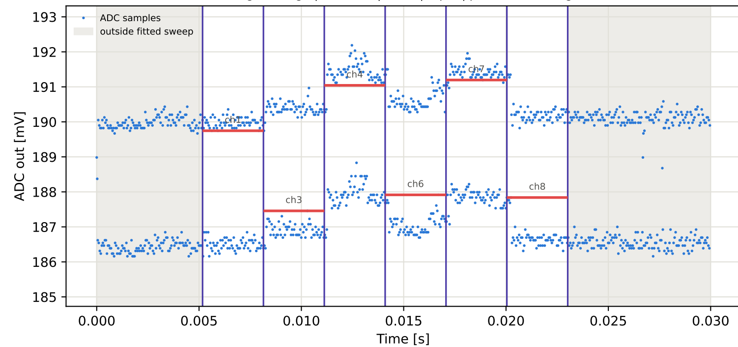
Tag3 &lt;- Tag15 | 805 MHz | run 0 | rep 1 | phase -115.60 deg
