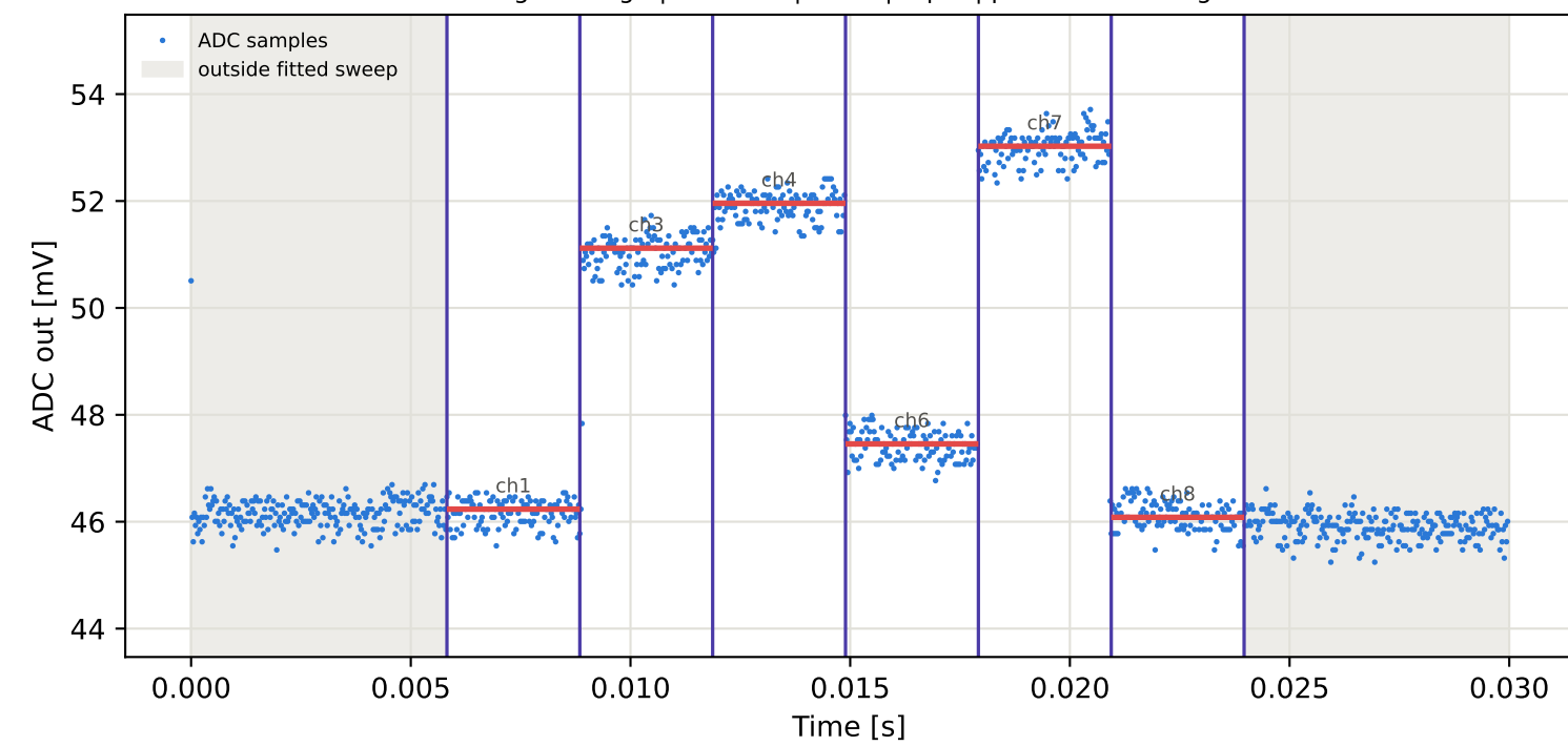
Tag5 &lt;- Tag9 | 785 MHz | run 0 | rep 1 | phase -125.28 deg
