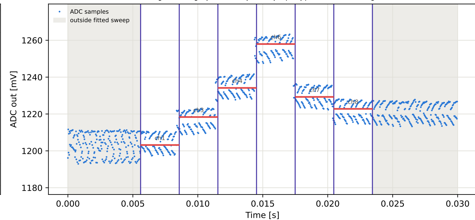
Tag10 &lt;- Tag5 | 895 MHz | run 0 | rep 1 | phase -139.88 deg
