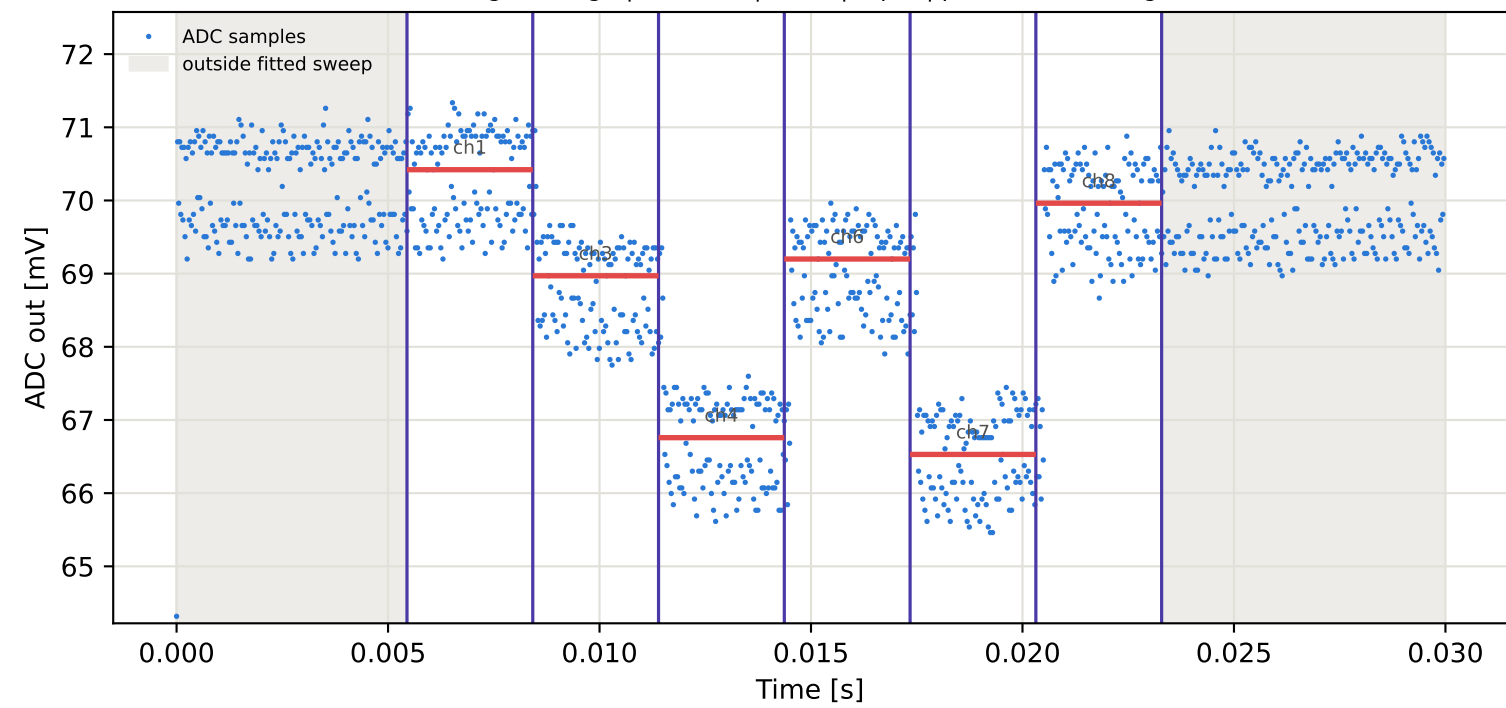
Tag1 &lt;- Tag8 | 785 MHz | run 0 | rep 1 | phase -176.32 deg
