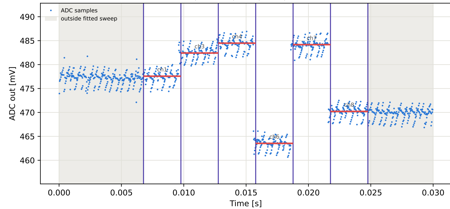
Tag10 &lt;- Tag4 | 955 MHz | run 0 | rep 1 | phase -22.14 deg
