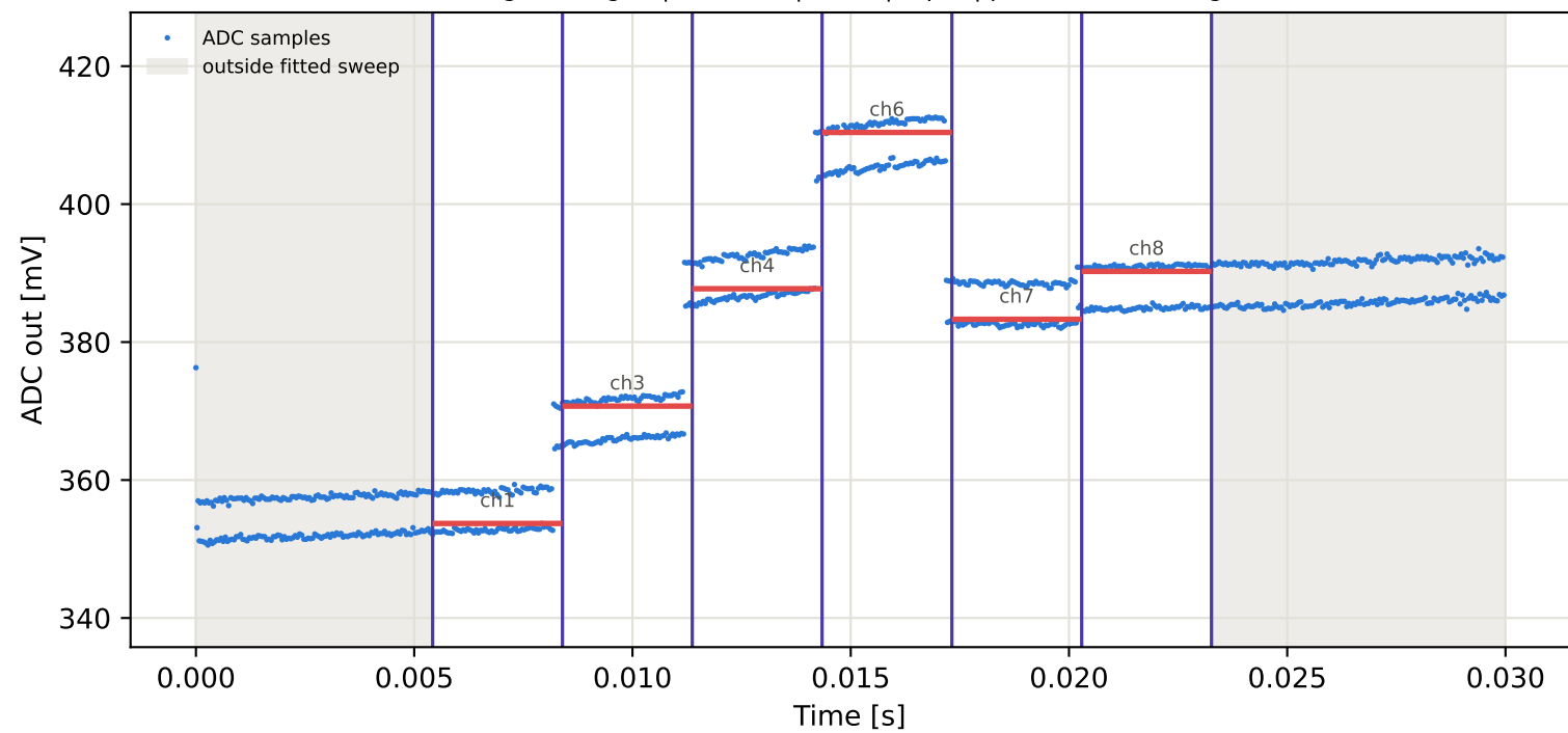
Tag4 &lt;- Tag16 | 875 MHz | run 0 | rep 1 | phase -122.41 deg
