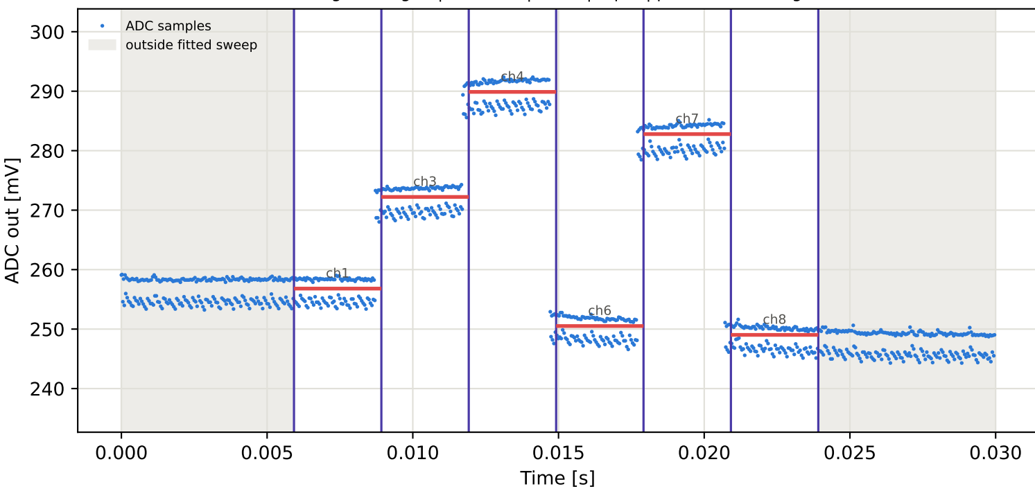
Tag3 &lt;- Tag16 | 995 MHz | run 0 | rep 1 | phase -69.30 deg
