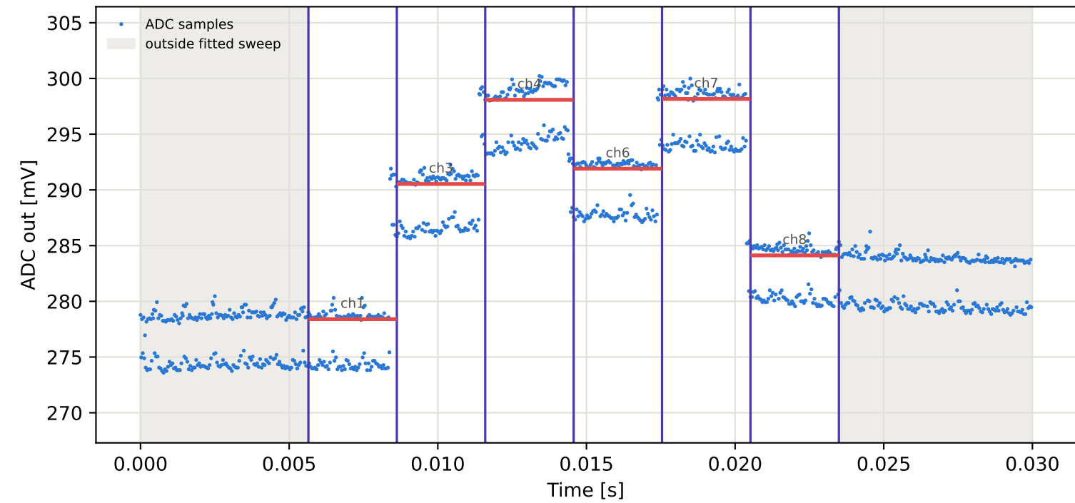
Tag2 &lt;- Tag8 | 845 MHz | run 0 | rep 1 | phase -115.58 deg
