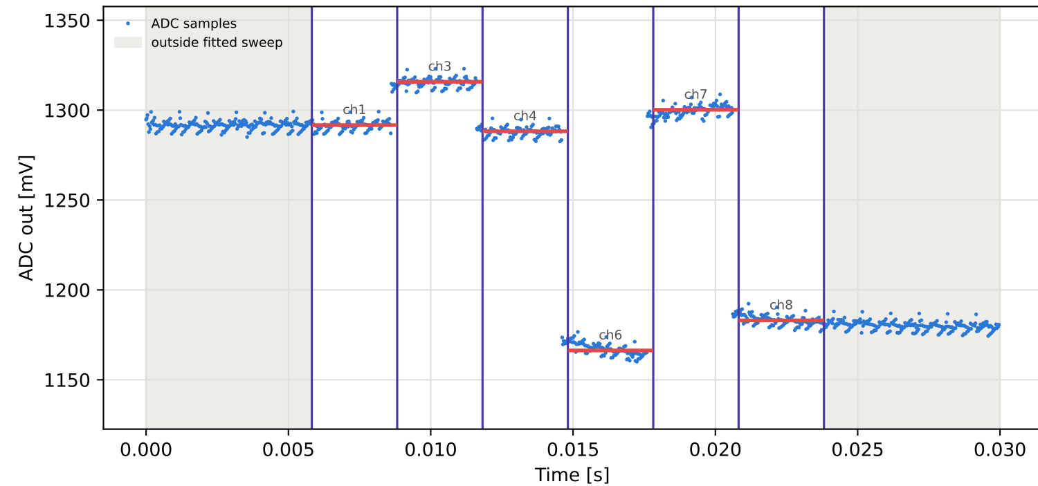
Tag10 &lt;- Tag5 | 885 MHz | run 0 | rep 1 | phase -173.54 deg
