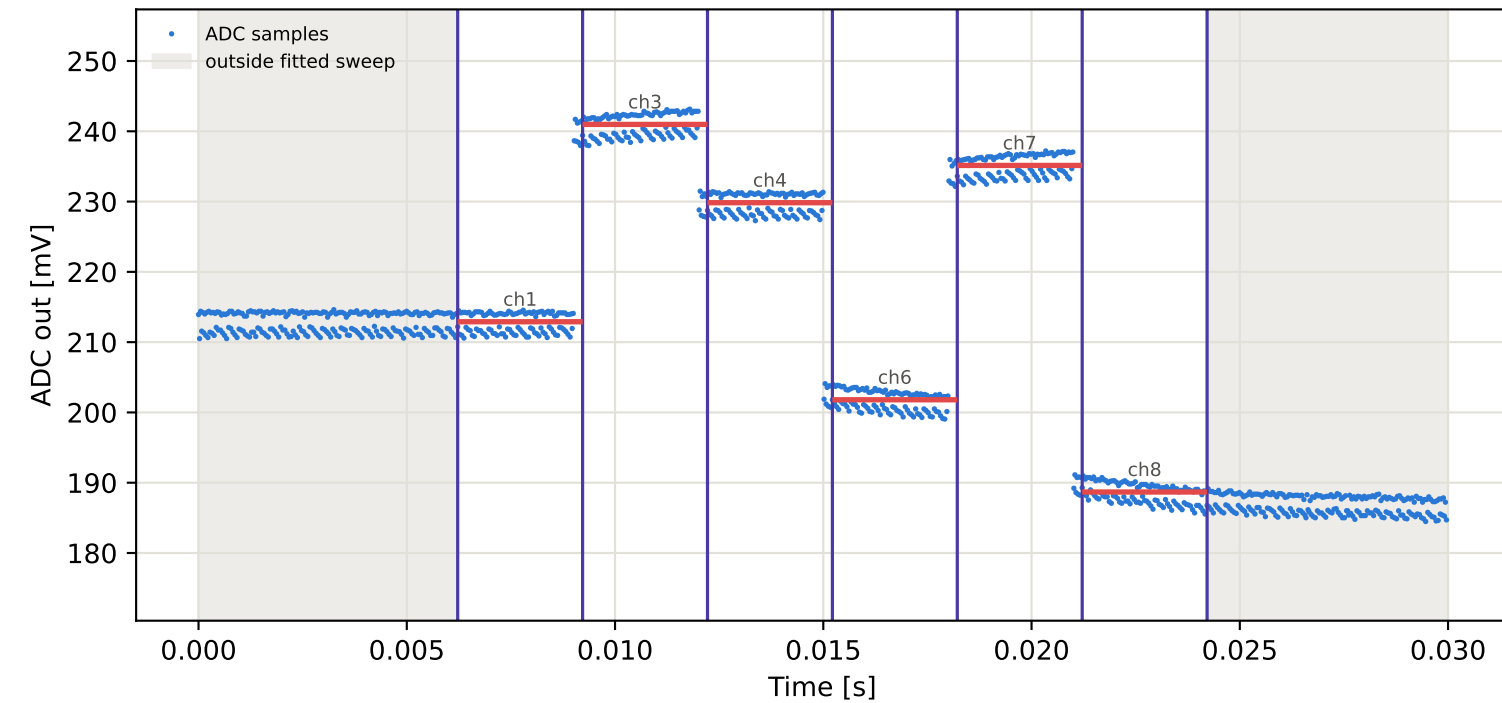
Tag1 &lt;- Tag3 | 865 MHz | run 0 | rep 1 | phase -168.15 deg
