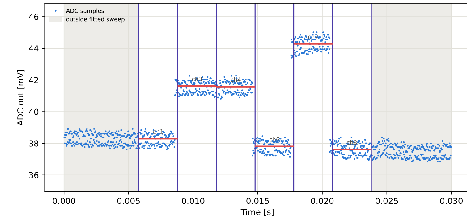
Tag16 &lt;- Tag10 | 775 MHz | run 0 | rep 1 | phase -30.41 deg
