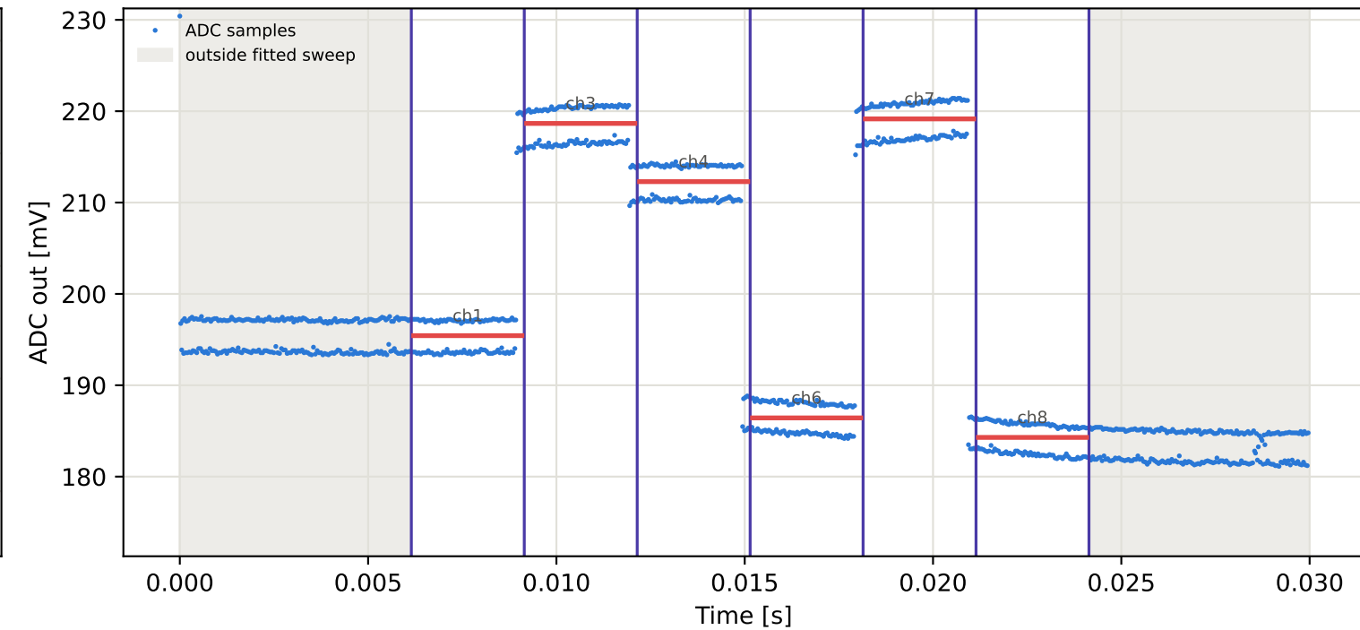
Tag15 &lt;- Tag10 | 805 MHz | run 0 | rep 1 | phase -75.78 deg
