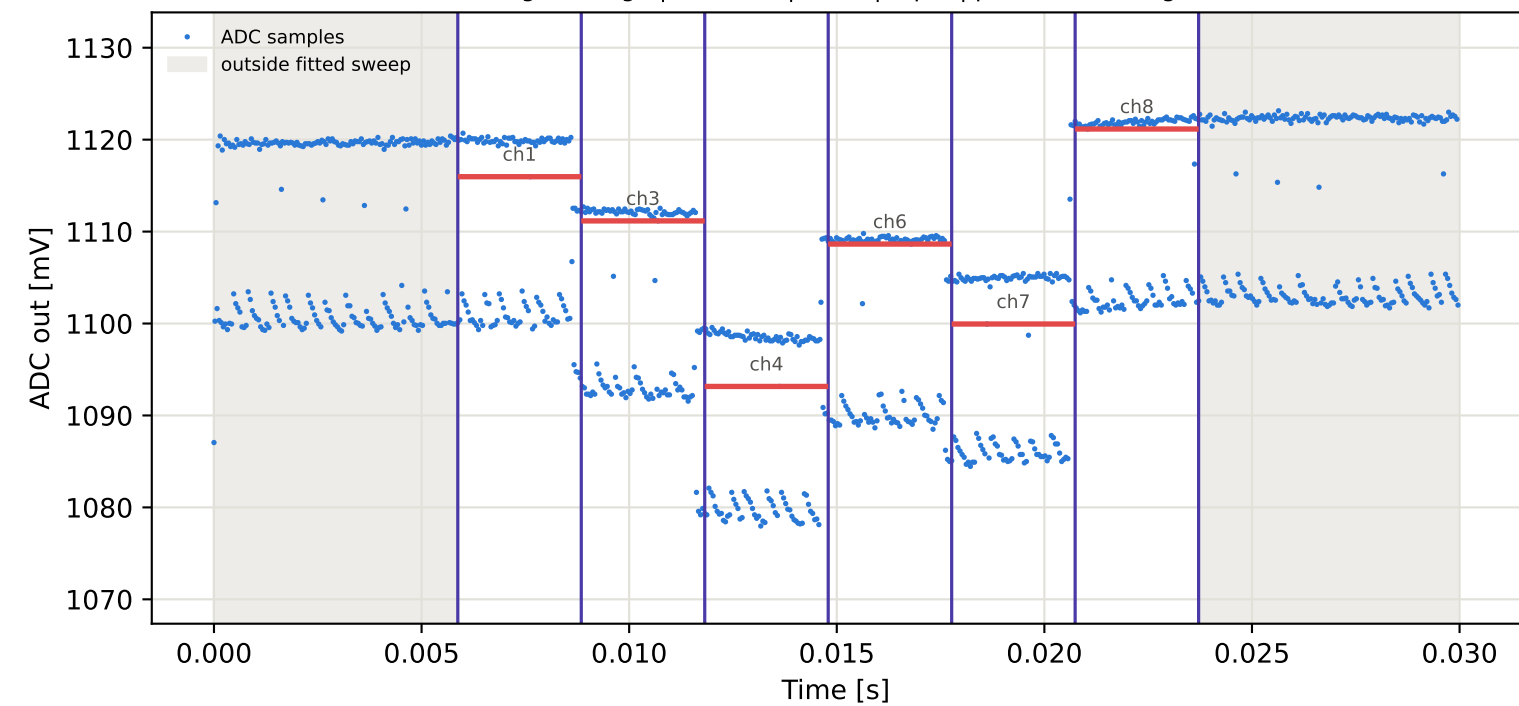
Tag9 &lt;- Tag8 | 935 MHz | run 0 | rep 1 | phase 145.96 deg
