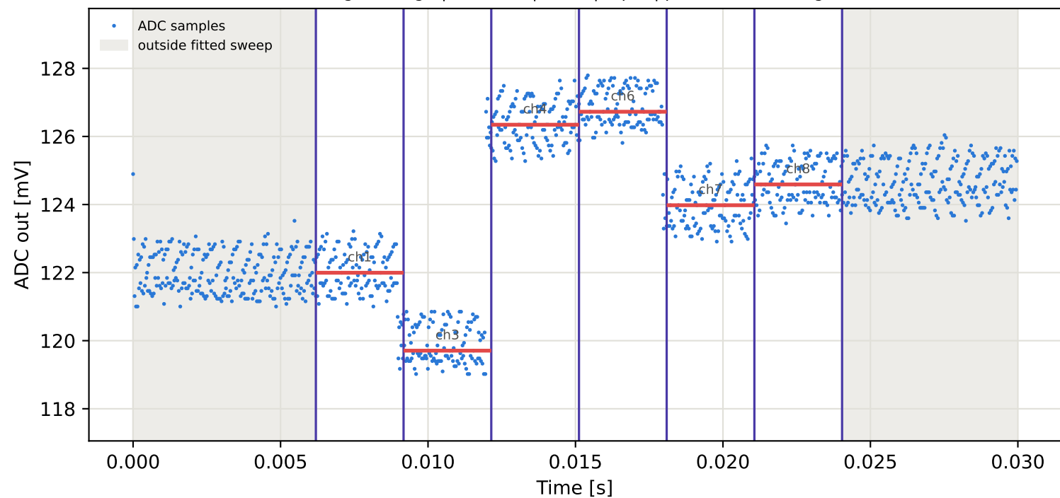
Tag4 &lt;- Tag7 | 785 MHz | run 0 | rep 1 | phase 155.40 deg
