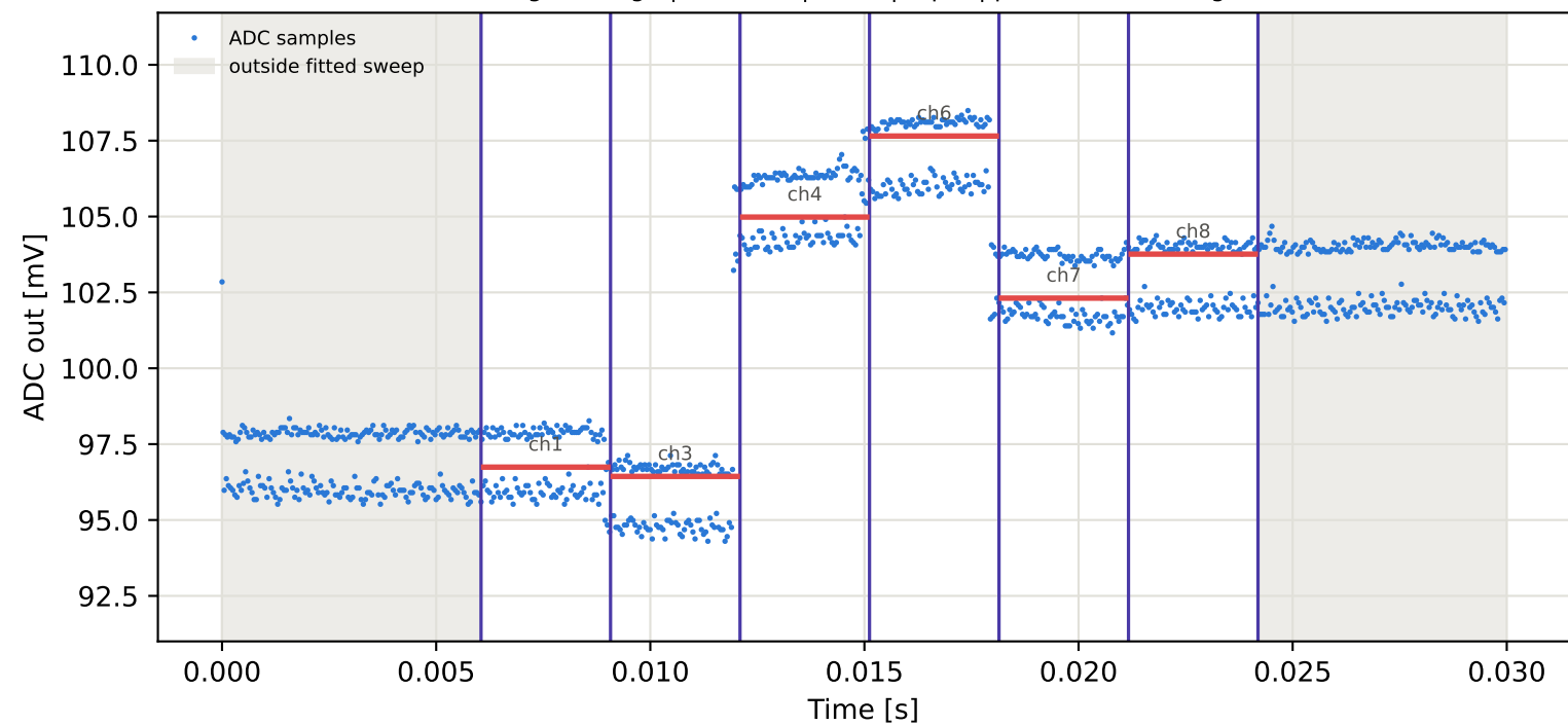
Tag1 &lt;- Tag9 | 795 MHz | run 0 | rep 1 | phase 157.06 deg
