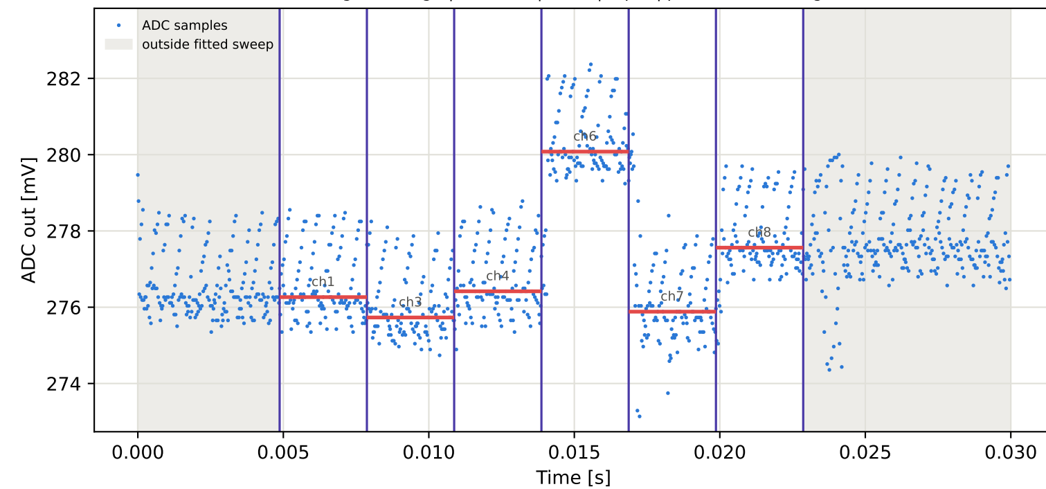
Tag16 &lt;- Tag4 | 985 MHz | run 0 | rep 1 | phase -54.28 deg
