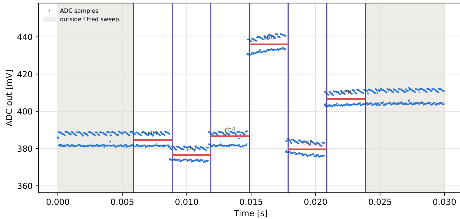
Tag15 &lt;- Tag9 | 935 MHz | run 0 | rep 1 | phase 63.27 deg
