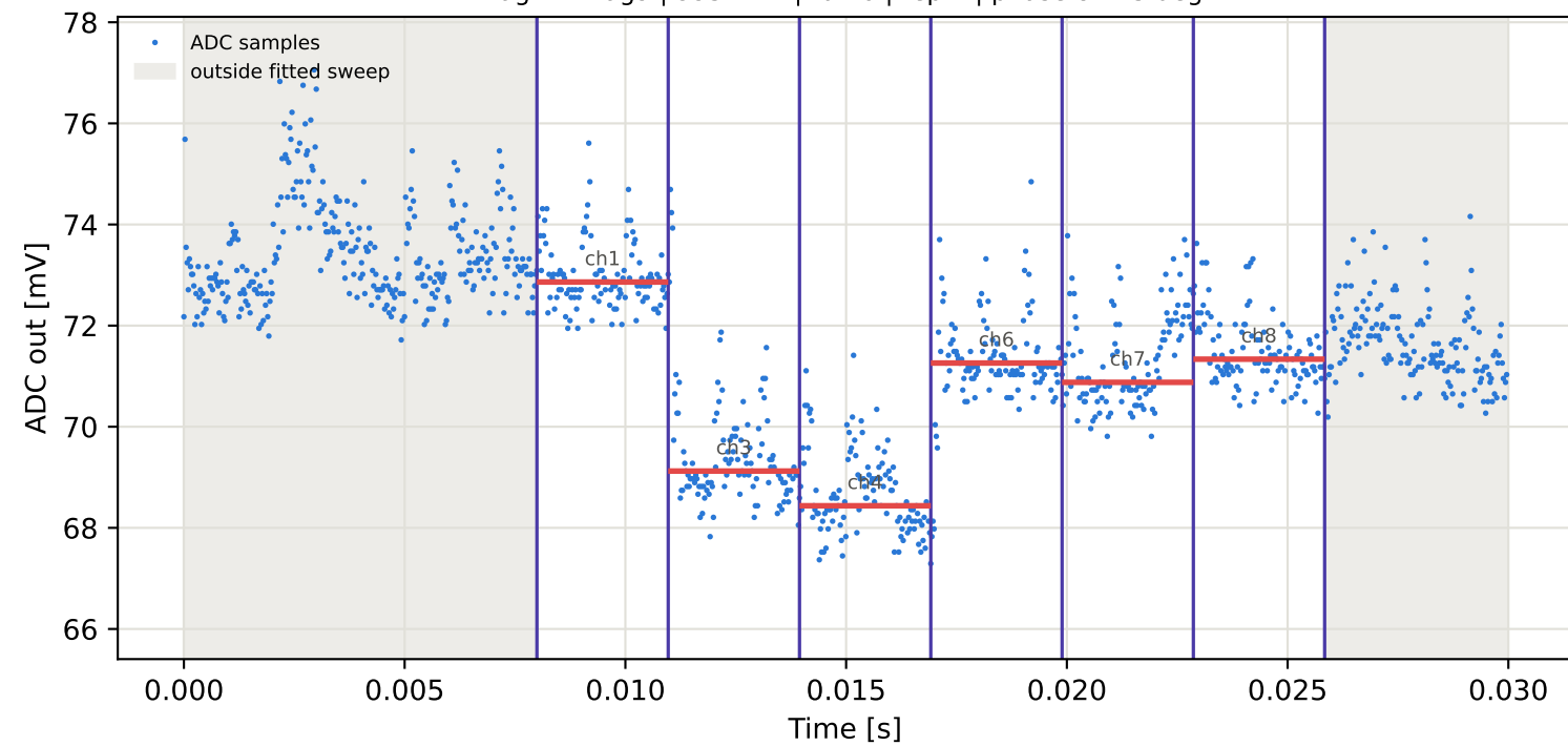
Tag3 &lt;- Tag10 | 995 MHz | run 0 | rep 1 | phase 118.88 deg
