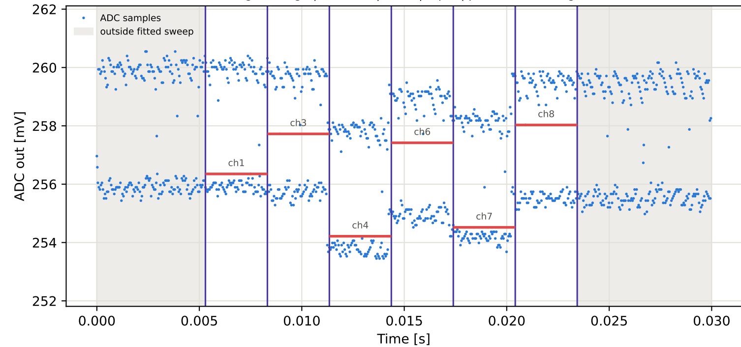
Tag9 &lt;- Tag15 | 805 MHz | run 0 | rep 1 | phase 116.27 deg
