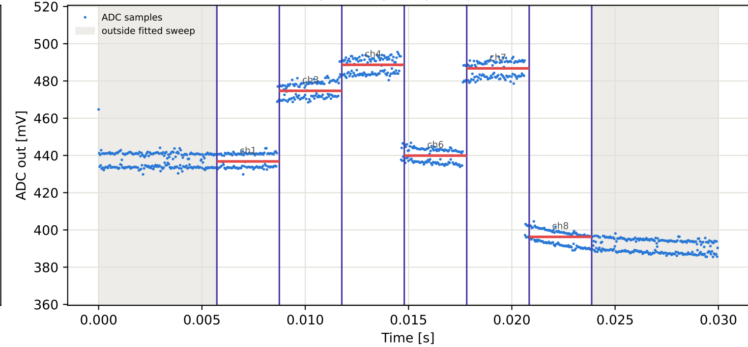
Tag4 &lt;- Tag3 | 885 MHz | run 0 | rep 1 | phase -59.66 deg
