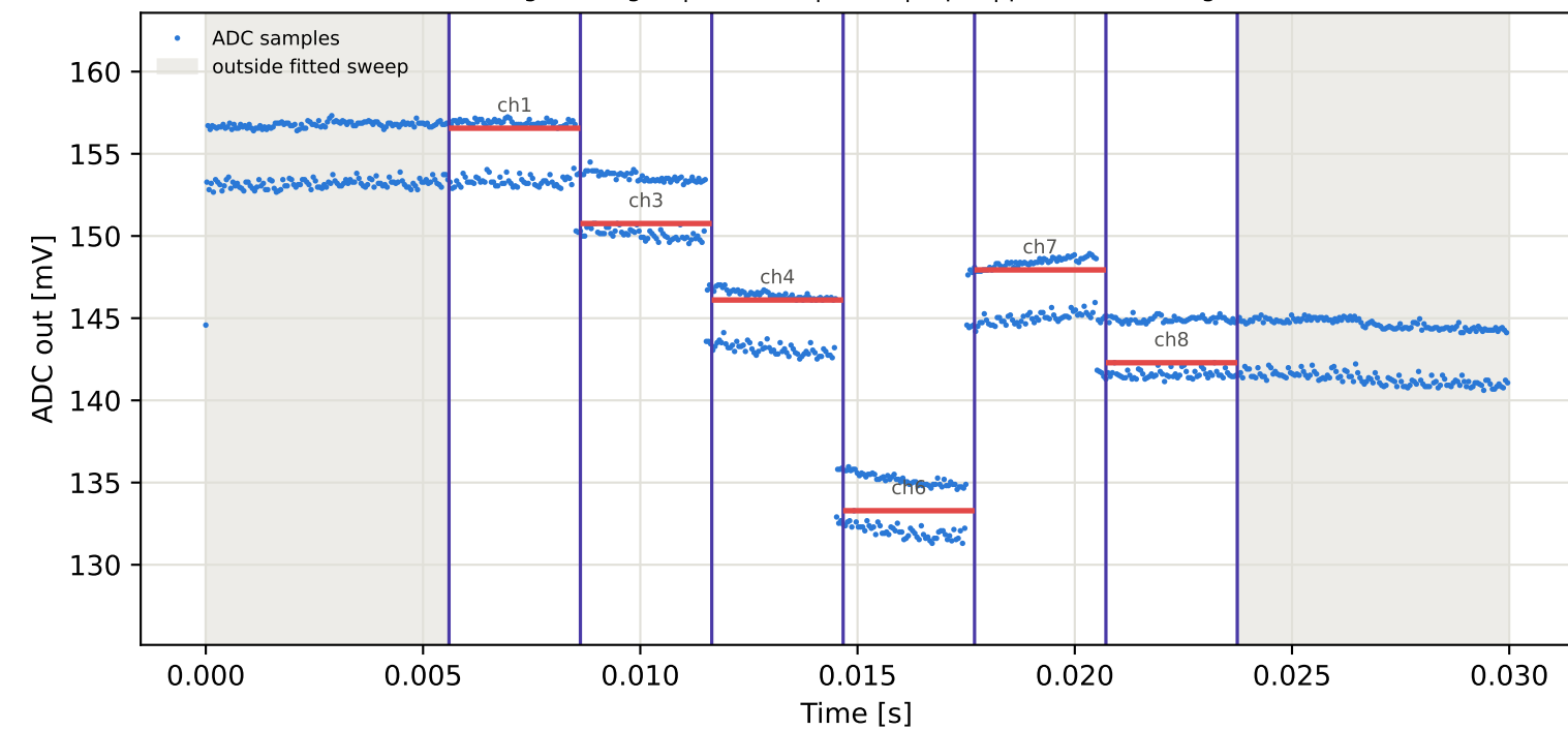
Tag1 &lt;- Tag3 | 895 MHz | run 0 | rep 1 | phase -176.18 deg
