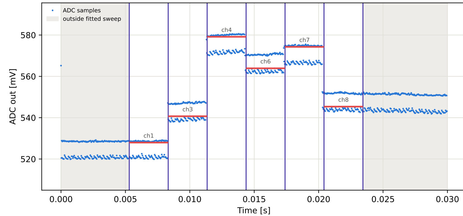
Tag3 &lt;- Tag8 | 835 MHz | run 0 | rep 1 | phase 71.14 deg
