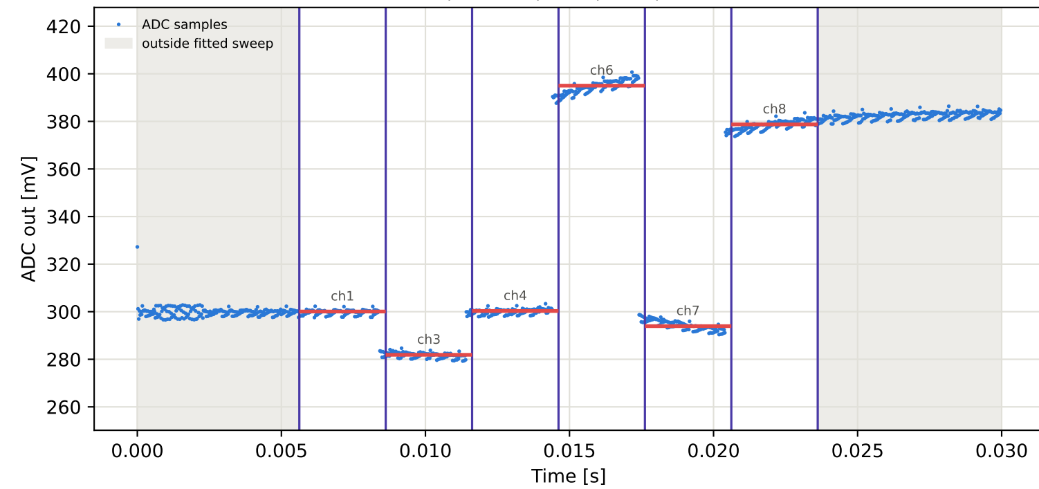
Tag15 &lt;- Tag5 | 895 MHz | run 0 | rep 1 | phase 179.04 deg
