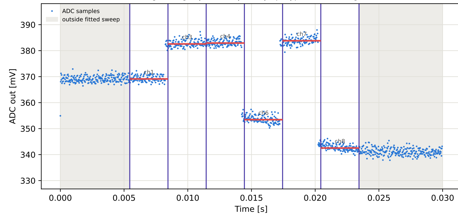
Tag1 &lt;- Tag16 | 885 MHz | run 0 | rep 1 | phase 14.98 deg
