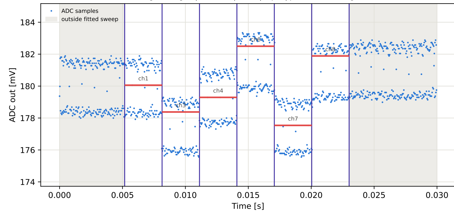
Tag7 &lt;- Tag3 | 775 MHz | run 0 | rep 1 | phase 93.51 deg
