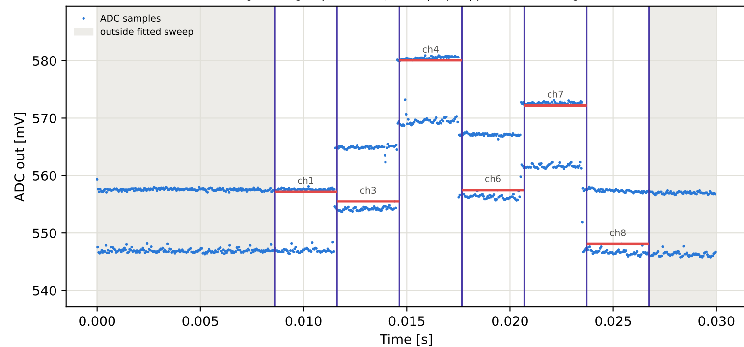
Tag8 &lt;- Tag16 | 955 MHz | run 0 | rep 1 | phase -93.44 deg
