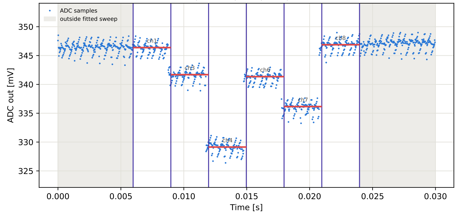
Tag10 &lt;- Tag5 | 975 MHz | run 0 | rep 1 | phase 76.27 deg
