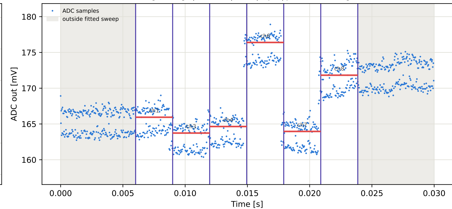
Tag2 &lt;- Tag6 | 925 MHz | run 0 | rep 1 | phase -170.80 deg
