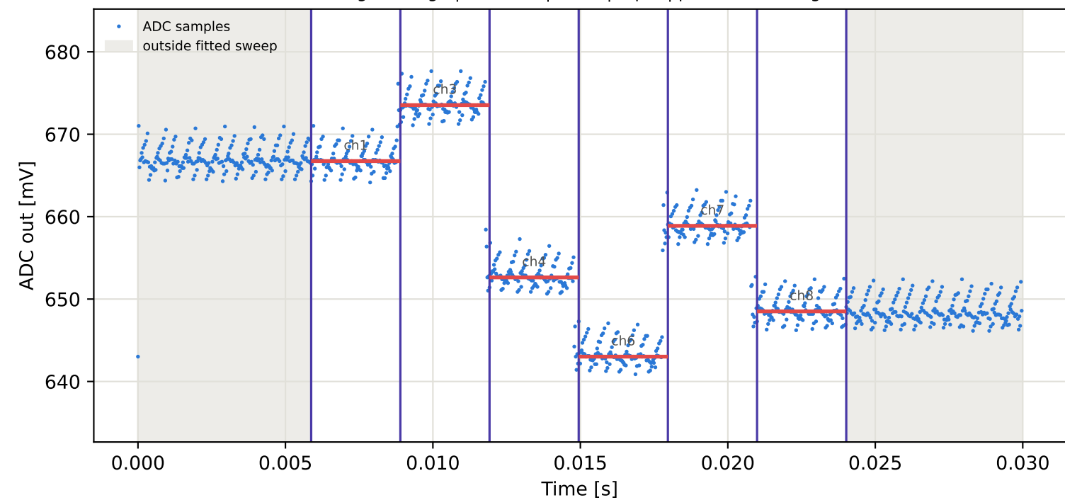
Tag9 &lt;- Tag8 | 835 MHz | run 0 | rep 1 | phase 34.82 deg
