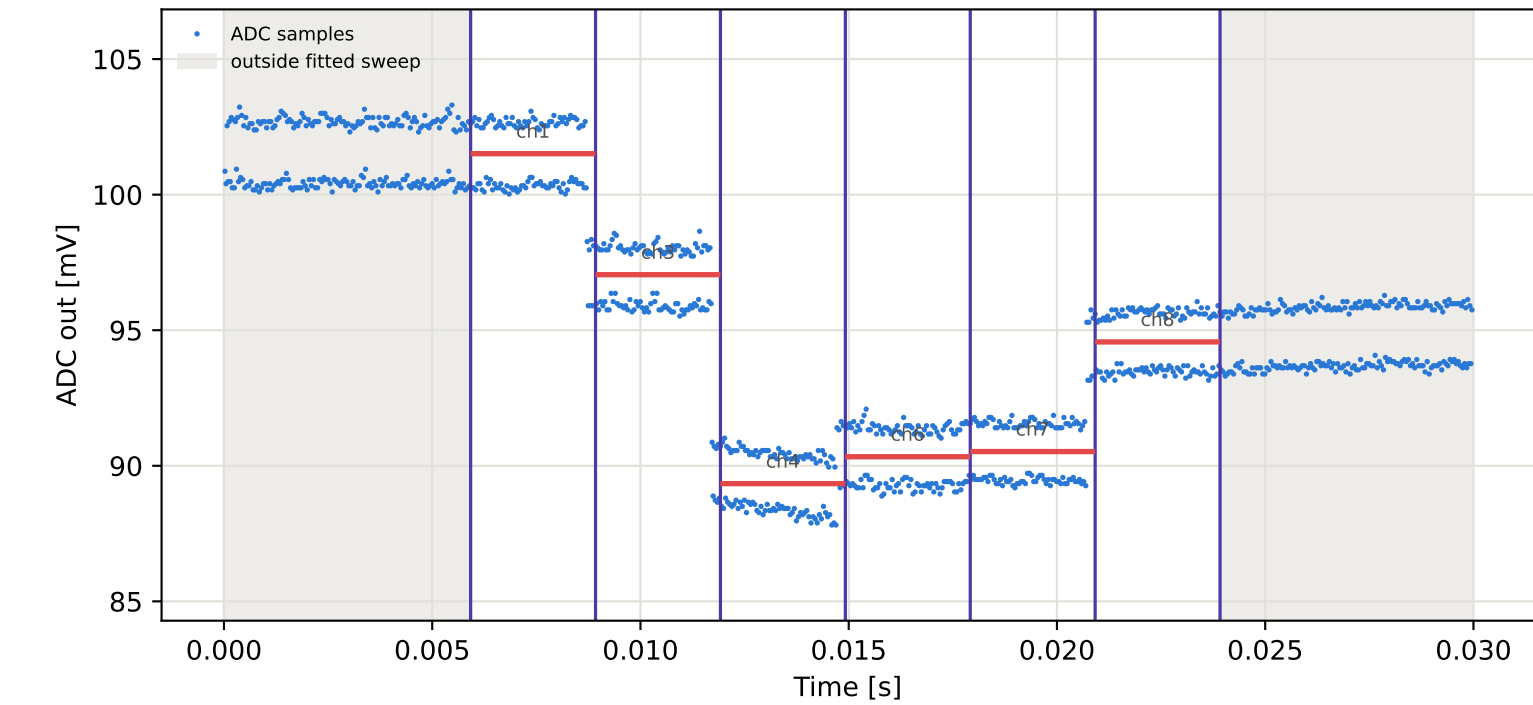
Tag4 &lt;- Tag2 | 855 MHz | run 0 | rep 1 | phase -85.17 deg
