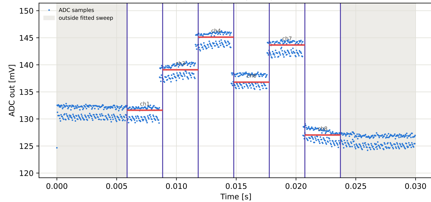
Tag1 &lt;- Tag9 | 905 MHz | run 0 | rep 1 | phase -81.03 deg
