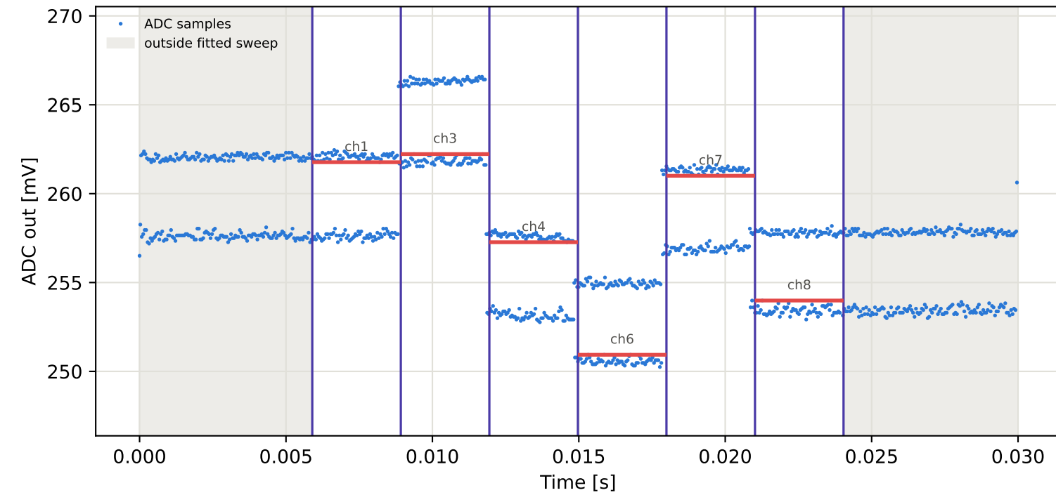
Tag9 &lt;- Tag7 | 805 MHz | run 0 | rep 1 | phase -51.85 deg
