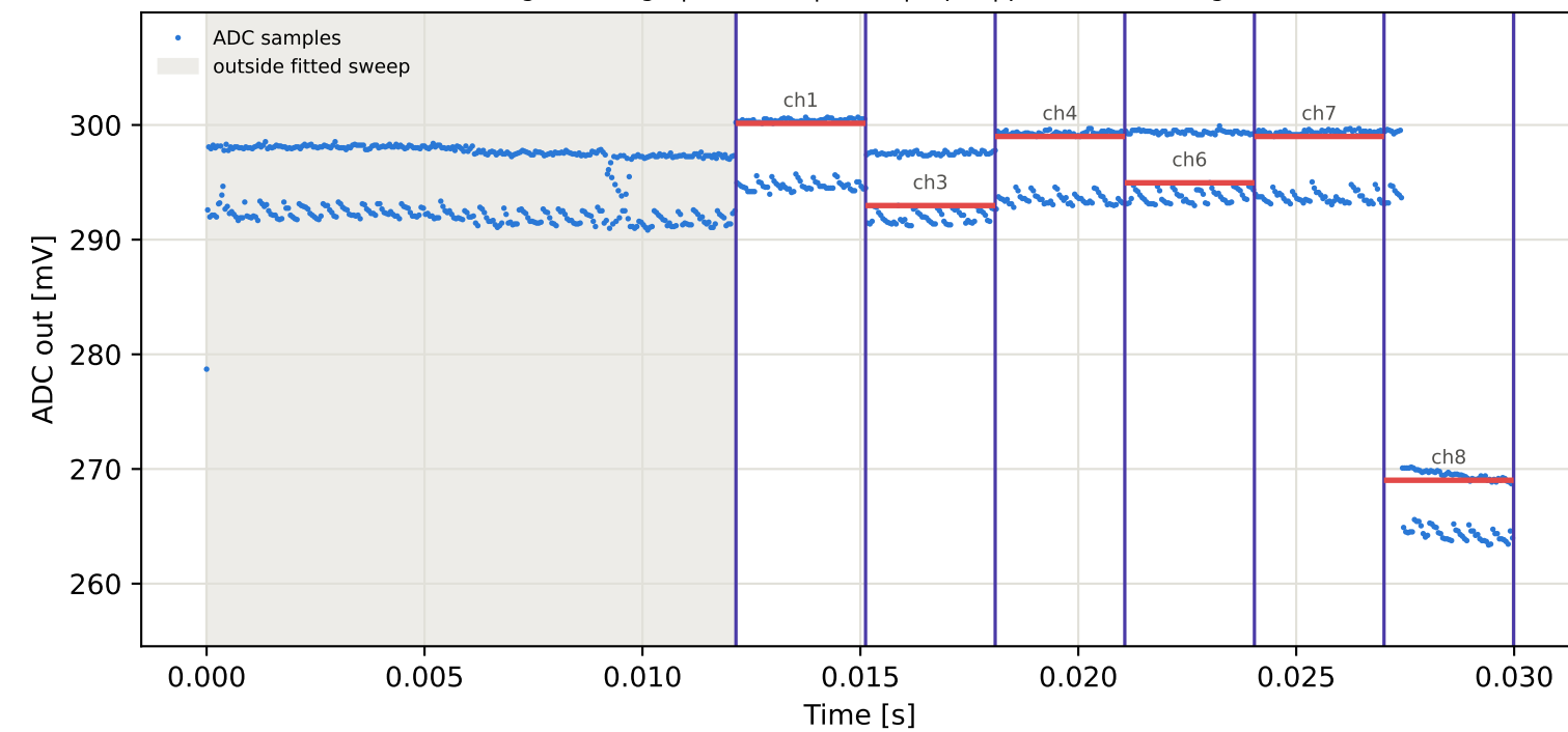
Tag16 &lt;- Tag4 | 955 MHz | run 0 | rep 1 | phase -149.28 deg
