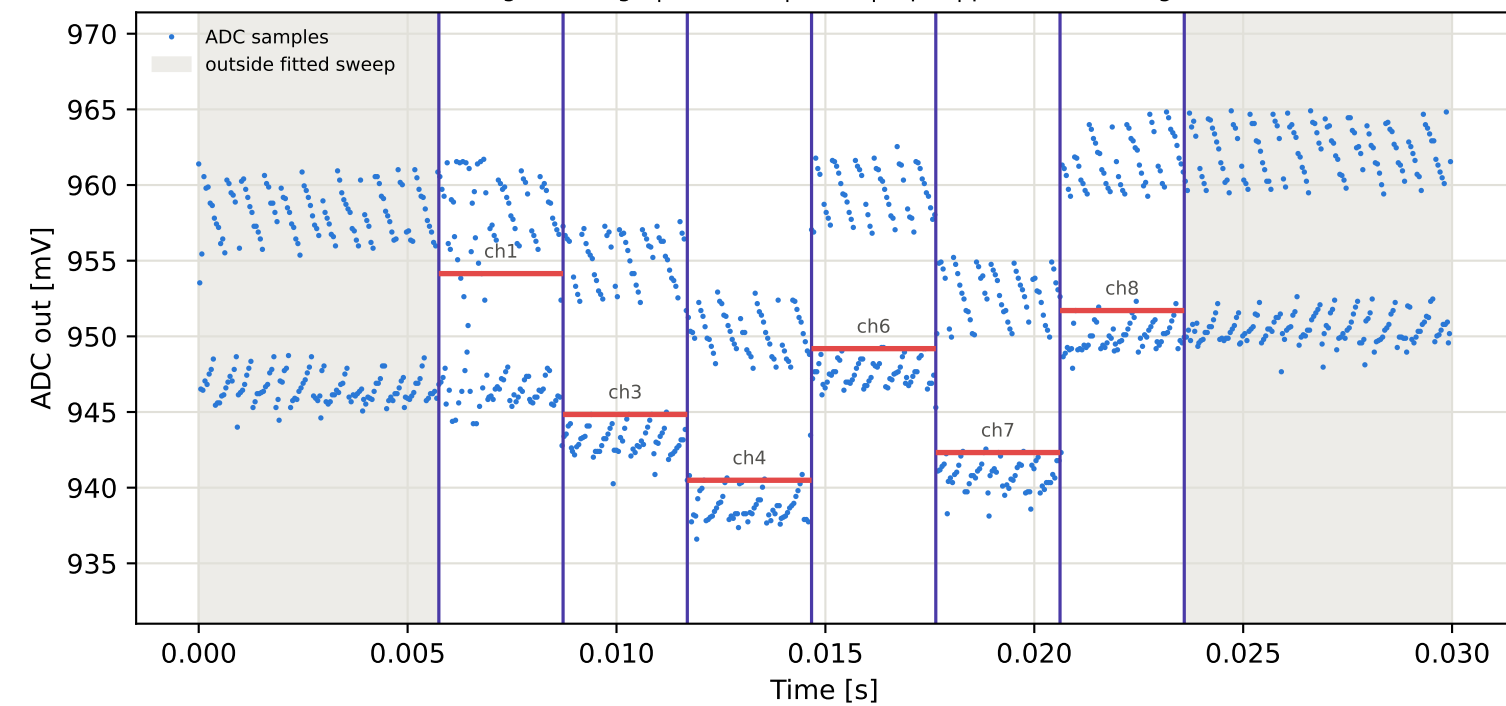
Tag10 &lt;- Tag4 | 935 MHz | run 0 | rep 1 | phase -32.84 deg
