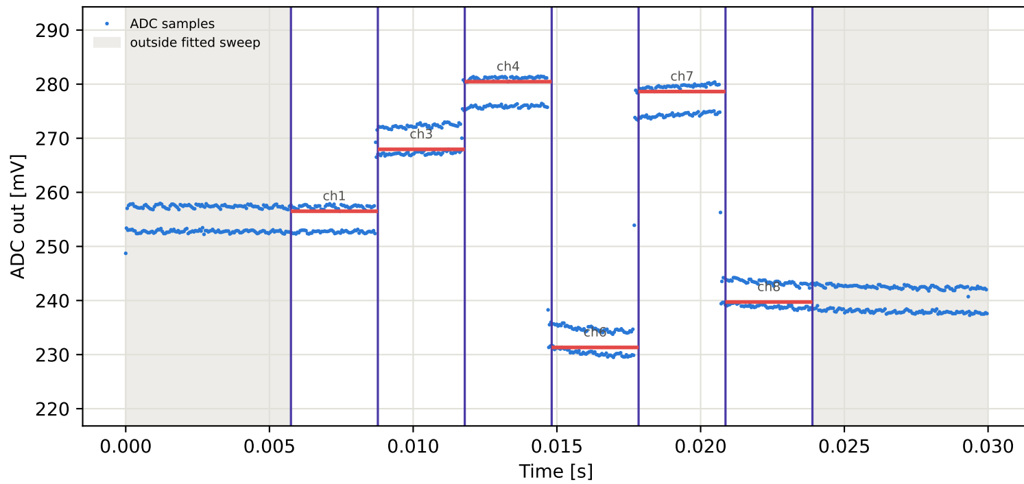
Tag2 &lt;- Tag1 | 995 MHz | run 0 | rep 1 | phase -155.00 deg
