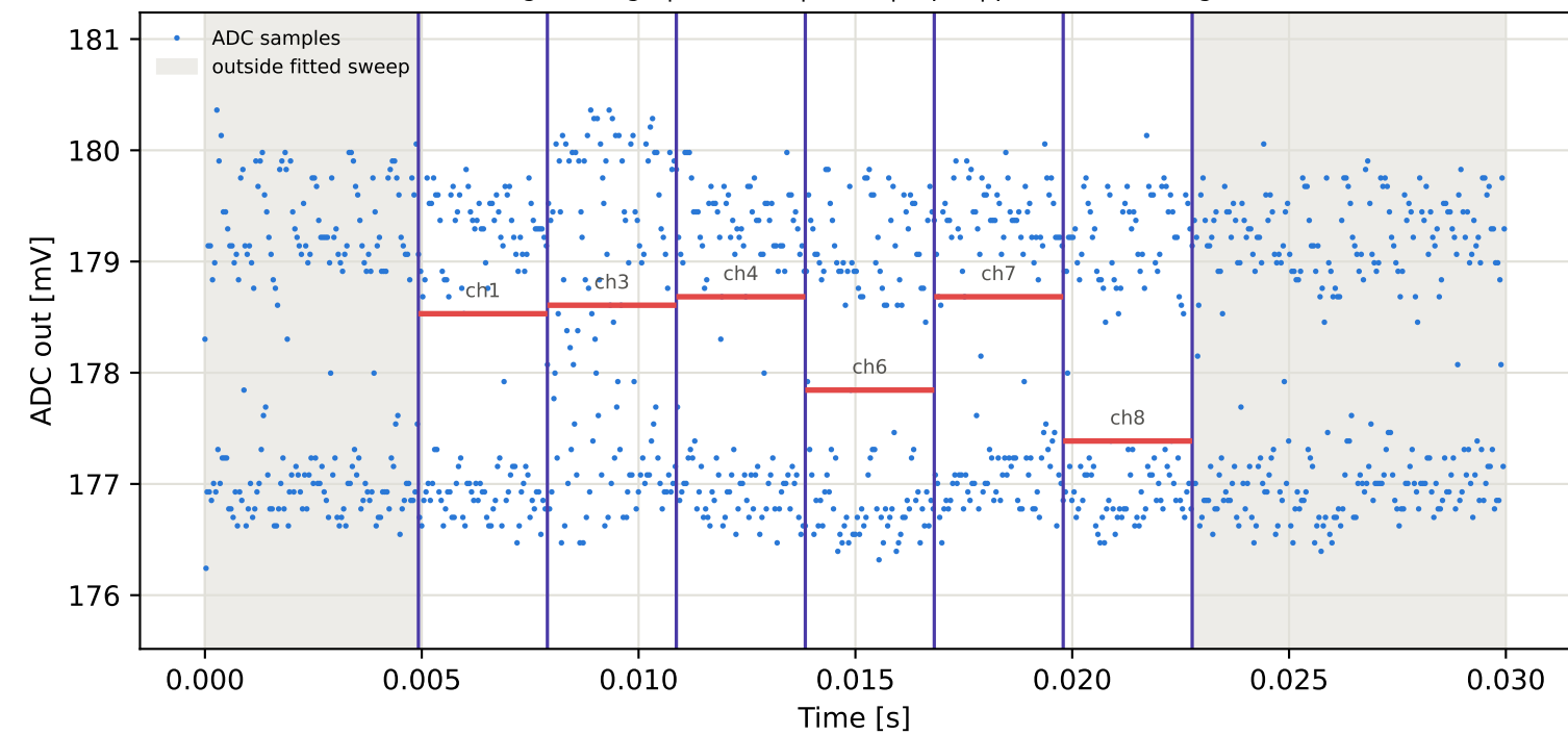
Tag9 &lt;- Tag15 | 775 MHz | run 0 | rep 1 | phase 28.94 deg
