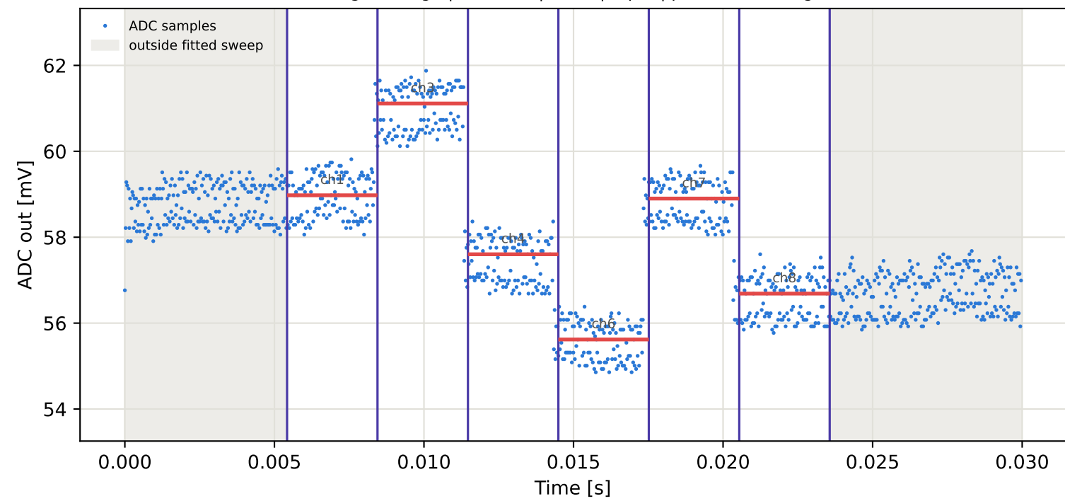
Tag1 &lt;- Tag8 | 805 MHz | run 0 | rep 1 | phase -111.24 deg
