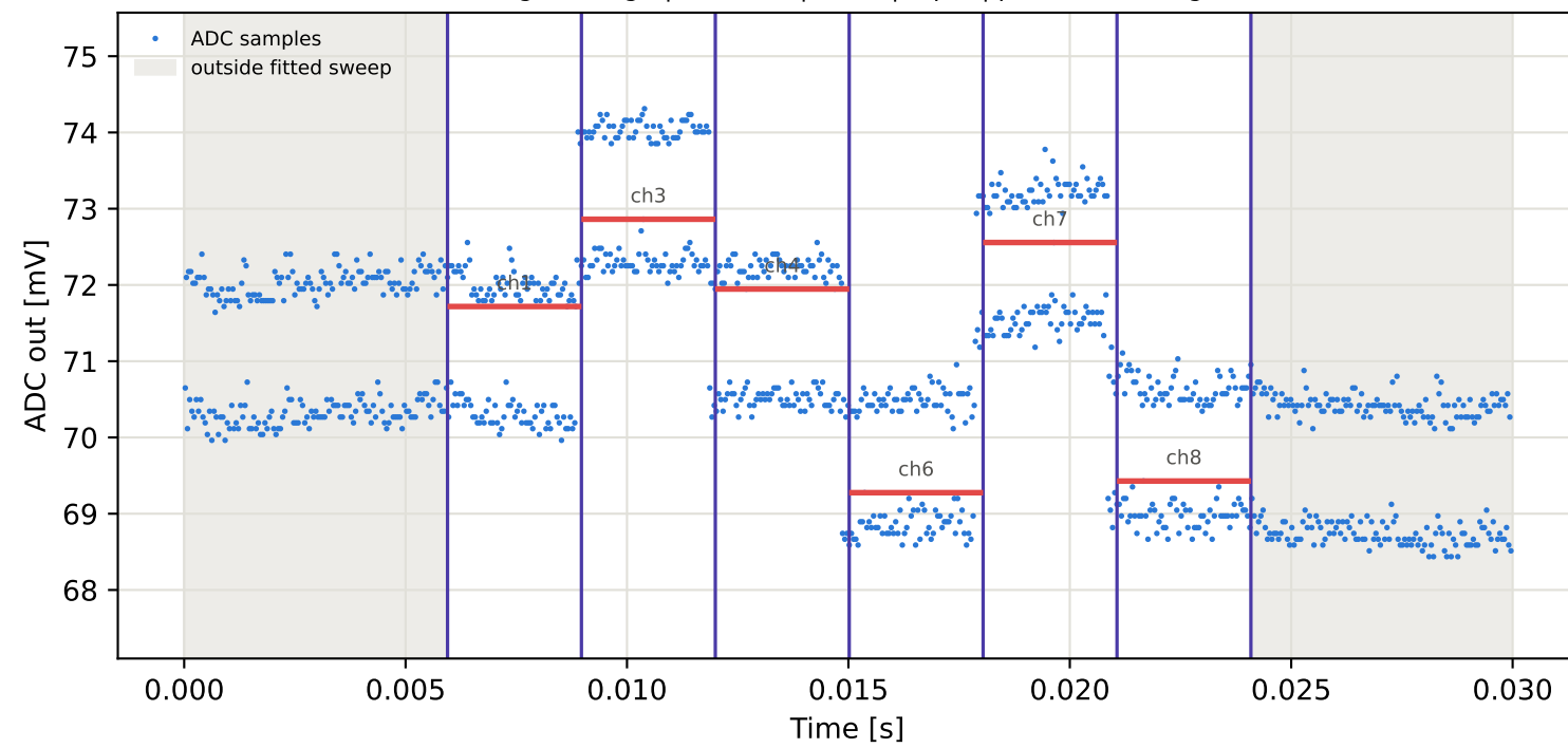
Tag1 &lt;- Tag7 | 835 MHz | run 0 | rep 1 | phase 65.30 deg
