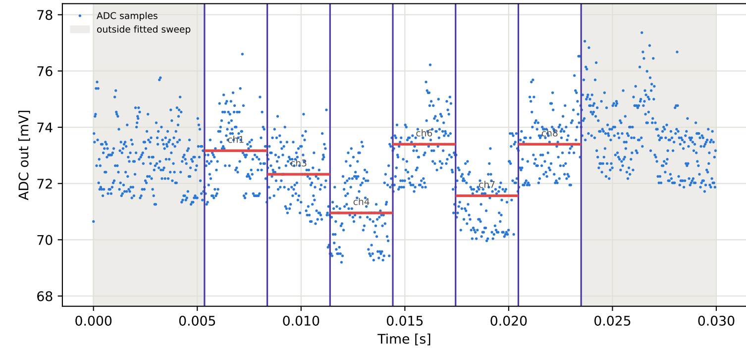
Tag2 &lt;- Tag16 | 995 MHz | run 0 | rep 1 | phase -43.80 deg
