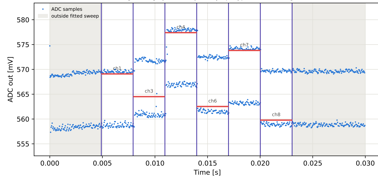
Tag3 &lt;- Tag6 | 975 MHz | run 0 | rep 1 | phase 146.18 deg
