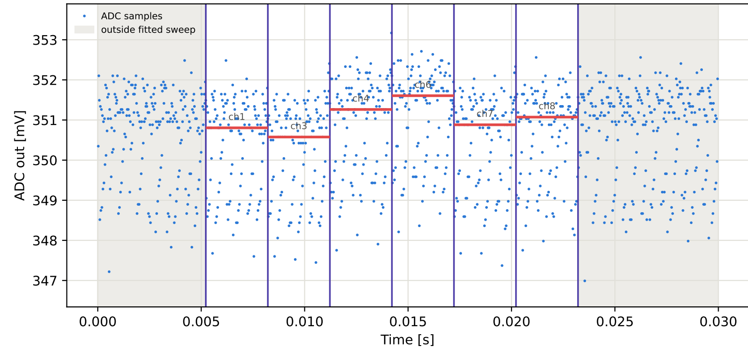
Tag15 &lt;- Tag6 | 985 MHz | run 0 | rep 1 | phase -155.82 deg
