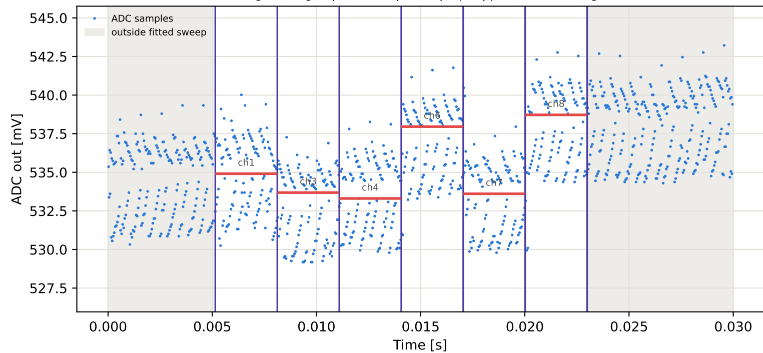
Tag4 &lt;- Tag2 | 895 MHz | run 0 | rep 1 | phase -174.73 deg
