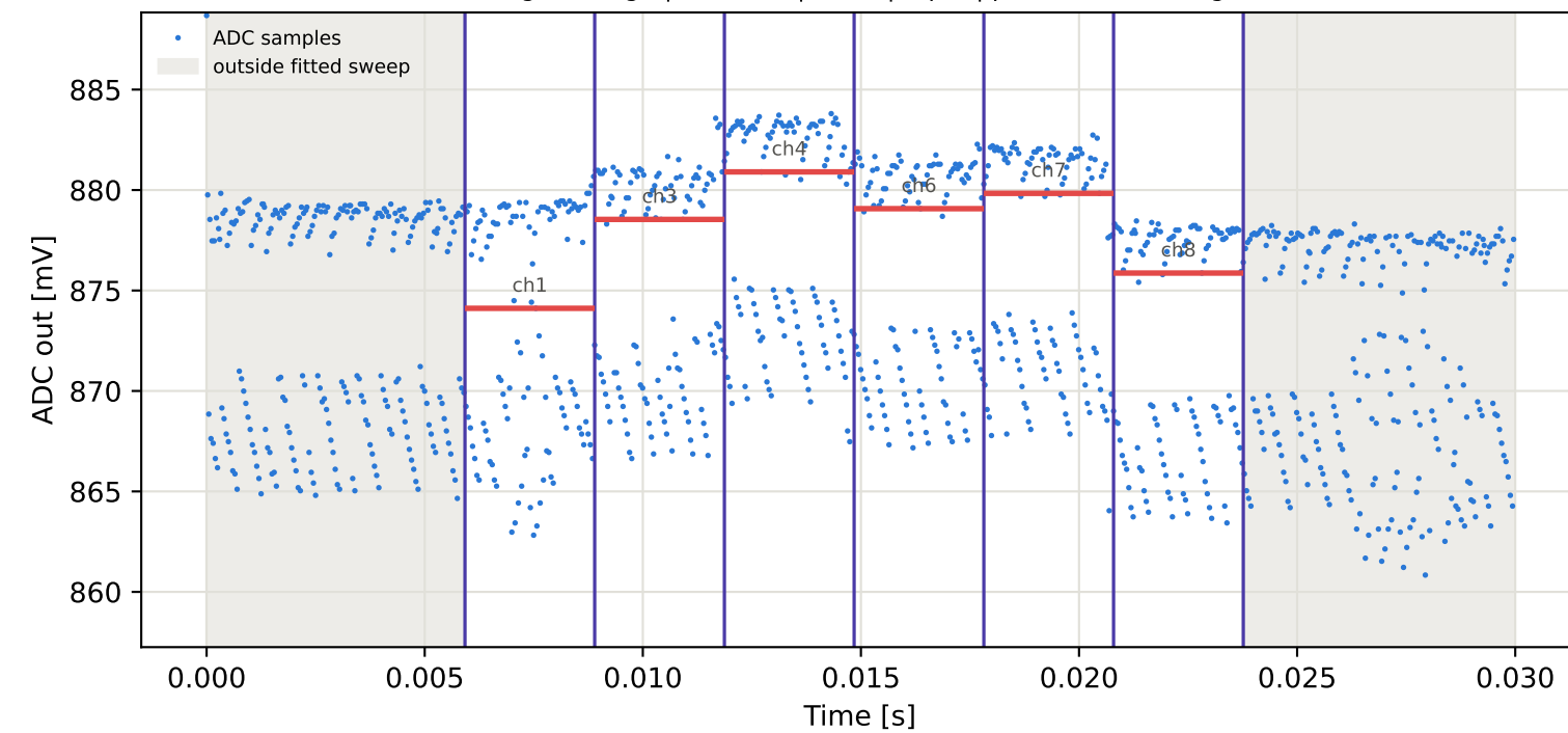
Tag8 &lt;- Tag4 | 935 MHz | run 0 | rep 1 | phase -153.75 deg
