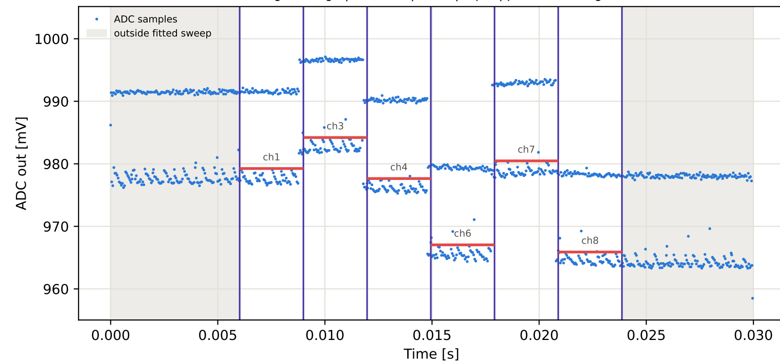
Tag7 &lt;- Tag5 | 865 MHz | run 0 | rep 1 | phase 4.99 deg
