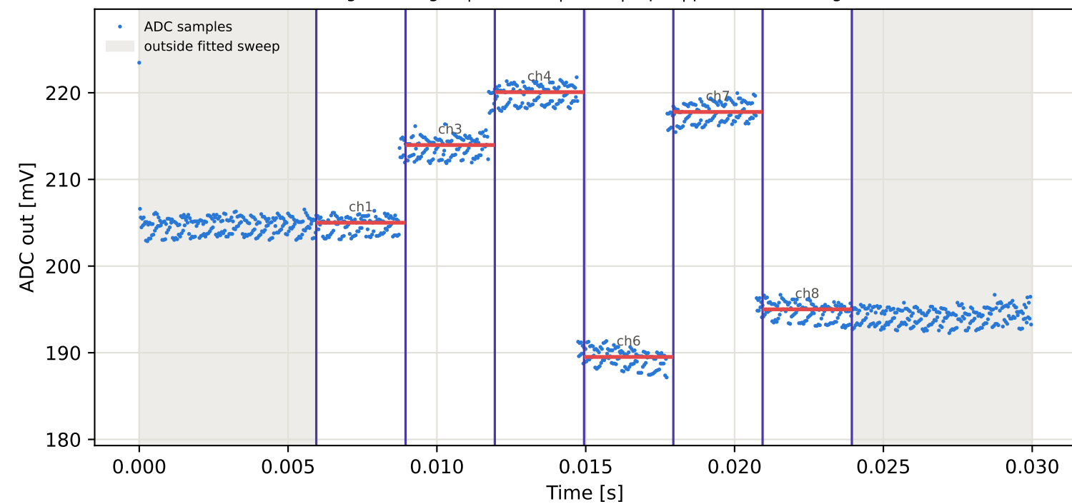
Tag15 &lt;- Tag10 | 955 MHz | run 0 | rep 1 | phase -34.84 deg
