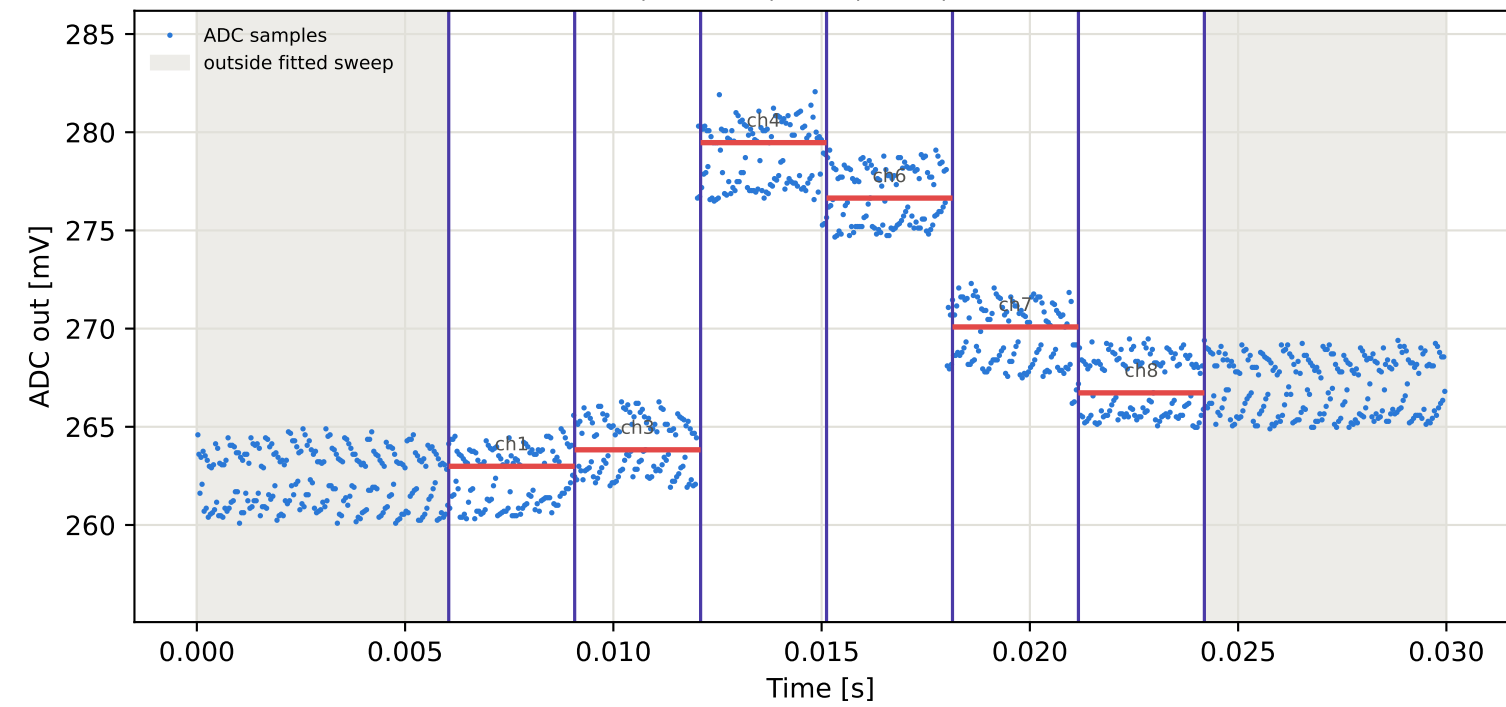
Tag15 &lt;- Tag6 | 975 MHz | run 0 | rep 1 | phase -133.62 deg
