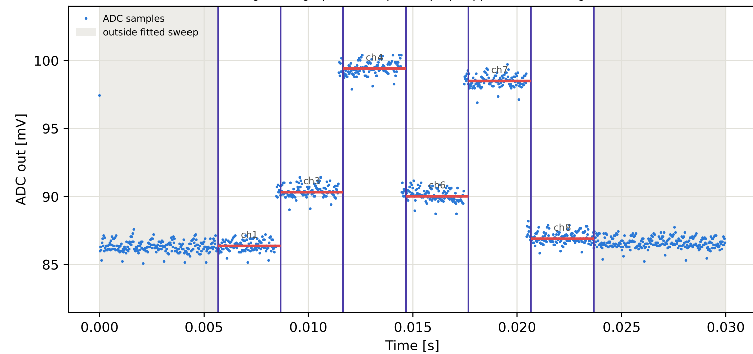
Tag4 &lt;- Tag15 | 795 MHz | run 0 | rep 1 | phase 84.80 deg
