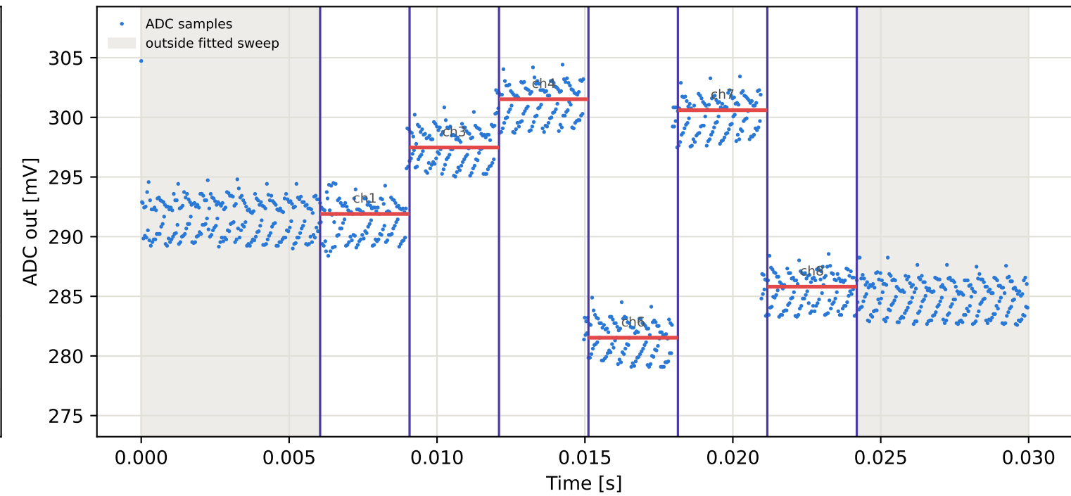
Tag5 &lt;- Tag1 | 965 MHz | run 0 | rep 1 | phase 128.01 deg
