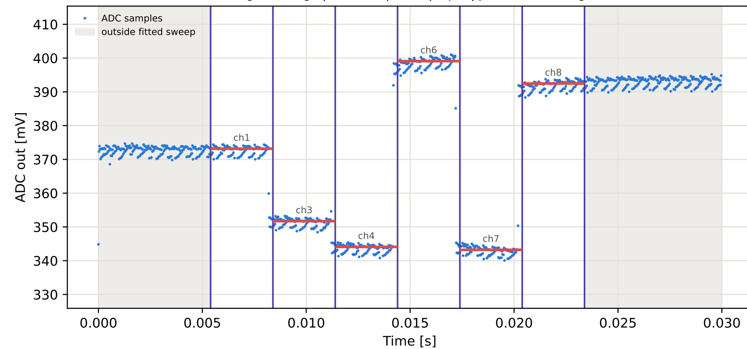
Tag16 &lt;- Tag10 | 985 MHz | run 0 | rep 1 | phase 79.27 deg
