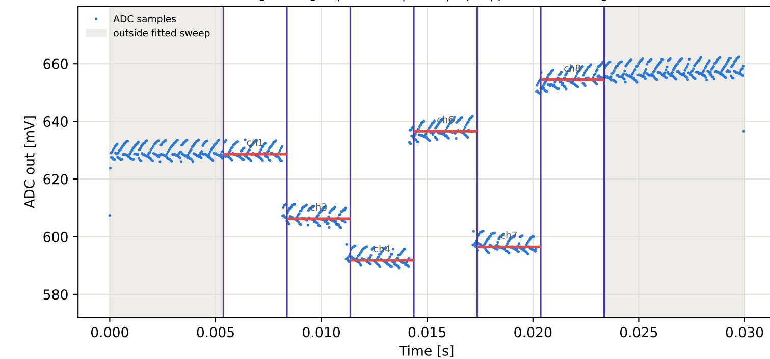
Tag8 &lt;- Tag15 | 915 MHz | run 0 | rep 1 | phase 126.14 deg
