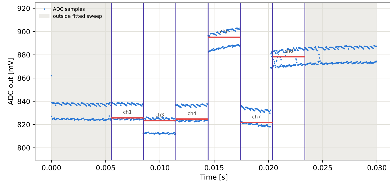
Tag5 &lt;- Tag3 | 895 MHz | run 0 | rep 1 | phase 176.26 deg
