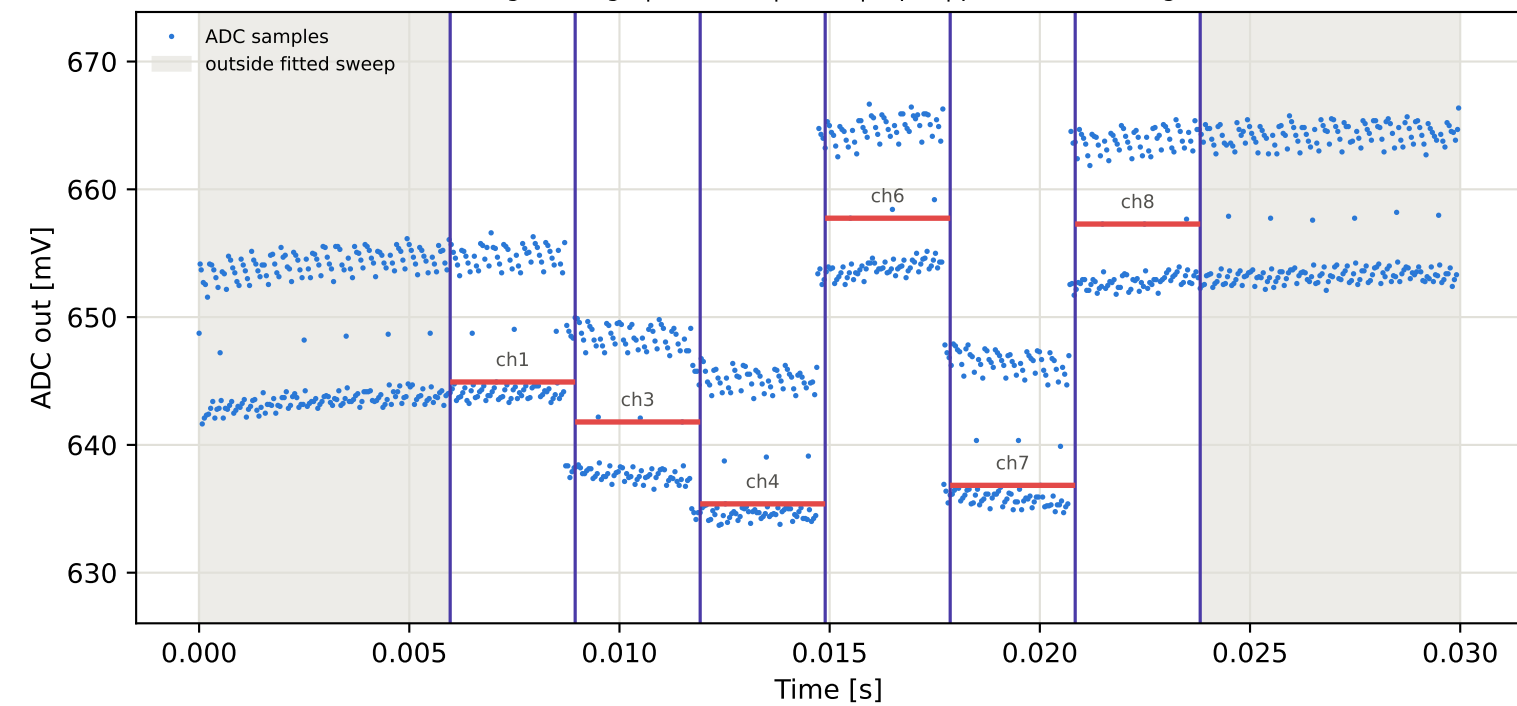
Tag3 &lt;- Tag6 | 925 MHz | run 0 | rep 1 | phase 102.94 deg
