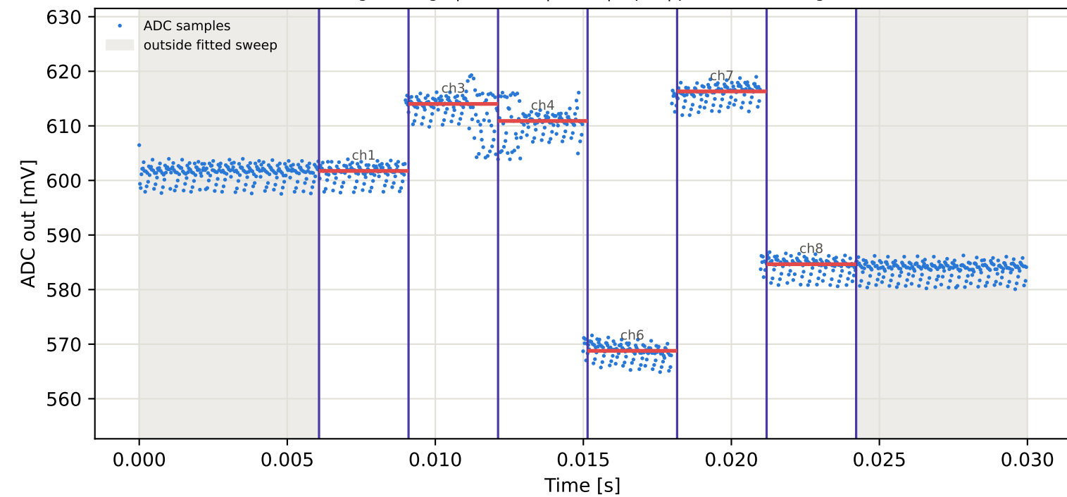
Tag1 &lt;- Tag8 | 975 MHz | run 0 | rep 1 | phase 47.63 deg
