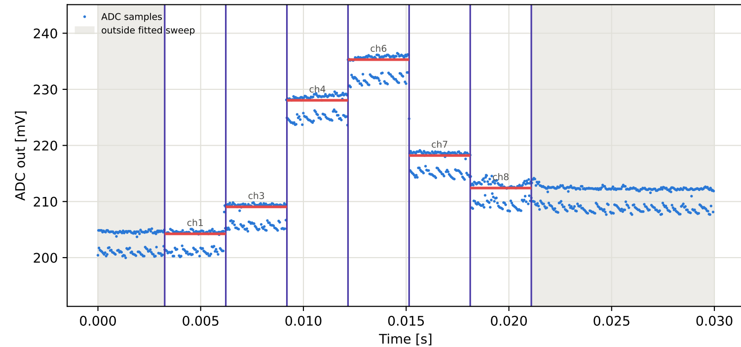
Tag15 &lt;- Tag5 | 955 MHz | run 0 | rep 1 | phase -105.49 deg
