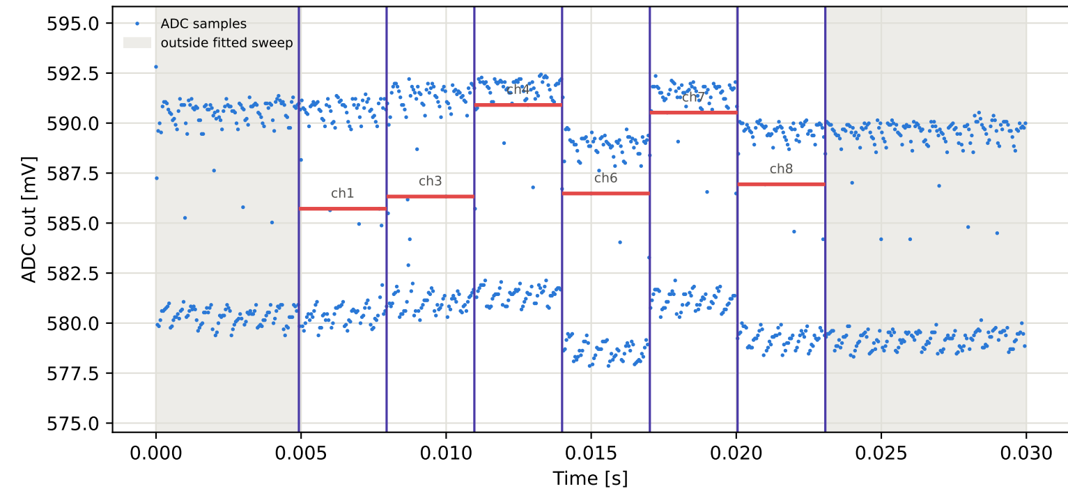
Tag6 &lt;- Tag4 | 975 MHz | run 0 | rep 1 | phase -112.43 deg
