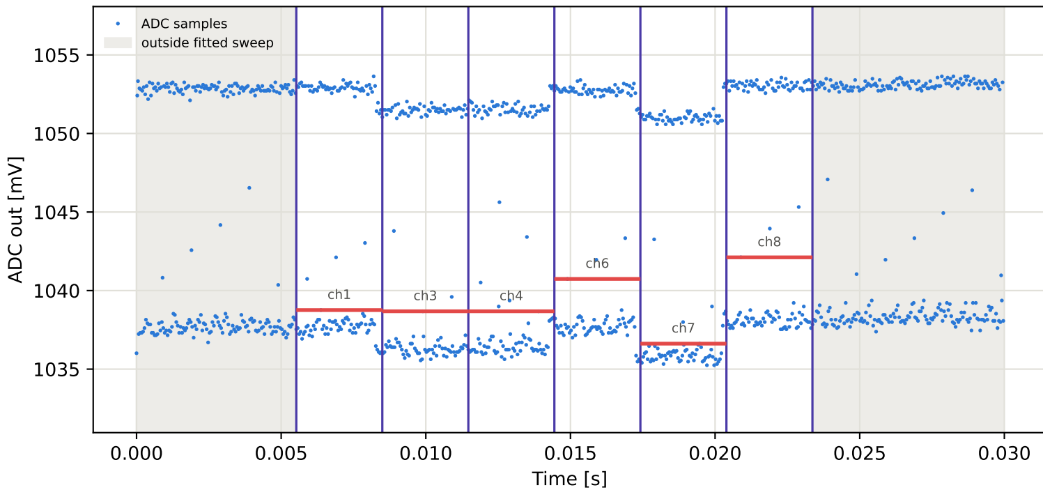
Tag7 &lt;- Tag15 | 835 MHz | run 0 | rep 1 | phase -31.72 deg
