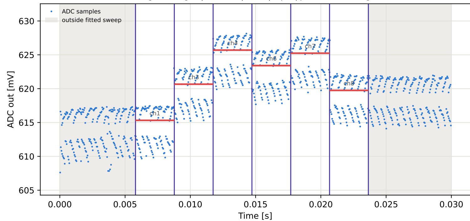
Tag10 &lt;- Tag2 | 855 MHz | run 0 | rep 1 | phase 47.36 deg
