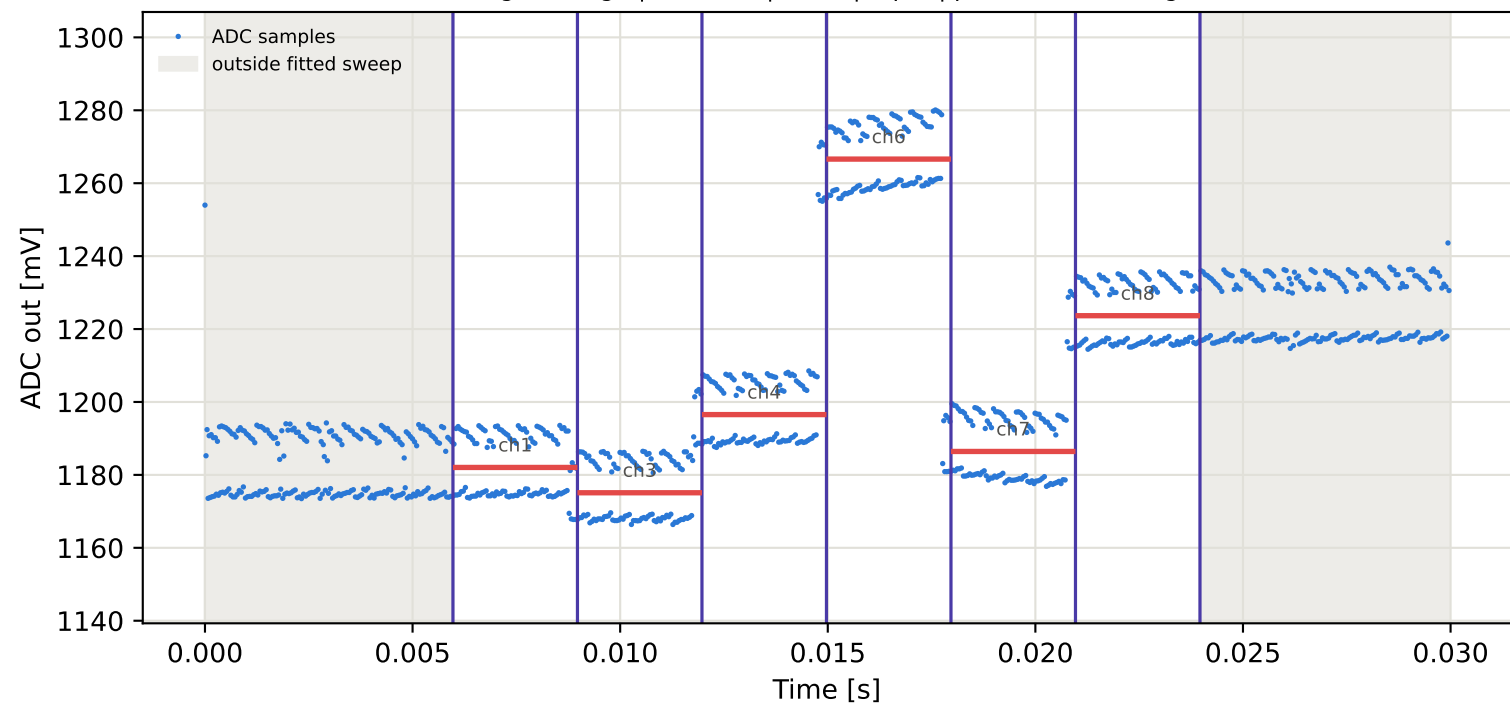
Tag8 &lt;- Tag10 | 925 MHz | run 0 | rep 1 | phase -53.89 deg
