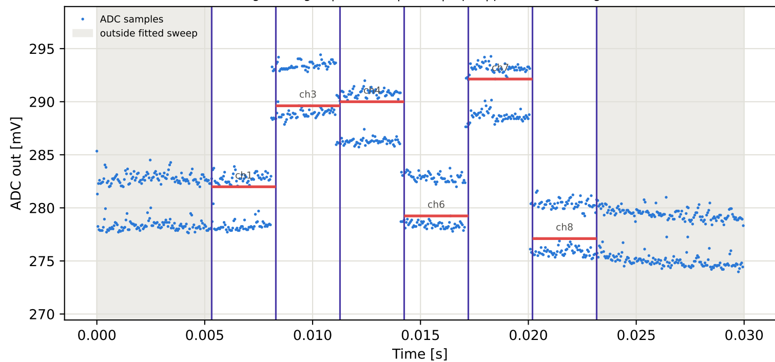
Tag2 &lt;- Tag16 | 855 MHz | run 0 | rep 1 | phase -37.09 deg
