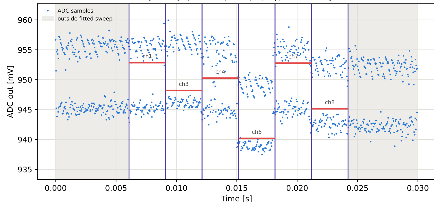
Tag9 &lt;- Tag2 | 885 MHz | run 0 | rep 1 | phase 4.39 deg
