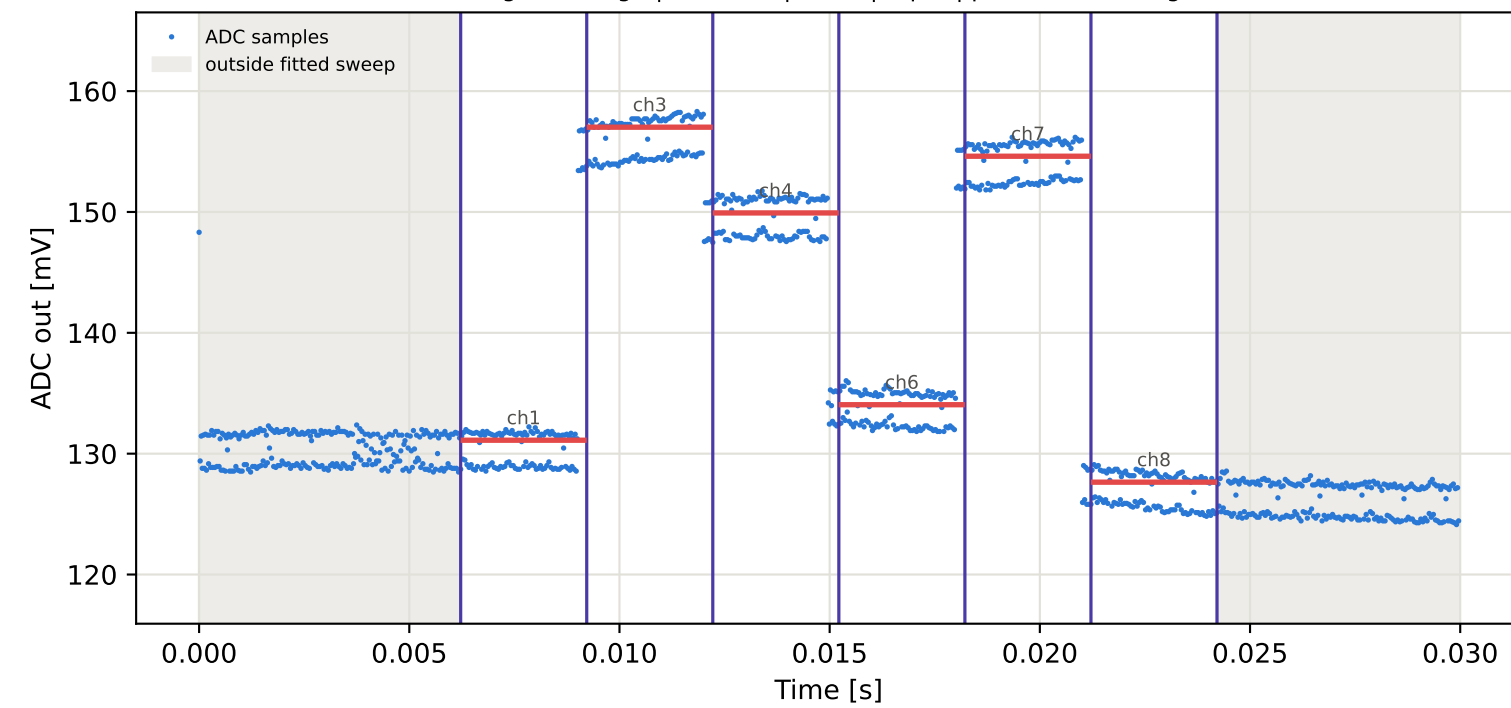
Tag15 &lt;- Tag5 | 835 MHz | run 0 | rep 1 | phase -85.34 deg
