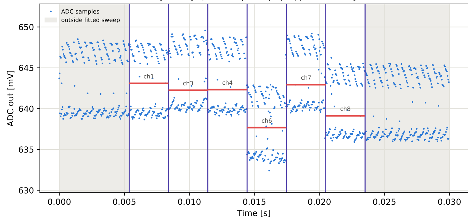
Tag9 &lt;- Tag2 | 855 MHz | run 0 | rep 1 | phase 5.19 deg
