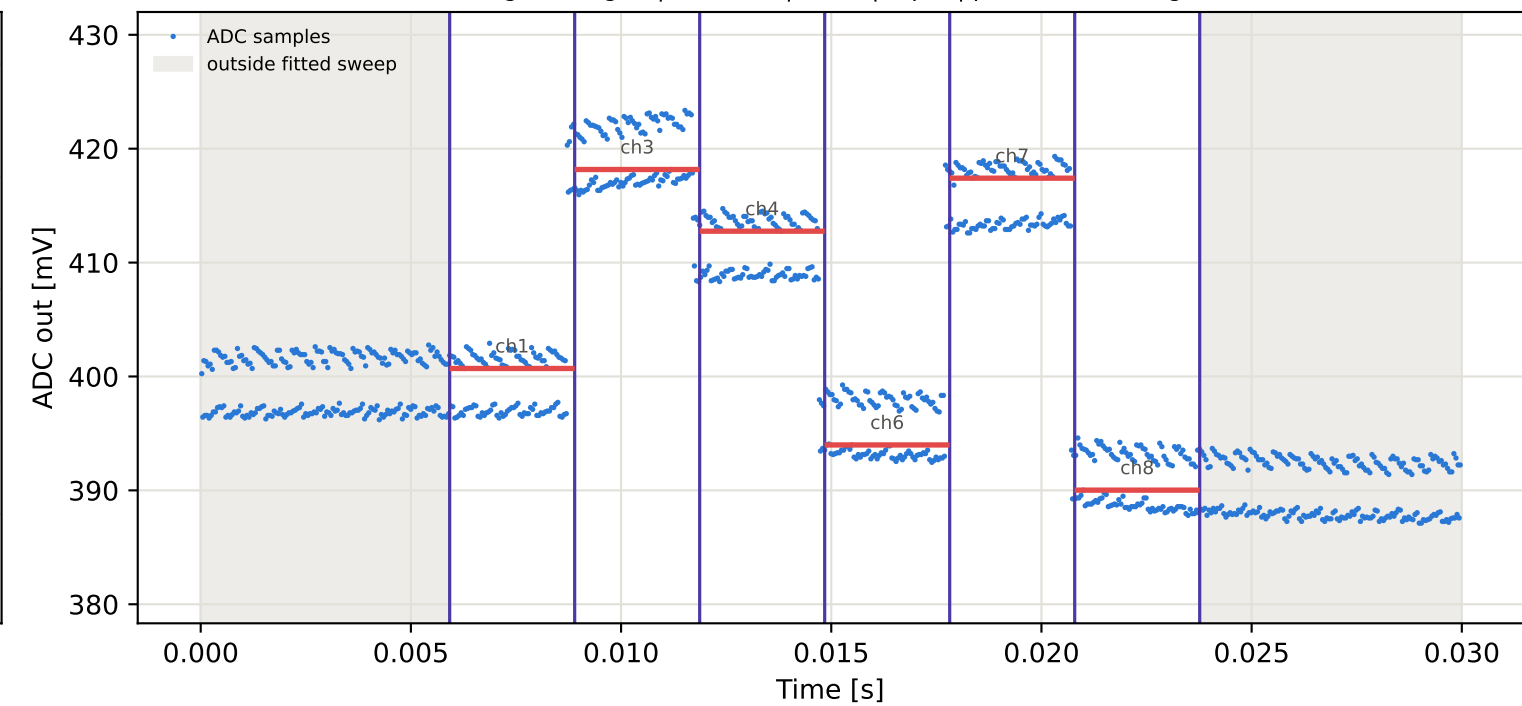
Tag5 &lt;- Tag2 | 855 MHz | run 0 | rep 1 | phase 168.26 deg
