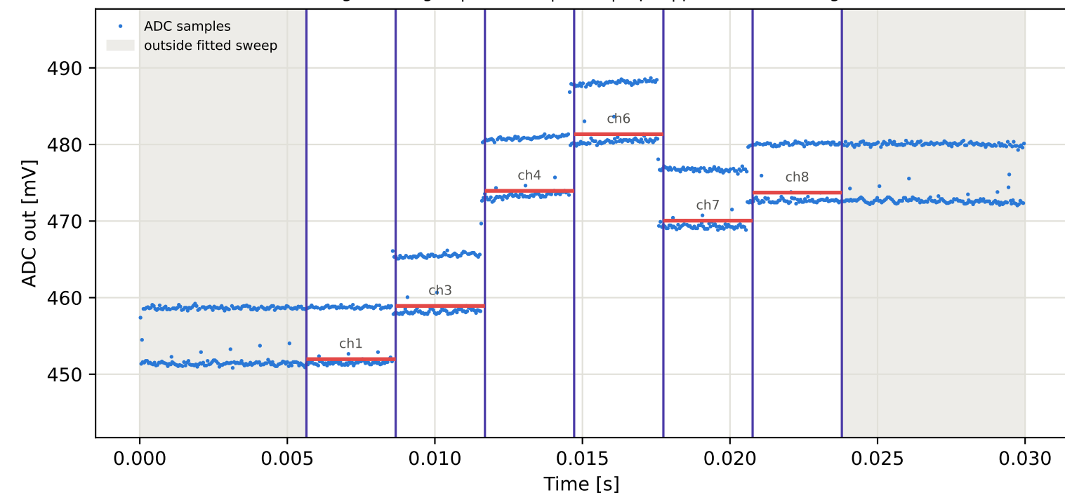
Tag16 &lt;- Tag10 | 855 MHz | run 0 | rep 1 | phase -134.07 deg
