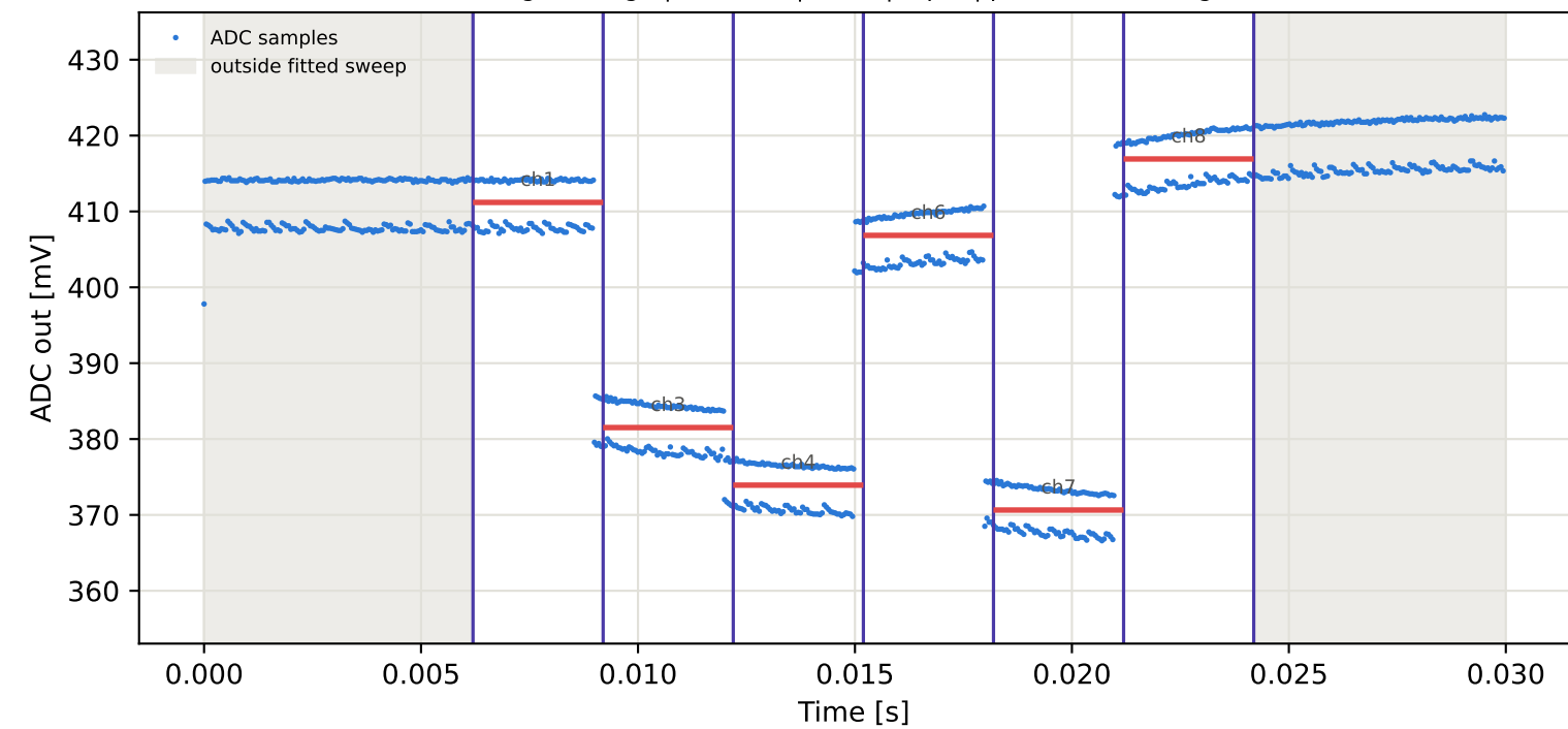
Tag5 &lt;- Tag9 | 865 MHz | run 0 | rep 1 | phase -37.19 deg
