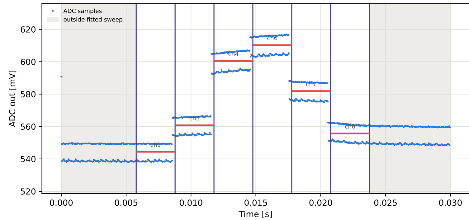
Tag5 &lt;- Tag4 | 935 MHz | run 0 | rep 1 | phase -130.24 deg
