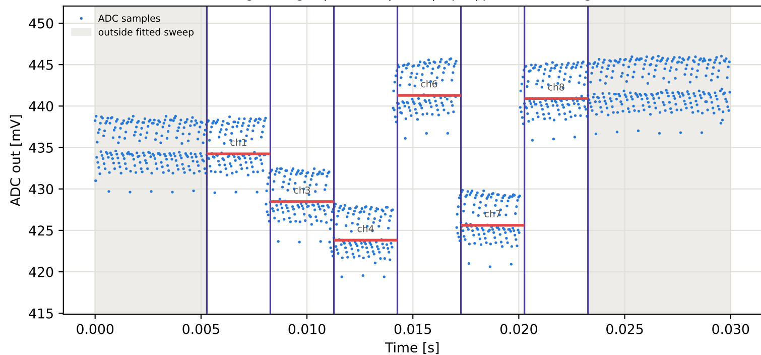
Tag1 &lt;- Tag2 | 935 MHz | run 0 | rep 1 | phase 53.85 deg
