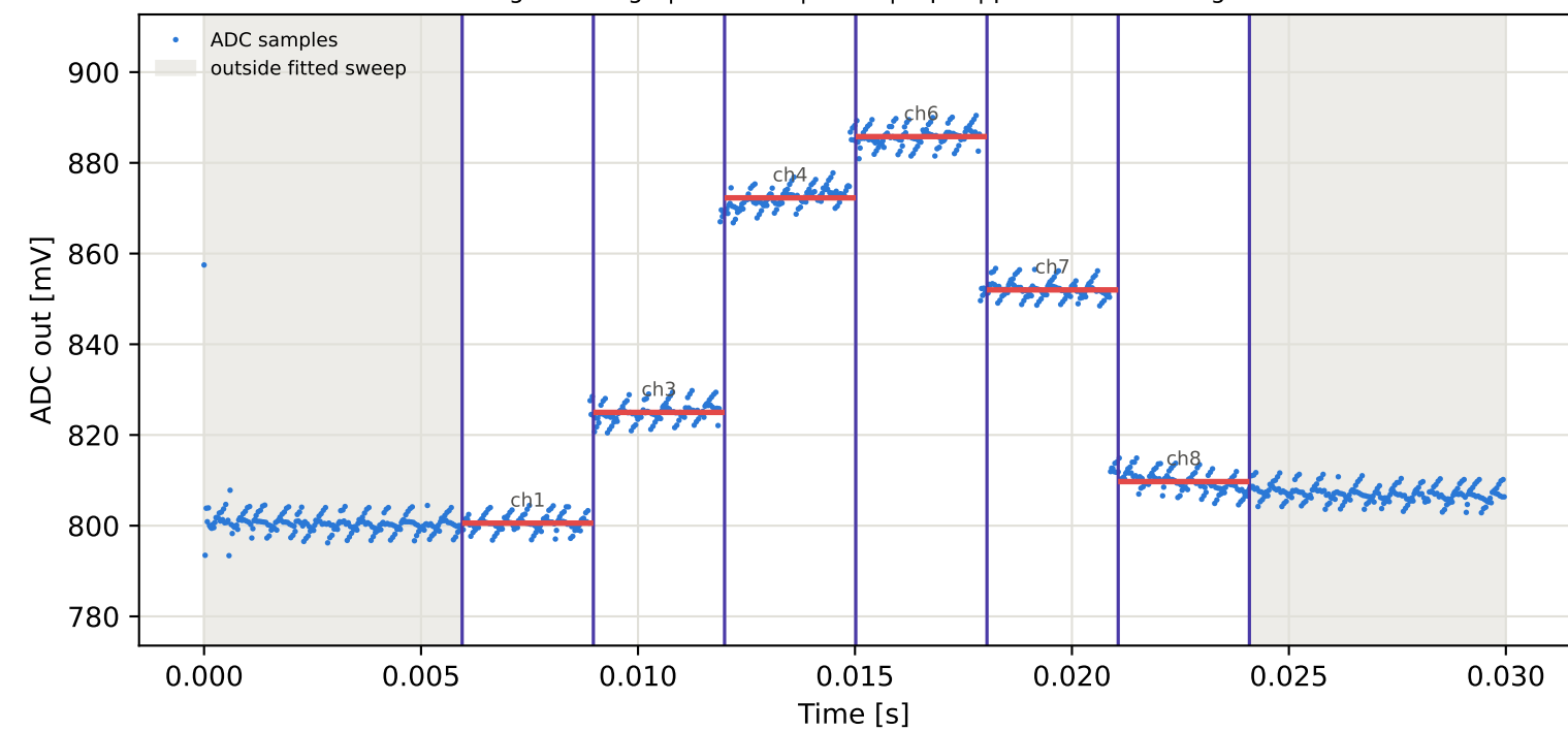
Tag10 &lt;- Tag9 | 925 MHz | run 0 | rep 1 | phase 72.62 deg
