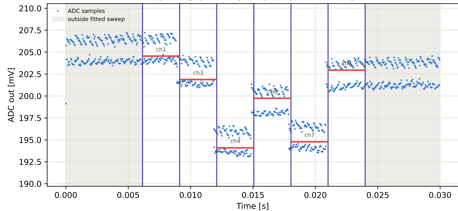
Tag7 &lt;- Tag1 | 805 MHz | run 0 | rep 1 | phase -41.47 deg
