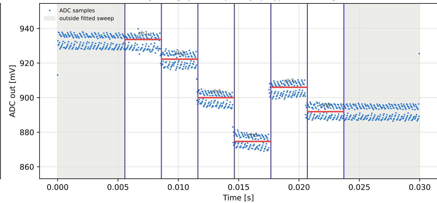
Tag3 &lt;- Tag7 | 875 MHz | run 0 | rep 1 | phase -87.91 deg
