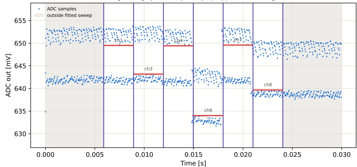
Tag3 &lt;- Tag2 | 925 MHz | run 0 | rep 1 | phase -14.36 deg
