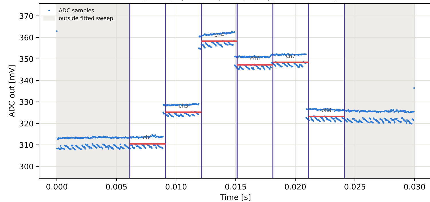
Tag6 &lt;- Tag9 | 825 MHz | run 0 | rep 1 | phase 17.73 deg
