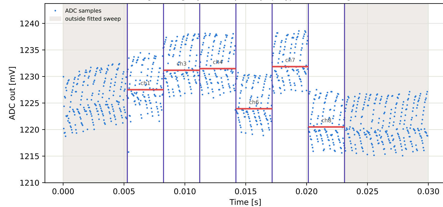
Tag10 &lt;- Tag2 | 895 MHz | run 0 | rep 1 | phase -178.19 deg
