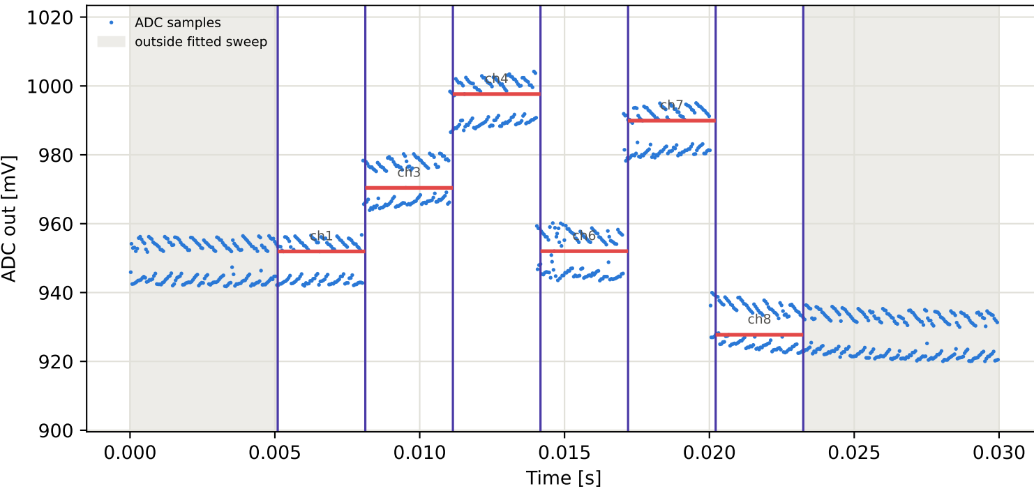
Tag16 &lt;- Tag10 | 915 MHz | run 0 | rep 1 | phase -69.85 deg
