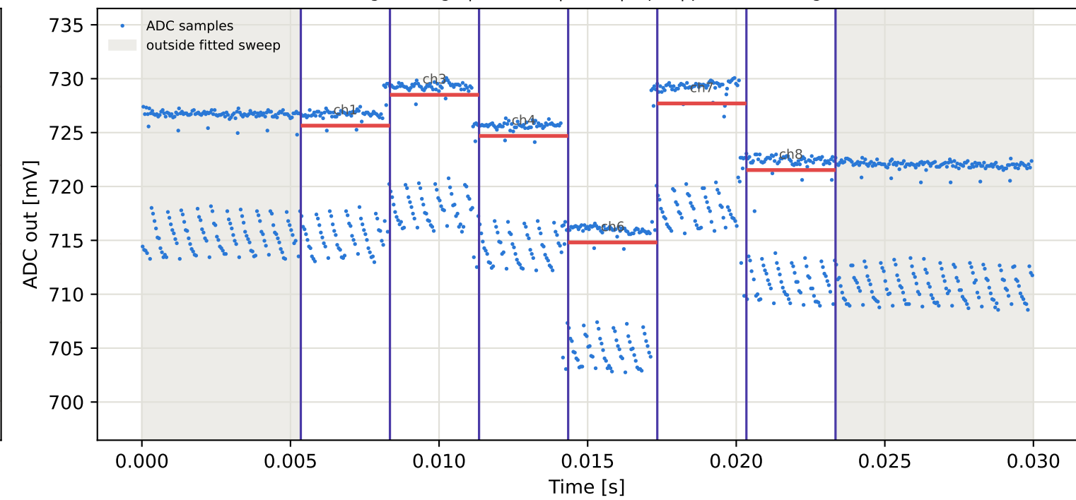
Tag9 &lt;- Tag6 | 985 MHz | run 0 | rep 1 | phase -172.94 deg
