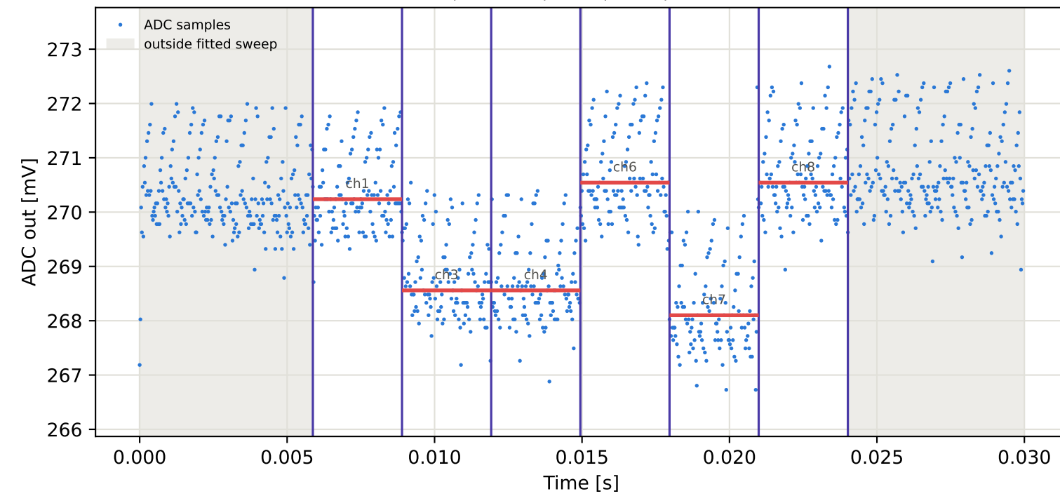
Tag7 &lt;- Tag5 | 795 MHz | run 0 | rep 1 | phase 148.09 deg
