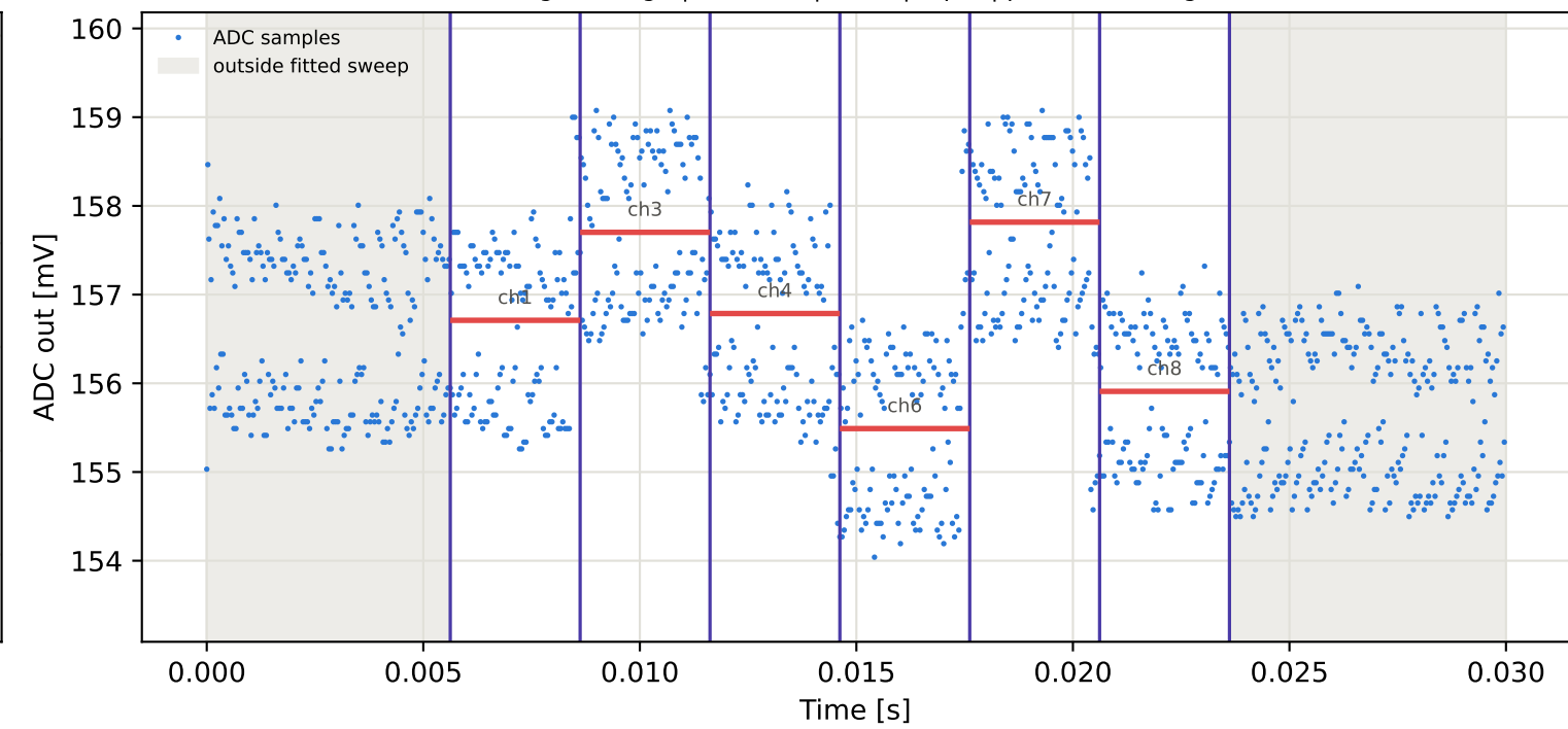
Tag9 &lt;- Tag15 | 785 MHz | run 0 | rep 1 | phase -13.94 deg
