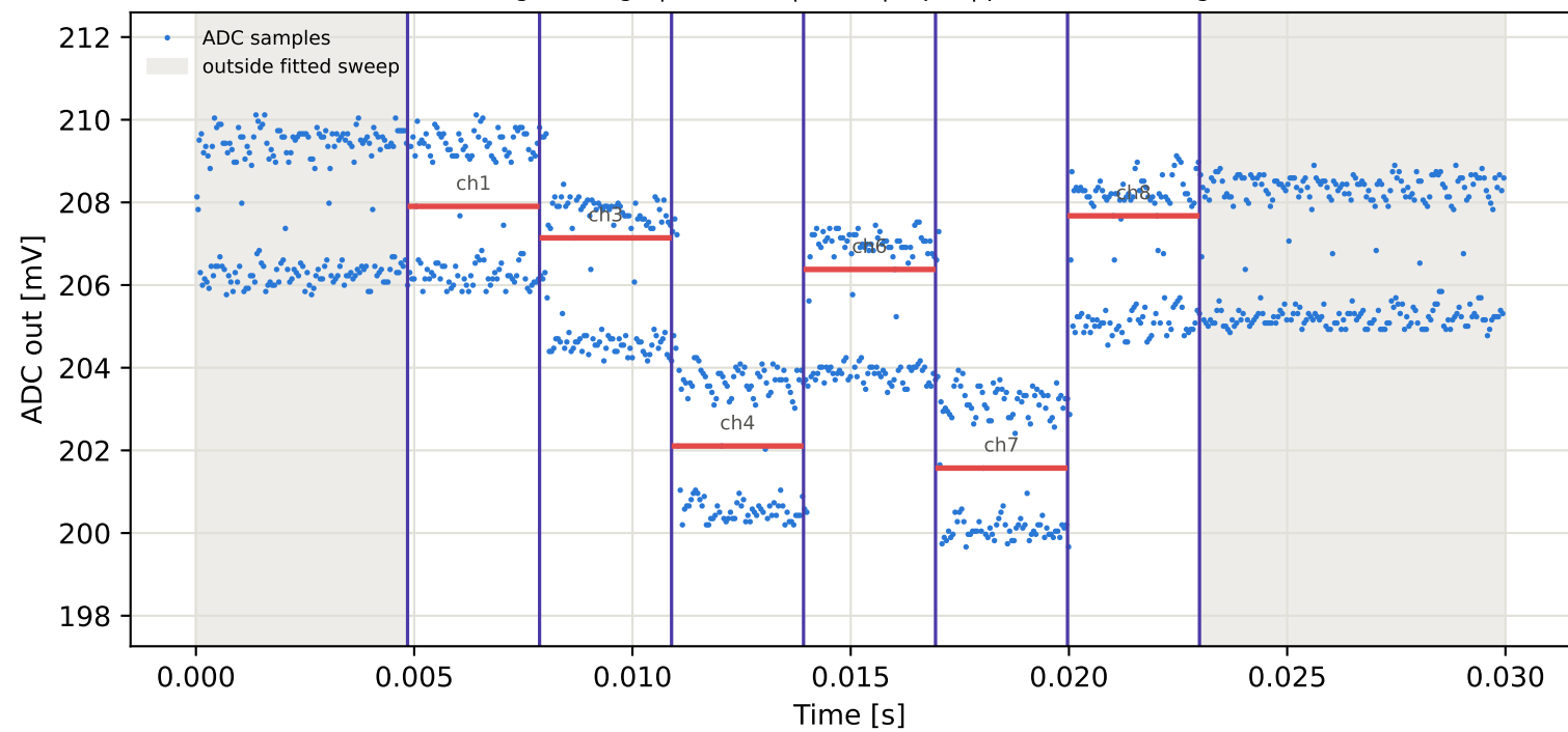
Tag9 &lt;- Tag6 | 795 MHz | run 0 | rep 1 | phase 15.68 deg
