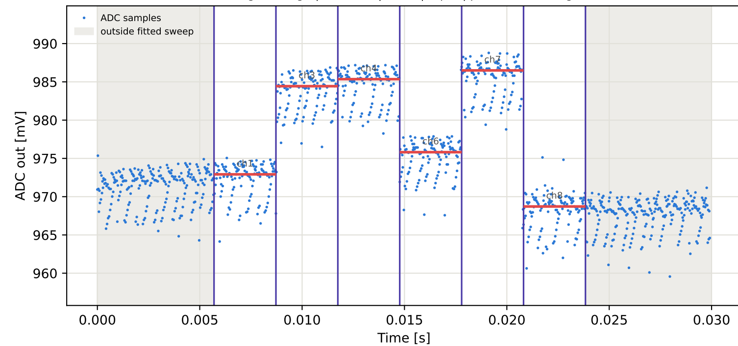
Tag8 &lt;- Tag1 | 865 MHz | run 0 | rep 1 | phase 152.36 deg
