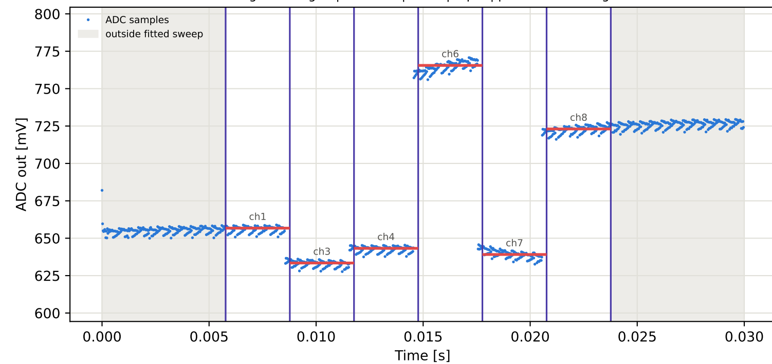
Tag15 &lt;- Tag3 | 915 MHz | run 0 | rep 1 | phase 117.95 deg
