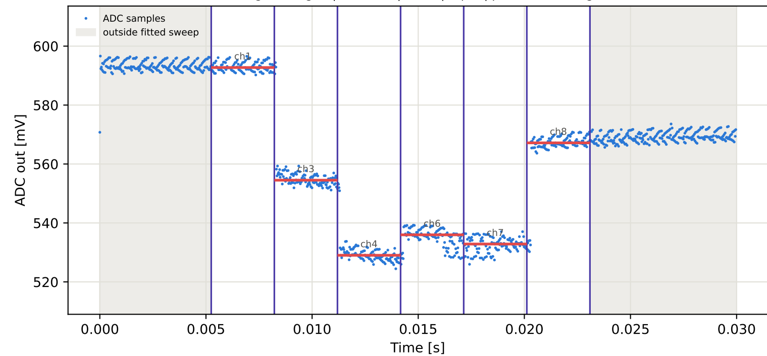
Tag5 &lt;- Tag2 | 875 MHz | run 0 | rep 1 | phase 97.59 deg
