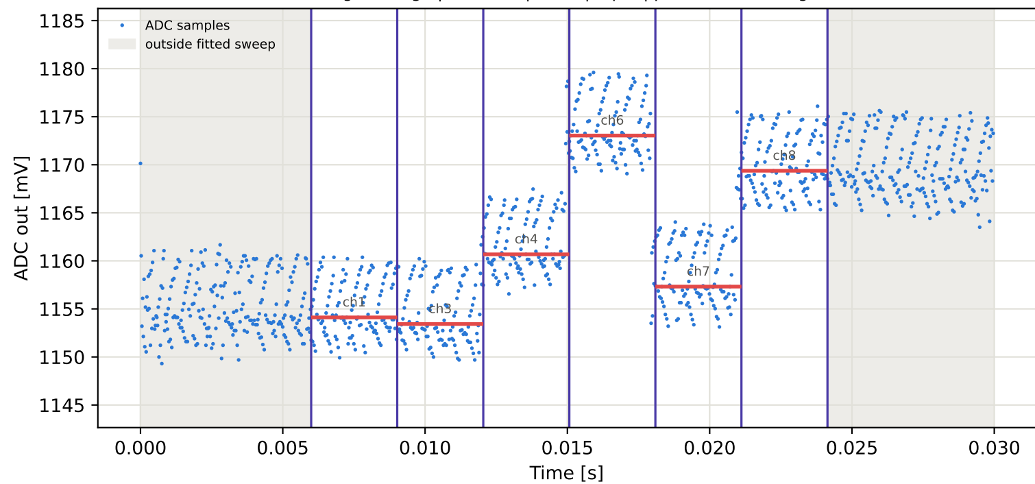
Tag9 &lt;- Tag8 | 875 MHz | run 0 | rep 1 | phase 33.77 deg
