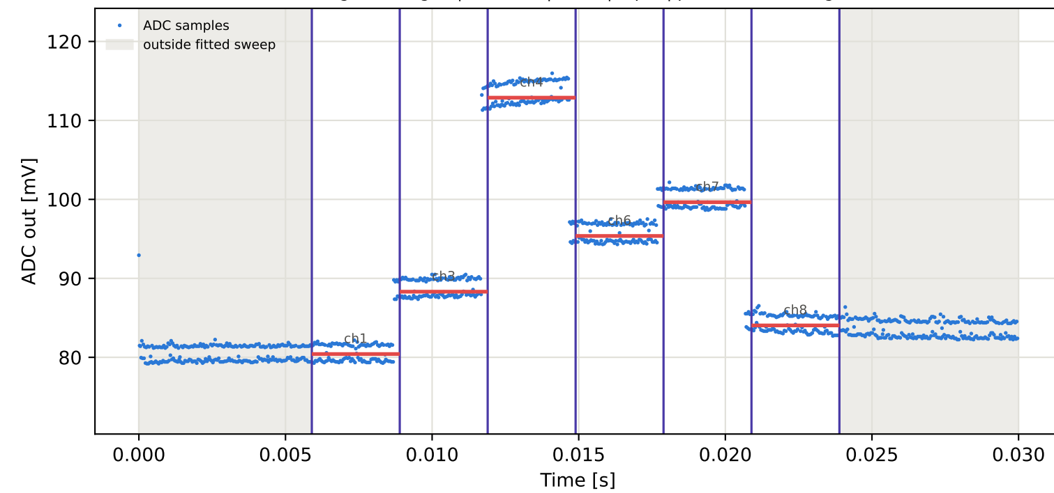
Tag15 &lt;- Tag3 | 995 MHz | run 0 | rep 1 | phase -46.45 deg
