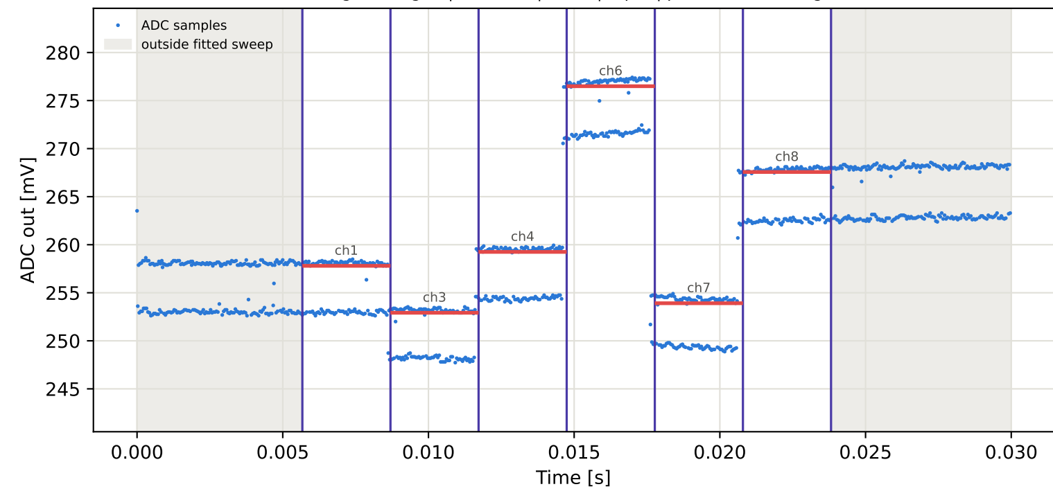
Tag5 &lt;- Tag2 | 985 MHz | run 0 | rep 1 | phase 64.53 deg
