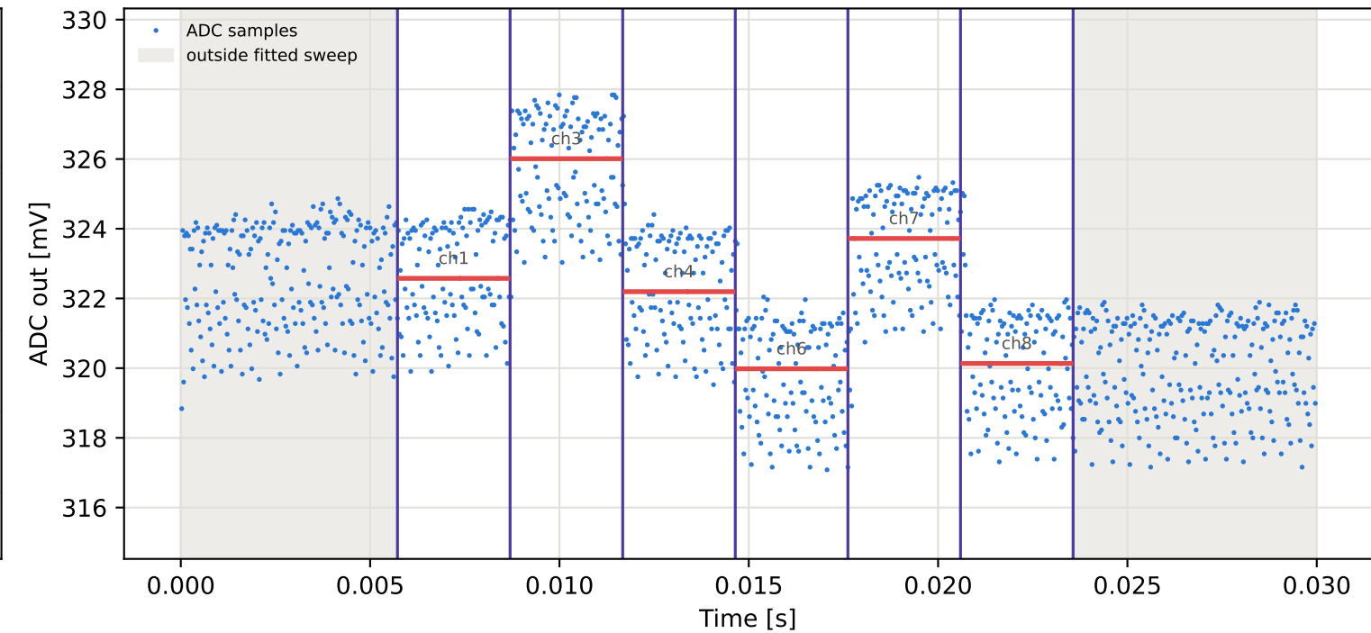
Tag3 &lt;- Tag2 | 845 MHz | run 0 | rep 1 | phase 19.84 deg
