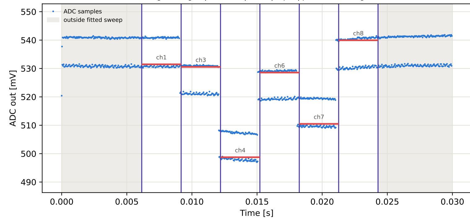
Tag1 &lt;- Tag3 | 965 MHz | run 0 | rep 1 | phase -22.28 deg
