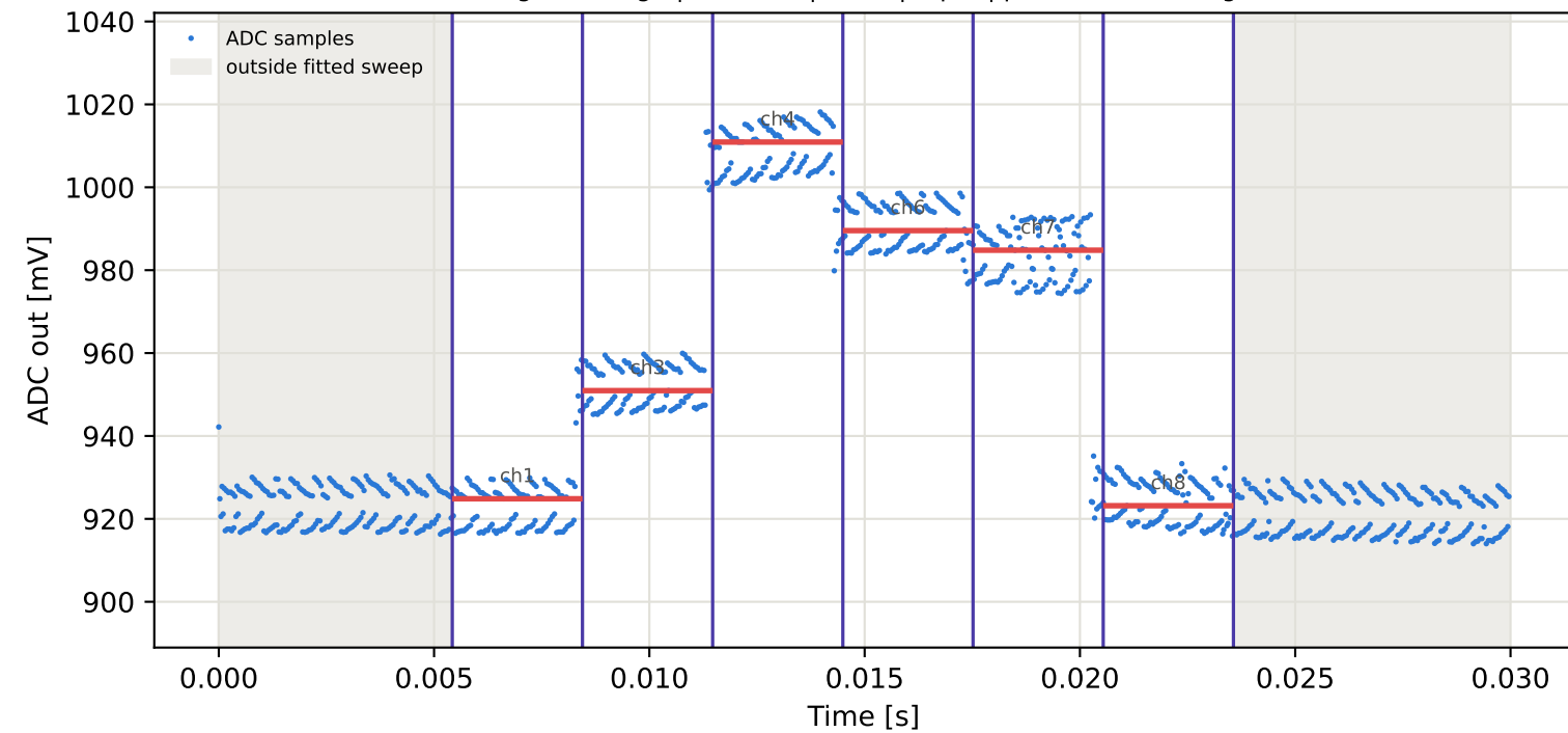
Tag16 &lt;- Tag7 | 935 MHz | run 0 | rep 1 | phase -83.78 deg
