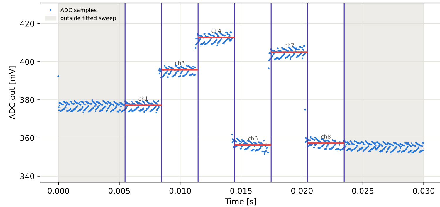
Tag16 &lt;- Tag1 | 935 MHz | run 0 | rep 1 | phase 177.67 deg
