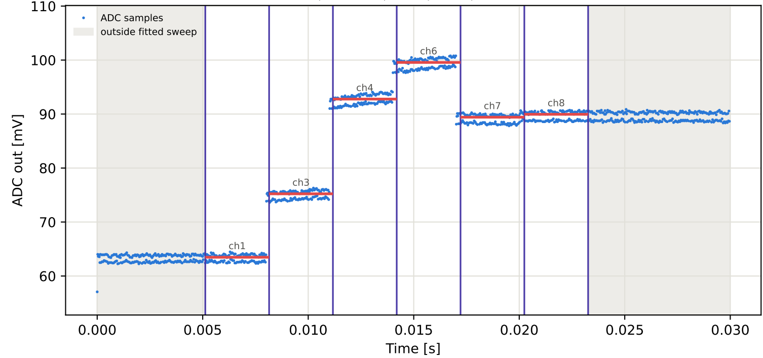
Tag4 &lt;- Tag3 | 855 MHz | run 0 | rep 1 | phase -130.73 deg
