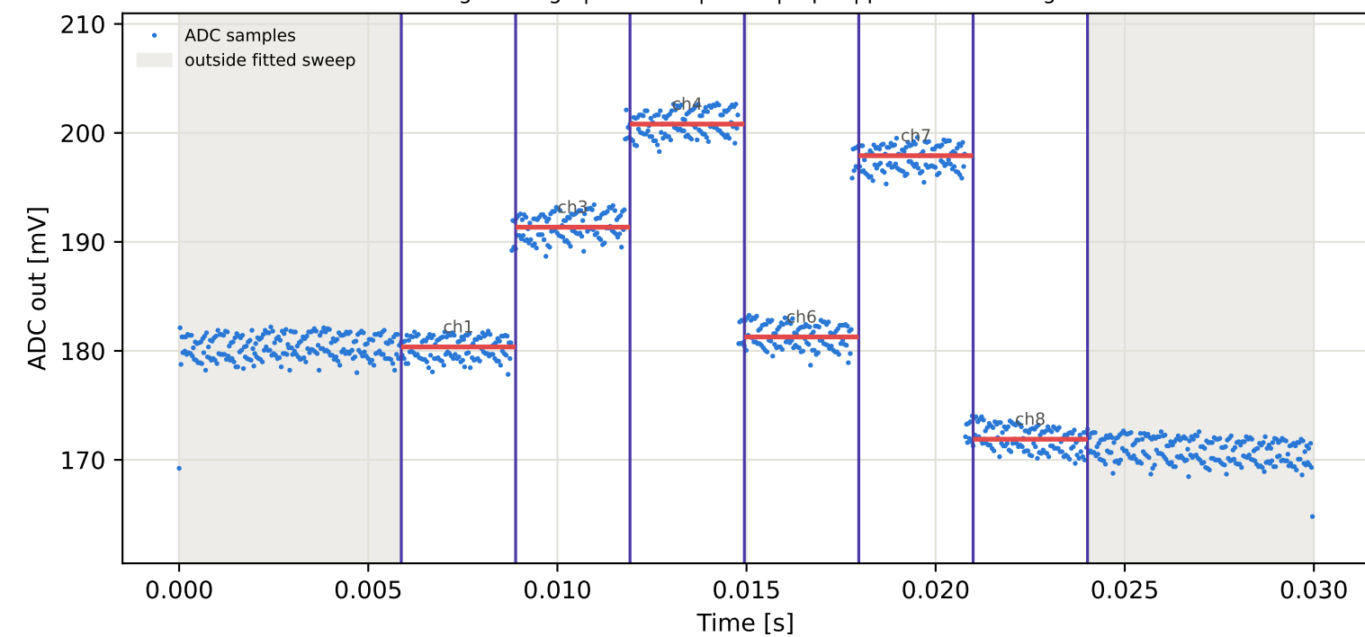
Tag4 &lt;- Tag9 | 925 MHz | run 0 | rep 1 | phase -68.51 deg
