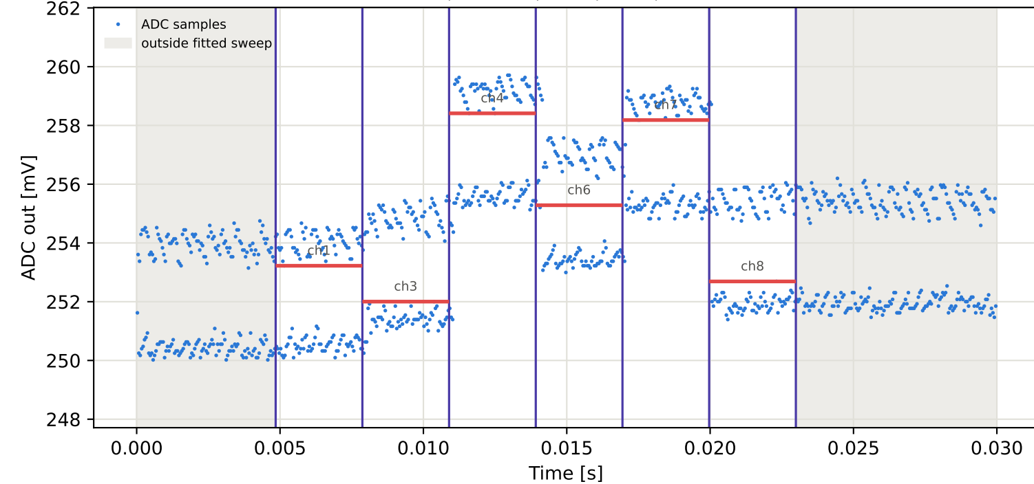
Tag9 &lt;- Tag16 | 805 MHz | run 0 | rep 1 | phase -94.33 deg
