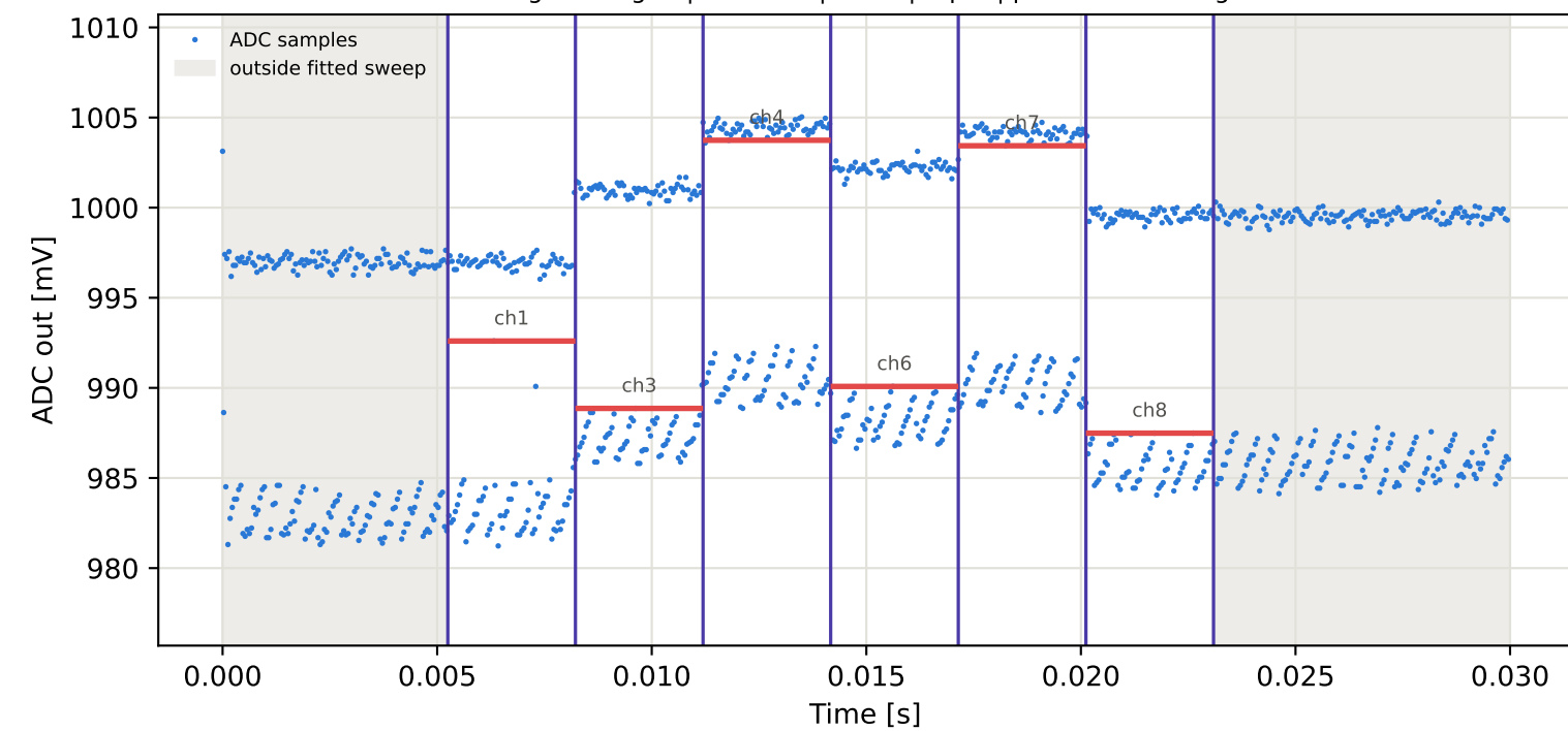
Tag7 &lt;- Tag3 | 845 MHz | run 0 | rep 1 | phase -79.18 deg
