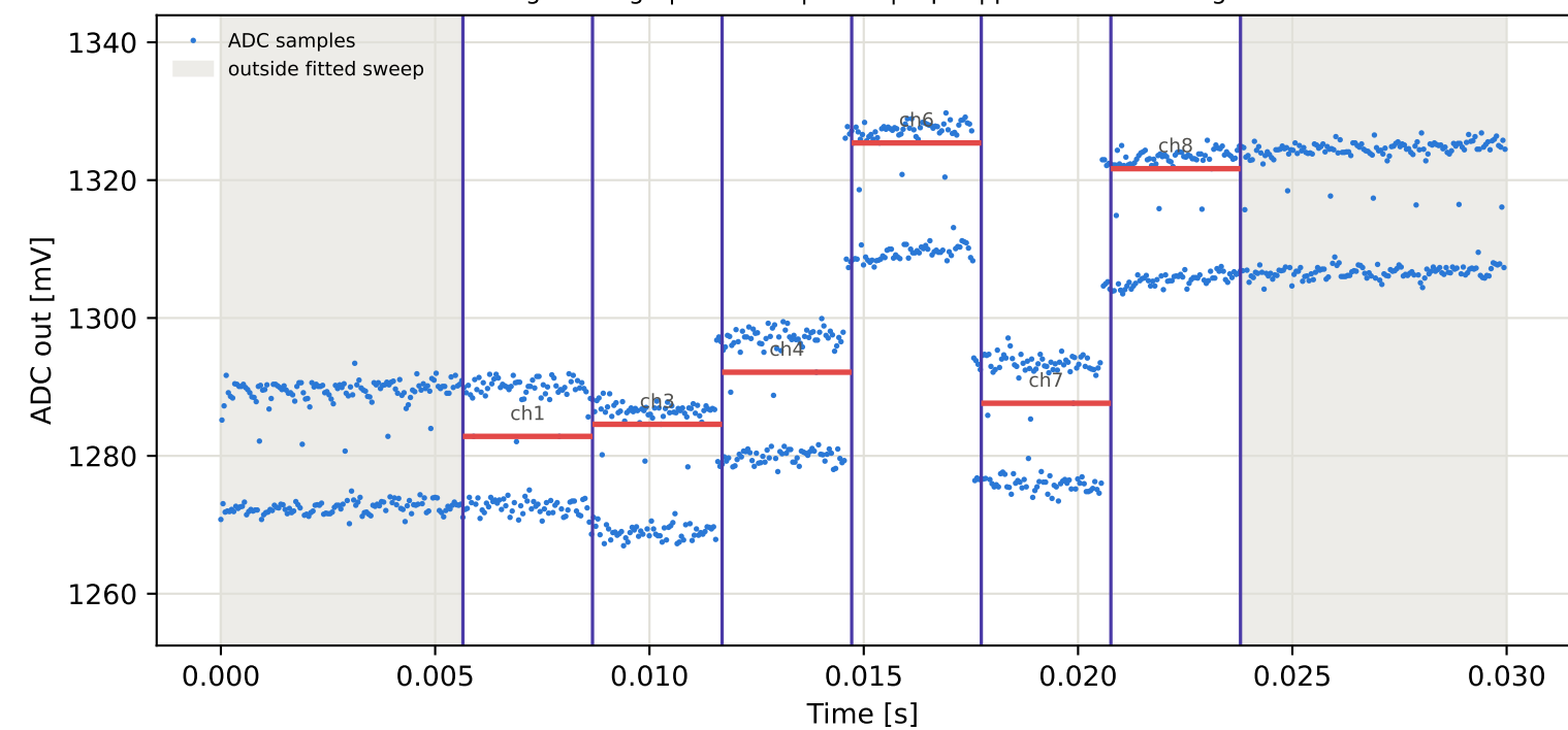
Tag6 &lt;- Tag5 | 885 MHz | run 0 | rep 1 | phase -173.59 deg
