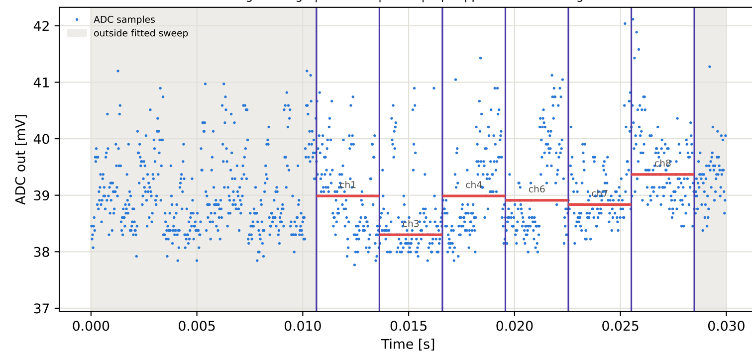
Tag2 &lt;- Tag7 | 985 MHz | run 0 | rep 1 | phase -174.66 deg
