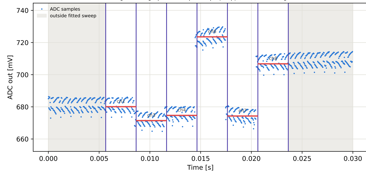
Tag15 &lt;- Tag5 | 915 MHz | run 0 | rep 1 | phase 174.67 deg
