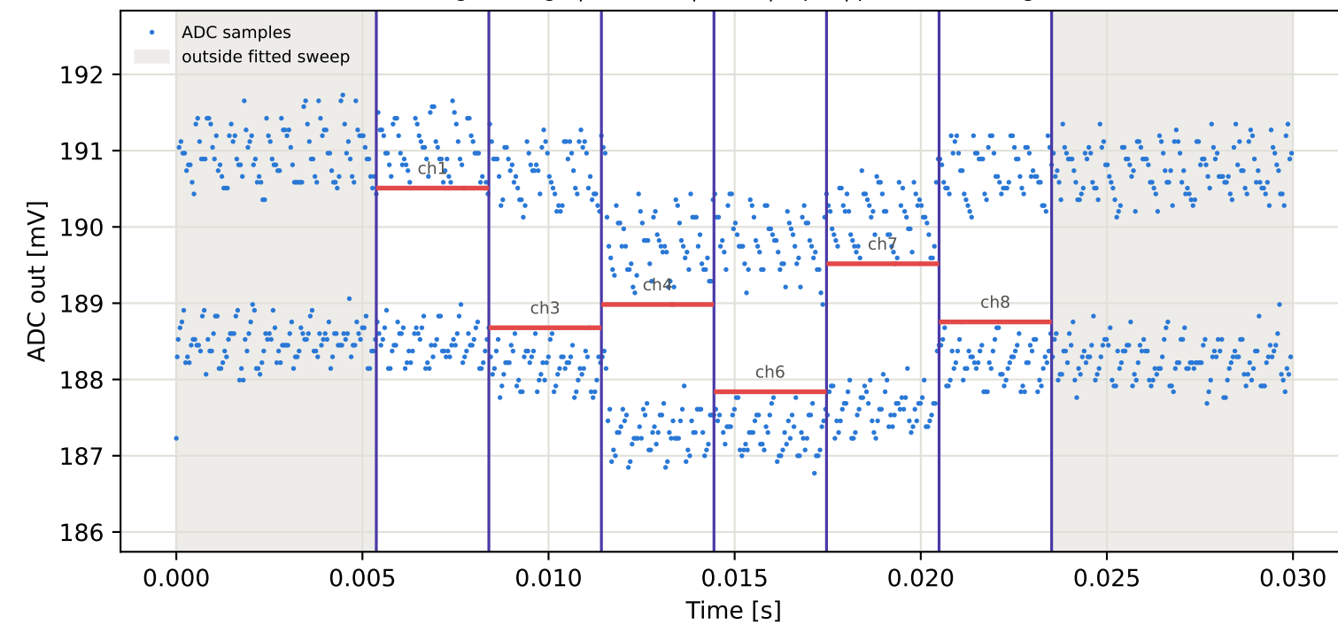
Tag8 &lt;- Tag4 | 775 MHz | run 0 | rep 1 | phase -69.43 deg
