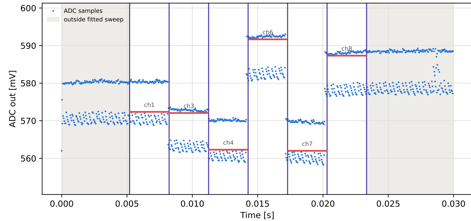
Tag3 &lt;- Tag15 | 975 MHz | run 0 | rep 1 | phase 86.98 deg
