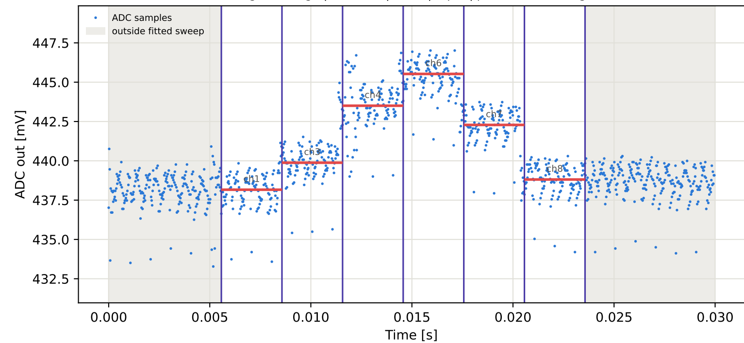
Tag16 &lt;- Tag4 | 845 MHz | run 0 | rep 1 | phase -71.37 deg
