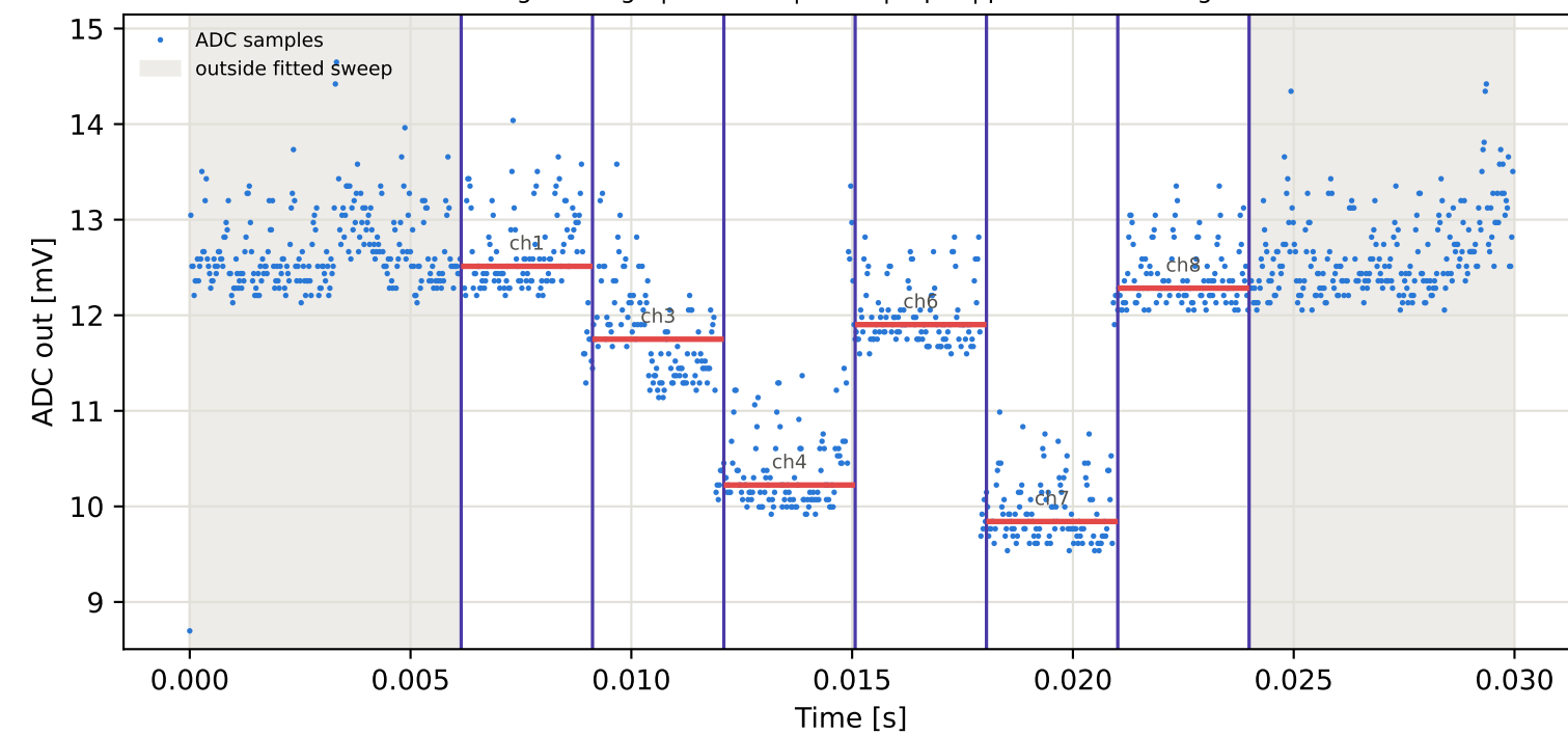
Tag3 &lt;- Tag10 | 775 MHz | run 0 | rep 1 | phase -50.05 deg
