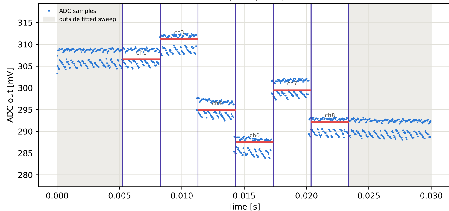
Tag4 &lt;- Tag15 | 865 MHz | run 0 | rep 1 | phase -151.94 deg
