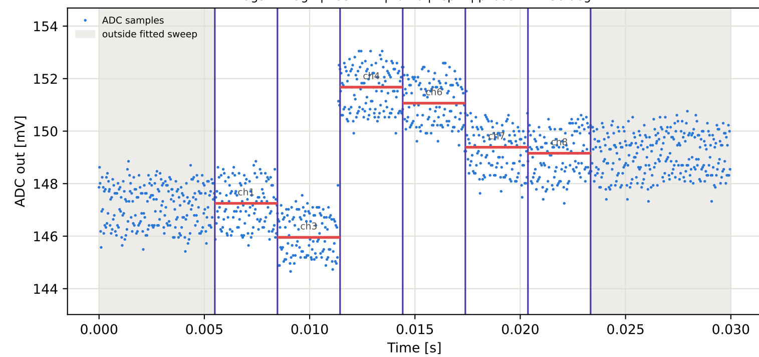
Tag3 &lt;- Tag15 | 795 MHz | run 0 | rep 1 | phase -159.05 deg
