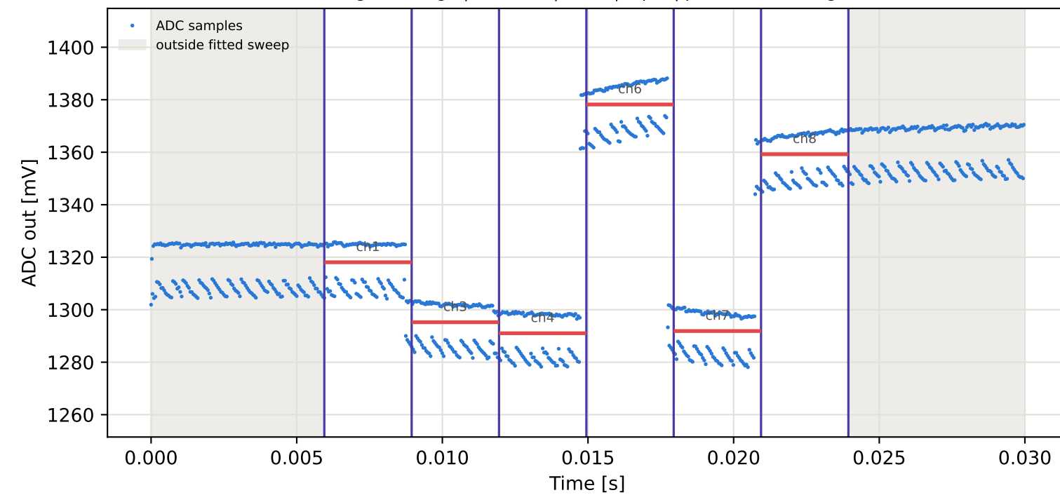
Tag10 &lt;- Tag8 | 915 MHz | run 0 | rep 1 | phase -106.20 deg
