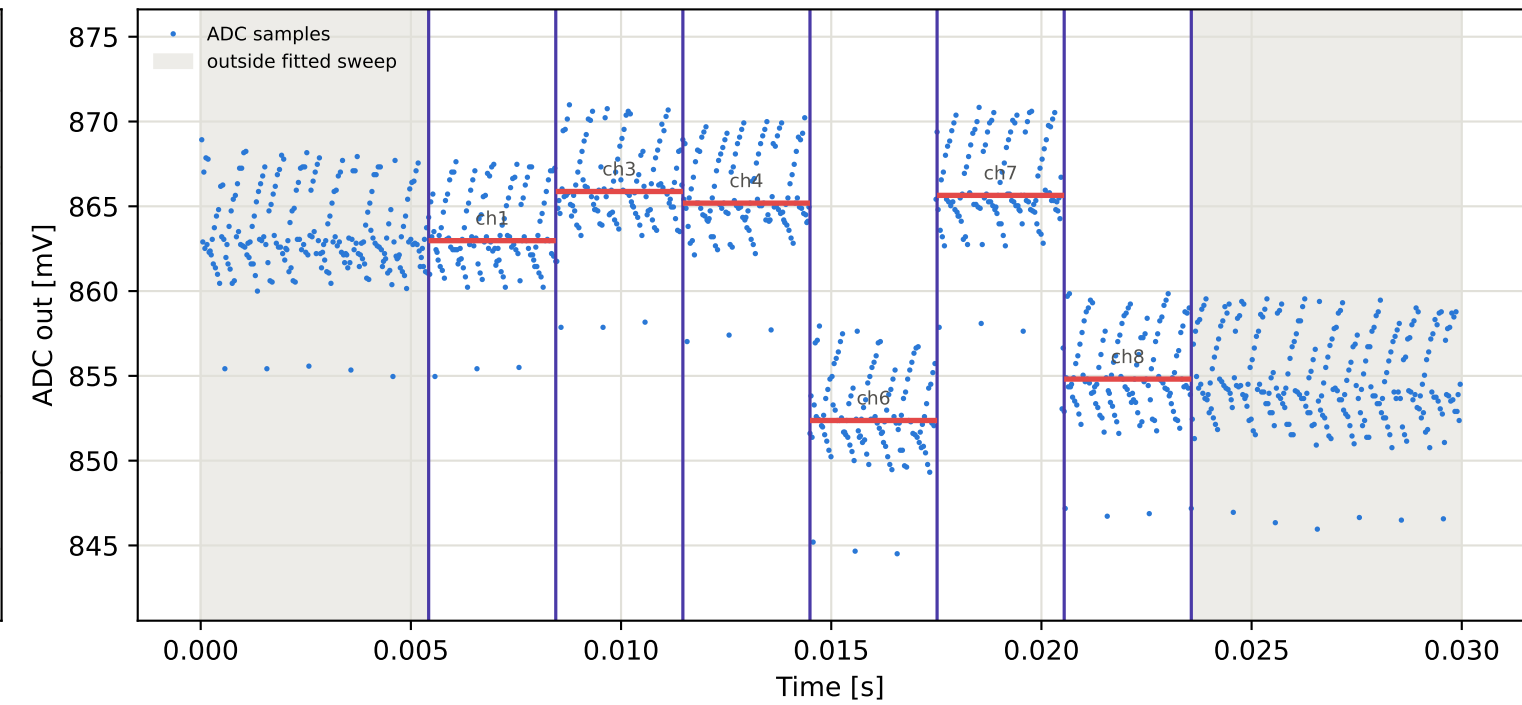
Tag7 &lt;- Tag6 | 905 MHz | run 0 | rep 1 | phase -47.69 deg
