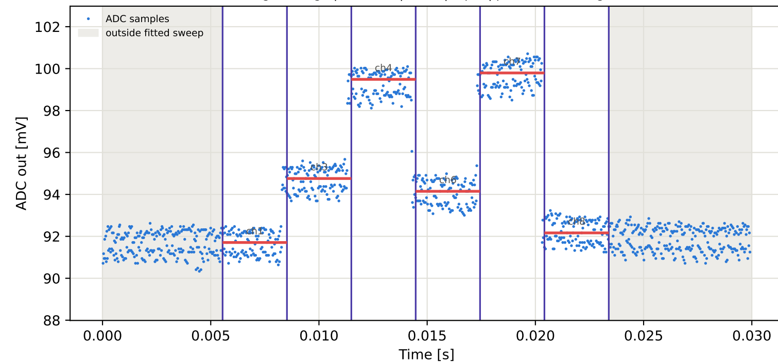
Tag5 &lt;- Tag8 | 775 MHz | run 0 | rep 1 | phase 65.87 deg
