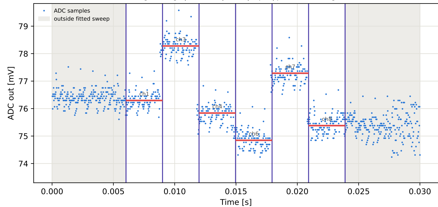
Tag7 &lt;- Tag1 | 775 MHz | run 0 | rep 1 | phase 113.02 deg
