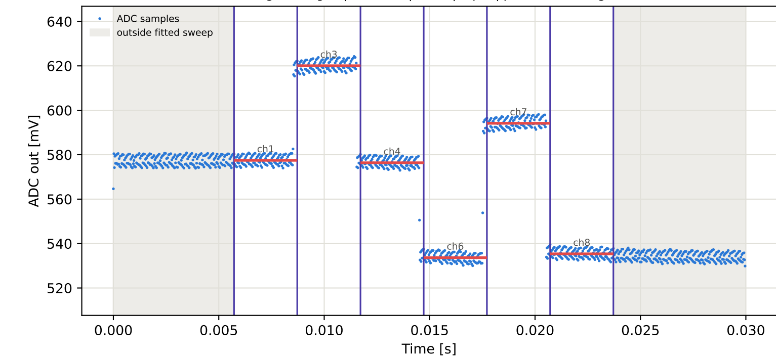
Tag3 &lt;- Tag16 | 835 MHz | run 0 | rep 1 | phase 87.91 deg
