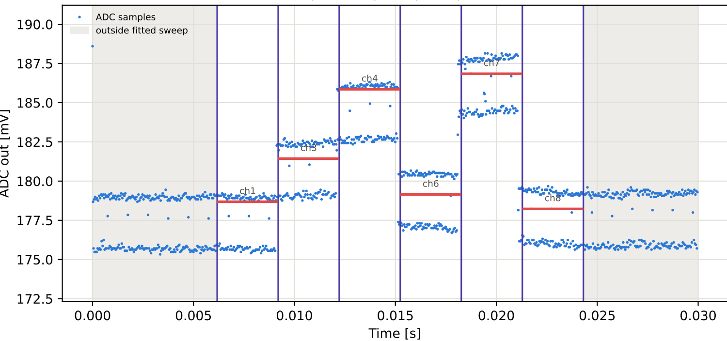
Tag10 &lt;- Tag4 | 785 MHz | run 0 | rep 1 | phase -59.16 deg
