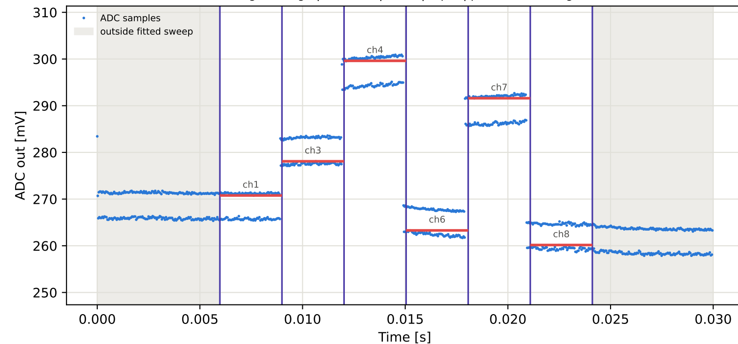
Tag6 &lt;- Tag1 | 965 MHz | run 0 | rep 1 | phase -165.98 deg
