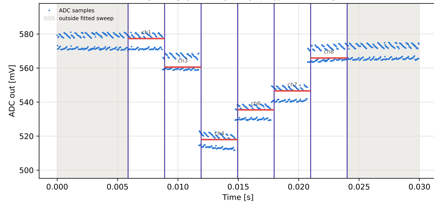
Tag9 &lt;- Tag5 | 975 MHz | run 0 | rep 1 | phase 84.56 deg
