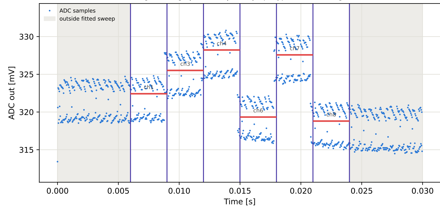
Tag15 &lt;- Tag4 | 895 MHz | run 0 | rep 1 | phase 141.14 deg
