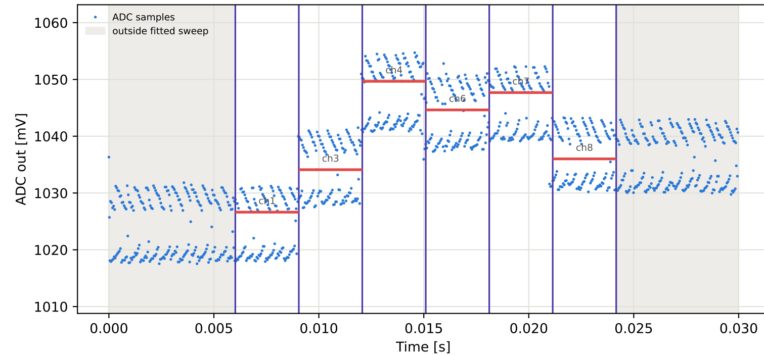
Tag7 &lt;- Tag5 | 835 MHz | run 0 | rep 1 | phase -77.71 deg
