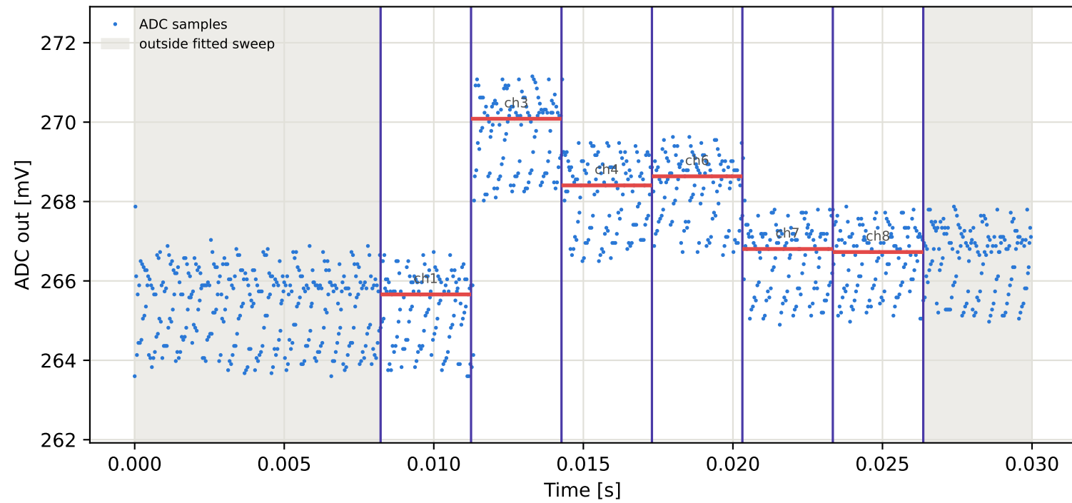
Tag7 &lt;- Tag15 | 795 MHz | run 0 | rep 1 | phase 132.96 deg
