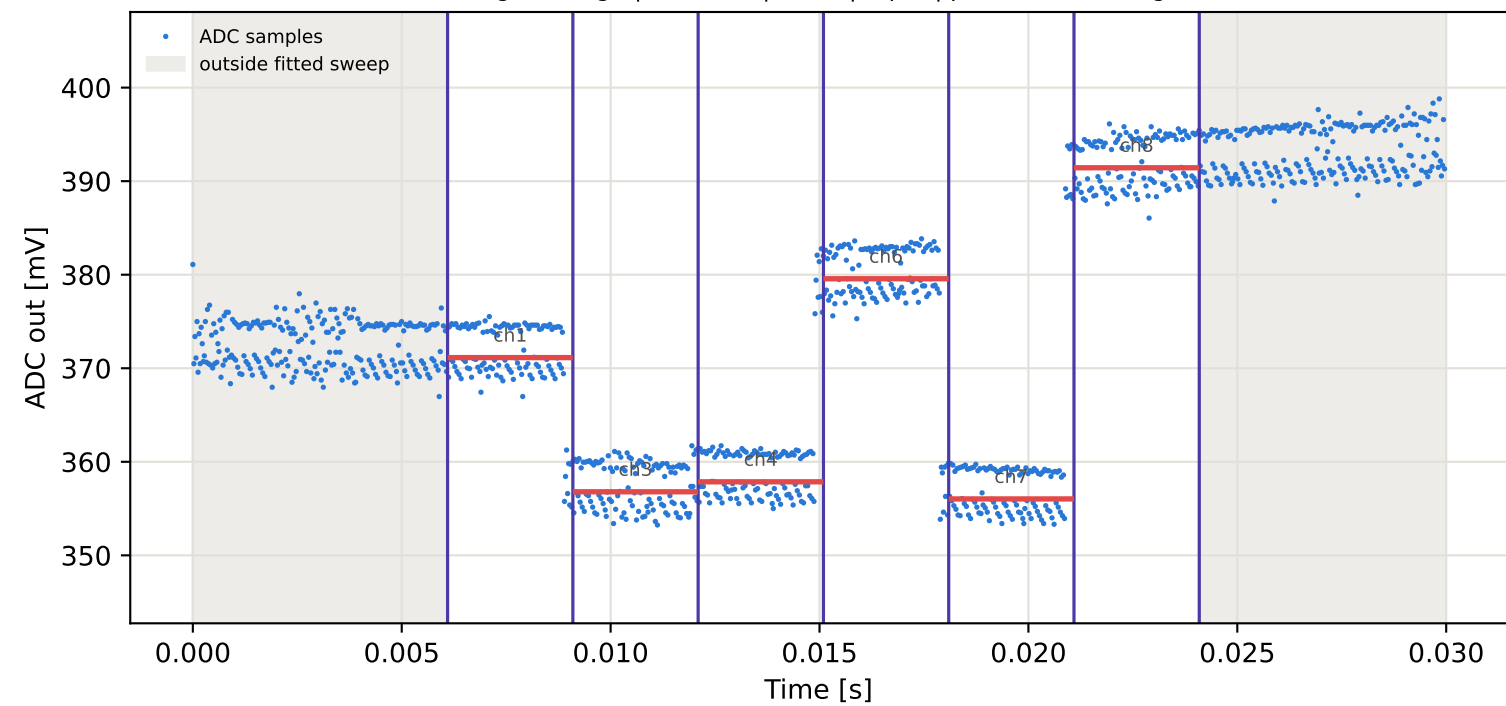
Tag1 &lt;- Tag8 | 875 MHz | run 0 | rep 1 | phase -161.78 deg
