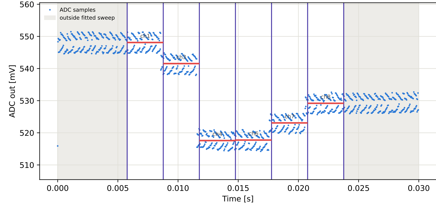
Tag8 &lt;- Tag16 | 835 MHz | run 0 | rep 1 | phase -41.51 deg
