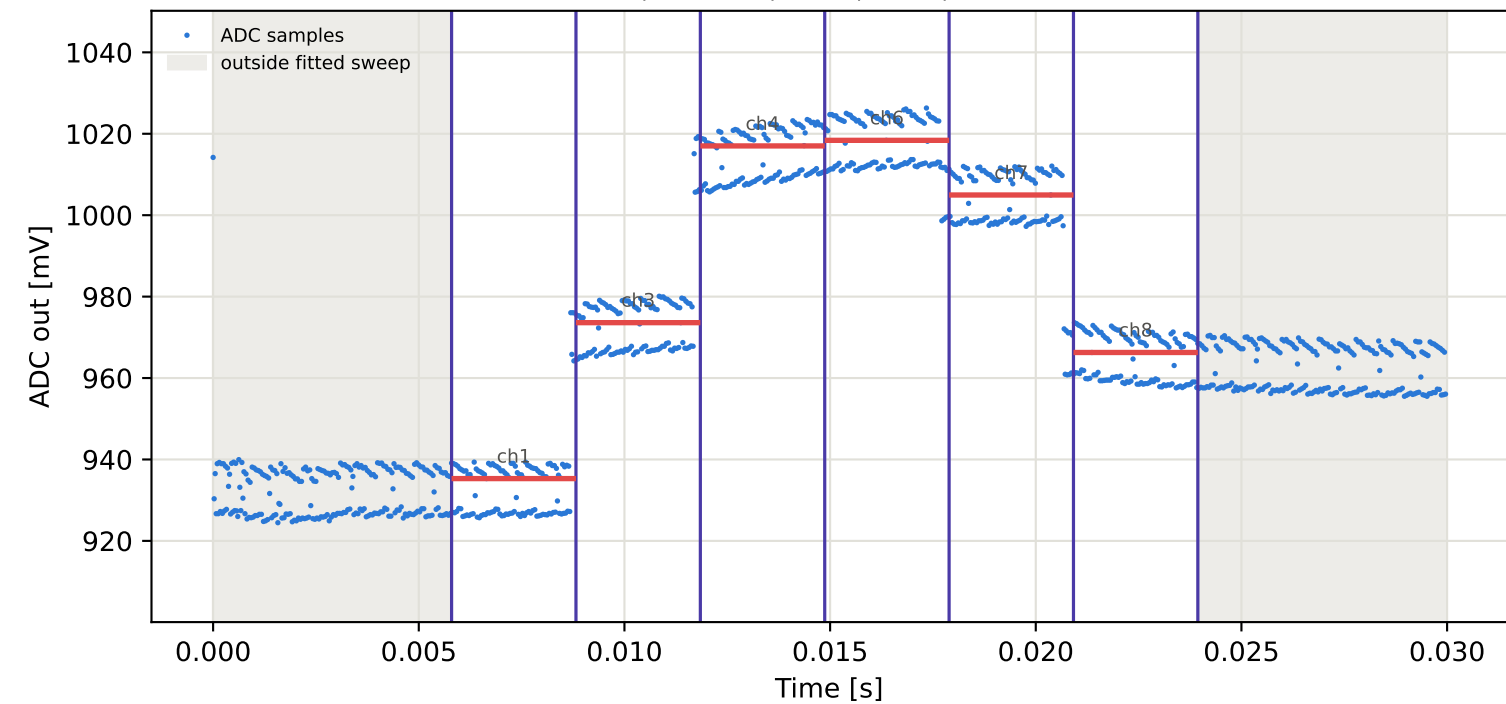
Tag8 &lt;- Tag7 | 895 MHz | run 0 | rep 1 | phase -120.62 deg
