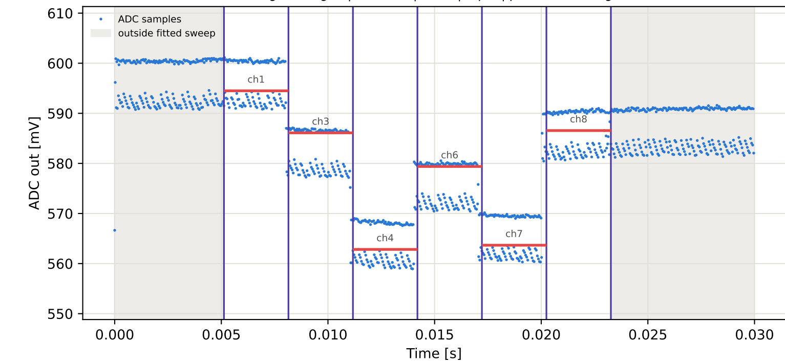
Tag3 &lt;- Tag16 | 835 MHz | run 0 | rep 1 | phase 87.91 deg
