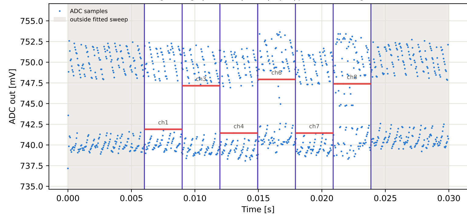
Tag7 &lt;- Tag4 | 945 MHz | run 0 | rep 1 | phase 140.13 deg
