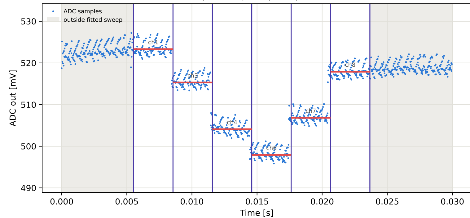
Tag2 &lt;- Tag5 | 895 MHz | run 0 | rep 1 | phase -126.63 deg
