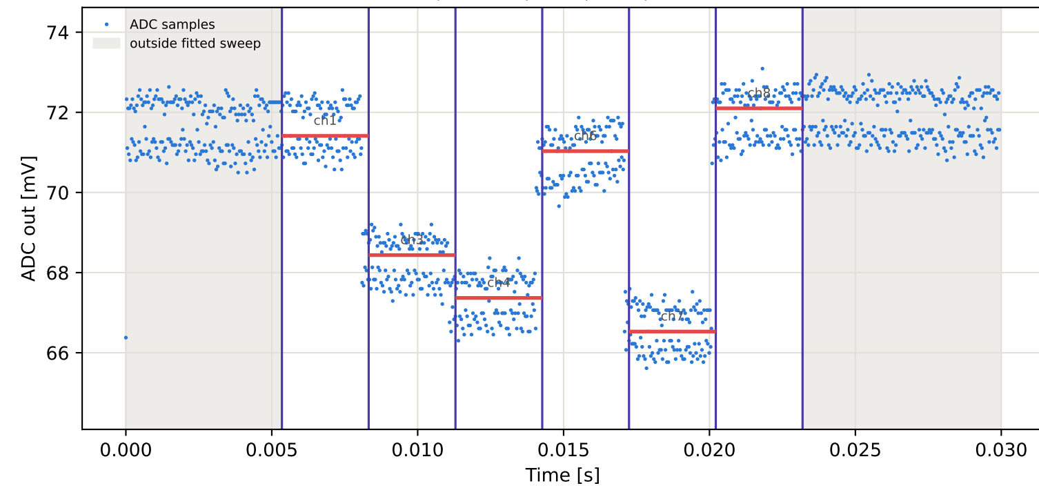
Tag1 &lt;- Tag9 | 785 MHz | run 0 | rep 1 | phase 132.44 deg
