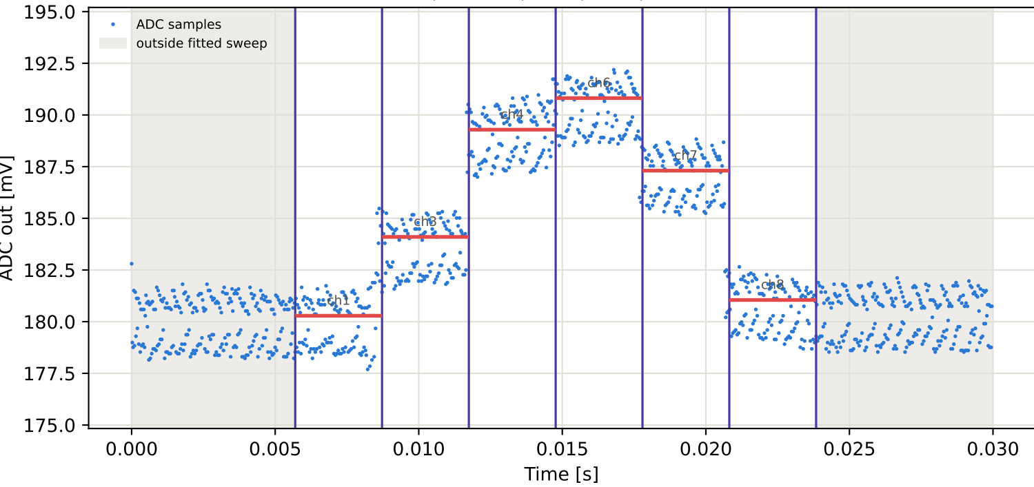
Tag4 &lt;- Tag2 | 905 MHz | run 0 | rep 1 | phase -123.29 deg
