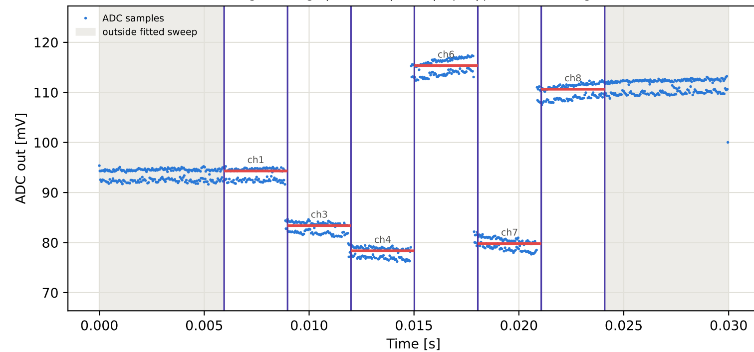
Tag15 &lt;- Tag9 | 925 MHz | run 0 | rep 1 | phase 47.81 deg
