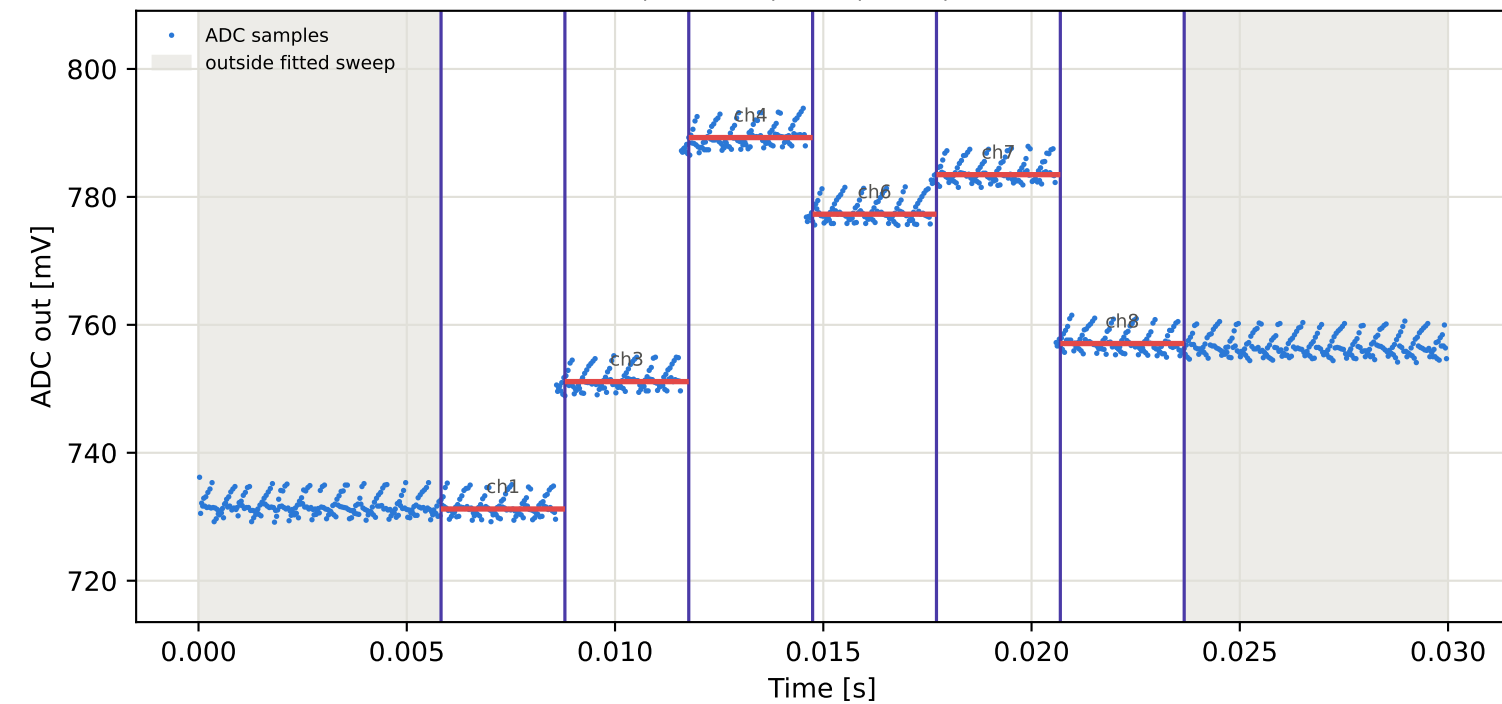
Tag7 &lt;- Tag10 | 825 MHz | run 0 | rep 1 | phase -105.74 deg
