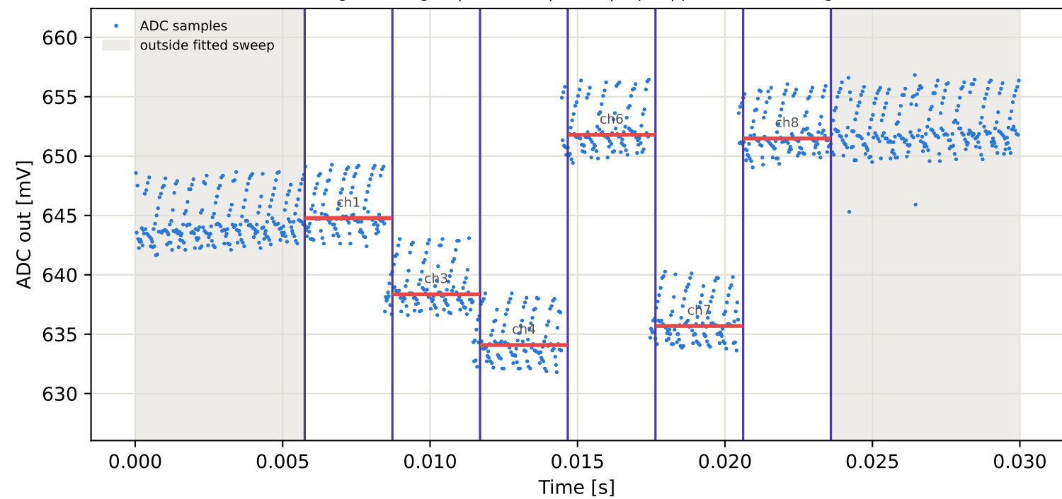
Tag10 &lt;- Tag2 | 945 MHz | run 0 | rep 1 | phase 175.40 deg
