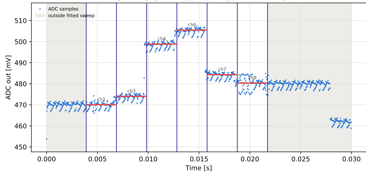
Tag10 &lt;- Tag8 | 955 MHz | run 0 | rep 1 | phase -89.01 deg
