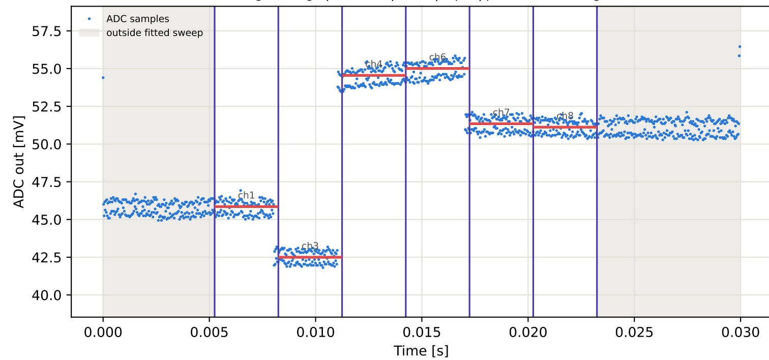
Tag6 &lt;- Tag10 | 785 MHz | run 0 | rep 1 | phase 78.94 deg
