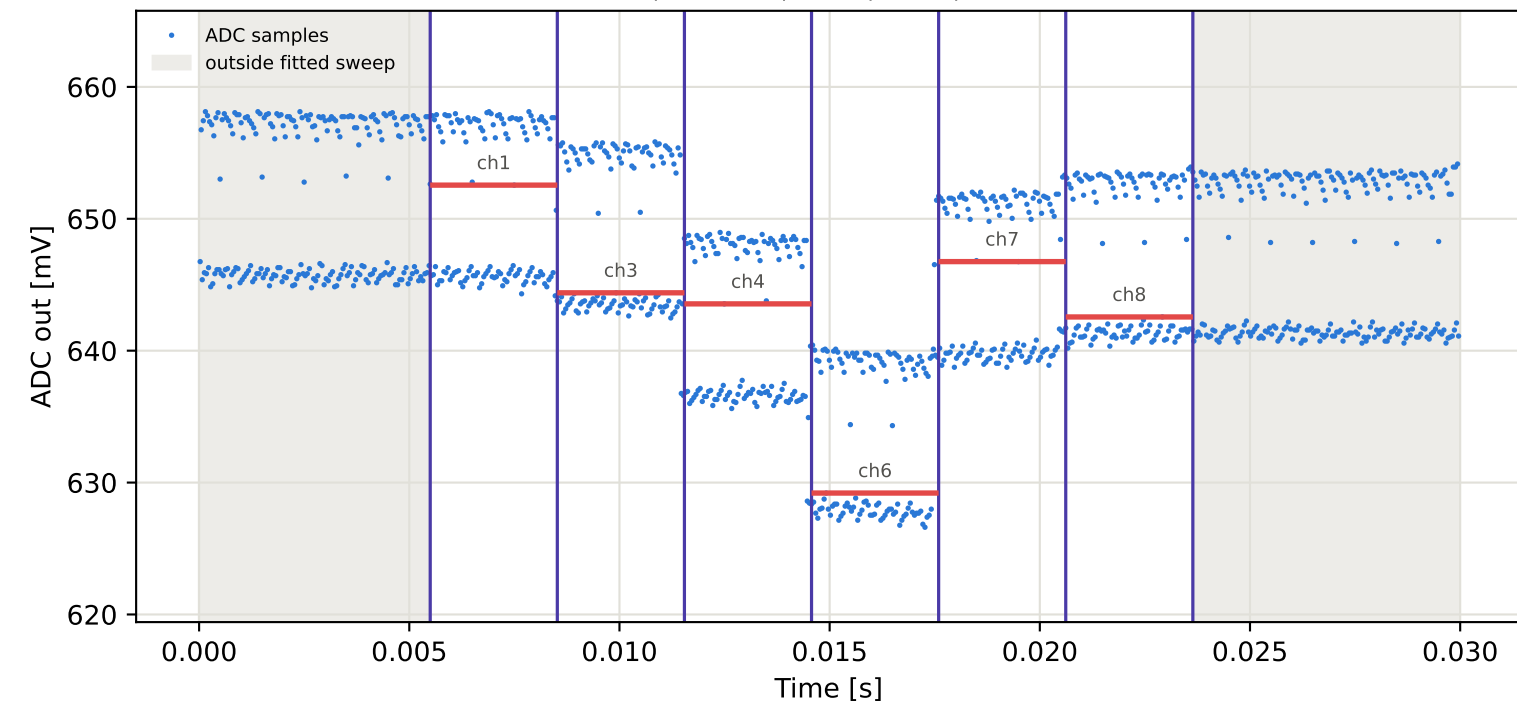
Tag3 &lt;- Tag8 | 925 MHz | run 0 | rep 1 | phase 22.30 deg
