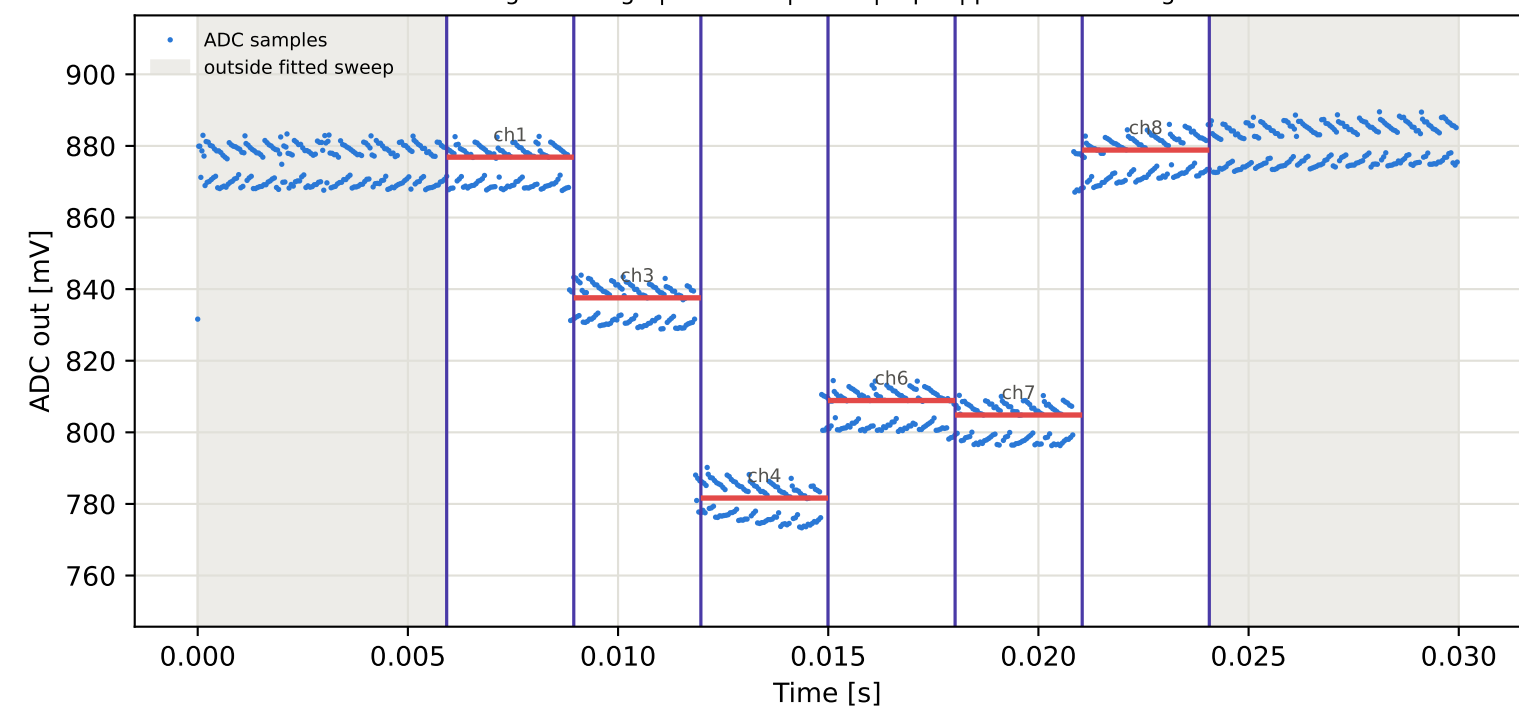
Tag15 &lt;- Tag10 | 925 MHz | run 0 | rep 1 | phase -133.89 deg
