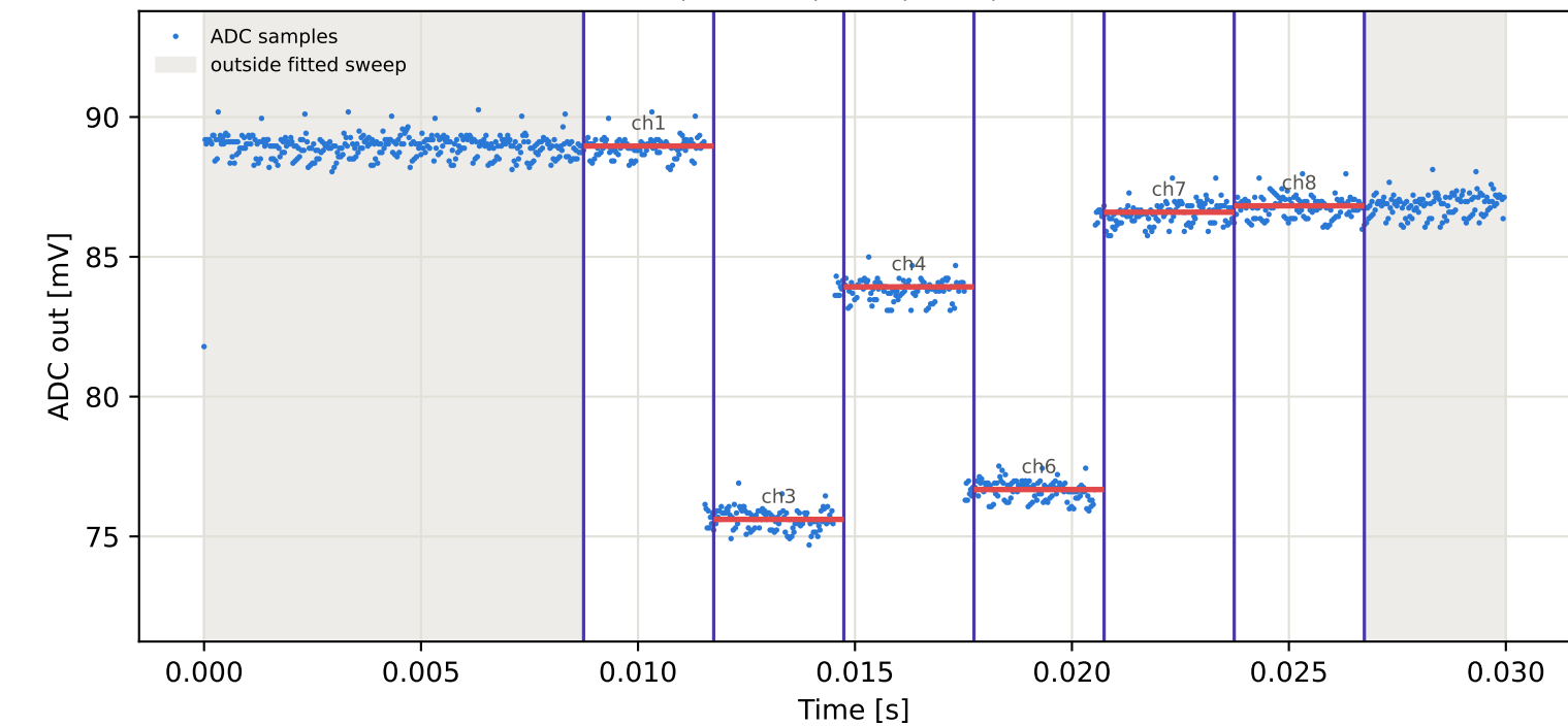
Tag6 &lt;- Tag10 | 775 MHz | run 0 | rep 1 | phase 44.59 deg
