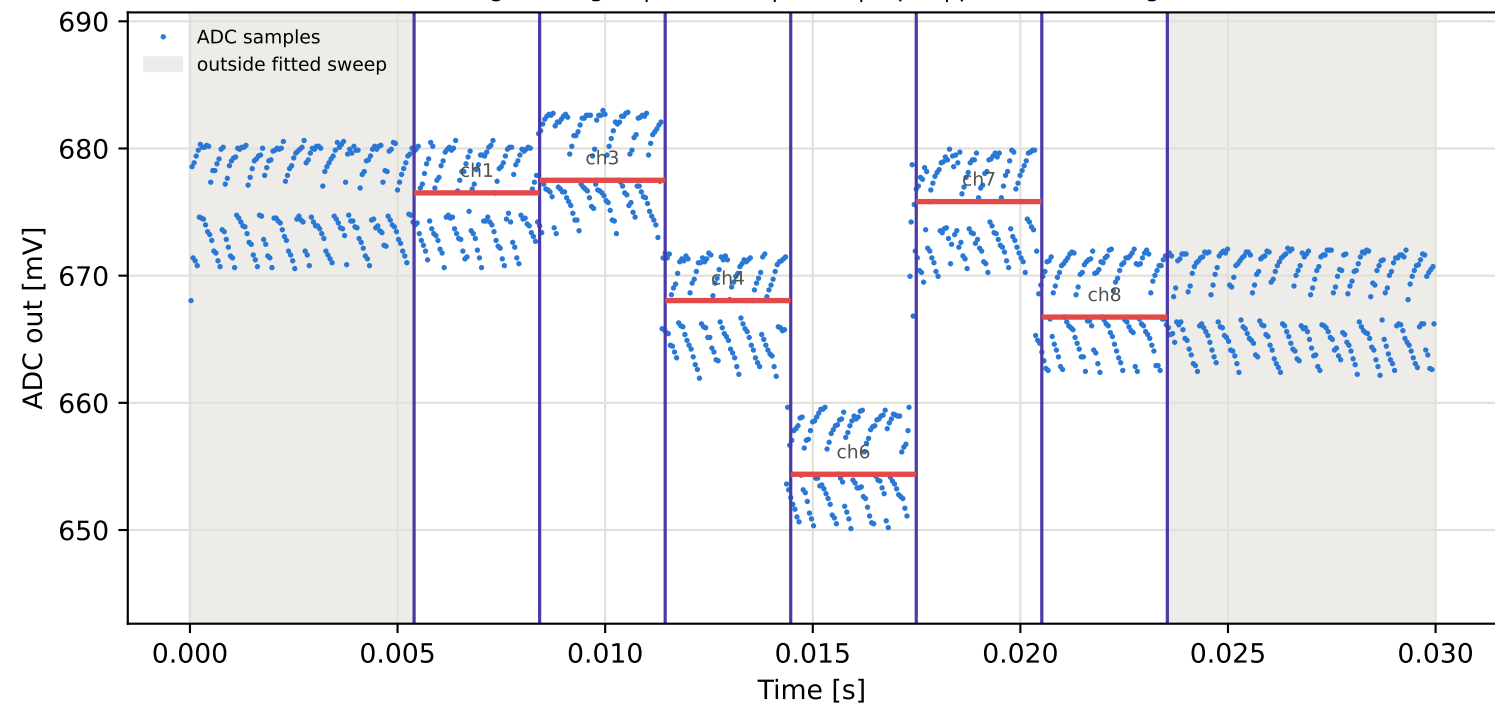
Tag8 &lt;- Tag16 | 975 MHz | run 0 | rep 1 | phase -62.23 deg
