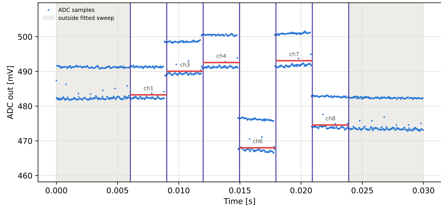
Tag8 &lt;- Tag7 | 985 MHz | run 0 | rep 1 | phase 7.11 deg
