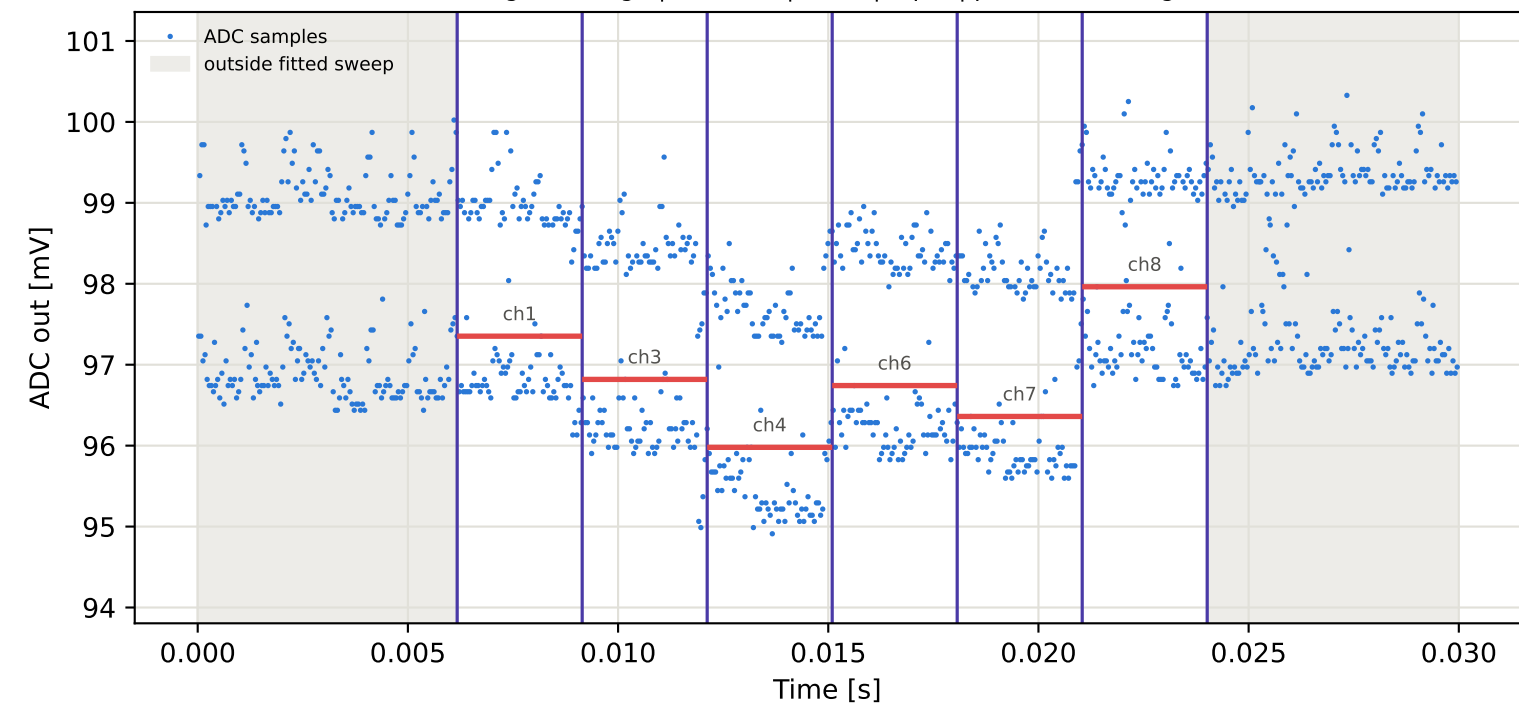
Tag15 &lt;- Tag4 | 995 MHz | run 0 | rep 1 | phase 61.32 deg
