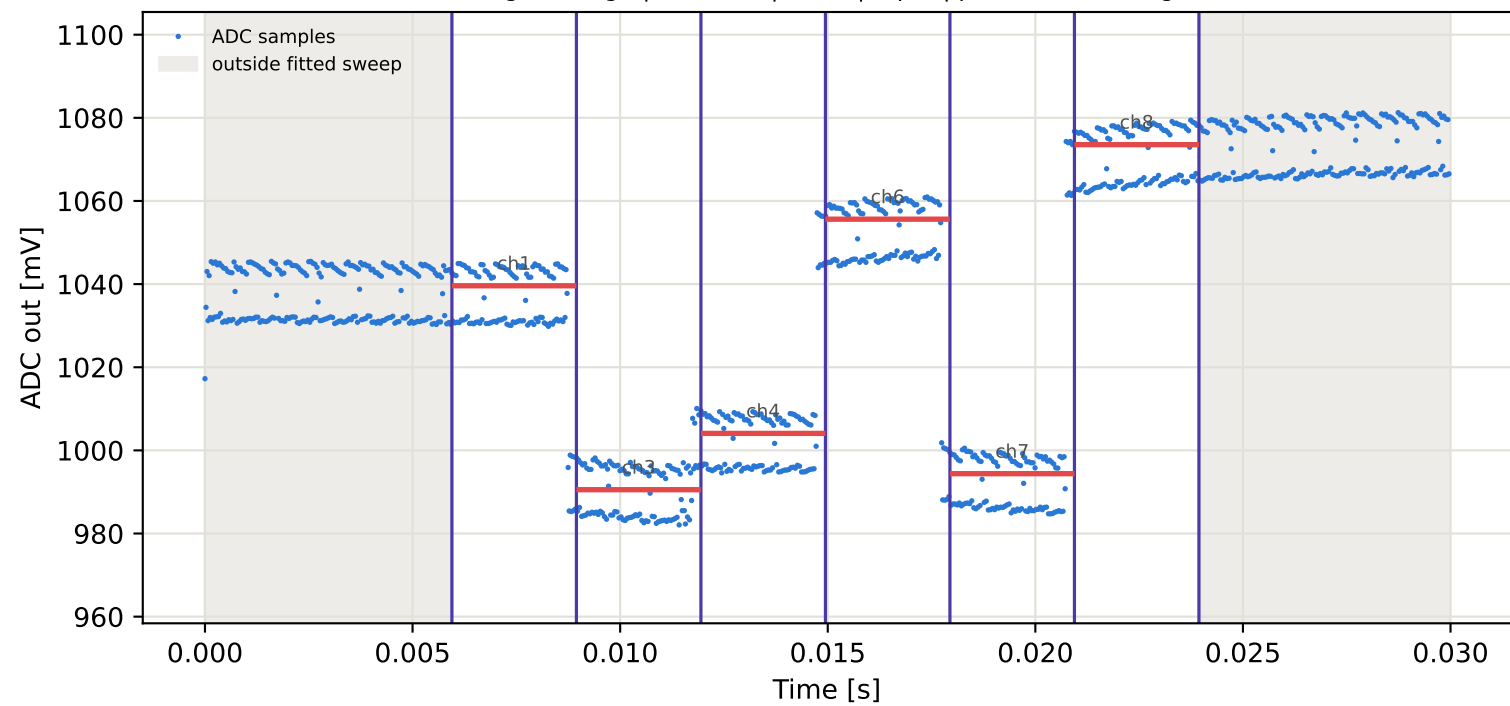
Tag8 &lt;- Tag10 | 875 MHz | run 0 | rep 1 | phase -167.49 deg
