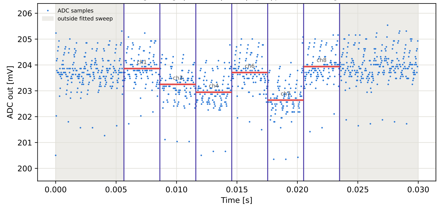
Tag9 &lt;- Tag15 | 795 MHz | run 0 | rep 1 | phase 74.53 deg
