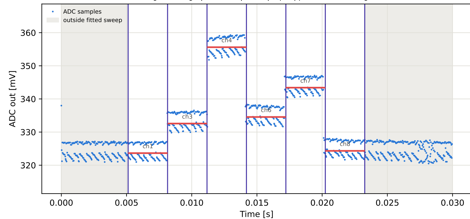
Tag10 &lt;- Tag1 | 975 MHz | run 0 | rep 1 | phase -103.87 deg
