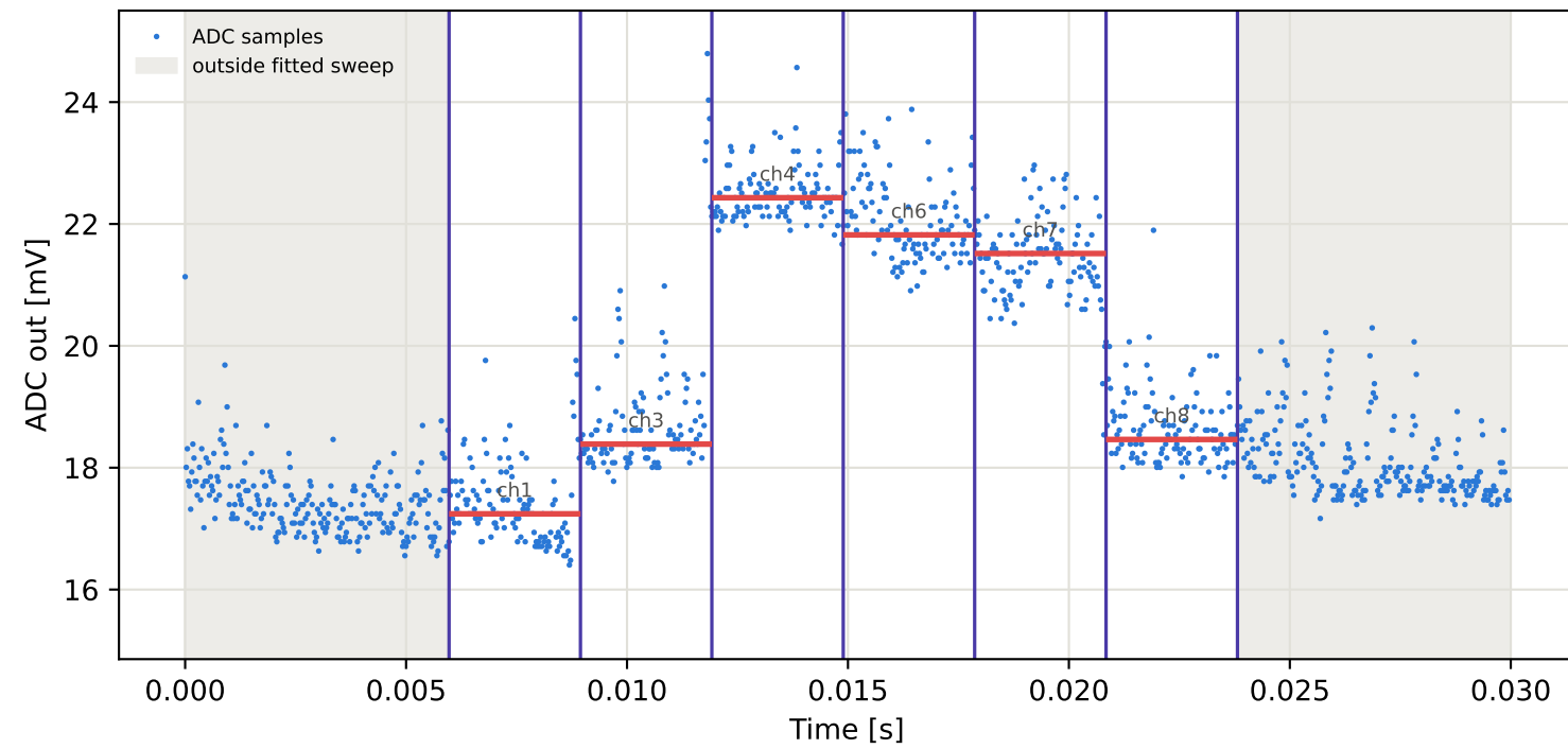
Tag3 &lt;- Tag10 | 955 MHz | run 0 | rep 1 | phase 162.36 deg
