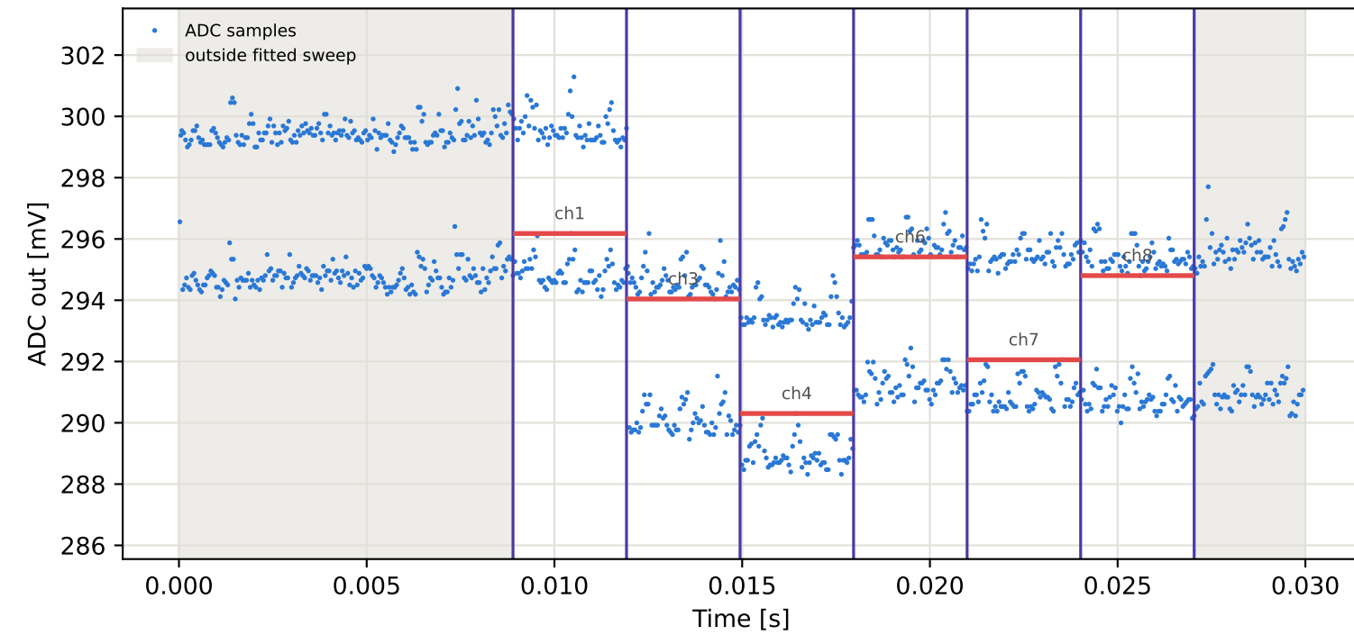
Tag2 &lt;- Tag7 | 845 MHz | run 0 | rep 1 | phase 87.02 deg
