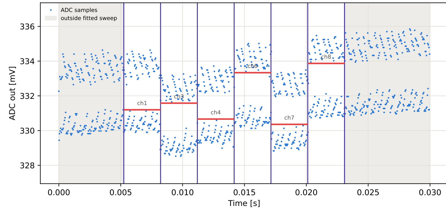
Tag8 &lt;- Tag15 | 865 MHz | run 0 | rep 1 | phase -19.96 deg
