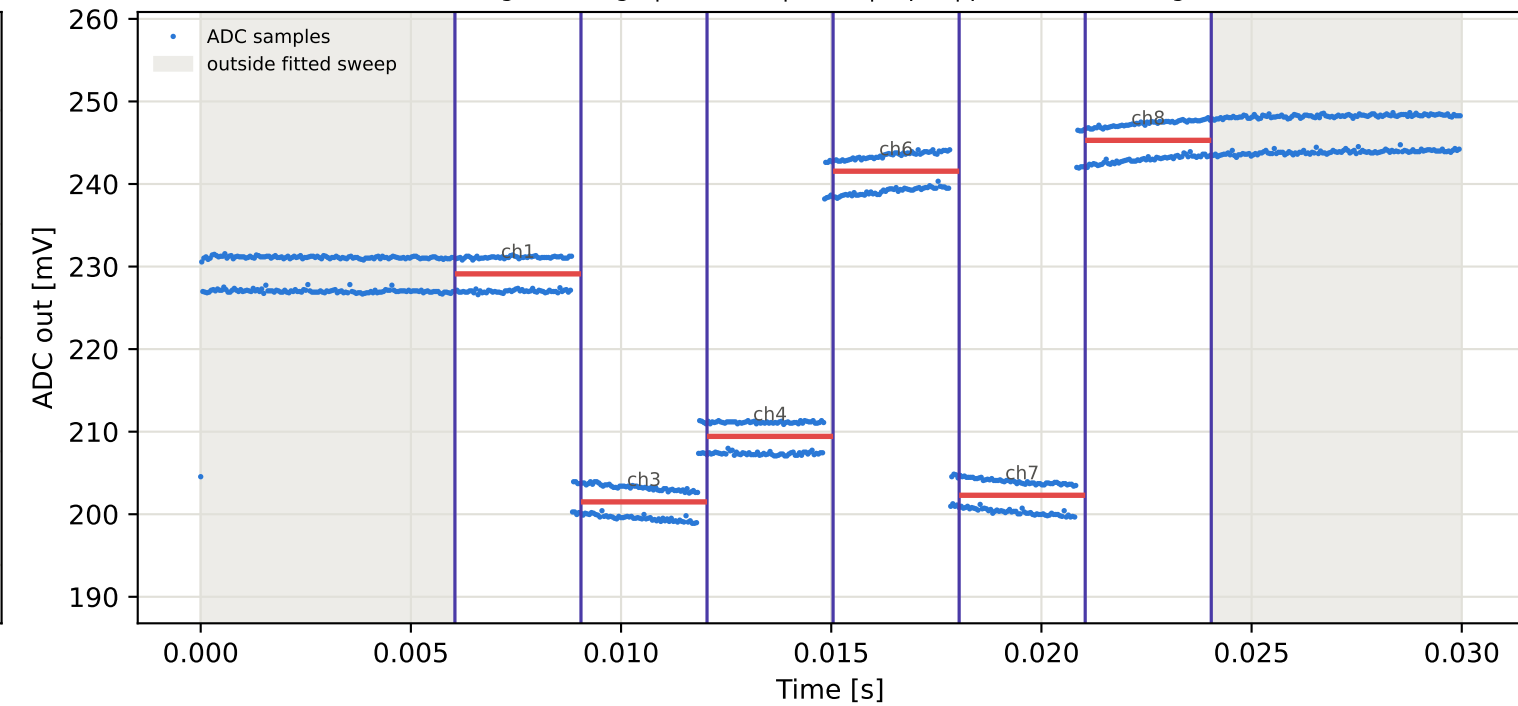
Tag10 &lt;- Tag9 | 805 MHz | run 0 | rep 1 | phase -19.77 deg
