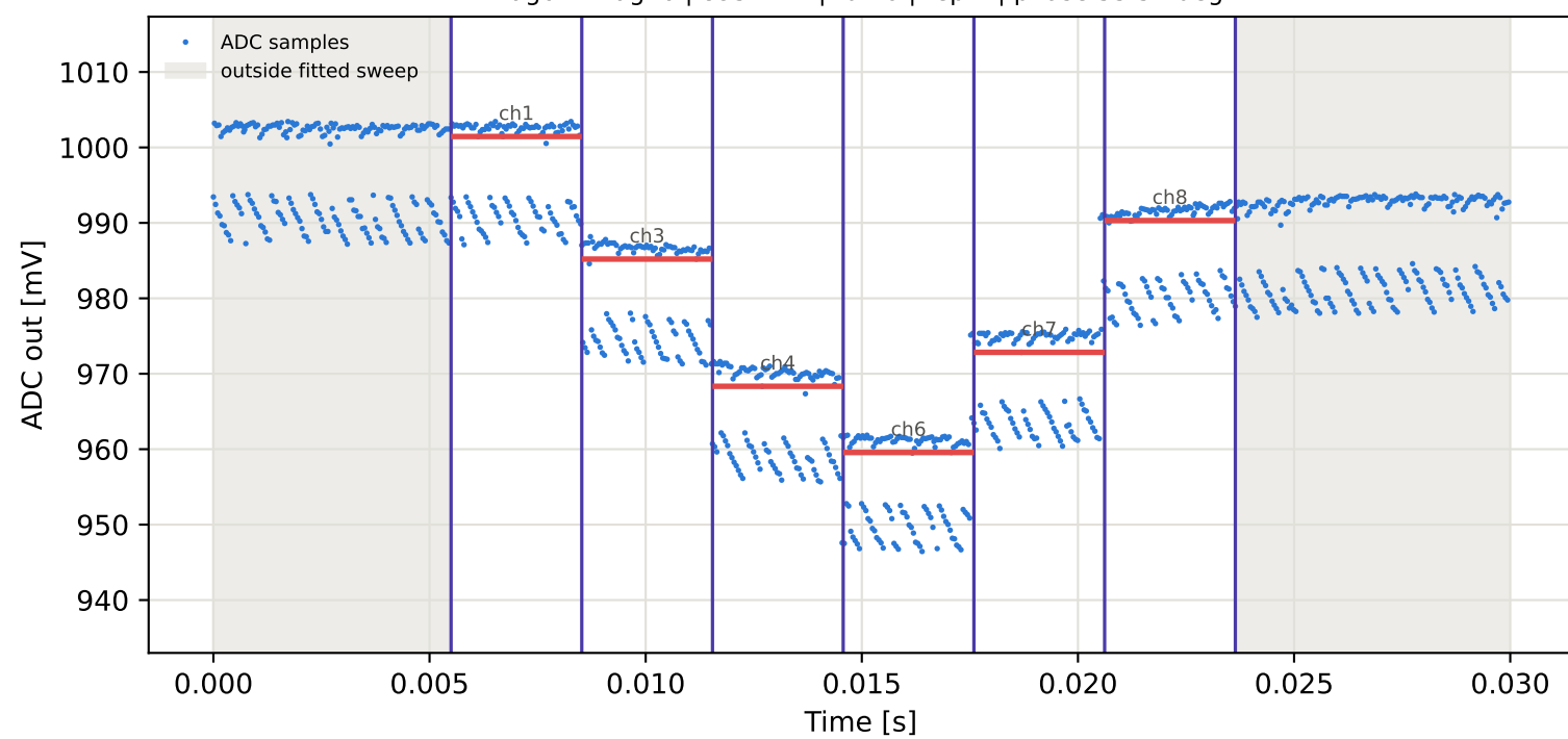
Tag6 &lt;- Tag3 | 895 MHz | run 0 | rep 1 | phase 104.57 deg
