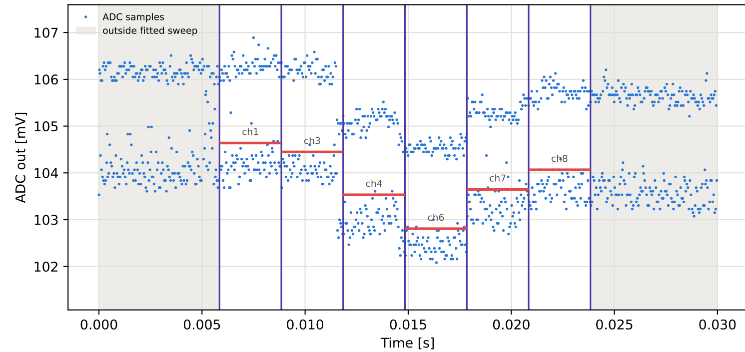
Tag1 &lt;- Tag4 | 795 MHz | run 0 | rep 1 | phase -96.14 deg
