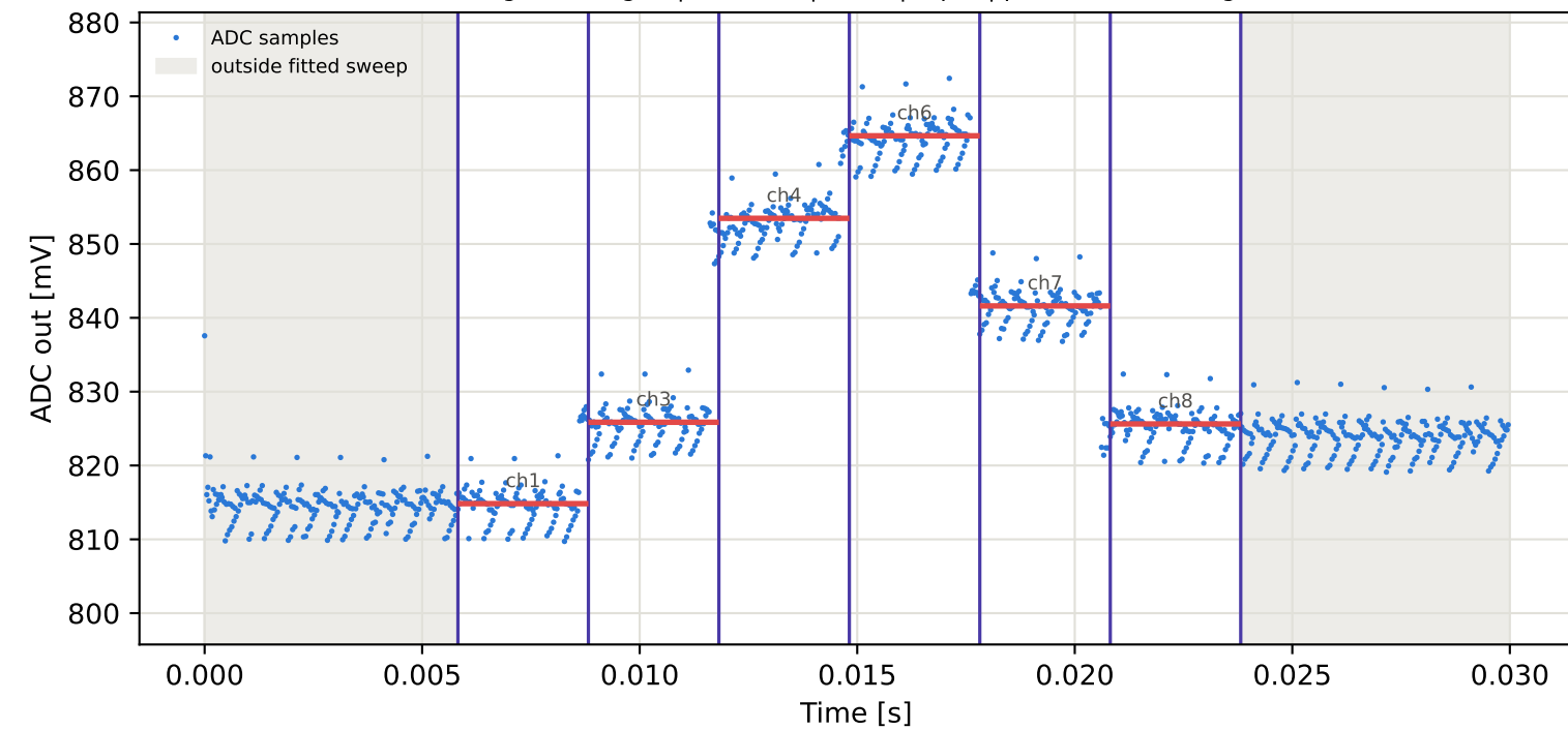
Tag10 &lt;- Tag3 | 925 MHz | run 0 | rep 1 | phase 55.57 deg
