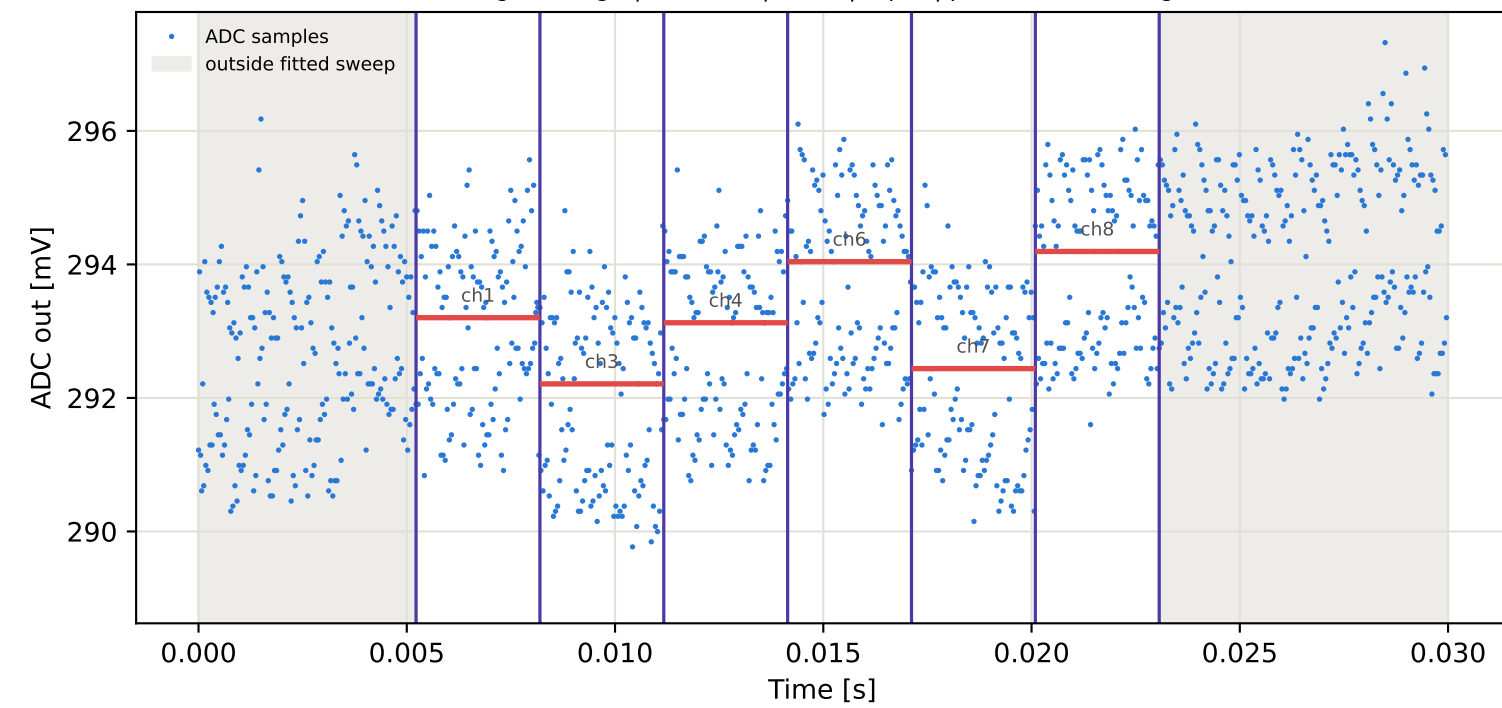
Tag2 &lt;- Tag5 | 845 MHz | run 0 | rep 1 | phase 102.08 deg
