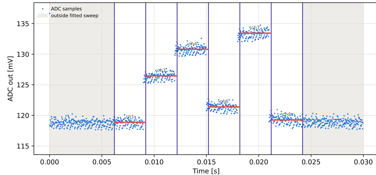
Tag3 &lt;- Tag8 | 785 MHz | run 0 | rep 1 | phase -57.14 deg
