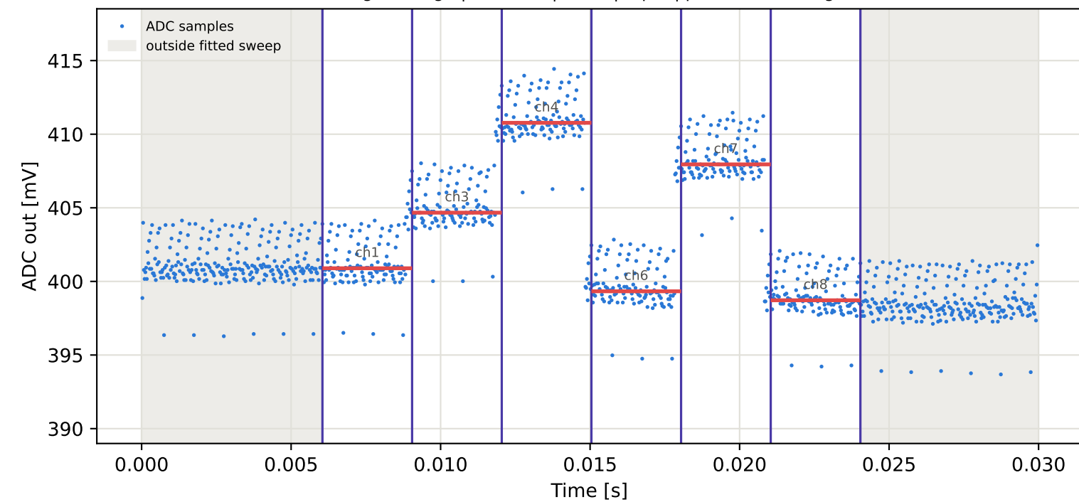
Tag1 &lt;- Tag9 | 955 MHz | run 0 | rep 1 | phase -101.35 deg
