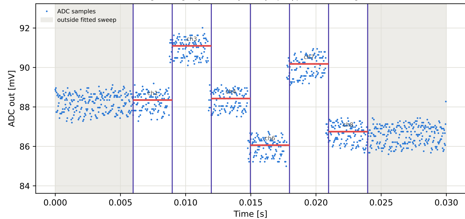
Tag5 &lt;- Tag2 | 795 MHz | run 0 | rep 1 | phase -123.81 deg
