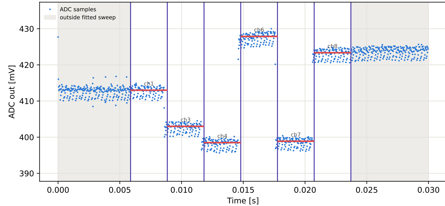
Tag3 &lt;- Tag2 | 985 MHz | run 0 | rep 1 | phase -164.02 deg
