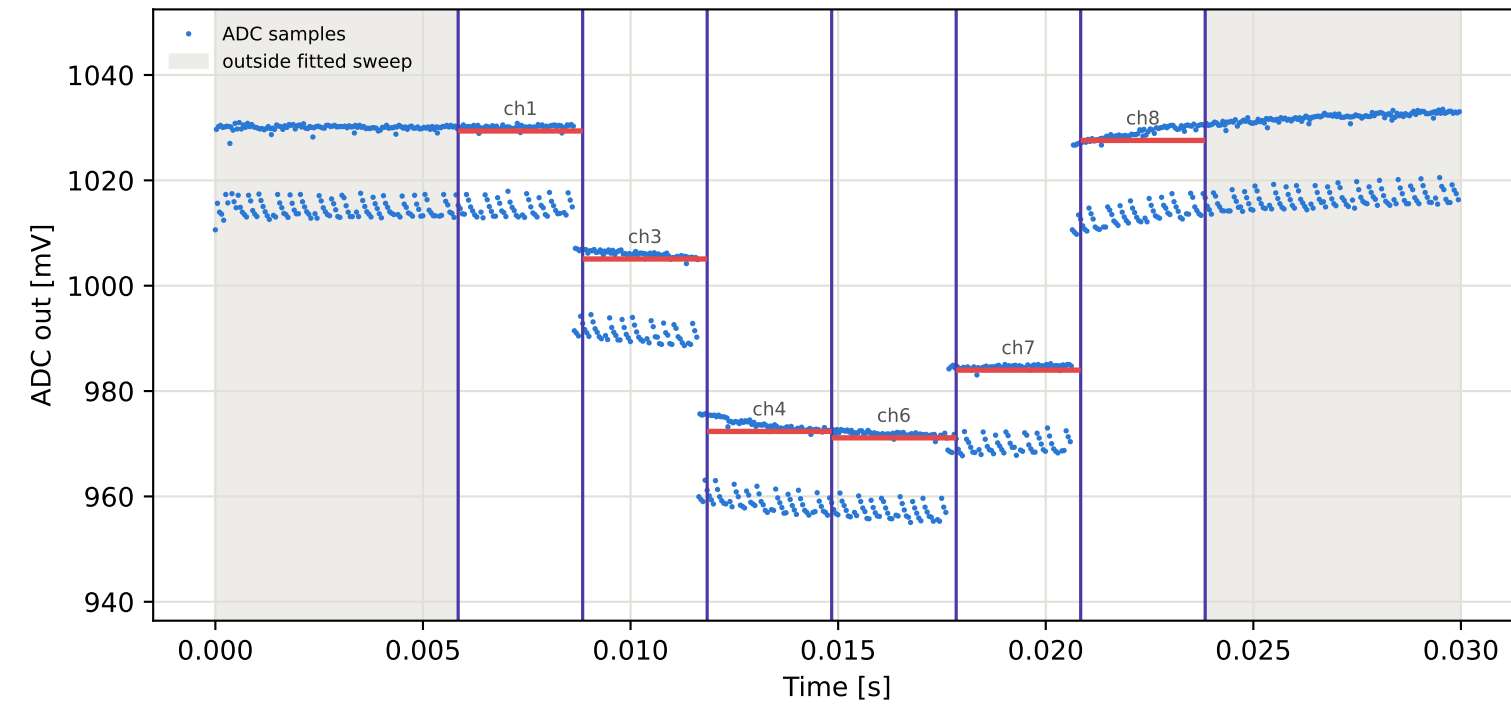
Tag3 &lt;- Tag8 | 905 MHz | run 0 | rep 1 | phase 13.74 deg
