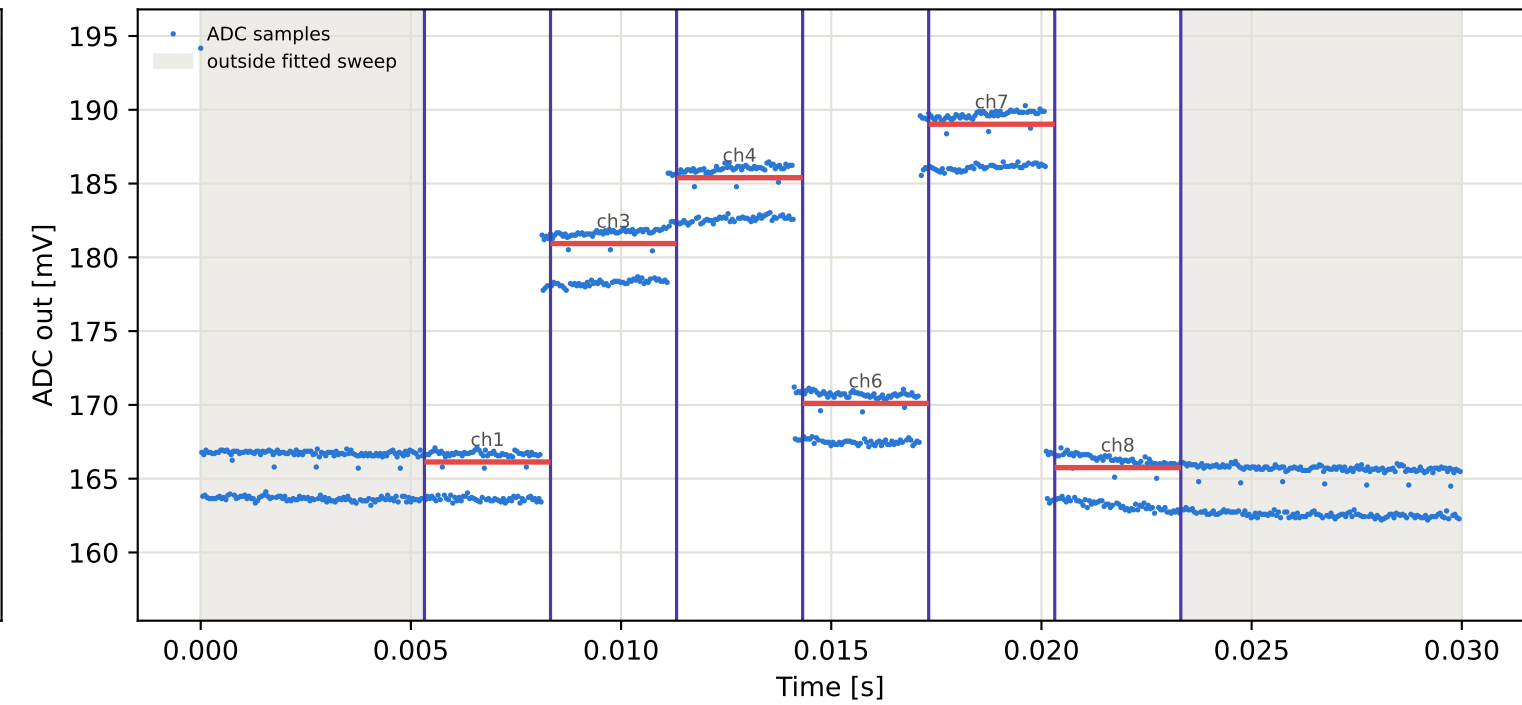
Tag15 &lt;- Tag10 | 785 MHz | run 0 | rep 1 | phase 40.05 deg
