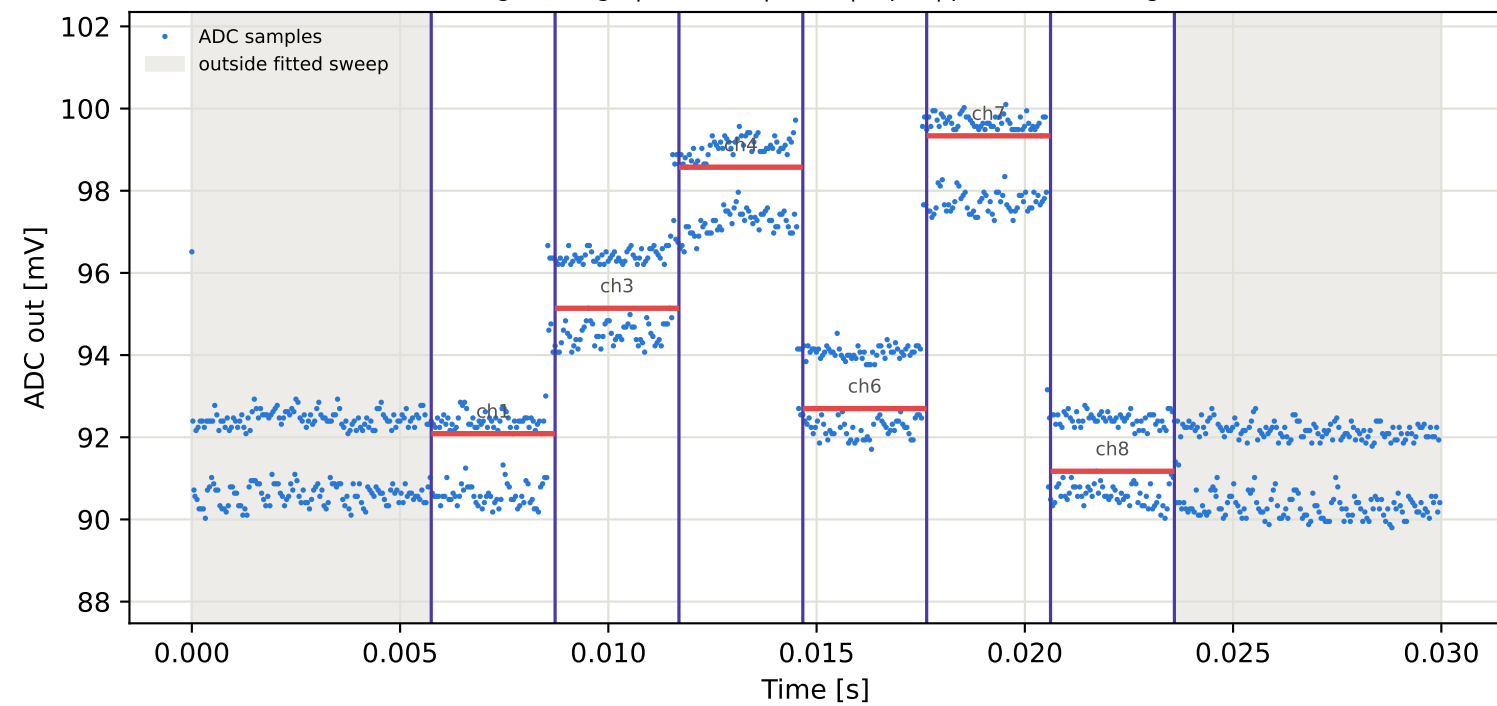
Tag4 &lt;- Tag8 | 795 MHz | run 0 | rep 1 | phase 111.80 deg
