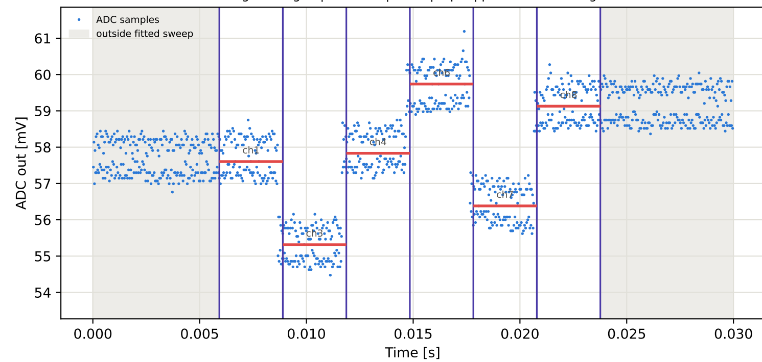
Tag1 &lt;- Tag2 | 805 MHz | run 0 | rep 1 | phase 83.59 deg
