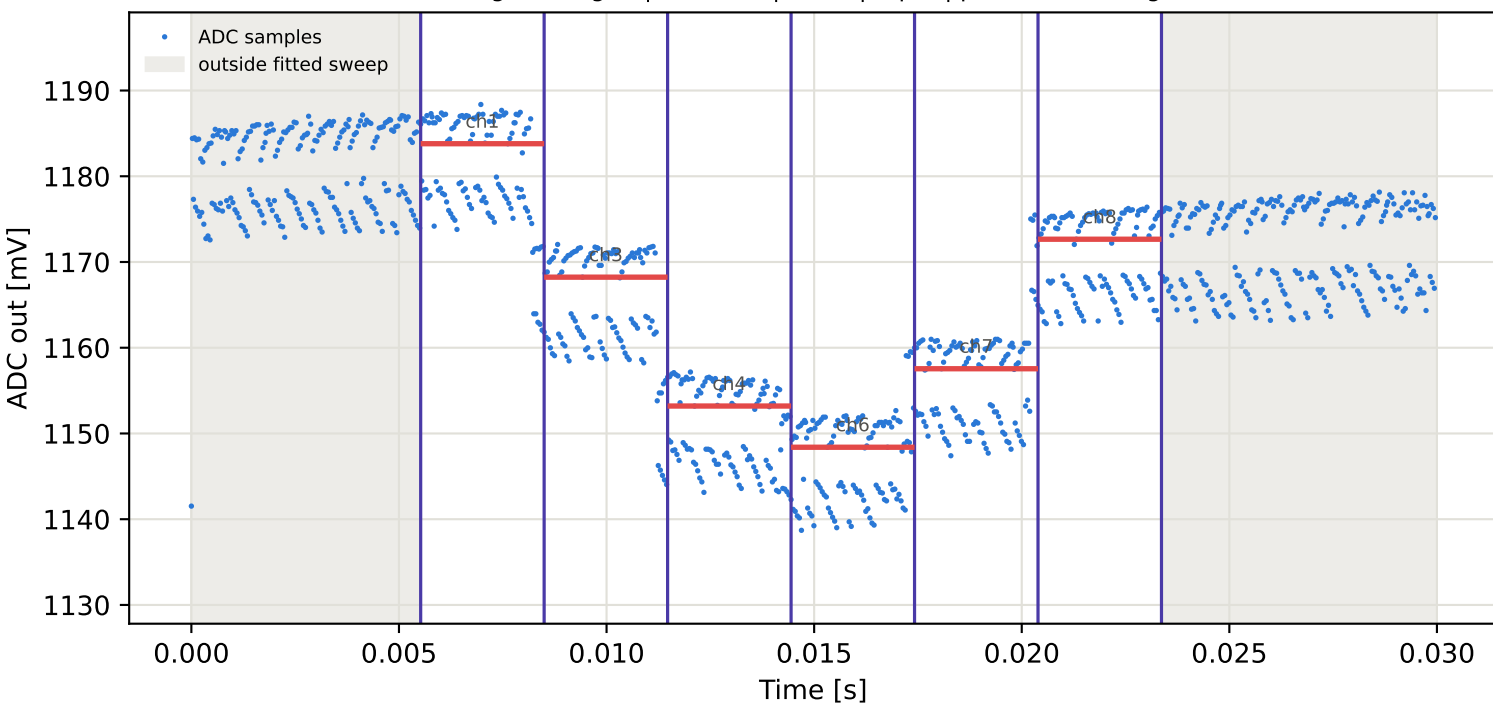
Tag9 &lt;- Tag16 | 875 MHz | run 0 | rep 1 | phase 74.82 deg
