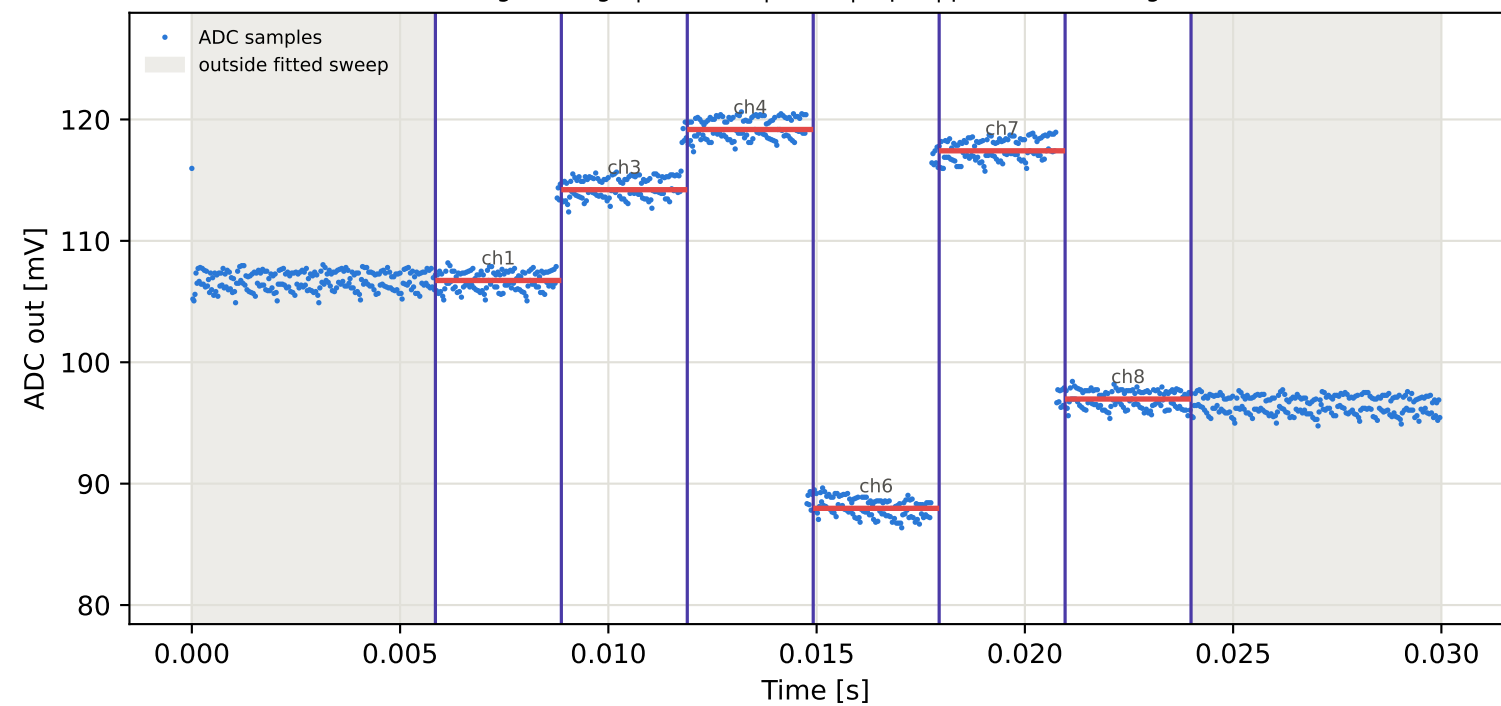
Tag4 &lt;- Tag3 | 975 MHz | run 0 | rep 1 | phase -30.11 deg
