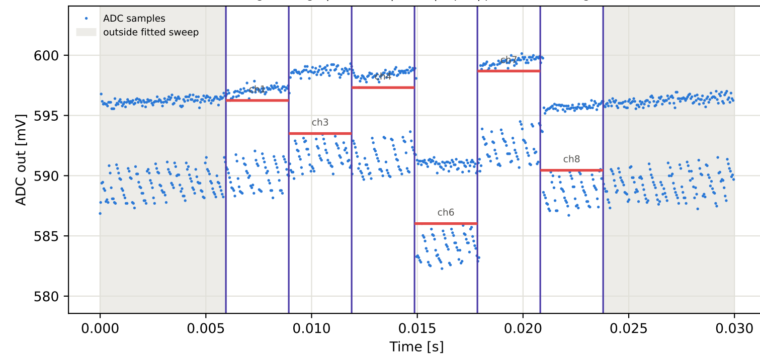
Tag8 &lt;- Tag4 | 875 MHz | run 0 | rep 1 | phase -84.47 deg
