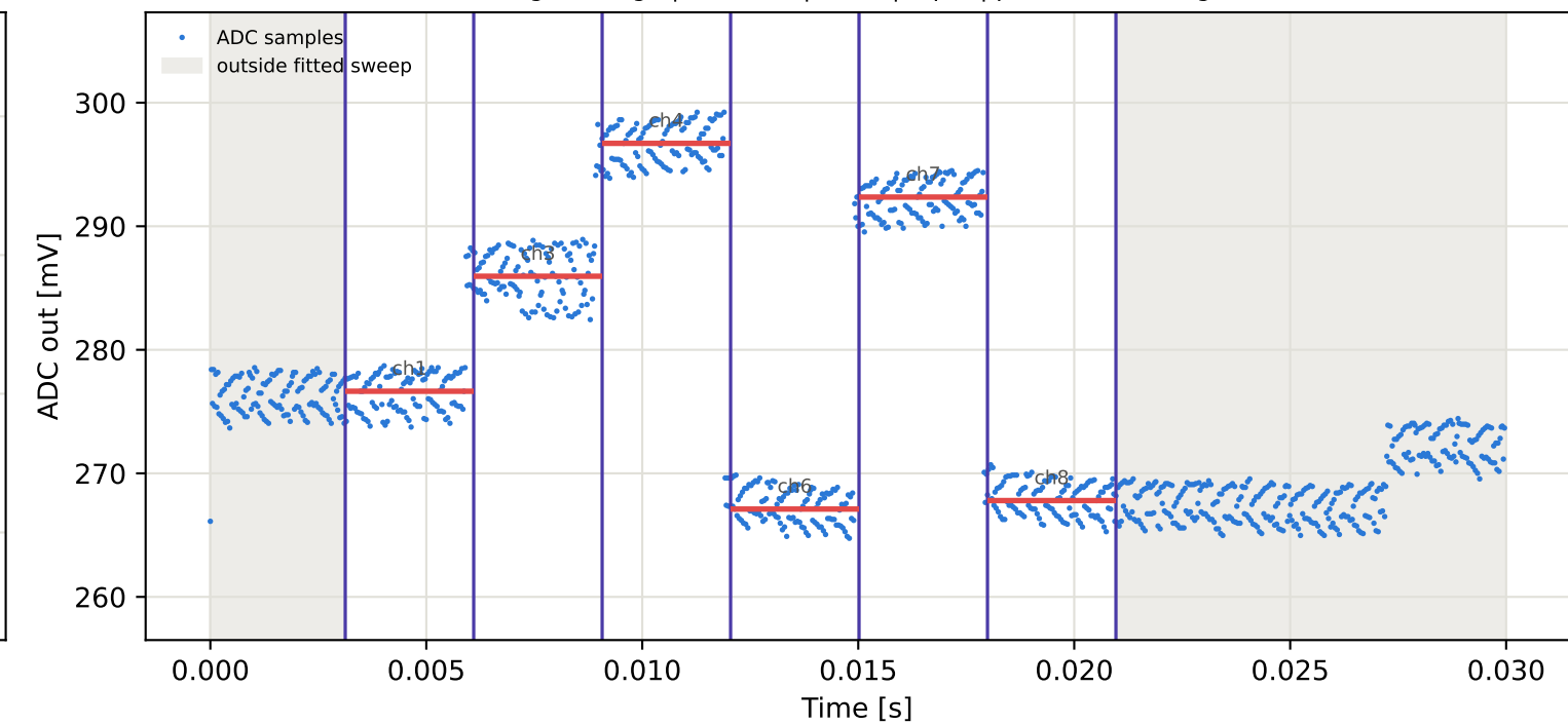
Tag4 &lt;- Tag8 | 955 MHz | run 0 | rep 1 | phase -61.48 deg
