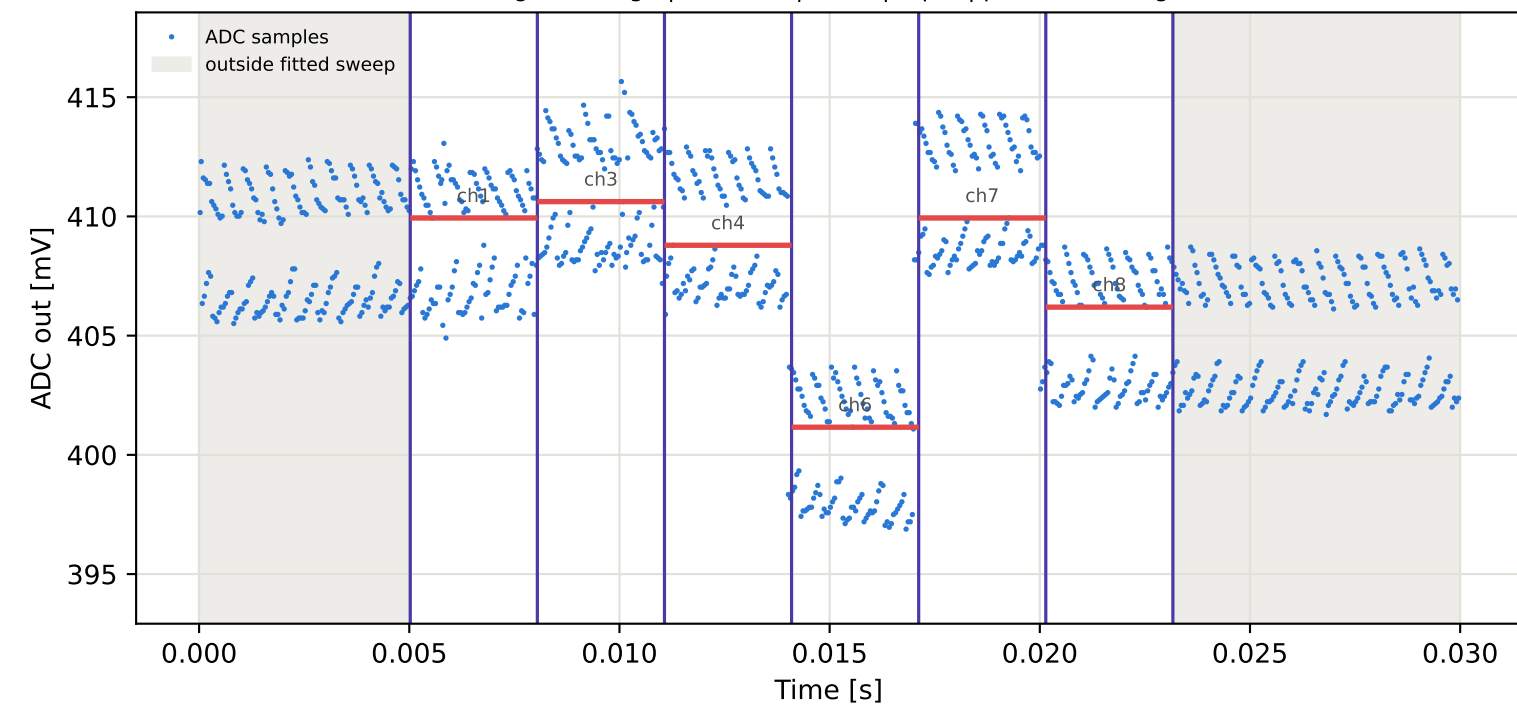
Tag16 &lt;- Tag6 | 975 MHz | run 0 | rep 1 | phase -153.86 deg
