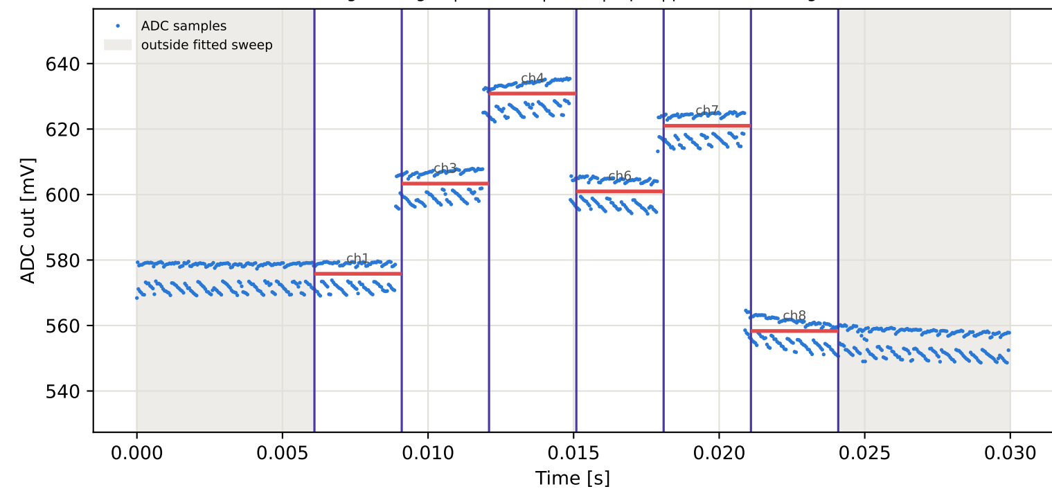
Tag6 &lt;- Tag10 | 905 MHz | run 0 | rep 1 | phase -87.21 deg
