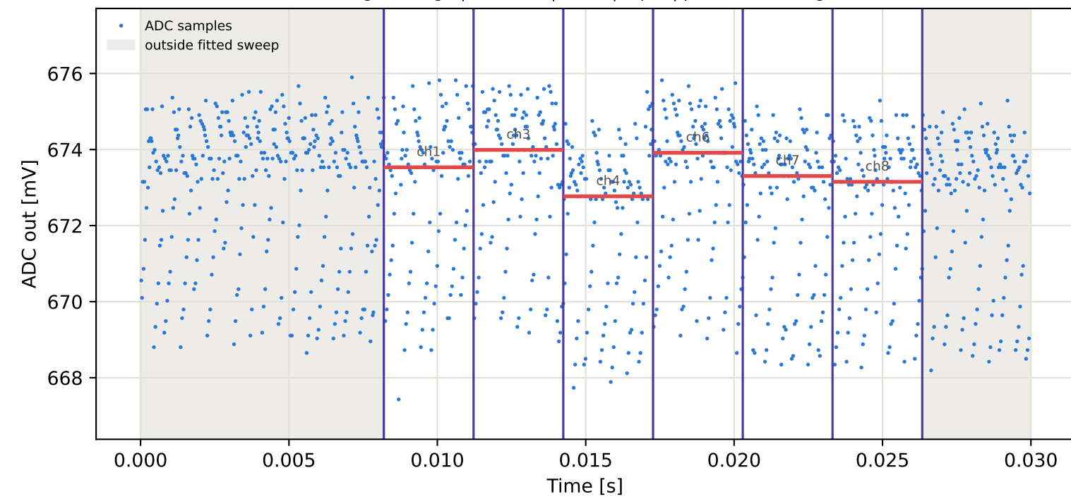
Tag8 &lt;- Tag4 | 975 MHz | run 0 | rep 1 | phase -20.61 deg
