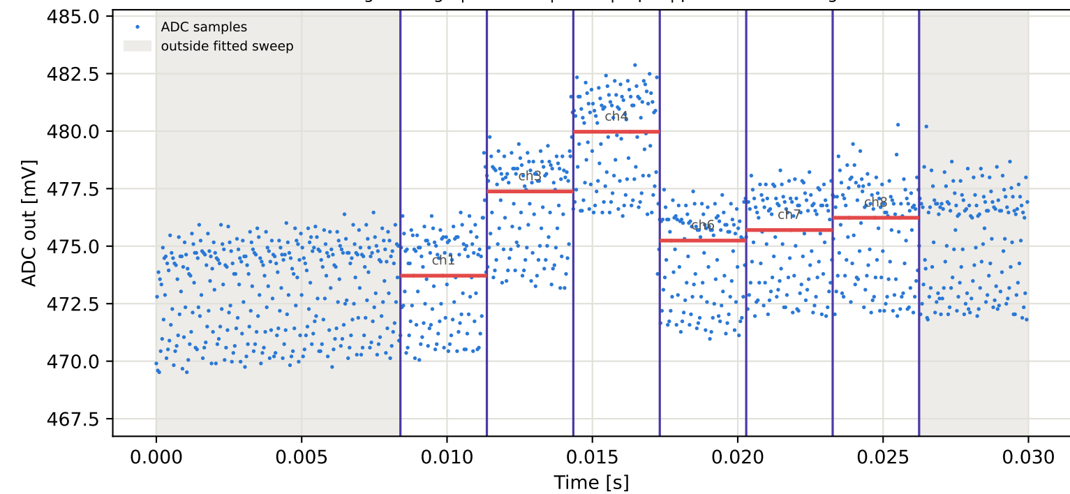
Tag3 &lt;- Tag6 | 965 MHz | run 0 | rep 1 | phase 137.51 deg
