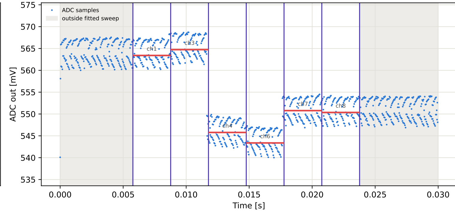
Tag8 &lt;- Tag16 | 825 MHz | run 0 | rep 1 | phase -53.04 deg
