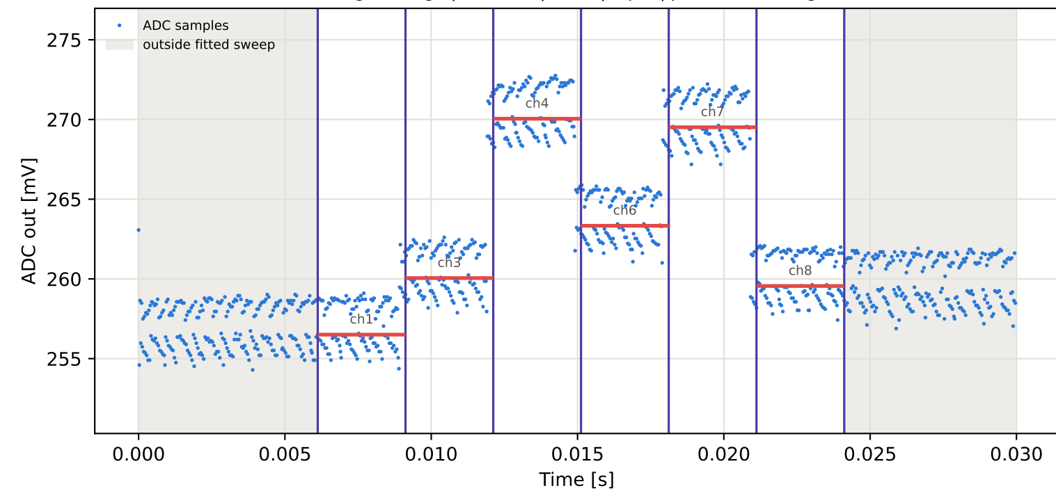
Tag8 &lt;- Tag1 | 795 MHz | run 0 | rep 1 | phase 45.66 deg
