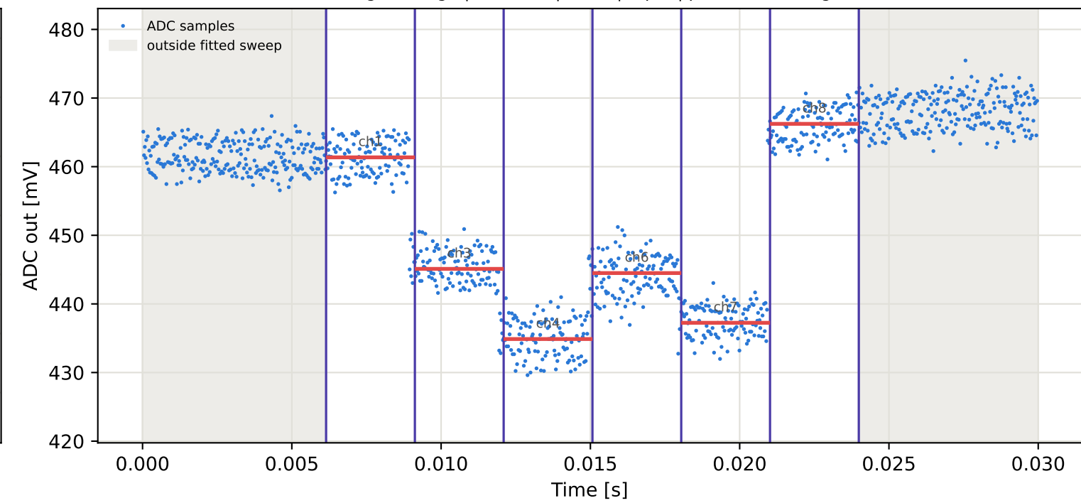
Tag4 &lt;- Tag8 | 885 MHz | run 0 | rep 1 | phase -108.15 deg
