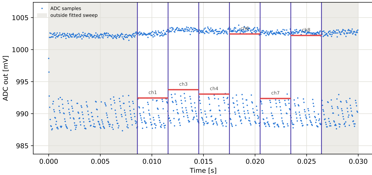
Tag7 &lt;- Tag15 | 845 MHz | run 0 | rep 1 | phase -4.48 deg
