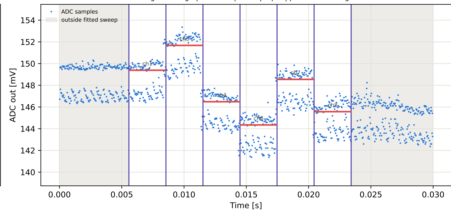
Tag15 &lt;- Tag6 | 835 MHz | run 0 | rep 1 | phase 30.95 deg
