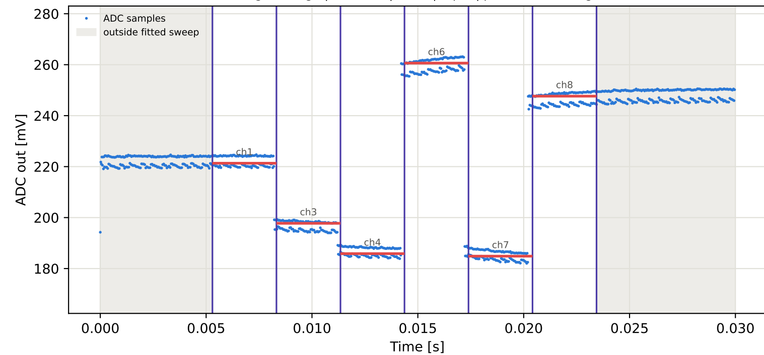
Tag4 &lt;- Tag15 | 985 MHz | run 0 | rep 1 | phase -76.96 deg
