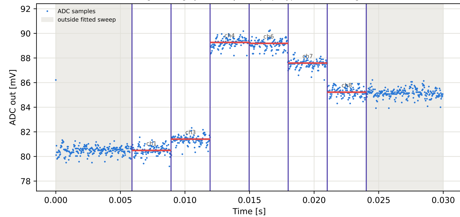
Tag15 &lt;- Tag9 | 795 MHz | run 0 | rep 1 | phase -148.66 deg
