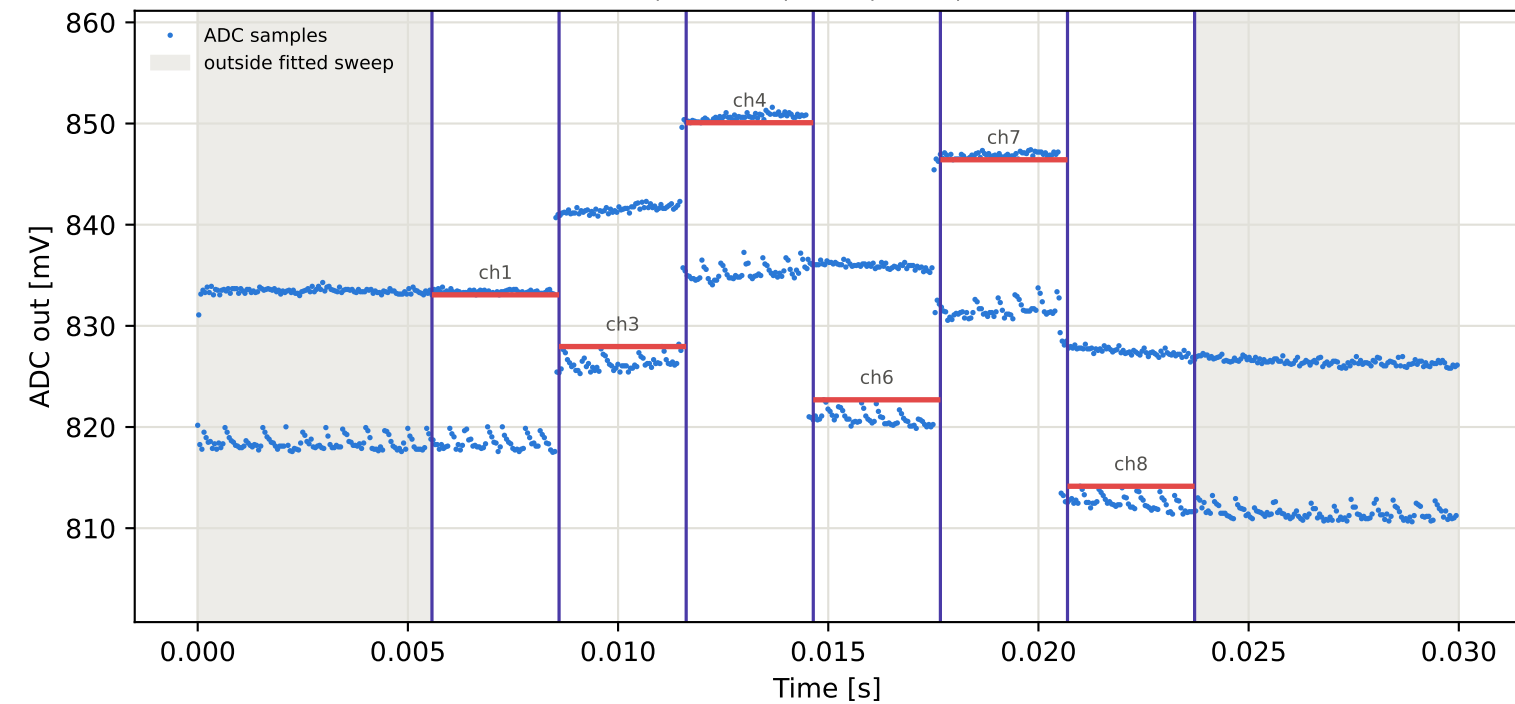
Tag10 &lt;- Tag5 | 925 MHz | run 0 | rep 1 | phase -71.07 deg
