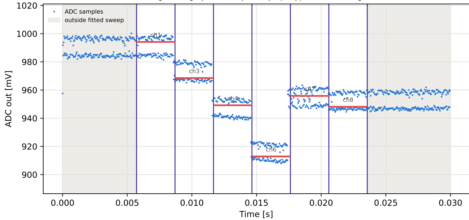
Tag9 &lt;- Tag8 | 885 MHz | run 0 | rep 1 | phase 35.86 deg
