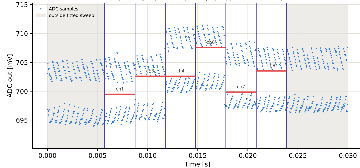
Tag8 &lt;- Tag15 | 965 MHz | run 0 | rep 1 | phase -165.99 deg
