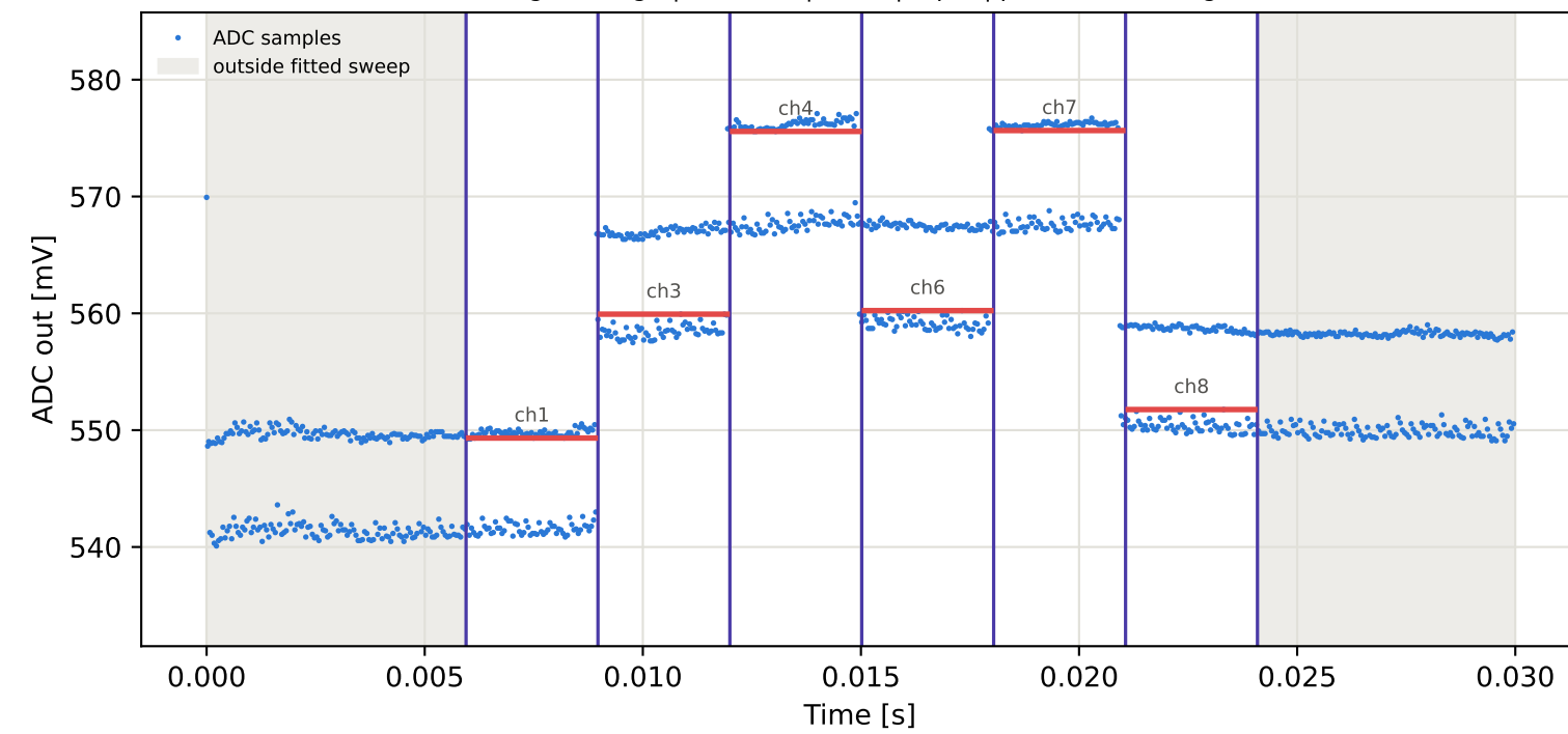
Tag3 &lt;- Tag6 | 835 MHz | run 0 | rep 1 | phase -105.39 deg
