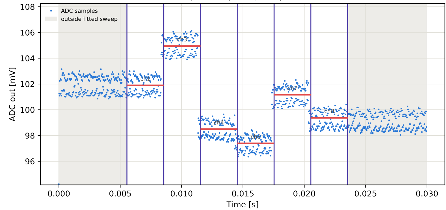
Tag4 &lt;- Tag8 | 775 MHz | run 0 | rep 1 | phase 144.53 deg
