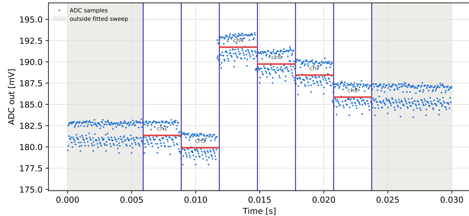
Tag3 &lt;- Tag2 | 805 MHz | run 0 | rep 1 | phase 171.00 deg
