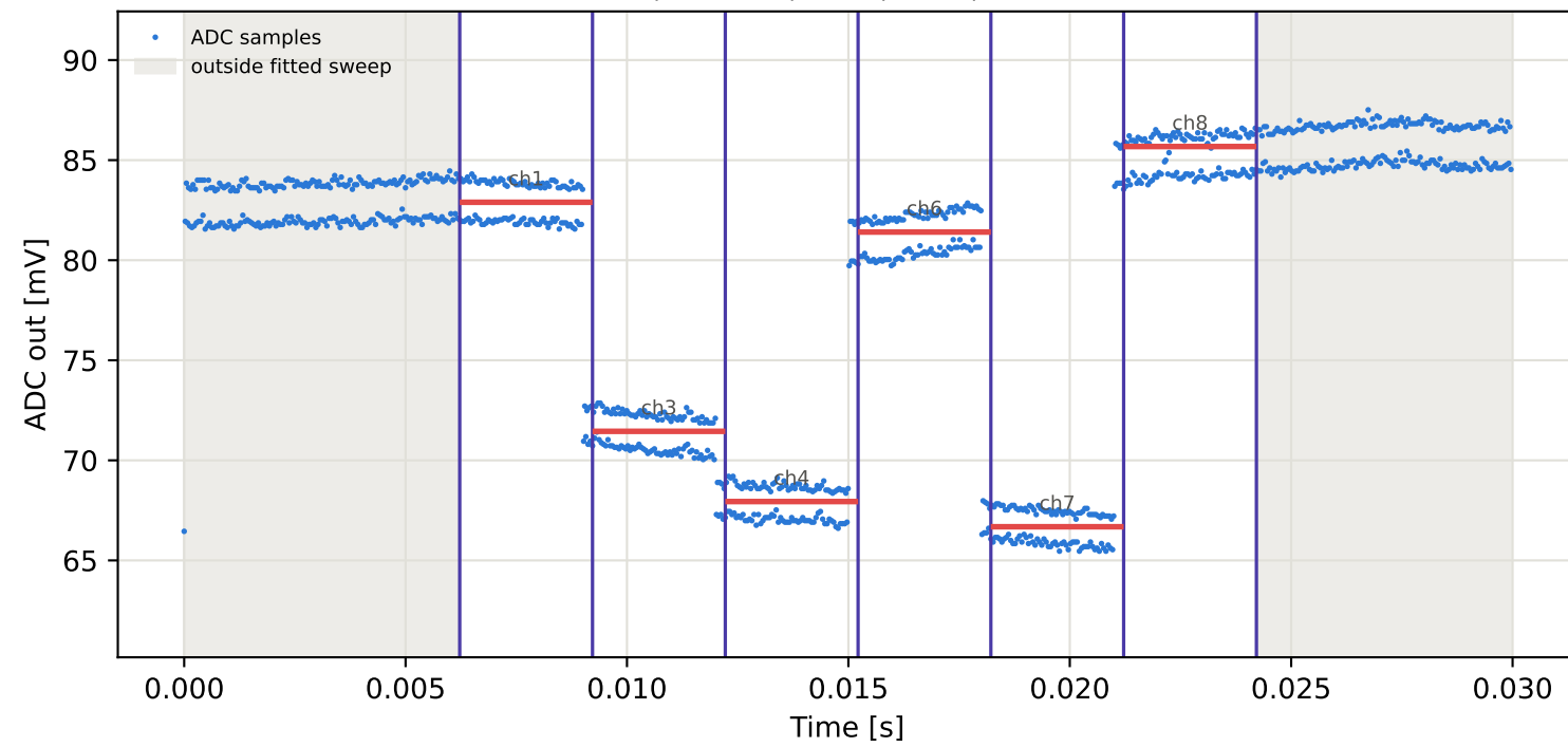
Tag1 &lt;- Tag9 | 835 MHz | run 0 | rep 1 | phase 127.29 deg
