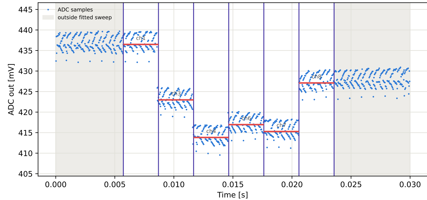
Tag8 &lt;- Tag16 | 855 MHz | run 0 | rep 1 | phase 6.29 deg
