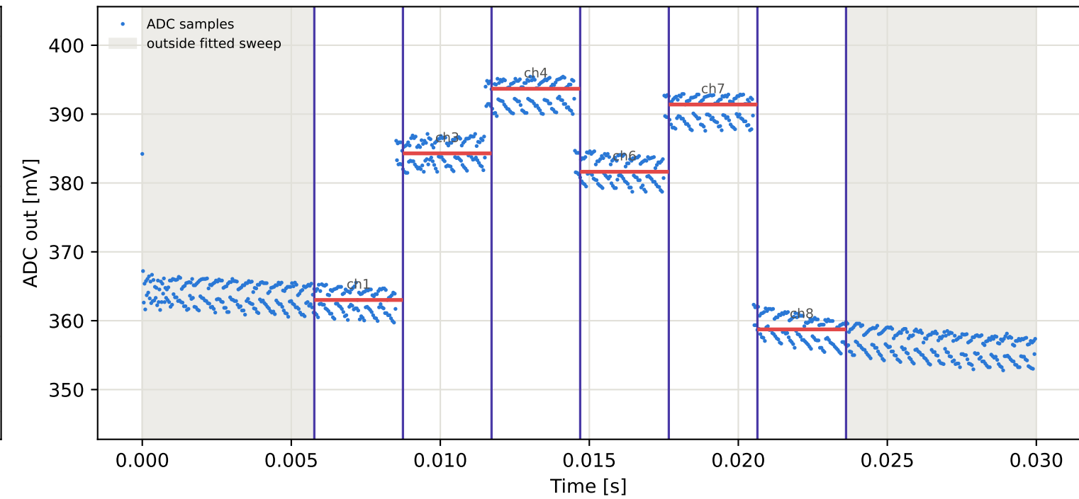
Tag5 &lt;- Tag1 | 875 MHz | run 0 | rep 1 | phase -61.89 deg
