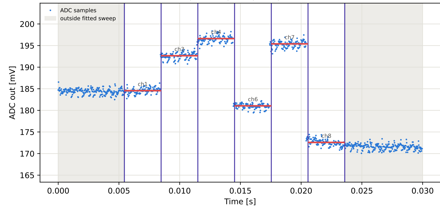
Tag2 &lt;- Tag16 | 905 MHz | run 0 | rep 1 | phase -51.52 deg
