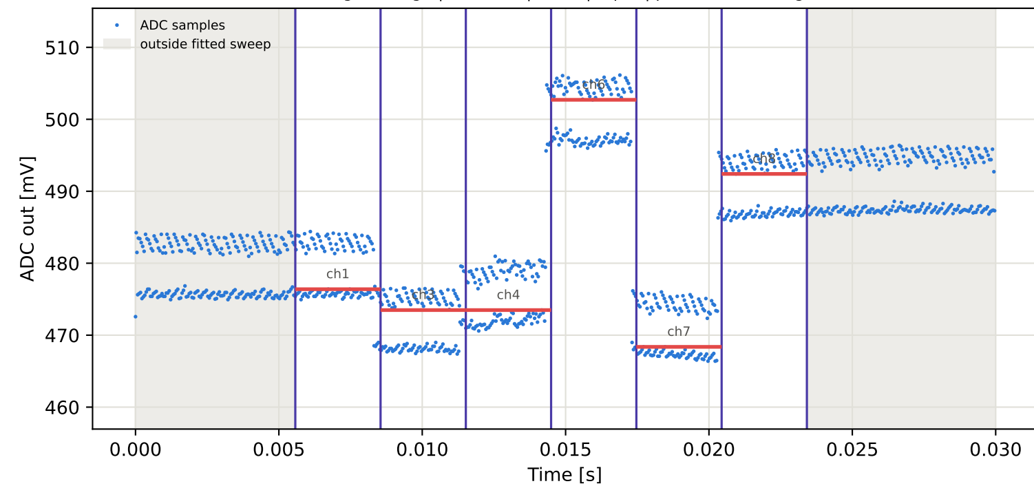
Tag3 &lt;- Tag15 | 965 MHz | run 0 | rep 1 | phase 90.70 deg
