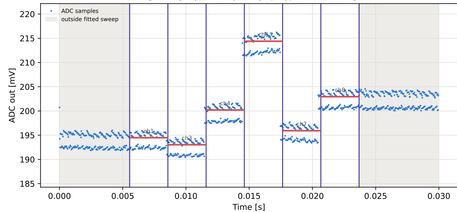
Tag5 &lt;- Tag2 | 945 MHz | run 0 | rep 1 | phase 141.55 deg
