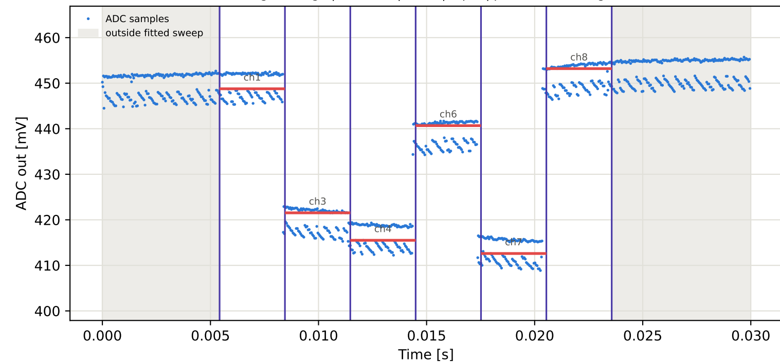
Tag5 &lt;- Tag8 | 845 MHz | run 0 | rep 1 | phase -80.94 deg
