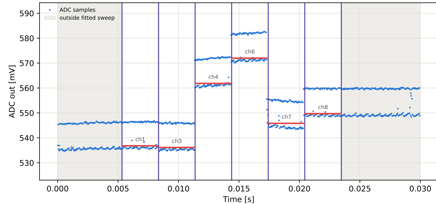
Tag9 &lt;- Tag16 | 975 MHz | run 0 | rep 1 | phase -145.45 deg
