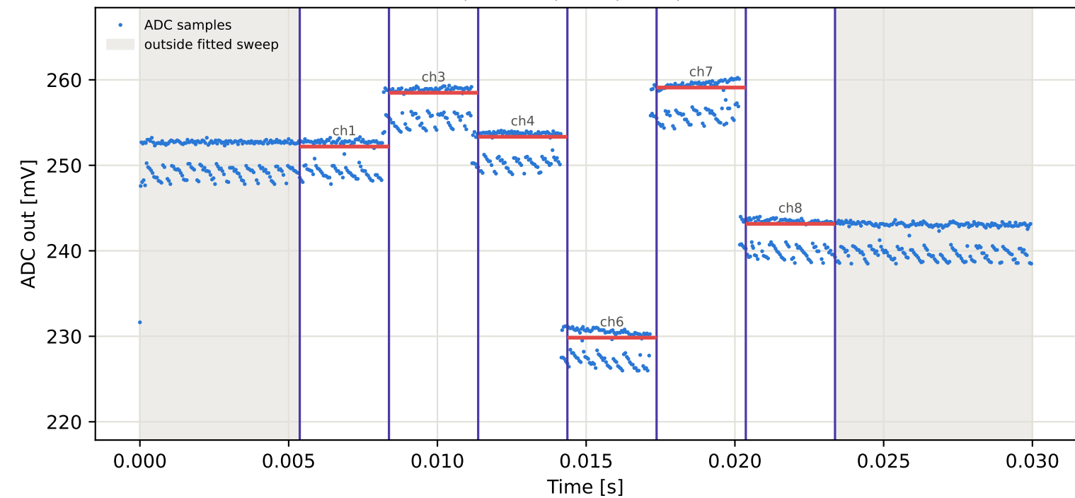
Tag5 &lt;- Tag4 | 985 MHz | run 0 | rep 1 | phase -3.79 deg
