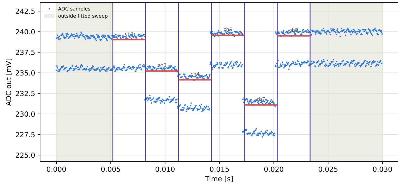
Tag7 &lt;- Tag5 | 785 MHz | run 0 | rep 1 | phase 140.79 deg
