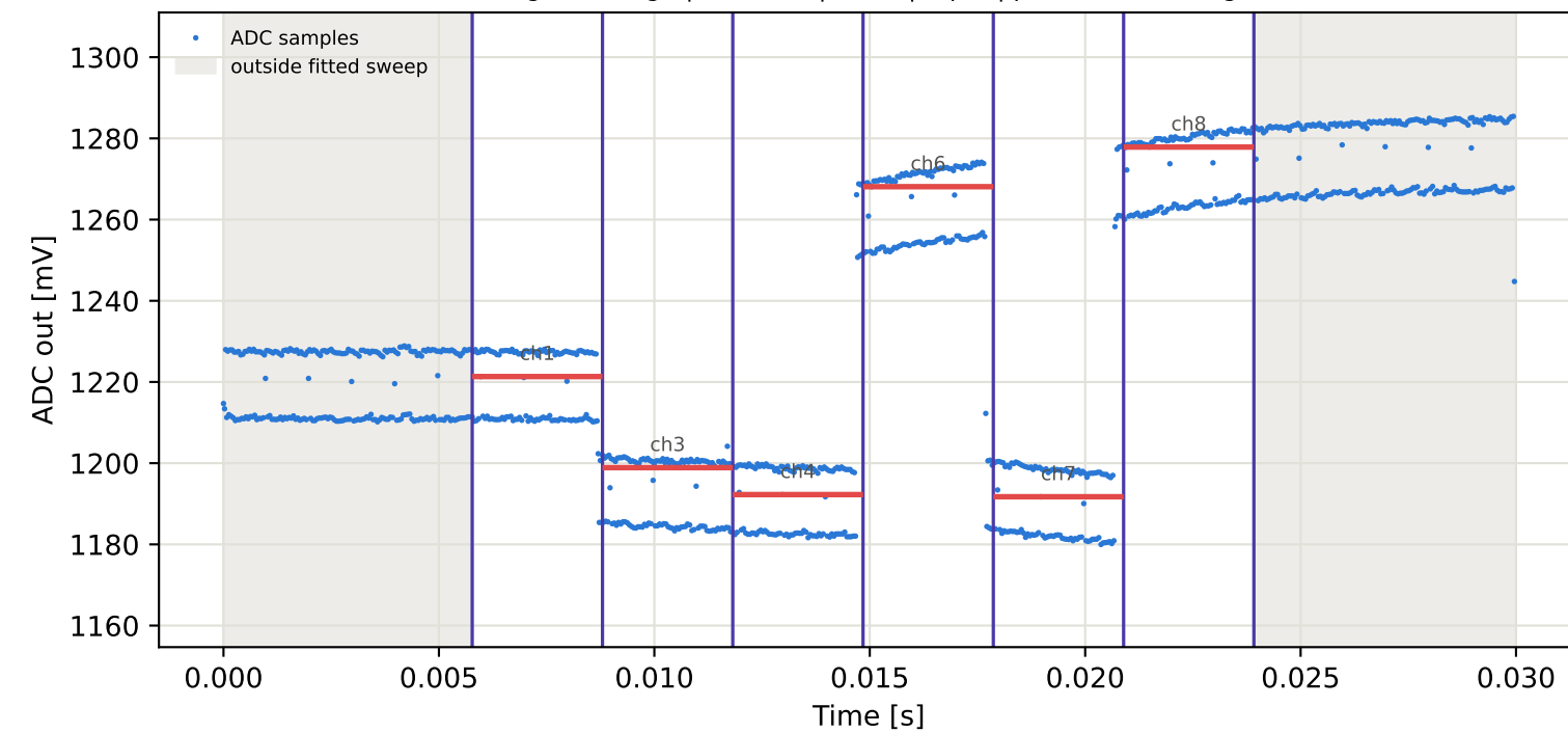
Tag10 &lt;- Tag8 | 895 MHz | run 0 | rep 1 | phase -129.50 deg
