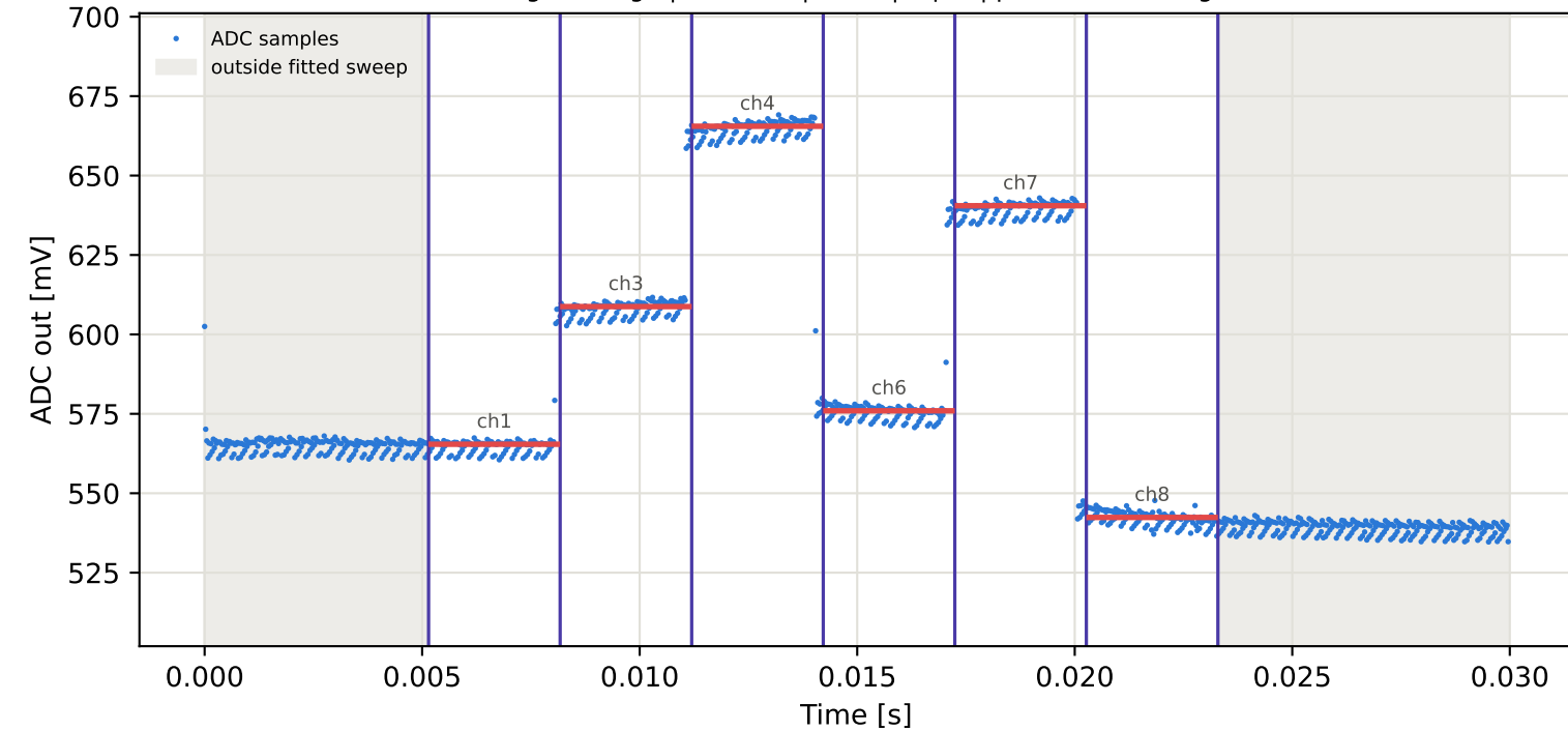
Tag3 &lt;- Tag9 | 945 MHz | run 0 | rep 1 | phase -78.92 deg
