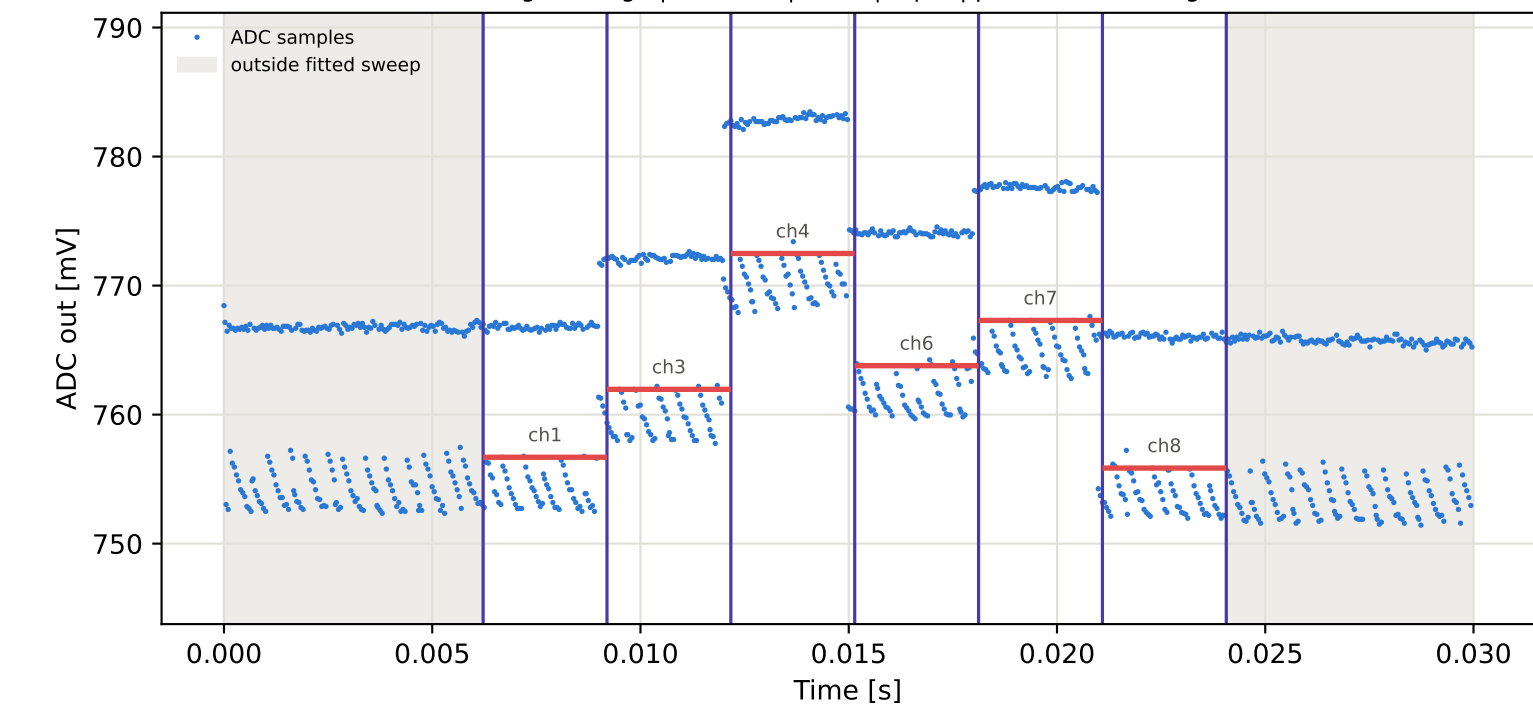
Tag8 &lt;- Tag6 | 945 MHz | run 0 | rep 1 | phase -103.37 deg
