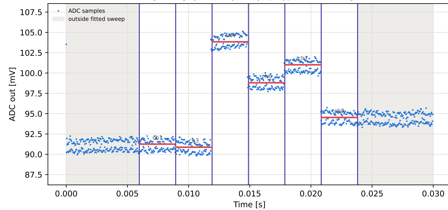
Tag4 &lt;- Tag7 | 775 MHz | run 0 | rep 1 | phase -101.12 deg
