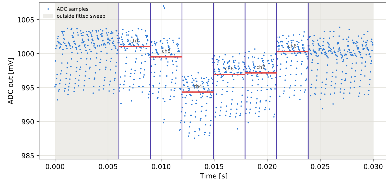
Tag7 &lt;- Tag5 | 975 MHz | run 0 | rep 1 | phase 59.51 deg
