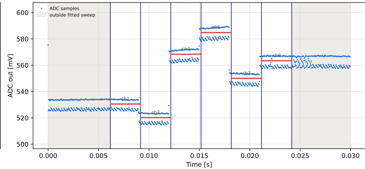
Tag3 &lt;- Tag9 | 835 MHz | run 0 | rep 1 | phase -139.32 deg
