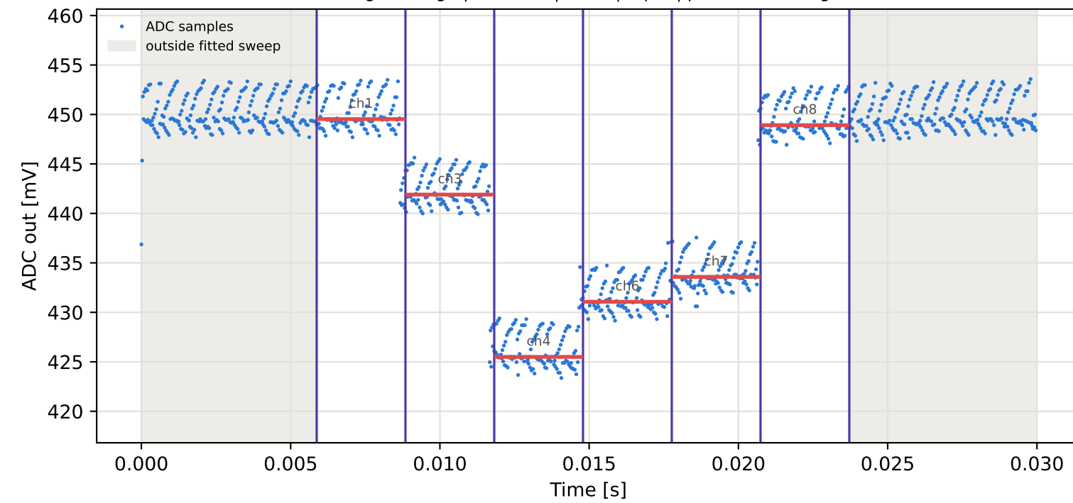
Tag6 &lt;- Tag1 | 935 MHz | run 0 | rep 1 | phase 64.89 deg
