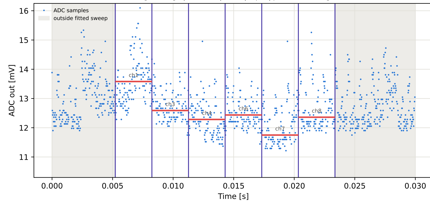
Tag2 &lt;- Tag5 | 795 MHz | run 0 | rep 1 | phase 34.84 deg
