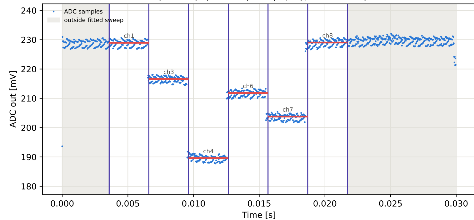
Tag16 &lt;- Tag10 | 955 MHz | run 0 | rep 1 | phase 56.58 deg
