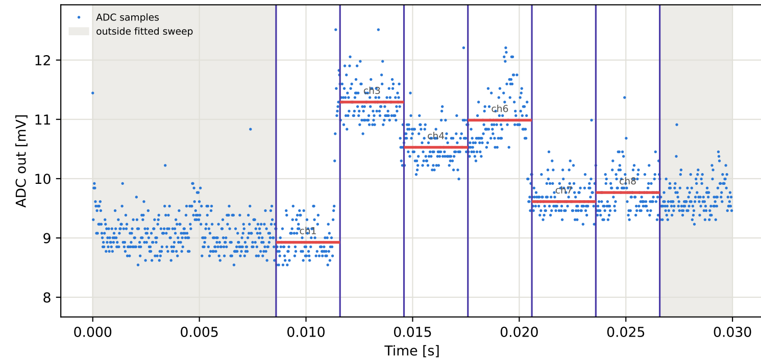
Tag2 &lt;- Tag8 | 775 MHz | run 0 | rep 1 | phase -61.15 deg
