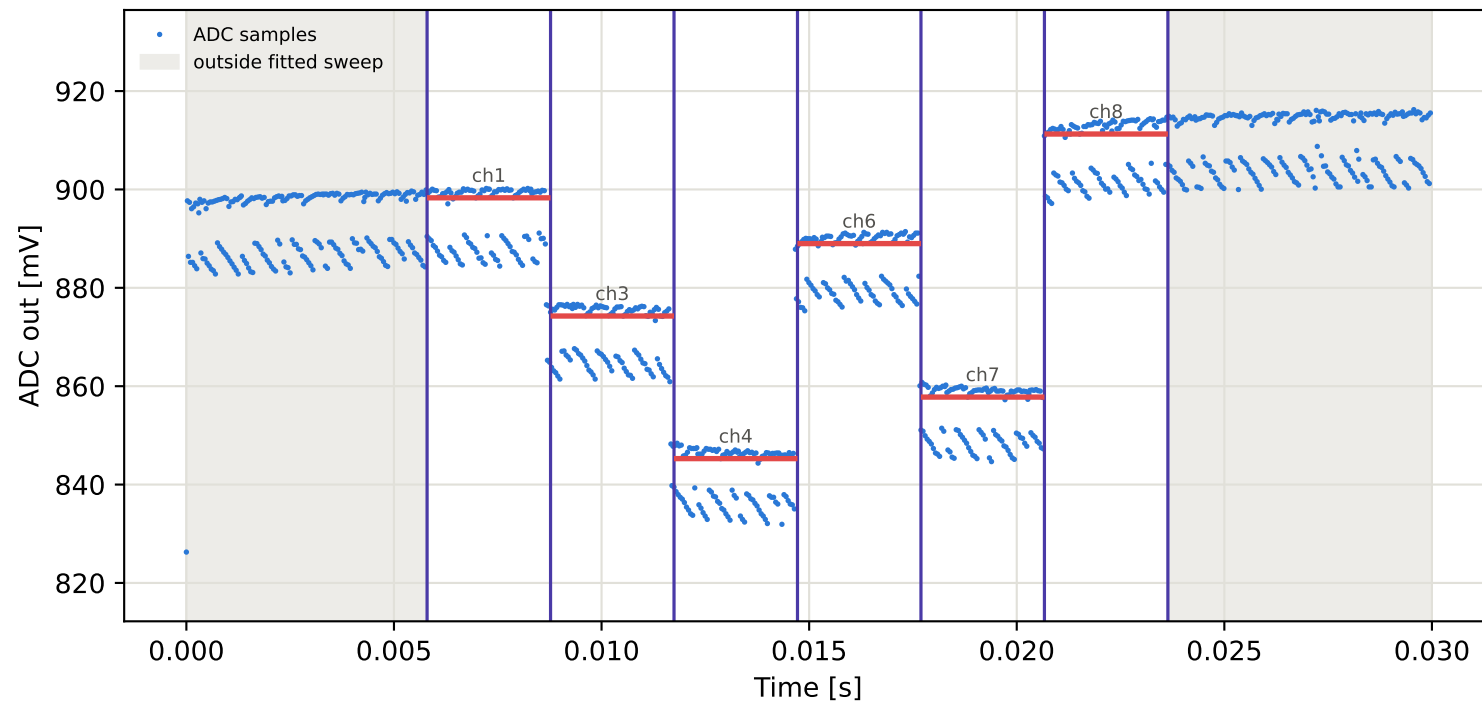
Tag9 &lt;- Tag10 | 935 MHz | run 0 | rep 1 | phase -164.11 deg
