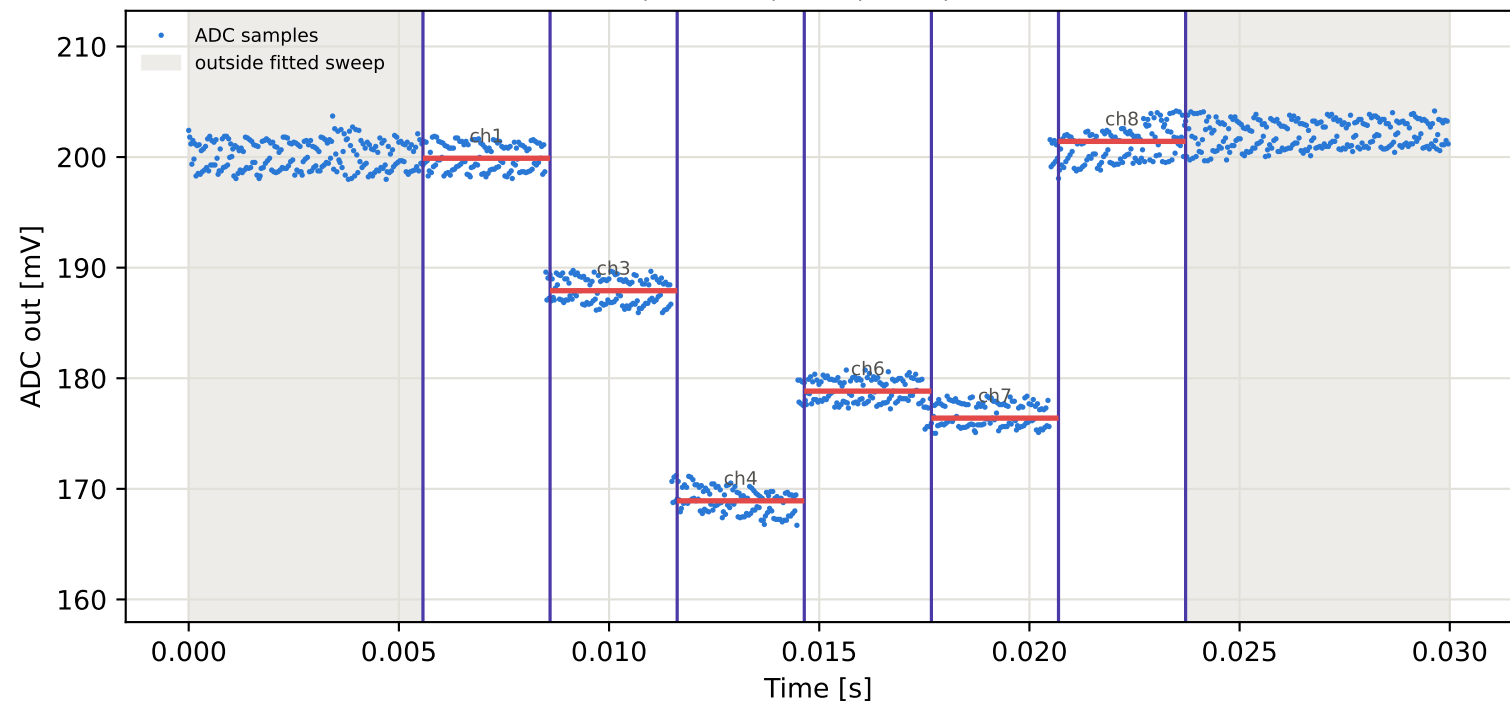
Tag4 &lt;- Tag3 | 925 MHz | run 0 | rep 1 | phase 71.69 deg
