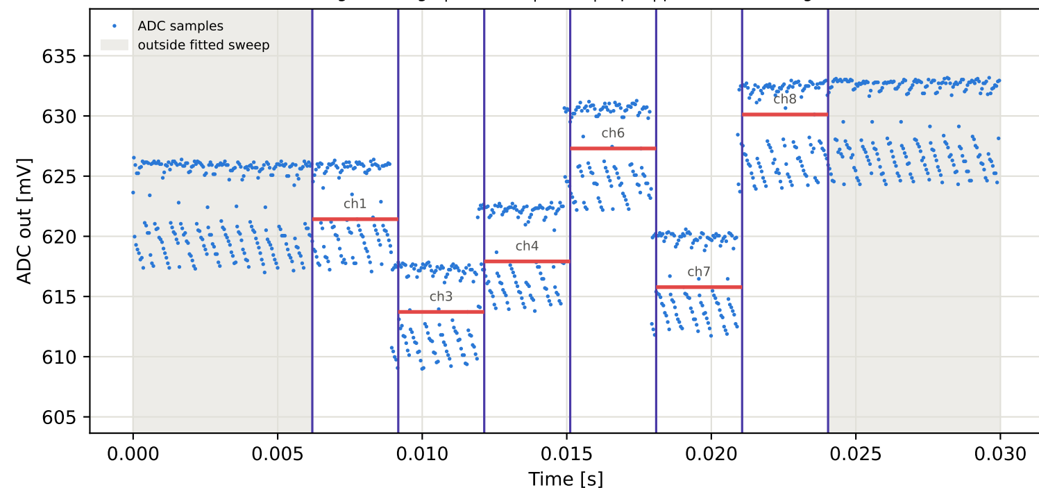
Tag10 &lt;- Tag5 | 855 MHz | run 0 | rep 1 | phase 166.77 deg
