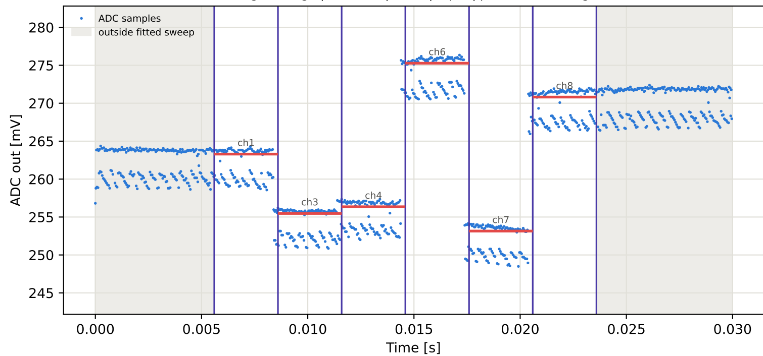
Tag5 &lt;- Tag9 | 985 MHz | run 0 | rep 1 | phase 13.62 deg
