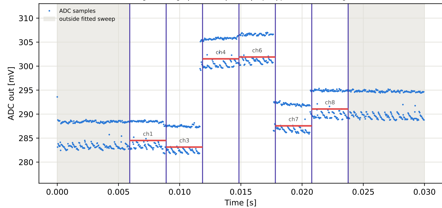
Tag10 &lt;- Tag5 | 995 MHz | run 0 | rep 1 | phase -178.97 deg
