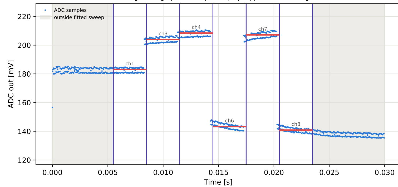
Tag4 &lt;- Tag7 | 905 MHz | run 0 | rep 1 | phase 12.39 deg
