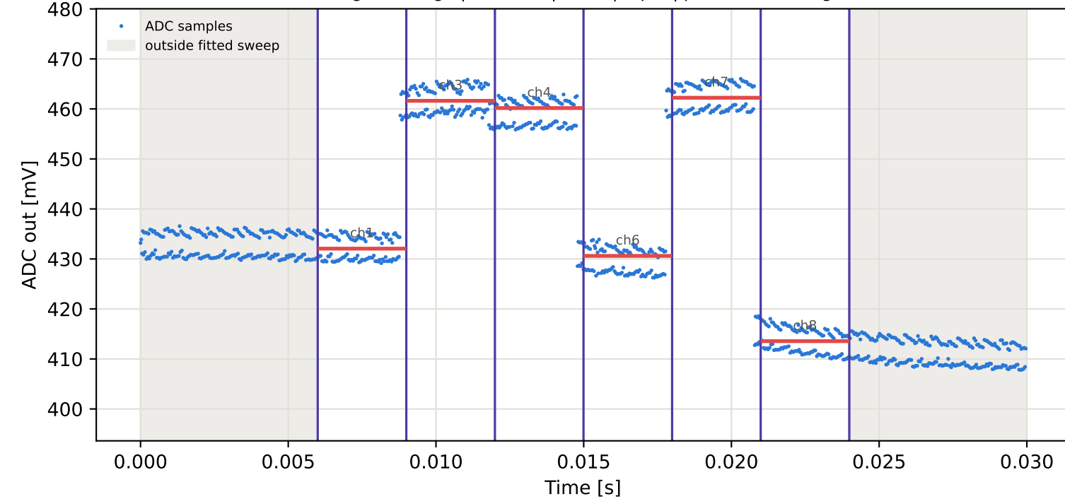
Tag16 &lt;- Tag10 | 875 MHz | run 0 | rep 1 | phase -102.83 deg
