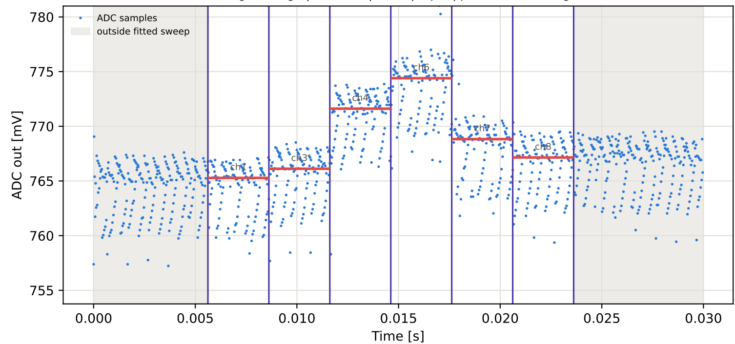
Tag8 &lt;- Tag7 | 945 MHz | run 0 | rep 1 | phase -19.65 deg
