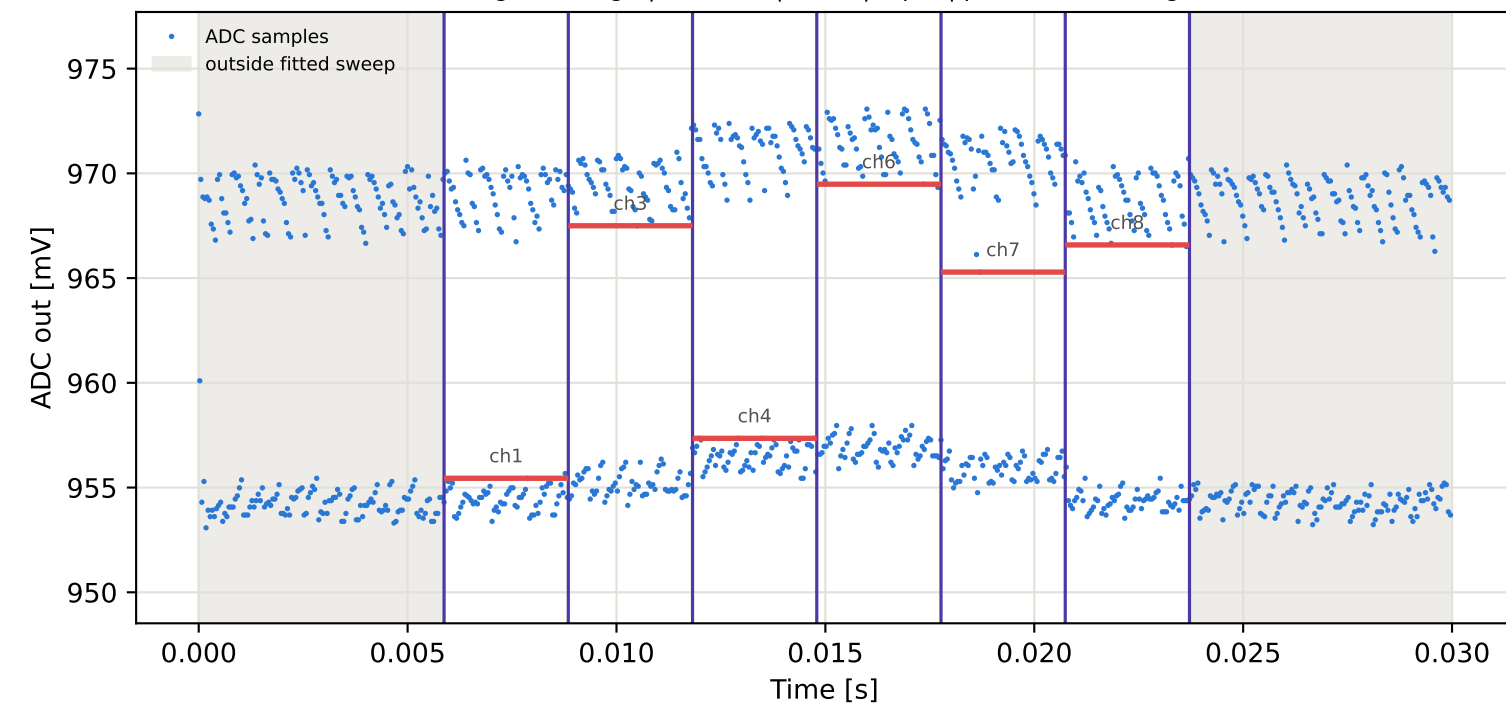
Tag16 &lt;- Tag4 | 915 MHz | run 0 | rep 1 | phase 116.55 deg
