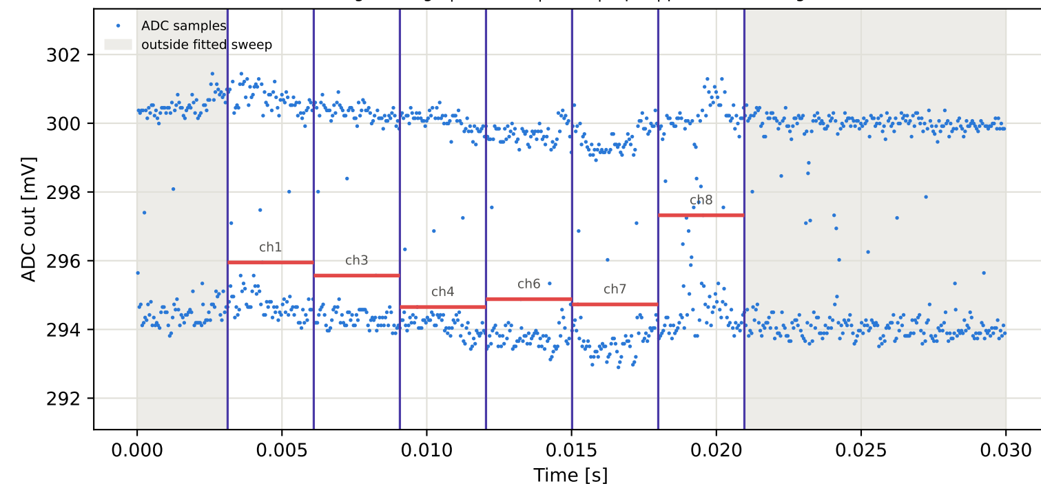
Tag4 &lt;- Tag2 | 965 MHz | run 0 | rep 1 | phase 74.28 deg
