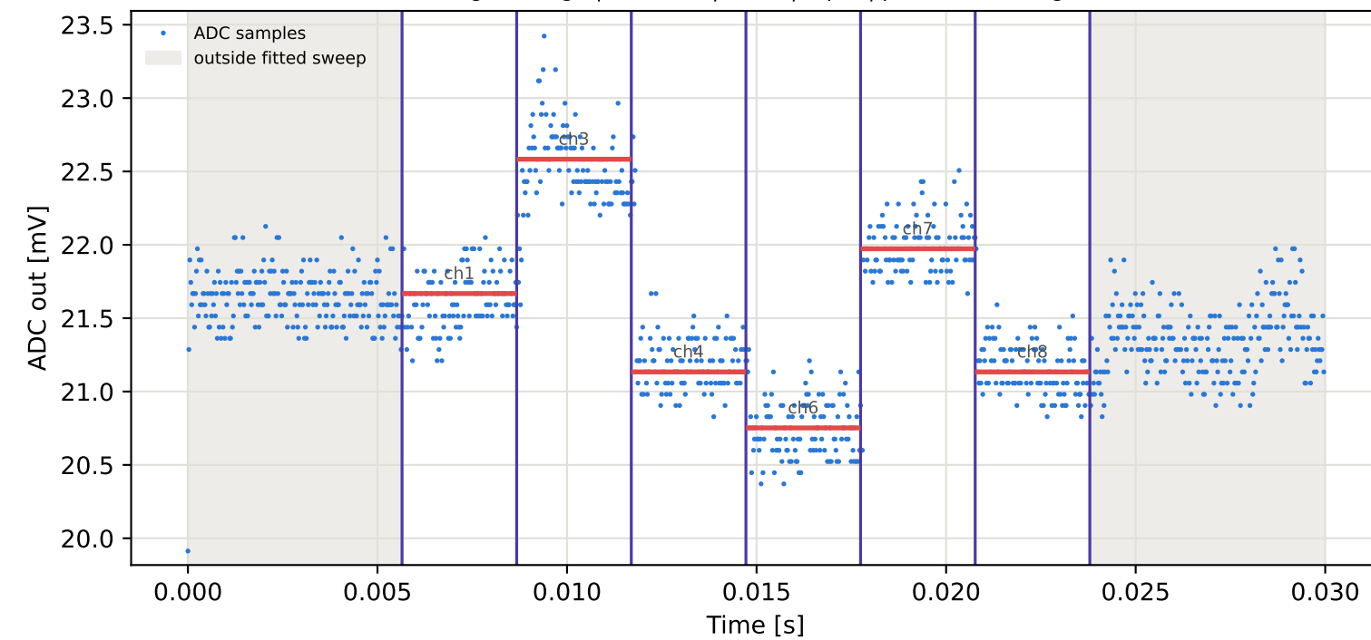
Tag1 &lt;- Tag7 | 775 MHz | run 0 | rep 1 | phase -165.40 deg
