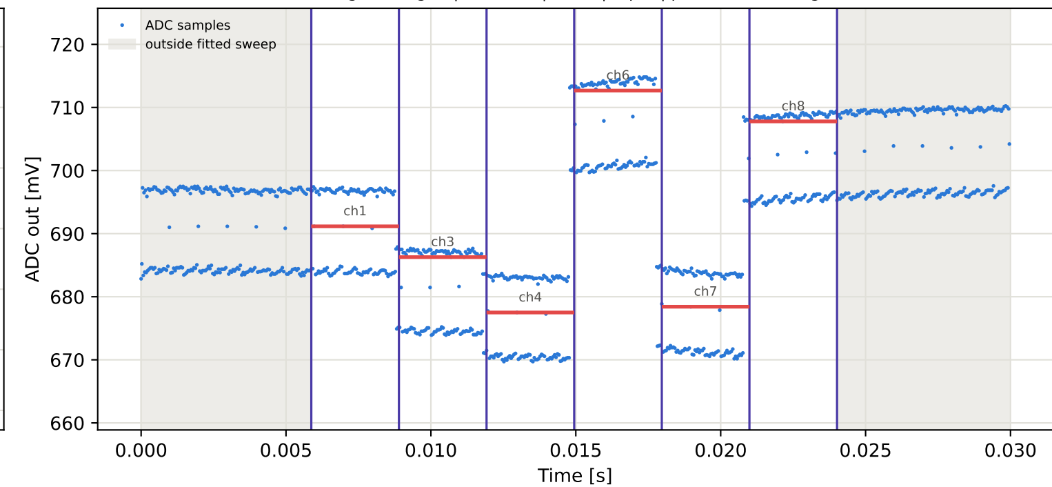
Tag6 &lt;- Tag3 | 945 MHz | run 0 | rep 1 | phase 176.68 deg
