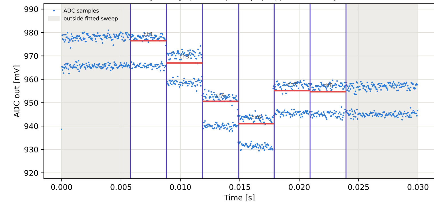
Tag9 &lt;- Tag7 | 885 MHz | run 0 | rep 1 | phase 43.16 deg
