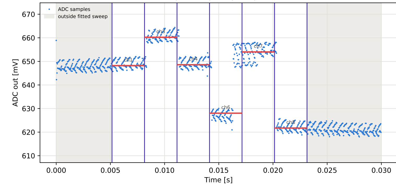
Tag8 &lt;- Tag15 | 875 MHz | run 0 | rep 1 | phase -0.22 deg
