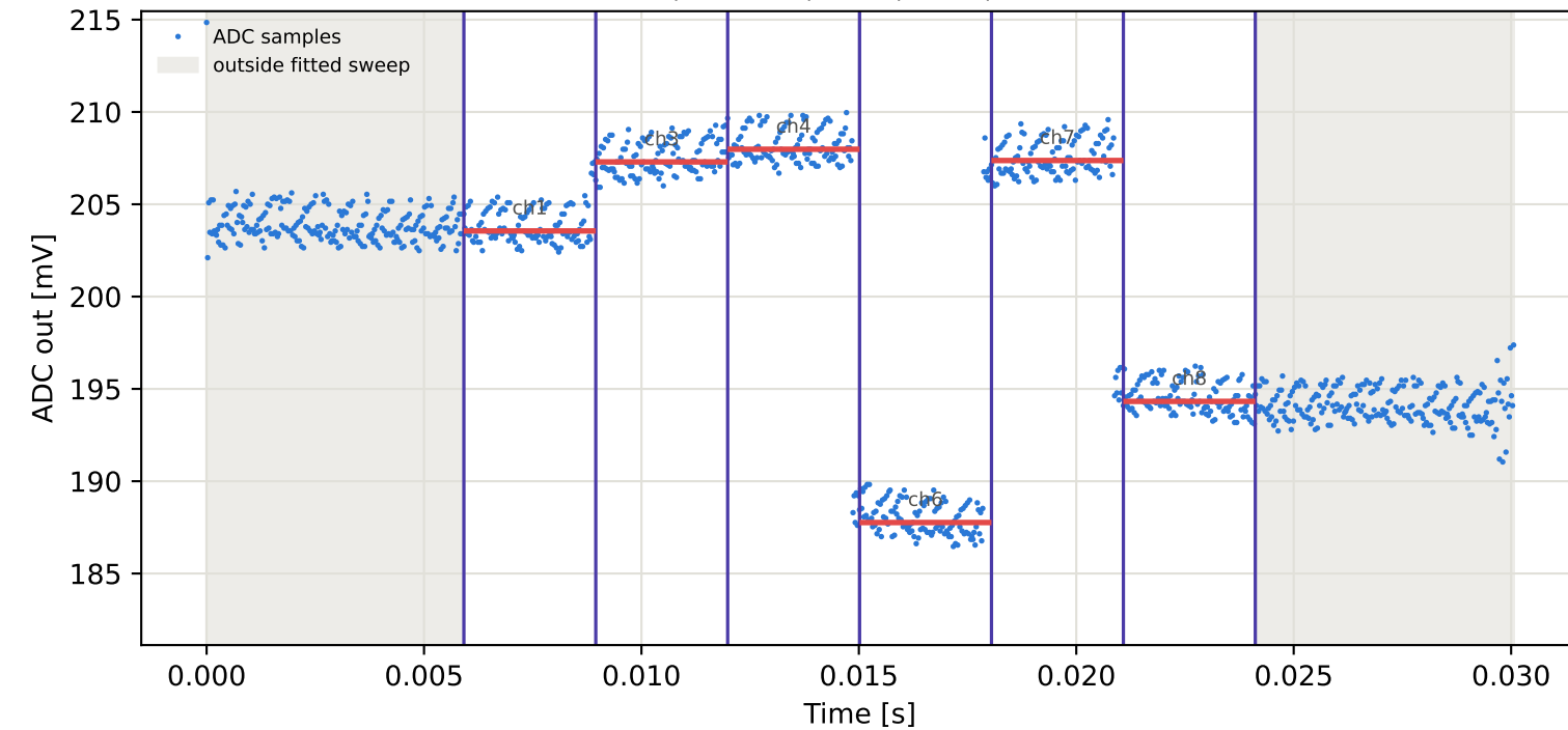
Tag4 &lt;- Tag2 | 915 MHz | run 0 | rep 1 | phase -11.62 deg
