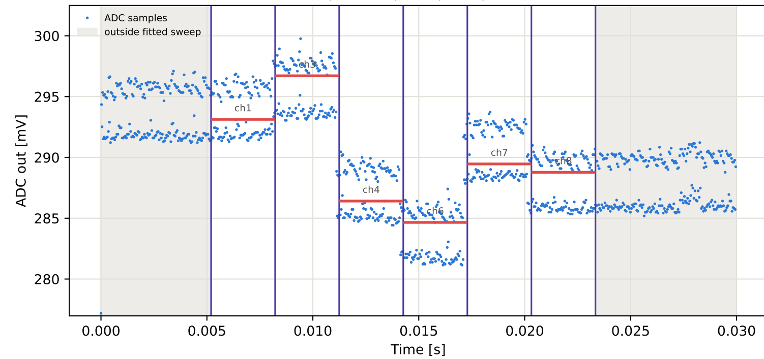
Tag2 &lt;- Tag7 | 855 MHz | run 0 | rep 1 | phase 42.74 deg
