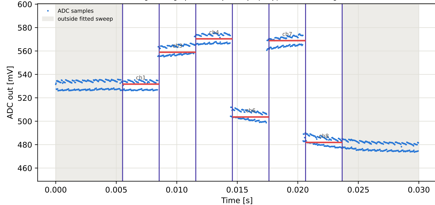
Tag4 &lt;- Tag3 | 895 MHz | run 0 | rep 1 | phase -39.32 deg
