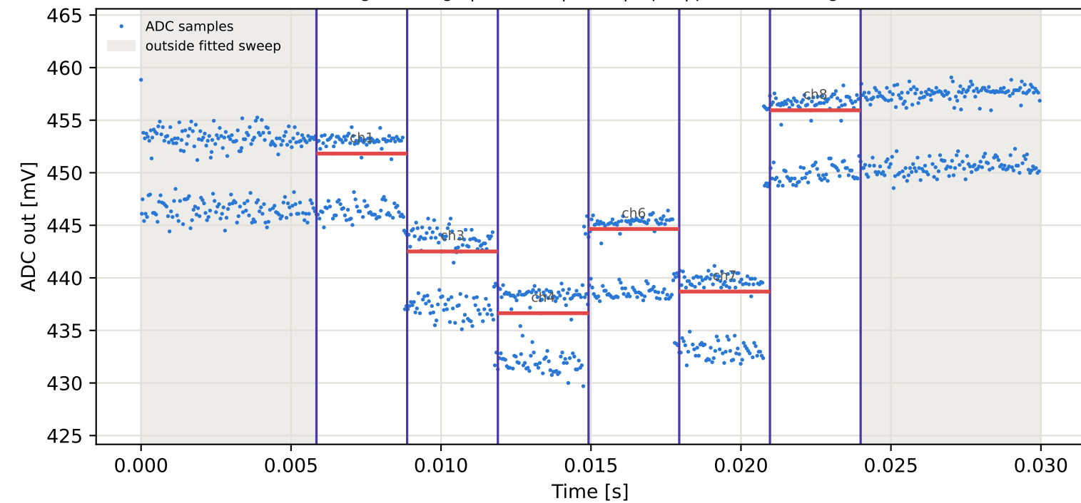
Tag15 &lt;- Tag6 | 885 MHz | run 0 | rep 1 | phase -139.94 deg
