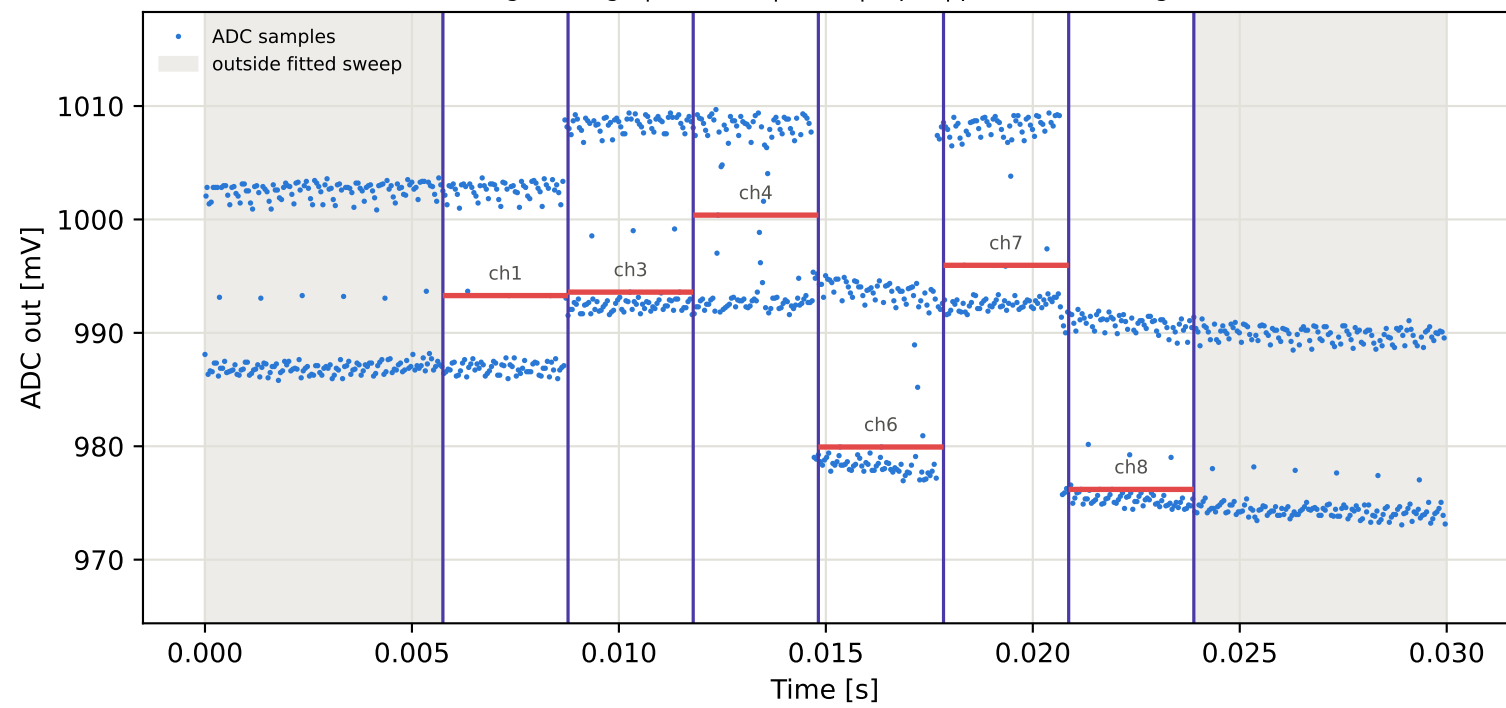
Tag3 &lt;- Tag15 | 905 MHz | run 0 | rep 1 | phase 18.90 deg
