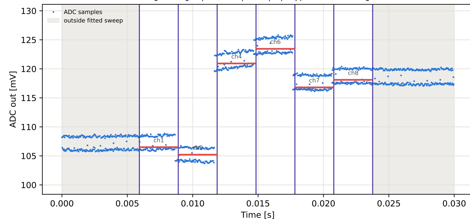
Tag5 &lt;- Tag16 | 825 MHz | run 0 | rep 1 | phase 80.85 deg
