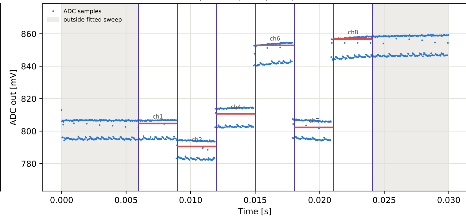
Tag16 &lt;- Tag5 | 865 MHz | run 0 | rep 1 | phase 96.72 deg
