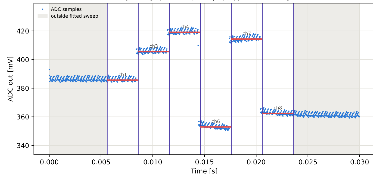
Tag1 &lt;- Tag3 | 955 MHz | run 0 | rep 1 | phase -37.54 deg
