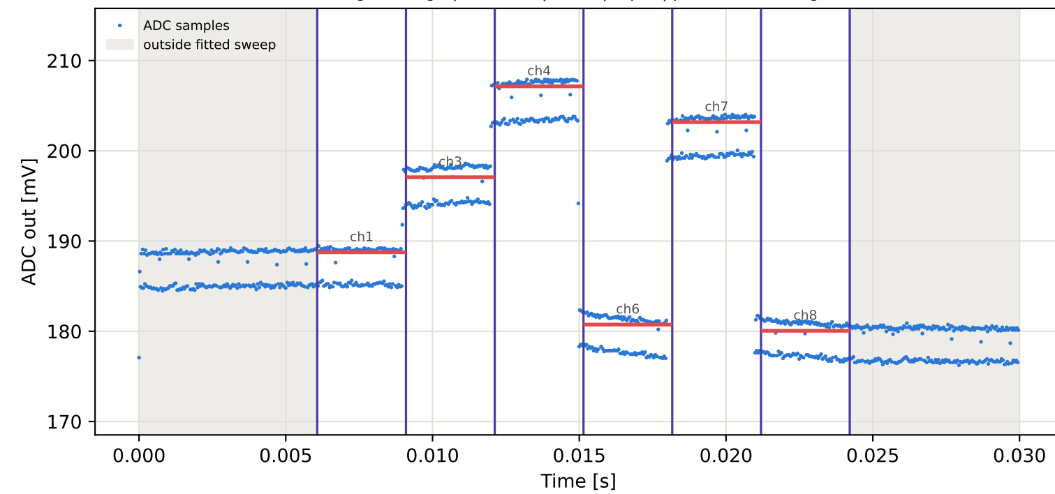
Tag5 &lt;- Tag8 | 945 MHz | run 0 | rep 1 | phase -100.30 deg
