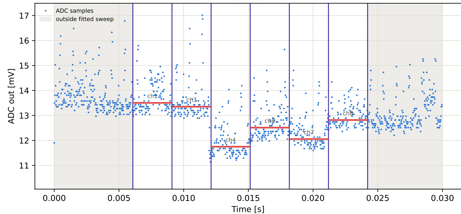
Tag2 &lt;- Tag8 | 795 MHz | run 0 | rep 1 | phase 78.21 deg
