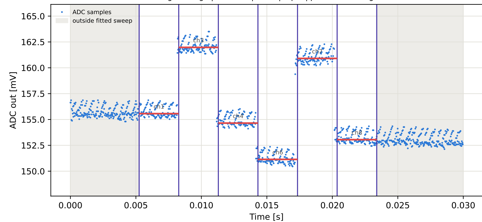
Tag9 &lt;- Tag5 | 785 MHz | run 0 | rep 1 | phase -30.15 deg
