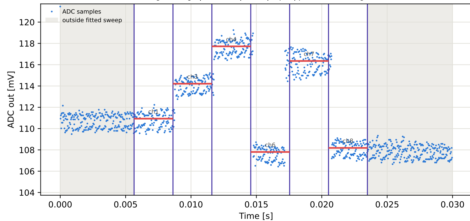
Tag5 &lt;- Tag1 | 975 MHz | run 0 | rep 1 | phase 82.70 deg
