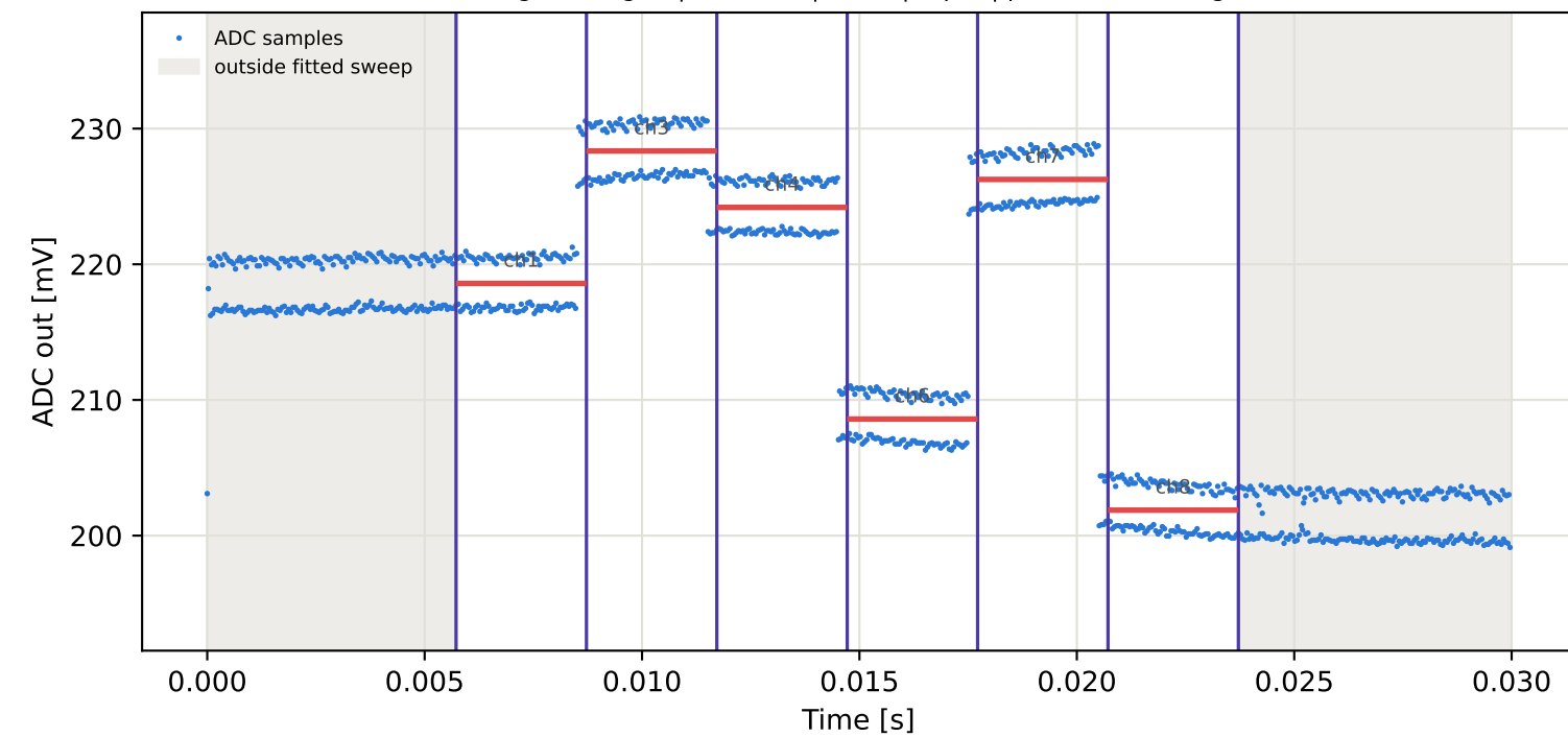
Tag1 &lt;- Tag16 | 865 MHz | run 0 | rep 1 | phase -24.17 deg
