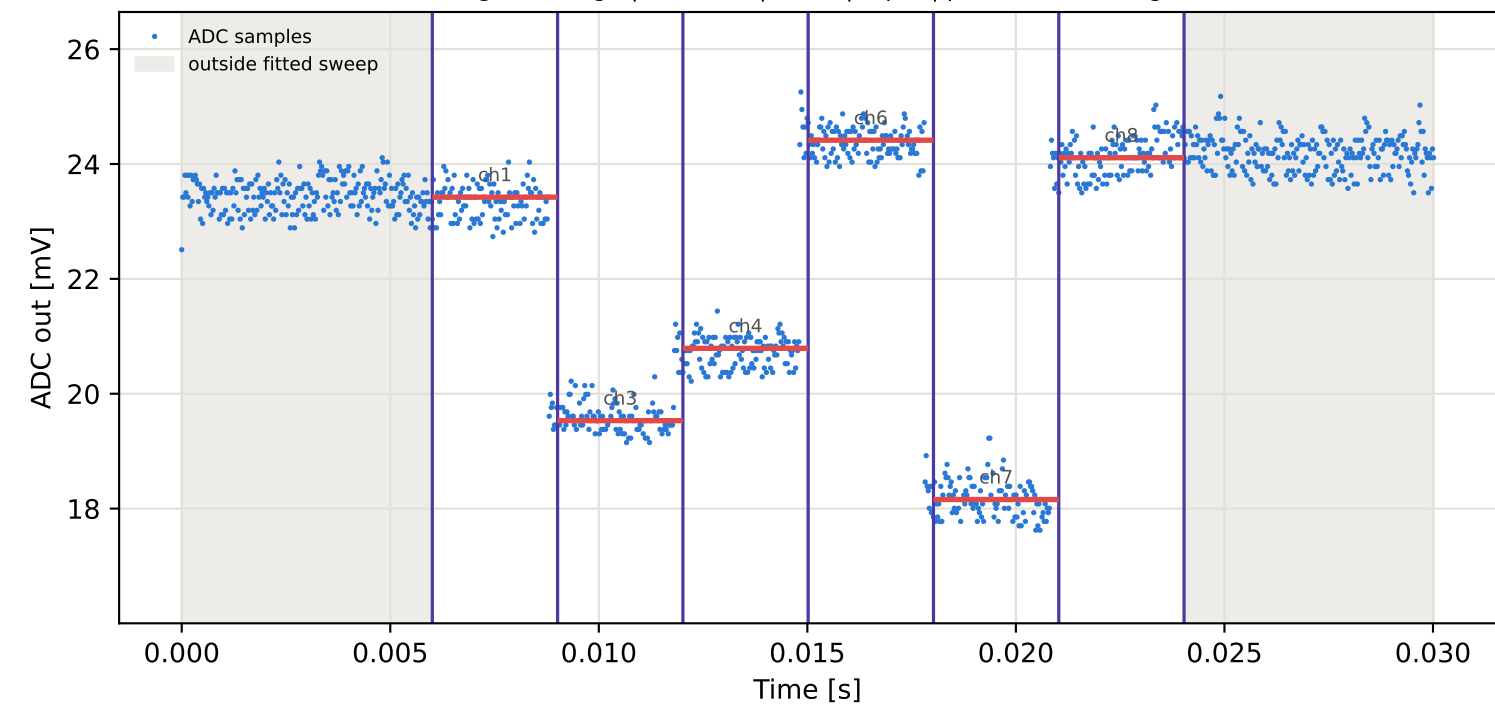
Tag16 &lt;- Tag1 | 775 MHz | run 0 | rep 1 | phase 73.61 deg
