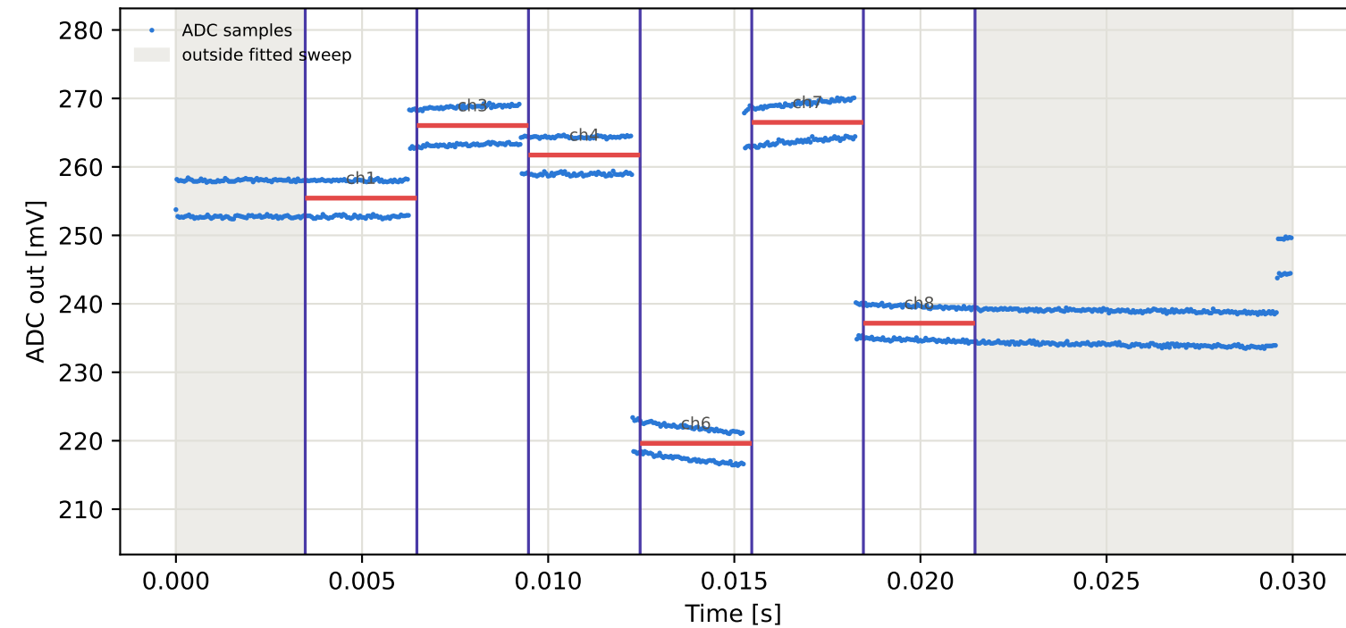
Tag6 &lt;- Tag10 | 955 MHz | run 0 | rep 1 | phase -75.01 deg
