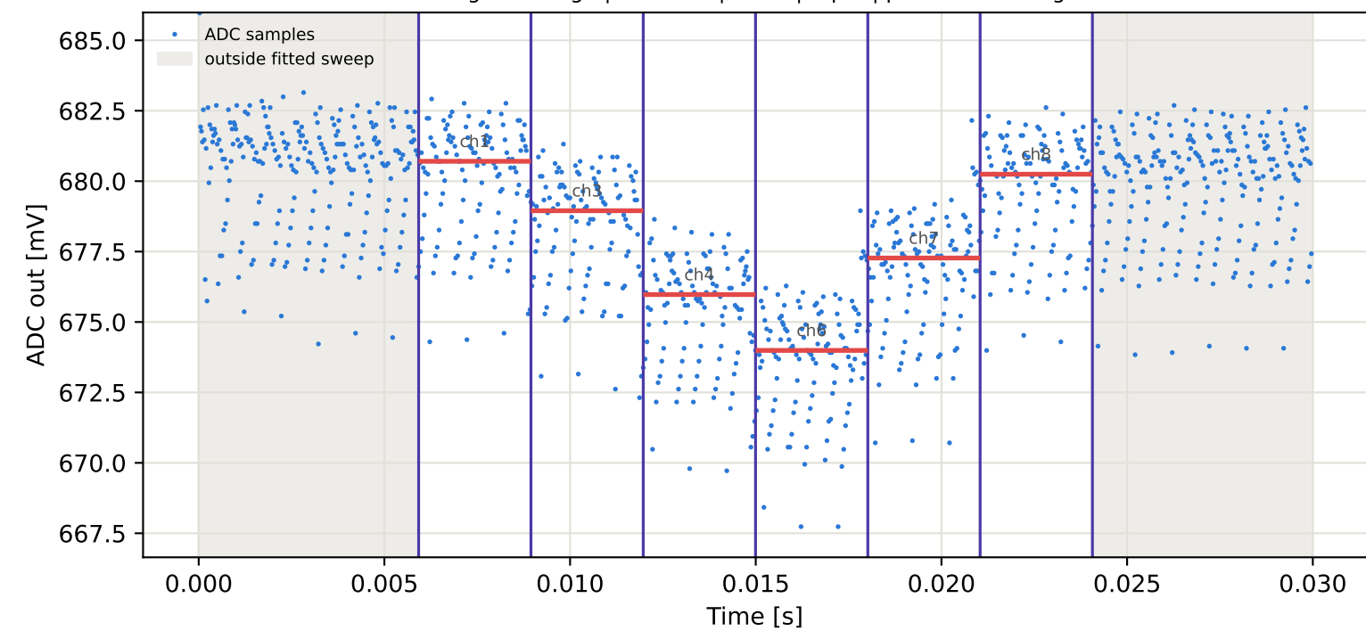
Tag15 &lt;- Tag4 | 915 MHz | run 0 | rep 1 | phase 143.23 deg
