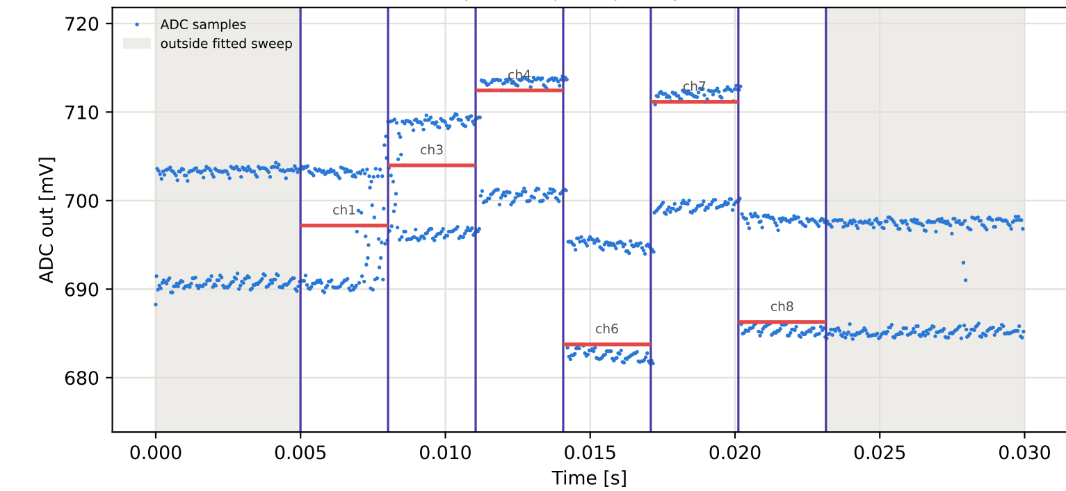
Tag8 &lt;- Tag6 | 965 MHz | run 0 | rep 1 | phase -44.82 deg
