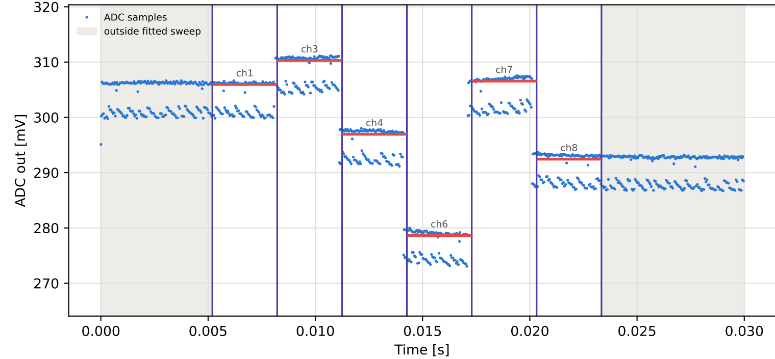
Tag6 &lt;- Tag10 | 975 MHz | run 0 | rep 1 | phase -80.90 deg
