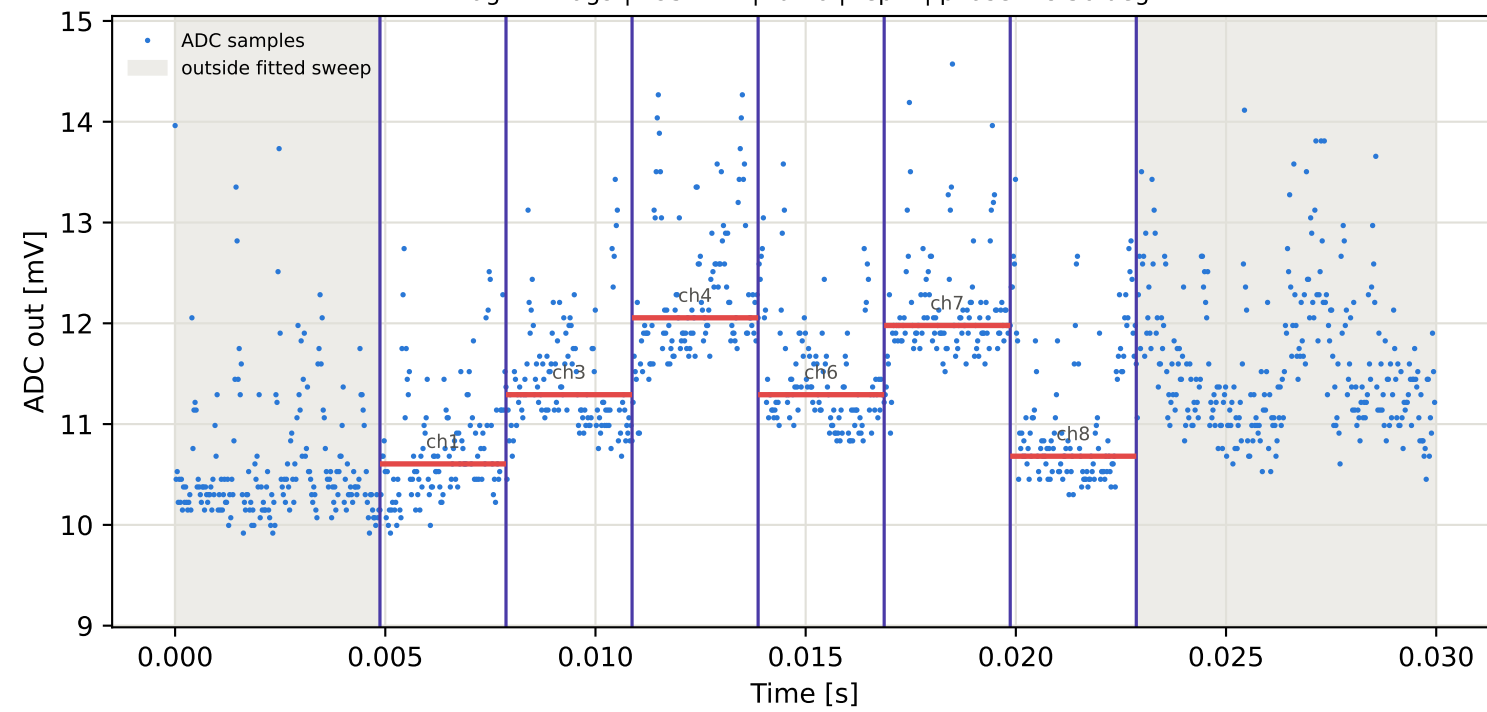
Tag3 &lt;- Tag10 | 795 MHz | run 0 | rep 1 | phase -39.62 deg
