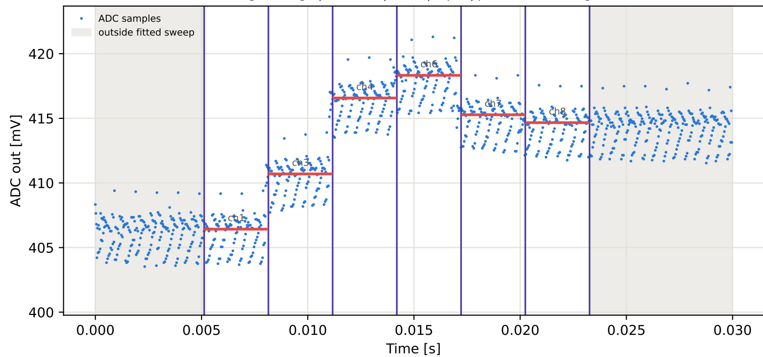
Tag8 &lt;- Tag5 | 855 MHz | run 0 | rep 1 | phase -21.44 deg
