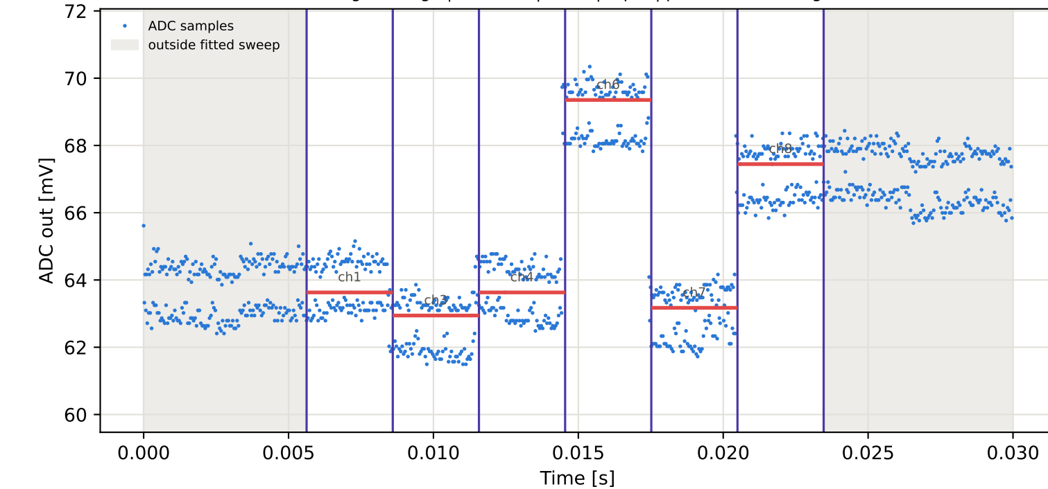
Tag4 &lt;- Tag2 | 825 MHz | run 0 | rep 1 | phase -174.07 deg
