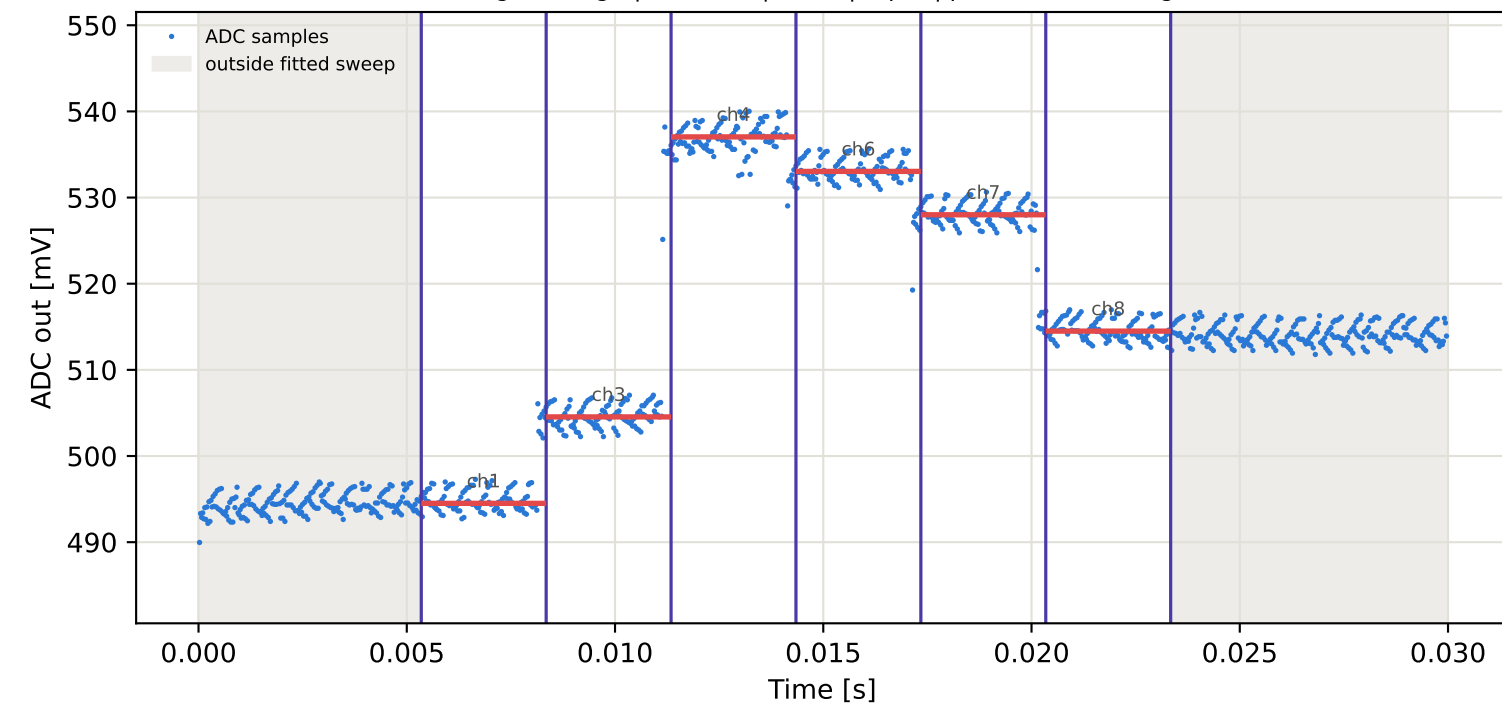
Tag9 &lt;- Tag10 | 845 MHz | run 0 | rep 1 | phase 59.76 deg
