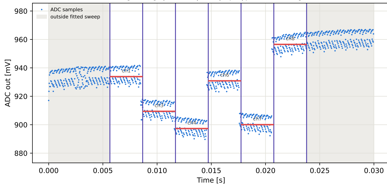
Tag3 &lt;- Tag6 | 895 MHz | run 0 | rep 1 | phase 68.03 deg
