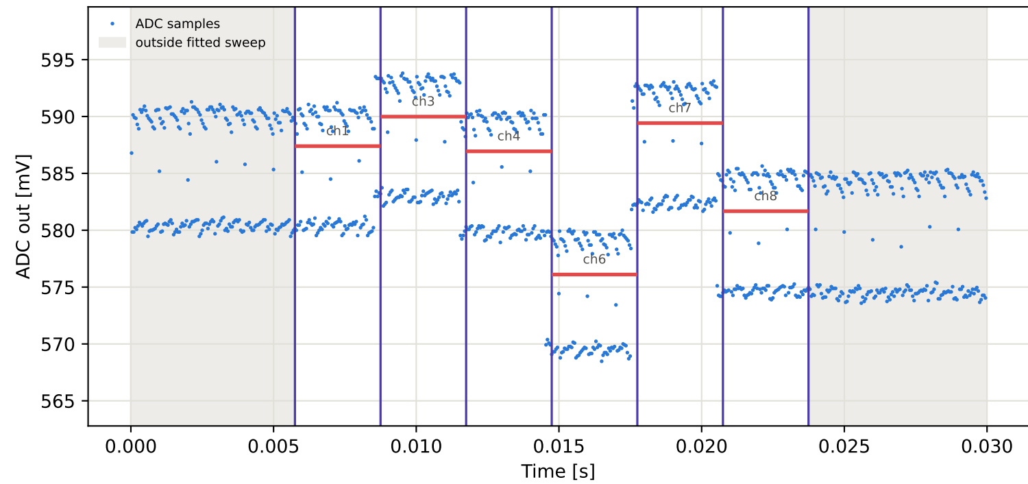
Tag6 &lt;- Tag2 | 975 MHz | run 0 | rep 1 | phase -99.06 deg
