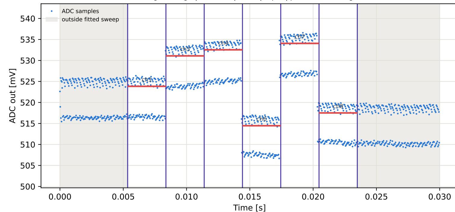
Tag1 &lt;- Tag9 | 985 MHz | run 0 | rep 1 | phase -105.96 deg
