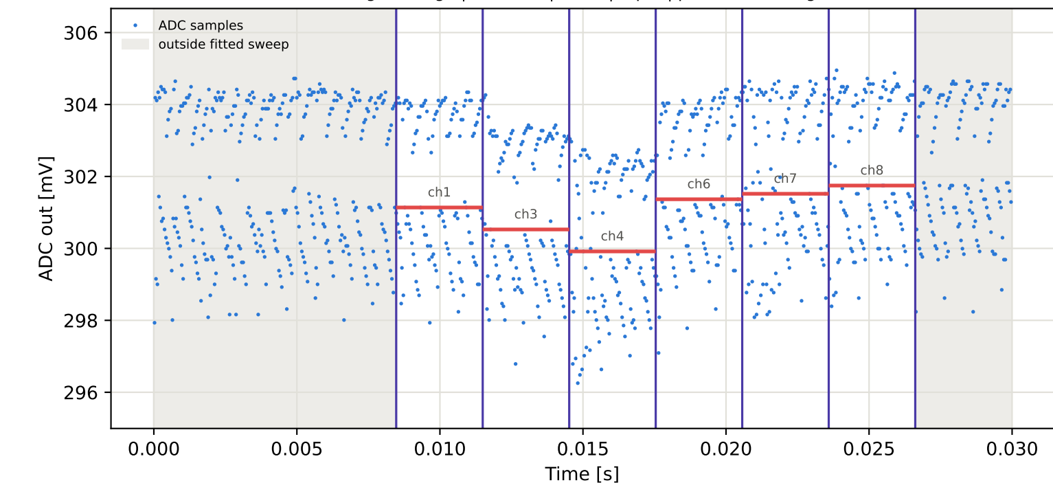
Tag6 &lt;- Tag4 | 955 MHz | run 0 | rep 1 | phase 136.90 deg
