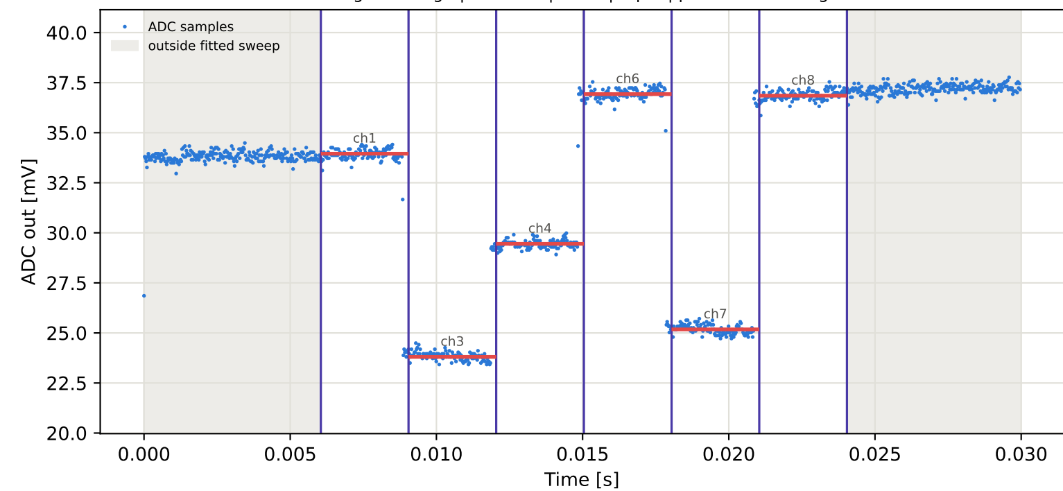
Tag2 &lt;- Tag1 | 805 MHz | run 0 | rep 1 | phase 172.40 deg
