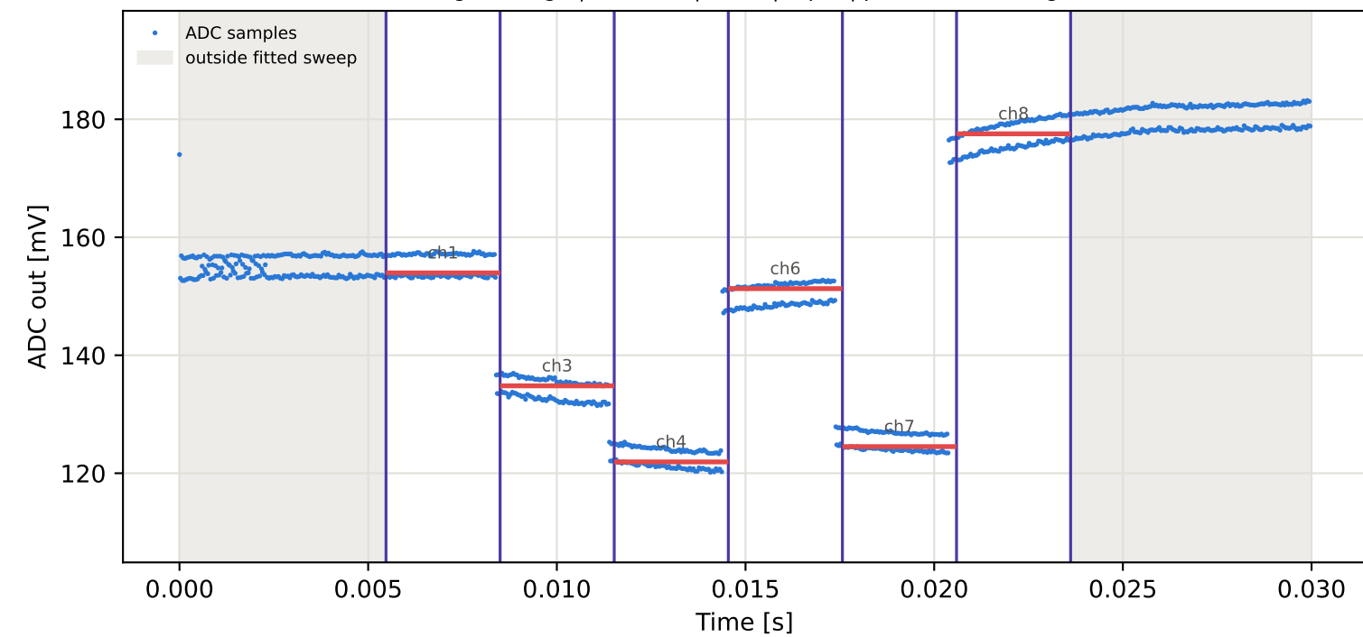
Tag1 &lt;- Tag7 | 895 MHz | run 0 | rep 1 | phase -77.49 deg
