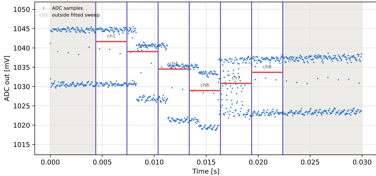
Tag7 &lt;- Tag15 | 875 MHz | run 0 | rep 1 | phase 47.05 deg
