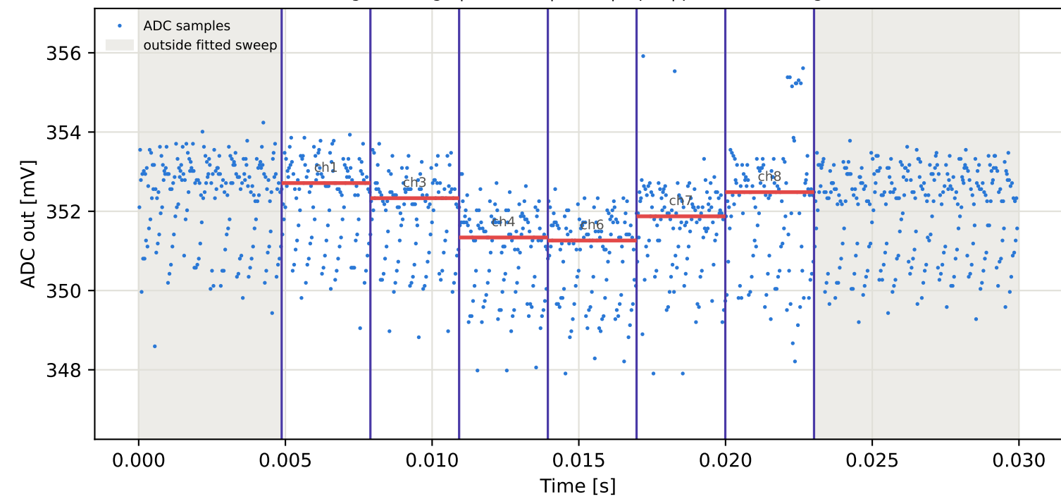
Tag15 &lt;- Tag4 | 985 MHz | run 0 | rep 1 | phase 6.03 deg
