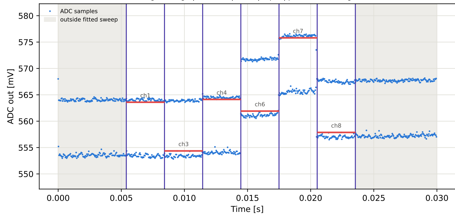
Tag8 &lt;- Tag7 | 955 MHz | run 0 | rep 1 | phase -14.28 deg
