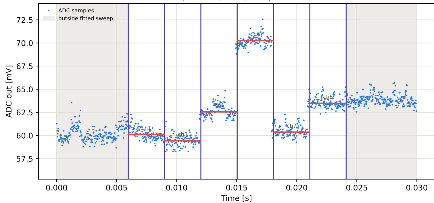
Tag2 &lt;- Tag6 | 945 MHz | run 0 | rep 1 | phase 122.79 deg
