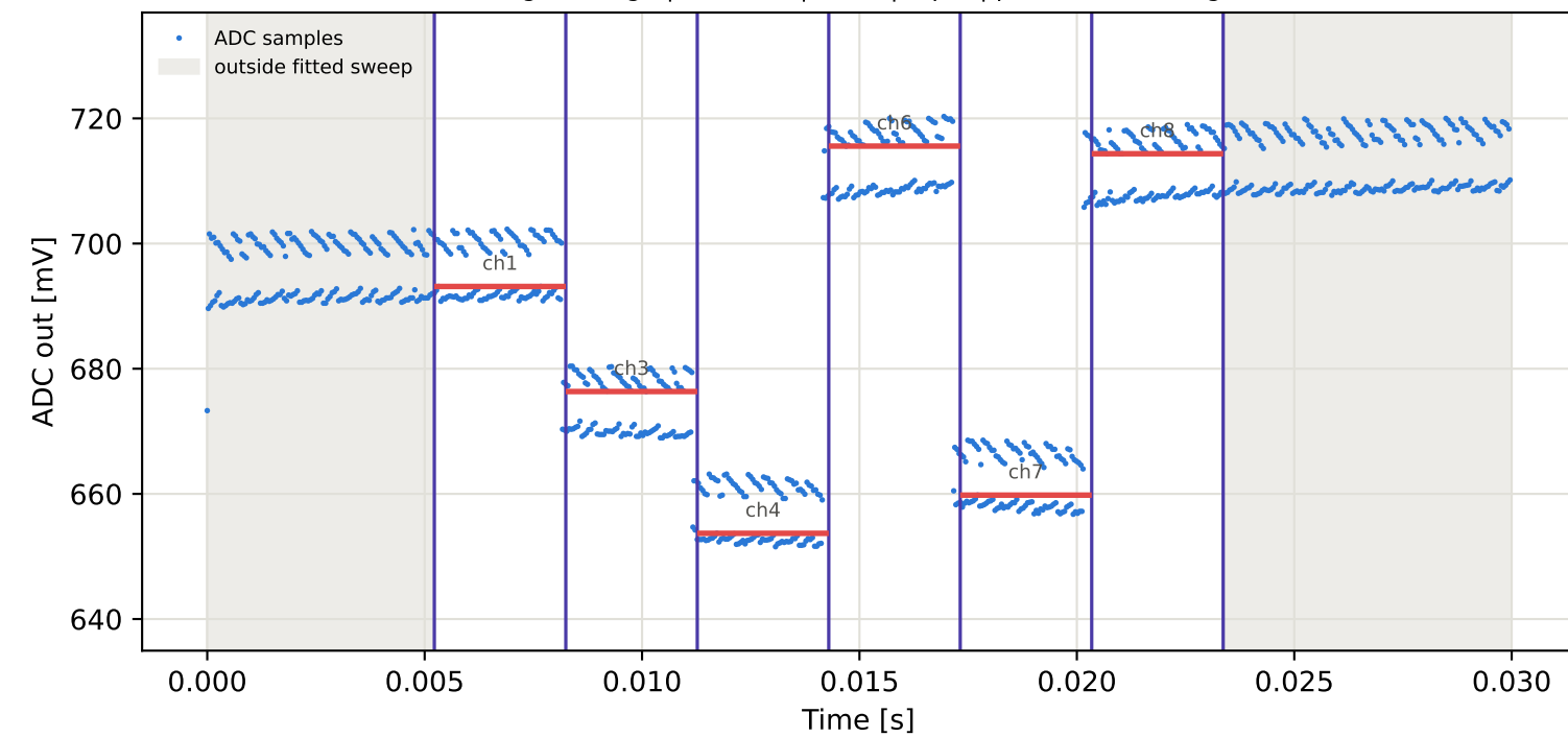
Tag9 &lt;- Tag10 | 975 MHz | run 0 | rep 1 | phase -147.00 deg
