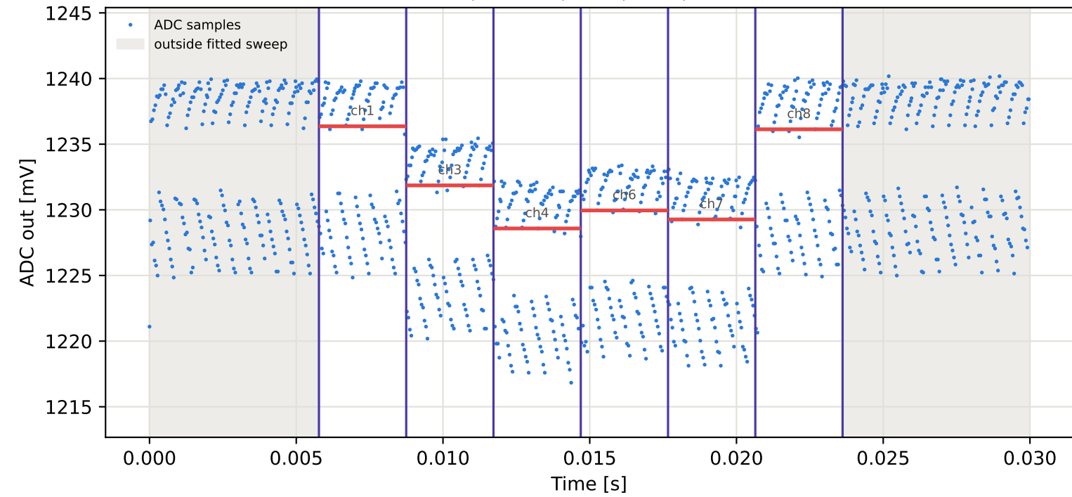
Tag10 &lt;- Tag1 | 895 MHz | run 0 | rep 1 | phase 77.72 deg
