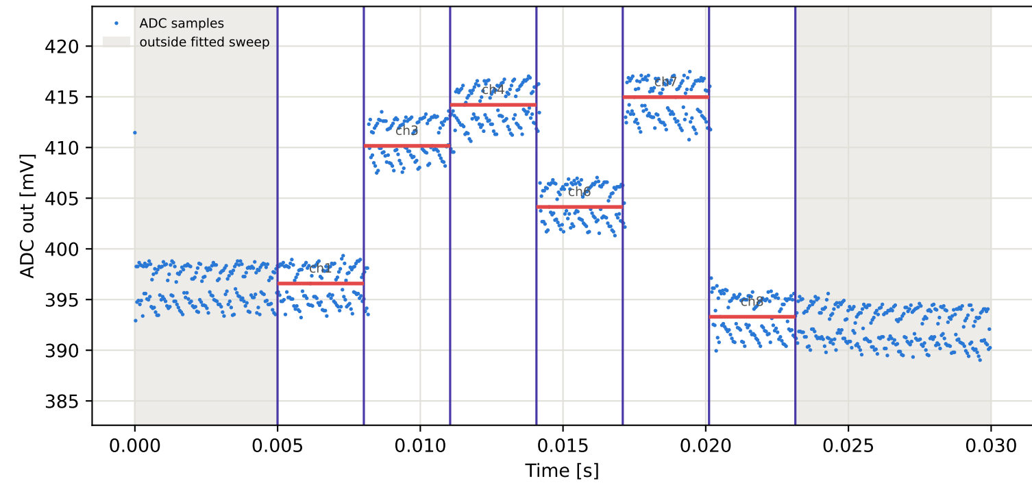
Tag2 &lt;- Tag8 | 865 MHz | run 0 | rep 1 | phase -58.96 deg
