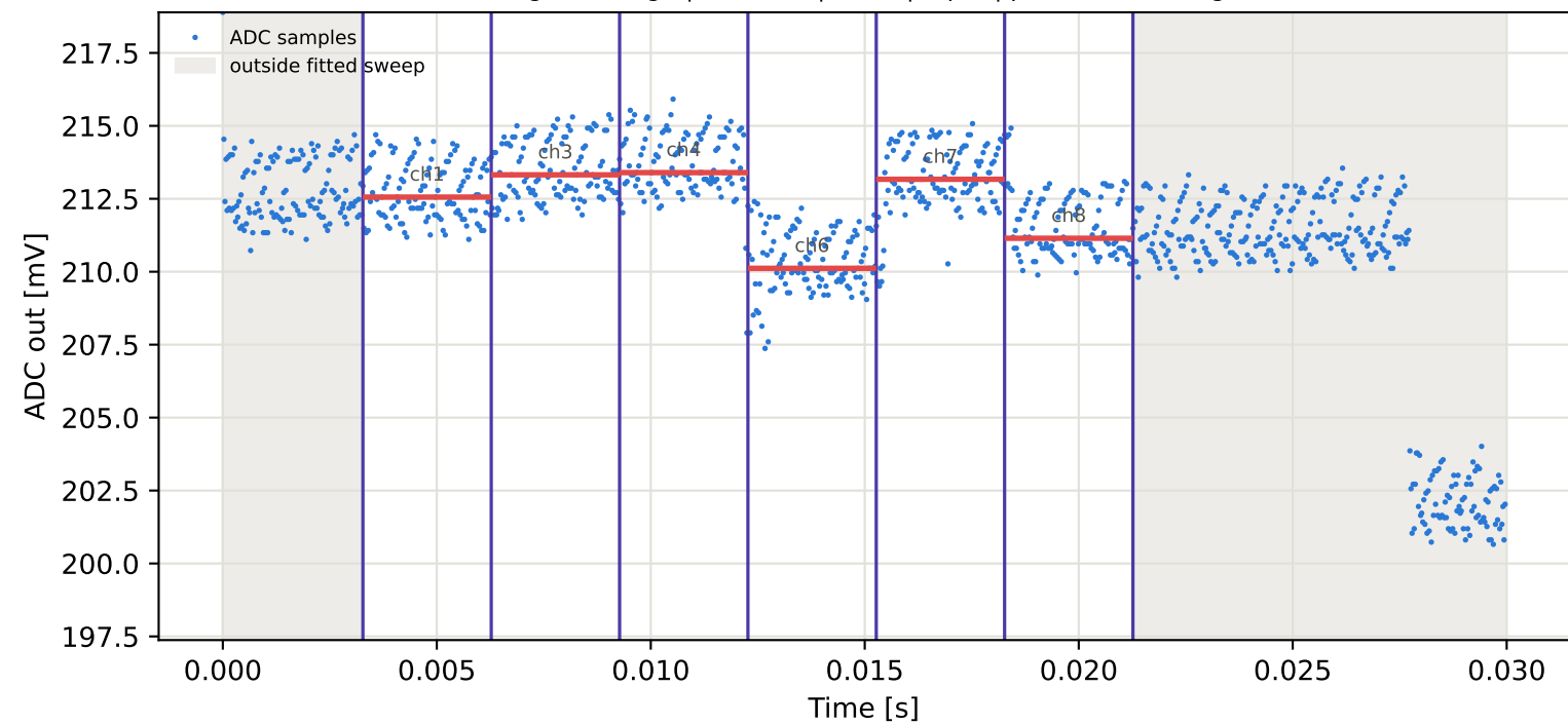
Tag15 &lt;- Tag4 | 955 MHz | run 0 | rep 1 | phase -161.41 deg
