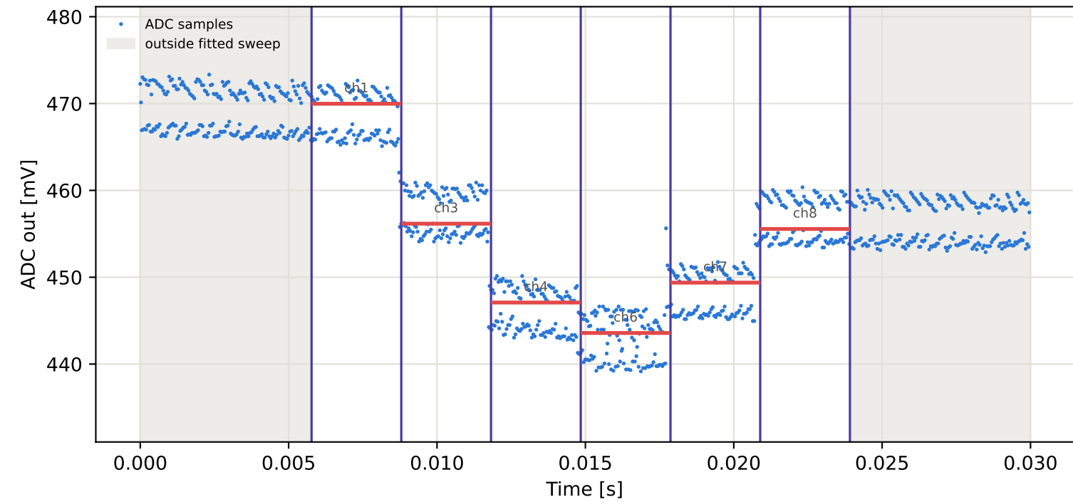
Tag15 &lt;- Tag6 | 875 MHz | run 0 | rep 1 | phase -175.01 deg
