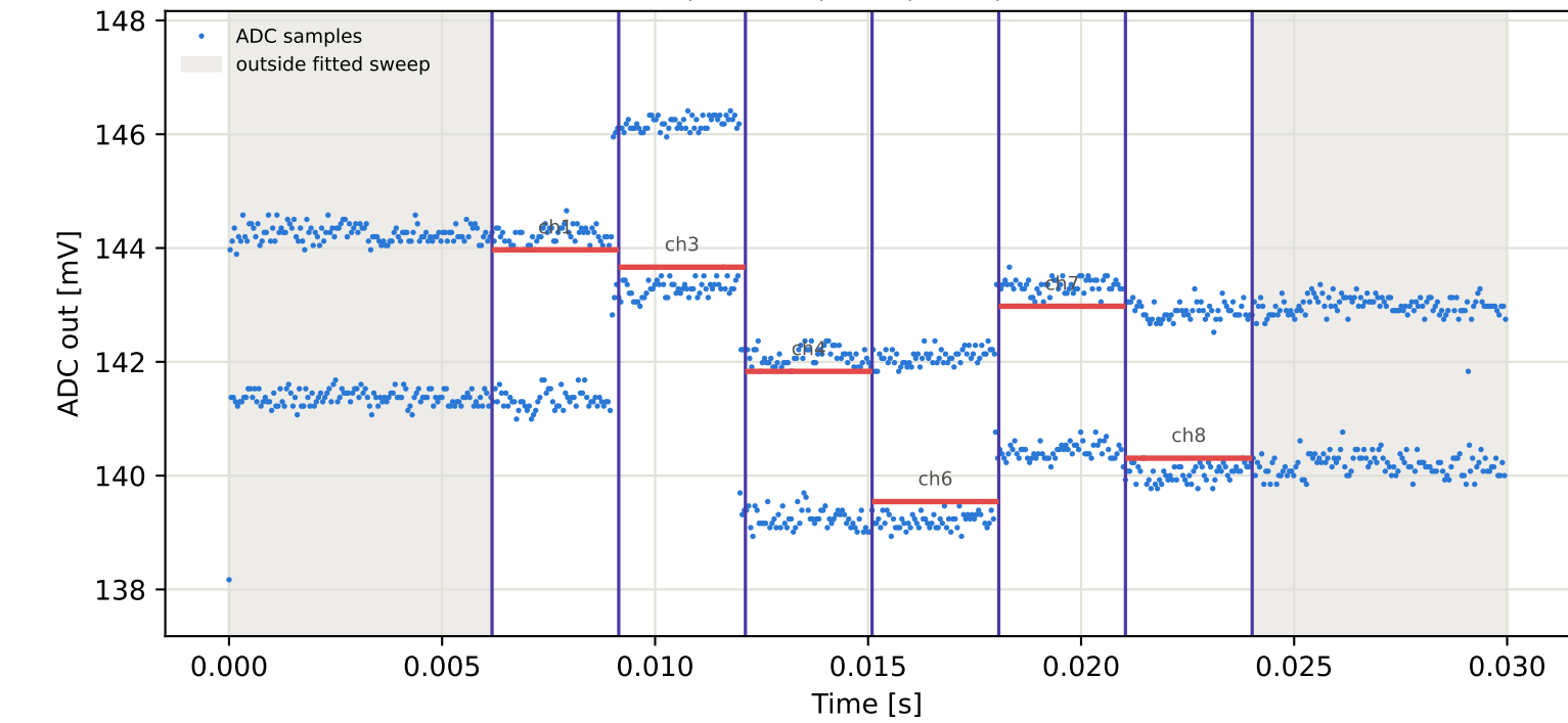
Tag5 &lt;- Tag3 | 805 MHz | run 0 | rep 1 | phase 27.50 deg
