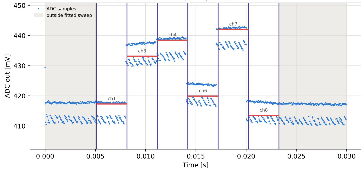
Tag6 &lt;- Tag3 | 835 MHz | run 0 | rep 1 | phase 27.71 deg
