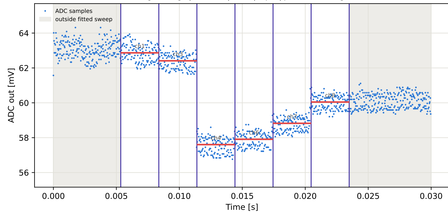
Tag1 &lt;- Tag8 | 825 MHz | run 0 | rep 1 | phase -99.10 deg
