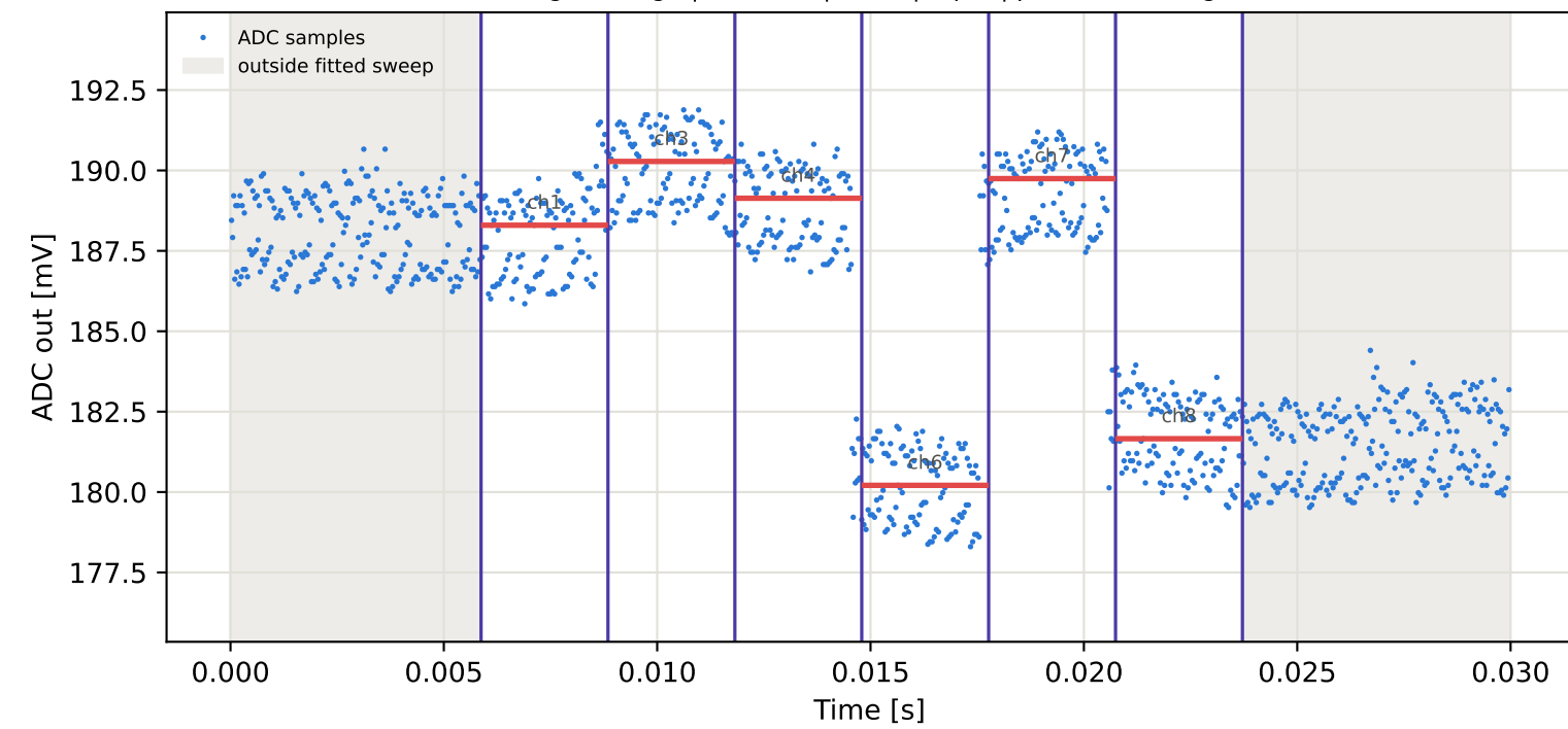
Tag3 &lt;- Tag10 | 905 MHz | run 0 | rep 1 | phase 70.04 deg
