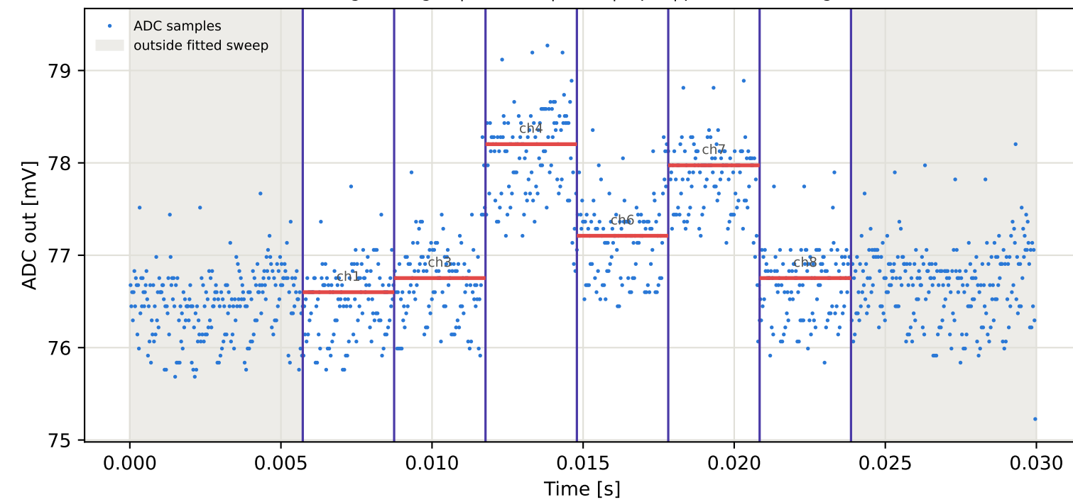
Tag6 &lt;- Tag2 | 775 MHz | run 0 | rep 1 | phase -4.01 deg
