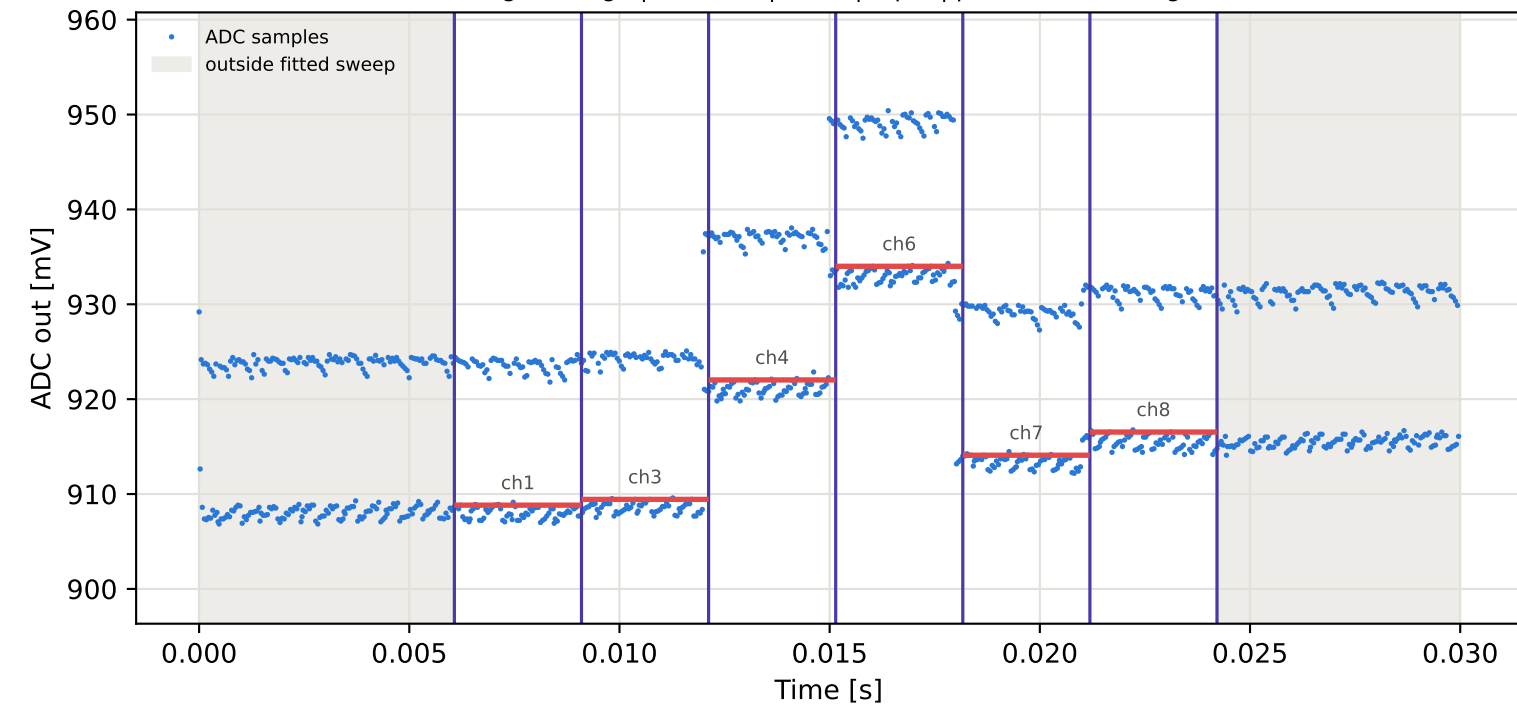
Tag7 &lt;- Tag5 | 965 MHz | run 0 | rep 1 | phase -39.37 deg
