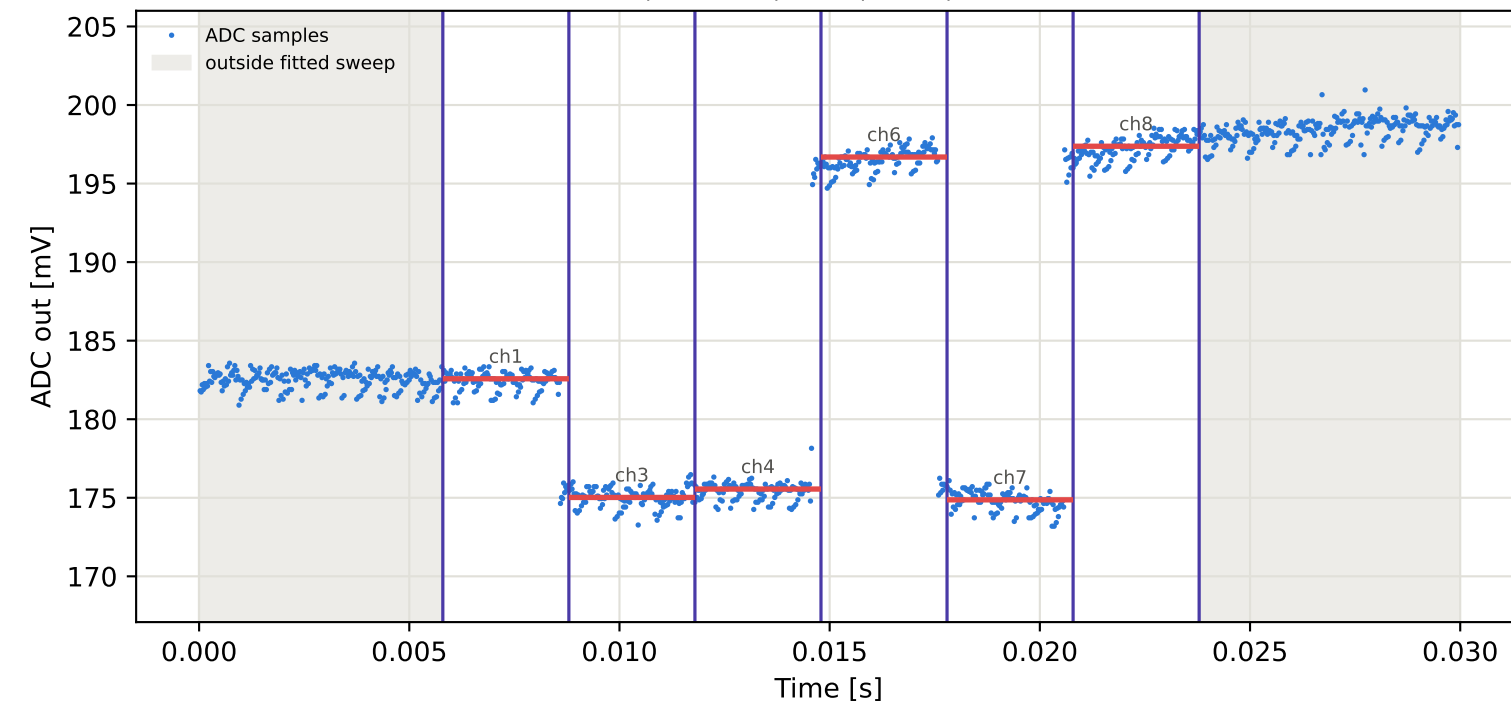
Tag4 &lt;- Tag9 | 905 MHz | run 0 | rep 1 | phase 159.30 deg
