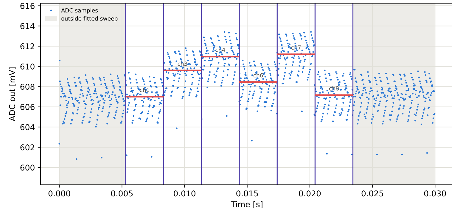
Tag6 &lt;- Tag1 | 845 MHz | run 0 | rep 1 | phase -70.97 deg
