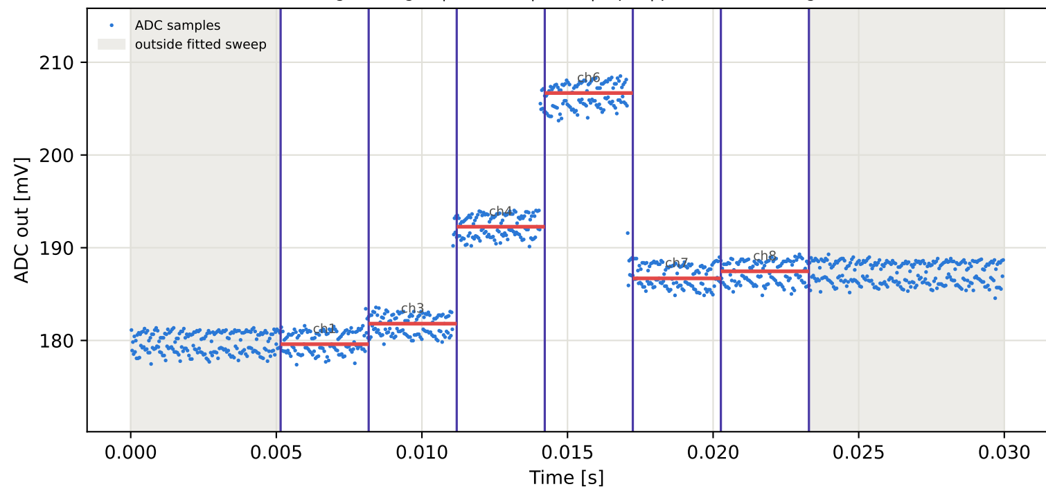
Tag4 &lt;- Tag16 | 925 MHz | run 0 | rep 1 | phase 3.71 deg
