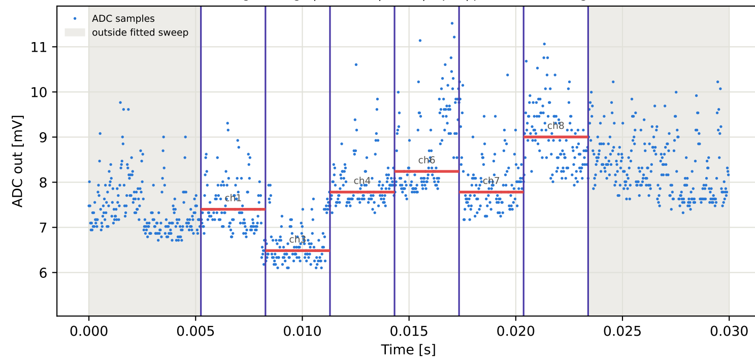
Tag3 &lt;- Tag10 | 785 MHz | run 0 | rep 1 | phase -61.09 deg
