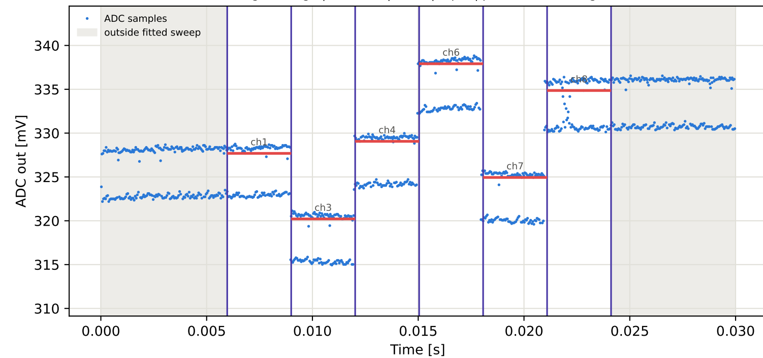
Tag9 &lt;- Tag10 | 805 MHz | run 0 | rep 1 | phase -44.74 deg
