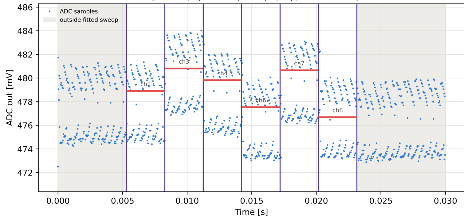
Tag16 &lt;- Tag15 | 855 MHz | run 0 | rep 1 | phase -30.99 deg
