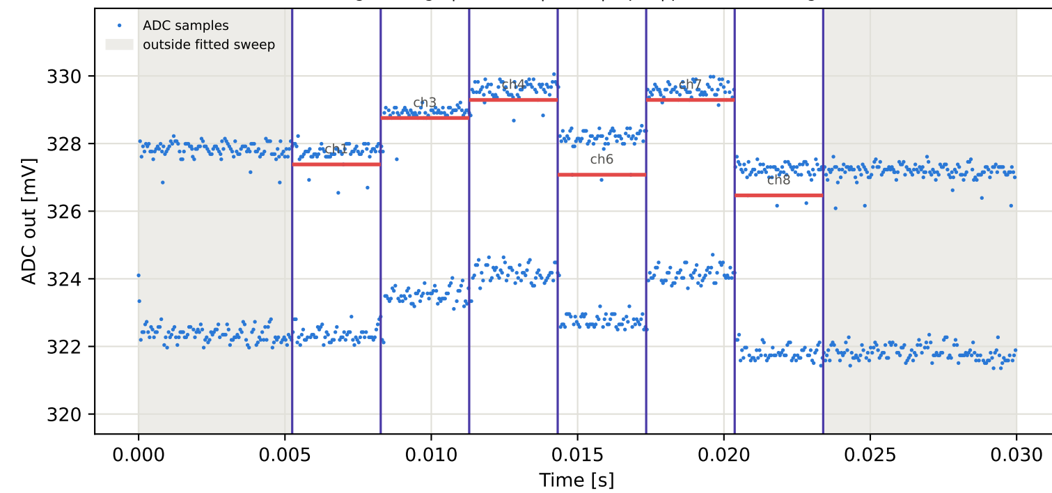
Tag8 &lt;- Tag4 | 805 MHz | run 0 | rep 1 | phase 23.20 deg
