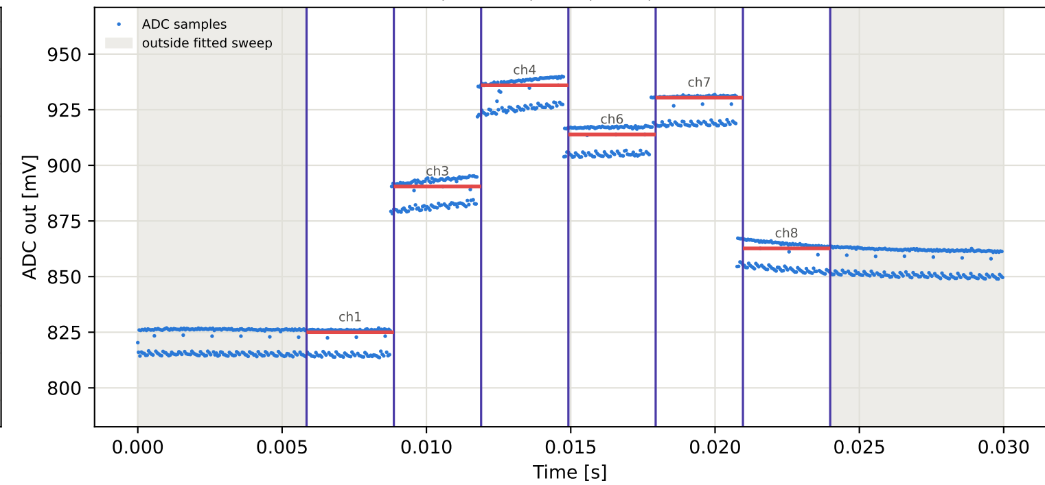
Tag3 &lt;- Tag9 | 875 MHz | run 0 | rep 1 | phase -102.90 deg
