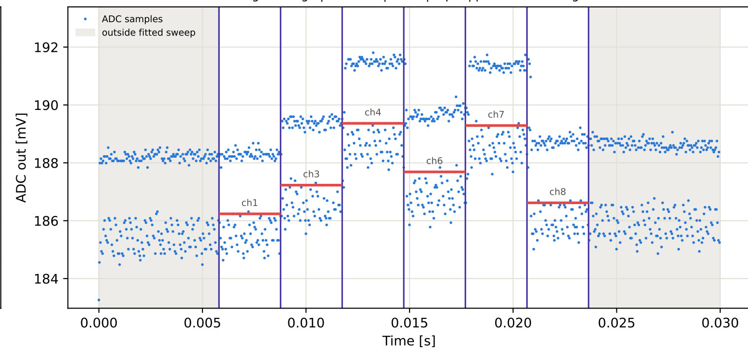
Tag3 &lt;- Tag7 | 805 MHz | run 0 | rep 1 | phase -106.23 deg
