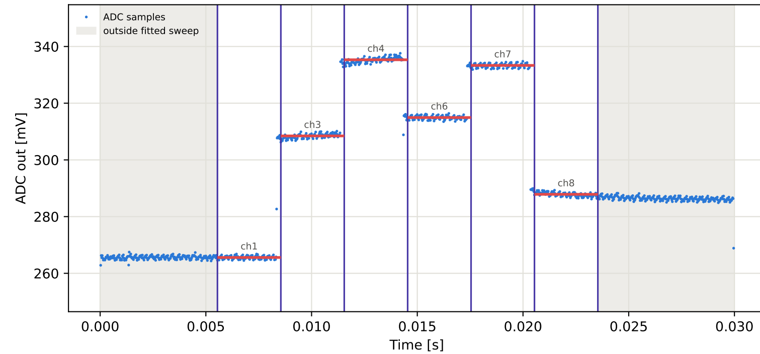
Tag3 &lt;- Tag8 | 845 MHz | run 0 | rep 1 | phase 43.97 deg
