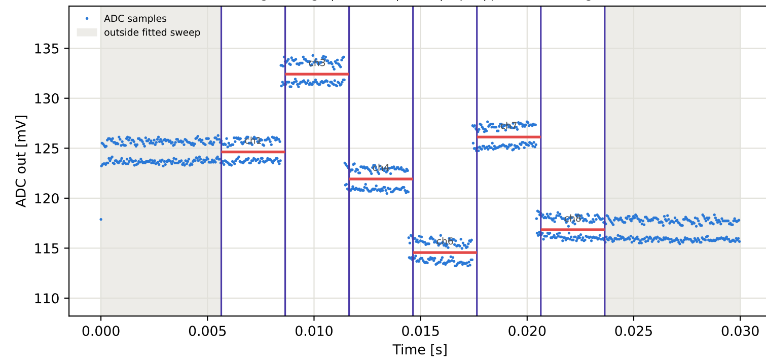
Tag5 &lt;- Tag8 | 825 MHz | run 0 | rep 1 | phase 171.68 deg
