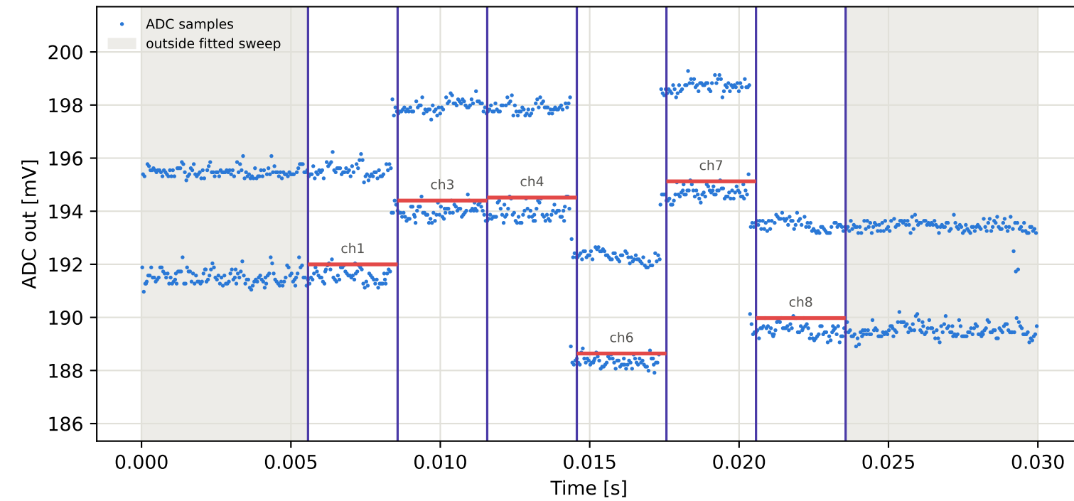
Tag4 &lt;- Tag9 | 985 MHz | run 0 | rep 1 | phase -56.48 deg
