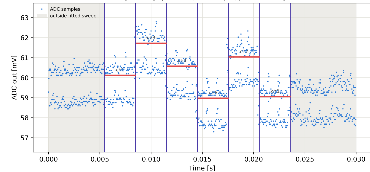
Tag15 &lt;- Tag1 | 845 MHz | run 0 | rep 1 | phase -1.80 deg
