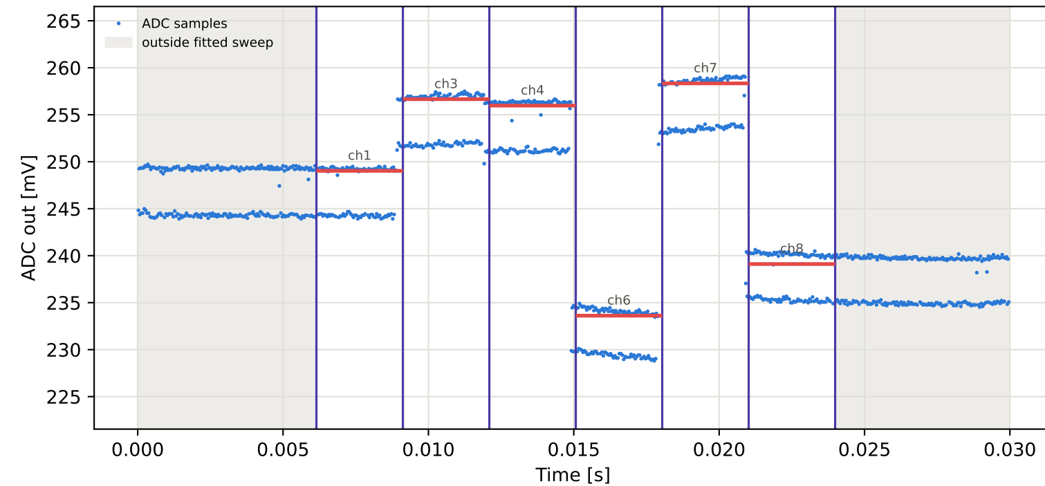
Tag5 &lt;- Tag3 | 985 MHz | run 0 | rep 1 | phase -107.15 deg
