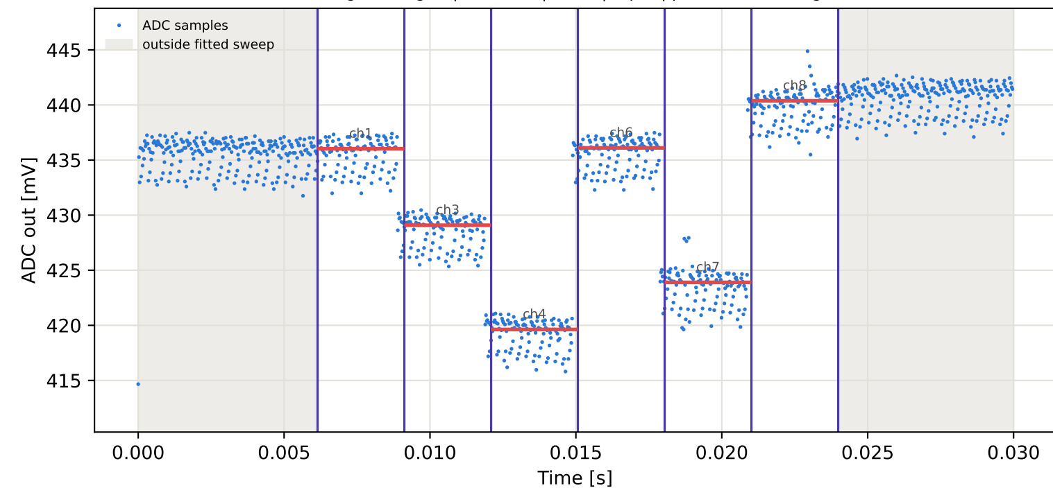
Tag1 &lt;- Tag16 | 935 MHz | run 0 | rep 1 | phase 101.50 deg
