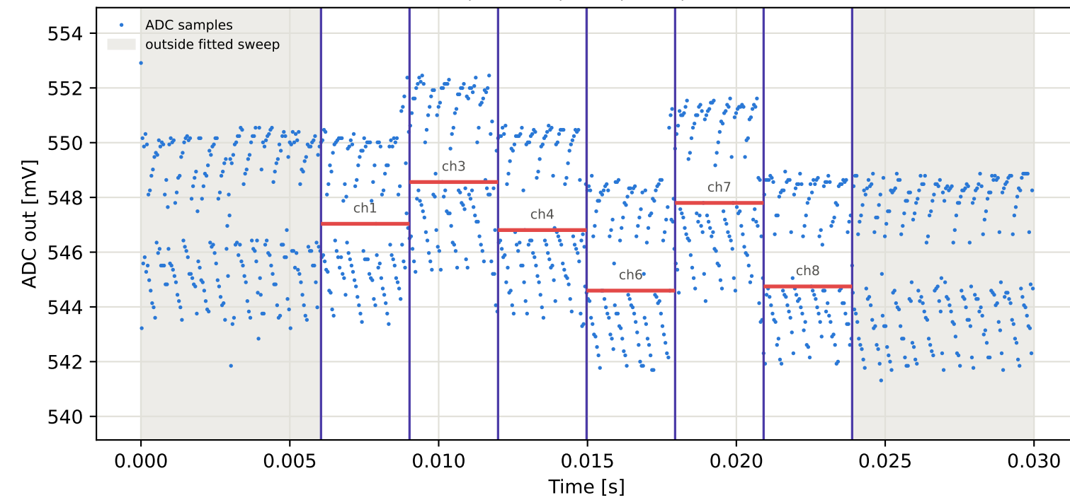
Tag8 &lt;- Tag15 | 825 MHz | run 0 | rep 1 | phase 11.64 deg
