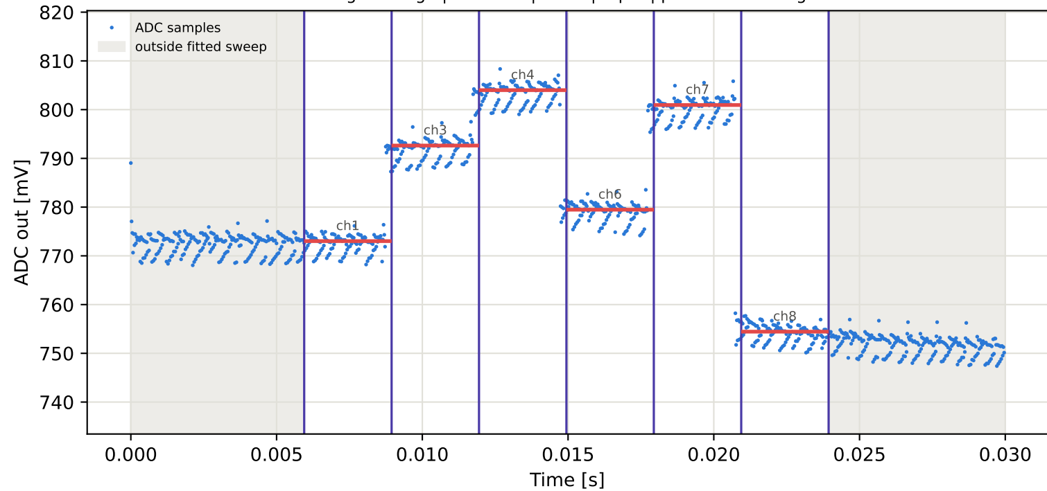
Tag9 &lt;- Tag8 | 895 MHz | run 0 | rep 1 | phase 57.06 deg
