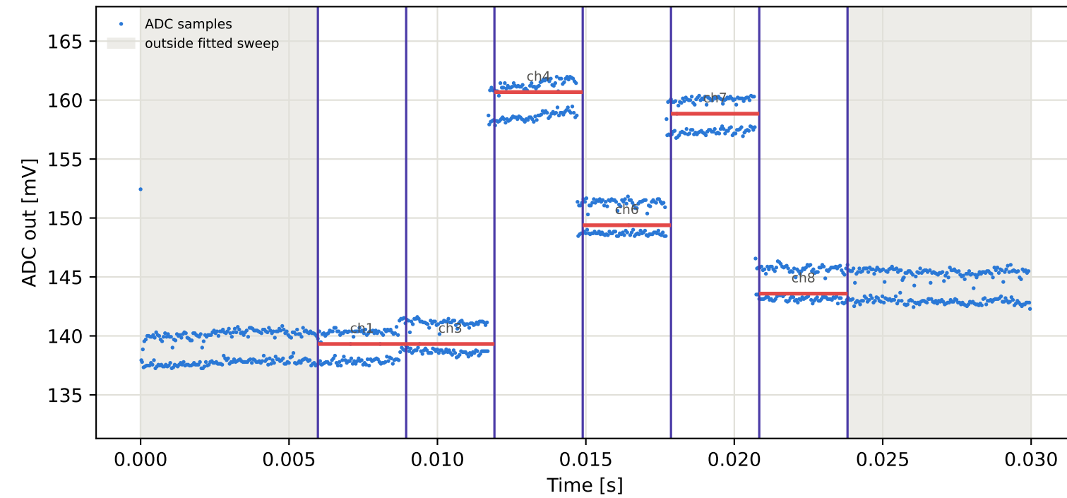
Tag9 &lt;- Tag16 | 785 MHz | run 0 | rep 1 | phase -22.48 deg
