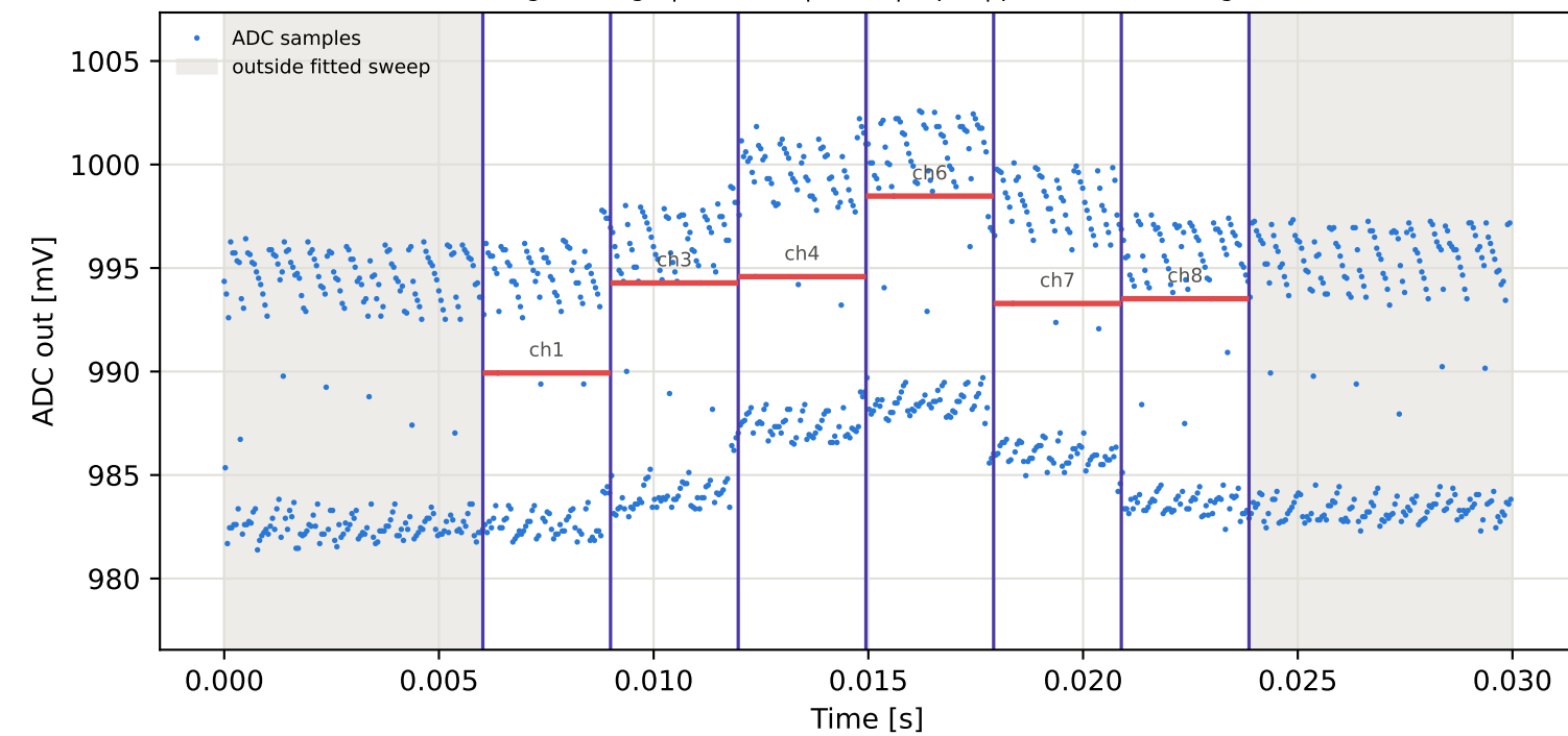
Tag8 &lt;- Tag4 | 895 MHz | run 0 | rep 1 | phase 26.40 deg
