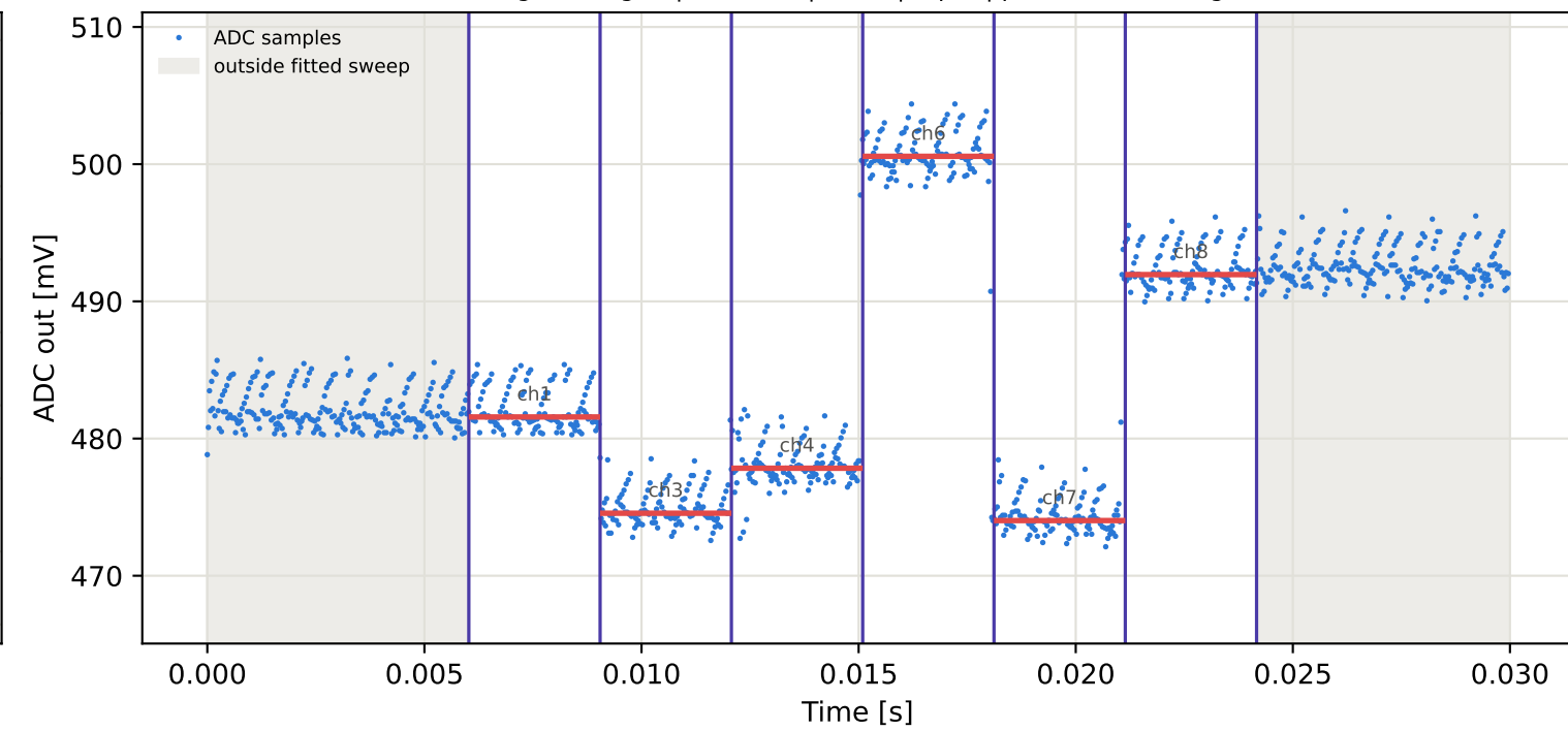
Tag6 &lt;- Tag3 | 965 MHz | run 0 | rep 1 | phase 166.09 deg
