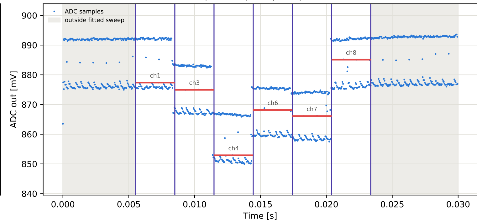
Tag8 &lt;- Tag5 | 935 MHz | run 0 | rep 1 | phase -170.17 deg
