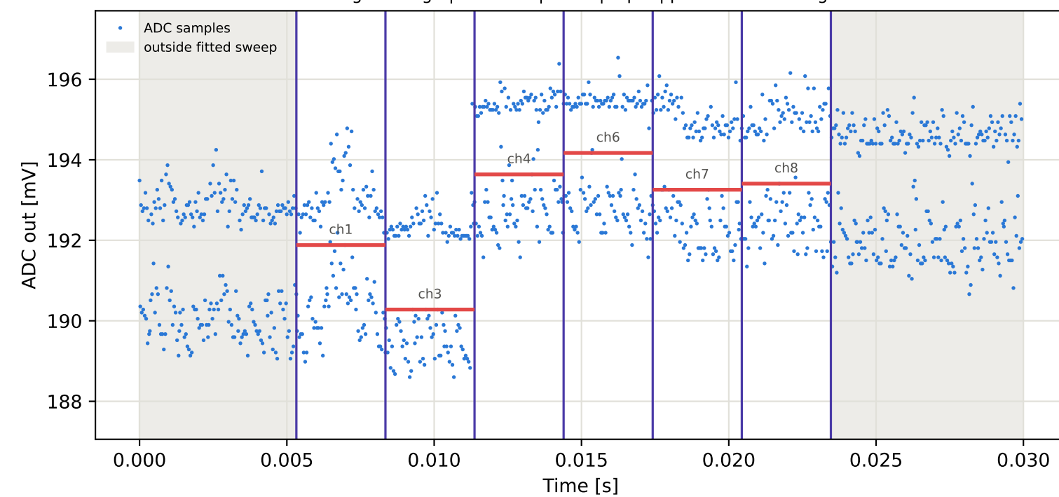
Tag2 &lt;- Tag15 | 835 MHz | run 0 | rep 1 | phase -89.72 deg
