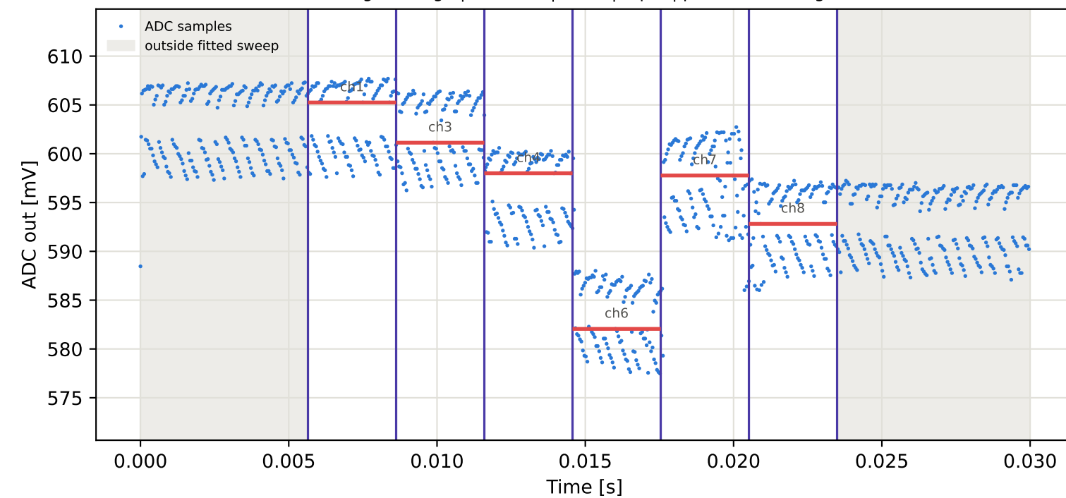
Tag6 &lt;- Tag1 | 905 MHz | run 0 | rep 1 | phase 21.20 deg
