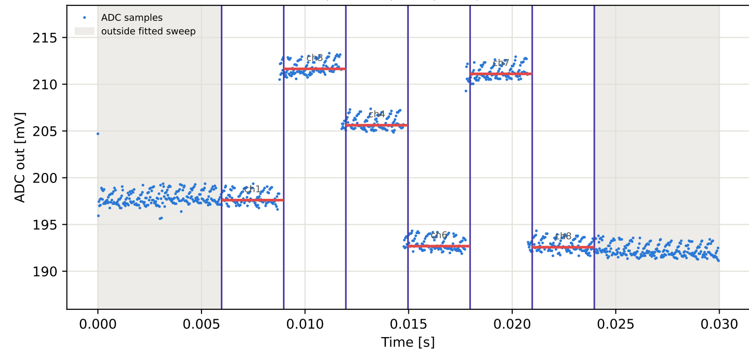
Tag16 &lt;- Tag15 | 825 MHz | run 0 | rep 1 | phase -12.85 deg
