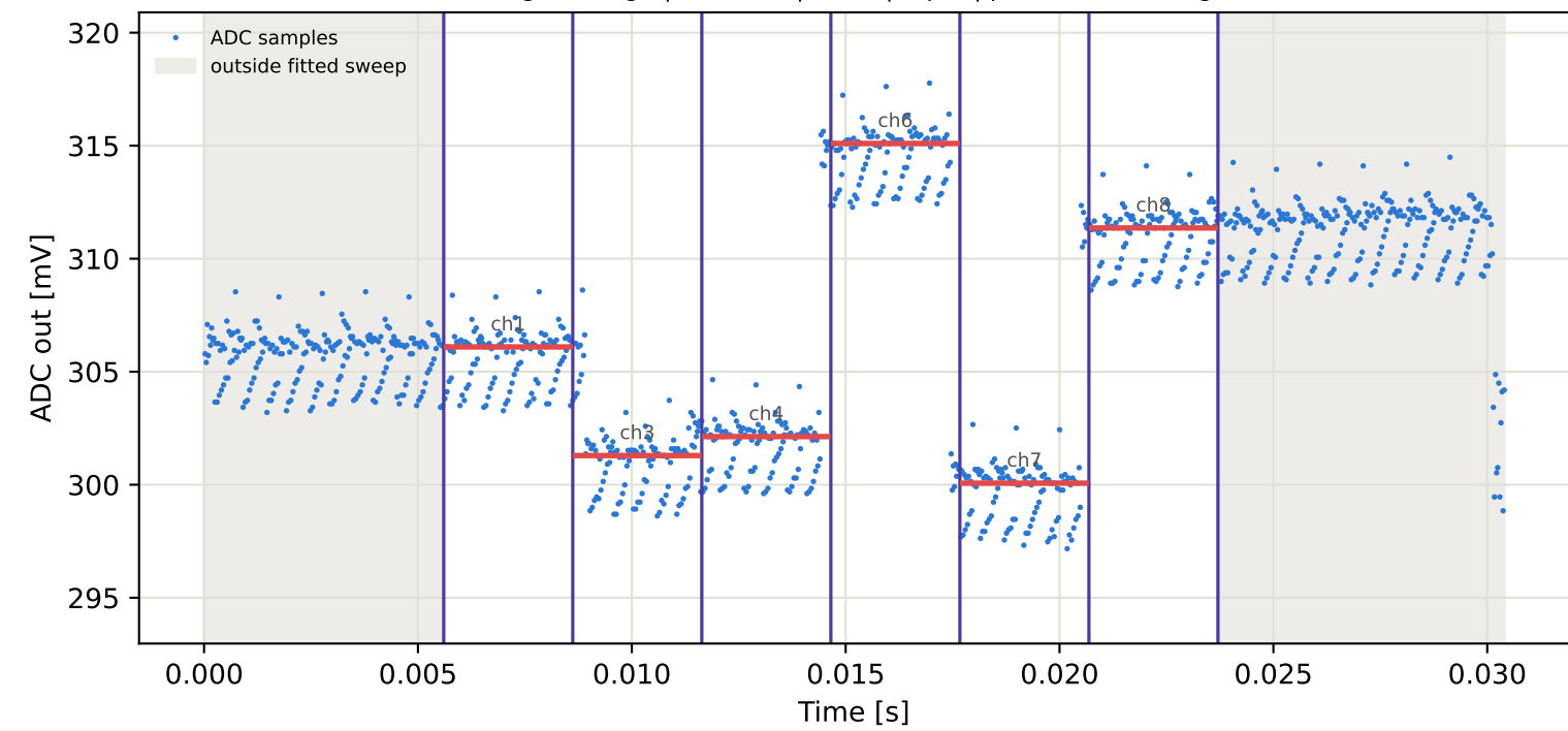
Tag5 &lt;- Tag9 | 975 MHz | run 0 | rep 1 | phase 13.06 deg
