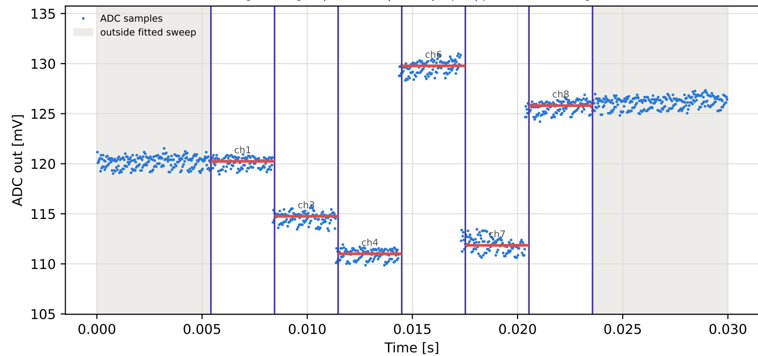
Tag4 &lt;- Tag16 | 975 MHz | run 0 | rep 1 | phase 16.25 deg
