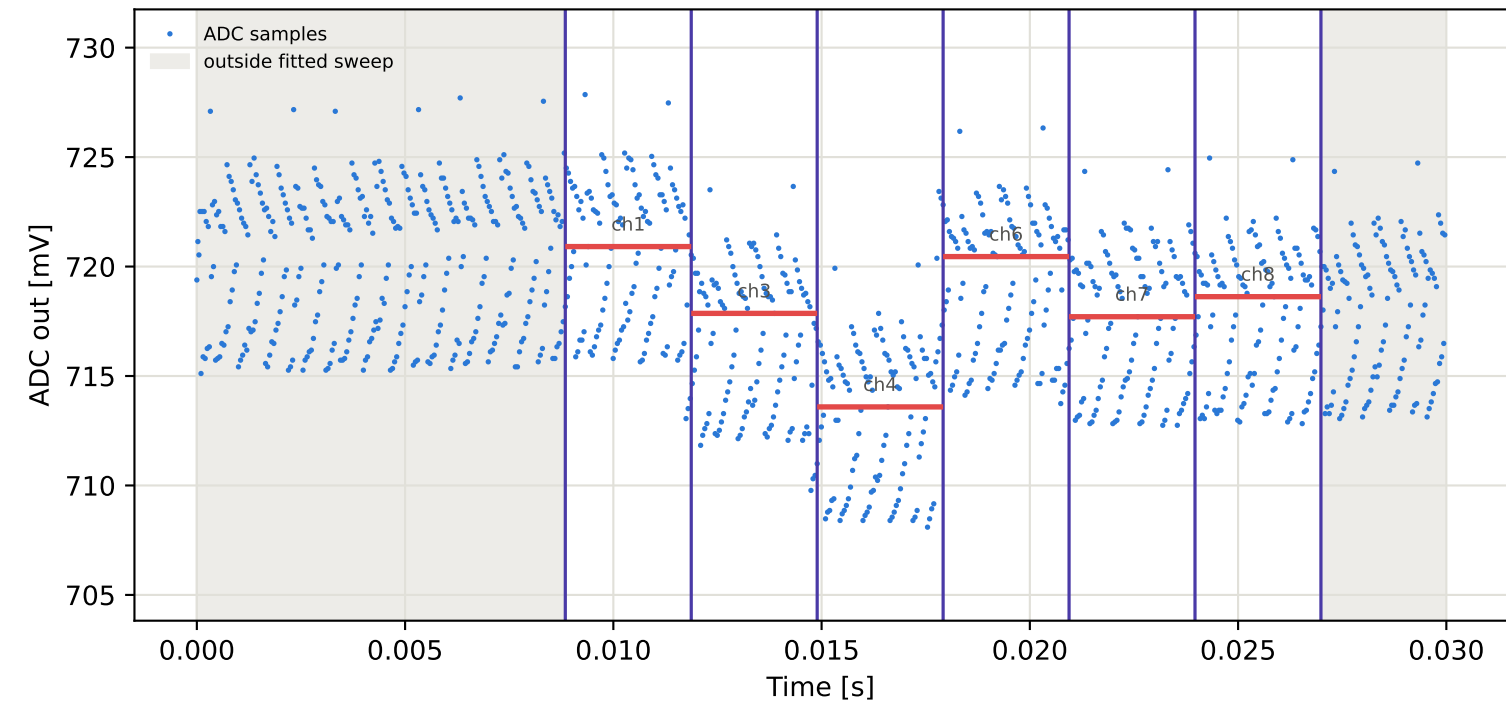
Tag9 &lt;- Tag2 | 965 MHz | run 0 | rep 1 | phase -68.27 deg
