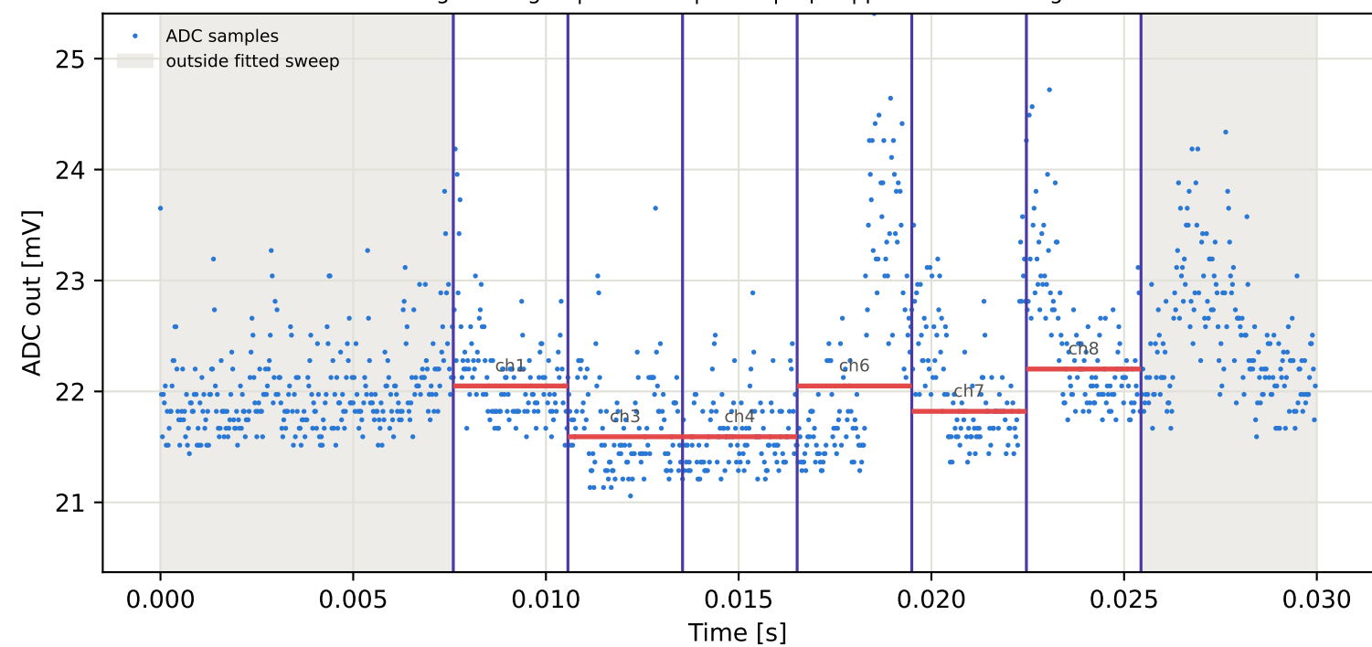
Tag2 &lt;- Tag16 | 805 MHz | run 0 | rep 1 | phase 141.73 deg
