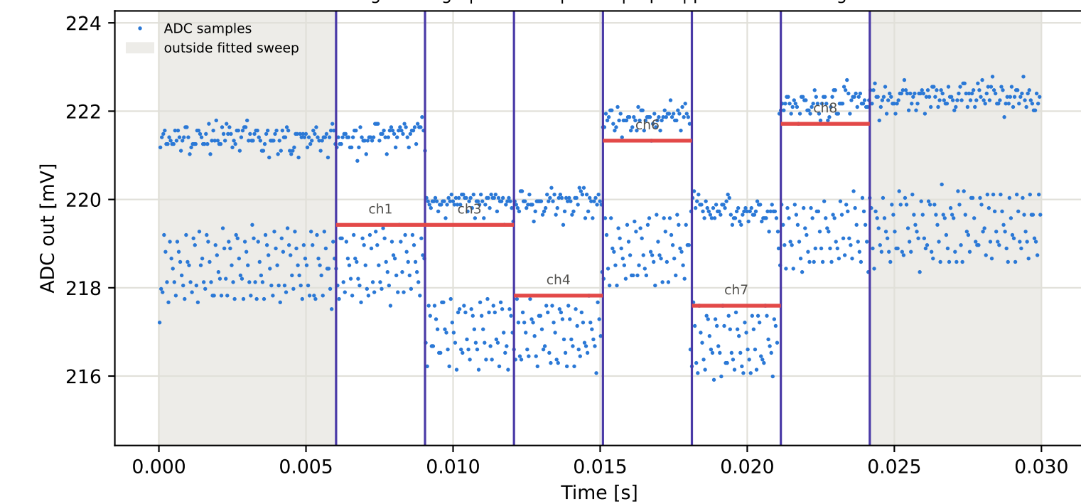
Tag1 &lt;- Tag9 | 865 MHz | run 0 | rep 1 | phase -101.84 deg
