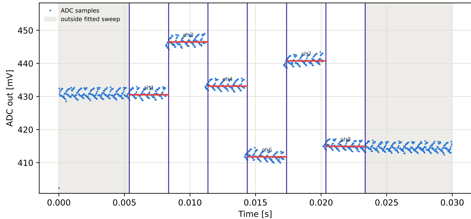
Tag6 &lt;- Tag10 | 845 MHz | run 0 | rep 1 | phase -168.10 deg
