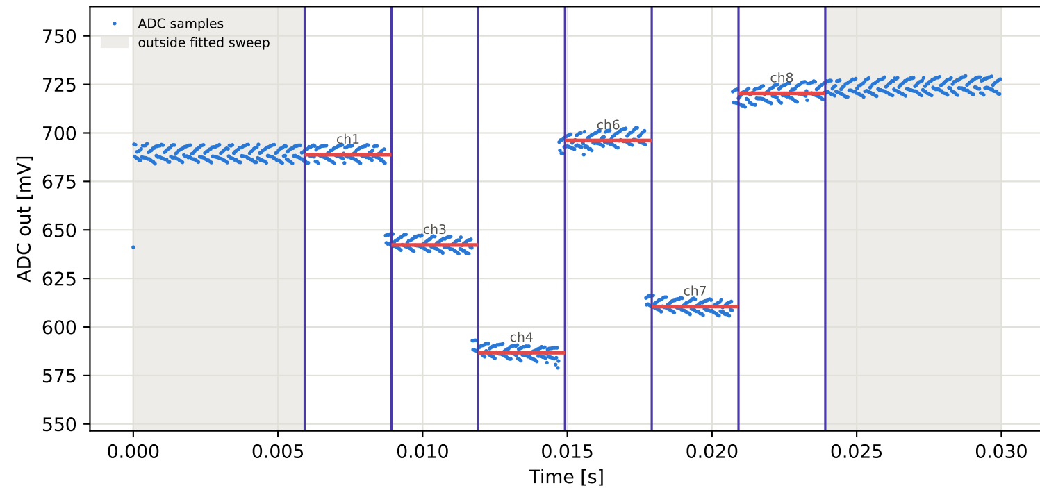
Tag10 &lt;- Tag5 | 945 MHz | run 0 | rep 1 | phase -50.32 deg
