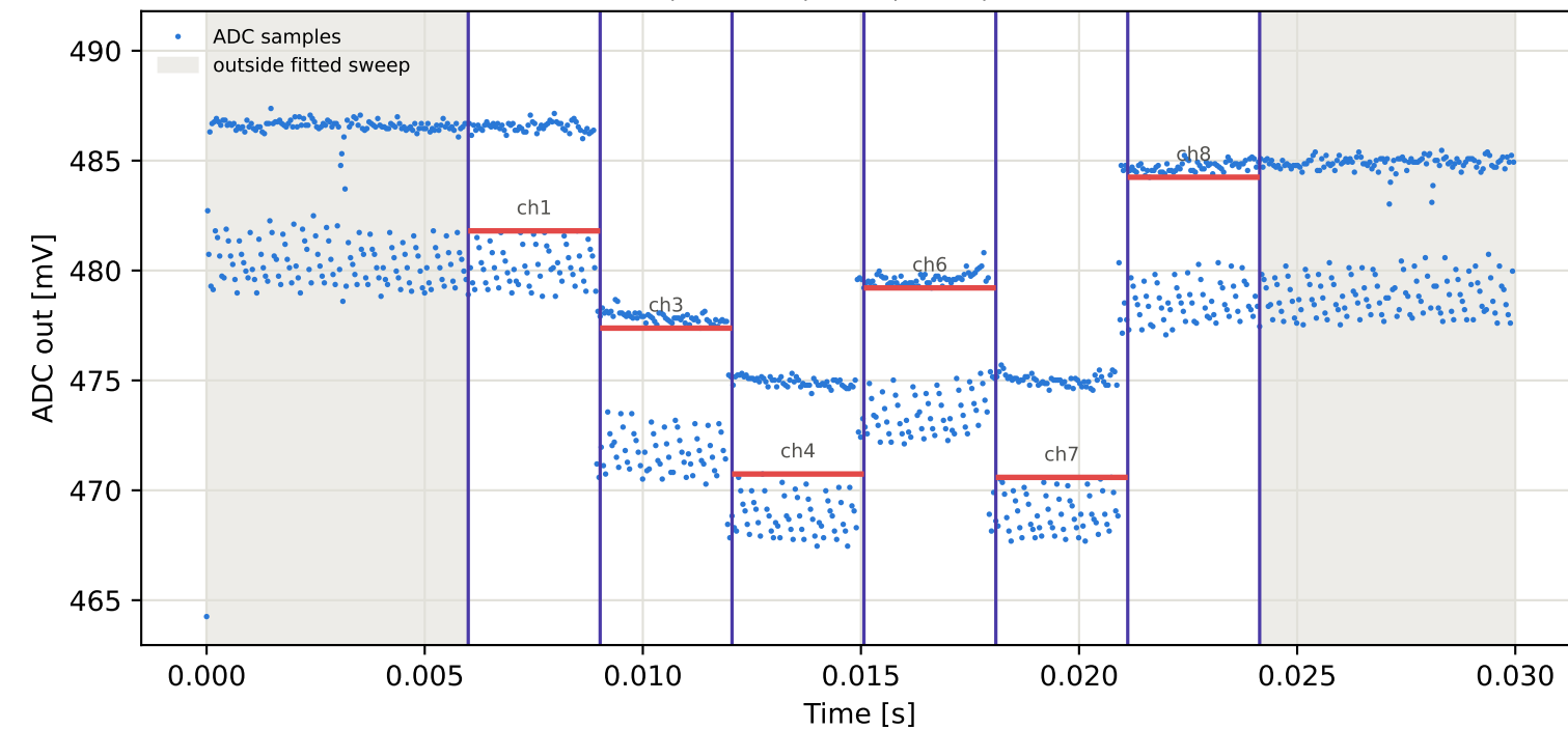
Tag3 &lt;- Tag8 | 855 MHz | run 0 | rep 1 | phase 104.16 deg
