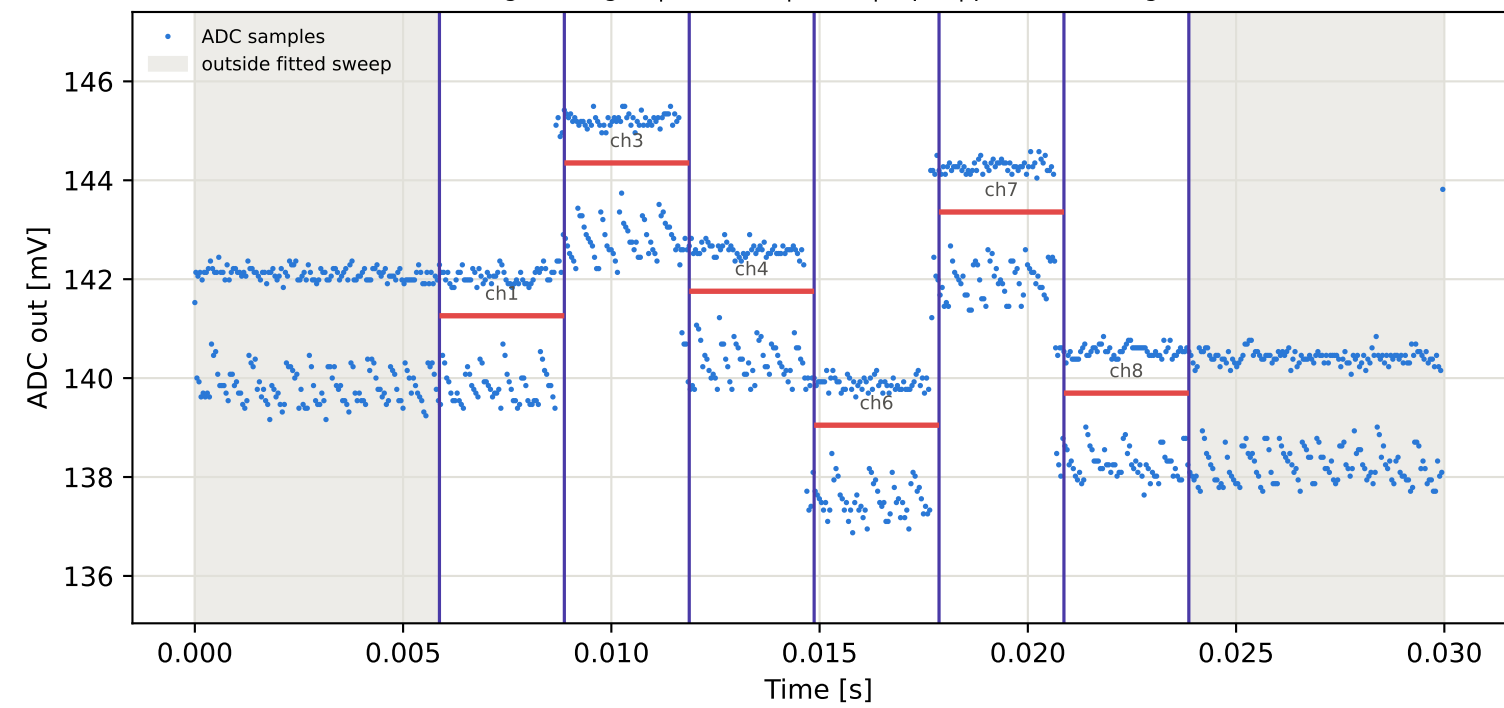
Tag5 &lt;- Tag2 | 805 MHz | run 0 | rep 1 | phase -30.91 deg
