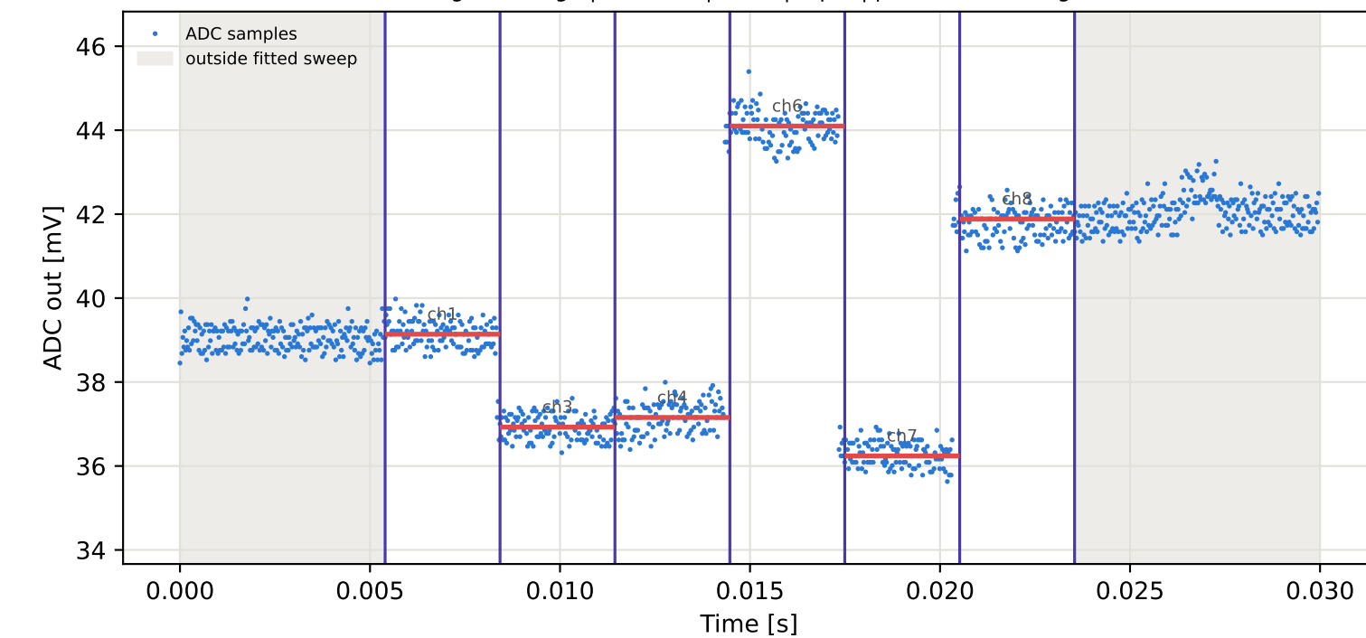
Tag15 &lt;- Tag1 | 965 MHz | run 0 | rep 1 | phase 160.06 deg
