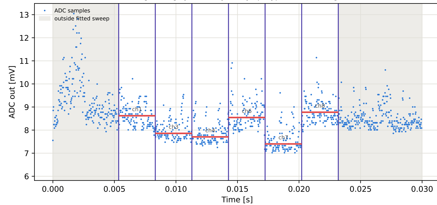
Tag2 &lt;- Tag5 | 785 MHz | run 0 | rep 1 | phase -170.38 deg
