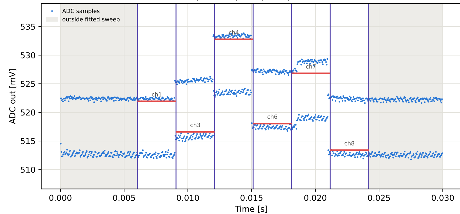
Tag1 &lt;- Tag7 | 965 MHz | run 0 | rep 1 | phase -6.20 deg
