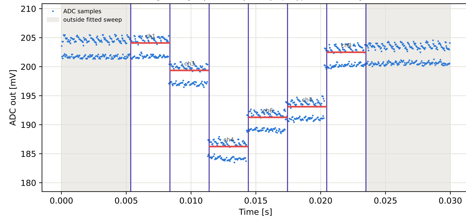
Tag5 &lt;- Tag16 | 945 MHz | run 0 | rep 1 | phase -35.80 deg
