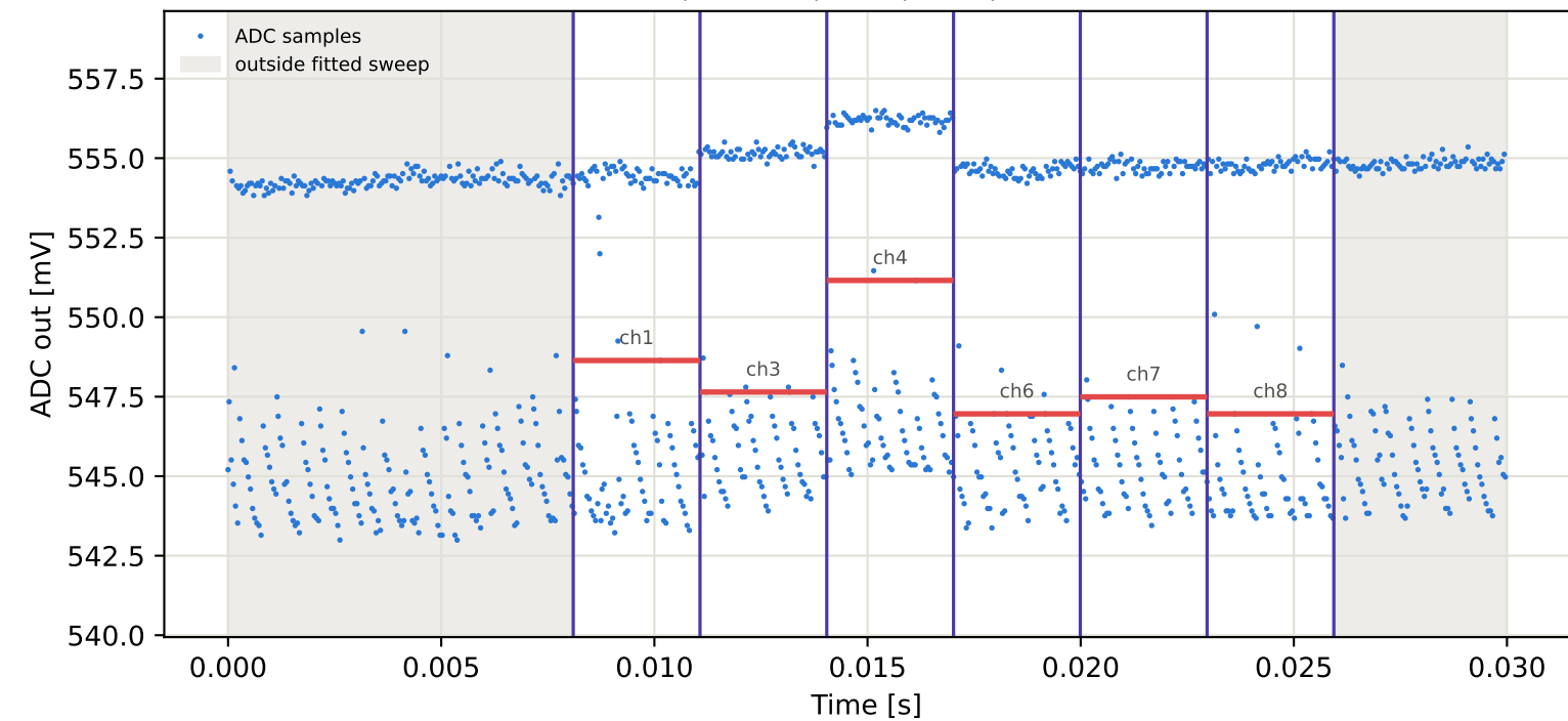
Tag9 &lt;- Tag2 | 975 MHz | run 0 | rep 1 | phase -95.42 deg
