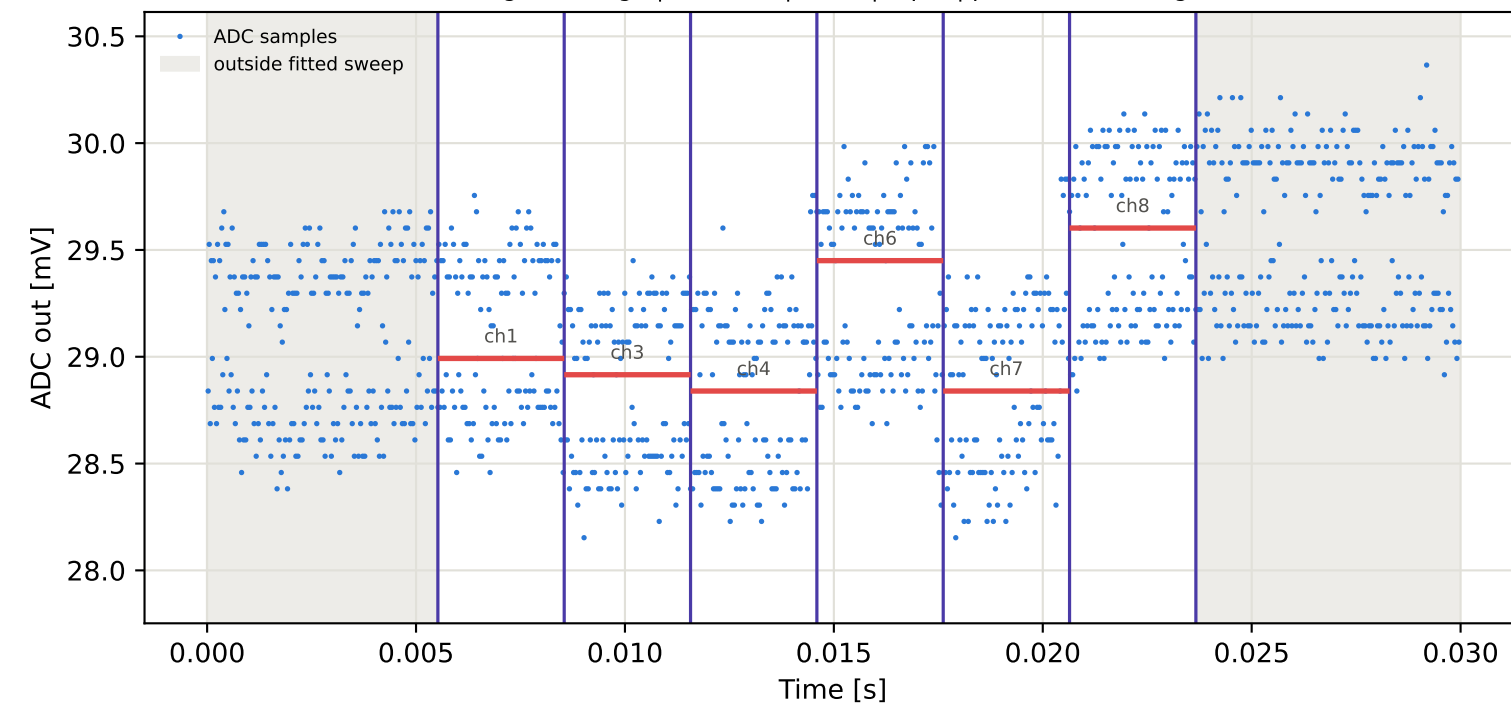
Tag16 &lt;- Tag4 | 805 MHz | run 0 | rep 1 | phase -32.29 deg
