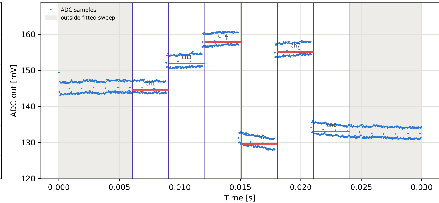
Tag1 &lt;- Tag4 | 925 MHz | run 0 | rep 1 | phase 113.91 deg
