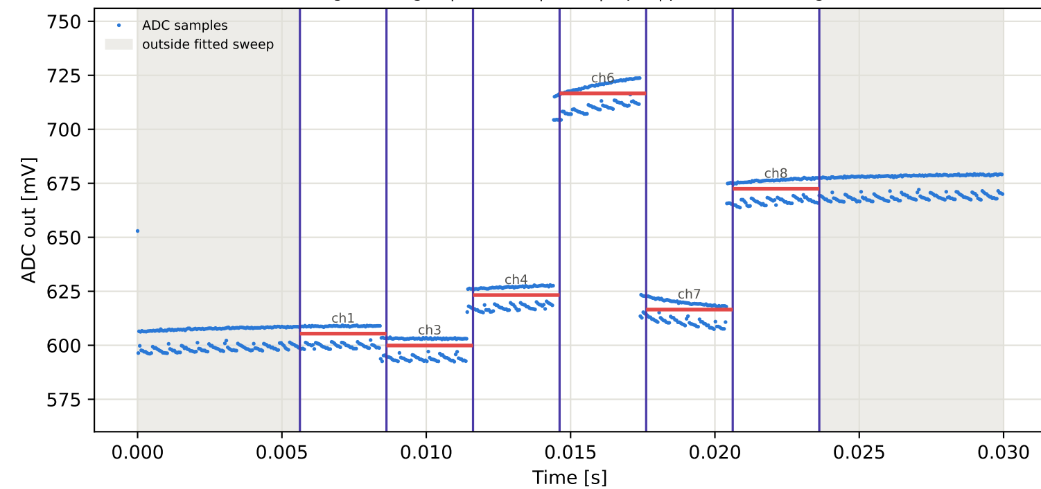
Tag15 &lt;- Tag3 | 905 MHz | run 0 | rep 1 | phase 163.87 deg
