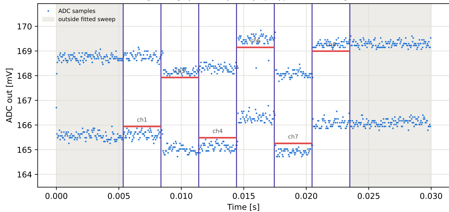
Tag8 &lt;- Tag4 | 785 MHz | run 0 | rep 1 | phase -118.59 deg
