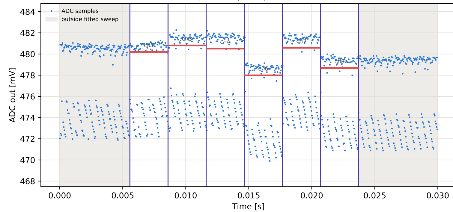
Tag6 &lt;- Tag2 | 965 MHz | run 0 | rep 1 | phase 56.51 deg
