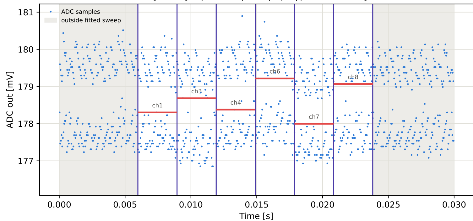
Tag7 &lt;- Tag15 | 775 MHz | run 0 | rep 1 | phase 173.59 deg
