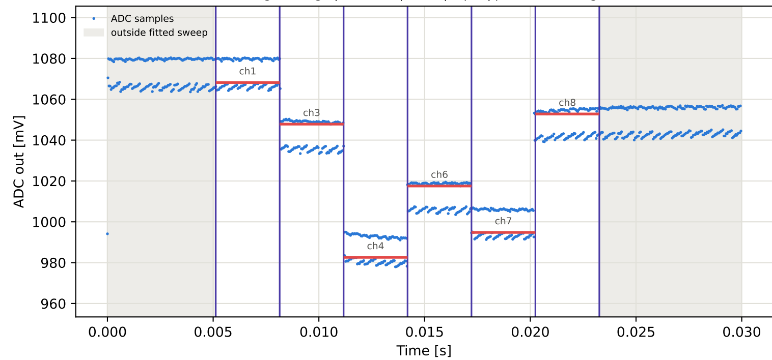
Tag8 &lt;- Tag10 | 845 MHz | run 0 | rep 1 | phase 76.88 deg
