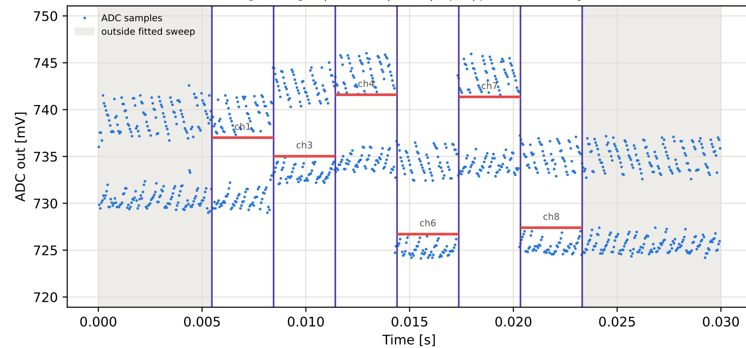
Tag6 &lt;- Tag2 | 925 MHz | run 0 | rep 1 | phase -149.55 deg
