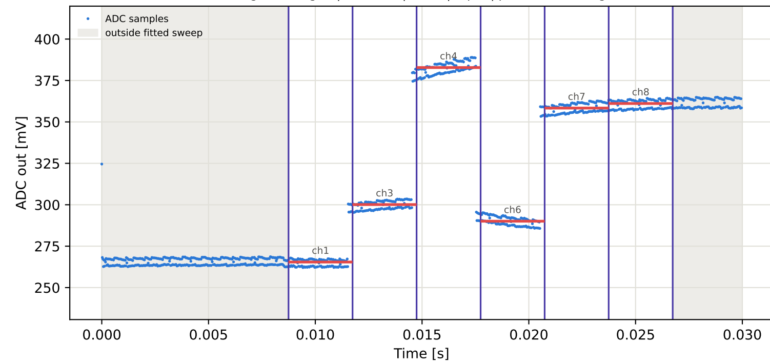
Tag15 &lt;- Tag3 | 895 MHz | run 0 | rep 1 | phase 146.57 deg
