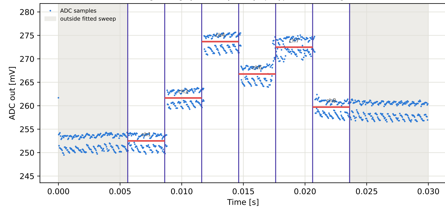
Tag4 &lt;- Tag7 | 835 MHz | run 0 | rep 1 | phase -9.75 deg
