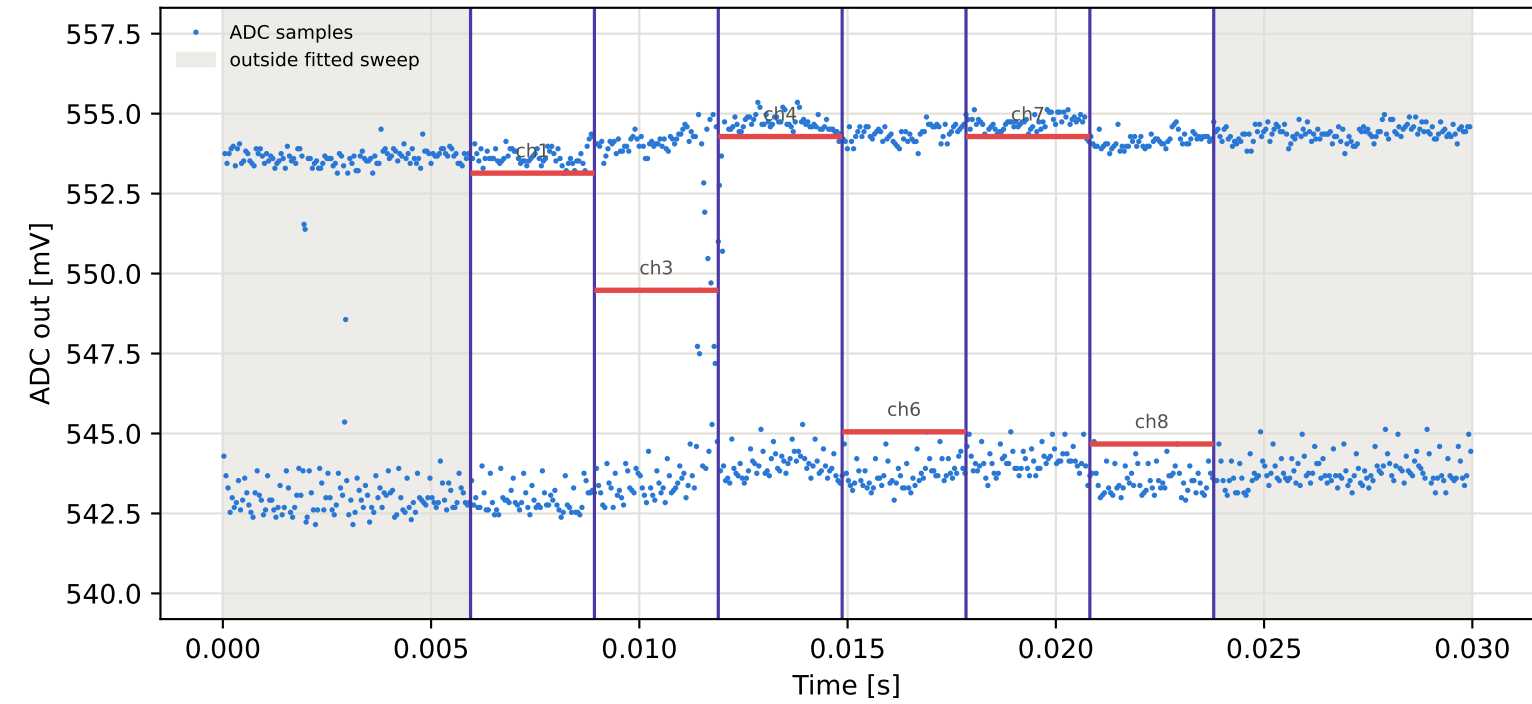
Tag3 &lt;- Tag2 | 955 MHz | run 0 | rep 1 | phase -35.57 deg
