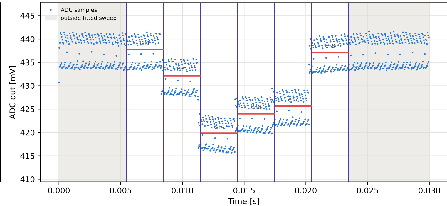
Tag10 &lt;- Tag1 | 935 MHz | run 0 | rep 1 | phase 137.32 deg
