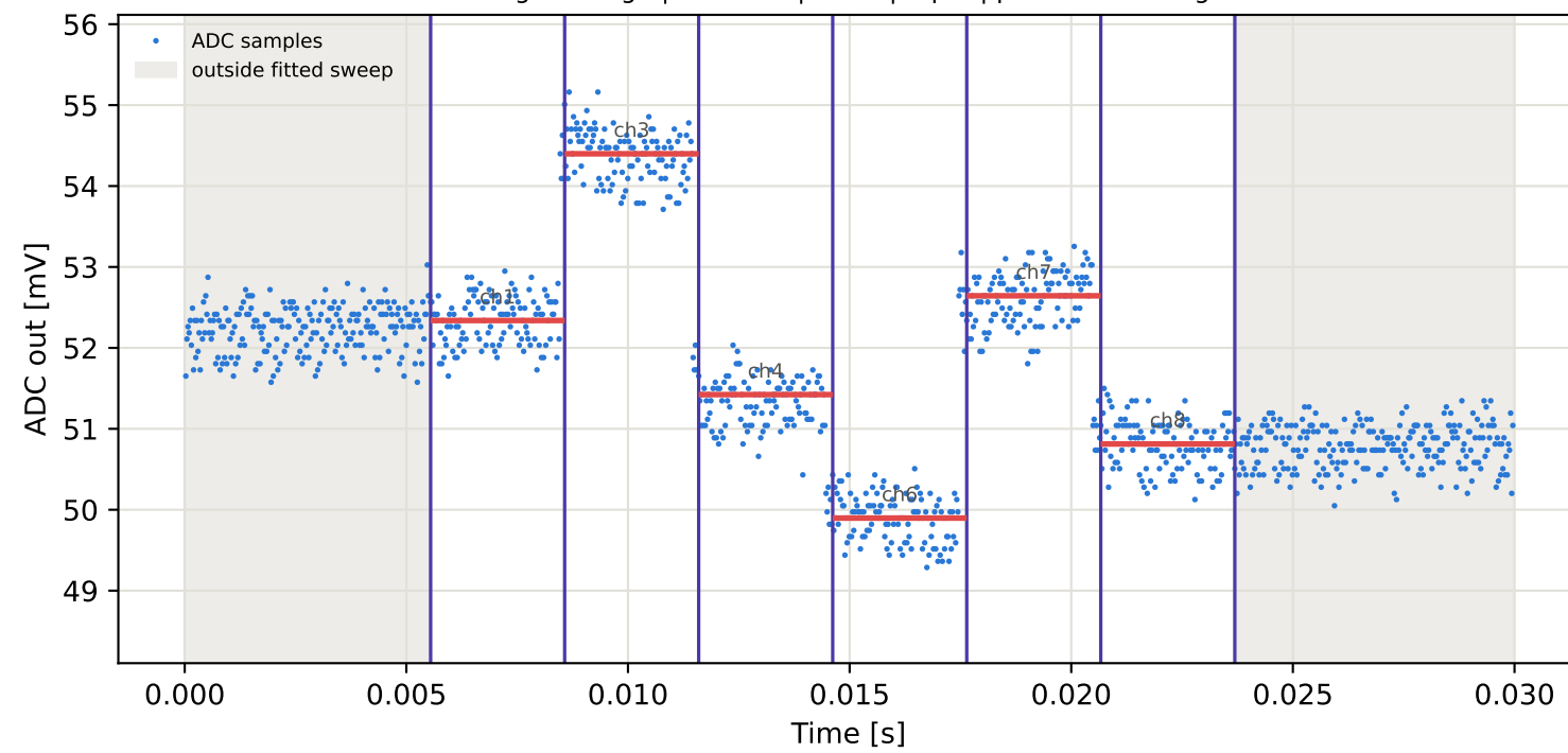
Tag5 &lt;- Tag8 | 785 MHz | run 0 | rep 1 | phase 99.46 deg
