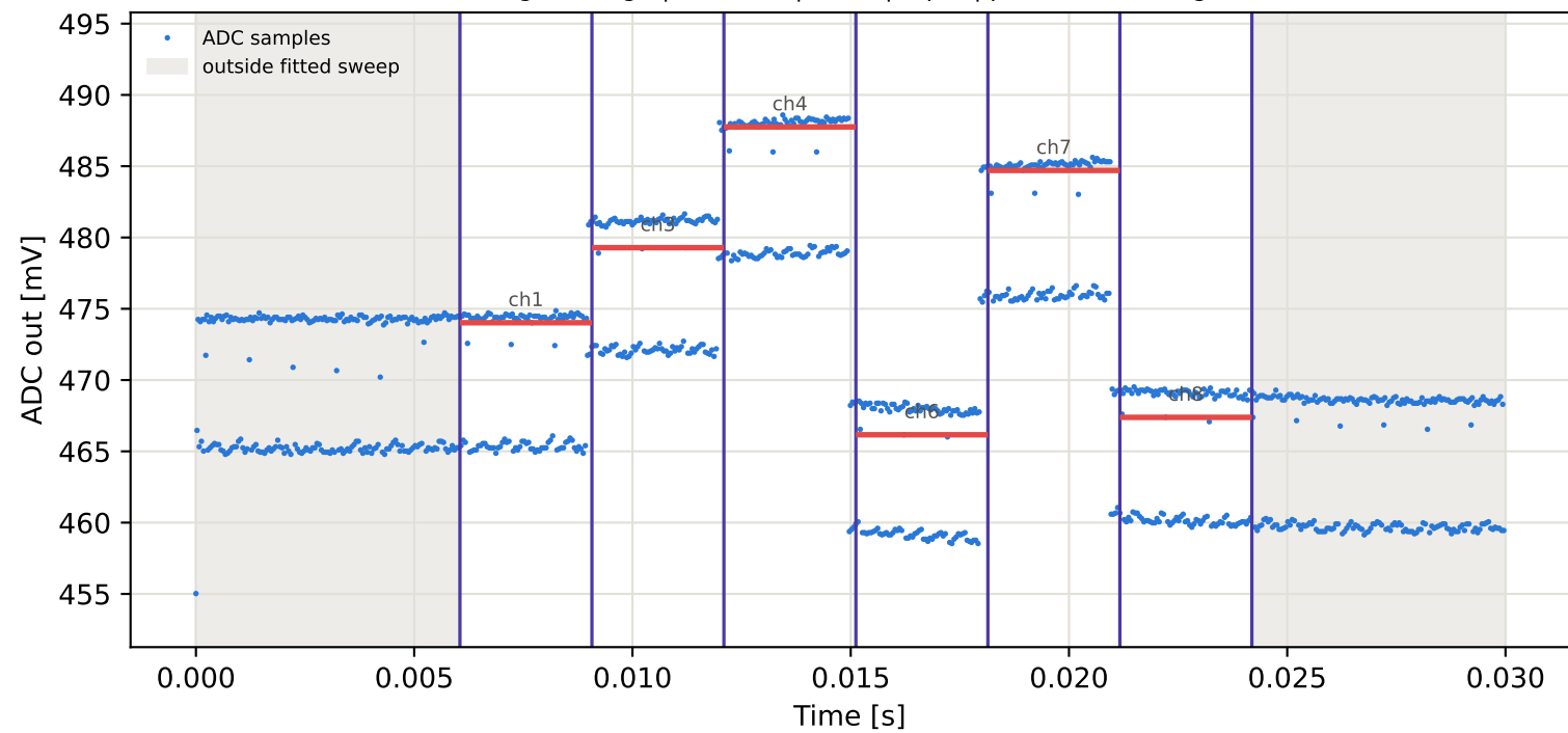
Tag7 &lt;- Tag1 | 965 MHz | run 0 | rep 1 | phase 58.24 deg
