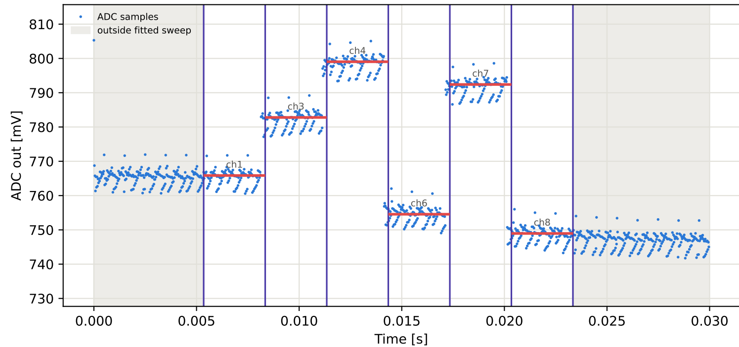
Tag8 &lt;- Tag16 | 925 MHz | run 0 | rep 1 | phase -112.54 deg
