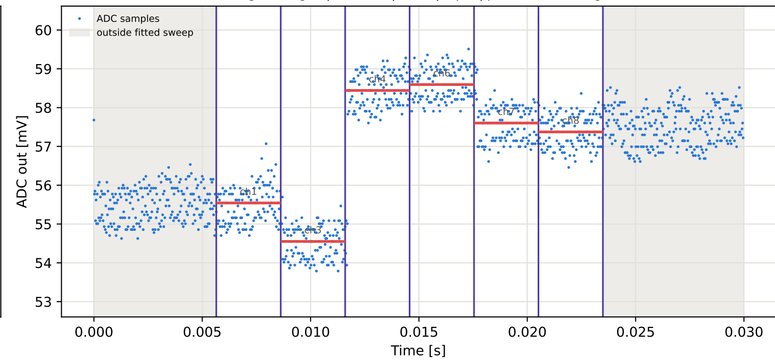
Tag1 &lt;- Tag2 | 825 MHz | run 0 | rep 1 | phase -112.50 deg
