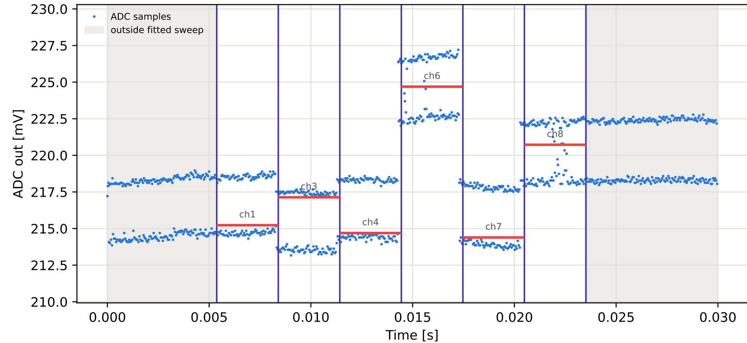
Tag1 &lt;- Tag4 | 865 MHz | run 0 | rep 1 | phase 43.78 deg
