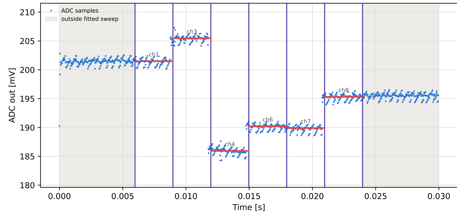
Tag8 &lt;- Tag7 | 775 MHz | run 0 | rep 1 | phase 67.89 deg
