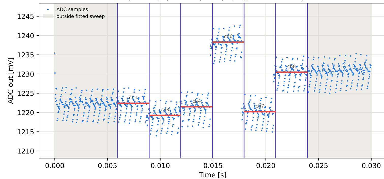
Tag10 &lt;- Tag4 | 895 MHz | run 0 | rep 1 | phase -33.16 deg
