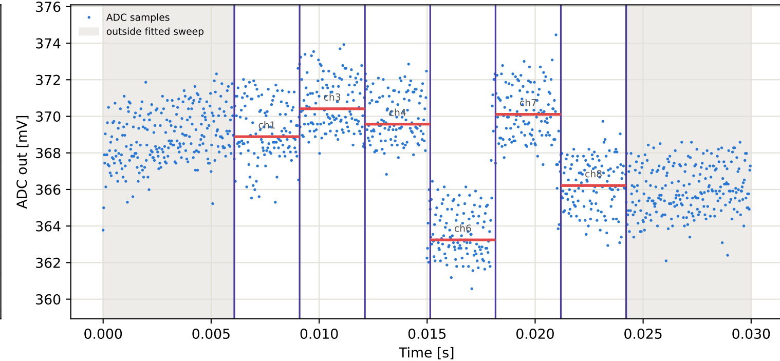
Tag1 &lt;- Tag4 | 885 MHz | run 0 | rep 1 | phase 52.77 deg
