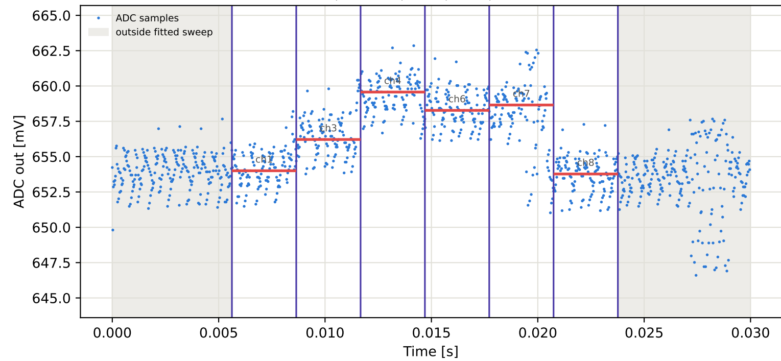
Tag9 &lt;- Tag2 | 845 MHz | run 0 | rep 1 | phase -102.39 deg
