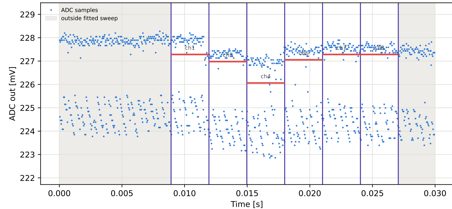
Tag10 &lt;- Tag4 | 795 MHz | run 0 | rep 1 | phase -40.51 deg
