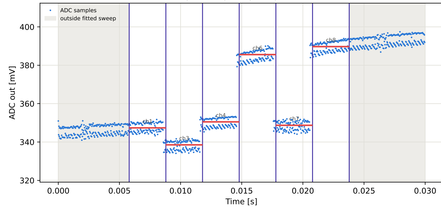
Tag1 &lt;- Tag3 | 875 MHz | run 0 | rep 1 | phase -178.63 deg
