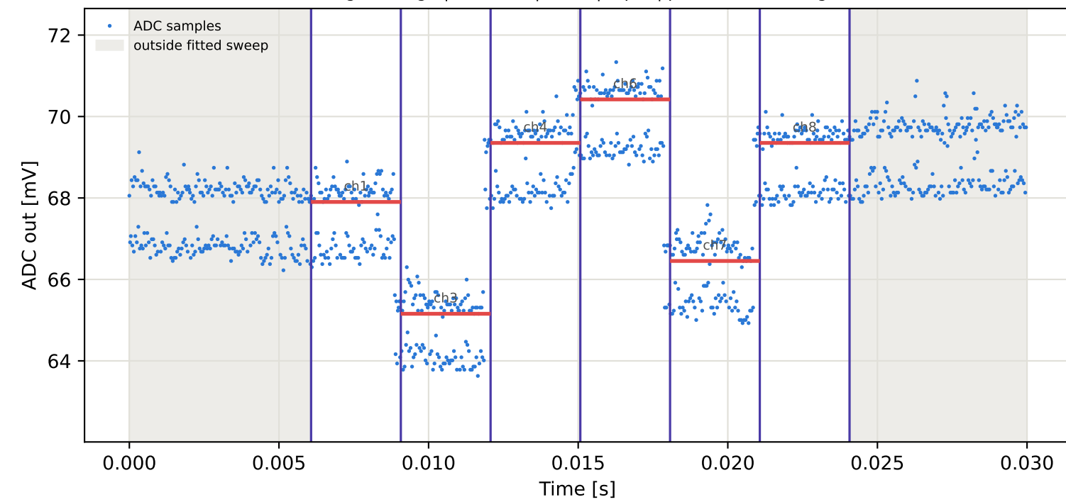
Tag3 &lt;- Tag6 | 775 MHz | run 0 | rep 1 | phase -121.58 deg
