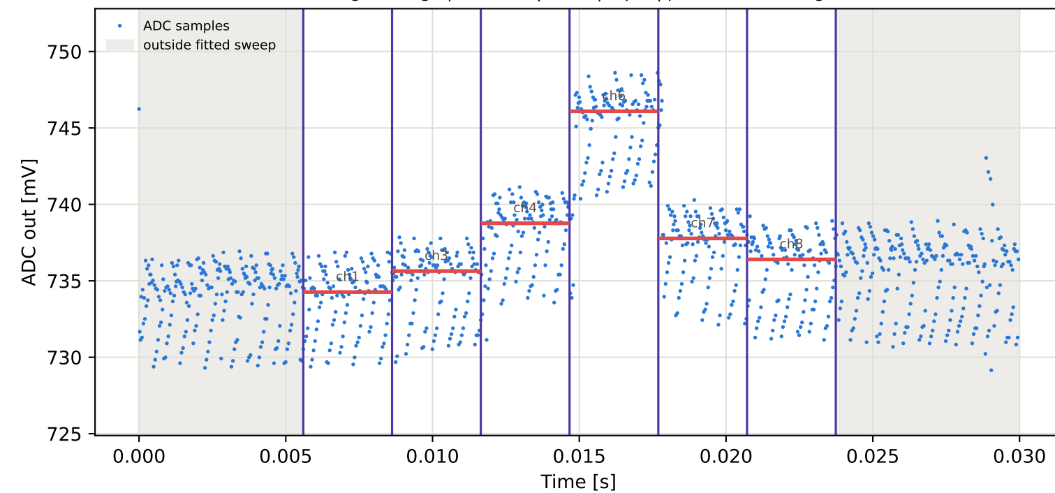
Tag6 &lt;- Tag4 | 925 MHz | run 0 | rep 1 | phase 22.65 deg
