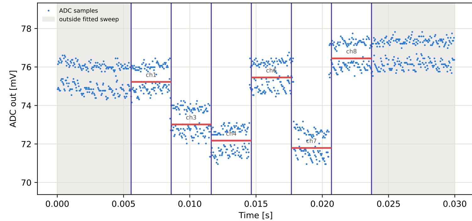
Tag6 &lt;- Tag4 | 795 MHz | run 0 | rep 1 | phase -119.64 deg
