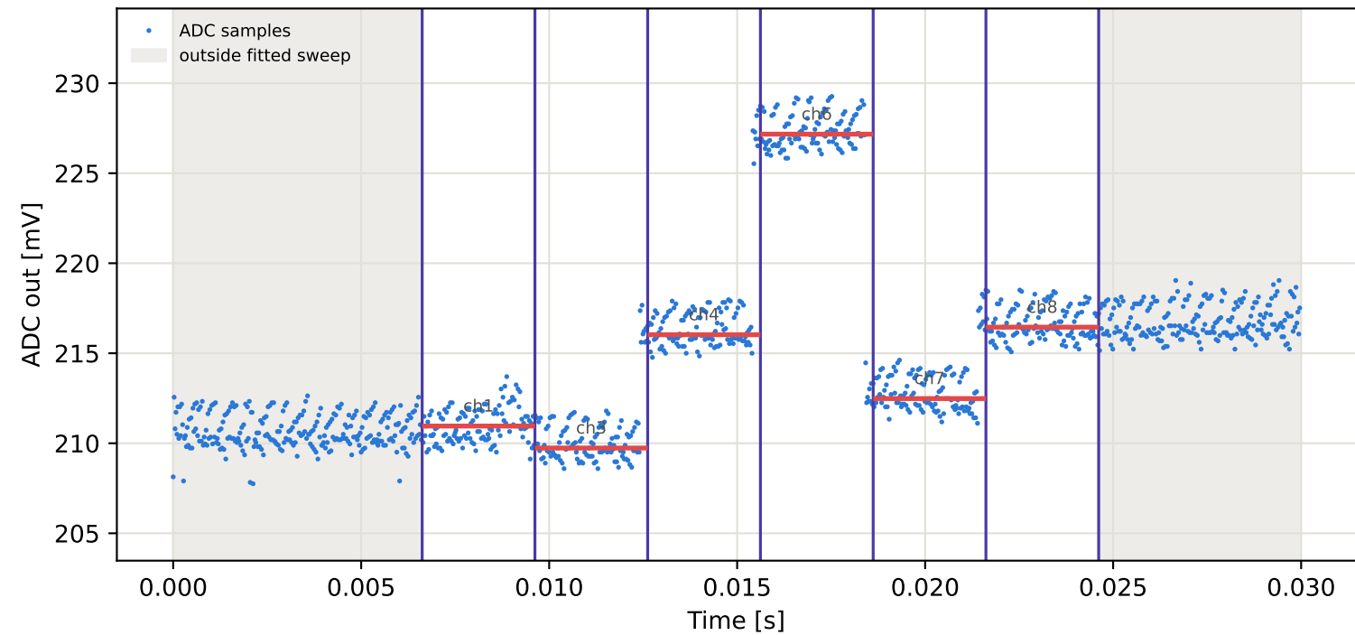
Tag15 &lt;- Tag6 | 955 MHz | run 0 | rep 1 | phase 86.26 deg
