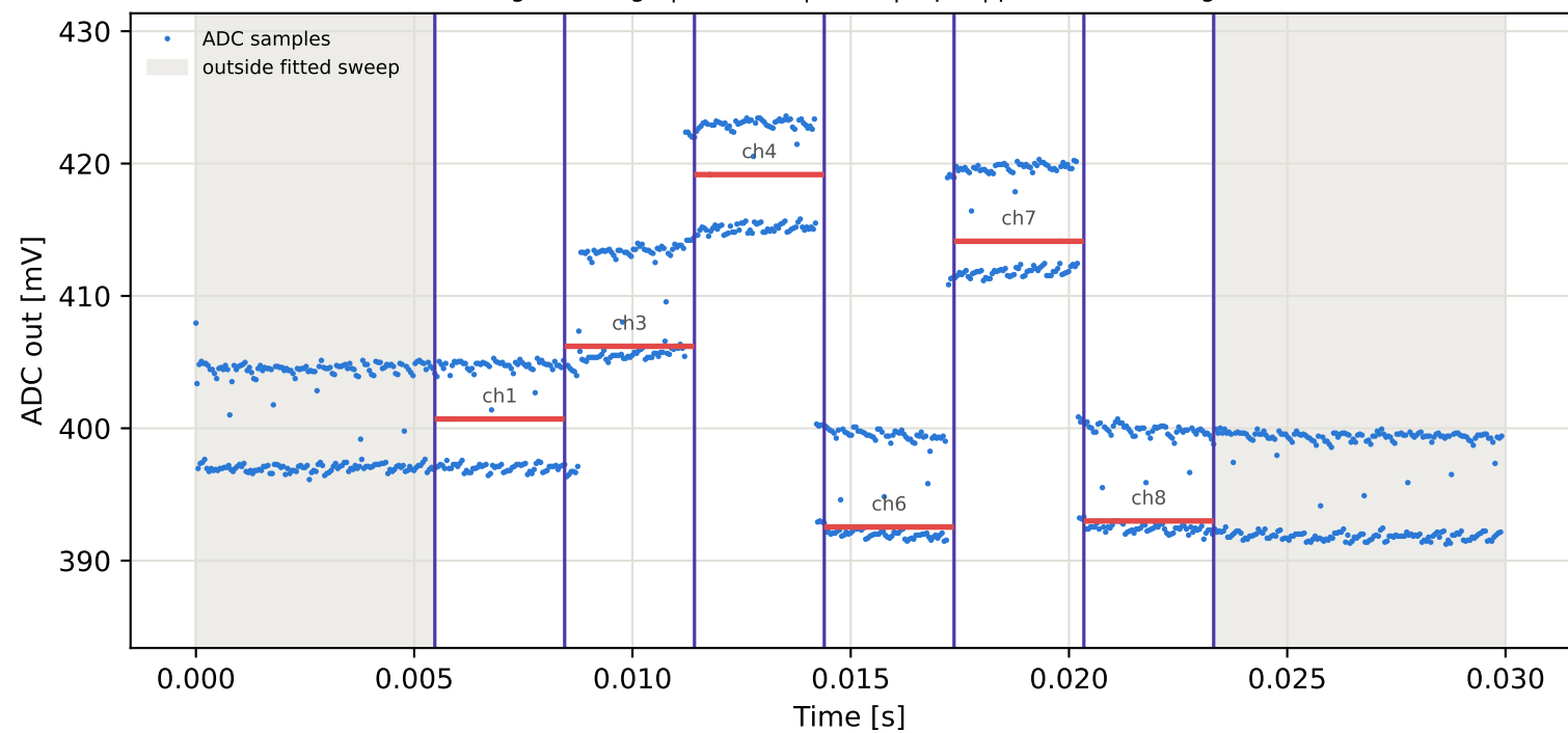
Tag16 &lt;- Tag7 | 975 MHz | run 0 | rep 1 | phase -64.55 deg
