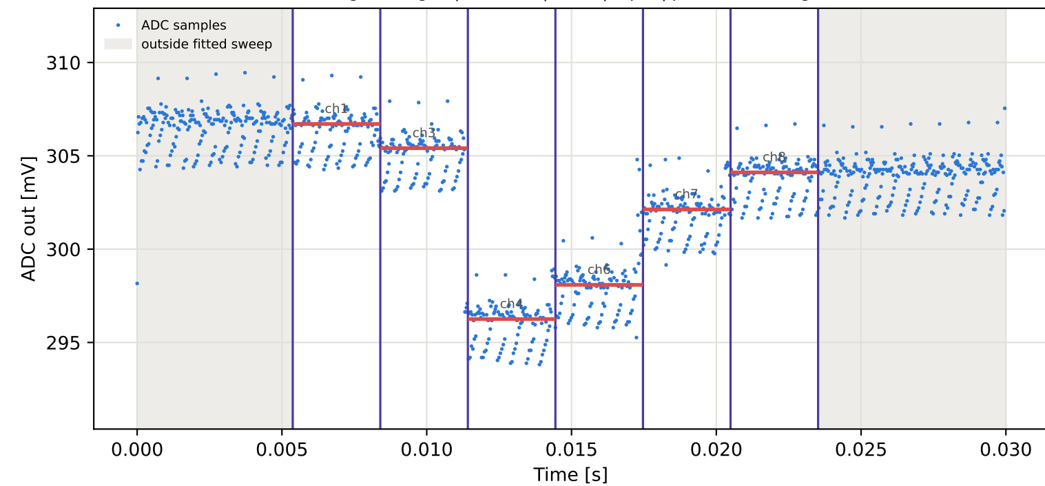
Tag5 &lt;- Tag16 | 975 MHz | run 0 | rep 1 | phase -38.16 deg
