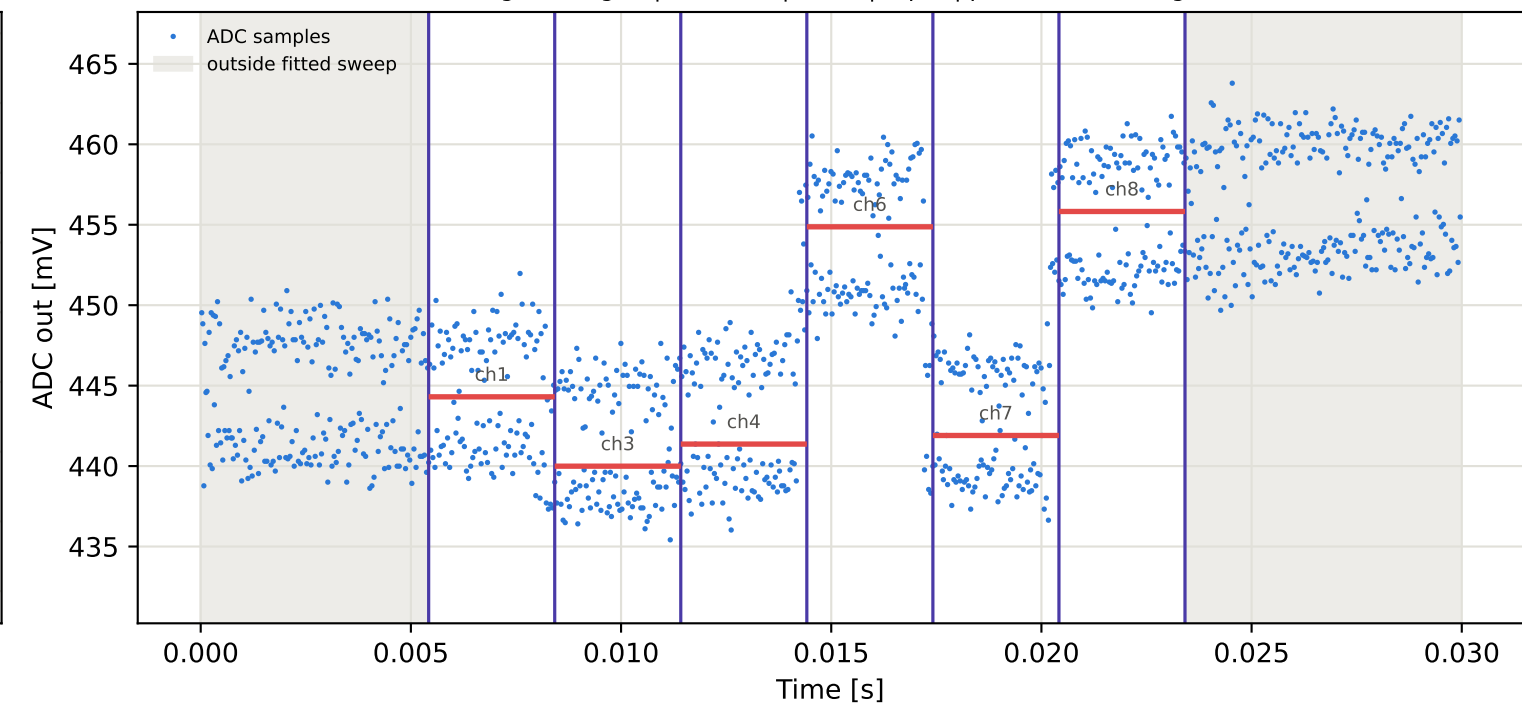
Tag4 &lt;- Tag16 | 885 MHz | run 0 | rep 1 | phase -93.76 deg
