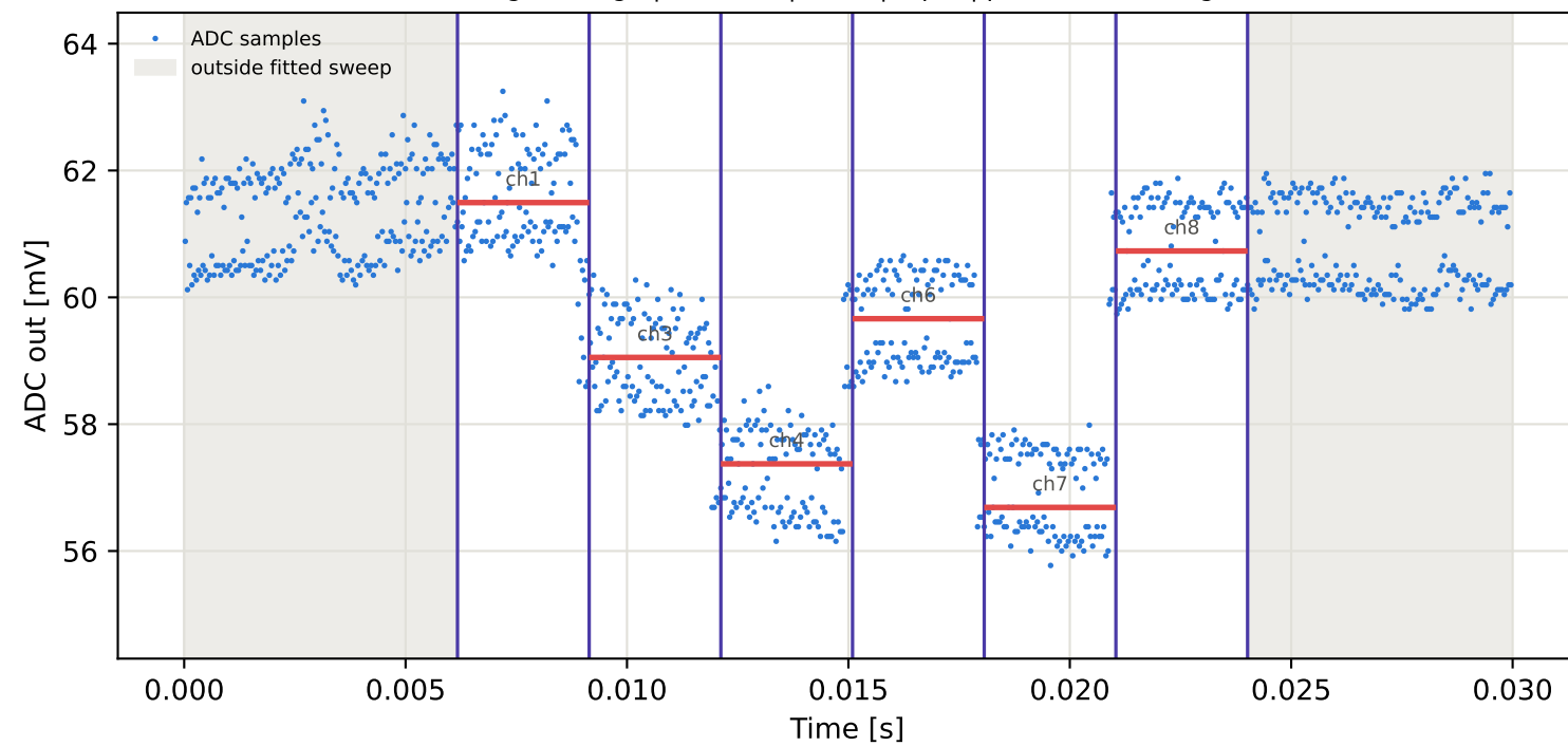
Tag1 &lt;- Tag7 | 825 MHz | run 0 | rep 1 | phase -63.86 deg
