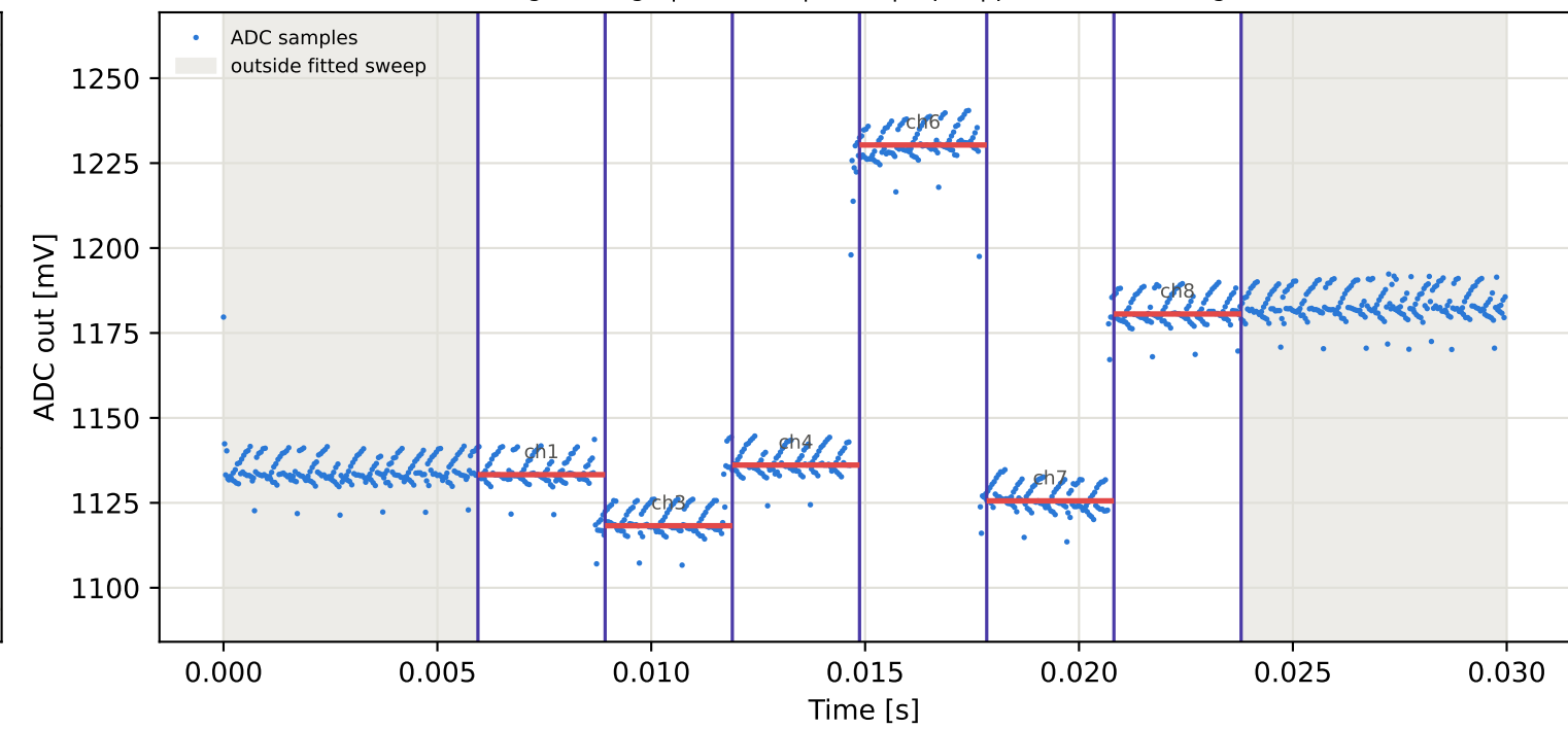
Tag8 &lt;- Tag10 | 935 MHz | run 0 | rep 1 | phase -34.52 deg
