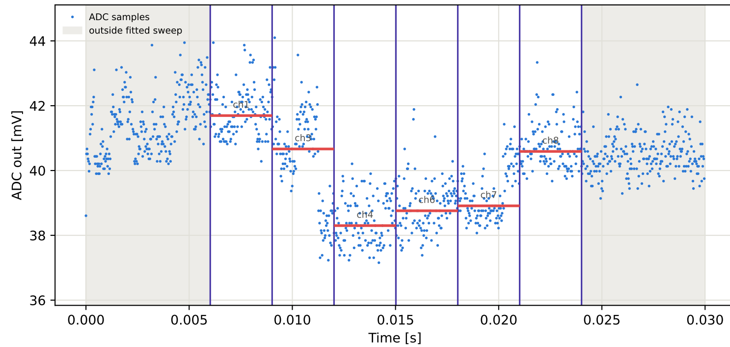
Tag3 &lt;- Tag10 | 985 MHz | run 0 | rep 1 | phase 133.82 deg
