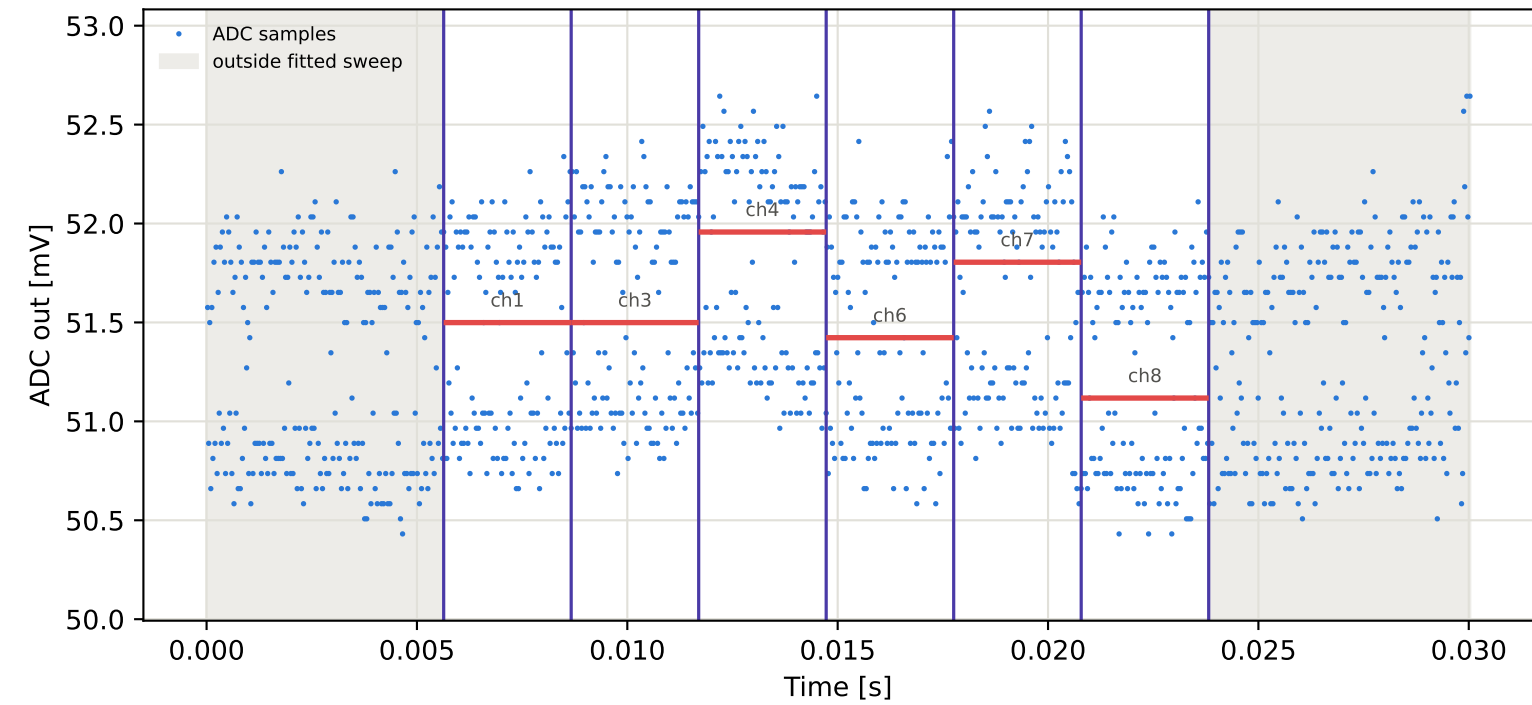
Tag5 &lt;- Tag4 | 785 MHz | run 0 | rep 1 | phase 22.01 deg
