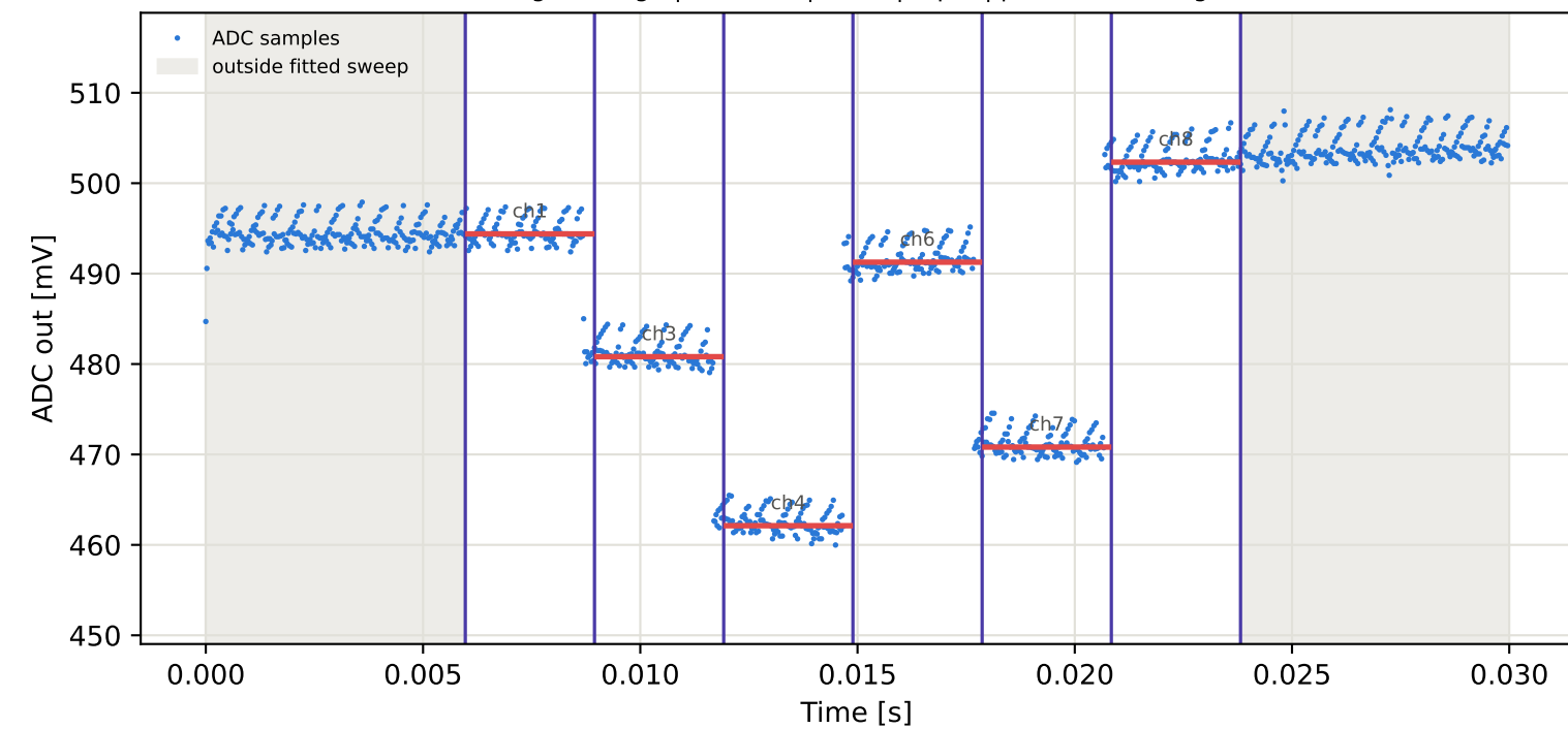
Tag4 &lt;- Tag9 | 935 MHz | run 0 | rep 1 | phase -107.13 deg
