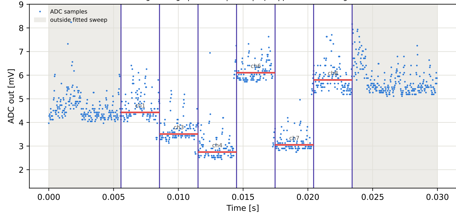
Tag2 &lt;- Tag6 | 965 MHz | run 0 | rep 1 | phase -125.02 deg
