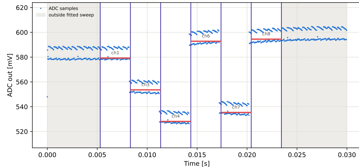
Tag9 &lt;- Tag7 | 995 MHz | run 0 | rep 1 | phase 115.29 deg
