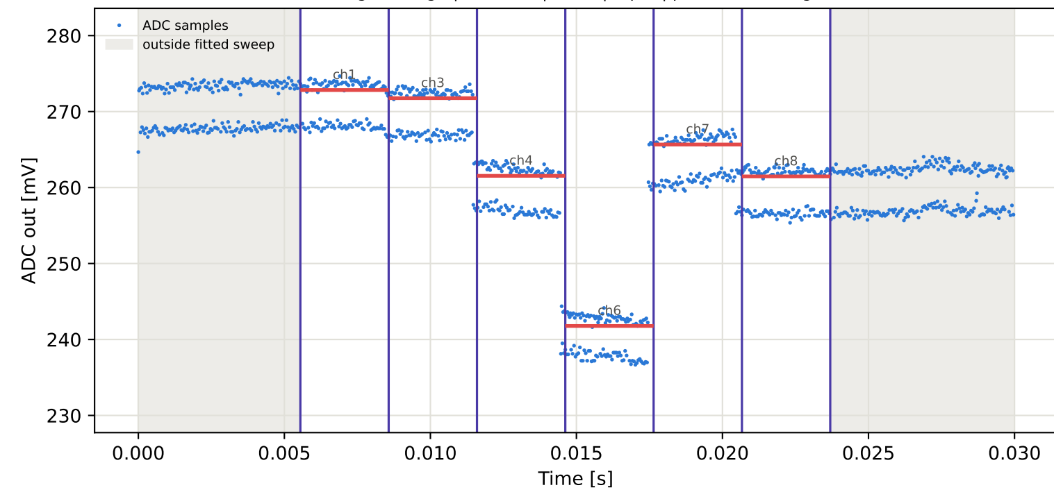
Tag2 &lt;- Tag5 | 915 MHz | run 0 | rep 1 | phase -154.20 deg
