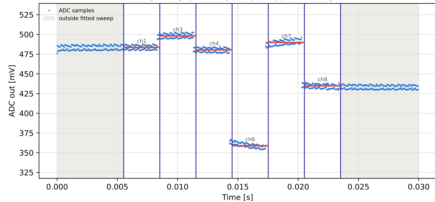
Tag4 &lt;- Tag7 | 935 MHz | run 0 | rep 1 | phase 98.89 deg
