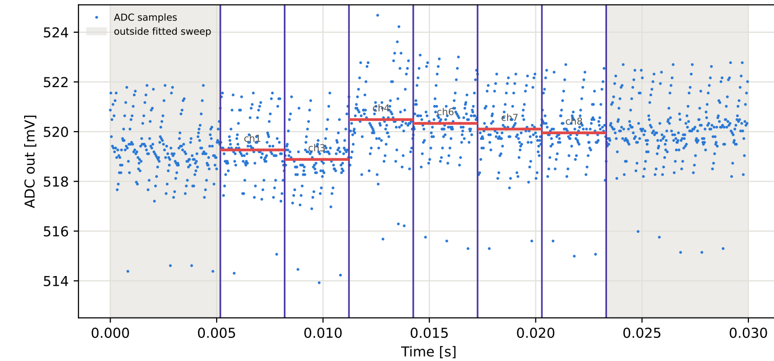
Tag8 &lt;- Tag15 | 835 MHz | run 0 | rep 1 | phase -147.98 deg
