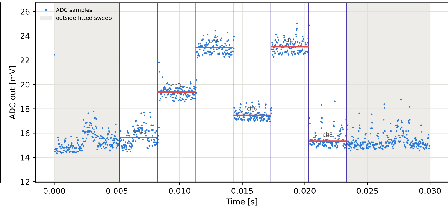
Tag2 &lt;- Tag8 | 805 MHz | run 0 | rep 1 | phase 122.10 deg
