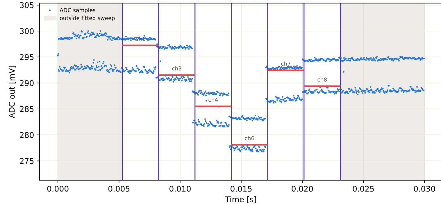
Tag15 &lt;- Tag1 | 945 MHz | run 0 | rep 1 | phase 31.68 deg
