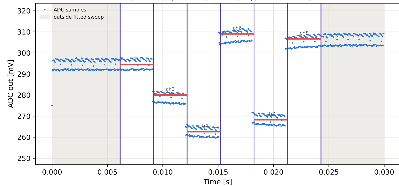
Tag16 &lt;- Tag15 | 995 MHz | run 0 | rep 1 | phase -109.71 deg
