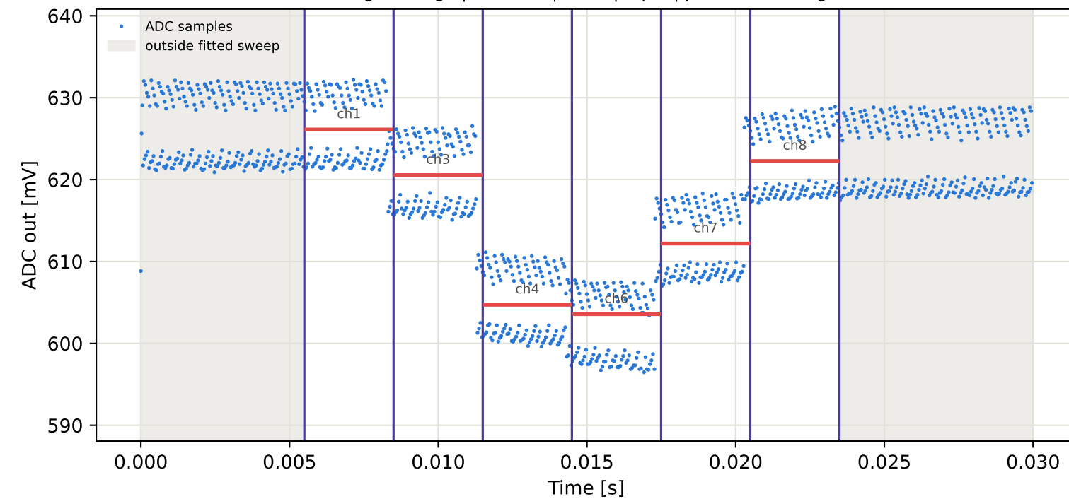
Tag3 &lt;- Tag8 | 935 MHz | run 0 | rep 1 | phase 51.17 deg
