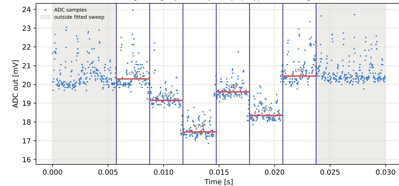
Tag2 &lt;- Tag15 | 975 MHz | run 0 | rep 1 | phase 88.15 deg
