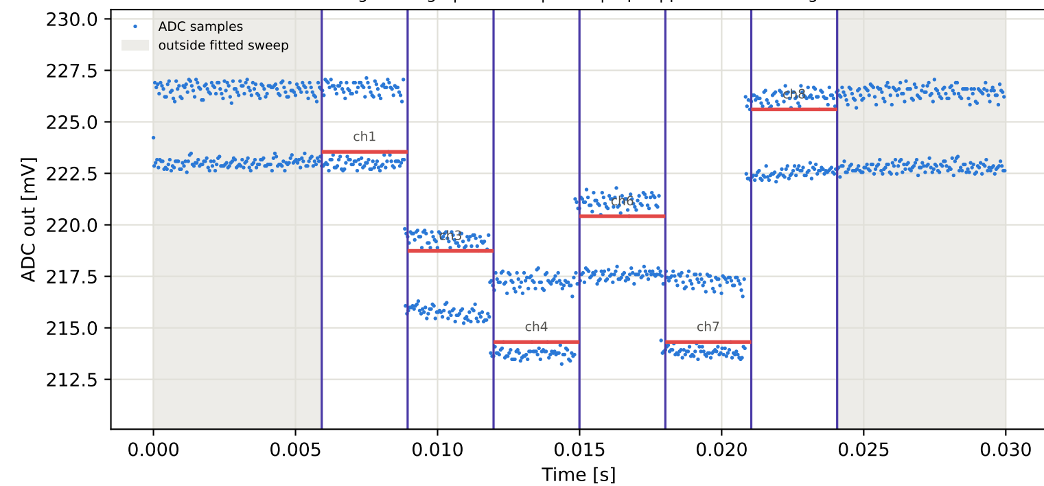
Tag1 &lt;- Tag7 | 865 MHz | run 0 | rep 1 | phase 137.00 deg
