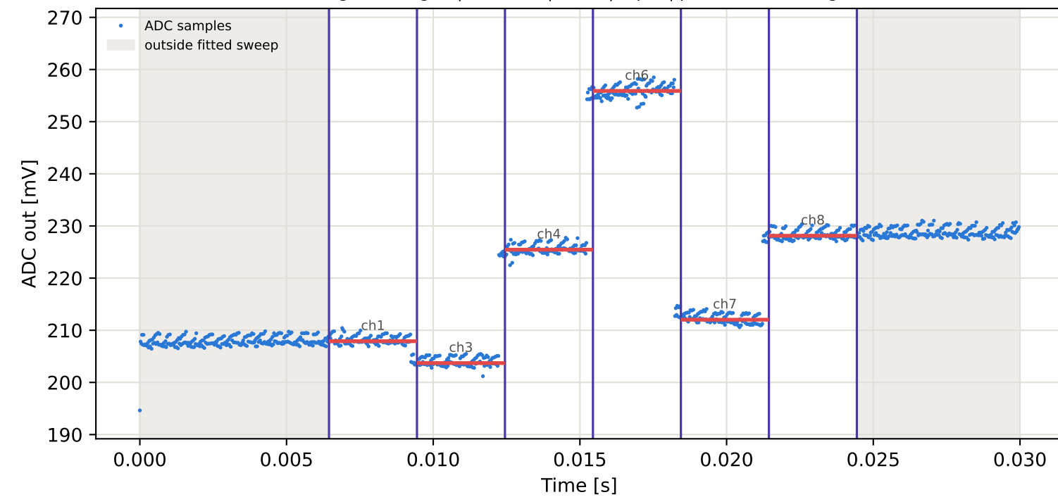
Tag15 &lt;- Tag3 | 955 MHz | run 0 | rep 1 | phase -139.68 deg
