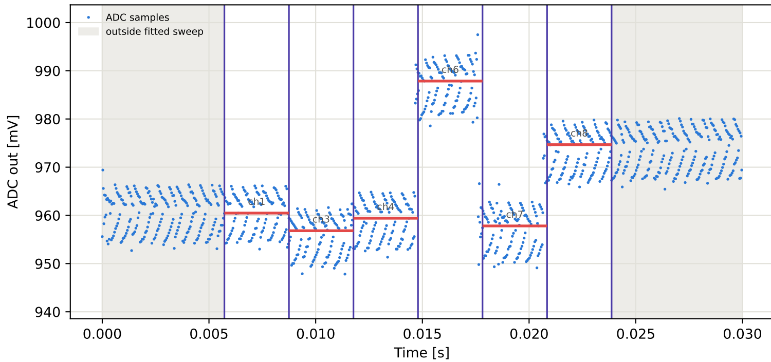
Tag16 &lt;- Tag15 | 935 MHz | run 0 | rep 1 | phase 102.11 deg
