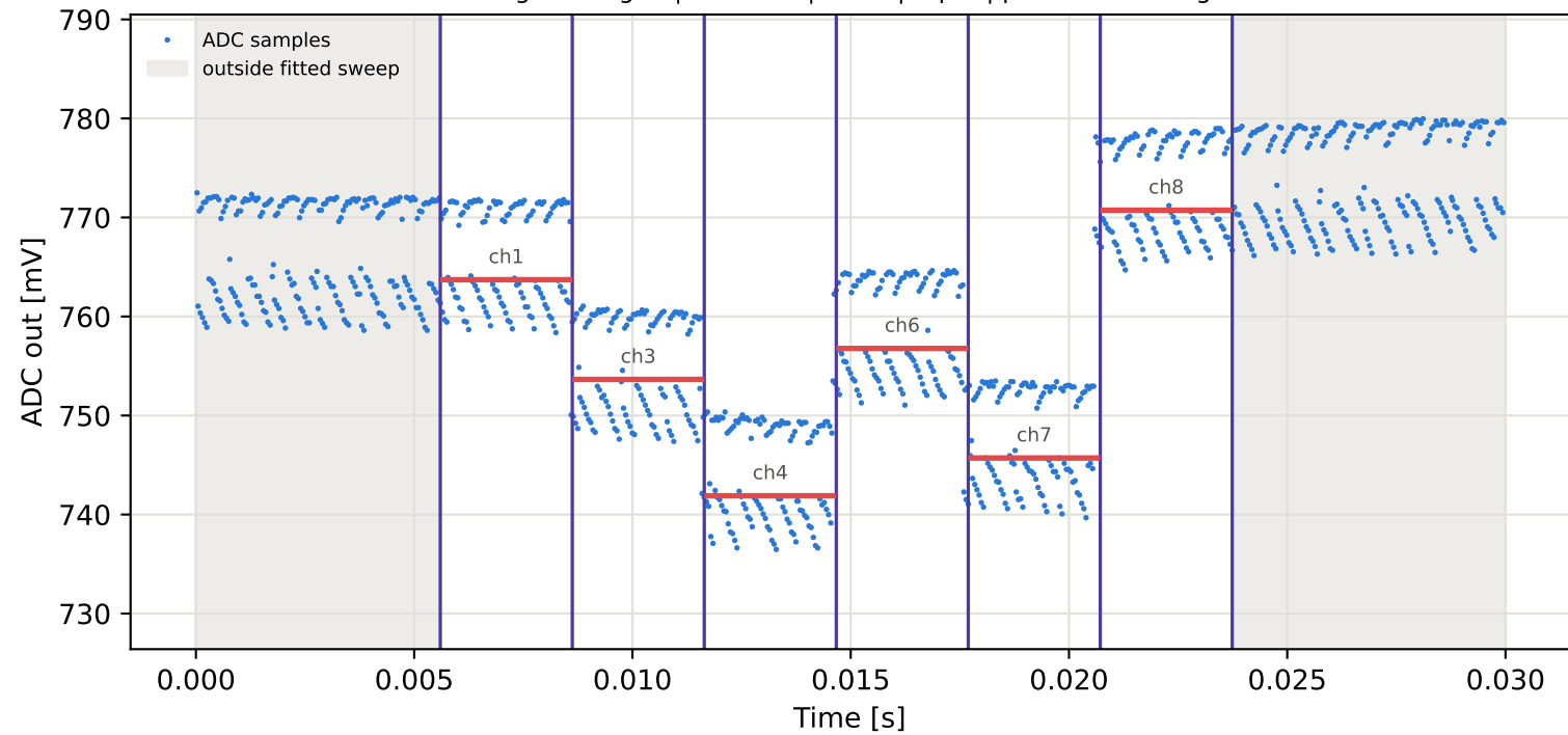
Tag6 &lt;- Tag3 | 915 MHz | run 0 | rep 1 | phase 162.78 deg
