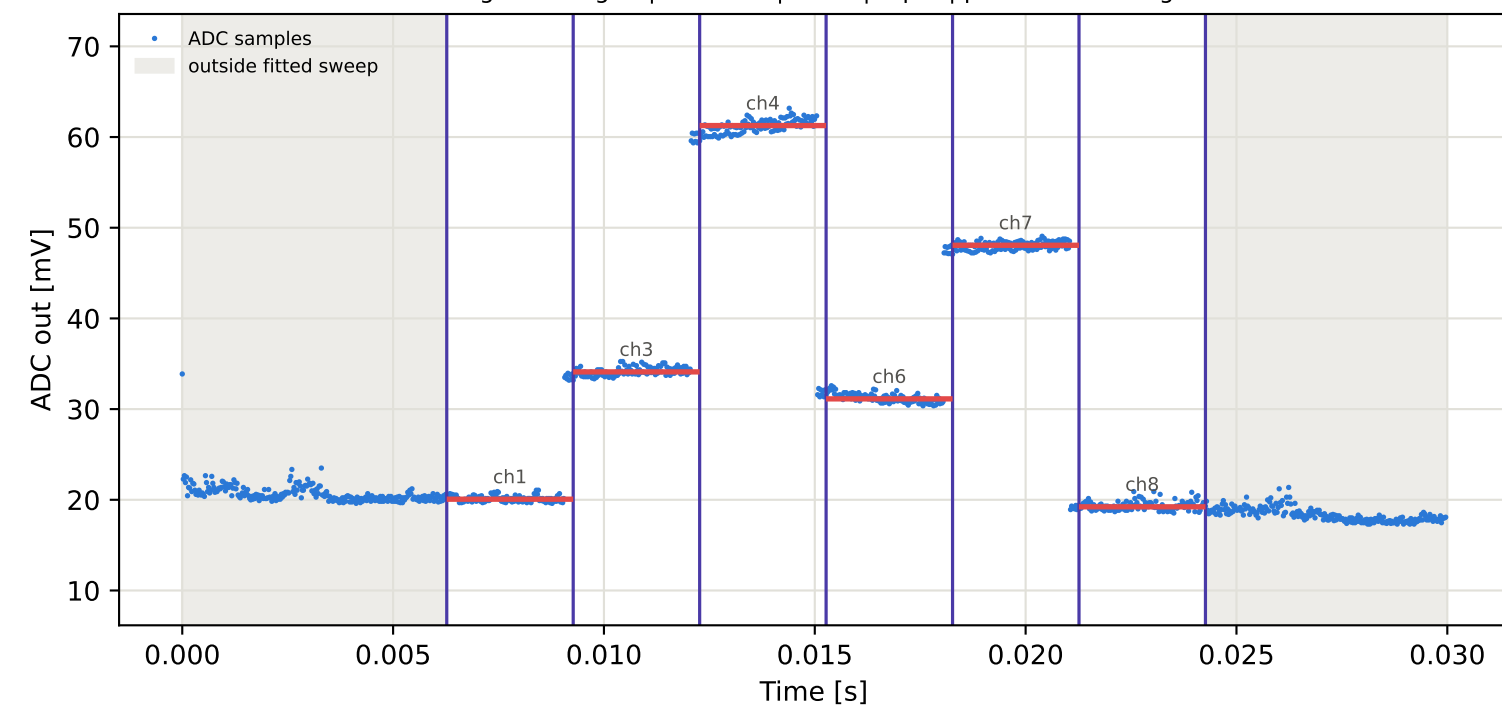
Tag15 &lt;- Tag3 | 965 MHz | run 0 | rep 1 | phase -72.75 deg
