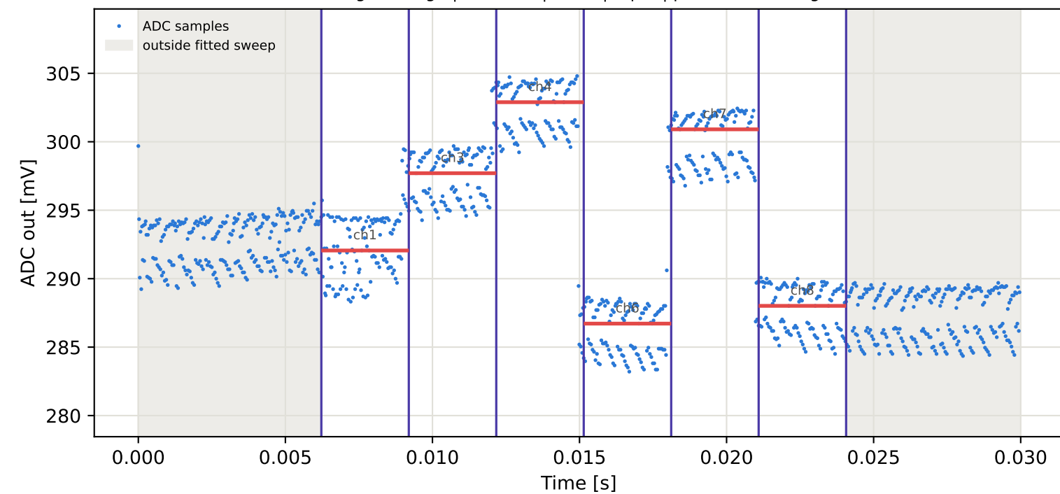
Tag4 &lt;- Tag3 | 965 MHz | run 0 | rep 1 | phase -52.81 deg
