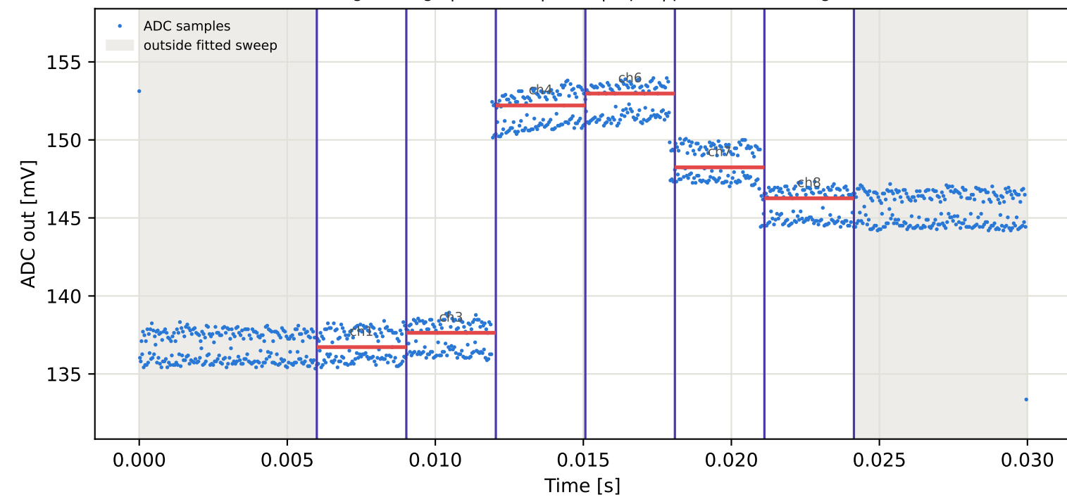
Tag3 &lt;- Tag9 | 795 MHz | run 0 | rep 1 | phase 144.60 deg
