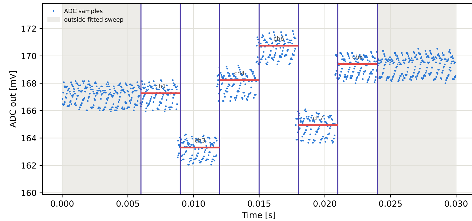
Tag8 &lt;- Tag15 | 785 MHz | run 0 | rep 1 | phase -156.17 deg
