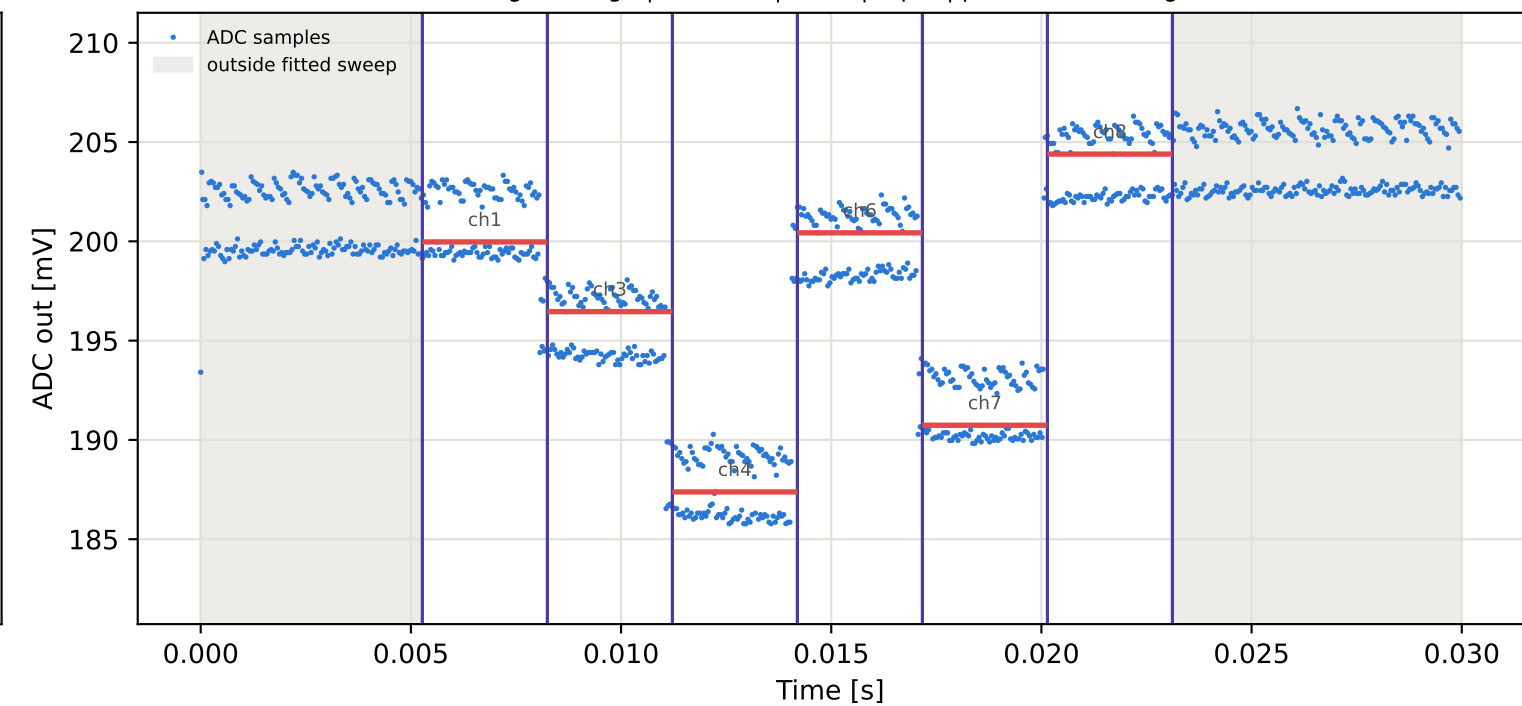
Tag5 &lt;- Tag1 | 945 MHz | run 0 | rep 1 | phase 102.03 deg
