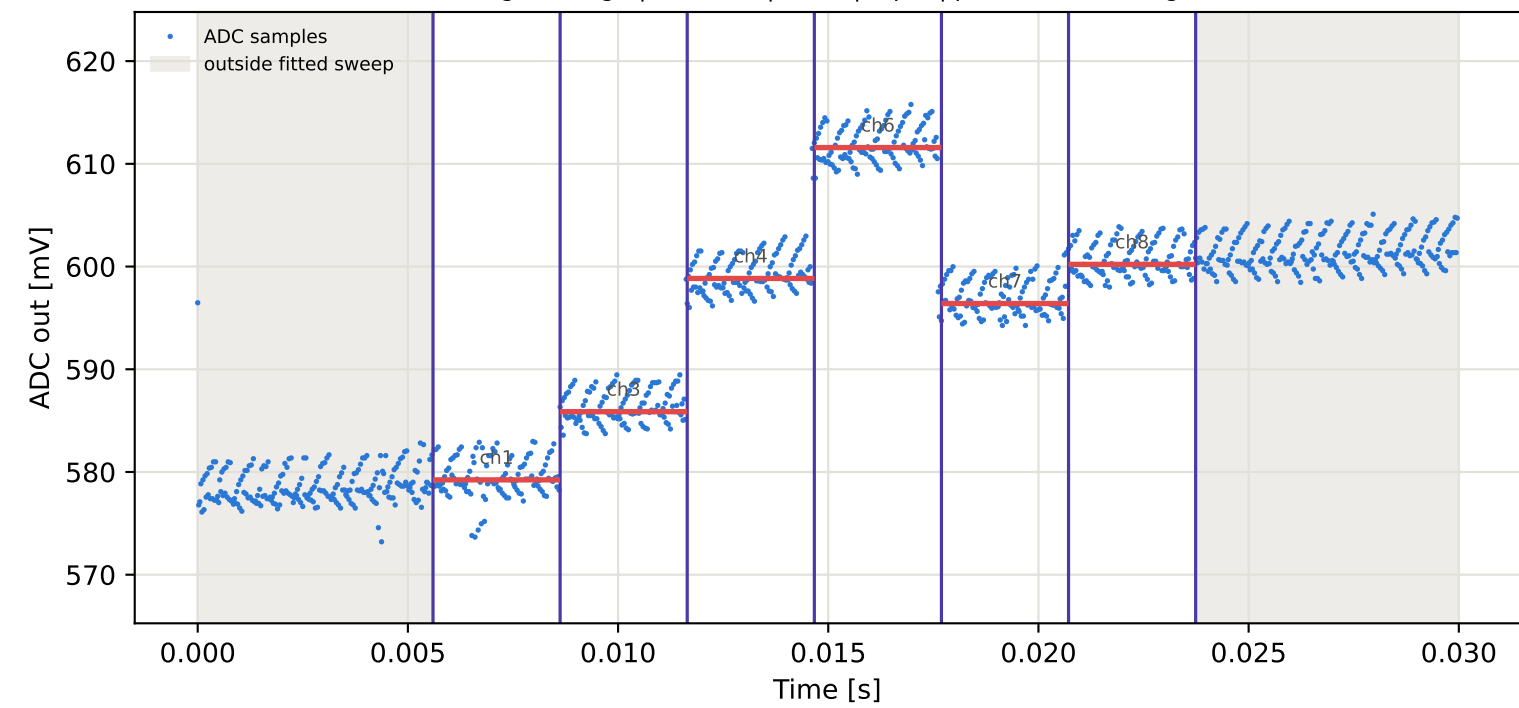
Tag8 &lt;- Tag5 | 875 MHz | run 0 | rep 1 | phase 87.74 deg
