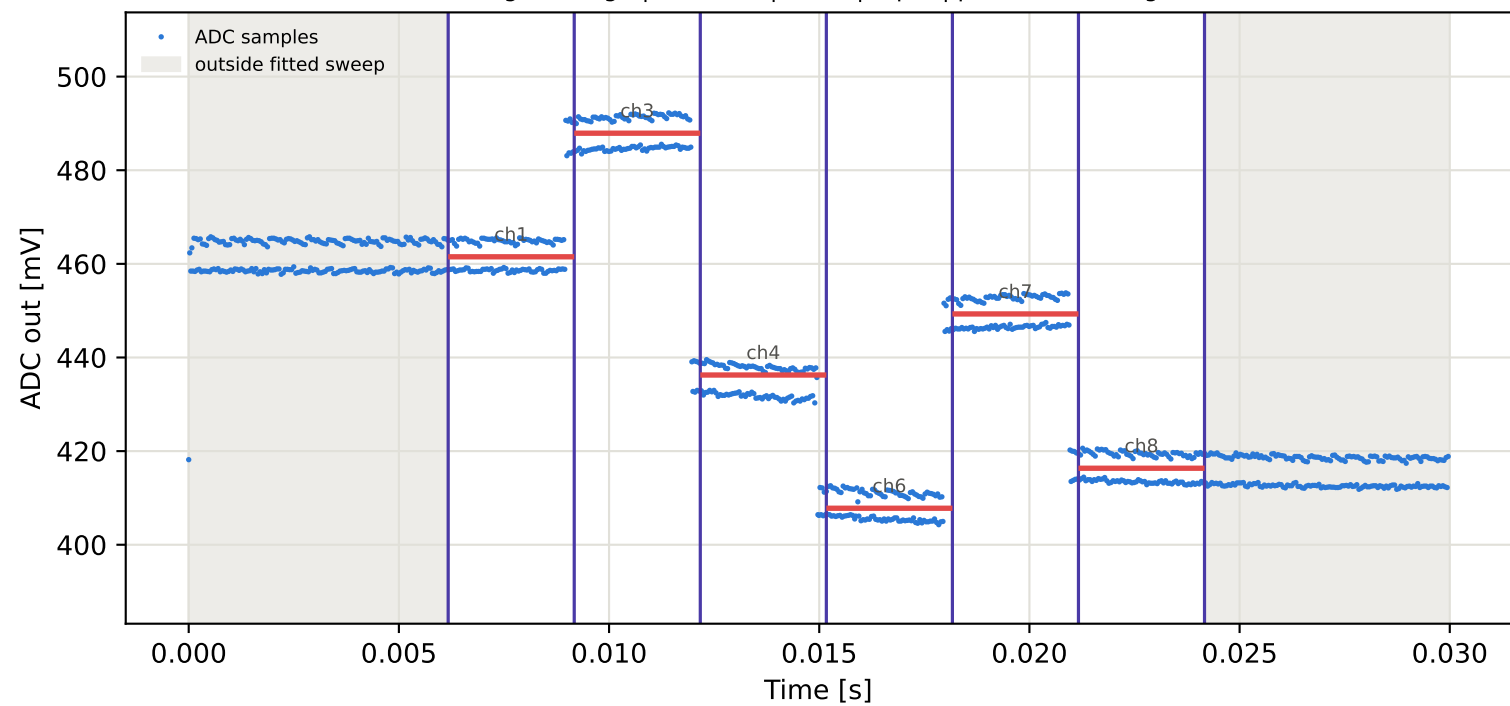
Tag6 &lt;- Tag5 | 835 MHz | run 0 | rep 1 | phase 58.85 deg
