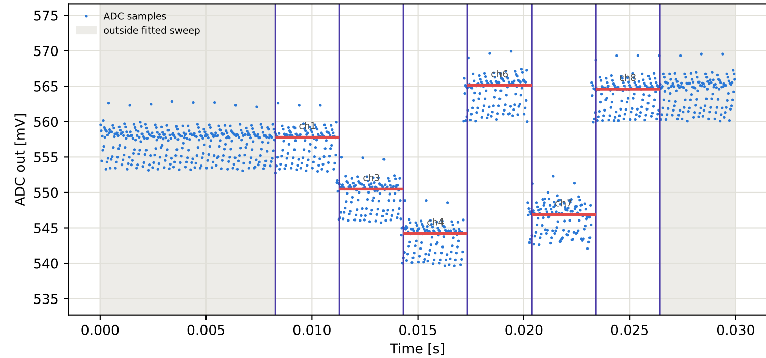
Tag3 &lt;- Tag2 | 955 MHz | run 0 | rep 1 | phase -35.57 deg
