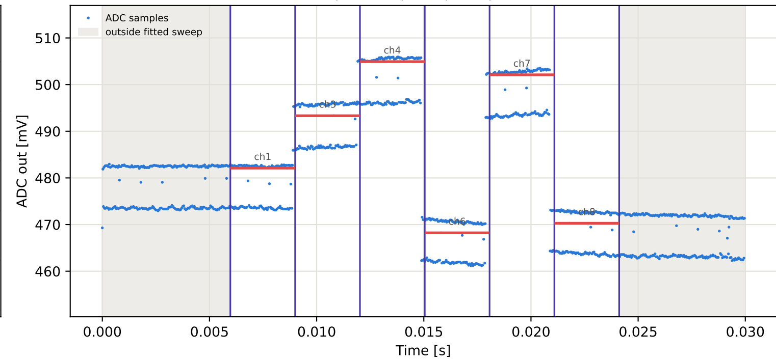
Tag8 &lt;- Tag16 | 985 MHz | run 0 | rep 1 | phase -51.99 deg
