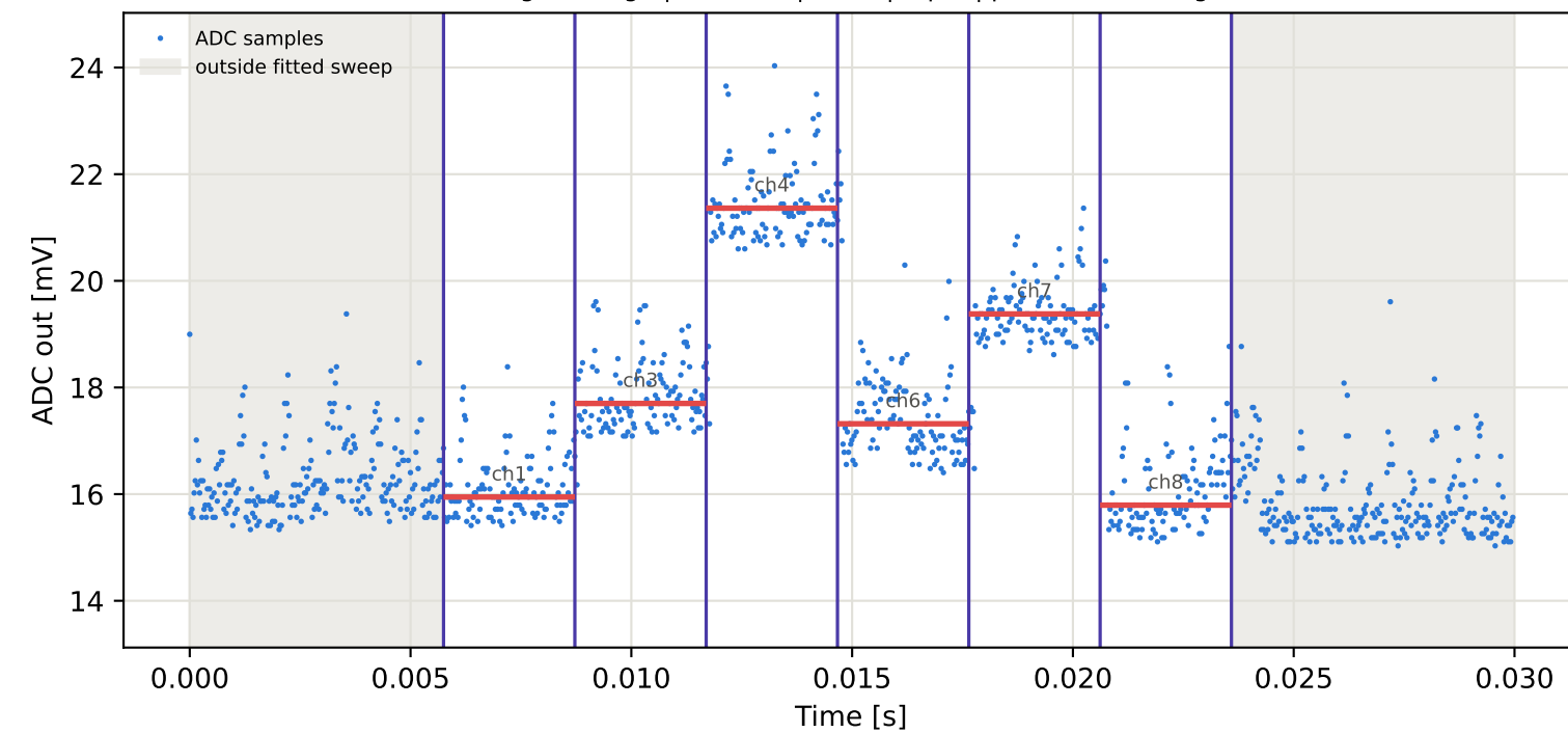
Tag2 &lt;- Tag7 | 975 MHz | run 0 | rep 1 | phase 64.91 deg
