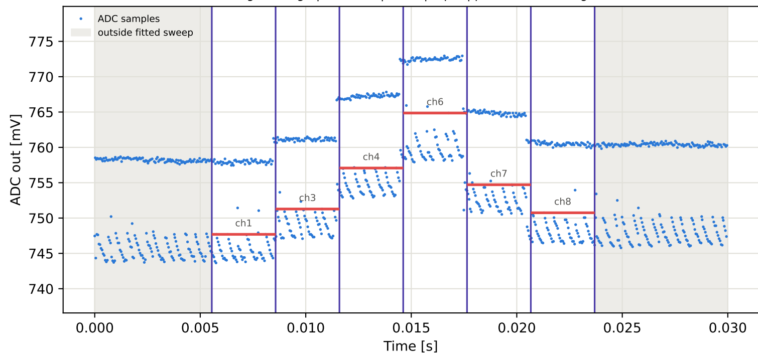
Tag6 &lt;- Tag5 | 915 MHz | run 0 | rep 1 | phase -140.34 deg
