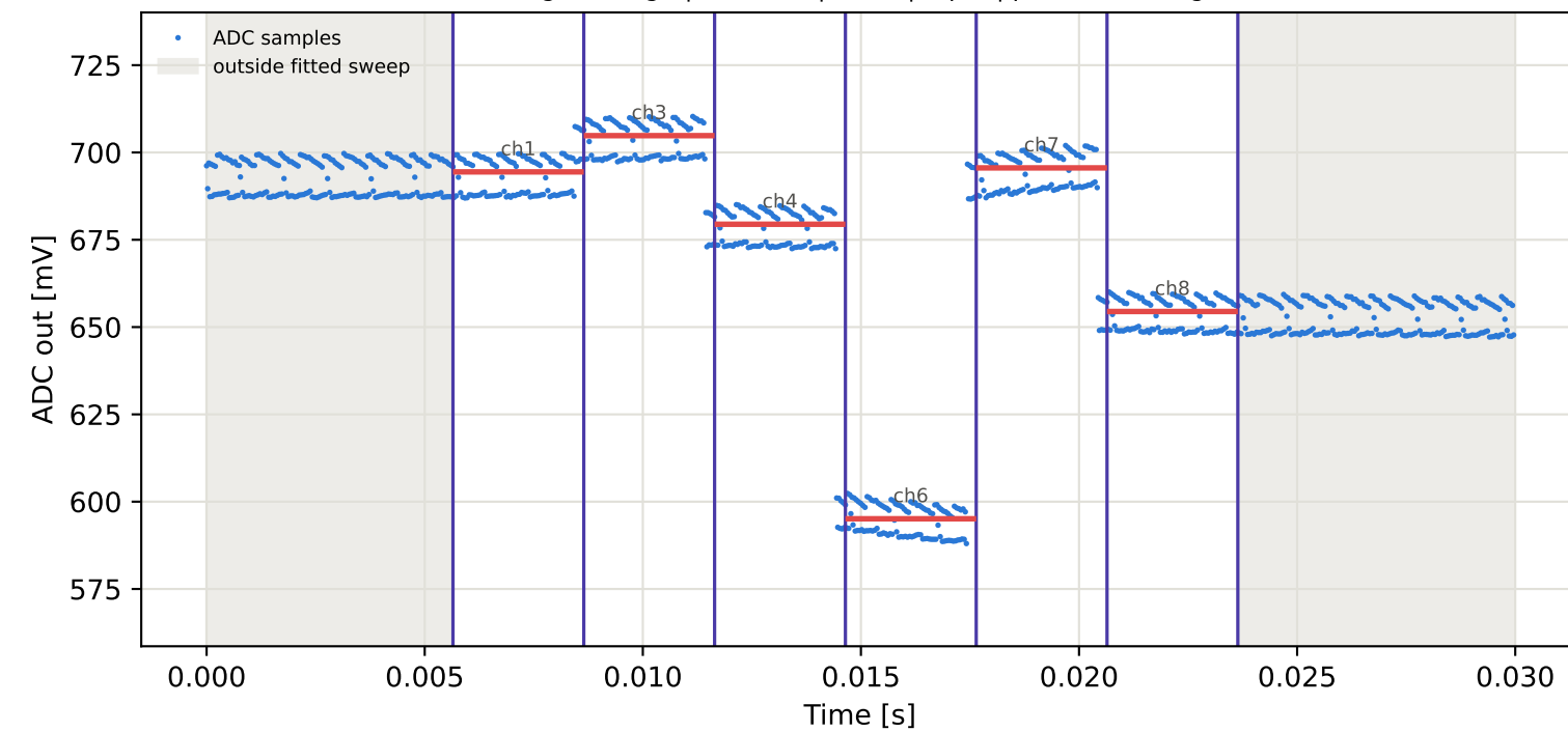
Tag9 &lt;- Tag5 | 955 MHz | run 0 | rep 1 | phase 20.82 deg
