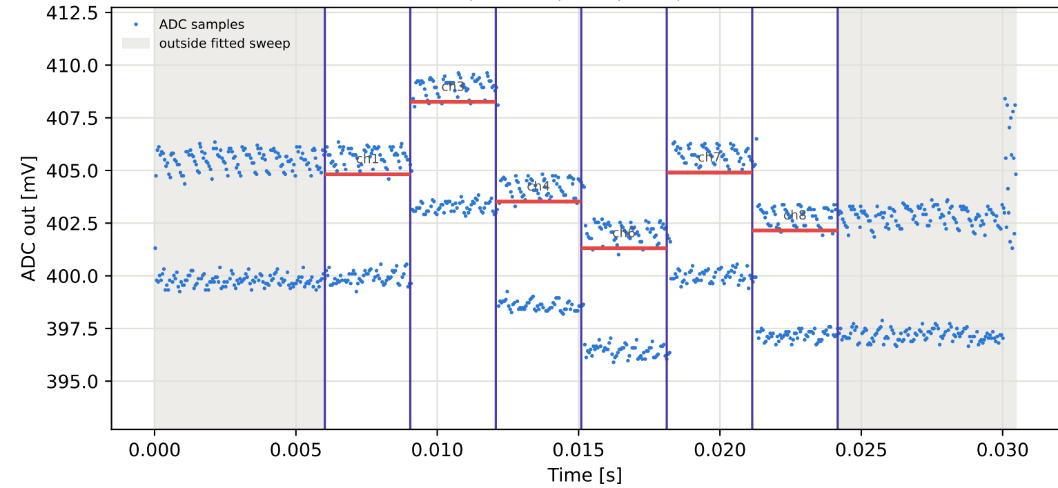
Tag10 &lt;- Tag4 | 825 MHz | run 0 | rep 1 | phase 26.80 deg
