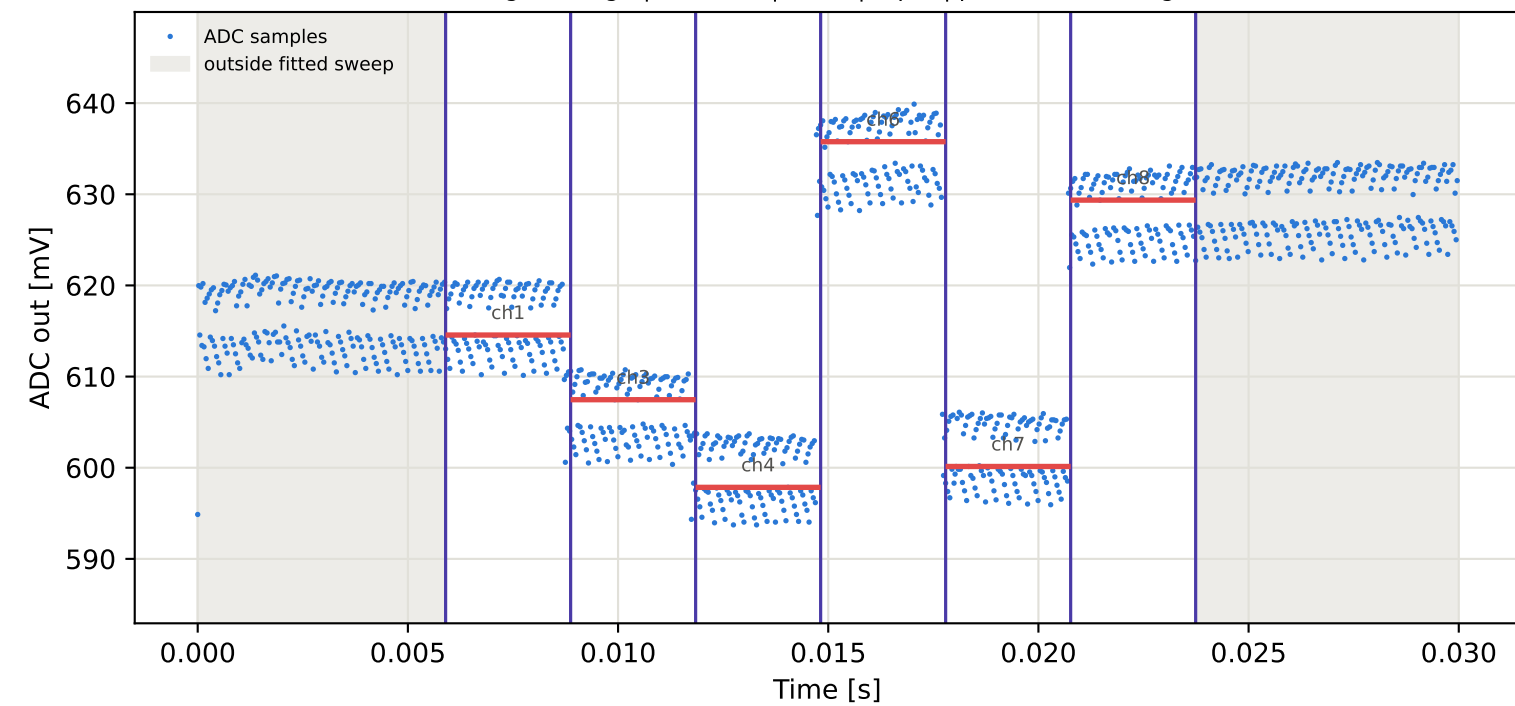
Tag3 &lt;- Tag7 | 945 MHz | run 0 | rep 1 | phase -9.10 deg
