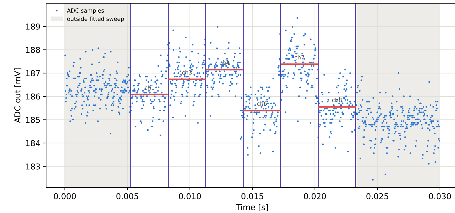
Tag2 &lt;- Tag15 | 905 MHz | run 0 | rep 1 | phase -38.38 deg
