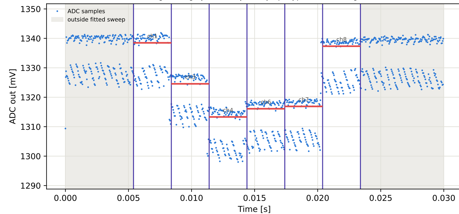
Tag7 &lt;- Tag5 | 885 MHz | run 0 | rep 1 | phase -134.97 deg
