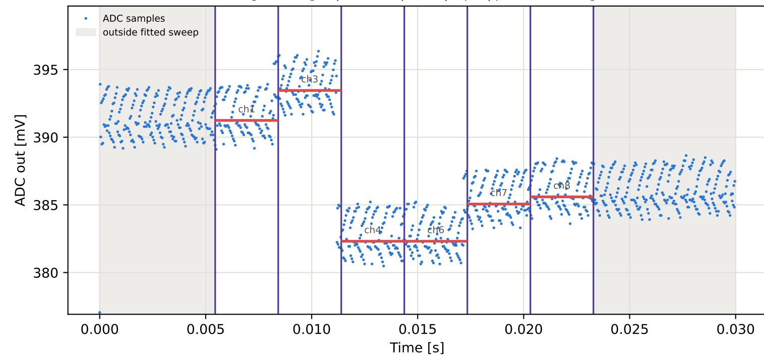
Tag10 &lt;- Tag3 | 825 MHz | run 0 | rep 1 | phase -24.51 deg
