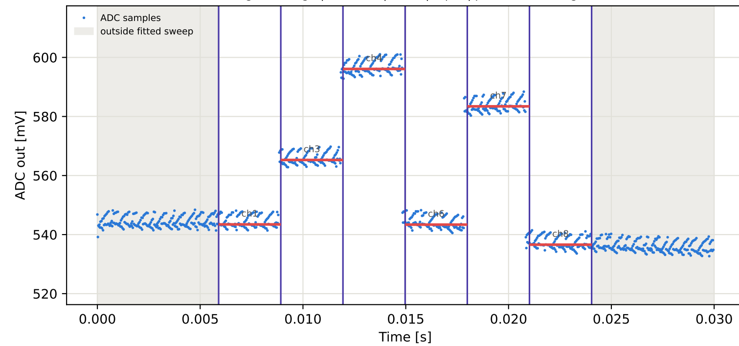
Tag15 &lt;- Tag9 | 985 MHz | run 0 | rep 1 | phase 50.12 deg
