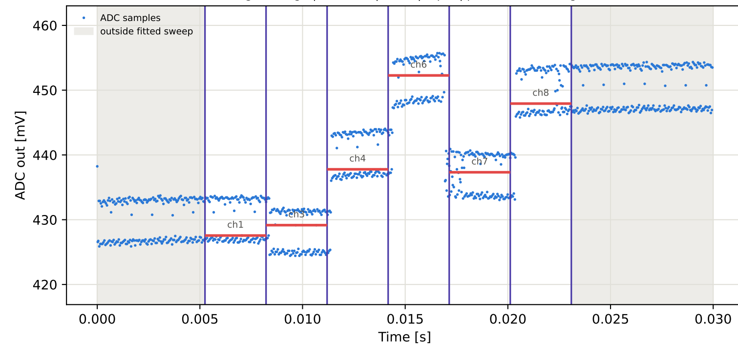
Tag3 &lt;- Tag6 | 855 MHz | run 0 | rep 1 | phase -131.74 deg
