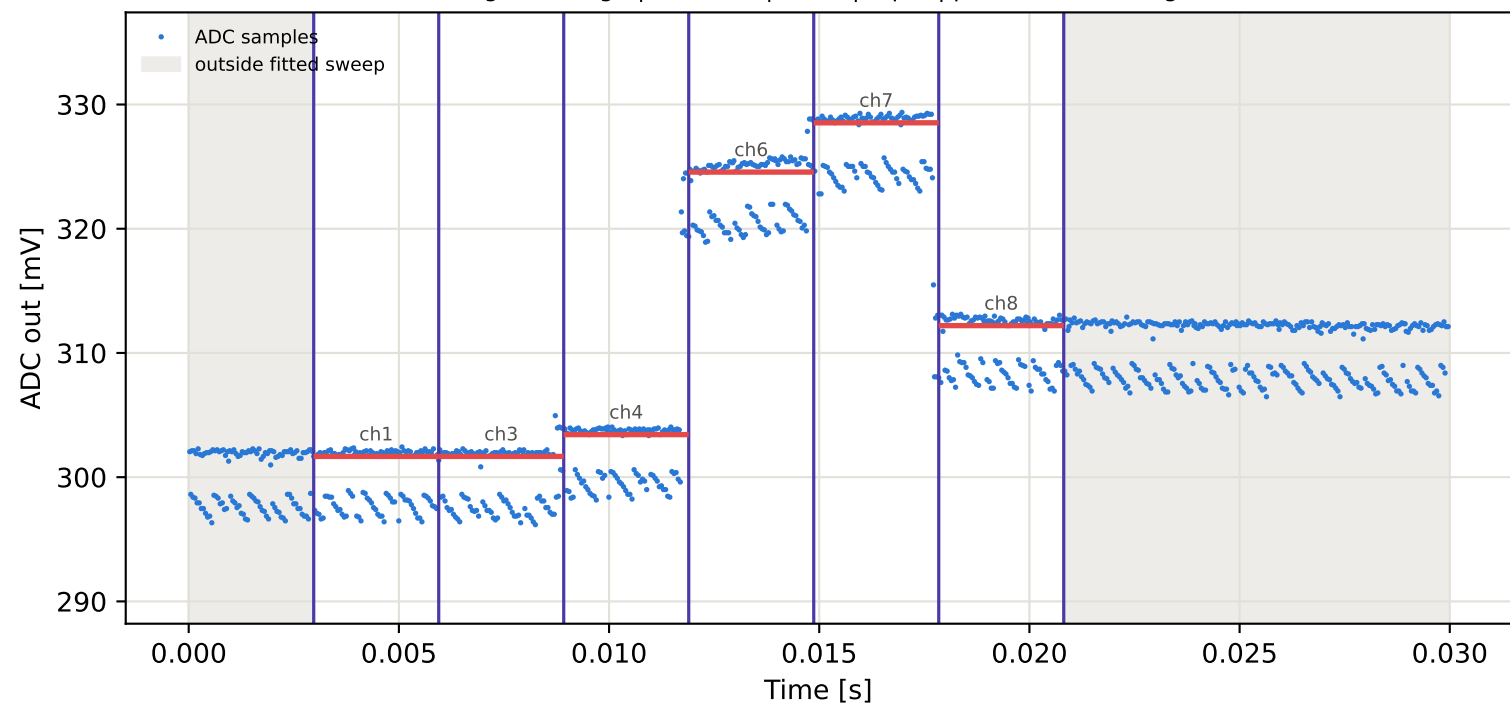
Tag15 &lt;- Tag10 | 975 MHz | run 0 | rep 1 | phase -11.48 deg
