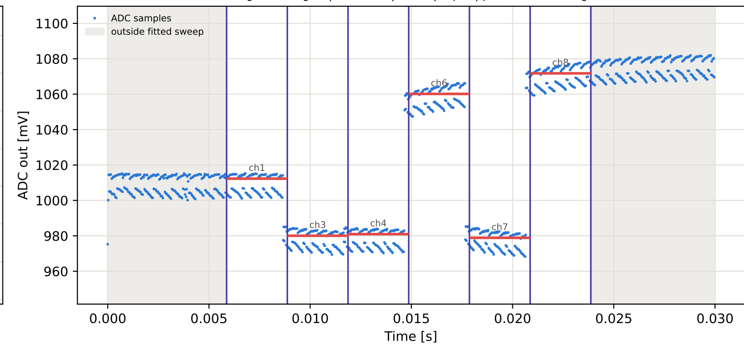
Tag16 &lt;- Tag15 | 905 MHz | run 0 | rep 1 | phase 157.34 deg
