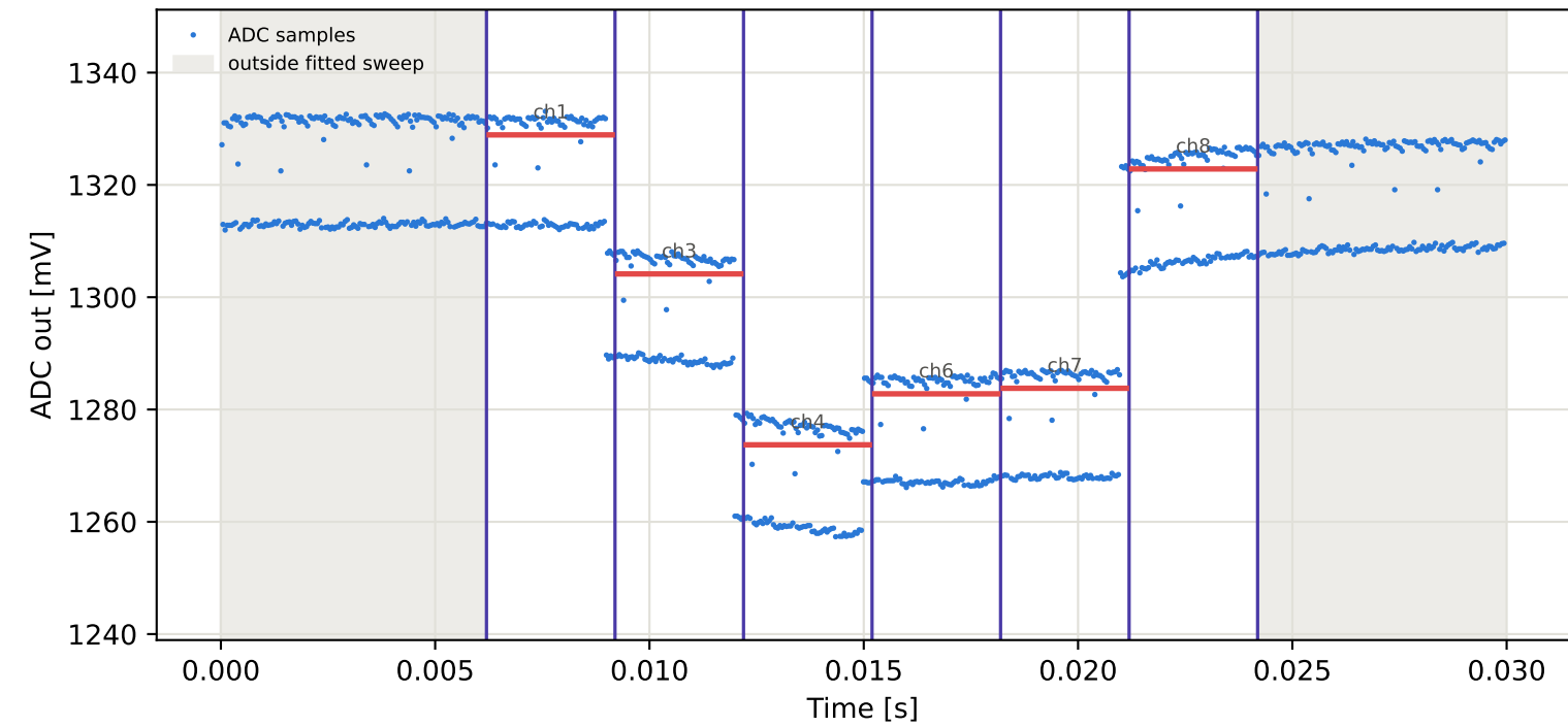
Tag15 &lt;- Tag10 | 905 MHz | run 0 | rep 1 | phase 85.40 deg
