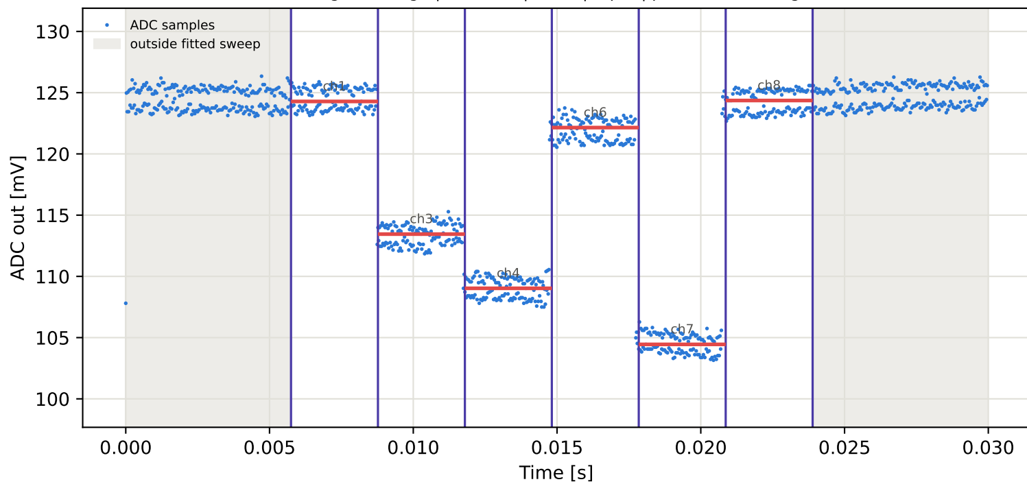
Tag2 &lt;- Tag1 | 795 MHz | run 0 | rep 1 | phase -40.28 deg
