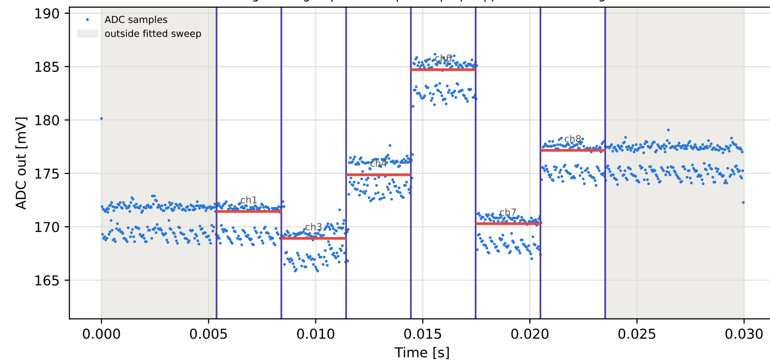
Tag5 &lt;- Tag16 | 985 MHz | run 0 | rep 1 | phase 59.44 deg
