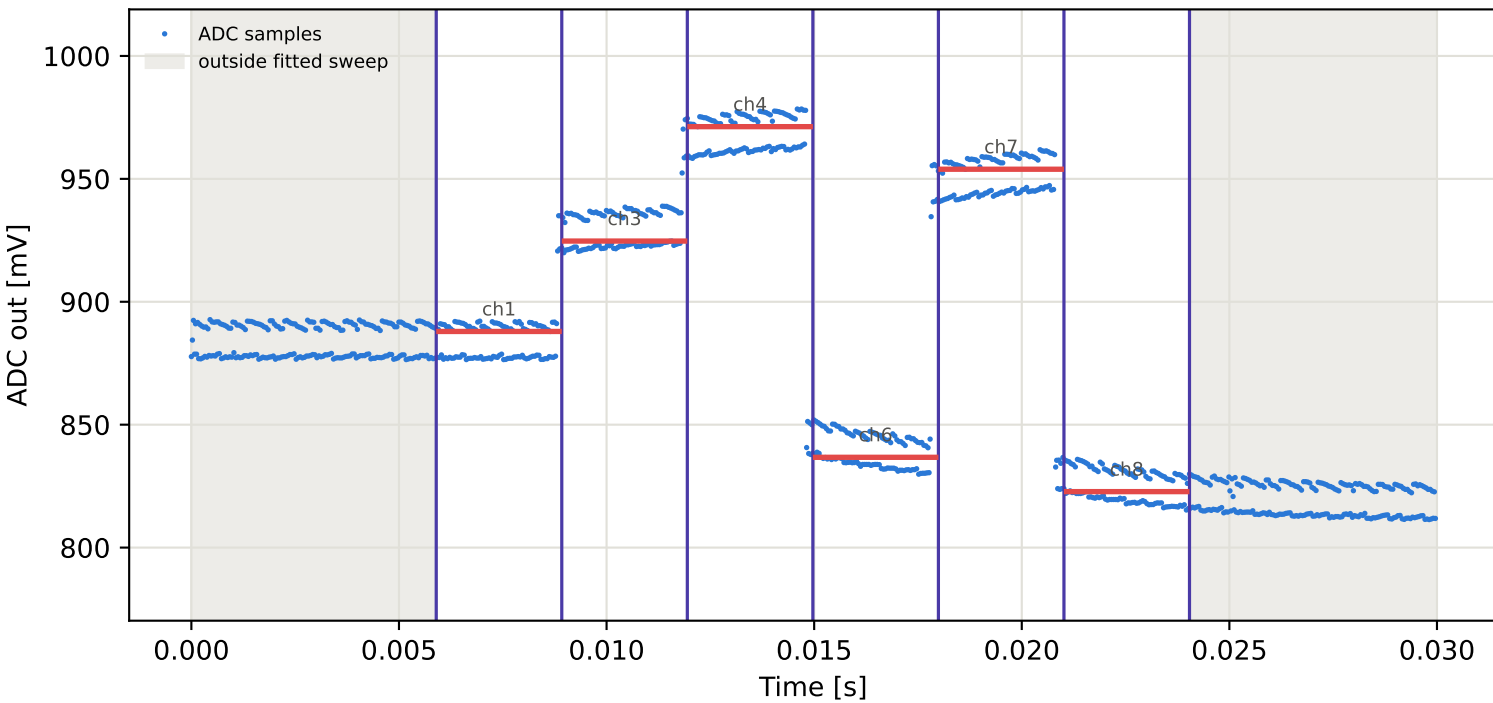
Tag15 &lt;- Tag1 | 925 MHz | run 0 | rep 1 | phase 120.85 deg
