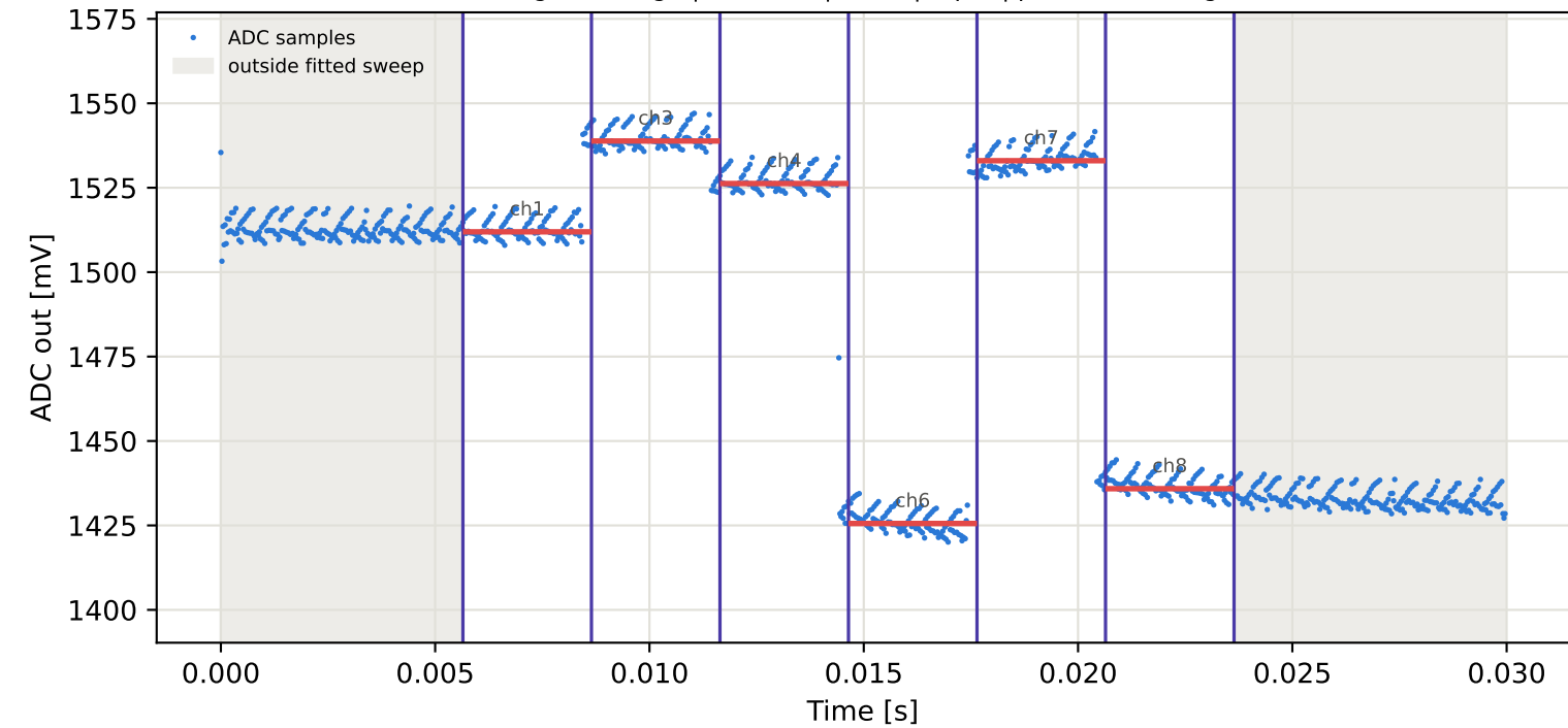
Tag16 &lt;- Tag5 | 895 MHz | run 0 | rep 1 | phase 7.67 deg
