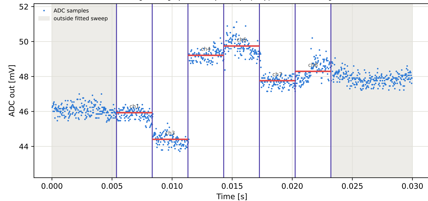
Tag9 &lt;- Tag7 | 775 MHz | run 0 | rep 1 | phase -129.21 deg
