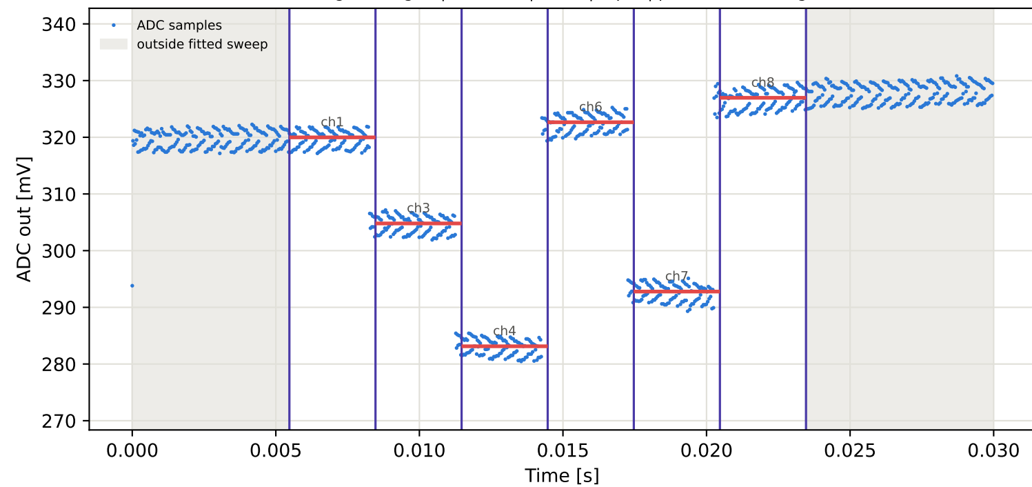
Tag6 &lt;- Tag3 | 975 MHz | run 0 | rep 1 | phase -79.77 deg
