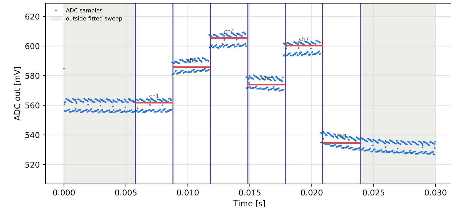
Tag9 &lt;- Tag16 | 905 MHz | run 0 | rep 1 | phase -76.08 deg
