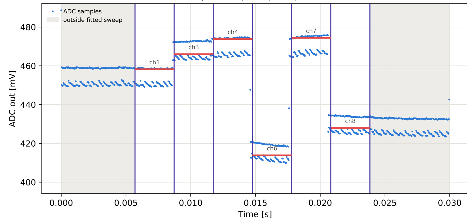
Tag5 &lt;- Tag2 | 935 MHz | run 0 | rep 1 | phase 27.57 deg
