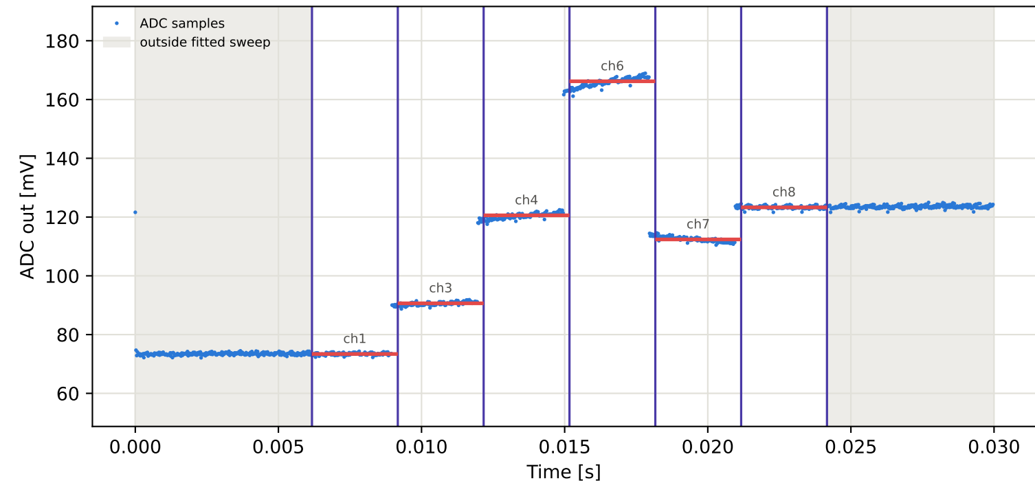
Tag5 &lt;- Tag1 | 895 MHz | run 0 | rep 1 | phase 162.34 deg
