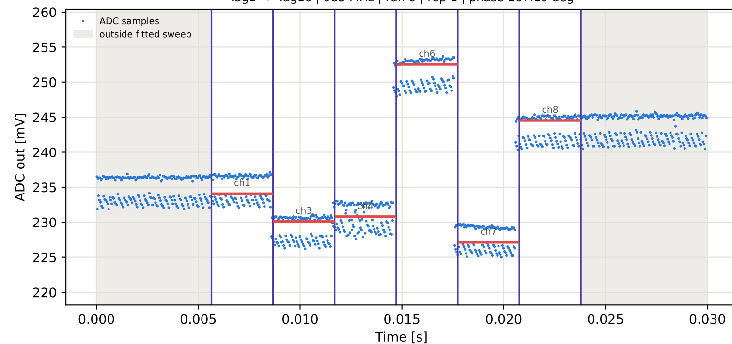
Tag1 &lt;- Tag16 | 985 MHz | run 0 | rep 1 | phase -69.69 deg
