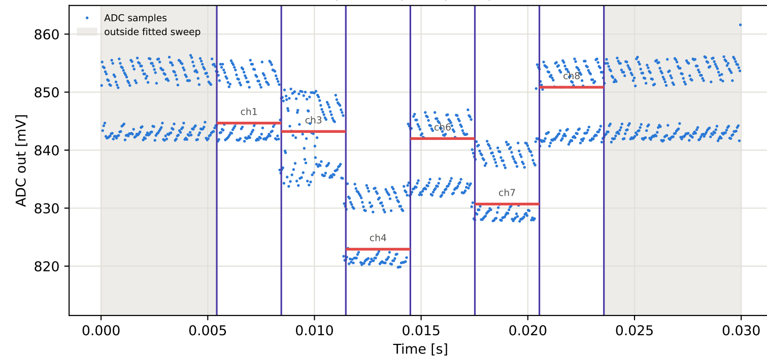
Tag16 &lt;- Tag6 | 955 MHz | run 0 | rep 1 | phase 83.84 deg
