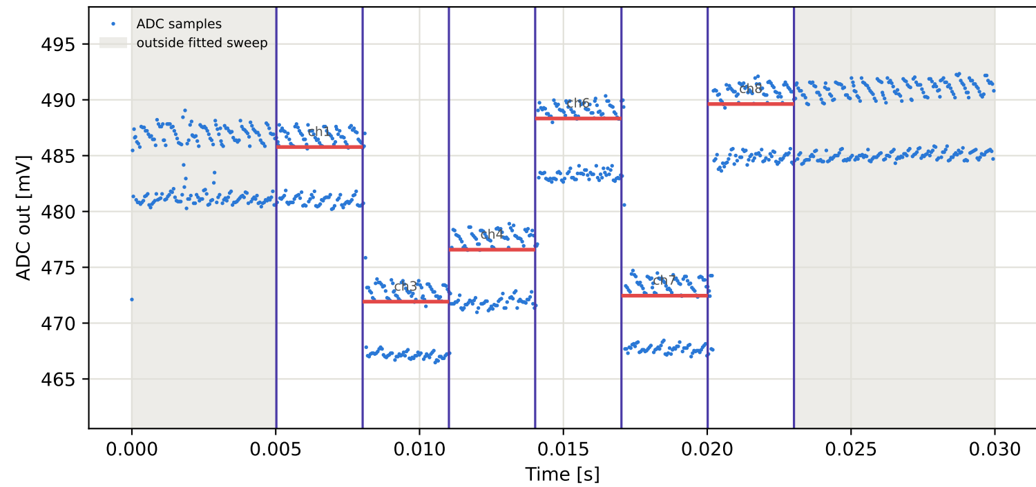
Tag6 &lt;- Tag2 | 835 MHz | run 0 | rep 1 | phase -98.46 deg
