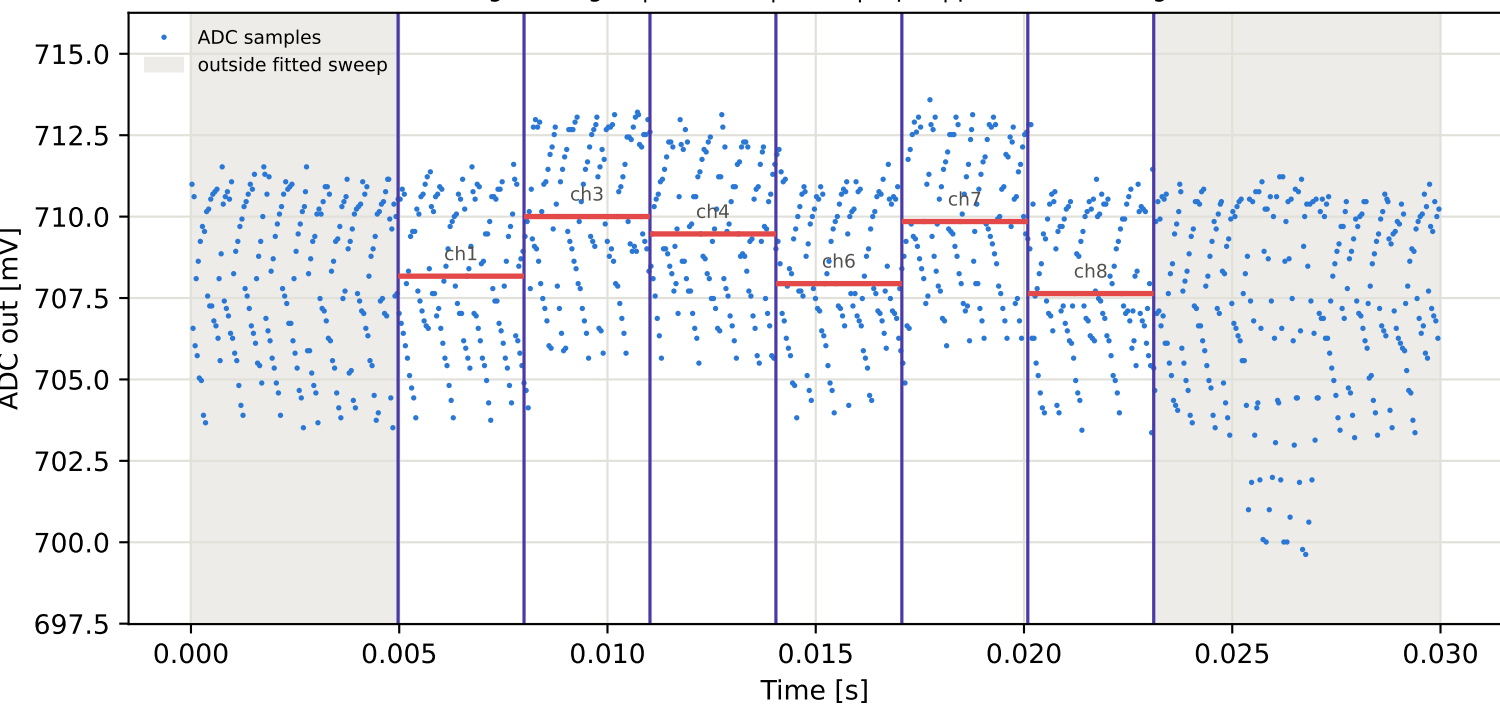
Tag8 &lt;- Tag15 | 845 MHz | run 0 | rep 1 | phase -24.93 deg
