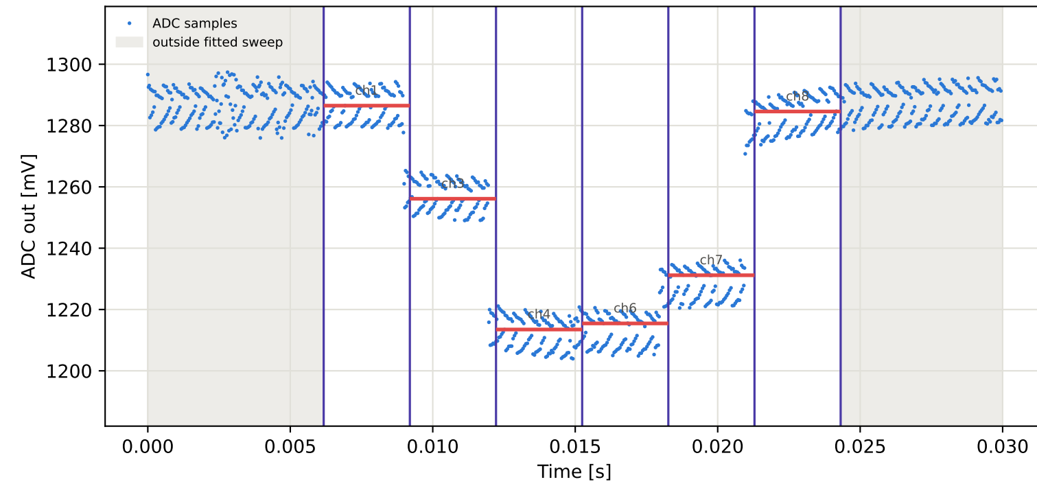
Tag15 &lt;- Tag5 | 915 MHz | run 0 | rep 1 | phase -67.55 deg
