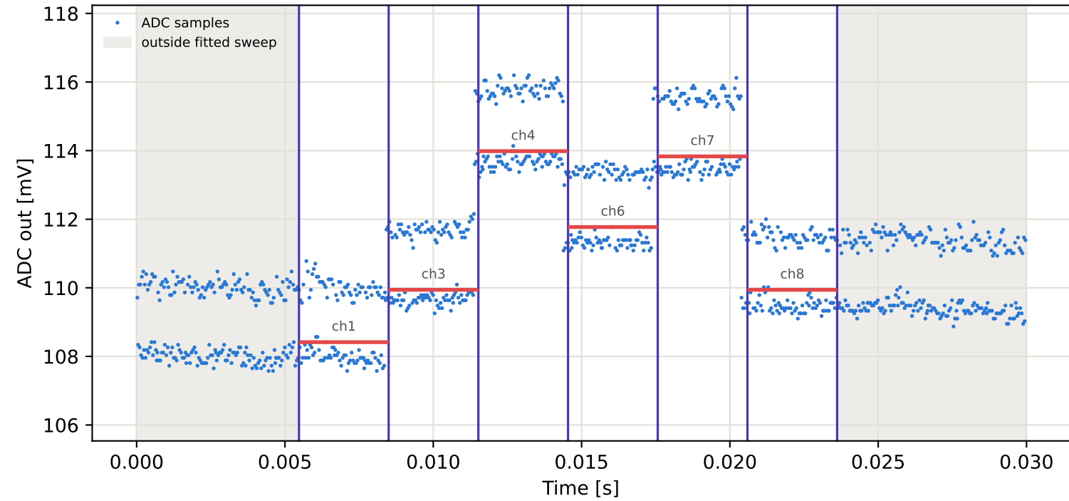
Tag6 &lt;- Tag10 | 795 MHz | run 0 | rep 1 | phase 113.03 deg
