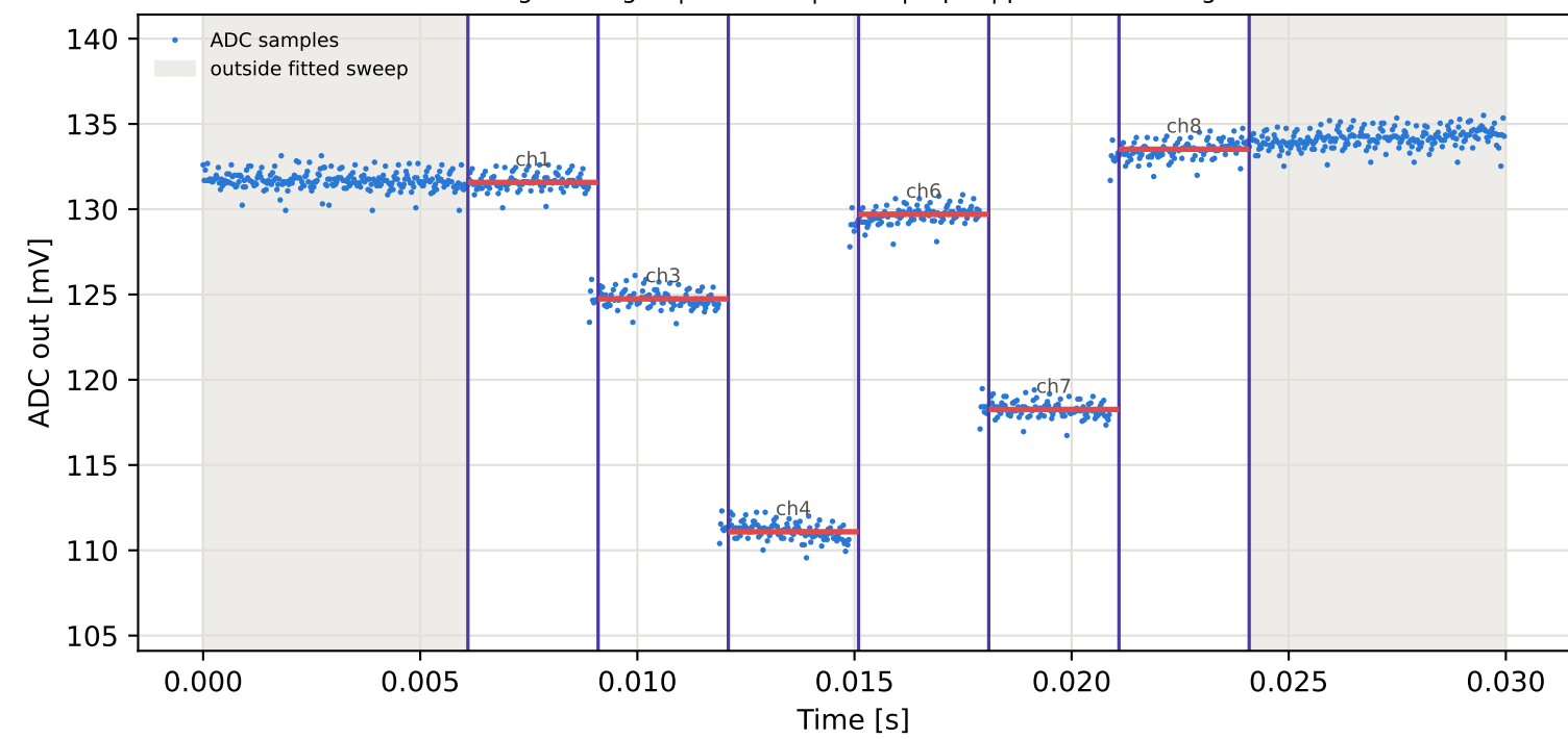
Tag1 &lt;- Tag2 | 995 MHz | run 0 | rep 1 | phase -70.16 deg
