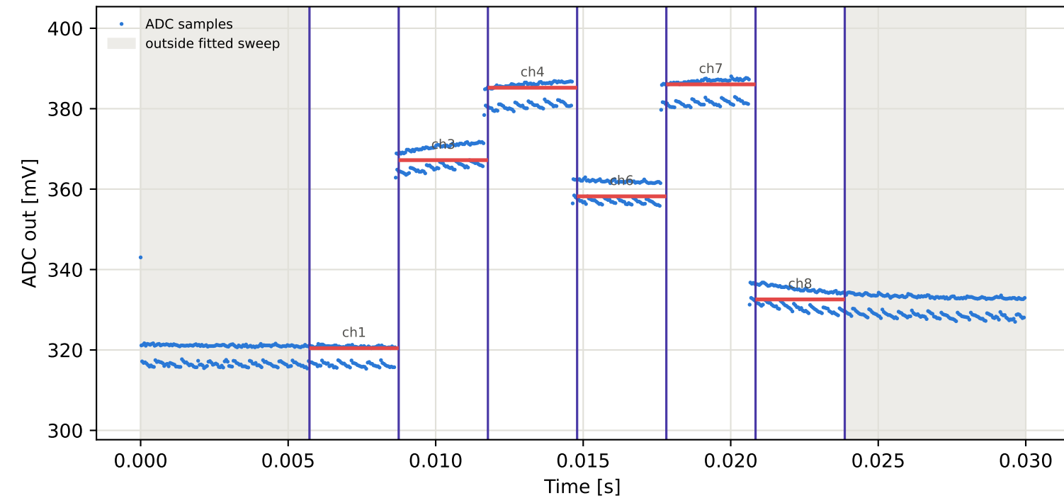
Tag5 &lt;- Tag3 | 855 MHz | run 0 | rep 1 | phase 59.24 deg
