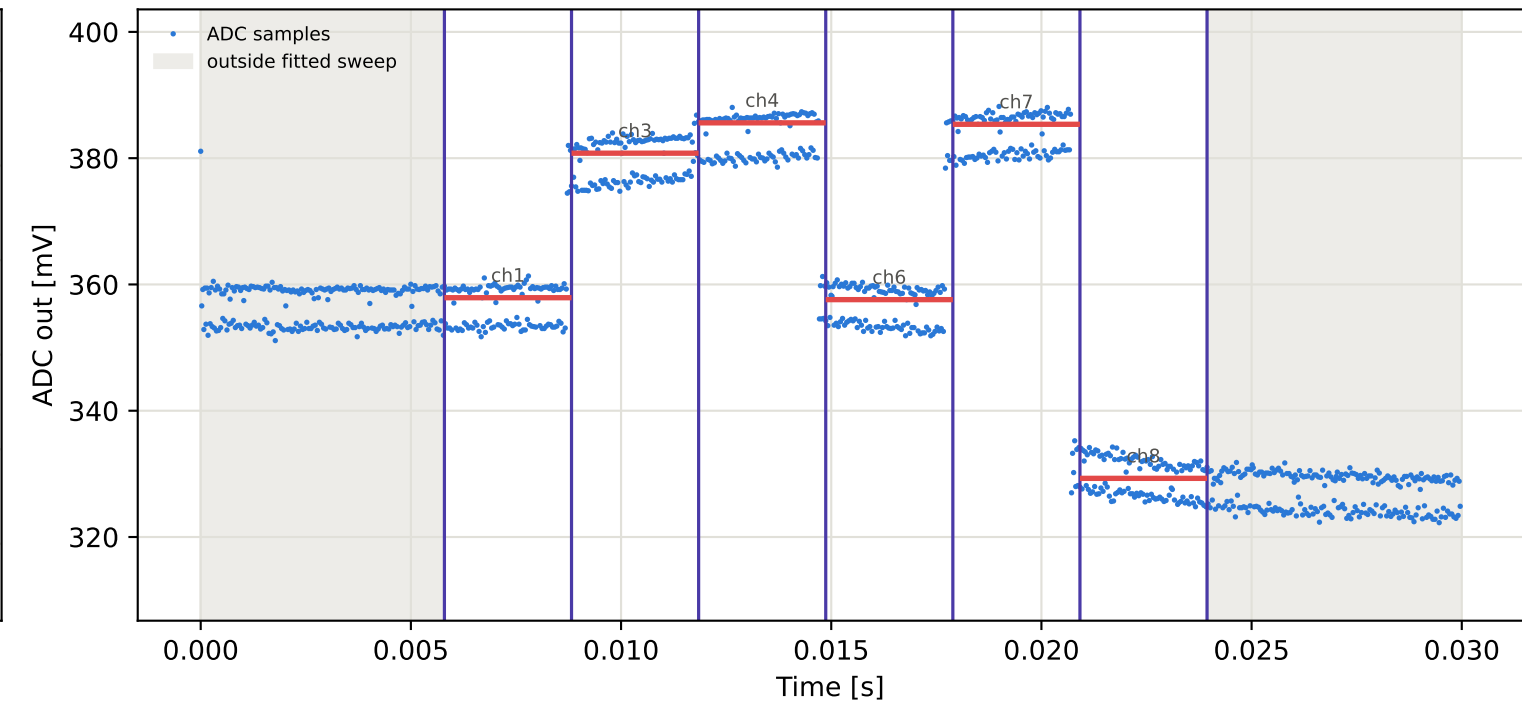
Tag10 &lt;- Tag1 | 885 MHz | run 0 | rep 1 | phase -4.53 deg
