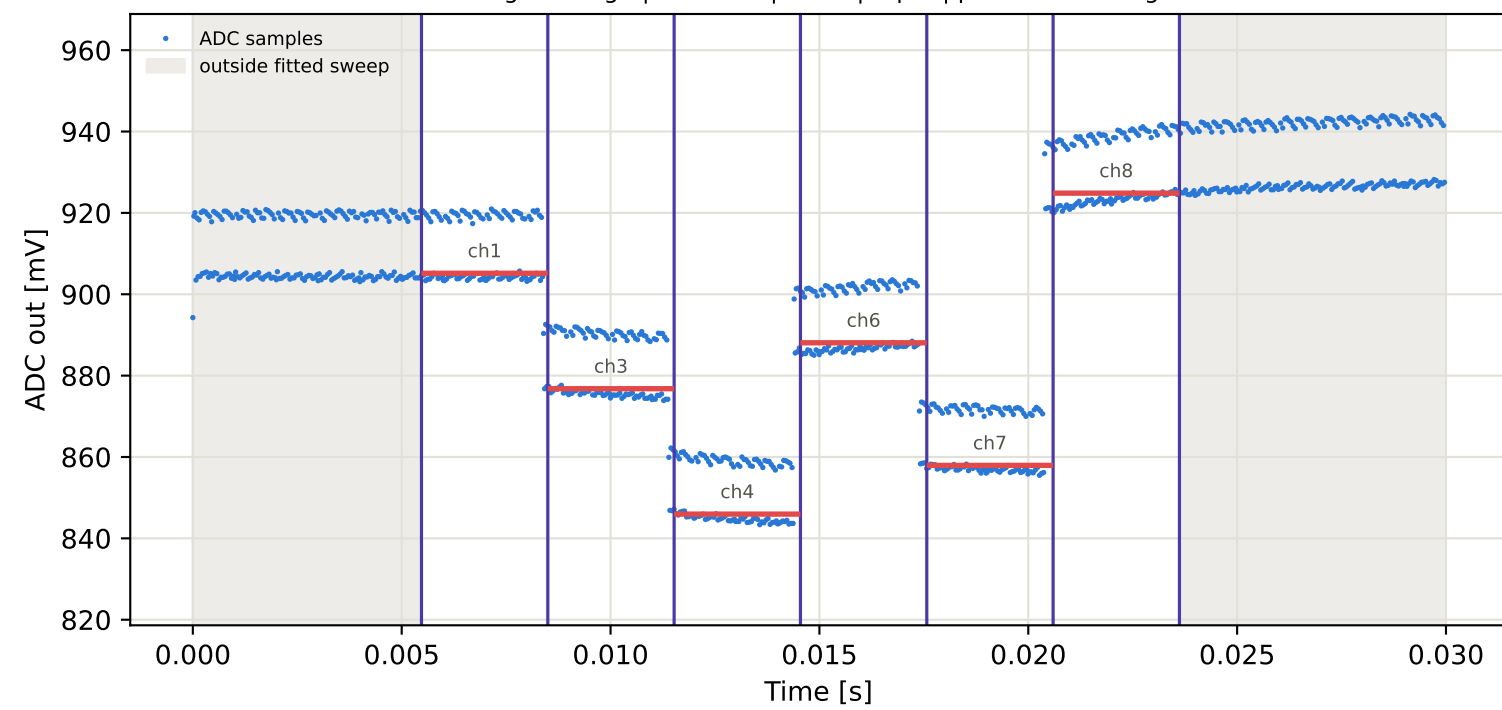
Tag3 &lt;- Tag7 | 915 MHz | run 0 | rep 1 | phase -150.27 deg
