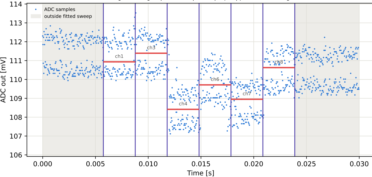
Tag16 &lt;- Tag10 | 795 MHz | run 0 | rep 1 | phase 80.23 deg
