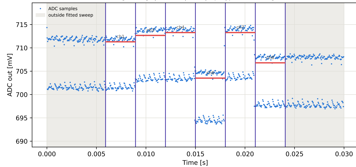
Tag8 &lt;- Tag4 | 845 MHz | run 0 | rep 1 | phase -130.27 deg
