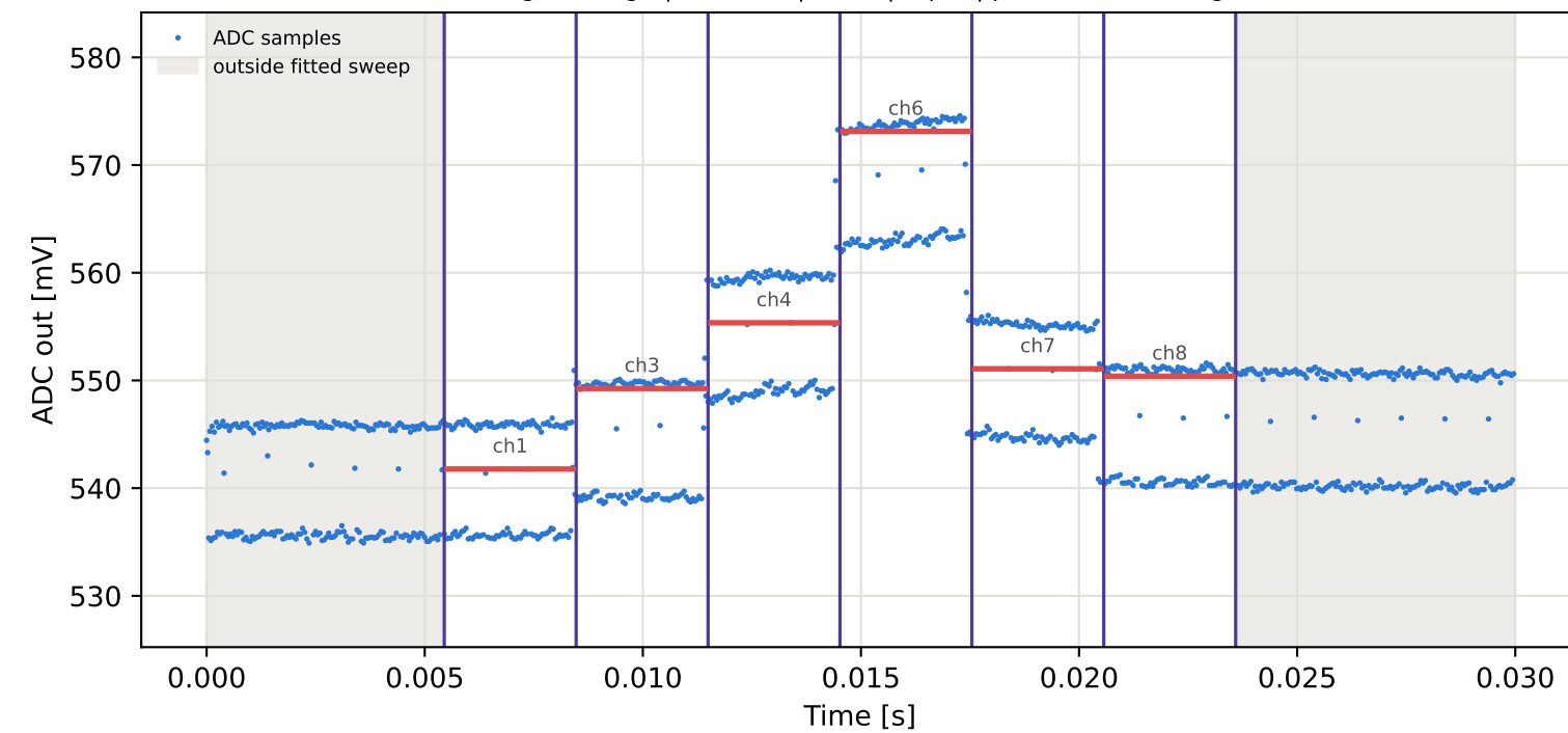
Tag8 &lt;- Tag4 | 945 MHz | run 0 | rep 1 | phase -126.71 deg
