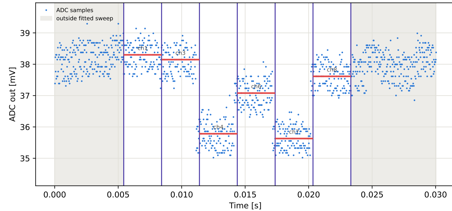
Tag16 &lt;- Tag10 | 775 MHz | run 0 | rep 1 | phase 42.27 deg
