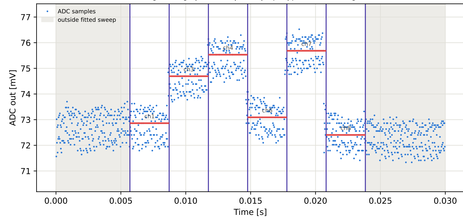
Tag1 &lt;- Tag9 | 795 MHz | run 0 | rep 1 | phase -150.36 deg
