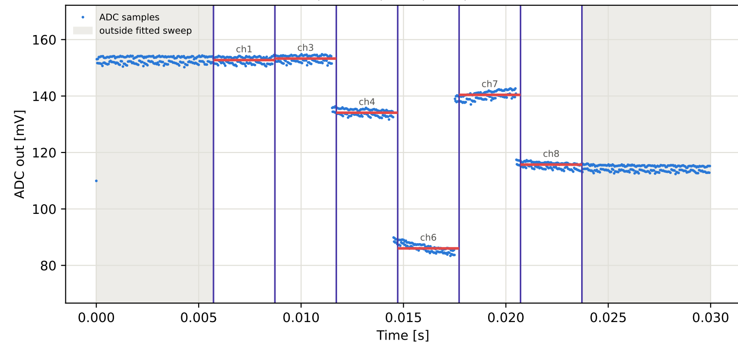
Tag4 &lt;- Tag3 | 895 MHz | run 0 | rep 1 | phase 17.47 deg
