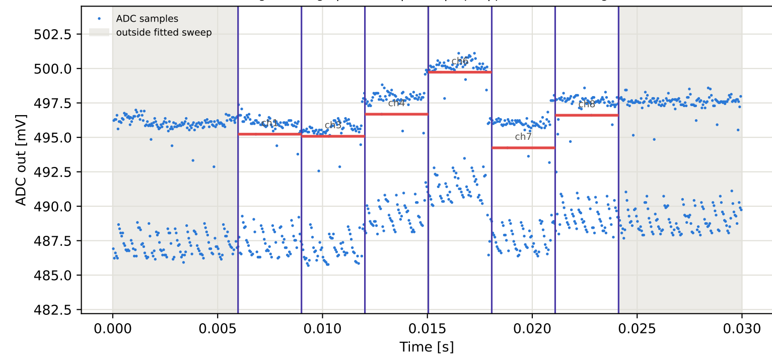
Tag16 &lt;- Tag6 | 985 MHz | run 0 | rep 1 | phase 145.50 deg
