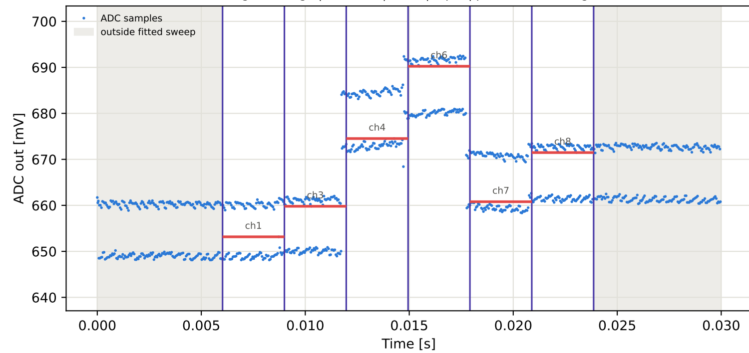
Tag2 &lt;- Tag10 | 975 MHz | run 0 | rep 1 | phase 99.76 deg
