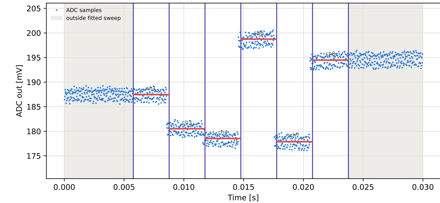
Tag3 &lt;- Tag8 | 995 MHz | run 0 | rep 1 | phase 147.56 deg
