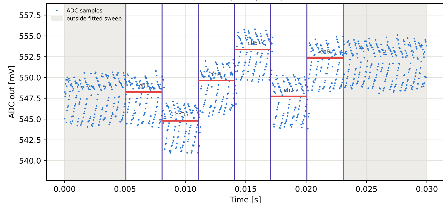
Tag2 &lt;- Tag10 | 825 MHz | run 0 | rep 1 | phase -96.18 deg
