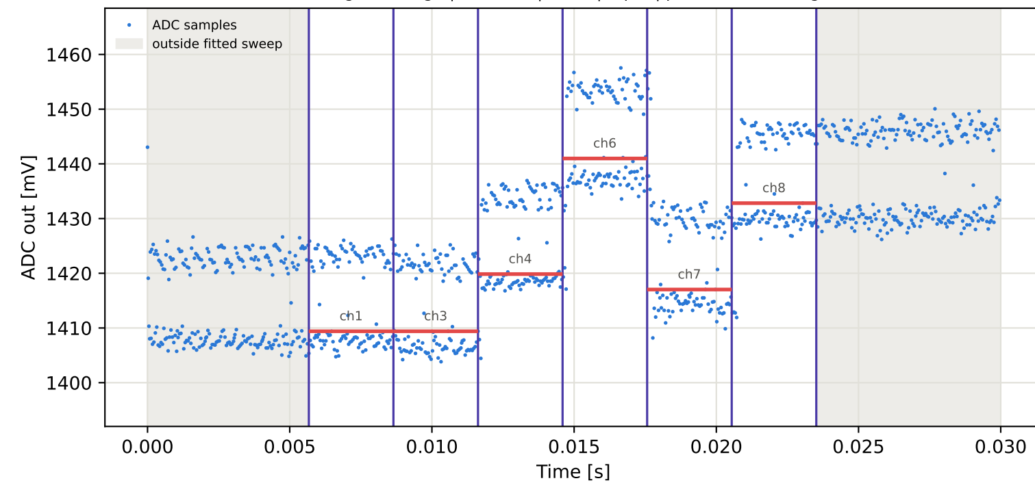
Tag15 &lt;- Tag9 | 885 MHz | run 0 | rep 1 | phase 79.04 deg
