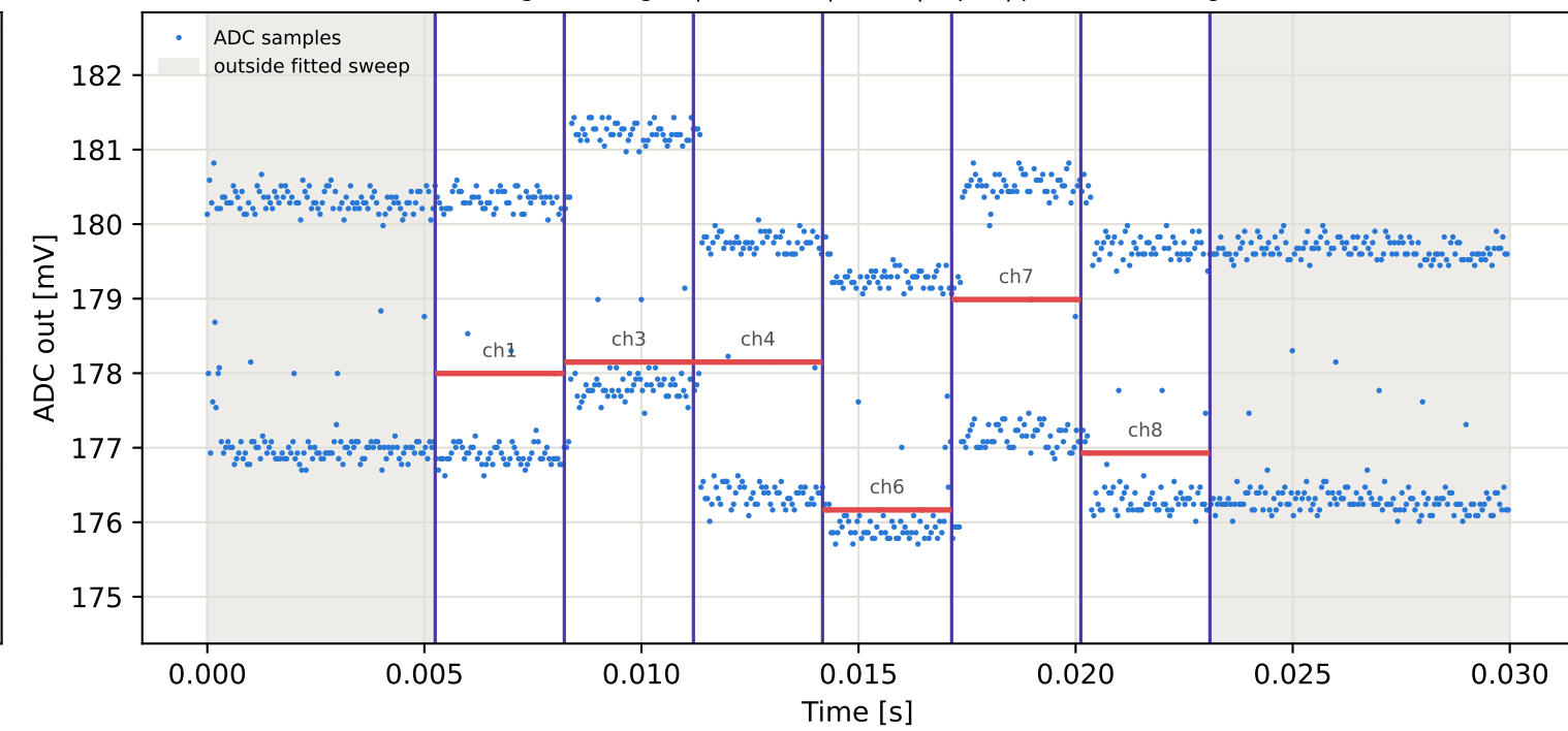
Tag10 &lt;- Tag3 | 795 MHz | run 0 | rep 1 | phase -69.99 deg
