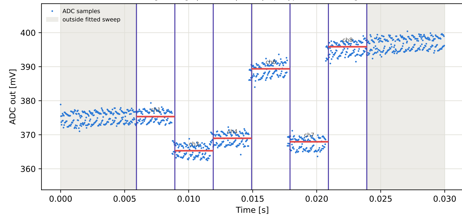
Tag2 &lt;- Tag5 | 875 MHz | run 0 | rep 1 | phase -141.26 deg
