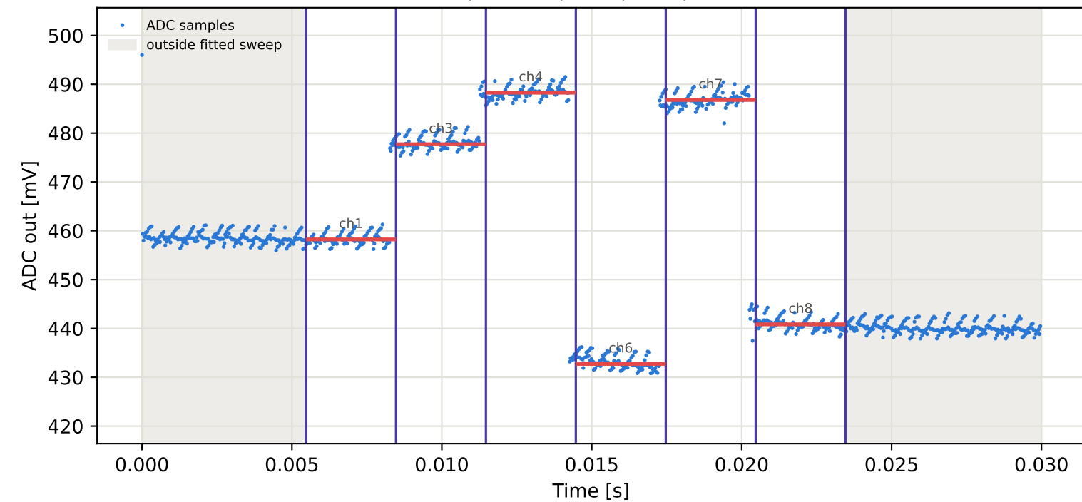
Tag9 &lt;- Tag16 | 975 MHz | run 0 | rep 1 | phase -41.05 deg
