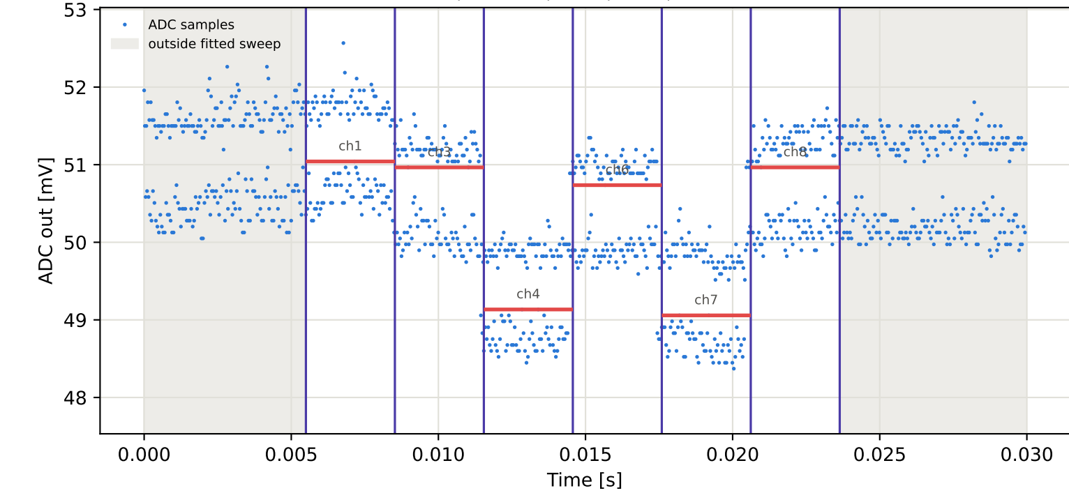
Tag1 &lt;- Tag4 | 785 MHz | run 0 | rep 1 | phase 103.73 deg
