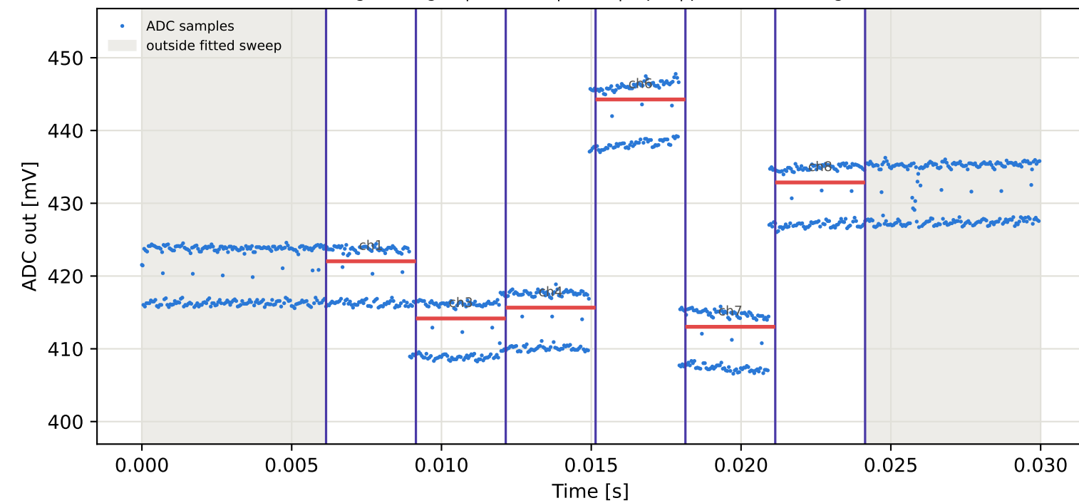
Tag5 &lt;- Tag16 | 965 MHz | run 0 | rep 1 | phase 48.96 deg
