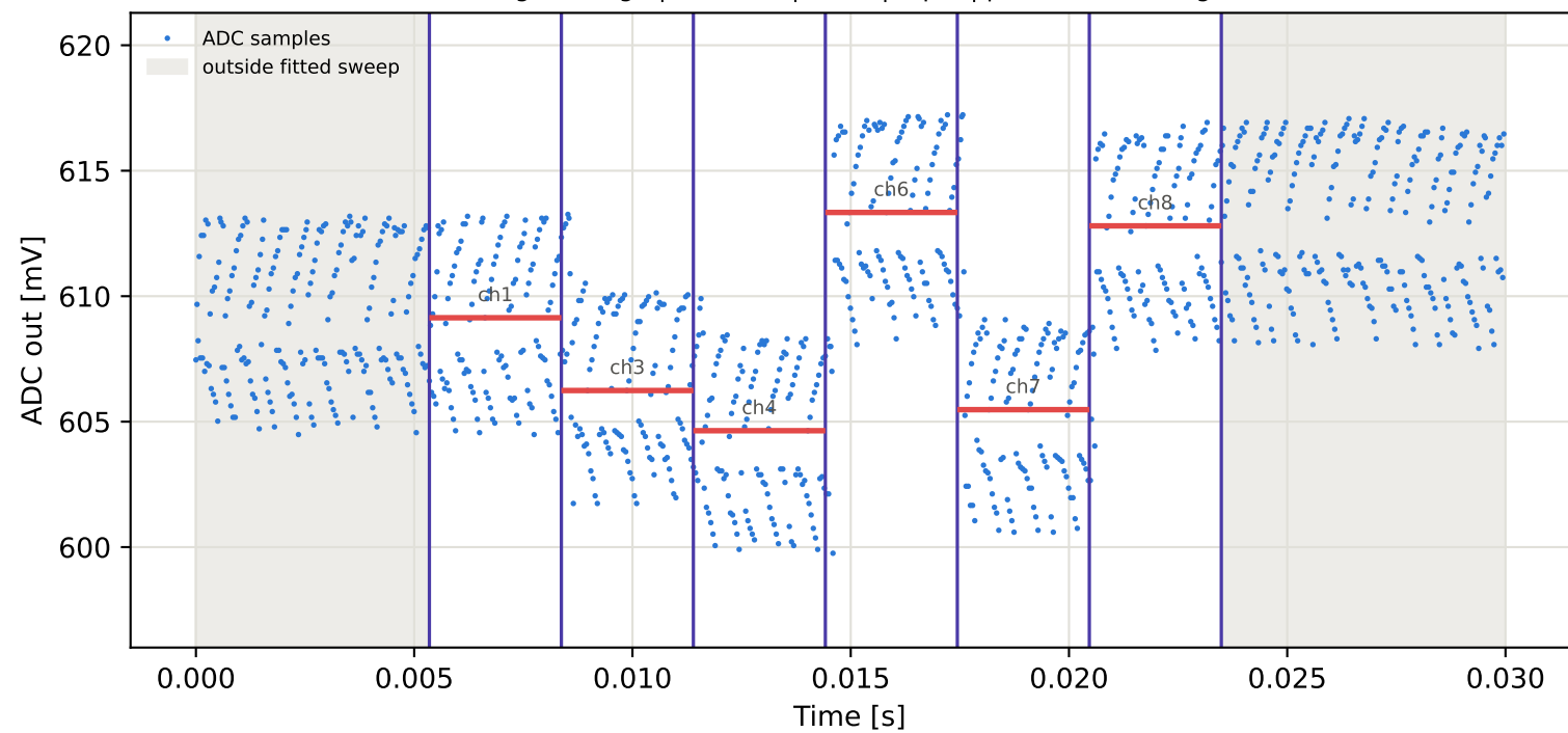
Tag7 &lt;- Tag15 | 935 MHz | run 0 | rep 1 | phase 82.28 deg
