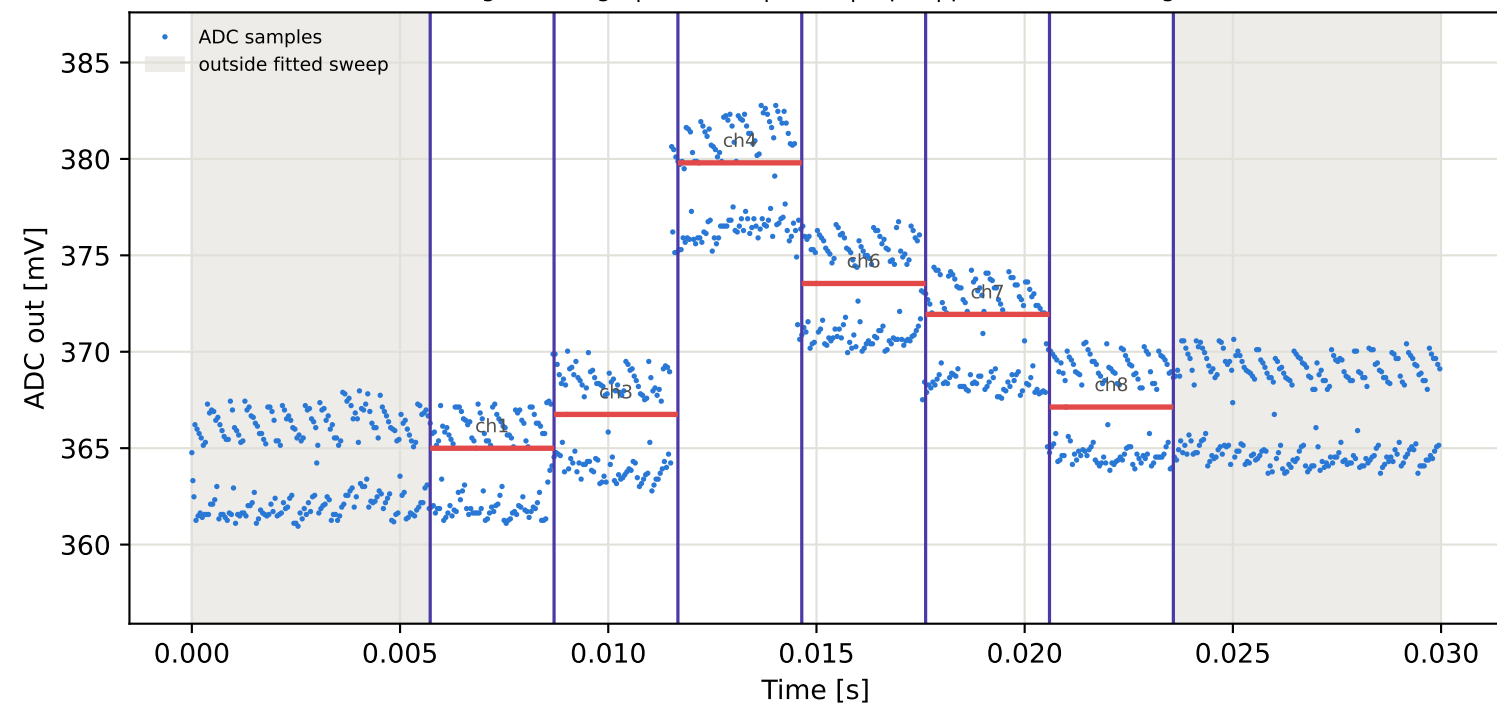
Tag16 &lt;- Tag7 | 995 MHz | run 0 | rep 1 | phase 139.57 deg
