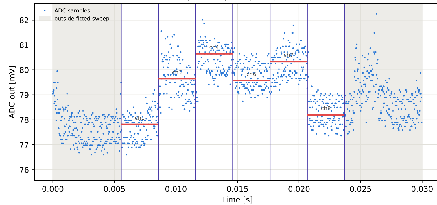
Tag16 &lt;- Tag4 | 775 MHz | run 0 | rep 1 | phase -28.75 deg
