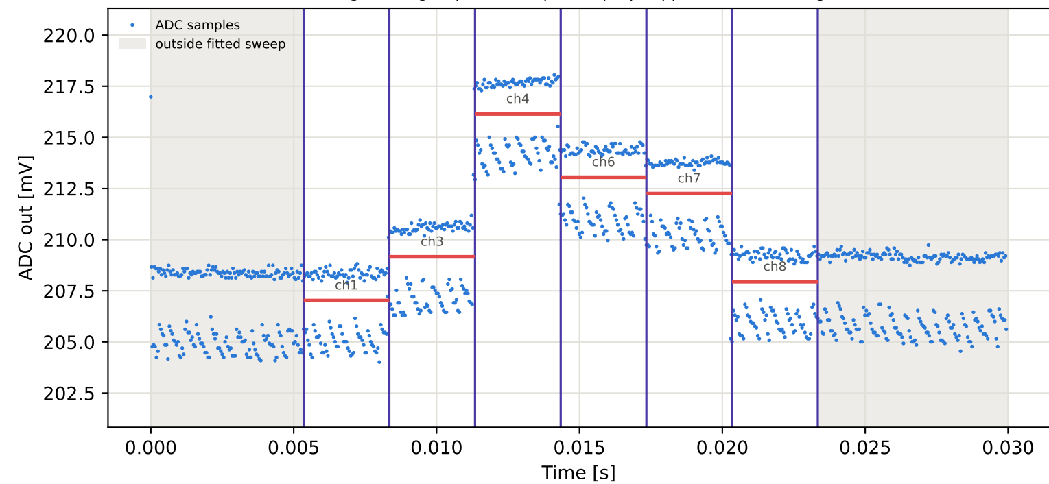
Tag4 &lt;- Tag16 | 955 MHz | run 0 | rep 1 | phase -12.03 deg
