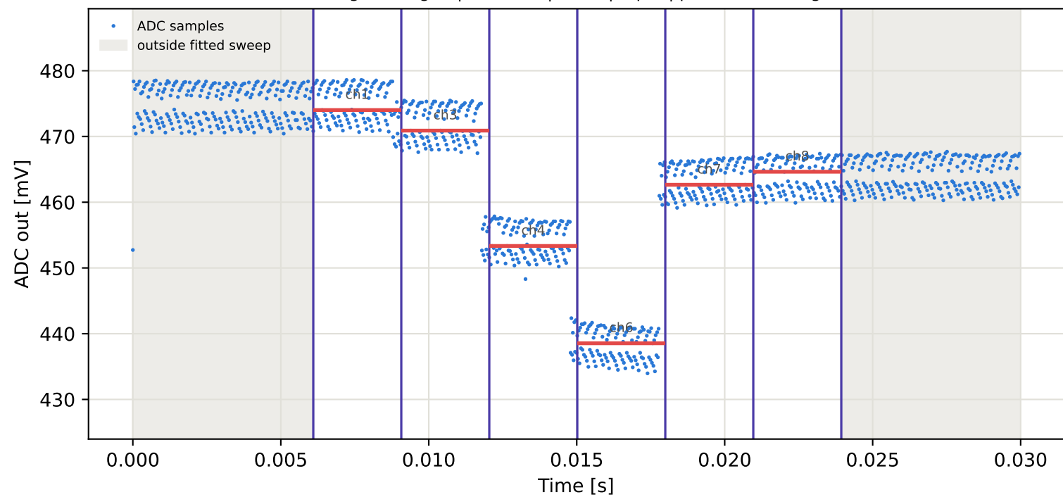
Tag3 &lt;- Tag2 | 945 MHz | run 0 | rep 1 | phase 19.91 deg
