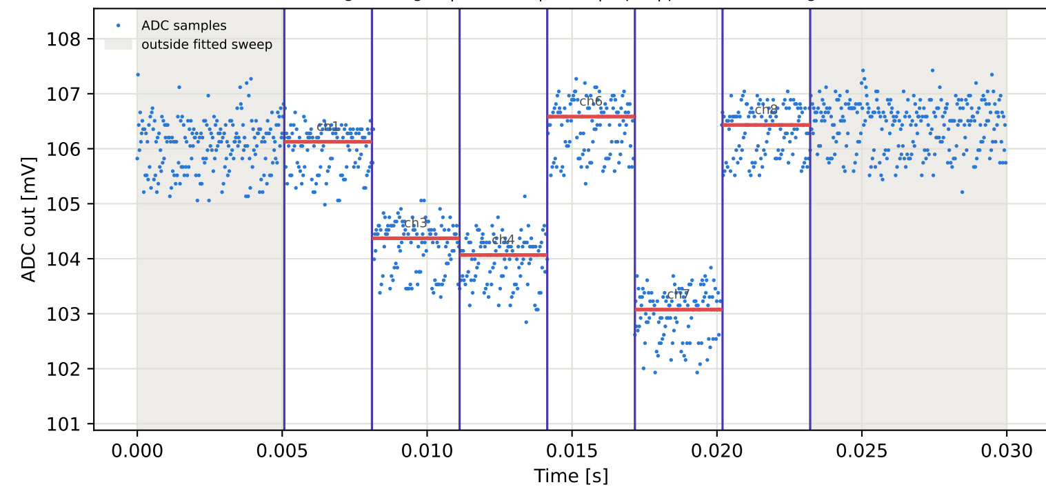
Tag5 &lt;- Tag3 | 775 MHz | run 0 | rep 1 | phase -77.23 deg
