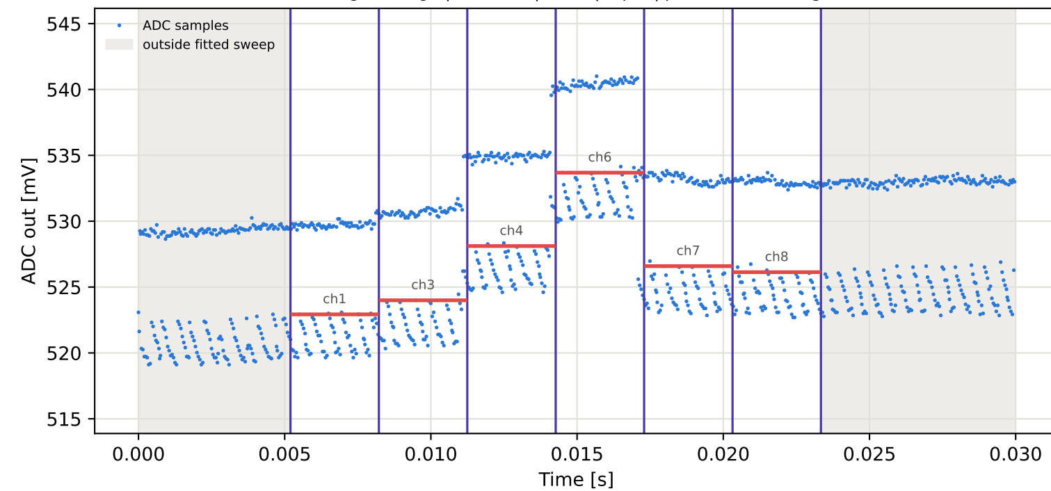
Tag5 &lt;- Tag8 | 925 MHz | run 0 | rep 1 | phase 1.25 deg
