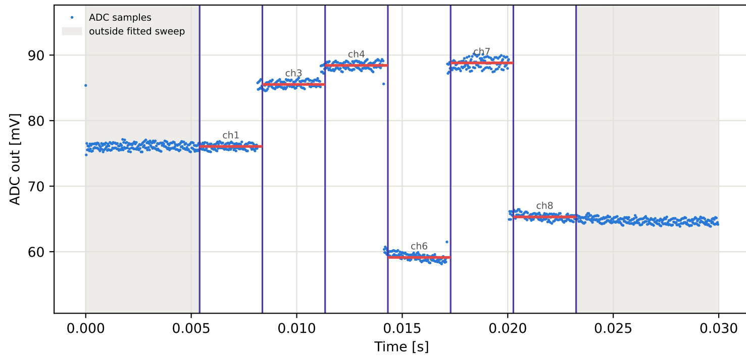
Tag6 &lt;- Tag9 | 965 MHz | run 0 | rep 1 | phase -34.35 deg
