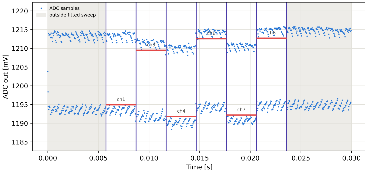
Tag16 &lt;- Tag15 | 935 MHz | run 0 | rep 1 | phase 171.96 deg
