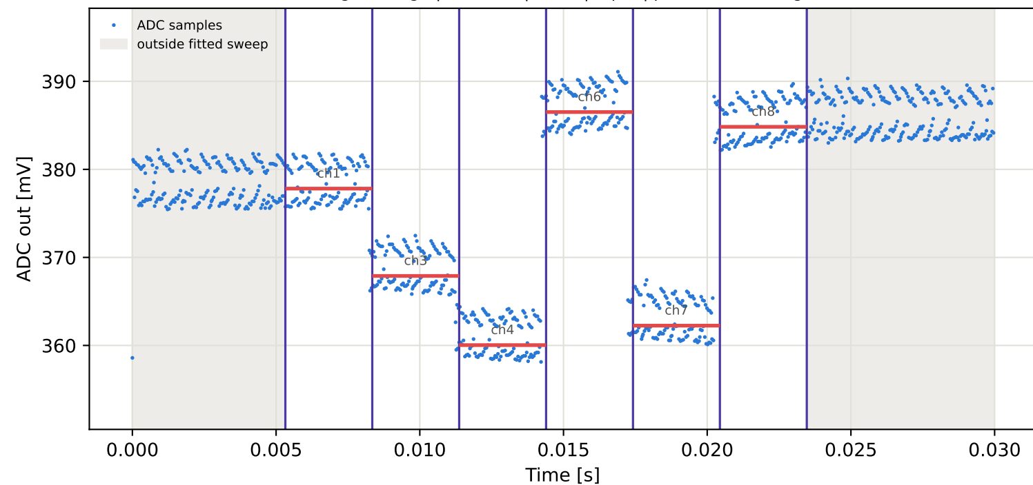
Tag5 &lt;- Tag9 | 975 MHz | run 0 | rep 1 | phase 137.22 deg
