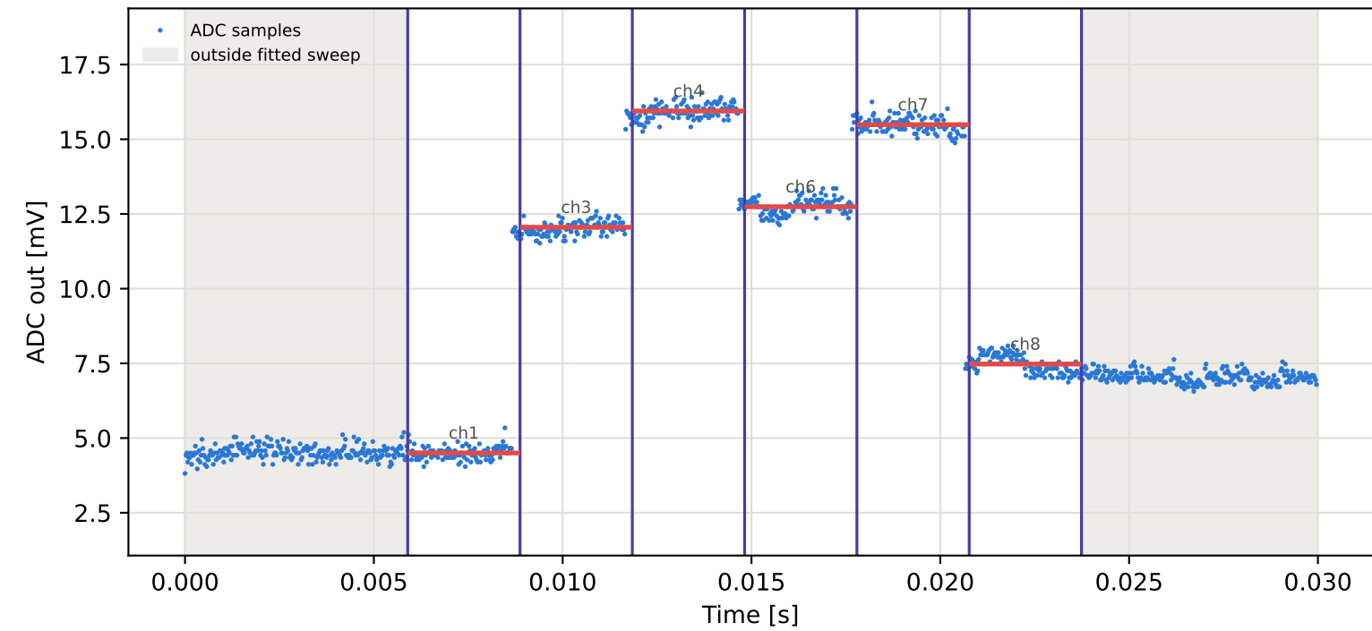
Tag4 &lt;- Tag3 | 865 MHz | run 0 | rep 1 | phase -99.27 deg
