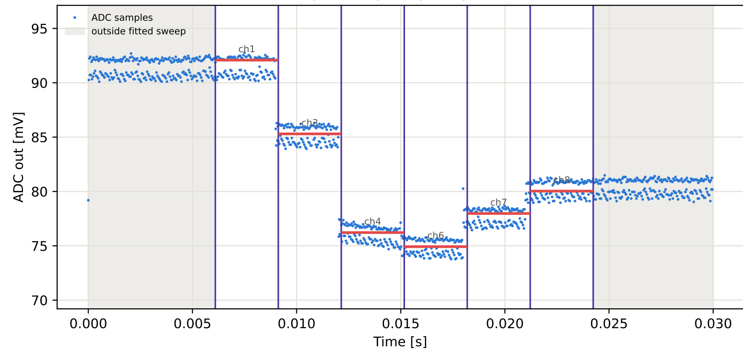
Tag1 &lt;- Tag4 | 845 MHz | run 0 | rep 1 | phase 57.38 deg
