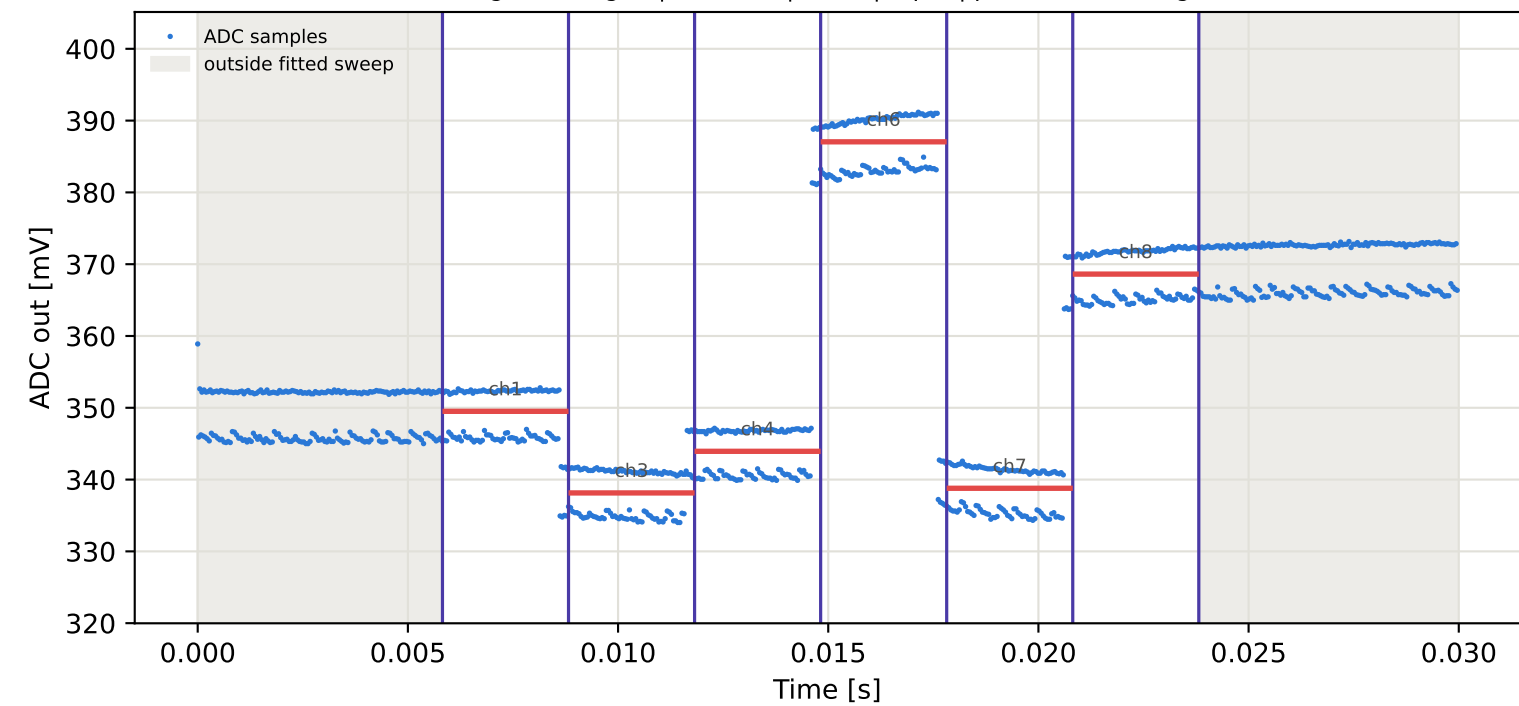
Tag10 &lt;- Tag3 | 955 MHz | run 0 | rep 1 | phase -124.63 deg
