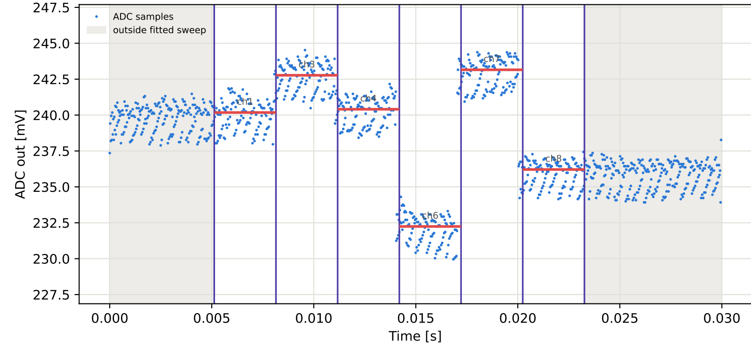
Tag8 &lt;- Tag6 | 995 MHz | run 0 | rep 1 | phase -60.25 deg
