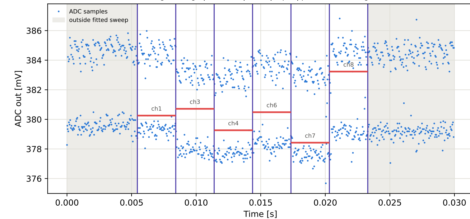
Tag2 &lt;- Tag15 | 875 MHz | run 0 | rep 1 | phase 85.96 deg
