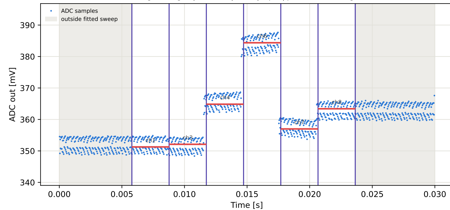
Tag1 &lt;- Tag16 | 945 MHz | run 0 | rep 1 | phase -45.32 deg
