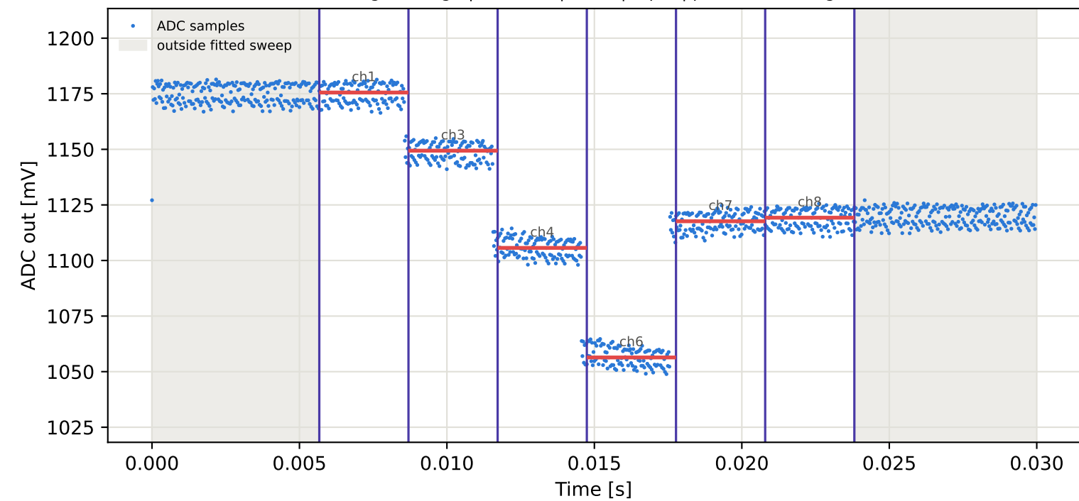
Tag3 &lt;- Tag7 | 885 MHz | run 0 | rep 1 | phase -131.52 deg
