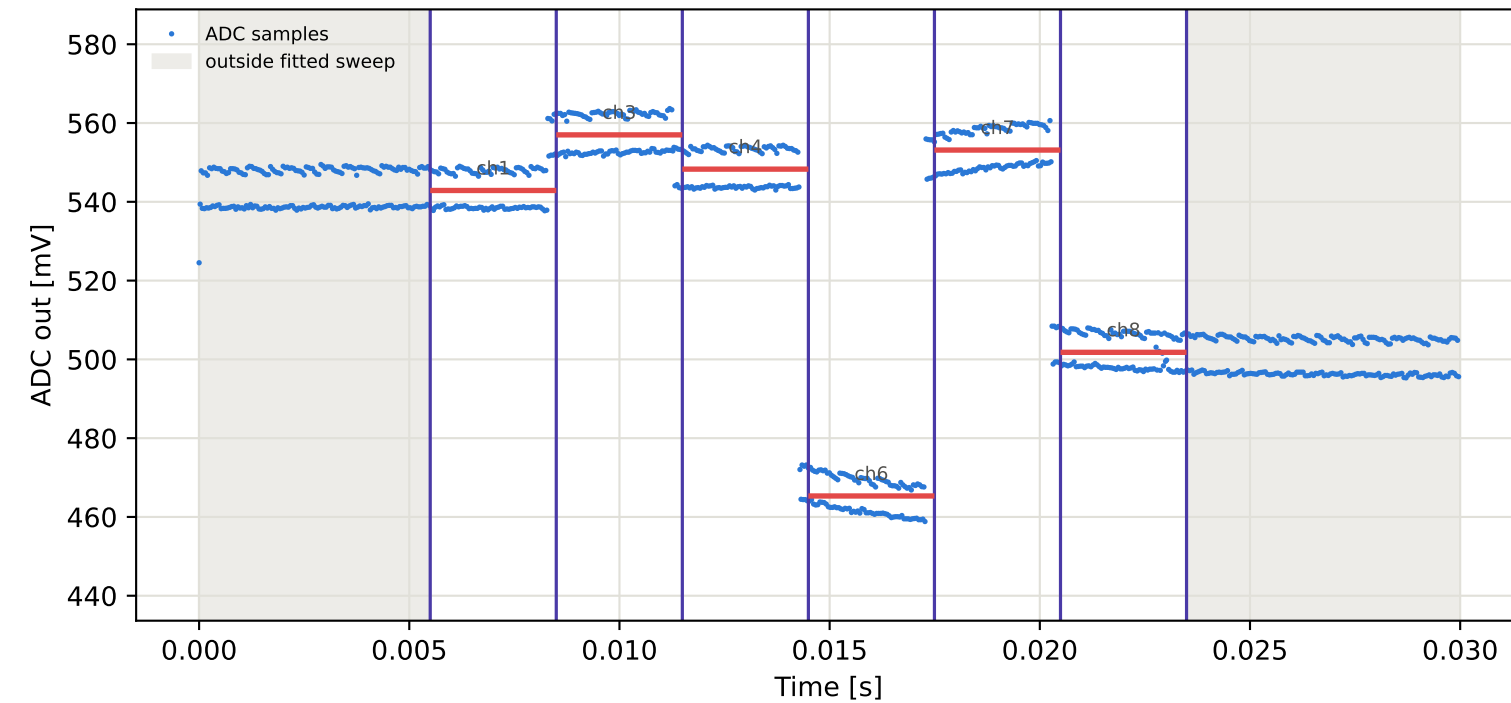
Tag5 &lt;- Tag3 | 925 MHz | run 0 | rep 1 | phase 177.33 deg
