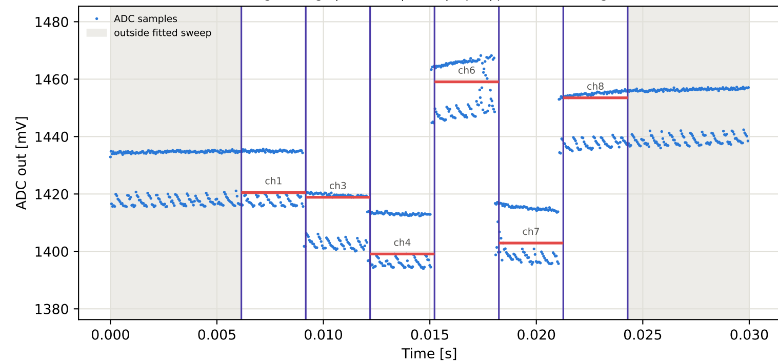
Tag8 &lt;- Tag4 | 895 MHz | run 0 | rep 1 | phase 43.61 deg
