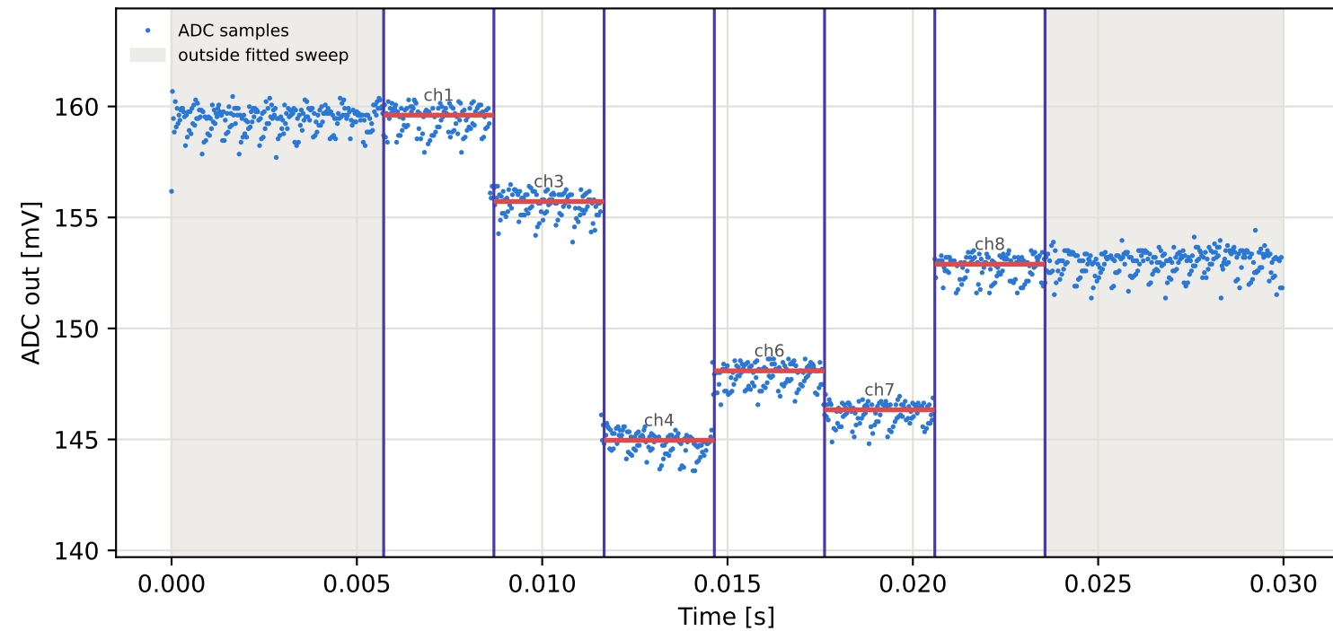
Tag5 &lt;- Tag1 | 825 MHz | run 0 | rep 1 | phase 29.16 deg
