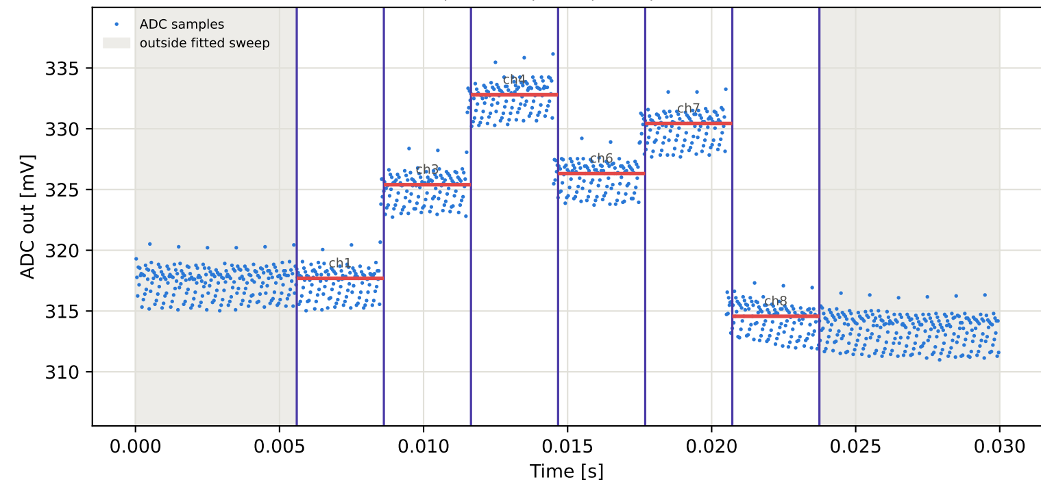
Tag1 &lt;- Tag4 | 905 MHz | run 0 | rep 1 | phase -93.91 deg
