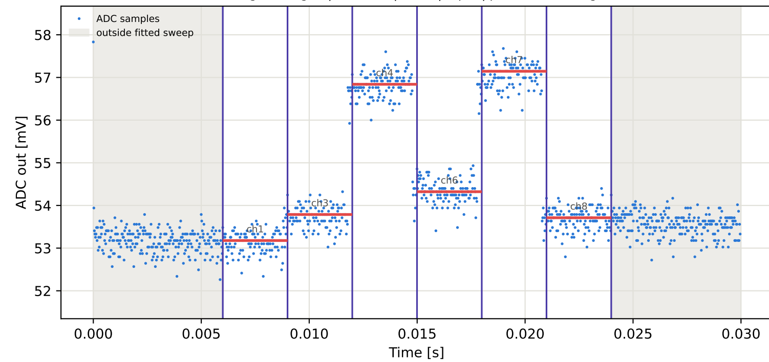
Tag1 &lt;- Tag16 | 775 MHz | run 0 | rep 1 | phase 108.57 deg
