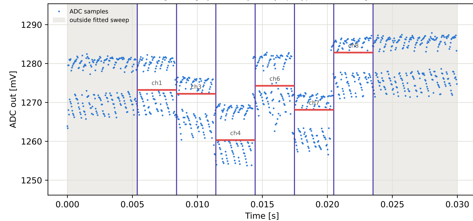
Tag8 &lt;- Tag4 | 875 MHz | run 0 | rep 1 | phase -1.49 deg
