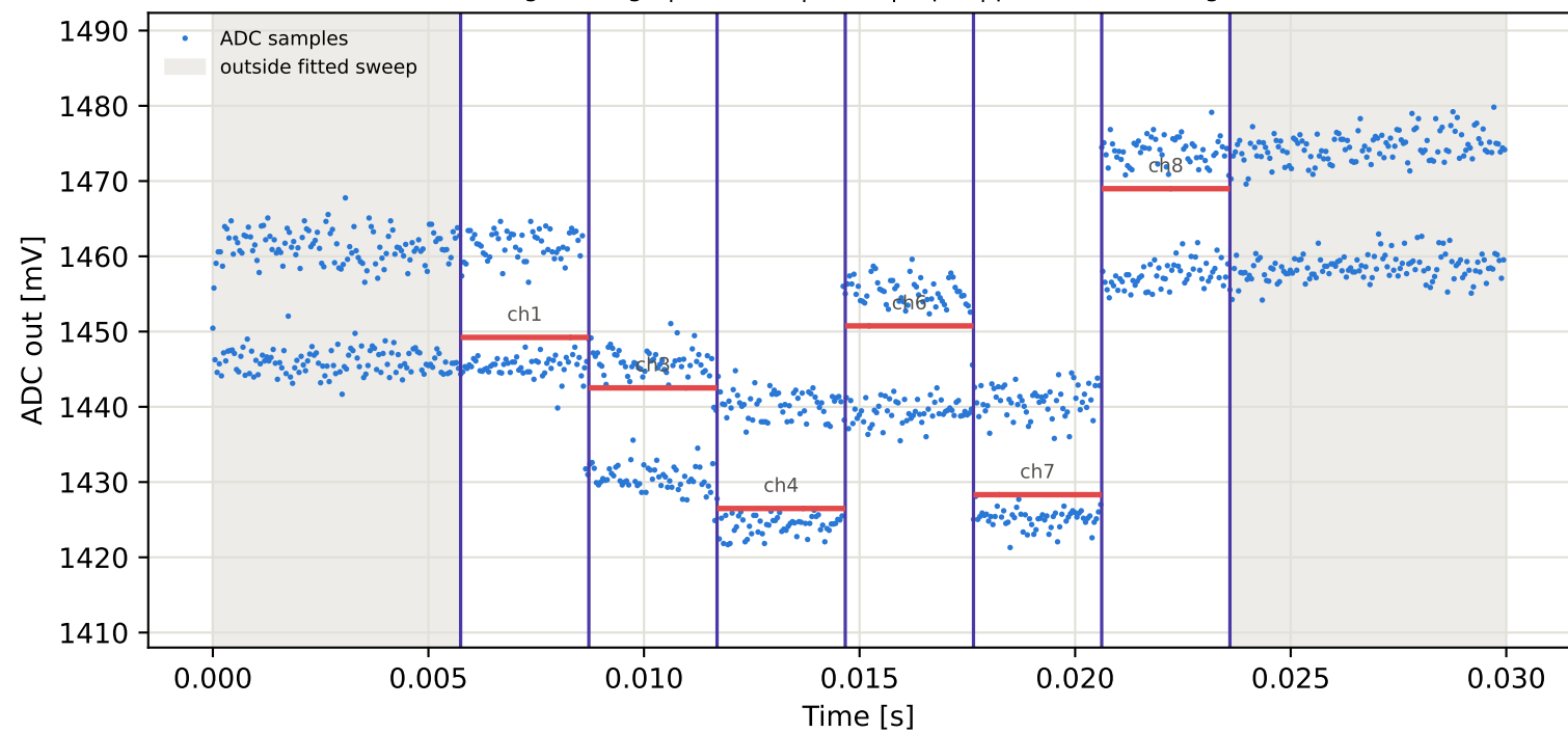
Tag8 &lt;- Tag7 | 885 MHz | run 0 | rep 1 | phase 31.05 deg
