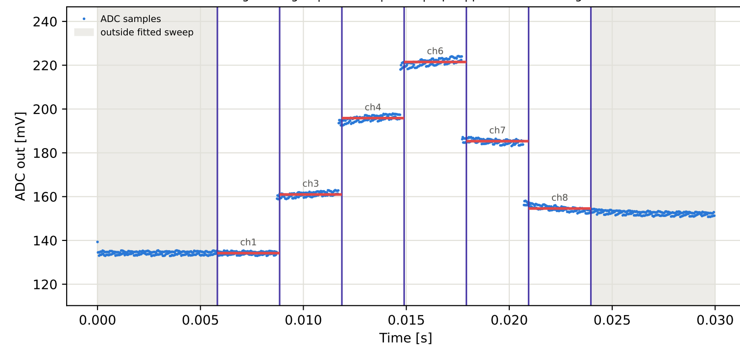
Tag7 &lt;- Tag3 | 905 MHz | run 0 | rep 1 | phase 157.29 deg
