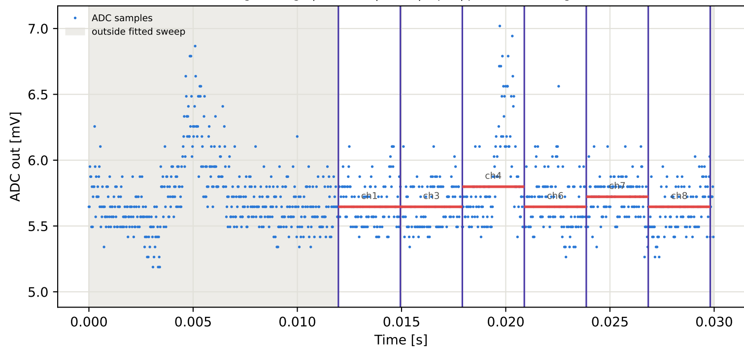
Tag2 &lt;- Tag6 | 775 MHz | run 0 | rep 1 | phase -178.55 deg
