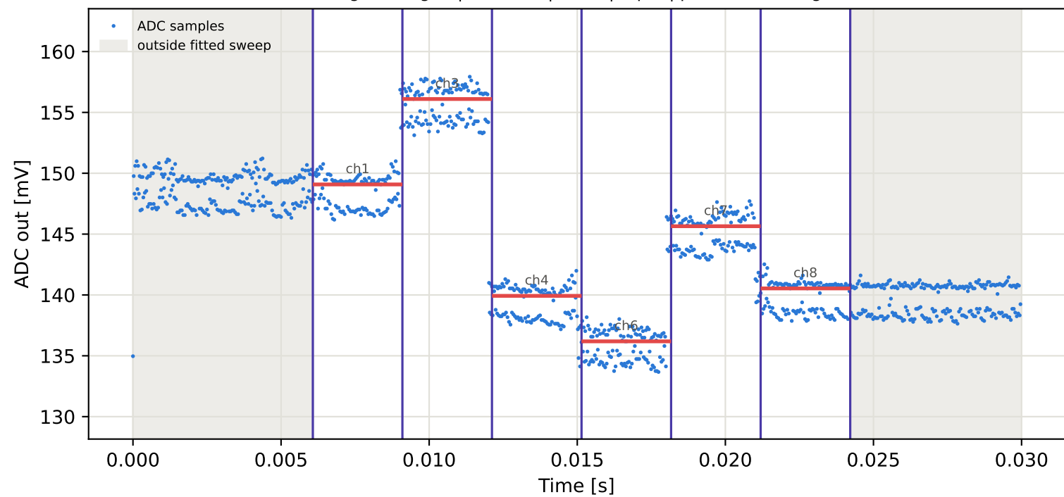
Tag9 &lt;- Tag2 | 825 MHz | run 0 | rep 1 | phase -105.29 deg
