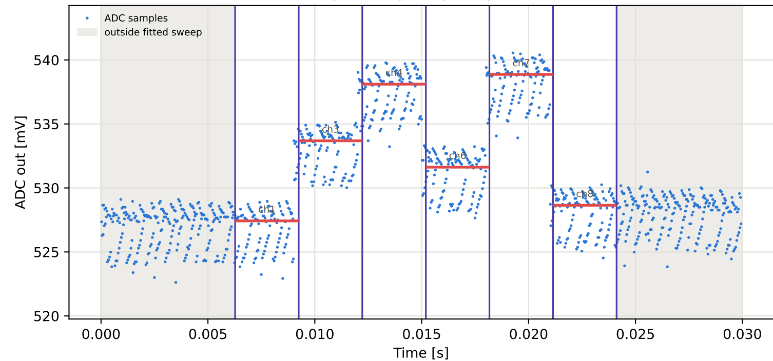
Tag7 &lt;- Tag15 | 825 MHz | run 0 | rep 1 | phase -72.36 deg
