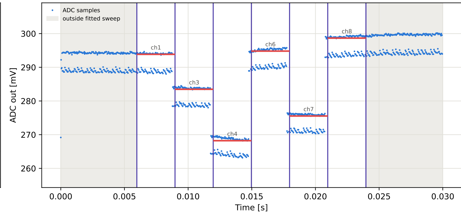
Tag3 &lt;- Tag2 | 985 MHz | run 0 | rep 1 | phase -7.14 deg
