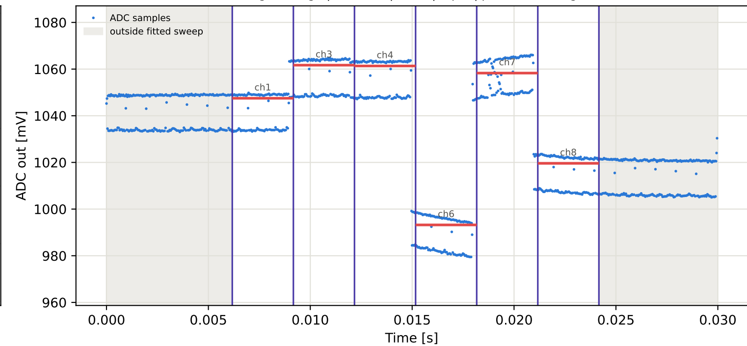
Tag7 &lt;- Tag4 | 895 MHz | run 0 | rep 1 | phase 138.22 deg
