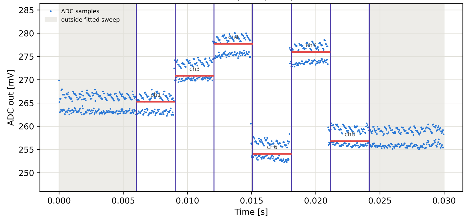
Tag5 &lt;- Tag2 | 995 MHz | run 0 | rep 1 | phase 132.92 deg
