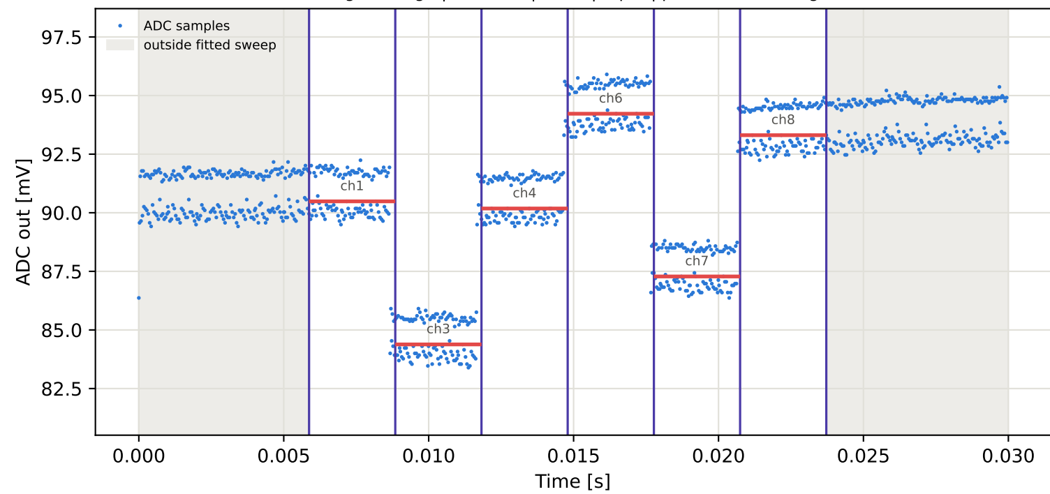
Tag10 &lt;- Tag1 | 805 MHz | run 0 | rep 1 | phase -94.10 deg
