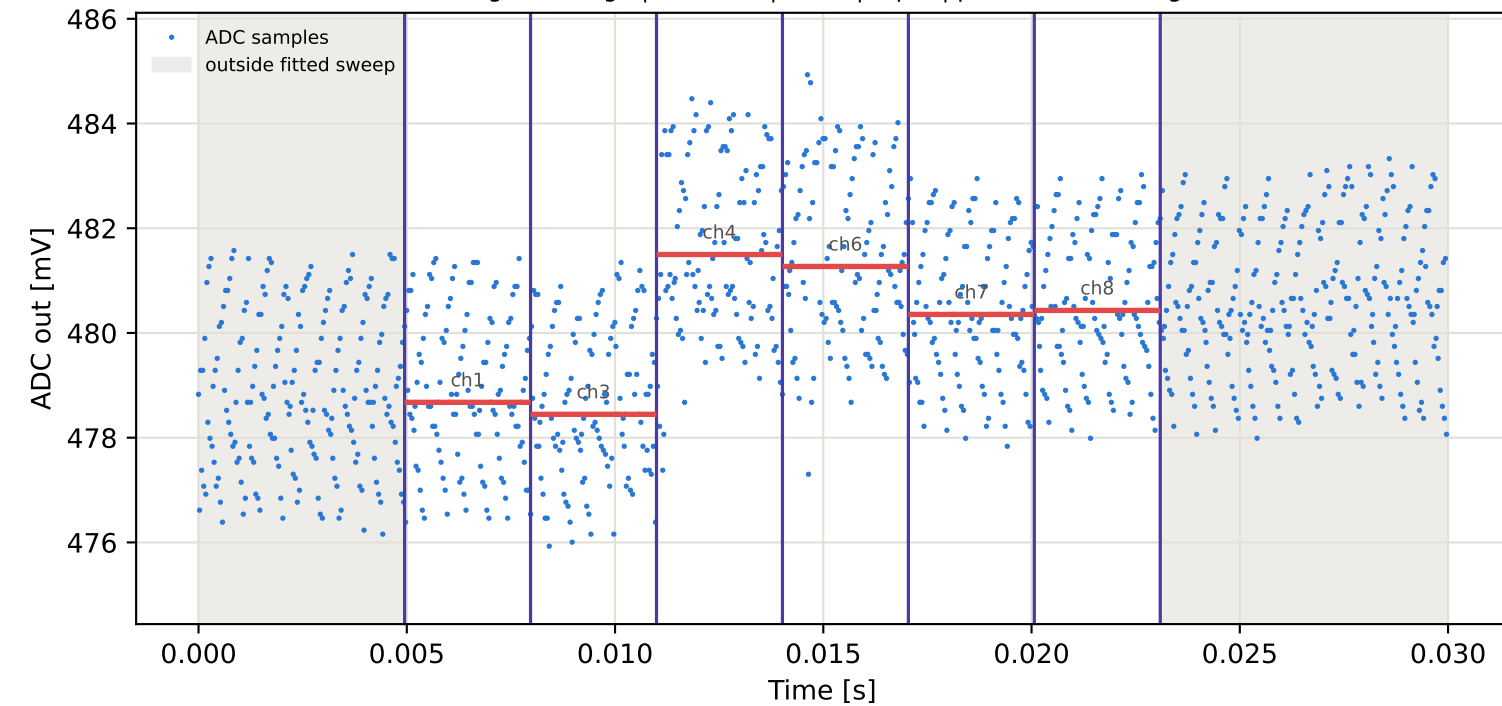
Tag15 &lt;- Tag1 | 845 MHz | run 0 | rep 1 | phase -127.49 deg
