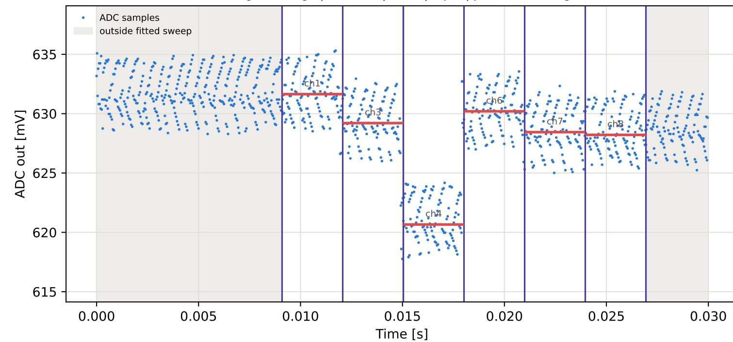
Tag16 &lt;- Tag4 | 845 MHz | run 0 | rep 1 | phase 154.78 deg
