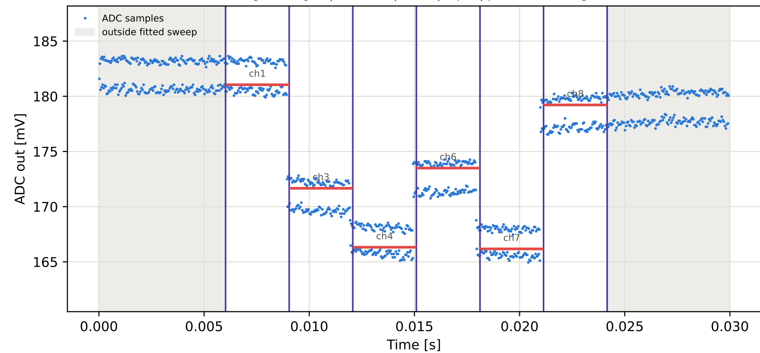
Tag4 &lt;- Tag16 | 845 MHz | run 0 | rep 1 | phase -90.20 deg
