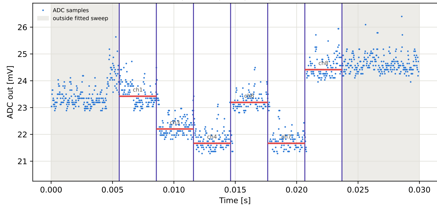
Tag9 &lt;- Tag2 | 805 MHz | run 0 | rep 1 | phase 122.87 deg
