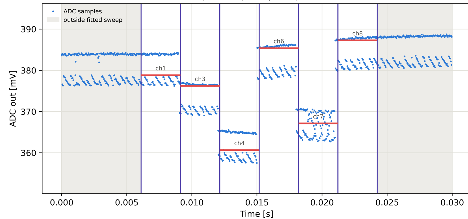
Tag10 &lt;- Tag8 | 965 MHz | run 0 | rep 1 | phase -42.59 deg
