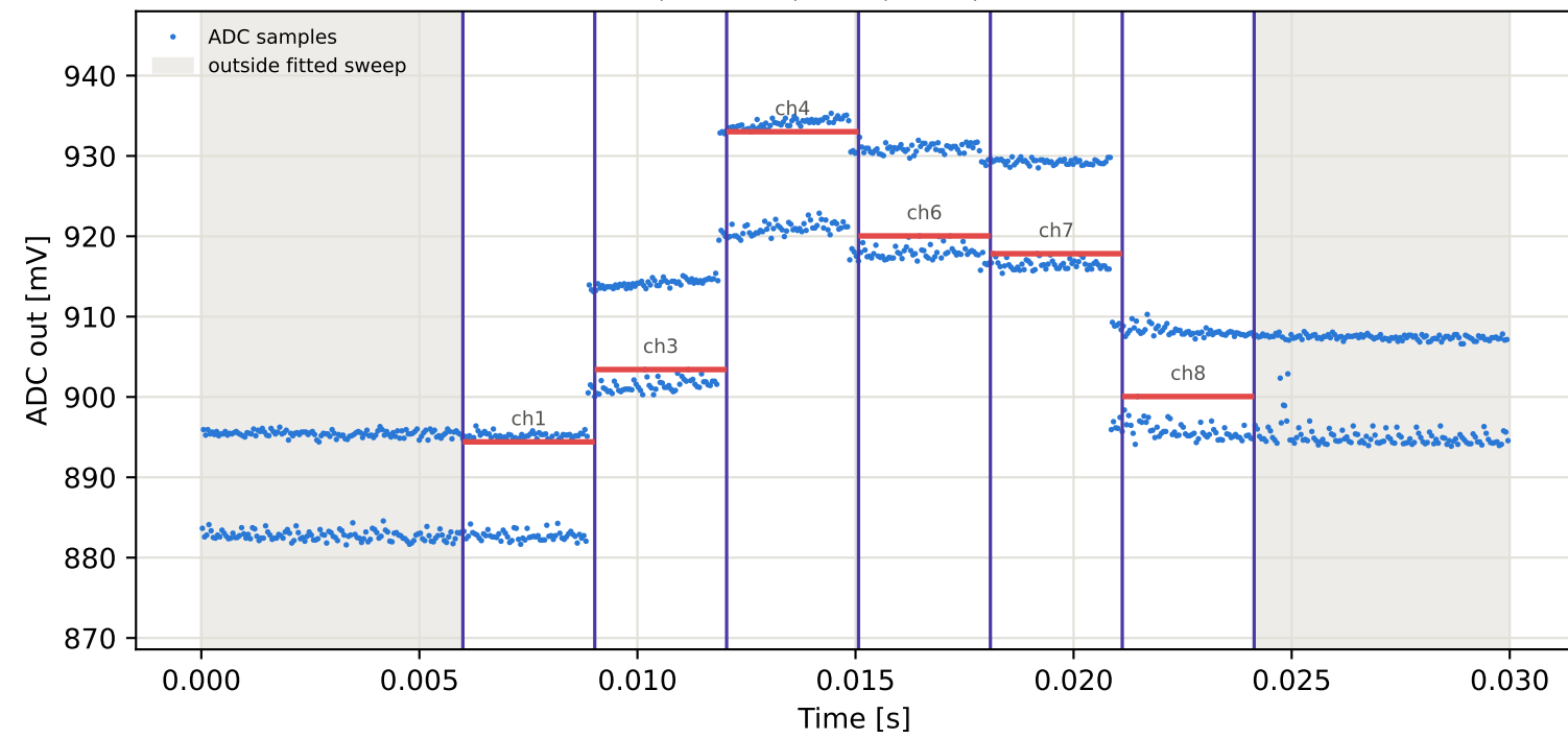
Tag3 &lt;- Tag9 | 875 MHz | run 0 | rep 1 | phase -110.36 deg
