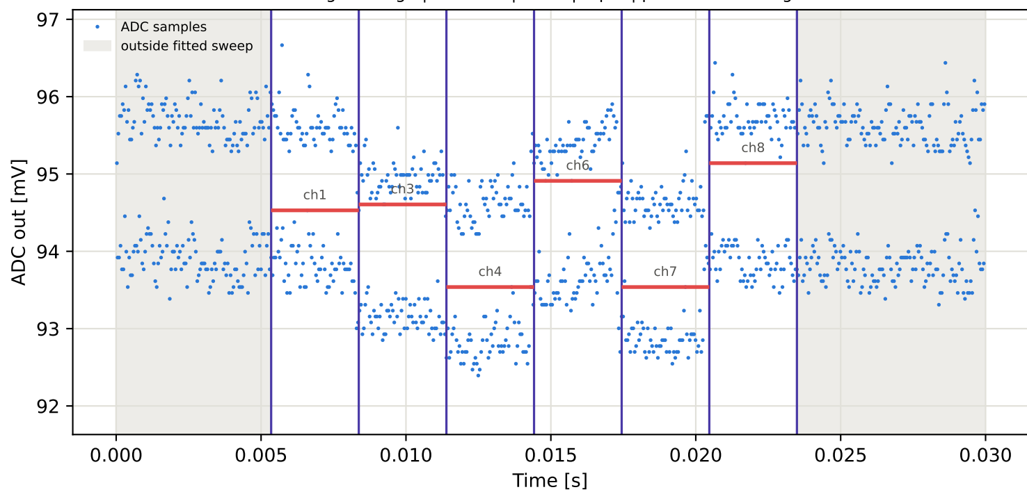
Tag3 &lt;- Tag10 | 805 MHz | run 0 | rep 1 | phase 50.95 deg
