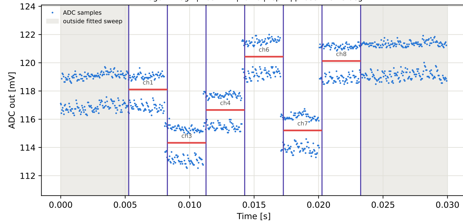
Tag6 &lt;- Tag9 | 785 MHz | run 0 | rep 1 | phase 72.20 deg
