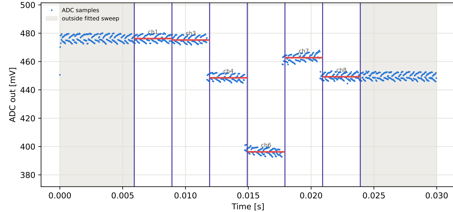
Tag5 &lt;- Tag3 | 935 MHz | run 0 | rep 1 | phase -170.43 deg
