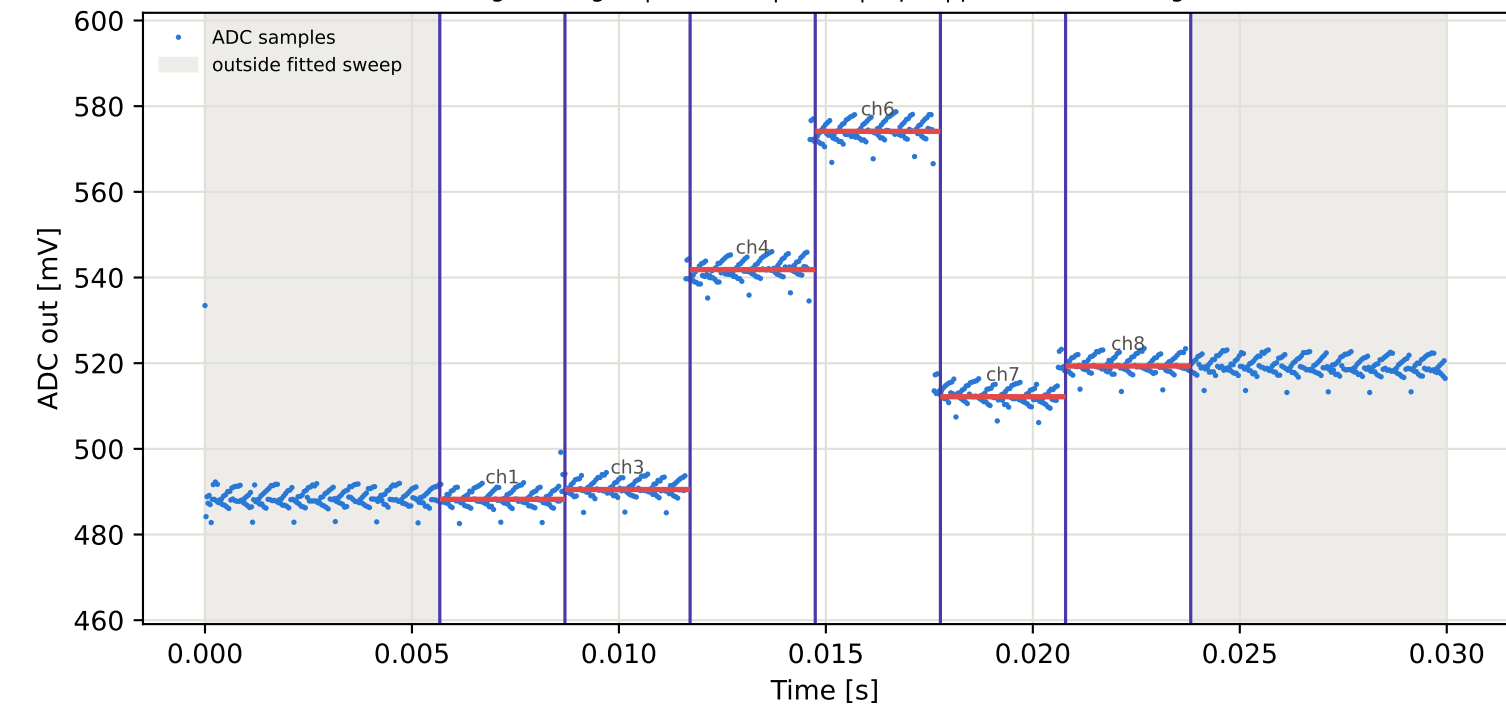
Tag8 &lt;- Tag16 | 955 MHz | run 0 | rep 1 | phase -148.20 deg
