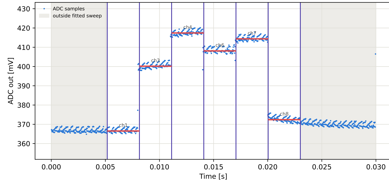
Tag9 &lt;- Tag7 | 875 MHz | run 0 | rep 1 | phase 120.92 deg
