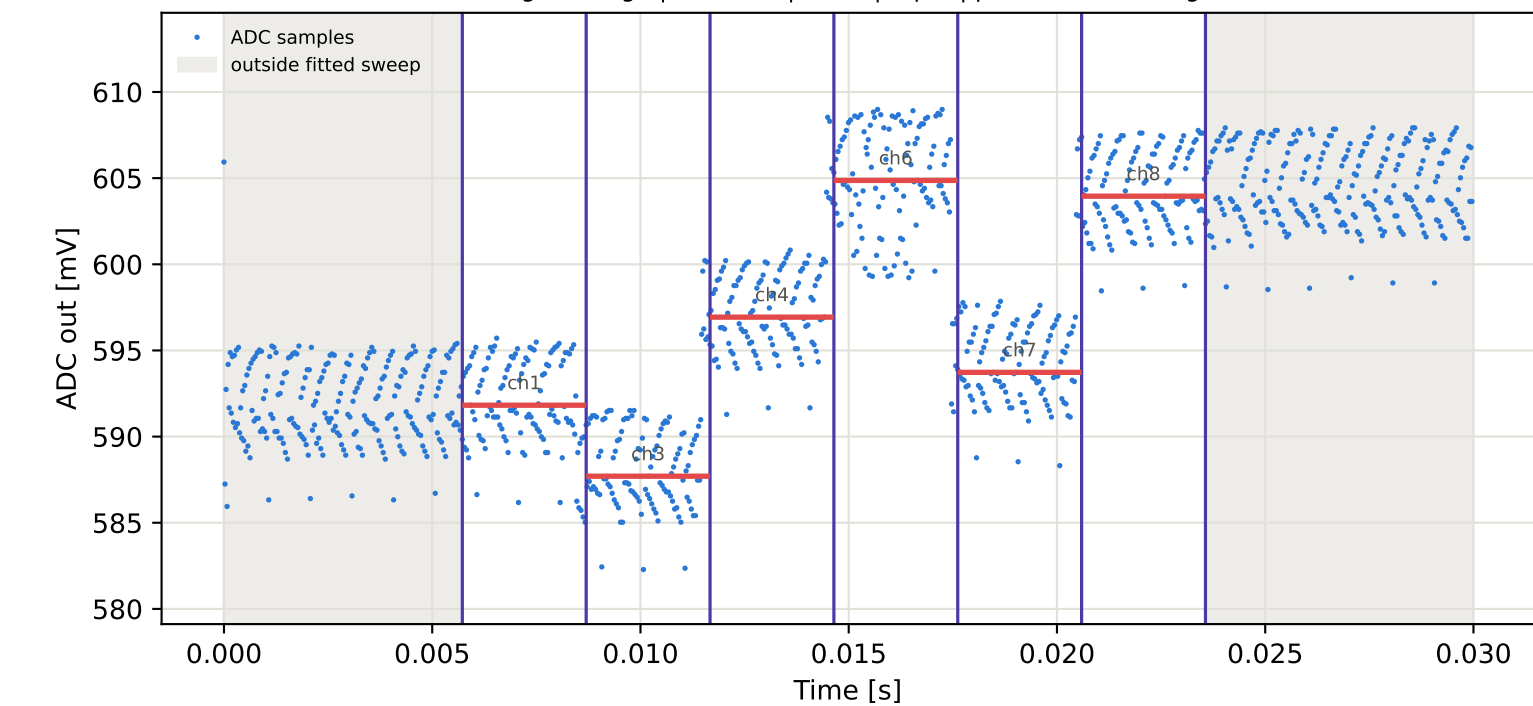
Tag8 &lt;- Tag6 | 855 MHz | run 0 | rep 1 | phase -159.93 deg
