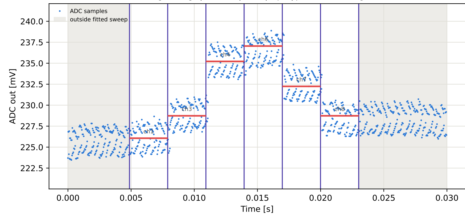
Tag6 &lt;- Tag9 | 925 MHz | run 0 | rep 1 | phase -161.67 deg
