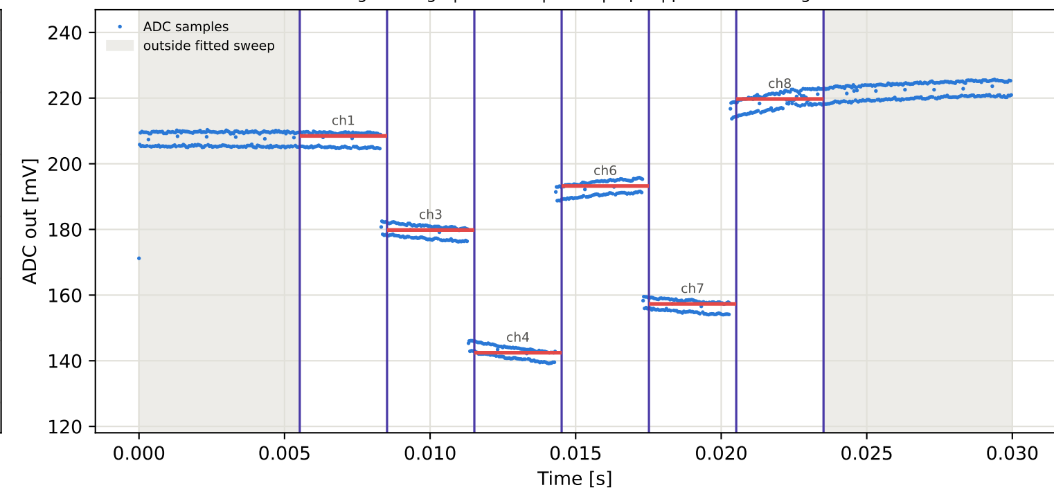
Tag7 &lt;- Tag4 | 905 MHz | run 0 | rep 1 | phase -166.56 deg
