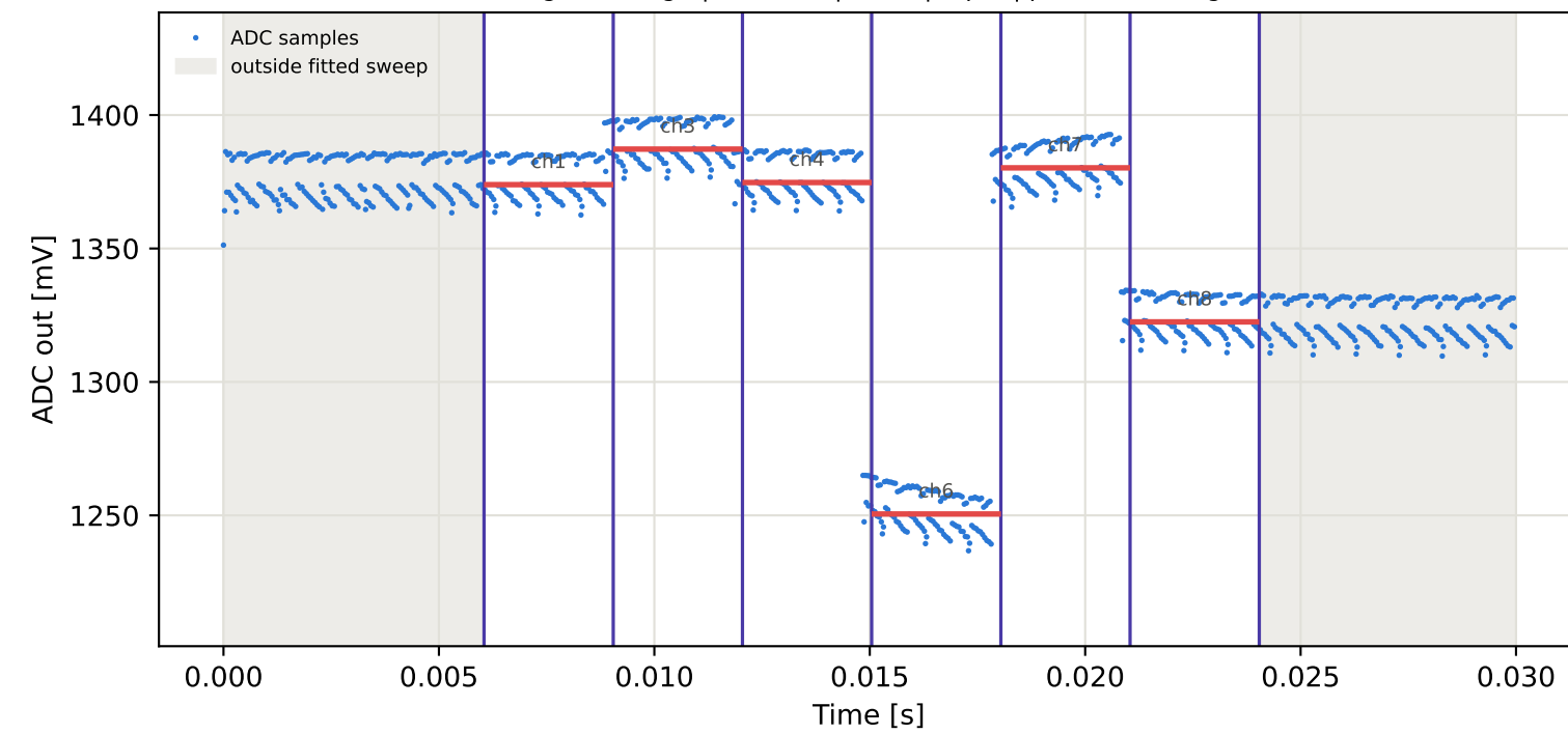
Tag2 &lt;- Tag1 | 925 MHz | run 0 | rep 1 | phase -37.01 deg
