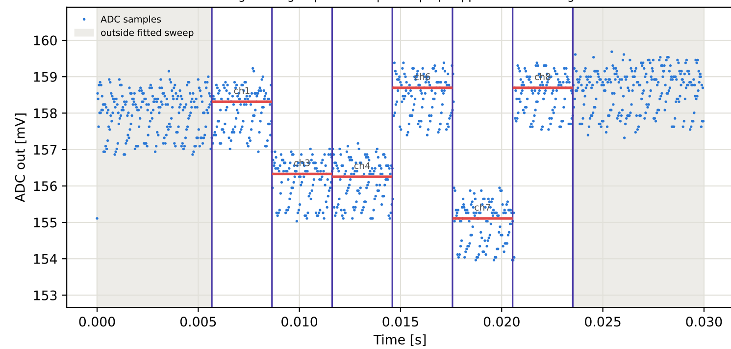
Tag7 &lt;- Tag15 | 785 MHz | run 0 | rep 1 | phase 149.86 deg
