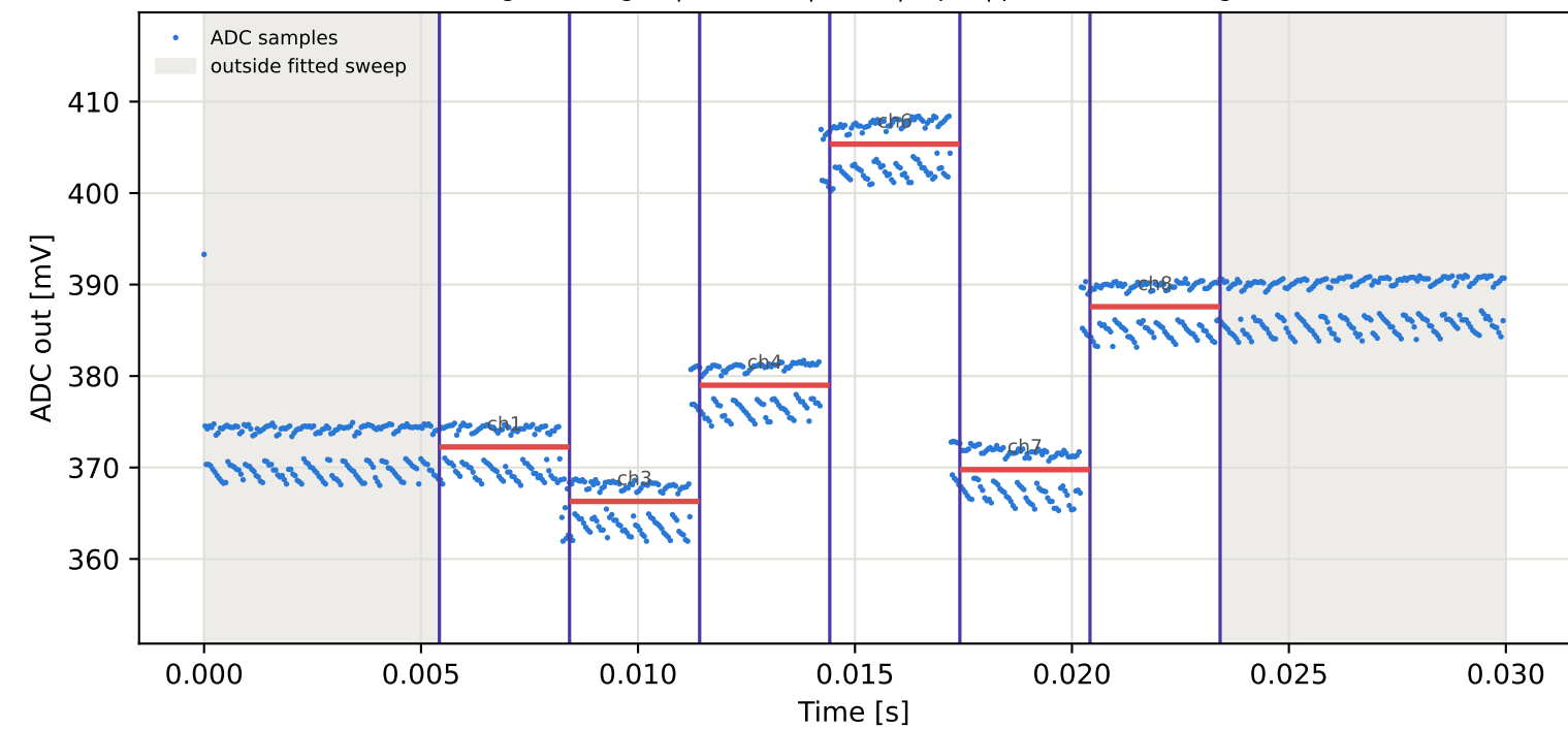
Tag10 &lt;- Tag3 | 965 MHz | run 0 | rep 1 | phase -122.60 deg
