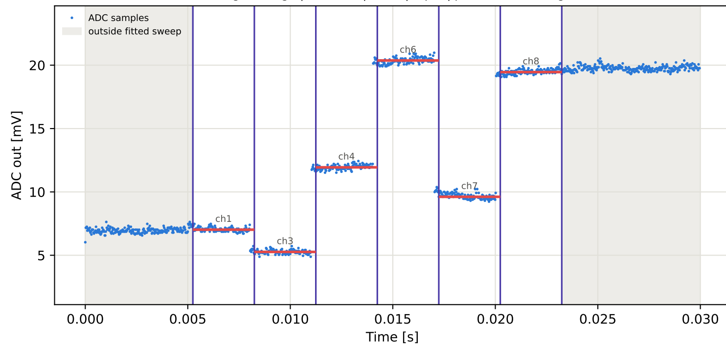
Tag4 &lt;- Tag7 | 865 MHz | run 0 | rep 1 | phase -97.65 deg
