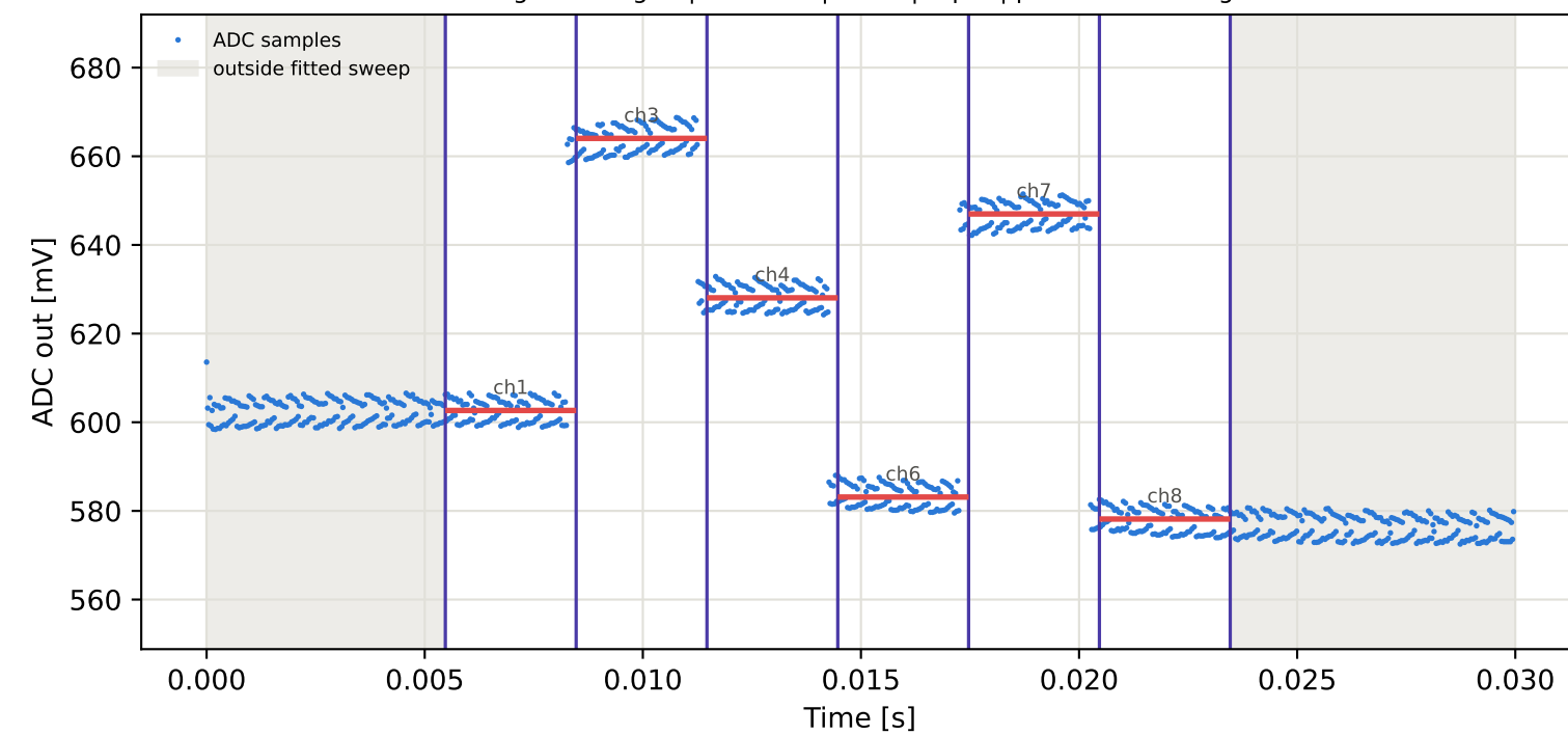
Tag15 &lt;- Tag3 | 835 MHz | run 0 | rep 1 | phase -148.24 deg
