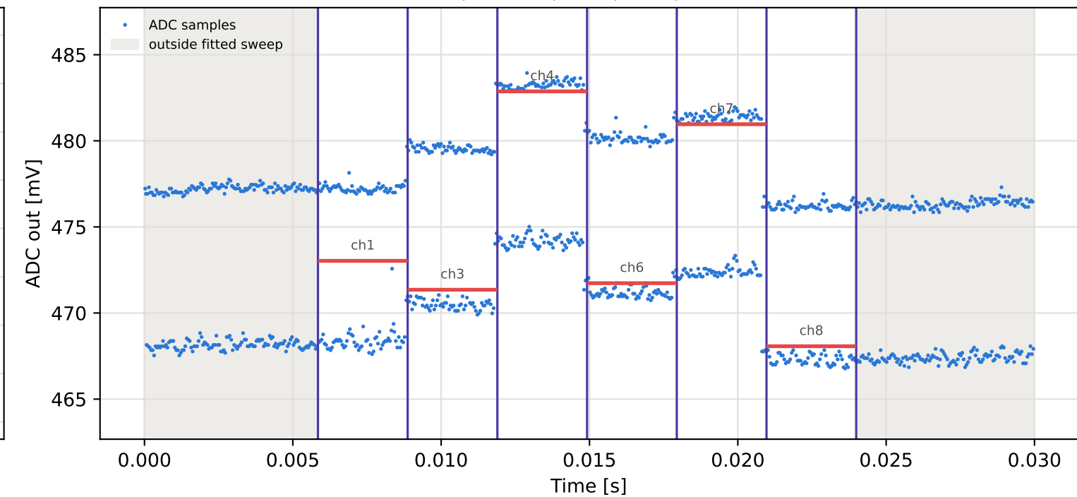
Tag9 &lt;- Tag2 | 975 MHz | run 0 | rep 1 | phase -91.71 deg
