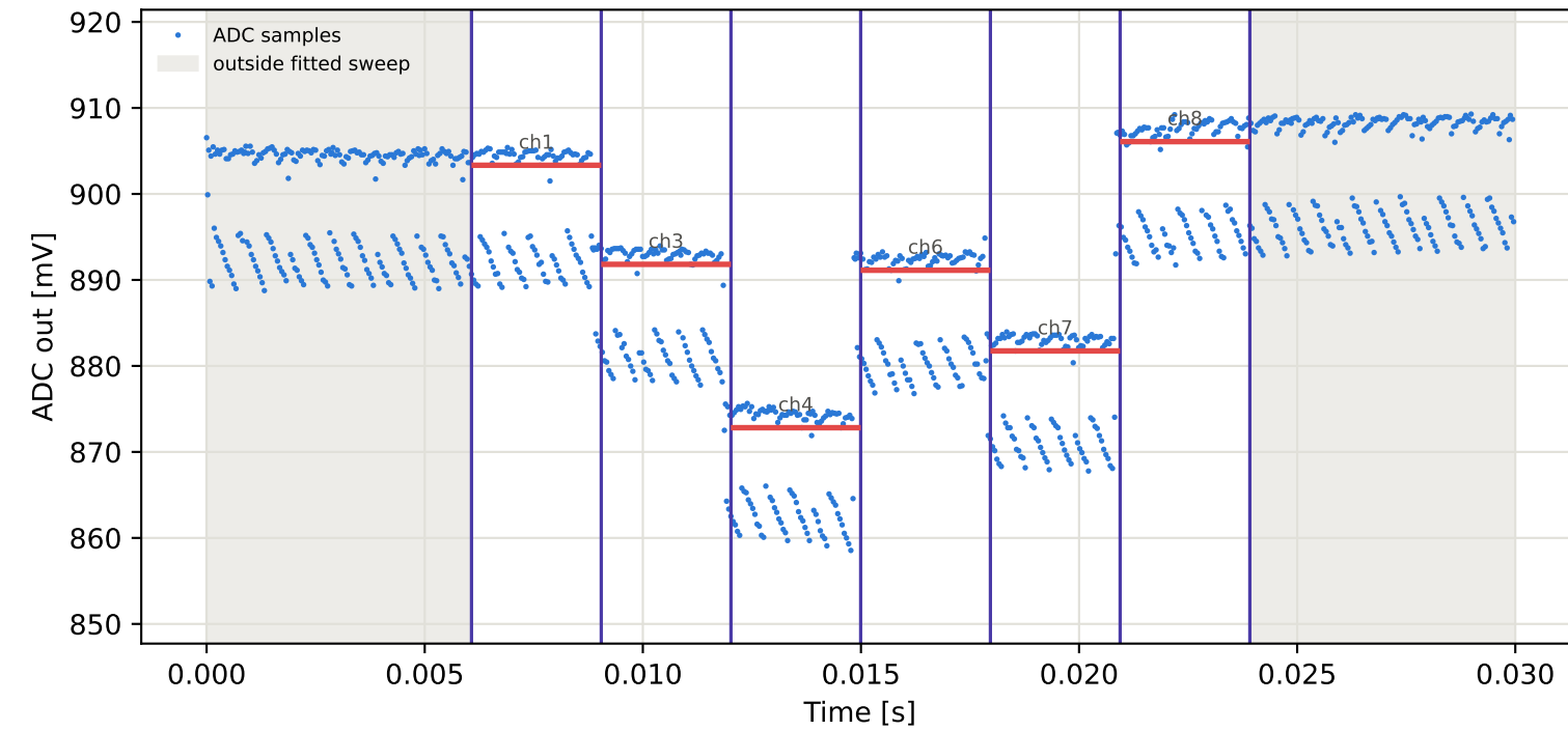
Tag16 &lt;- Tag6 | 945 MHz | run 0 | rep 1 | phase 38.59 deg
