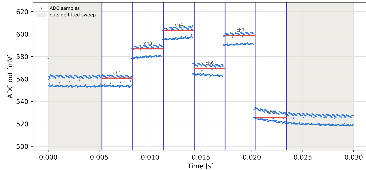
Tag6 &lt;- Tag1 | 905 MHz | run 0 | rep 1 | phase -18.50 deg
