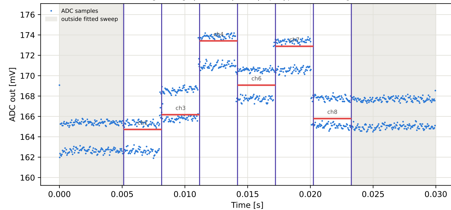
Tag4 &lt;- Tag15 | 845 MHz | run 0 | rep 1 | phase -105.69 deg
