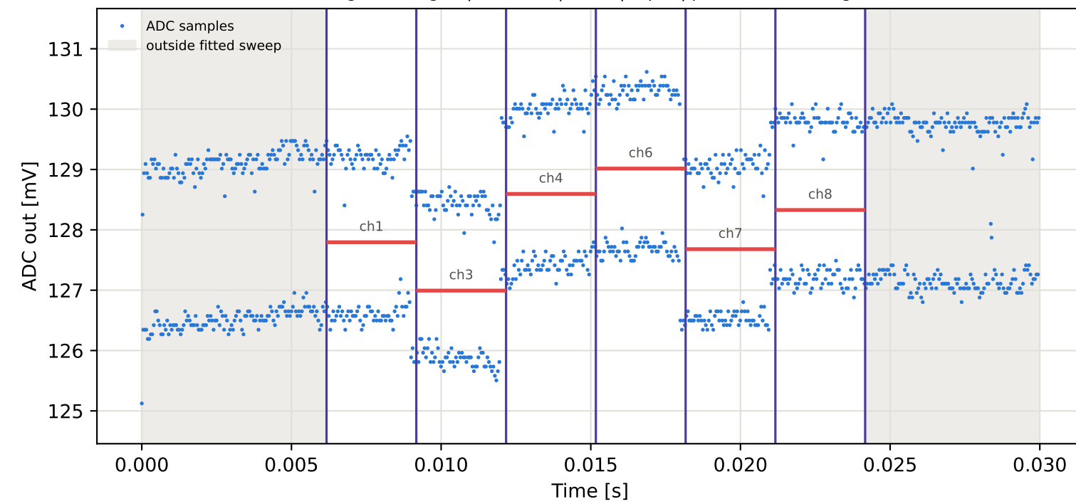
Tag10 &lt;- Tag2 | 775 MHz | run 0 | rep 1 | phase -54.72 deg
