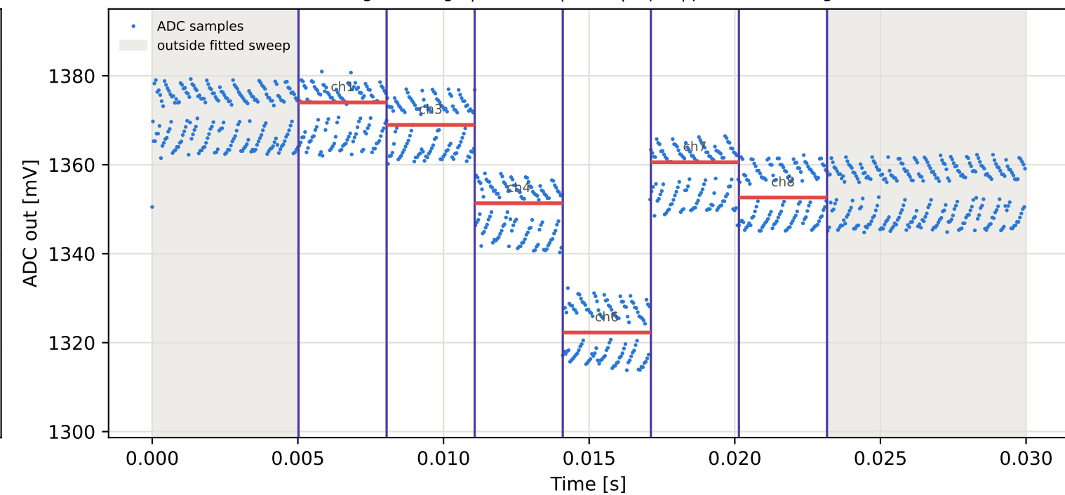
Tag16 &lt;- Tag7 | 925 MHz | run 0 | rep 1 | phase 26.07 deg
