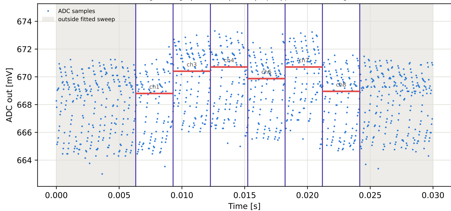
Tag7 &lt;- Tag6 | 835 MHz | run 0 | rep 1 | phase -93.68 deg
