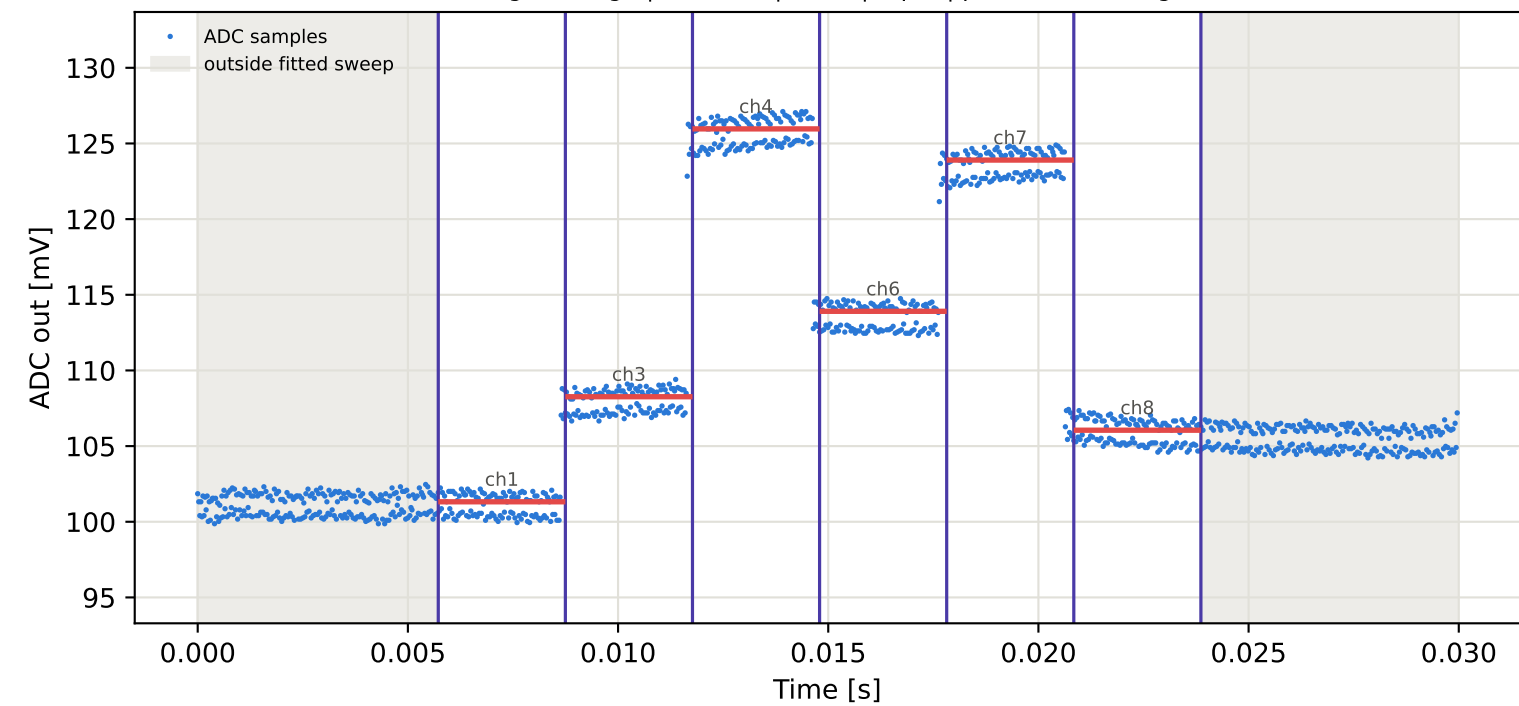
Tag3 &lt;- Tag7 | 795 MHz | run 0 | rep 1 | phase 131.36 deg
