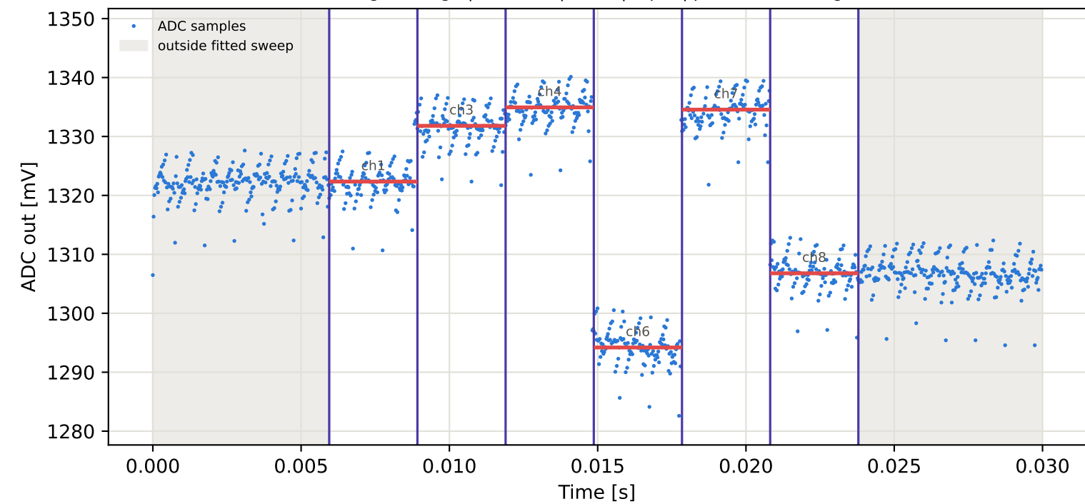
Tag7 &lt;- Tag4 | 885 MHz | run 0 | rep 1 | phase 153.54 deg
