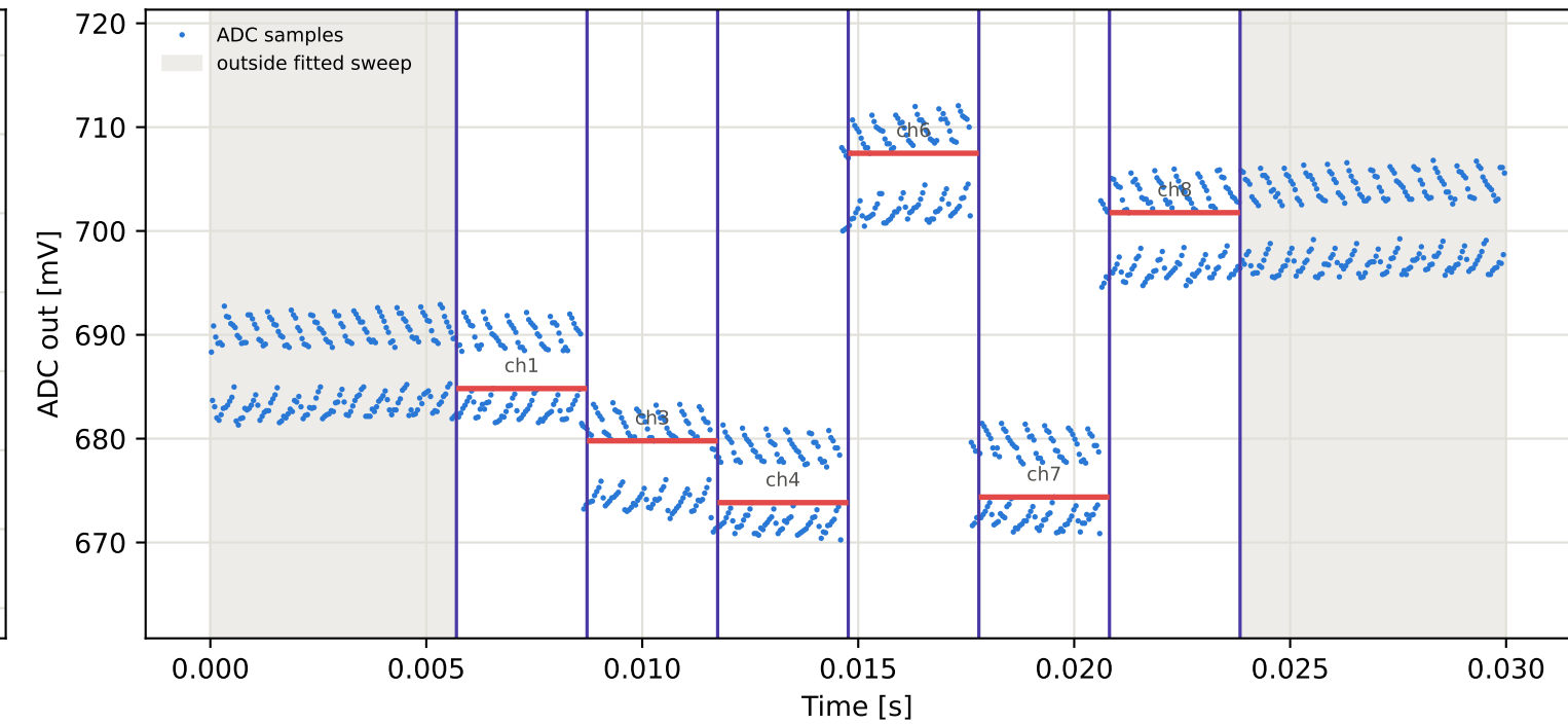
Tag9 &lt;- Tag2 | 935 MHz | run 0 | rep 1 | phase -86.45 deg
