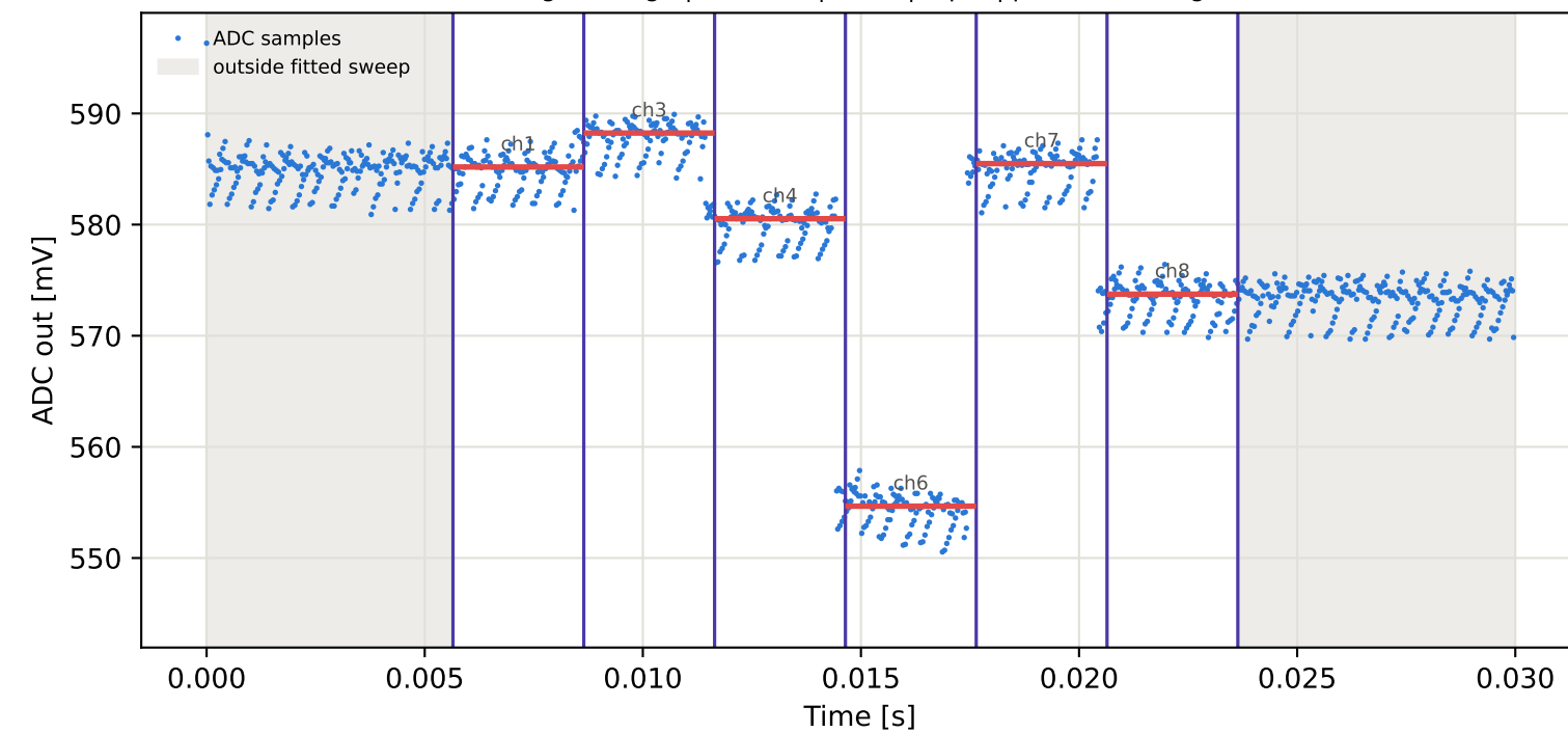
Tag6 &lt;- Tag1 | 945 MHz | run 0 | rep 1 | phase 131.88 deg
