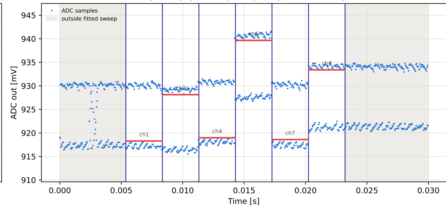
Tag7 &lt;- Tag4 | 855 MHz | run 0 | rep 1 | phase 12.14 deg
