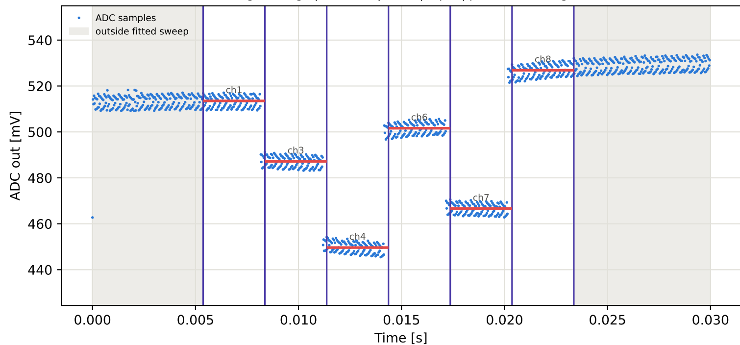
Tag3 &lt;- Tag7 | 935 MHz | run 0 | rep 1 | phase -170.28 deg
