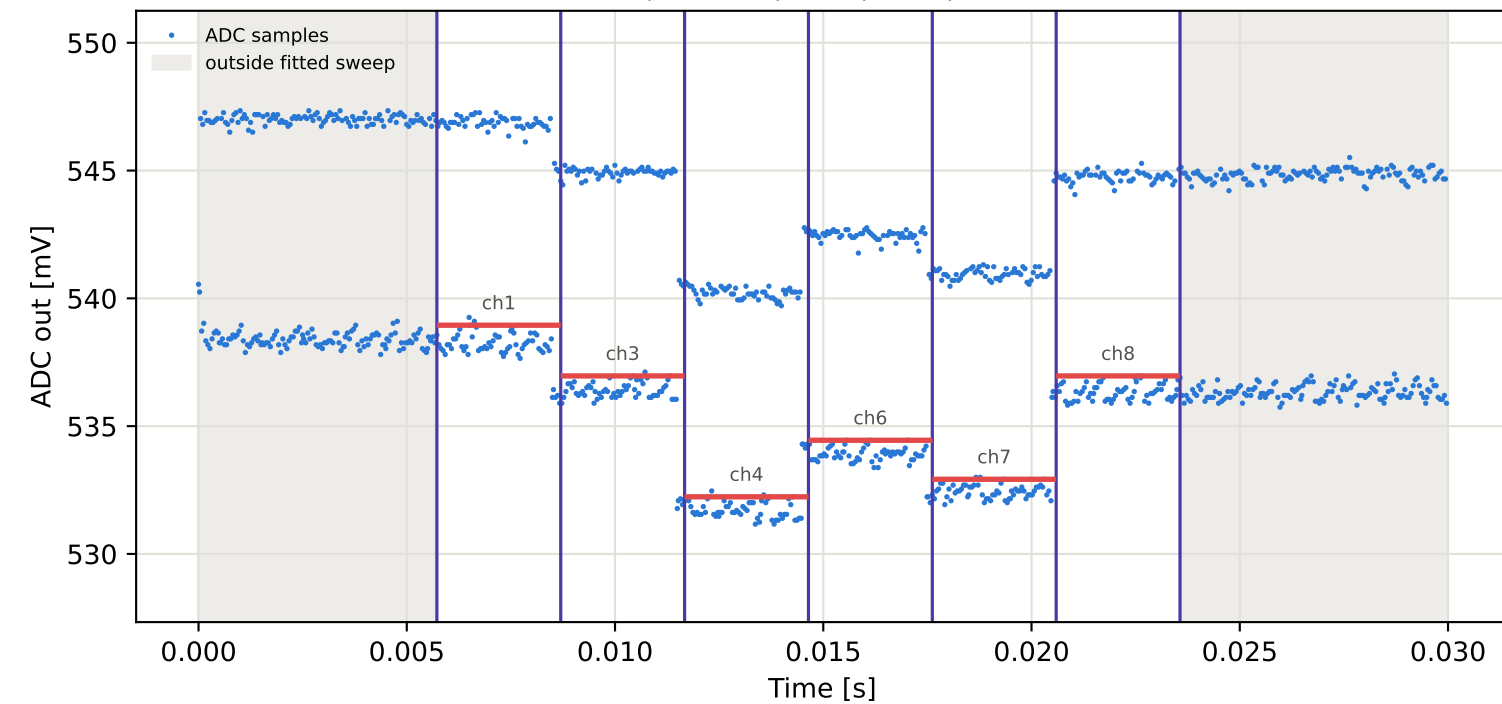
Tag7 &lt;- Tag5 | 825 MHz | run 0 | rep 1 | phase 78.25 deg
