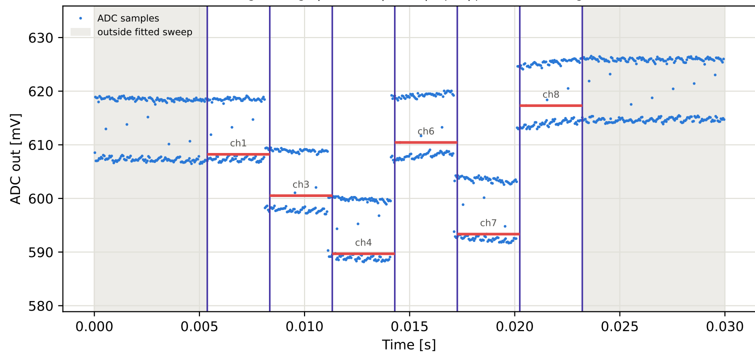
Tag8 &lt;- Tag10 | 935 MHz | run 0 | rep 1 | phase -43.09 deg
