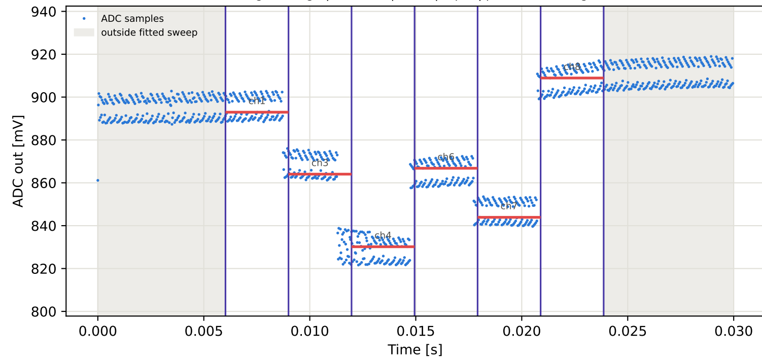
Tag3 &lt;- Tag7 | 925 MHz | run 0 | rep 1 | phase -169.38 deg
