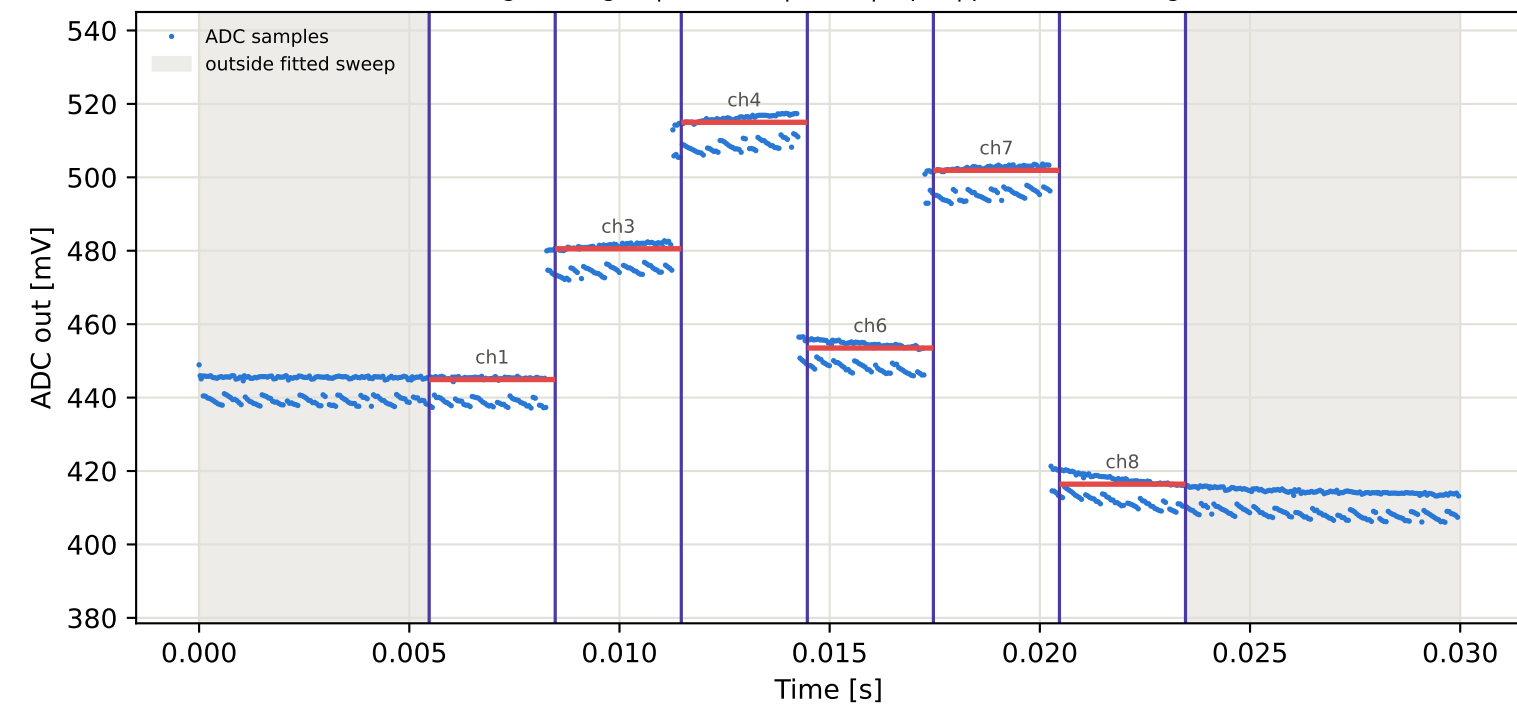
Tag7 &lt;- Tag3 | 925 MHz | run 0 | rep 1 | phase -112.38 deg
