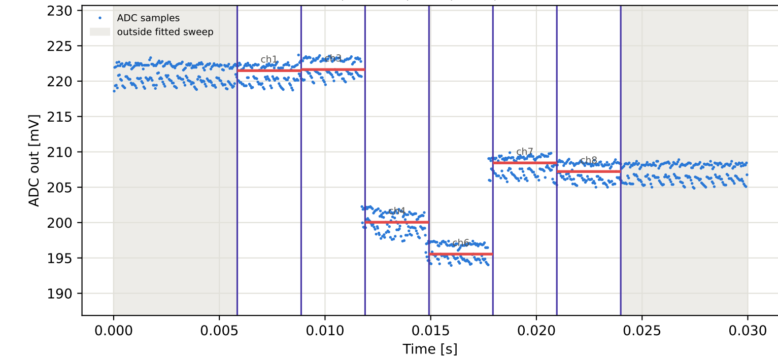
Tag9 &lt;- Tag7 | 845 MHz | run 0 | rep 1 | phase 46.84 deg
