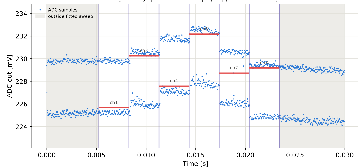
Tag1 &lt;- Tag4 | 985 MHz | run 0 | rep 1 | phase -68.39 deg
