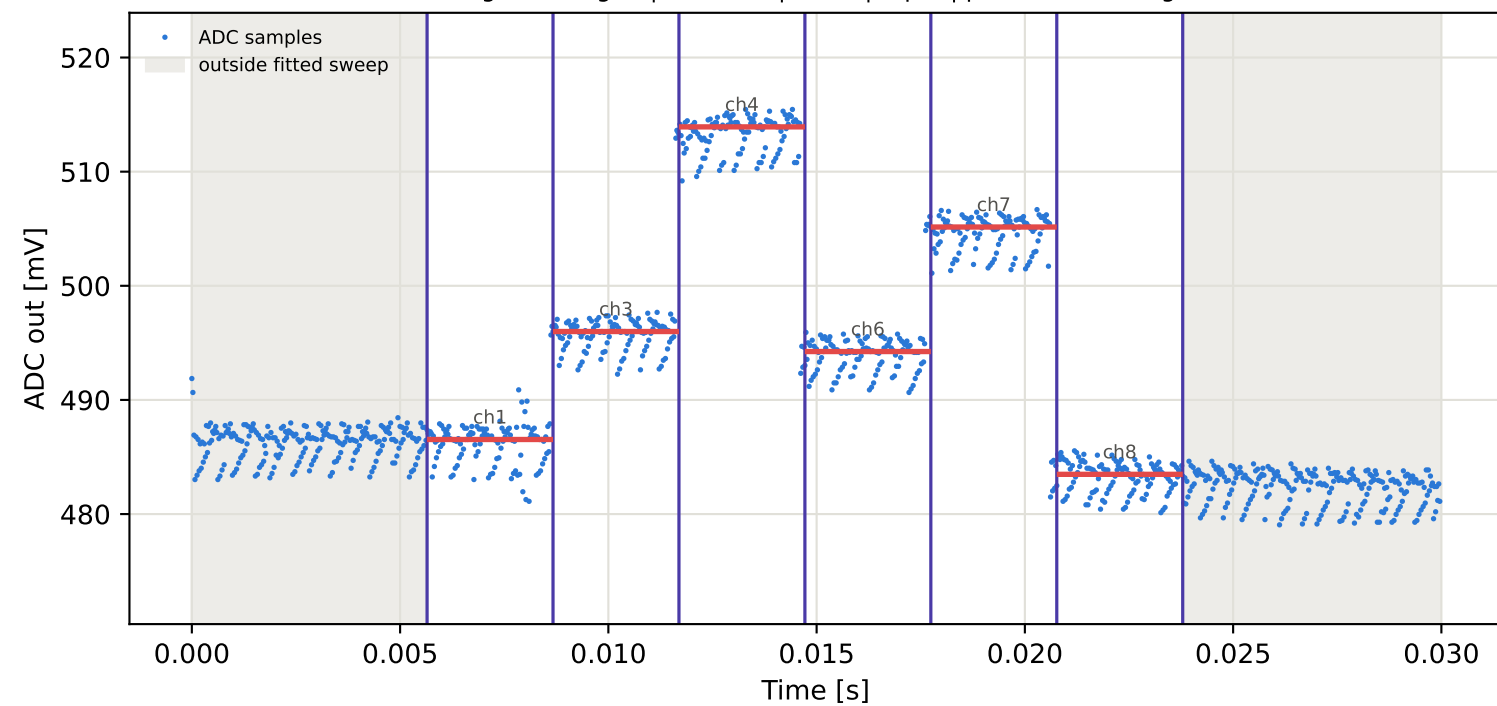
Tag15 &lt;- Tag10 | 945 MHz | run 0 | rep 1 | phase -92.66 deg
