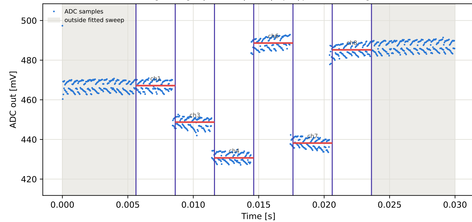
Tag5 &lt;- Tag16 | 935 MHz | run 0 | rep 1 | phase 22.11 deg
