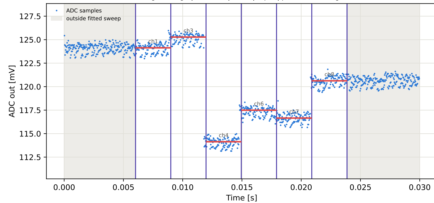
Tag7 &lt;- Tag10 | 785 MHz | run 0 | rep 1 | phase 32.35 deg
