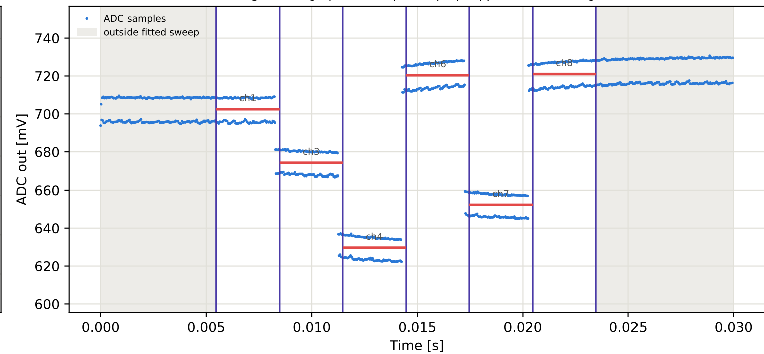
Tag16 &lt;- Tag5 | 975 MHz | run 0 | rep 1 | phase -168.36 deg
