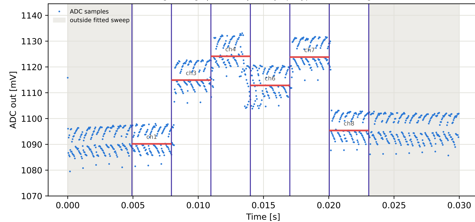
Tag8 &lt;- Tag1 | 865 MHz | run 0 | rep 1 | phase -128.88 deg
