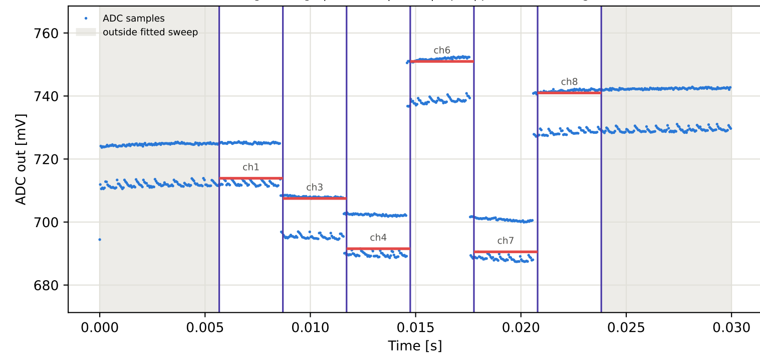
Tag8 &lt;- Tag1 | 995 MHz | run 0 | rep 1 | phase -134.71 deg
