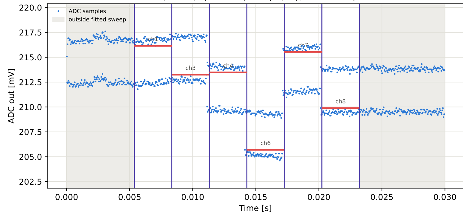
Tag10 &lt;- Tag1 | 955 MHz | run 0 | rep 1 | phase 174.13 deg
