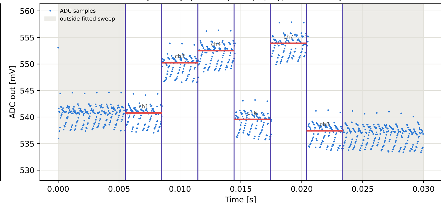
Tag16 &lt;- Tag7 | 825 MHz | run 0 | rep 1 | phase -44.40 deg
