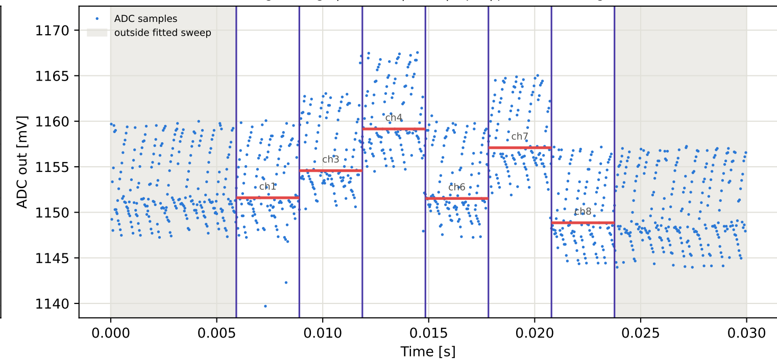
Tag7 &lt;- Tag4 | 975 MHz | run 0 | rep 1 | phase 158.45 deg
