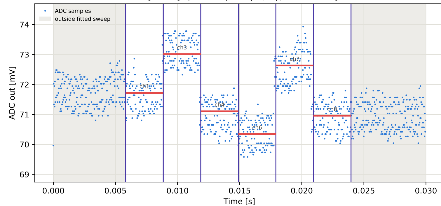
Tag6 &lt;- Tag4 | 775 MHz | run 0 | rep 1 | phase 26.07 deg
