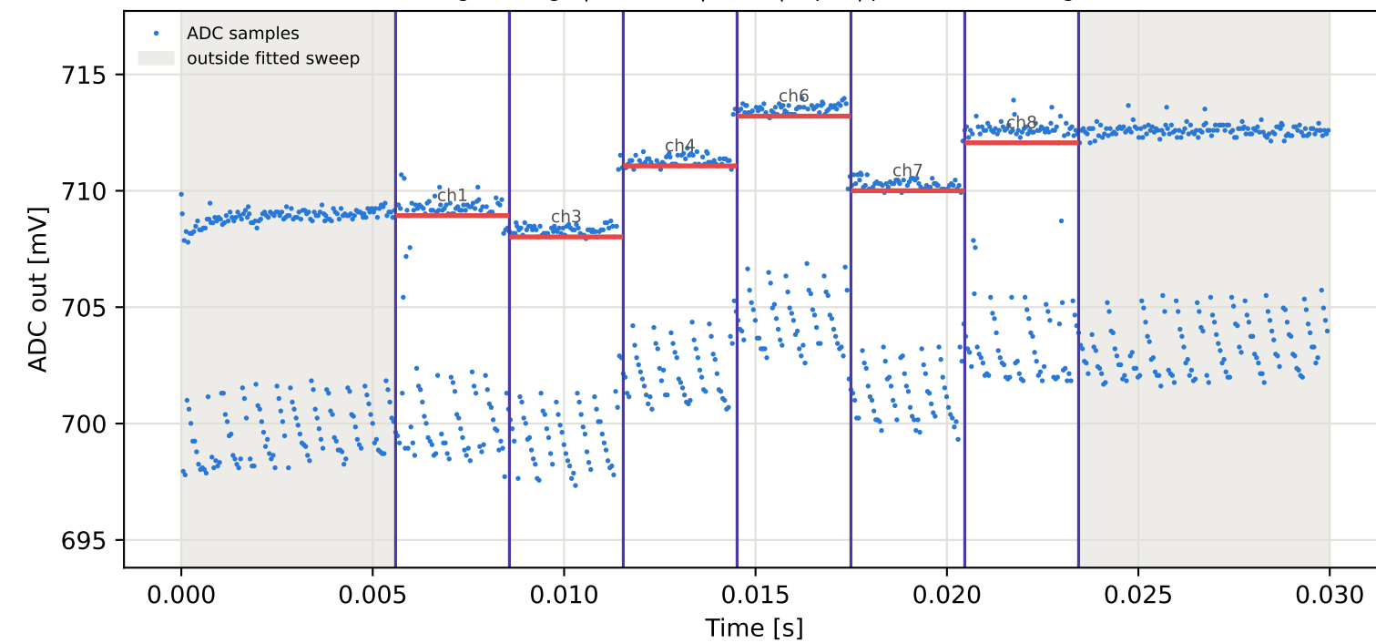
Tag9 &lt;- Tag10 | 845 MHz | run 0 | rep 1 | phase 40.04 deg
