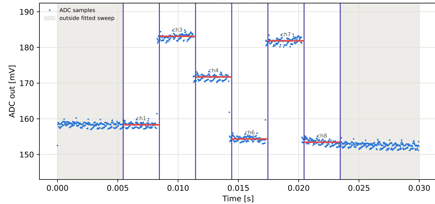
Tag5 &lt;- Tag3 | 805 MHz | run 0 | rep 1 | phase -16.10 deg
