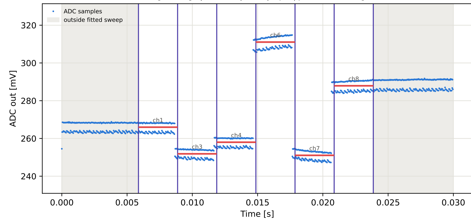
Tag1 &lt;- Tag7 | 965 MHz | run 0 | rep 1 | phase 109.08 deg
