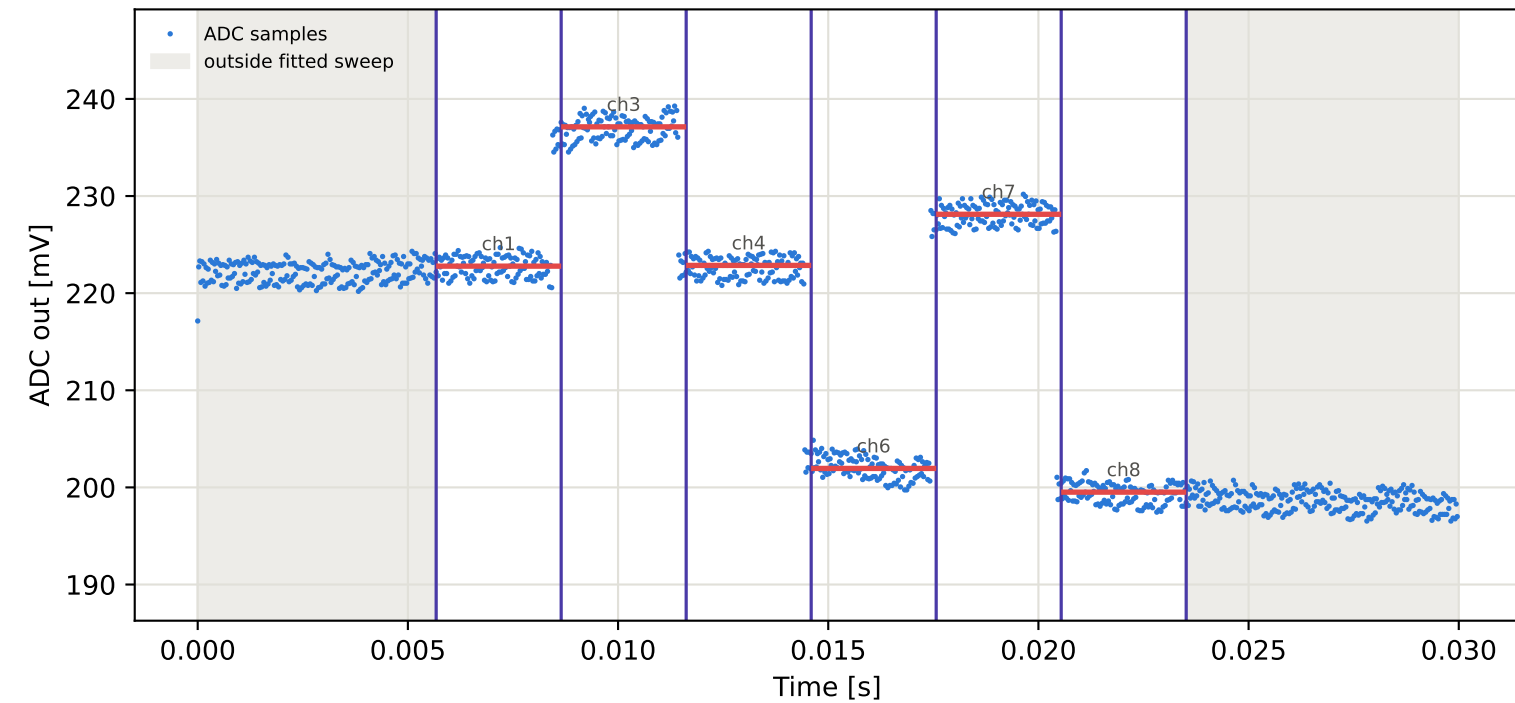
Tag9 &lt;- Tag8 | 855 MHz | run 0 | rep 1 | phase 172.47 deg
