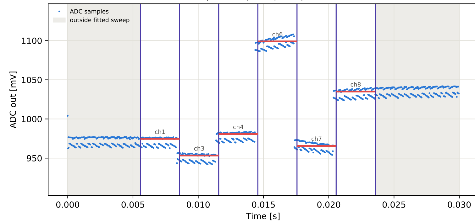
Tag16 &lt;- Tag4 | 905 MHz | run 0 | rep 1 | phase -110.77 deg
