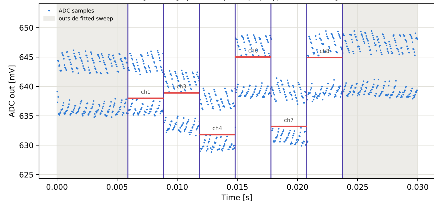
Tag10 &lt;- Tag4 | 945 MHz | run 0 | rep 1 | phase 127.70 deg
