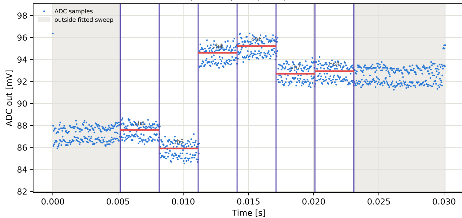
Tag2 &lt;- Tag5 | 825 MHz | run 0 | rep 1 | phase -169.99 deg
