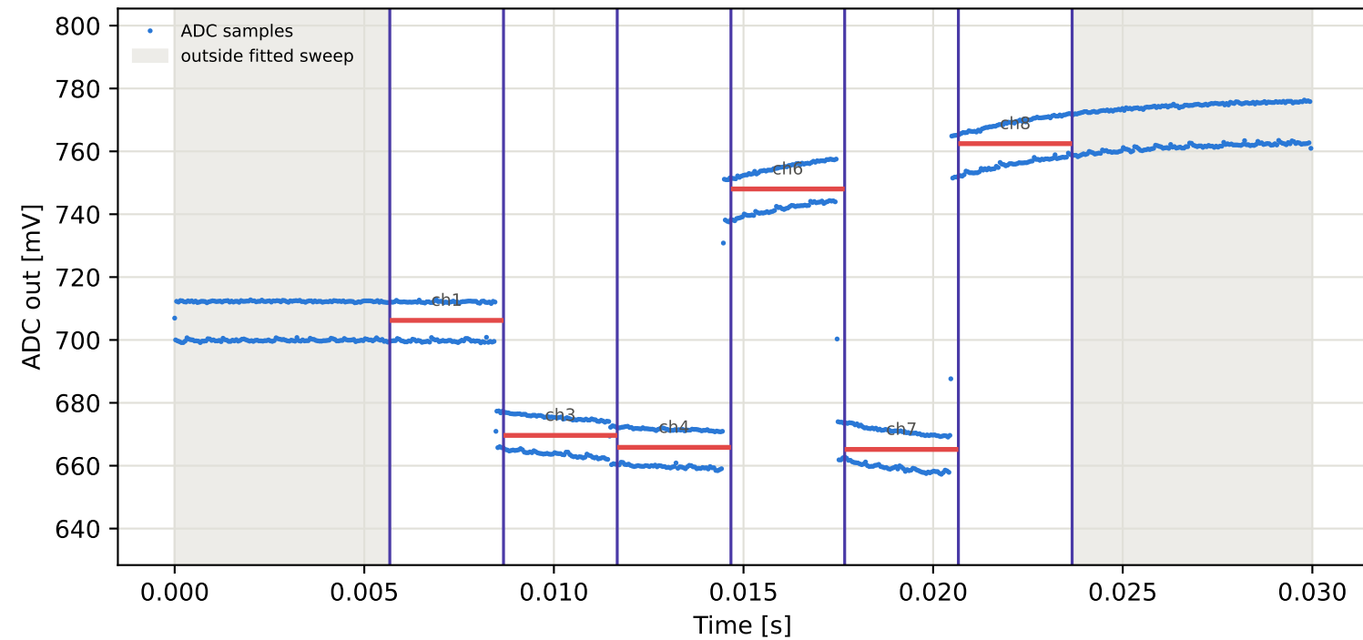
Tag6 &lt;- Tag5 | 895 MHz | run 0 | rep 1 | phase -87.53 deg
