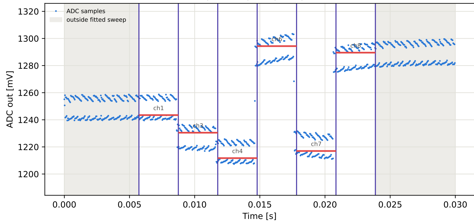
Tag15 &lt;- Tag10 | 915 MHz | run 0 | rep 1 | phase 150.59 deg
