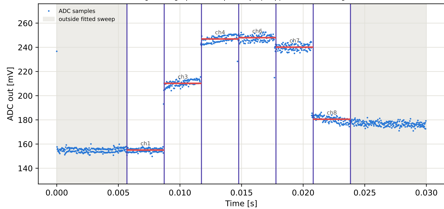
Tag9 &lt;- Tag8 | 885 MHz | run 0 | rep 1 | phase -113.42 deg
