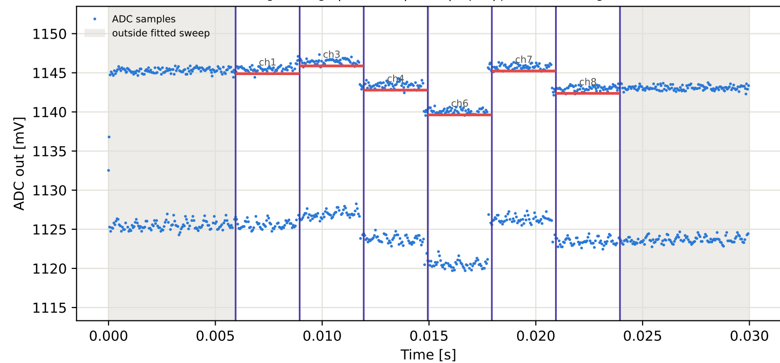
Tag7 &lt;- Tag15 | 985 MHz | run 0 | rep 1 | phase -166.31 deg
