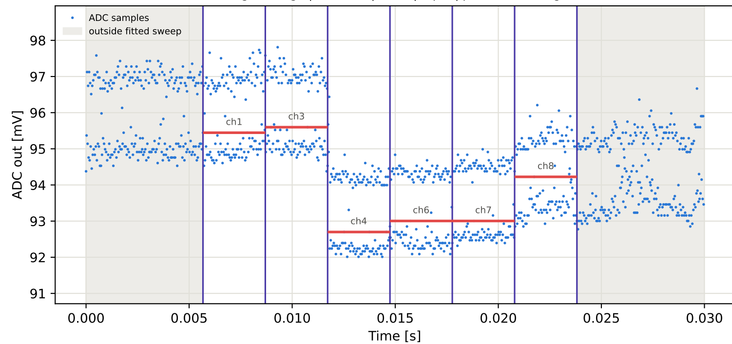
Tag2 &lt;- Tag6 | 825 MHz | run 0 | rep 1 | phase -147.51 deg
