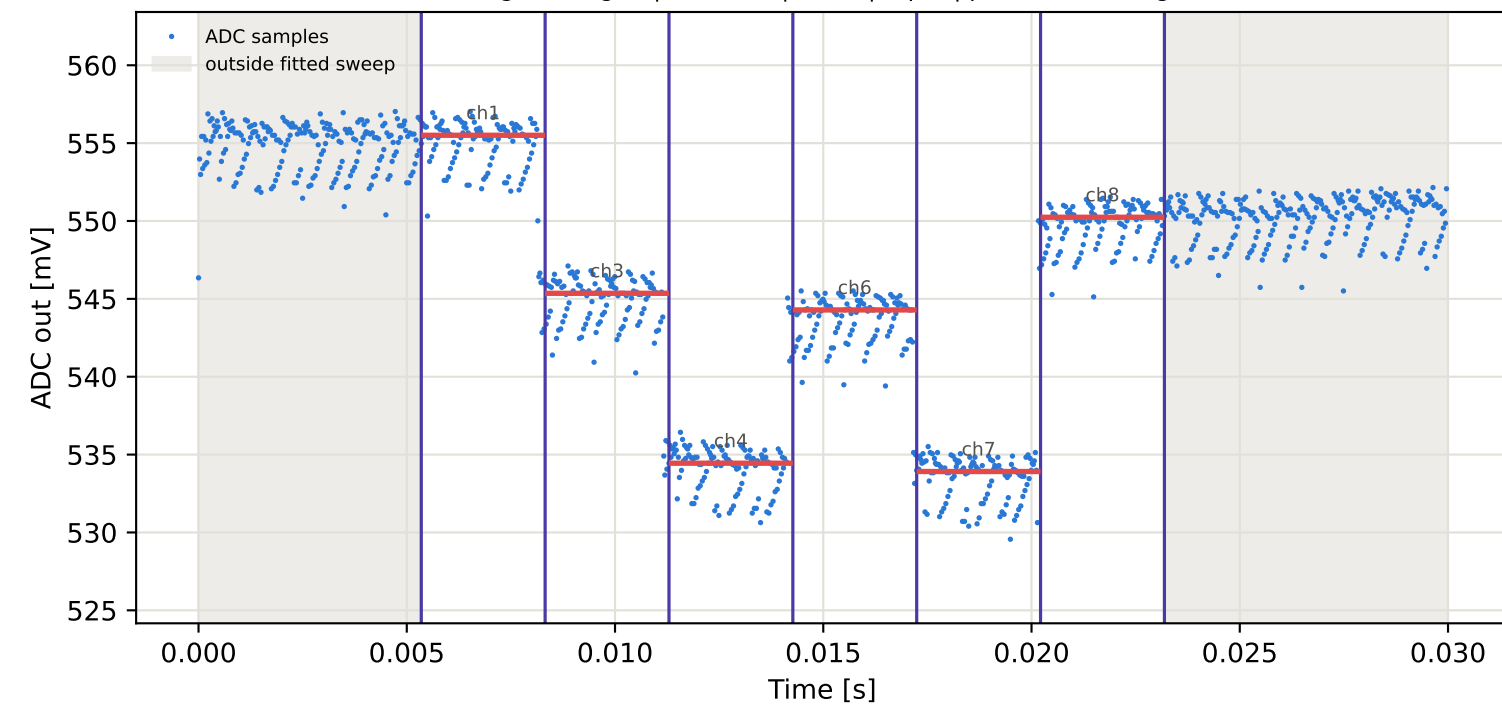
Tag7 &lt;- Tag3 | 825 MHz | run 0 | rep 1 | phase 31.72 deg
