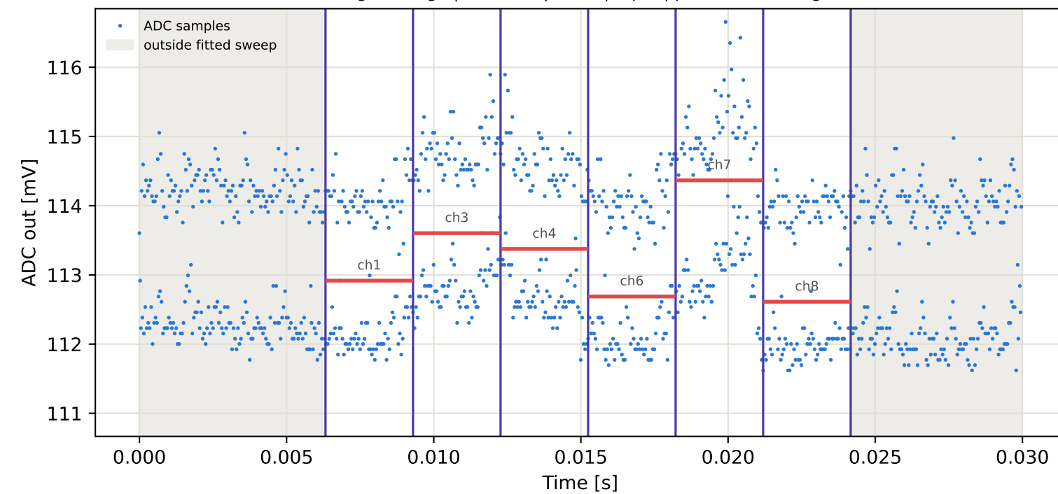
Tag2 &lt;- Tag15 | 835 MHz | run 0 | rep 1 | phase 115.63 deg
