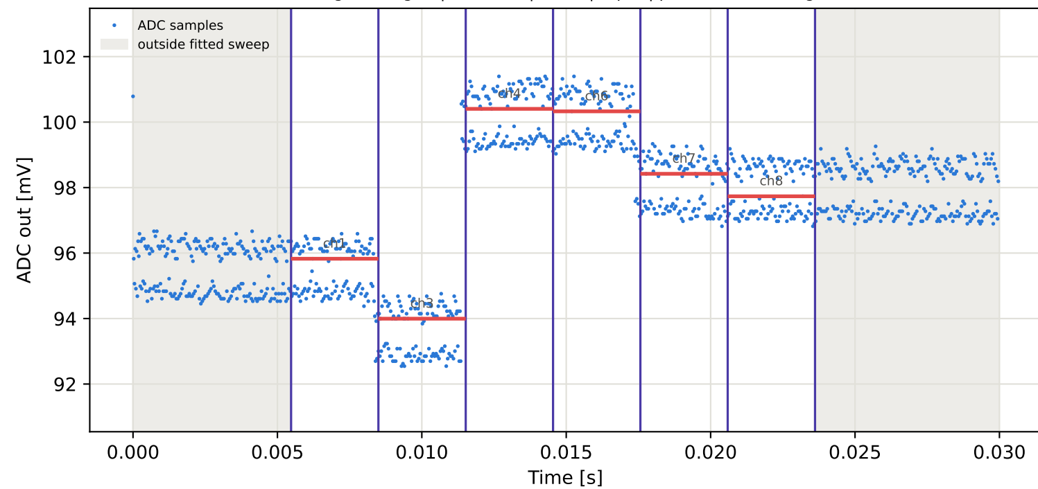
Tag6 &lt;- Tag3 | 795 MHz | run 0 | rep 1 | phase 11.04 deg
