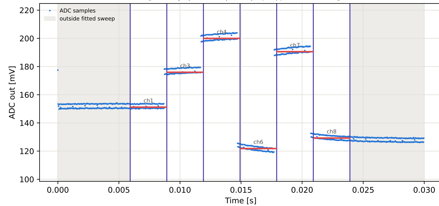
Tag4 &lt;- Tag7 | 965 MHz | run 0 | rep 1 | phase 98.32 deg
