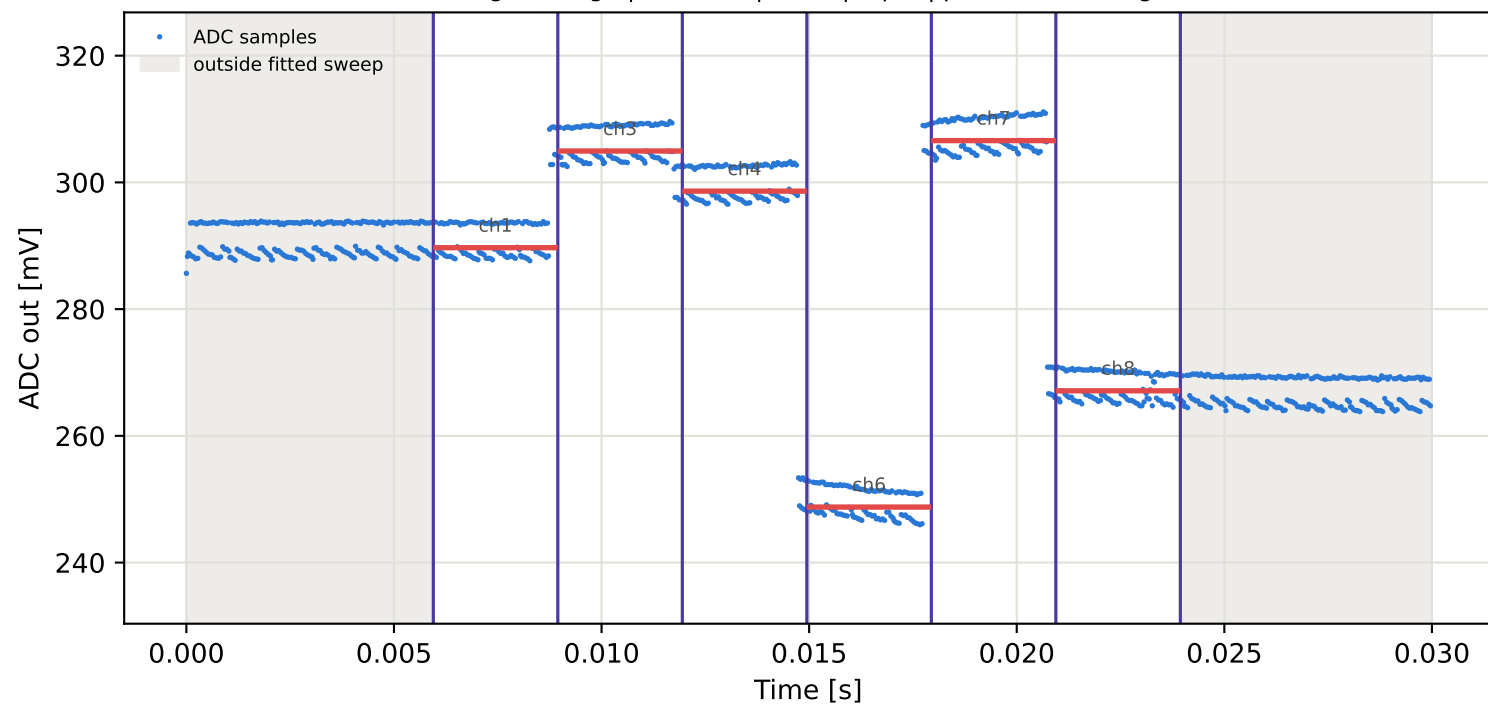
Tag7 &lt;- Tag10 | 975 MHz | run 0 | rep 1 | phase 79.59 deg
