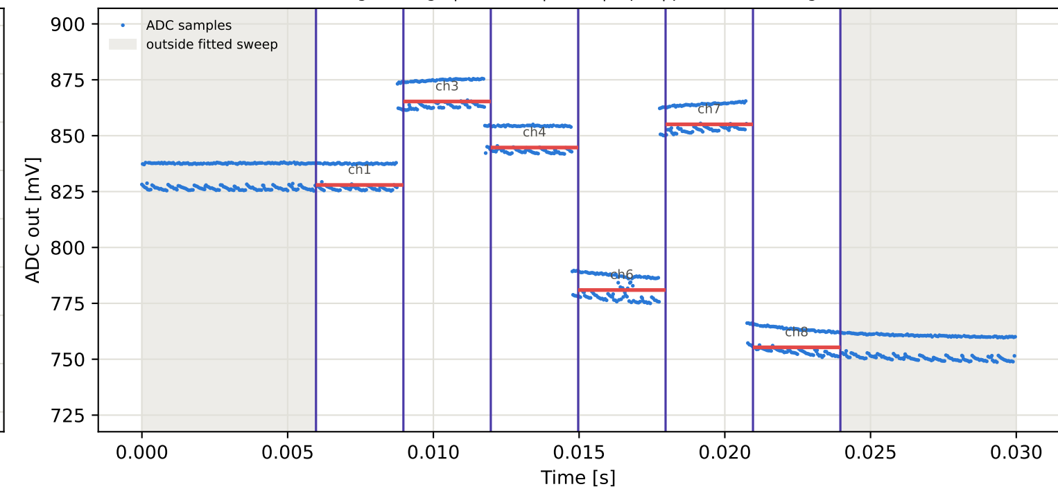
Tag8 &lt;- Tag5 | 865 MHz | run 0 | rep 1 | phase 119.59 deg
