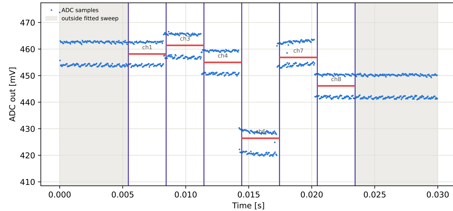
Tag6 &lt;- Tag1 | 935 MHz | run 0 | rep 1 | phase 134.98 deg
