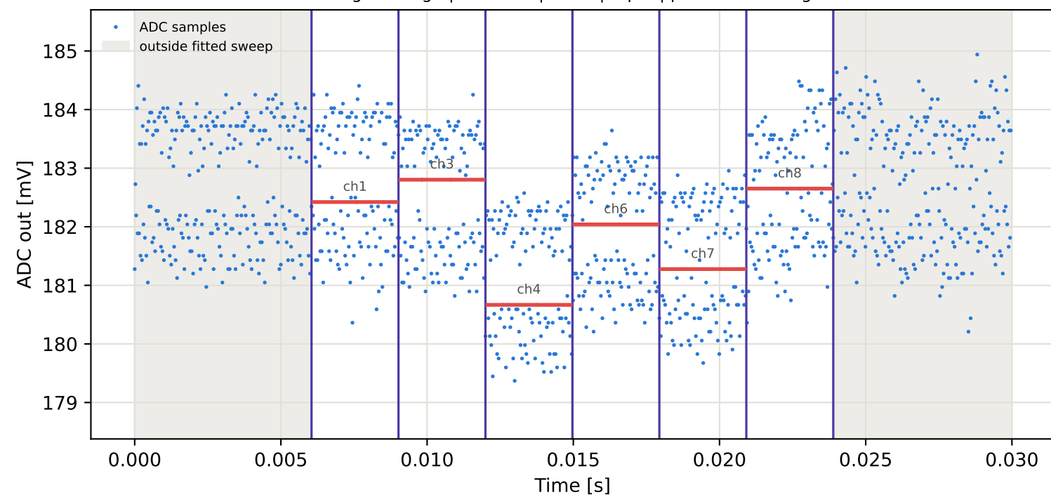
Tag3 &lt;- Tag15 | 805 MHz | run 0 | rep 1 | phase -132.76 deg
