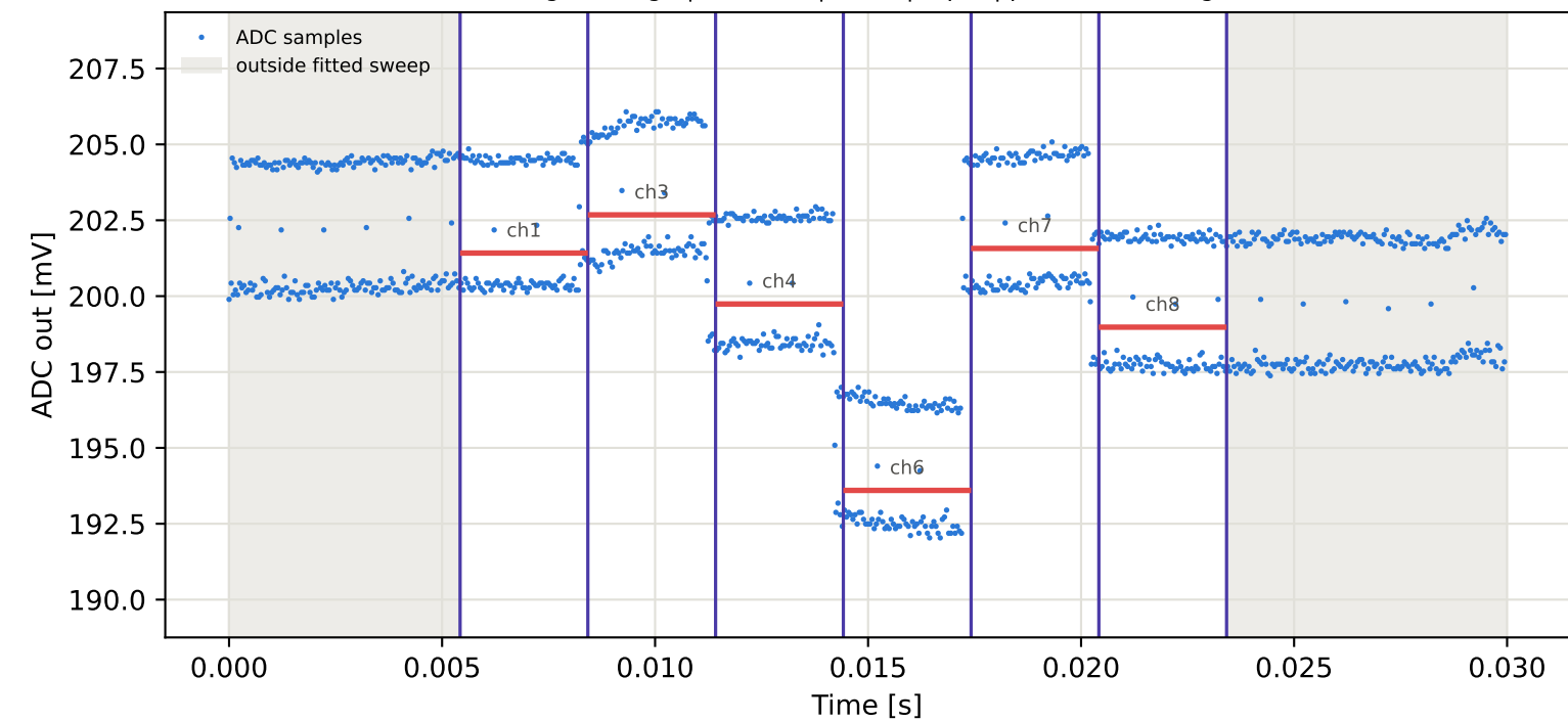
Tag3 &lt;- Tag6 | 965 MHz | run 0 | rep 1 | phase 107.36 deg
