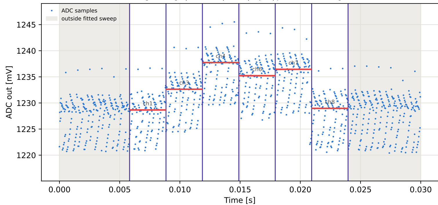
Tag2 &lt;- Tag6 | 915 MHz | run 0 | rep 1 | phase -13.93 deg
