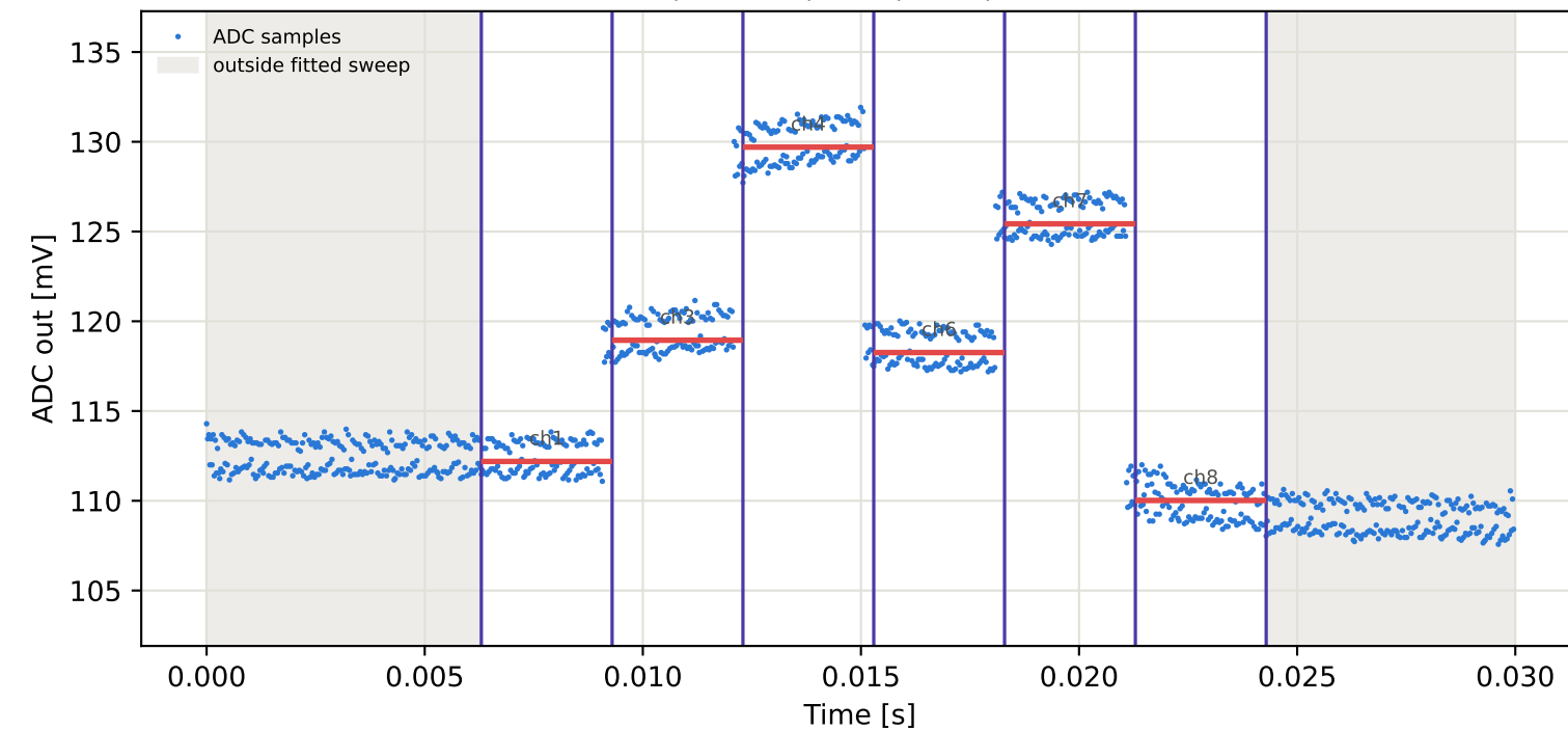
Tag4 &lt;- Tag2 | 895 MHz | run 0 | rep 1 | phase -90.81 deg
