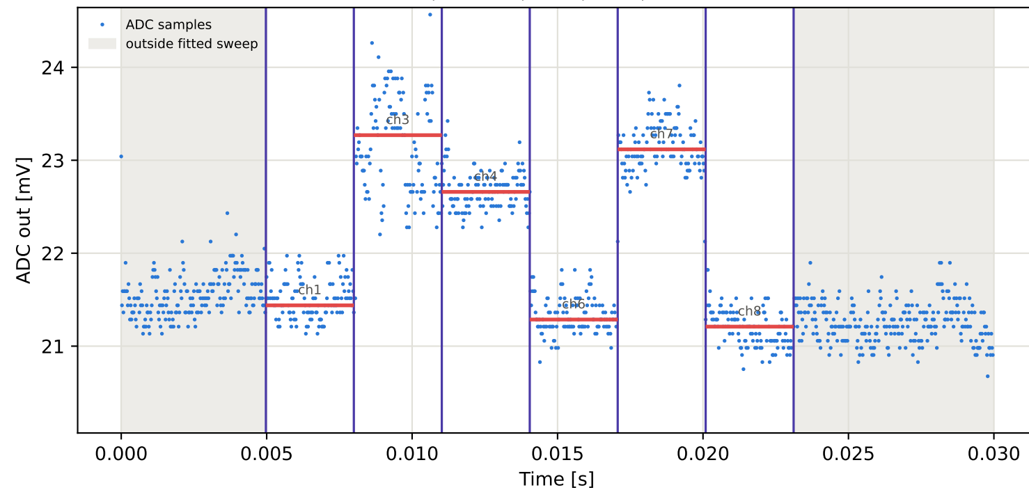
Tag2 &lt;- Tag7 | 785 MHz | run 0 | rep 1 | phase -20.29 deg
