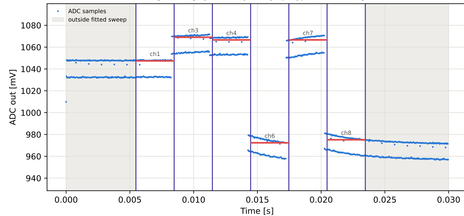
Tag2 &lt;- Tag1 | 905 MHz | run 0 | rep 1 | phase 145.50 deg
