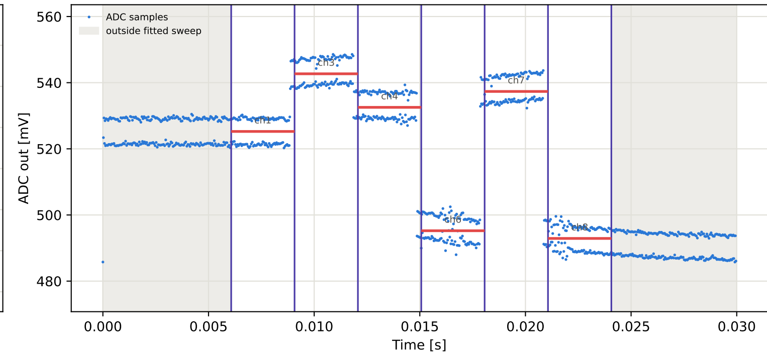
Tag6 &lt;- Tag10 | 875 MHz | run 0 | rep 1 | phase -143.56 deg
