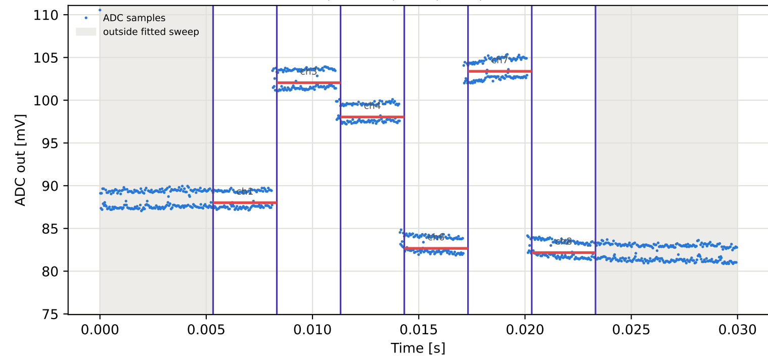
Tag8 &lt;- Tag7 | 785 MHz | run 0 | rep 1 | phase -18.10 deg
