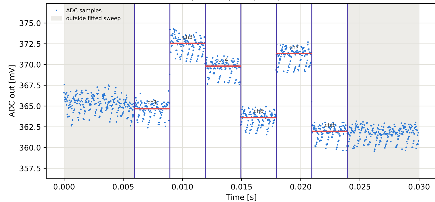
Tag5 &lt;- Tag16 | 835 MHz | run 0 | rep 1 | phase -121.47 deg
