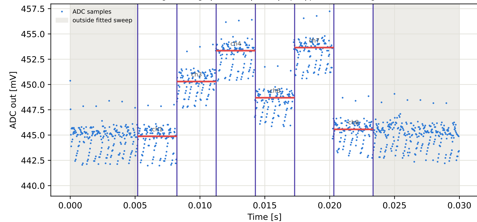
Tag16 &lt;- Tag10 | 825 MHz | run 0 | rep 1 | phase -172.90 deg
