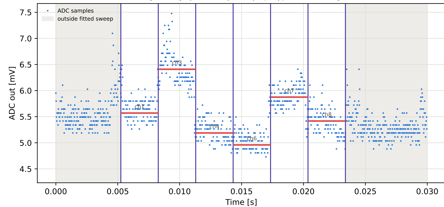
Tag2 &lt;- Tag5 | 775 MHz | run 0 | rep 1 | phase 66.16 deg
