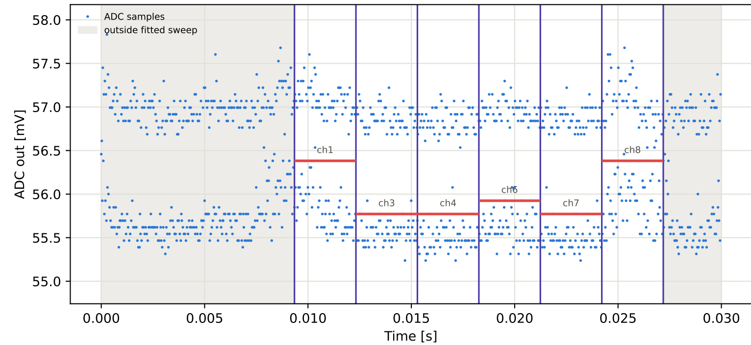
Tag1 &lt;- Tag4 | 775 MHz | run 0 | rep 1 | phase 121.69 deg
