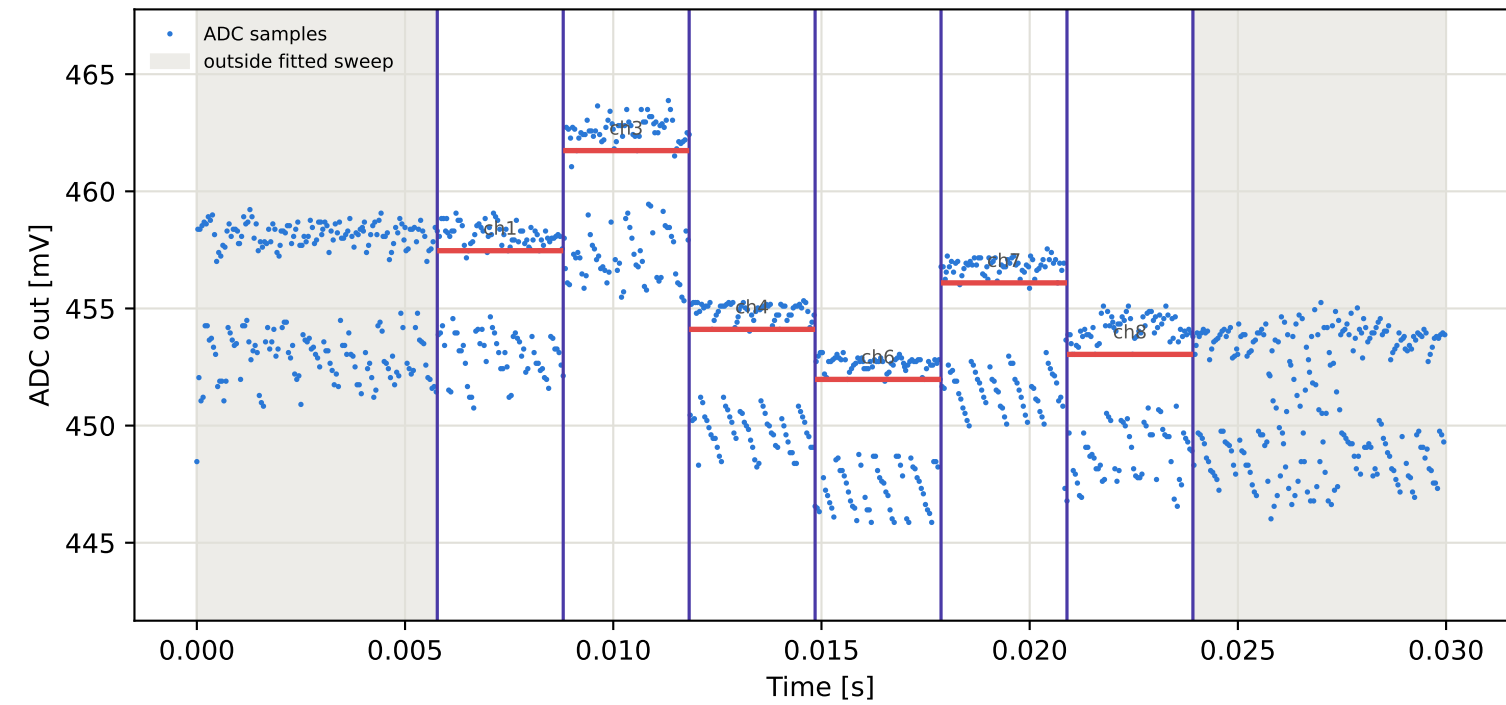
Tag15 &lt;- Tag6 | 825 MHz | run 0 | rep 1 | phase -155.57 deg
