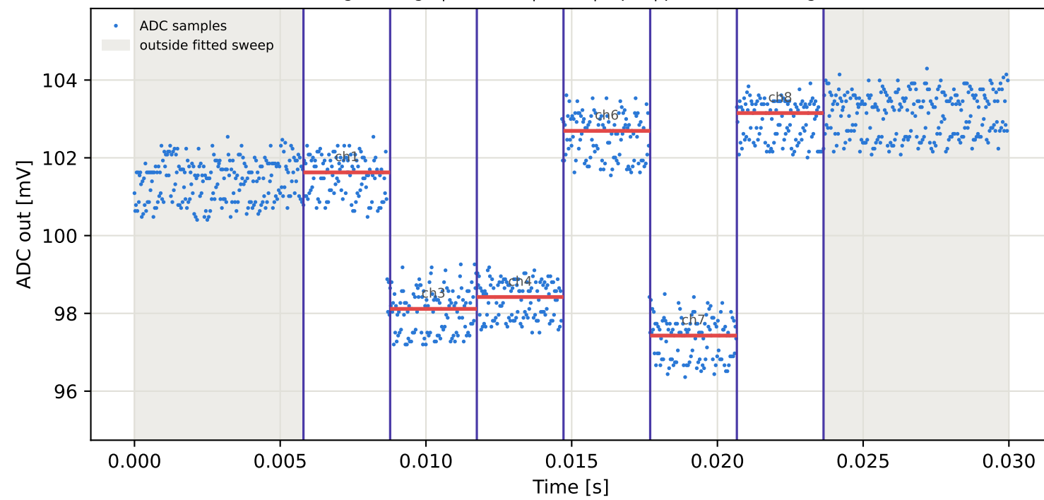
Tag6 &lt;- Tag9 | 795 MHz | run 0 | rep 1 | phase 88.15 deg
