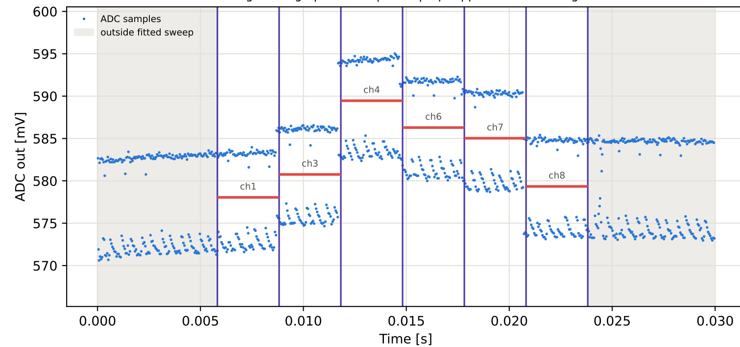
Tag5 &lt;- Tag8 | 945 MHz | run 0 | rep 1 | phase 9.99 deg
