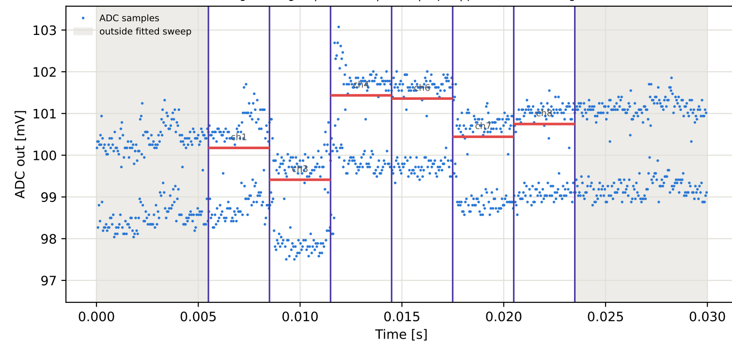
Tag8 &lt;- Tag15 | 785 MHz | run 0 | rep 1 | phase -127.65 deg
