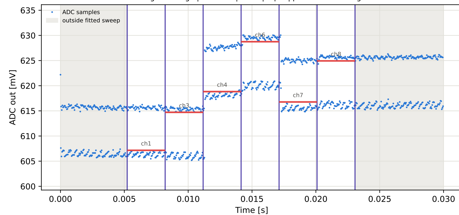
Tag15 &lt;- Tag5 | 835 MHz | run 0 | rep 1 | phase 36.91 deg
