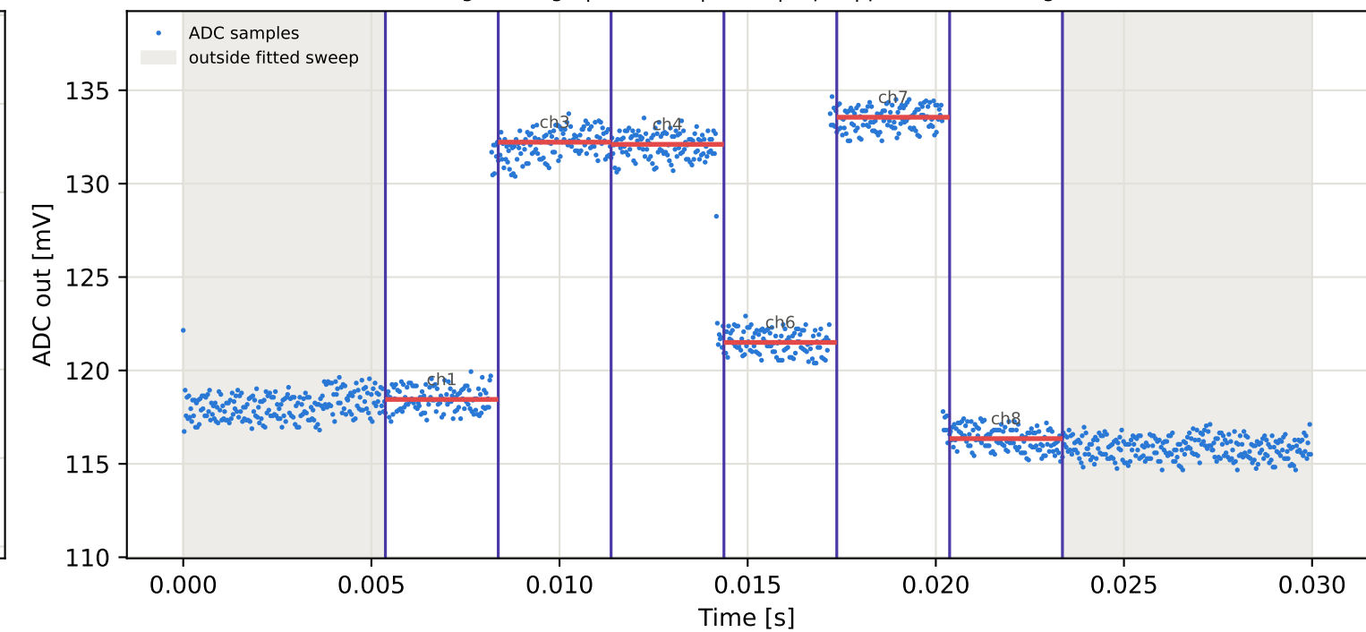
Tag2 &lt;- Tag8 | 845 MHz | run 0 | rep 1 | phase -102.36 deg
