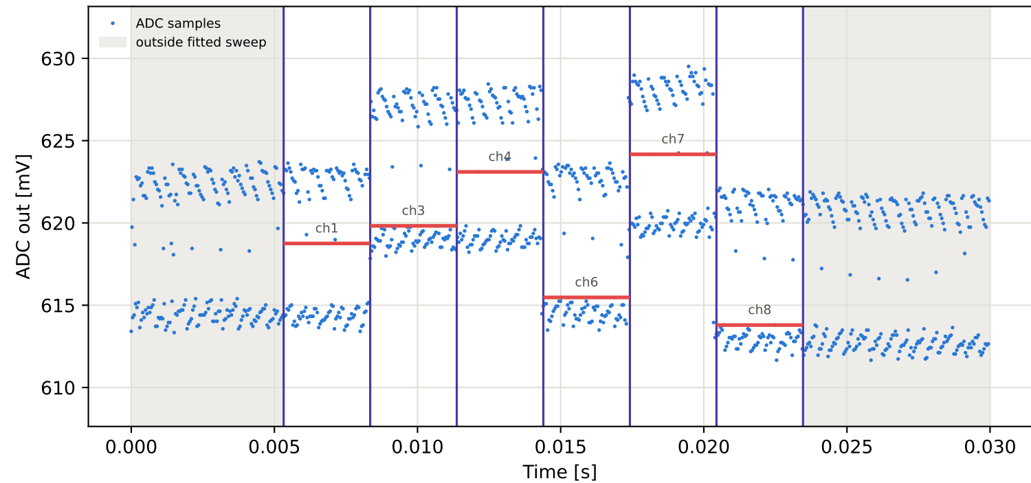
Tag16 &lt;- Tag10 | 835 MHz | run 0 | rep 1 | phase 141.70 deg
