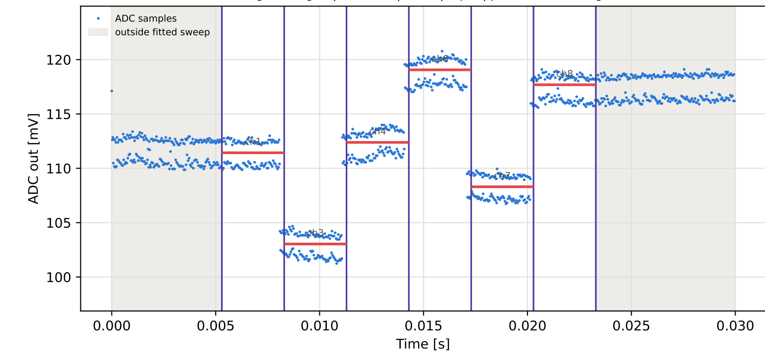
Tag4 &lt;- Tag2 | 835 MHz | run 0 | rep 1 | phase 13.47 deg
