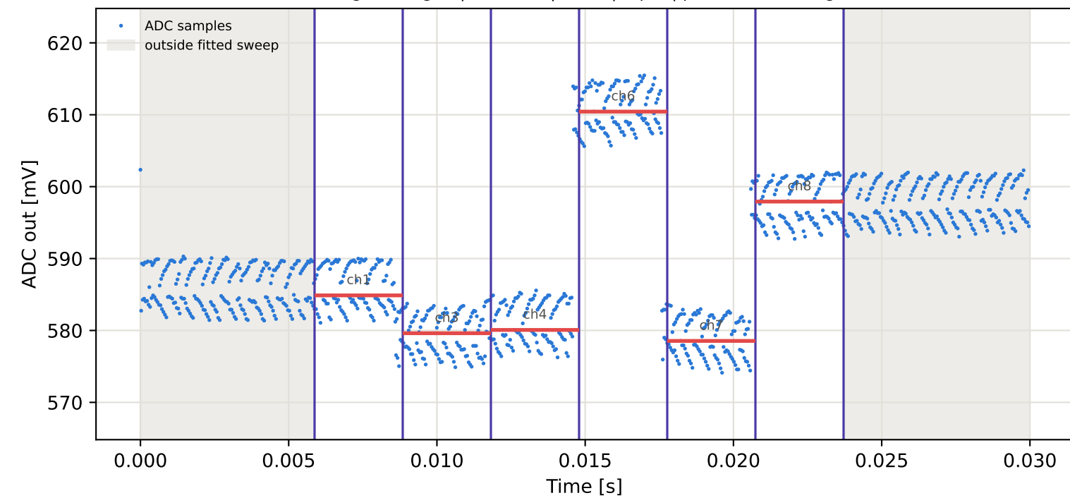
Tag5 &lt;- Tag16 | 945 MHz | run 0 | rep 1 | phase 23.61 deg
