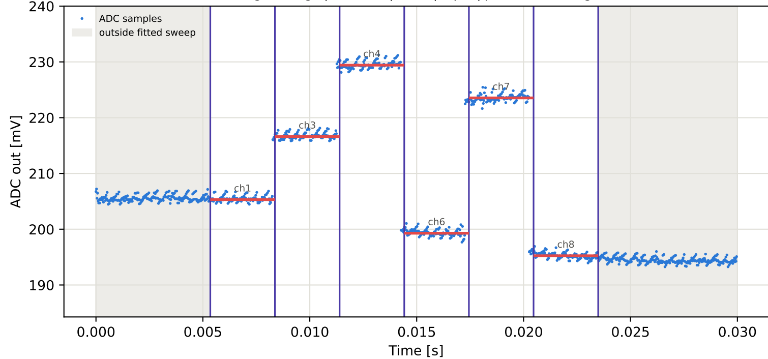
Tag7 &lt;- Tag1 | 935 MHz | run 0 | rep 1 | phase 142.66 deg
