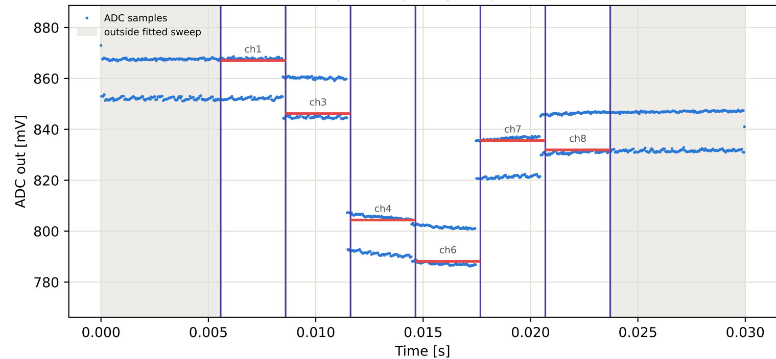
Tag16 &lt;- Tag7 | 955 MHz | run 0 | rep 1 | phase 37.30 deg
