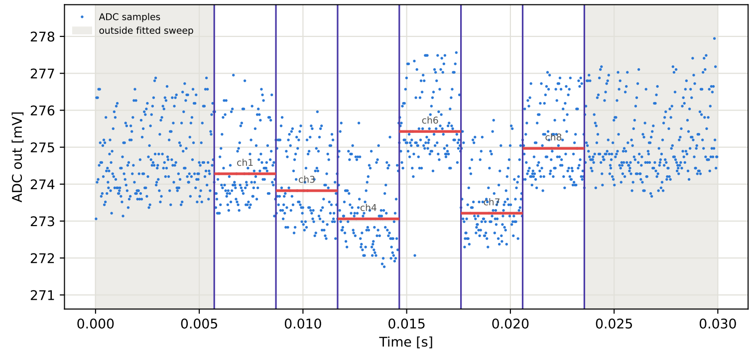
Tag5 &lt;- Tag4 | 995 MHz | run 0 | rep 1 | phase 16.95 deg
