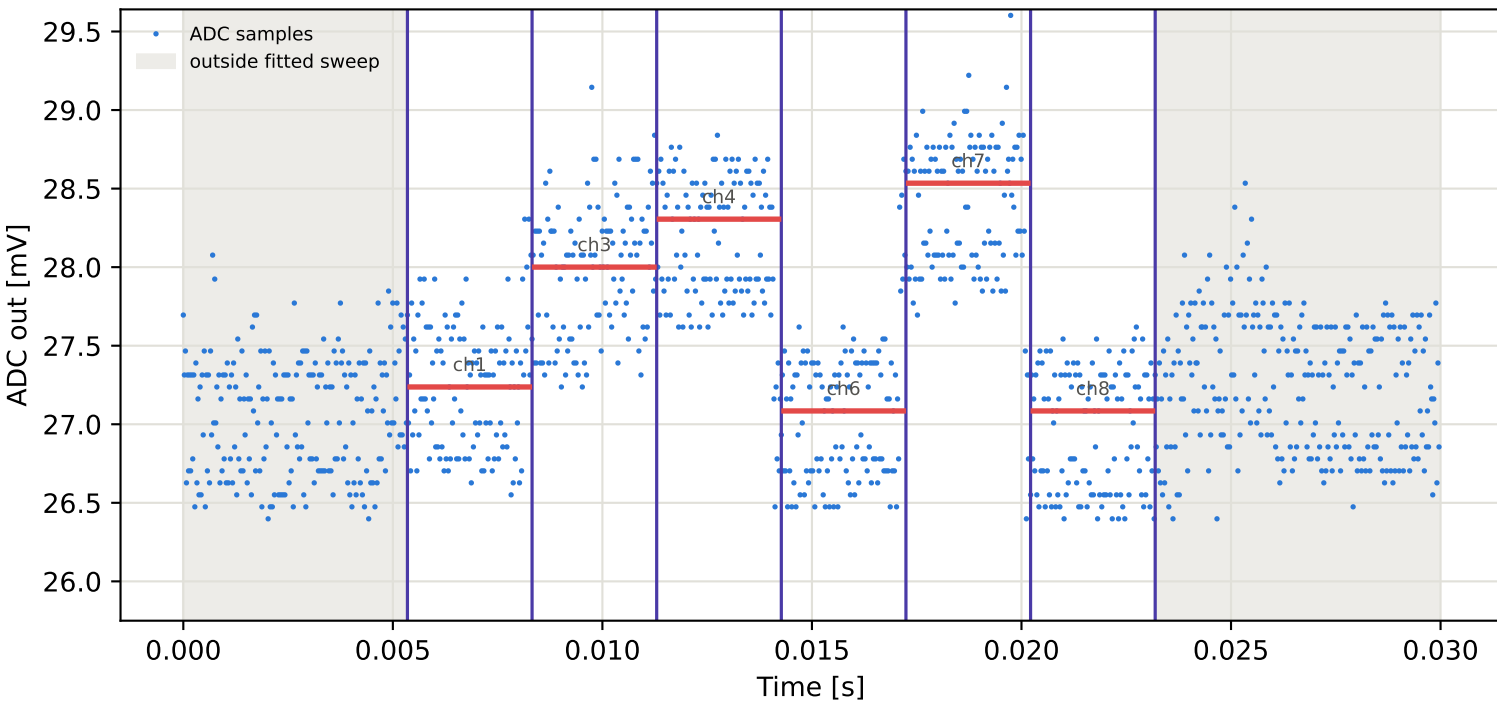
Tag2 &lt;- Tag15 | 795 MHz | run 0 | rep 1 | phase 1.25 deg
