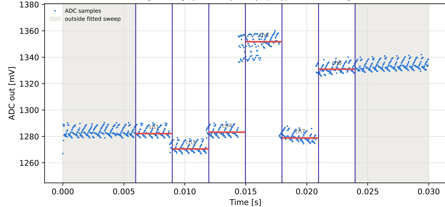
Tag10 &lt;- Tag5 | 905 MHz | run 0 | rep 1 | phase -32.64 deg
