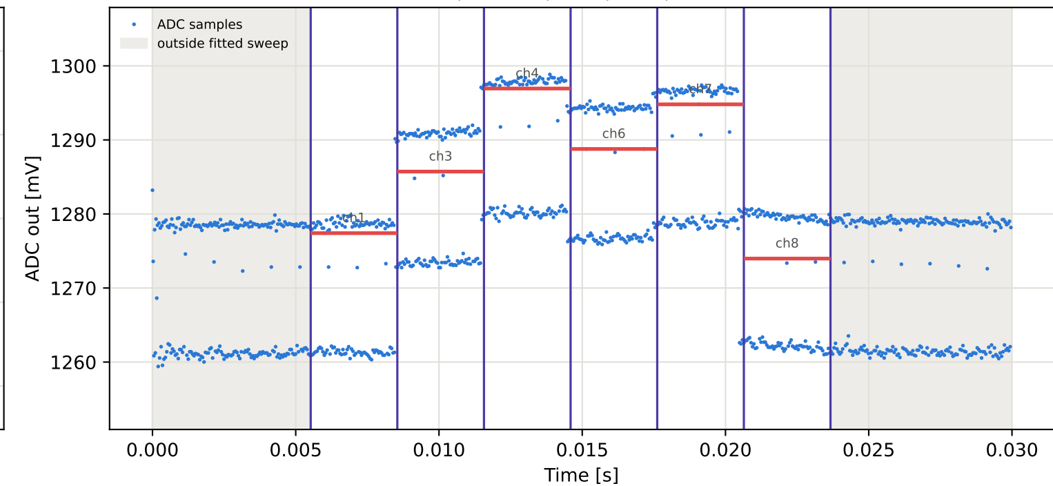
Tag7 &lt;- Tag6 | 875 MHz | run 0 | rep 1 | phase -93.98 deg
