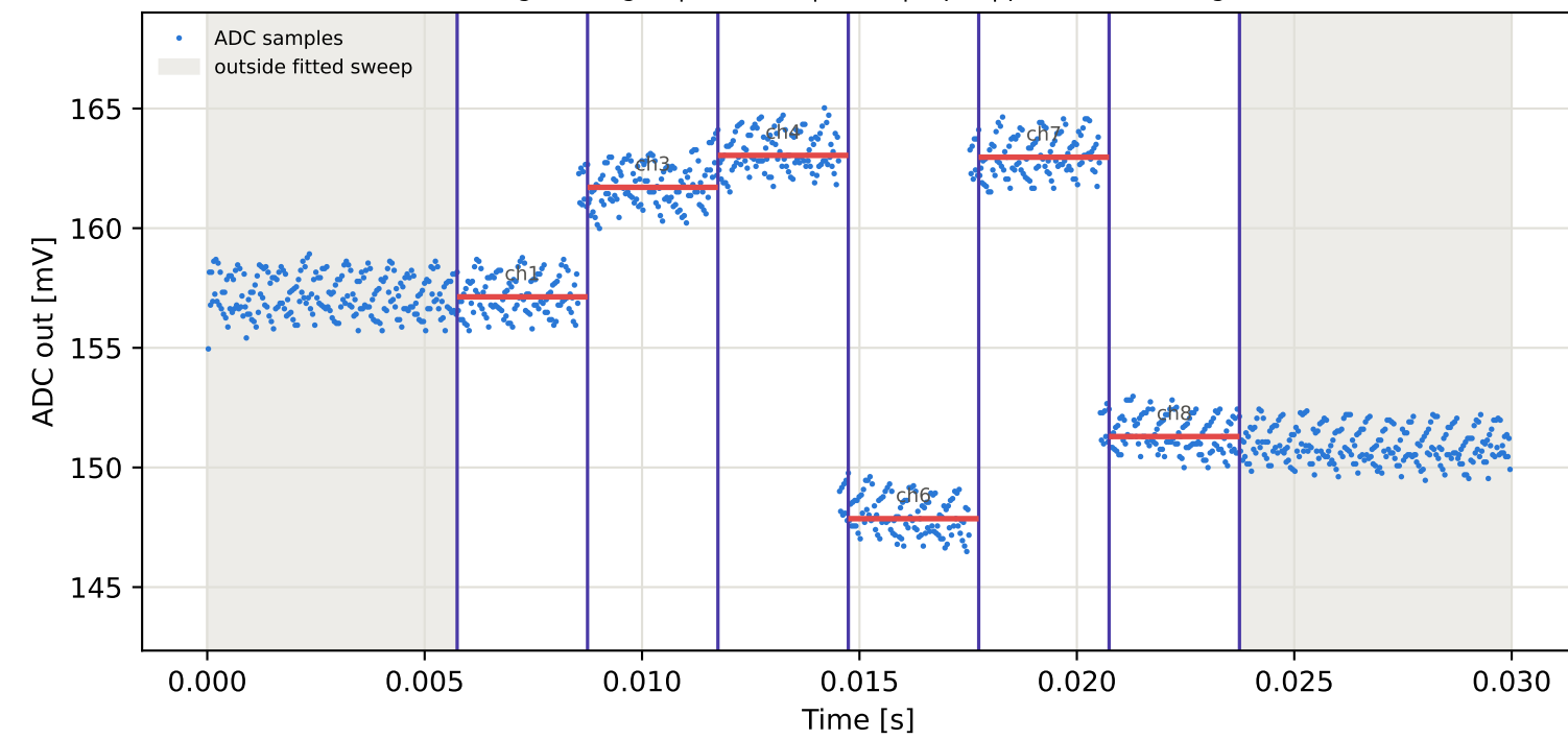
Tag6 &lt;- Tag2 | 955 MHz | run 0 | rep 1 | phase 89.65 deg
