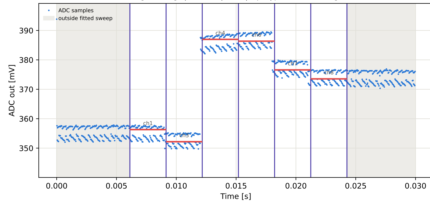
Tag10 &lt;- Tag8 | 825 MHz | run 0 | rep 1 | phase 162.25 deg
