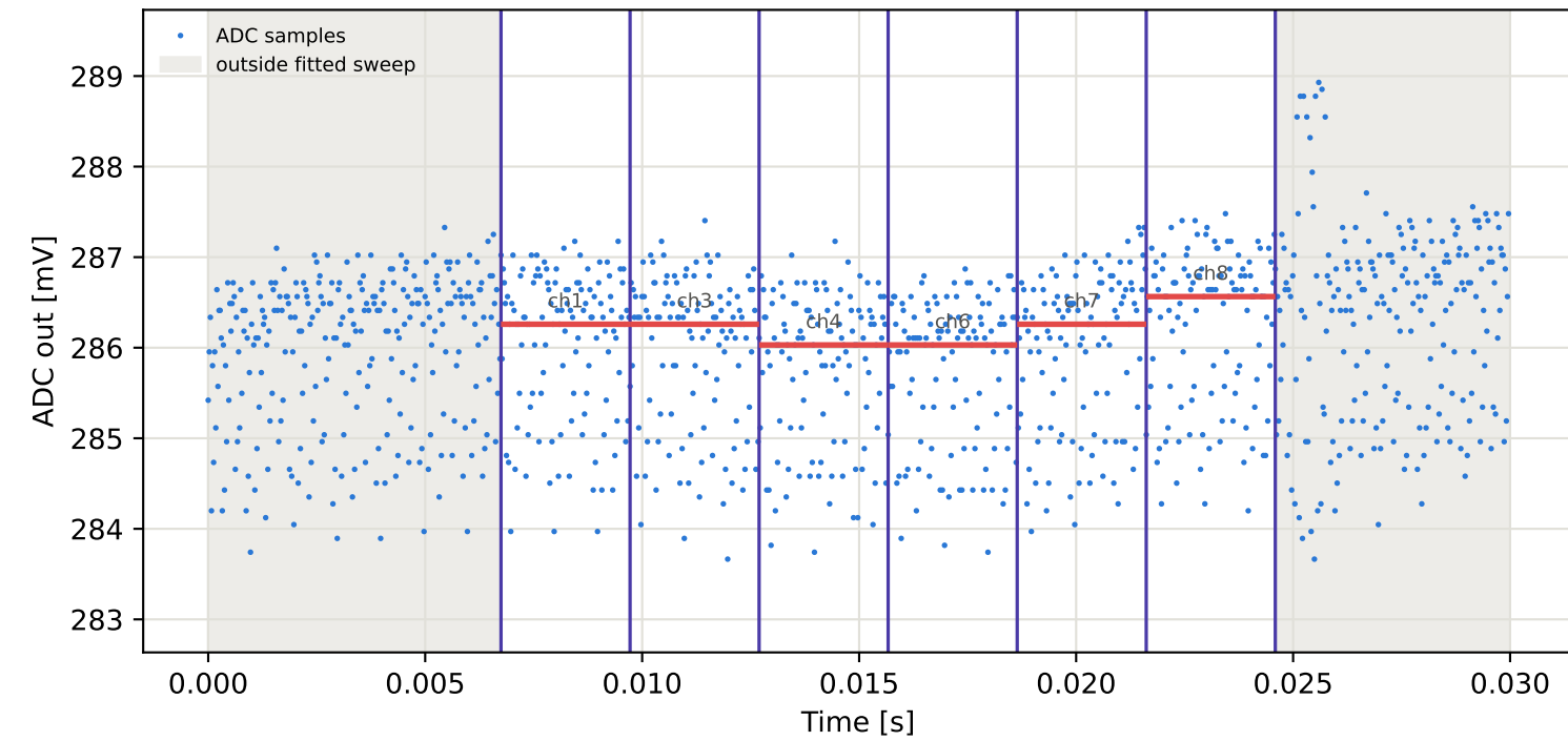
Tag1 &lt;- Tag4 | 835 MHz | run 0 | rep 1 | phase 77.50 deg
