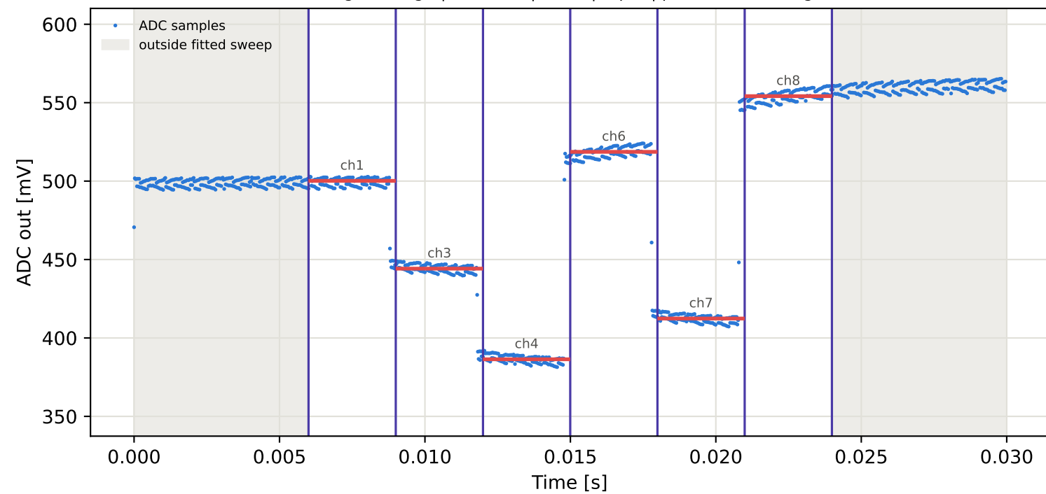
Tag8 &lt;- Tag1 | 925 MHz | run 0 | rep 1 | phase 15.97 deg
