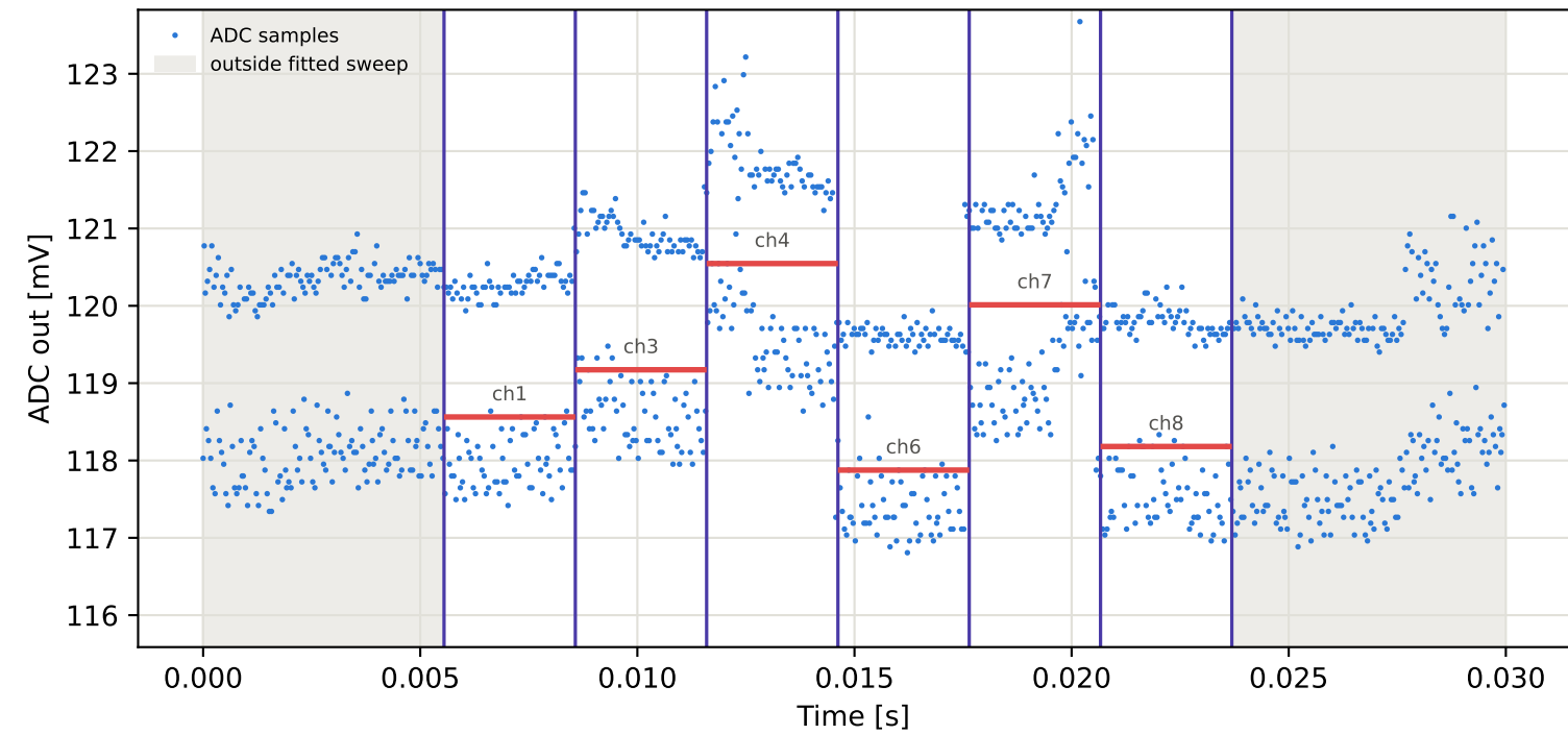
Tag1 &lt;- Tag4 | 995 MHz | run 0 | rep 1 | phase -57.69 deg
