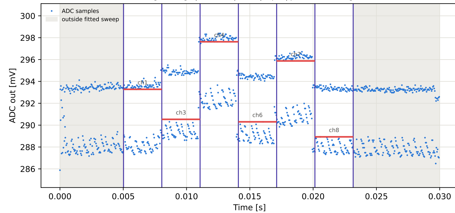
Tag2 &lt;- Tag5 | 975 MHz | run 0 | rep 1 | phase -6.43 deg
