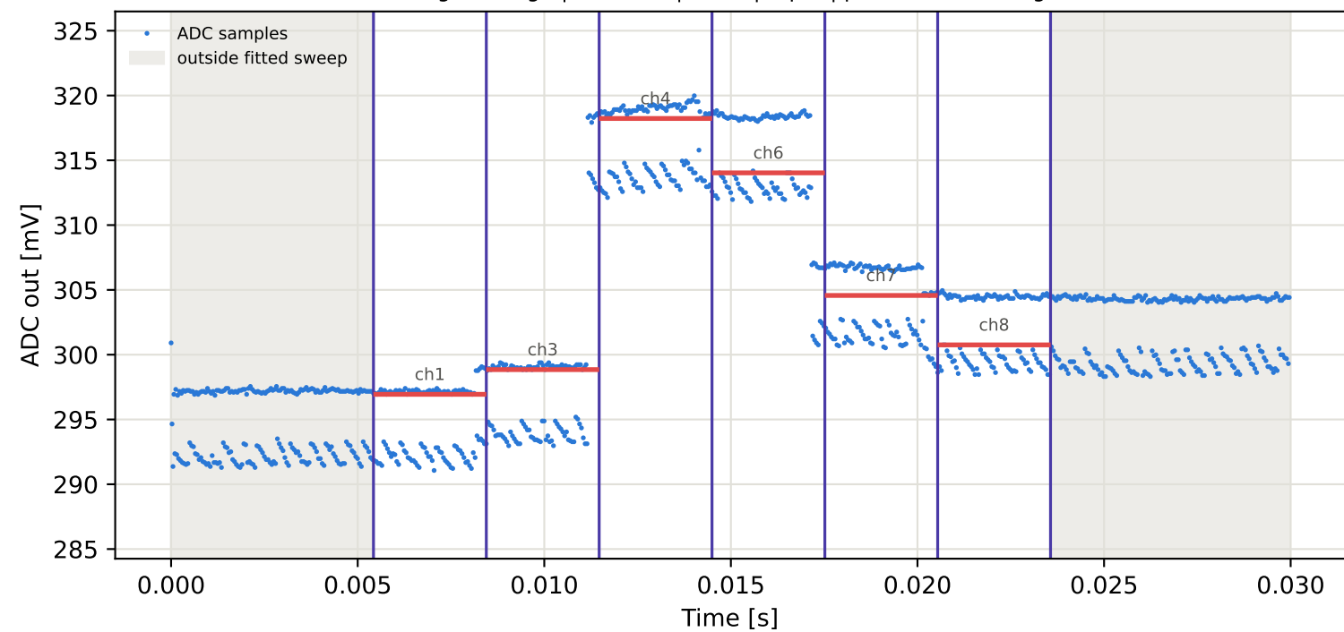
Tag6 &lt;- Tag1 | 975 MHz | run 0 | rep 1 | phase -131.99 deg
