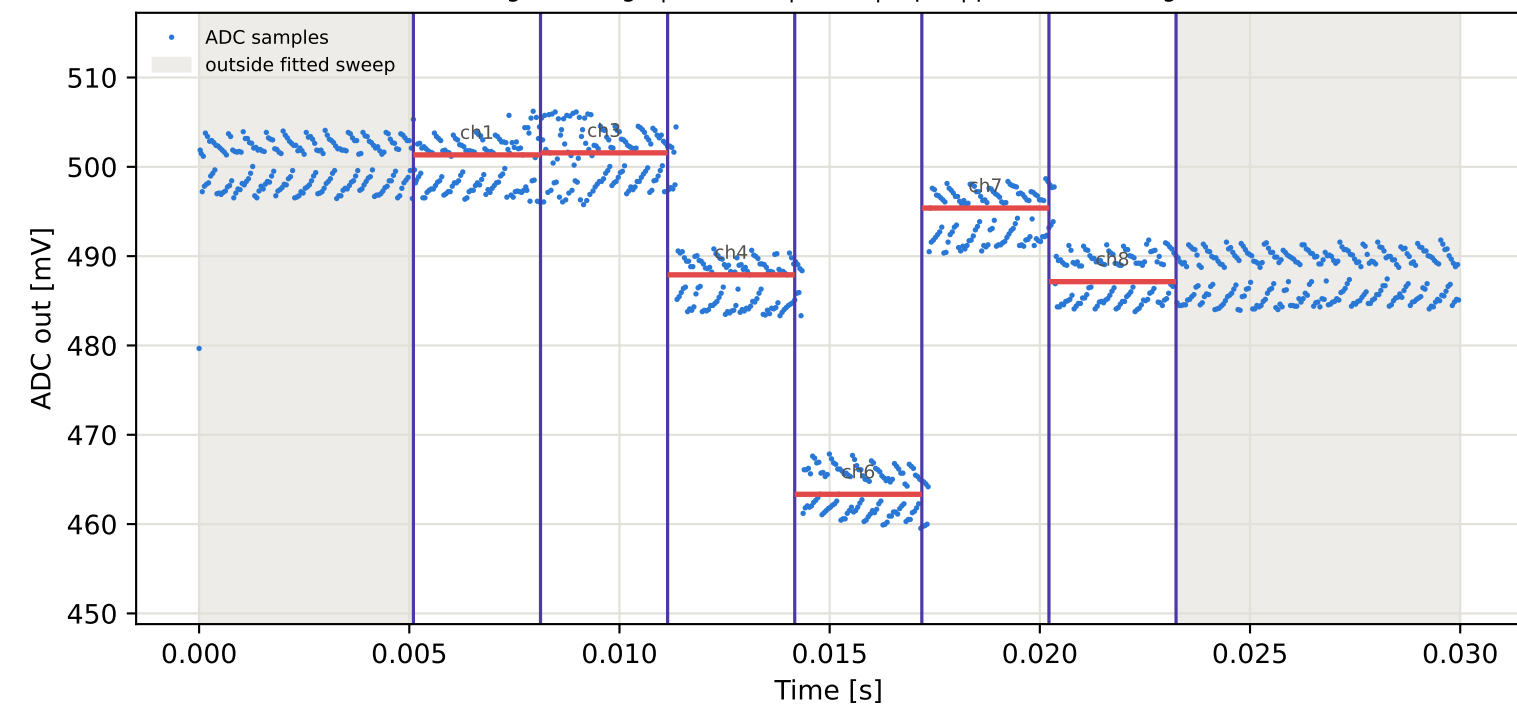
Tag15 &lt;- Tag5 | 945 MHz | run 0 | rep 1 | phase 20.16 deg
