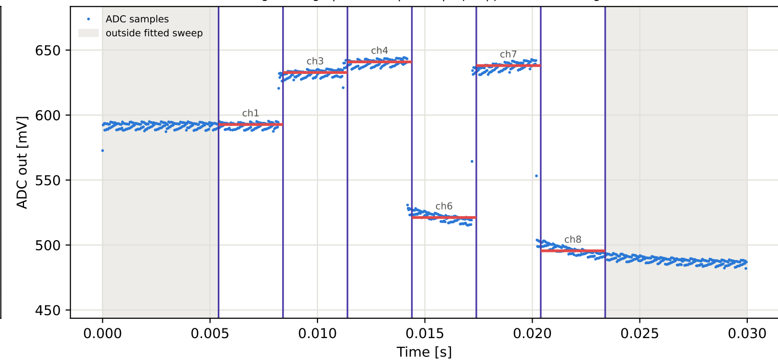
Tag9 &lt;- Tag8 | 905 MHz | run 0 | rep 1 | phase -27.59 deg
