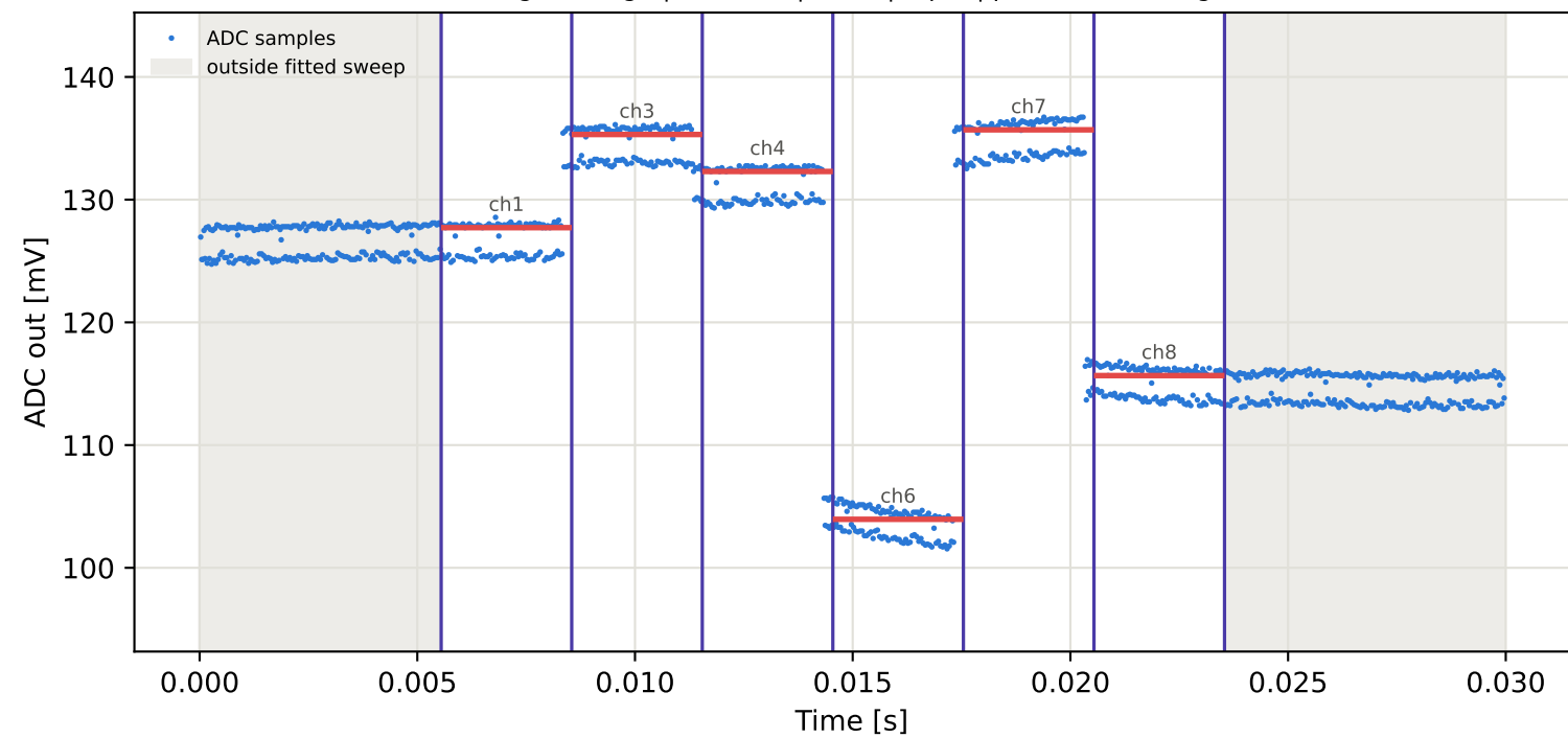
Tag4 &lt;- Tag7 | 985 MHz | run 0 | rep 1 | phase 82.18 deg
