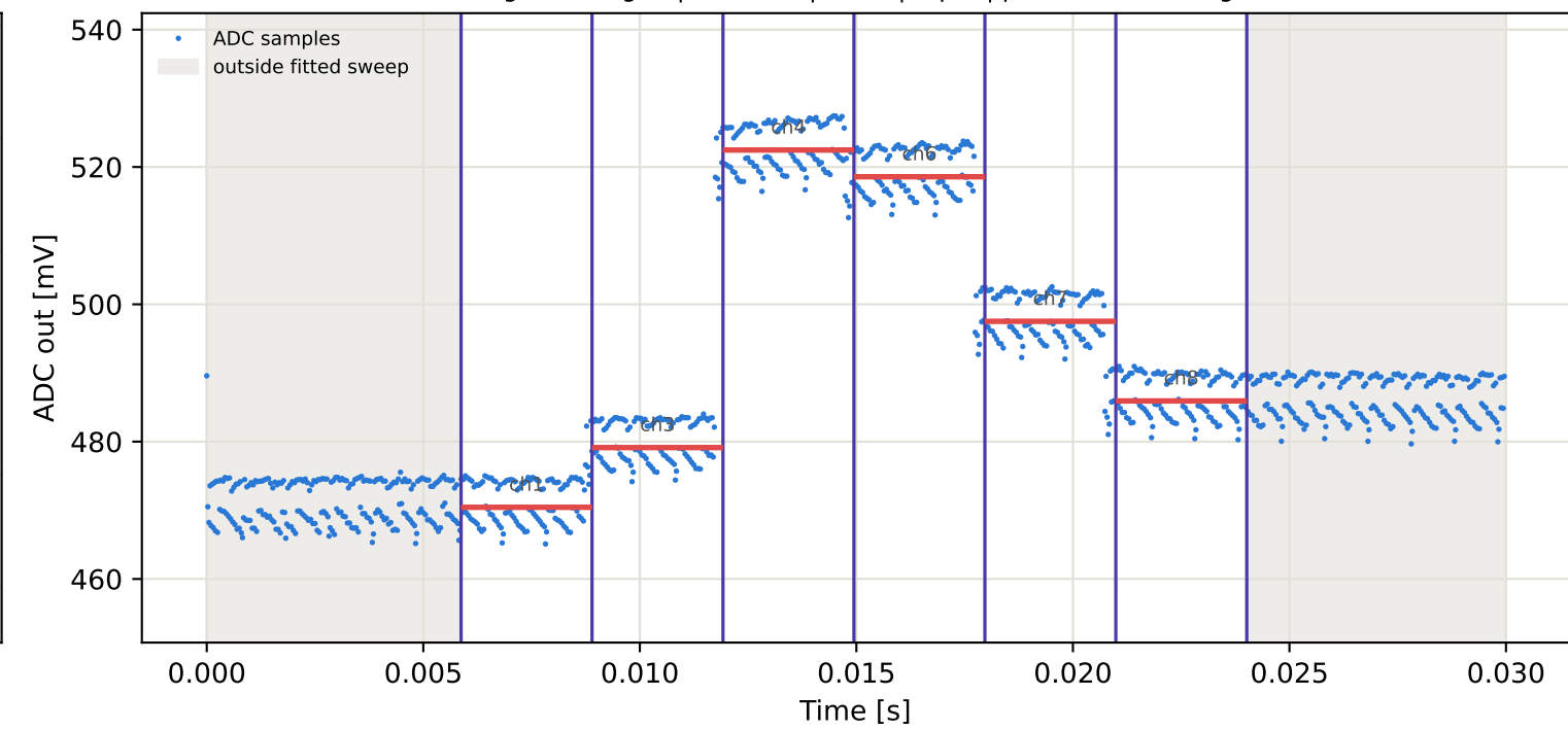
Tag16 &lt;- Tag15 | 985 MHz | run 0 | rep 1 | phase -133.09 deg
