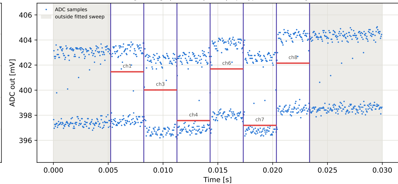
Tag2 &lt;- Tag6 | 865 MHz | run 0 | rep 1 | phase -36.17 deg
