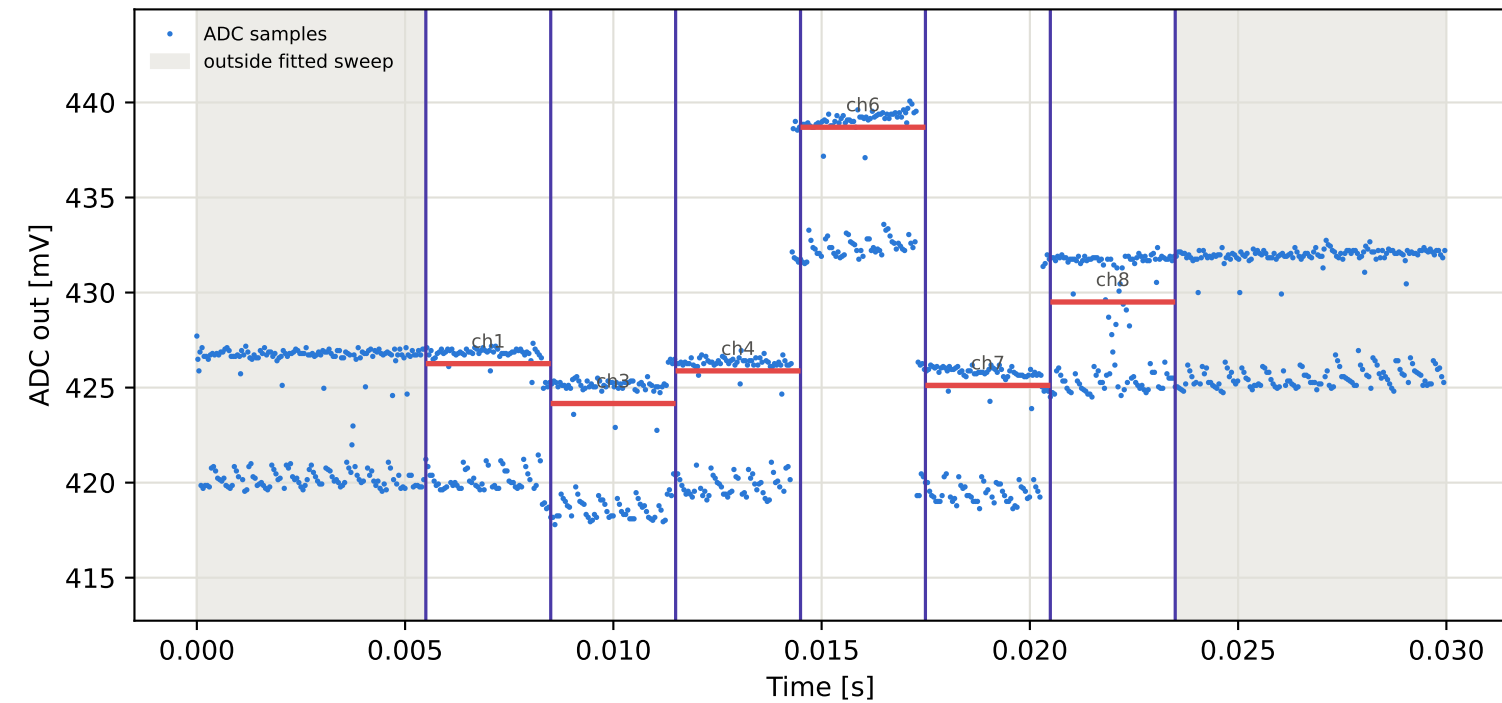
Tag5 &lt;- Tag4 | 865 MHz | run 0 | rep 1 | phase 164.72 deg
