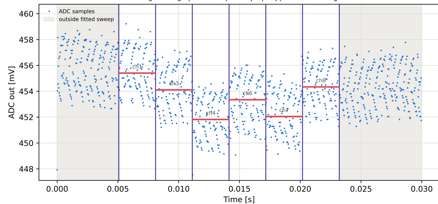
Tag5 &lt;- Tag1 | 845 MHz | run 0 | rep 1 | phase 84.28 deg
