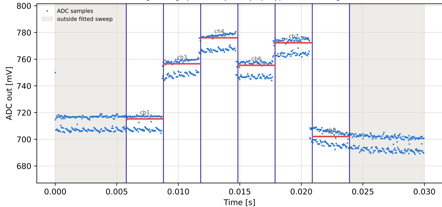
Tag2 &lt;- Tag8 | 885 MHz | run 0 | rep 1 | phase -90.07 deg
