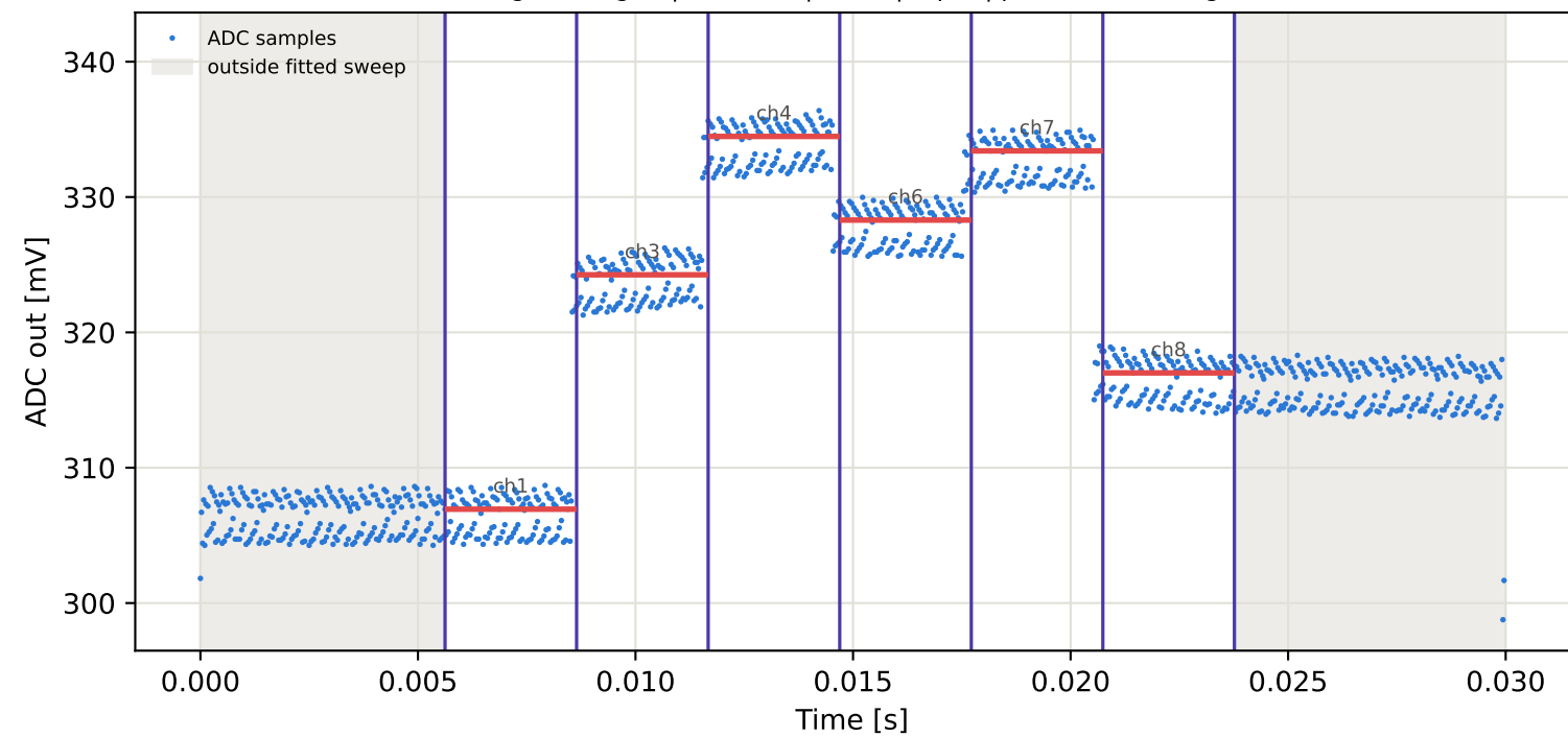
Tag1 &lt;- Tag2 | 865 MHz | run 0 | rep 1 | phase 8.14 deg
