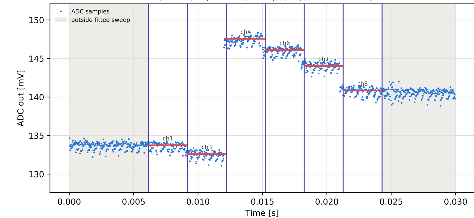
Tag4 &lt;- Tag2 | 825 MHz | run 0 | rep 1 | phase 3.77 deg
