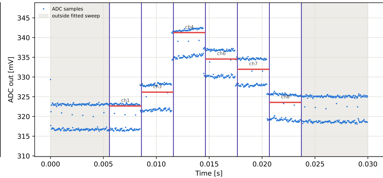
Tag5 &lt;- Tag1 | 955 MHz | run 0 | rep 1 | phase -118.89 deg
