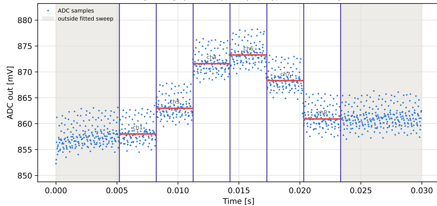
Tag3 &lt;- Tag6 | 925 MHz | run 0 | rep 1 | phase 54.62 deg
