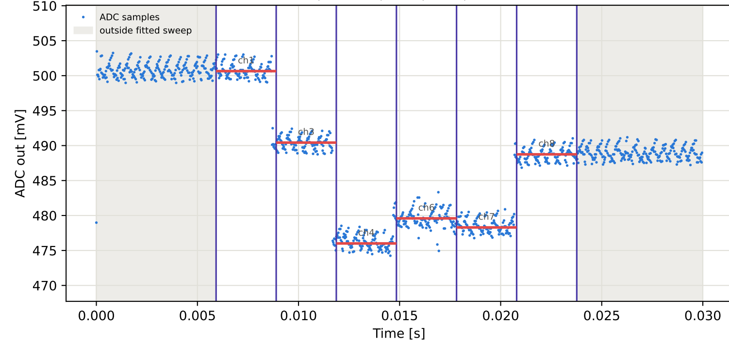
Tag15 &lt;- Tag5 | 845 MHz | run 0 | rep 1 | phase 68.87 deg
