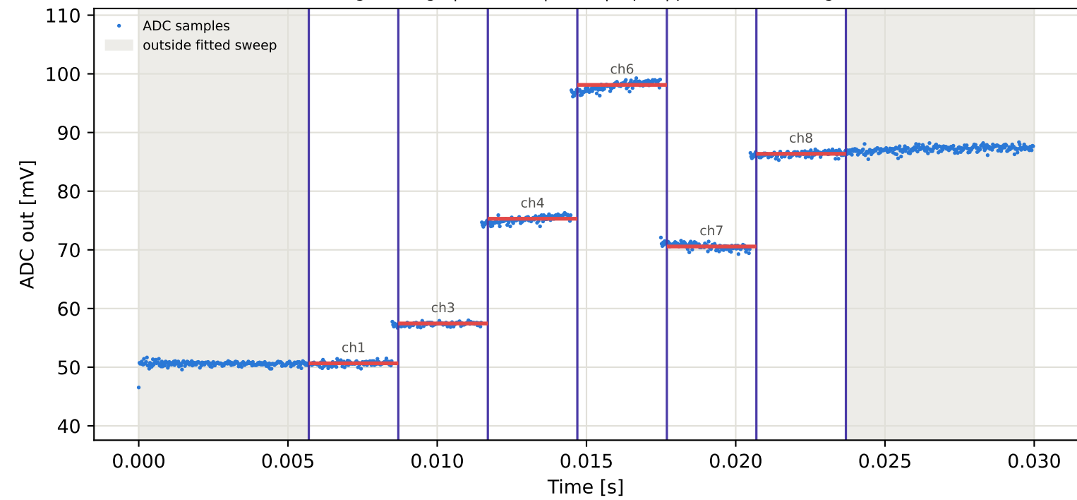
Tag1 &lt;- Tag8 | 875 MHz | run 0 | rep 1 | phase -97.27 deg
