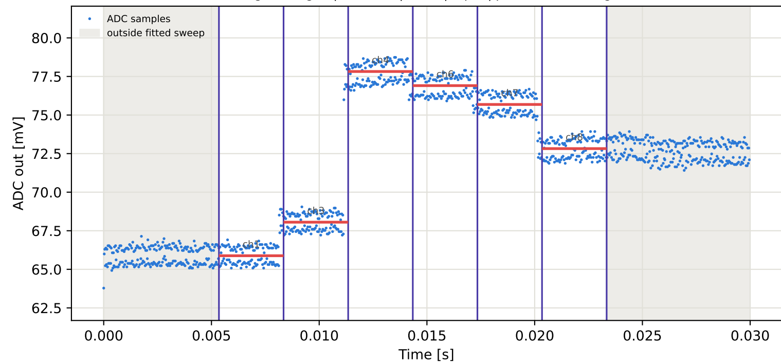
Tag1 &lt;- Tag2 | 845 MHz | run 0 | rep 1 | phase -77.14 deg
