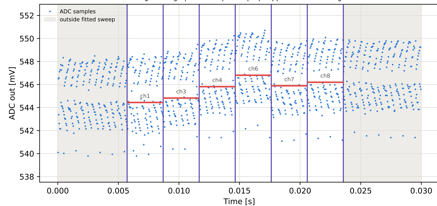
Tag6 &lt;- Tag4 | 865 MHz | run 0 | rep 1 | phase -141.72 deg
