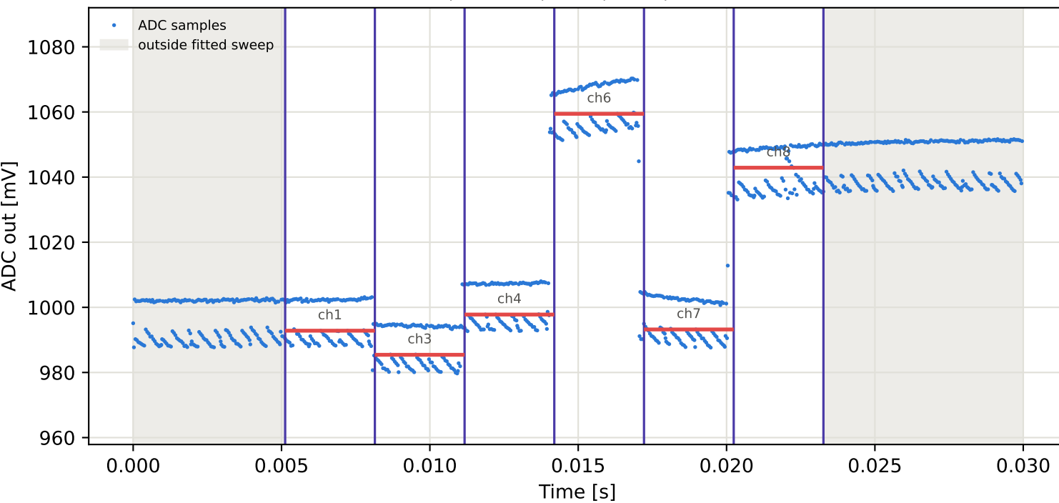
Tag7 &lt;- Tag10 | 895 MHz | run 0 | rep 1 | phase -175.22 deg
