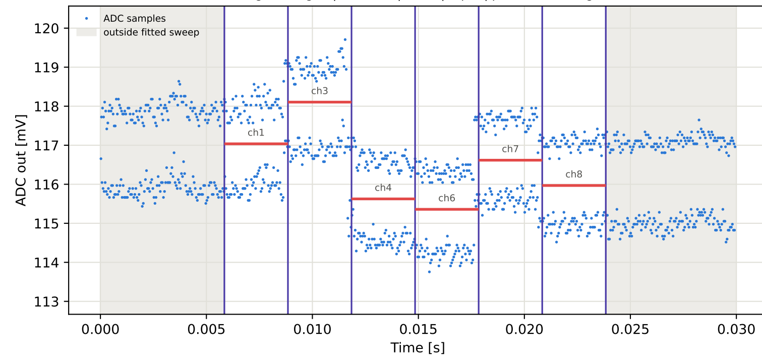
Tag6 &lt;- Tag2 | 785 MHz | run 0 | rep 1 | phase 167.33 deg
