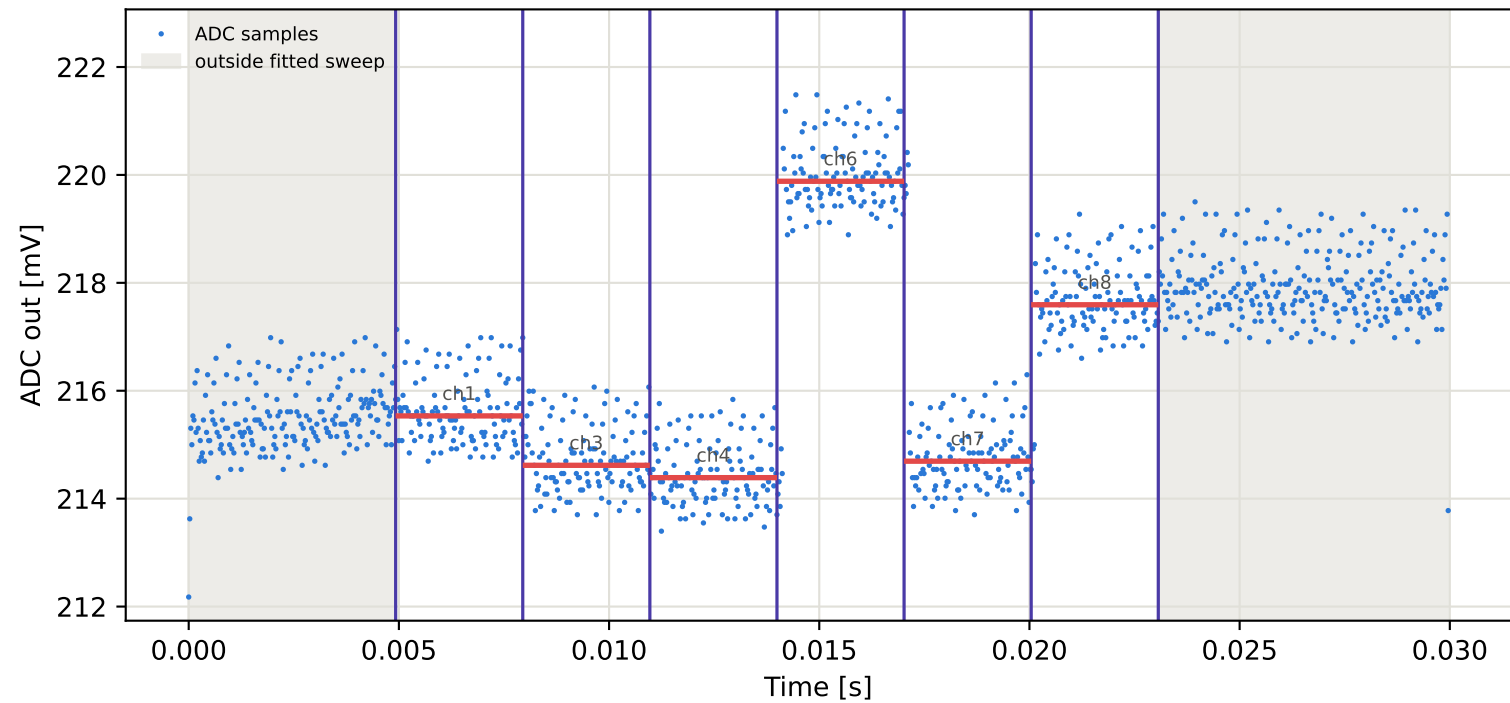
Tag1 &lt;- Tag4 | 955 MHz | run 0 | rep 1 | phase -39.07 deg
