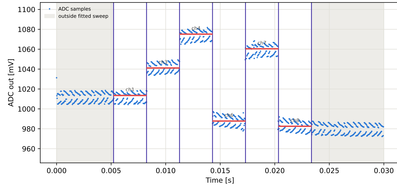
Tag15 &lt;- Tag1 | 935 MHz | run 0 | rep 1 | phase 155.52 deg
