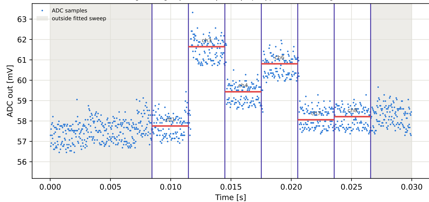
Tag9 &lt;- Tag2 | 785 MHz | run 0 | rep 1 | phase 116.84 deg
