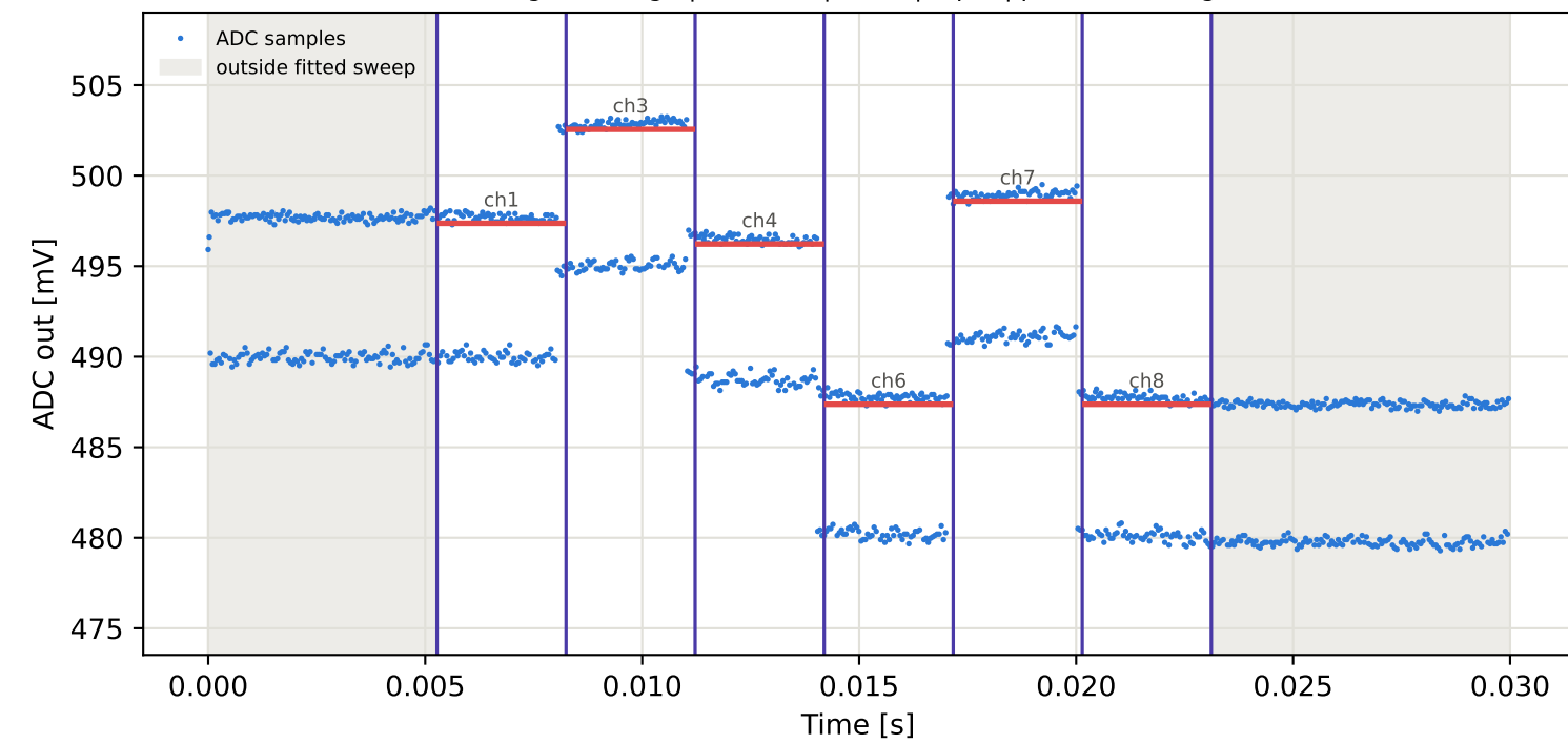
Tag16 &lt;- Tag1 | 855 MHz | run 0 | rep 1 | phase -177.05 deg
