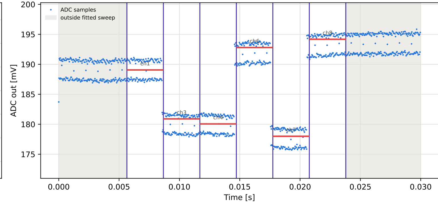
Tag3 &lt;- Tag9 | 805 MHz | run 0 | rep 1 | phase -148.76 deg
