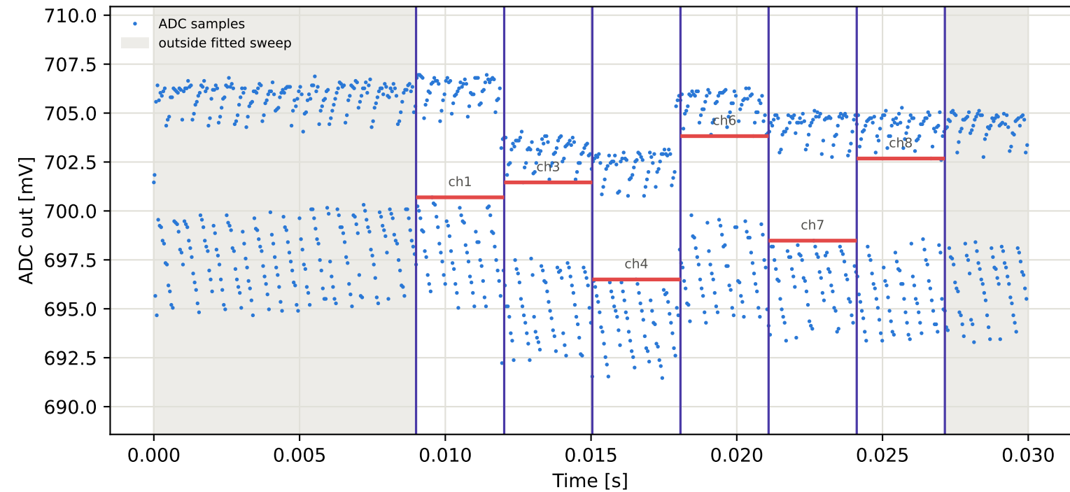
Tag7 &lt;- Tag15 | 995 MHz | run 0 | rep 1 | phase -140.21 deg
