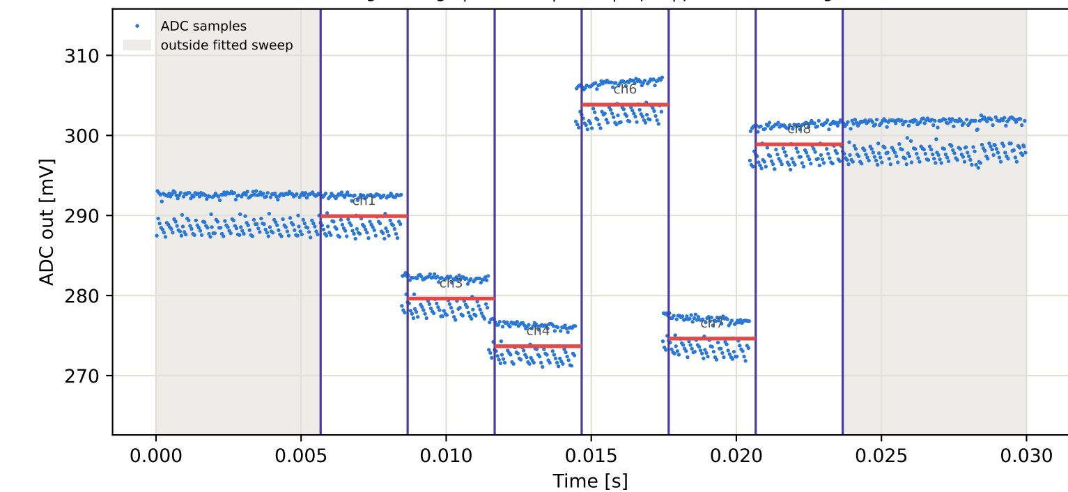
Tag3 &lt;- Tag8 | 985 MHz | run 0 | rep 1 | phase 139.07 deg
