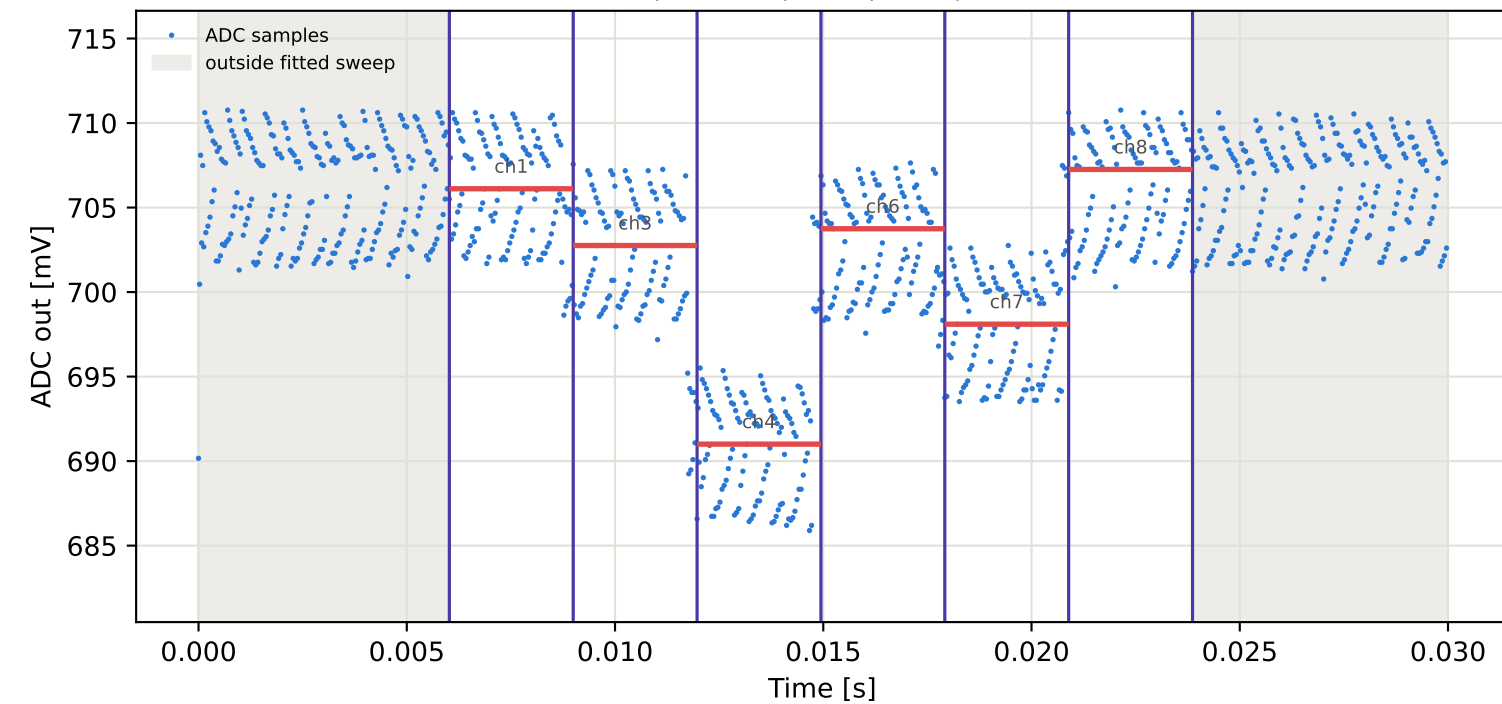
Tag7 &lt;- Tag10 | 995 MHz | run 0 | rep 1 | phase 80.87 deg
