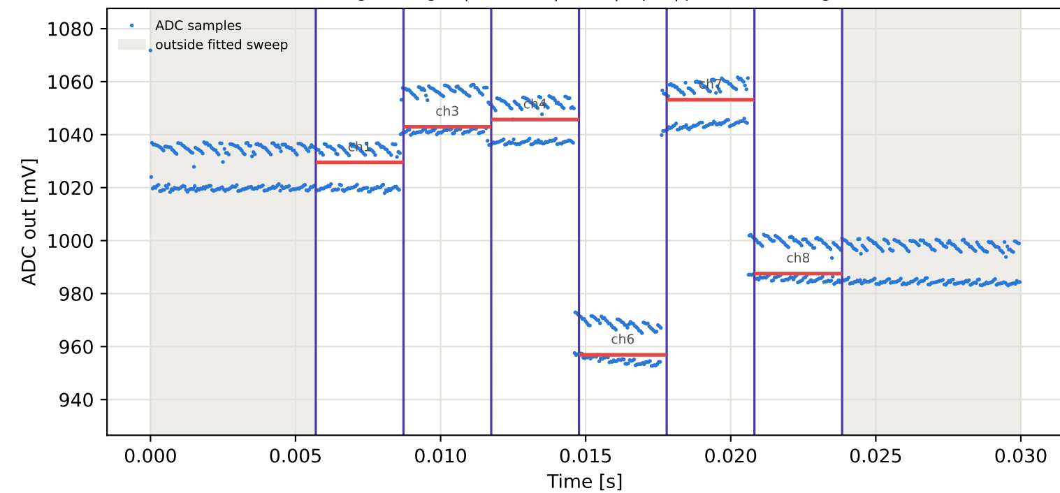
Tag7 &lt;- Tag3 | 955 MHz | run 0 | rep 1 | phase 8.38 deg
