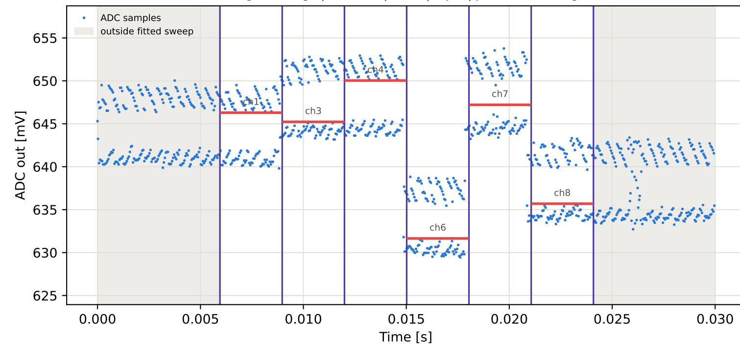
Tag16 &lt;- Tag4 | 835 MHz | run 0 | rep 1 | phase 136.64 deg
