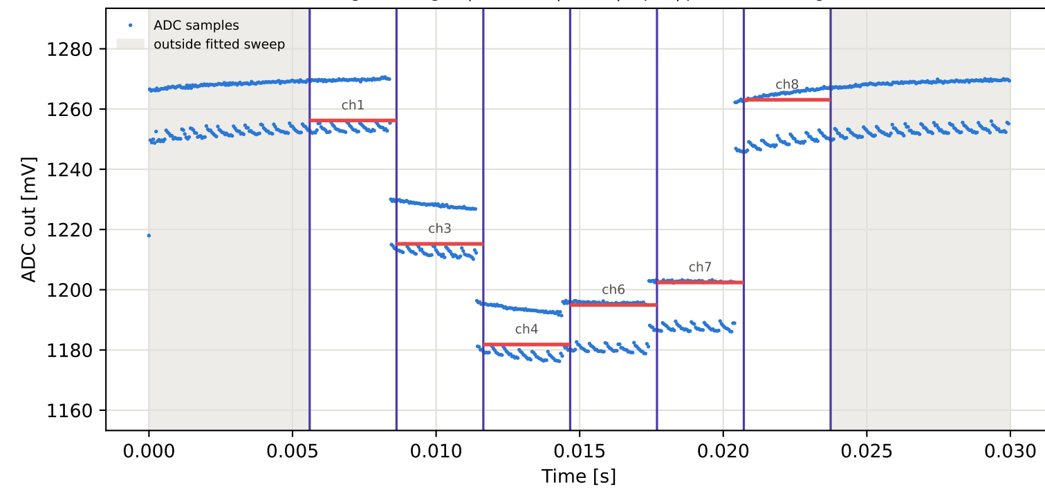
Tag15 &lt;- Tag3 | 895 MHz | run 0 | rep 1 | phase 38.86 deg
