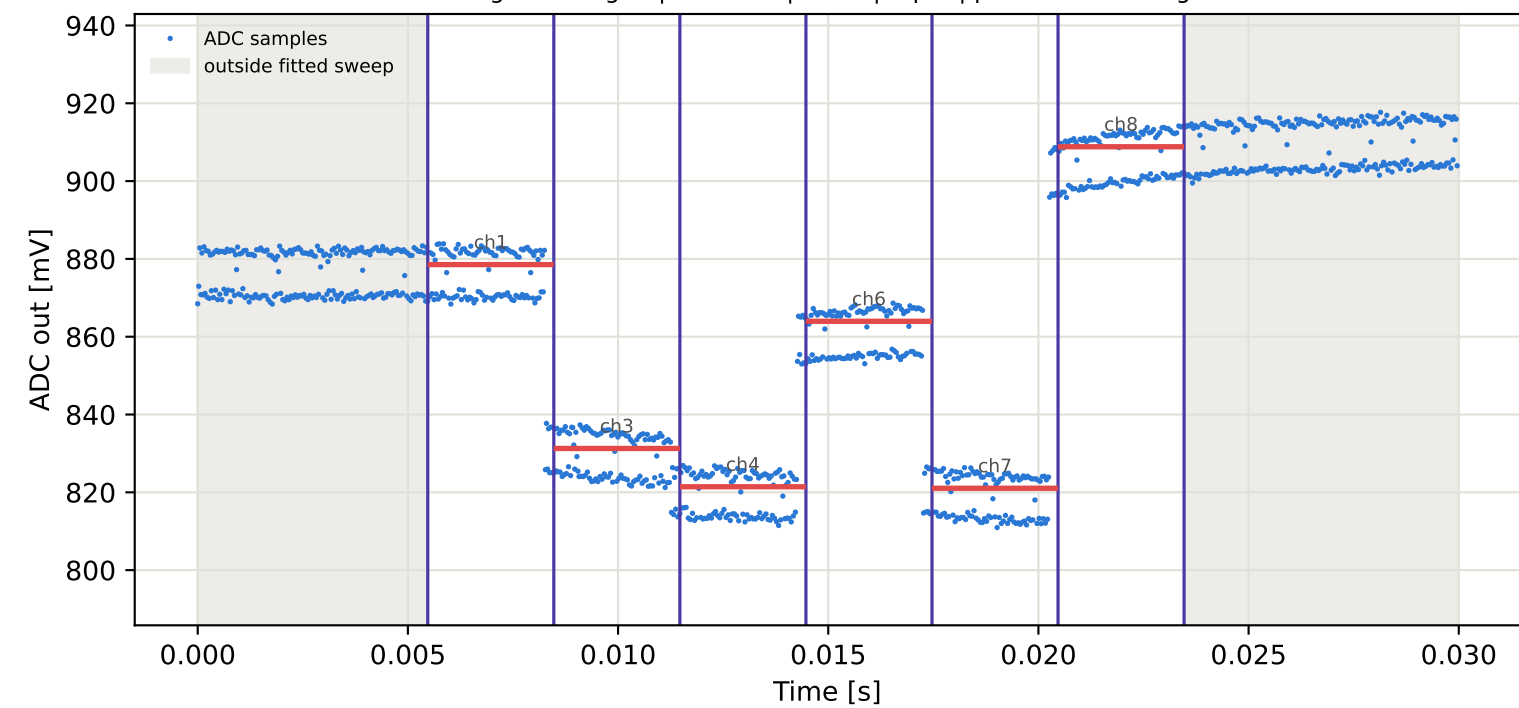
Tag10 &lt;- Tag3 | 885 MHz | run 0 | rep 1 | phase 113.67 deg
