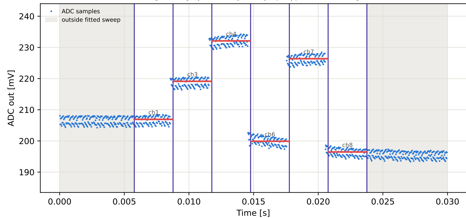
Tag1 &lt;- Tag8 | 935 MHz | run 0 | rep 1 | phase 57.51 deg
