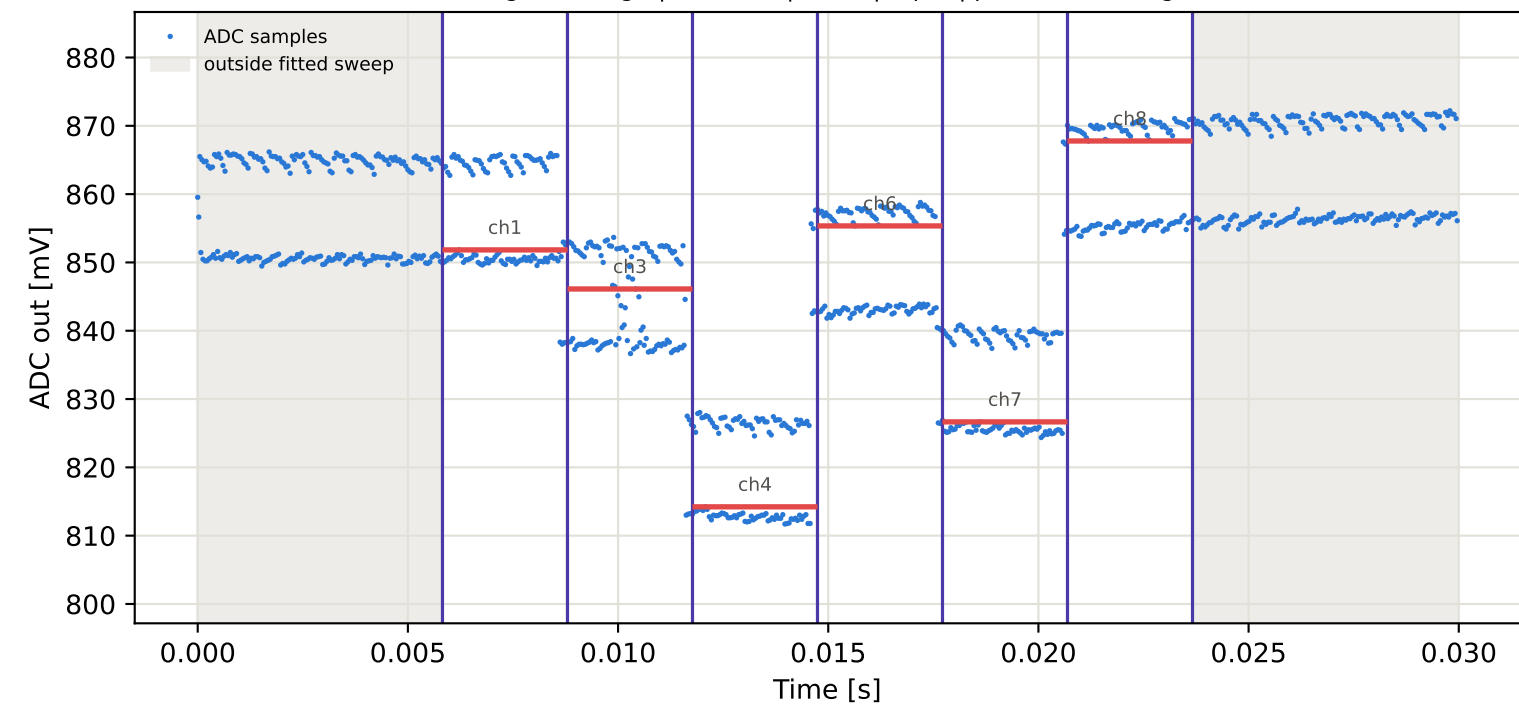
Tag16 &lt;- Tag5 | 955 MHz | run 0 | rep 1 | phase 149.78 deg
