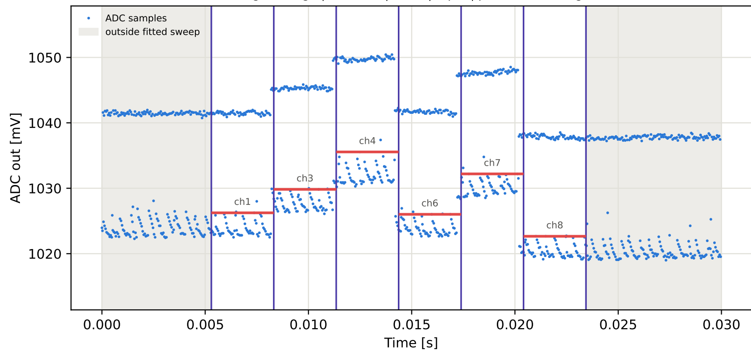
Tag7 &lt;- Tag4 | 955 MHz | run 0 | rep 1 | phase 121.25 deg
