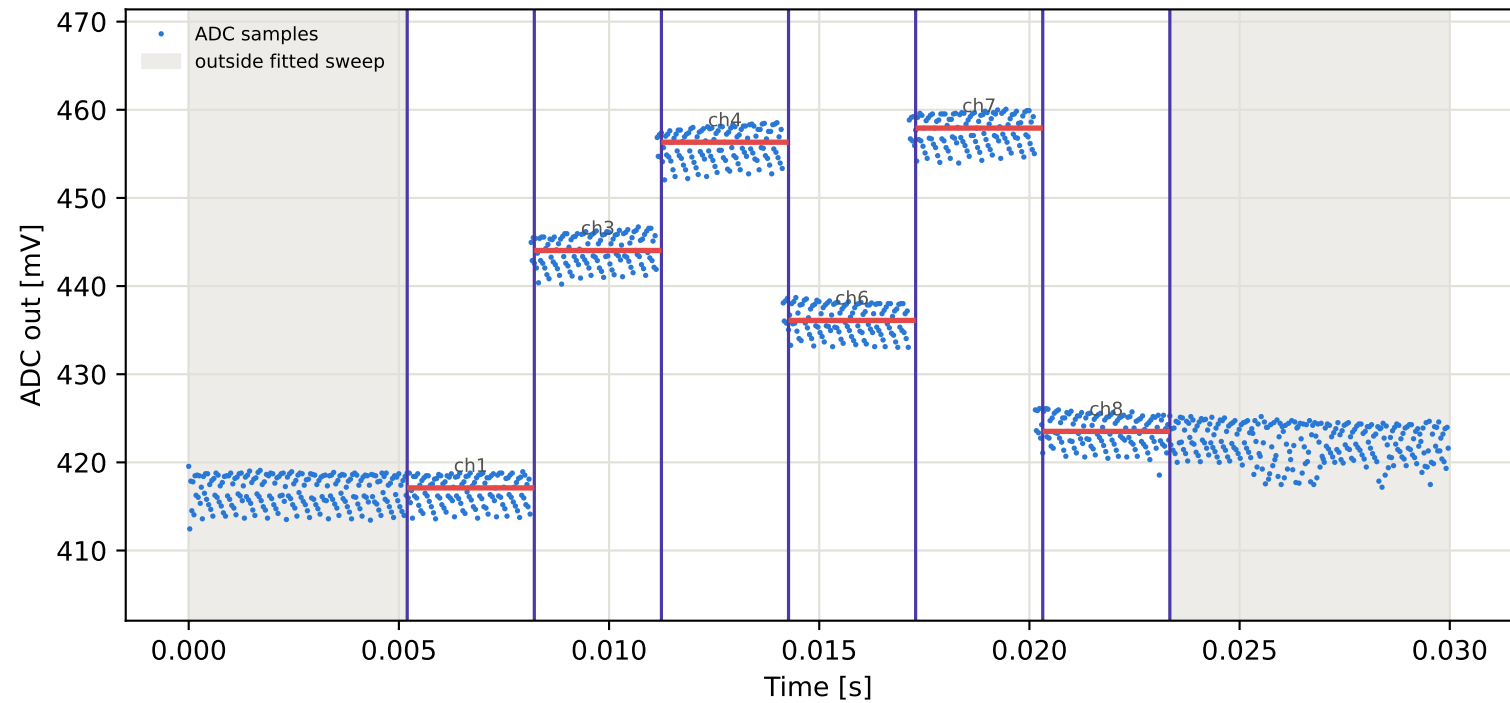
Tag3 &lt;- Tag2 | 845 MHz | run 0 | rep 1 | phase 77.34 deg
