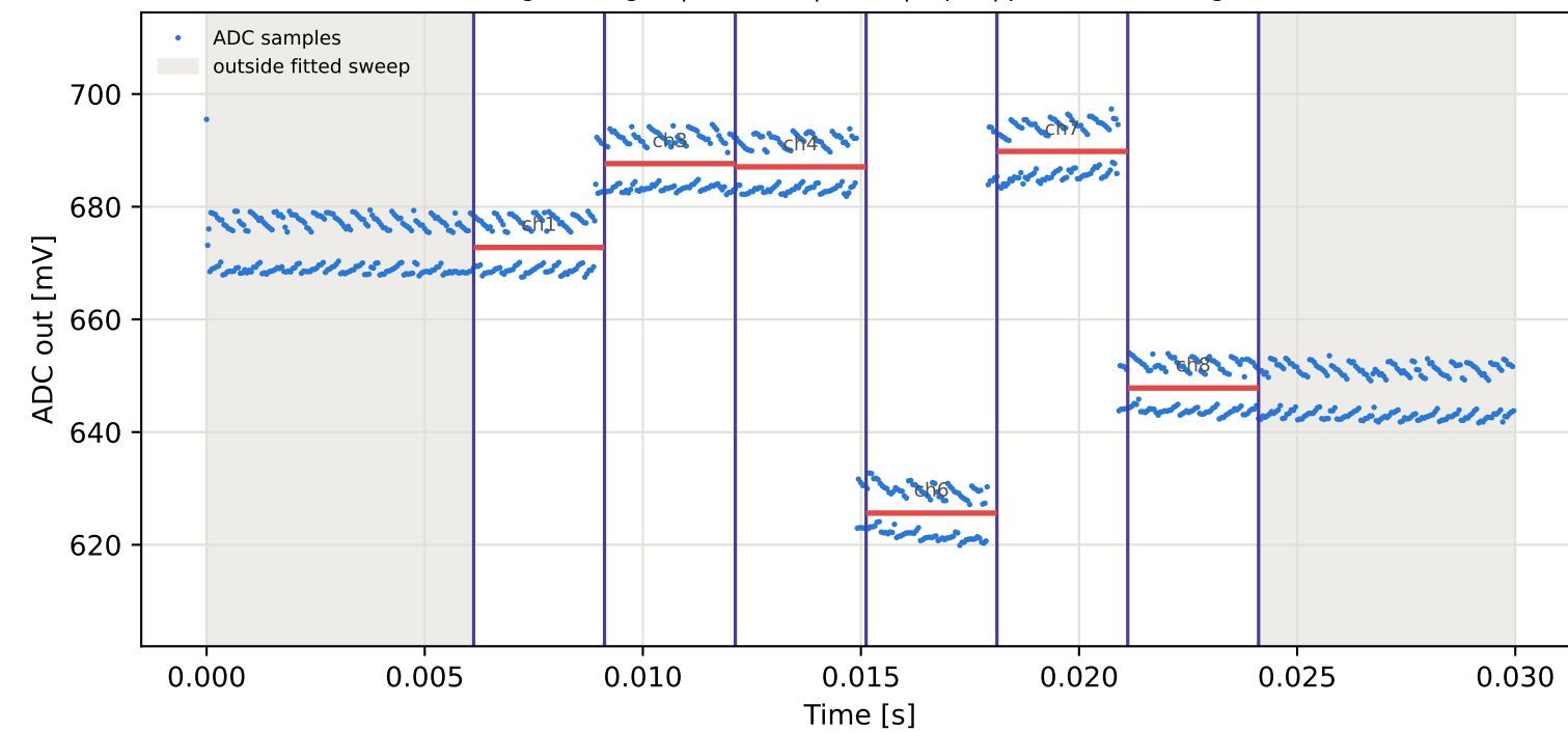
Tag7 &lt;- Tag3 | 945 MHz | run 0 | rep 1 | phase -31.22 deg
