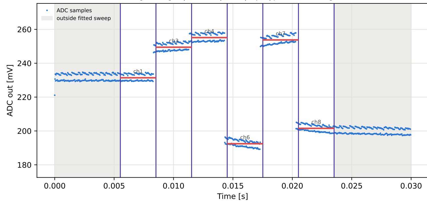
Tag6 &lt;- Tag3 | 925 MHz | run 0 | rep 1 | phase -160.30 deg
