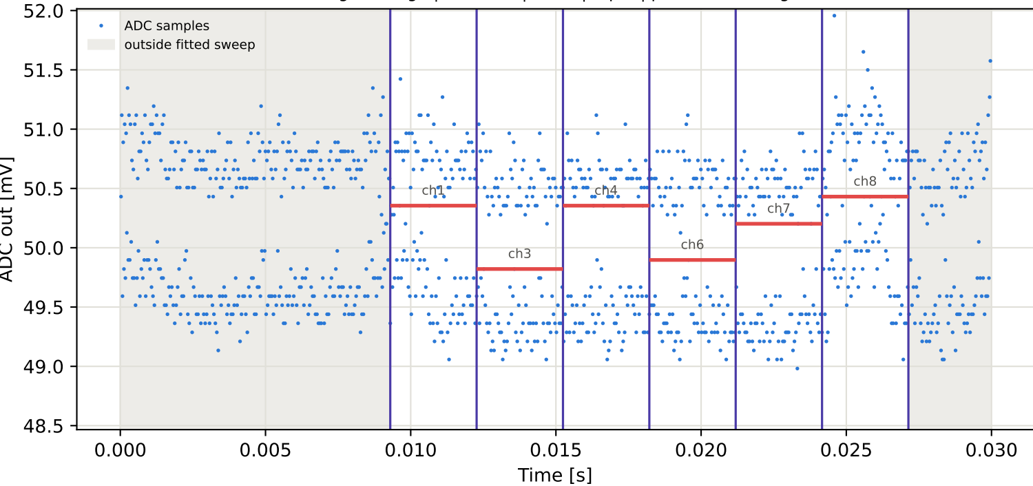
Tag4 &lt;- Tag2 | 775 MHz | run 0 | rep 1 | phase 14.70 deg
