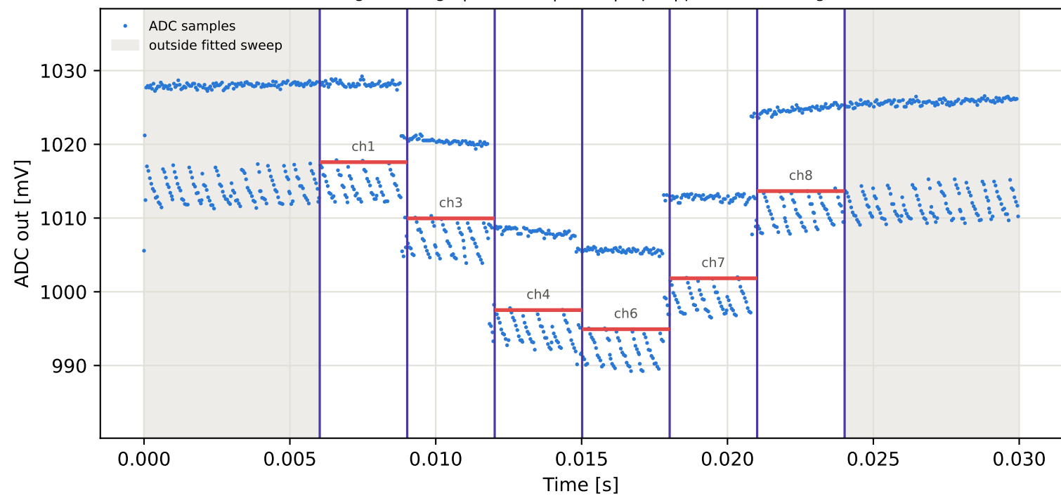
Tag16 &lt;- Tag15 | 915 MHz | run 0 | rep 1 | phase -171.57 deg
