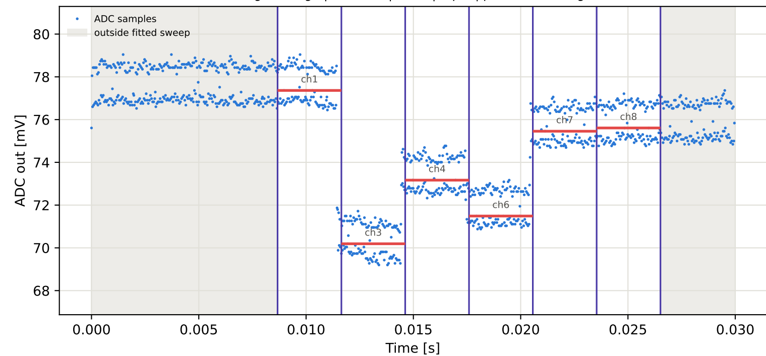
Tag6 &lt;- Tag5 | 775 MHz | run 0 | rep 1 | phase 73.43 deg
