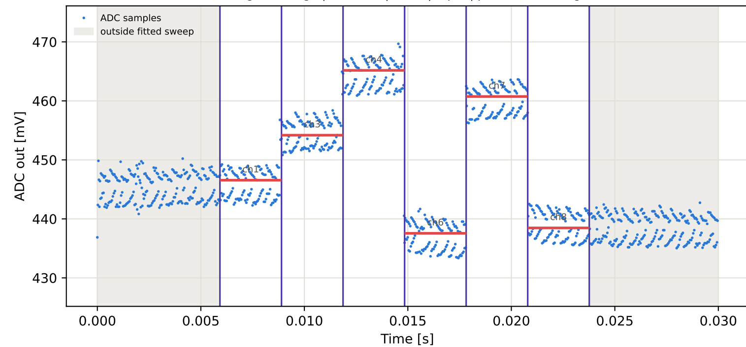
Tag16 &lt;- Tag1 | 975 MHz | run 0 | rep 1 | phase -170.74 deg
