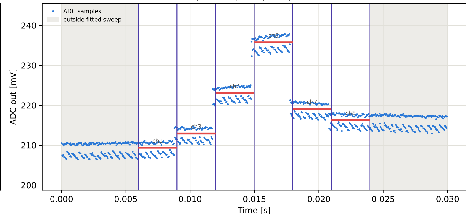
Tag4 &lt;- Tag8 | 915 MHz | run 0 | rep 1 | phase -49.18 deg
