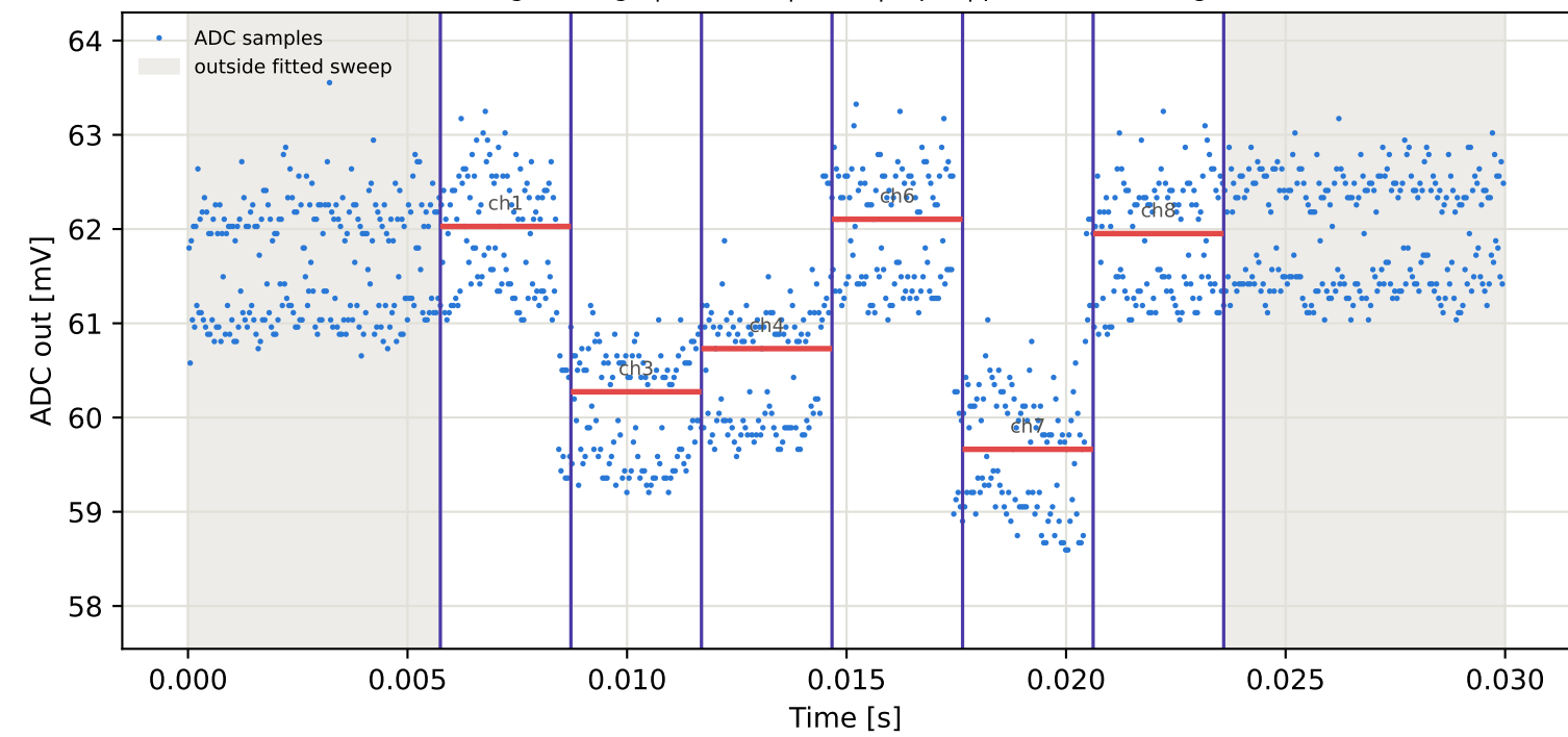
Tag9 &lt;- Tag6 | 785 MHz | run 0 | rep 1 | phase -146.03 deg
