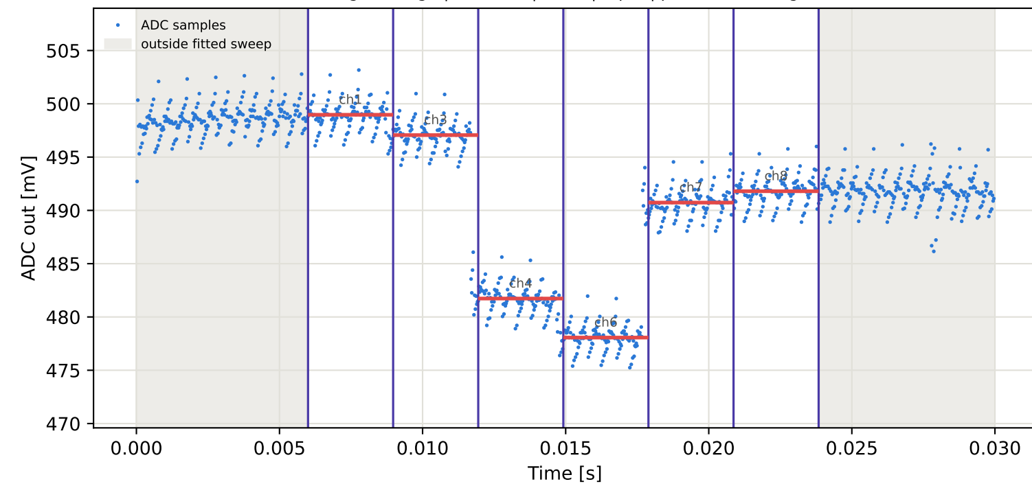
Tag9 &lt;- Tag10 | 965 MHz | run 0 | rep 1 | phase -162.84 deg
