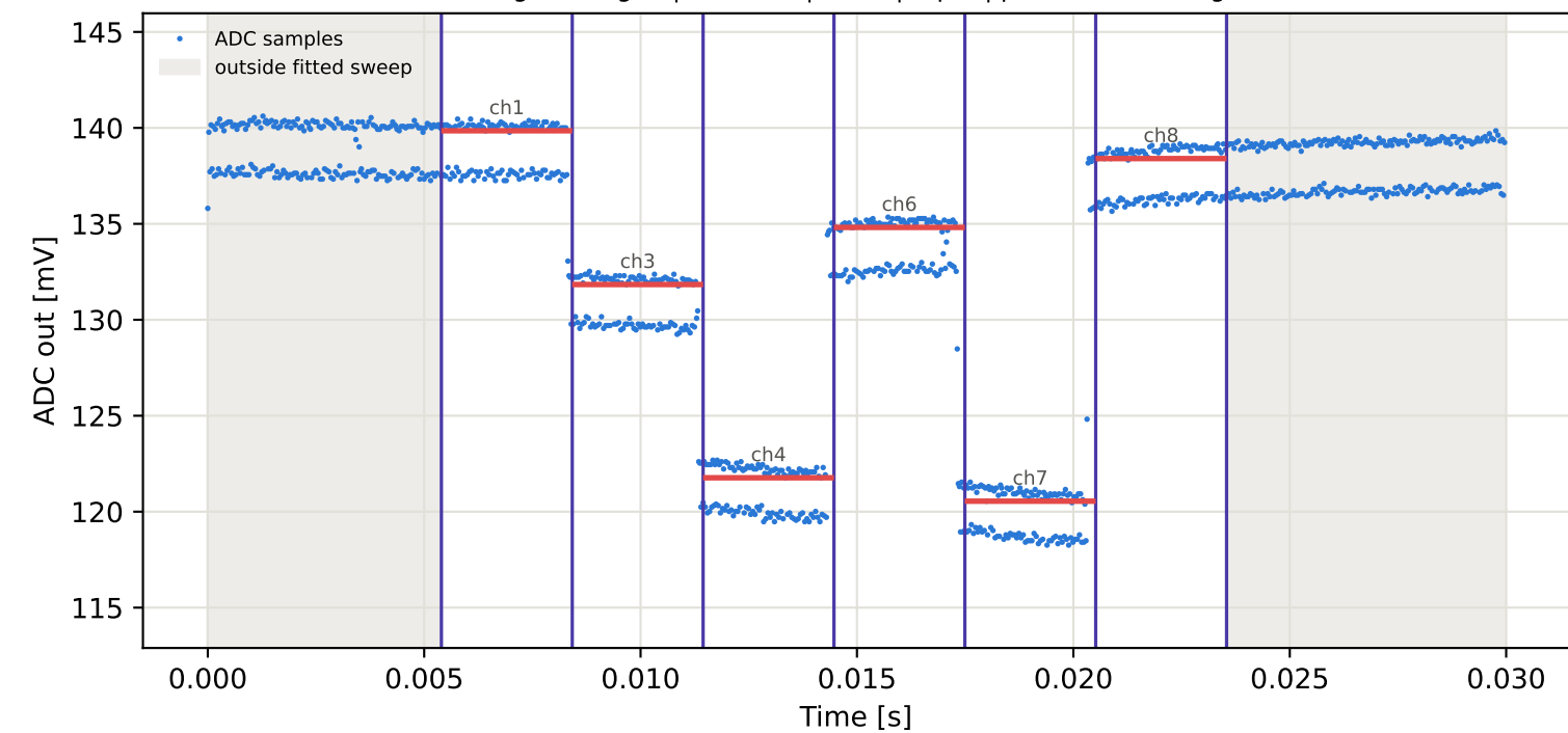
Tag3 &lt;- Tag16 | 795 MHz | run 0 | rep 1 | phase 110.98 deg
