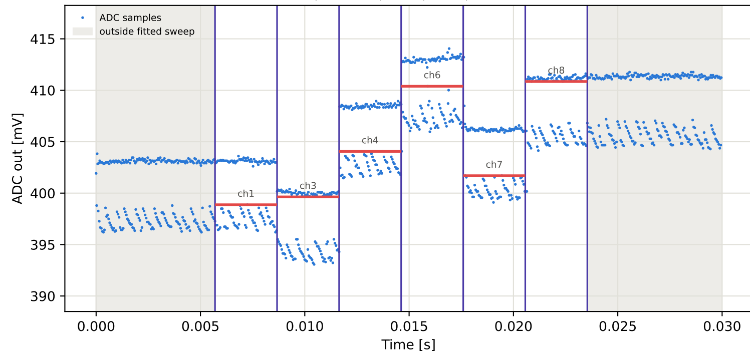
Tag6 &lt;- Tag5 | 845 MHz | run 0 | rep 1 | phase -160.84 deg
