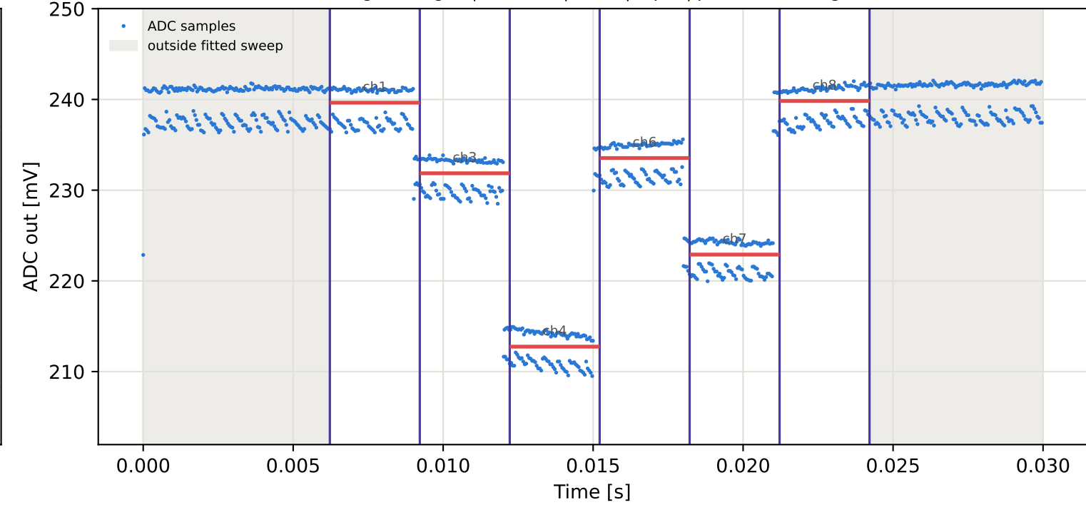
Tag6 &lt;- Tag3 | 995 MHz | run 0 | rep 1 | phase -90.82 deg
