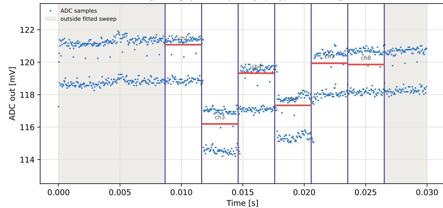
Tag3 &lt;- Tag6 | 775 MHz | run 0 | rep 1 | phase 102.51 deg
