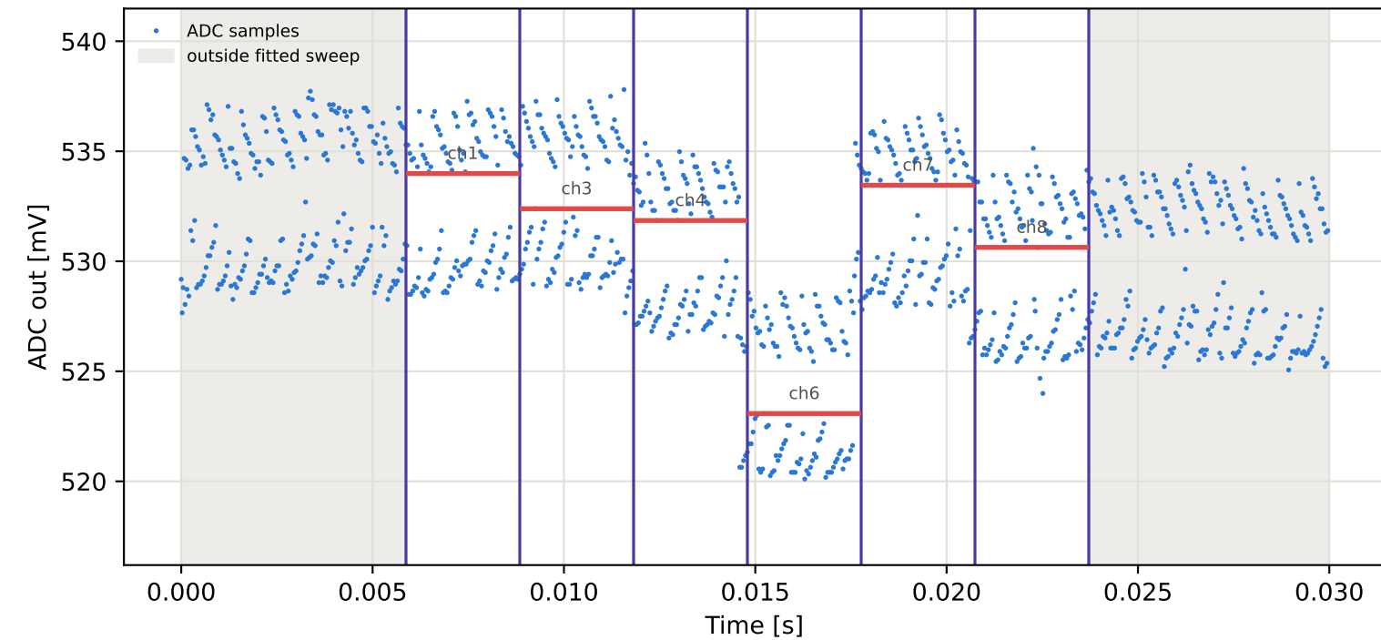
Tag8 &lt;- Tag15 | 935 MHz | run 0 | rep 1 | phase 94.12 deg
