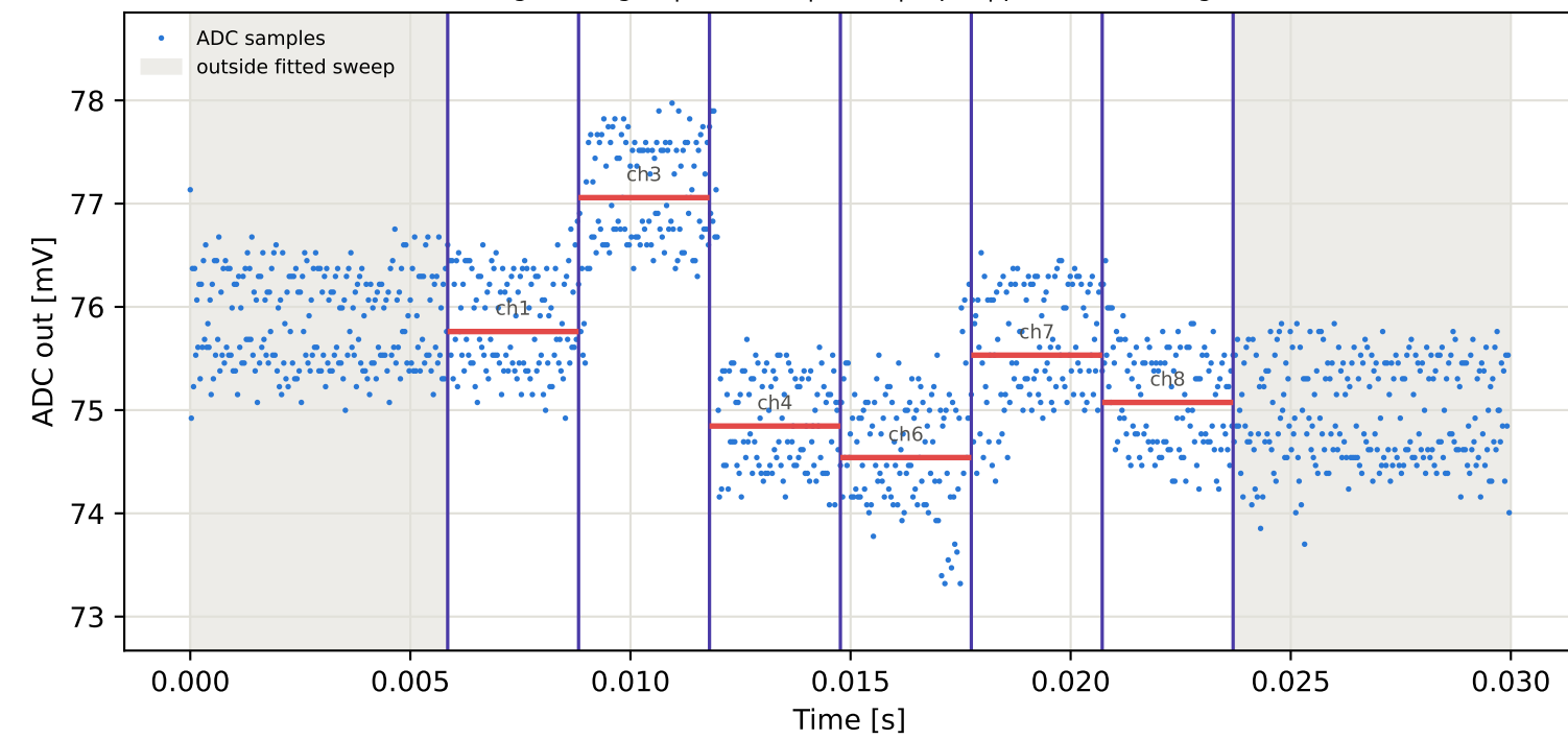
Tag1 &lt;- Tag16 | 795 MHz | run 0 | rep 1 | phase 129.22 deg
