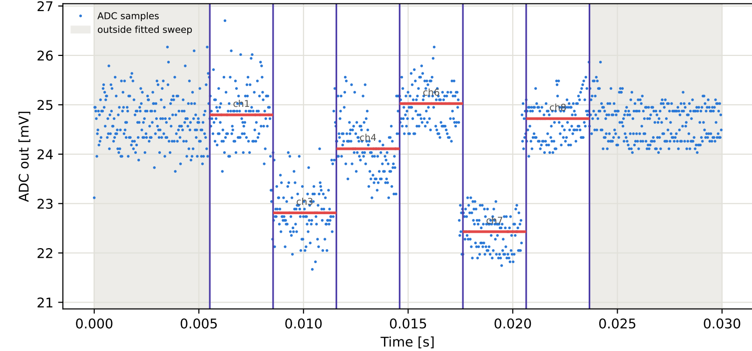
Tag2 &lt;- Tag16 | 785 MHz | run 0 | rep 1 | phase 143.00 deg
