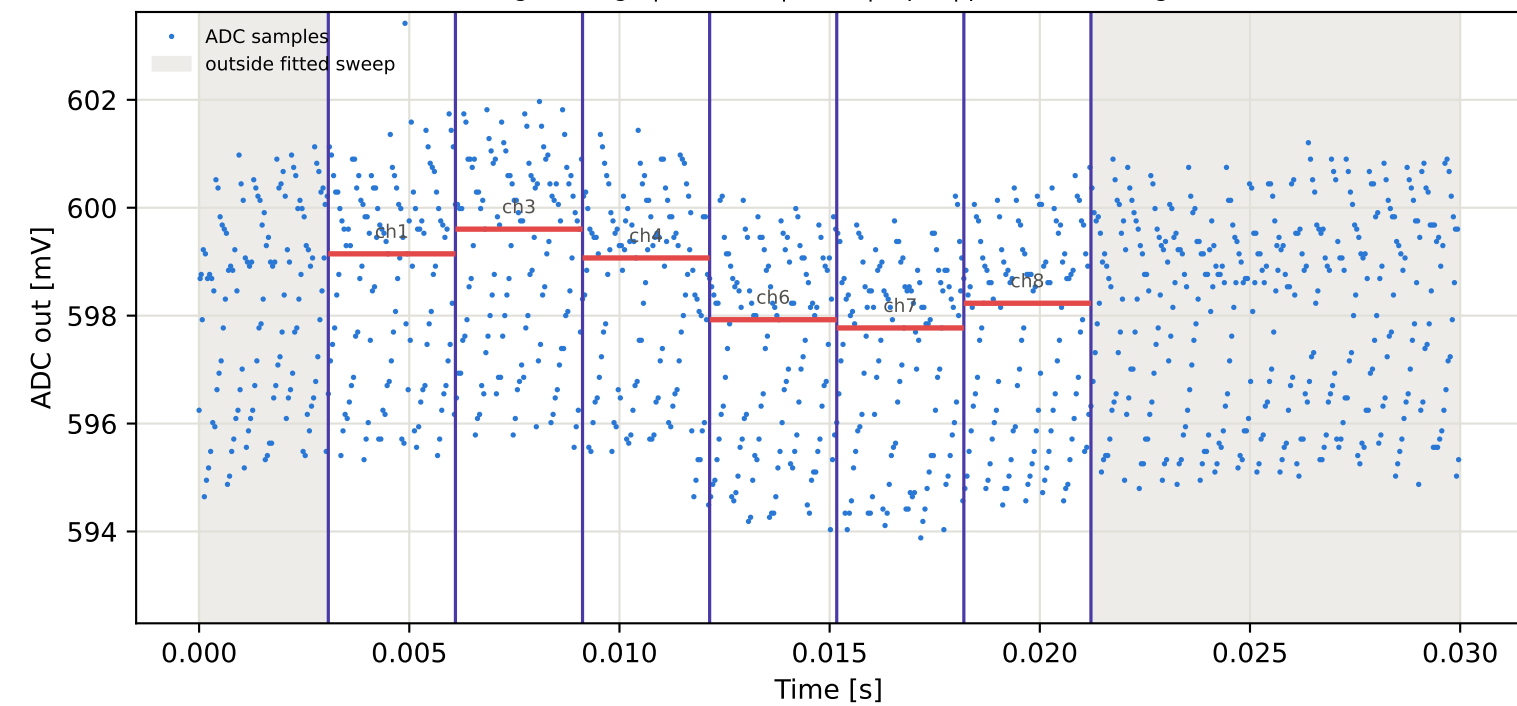
Tag9 &lt;- Tag10 | 855 MHz | run 0 | rep 1 | phase 58.69 deg
