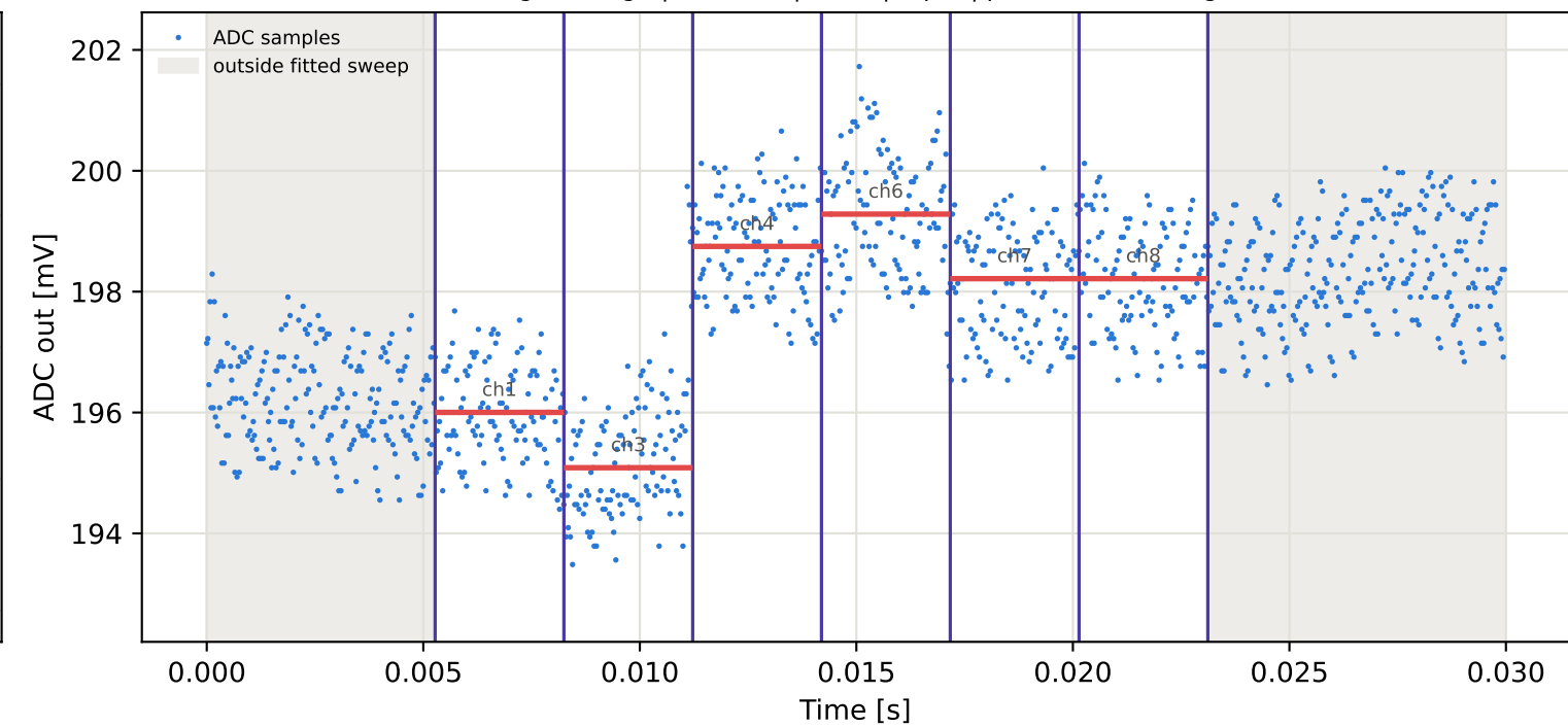
Tag9 &lt;- Tag15 | 845 MHz | run 0 | rep 1 | phase 51.49 deg
