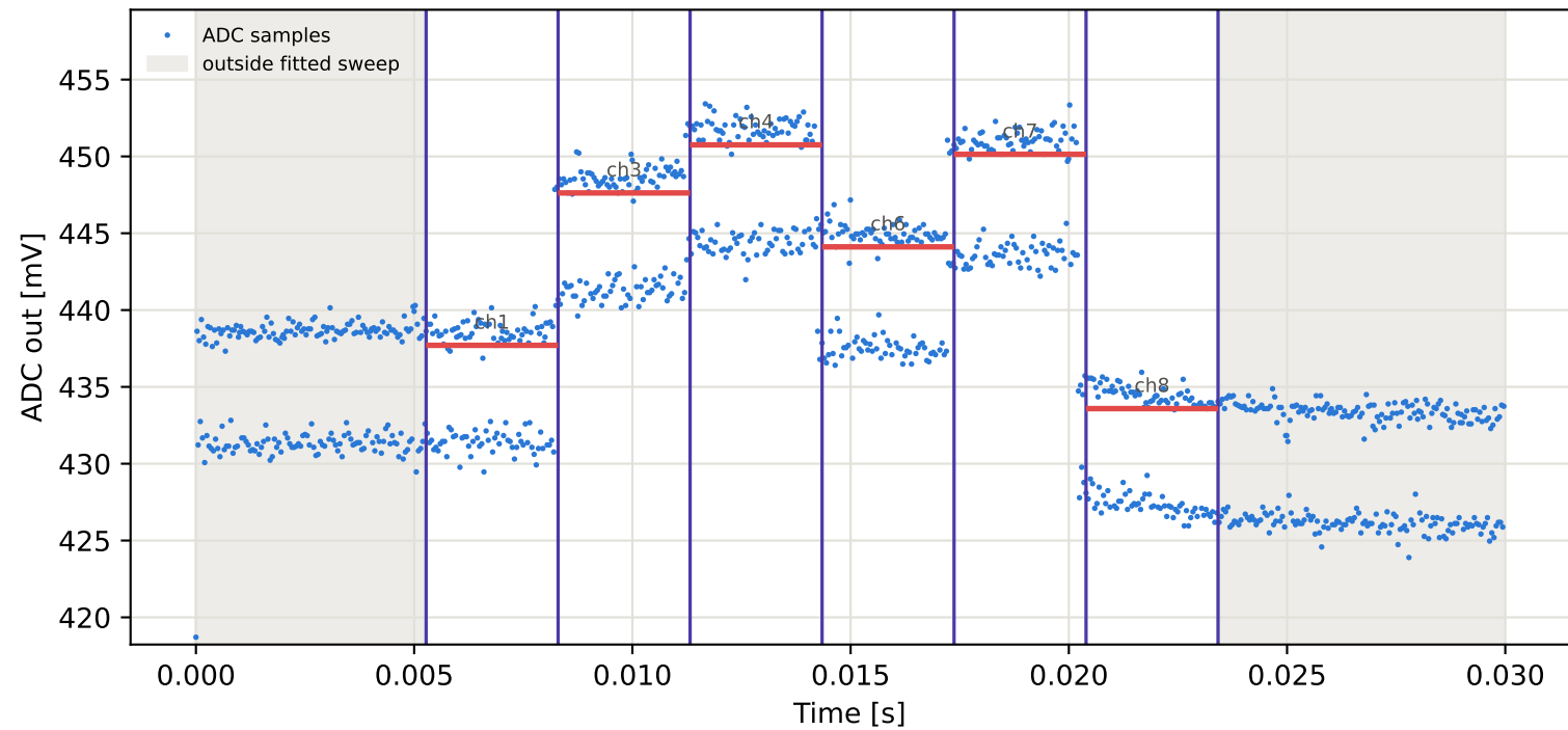
Tag4 &lt;- Tag3 | 885 MHz | run 0 | rep 1 | phase -61.12 deg
