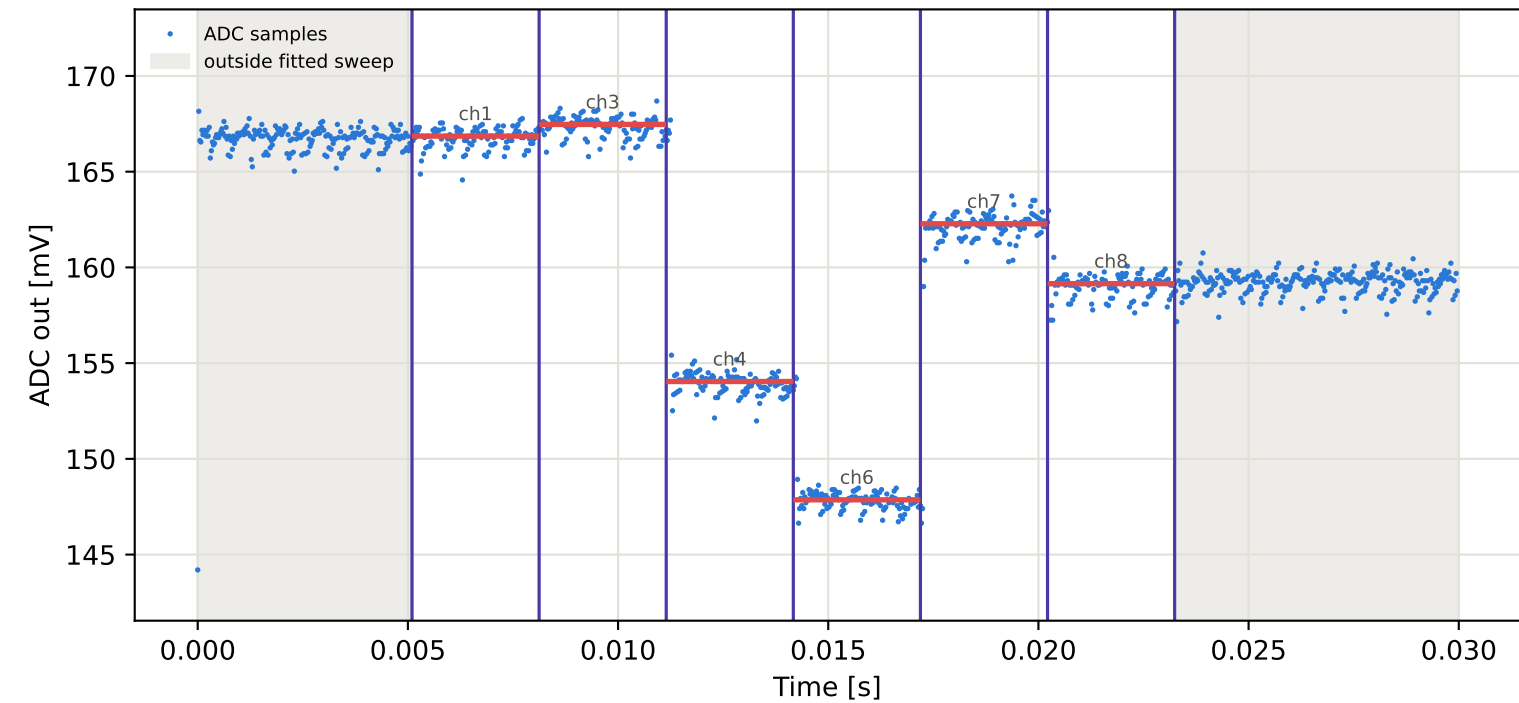
Tag4 &lt;- Tag3 | 975 MHz | run 0 | rep 1 | phase 18.70 deg
