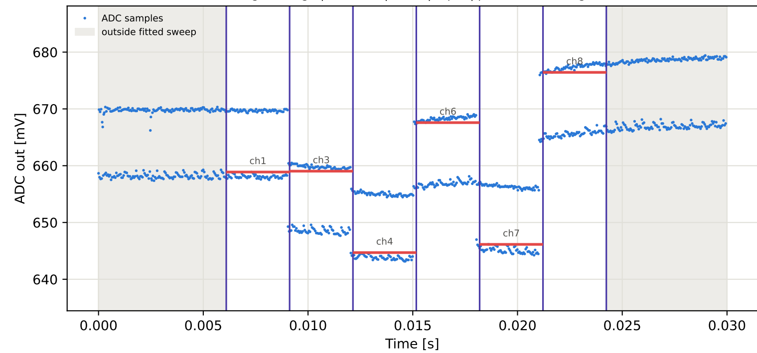
Tag5 &lt;- Tag9 | 895 MHz | run 0 | rep 1 | phase 12.38 deg
