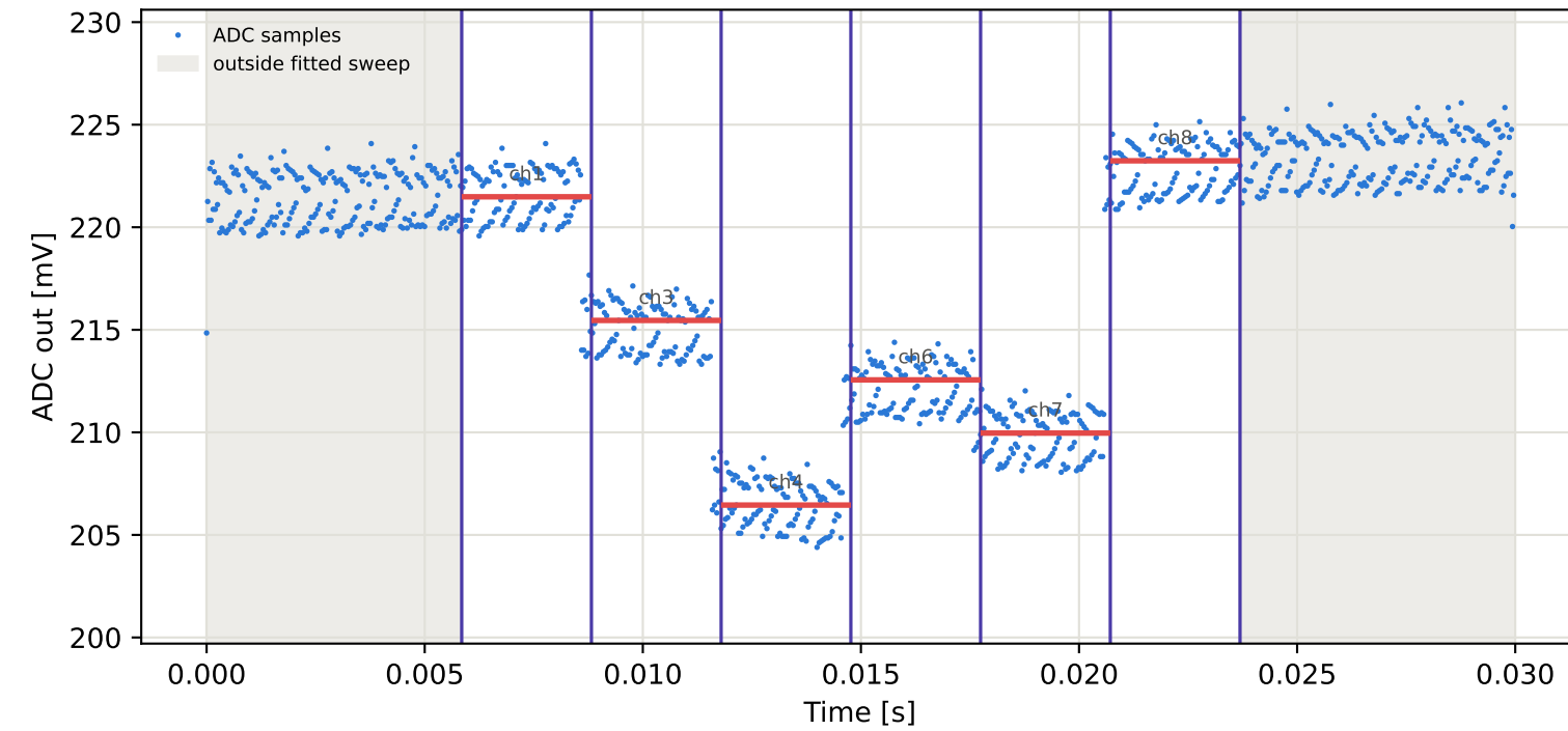
Tag4 &lt;- Tag9 | 915 MHz | run 0 | rep 1 | phase 28.02 deg
