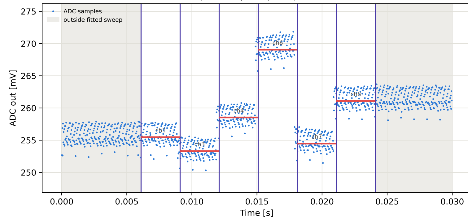
Tag1 &lt;- Tag16 | 965 MHz | run 0 | rep 1 | phase -47.14 deg
