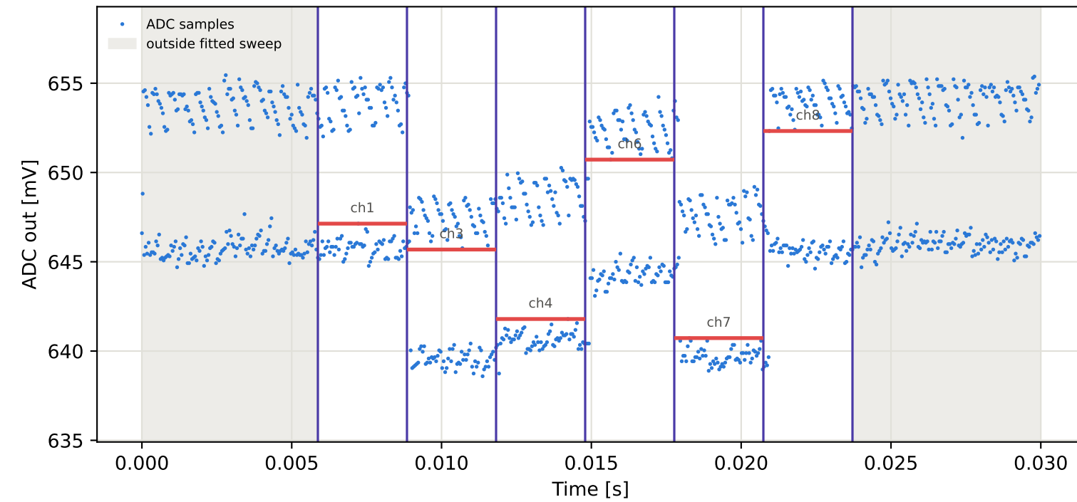
Tag16 &lt;- Tag6 | 835 MHz | run 0 | rep 1 | phase 44.91 deg
