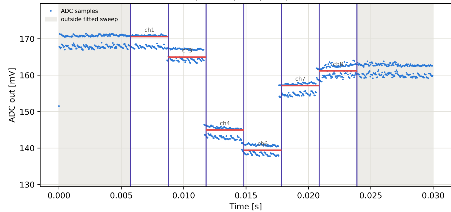
Tag6 &lt;- Tag3 | 955 MHz | run 0 | rep 1 | phase -116.91 deg
