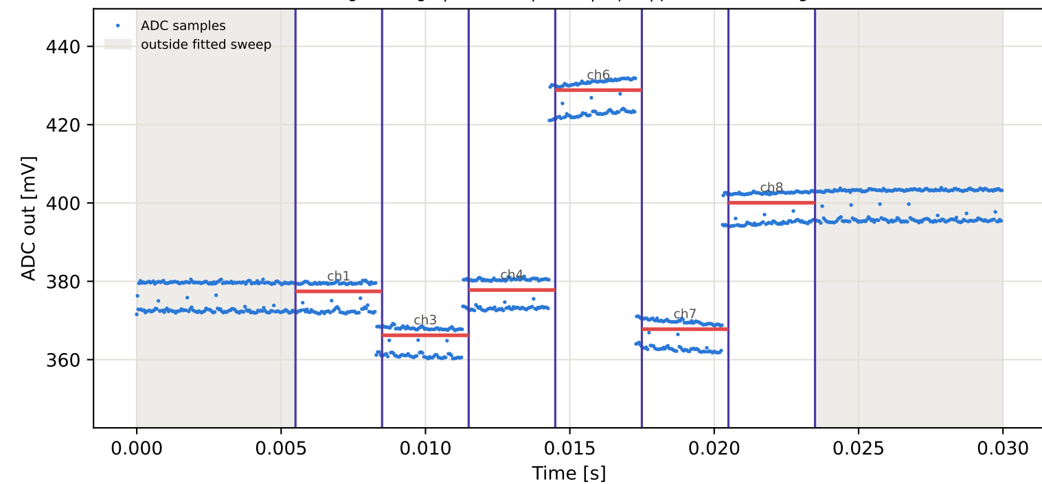
Tag5 &lt;- Tag3 | 975 MHz | run 0 | rep 1 | phase 178.06 deg
