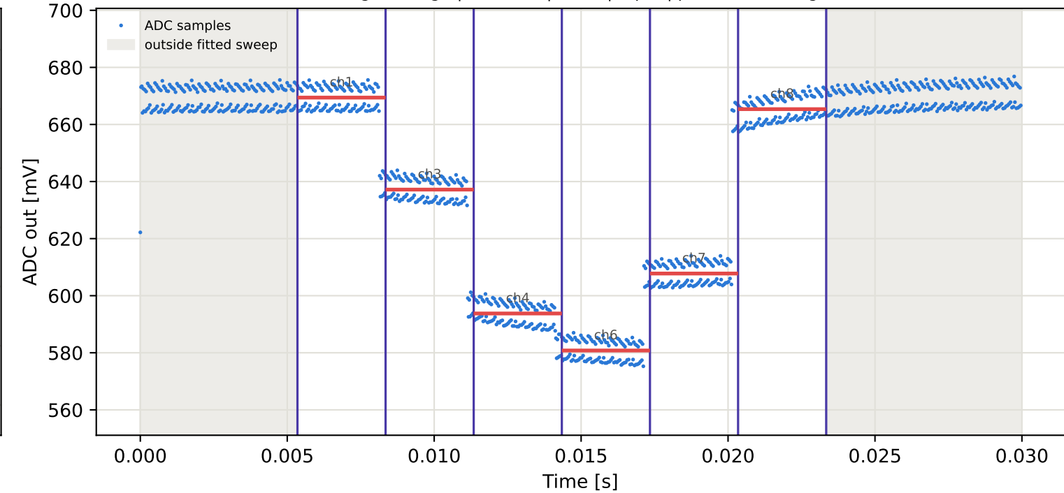
Tag3 &lt;- Tag7 | 905 MHz | run 0 | rep 1 | phase -98.19 deg
