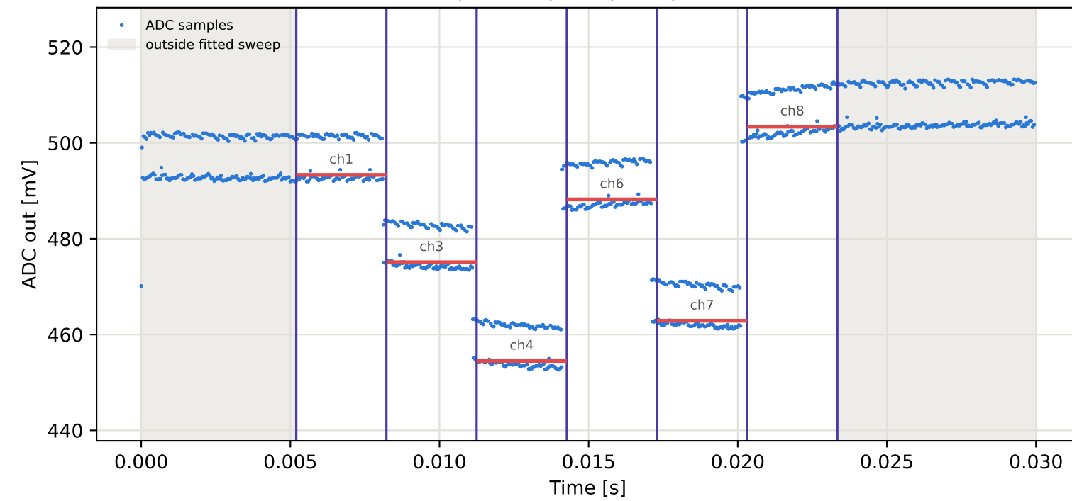
Tag4 &lt;- Tag9 | 935 MHz | run 0 | rep 1 | phase 102.48 deg
