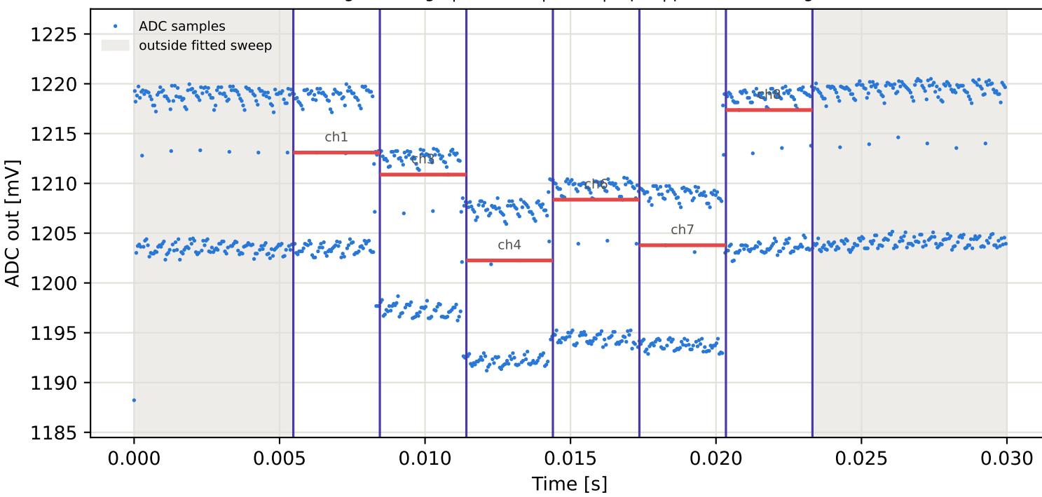
Tag15 &lt;- Tag1 | 895 MHz | run 0 | rep 1 | phase 87.14 deg
