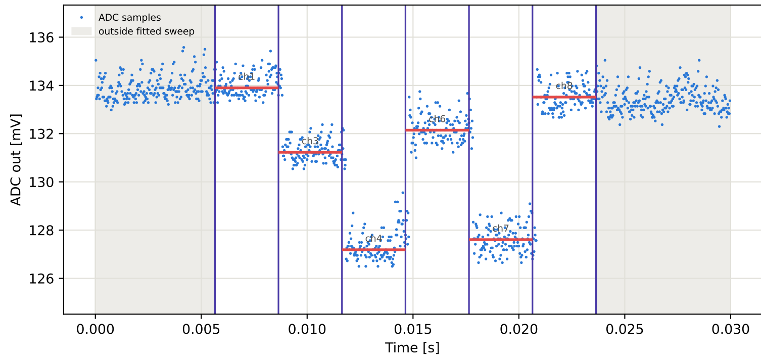
Tag2 &lt;- Tag10 | 785 MHz | run 0 | rep 1 | phase 175.11 deg
