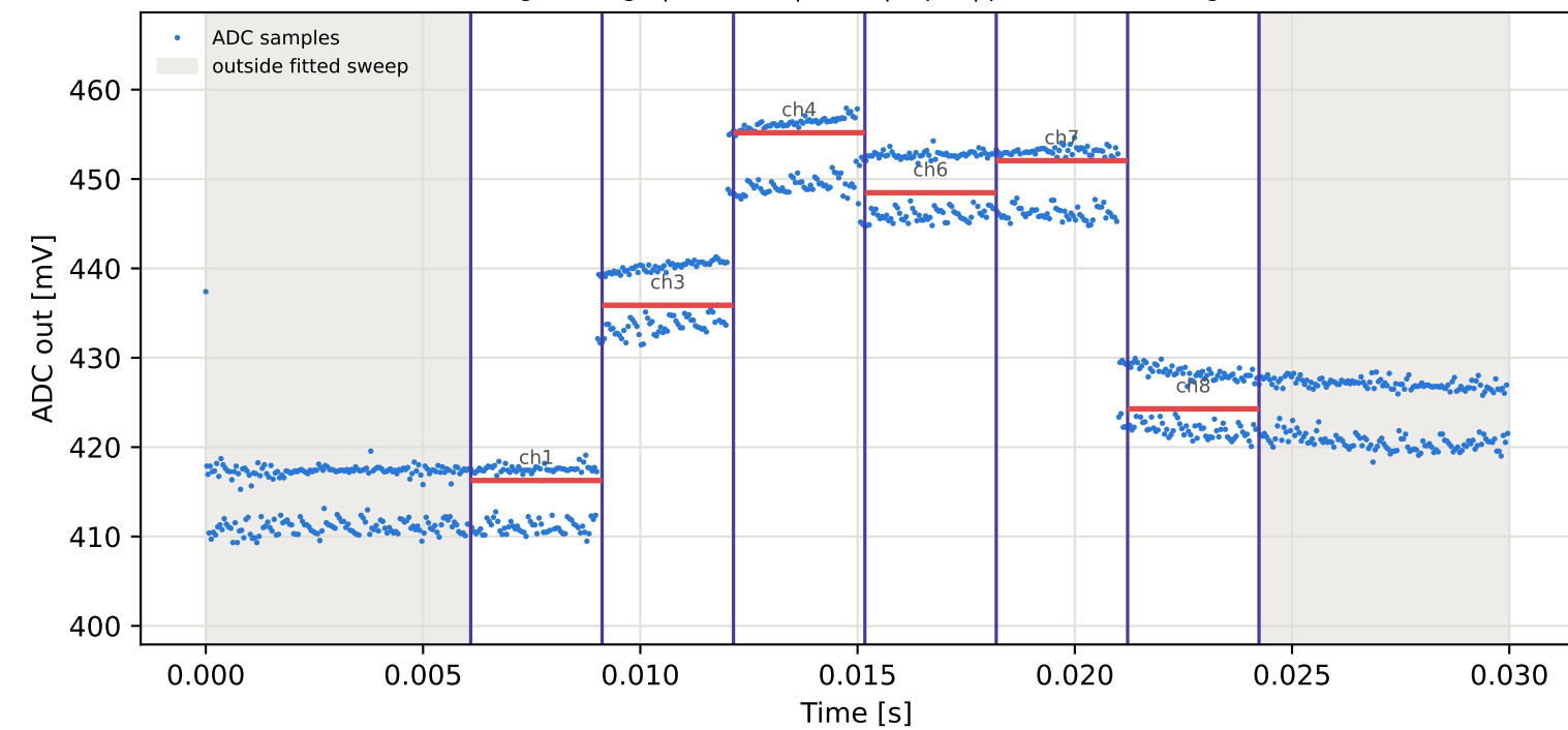
Tag4 &lt;- Tag15 | 885 MHz | run 0 | rep 1 | phase -114.47 deg
