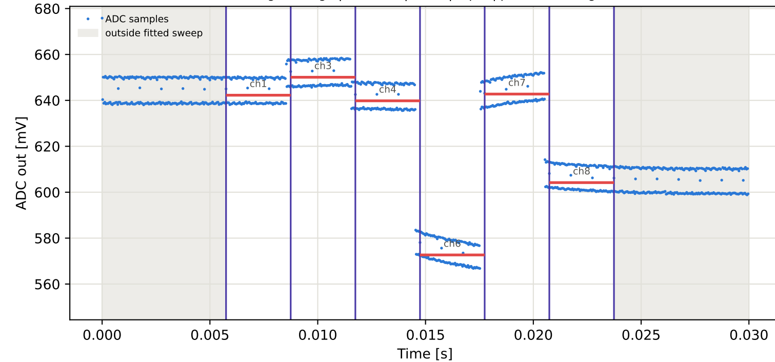
Tag3 &lt;- Tag8 | 905 MHz | run 0 | rep 1 | phase 91.40 deg
