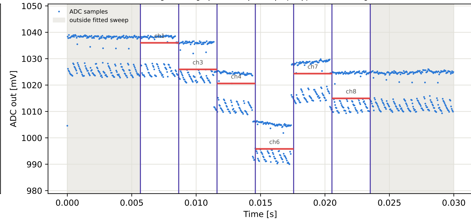
Tag16 &lt;- Tag7 | 905 MHz | run 0 | rep 1 | phase 22.91 deg
