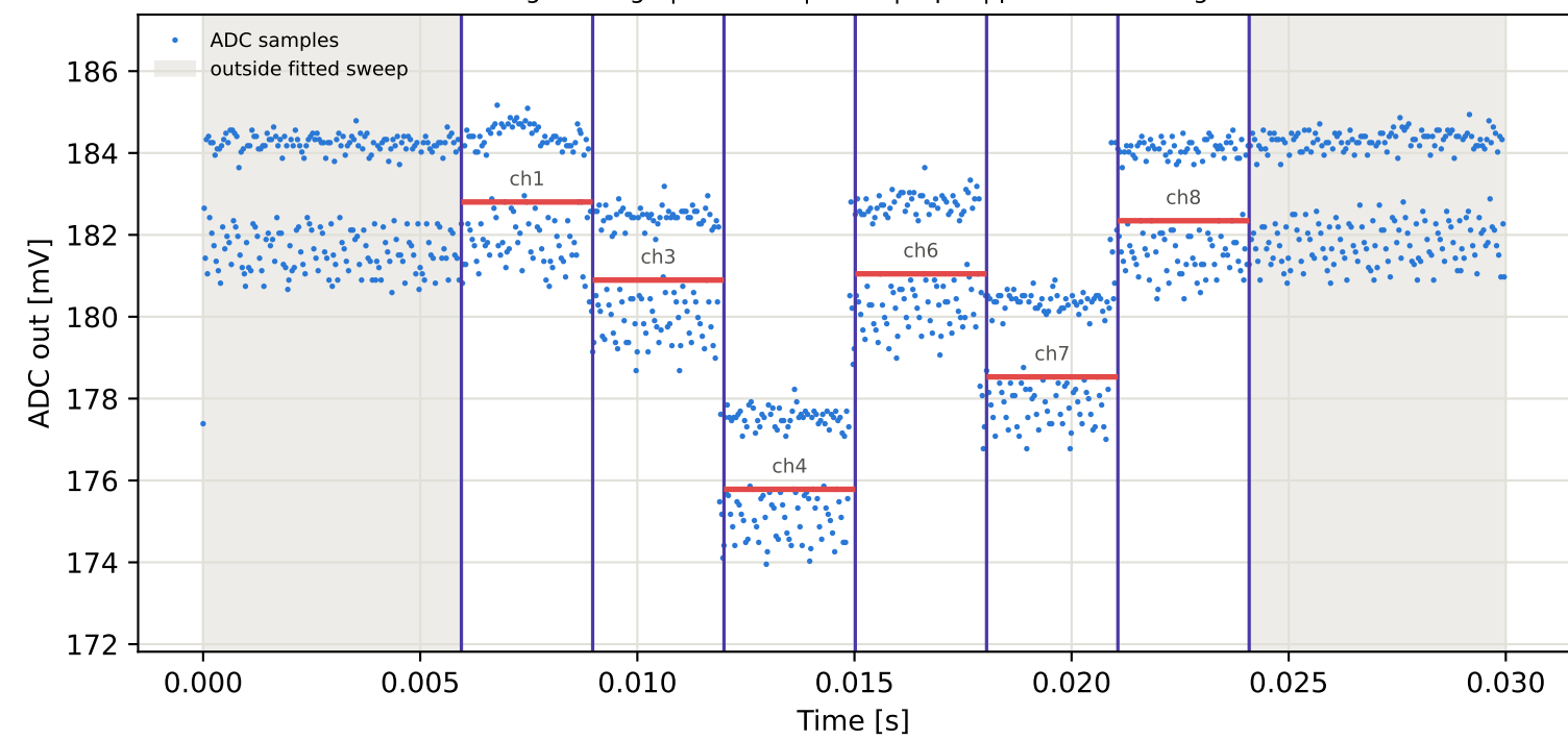
Tag3 &lt;- Tag15 | 995 MHz | run 0 | rep 1 | phase 101.02 deg
