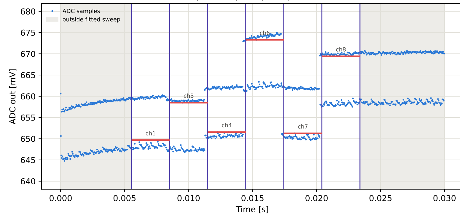
Tag5 &lt;- Tag8 | 895 MHz | run 0 | rep 1 | phase -96.81 deg
