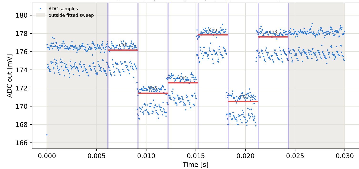
Tag5 &lt;- Tag2 | 805 MHz | run 0 | rep 1 | phase -63.15 deg
