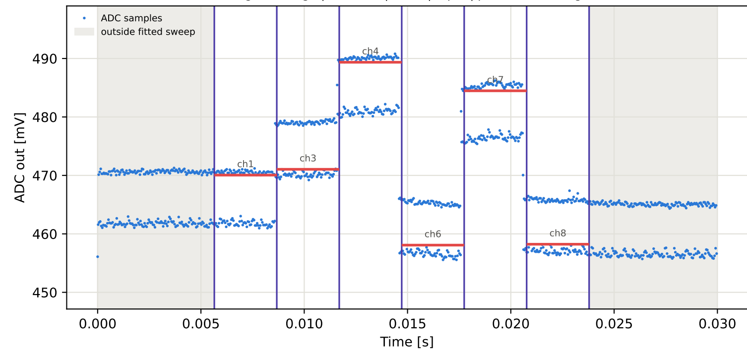
Tag16 &lt;- Tag1 | 995 MHz | run 0 | rep 1 | phase -49.30 deg
