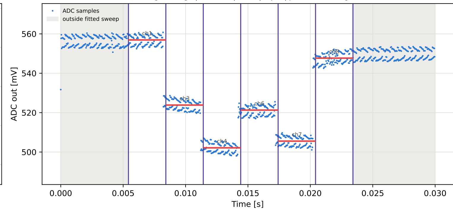
Tag5 &lt;- Tag9 | 875 MHz | run 0 | rep 1 | phase -8.30 deg
