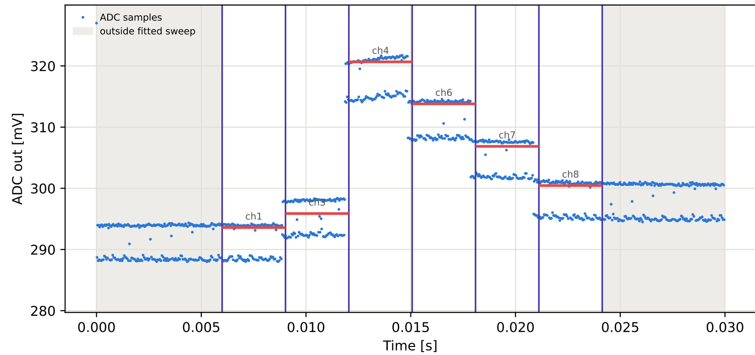
Tag10 &lt;- Tag3 | 985 MHz | run 0 | rep 1 | phase -73.84 deg
