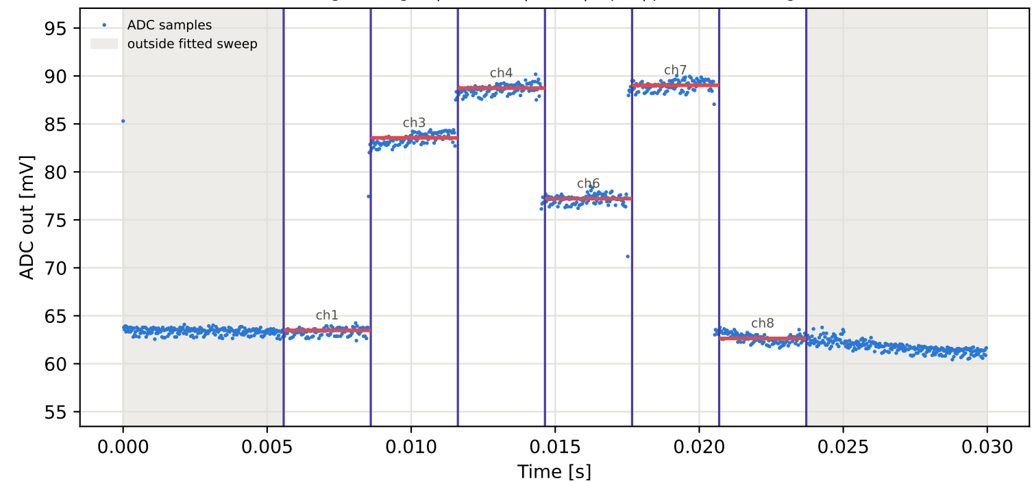
Tag1 &lt;- Tag2 | 875 MHz | run 0 | rep 1 | phase 112.31 deg
