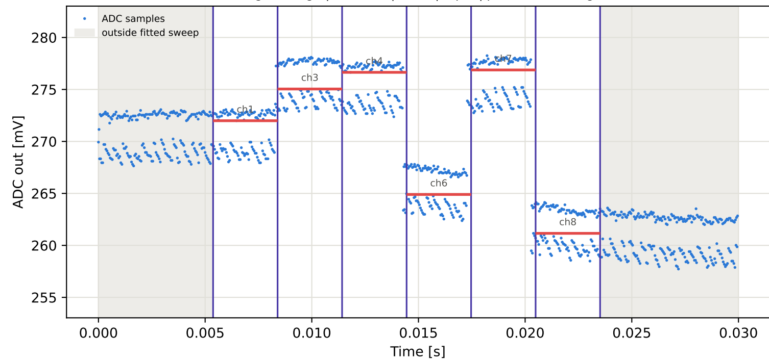
Tag9 &lt;- Tag15 | 895 MHz | run 0 | rep 1 | phase 93.12 deg
