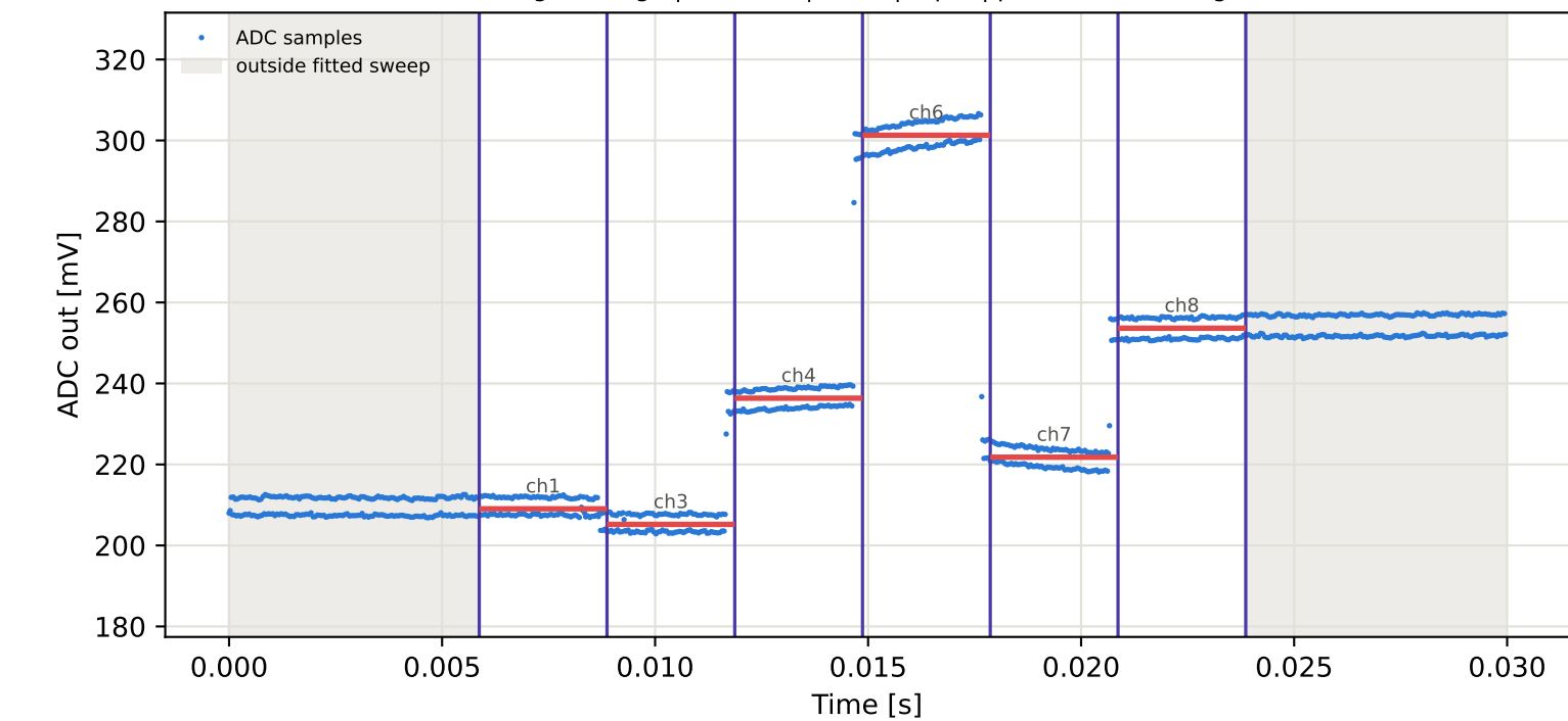
Tag7 &lt;- Tag10 | 925 MHz | run 0 | rep 1 | phase -11.19 deg
