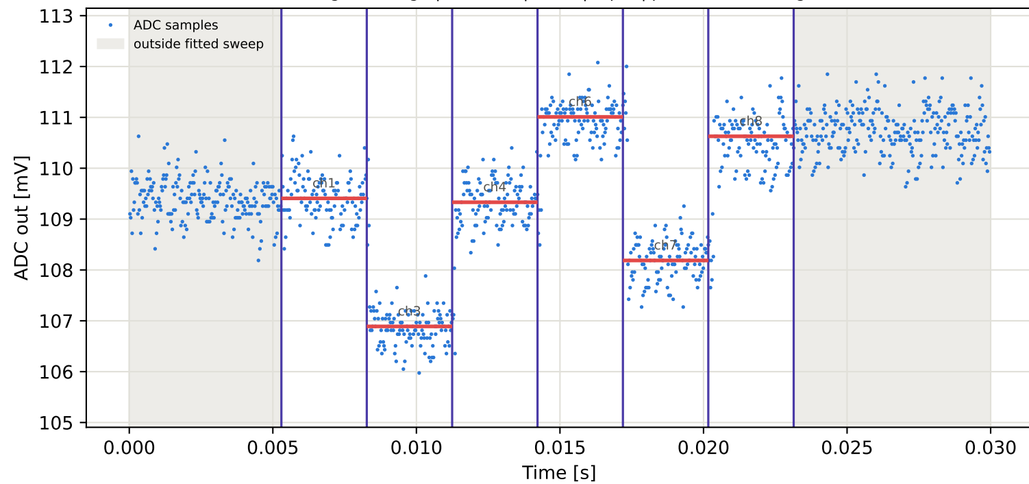
Tag2 &lt;- Tag10 | 795 MHz | run 0 | rep 1 | phase -121.08 deg
