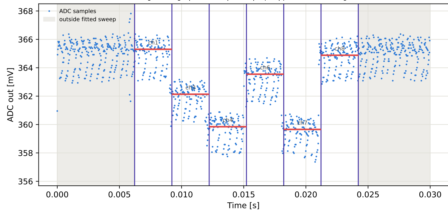
Tag7 &lt;- Tag6 | 805 MHz | run 0 | rep 1 | phase 111.30 deg
