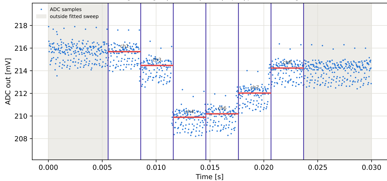
Tag1 &lt;- Tag2 | 955 MHz | run 0 | rep 1 | phase 167.29 deg
