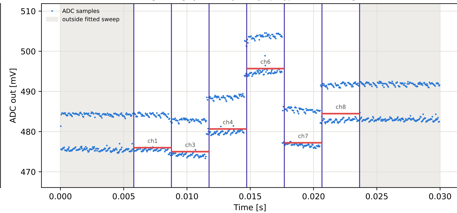
Tag4 &lt;- Tag8 | 935 MHz | run 0 | rep 1 | phase -59.34 deg
