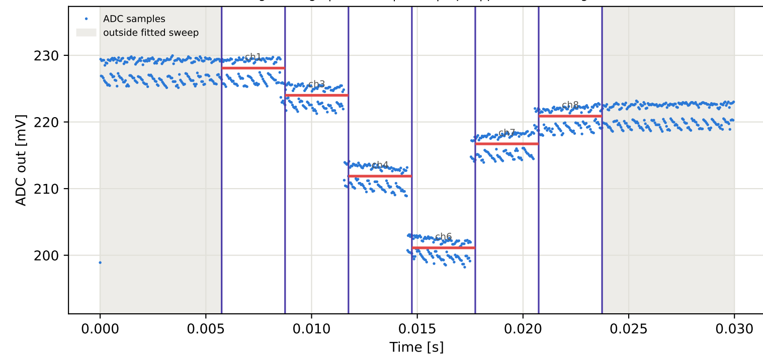
Tag4 &lt;- Tag2 | 915 MHz | run 0 | rep 1 | phase 39.43 deg
