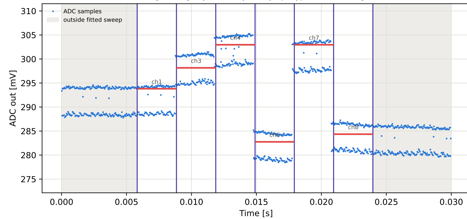
Tag6 &lt;- Tag2 | 945 MHz | run 0 | rep 1 | phase -60.55 deg
