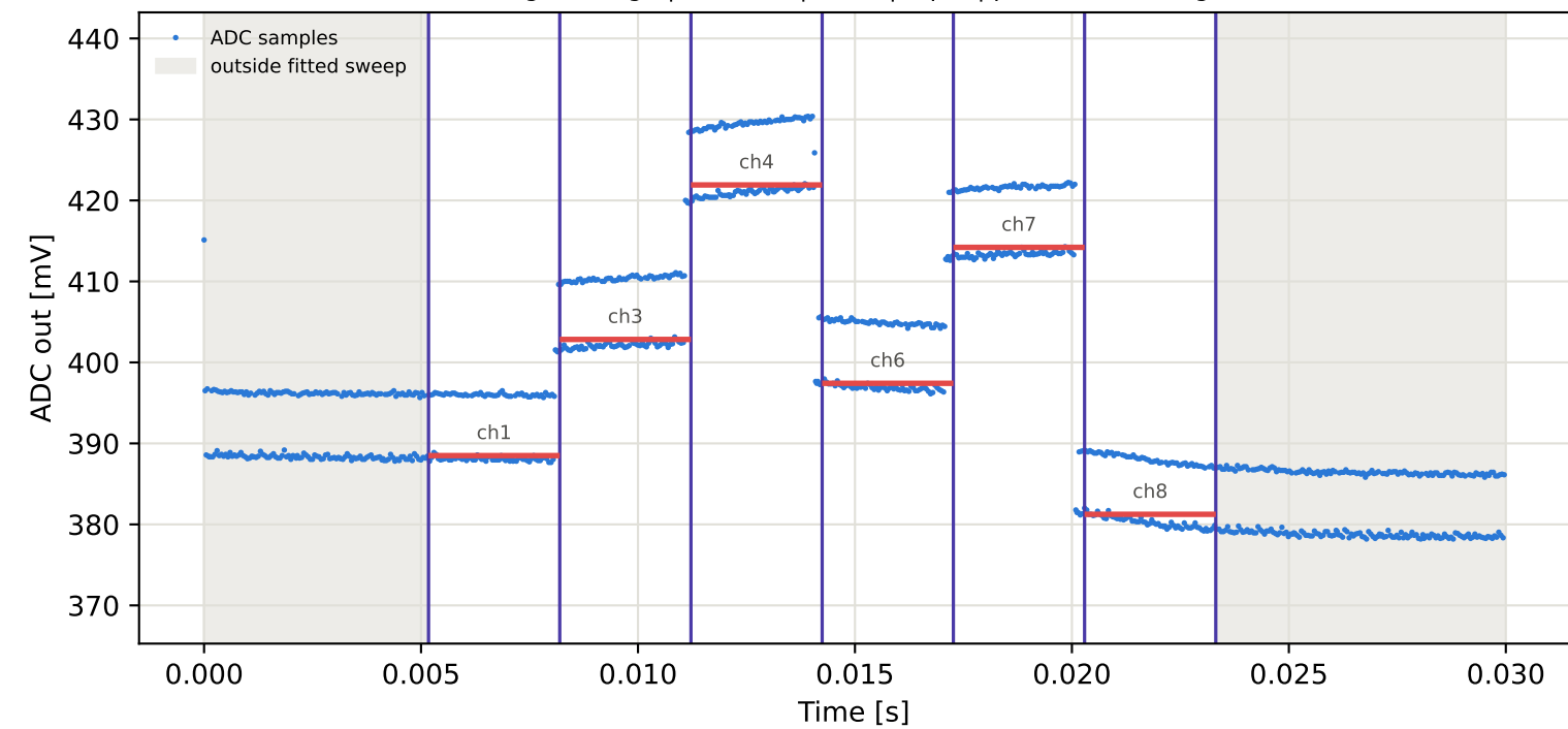
Tag1 &lt;- Tag8 | 925 MHz | run 0 | rep 1 | phase 21.37 deg
