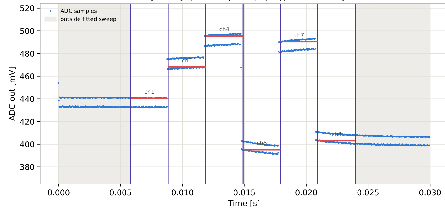
Tag1 &lt;- Tag9 | 975 MHz | run 0 | rep 1 | phase -44.36 deg
