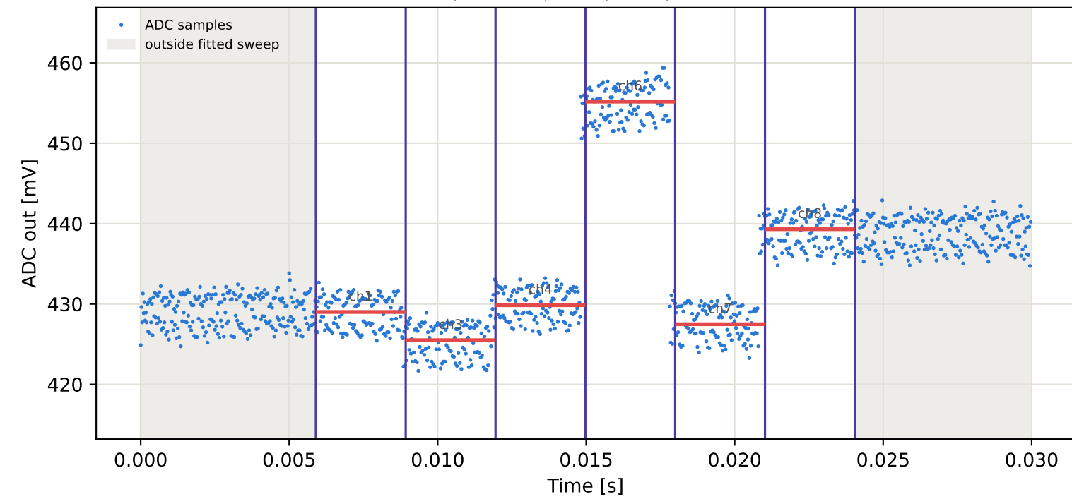
Tag4 &lt;- Tag2 | 885 MHz | run 0 | rep 1 | phase -170.97 deg
