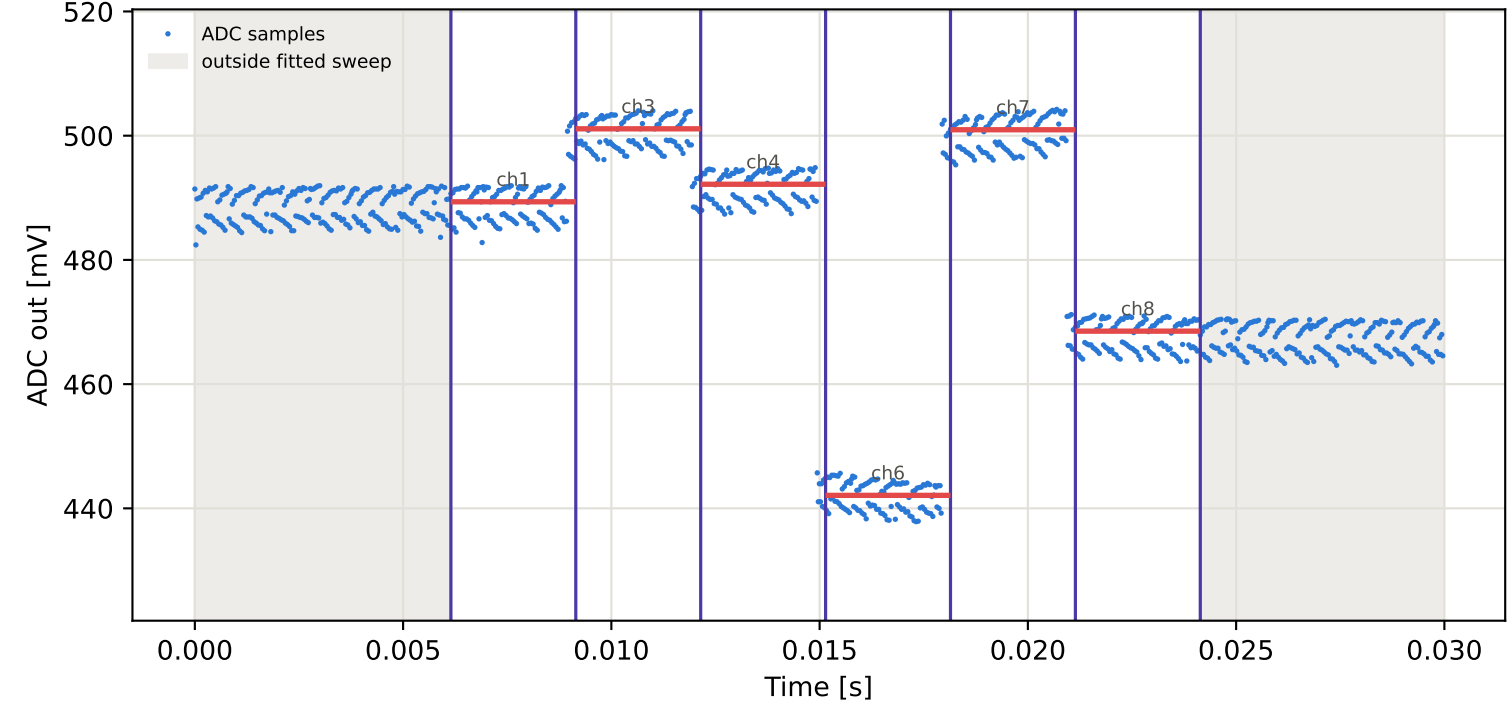
Tag8 &lt;- Tag16 | 965 MHz | run 0 | rep 1 | phase -136.81 deg
