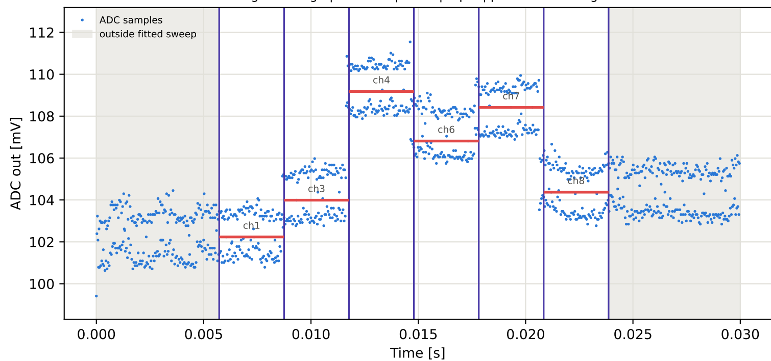
Tag16 &lt;- Tag7 | 795 MHz | run 0 | rep 1 | phase -99.52 deg
