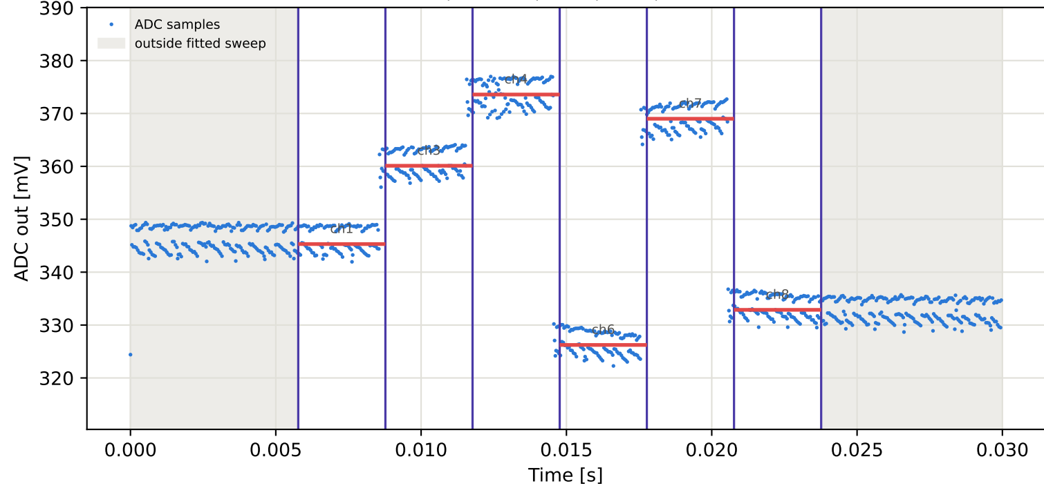
Tag6 &lt;- Tag10 | 985 MHz | run 0 | rep 1 | phase -46.84 deg
