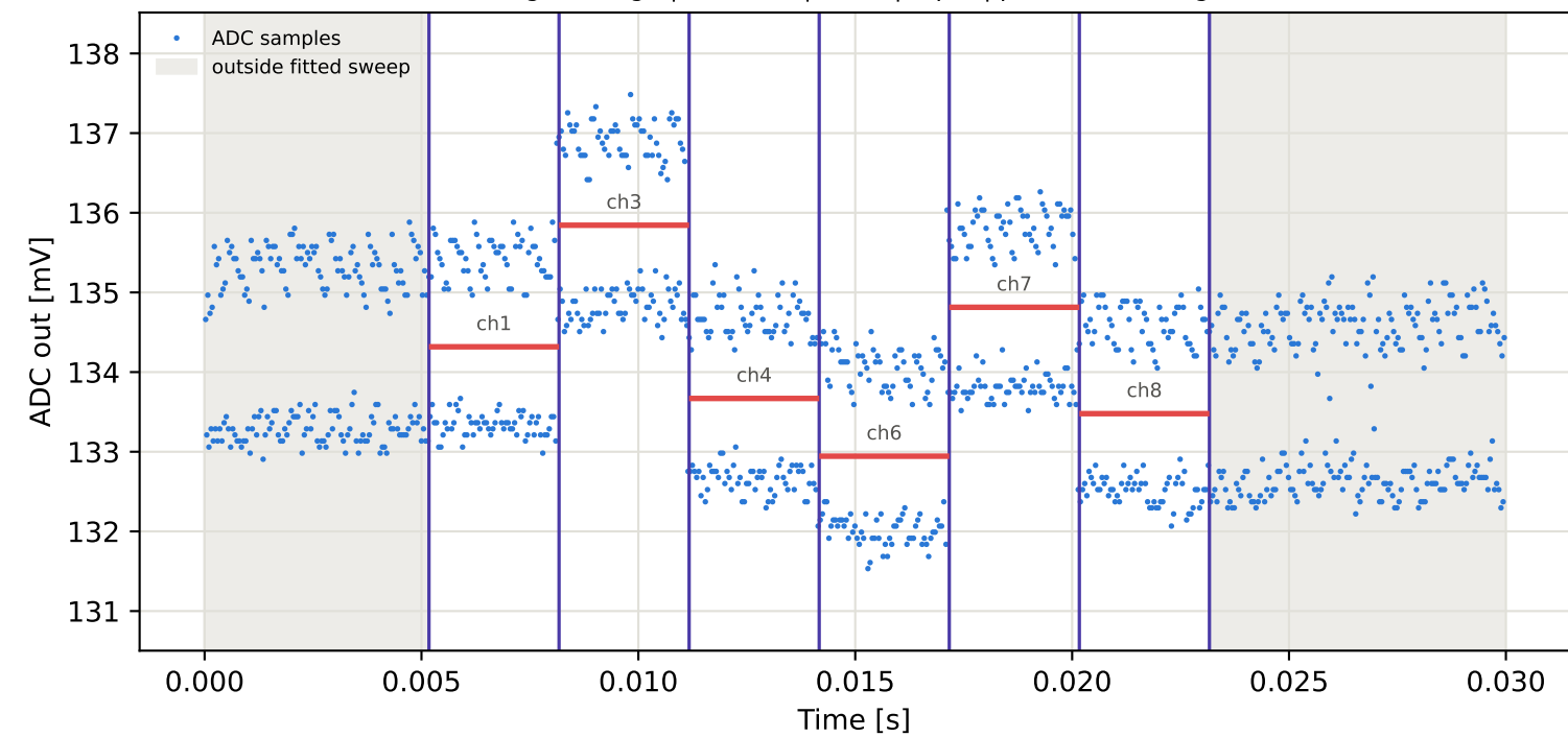
Tag8 &lt;- Tag10 | 775 MHz | run 0 | rep 1 | phase 12.25 deg
