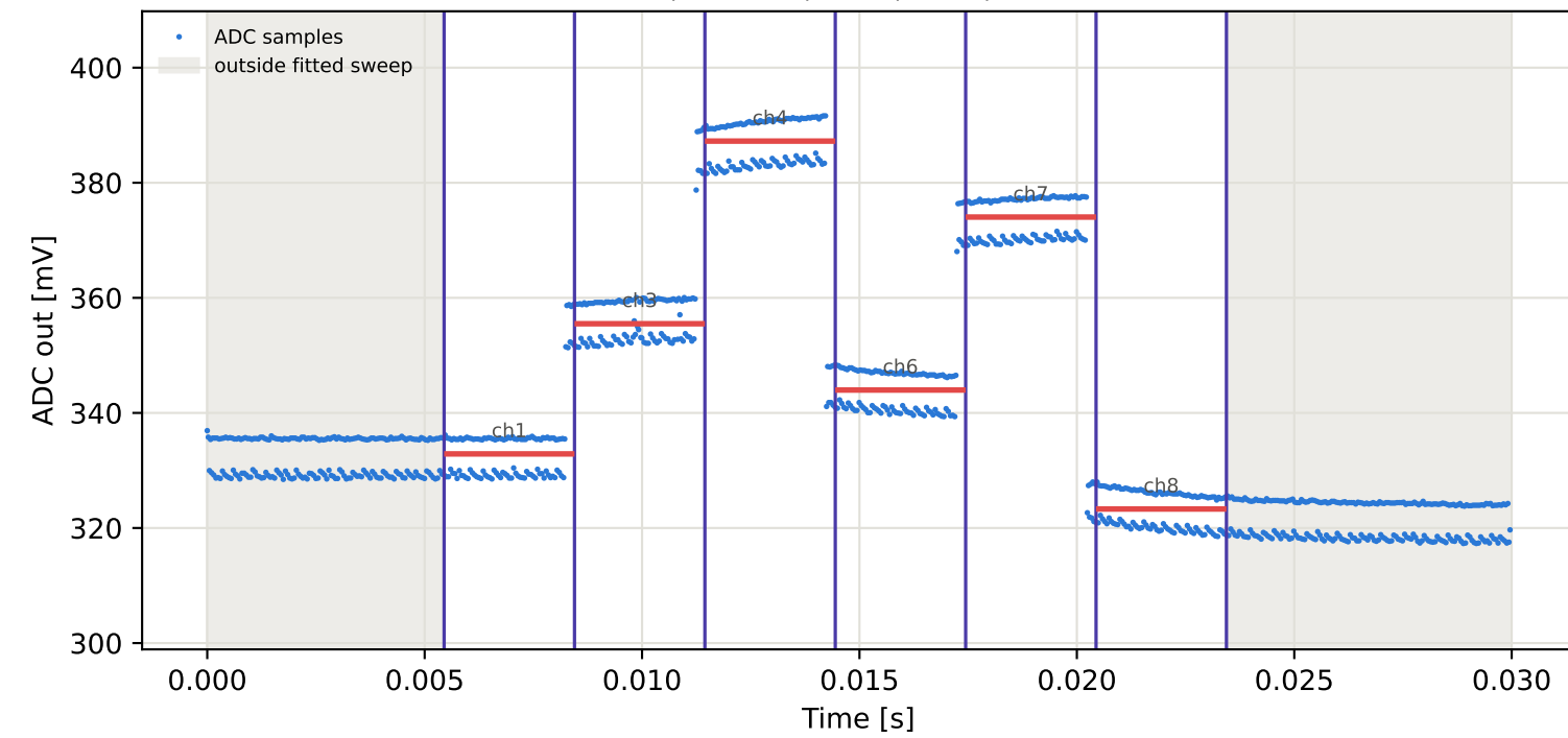
Tag1 &lt;- Tag9 | 945 MHz | run 0 | rep 1 | phase -84.59 deg
