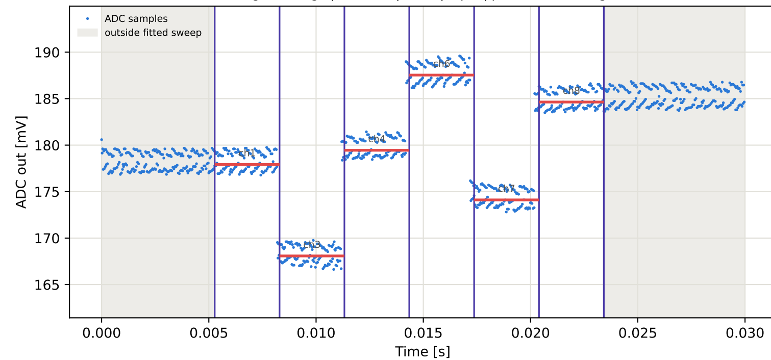
Tag10 &lt;- Tag8 | 795 MHz | run 0 | rep 1 | phase 122.50 deg
