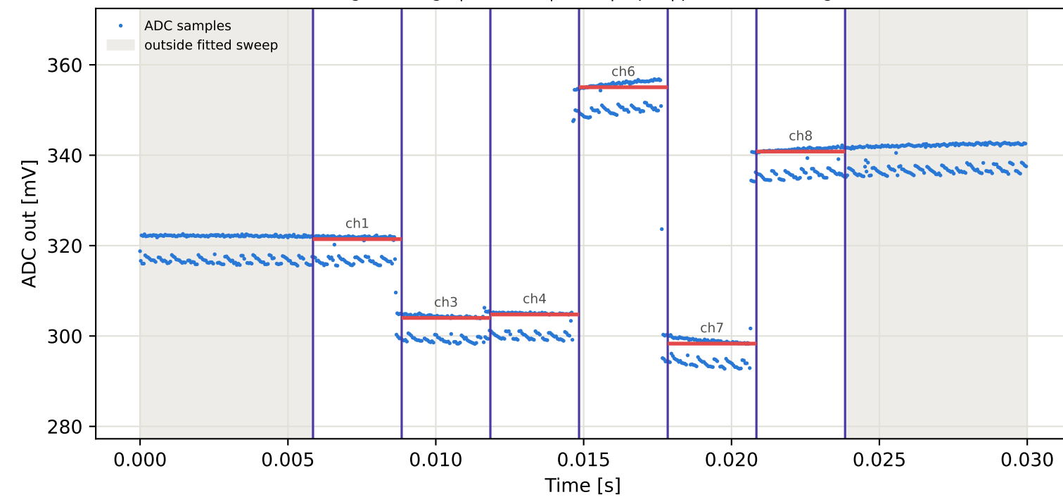
Tag10 &lt;- Tag8 | 985 MHz | run 0 | rep 1 | phase -32.20 deg
