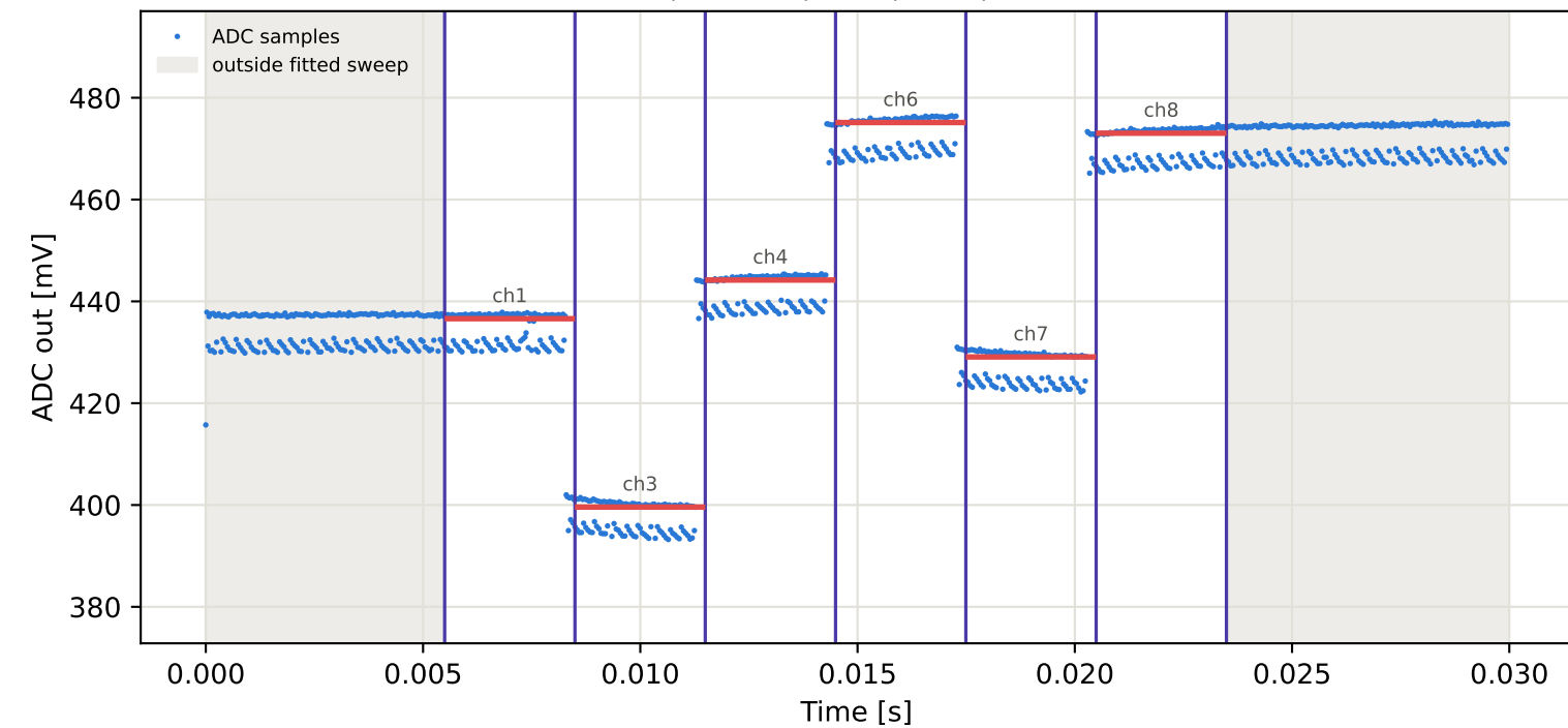
Tag3 &lt;- Tag16 | 845 MHz | run 0 | rep 1 | phase -165.45 deg
