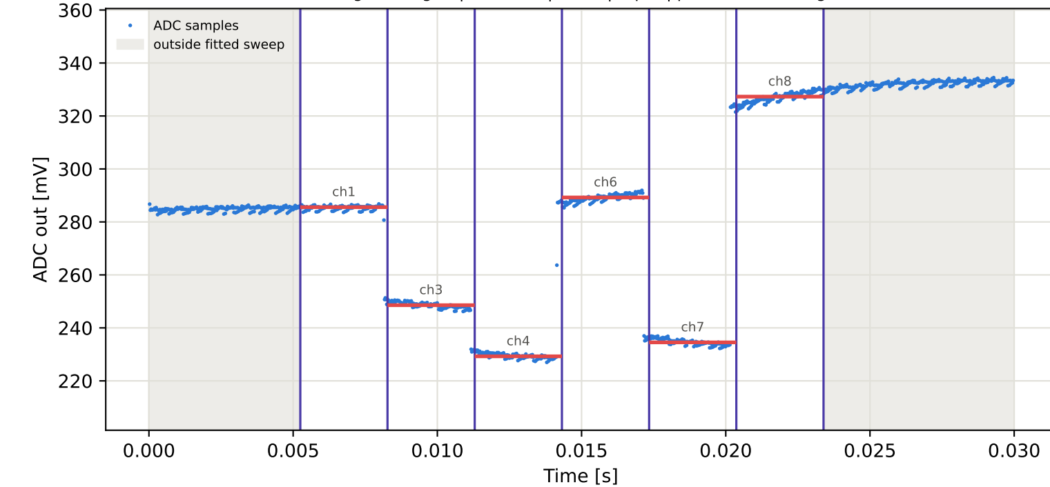
Tag9 &lt;- Tag16 | 895 MHz | run 0 | rep 1 | phase -108.52 deg
