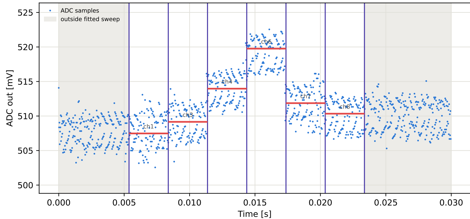
Tag5 &lt;- Tag4 | 875 MHz | run 0 | rep 1 | phase -176.31 deg
