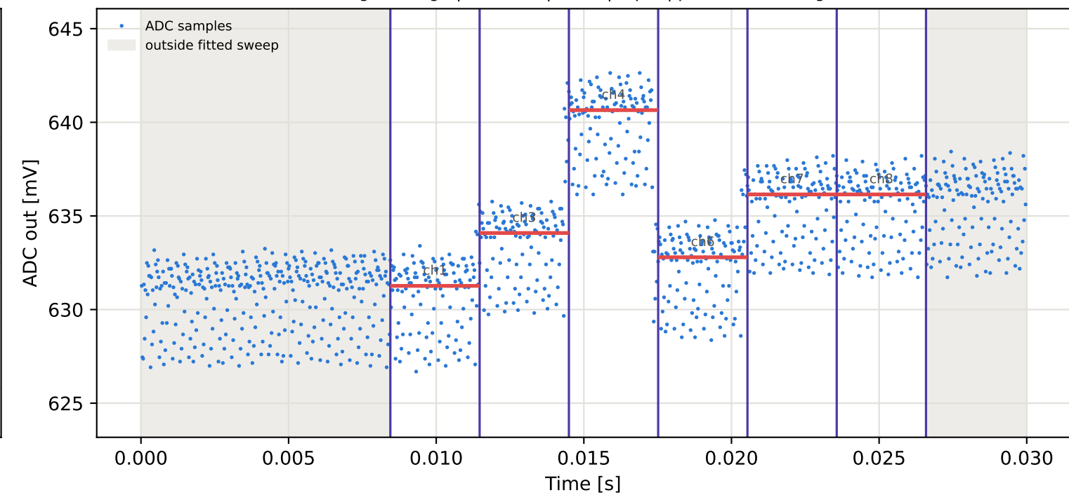
Tag3 &lt;- Tag9 | 905 MHz | run 0 | rep 1 | phase -110.28 deg
