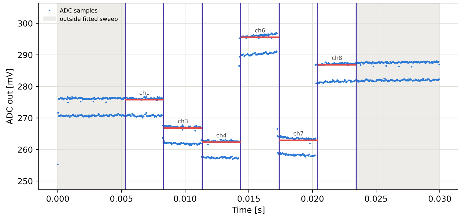
Tag8 &lt;- Tag5 | 975 MHz | run 0 | rep 1 | phase 35.44 deg
