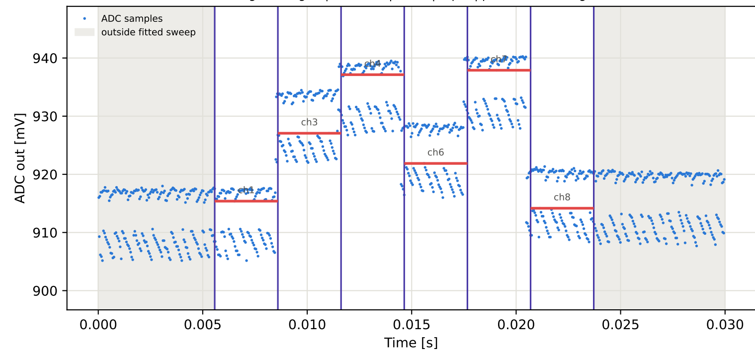
Tag7 &lt;- Tag15 | 855 MHz | run 0 | rep 1 | phase -72.30 deg
