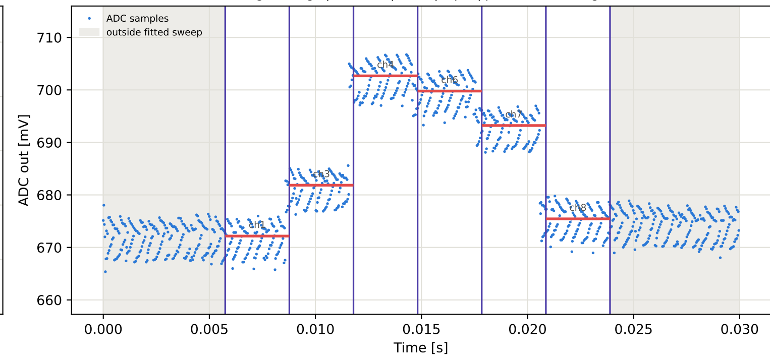
Tag9 &lt;- Tag15 | 935 MHz | run 0 | rep 1 | phase 155.73 deg
