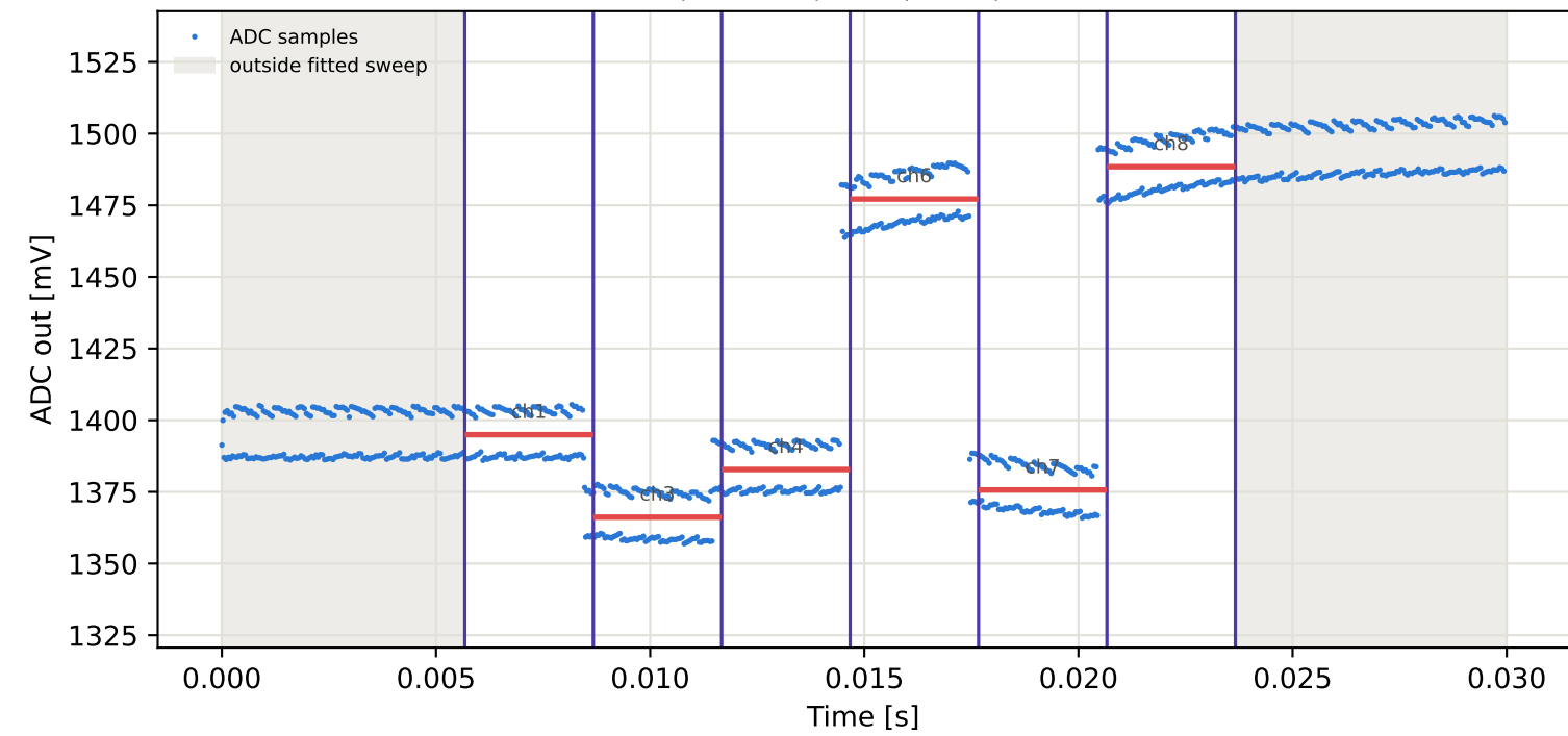
Tag8 &lt;- Tag16 | 895 MHz | run 0 | rep 1 | phase 169.11 deg
