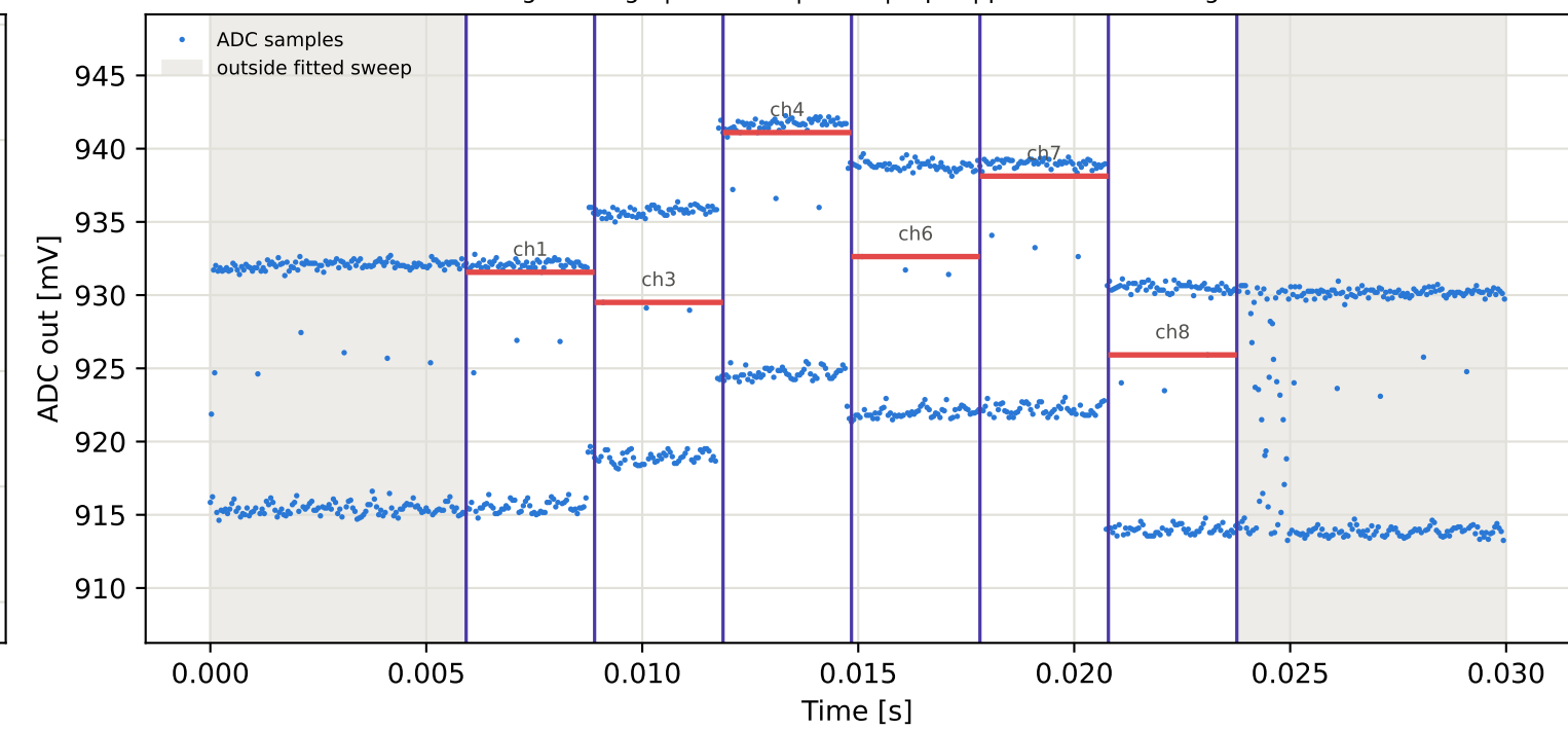
Tag7 &lt;- Tag4 | 965 MHz | run 0 | rep 1 | phase 141.22 deg
