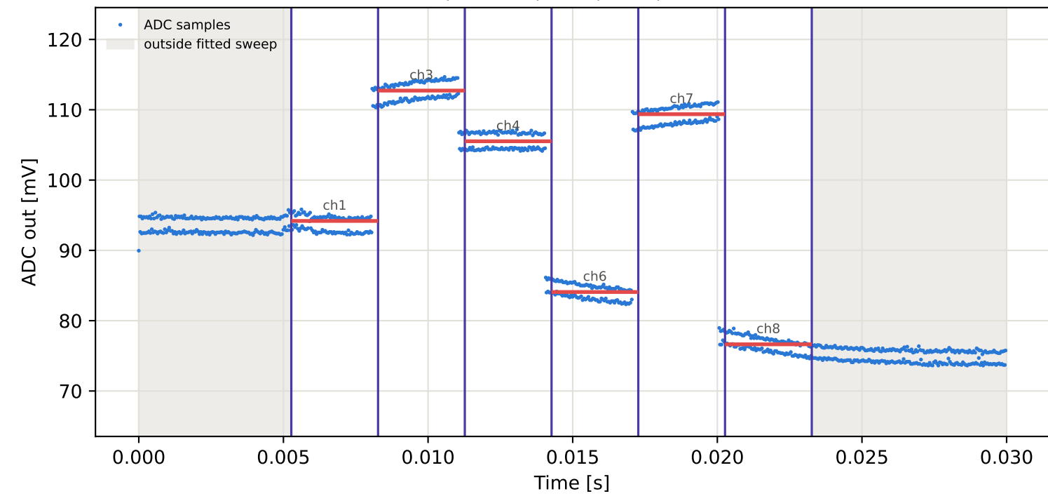
Tag2 &lt;- Tag8 | 855 MHz | run 0 | rep 1 | phase -19.07 deg
