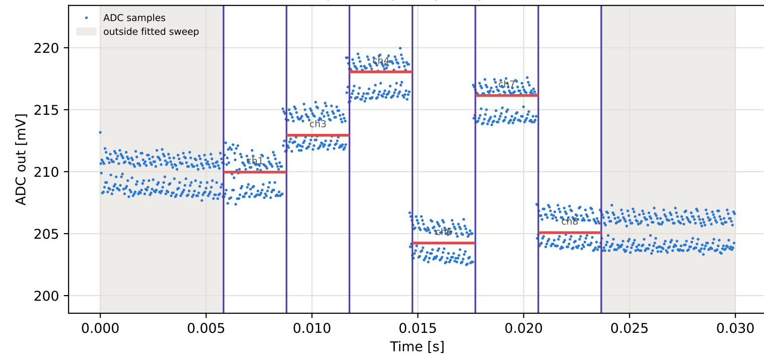
Tag1 &lt;- Tag3 | 955 MHz | run 0 | rep 1 | phase -50.32 deg
