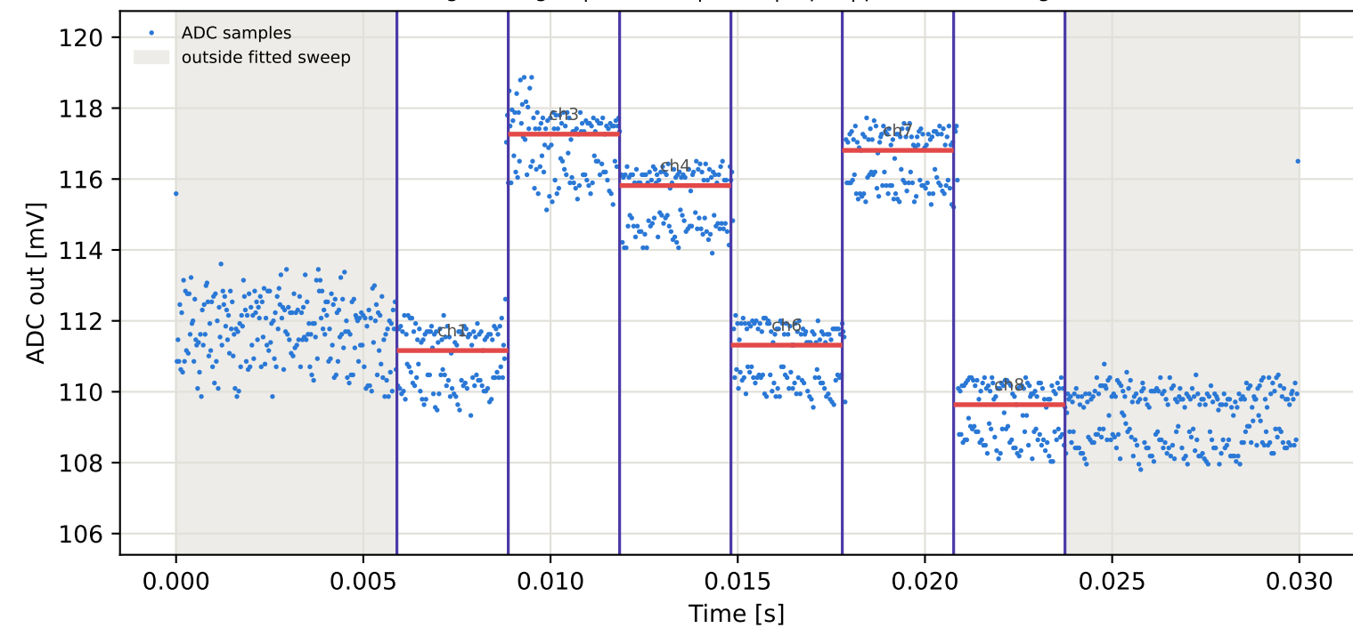
Tag2 &lt;- Tag16 | 835 MHz | run 0 | rep 1 | phase 169.39 deg
