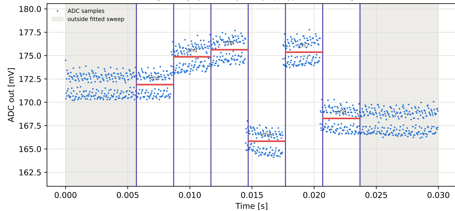
Tag3 &lt;- Tag15 | 955 MHz | run 0 | rep 1 | phase 59.33 deg
