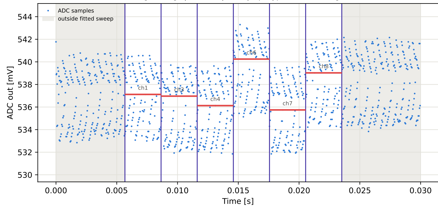
Tag2 &lt;- Tag6 | 955 MHz | run 0 | rep 1 | phase 78.00 deg
