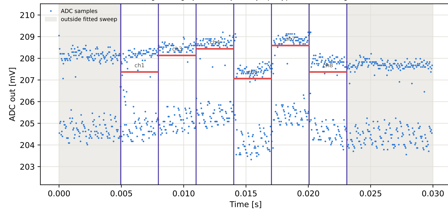
Tag4 &lt;- Tag2 | 855 MHz | run 0 | rep 1 | phase -42.11 deg
