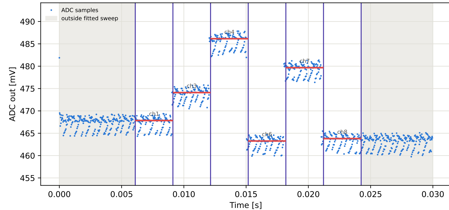
Tag15 &lt;- Tag5 | 995 MHz | run 0 | rep 1 | phase 96.59 deg
