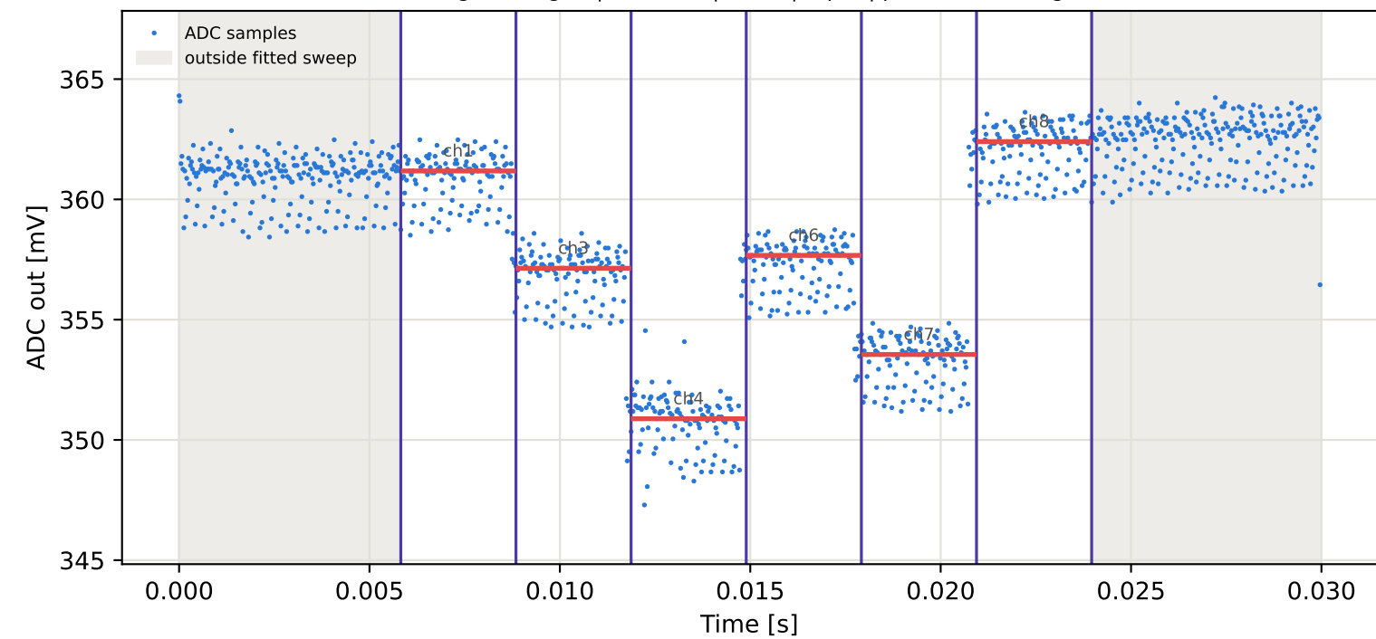
Tag1 &lt;- Tag2 | 945 MHz | run 0 | rep 1 | phase -17.74 deg
