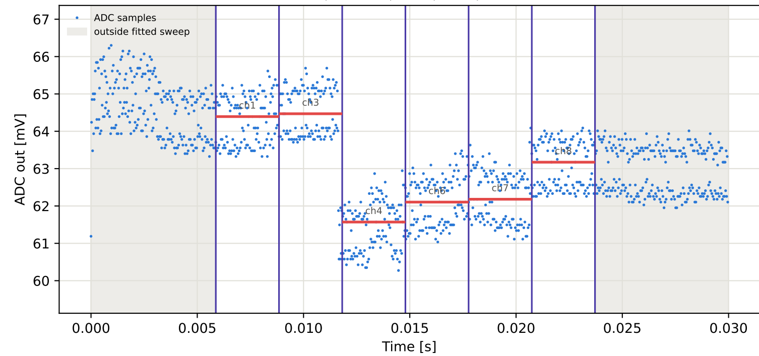
Tag15 &lt;- Tag6 | 785 MHz | run 0 | rep 1 | phase 67.66 deg
