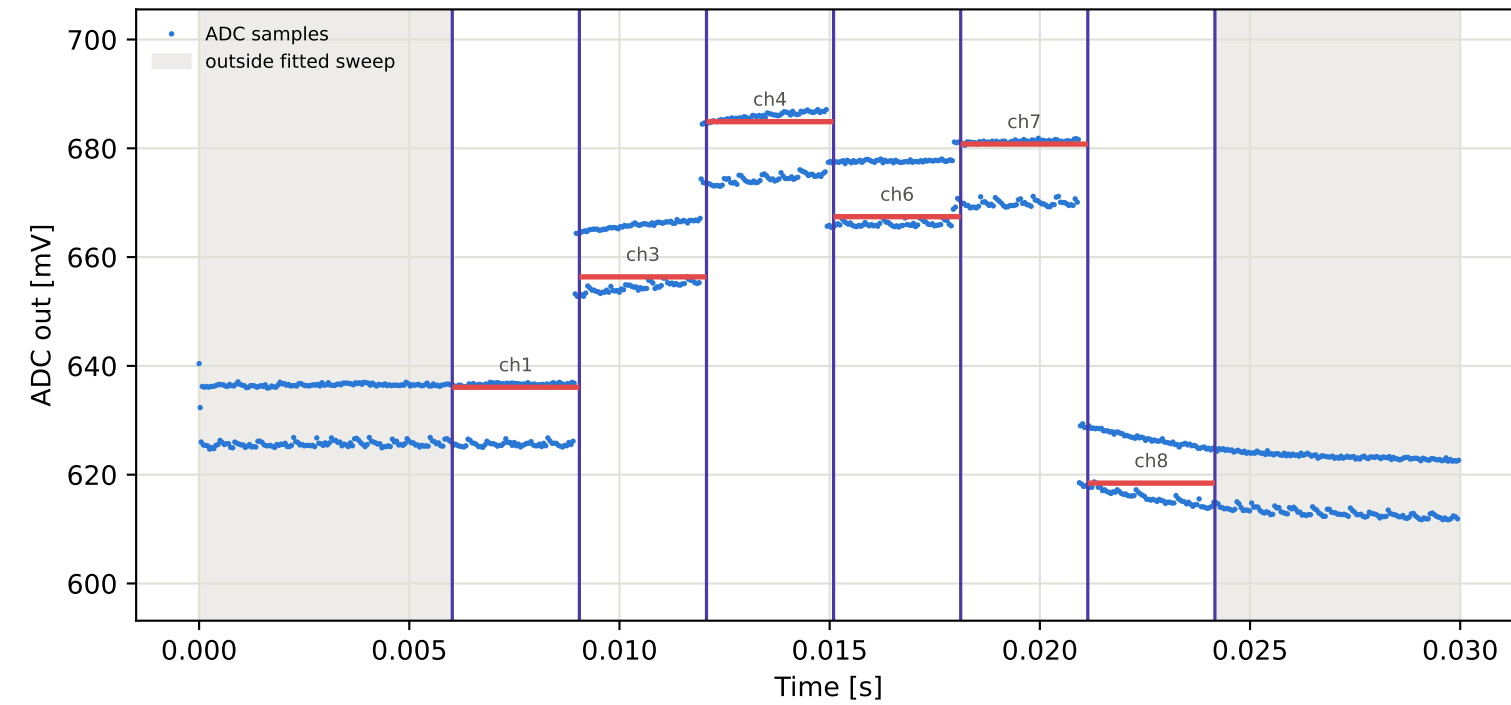
Tag6 &lt;- Tag1 | 895 MHz | run 0 | rep 1 | phase 78.13 deg
