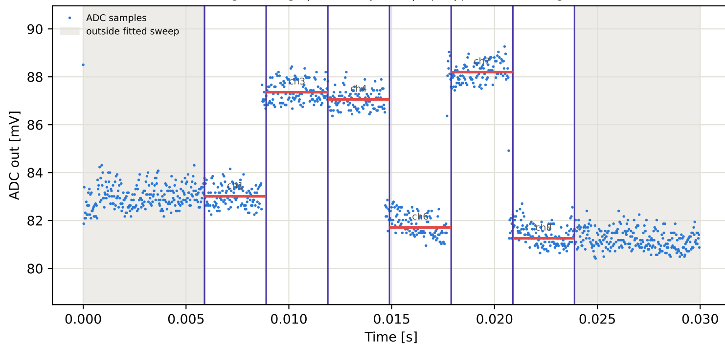
Tag15 &lt;- Tag9 | 795 MHz | run 0 | rep 1 | phase -150.55 deg
