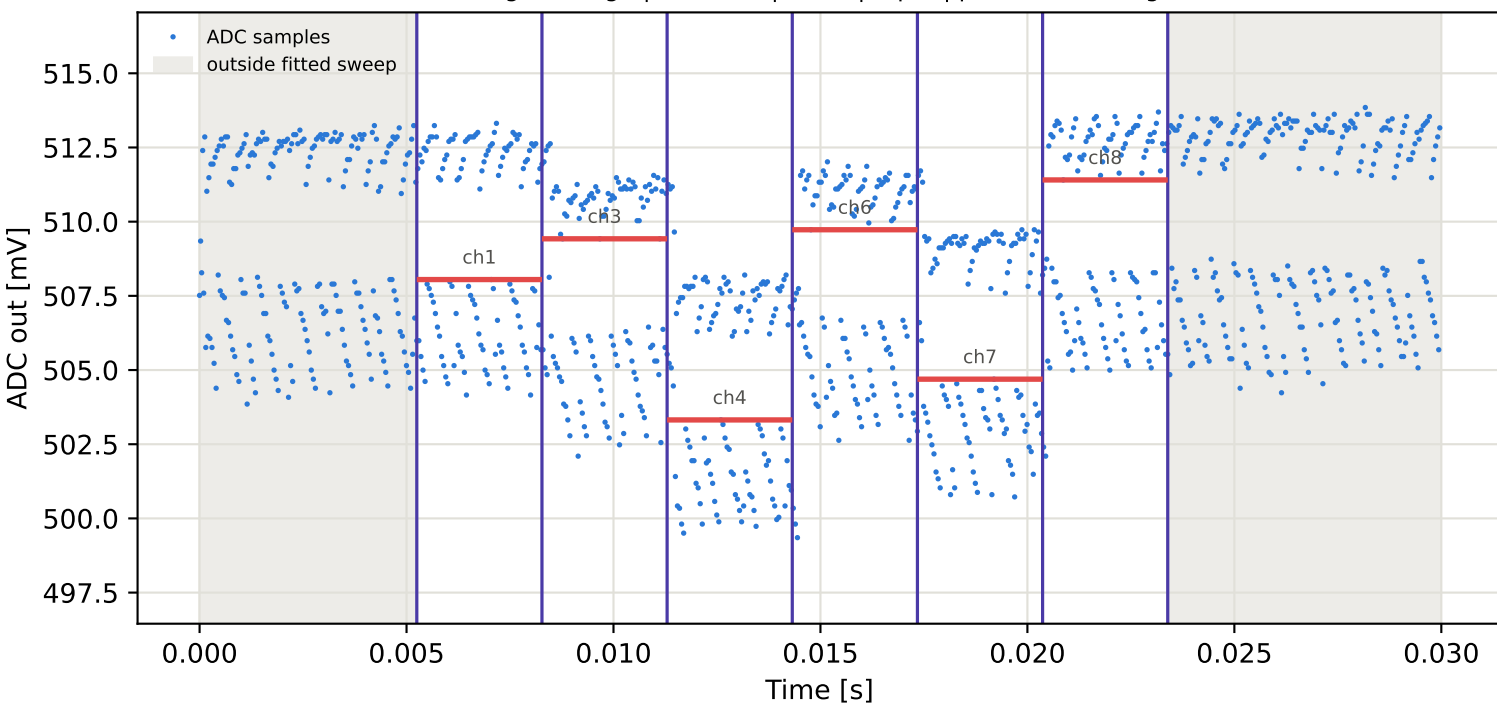
Tag8 &lt;- Tag15 | 955 MHz | run 0 | rep 1 | phase 107.75 deg
