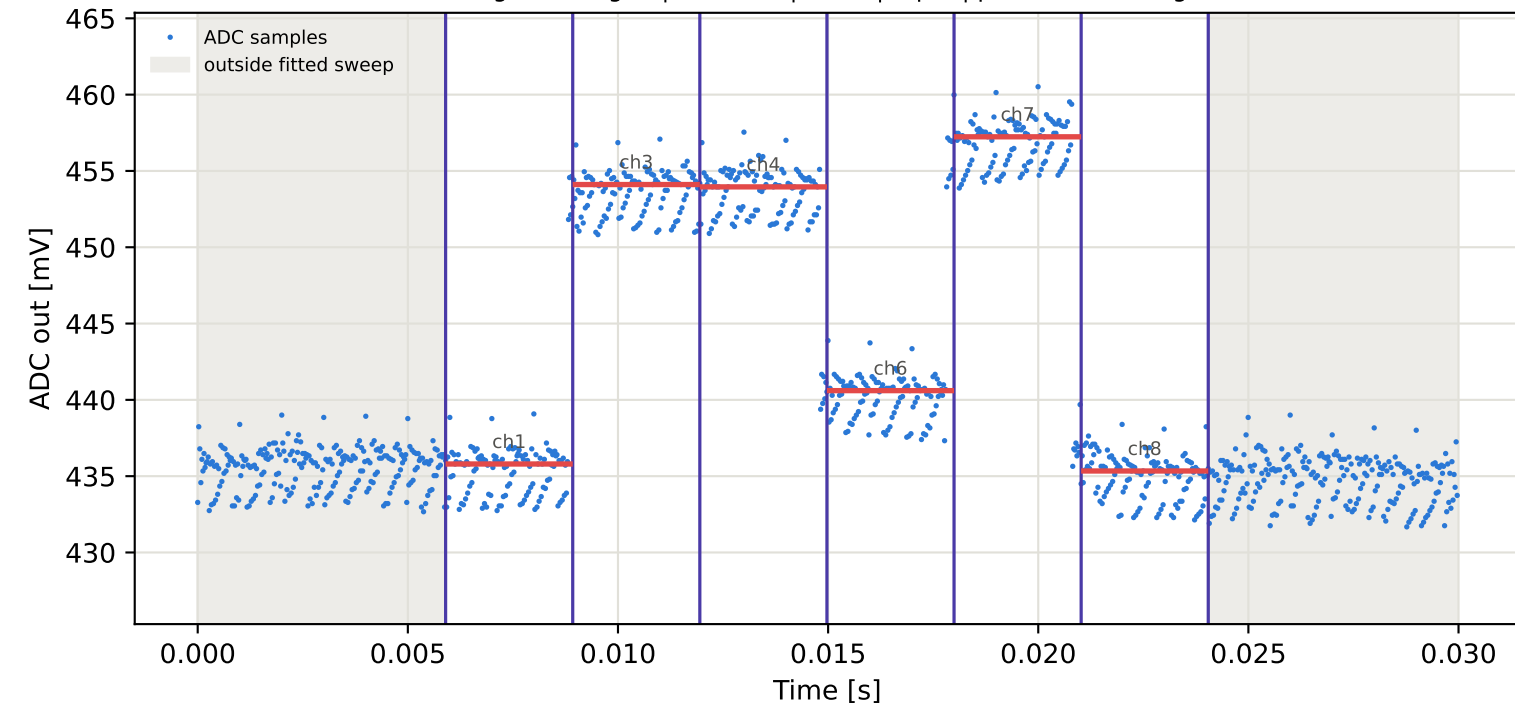
Tag15 &lt;- Tag10 | 825 MHz | run 0 | rep 1 | phase -49.02 deg
