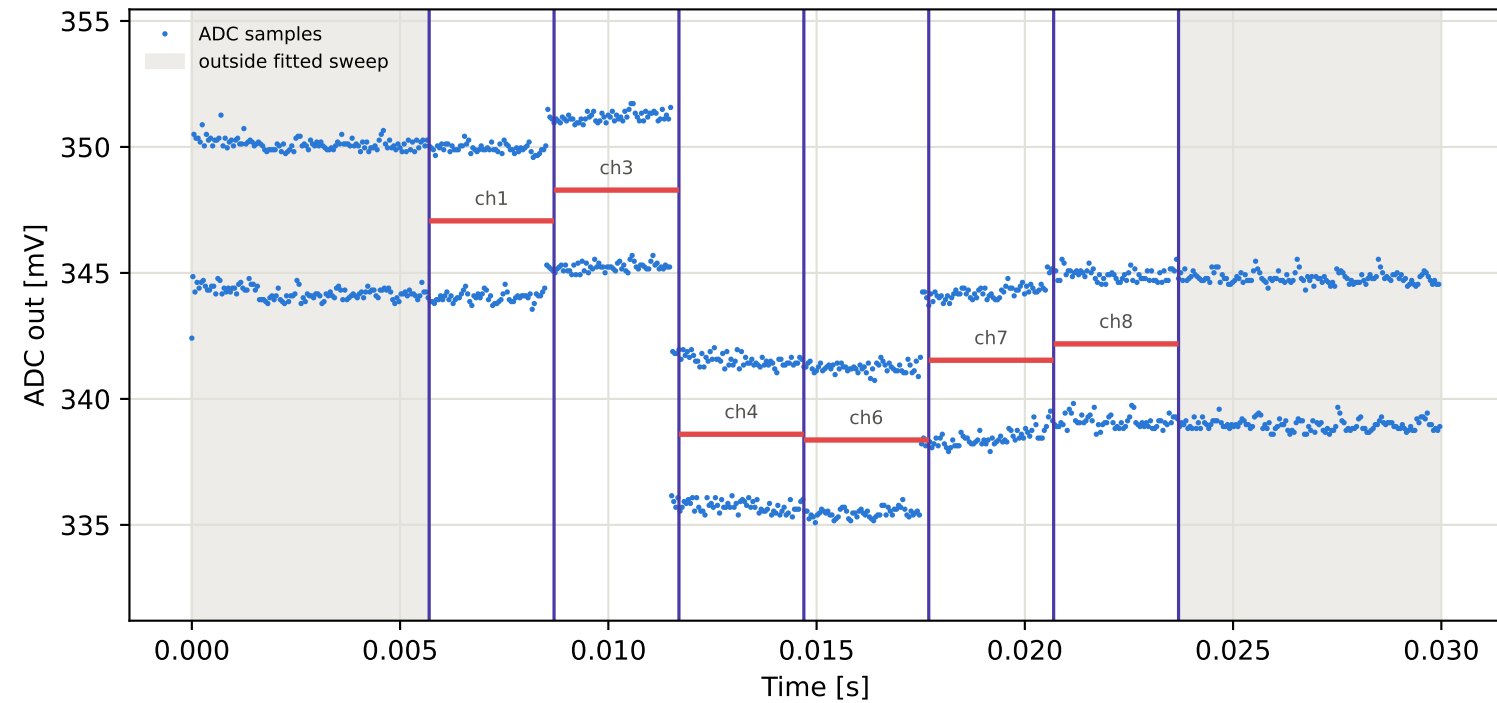
Tag8 &lt;- Tag7 | 825 MHz | run 0 | rep 1 | phase 12.10 deg
