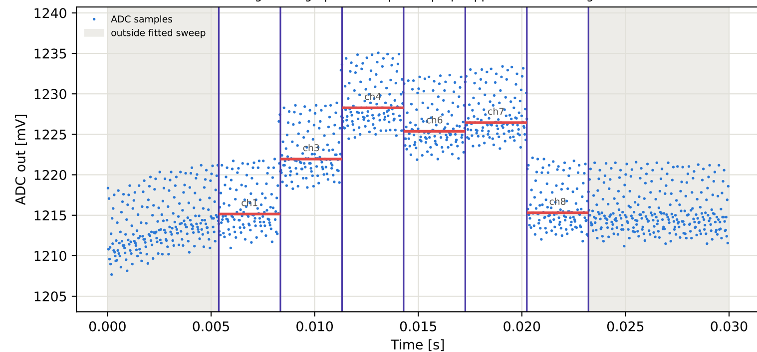
Tag3 &lt;- Tag6 | 895 MHz | run 0 | rep 1 | phase -14.38 deg
