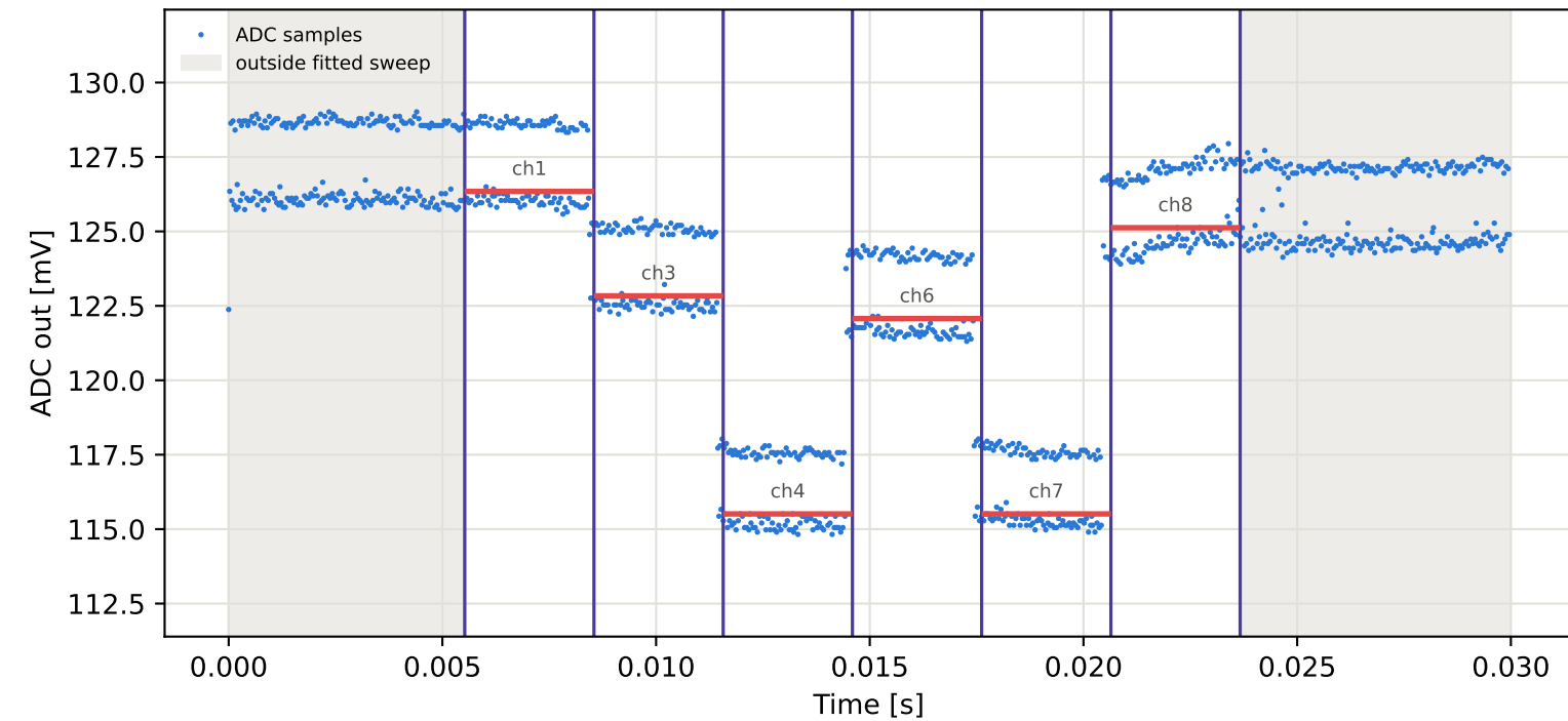
Tag3 &lt;- Tag9 | 775 MHz | run 0 | rep 1 | phase 152.77 deg
