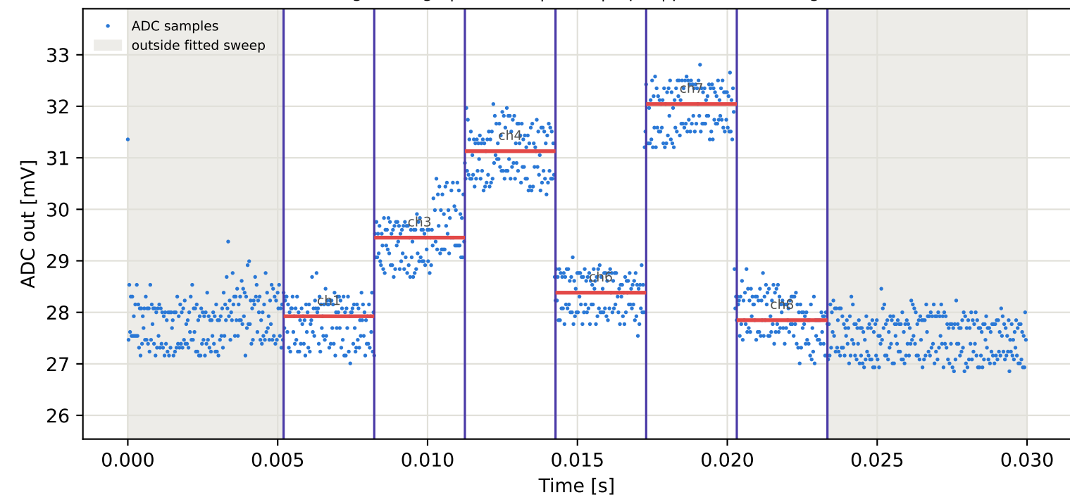
Tag5 &lt;- Tag1 | 785 MHz | run 0 | rep 1 | phase -55.39 deg
