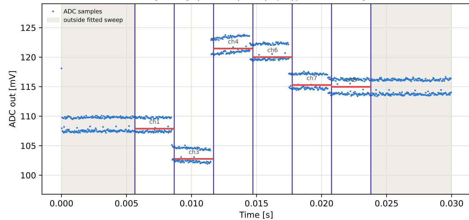
Tag3 &lt;- Tag7 | 775 MHz | run 0 | rep 1 | phase 100.98 deg
