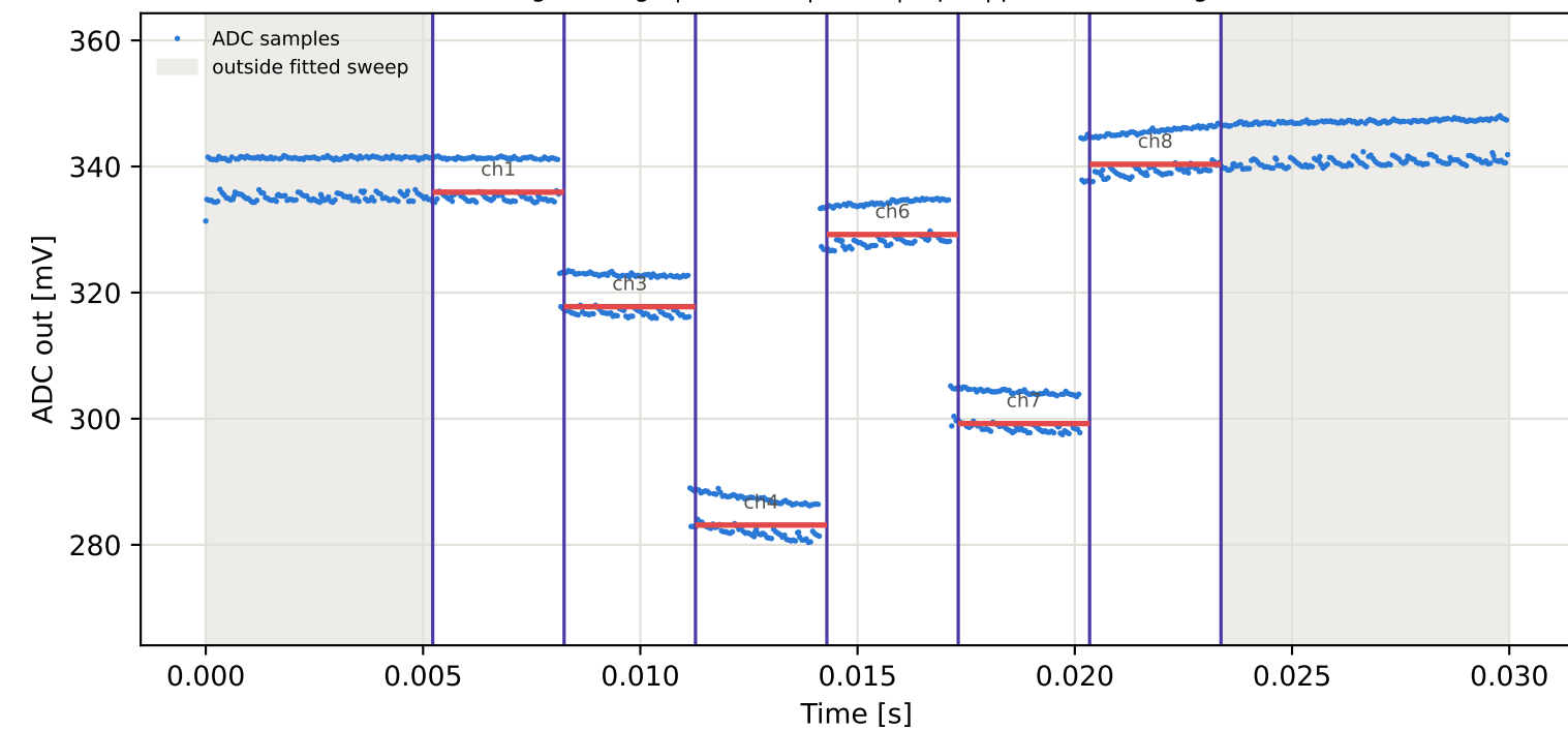
Tag9 &lt;- Tag7 | 965 MHz | run 0 | rep 1 | phase 89.83 deg
