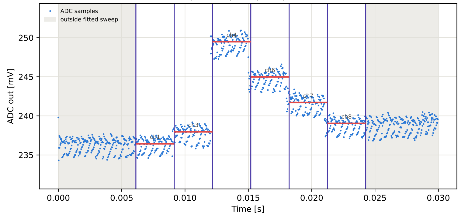
Tag8 &lt;- Tag5 | 995 MHz | run 0 | rep 1 | phase 44.67 deg
