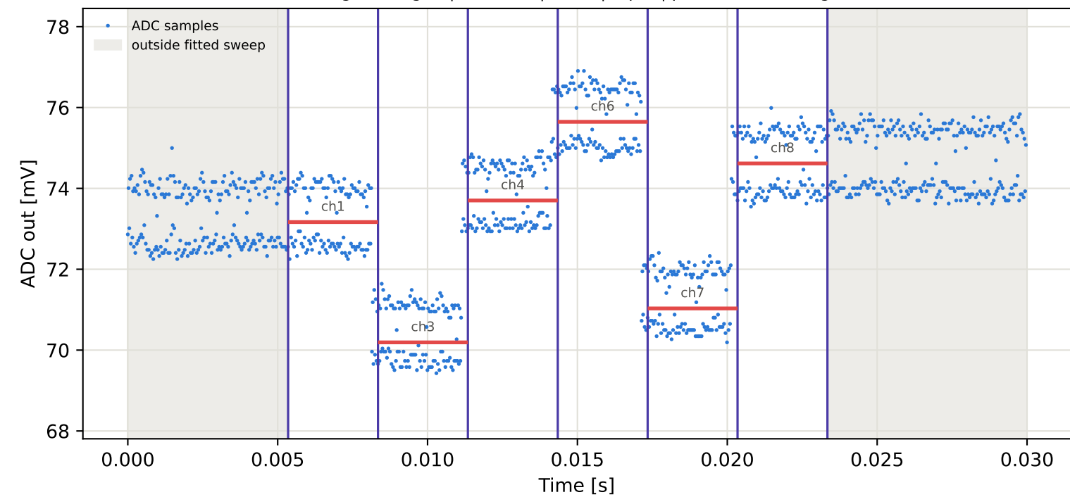
Tag6 &lt;- Tag3 | 775 MHz | run 0 | rep 1 | phase 11.93 deg
