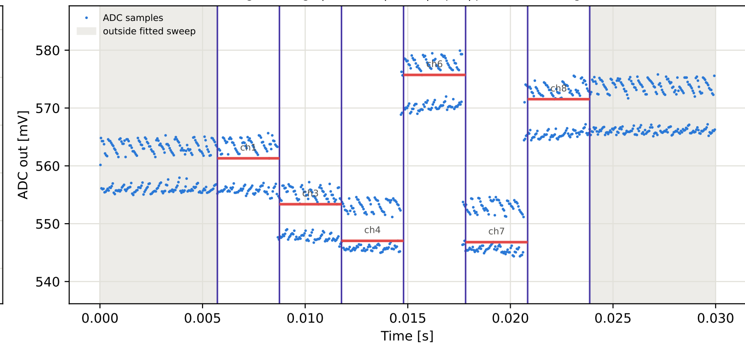
Tag2 &lt;- Tag10 | 965 MHz | run 0 | rep 1 | phase 0.80 deg
