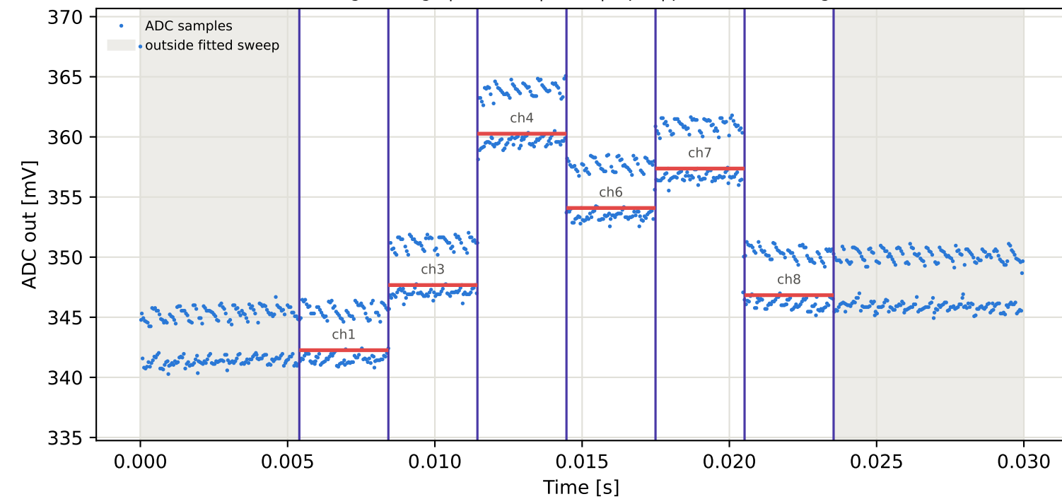
Tag6 &lt;- Tag9 | 825 MHz | run 0 | rep 1 | phase 125.10 deg
