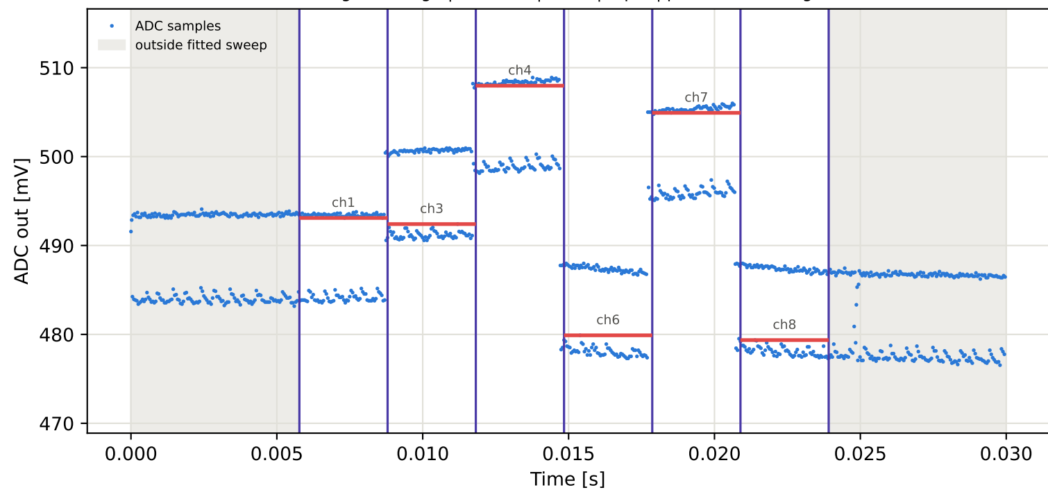
Tag15 &lt;- Tag6 | 945 MHz | run 0 | rep 1 | phase -56.31 deg
