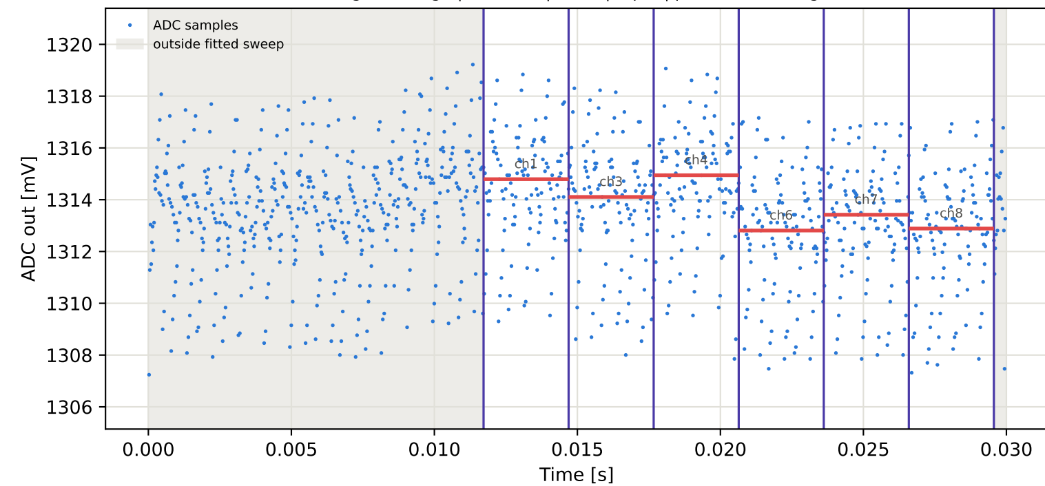
Tag15 &lt;- Tag9 | 905 MHz | run 0 | rep 1 | phase 132.52 deg
