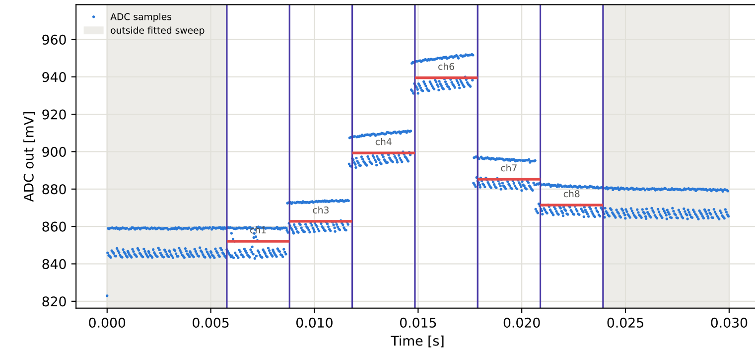
Tag3 &lt;- Tag16 | 915 MHz | run 0 | rep 1 | phase -129.03 deg
