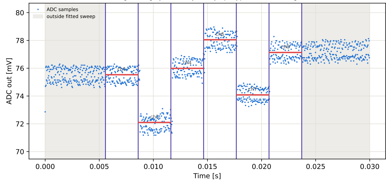
Tag10 &lt;- Tag1 | 795 MHz | run 0 | rep 1 | phase 167.01 deg
