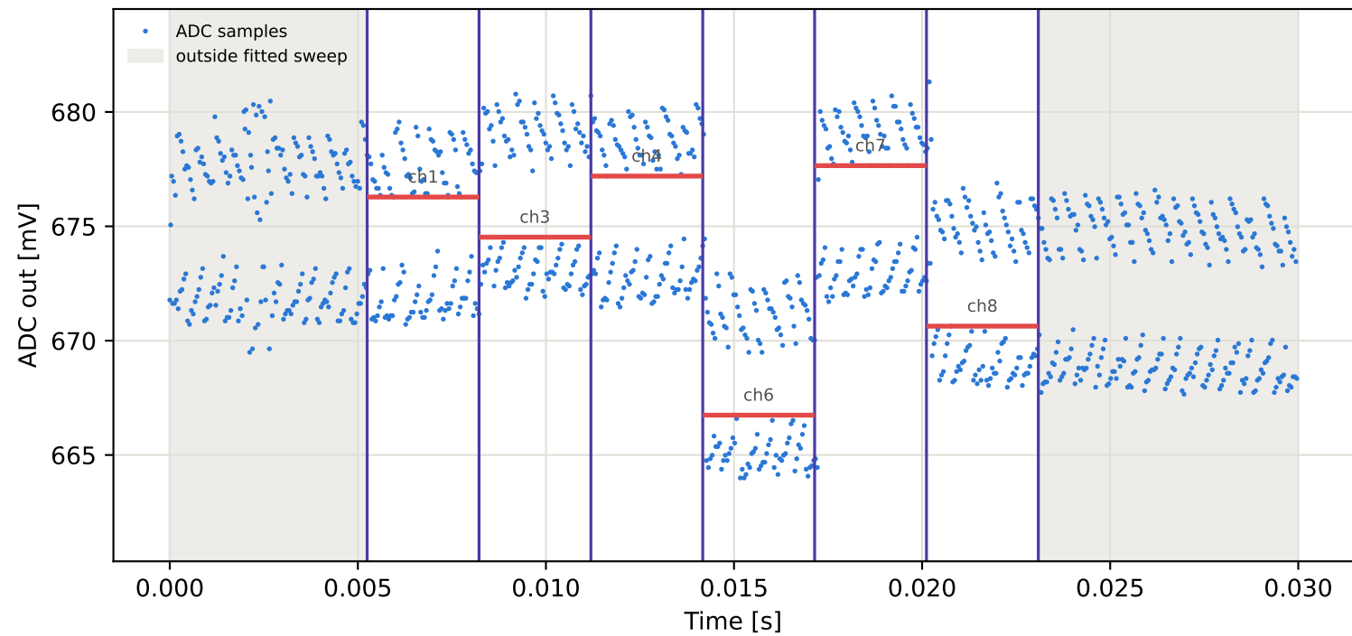
Tag16 &lt;- Tag4 | 855 MHz | run 0 | rep 1 | phase -129.46 deg
