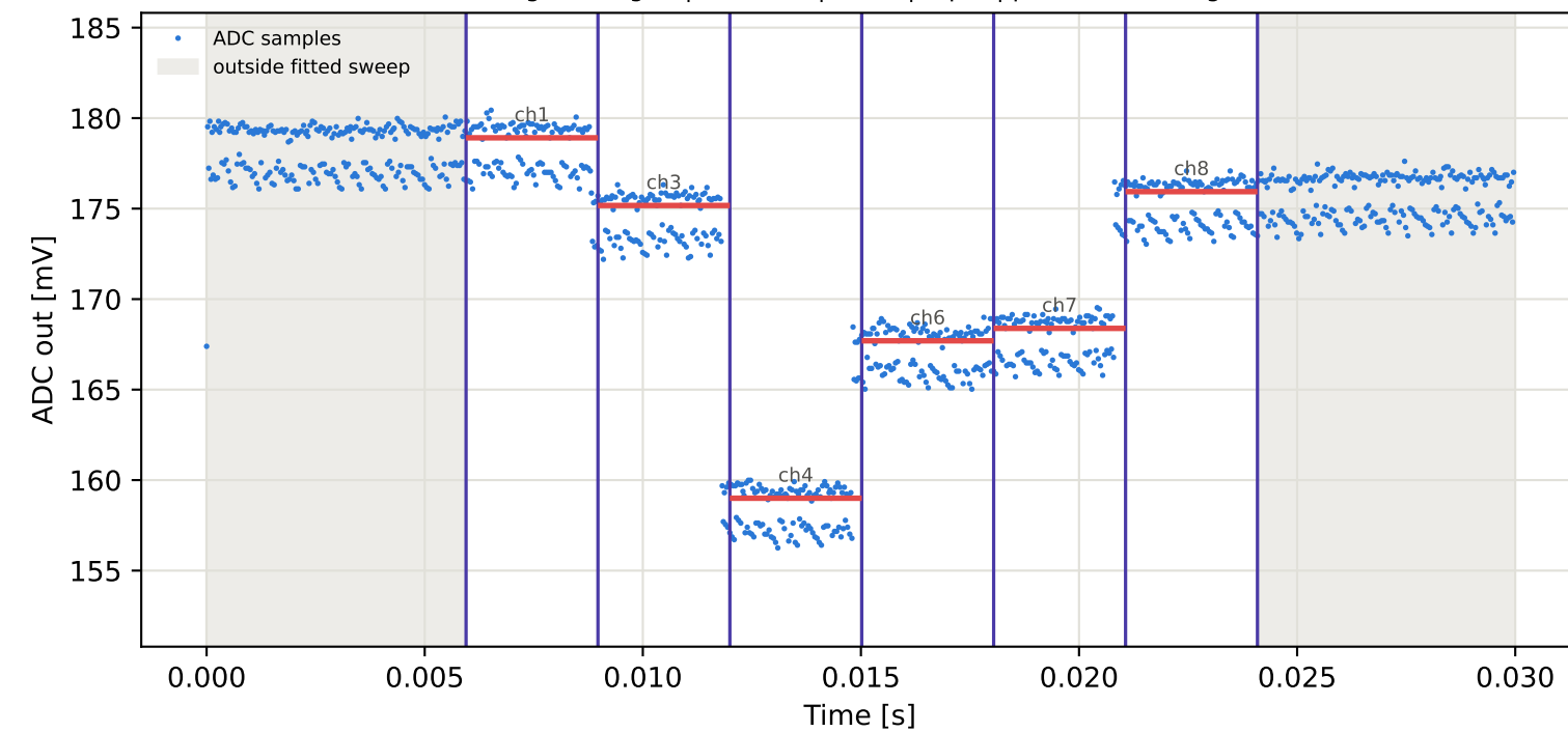
Tag5 &lt;- Tag3 | 985 MHz | run 0 | rep 1 | phase -145.95 deg
