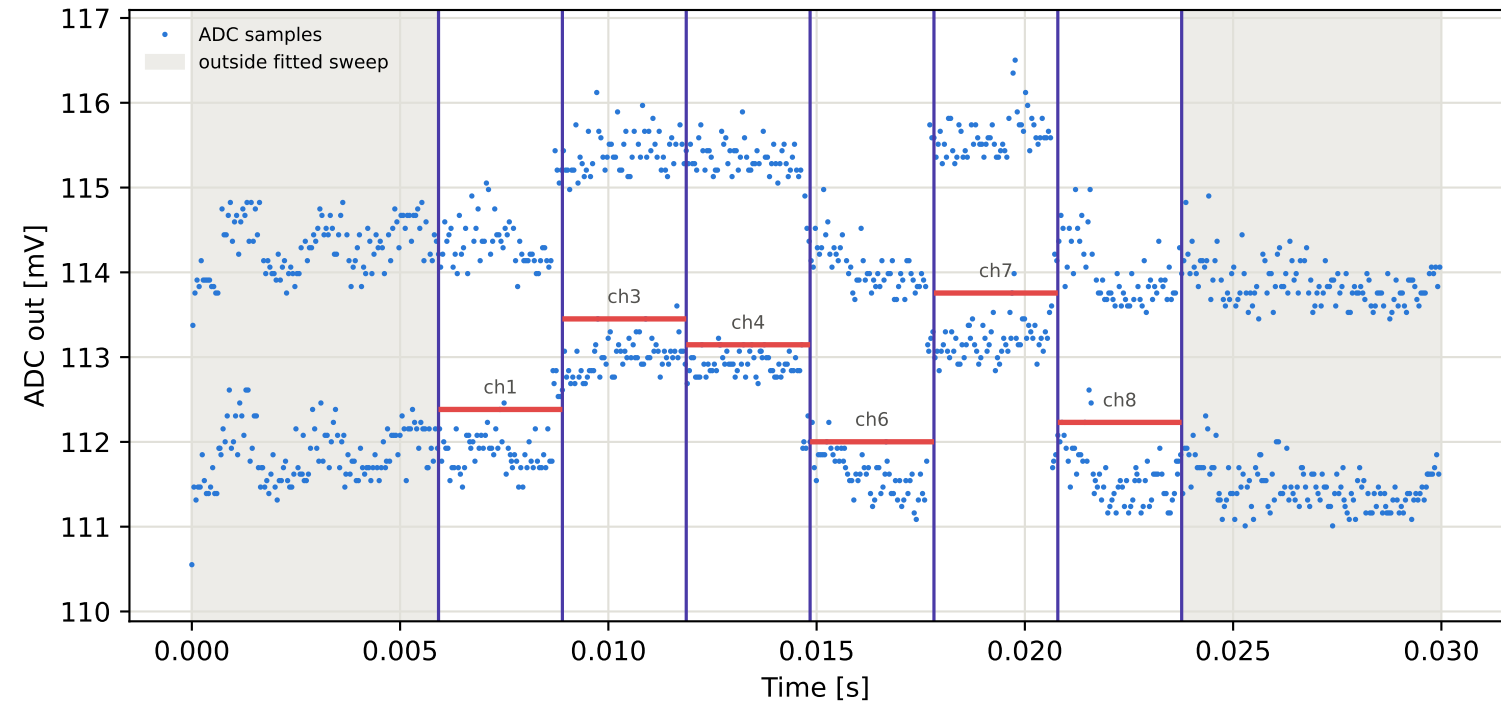
Tag5 &lt;- Tag9 | 795 MHz | run 0 | rep 1 | phase -92.72 deg
