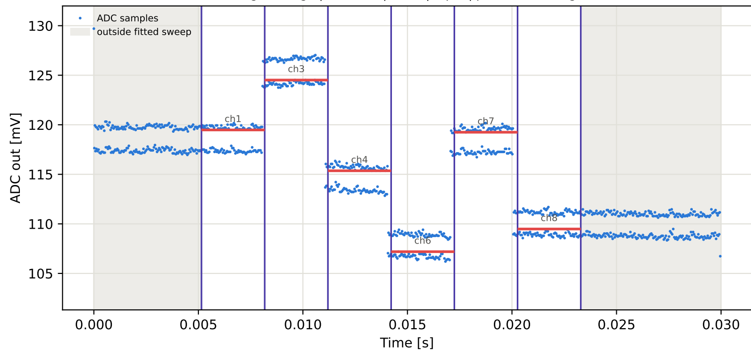
Tag4 &lt;- Tag8 | 835 MHz | run 0 | rep 1 | phase 53.74 deg
