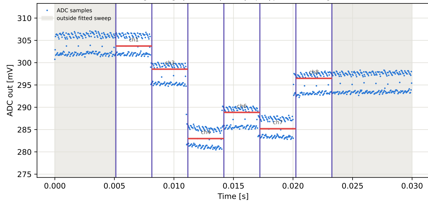
Tag1 &lt;- Tag8 | 835 MHz | run 0 | rep 1 | phase -158.97 deg
