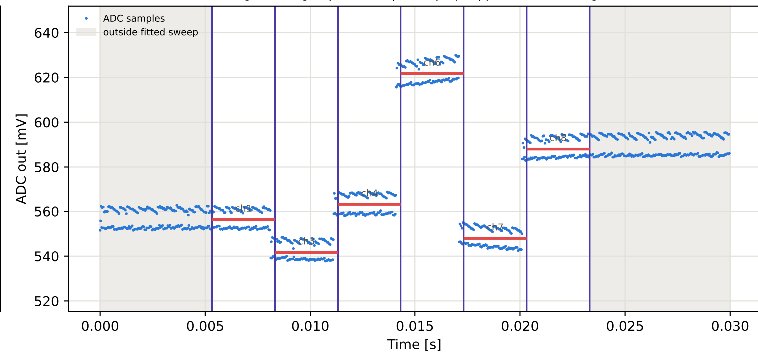
Tag16 &lt;- Tag15 | 965 MHz | run 0 | rep 1 | phase -173.99 deg
