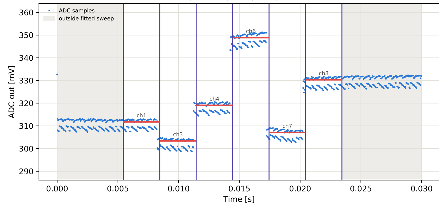
Tag10 &lt;- Tag3 | 975 MHz | run 0 | rep 1 | phase -109.44 deg
