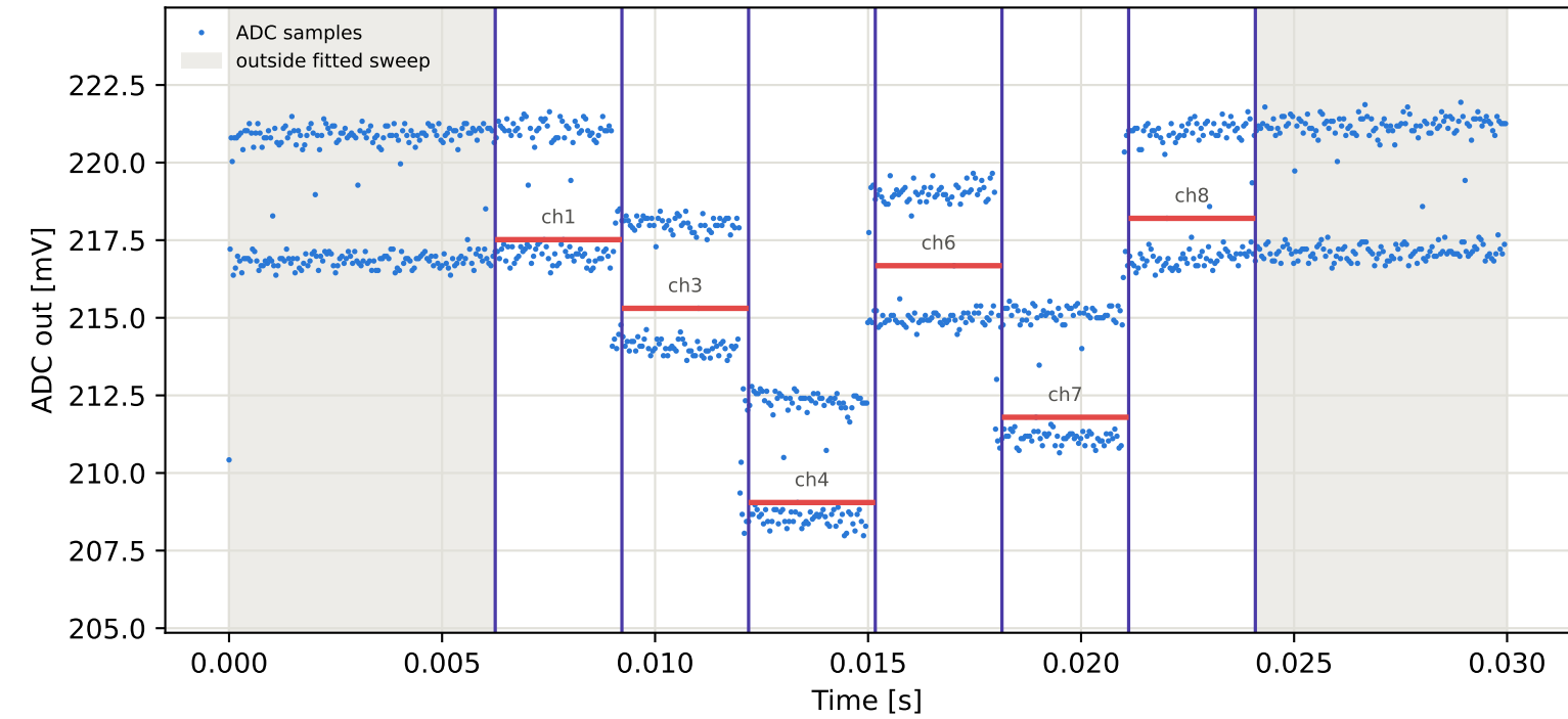
Tag4 &lt;- Tag9 | 995 MHz | run 0 | rep 1 | phase 175.95 deg
