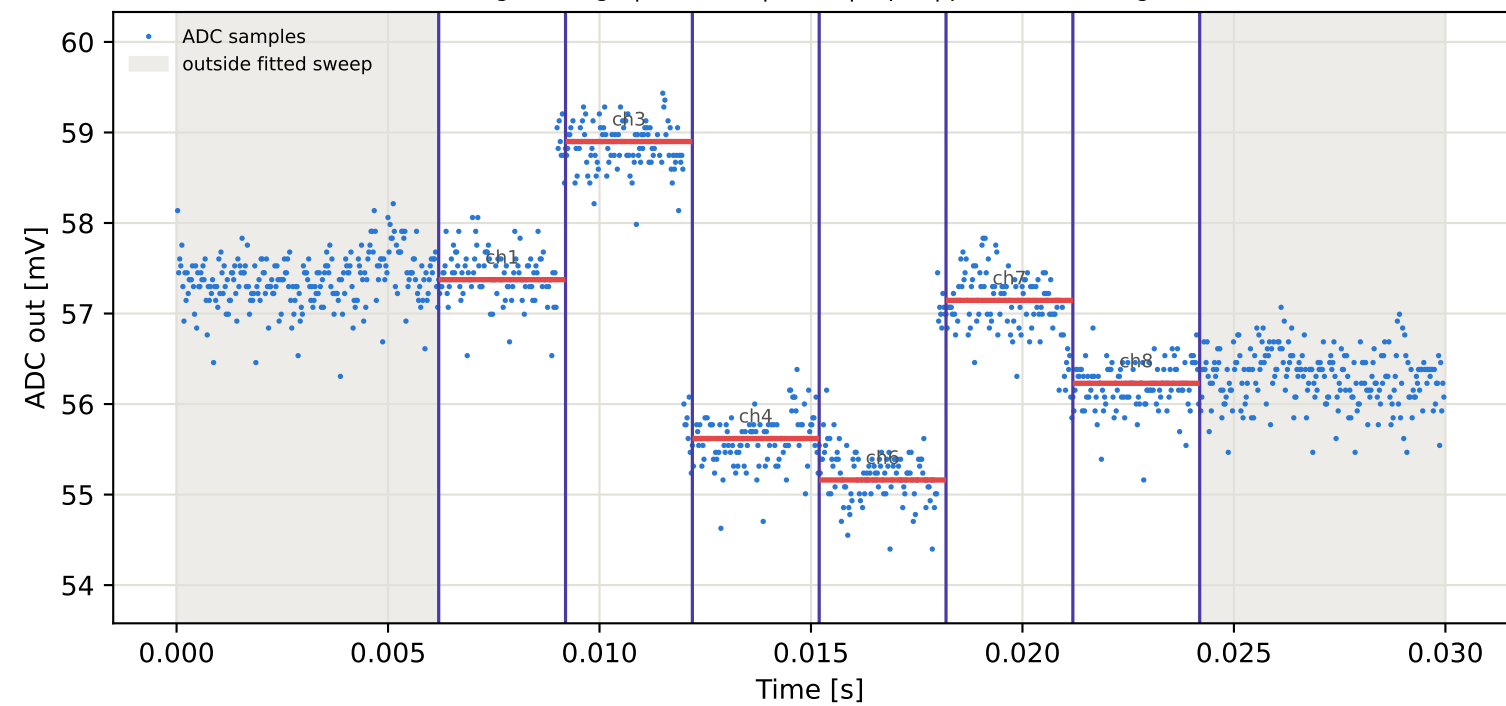
Tag1 &lt;- Tag8 | 775 MHz | run 0 | rep 1 | phase 139.79 deg
