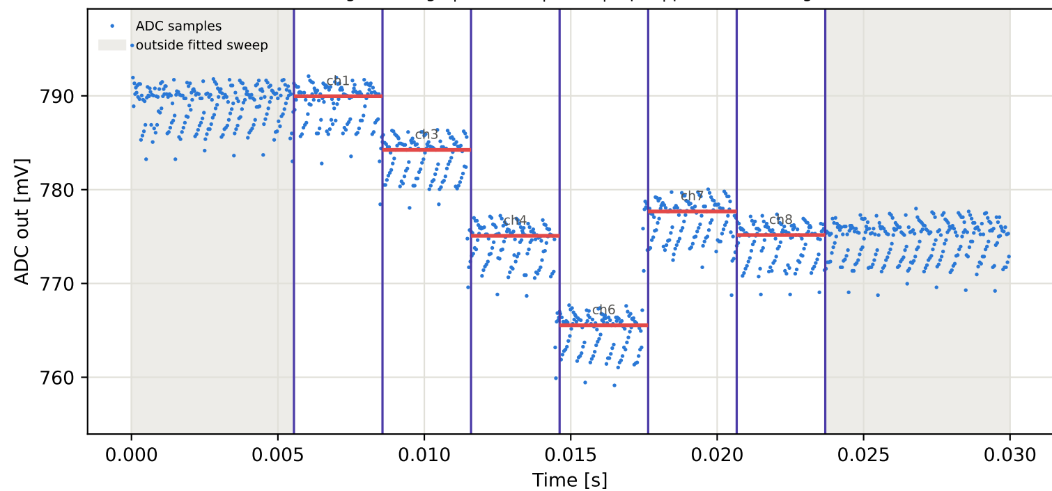
Tag15 &lt;- Tag6 | 875 MHz | run 0 | rep 1 | phase 38.31 deg
