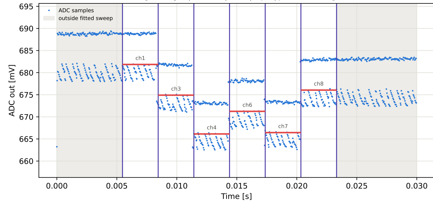
Tag7 &lt;- Tag3 | 835 MHz | run 0 | rep 1 | phase 15.77 deg
