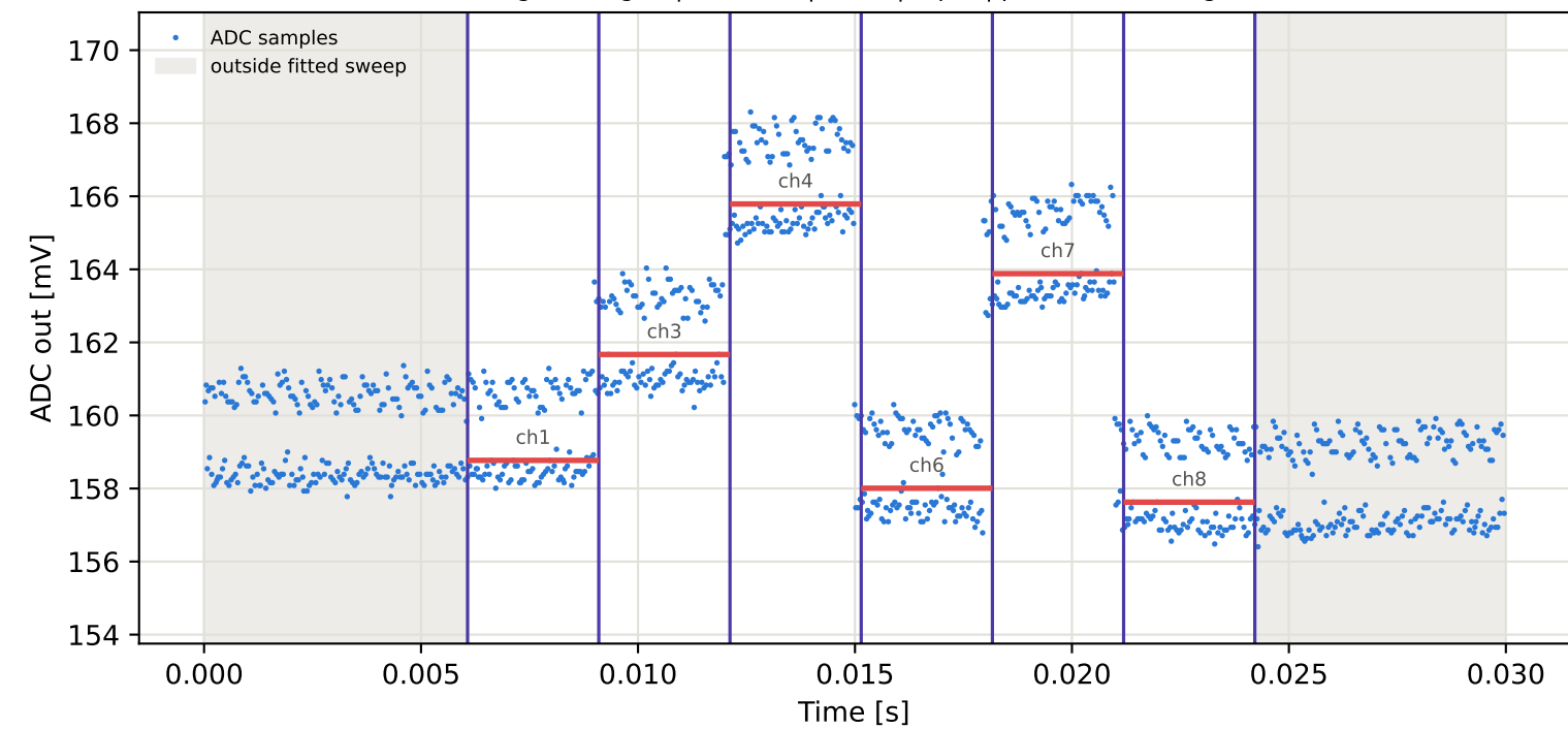
Tag4 &lt;- Tag16 | 975 MHz | run 0 | rep 1 | phase 29.59 deg
