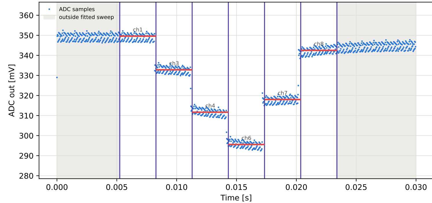
Tag10 &lt;- Tag1 | 905 MHz | run 0 | rep 1 | phase -15.42 deg
