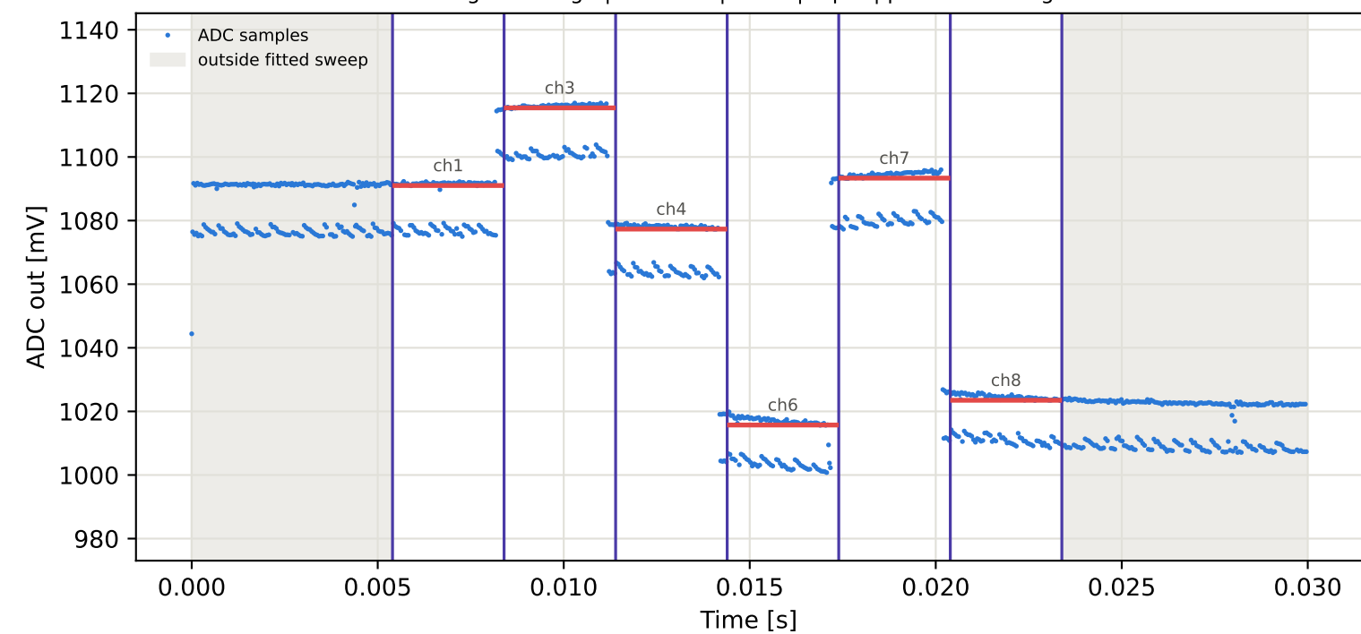
Tag16 &lt;- Tag7 | 875 MHz | run 0 | rep 1 | phase 9.55 deg
