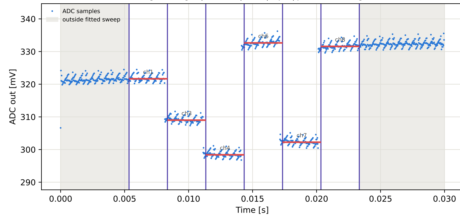
Tag10 &lt;- Tag2 | 975 MHz | run 0 | rep 1 | phase -3.03 deg
