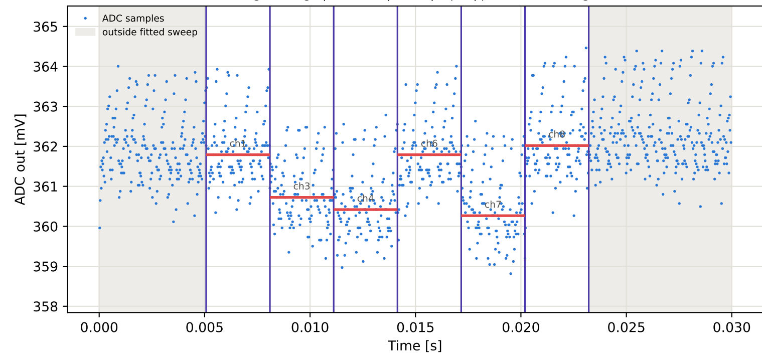
Tag8 &lt;- Tag10 | 805 MHz | run 0 | rep 1 | phase 108.24 deg
