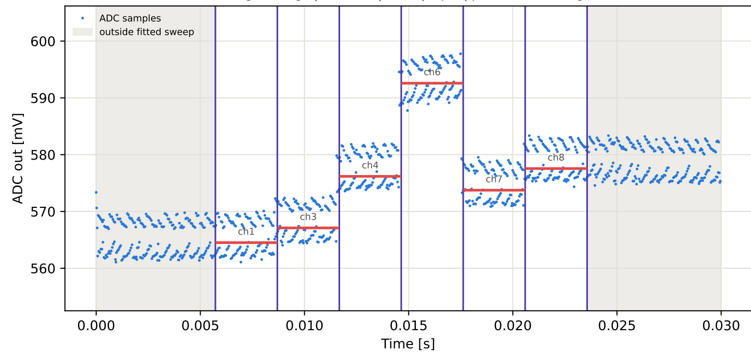
Tag9 &lt;- Tag15 | 905 MHz | run 0 | rep 1 | phase 175.70 deg
