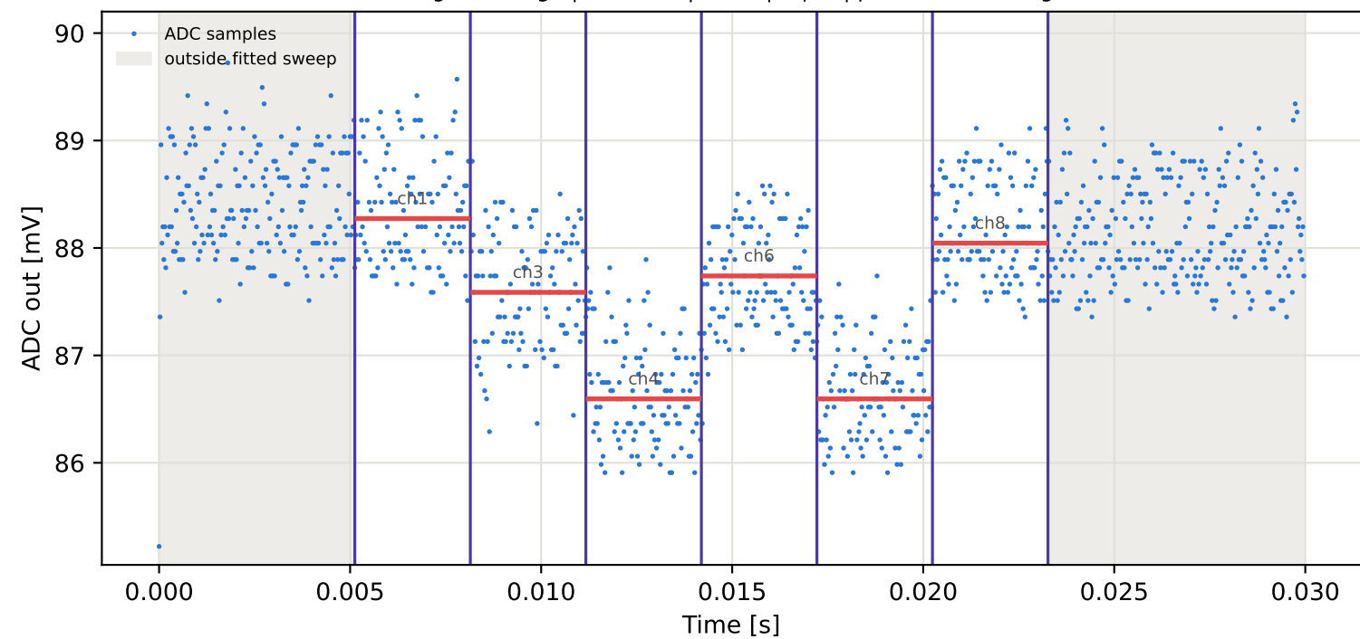
Tag15 &lt;- Tag6 | 795 MHz | run 0 | rep 1 | phase 105.73 deg
