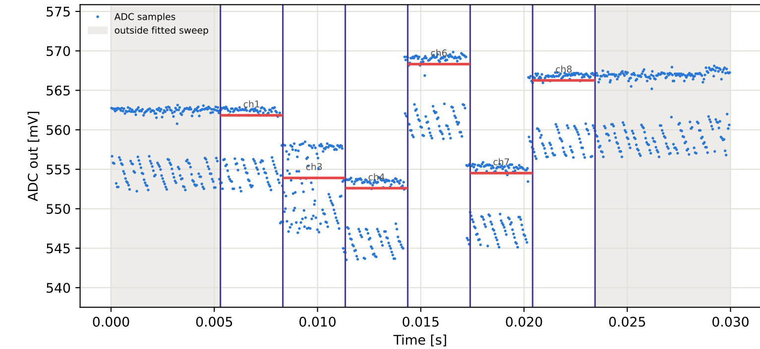
Tag16 &lt;- Tag6 | 965 MHz | run 0 | rep 1 | phase 62.08 deg
