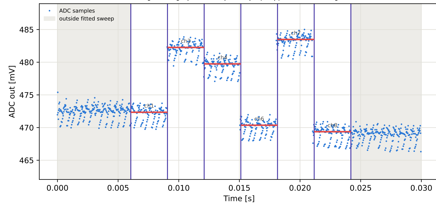
Tag6 &lt;- Tag1 | 835 MHz | run 0 | rep 1 | phase -27.90 deg
