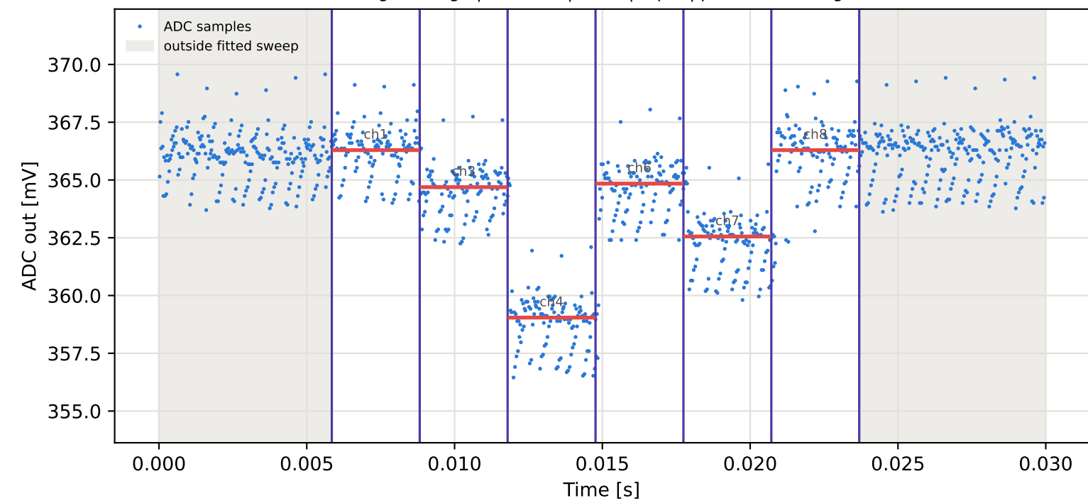
Tag6 &lt;- Tag4 | 985 MHz | run 0 | rep 1 | phase 76.84 deg
