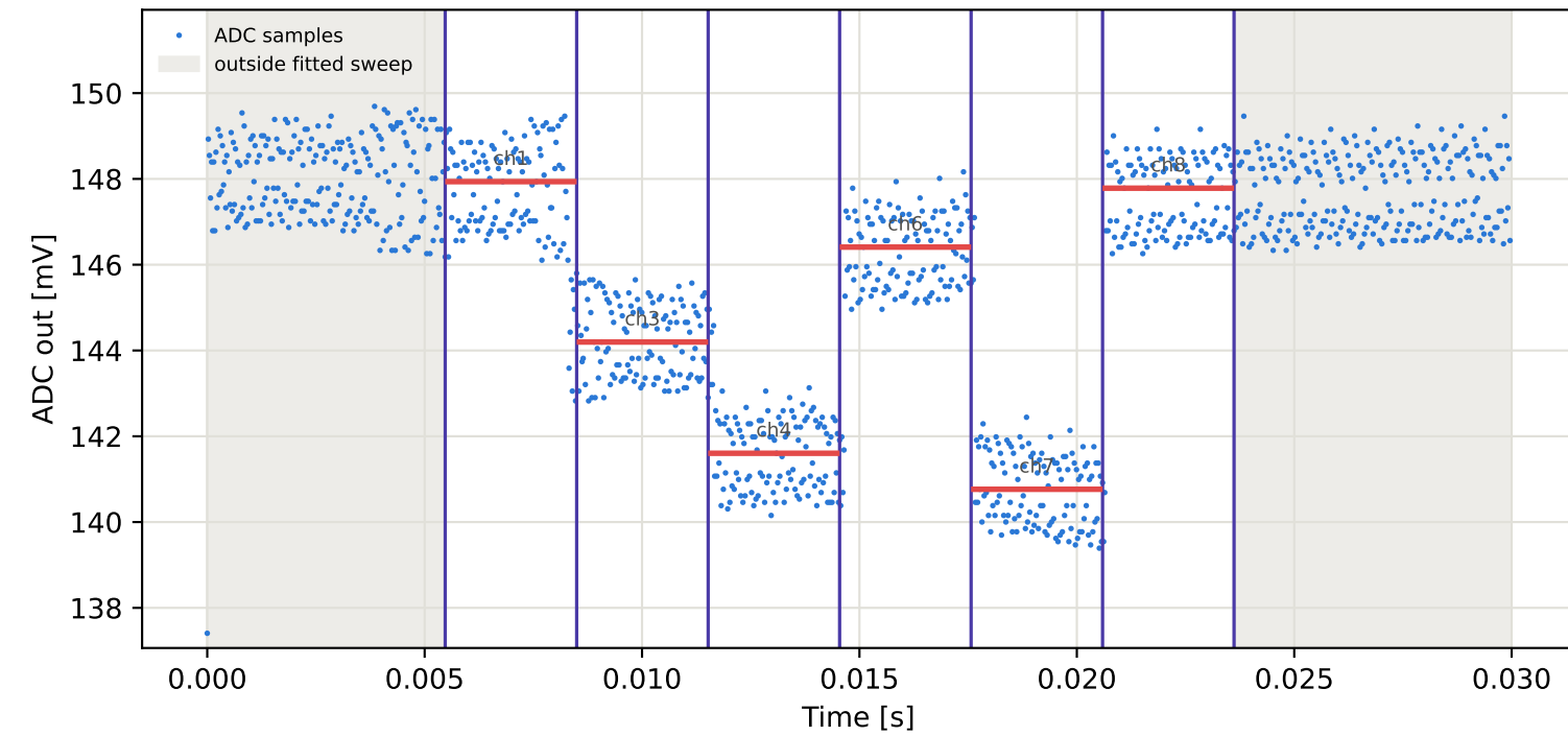
Tag3 &lt;- Tag8 | 785 MHz | run 0 | rep 1 | phase -92.32 deg
