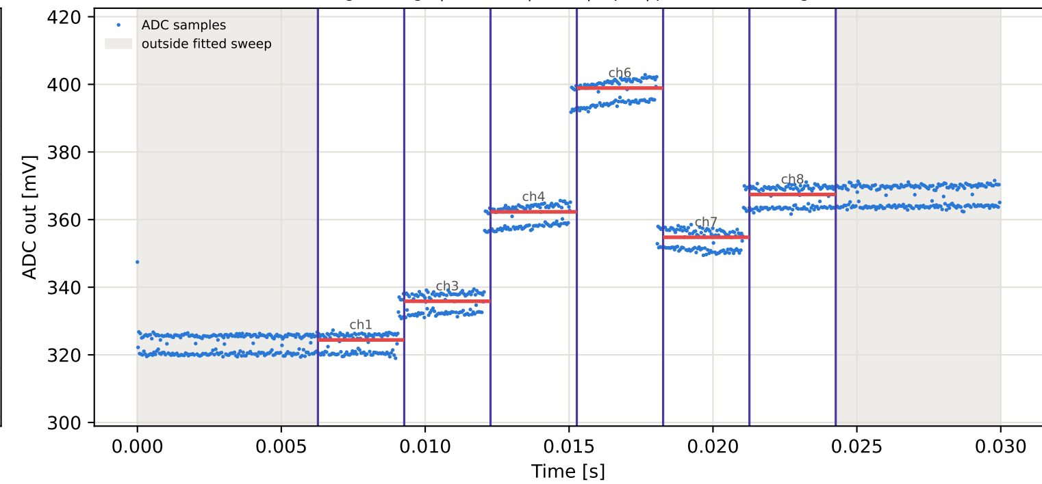
Tag1 &lt;- Tag8 | 885 MHz | run 0 | rep 1 | phase -54.23 deg
