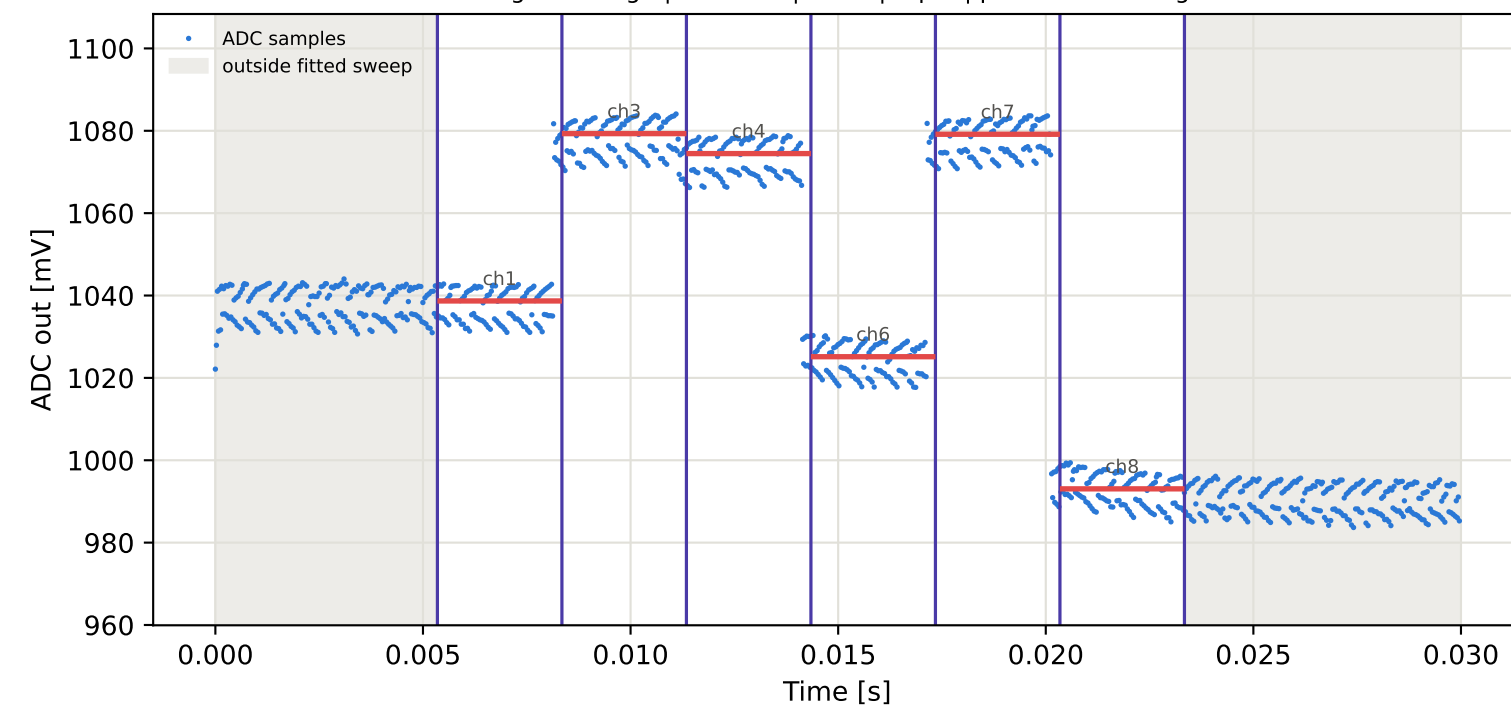
Tag2 &lt;- Tag1 | 875 MHz | run 0 | rep 1 | phase 111.46 deg
