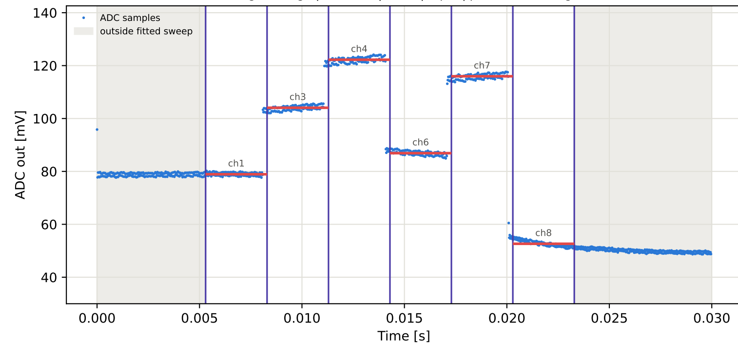
Tag4 &lt;- Tag7 | 905 MHz | run 0 | rep 1 | phase 43.35 deg
