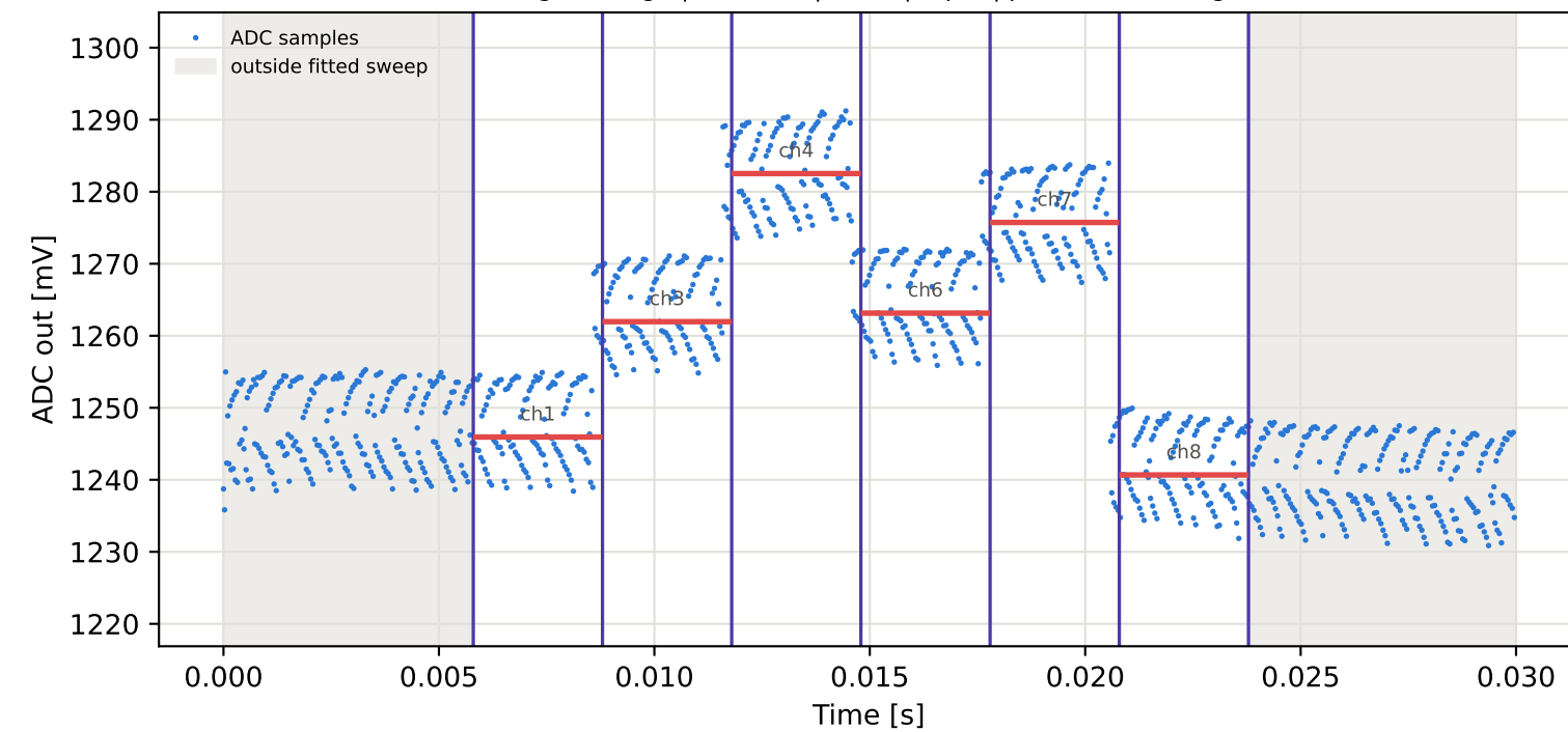
Tag8 &lt;- Tag4 | 915 MHz | run 0 | rep 1 | phase 147.10 deg
