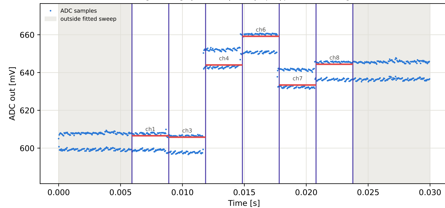
Tag2 &lt;- Tag1 | 835 MHz | run 0 | rep 1 | phase -27.96 deg
