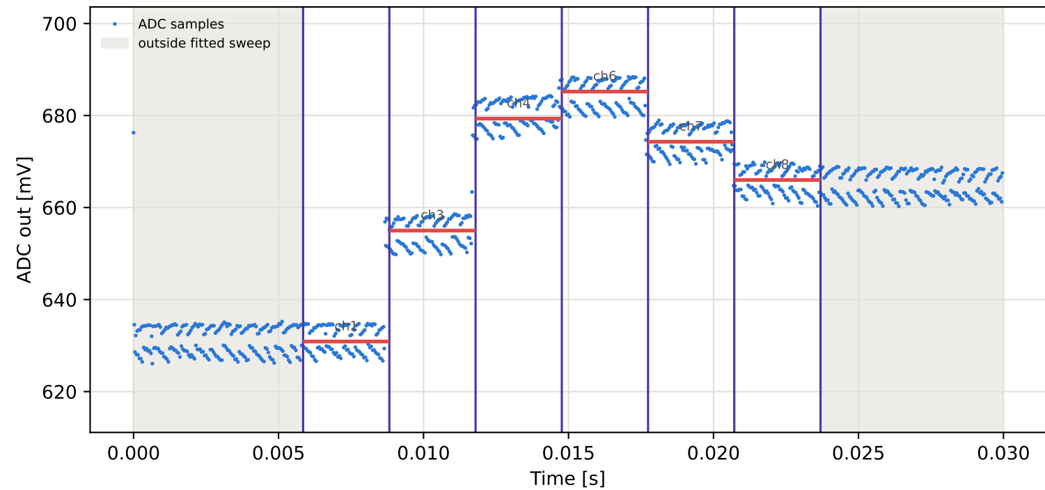
Tag16 &lt;- Tag5 | 855 MHz | run 0 | rep 1 | phase -94.11 deg
