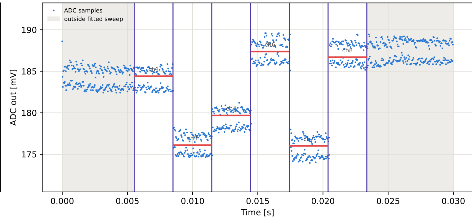
Tag16 &lt;- Tag7 | 805 MHz | run 0 | rep 1 | phase -40.82 deg
