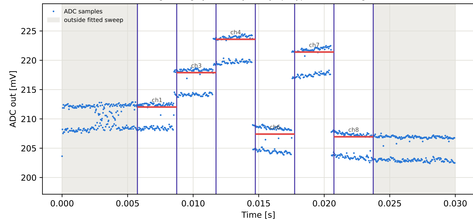
Tag6 &lt;- Tag9 | 935 MHz | run 0 | rep 1 | phase -80.84 deg
