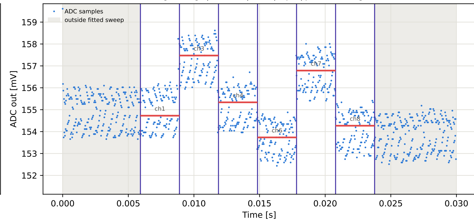
Tag8 &lt;- Tag10 | 785 MHz | run 0 | rep 1 | phase 79.16 deg
