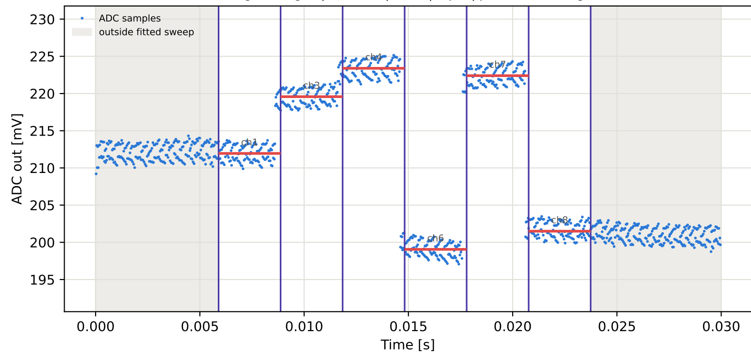
Tag6 &lt;- Tag2 | 935 MHz | run 0 | rep 1 | phase -19.94 deg
