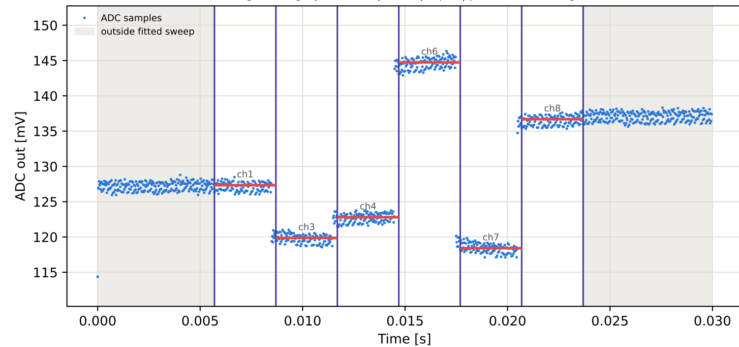
Tag1 &lt;- Tag7 | 995 MHz | run 0 | rep 1 | phase 151.78 deg
