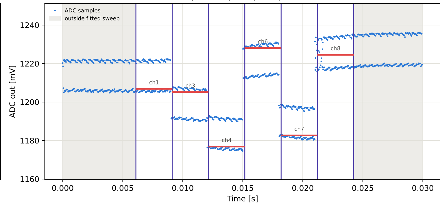
Tag15 &lt;- Tag4 | 895 MHz | run 0 | rep 1 | phase -178.92 deg
