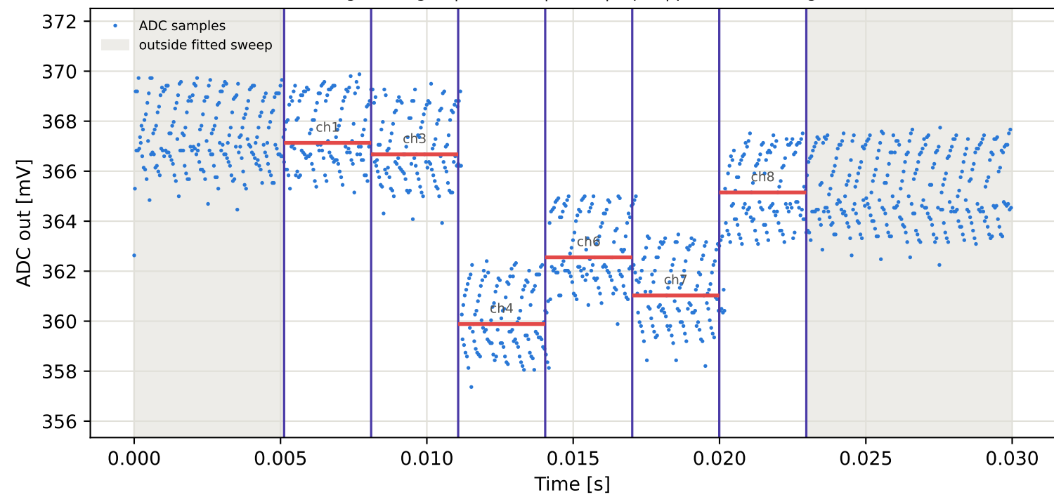
Tag7 &lt;- Tag3 | 805 MHz | run 0 | rep 1 | phase -61.83 deg
