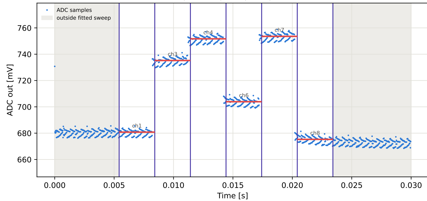
Tag16 &lt;- Tag7 | 865 MHz | run 0 | rep 1 | phase -69.04 deg
