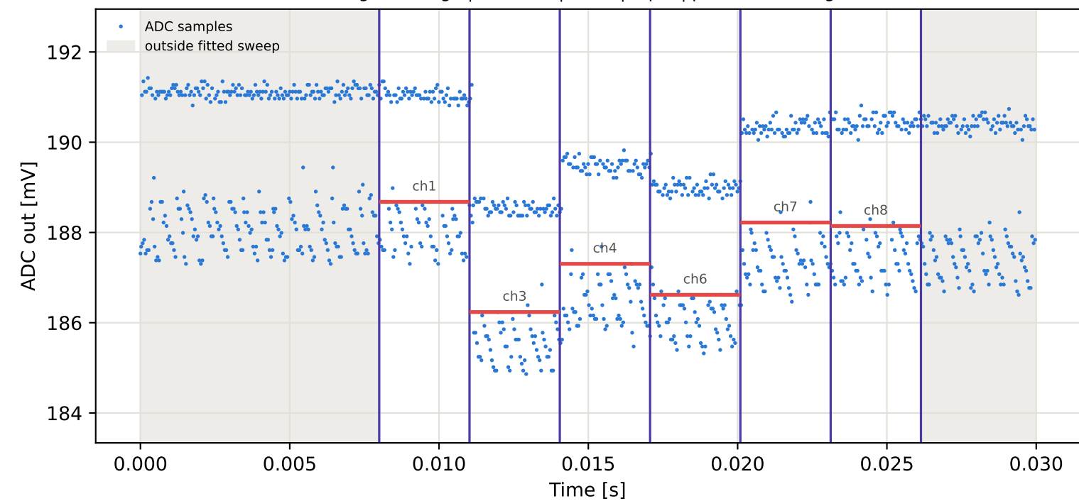
Tag10 &lt;- Tag5 | 785 MHz | run 0 | rep 1 | phase 64.03 deg
