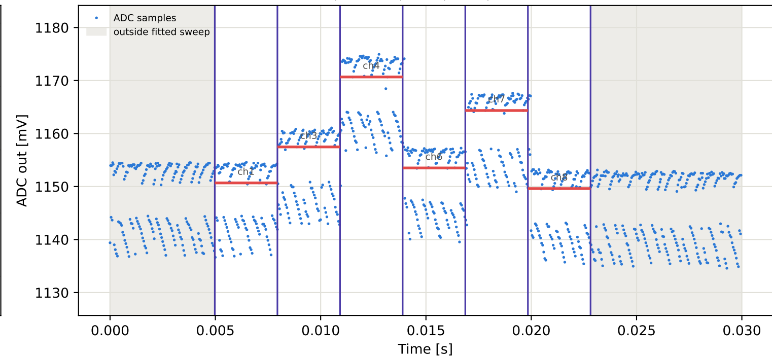
Tag7 &lt;- Tag6 | 975 MHz | run 0 | rep 1 | phase -91.53 deg
