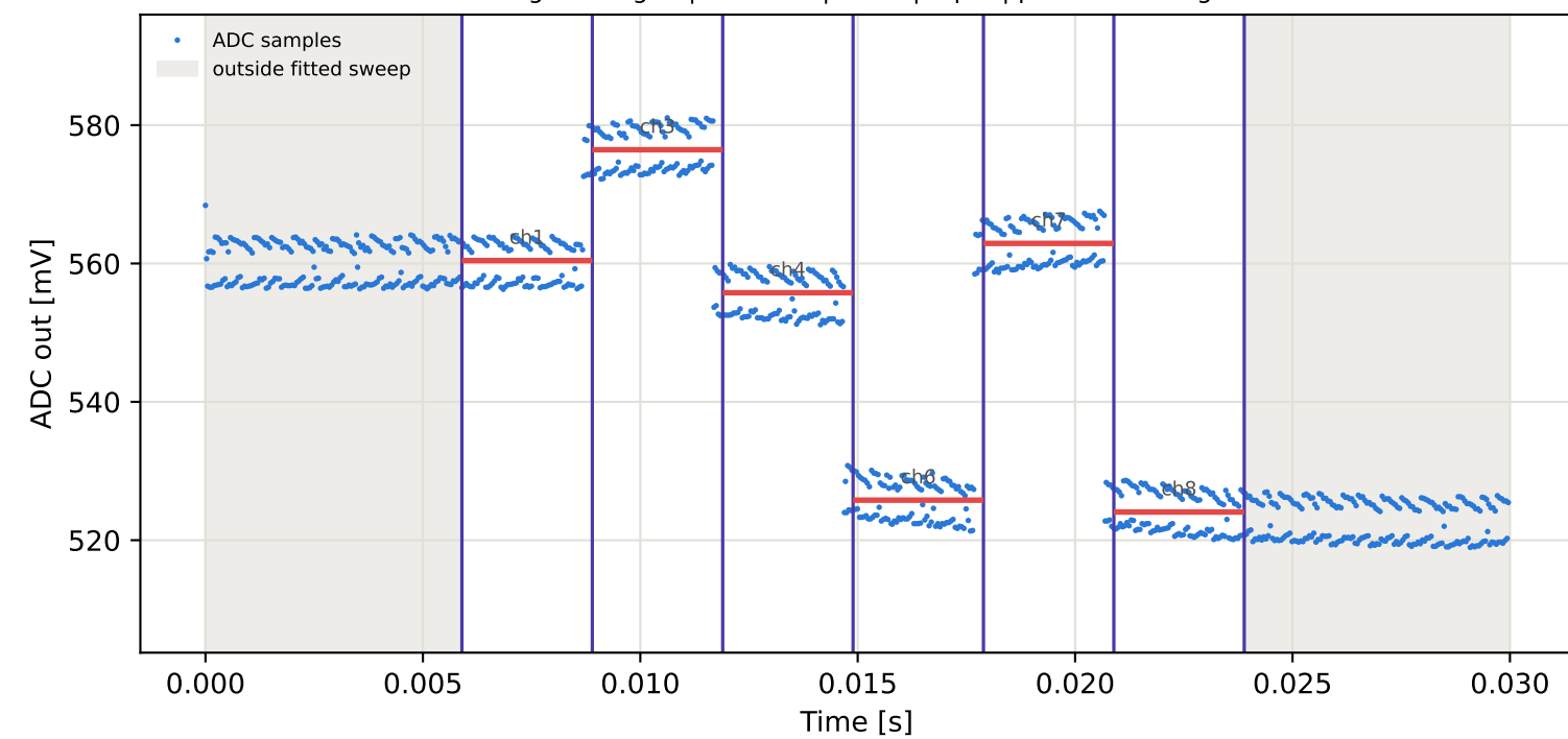
Tag6 &lt;- Tag3 | 865 MHz | run 0 | rep 1 | phase 81.56 deg
