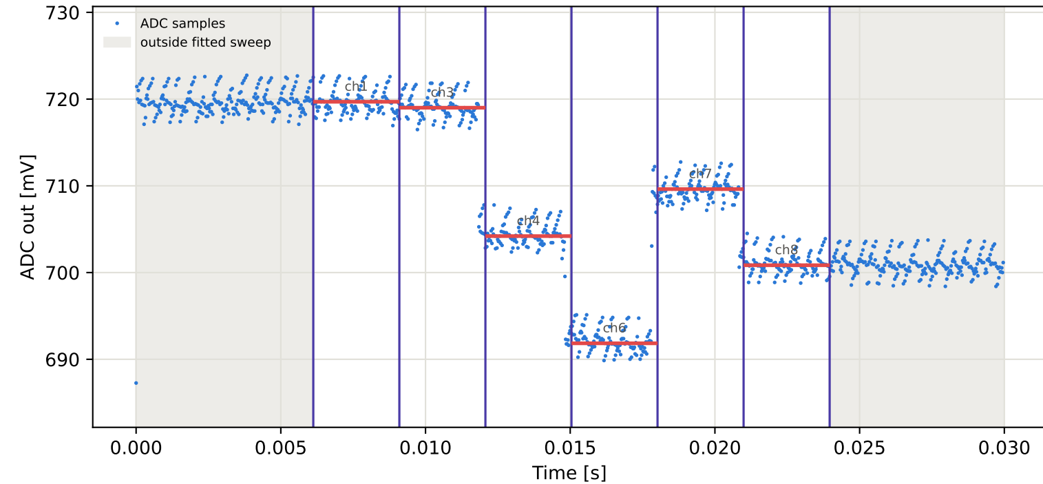
Tag15 &lt;- Tag10 | 865 MHz | run 0 | rep 1 | phase 6.34 deg
