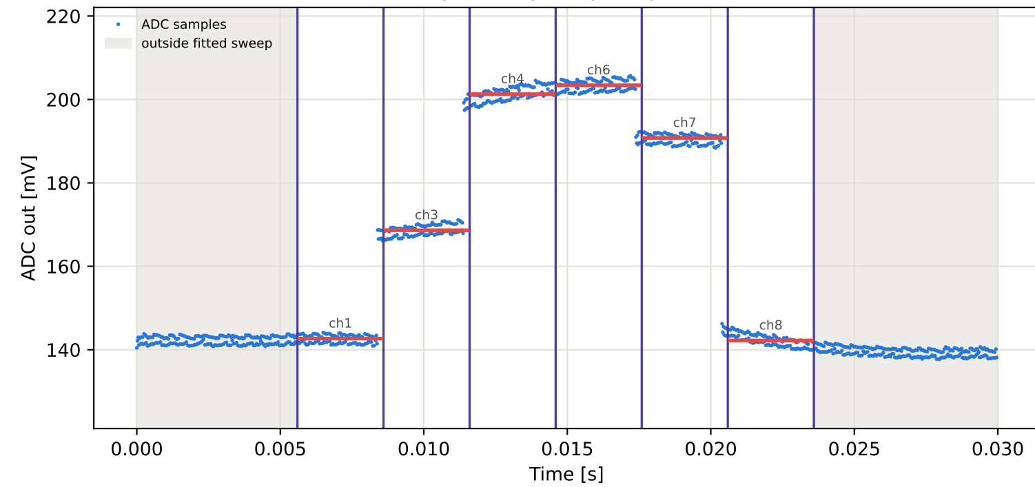
Tag7 &lt;- Tag10 | 905 MHz | run 0 | rep 1 | phase -114.41 deg
