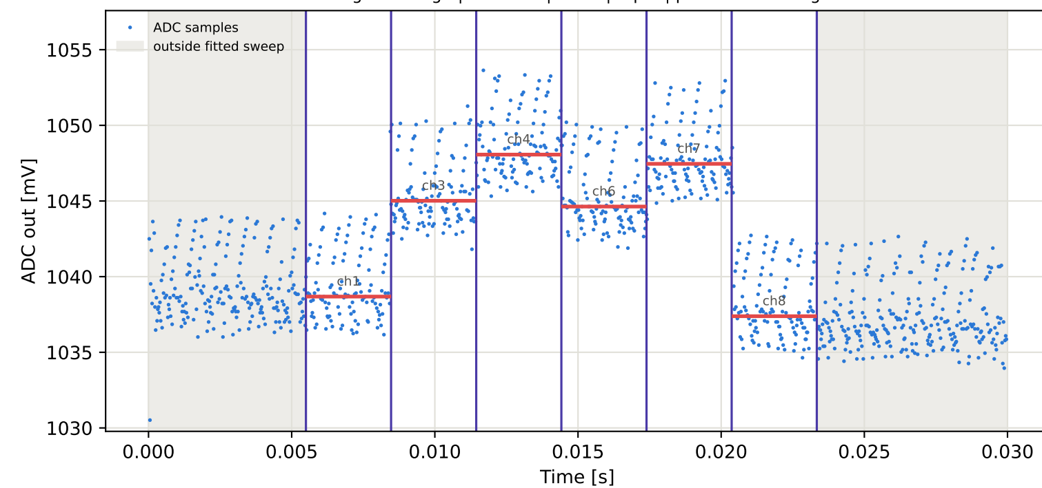
Tag16 &lt;- Tag6 | 875 MHz | run 0 | rep 1 | phase -120.98 deg
