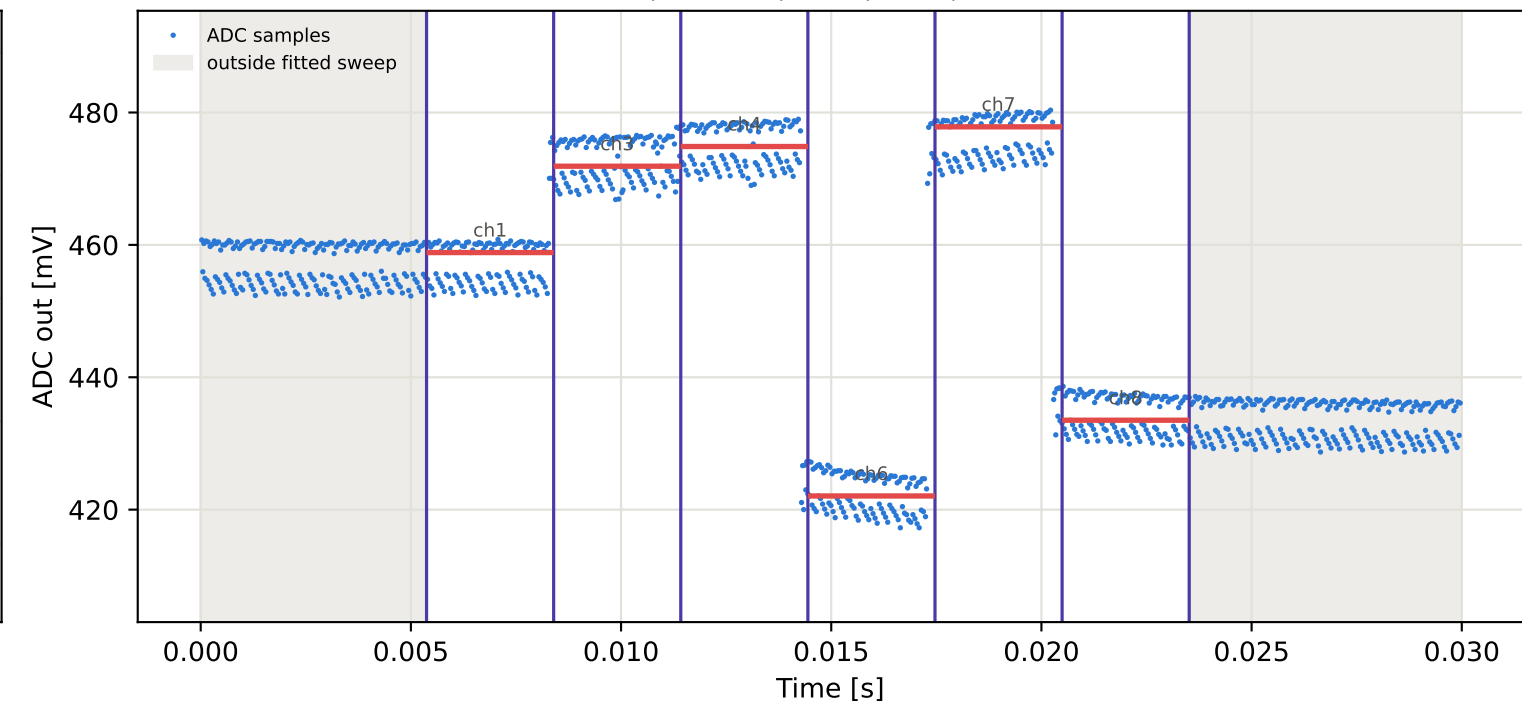
Tag3 &lt;- Tag9 | 945 MHz | run 0 | rep 1 | phase -21.29 deg
