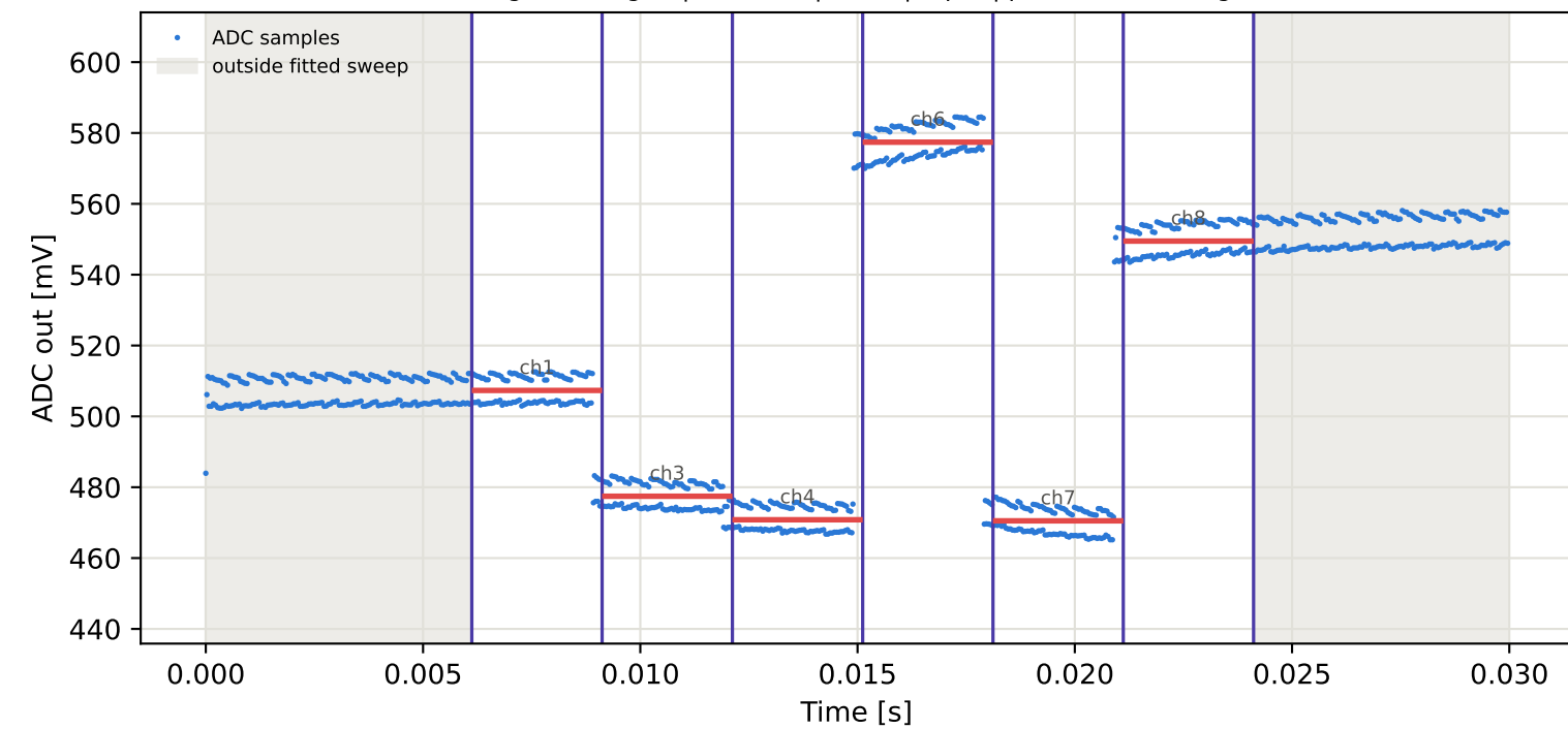
Tag15 &lt;- Tag3 | 945 MHz | run 0 | rep 1 | phase 177.43 deg
