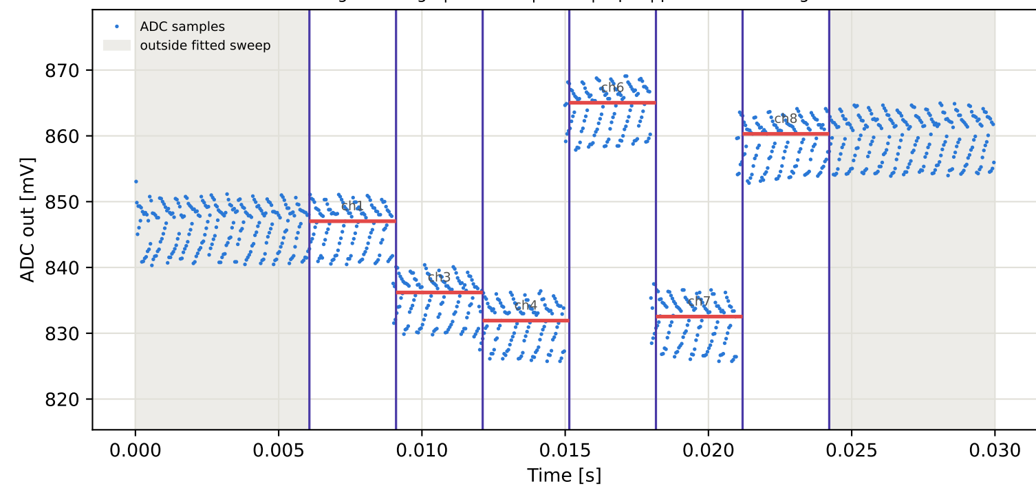
Tag2 &lt;- Tag10 | 955 MHz | run 0 | rep 1 | phase -20.19 deg
