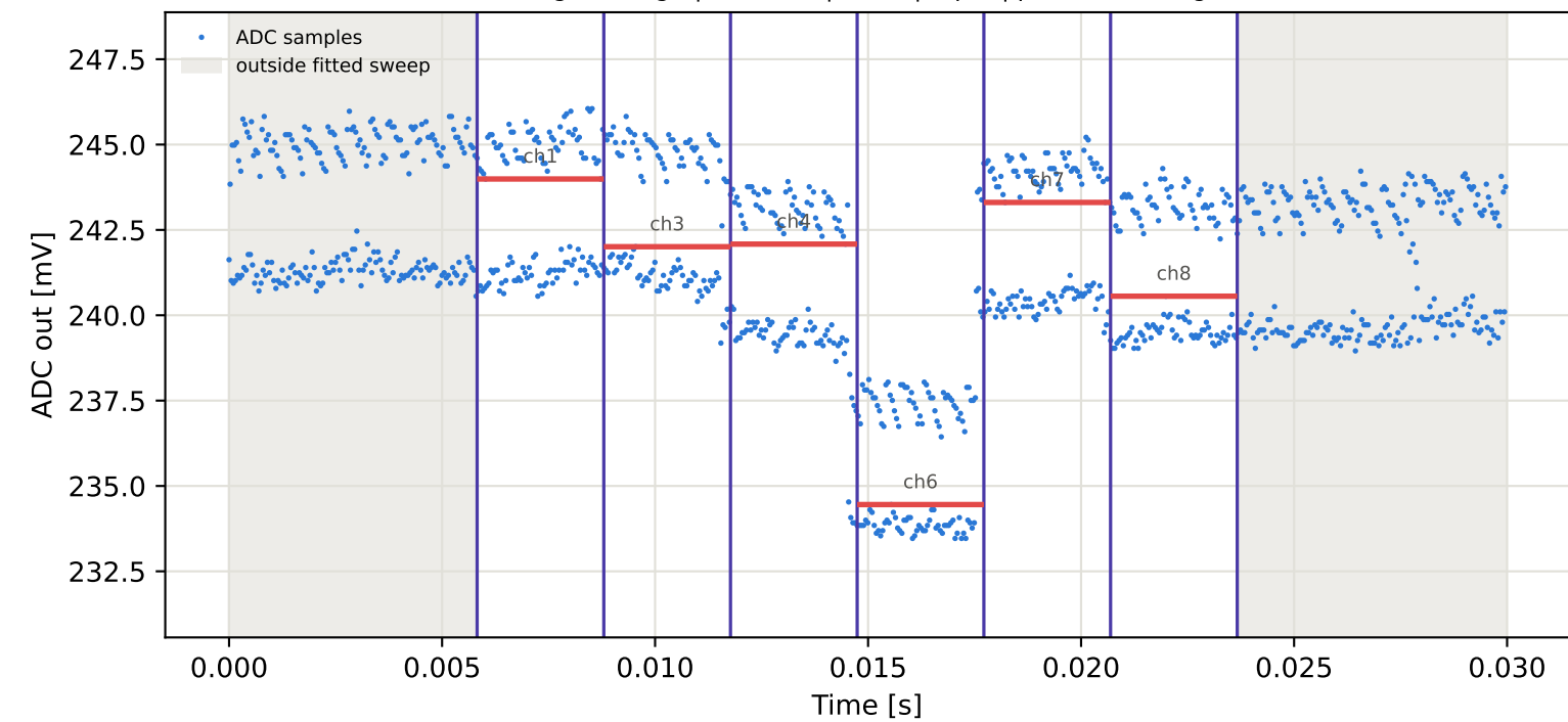
Tag8 &lt;- Tag4 | 995 MHz | run 0 | rep 1 | phase -4.93 deg
