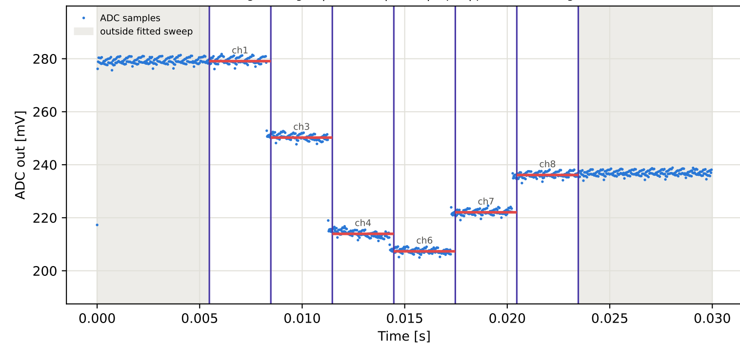
Tag9 &lt;- Tag16 | 855 MHz | run 0 | rep 1 | phase -127.39 deg
