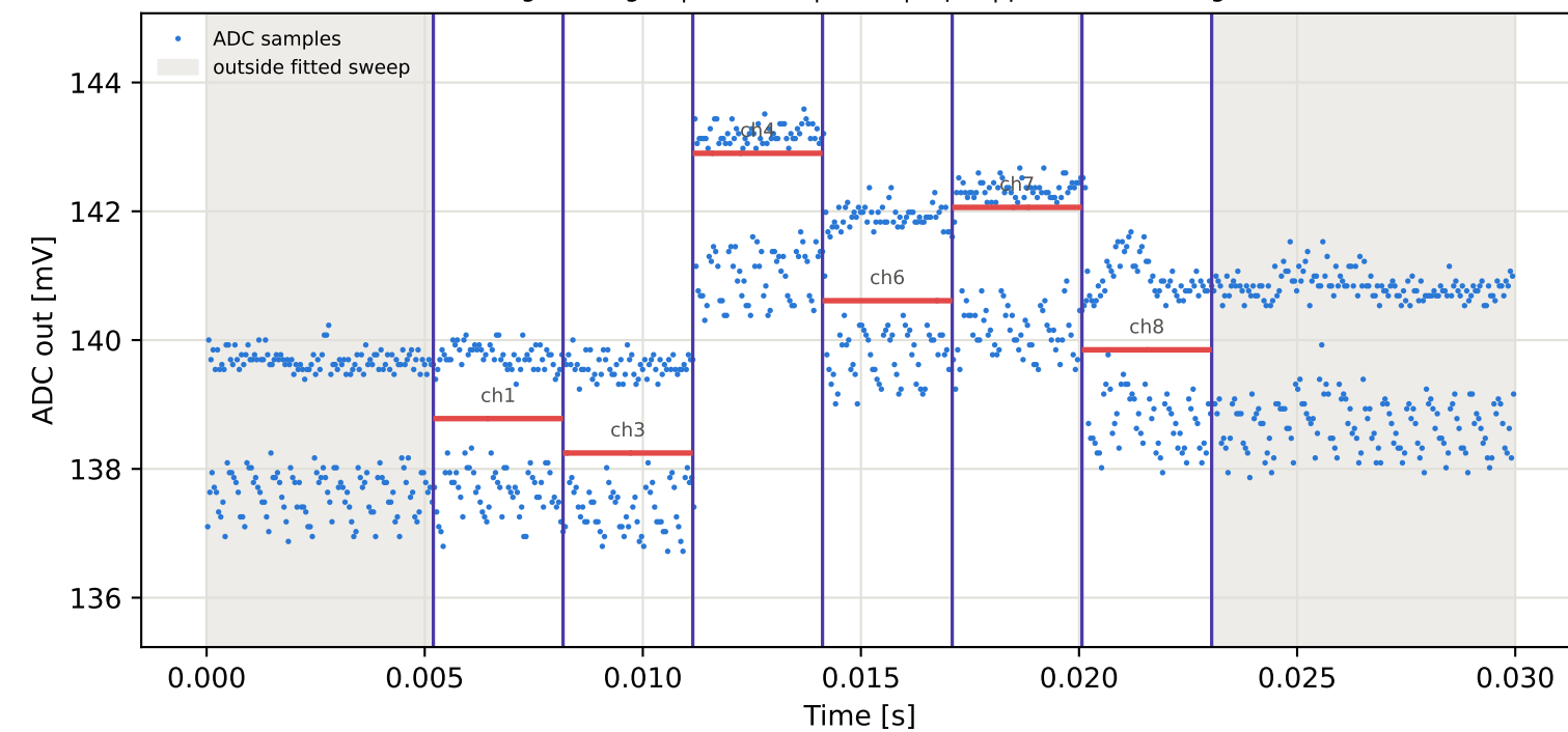
Tag8 &lt;- Tag15 | 795 MHz | run 0 | rep 1 | phase -98.86 deg
