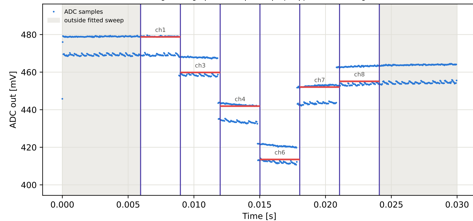
Tag6 &lt;- Tag1 | 915 MHz | run 0 | rep 1 | phase 37.52 deg
