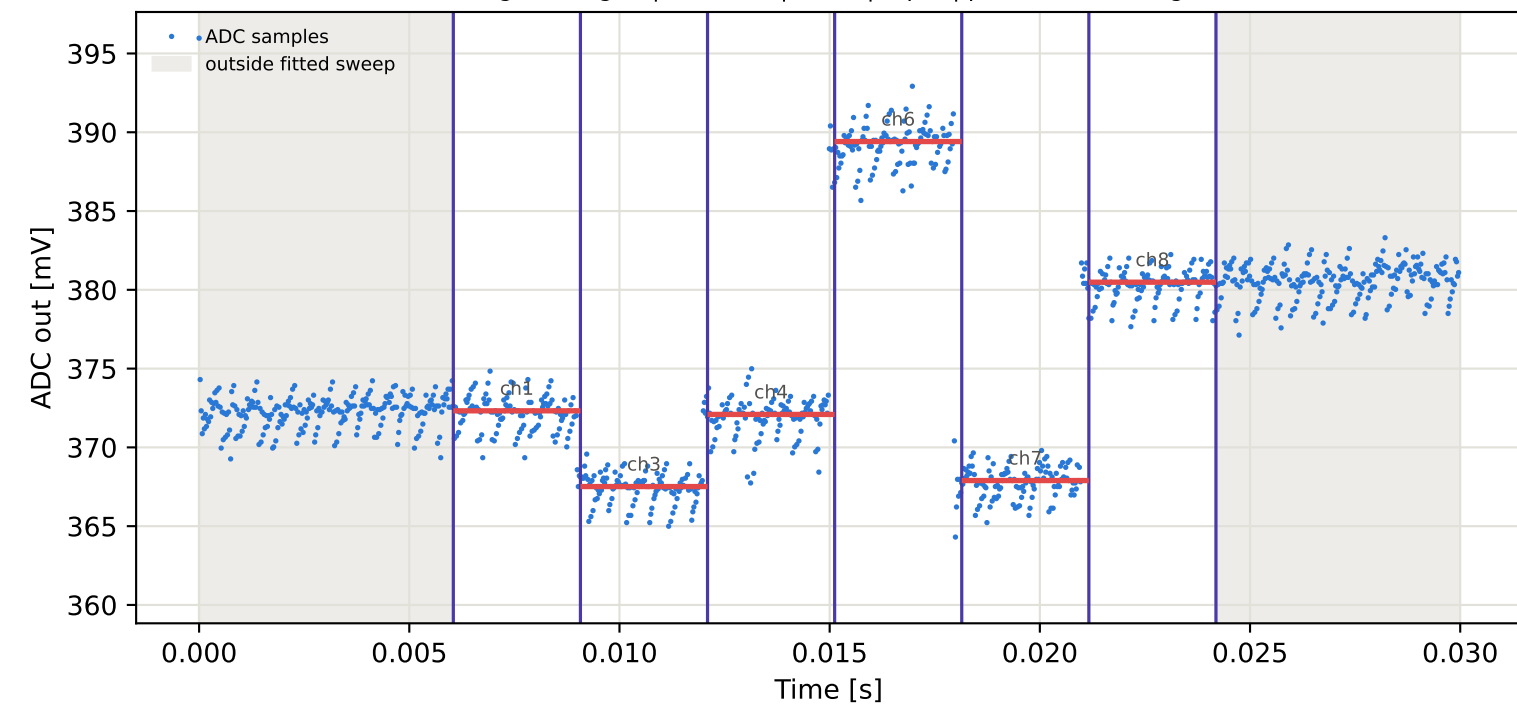
Tag5 &lt;- Tag16 | 975 MHz | run 0 | rep 1 | phase 87.80 deg
