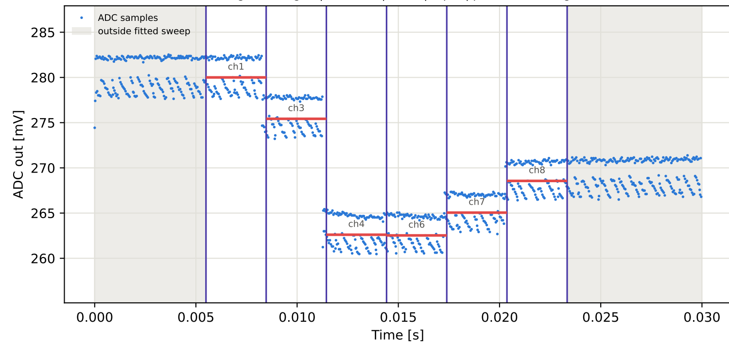
Tag10 &lt;- Tag3 | 845 MHz | run 0 | rep 1 | phase 42.70 deg
