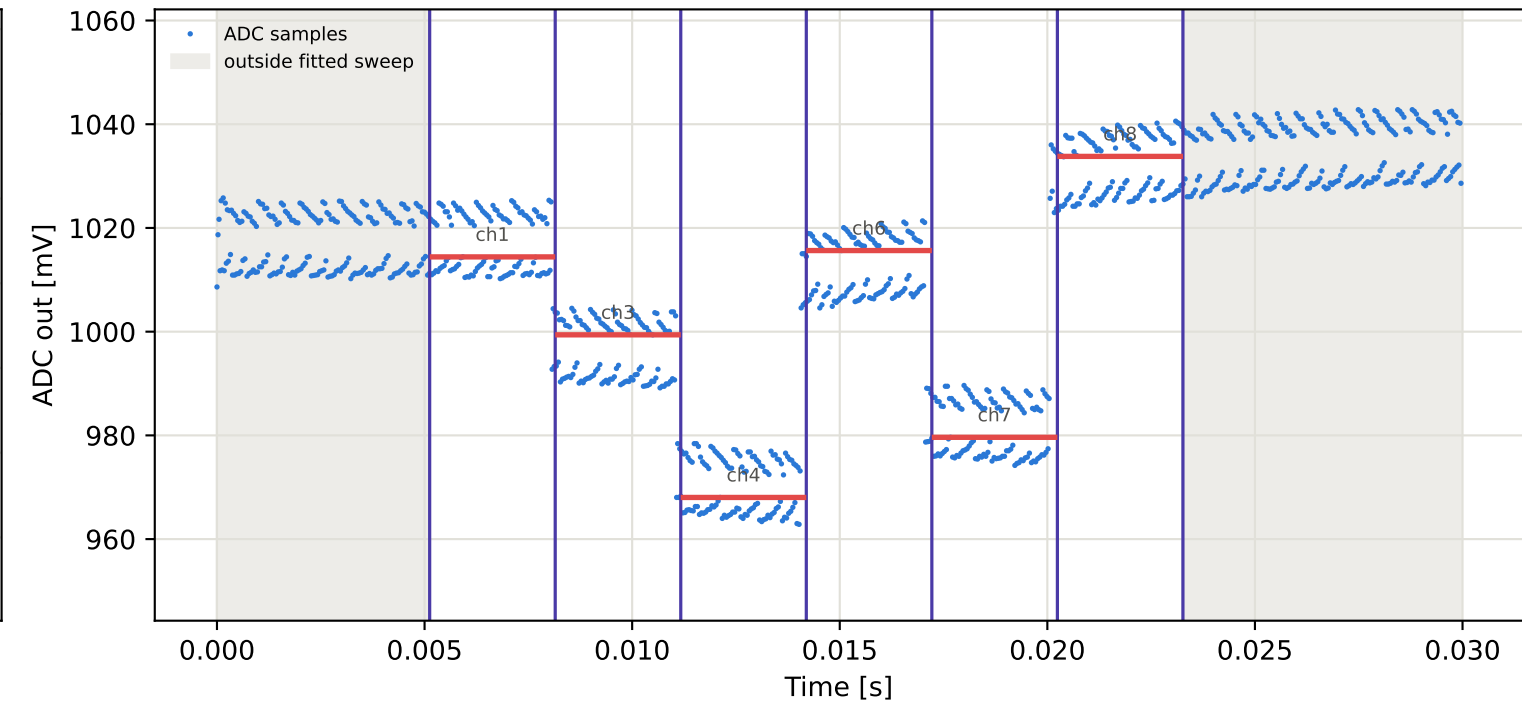
Tag9 &lt;- Tag8 | 925 MHz | run 0 | rep 1 | phase 8.49 deg
