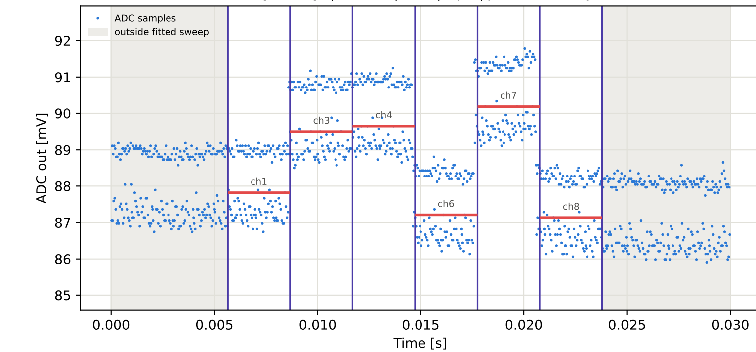
Tag1 &lt;- Tag9 | 805 MHz | run 0 | rep 1 | phase -126.72 deg
