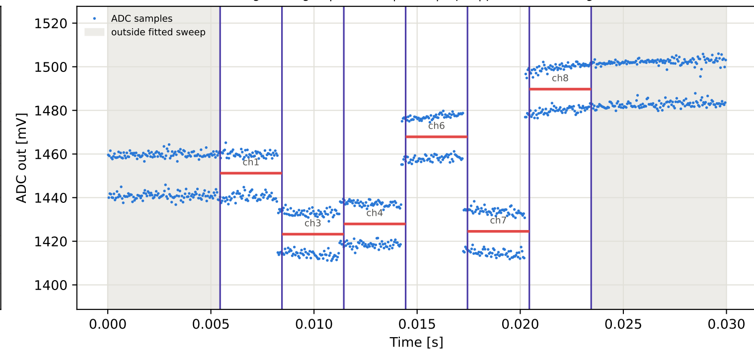
Tag8 &lt;- Tag16 | 885 MHz | run 0 | rep 1 | phase 147.92 deg
