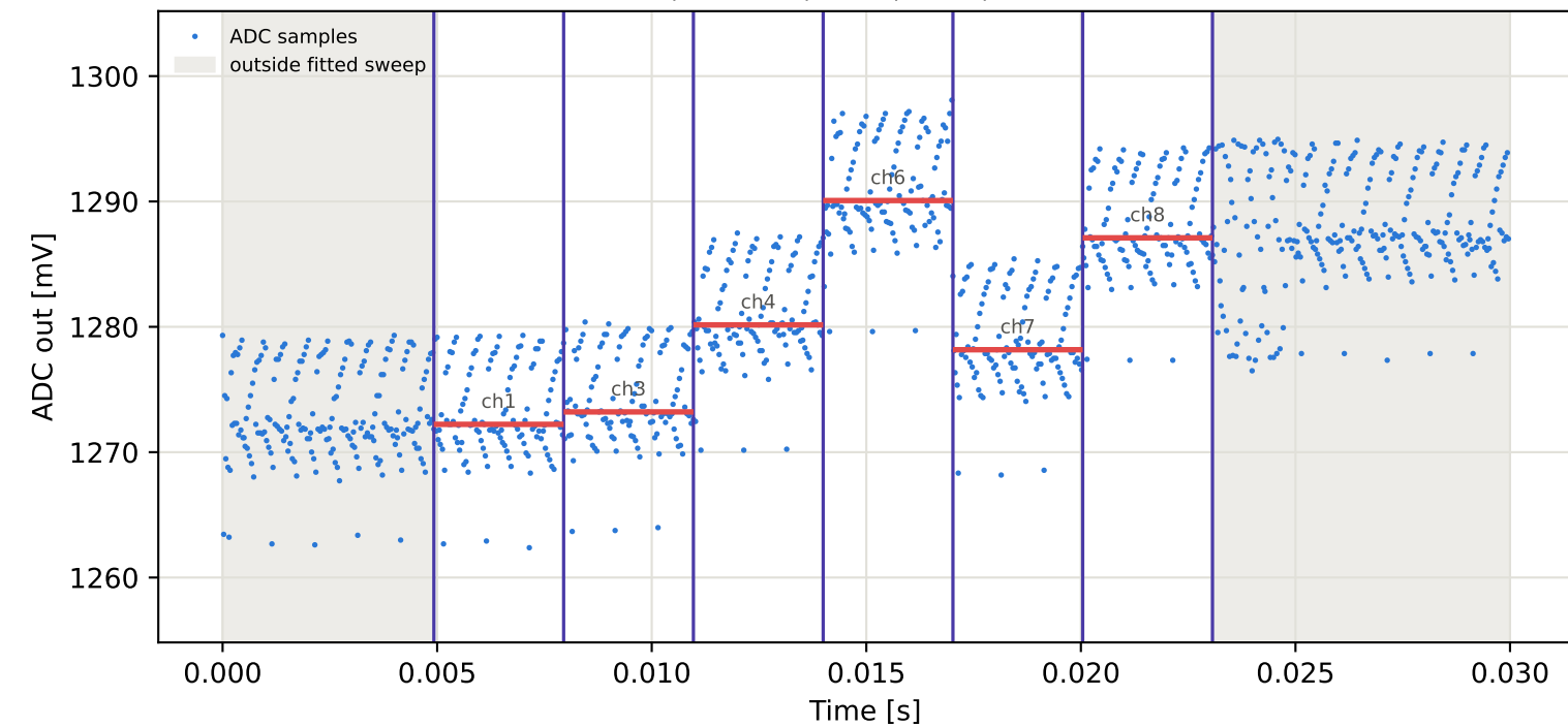
Tag7 &lt;- Tag5 | 875 MHz | run 0 | rep 1 | phase -156.85 deg
