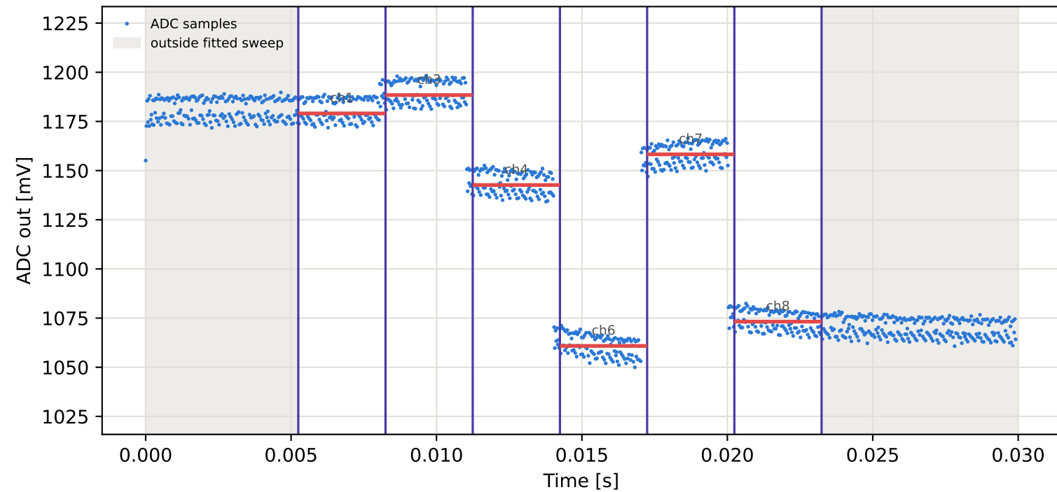
Tag3 &lt;- Tag2 | 885 MHz | run 0 | rep 1 | phase 75.15 deg
