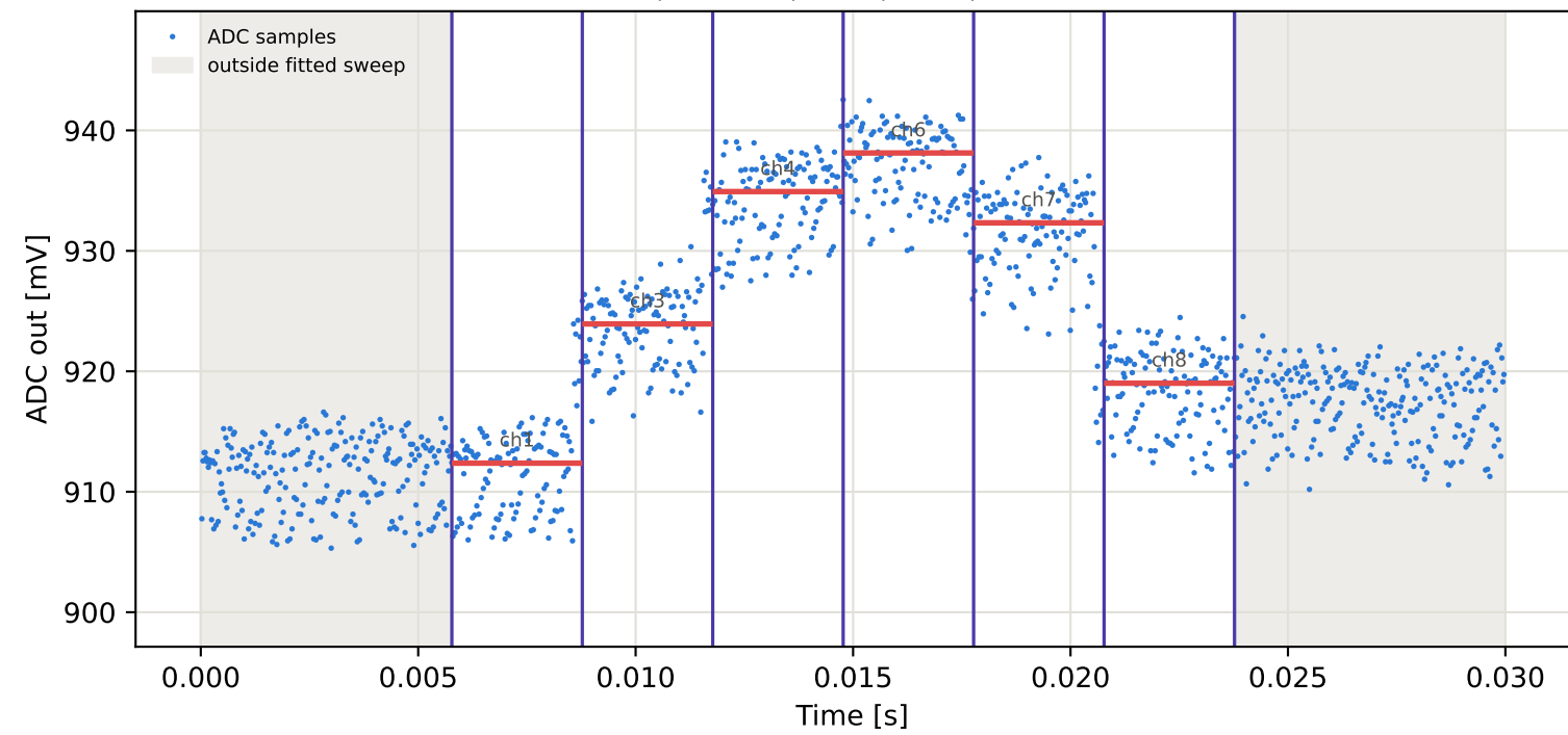
Tag6 &lt;- Tag5 | 885 MHz | run 0 | rep 1 | phase -120.37 deg
