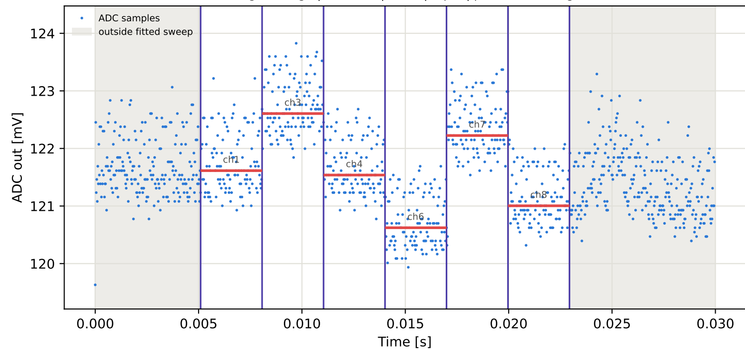
Tag3 &lt;- Tag15 | 795 MHz | run 0 | rep 1 | phase -105.50 deg
