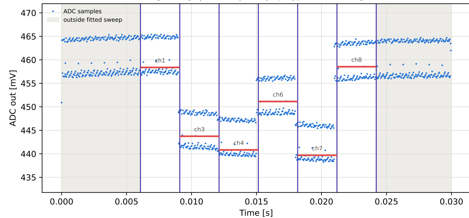
Tag3 &lt;- Tag6 | 845 MHz | run 0 | rep 1 | phase -132.62 deg
