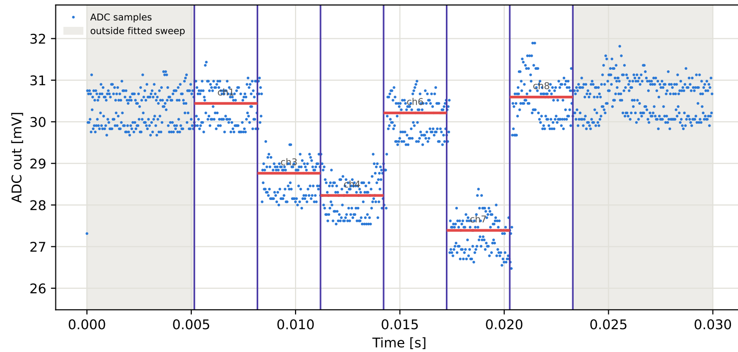
Tag2 &lt;- Tag5 | 795 MHz | run 0 | rep 1 | phase 166.64 deg
