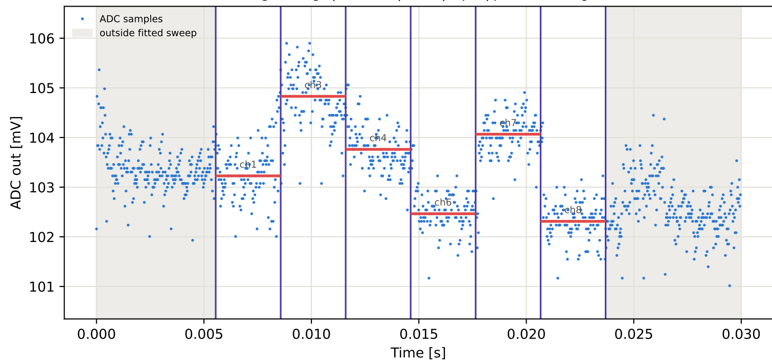
Tag5 &lt;- Tag4 | 775 MHz | run 0 | rep 1 | phase 69.41 deg
