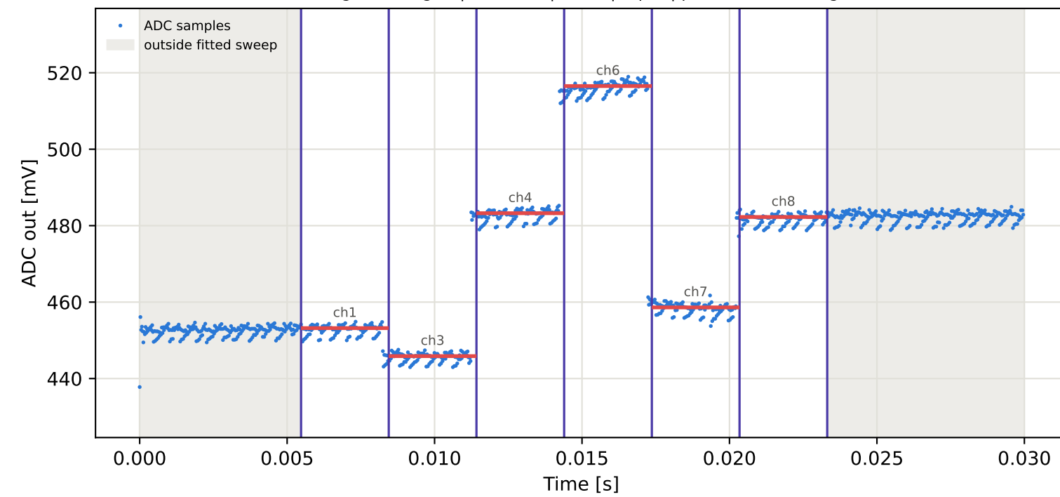
Tag15 &lt;- Tag3 | 975 MHz | run 0 | rep 1 | phase -120.30 deg
