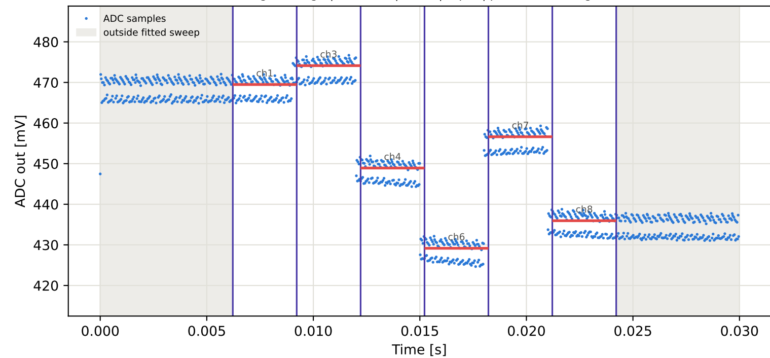
Tag3 &lt;- Tag7 | 855 MHz | run 0 | rep 1 | phase -125.81 deg
