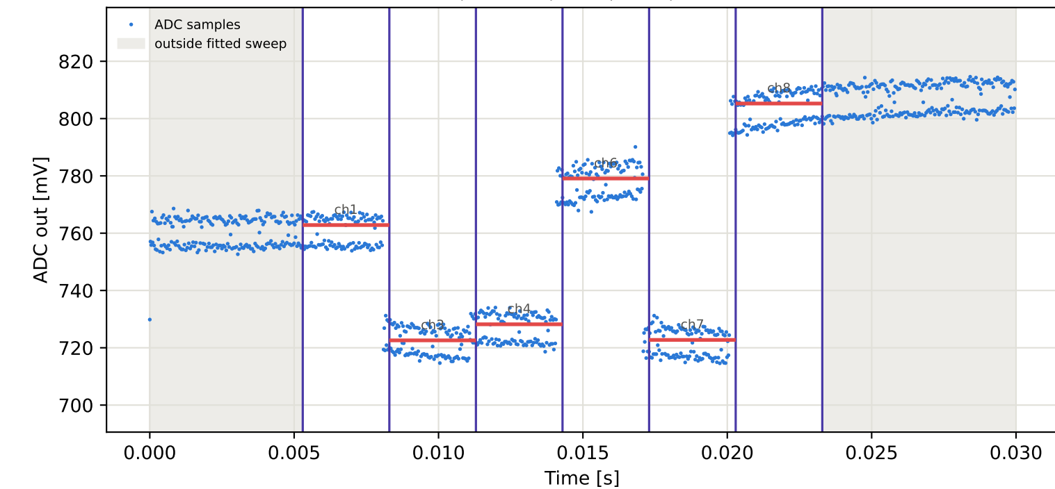
Tag2 &lt;- Tag15 | 885 MHz | run 0 | rep 1 | phase 148.05 deg
