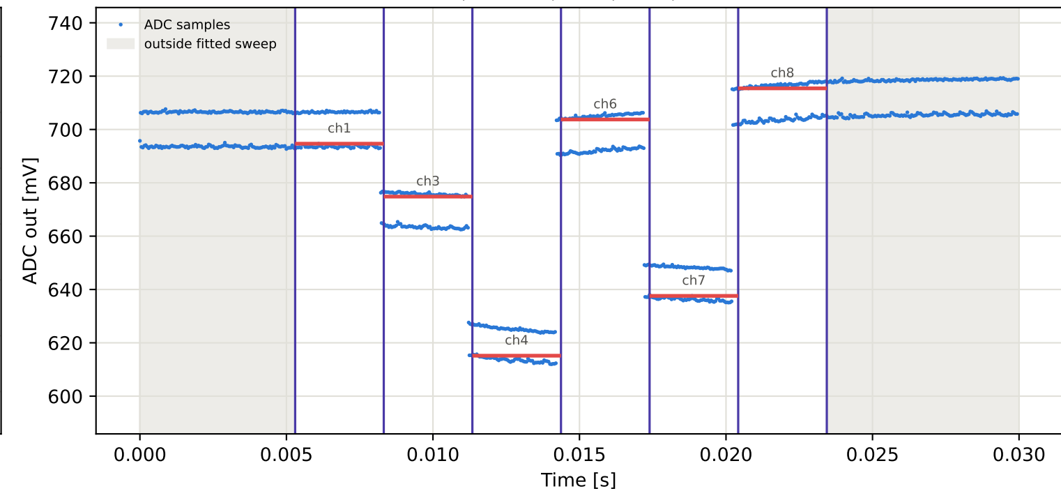
Tag16 &lt;- Tag7 | 975 MHz | run 0 | rep 1 | phase 98.40 deg
