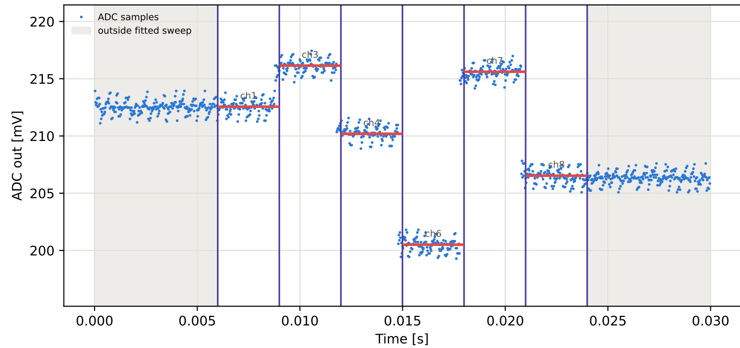
Tag4 &lt;- Tag8 | 995 MHz | run 0 | rep 1 | phase -76.22 deg
