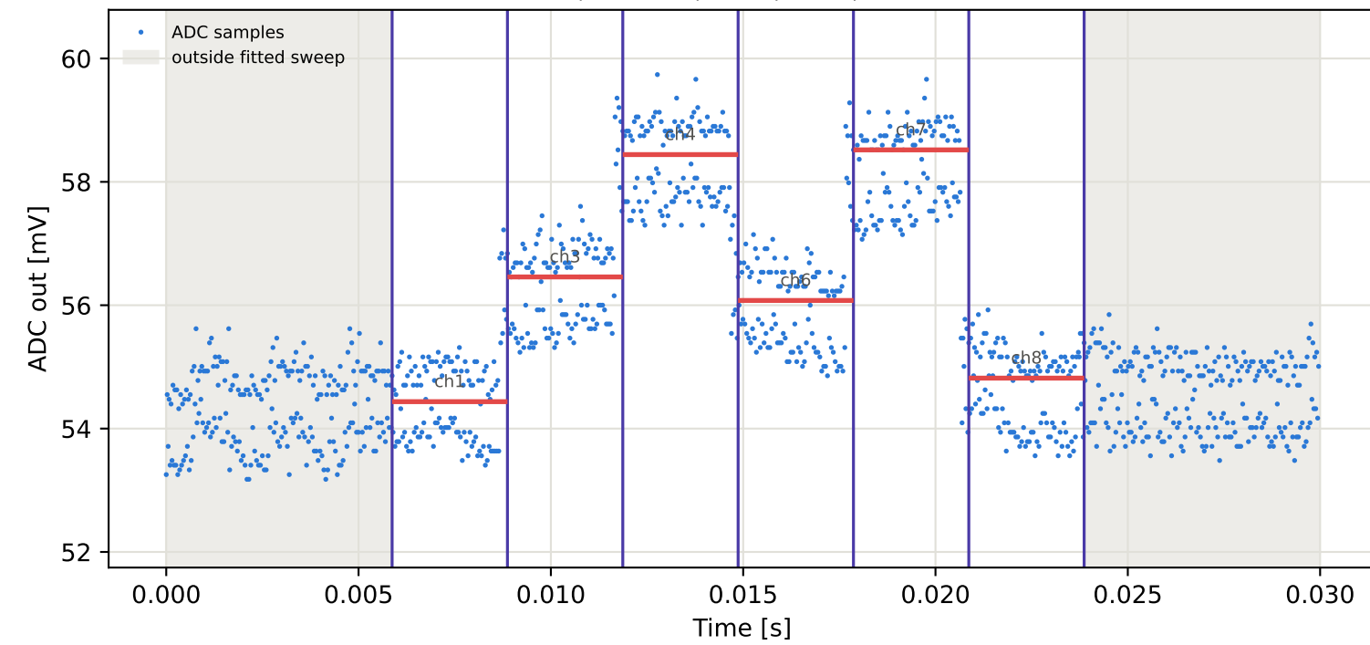
Tag9 &lt;- Tag7 | 795 MHz | run 0 | rep 1 | phase -75.93 deg
