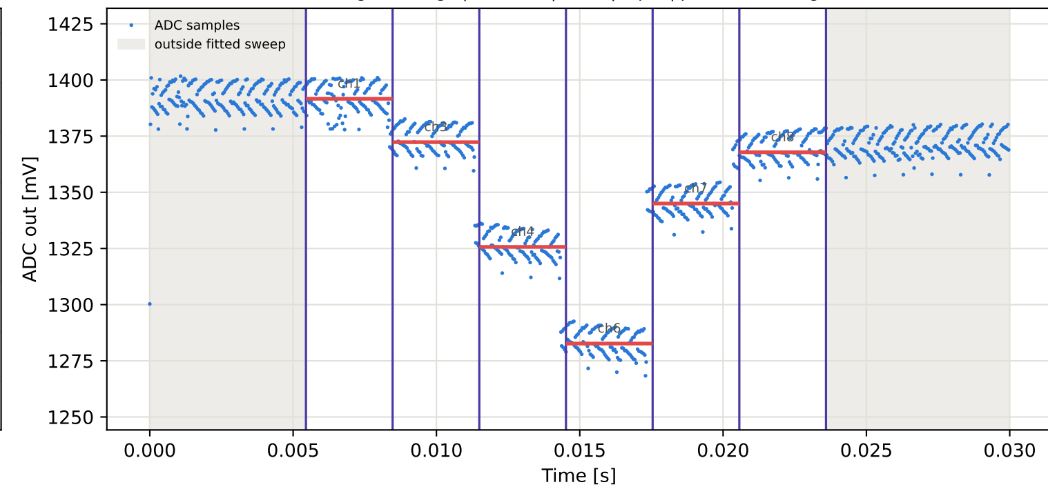
Tag16 &lt;- Tag5 | 925 MHz | run 0 | rep 1 | phase 57.38 deg
