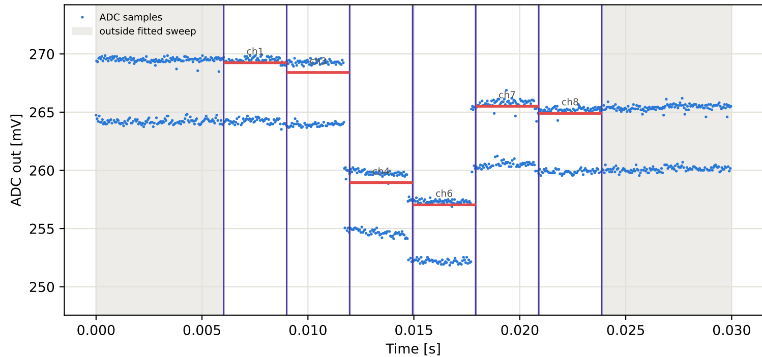
Tag8 &lt;- Tag7 | 975 MHz | run 0 | rep 1 | phase 91.65 deg
