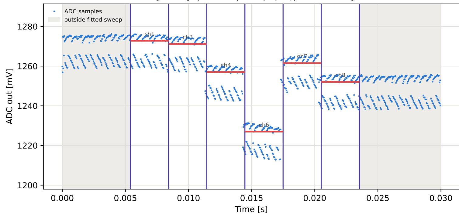
Tag8 &lt;- Tag7 | 905 MHz | run 0 | rep 1 | phase 23.16 deg
