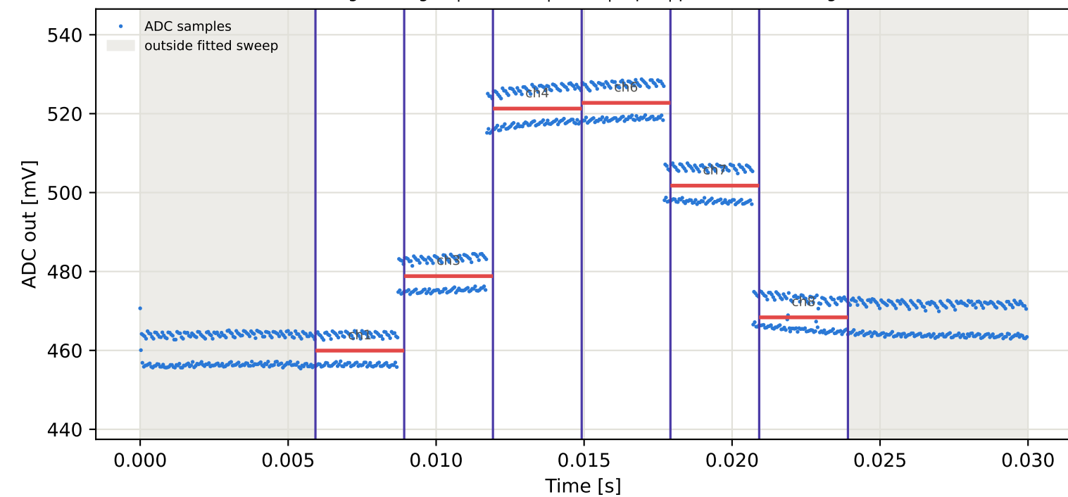
Tag3 &lt;- Tag16 | 935 MHz | run 0 | rep 1 | phase -124.66 deg
