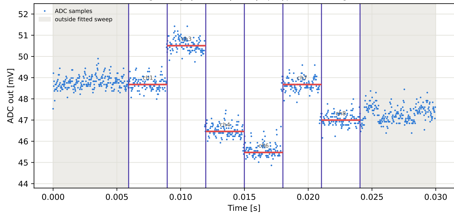
Tag9 &lt;- Tag15 | 775 MHz | run 0 | rep 1 | phase -119.34 deg
