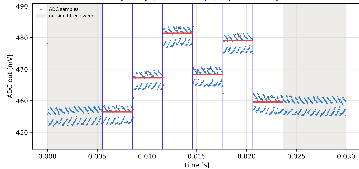
Tag6 &lt;- Tag9 | 835 MHz | run 0 | rep 1 | phase 152.82 deg
