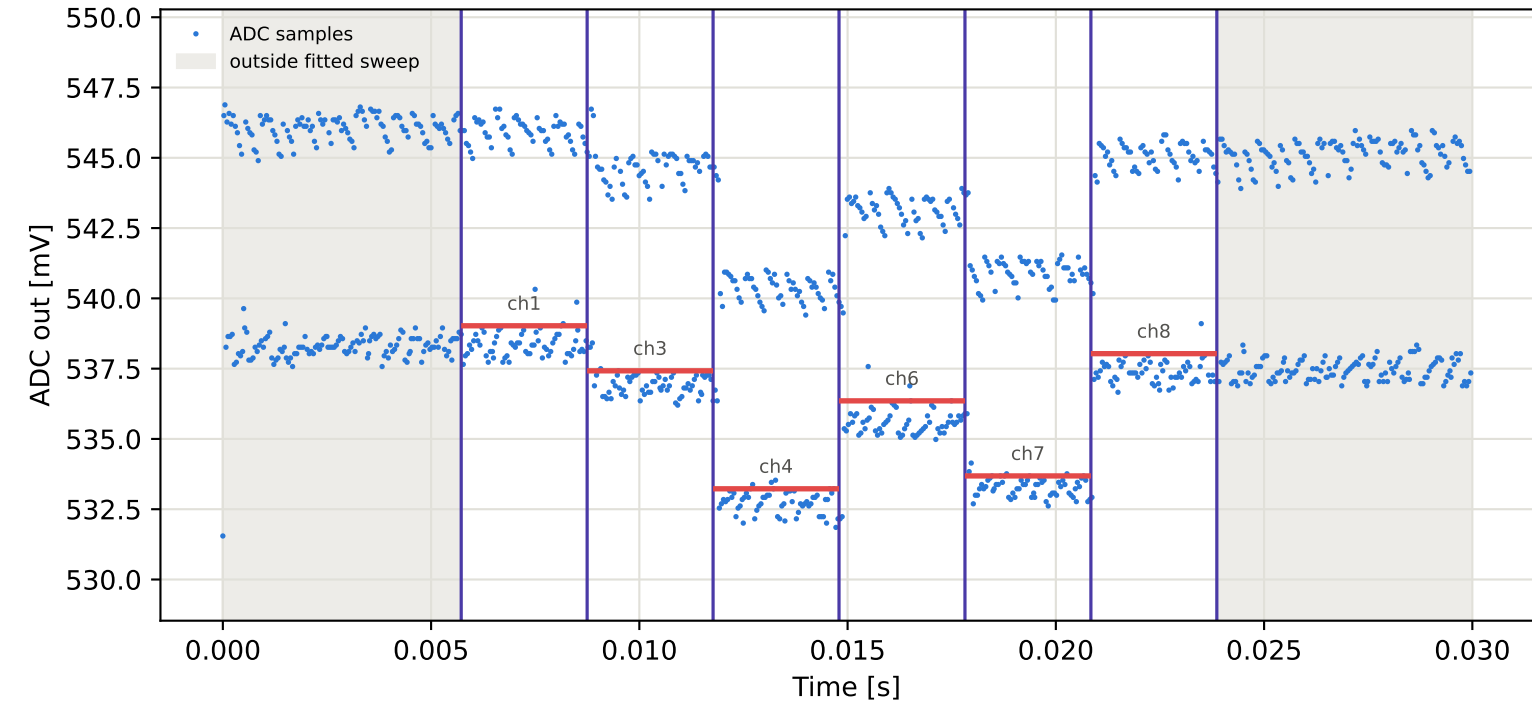
Tag7 &lt;- Tag15 | 825 MHz | run 0 | rep 1 | phase -72.36 deg
