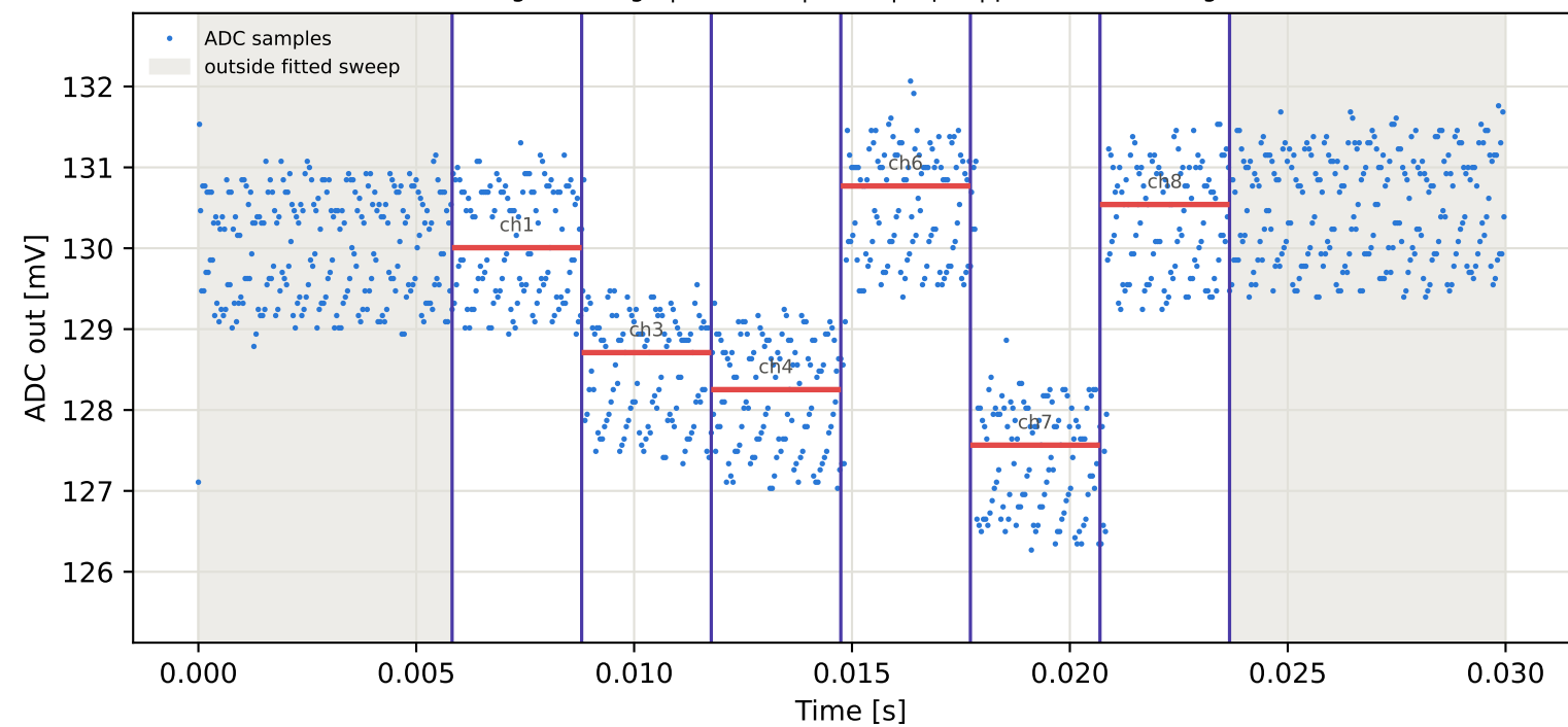
Tag10 &lt;- Tag1 | 775 MHz | run 0 | rep 1 | phase 149.99 deg
