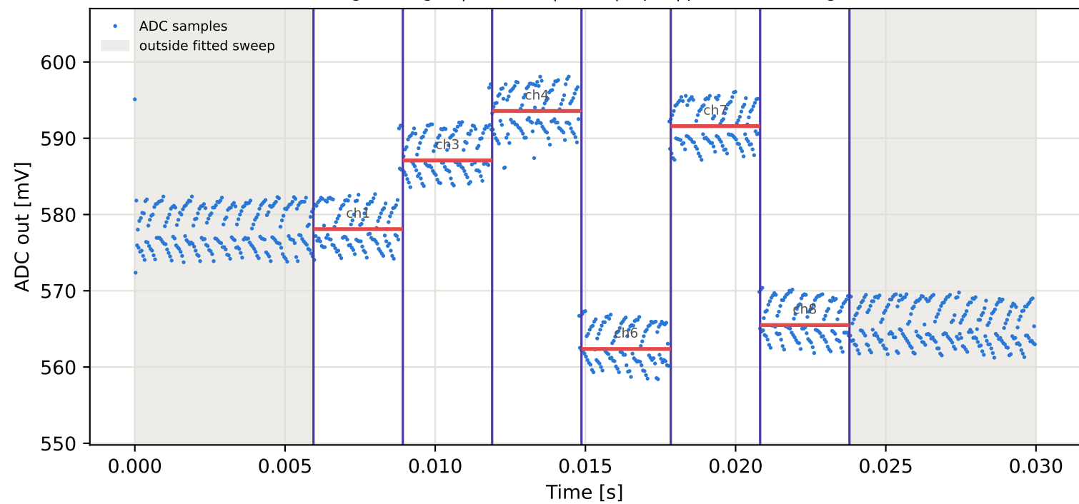
Tag5 &lt;- Tag2 | 945 MHz | run 0 | rep 1 | phase 22.73 deg
