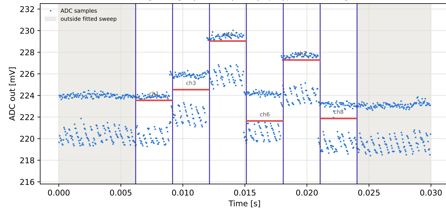
Tag6 &lt;- Tag2 | 995 MHz | run 0 | rep 1 | phase -38.91 deg
