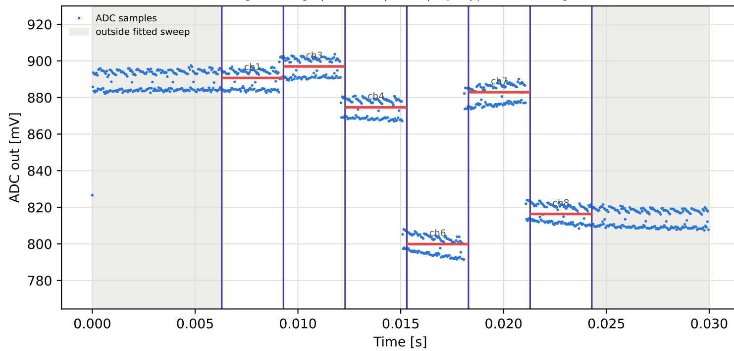
Tag10 &lt;- Tag8 | 885 MHz | run 0 | rep 1 | phase -81.70 deg
