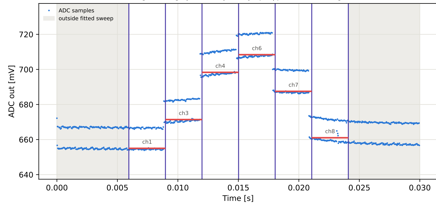
Tag15 &lt;- Tag4 | 925 MHz | run 0 | rep 1 | phase -148.14 deg
