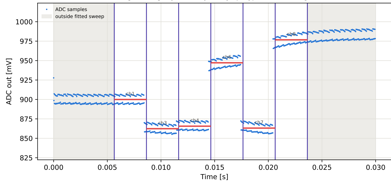
Tag10 &lt;- Tag3 | 895 MHz | run 0 | rep 1 | phase 163.07 deg
