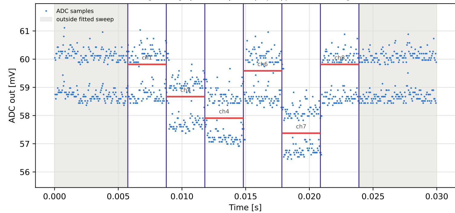
Tag9 &lt;- Tag6 | 795 MHz | run 0 | rep 1 | phase -134.63 deg
