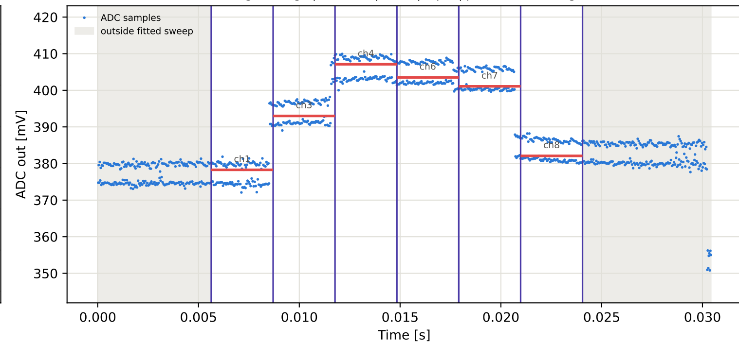
Tag9 &lt;- Tag6 | 875 MHz | run 0 | rep 1 | phase 21.89 deg
