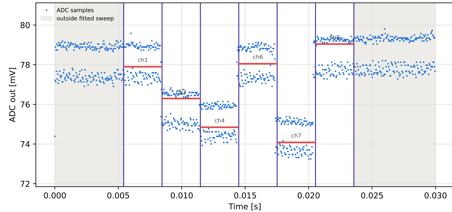
Tag1 &lt;- Tag3 | 795 MHz | run 0 | rep 1 | phase 137.01 deg
