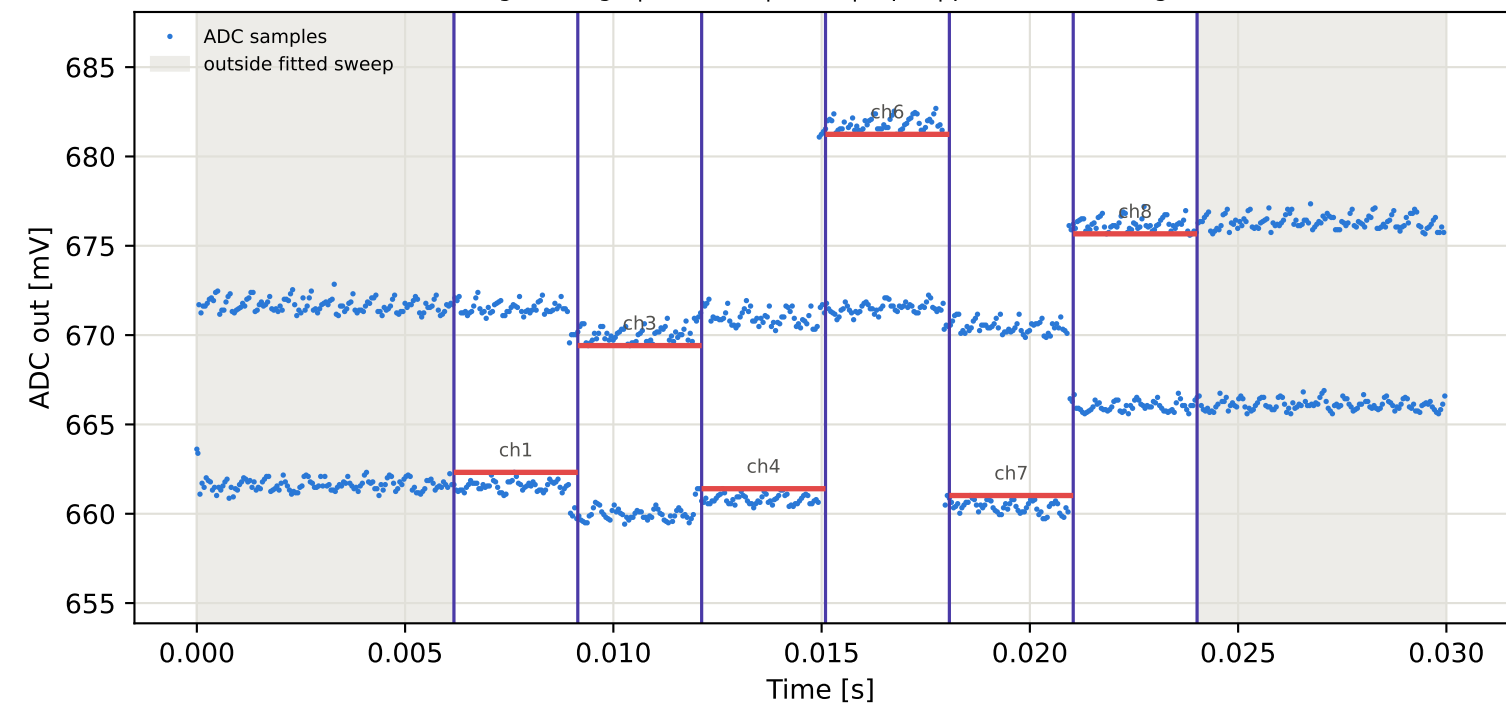
Tag7 &lt;- Tag4 | 845 MHz | run 0 | rep 1 | phase -77.48 deg
