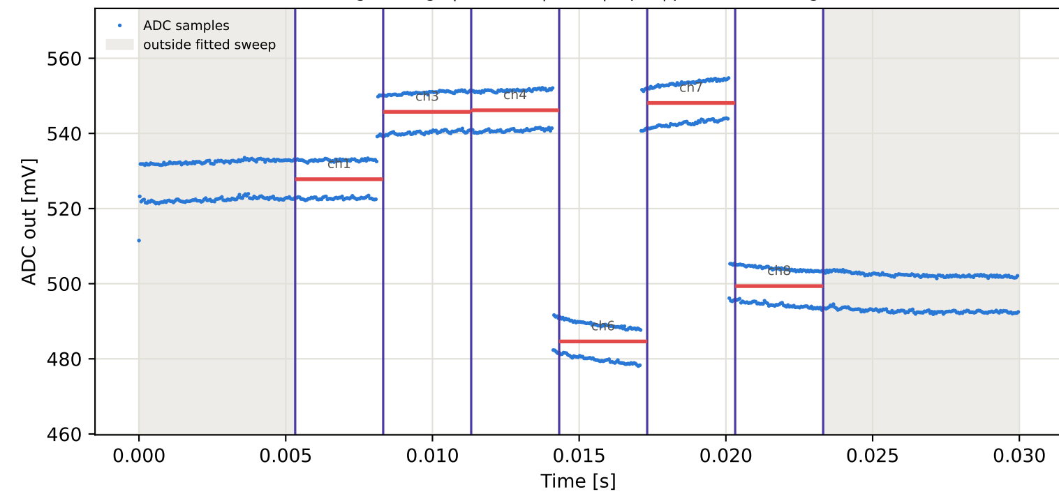
Tag9 &lt;- Tag10 | 935 MHz | run 0 | rep 1 | phase 172.36 deg
