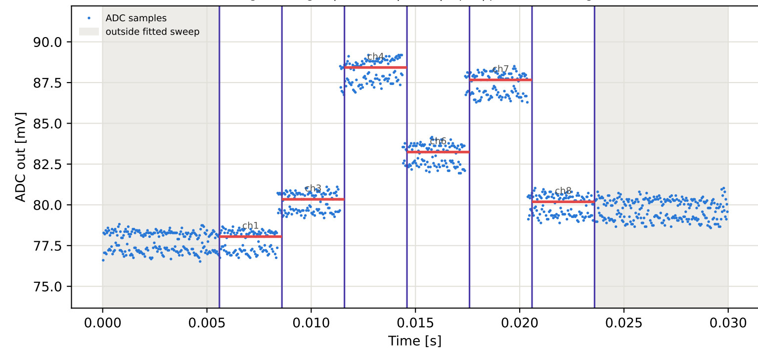
Tag15 &lt;- Tag3 | 795 MHz | run 0 | rep 1 | phase 125.66 deg
