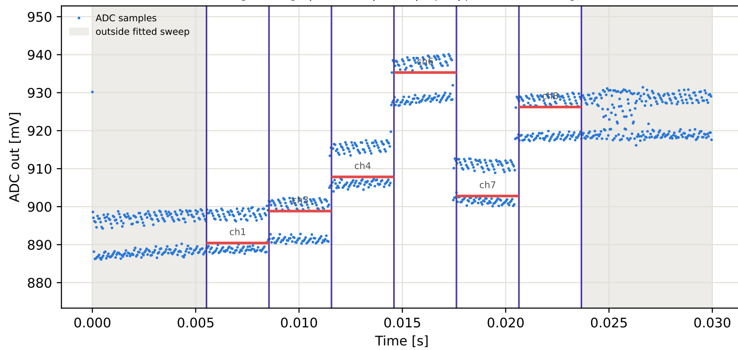
Tag3 &lt;- Tag6 | 875 MHz | run 0 | rep 1 | phase -102.11 deg
