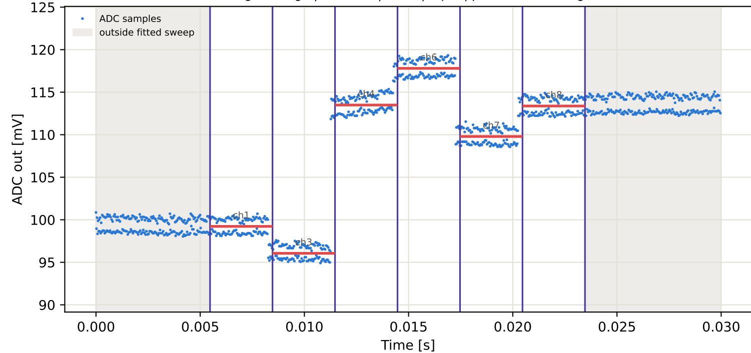
Tag4 &lt;- Tag3 | 835 MHz | run 0 | rep 1 | phase -137.15 deg
