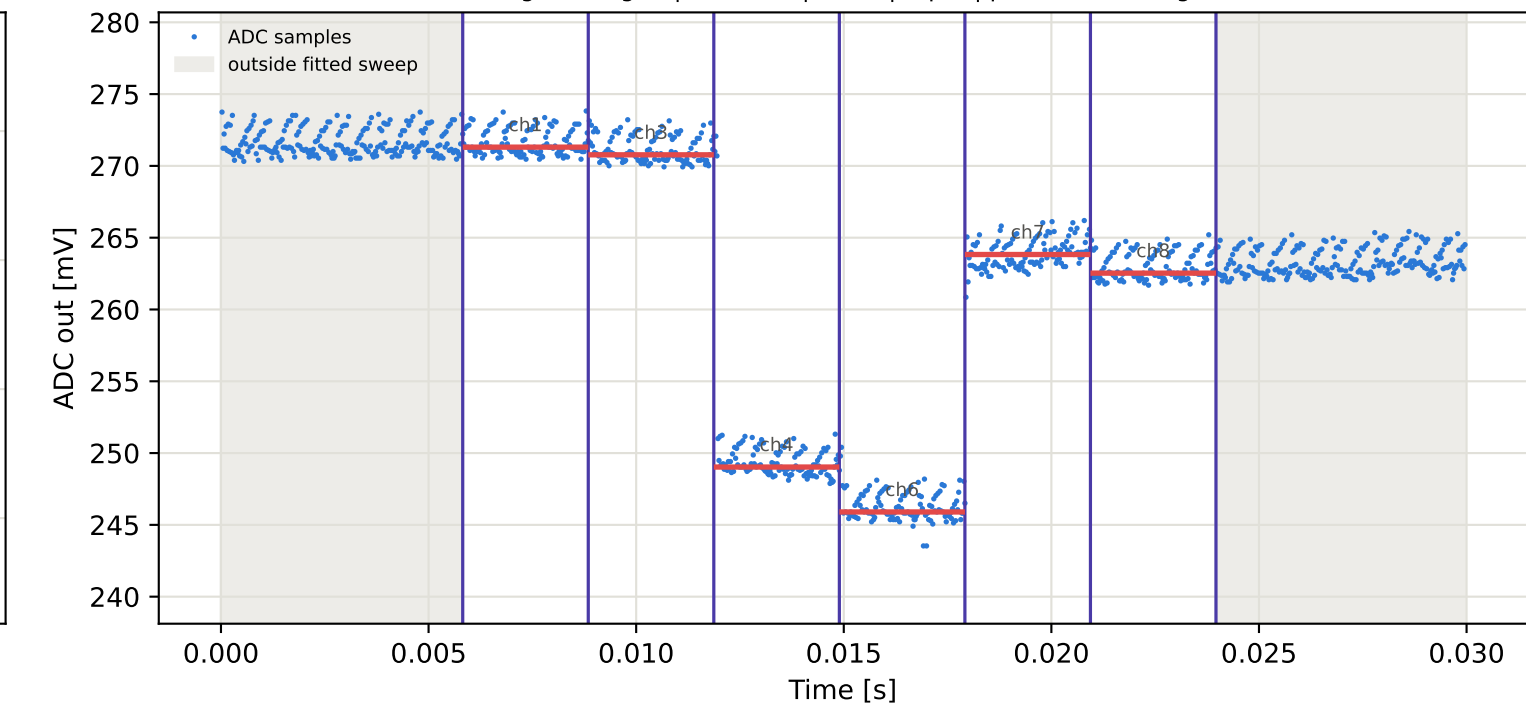
Tag8 &lt;- Tag16 | 975 MHz | run 0 | rep 1 | phase -128.39 deg
