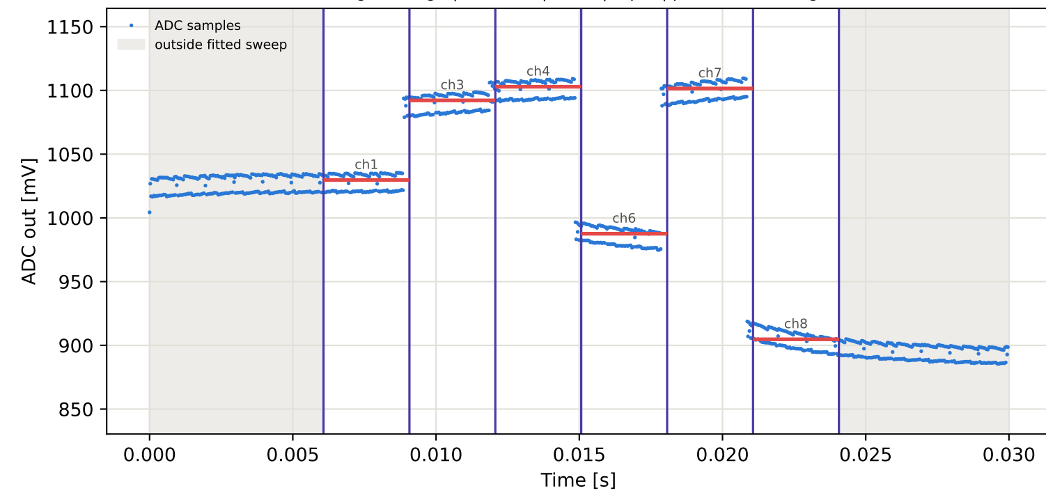
Tag8 &lt;- Tag1 | 895 MHz | run 0 | rep 1 | phase -52.57 deg
