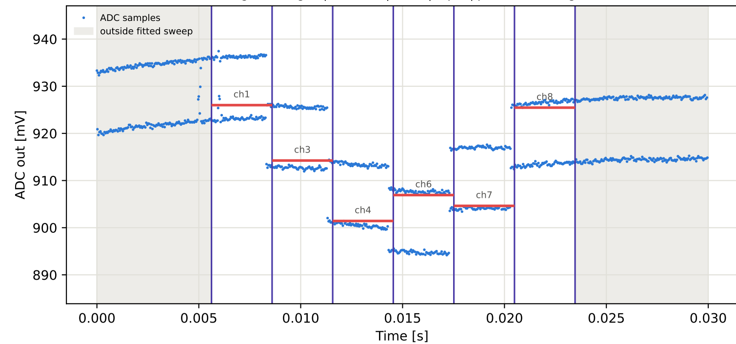
Tag10 &lt;- Tag2 | 895 MHz | run 0 | rep 1 | phase -159.58 deg
