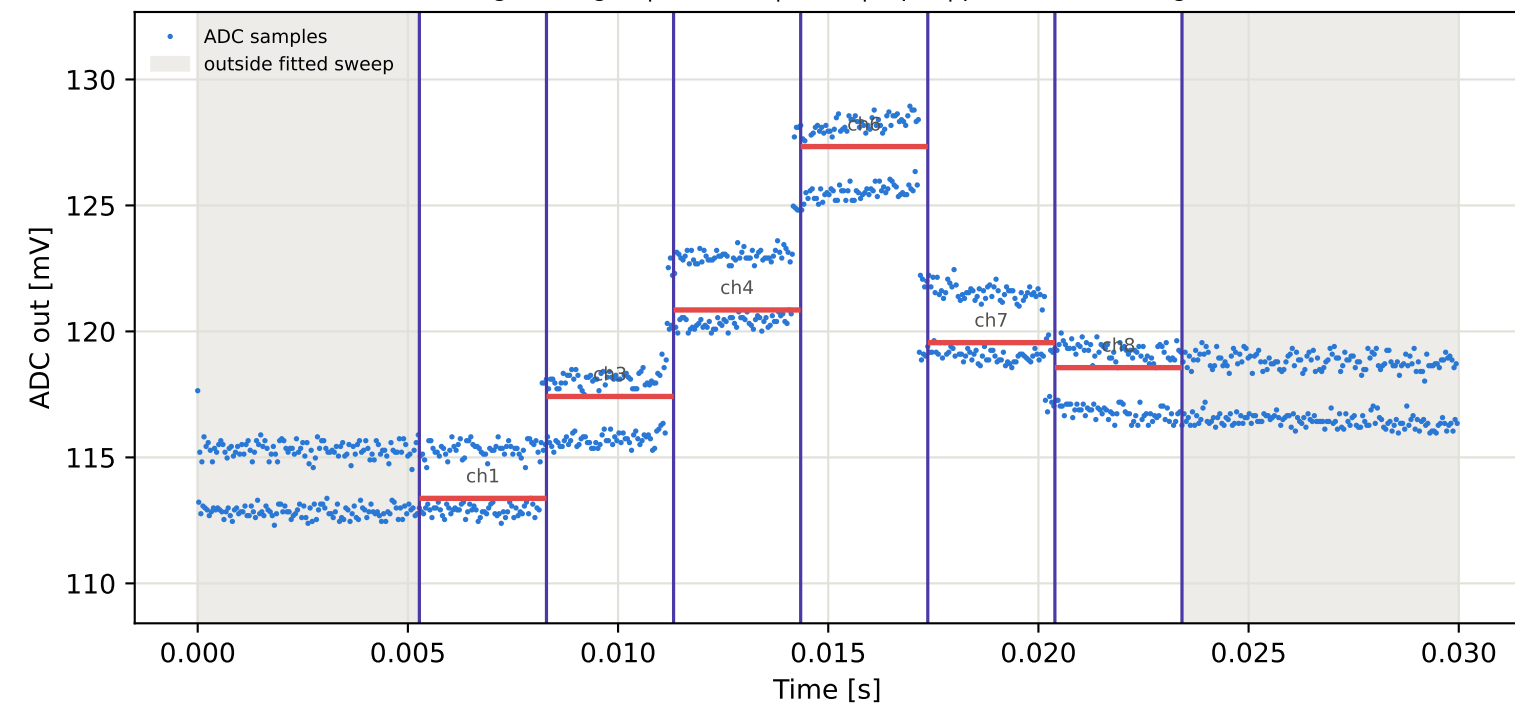
Tag4 &lt;- Tag16 | 895 MHz | run 0 | rep 1 | phase -95.21 deg
