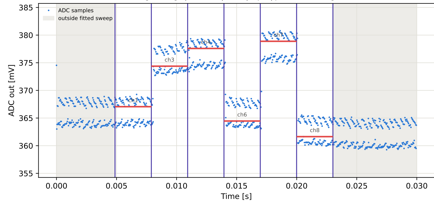
Tag5 &lt;- Tag9 | 855 MHz | run 0 | rep 1 | phase -113.04 deg
