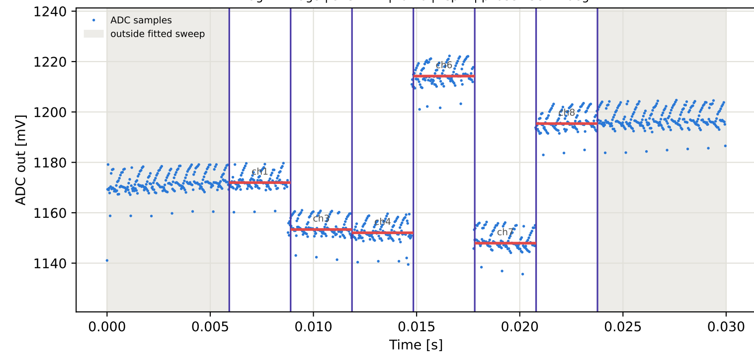
Tag8 &lt;- Tag1 | 975 MHz | run 0 | rep 1 | phase 95.32 deg
