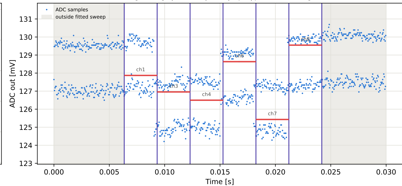
Tag2 &lt;- Tag6 | 845 MHz | run 0 | rep 1 | phase -51.54 deg
