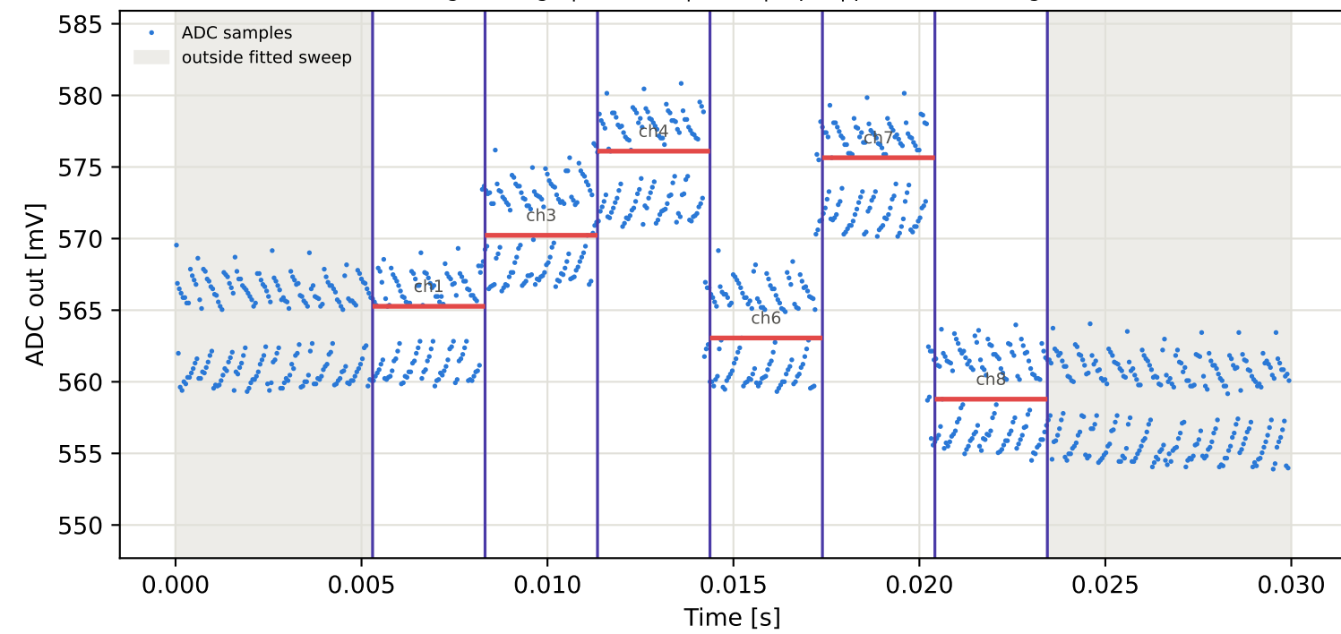
Tag8 &lt;- Tag10 | 915 MHz | run 0 | rep 1 | phase -69.56 deg
