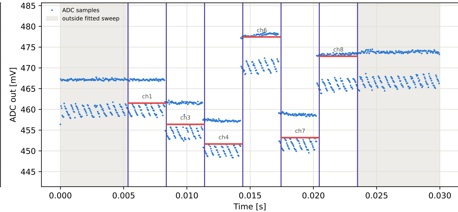
Tag15 &lt;- Tag6 | 975 MHz | run 0 | rep 1 | phase 18.25 deg
