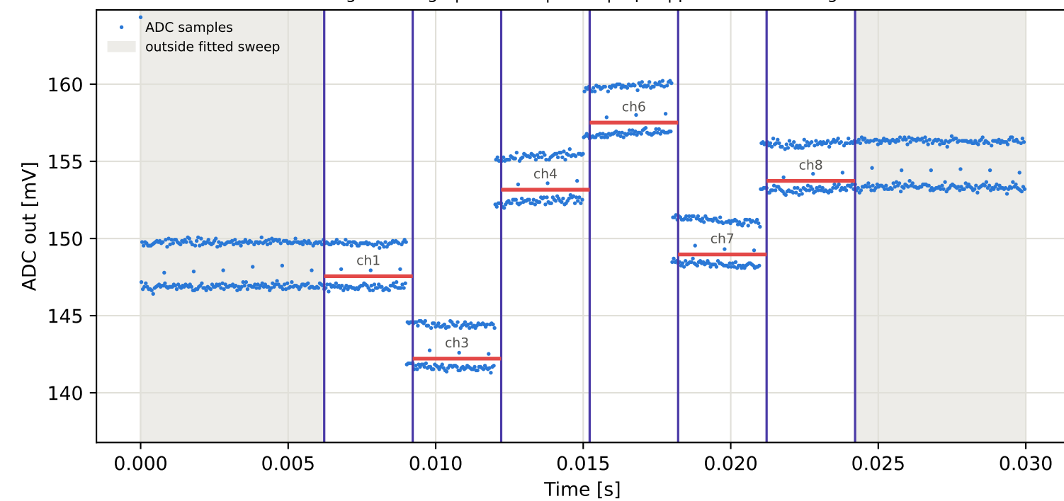
Tag10 &lt;- Tag8 | 805 MHz | run 0 | rep 1 | phase 162.13 deg
