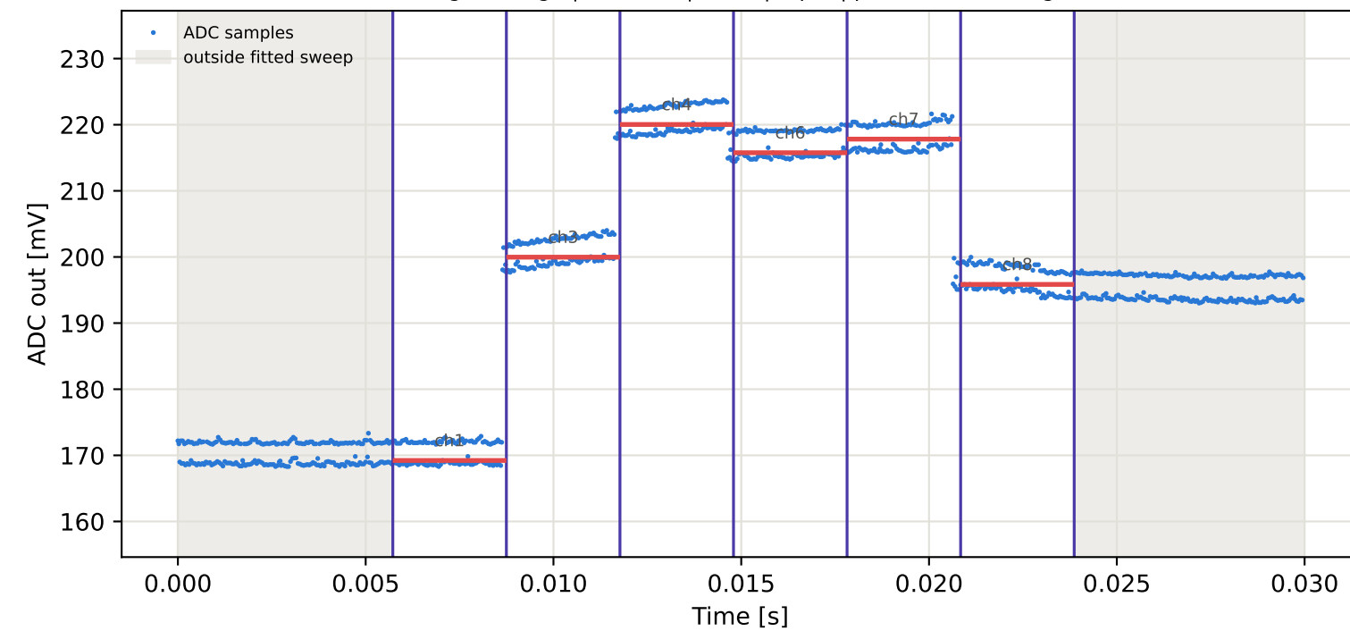
Tag9 &lt;- Tag5 | 855 MHz | run 0 | rep 1 | phase -132.59 deg
