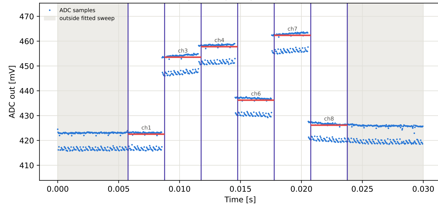
Tag3 &lt;- Tag8 | 825 MHz | run 0 | rep 1 | phase -61.66 deg
