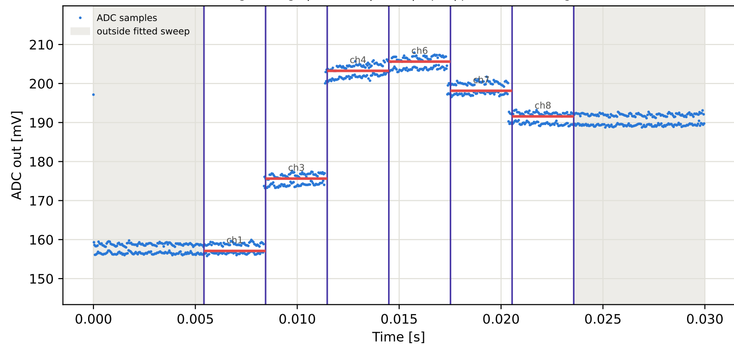
Tag9 &lt;- Tag5 | 845 MHz | run 0 | rep 1 | phase -137.16 deg
