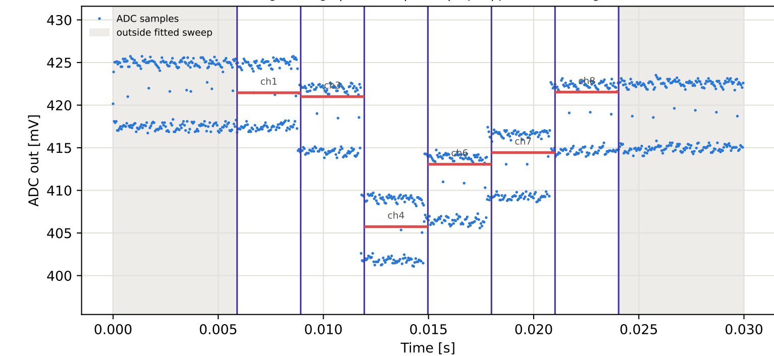
Tag6 &lt;- Tag1 | 965 MHz | run 0 | rep 1 | phase -156.55 deg
