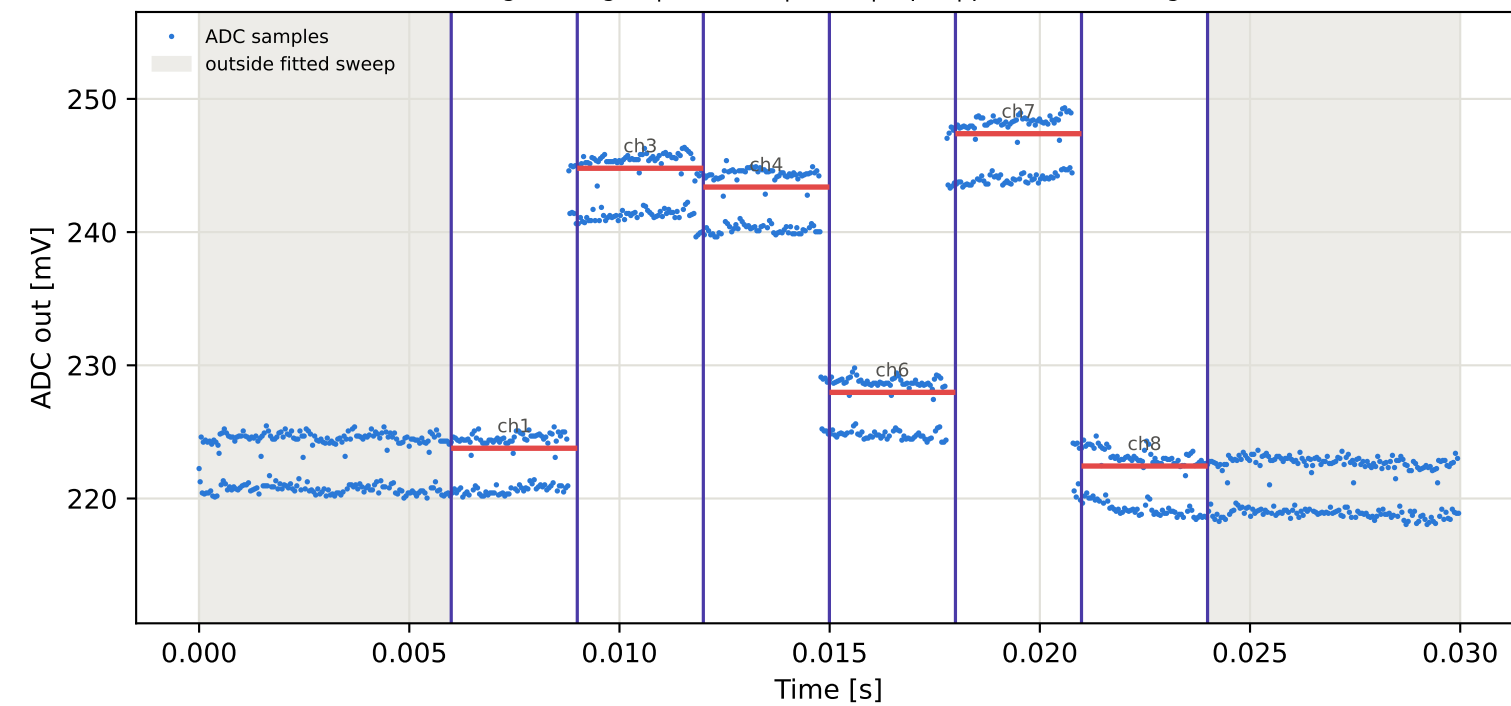
Tag5 &lt;- Tag16 | 825 MHz | run 0 | rep 1 | phase -129.68 deg
