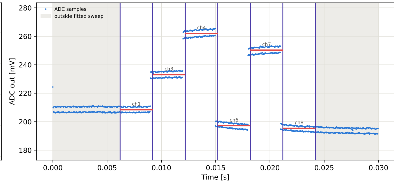
Tag8 &lt;- Tag16 | 995 MHz | run 0 | rep 1 | phase -68.46 deg
