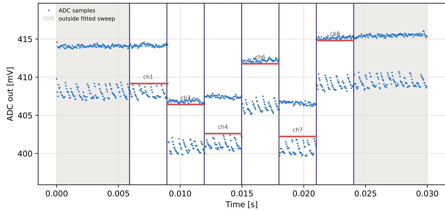
Tag6 &lt;- Tag4 | 845 MHz | run 0 | rep 1 | phase 131.50 deg
