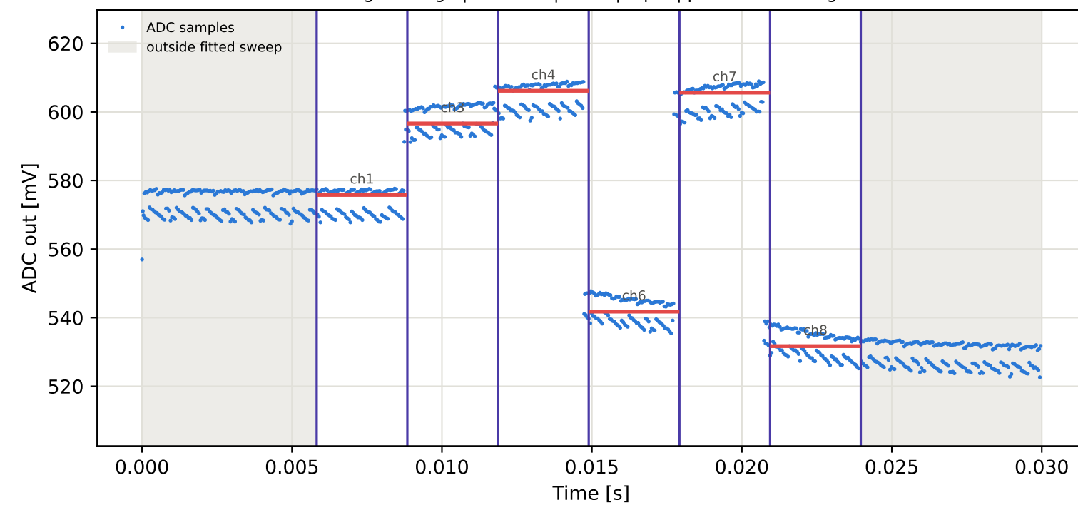
Tag9 &lt;- Tag5 | 905 MHz | run 0 | rep 1 | phase 19.76 deg
