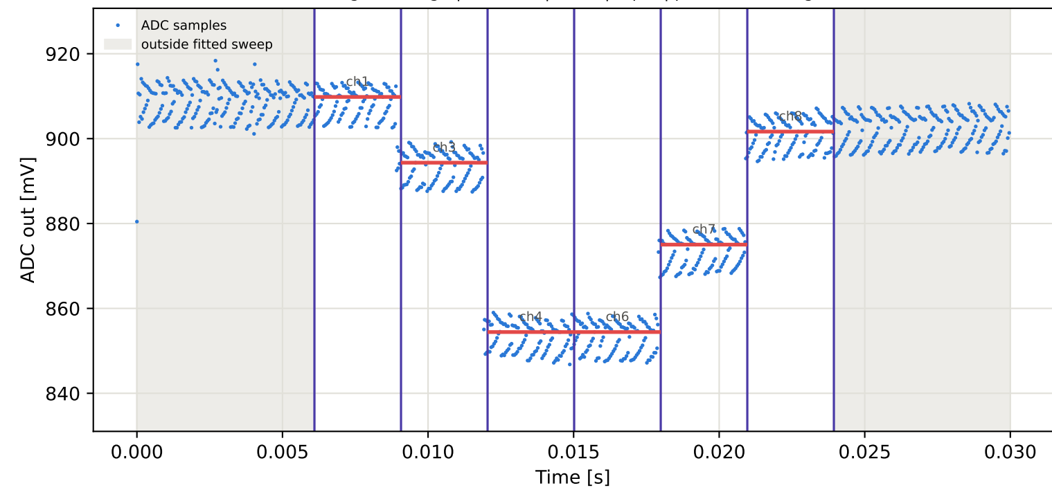
Tag16 &lt;- Tag5 | 945 MHz | run 0 | rep 1 | phase 115.17 deg
