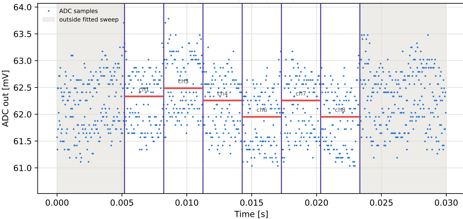
Tag15 &lt;- Tag1 | 785 MHz | run 0 | rep 1 | phase 19.04 deg
