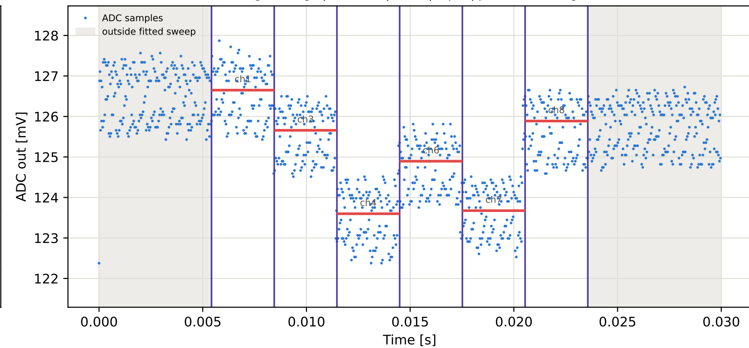
Tag8 &lt;- Tag10 | 795 MHz | run 0 | rep 1 | phase 101.64 deg
