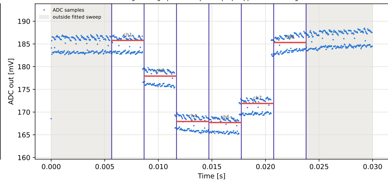
Tag7 &lt;- Tag6 | 905 MHz | run 0 | rep 1 | phase 62.81 deg
