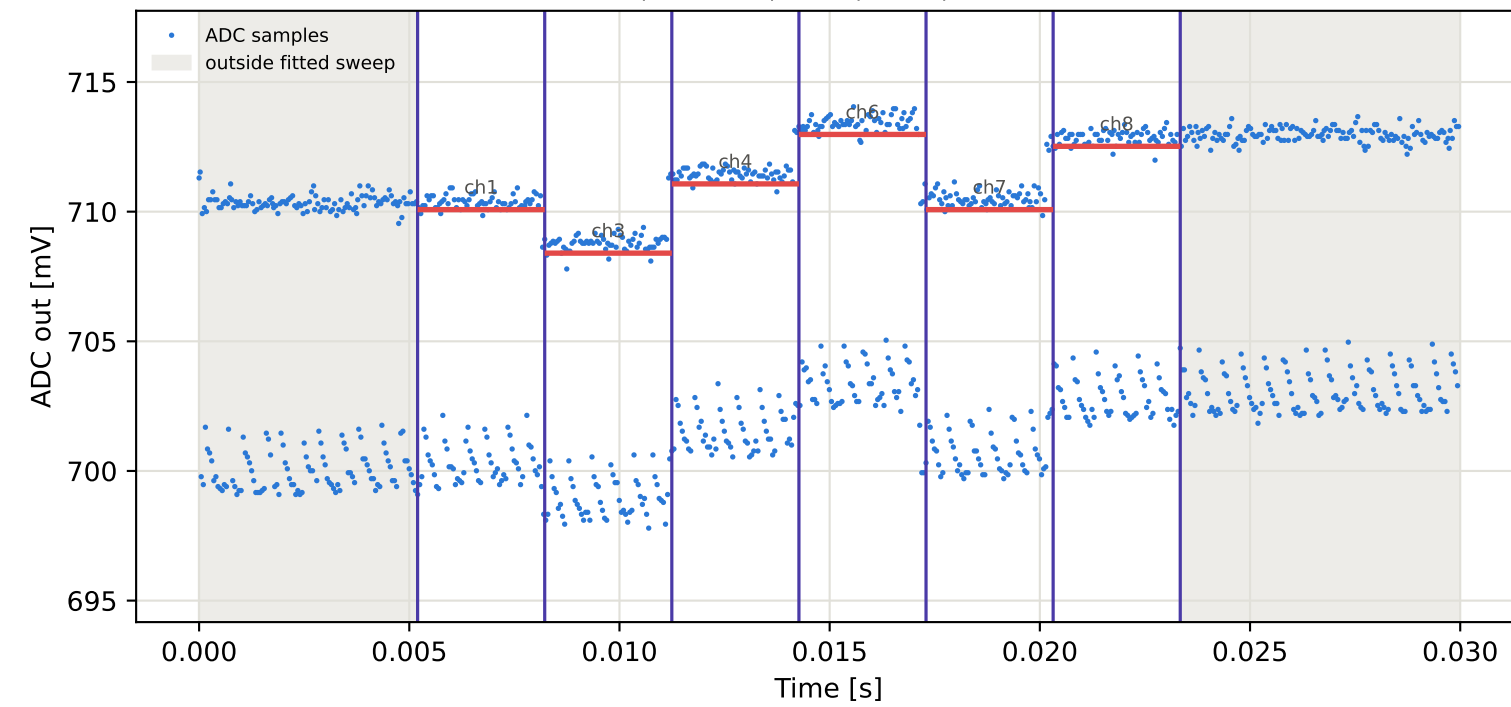
Tag8 &lt;- Tag6 | 845 MHz | run 0 | rep 1 | phase -159.61 deg
