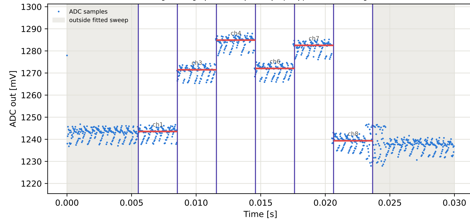
Tag8 &lt;- Tag6 | 875 MHz | run 0 | rep 1 | phase -91.09 deg
