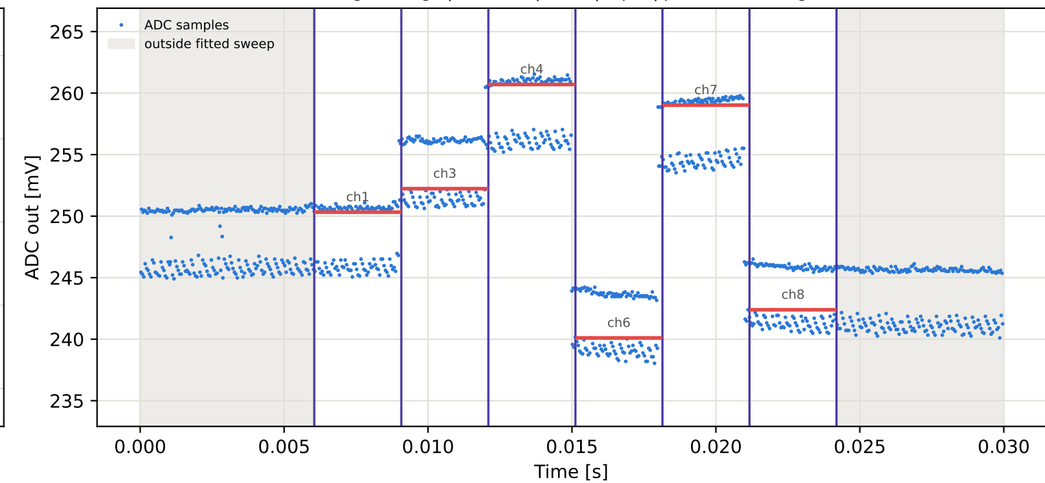
Tag1 &lt;- Tag8 | 965 MHz | run 0 | rep 1 | phase -46.52 deg
