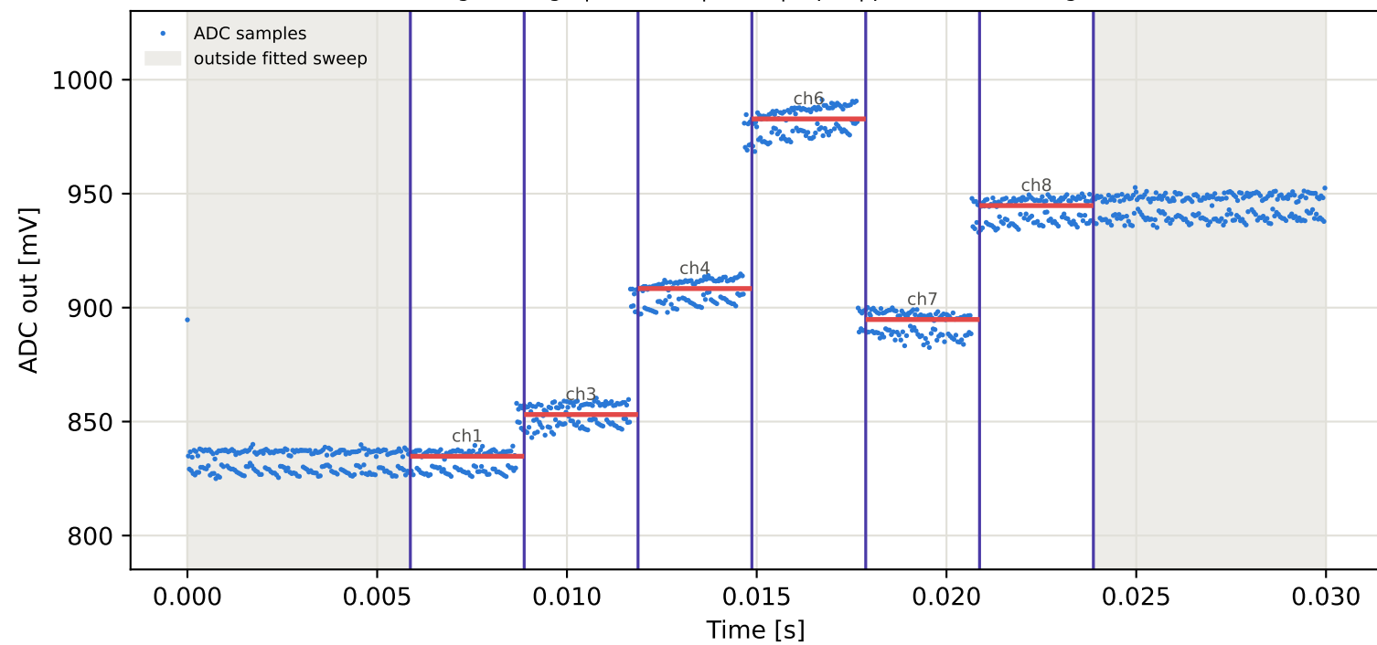
Tag7 &lt;- Tag1 | 885 MHz | run 0 | rep 1 | phase -93.21 deg
