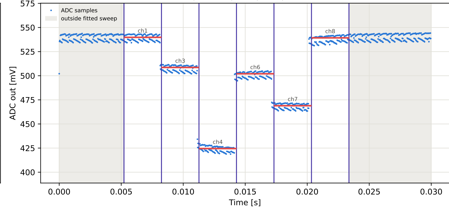
Tag8 &lt;- Tag7 | 965 MHz | run 0 | rep 1 | phase 75.01 deg
