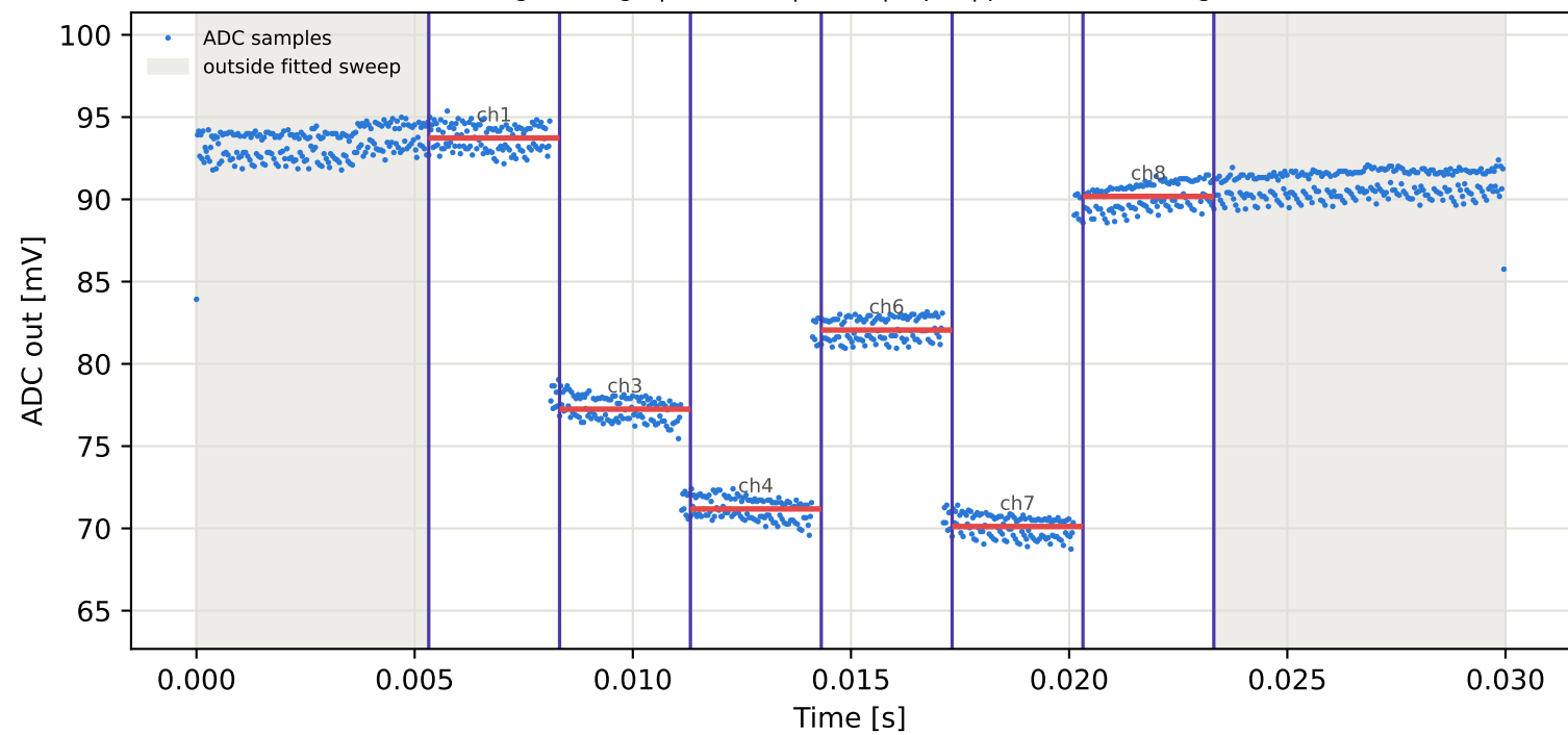
Tag1 &lt;- Tag8 | 845 MHz | run 0 | rep 1 | phase -173.14 deg
