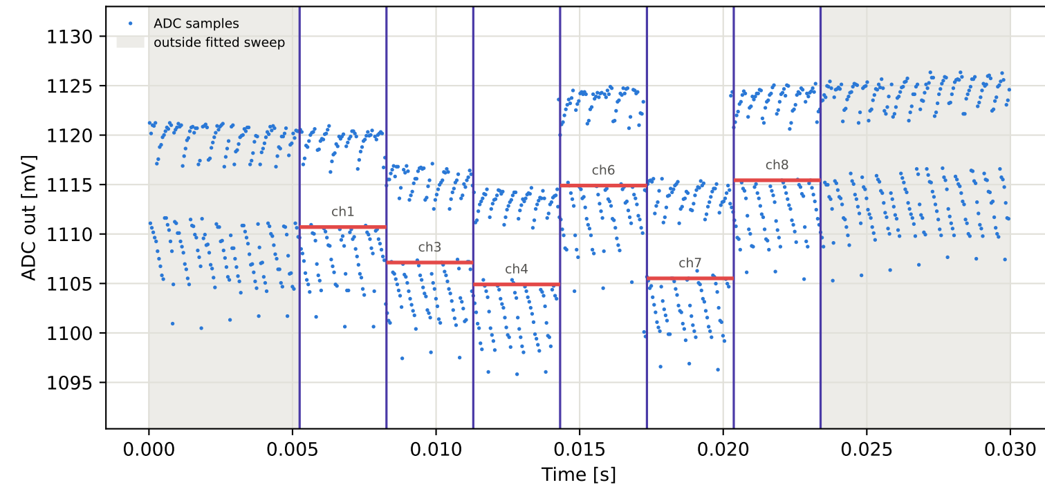
Tag8 &lt;- Tag6 | 925 MHz | run 0 | rep 1 | phase 73.04 deg
