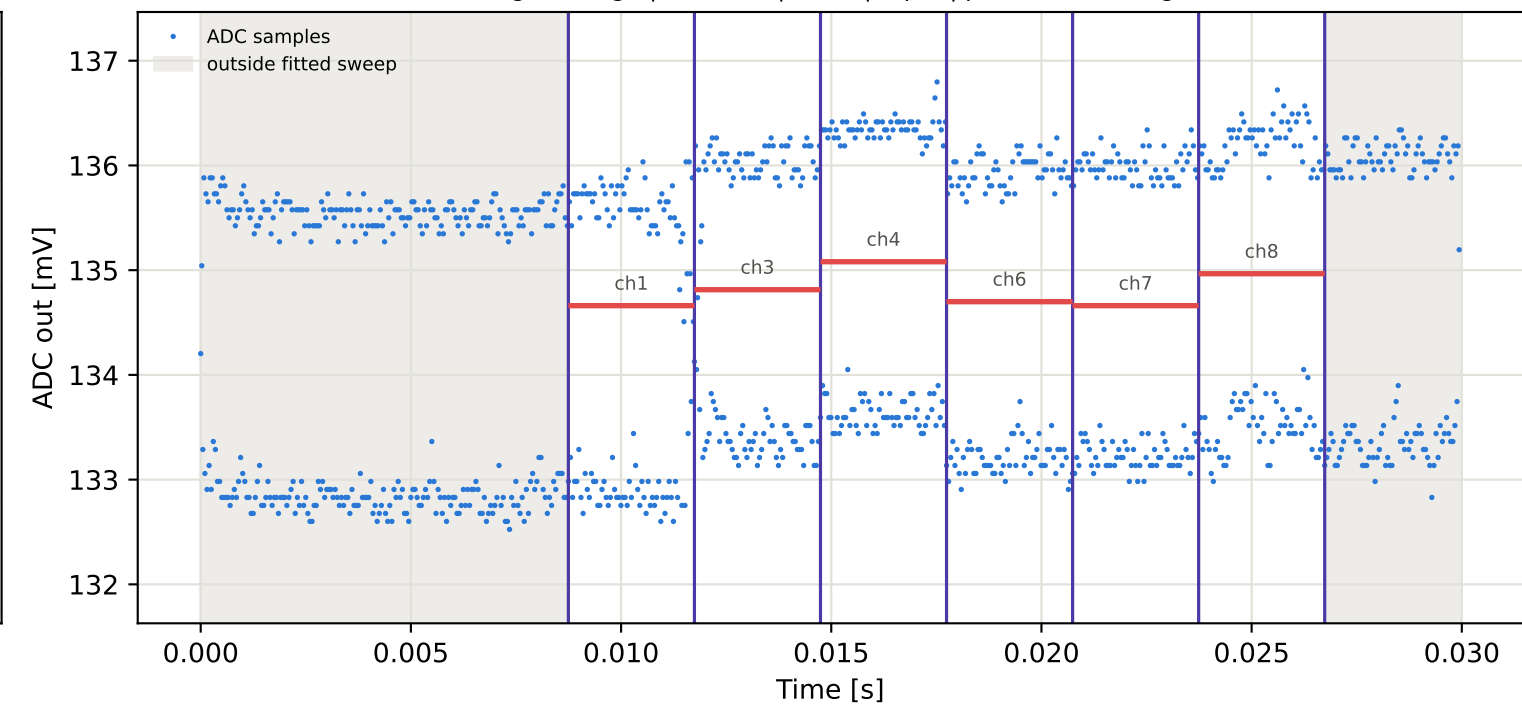
Tag7 &lt;- Tag4 | 775 MHz | run 0 | rep 1 | phase 157.44 deg
