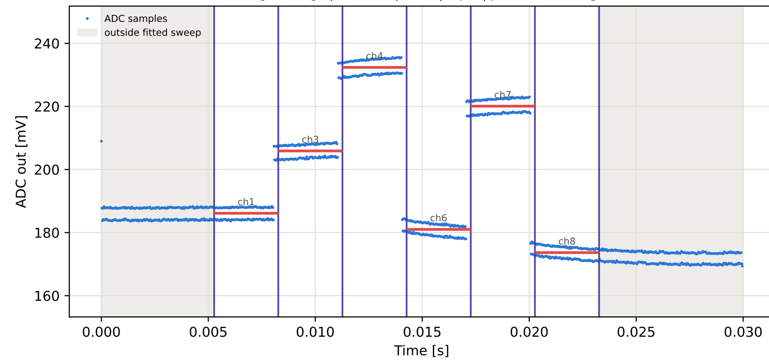
Tag4 &lt;- Tag7 | 955 MHz | run 0 | rep 1 | phase -2.71 deg
