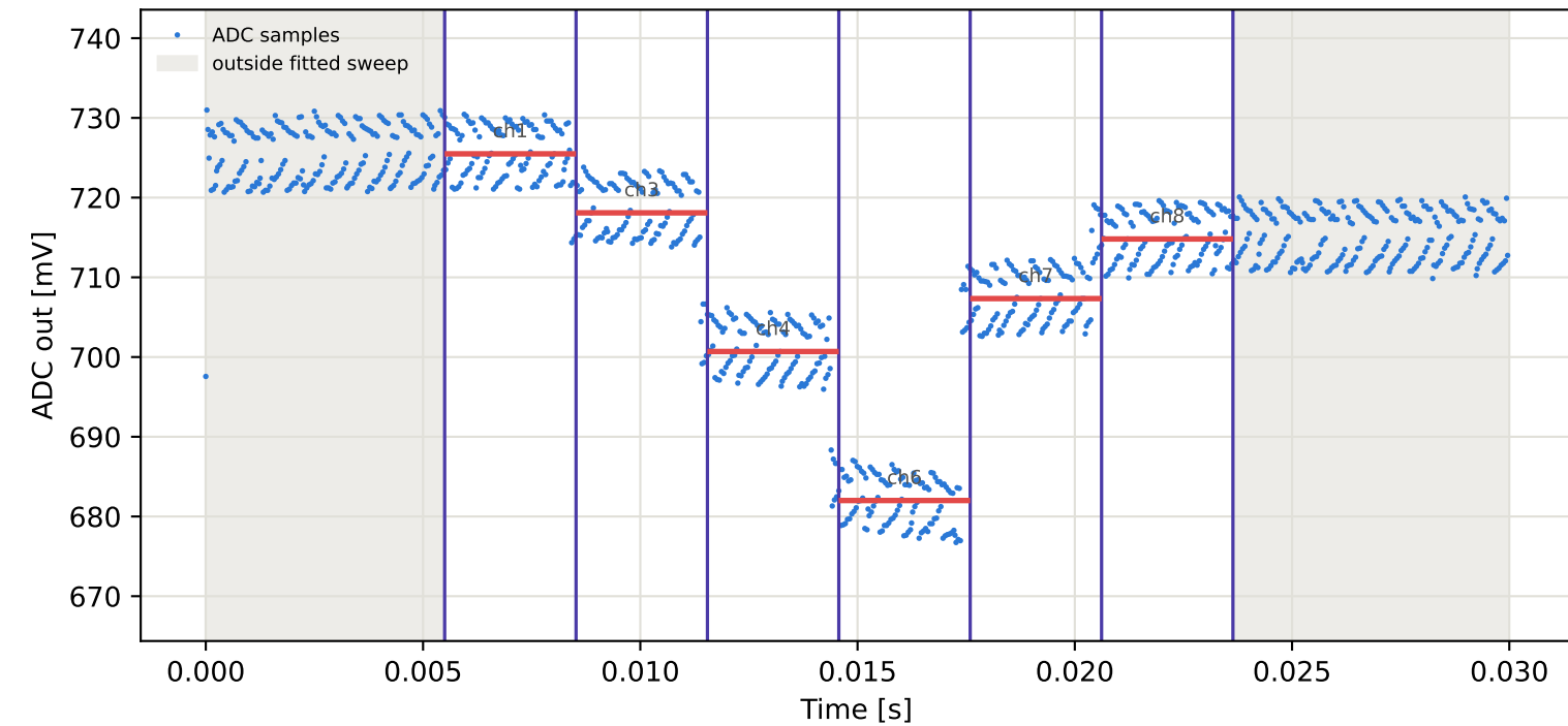
Tag9 &lt;- Tag7 | 915 MHz | run 0 | rep 1 | phase 48.89 deg
