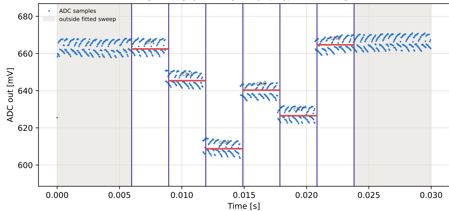
Tag10 &lt;- Tag8 | 945 MHz | run 0 | rep 1 | phase -87.67 deg
