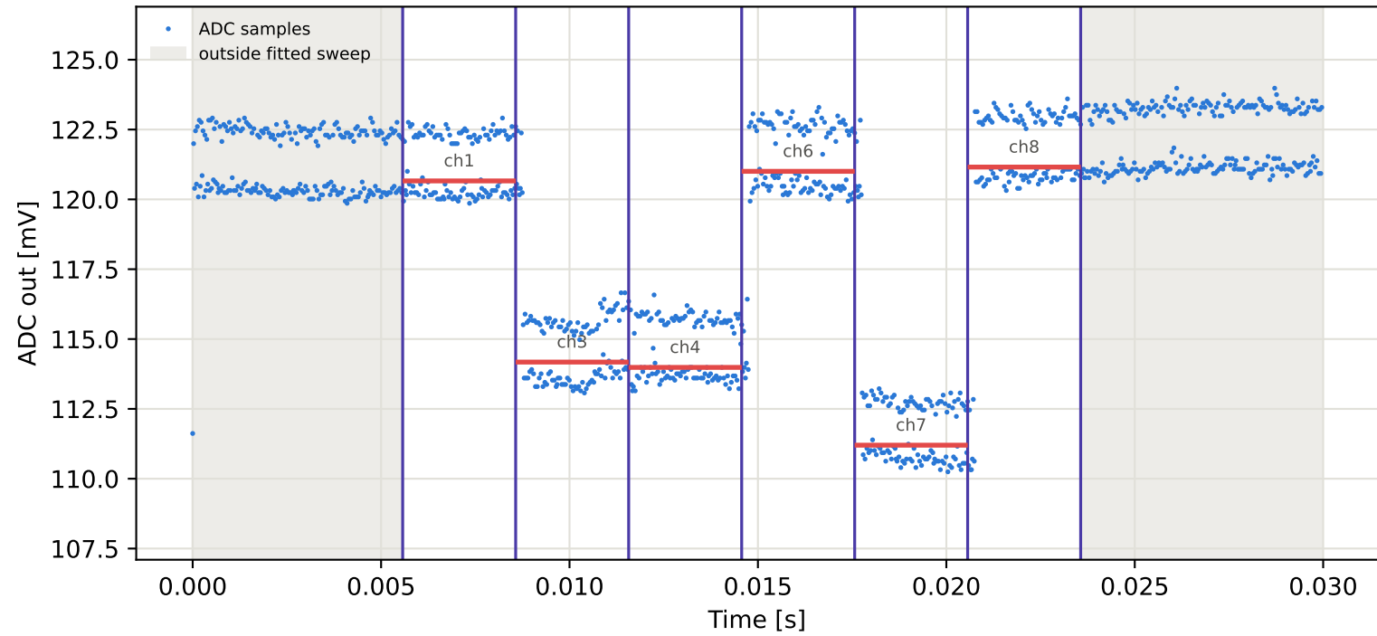
Tag6 &lt;- Tag1 | 795 MHz | run 0 | rep 1 | phase -168.62 deg
