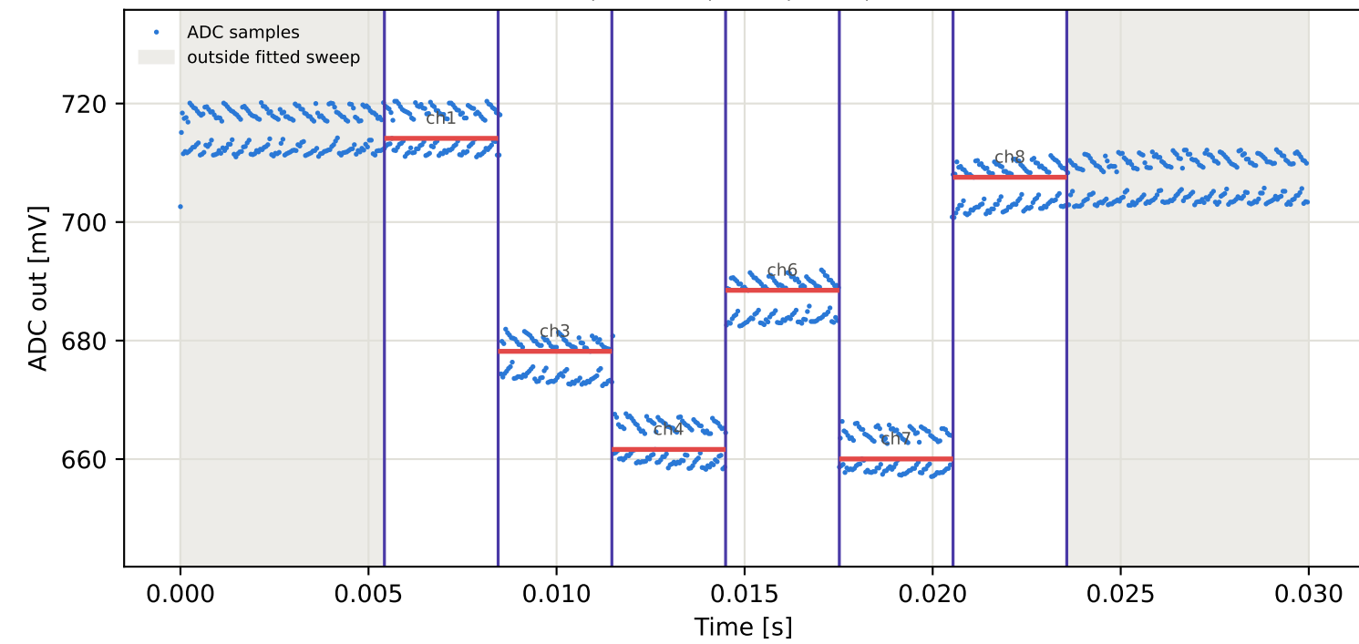
Tag16 &lt;- Tag15 | 855 MHz | run 0 | rep 1 | phase 102.47 deg
