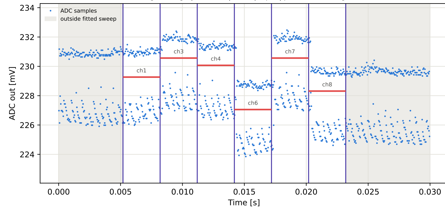
Tag3 &lt;- Tag10 | 985 MHz | run 0 | rep 1 | phase -50.22 deg
