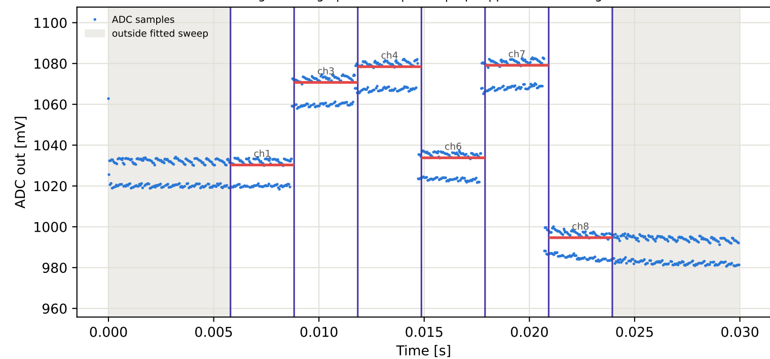
Tag16 &lt;- Tag5 | 875 MHz | run 0 | rep 1 | phase -54.43 deg
