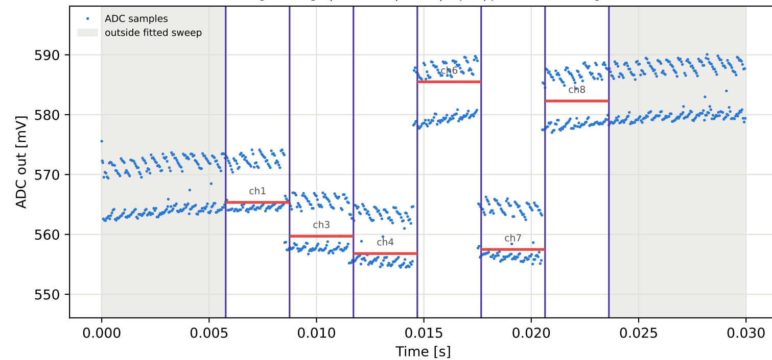
Tag5 &lt;- Tag8 | 905 MHz | run 0 | rep 1 | phase -70.77 deg
