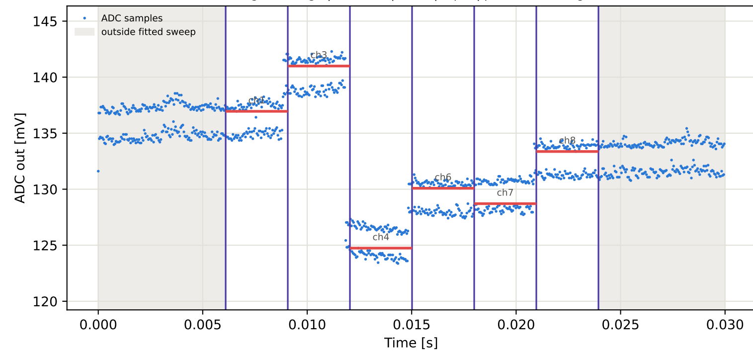
Tag16 &lt;- Tag5 | 785 MHz | run 0 | rep 1 | phase 97.81 deg
