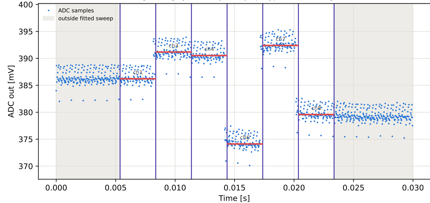
Tag3 &lt;- Tag15 | 975 MHz | run 0 | rep 1 | phase 93.49 deg
