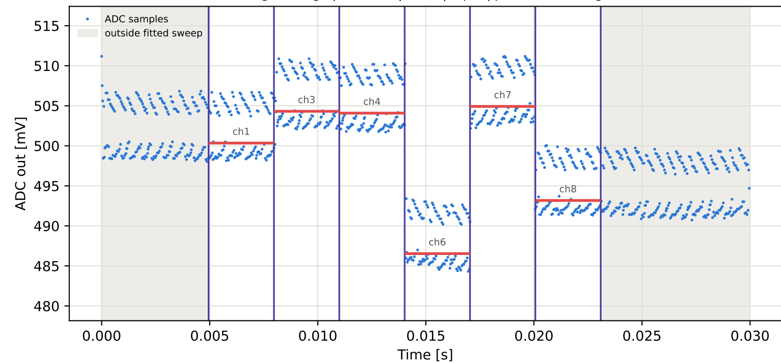
Tag8 &lt;- Tag7 | 955 MHz | run 0 | rep 1 | phase 44.09 deg
