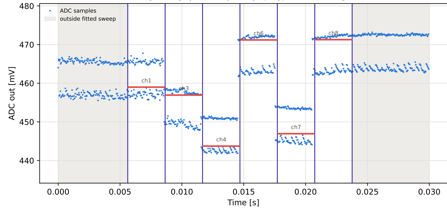
Tag5 &lt;- Tag9 | 935 MHz | run 0 | rep 1 | phase 141.81 deg
