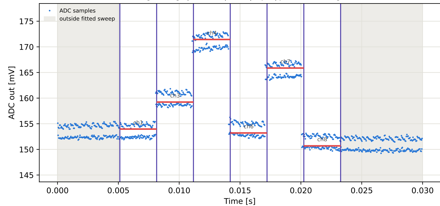
Tag4 &lt;- Tag8 | 975 MHz | run 0 | rep 1 | phase -88.46 deg
