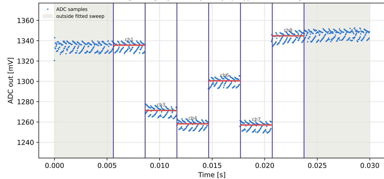
Tag7 &lt;- Tag3 | 875 MHz | run 0 | rep 1 | phase 57.87 deg
