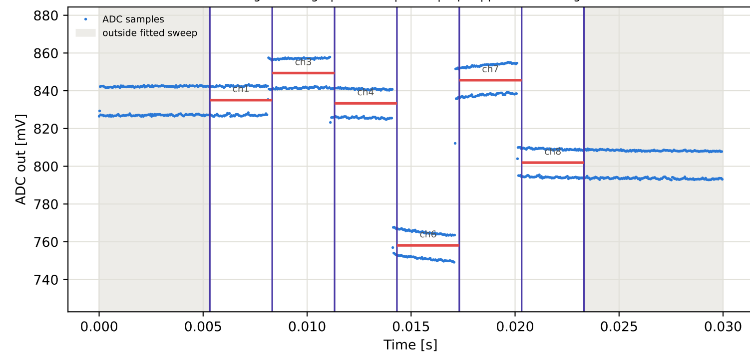
Tag2 &lt;- Tag1 | 955 MHz | run 0 | rep 1 | phase -87.61 deg
