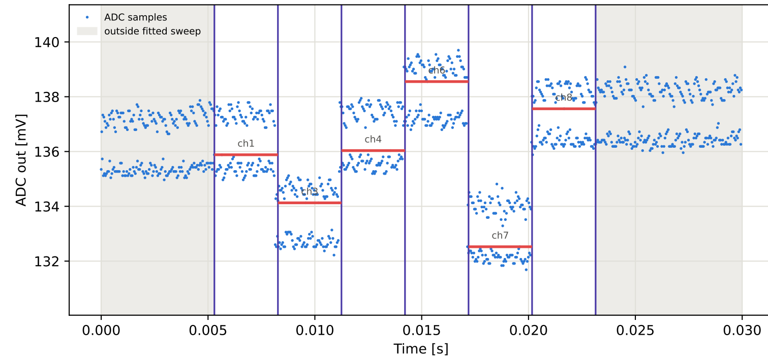
Tag7 &lt;- Tag5 | 775 MHz | run 0 | rep 1 | phase -63.26 deg
