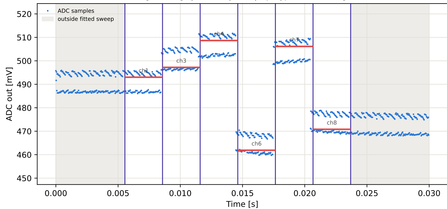
Tag15 &lt;- Tag4 | 945 MHz | run 0 | rep 1 | phase 9.62 deg
