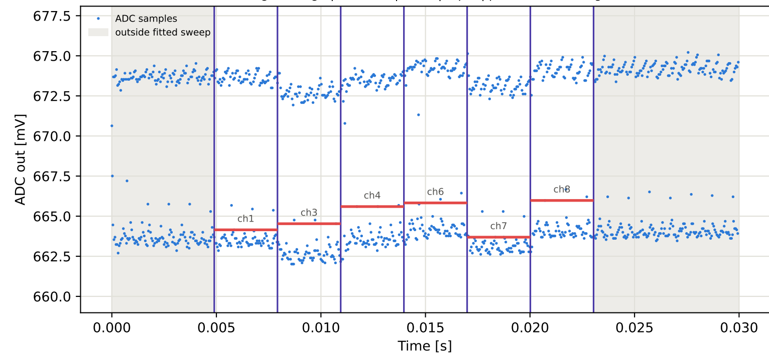
Tag7 &lt;- Tag15 | 845 MHz | run 0 | rep 1 | phase -76.34 deg
