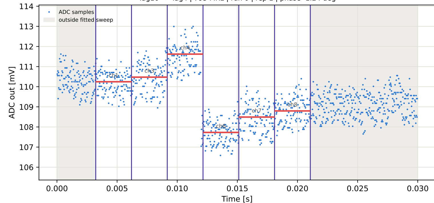
Tag16 &lt;- Tag6 | 795 MHz | run 0 | rep 1 | phase -3.41 deg
