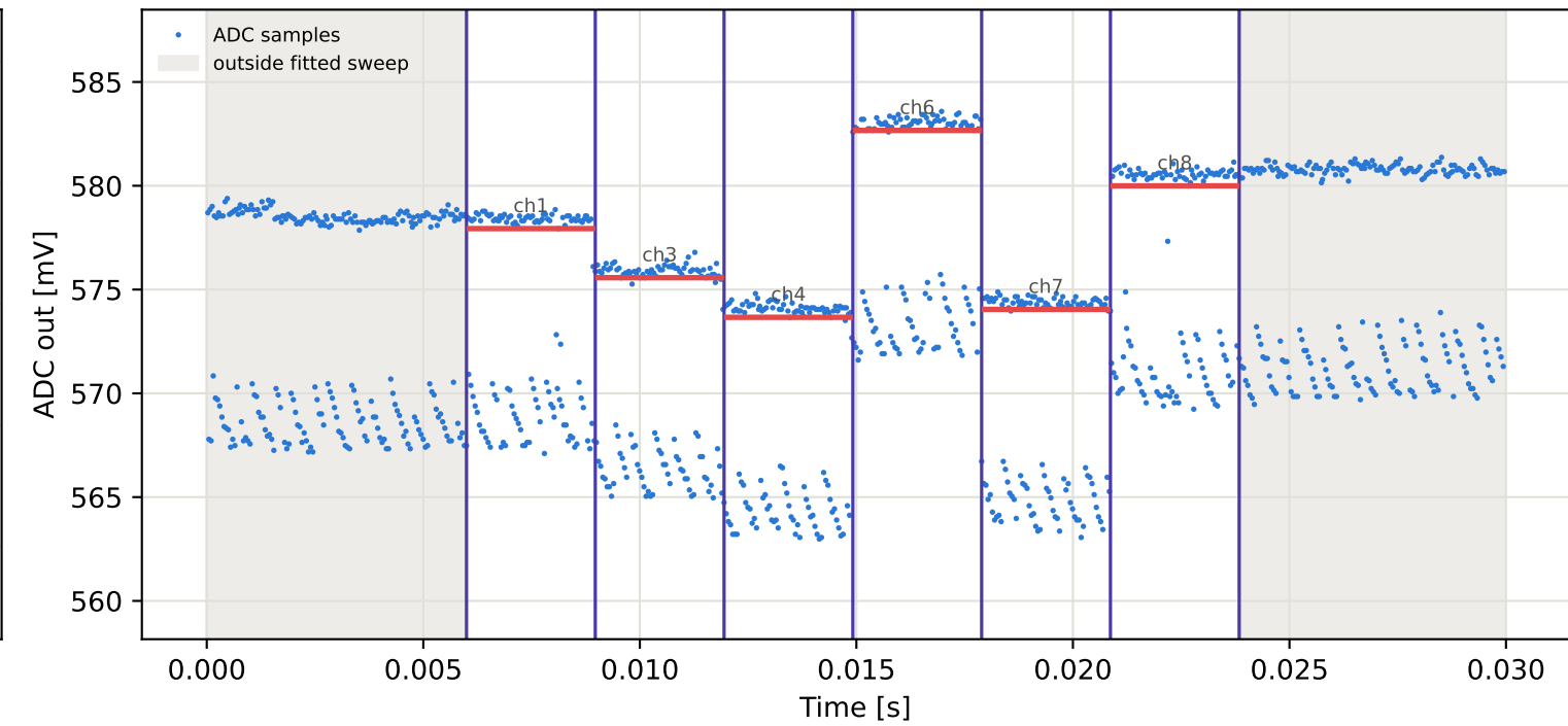
Tag15 &lt;- Tag6 | 985 MHz | run 0 | rep 1 | phase 94.61 deg
