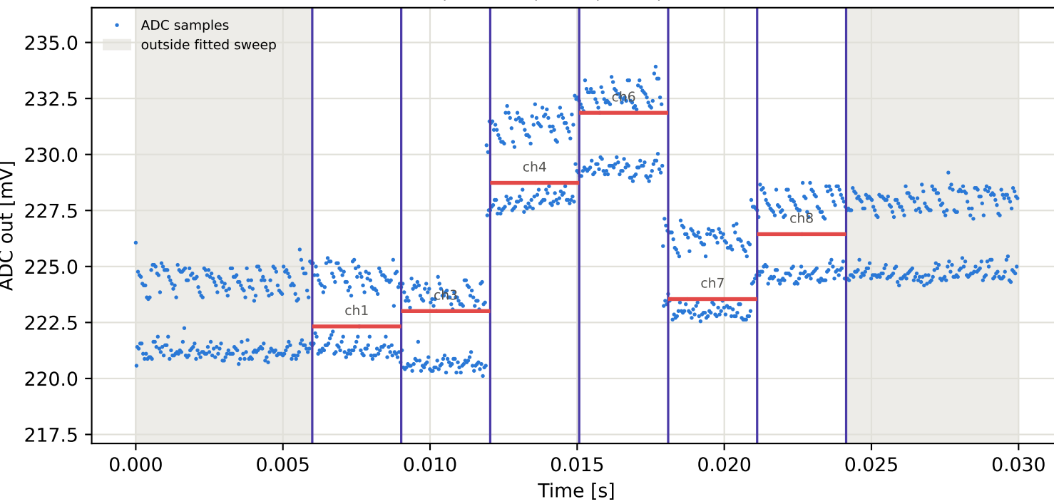
Tag6 &lt;- Tag1 | 995 MHz | run 0 | rep 1 | phase -154.19 deg
