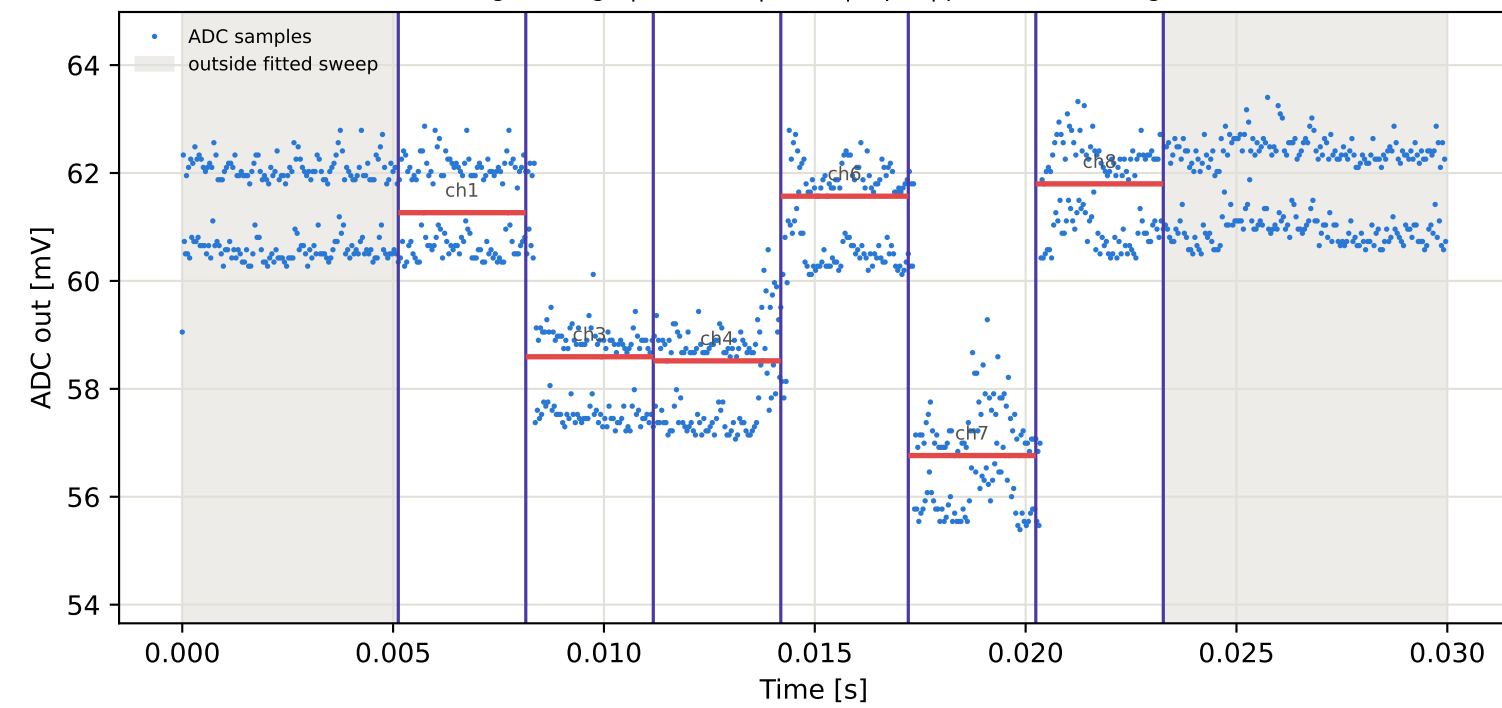
Tag9 &lt;- Tag5 | 795 MHz | run 0 | rep 1 | phase 171.86 deg
