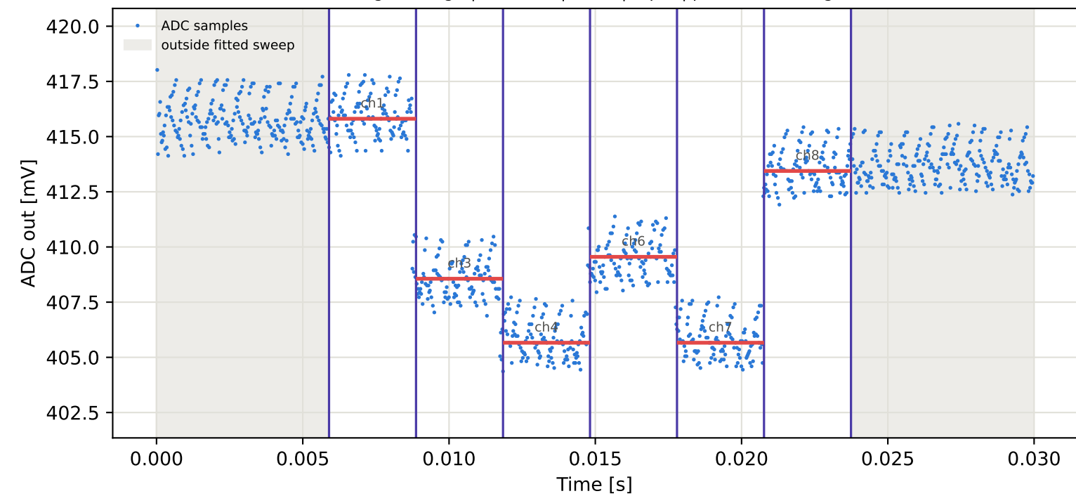
Tag7 &lt;- Tag1 | 845 MHz | run 0 | rep 1 | phase -158.33 deg
