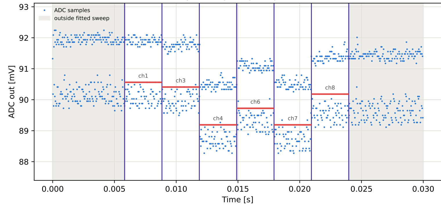
Tag1 &lt;- Tag4 | 805 MHz | run 0 | rep 1 | phase 81.39 deg
