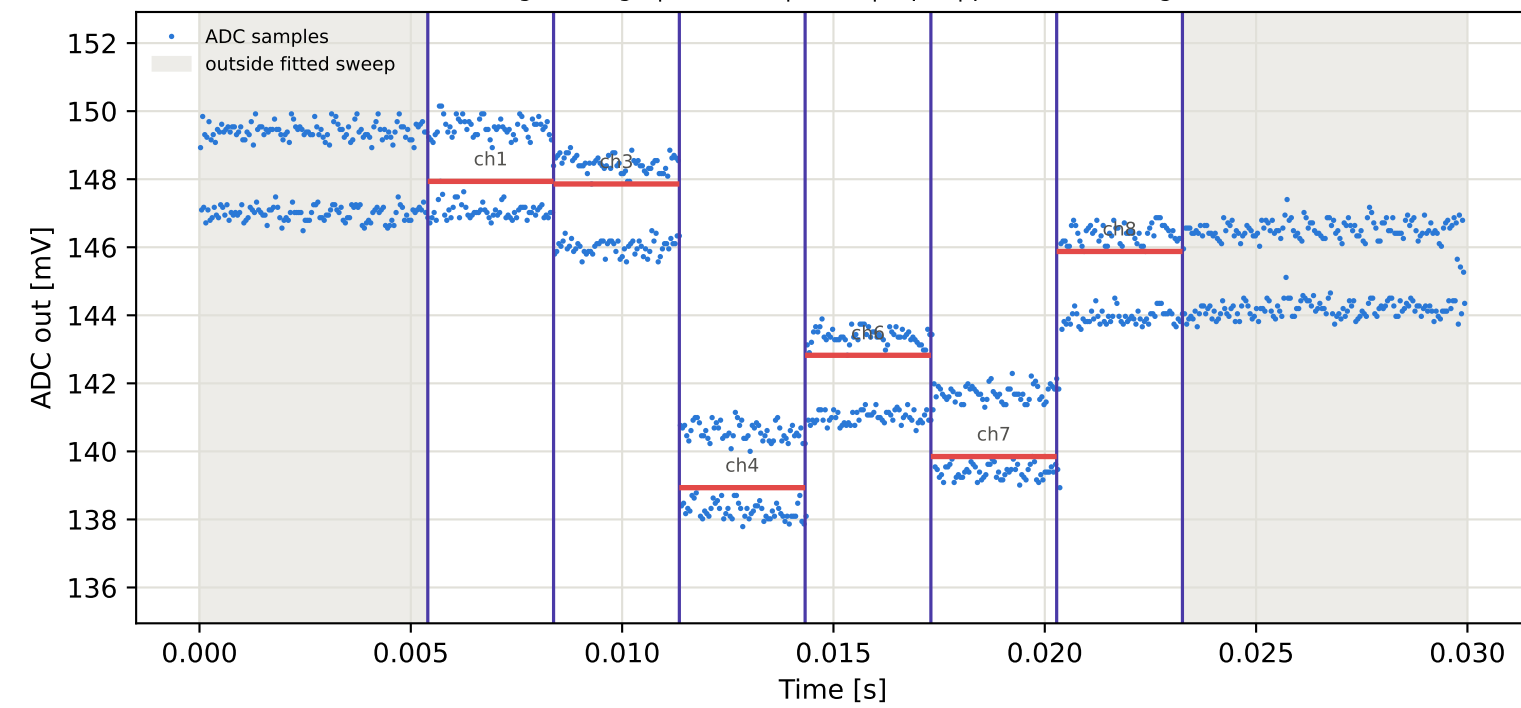
Tag9 &lt;- Tag10 | 795 MHz | run 0 | rep 1 | phase -64.54 deg
