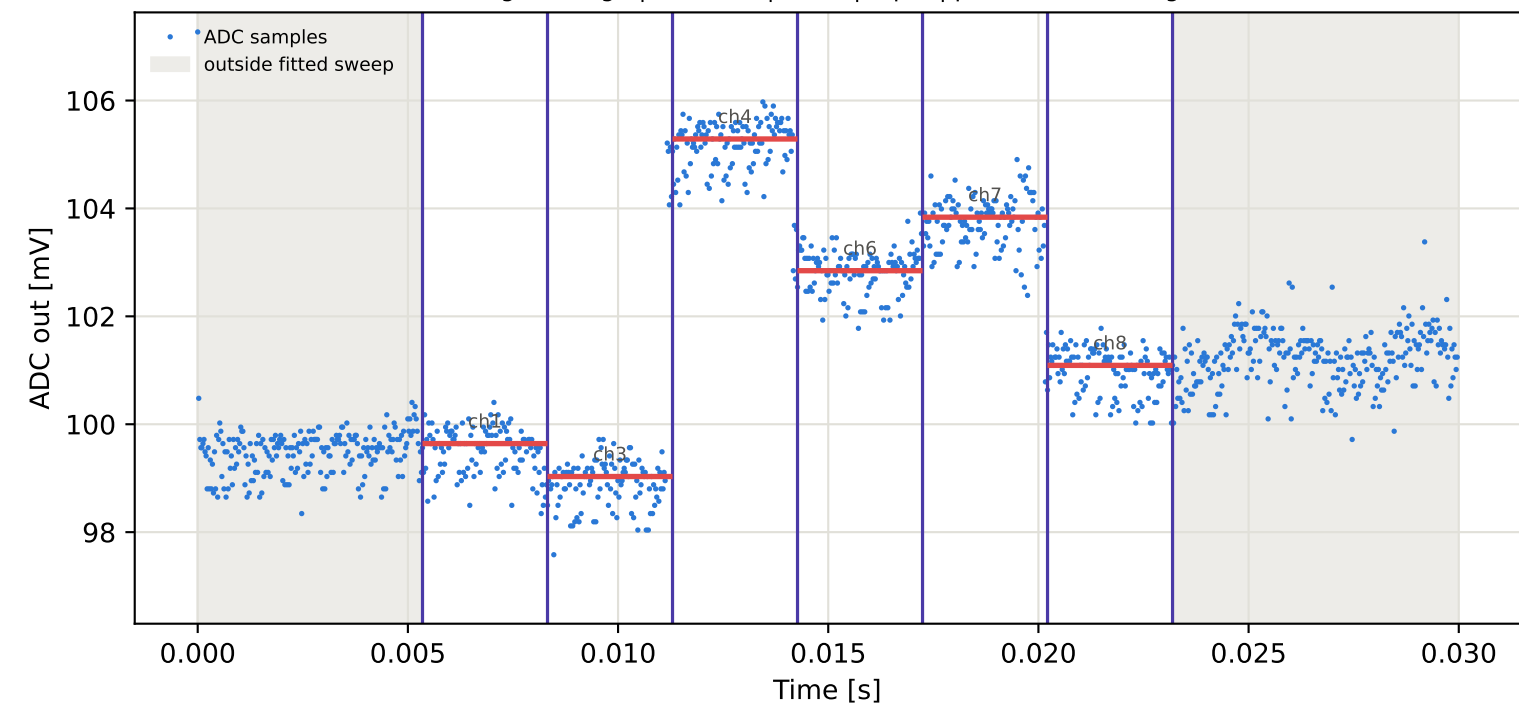
Tag6 &lt;- Tag10 | 775 MHz | run 0 | rep 1 | phase 82.80 deg
