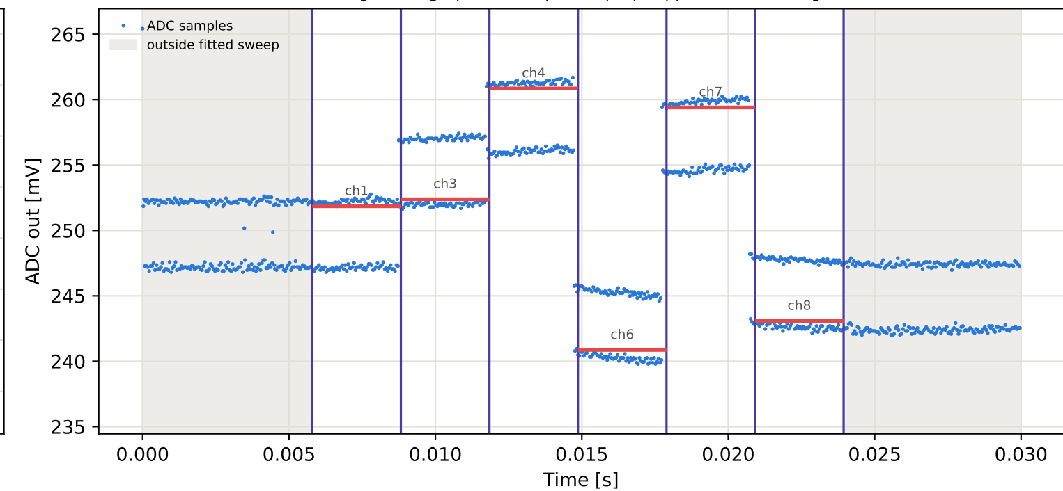
Tag10 &lt;- Tag1 | 965 MHz | run 0 | rep 1 | phase -167.54 deg
