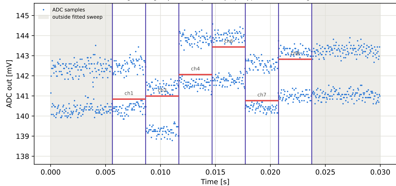
Tag3 &lt;- Tag2 | 785 MHz | run 0 | rep 1 | phase -155.16 deg
