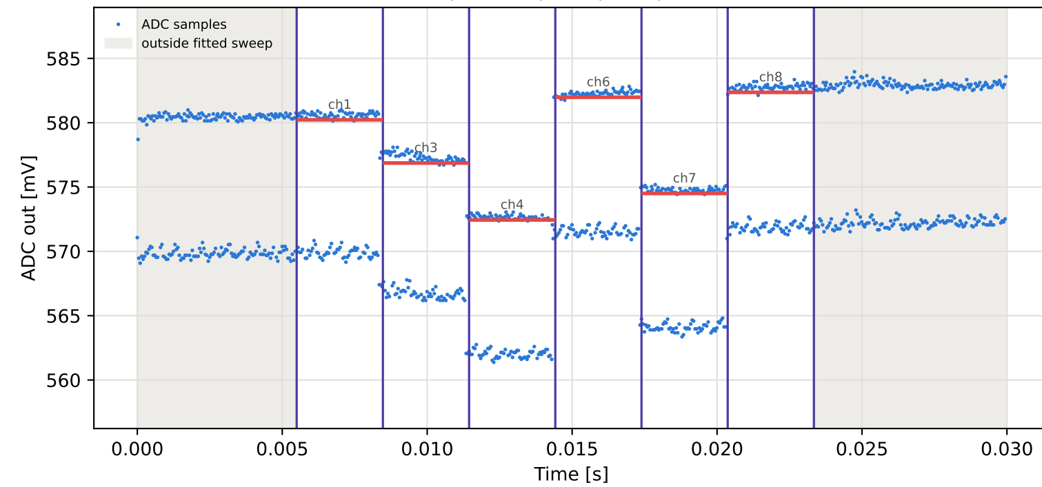
Tag15 &lt;- Tag5 | 985 MHz | run 0 | rep 1 | phase 110.58 deg
