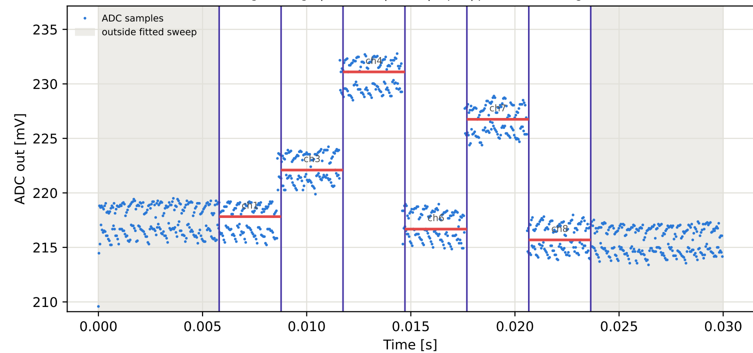
Tag7 &lt;- Tag1 | 995 MHz | run 0 | rep 1 | phase 108.88 deg
