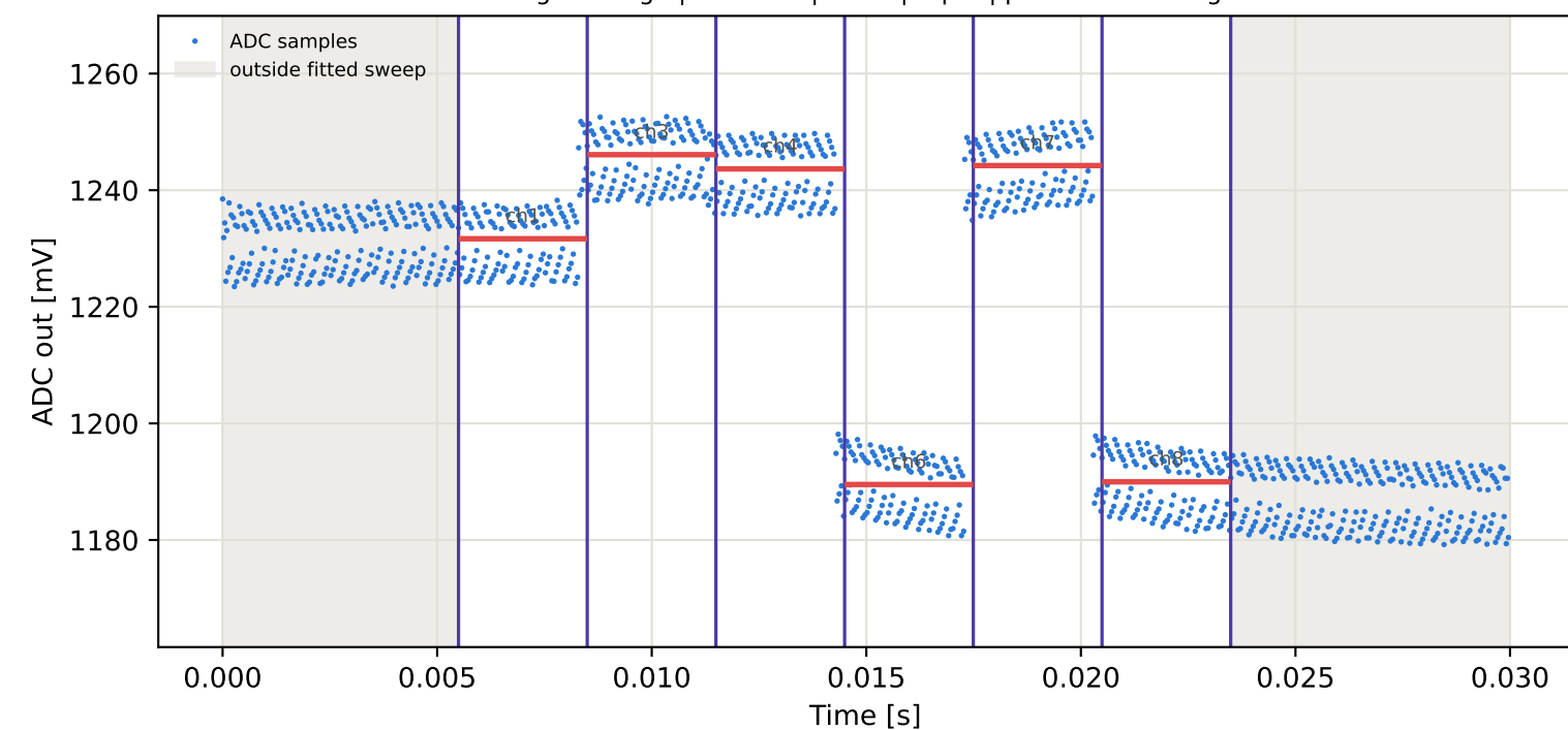
Tag3 &lt;- Tag8 | 895 MHz | run 0 | rep 1 | phase 55.91 deg
