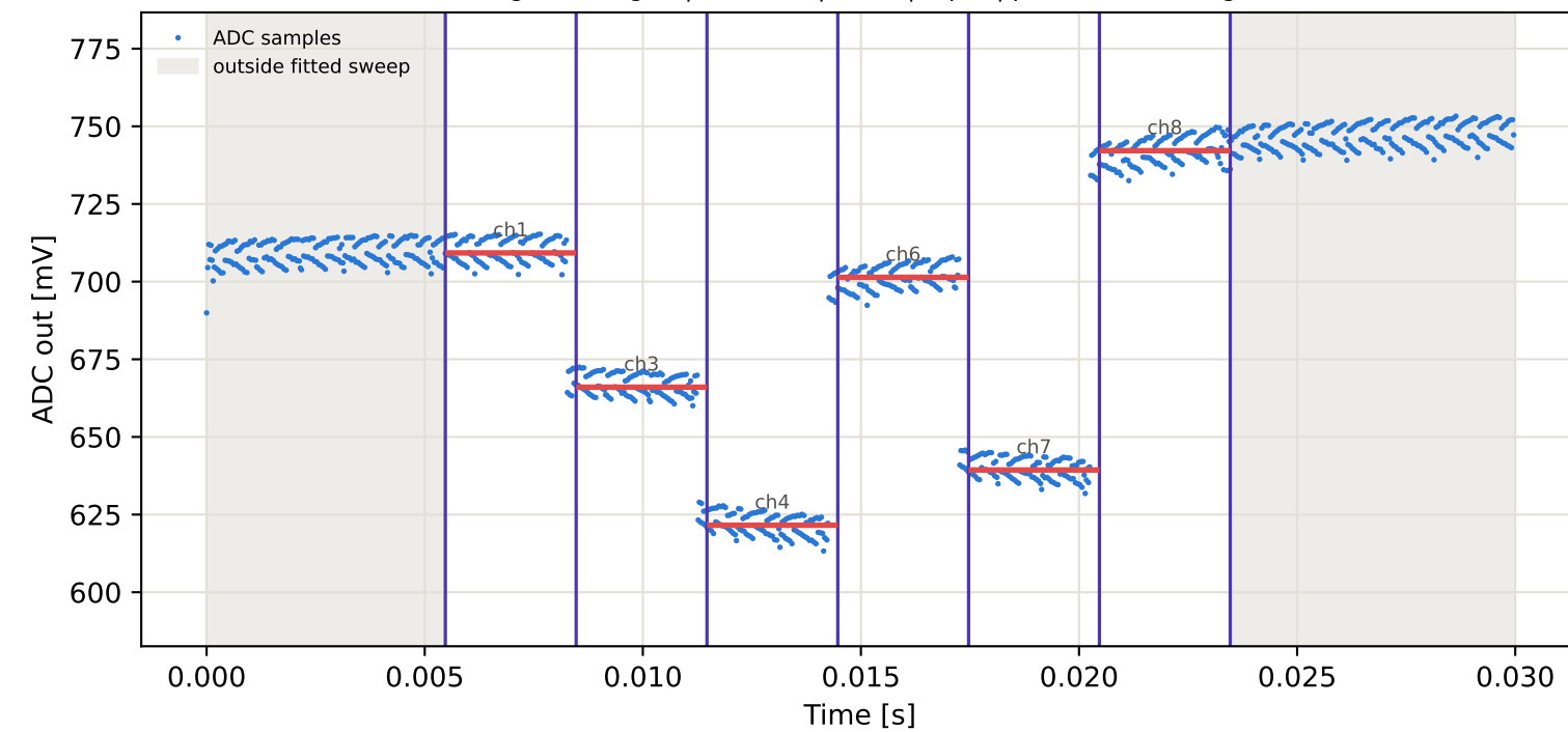
Tag15 &lt;- Tag3 | 925 MHz | run 0 | rep 1 | phase 121.64 deg
