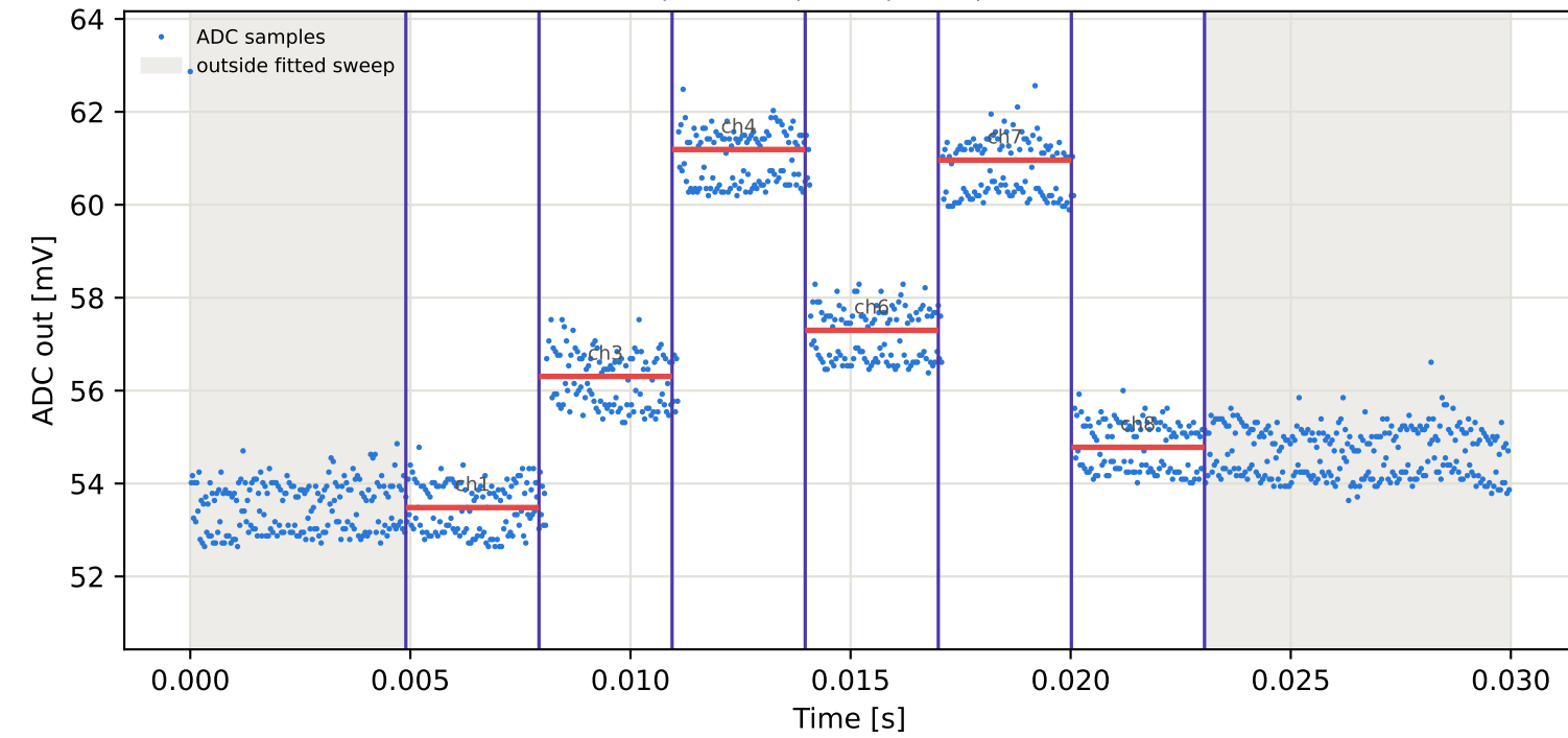
Tag9 &lt;- Tag7 | 785 MHz | run 0 | rep 1 | phase -84.90 deg
