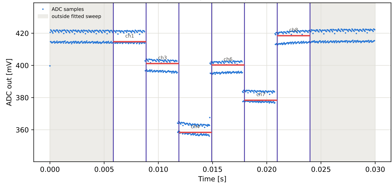
Tag3 &lt;- Tag9 | 975 MHz | run 0 | rep 1 | phase 80.51 deg
