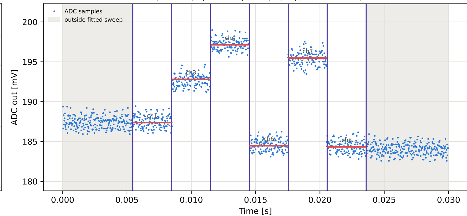
Tag15 &lt;- Tag10 | 995 MHz | run 0 | rep 1 | phase 56.71 deg
