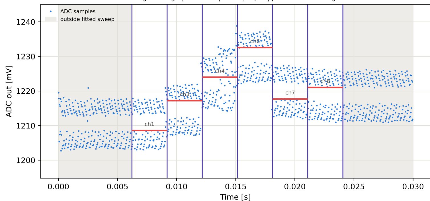
Tag3 &lt;- Tag9 | 895 MHz | run 0 | rep 1 | phase -90.77 deg
