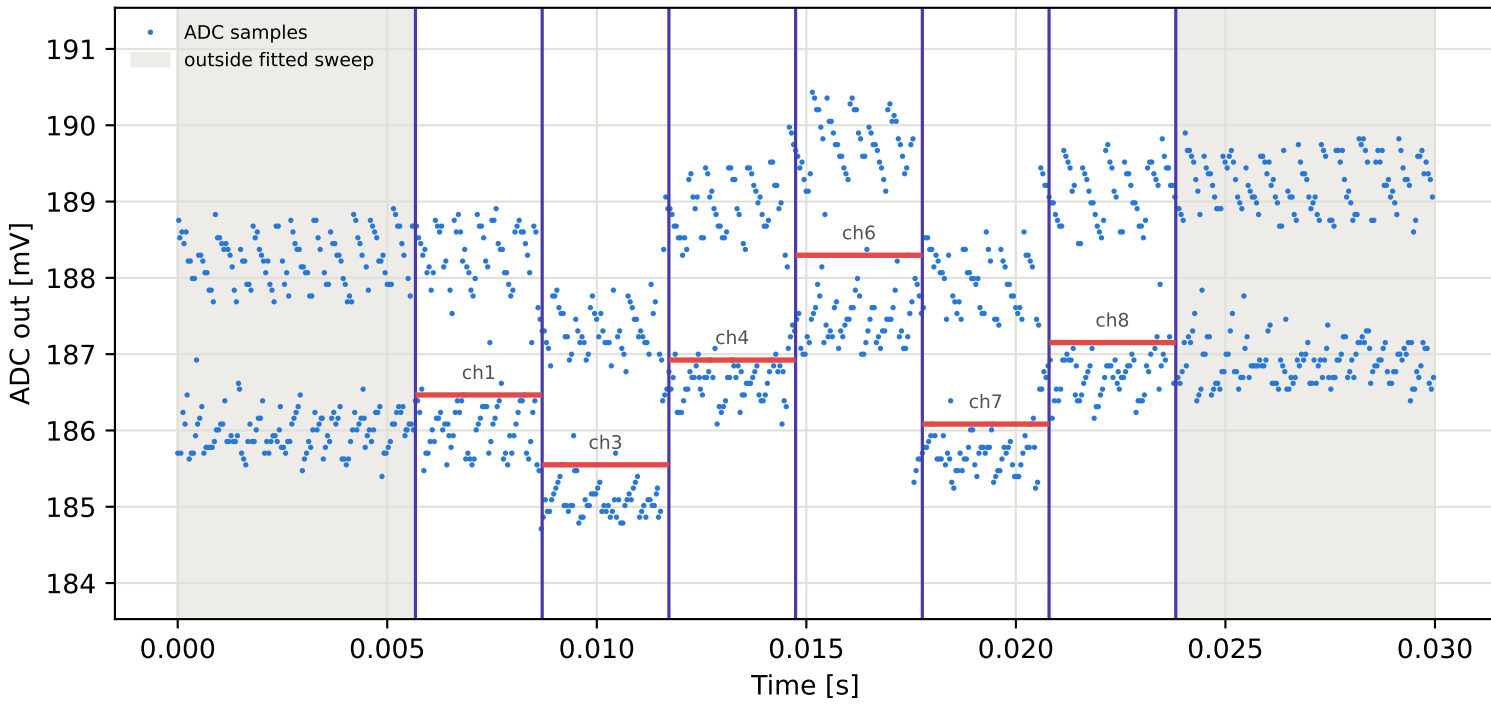
Tag10 &lt;- Tag1 | 785 MHz | run 0 | rep 1 | phase -154.36 deg
