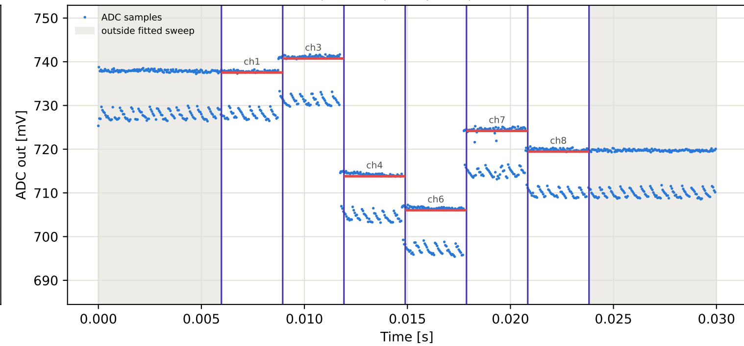
Tag8 &lt;- Tag7 | 845 MHz | run 0 | rep 1 | phase 42.83 deg
