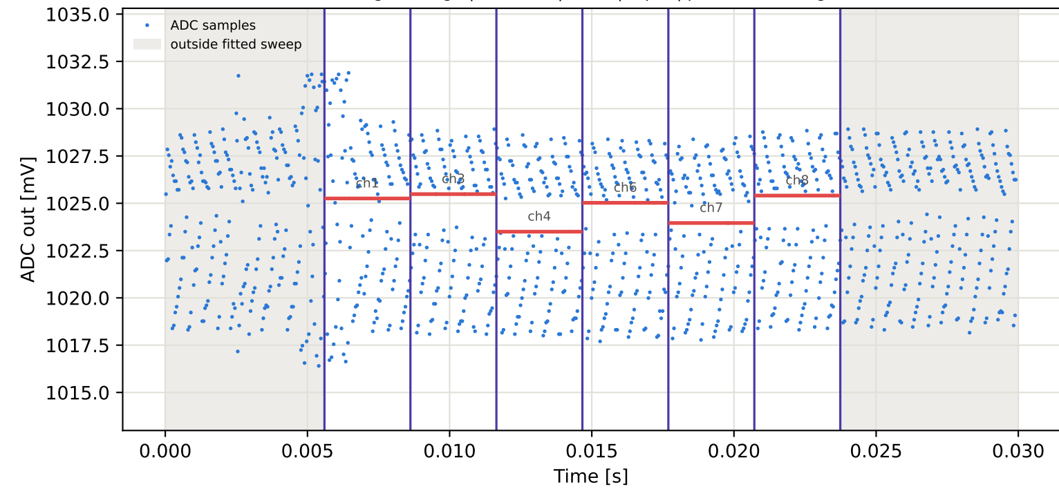
Tag8 &lt;- Tag10 | 895 MHz | run 0 | rep 1 | phase -144.59 deg
