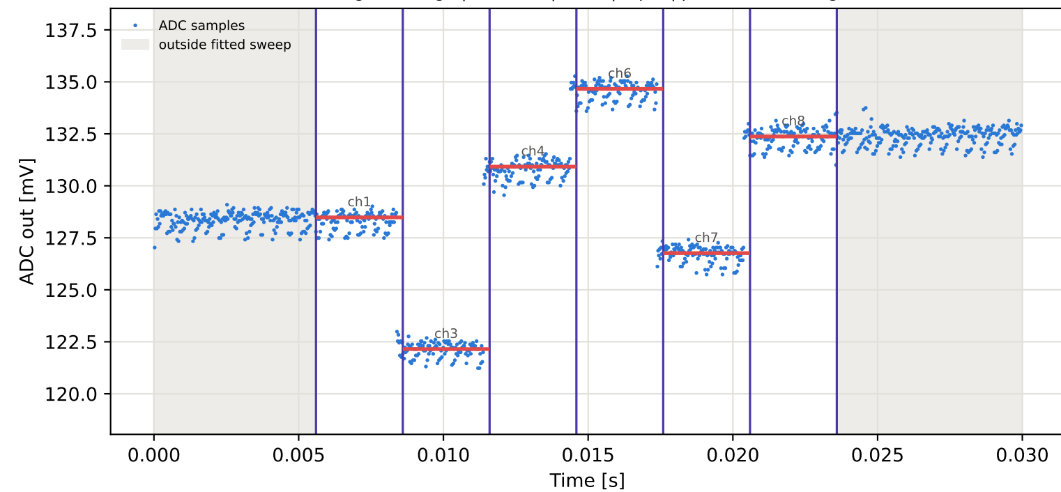
Tag10 &lt;- Tag9 | 775 MHz | run 0 | rep 1 | phase -91.80 deg
