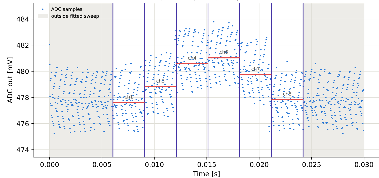
Tag15 &lt;- Tag4 | 845 MHz | run 0 | rep 1 | phase 91.15 deg
