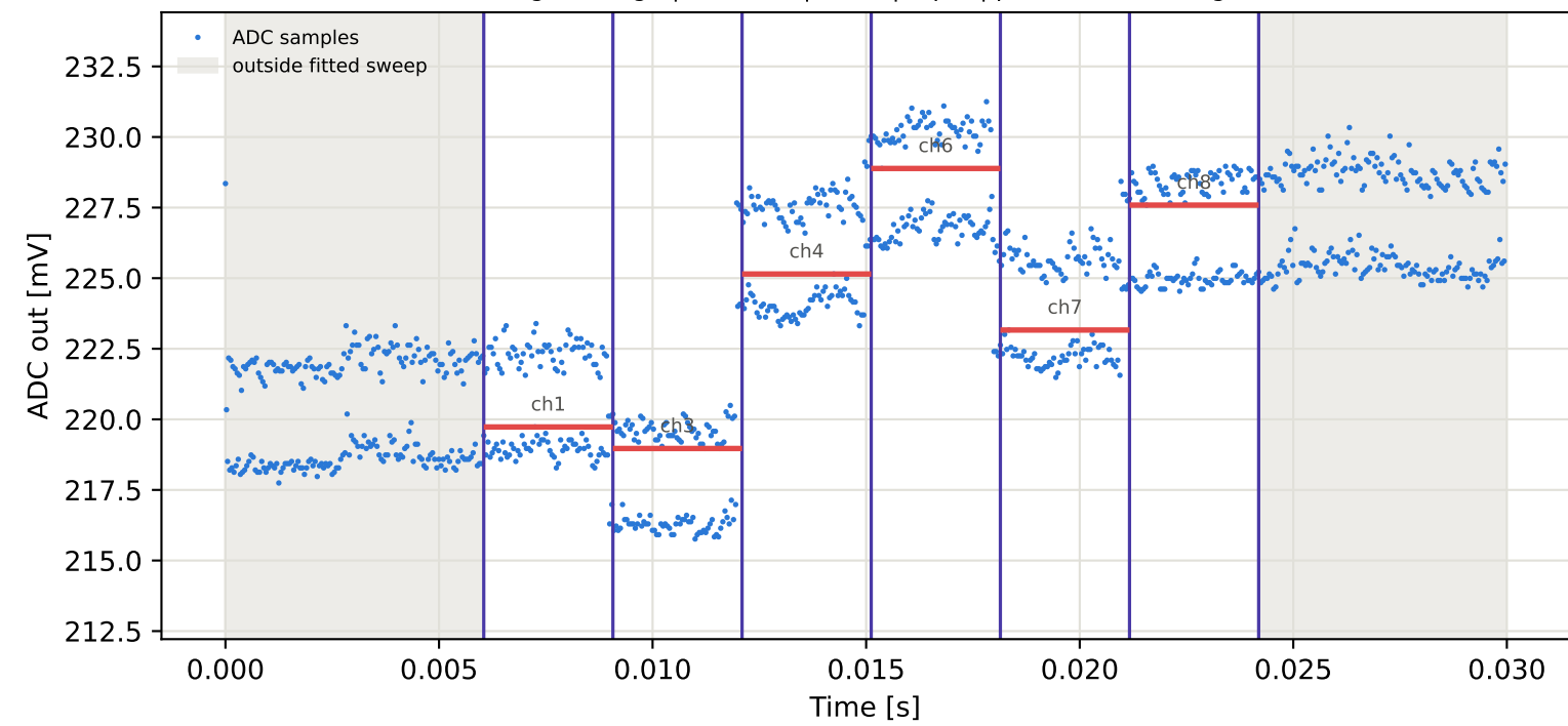
Tag9 &lt;- Tag6 | 835 MHz | run 0 | rep 1 | phase -67.56 deg
