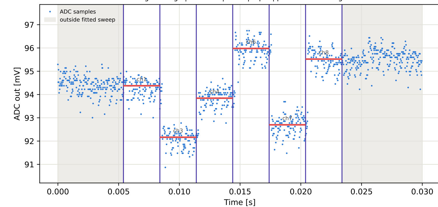
Tag2 &lt;- Tag7 | 805 MHz | run 0 | rep 1 | phase 64.56 deg
