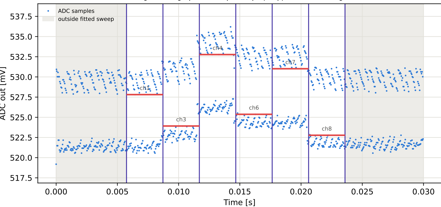
Tag15 &lt;- Tag1 | 955 MHz | run 0 | rep 1 | phase -88.95 deg
