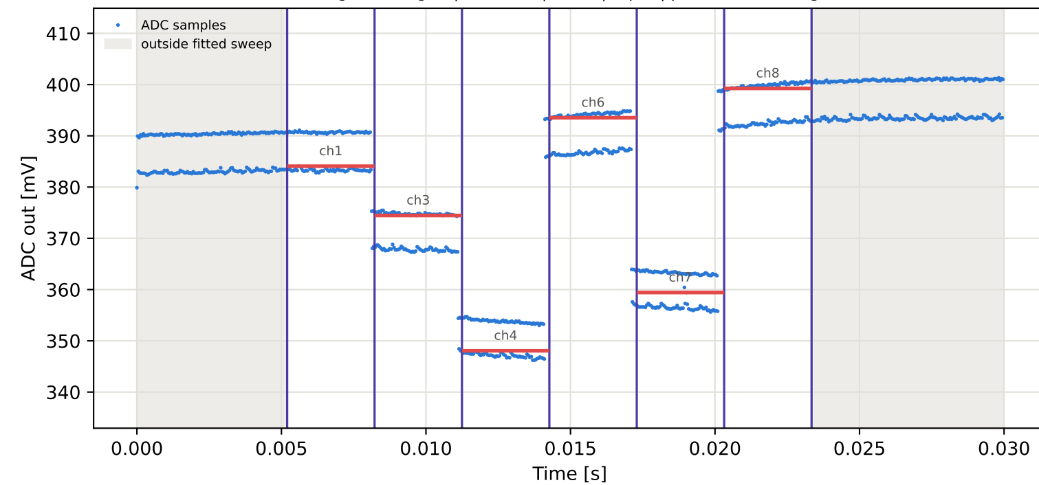
Tag10 &lt;- Tag2 | 965 MHz | run 0 | rep 1 | phase -16.02 deg
