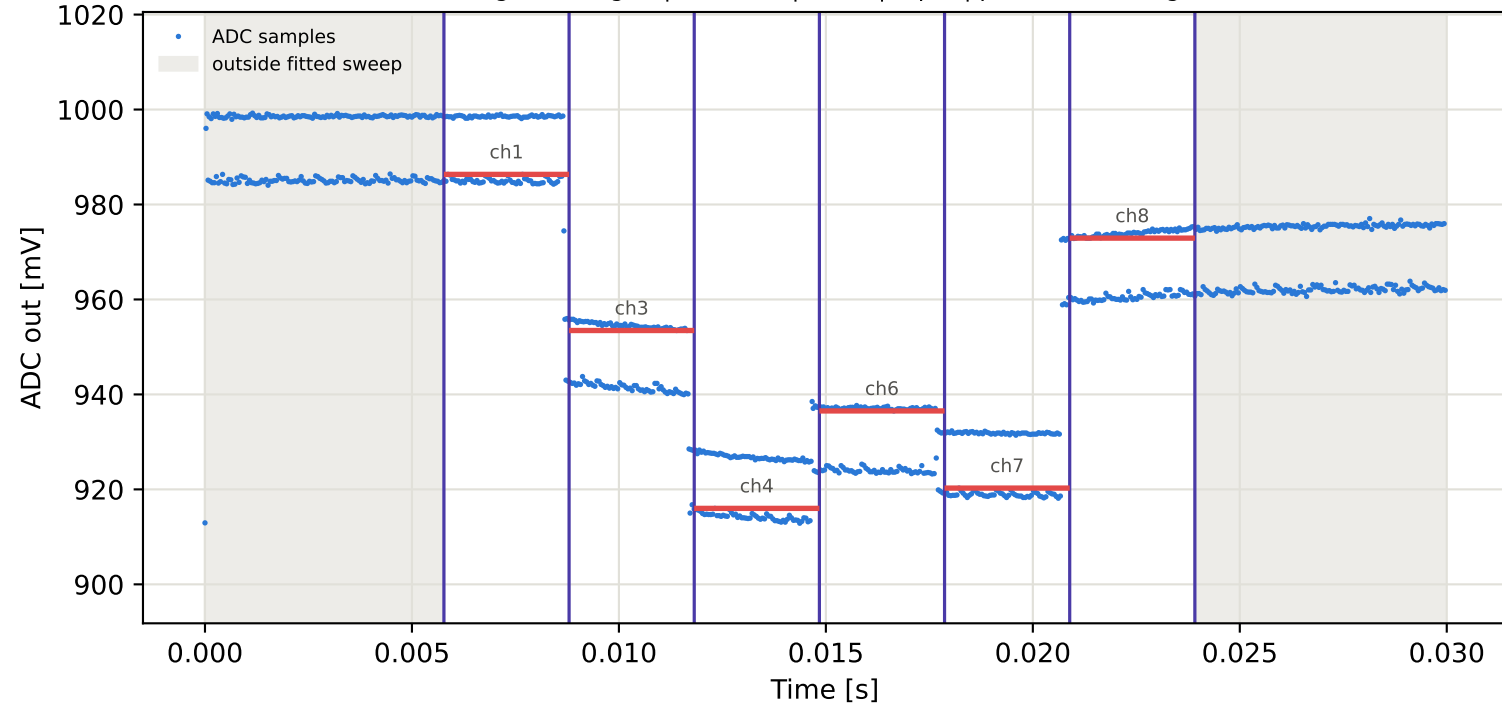
Tag10 &lt;- Tag3 | 875 MHz | run 0 | rep 1 | phase 90.20 deg
