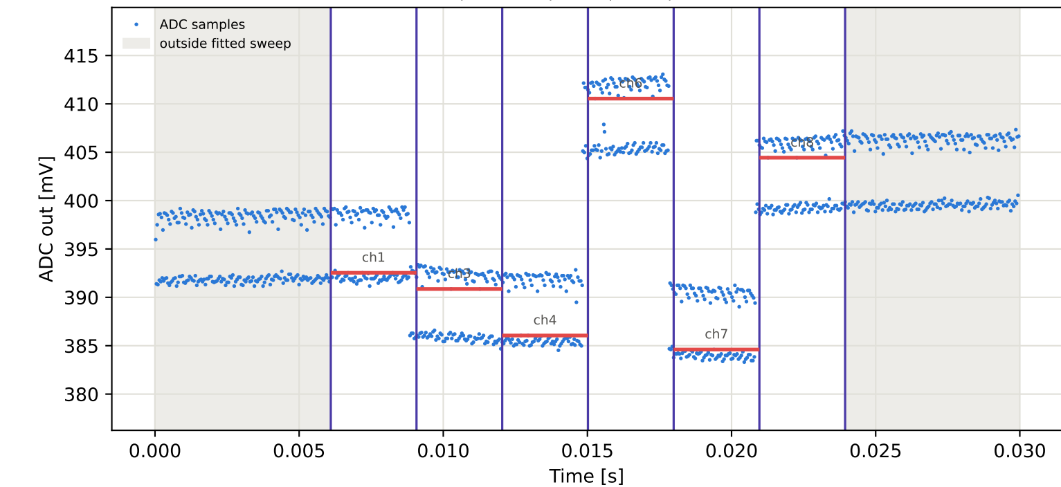
Tag3 &lt;- Tag8 | 975 MHz | run 0 | rep 1 | phase 153.70 deg
