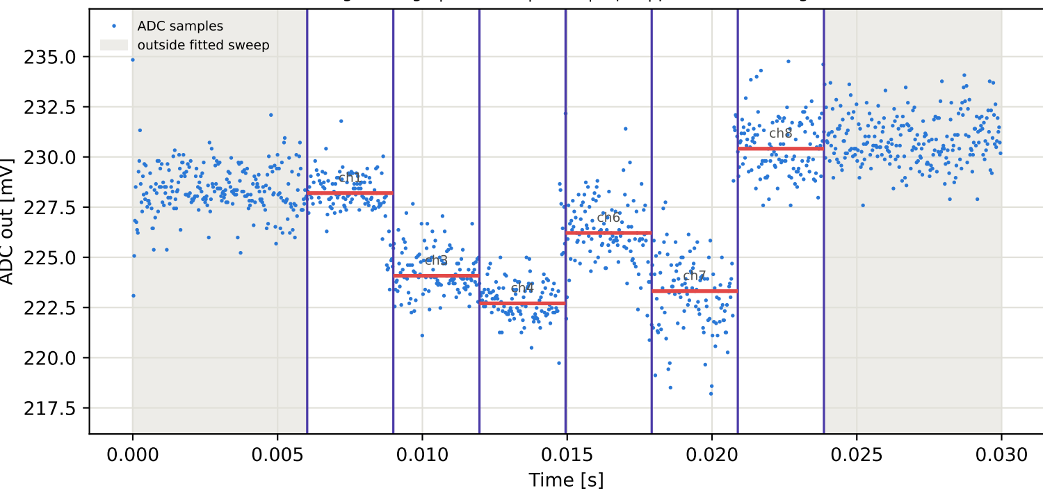
Tag9 &lt;- Tag7 | 885 MHz | run 0 | rep 1 | phase 105.91 deg
