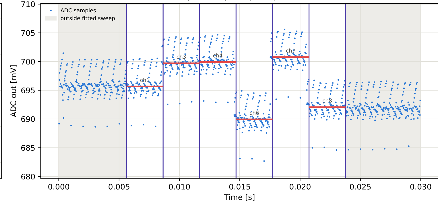
Tag8 &lt;- Tag10 | 995 MHz | run 0 | rep 1 | phase 76.81 deg
