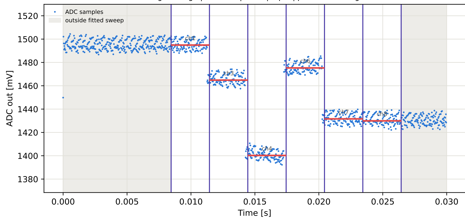
Tag8 &lt;- Tag5 | 885 MHz | run 0 | rep 1 | phase 111.09 deg
