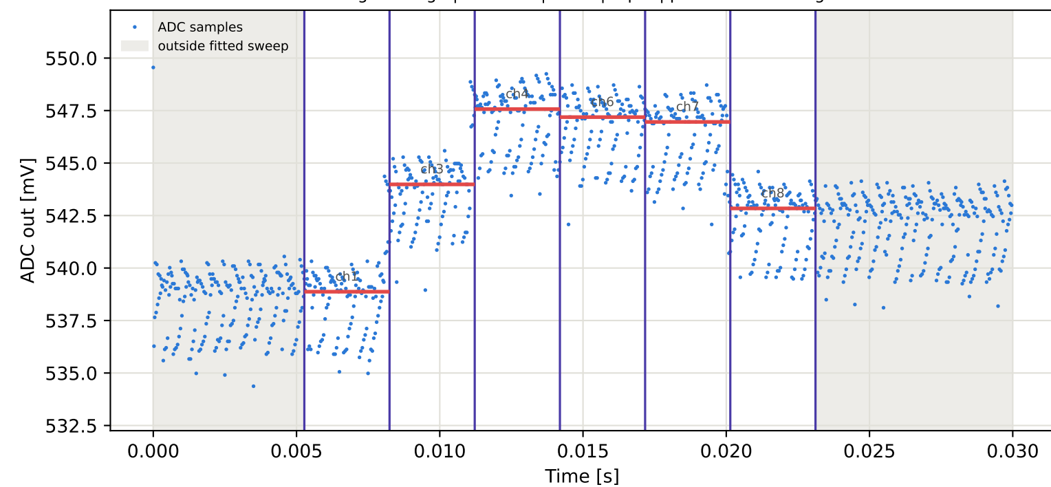
Tag6 &lt;- Tag5 | 865 MHz | run 0 | rep 1 | phase -112.52 deg
