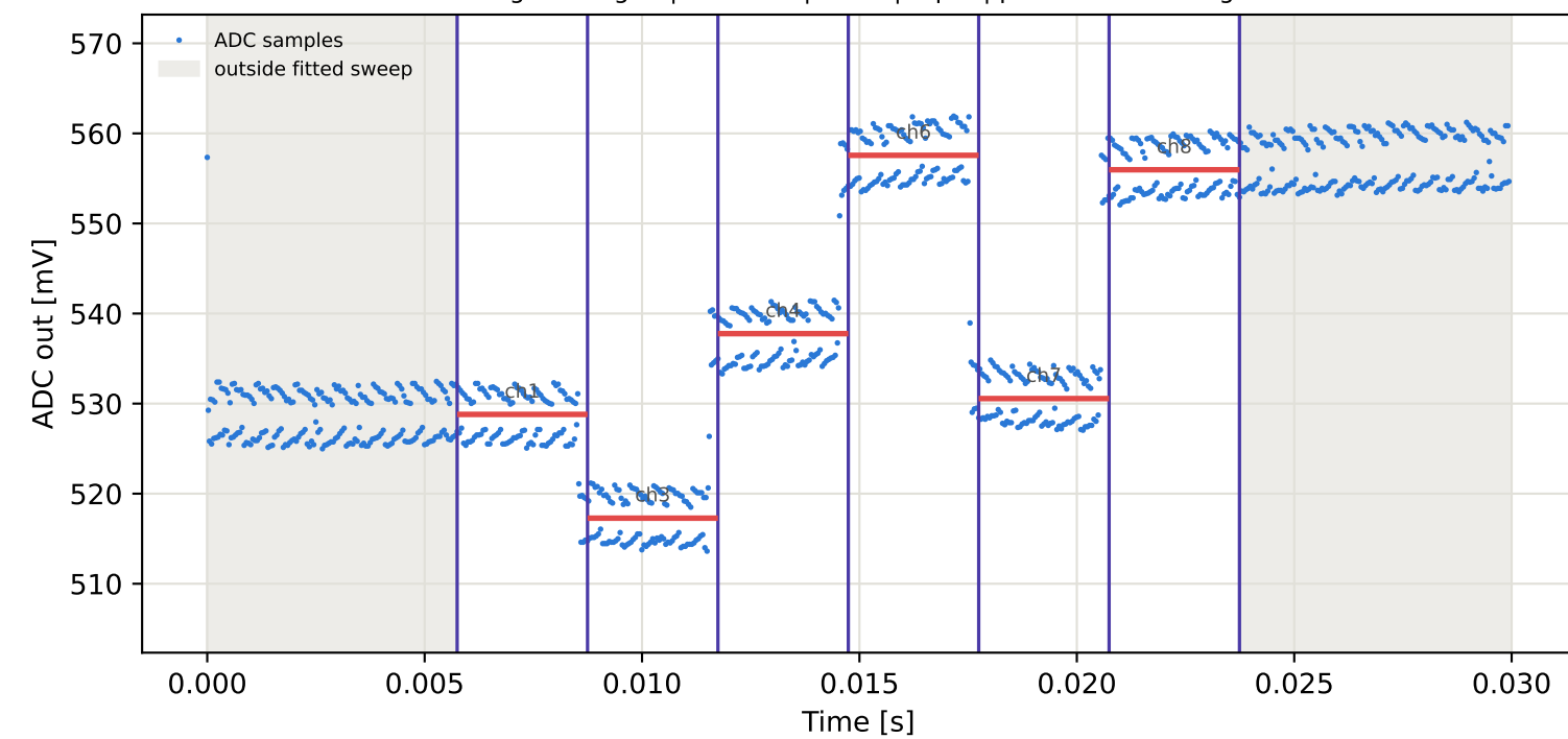
Tag6 &lt;- Tag2 | 865 MHz | run 0 | rep 1 | phase 42.95 deg
