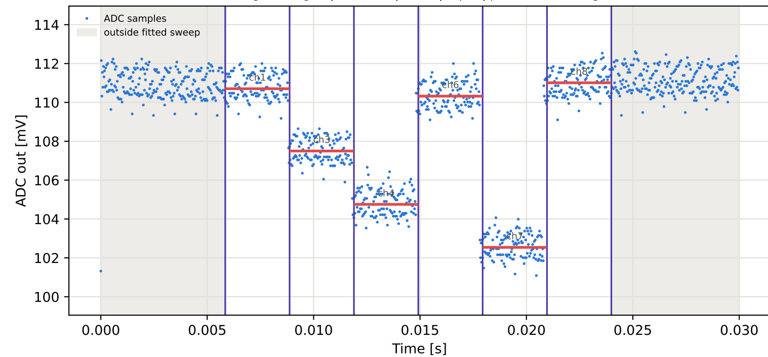
Tag5 &lt;- Tag16 | 775 MHz | run 0 | rep 1 | phase 147.37 deg
