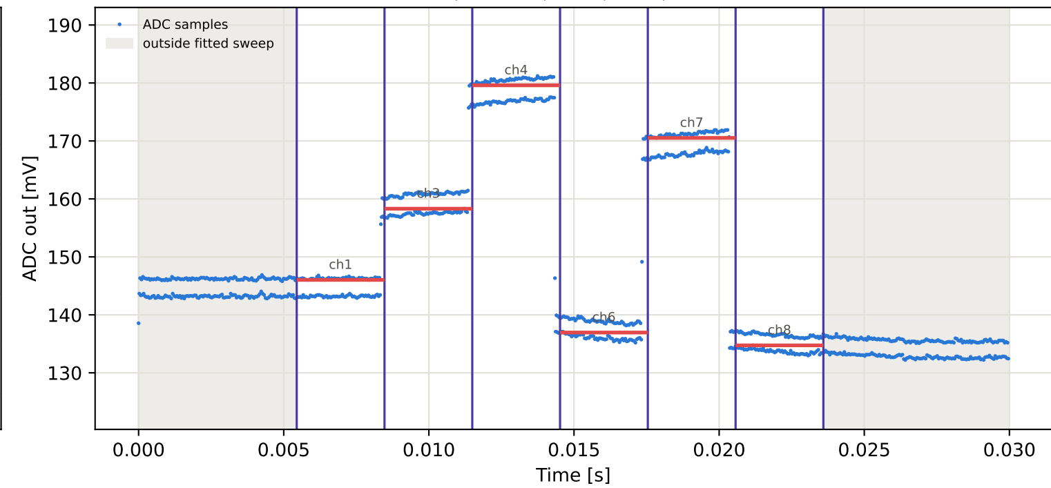
Tag6 &lt;- Tag10 | 955 MHz | run 0 | rep 1 | phase -64.15 deg
