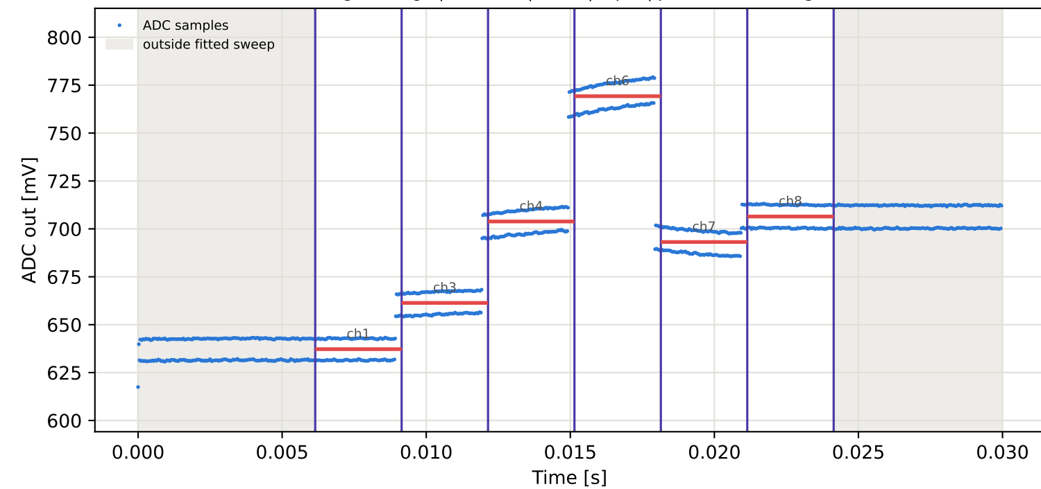
Tag7 &lt;- Tag1 | 895 MHz | run 0 | rep 1 | phase 27.14 deg
