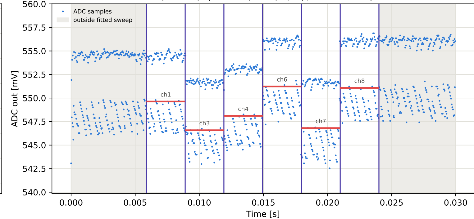
Tag16 &lt;- Tag15 | 825 MHz | run 0 | rep 1 | phase 63.87 deg
