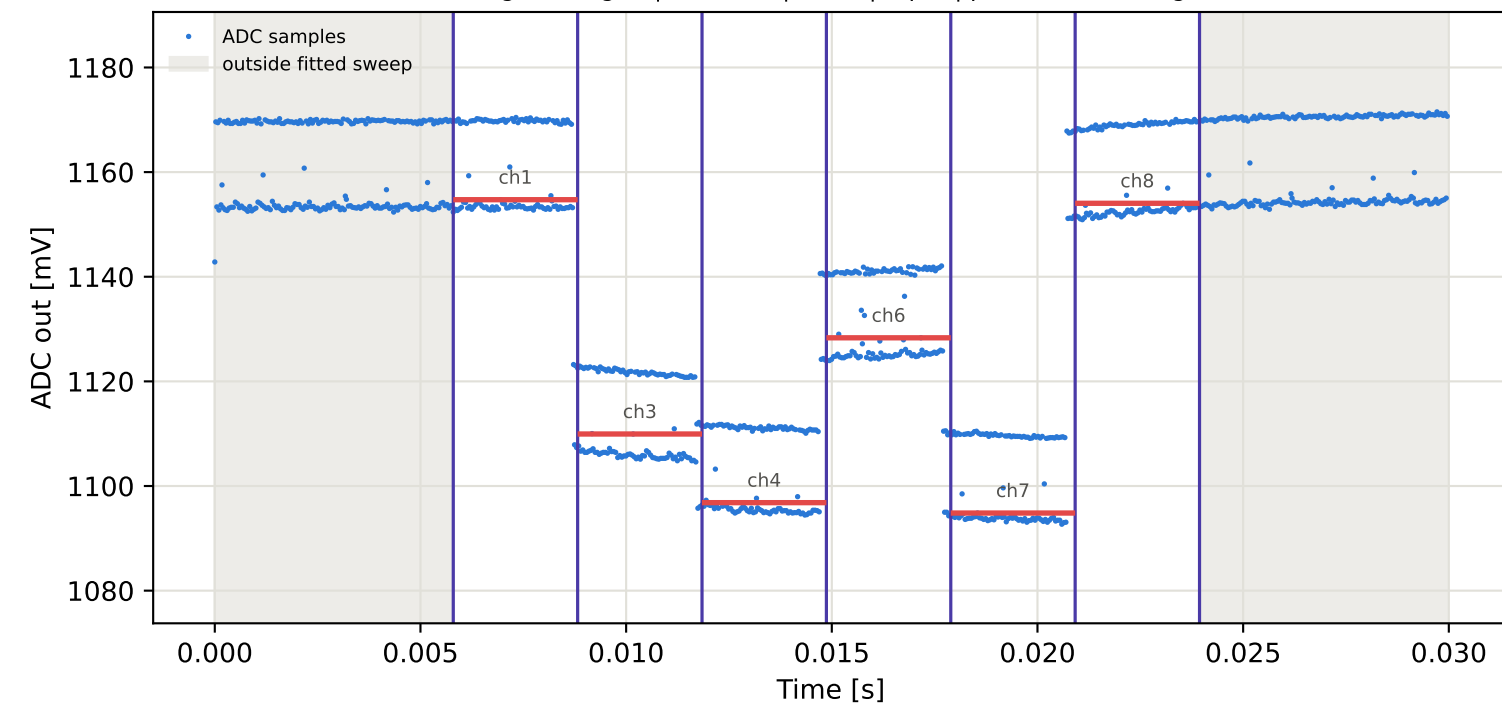
Tag7 &lt;- Tag3 | 865 MHz | run 0 | rep 1 | phase 98.23 deg
