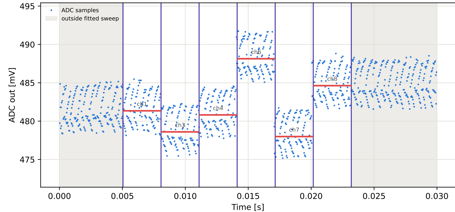
Tag15 &lt;- Tag6 | 995 MHz | run 0 | rep 1 | phase 75.02 deg
