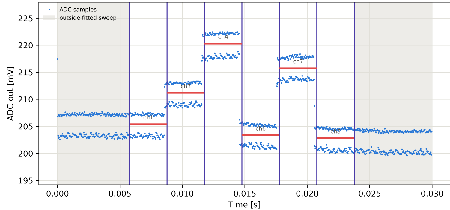
Tag5 &lt;- Tag1 | 995 MHz | run 0 | rep 1 | phase 6.16 deg
