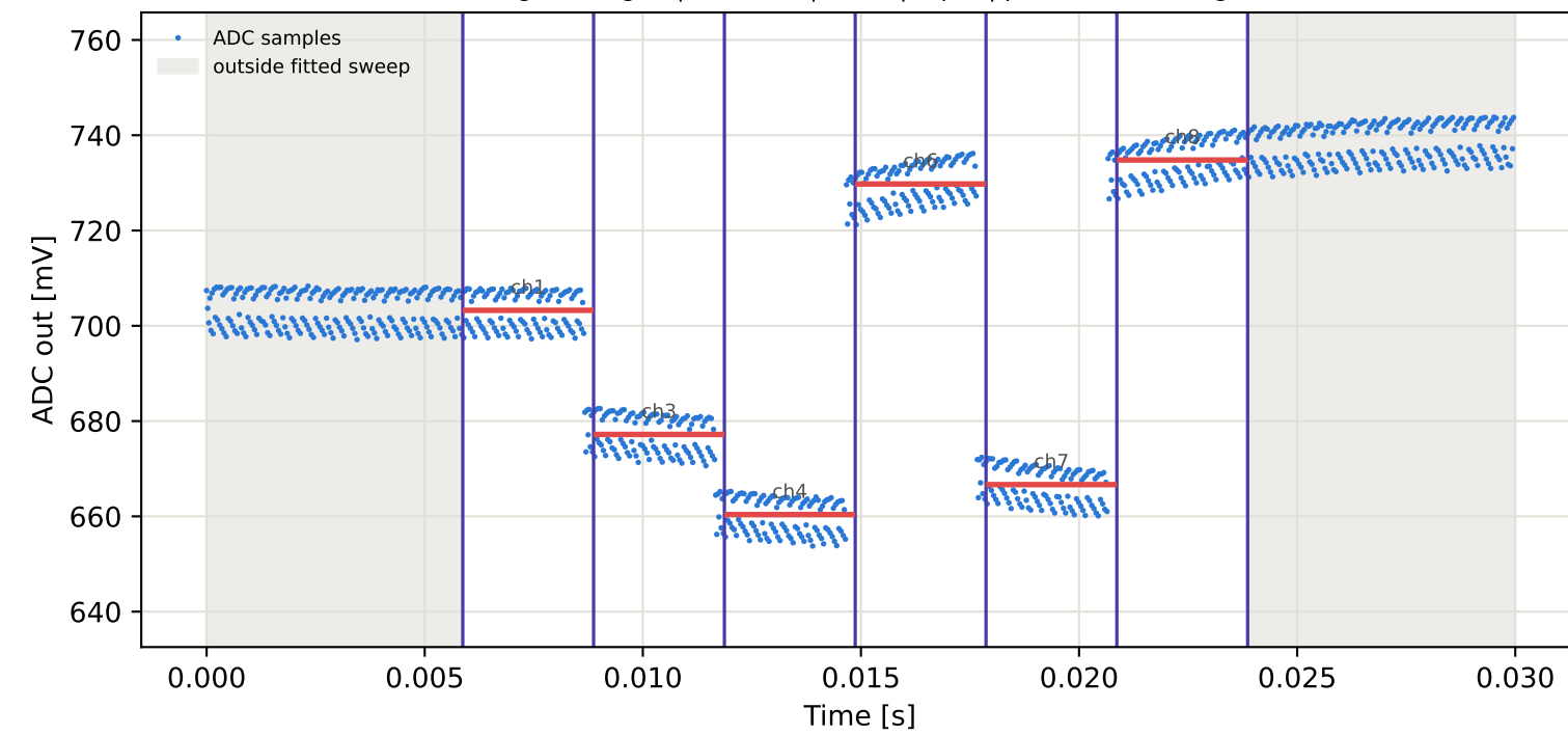
Tag1 &lt;- Tag16 | 915 MHz | run 0 | rep 1 | phase -60.50 deg
