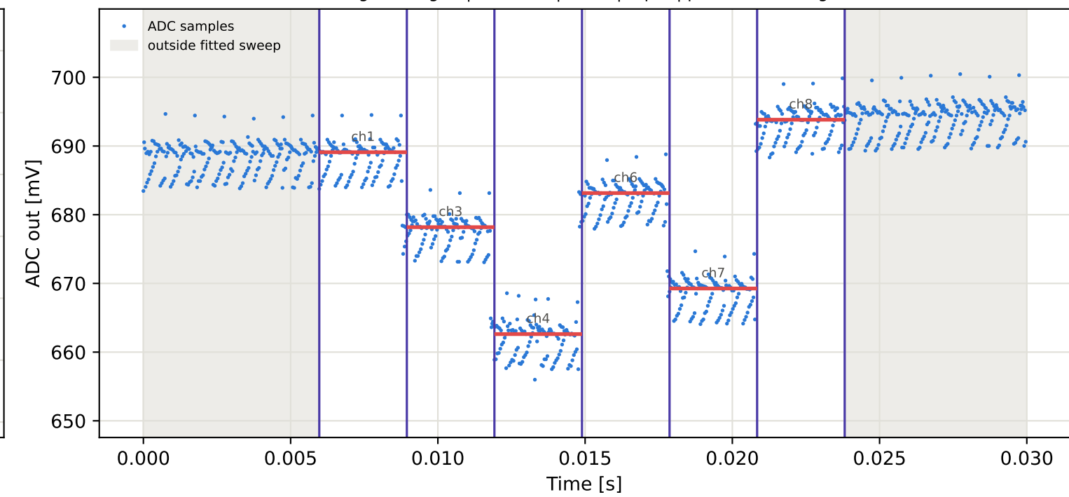
Tag7 &lt;- Tag15 | 945 MHz | run 0 | rep 1 | phase 94.48 deg
