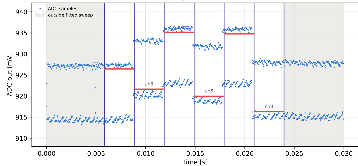
Tag8 &lt;- Tag10 | 855 MHz | run 0 | rep 1 | phase -161.92 deg
