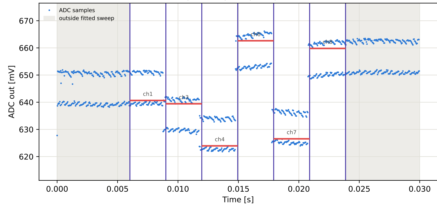
Tag10 &lt;- Tag1 | 945 MHz | run 0 | rep 1 | phase 136.89 deg
