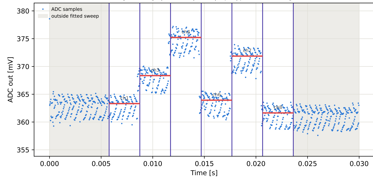
Tag2 &lt;- Tag10 | 995 MHz | run 0 | rep 1 | phase 49.27 deg
