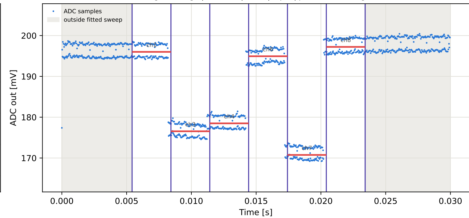
Tag16 &lt;- Tag5 | 805 MHz | run 0 | rep 1 | phase 166.61 deg
