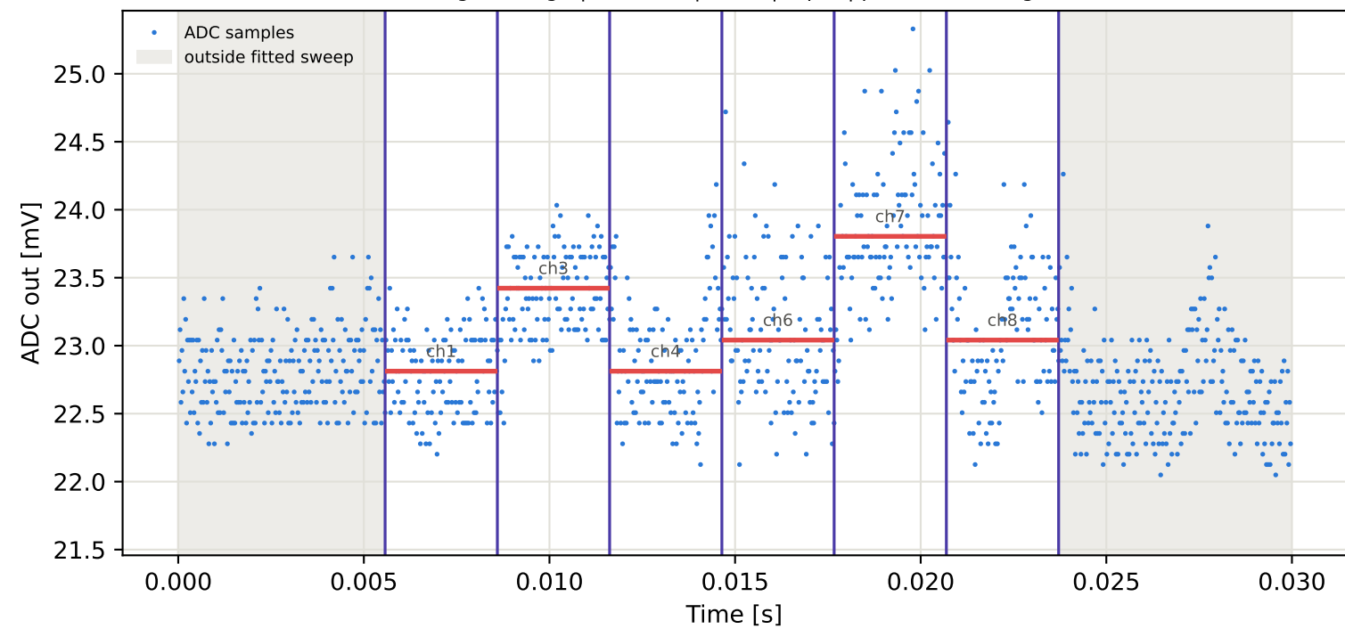
Tag3 &lt;- Tag10 | 785 MHz | run 0 | rep 1 | phase 0.59 deg
