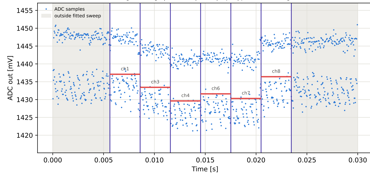
Tag16 &lt;- Tag10 | 885 MHz | run 0 | rep 1 | phase -122.47 deg
