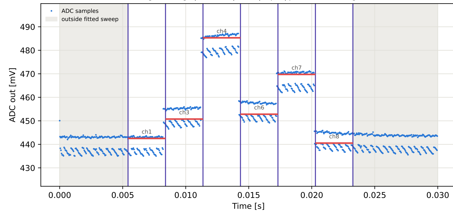
Tag15 &lt;- Tag9 | 975 MHz | run 0 | rep 1 | phase -1.02 deg
