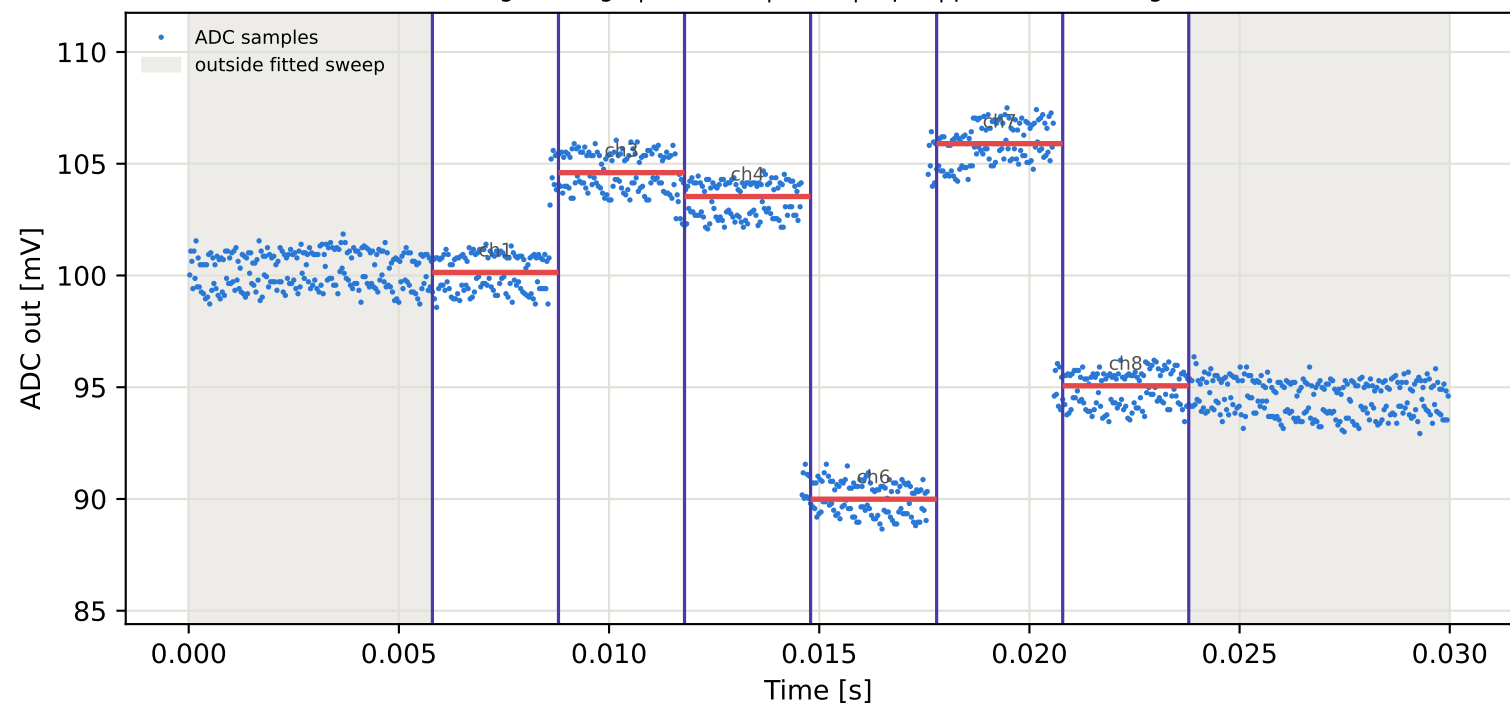
Tag9 &lt;- Tag8 | 995 MHz | run 0 | rep 1 | phase -16.69 deg
