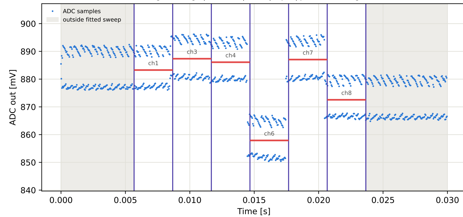
Tag16 &lt;- Tag4 | 945 MHz | run 0 | rep 1 | phase 81.93 deg
