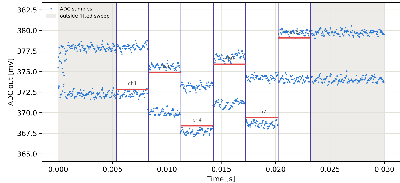
Tag5 &lt;- Tag4 | 855 MHz | run 0 | rep 1 | phase -172.73 deg
