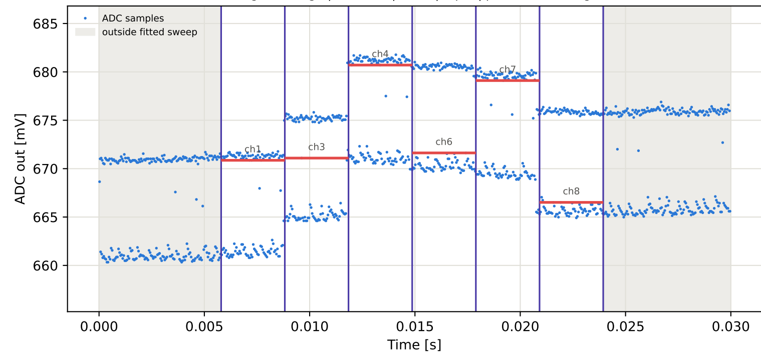
Tag2 &lt;- Tag10 | 855 MHz | run 0 | rep 1 | phase -30.32 deg
