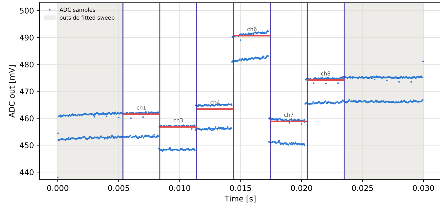
Tag9 &lt;- Tag16 | 955 MHz | run 0 | rep 1 | phase -27.49 deg
