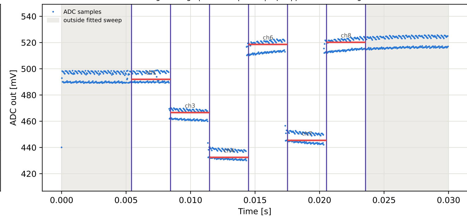
Tag3 &lt;- Tag7 | 945 MHz | run 0 | rep 1 | phase -152.13 deg
