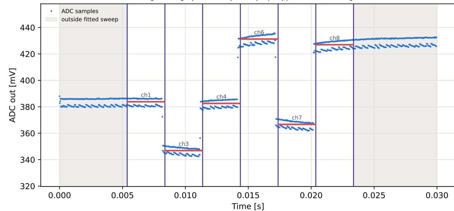
Tag2 &lt;- Tag7 | 865 MHz | run 0 | rep 1 | phase -175.20 deg
