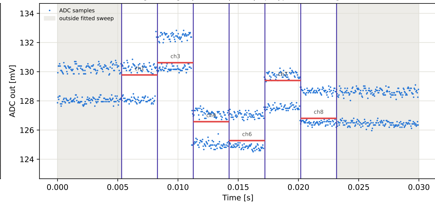
Tag10 &lt;- Tag3 | 775 MHz | run 0 | rep 1 | phase -55.02 deg
