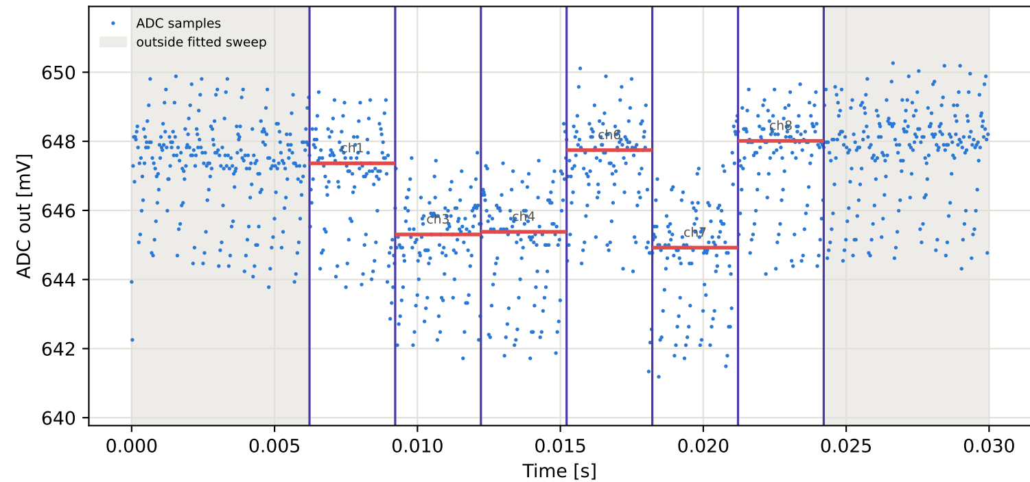
Tag16 &lt;- Tag15 | 835 MHz | run 0 | rep 1 | phase 78.34 deg
