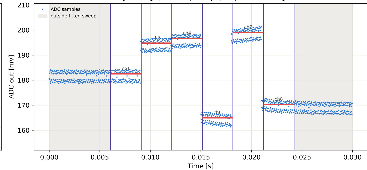
Tag10 &lt;- Tag9 | 995 MHz | run 0 | rep 1 | phase -60.43 deg
