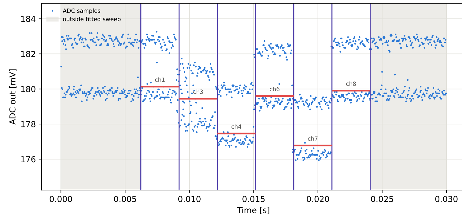
Tag10 &lt;- Tag4 | 795 MHz | run 0 | rep 1 | phase 109.97 deg
