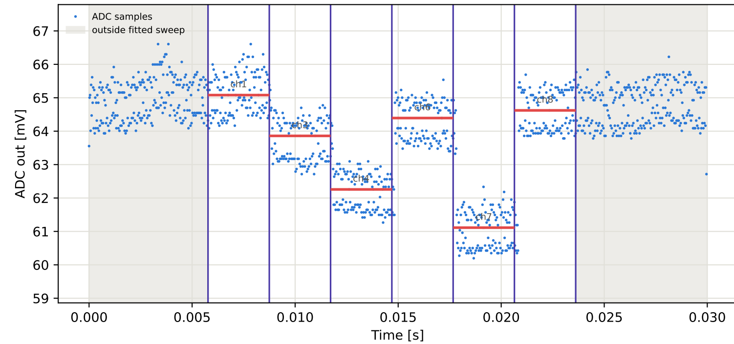
Tag15 &lt;- Tag5 | 785 MHz | run 0 | rep 1 | phase 35.83 deg
