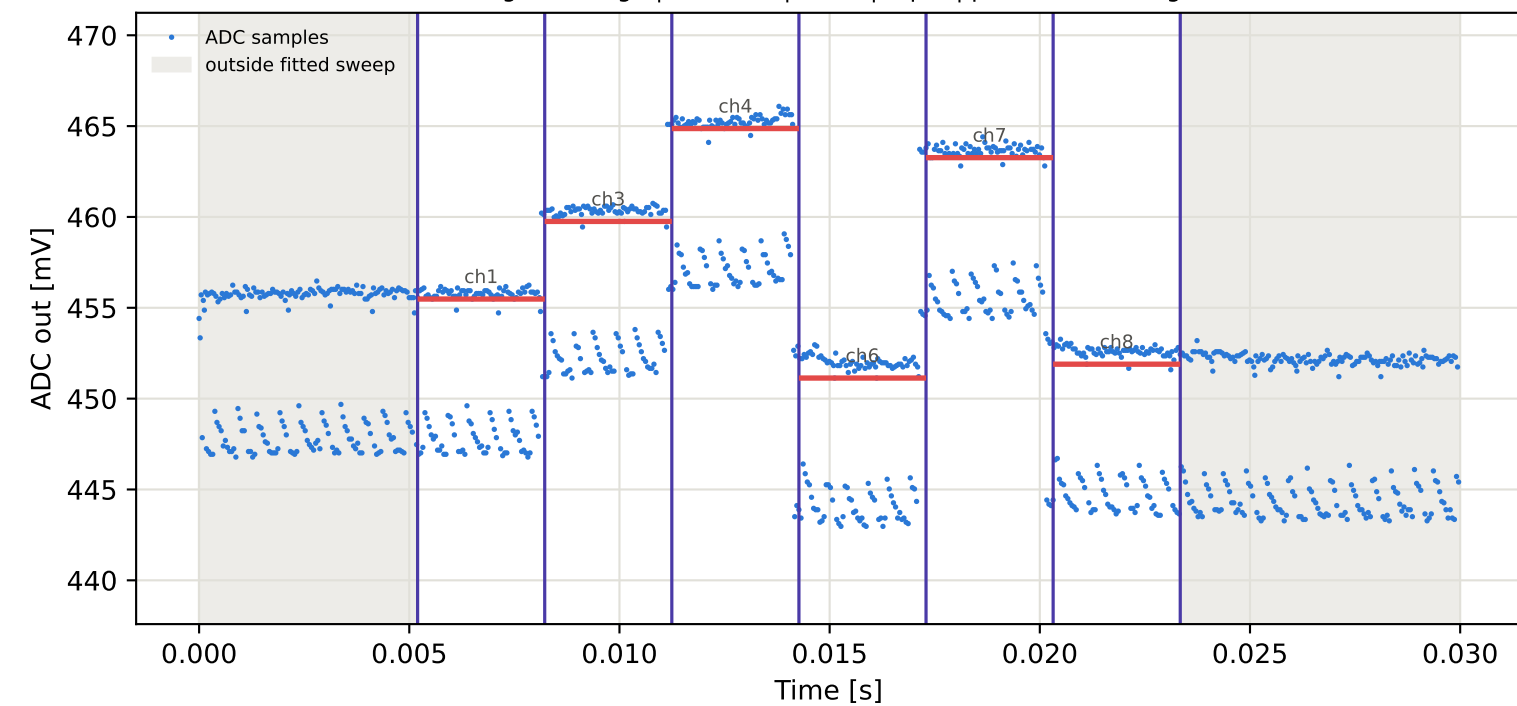
Tag15 &lt;- Tag1 | 975 MHz | run 0 | rep 1 | phase -56.83 deg
