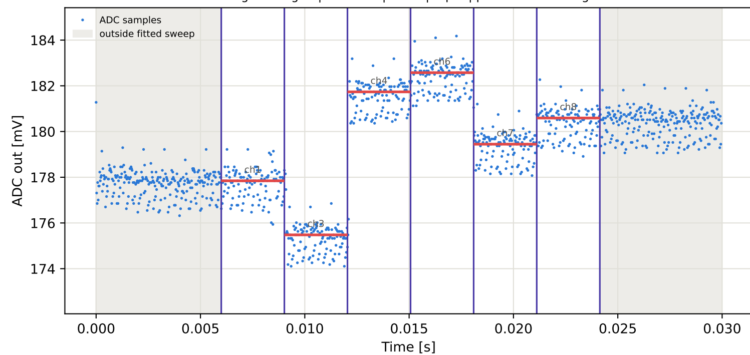
Tag3 &lt;- Tag2 | 805 MHz | run 0 | rep 1 | phase -105.46 deg
