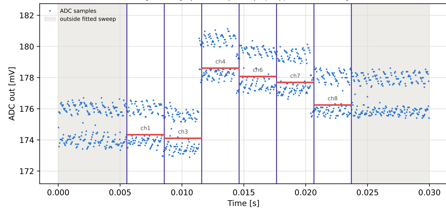
Tag15 &lt;- Tag10 | 795 MHz | run 0 | rep 1 | phase 163.89 deg
