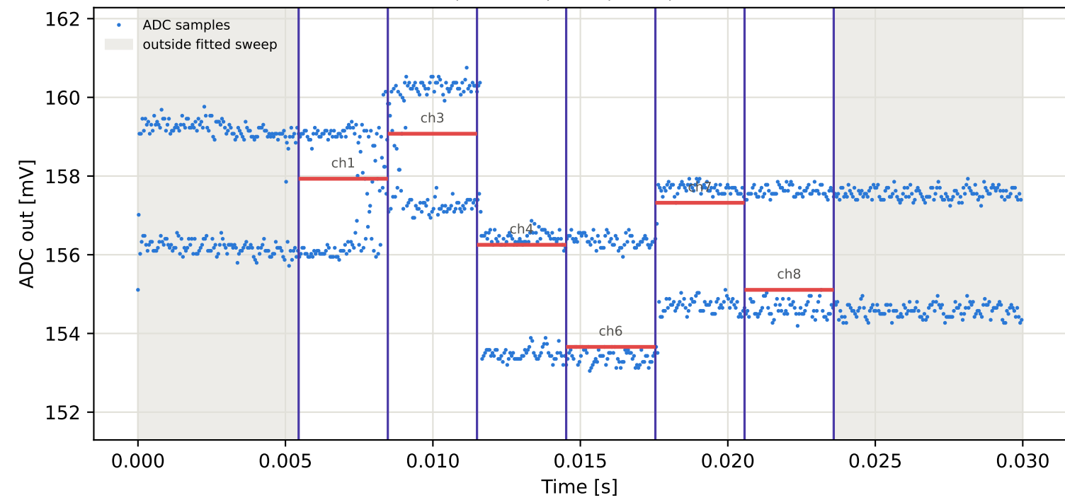
Tag7 &lt;- Tag6 | 785 MHz | run 0 | rep 1 | phase 29.98 deg
