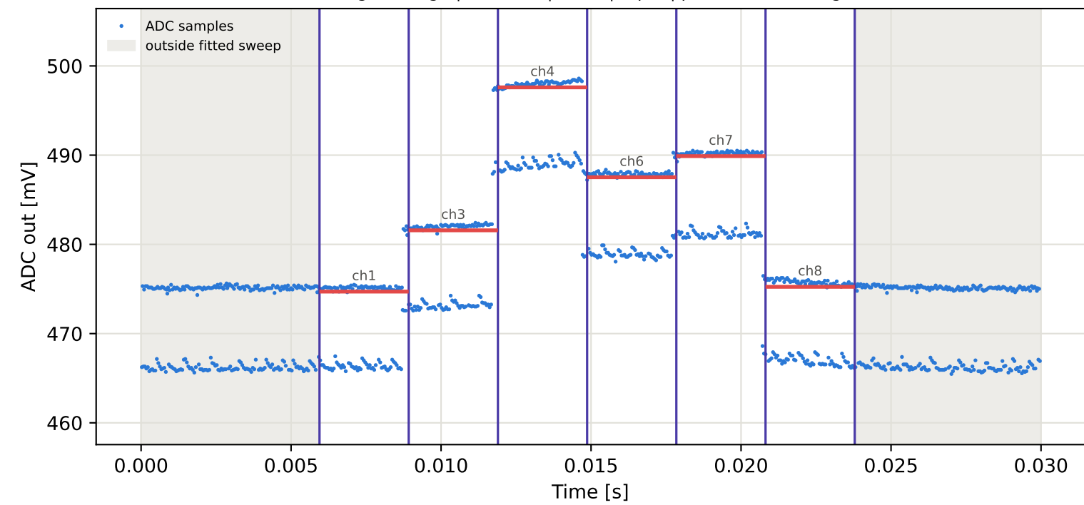
Tag4 &lt;- Tag8 | 945 MHz | run 0 | rep 1 | phase -66.72 deg
