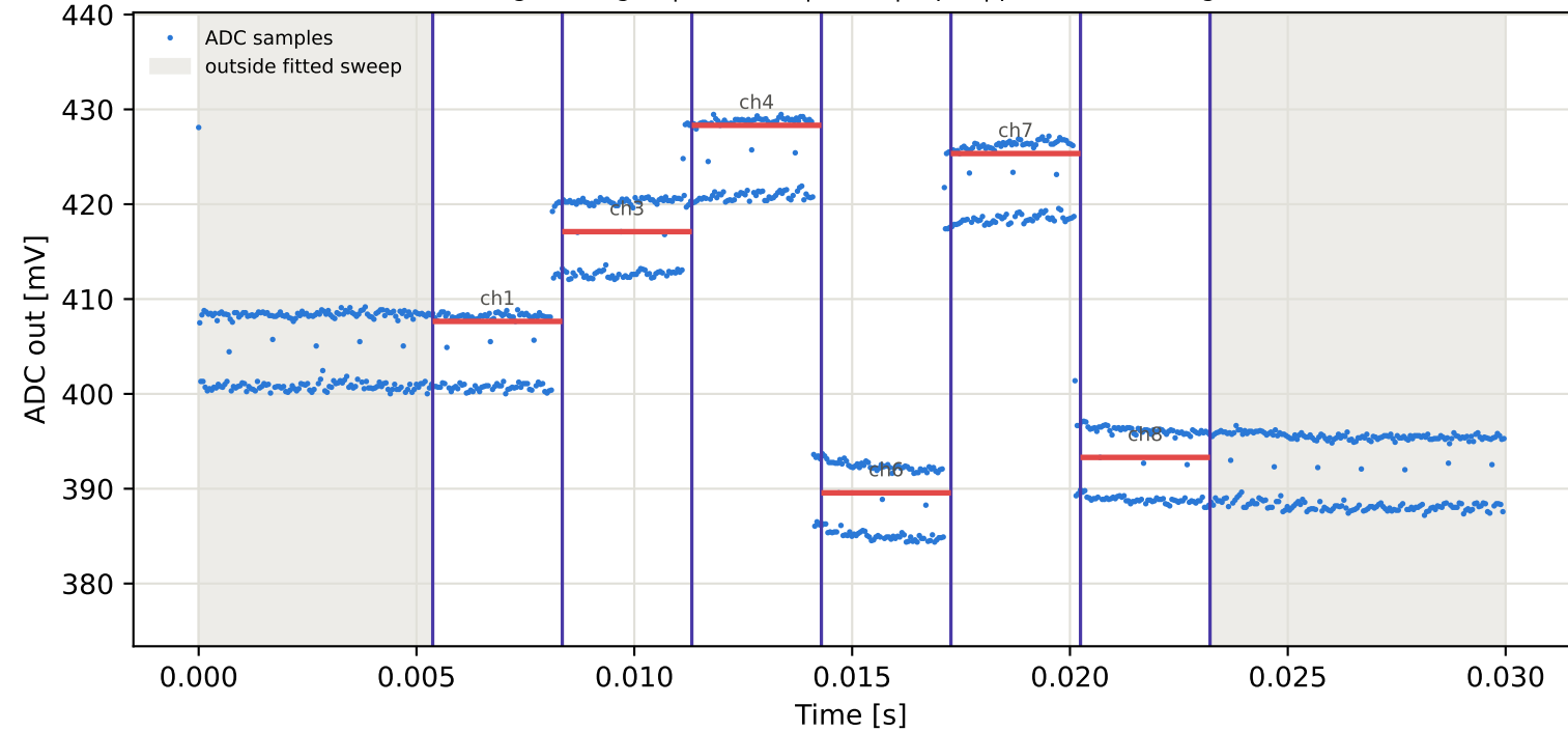
Tag5 &lt;- Tag2 | 965 MHz | run 0 | rep 1 | phase 89.08 deg
