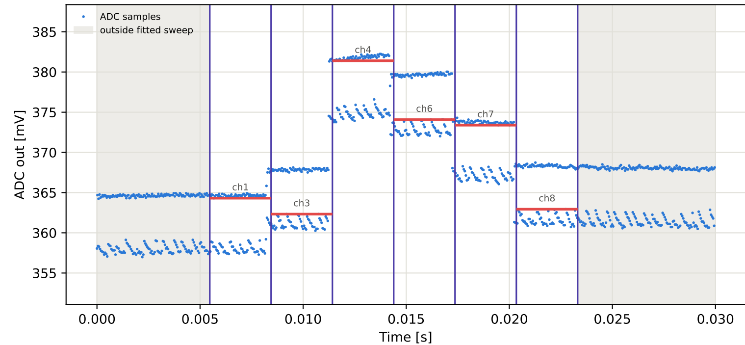
Tag10 &lt;- Tag5 | 965 MHz | run 0 | rep 1 | phase 78.13 deg
