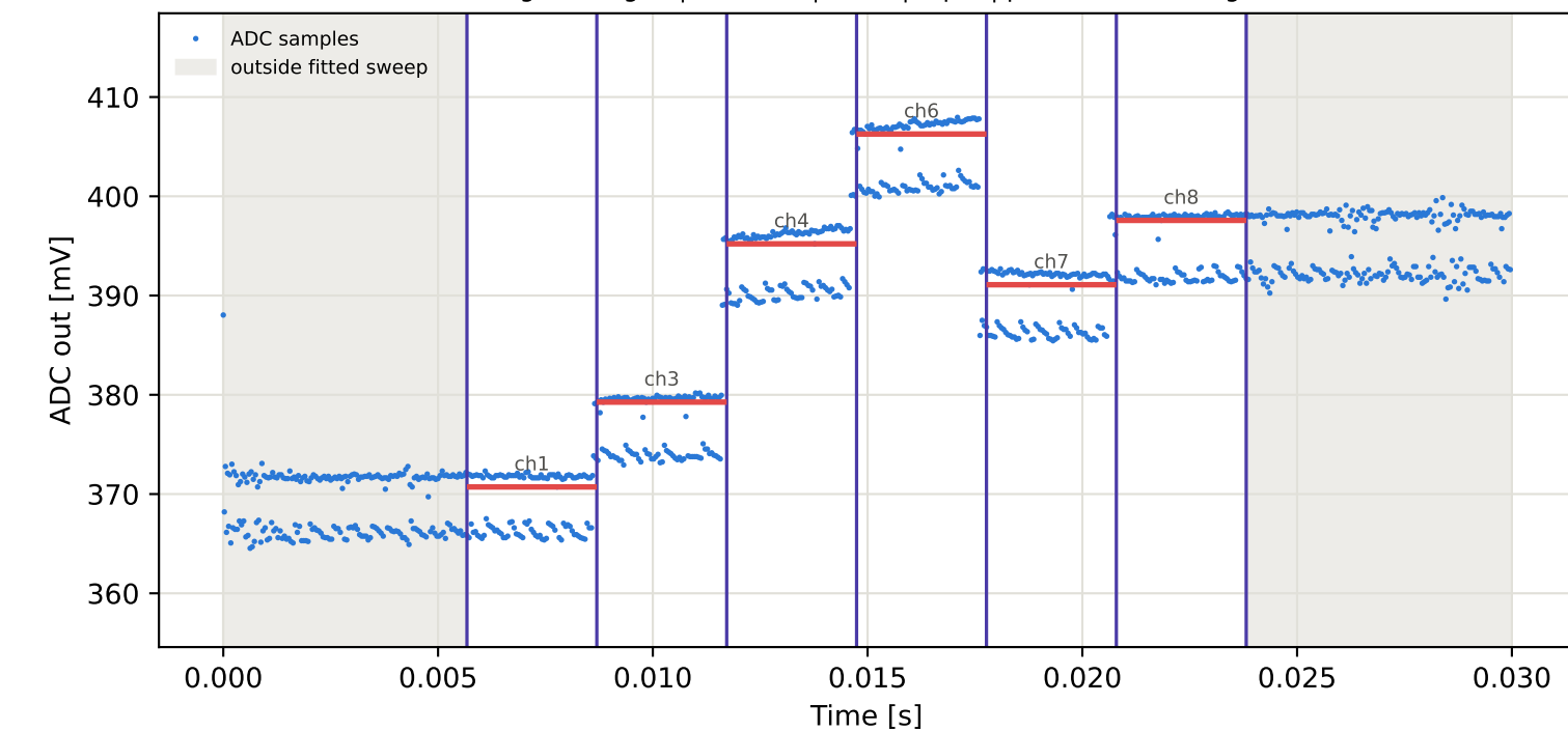
Tag9 &lt;- Tag16 | 875 MHz | run 0 | rep 1 | phase -140.07 deg
