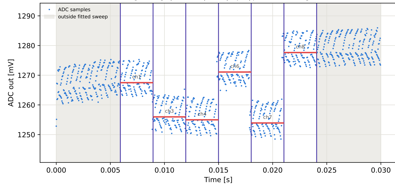
Tag9 &lt;- Tag10 | 875 MHz | run 0 | rep 1 | phase 104.50 deg
