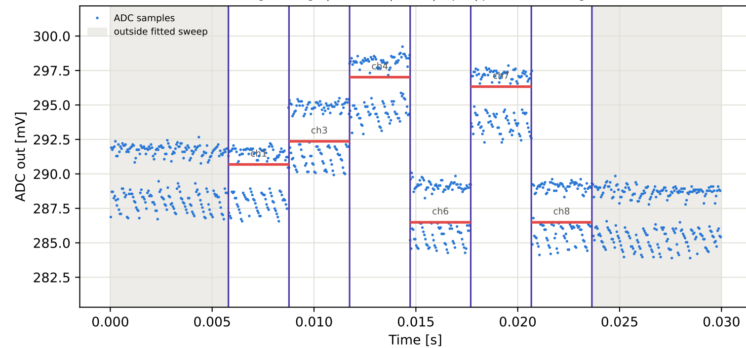
Tag3 &lt;- Tag10 | 975 MHz | run 0 | rep 1 | phase -38.84 deg
