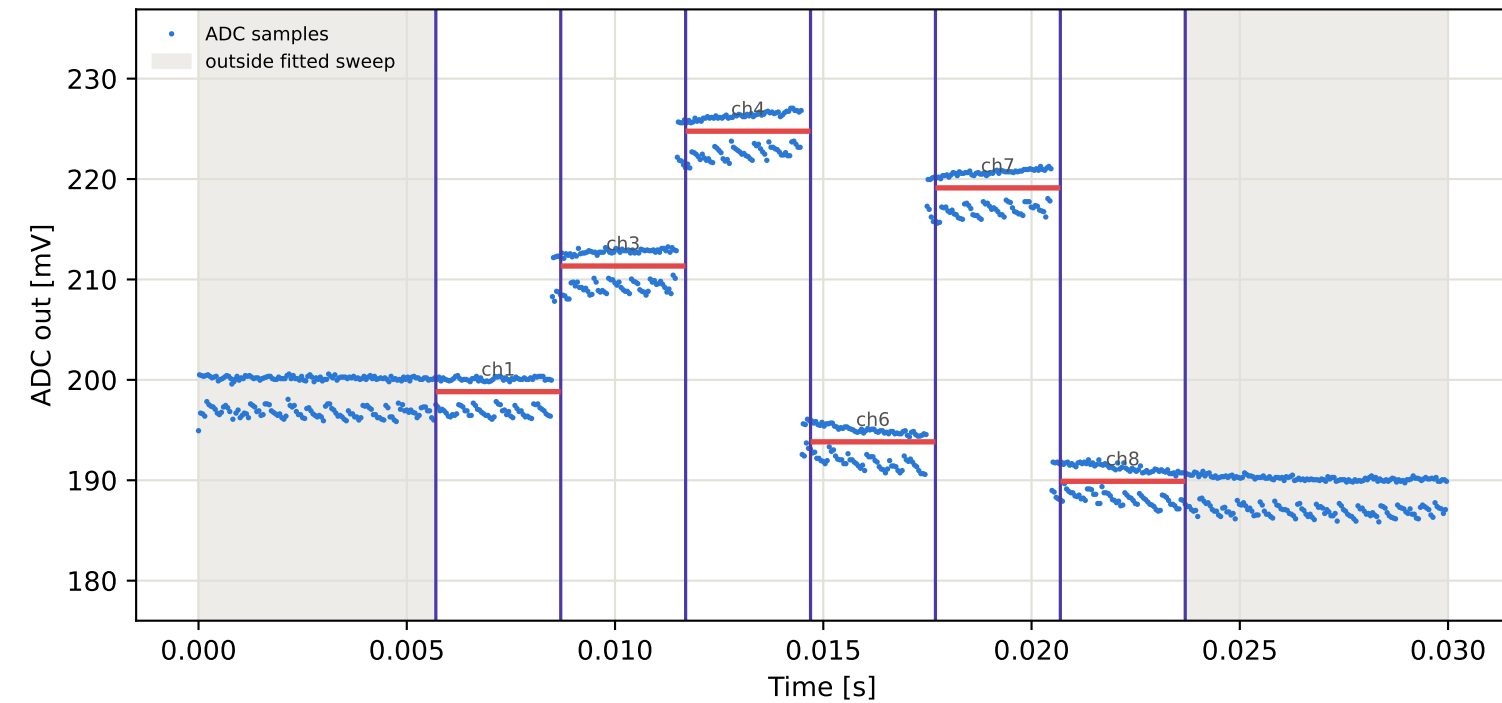
Tag4 &lt;- Tag2 | 955 MHz | run 0 | rep 1 | phase 161.36 deg
