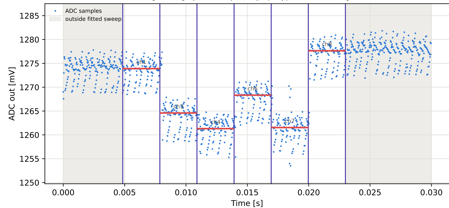
Tag8 &lt;- Tag7 | 875 MHz | run 0 | rep 1 | phase 17.14 deg
