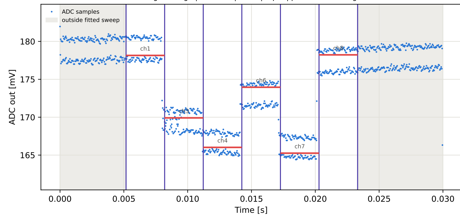
Tag4 &lt;- Tag8 | 845 MHz | run 0 | rep 1 | phase 112.42 deg
