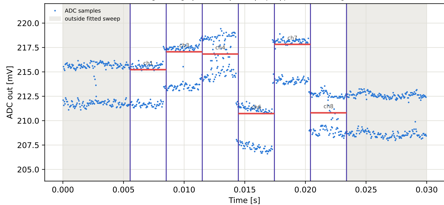
Tag6 &lt;- Tag4 | 935 MHz | run 0 | rep 1 | phase -33.38 deg
