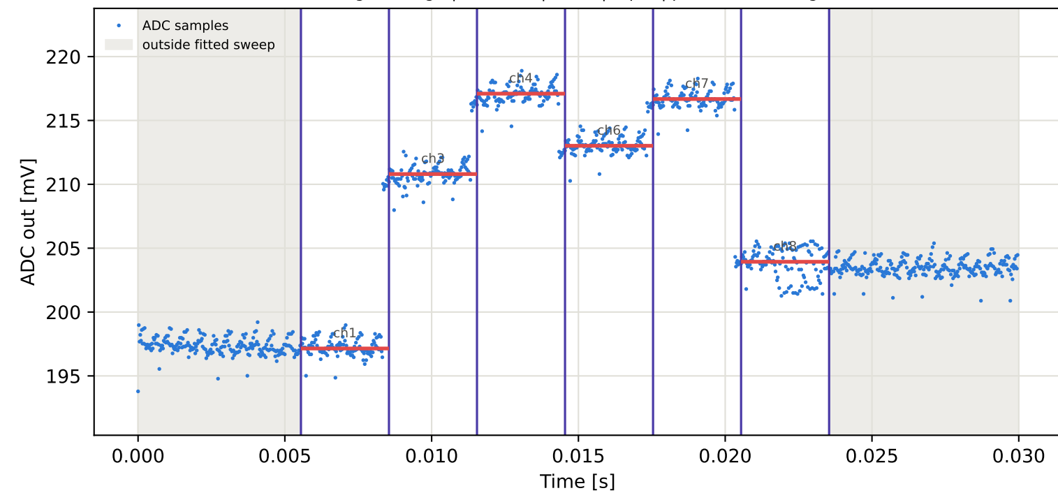
Tag9 &lt;- Tag6 | 855 MHz | run 0 | rep 1 | phase 2.86 deg
