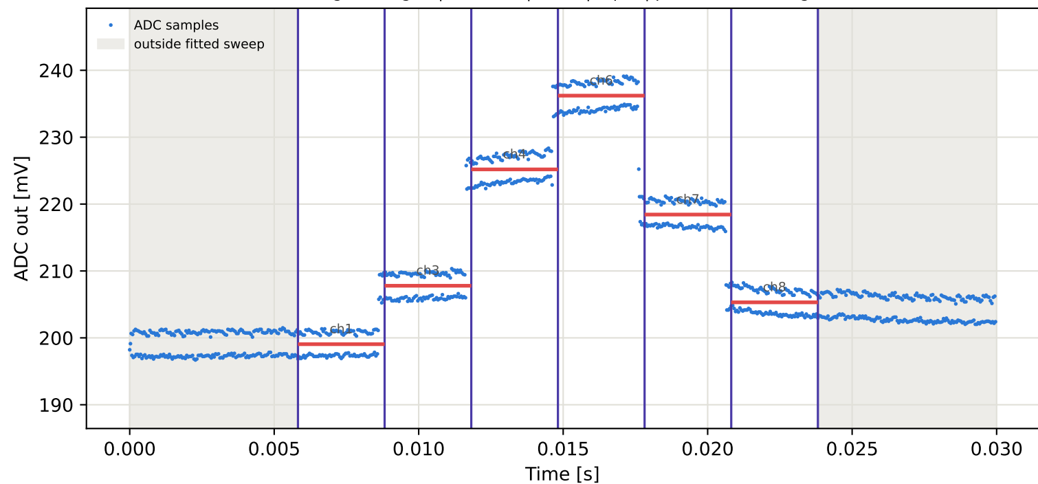
Tag4 &lt;- Tag16 | 915 MHz | run 0 | rep 1 | phase -54.96 deg
