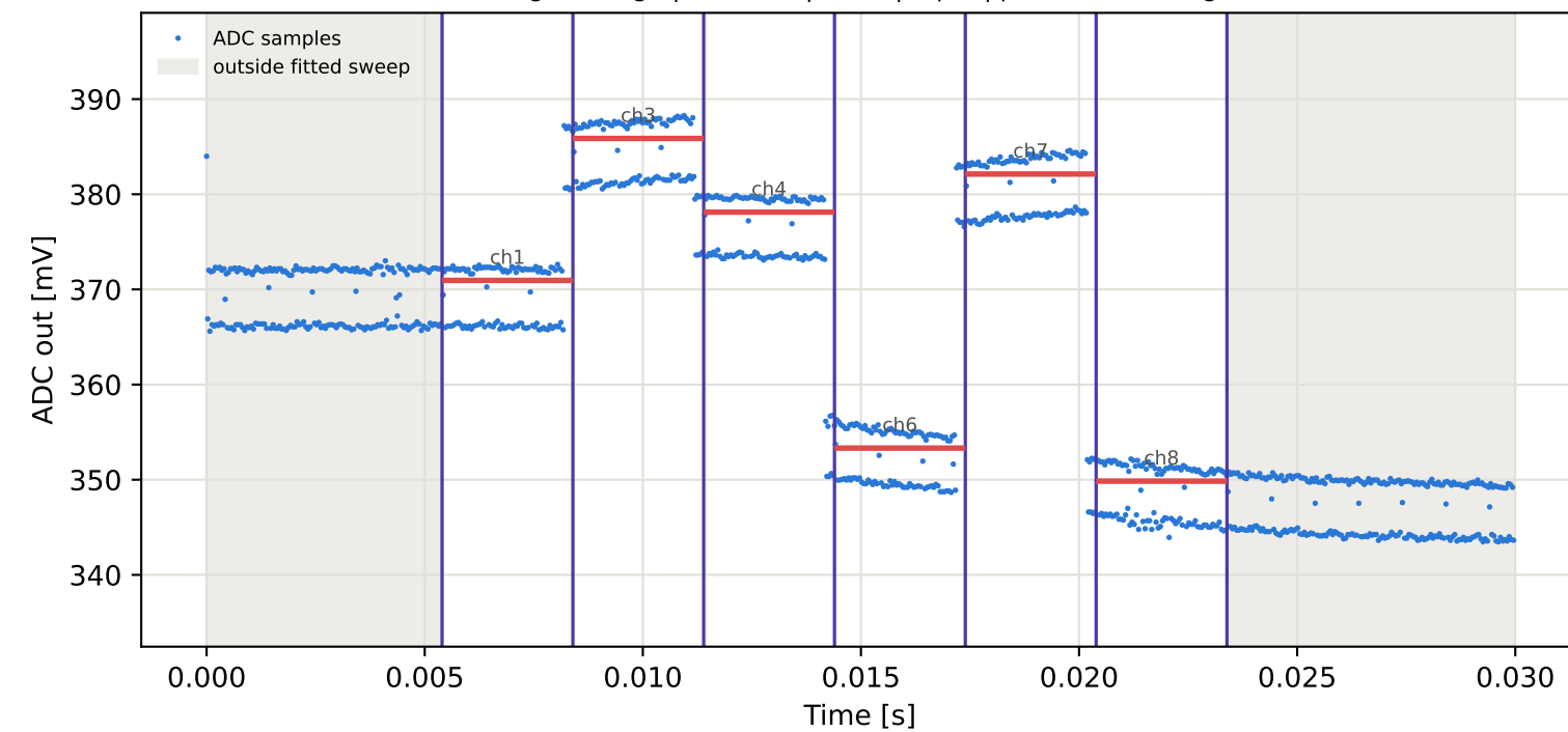
Tag4 &lt;- Tag9 | 875 MHz | run 0 | rep 1 | phase 17.32 deg
