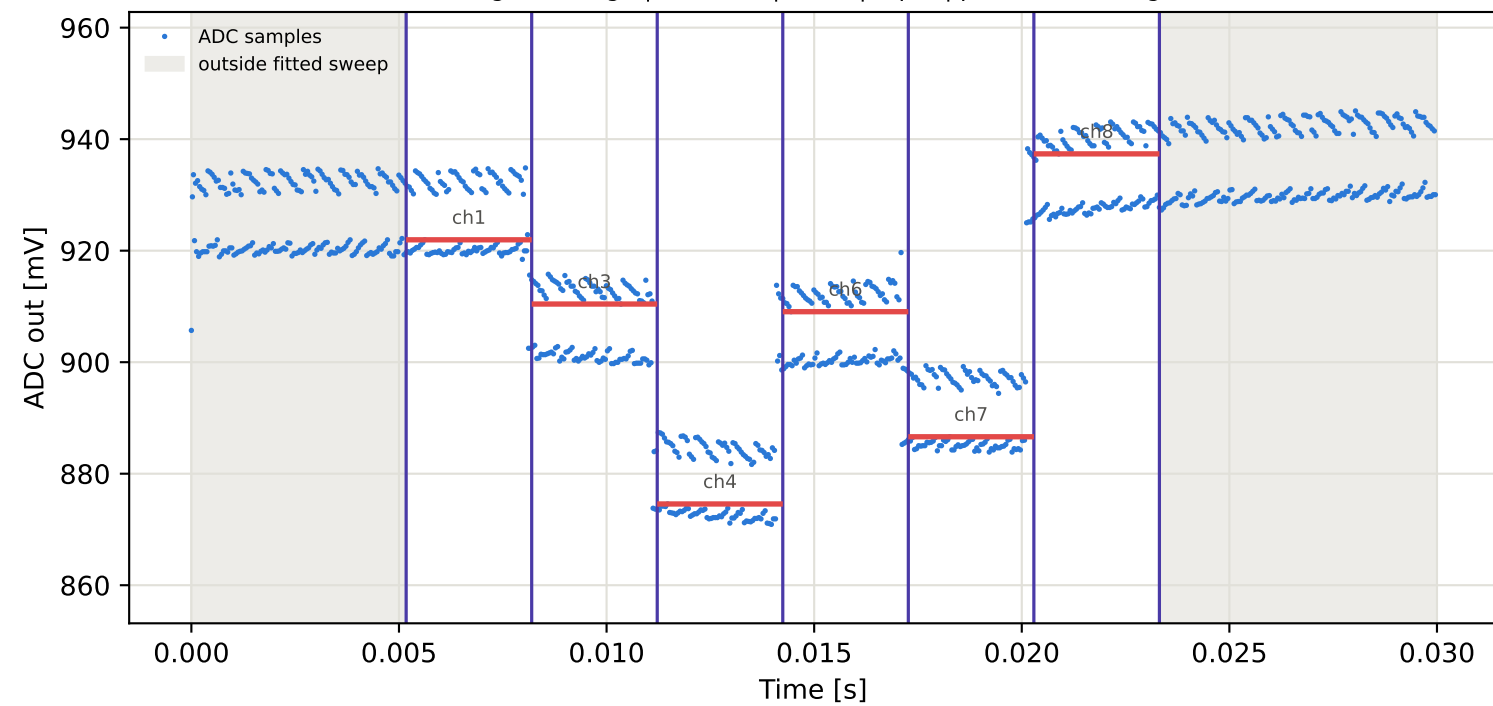
Tag10 &lt;- Tag8 | 925 MHz | run 0 | rep 1 | phase -48.91 deg
