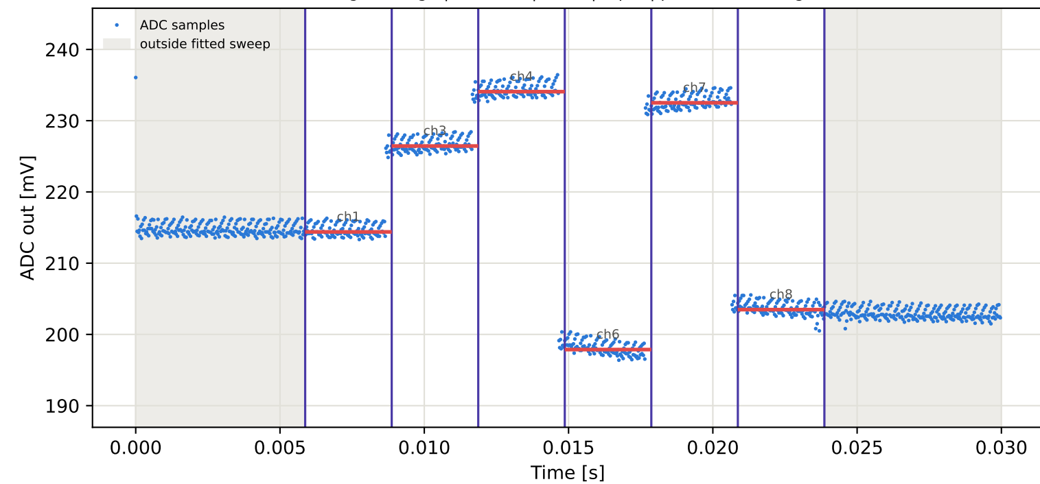
Tag1 &lt;- Tag8 | 985 MHz | run 0 | rep 1 | phase -22.18 deg
