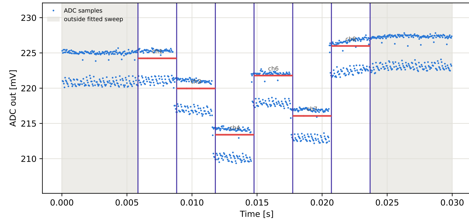
Tag1 &lt;- Tag9 | 935 MHz | run 0 | rep 1 | phase -75.09 deg
