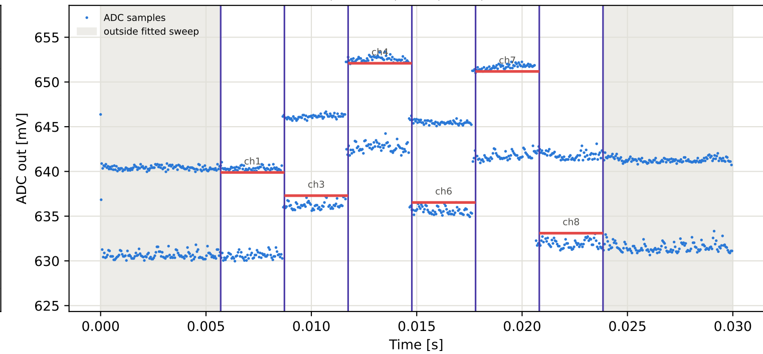
Tag16 &lt;- Tag7 | 835 MHz | run 0 | rep 1 | phase -71.90 deg
