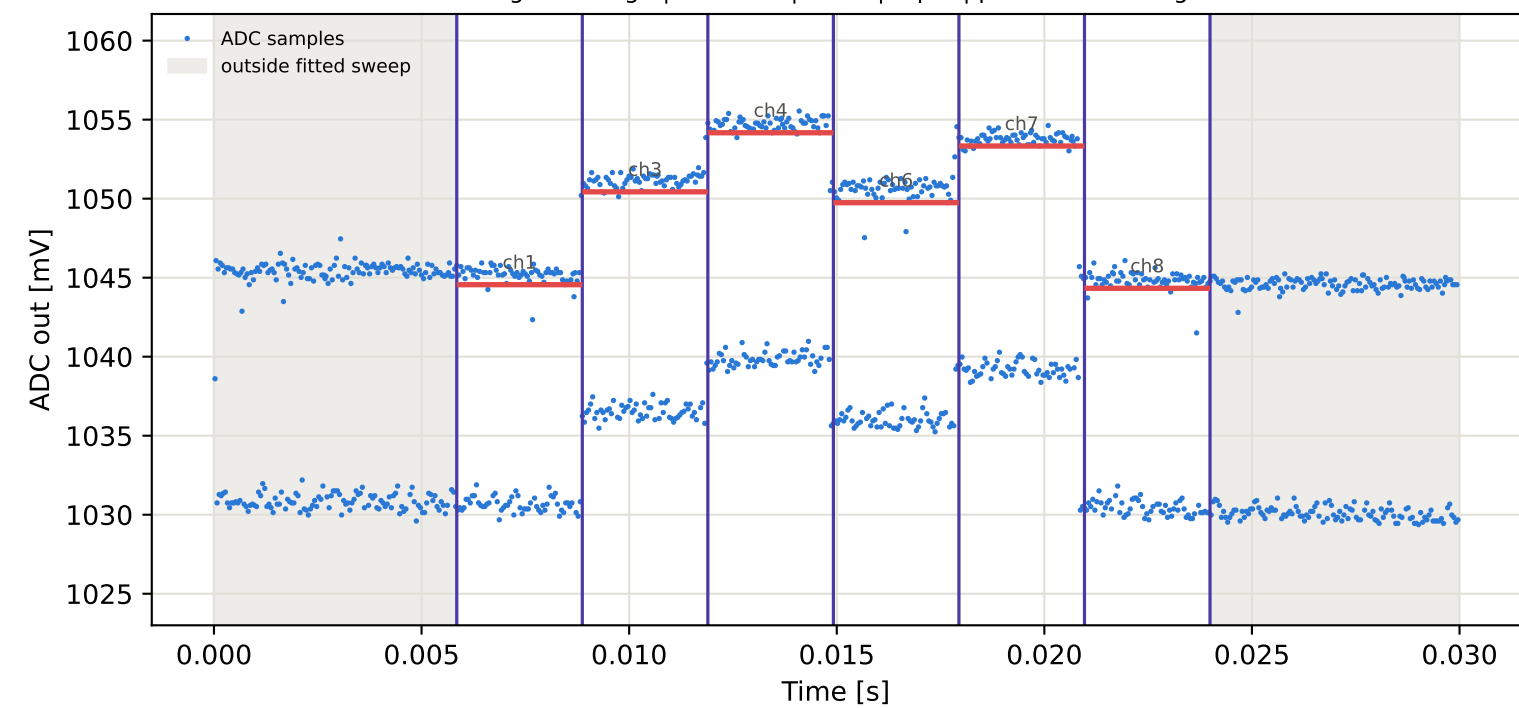
Tag2 &lt;- Tag10 | 875 MHz | run 0 | rep 1 | phase -141.99 deg
