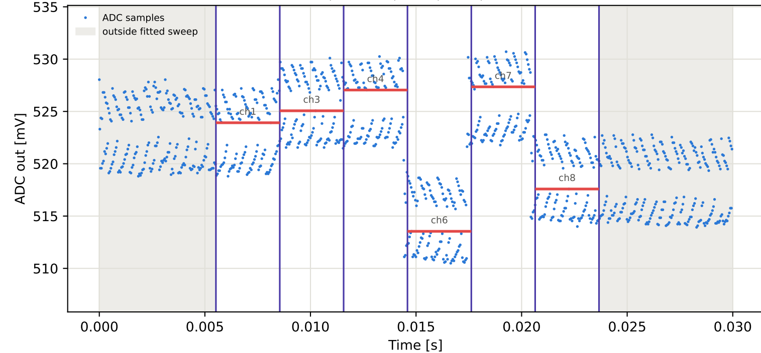
Tag15 &lt;- Tag6 | 955 MHz | run 0 | rep 1 | phase -20.71 deg
