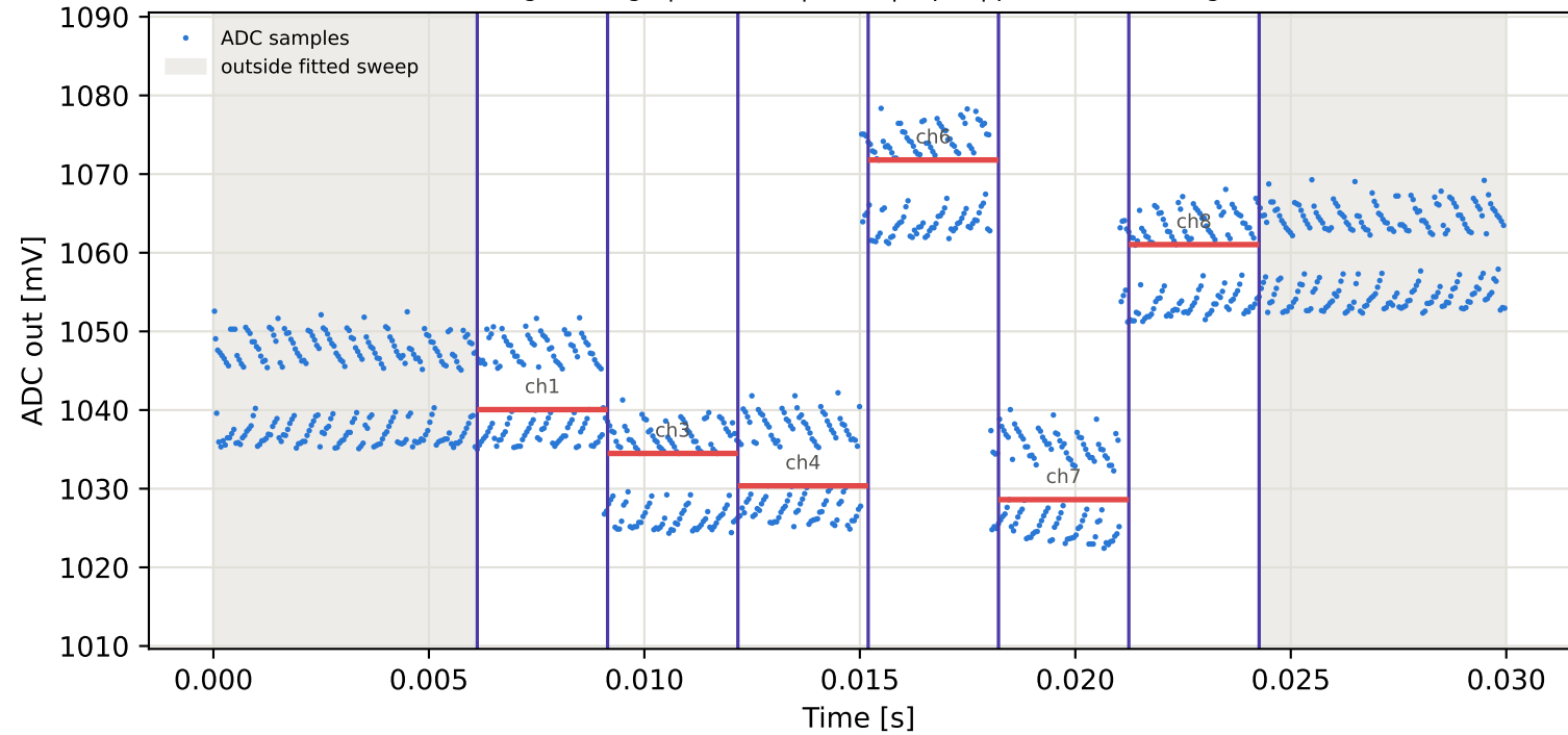
Tag8 &lt;- Tag10 | 955 MHz | run 0 | rep 1 | phase -12.37 deg
