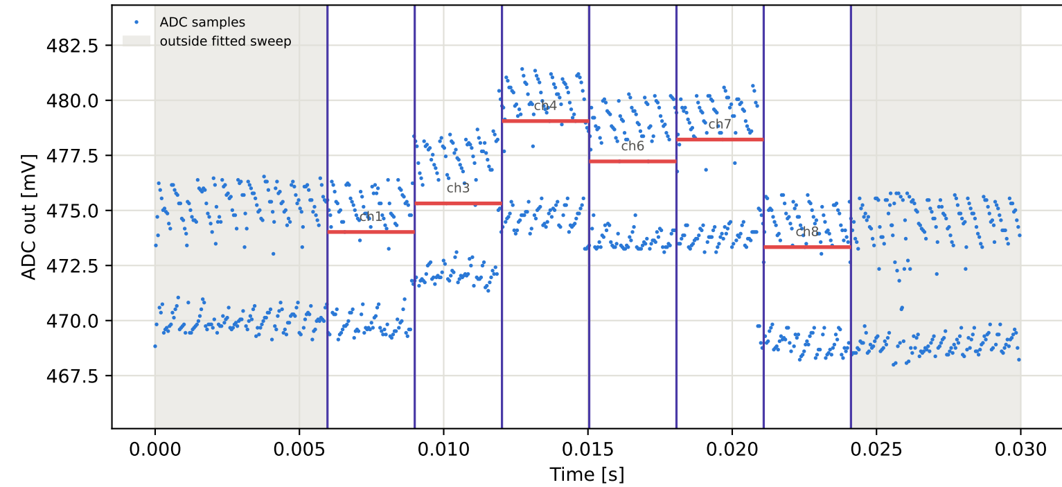
Tag6 &lt;- Tag4 | 835 MHz | run 0 | rep 1 | phase 175.84 deg
