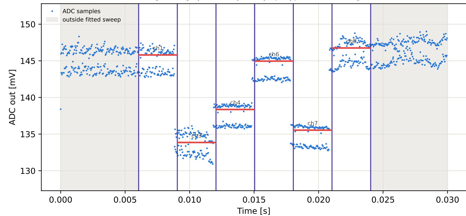
Tag9 &lt;- Tag6 | 825 MHz | run 0 | rep 1 | phase -75.67 deg
