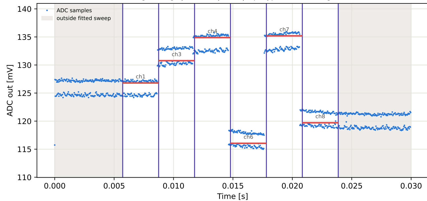
Tag4 &lt;- Tag8 | 985 MHz | run 0 | rep 1 | phase -84.58 deg
