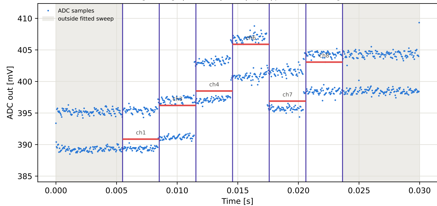
Tag9 &lt;- Tag15 | 875 MHz | run 0 | rep 1 | phase 80.69 deg
