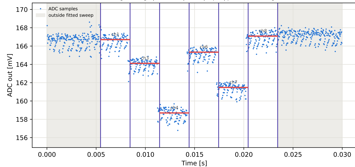
Tag4 &lt;- Tag9 | 975 MHz | run 0 | rep 1 | phase 118.75 deg
