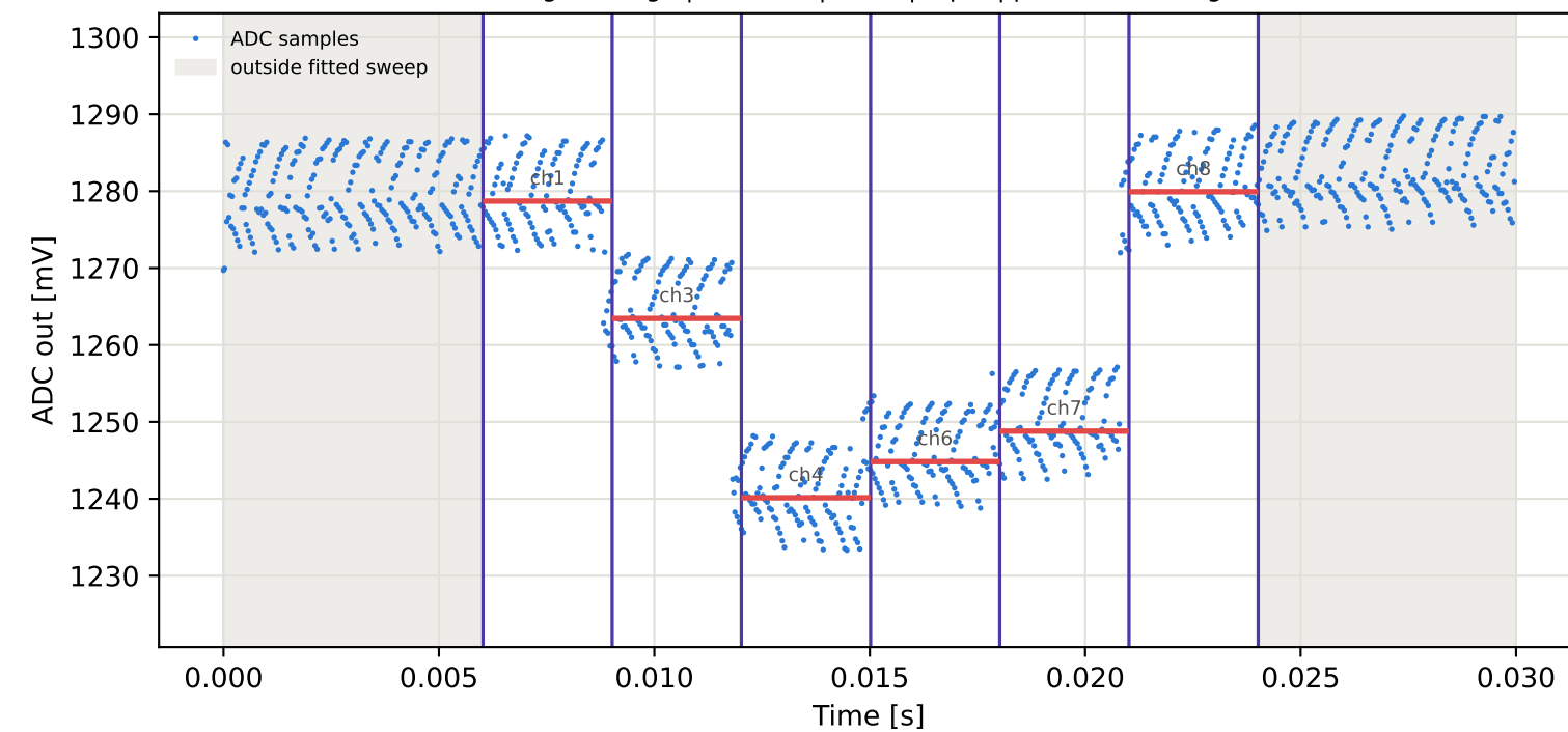
Tag8 &lt;- Tag6 | 915 MHz | run 0 | rep 1 | phase 66.28 deg
