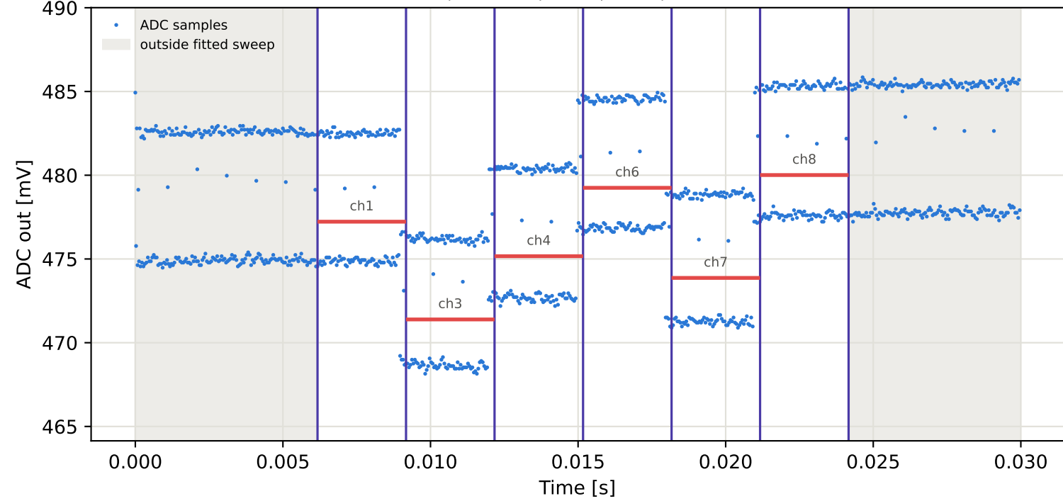
Tag6 &lt;- Tag4 | 835 MHz | run 0 | rep 1 | phase 175.84 deg
