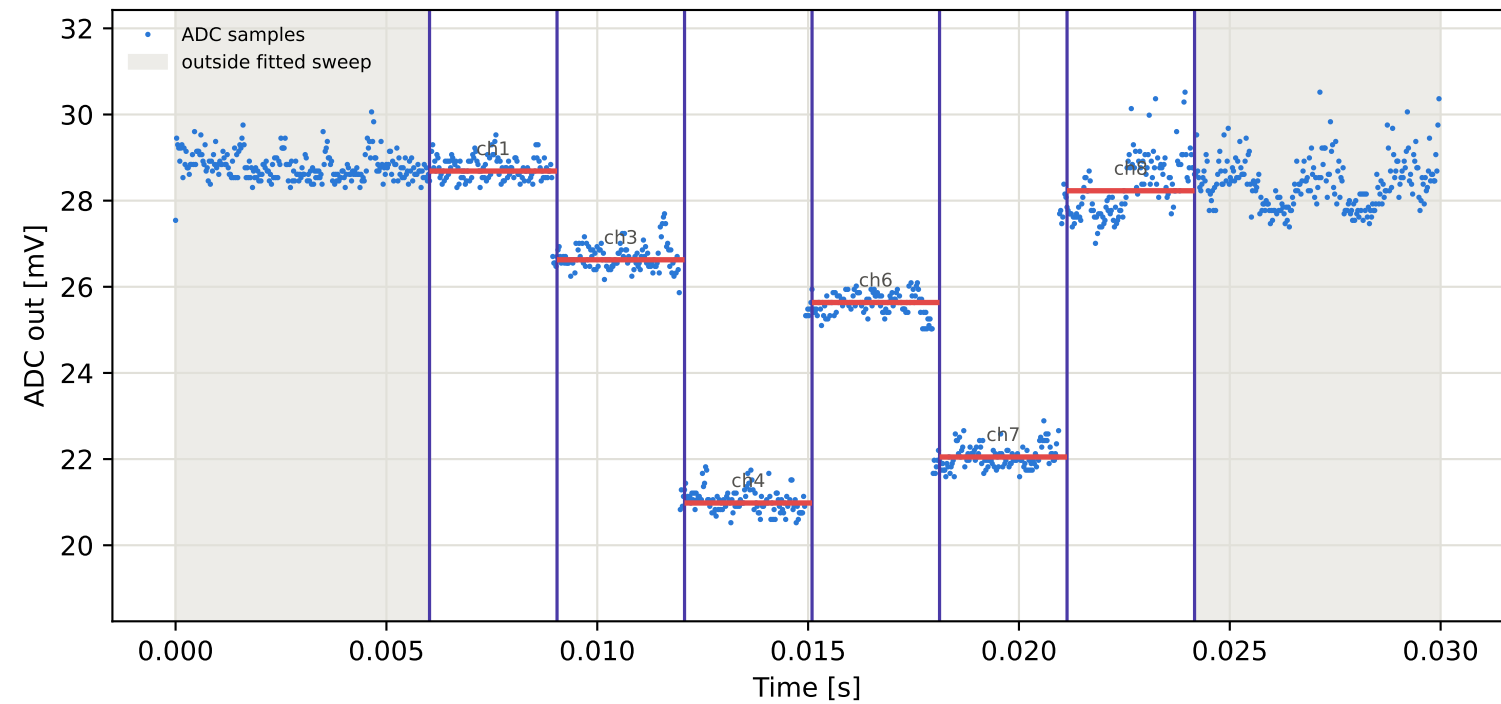
Tag9 &lt;- Tag15 | 805 MHz | run 0 | rep 1 | phase -113.98 deg
