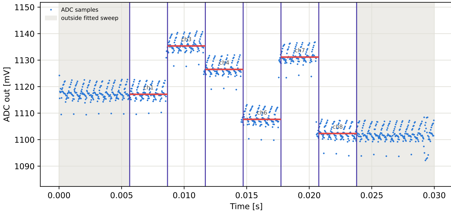
Tag7 &lt;- Tag15 | 865 MHz | run 0 | rep 1 | phase -13.81 deg
