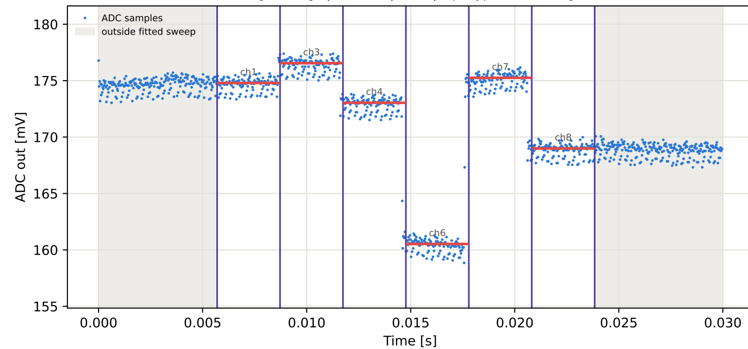
Tag3 &lt;- Tag6 | 955 MHz | run 0 | rep 1 | phase 93.03 deg
