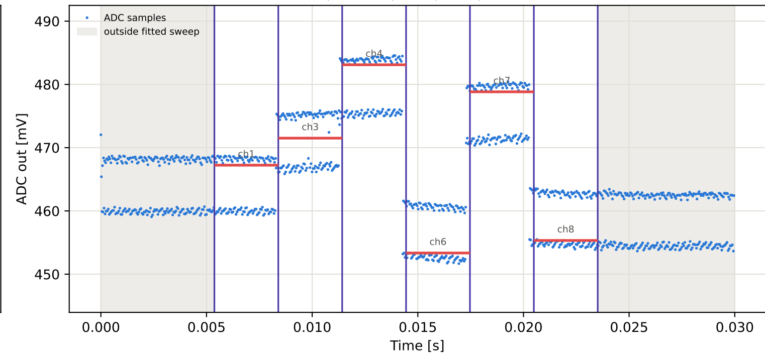
Tag1 &lt;- Tag4 | 975 MHz | run 0 | rep 1 | phase -49.94 deg
