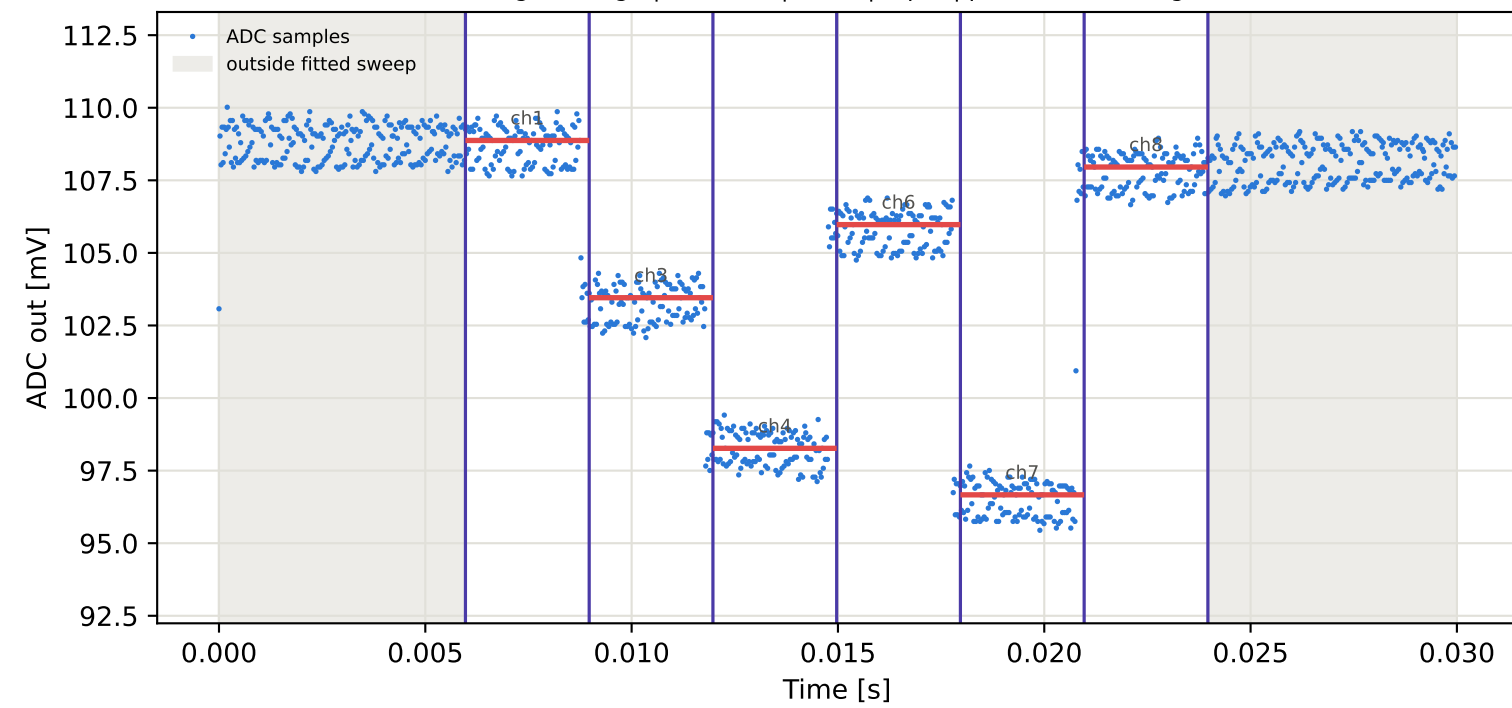
Tag7 &lt;- Tag1 | 795 MHz | run 0 | rep 1 | phase -41.49 deg
