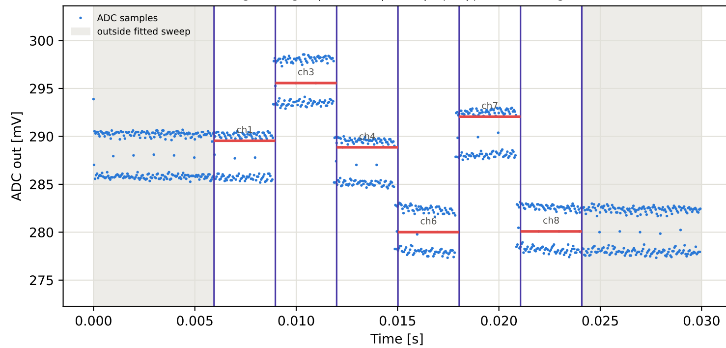
Tag1 &lt;- Tag16 | 835 MHz | run 0 | rep 1 | phase 97.41 deg
