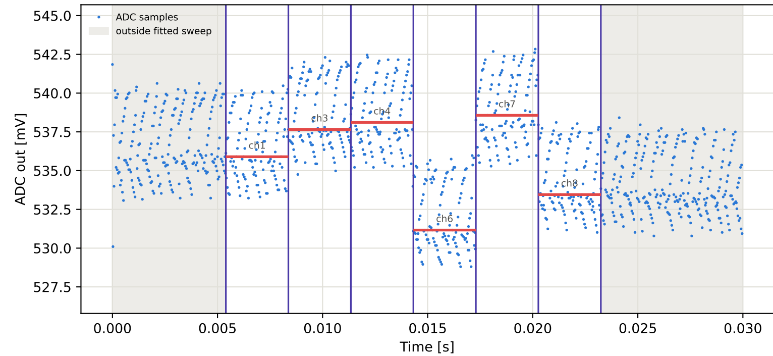
Tag2 &lt;- Tag16 | 955 MHz | run 0 | rep 1 | phase 174.96 deg
