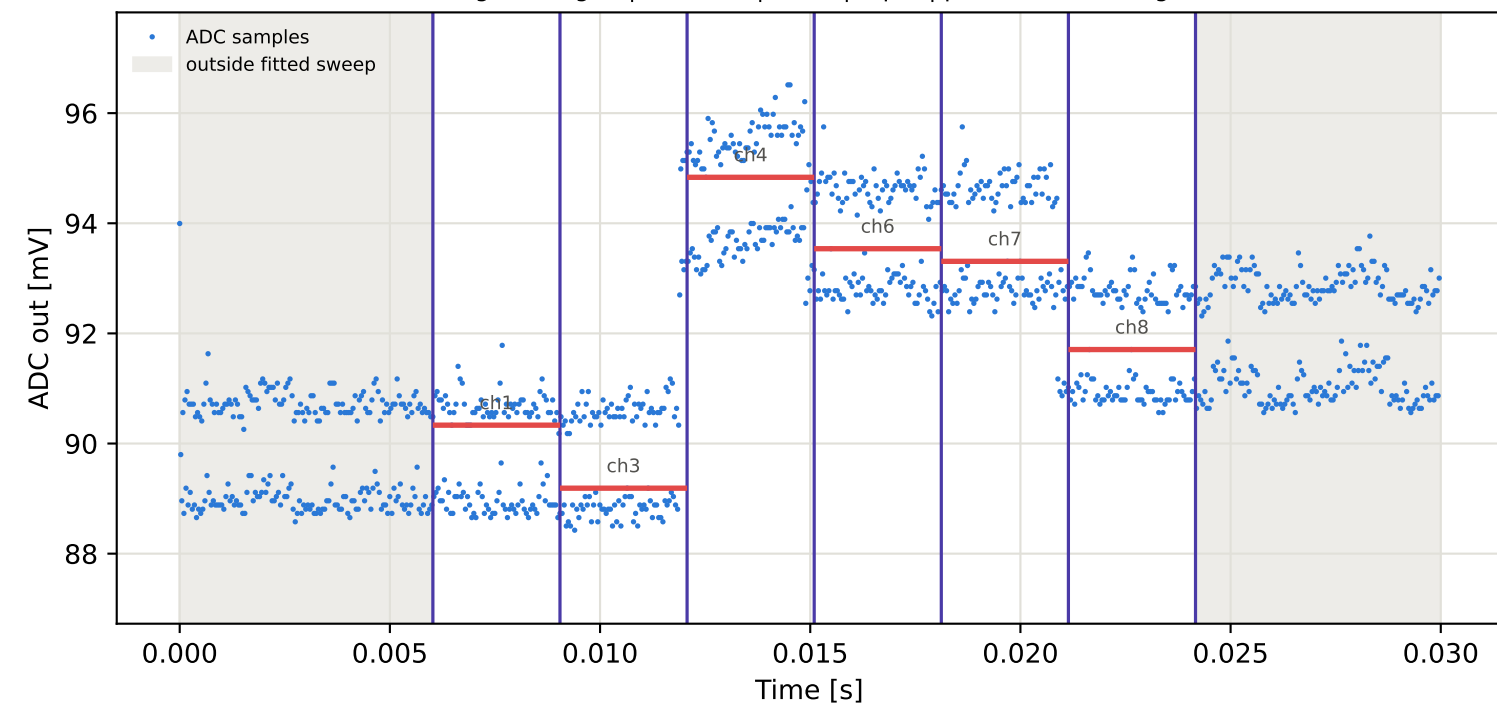
Tag2 &lt;- Tag16 | 805 MHz | run 0 | rep 1 | phase 130.47 deg
