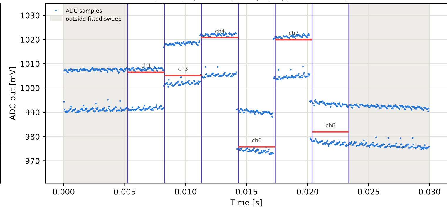
Tag9 &lt;- Tag6 | 925 MHz | run 0 | rep 1 | phase 104.27 deg
