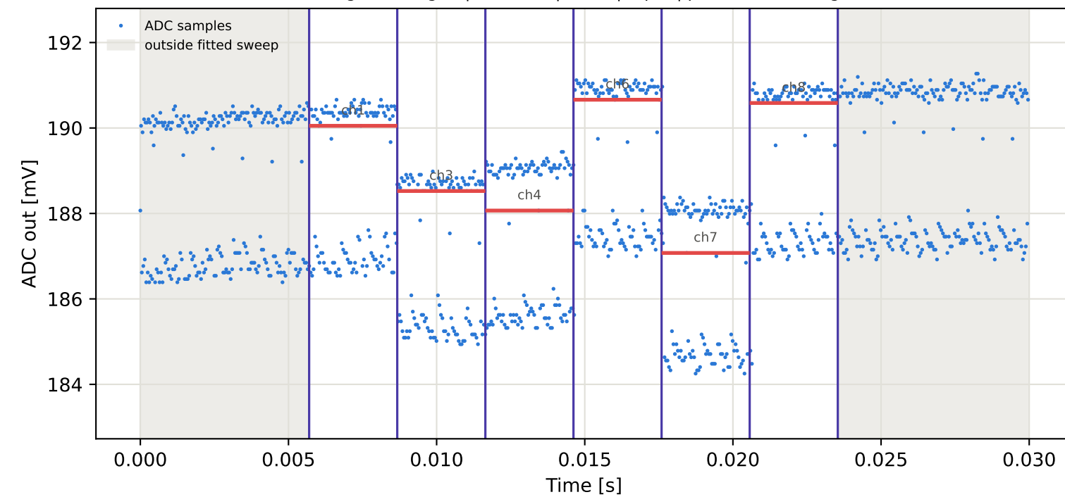
Tag10 &lt;- Tag2 | 785 MHz | run 0 | rep 1 | phase -143.66 deg
