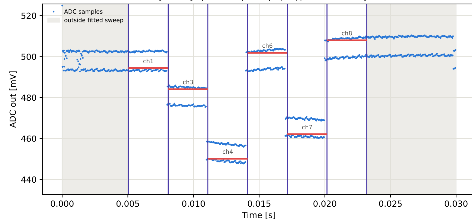
Tag9 &lt;- Tag7 | 975 MHz | run 0 | rep 1 | phase 100.71 deg
