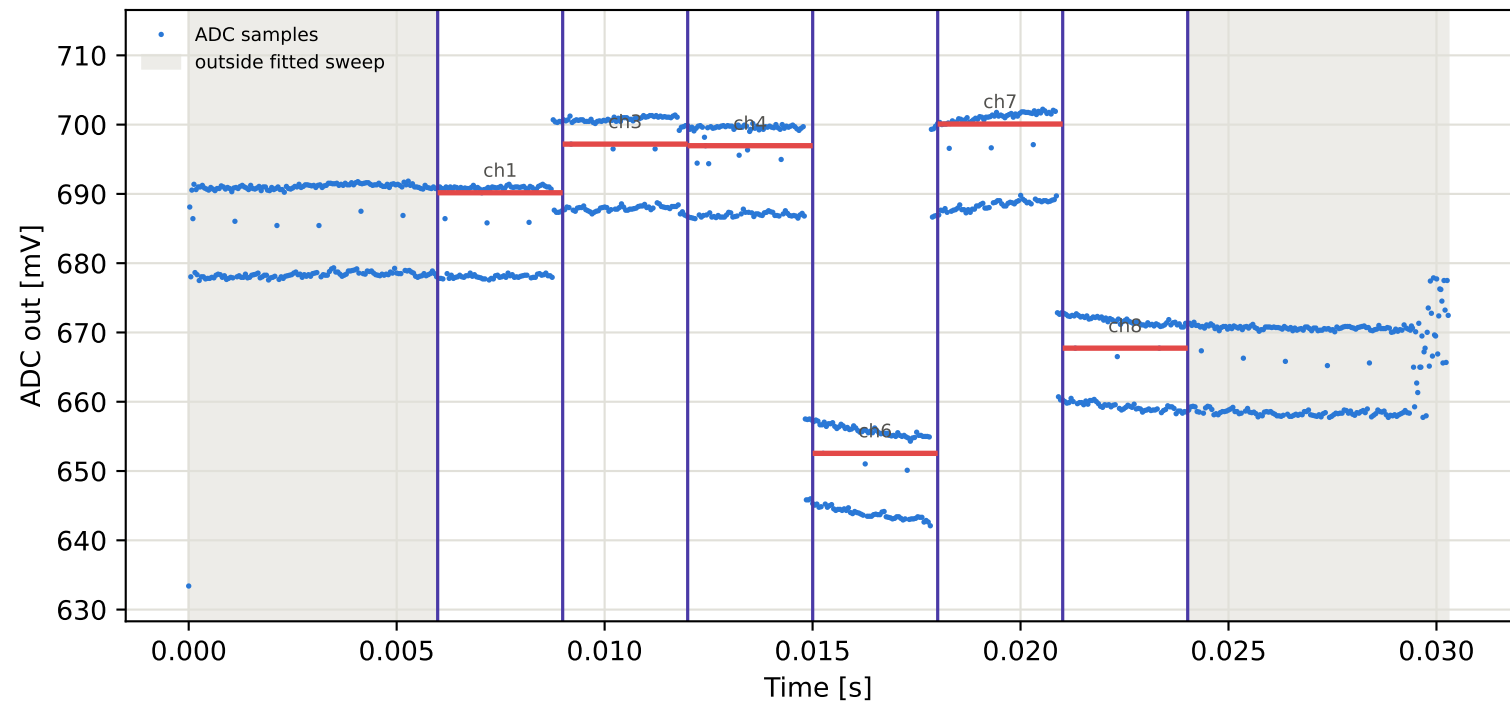
Tag9 &lt;- Tag6 | 935 MHz | run 0 | rep 1 | phase 42.50 deg
