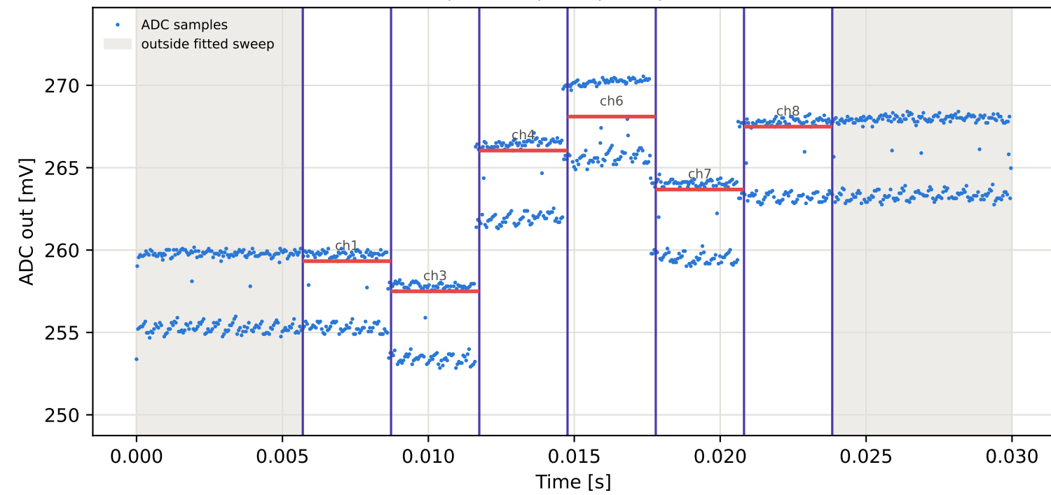
Tag10 &lt;- Tag5 | 845 MHz | run 0 | rep 1 | phase -142.16 deg
