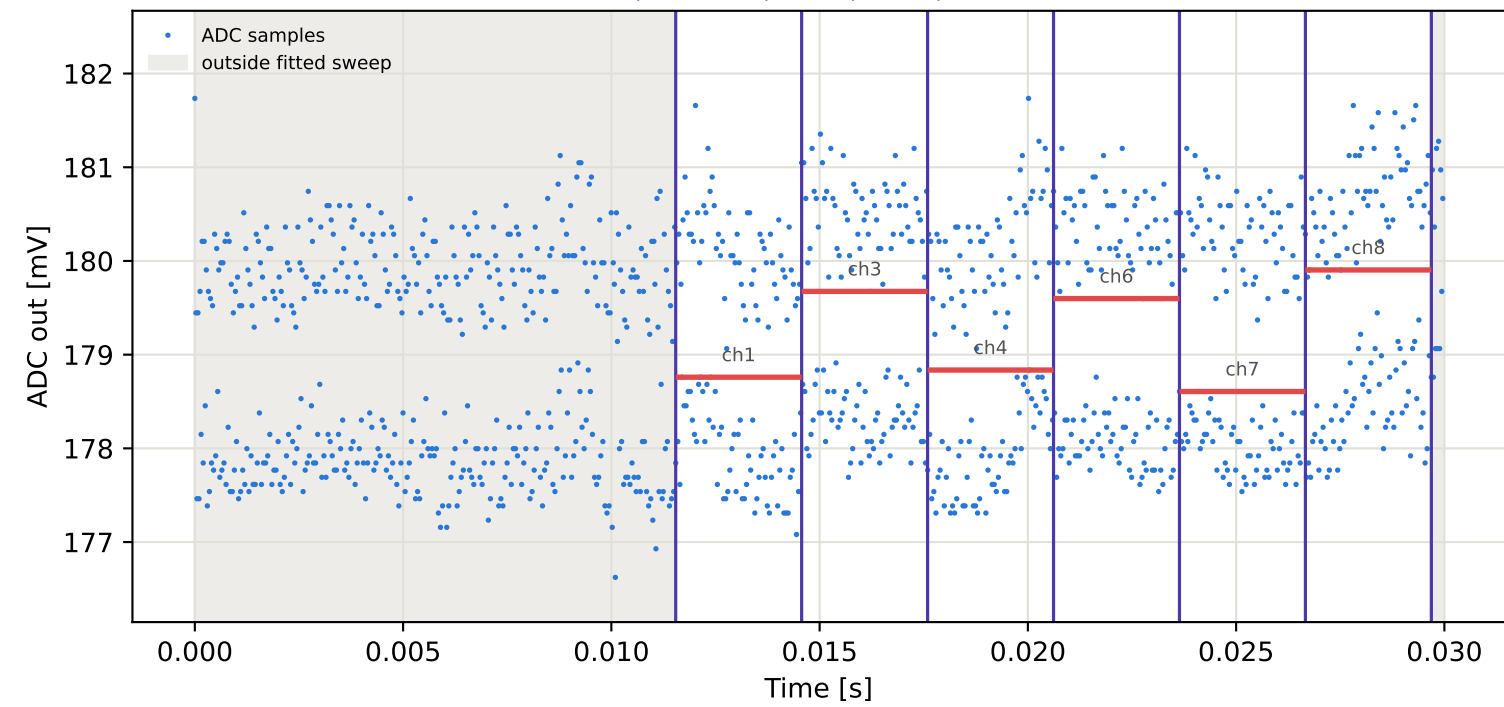
Tag3 &lt;- Tag2 | 995 MHz | run 0 | rep 1 | phase 123.30 deg
