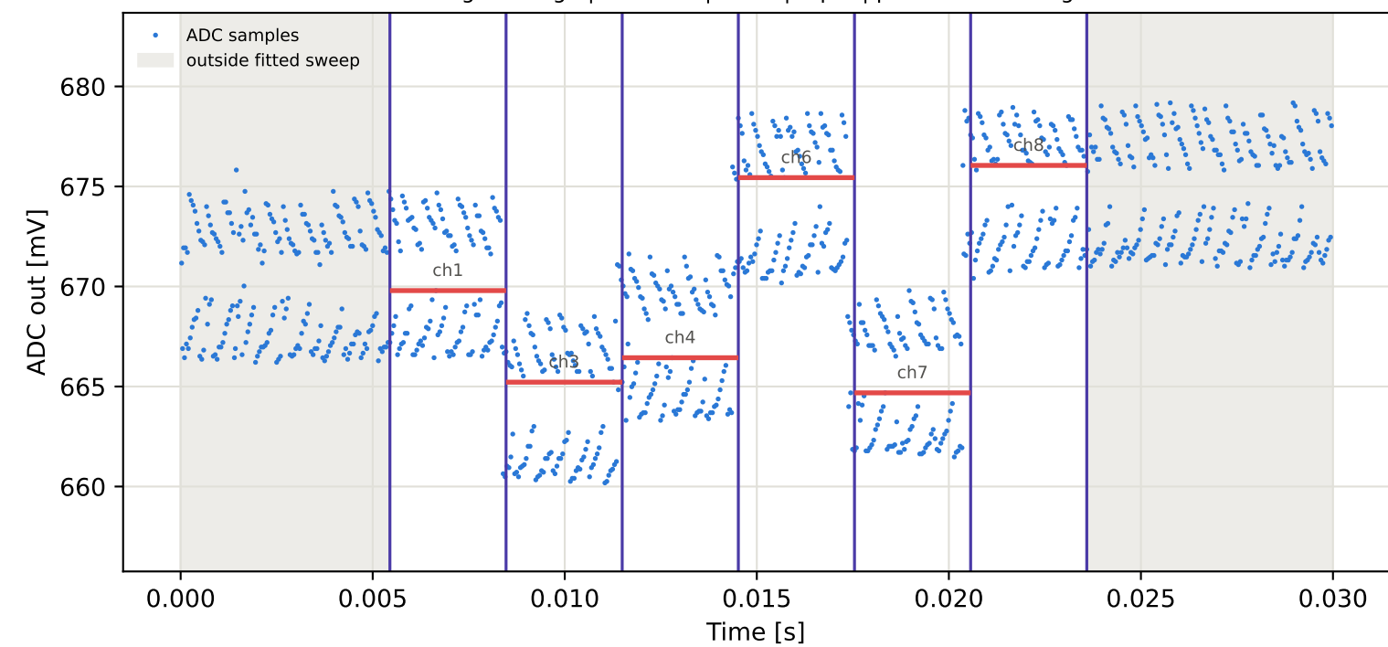
Tag8 &lt;- Tag10 | 835 MHz | run 0 | rep 1 | phase -139.28 deg
