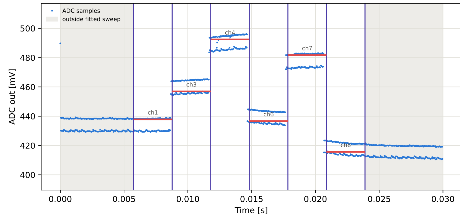
Tag5 &lt;- Tag4 | 935 MHz | run 0 | rep 1 | phase -74.30 deg
