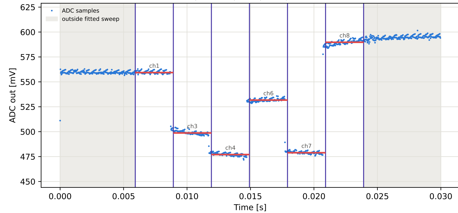
Tag5 &lt;- Tag3 | 875 MHz | run 0 | rep 1 | phase 109.62 deg
