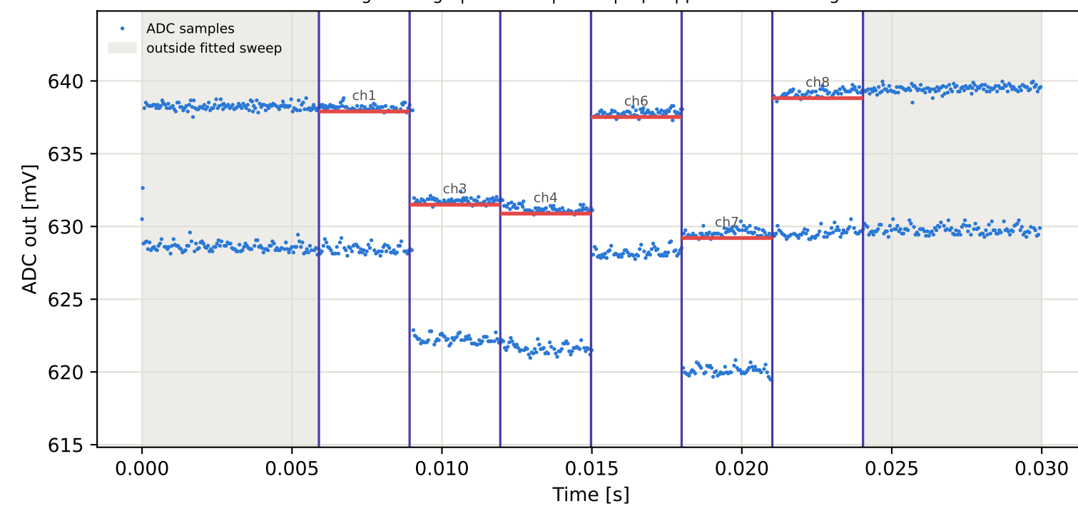
Tag8 &lt;- Tag15 | 835 MHz | run 0 | rep 1 | phase 4.54 deg
