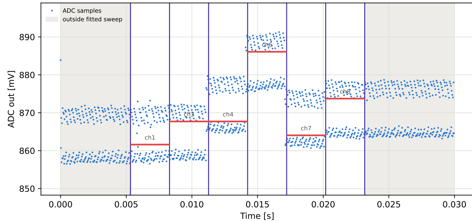
Tag3 &lt;- Tag9 | 925 MHz | run 0 | rep 1 | phase -65.14 deg
