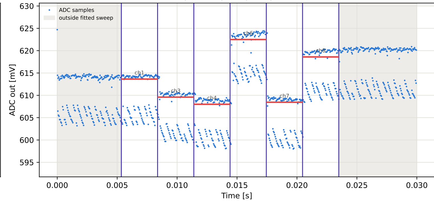
Tag7 &lt;- Tag6 | 935 MHz | run 0 | rep 1 | phase 154.61 deg
