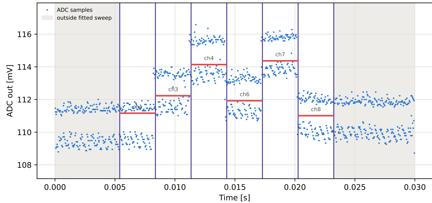
Tag5 &lt;- Tag8 | 795 MHz | run 0 | rep 1 | phase 144.54 deg
