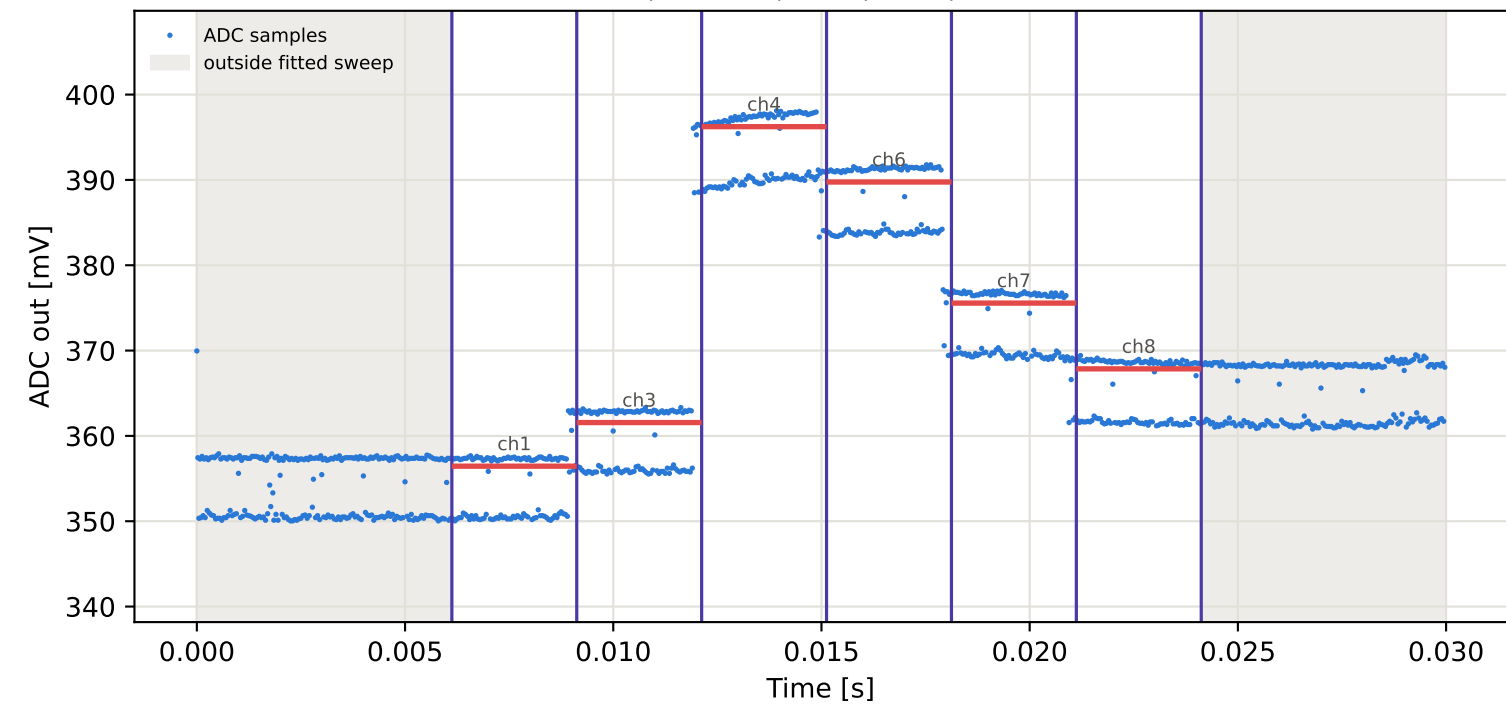
Tag16 &lt;- Tag15 | 995 MHz | run 0 | rep 1 | phase -132.92 deg
