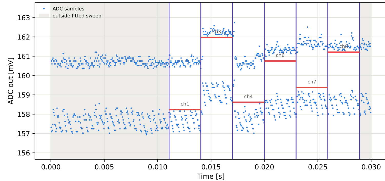
Tag6 &lt;- Tag4 | 955 MHz | run 0 | rep 1 | phase 38.39 deg
