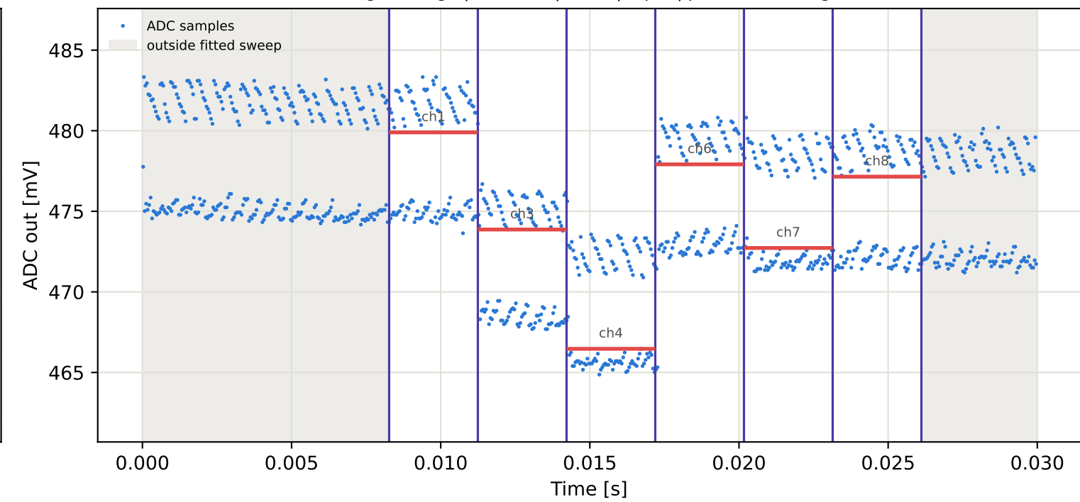
Tag9 &lt;- Tag6 | 975 MHz | run 0 | rep 1 | phase 107.37 deg
