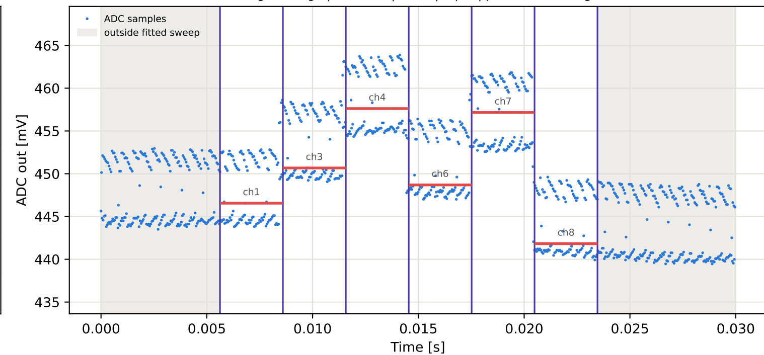
Tag6 &lt;- Tag5 | 915 MHz | run 0 | rep 1 | phase -80.47 deg
