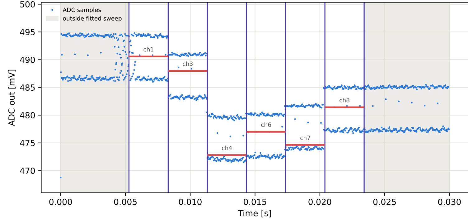
Tag6 &lt;- Tag5 | 835 MHz | run 0 | rep 1 | phase -150.19 deg
