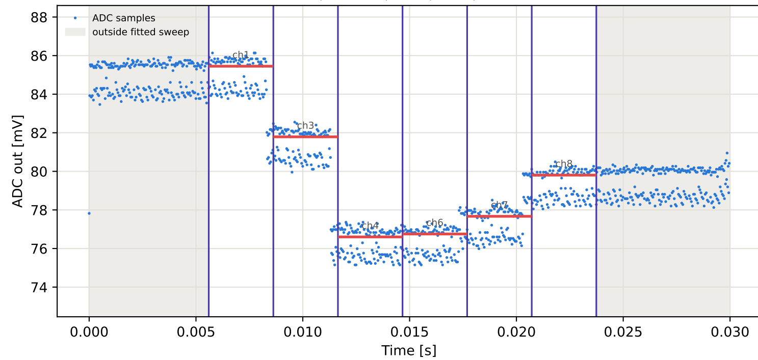
Tag1 &lt;- Tag3 | 845 MHz | run 0 | rep 1 | phase 61.07 deg
