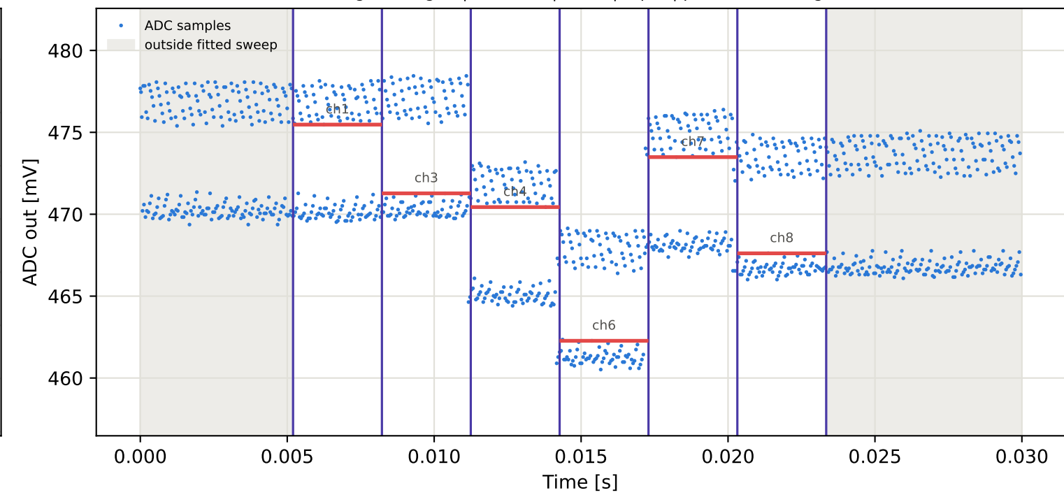
Tag1 &lt;- Tag2 | 975 MHz | run 0 | rep 1 | phase -128.67 deg
