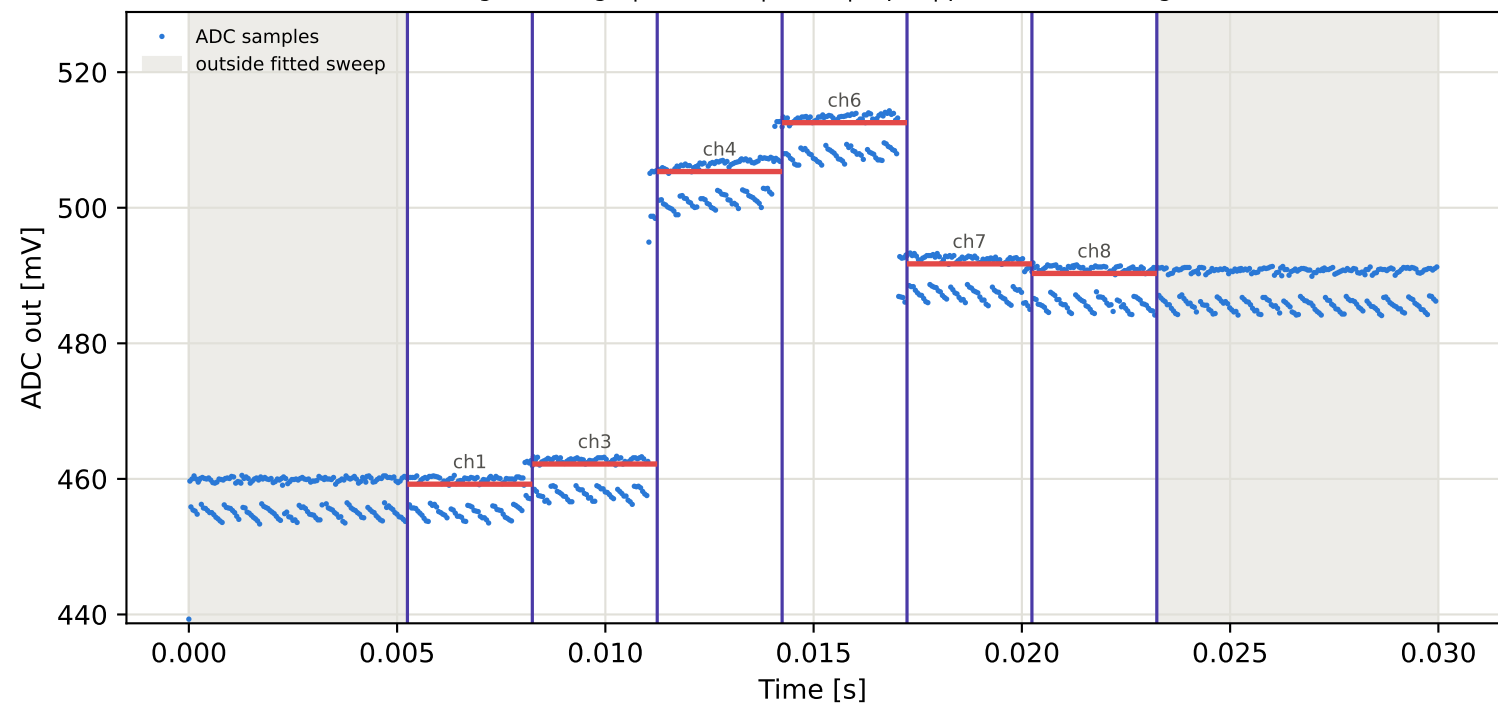
Tag10 &lt;- Tag9 | 855 MHz | run 0 | rep 1 | phase 17.26 deg
