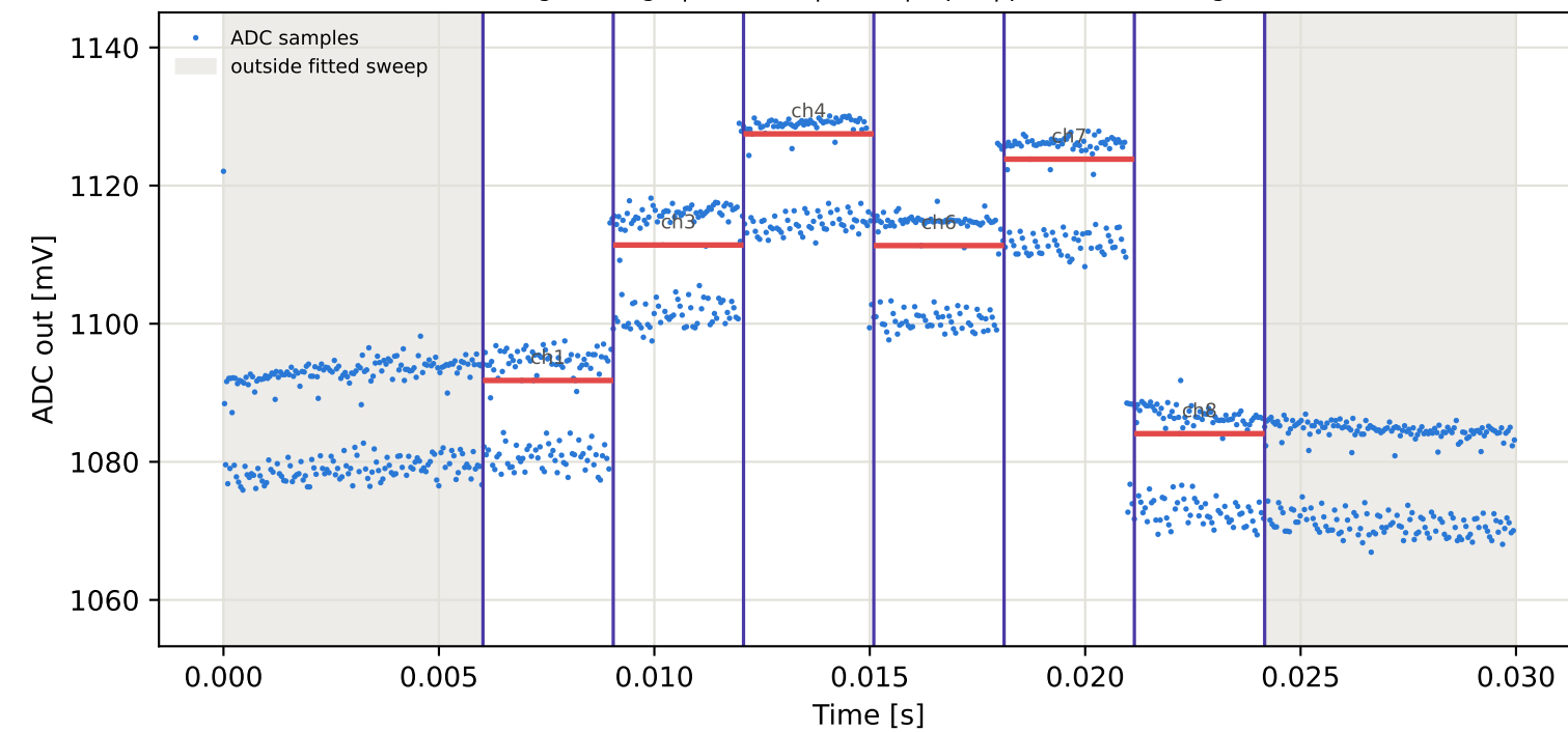
Tag3 &lt;- Tag6 | 885 MHz | run 0 | rep 1 | phase -42.60 deg
