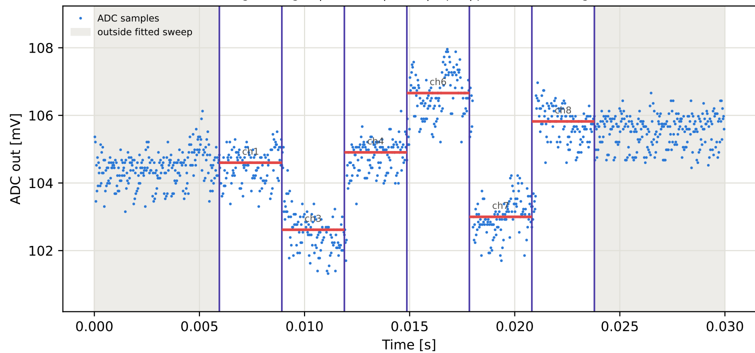
Tag5 &lt;- Tag2 | 775 MHz | run 0 | rep 1 | phase 0.90 deg
