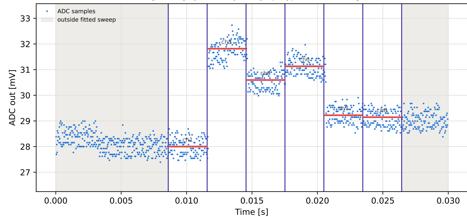
Tag4 &lt;- Tag8 | 785 MHz | run 0 | rep 1 | phase -59.23 deg
