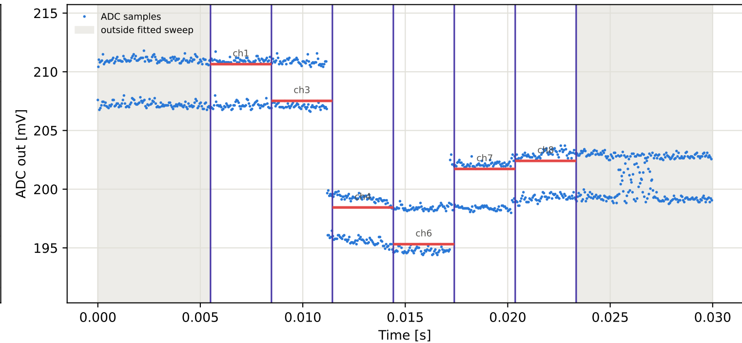
Tag9 &lt;- Tag2 | 845 MHz | run 0 | rep 1 | phase -82.78 deg
