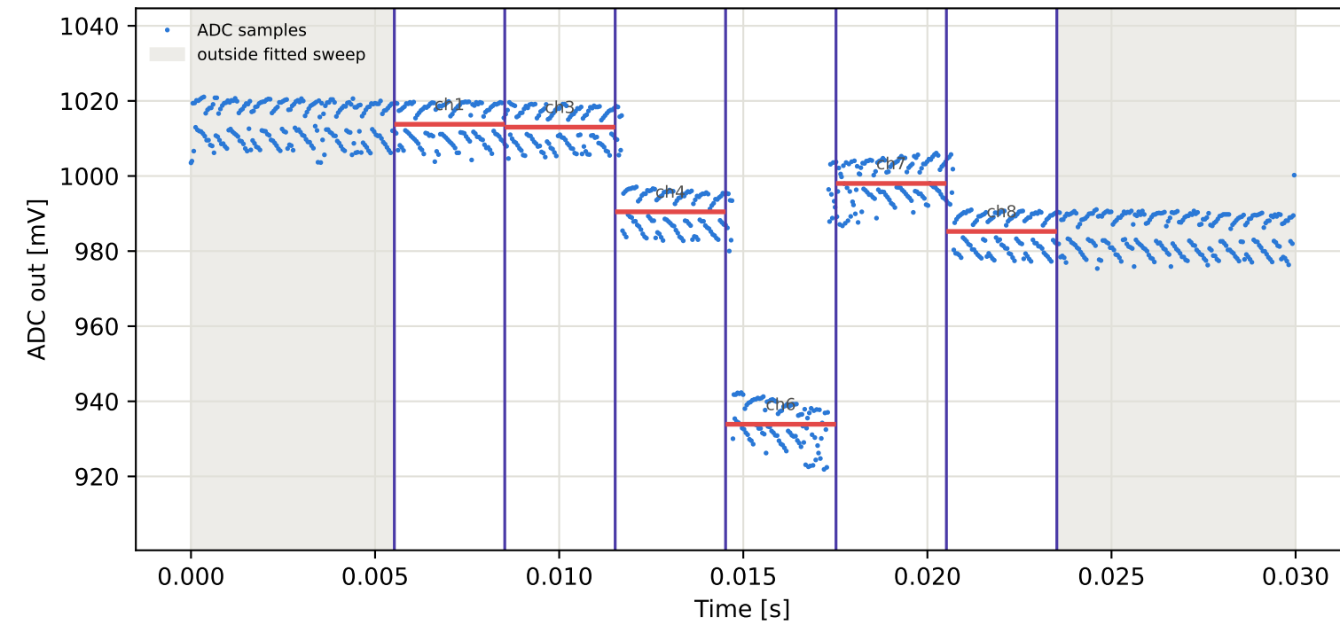
Tag9 &lt;- Tag7 | 925 MHz | run 0 | rep 1 | phase -3.62 deg
