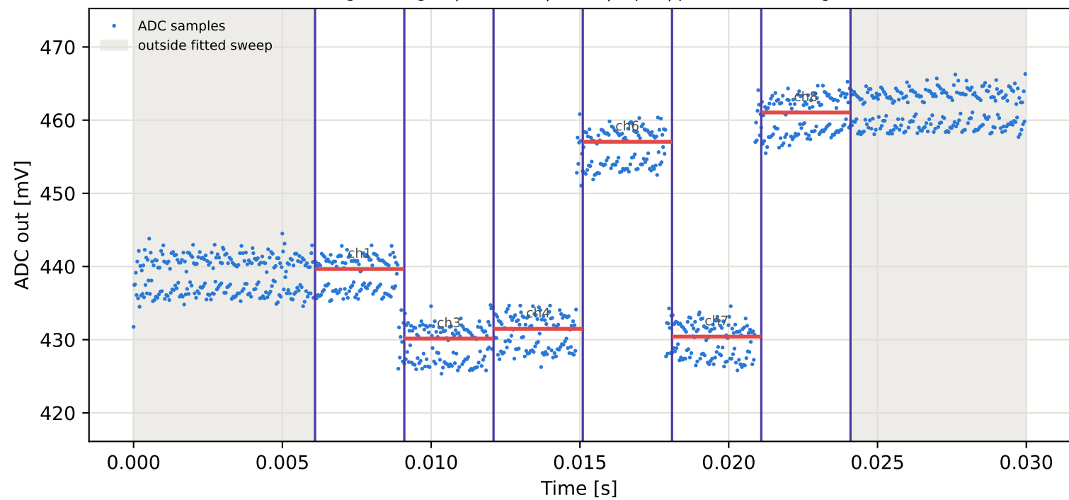
Tag4 &lt;- Tag16 | 885 MHz | run 0 | rep 1 | phase -77.09 deg
