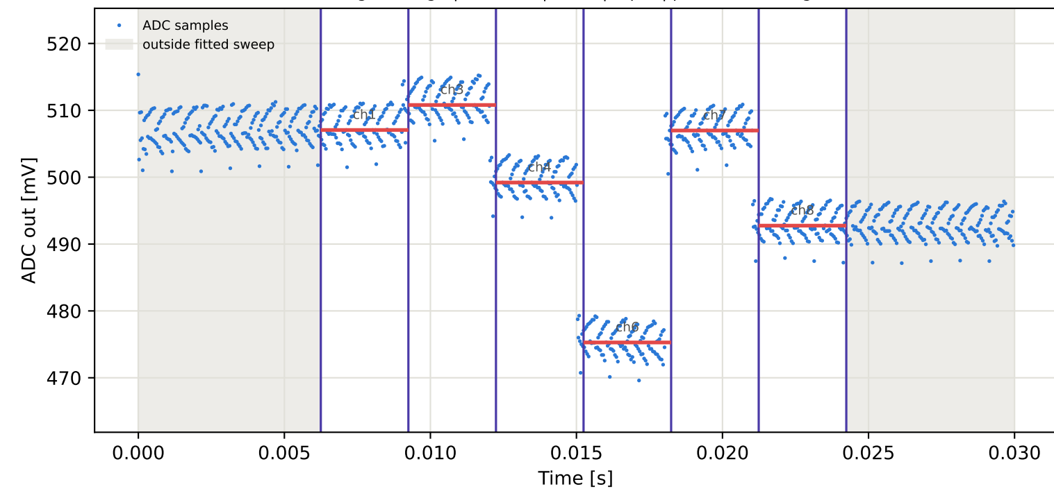
Tag9 &lt;- Tag10 | 955 MHz | run 0 | rep 1 | phase -175.01 deg
