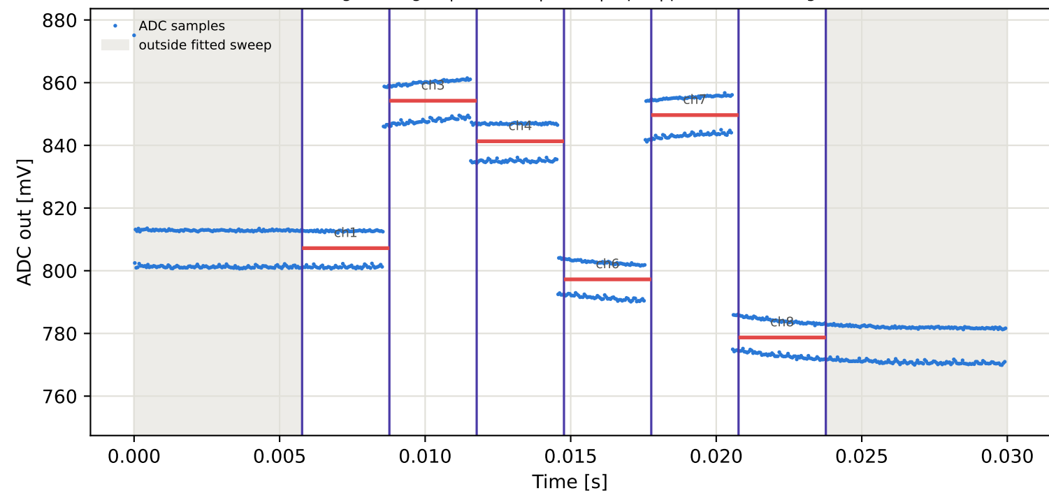
Tag3 &lt;- Tag2 | 865 MHz | run 0 | rep 1 | phase 34.99 deg
