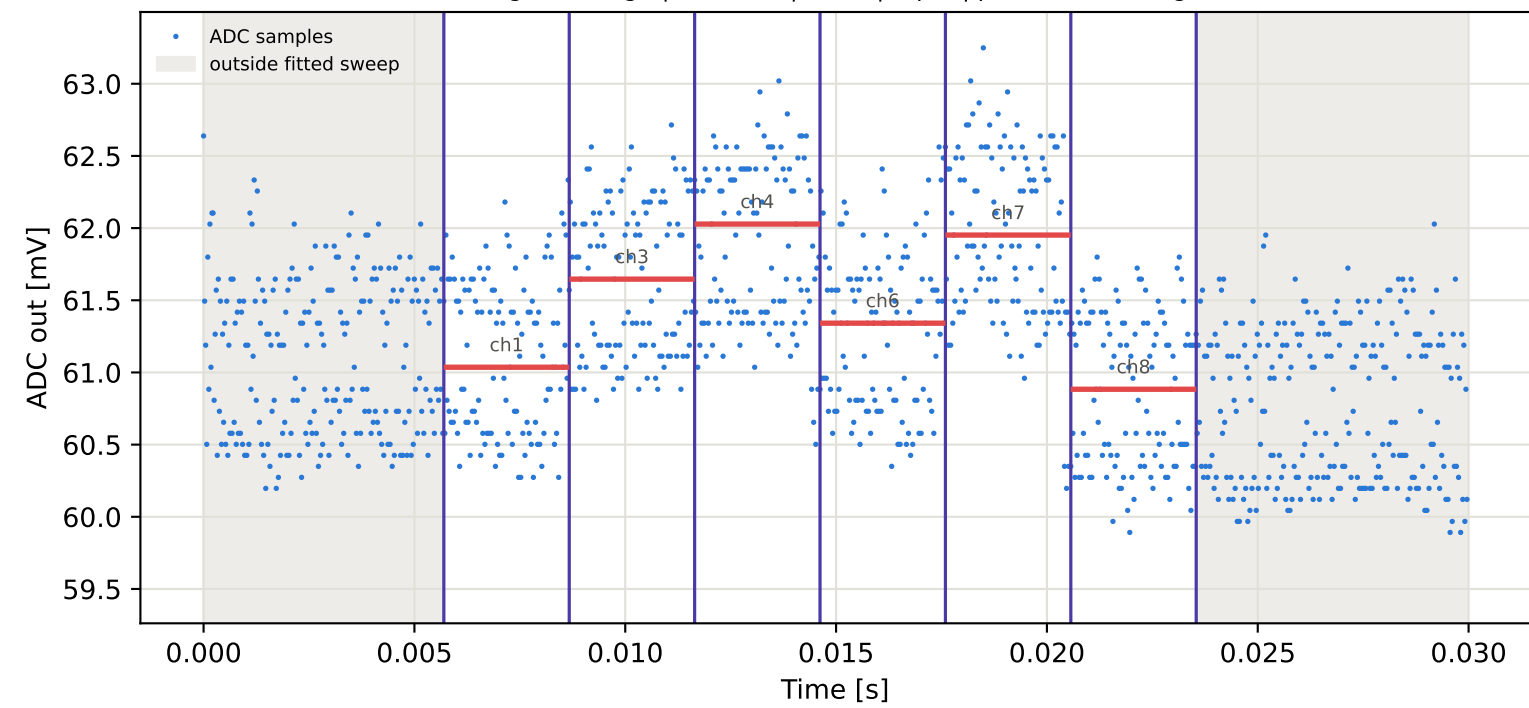
Tag15 &lt;- Tag4 | 785 MHz | run 0 | rep 1 | phase -110.96 deg
