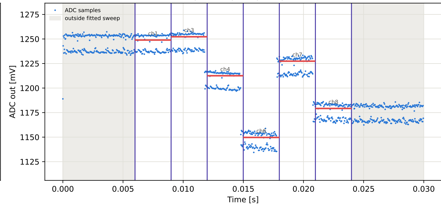
Tag16 &lt;- Tag7 | 885 MHz | run 0 | rep 1 | phase 20.49 deg
