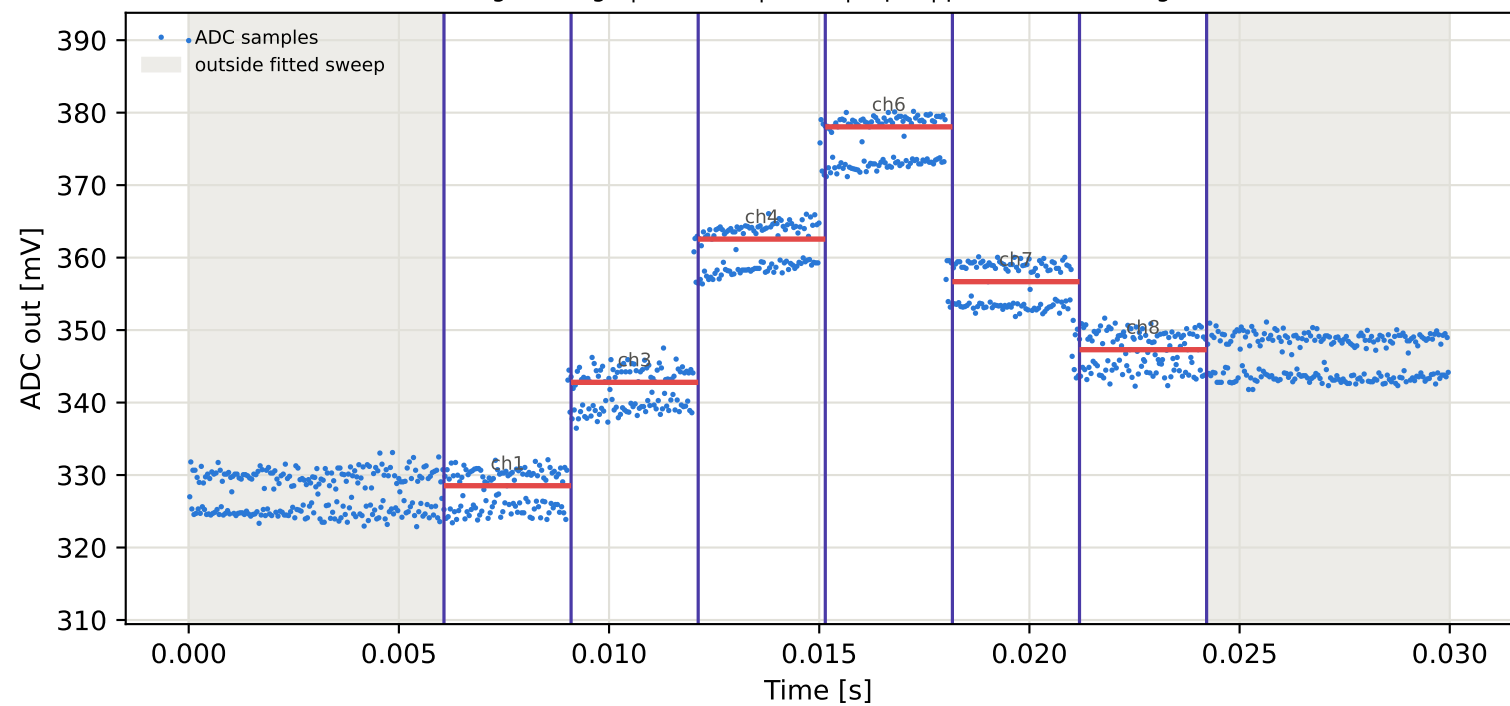
Tag1 &lt;- Tag4 | 885 MHz | run 0 | rep 1 | phase -132.53 deg
