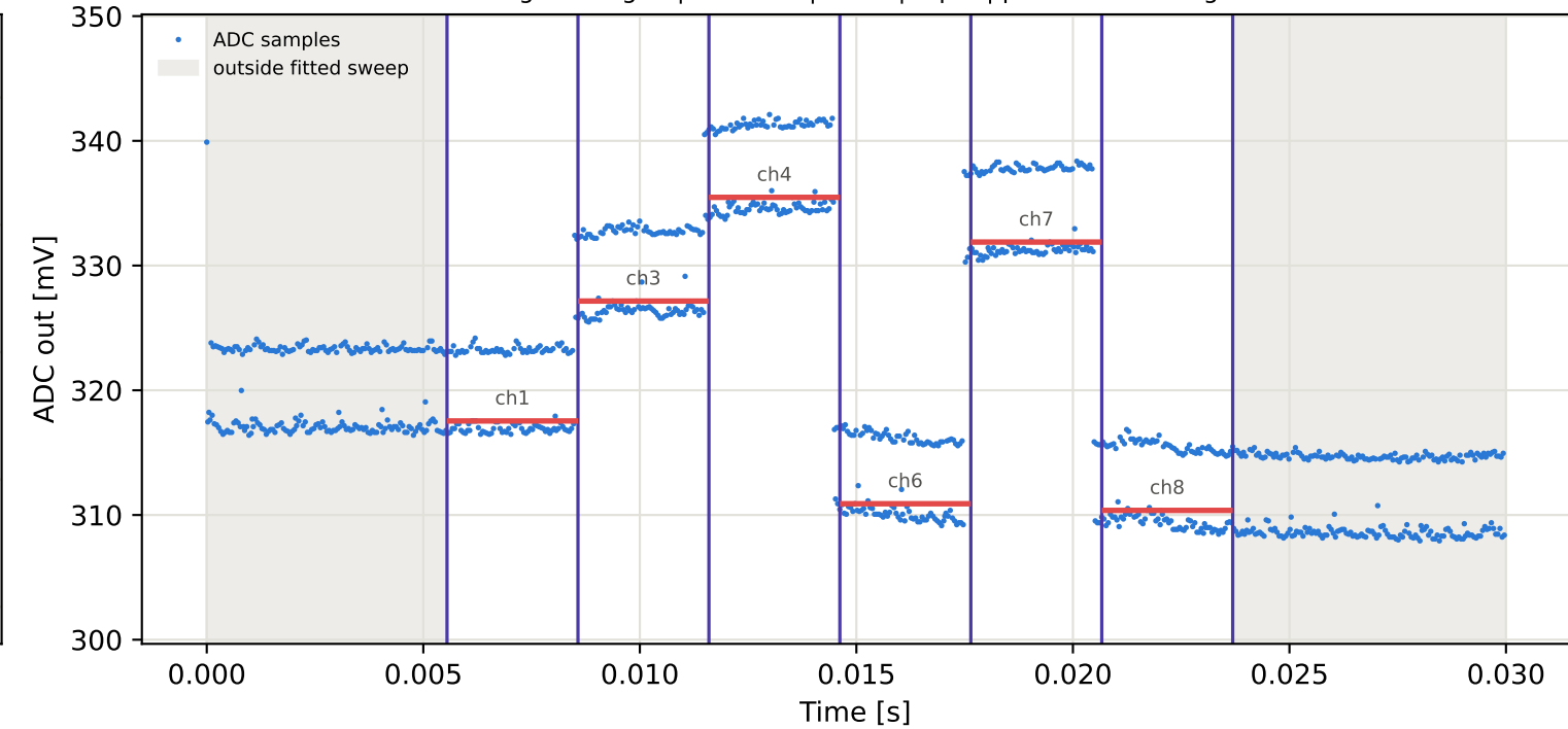
Tag5 &lt;- Tag2 | 955 MHz | run 0 | rep 1 | phase -2.41 deg
