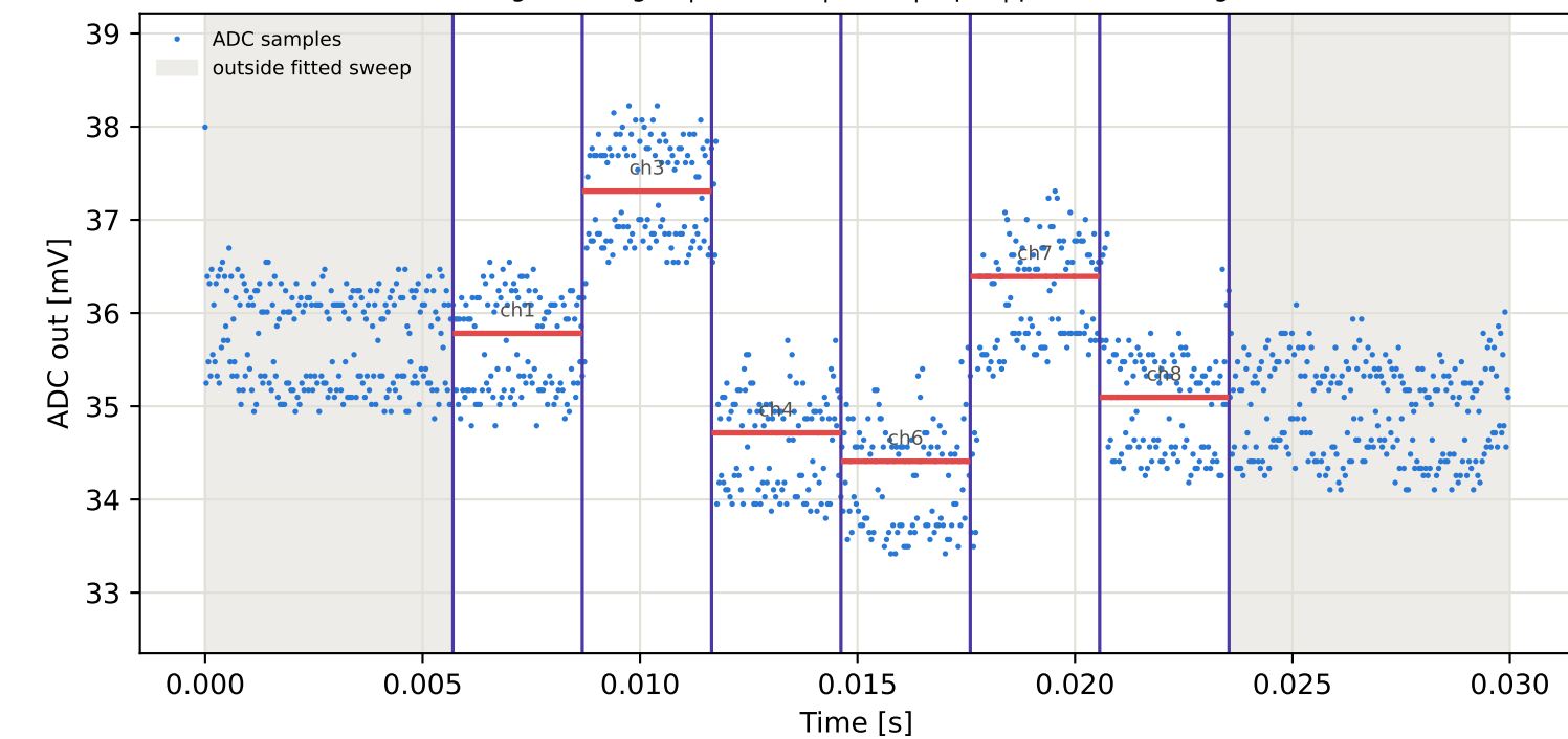
Tag15 &lt;- Tag10 | 775 MHz | run 0 | rep 1 | phase 37.98 deg
