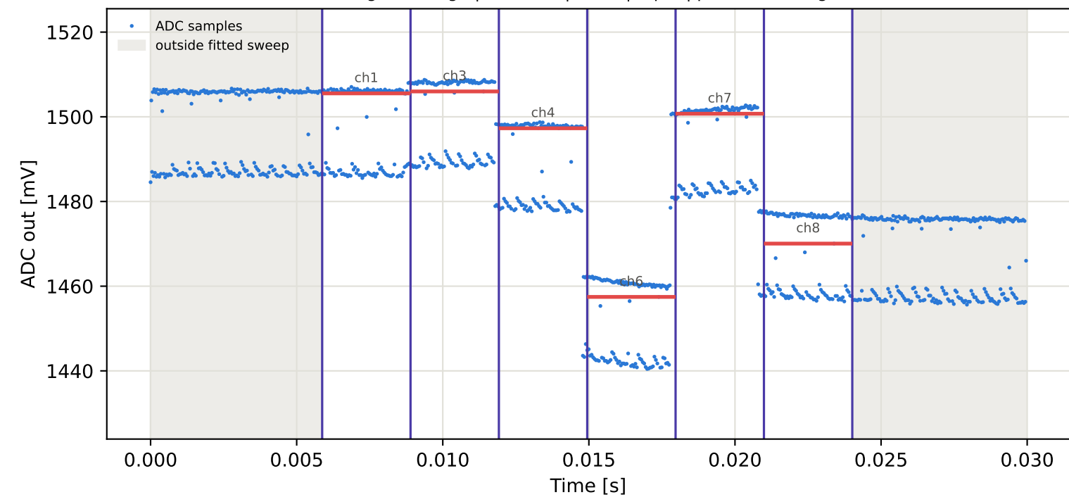
Tag16 &lt;- Tag7 | 895 MHz | run 0 | rep 1 | phase 36.55 deg
