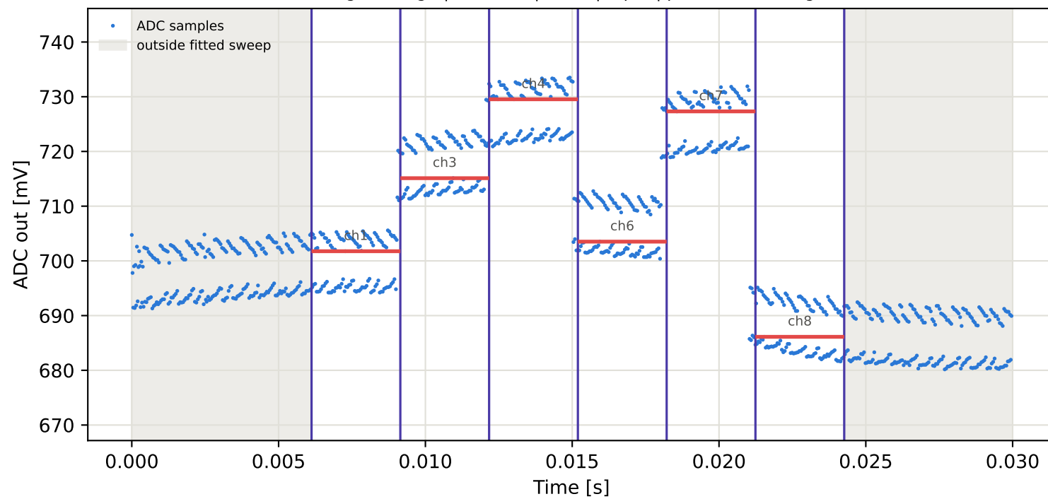
Tag6 &lt;- Tag9 | 895 MHz | run 0 | rep 1 | phase 164.93 deg
