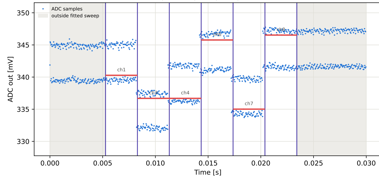
Tag1 &lt;- Tag3 | 825 MHz | run 0 | rep 1 | phase 160.07 deg
