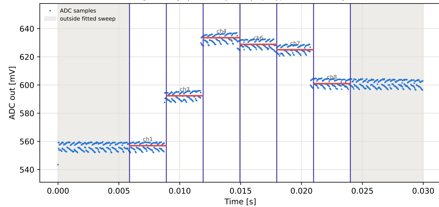
Tag2 &lt;- Tag1 | 845 MHz | run 0 | rep 1 | phase 116.36 deg
