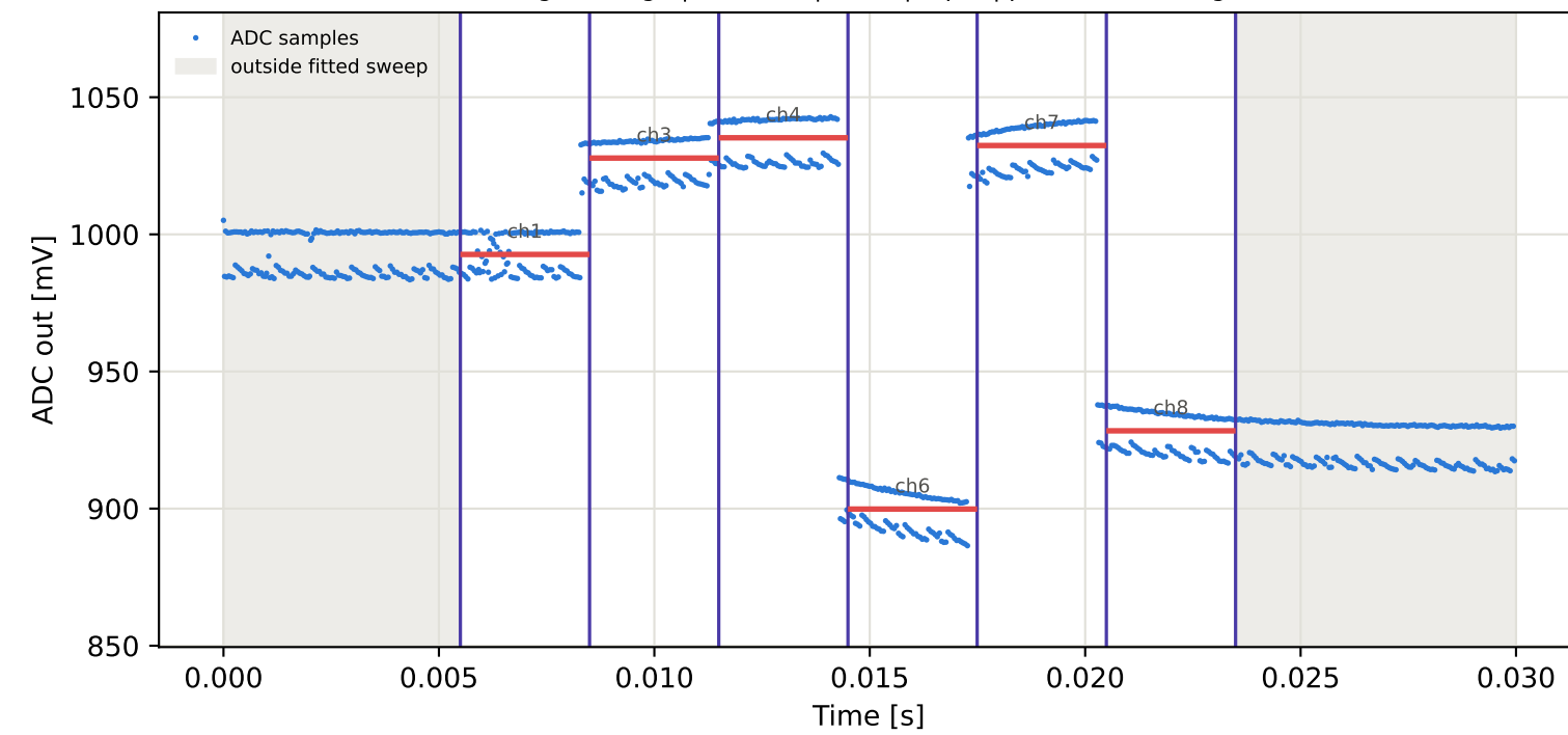
Tag9 &lt;- Tag5 | 925 MHz | run 0 | rep 1 | phase 20.46 deg
