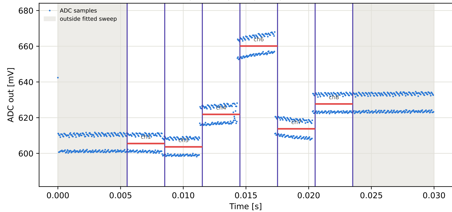
Tag3 &lt;- Tag2 | 905 MHz | run 0 | rep 1 | phase -158.38 deg
