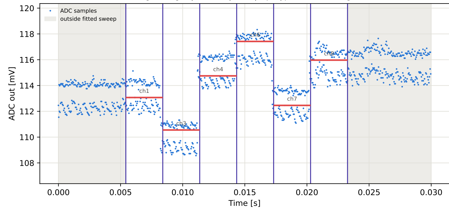
Tag5 &lt;- Tag2 | 795 MHz | run 0 | rep 1 | phase -63.54 deg
