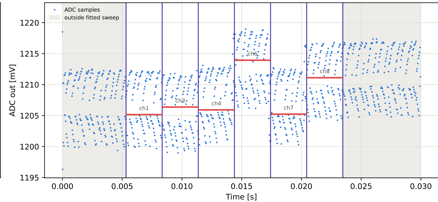
Tag15 &lt;- Tag6 | 895 MHz | run 0 | rep 1 | phase 127.61 deg
