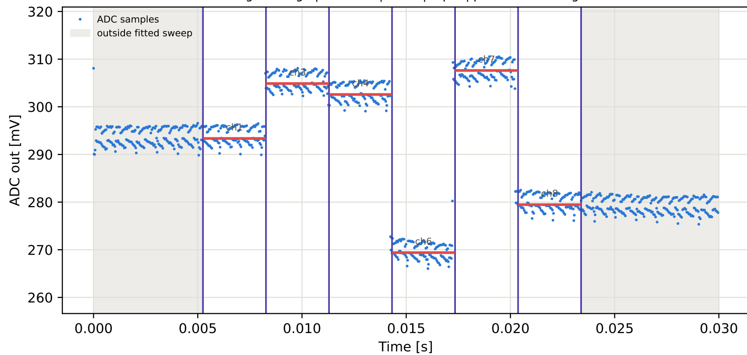
Tag6 &lt;- Tag9 | 975 MHz | run 0 | rep 1 | phase -11.93 deg
