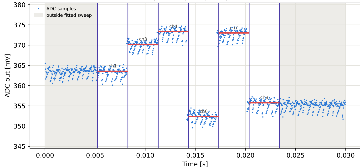
Tag5 &lt;- Tag2 | 975 MHz | run 0 | rep 1 | phase 38.87 deg
