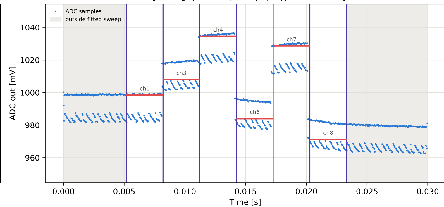
Tag9 &lt;- Tag15 | 925 MHz | run 0 | rep 1 | phase 163.80 deg
