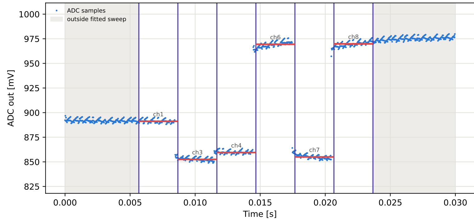
Tag10 &lt;- Tag5 | 895 MHz | run 0 | rep 1 | phase -36.03 deg
