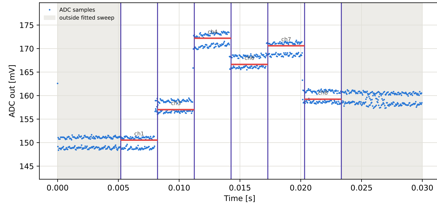
Tag4 &lt;- Tag2 | 845 MHz | run 0 | rep 1 | phase 114.82 deg
