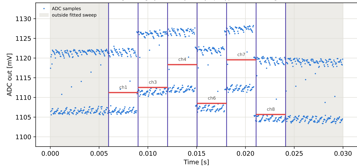
Tag8 &lt;- Tag10 | 865 MHz | run 0 | rep 1 | phase -132.68 deg
