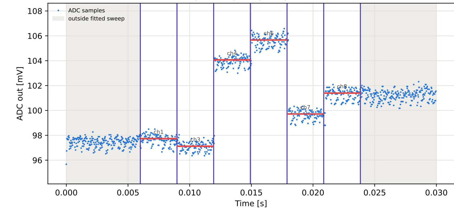
Tag2 &lt;- Tag7 | 995 MHz | run 0 | rep 1 | phase -150.49 deg
