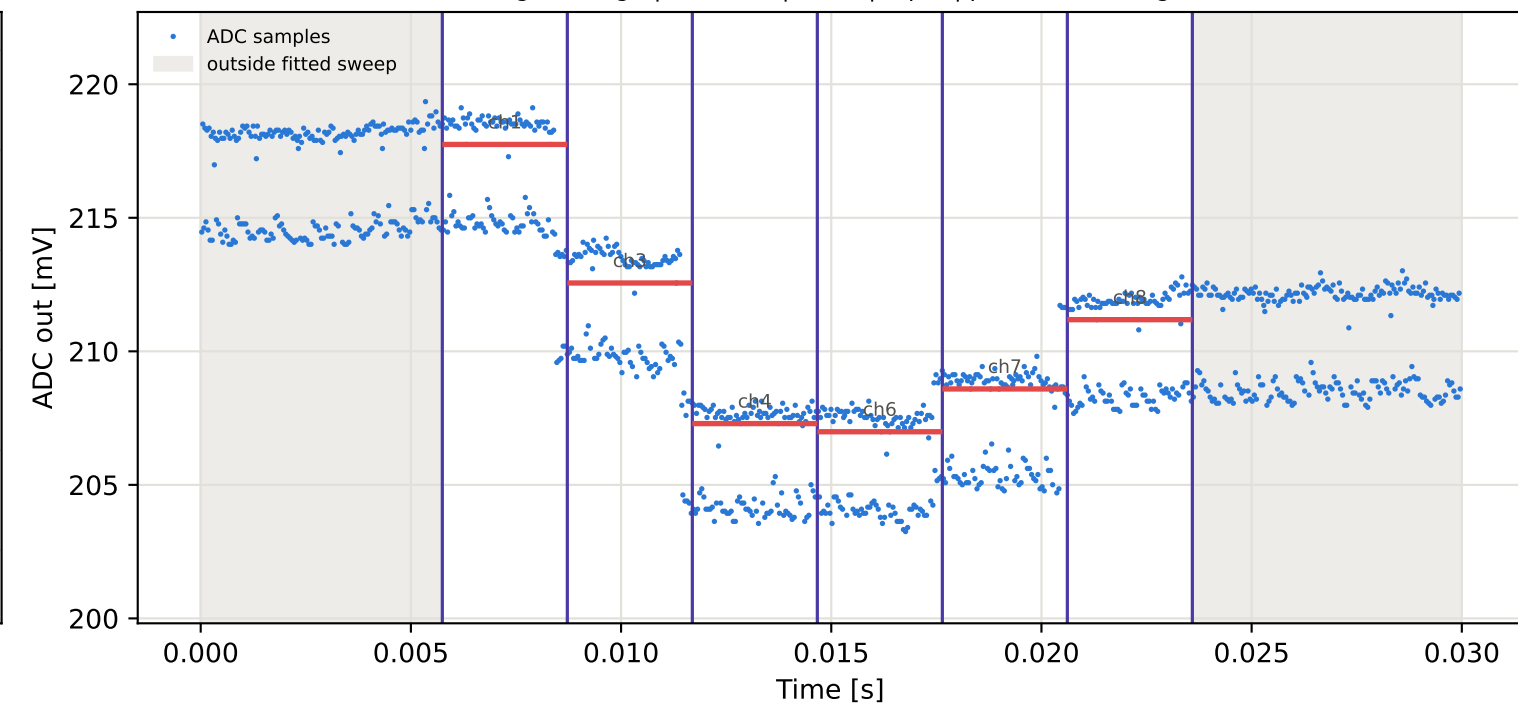
Tag4 &lt;- Tag8 | 855 MHz | run 0 | rep 1 | phase 96.43 deg
