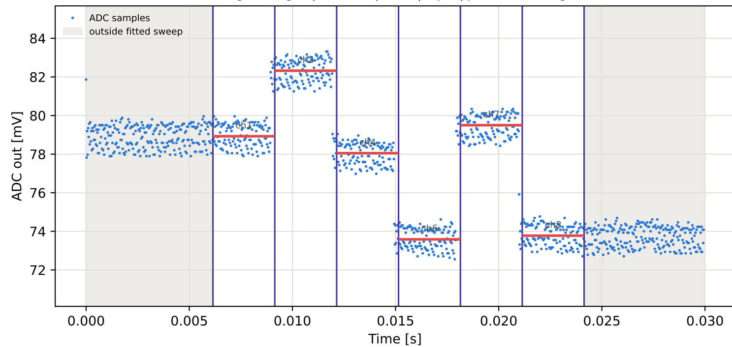
Tag1 &lt;- Tag16 | 845 MHz | run 0 | rep 1 | phase 99.63 deg
