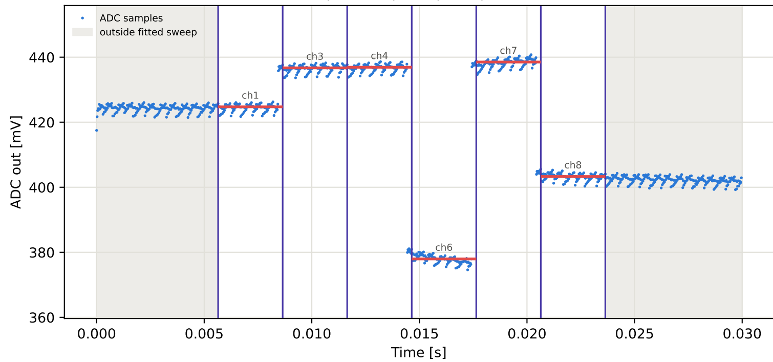
Tag9 &lt;- Tag8 | 945 MHz | run 0 | rep 1 | phase -11.13 deg
