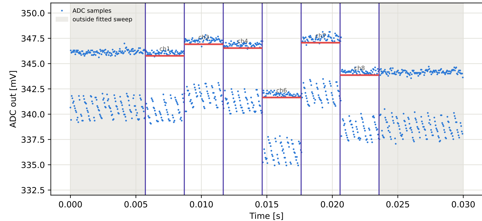
Tag2 &lt;- Tag7 | 965 MHz | run 0 | rep 1 | phase 144.96 deg
