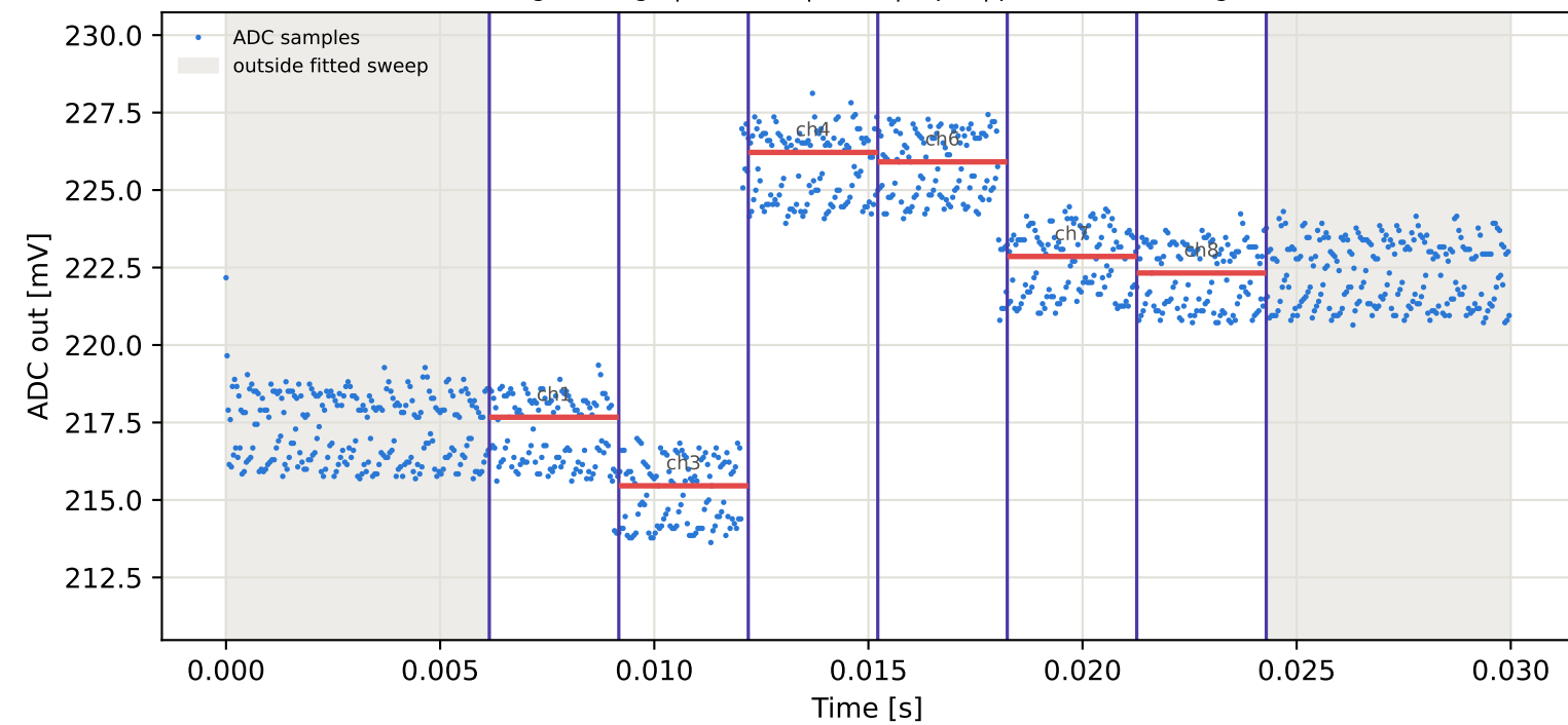
Tag9 &lt;- Tag15 | 835 MHz | run 0 | rep 1 | phase 53.19 deg
