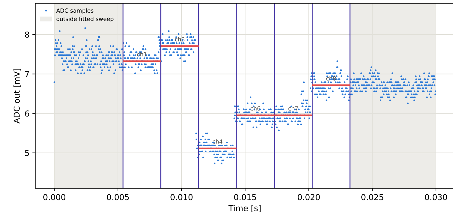
Tag2 &lt;- Tag16 | 775 MHz | run 0 | rep 1 | phase 72.53 deg
