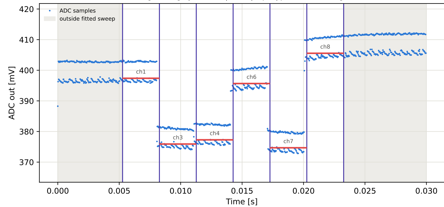
Tag7 &lt;- Tag1 | 855 MHz | run 0 | rep 1 | phase -74.64 deg
