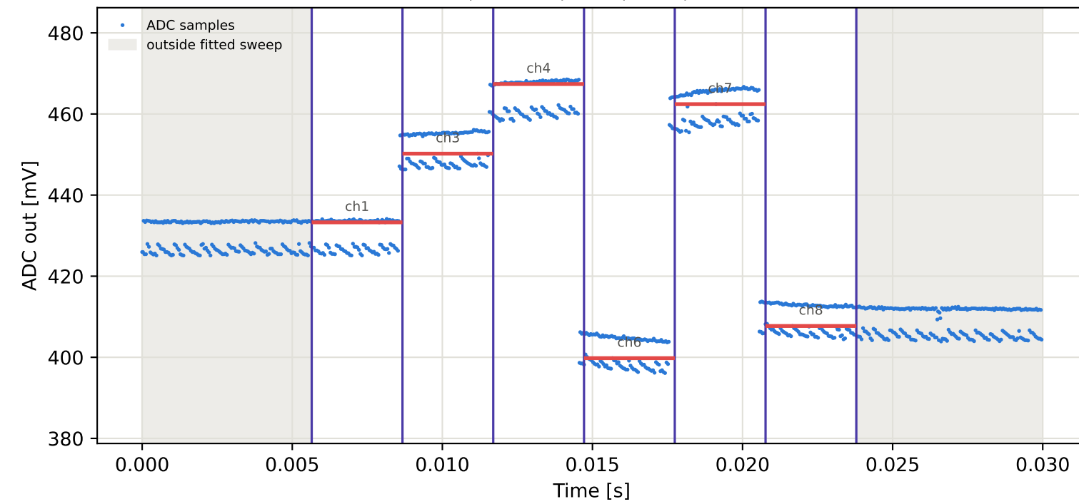
Tag8 &lt;- Tag15 | 975 MHz | run 0 | rep 1 | phase -39.44 deg
