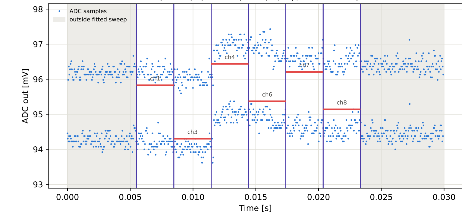
Tag4 &lt;- Tag9 | 775 MHz | run 0 | rep 1 | phase -124.33 deg
