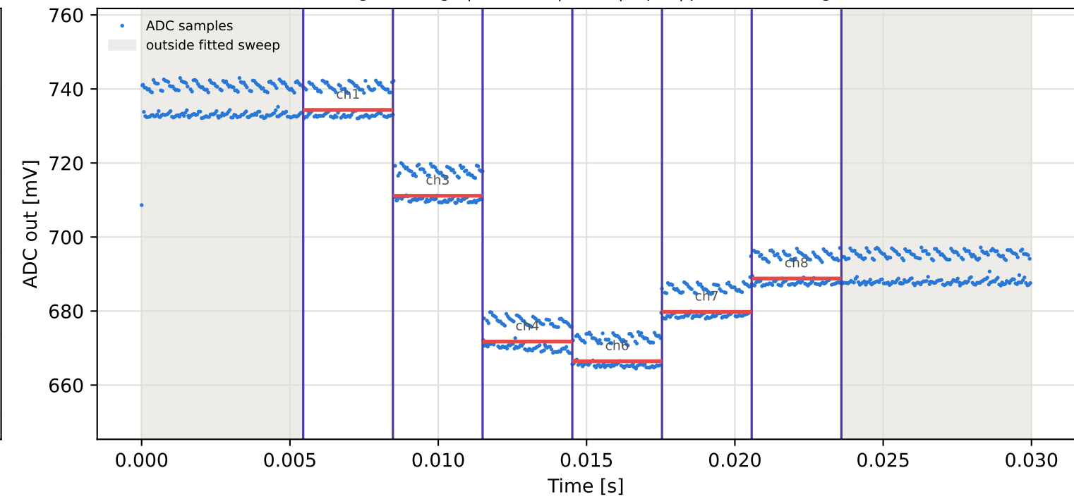
Tag16 &lt;- Tag5 | 845 MHz | run 0 | rep 1 | phase 15.84 deg
