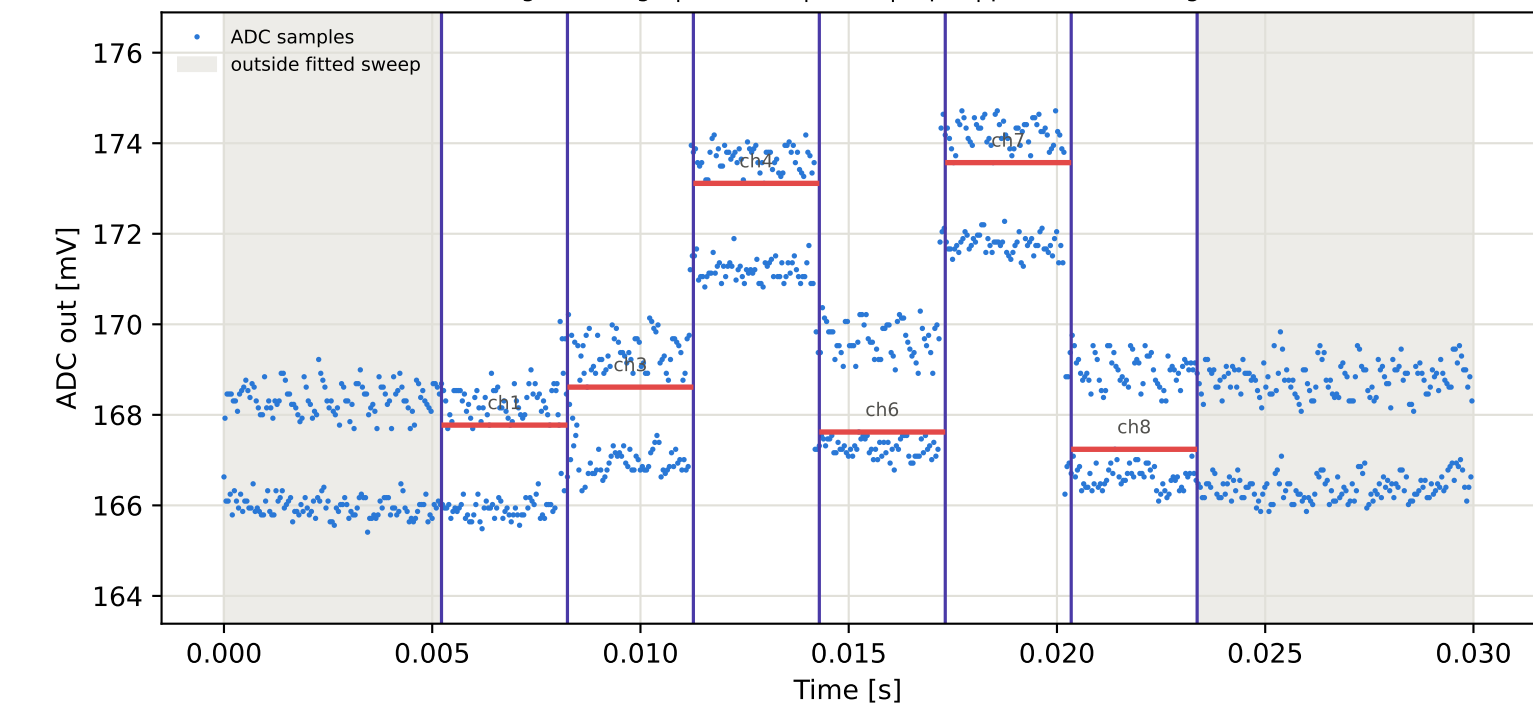
Tag15 &lt;- Tag5 | 775 MHz | run 0 | rep 1 | phase 71.96 deg
