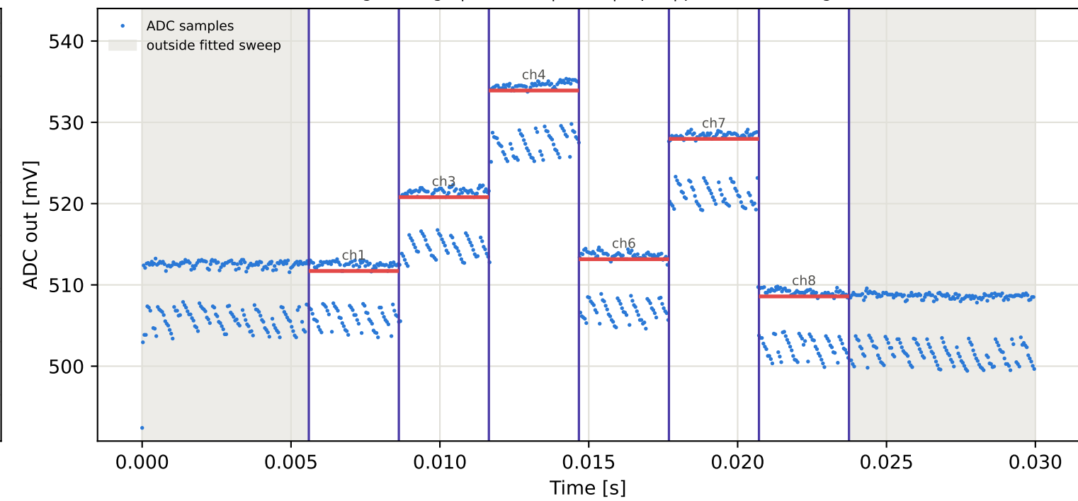
Tag8 &lt;- Tag10 | 985 MHz | run 0 | rep 1 | phase 7.84 deg
