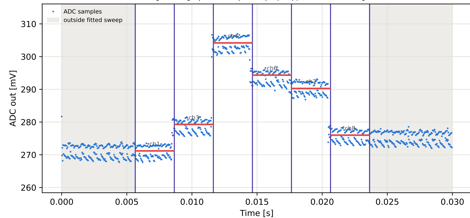
Tag6 &lt;- Tag1 | 965 MHz | run 0 | rep 1 | phase -120.79 deg
