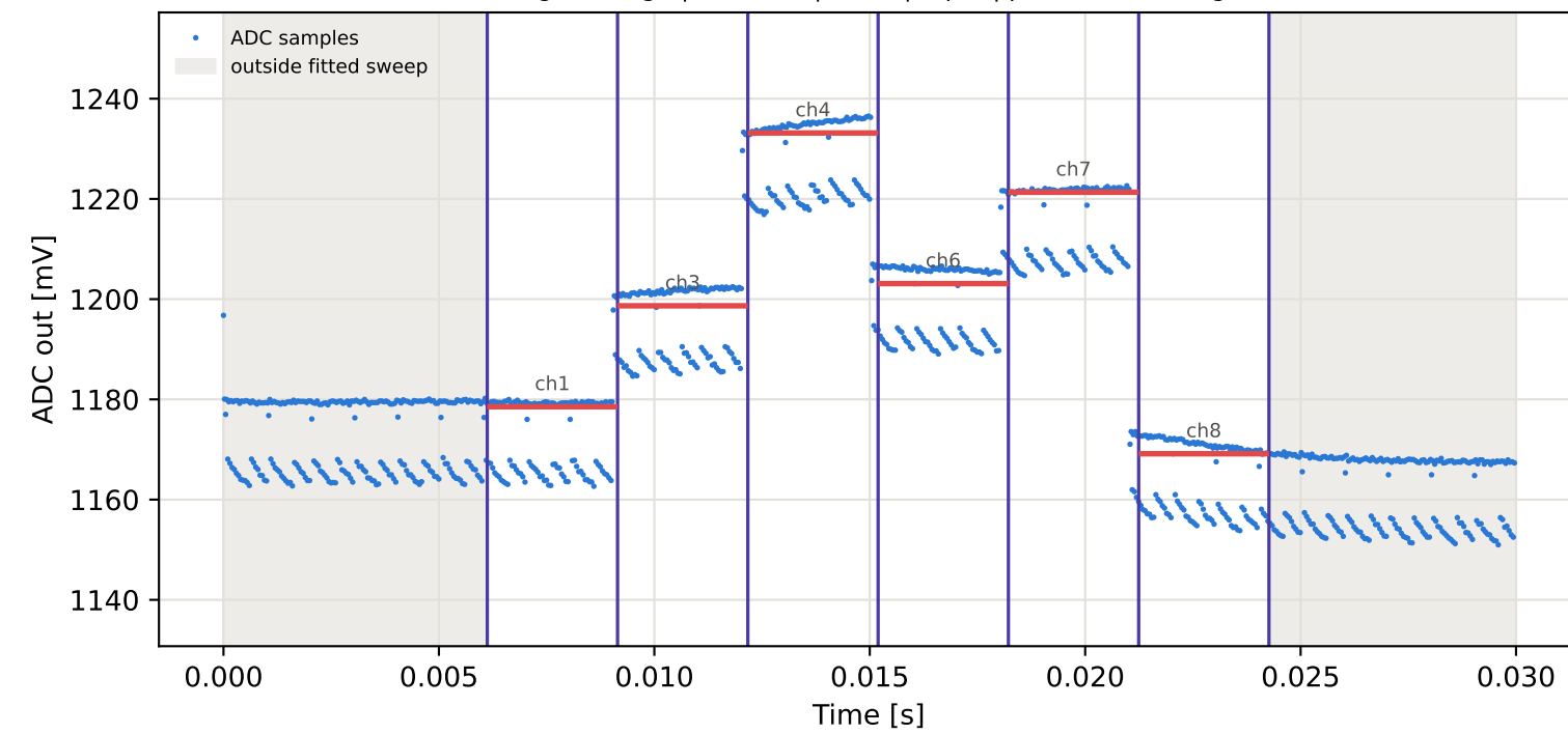
Tag8 &lt;- Tag4 | 895 MHz | run 0 | rep 1 | phase -140.86 deg
