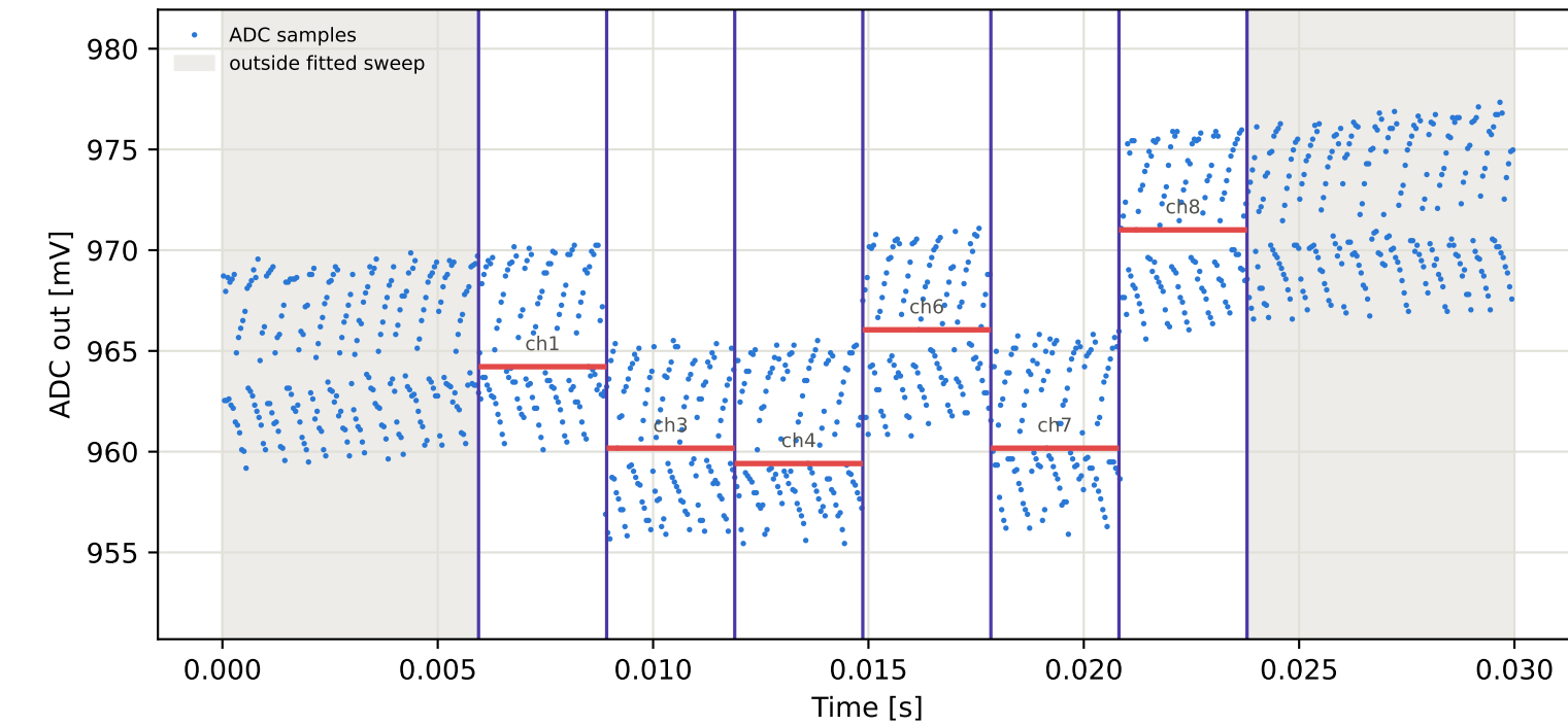
Tag8 &lt;- Tag6 | 875 MHz | run 0 | rep 1 | phase -48.22 deg
