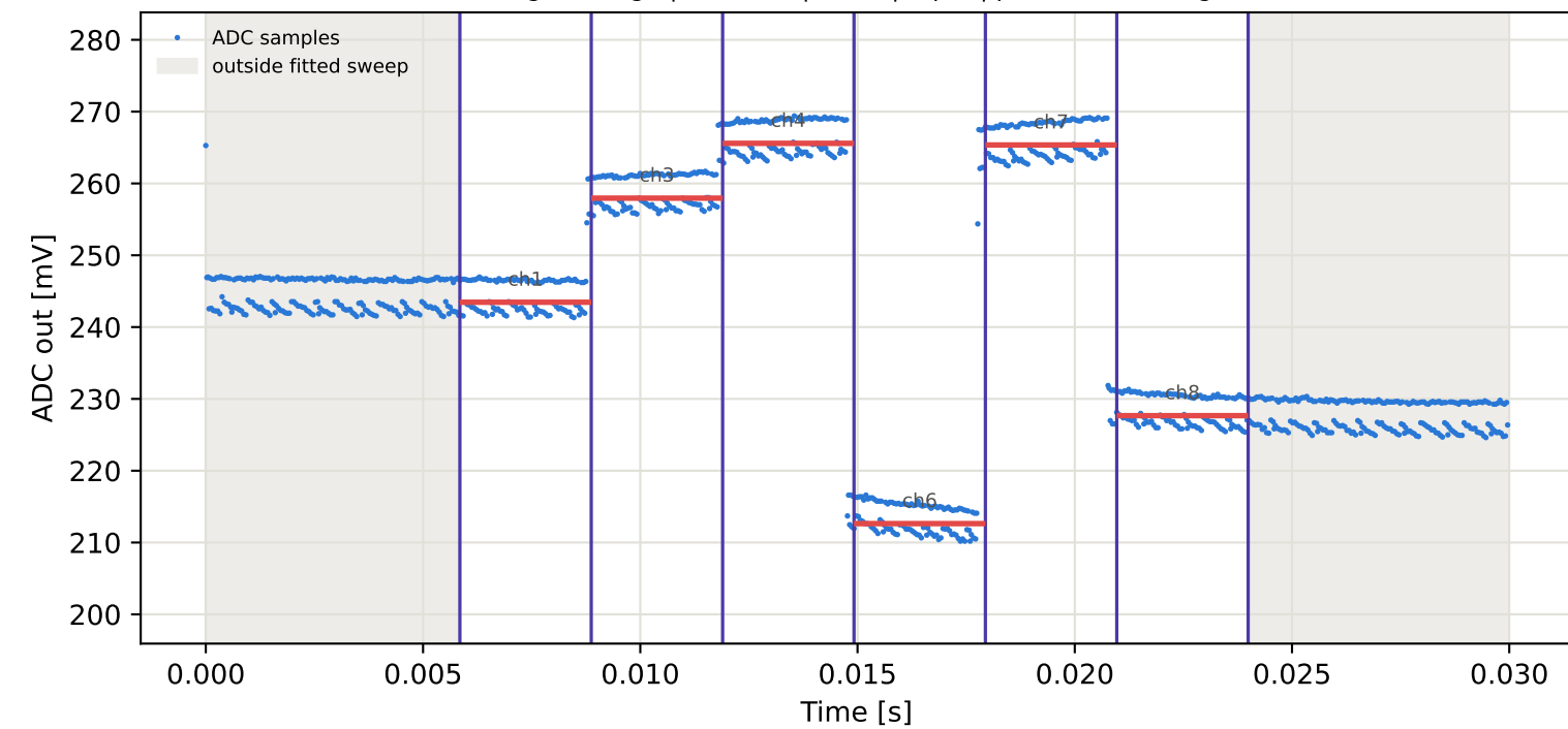
Tag9 &lt;- Tag5 | 995 MHz | run 0 | rep 1 | phase 35.66 deg
