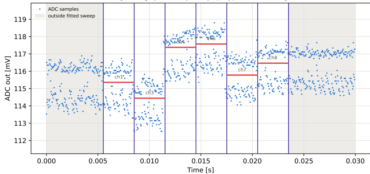
Tag2 &lt;- Tag7 | 775 MHz | run 0 | rep 1 | phase -17.60 deg
