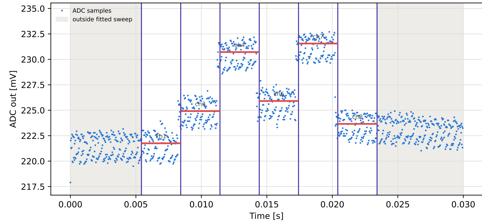
Tag7 &lt;- Tag5 | 805 MHz | run 0 | rep 1 | phase 31.43 deg
