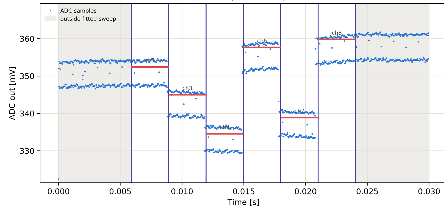
Tag10 &lt;- Tag2 | 955 MHz | run 0 | rep 1 | phase -86.49 deg
