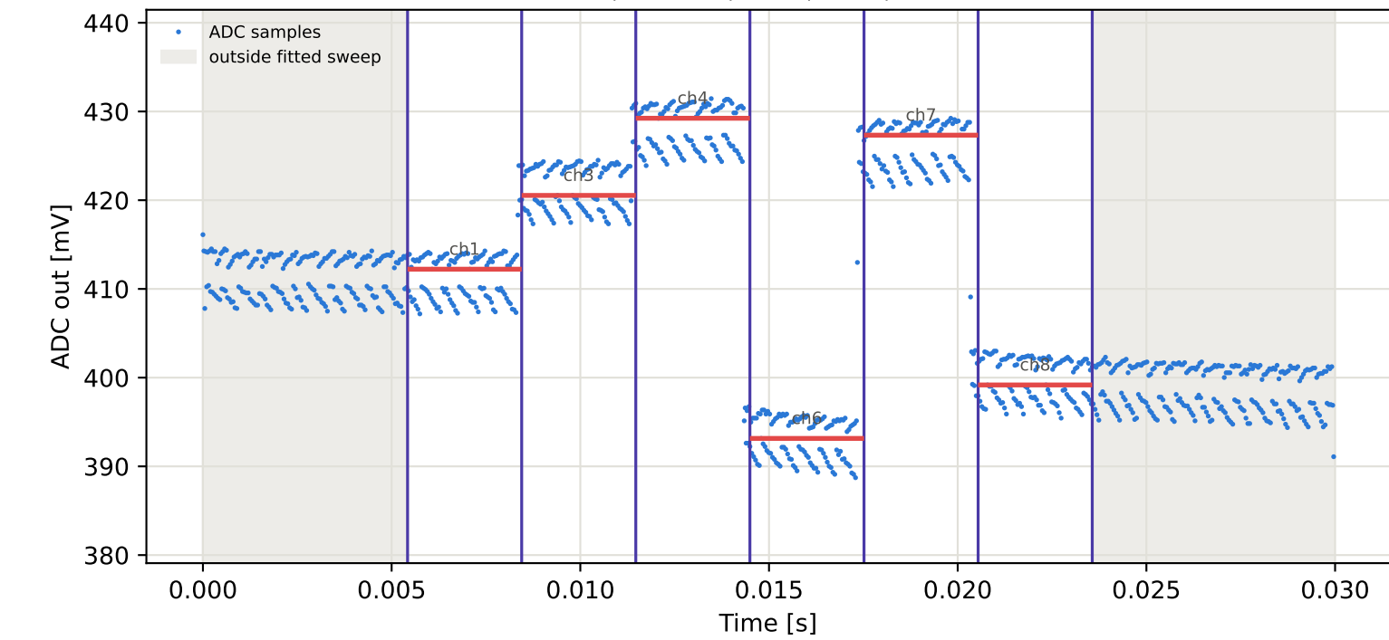
Tag7 &lt;- Tag10 | 965 MHz | run 0 | rep 1 | phase -36.75 deg
