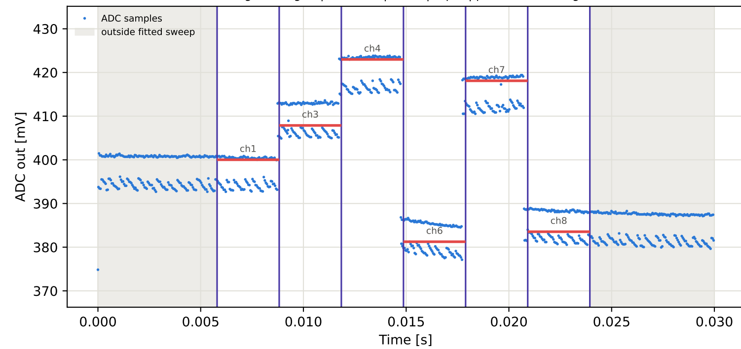
Tag9 &lt;- Tag16 | 975 MHz | run 0 | rep 1 | phase -49.92 deg
