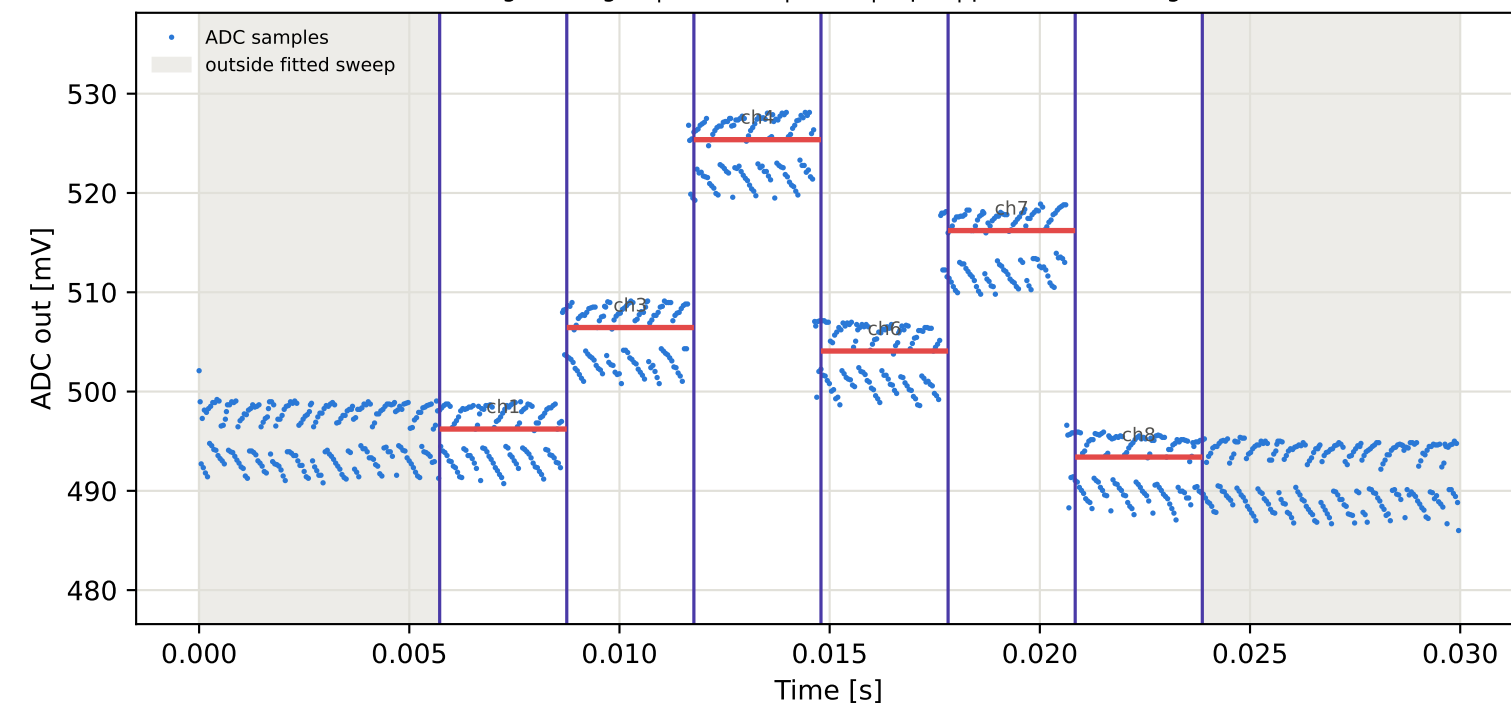
Tag7 &lt;- Tag10 | 945 MHz | run 0 | rep 1 | phase -91.97 deg
