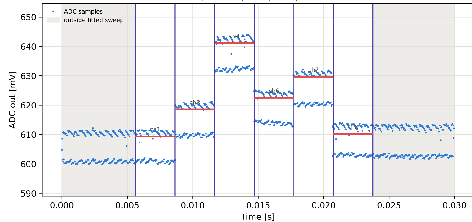
Tag2 &lt;- Tag10 | 985 MHz | run 0 | rep 1 | phase 16.77 deg
