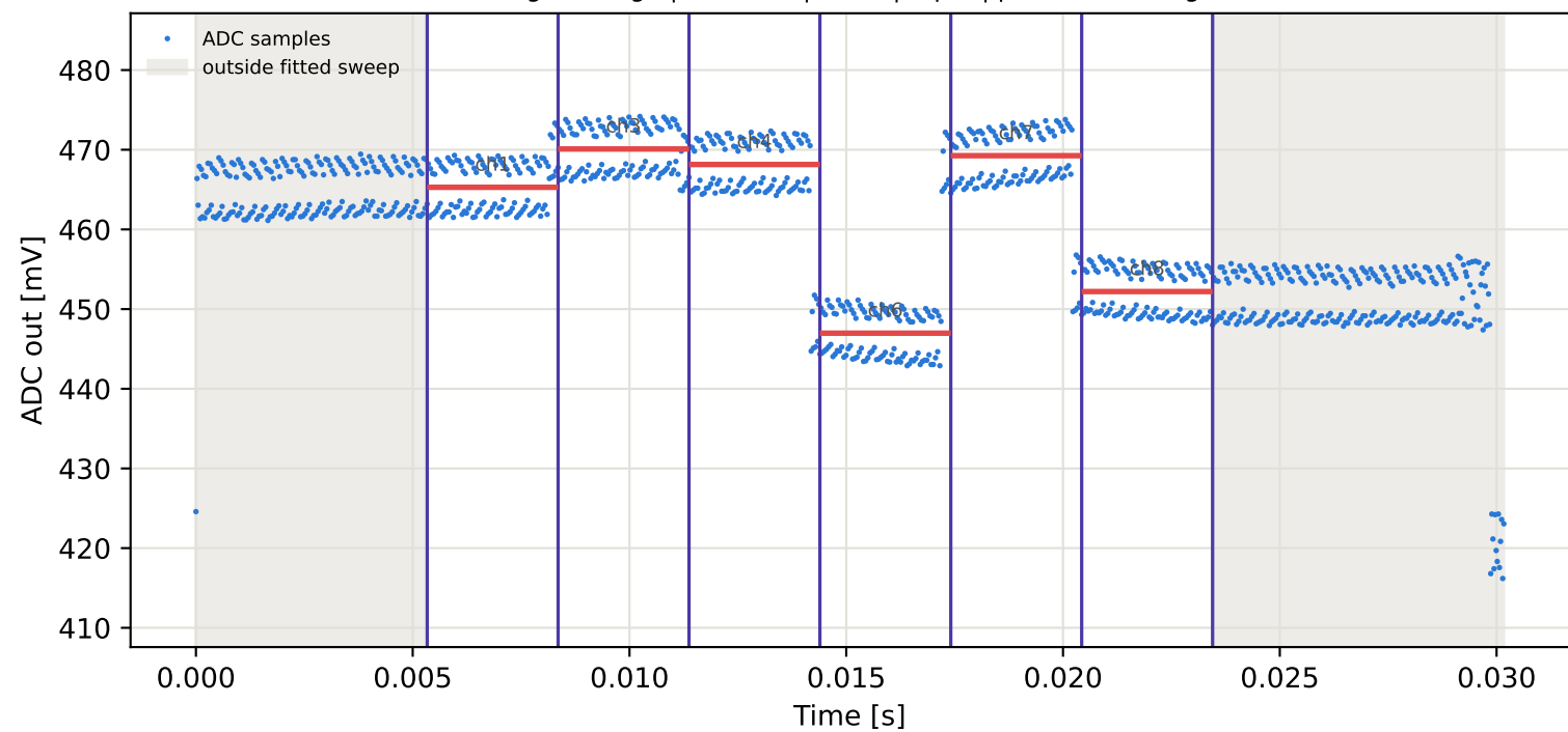
Tag1 &lt;- Tag4 | 905 MHz | run 0 | rep 1 | phase -6.18 deg
