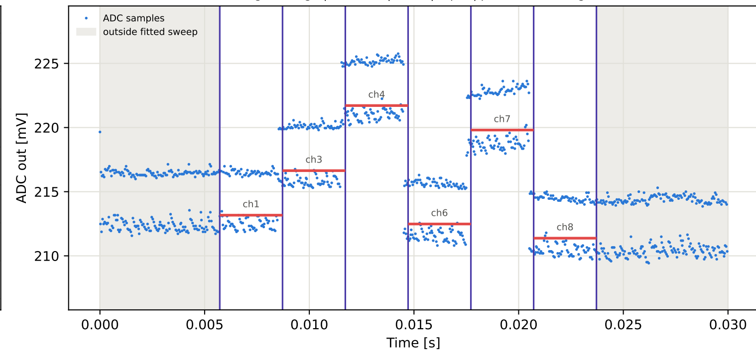
Tag7 &lt;- Tag1 | 955 MHz | run 0 | rep 1 | phase 137.31 deg
