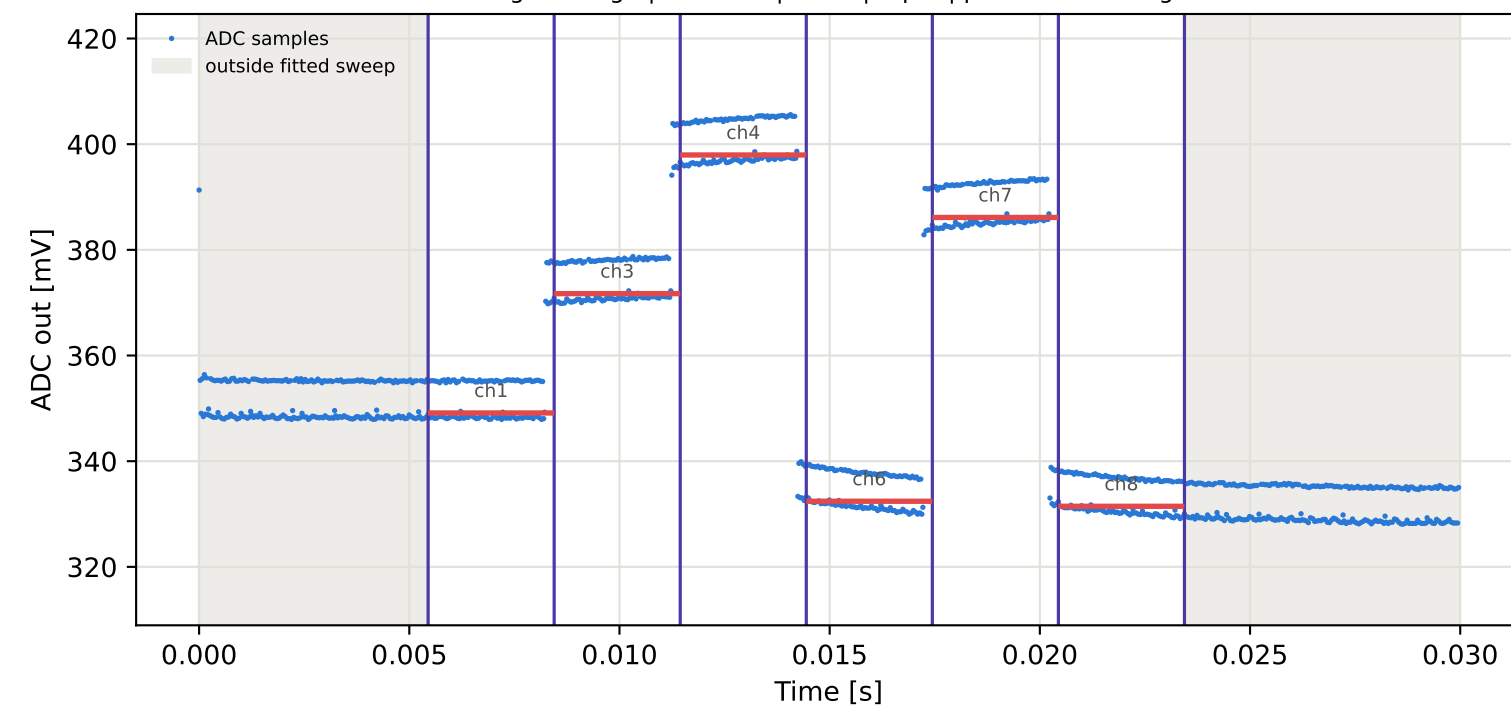
Tag1 &lt;- Tag7 | 955 MHz | run 0 | rep 1 | phase 177.37 deg
