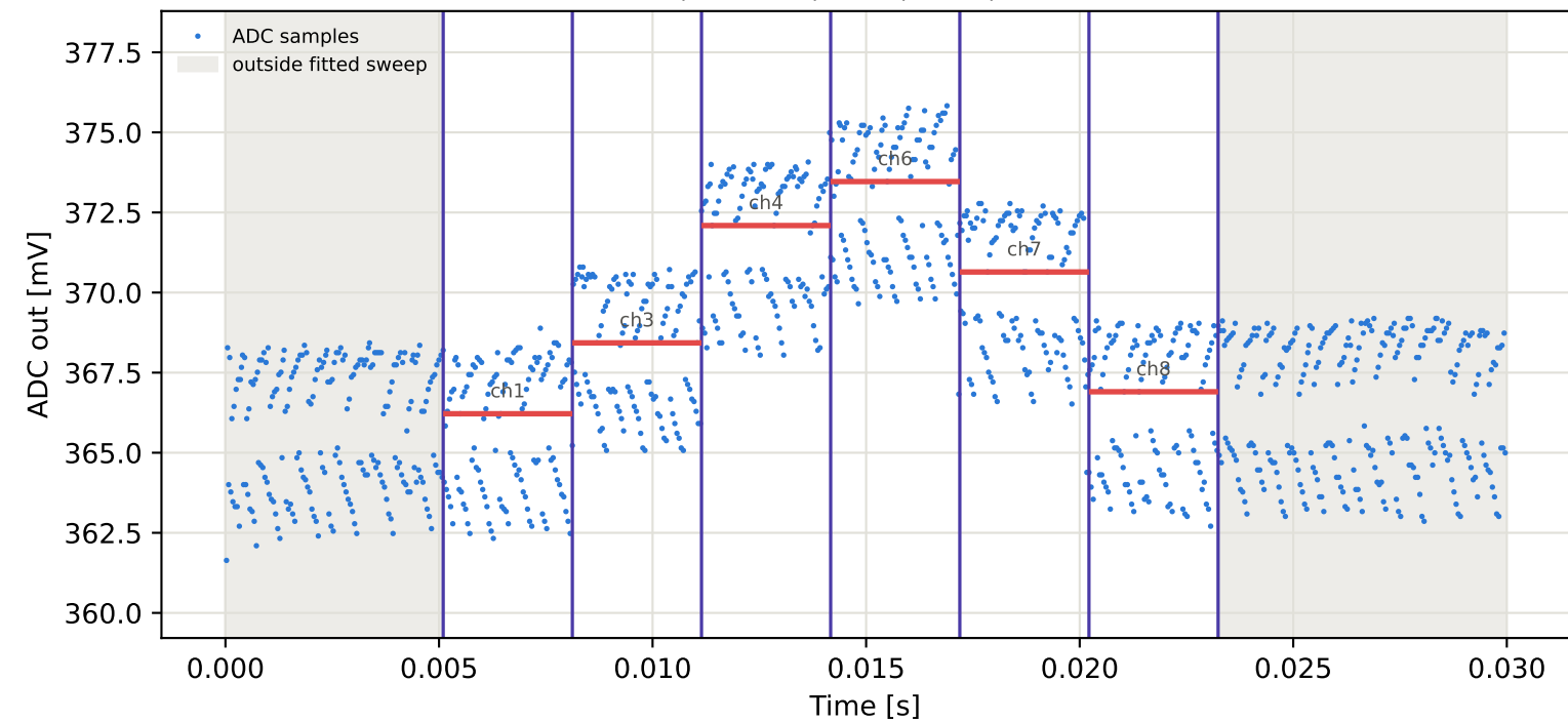
Tag7 &lt;- Tag15 | 915 MHz | run 0 | rep 1 | phase -124.98 deg
