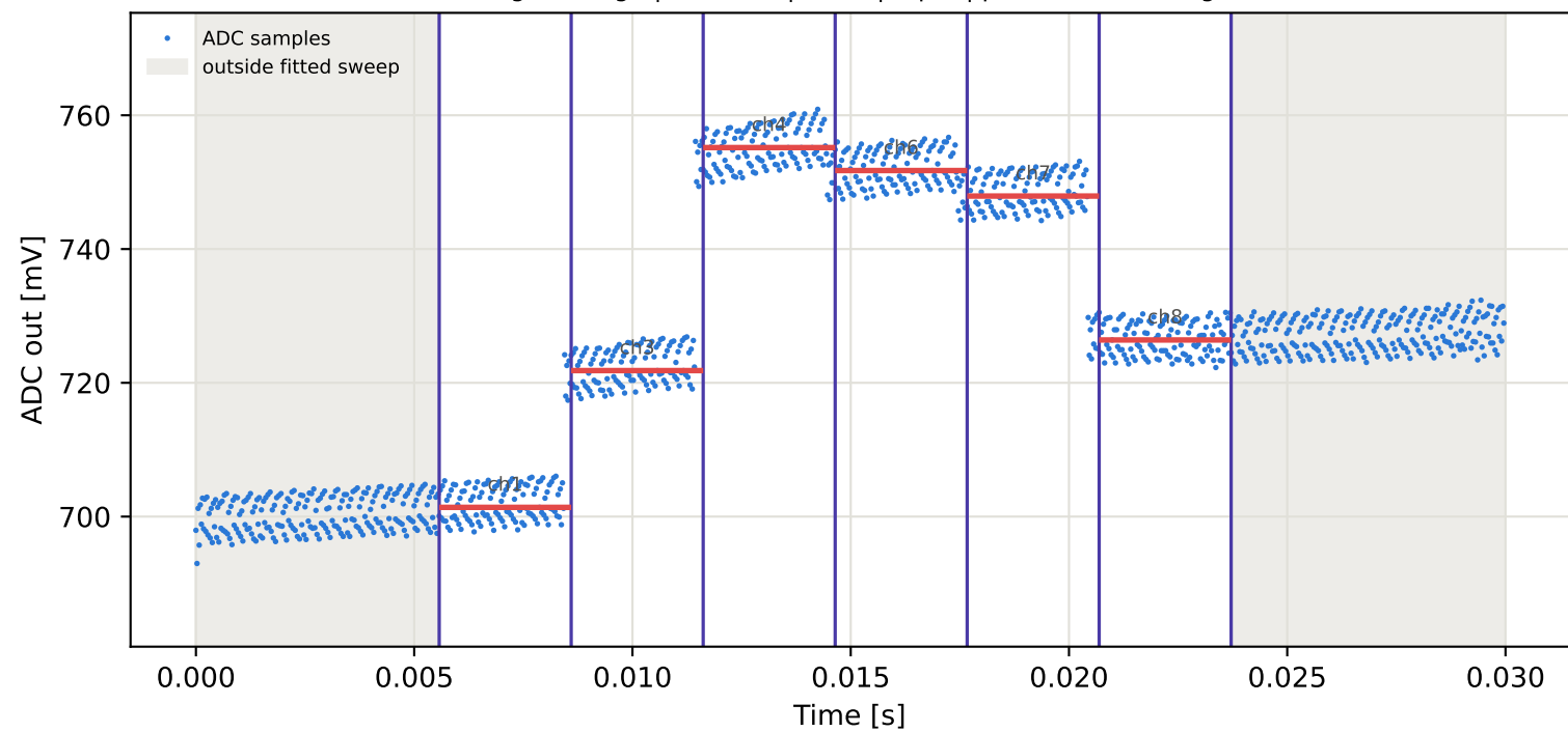
Tag3 &lt;- Tag9 | 875 MHz | run 0 | rep 1 | phase 88.79 deg
