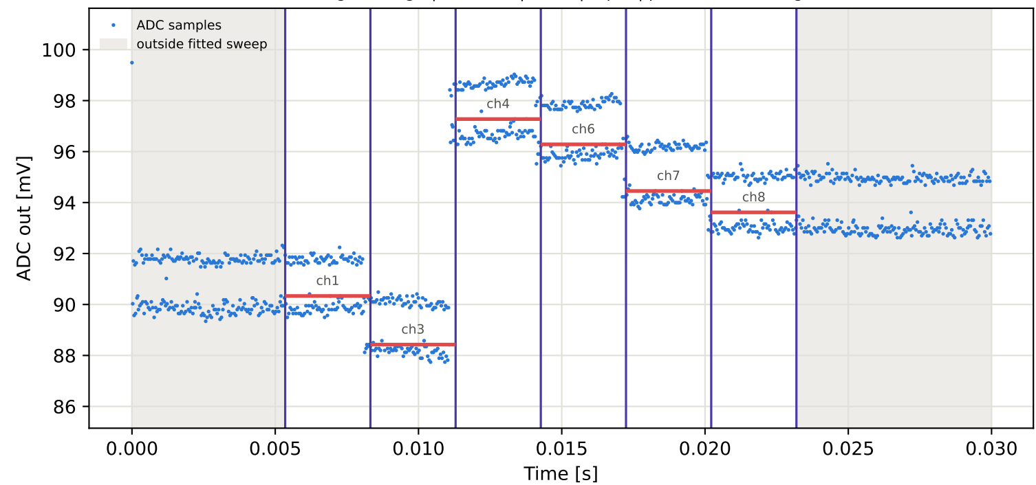
Tag4 &lt;- Tag8 | 775 MHz | run 0 | rep 1 | phase 74.98 deg
