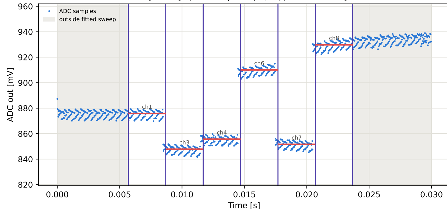
Tag5 &lt;- Tag3 | 875 MHz | run 0 | rep 1 | phase 158.78 deg
