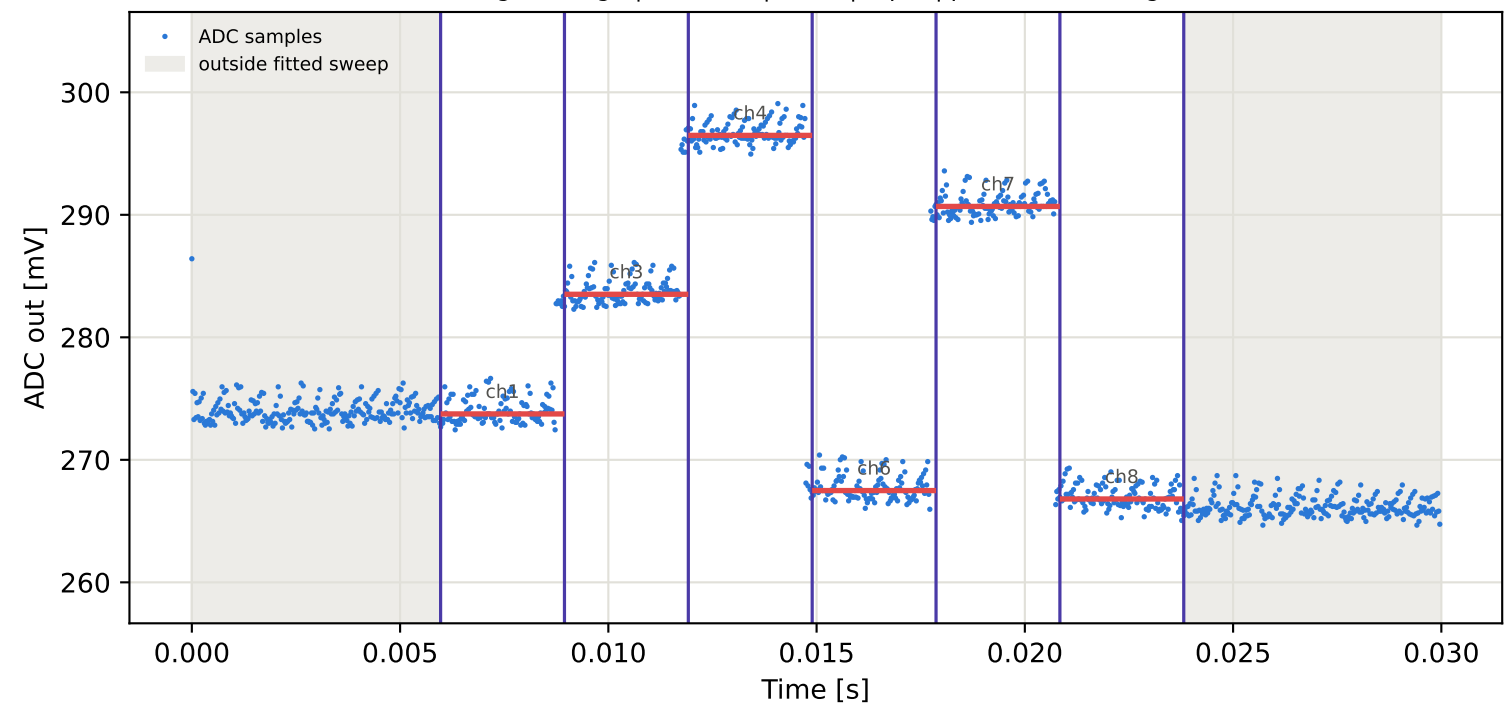
Tag7 &lt;- Tag1 | 965 MHz | run 0 | rep 1 | phase 175.09 deg
