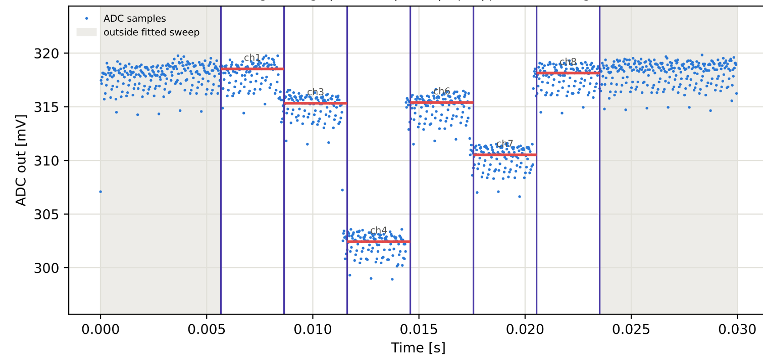
Tag3 &lt;- Tag6 | 995 MHz | run 0 | rep 1 | phase 175.10 deg
