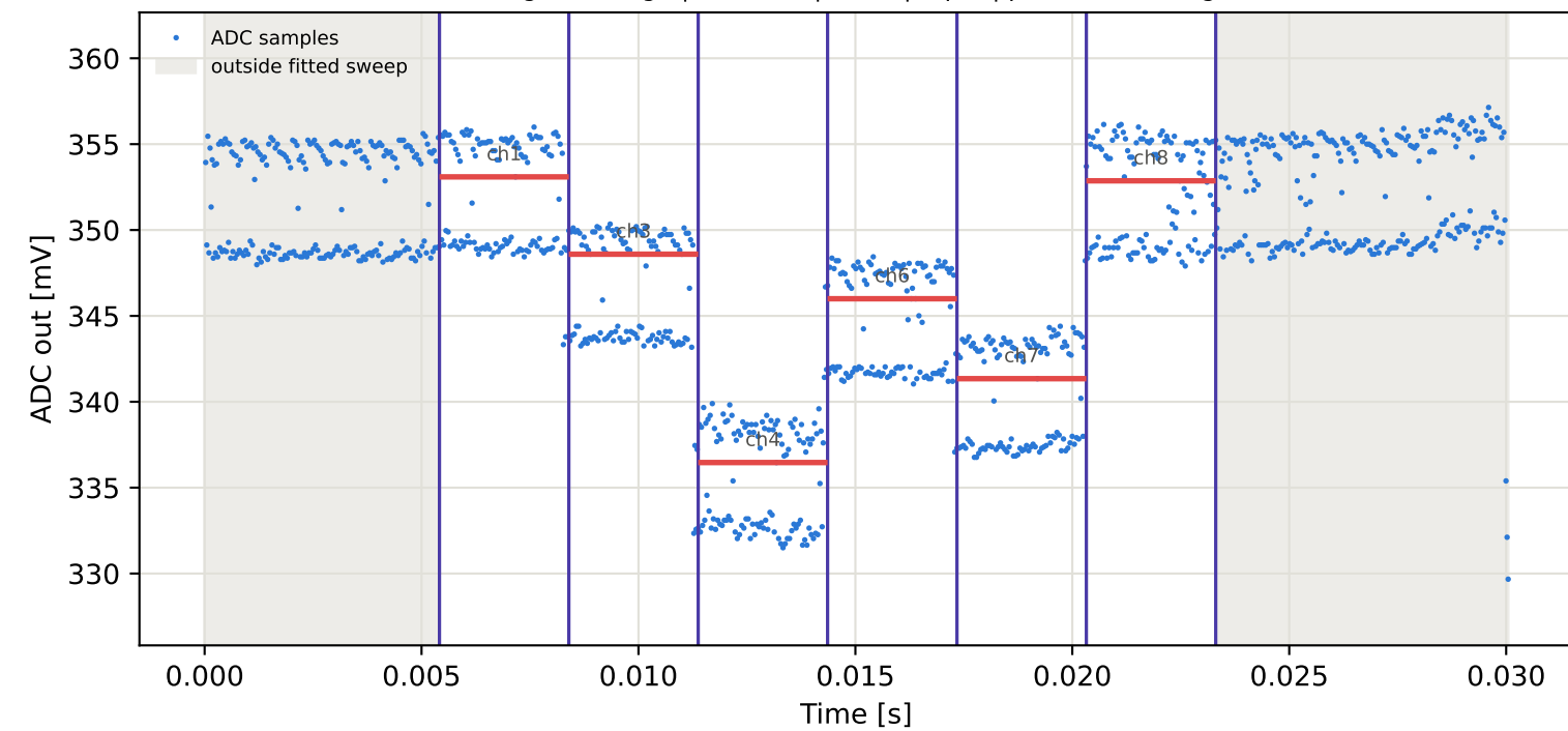
Tag10 &lt;- Tag9 | 955 MHz | run 0 | rep 1 | phase 2.57 deg
