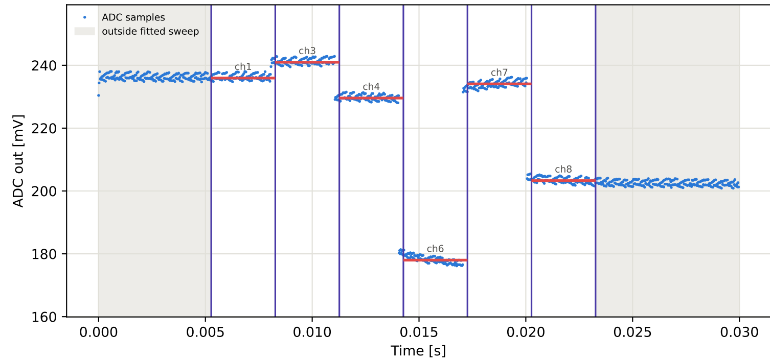
Tag9 &lt;- Tag2 | 915 MHz | run 0 | rep 1 | phase 135.01 deg
