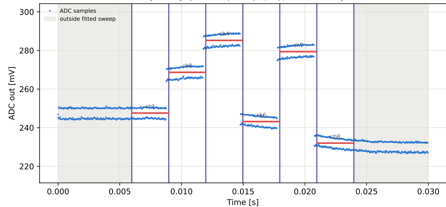
Tag3 &lt;- Tag9 | 925 MHz | run 0 | rep 1 | phase 123.41 deg
