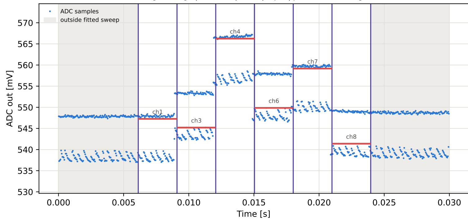
Tag4 &lt;- Tag8 | 955 MHz | run 0 | rep 1 | phase -20.57 deg
