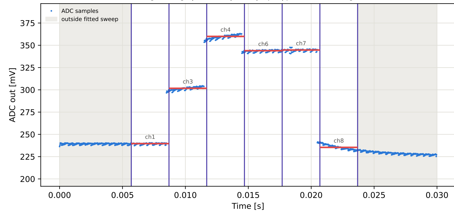
Tag9 &lt;- Tag5 | 895 MHz | run 0 | rep 1 | phase -101.98 deg
