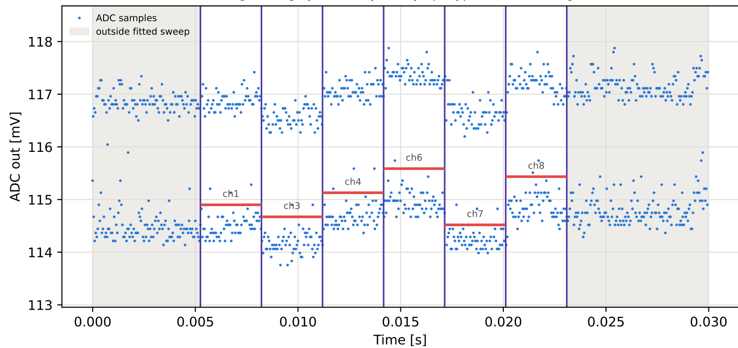
Tag2 &lt;- Tag5 | 775 MHz | run 0 | rep 1 | phase -131.69 deg
