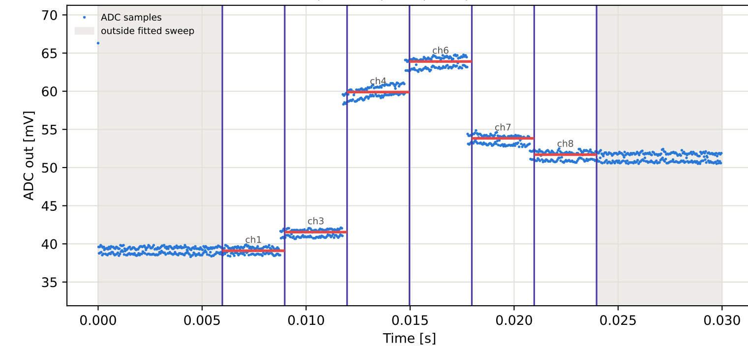
Tag9 &lt;- Tag7 | 855 MHz | run 0 | rep 1 | phase -130.55 deg
