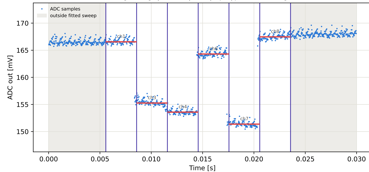
Tag5 &lt;- Tag8 | 825 MHz | run 0 | rep 1 | phase 52.44 deg
