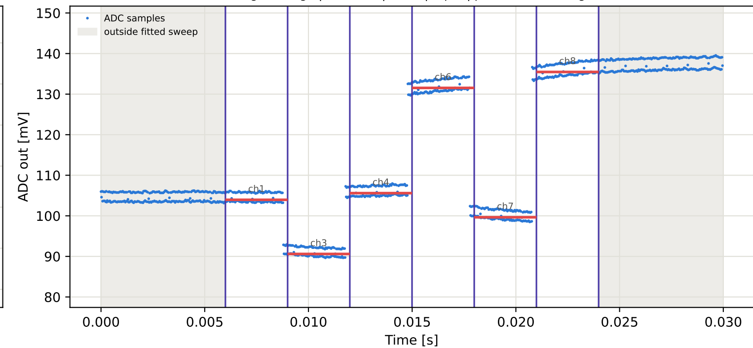
Tag9 &lt;- Tag8 | 865 MHz | run 0 | rep 1 | phase 69.76 deg
