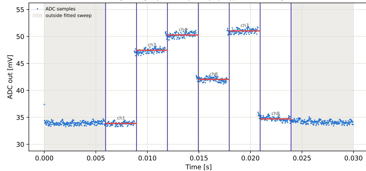
Tag1 &lt;- Tag16 | 845 MHz | run 0 | rep 1 | phase -139.03 deg
