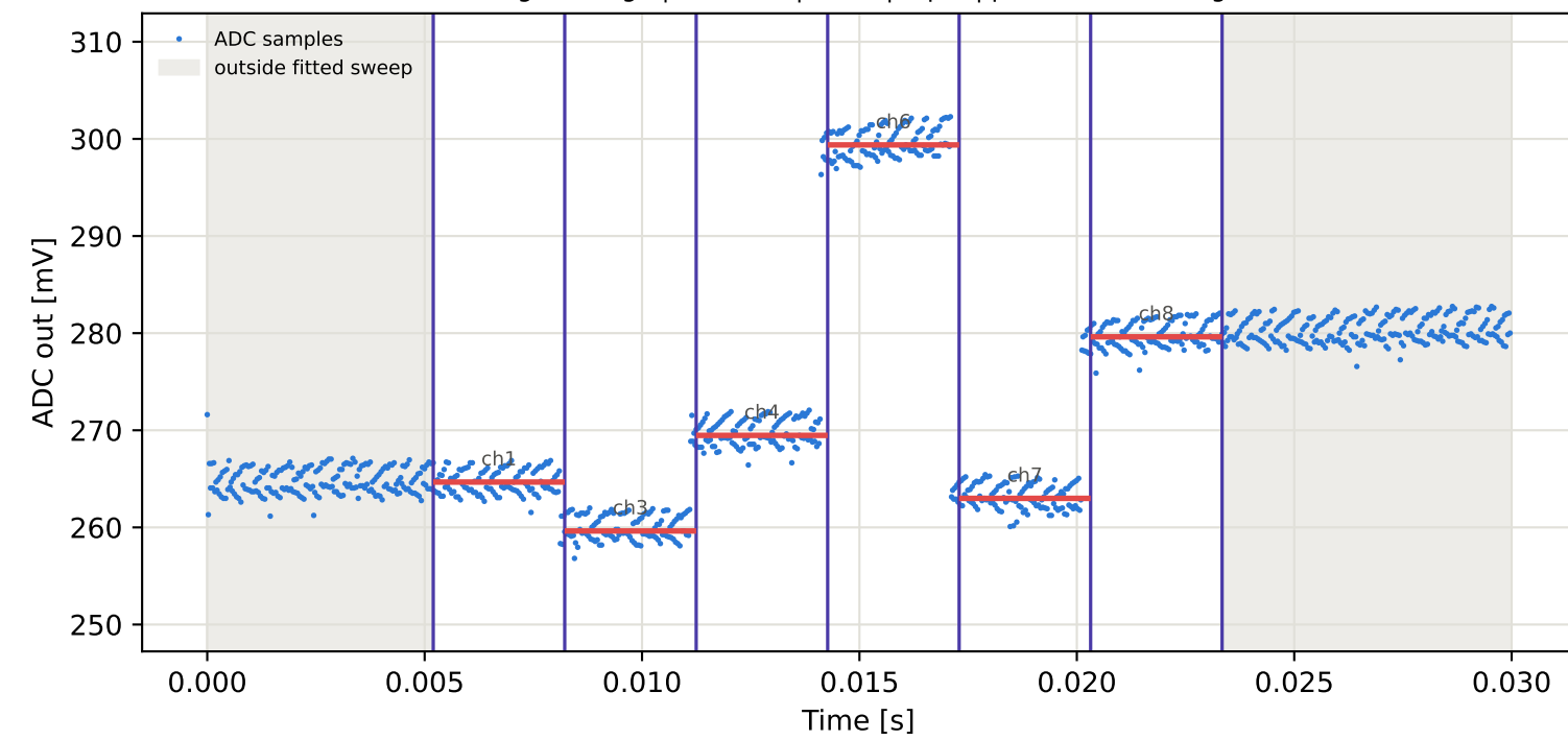
Tag5 &lt;- Tag3 | 965 MHz | run 0 | rep 1 | phase -174.13 deg
