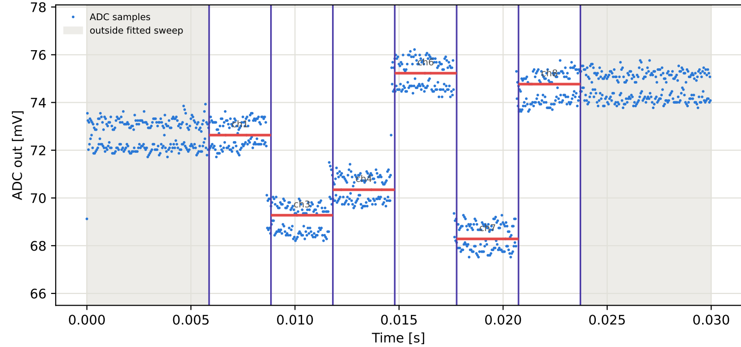
Tag9 &lt;- Tag15 | 795 MHz | run 0 | rep 1 | phase 125.26 deg
