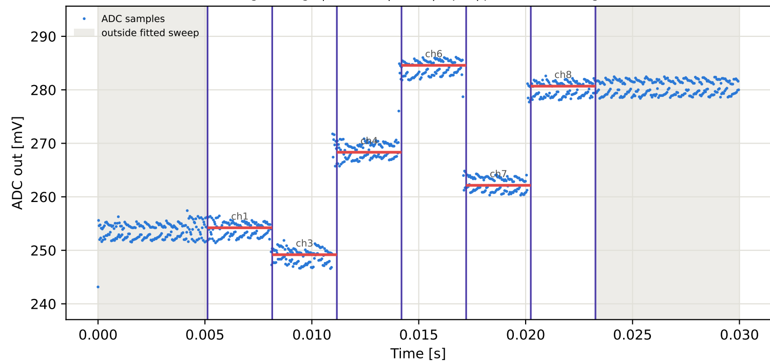
Tag4 &lt;- Tag7 | 855 MHz | run 0 | rep 1 | phase 88.93 deg
