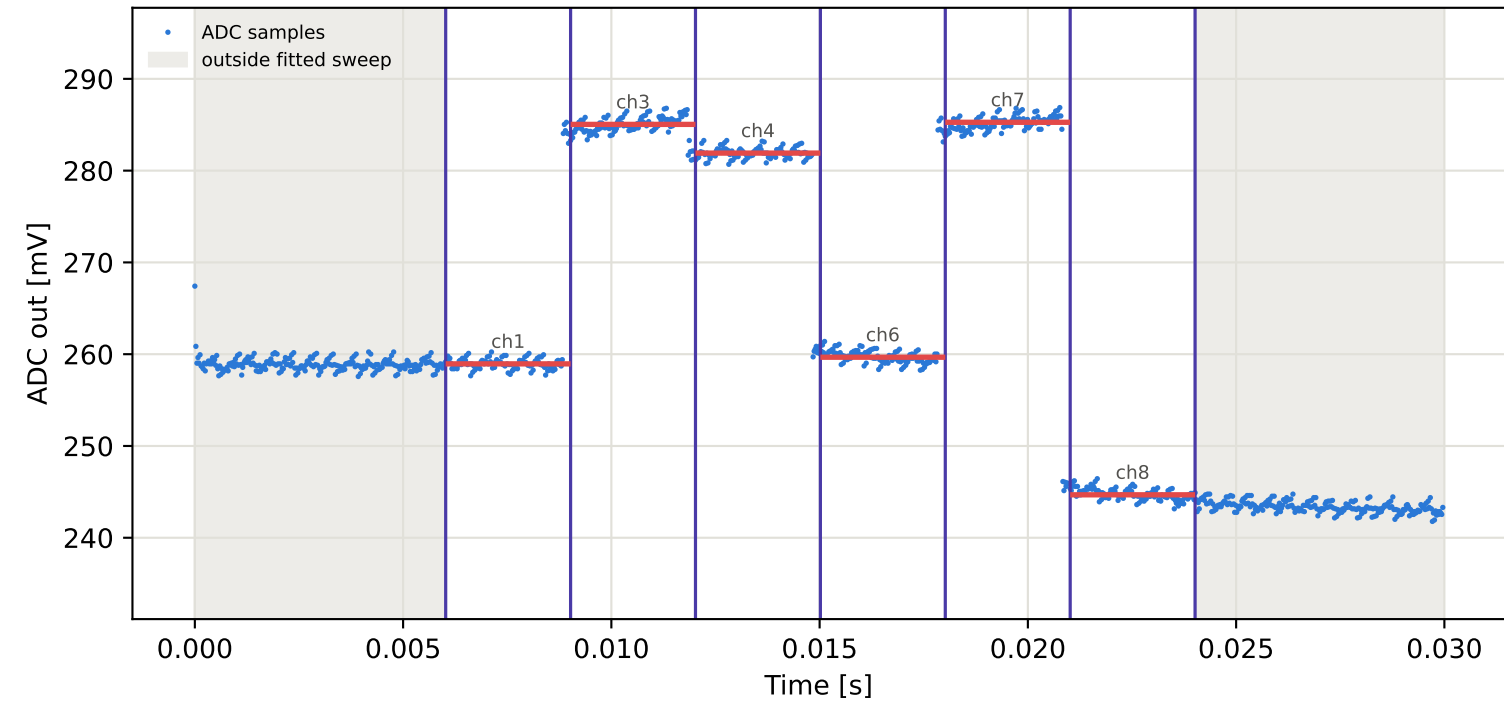
Tag4 &lt;- Tag3 | 855 MHz | run 0 | rep 1 | phase -43.12 deg
