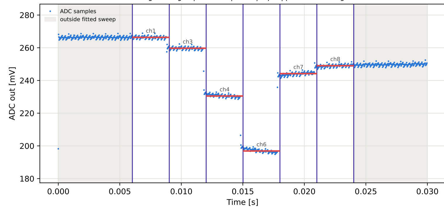
Tag1 &lt;- Tag16 | 925 MHz | run 0 | rep 1 | phase -61.23 deg
