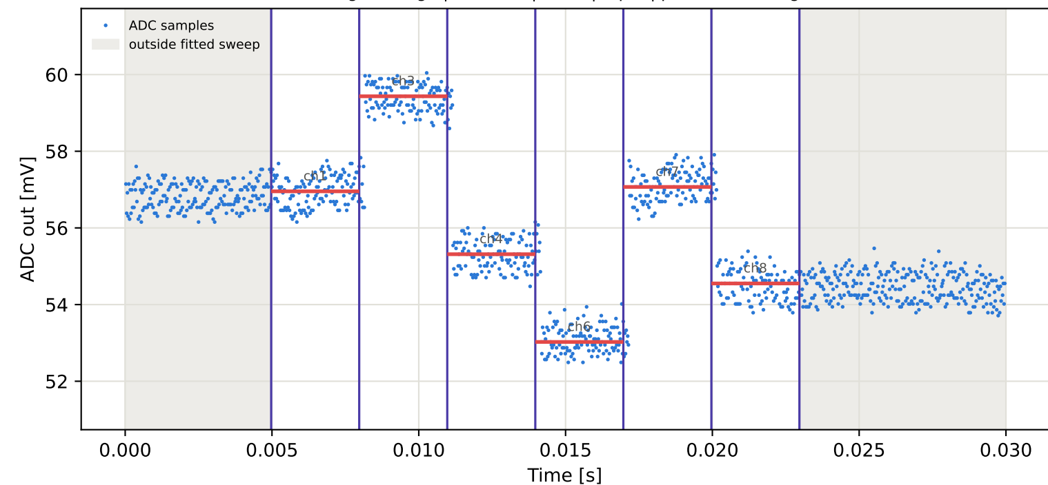
Tag9 &lt;- Tag8 | 805 MHz | run 0 | rep 1 | phase 13.07 deg
