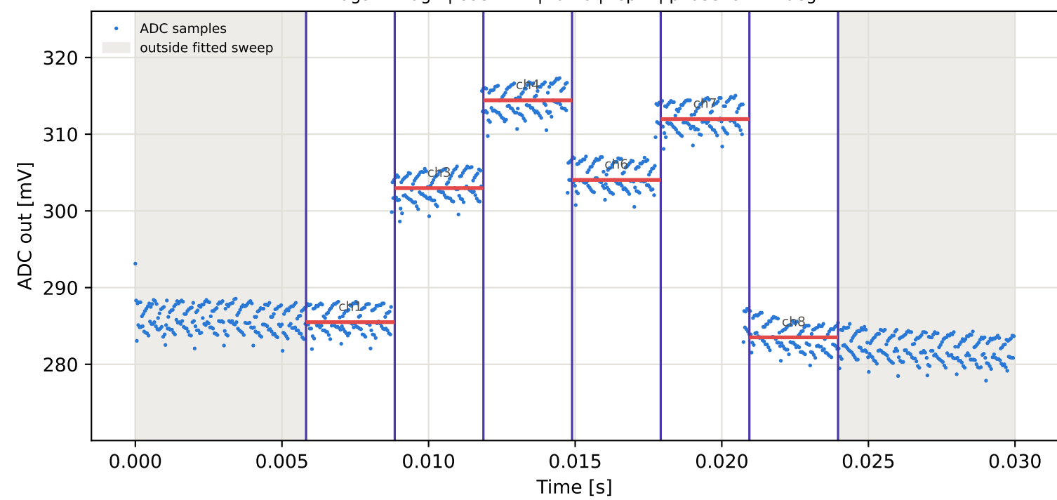
Tag9 &lt;- Tag15 | 895 MHz | run 0 | rep 1 | phase -93.08 deg
