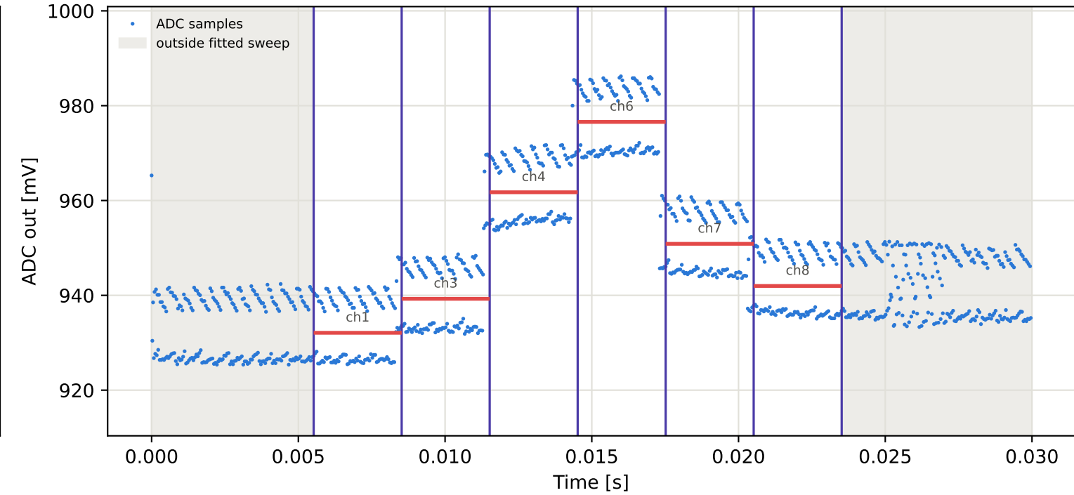
Tag16 &lt;- Tag7 | 935 MHz | run 0 | rep 1 | phase -162.14 deg
