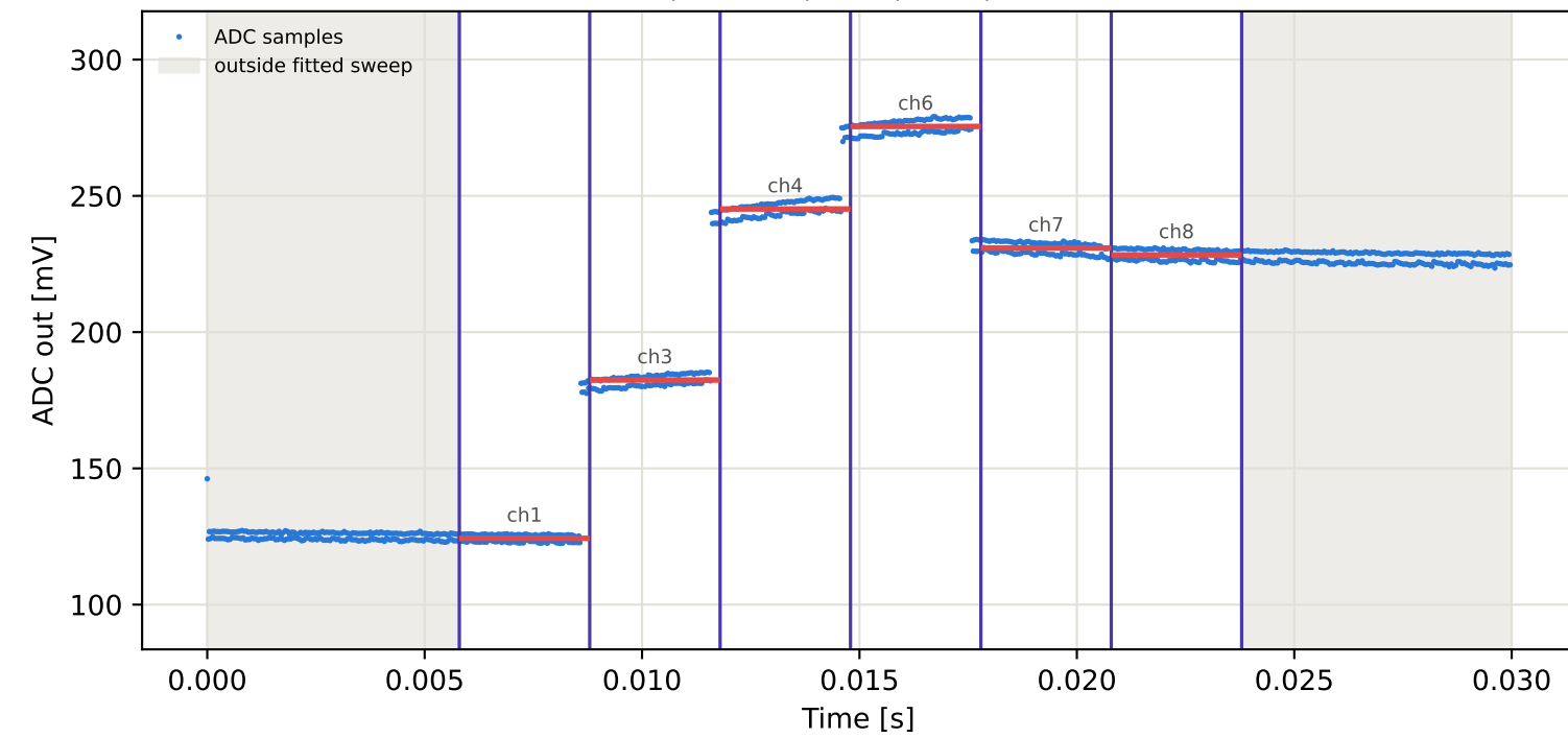
Tag9 &lt;- Tag16 | 875 MHz | run 0 | rep 1 | phase -130.39 deg
