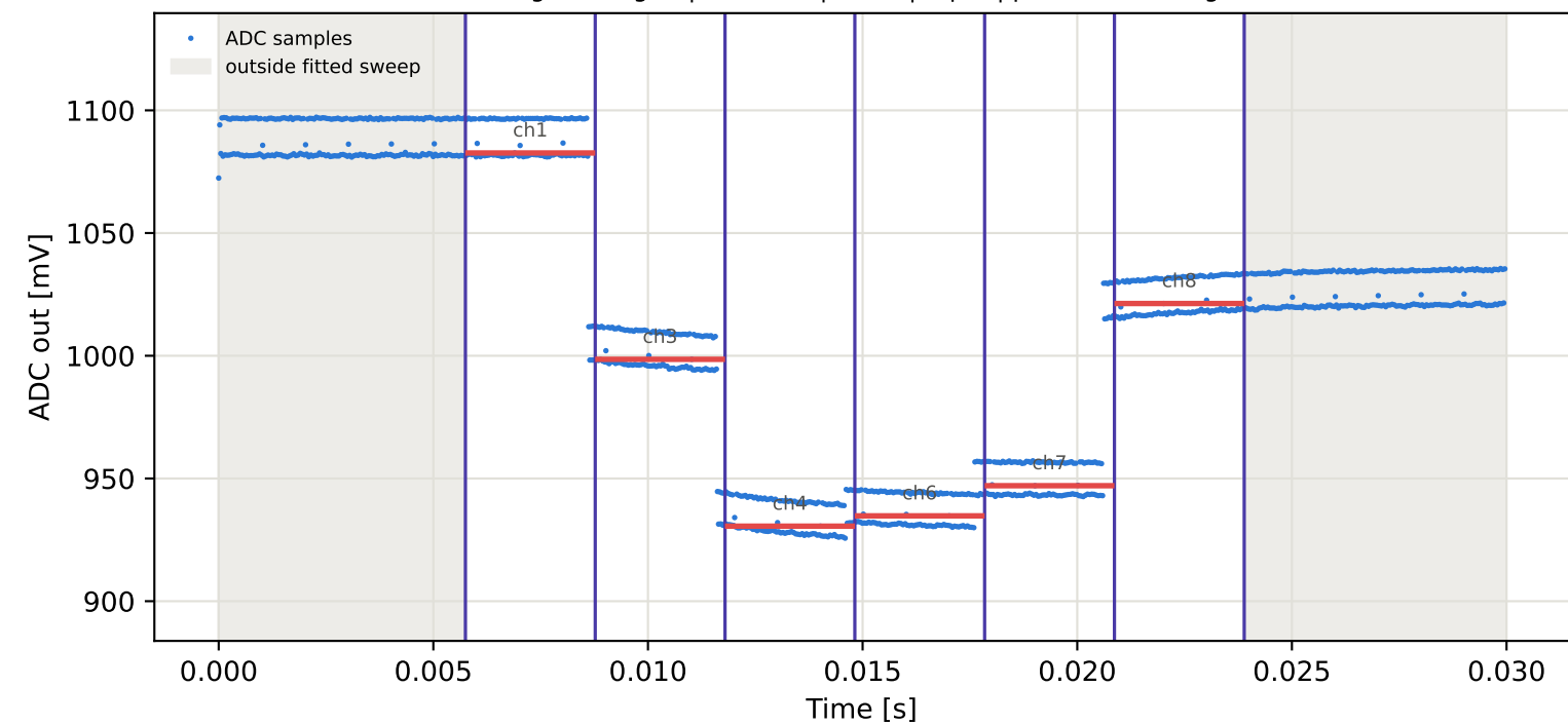
Tag8 &lt;- Tag16 | 875 MHz | run 0 | rep 1 | phase 66.80 deg
