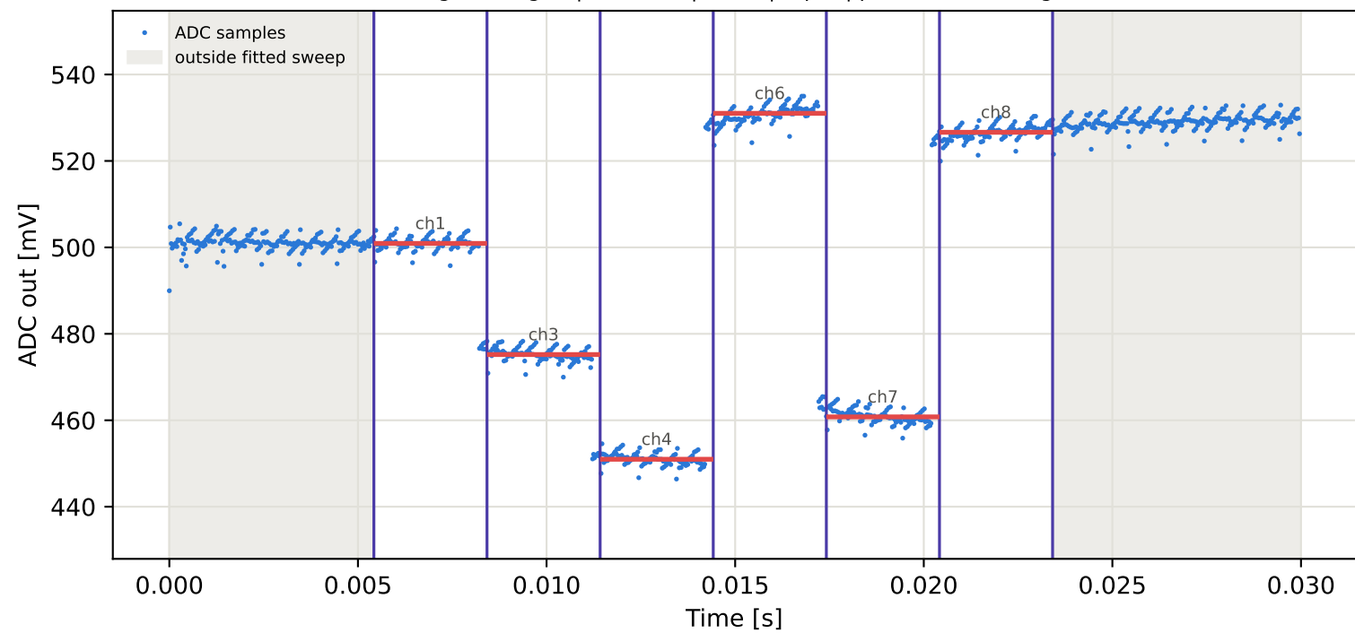
Tag4 &lt;- Tag16 | 935 MHz | run 0 | rep 1 | phase -10.95 deg
