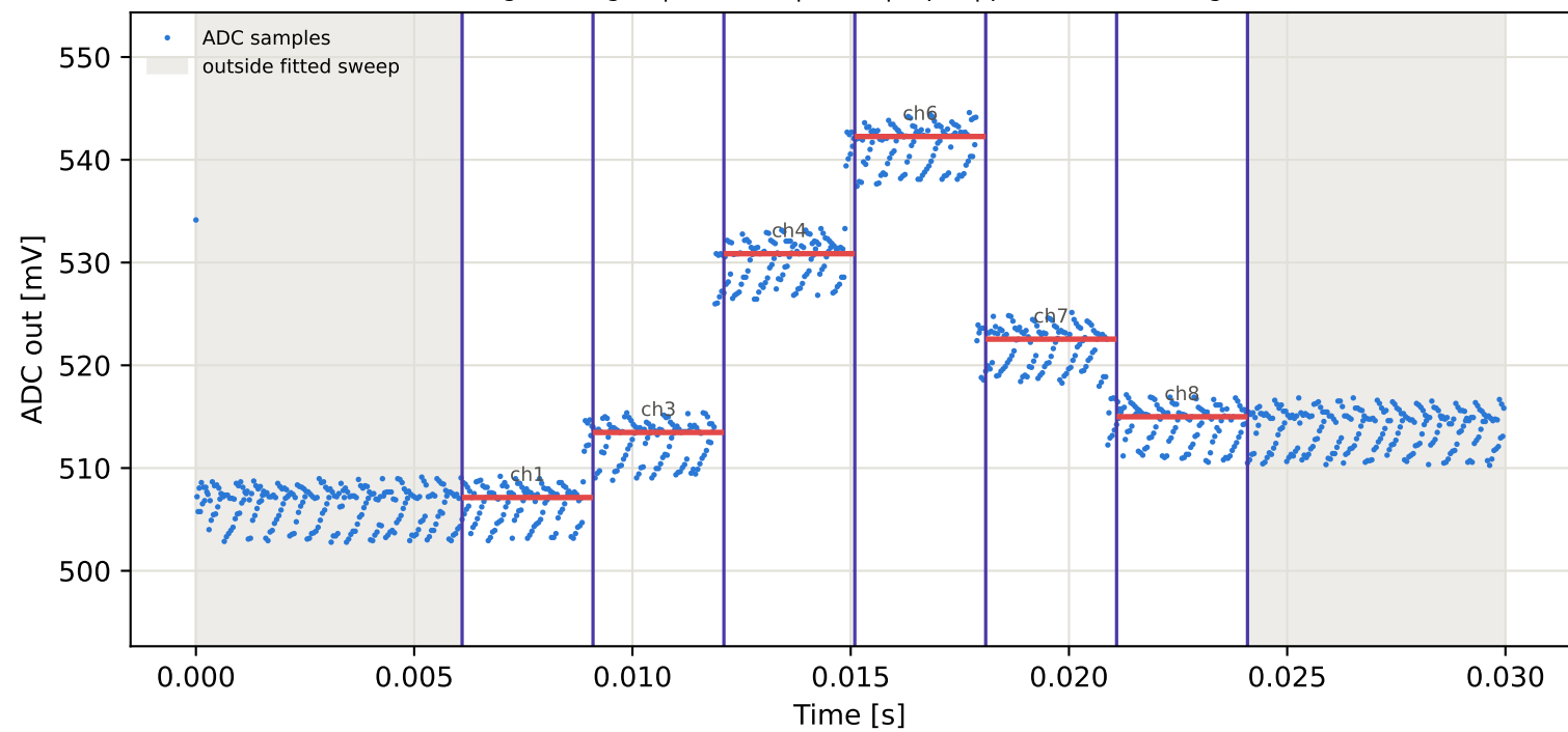
Tag5 &lt;- Tag2 | 935 MHz | run 0 | rep 1 | phase 95.38 deg
