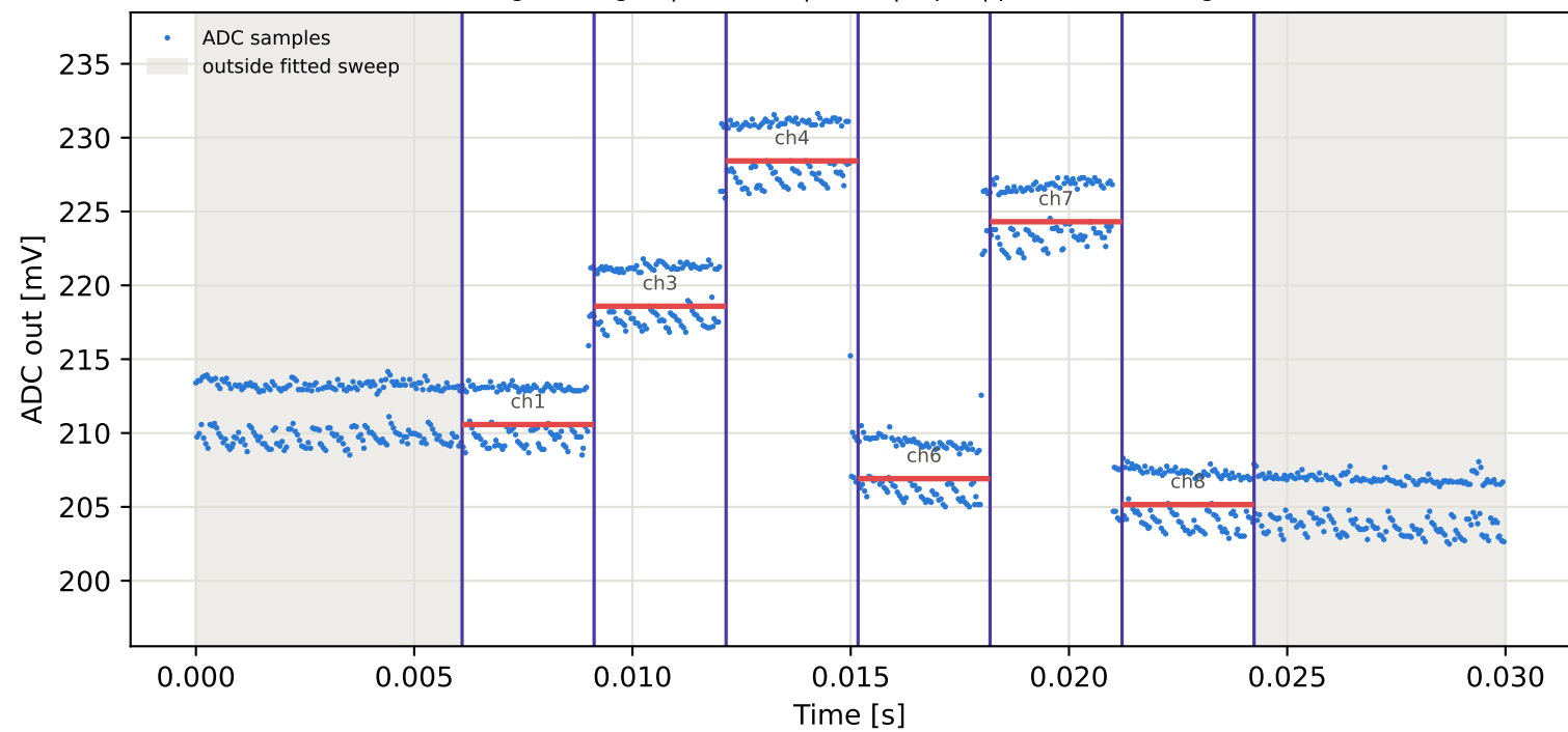
Tag6 &lt;- Tag3 | 955 MHz | run 0 | rep 1 | phase -37.96 deg
