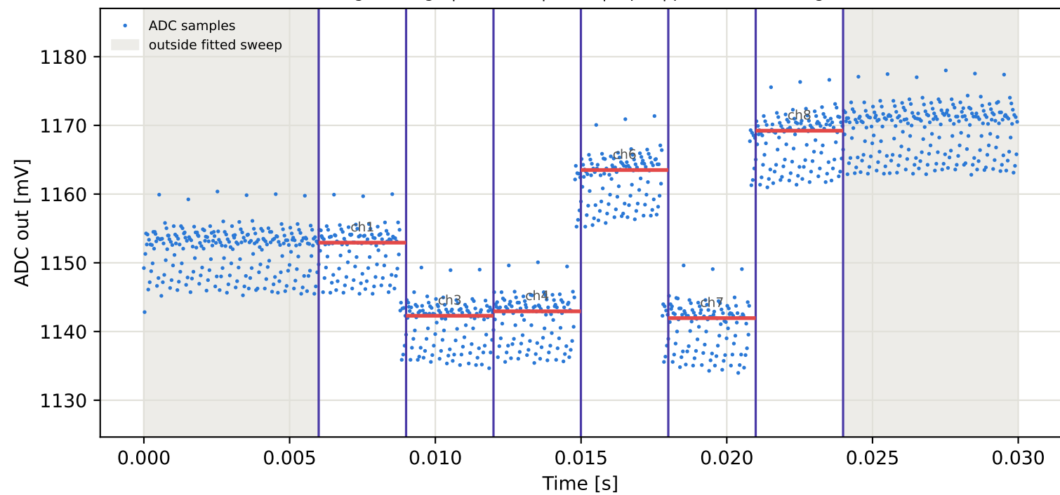
Tag3 &lt;- Tag15 | 895 MHz | run 0 | rep 1 | phase -2.67 deg
