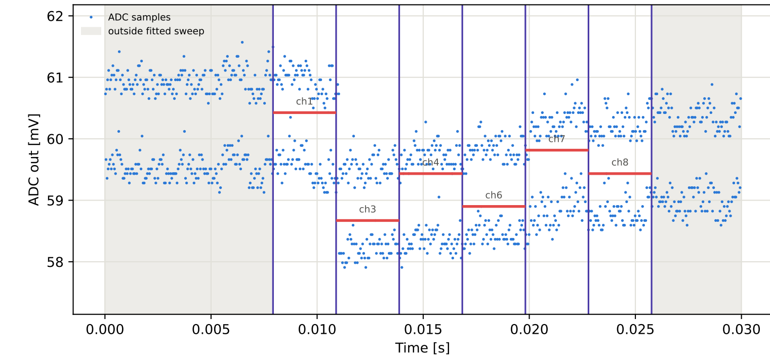
Tag4 &lt;- Tag9 | 795 MHz | run 0 | rep 1 | phase -71.54 deg
