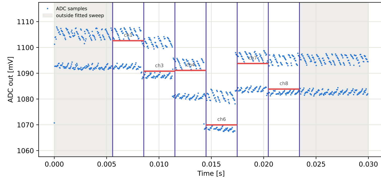
Tag16 &lt;- Tag10 | 905 MHz | run 0 | rep 1 | phase 74.70 deg
