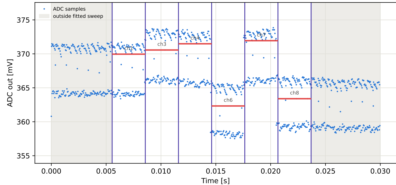
Tag7 &lt;- Tag15 | 915 MHz | run 0 | rep 1 | phase -124.98 deg
