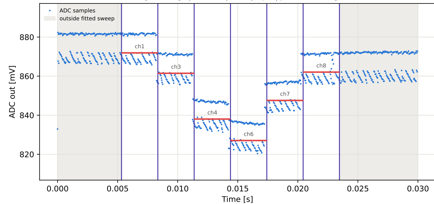
Tag2 &lt;- Tag10 | 925 MHz | run 0 | rep 1 | phase 138.09 deg
