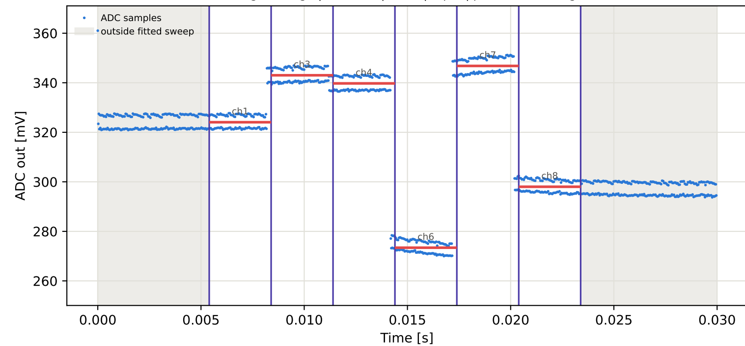
Tag4 &lt;- Tag7 | 985 MHz | run 0 | rep 1 | phase 166.10 deg
