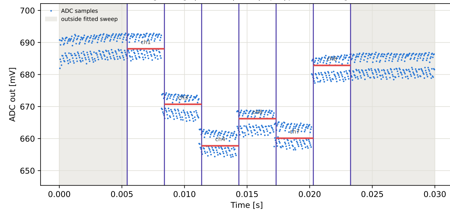
Tag3 &lt;- Tag6 | 865 MHz | run 0 | rep 1 | phase -151.76 deg
