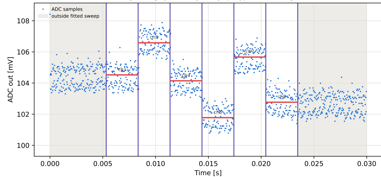
Tag5 &lt;- Tag8 | 795 MHz | run 0 | rep 1 | phase -20.58 deg
