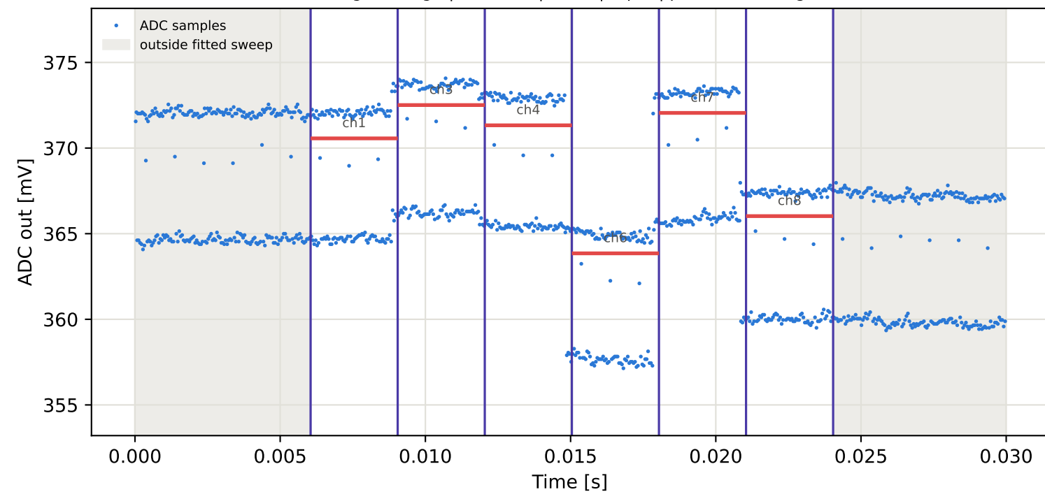
Tag8 &lt;- Tag10 | 915 MHz | run 0 | rep 1 | phase -127.32 deg
