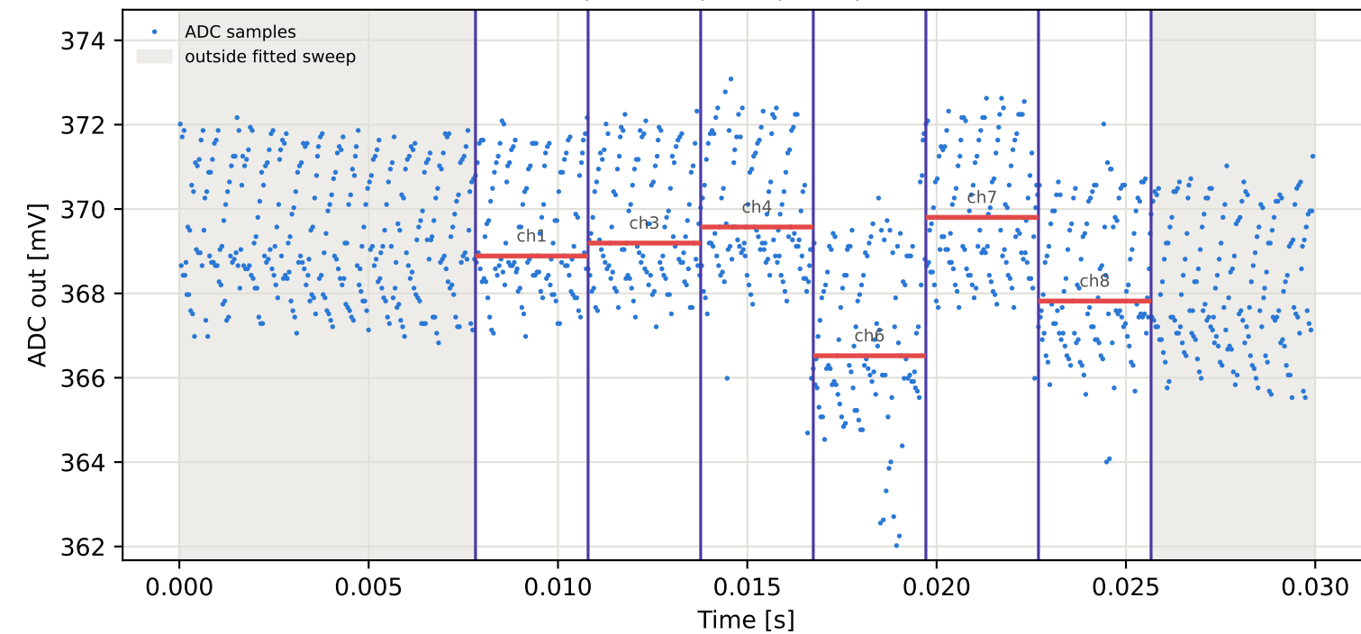
Tag4 &lt;- Tag2 | 965 MHz | run 0 | rep 1 | phase -18.14 deg
