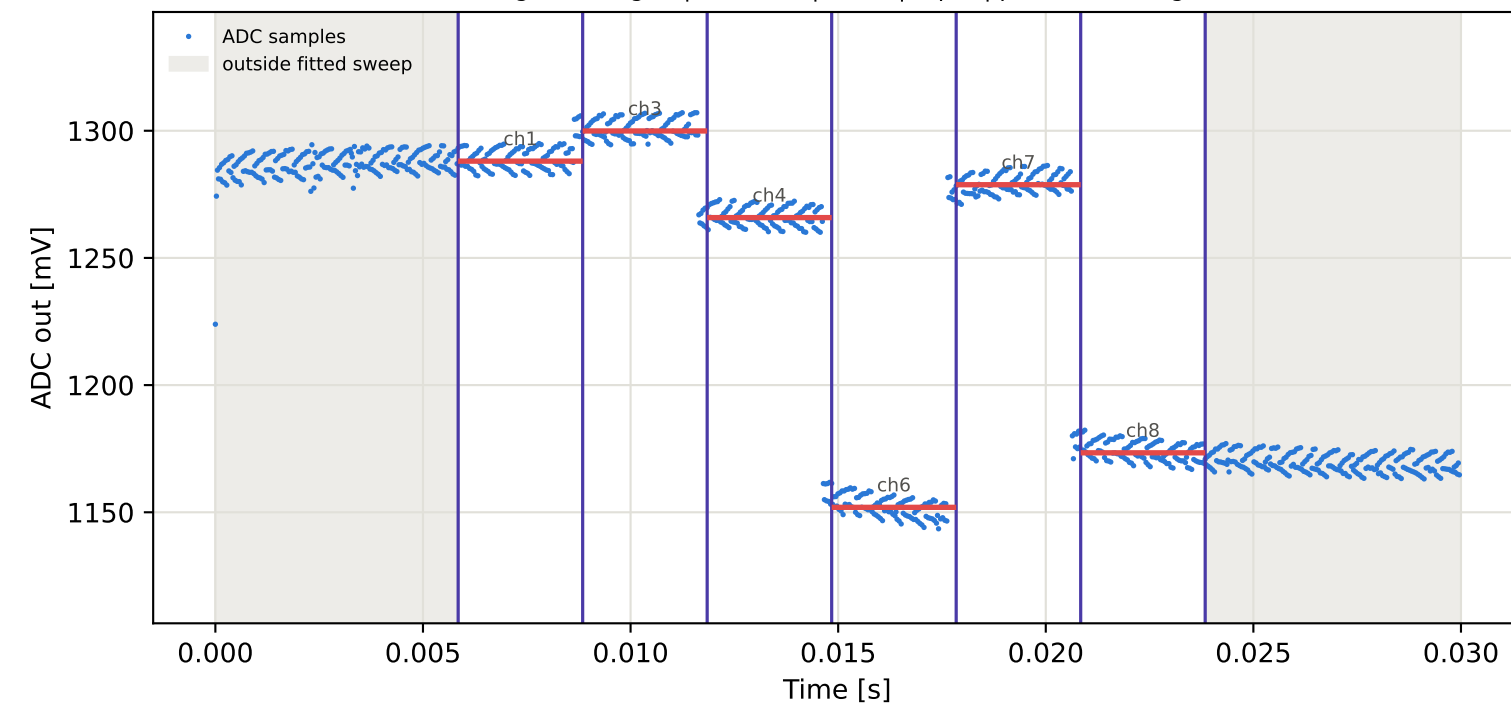
Tag15 &lt;- Tag3 | 895 MHz | run 0 | rep 1 | phase 177.14 deg
