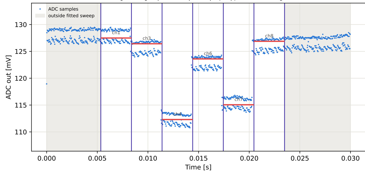
Tag2 &lt;- Tag16 | 775 MHz | run 0 | rep 1 | phase 99.11 deg
