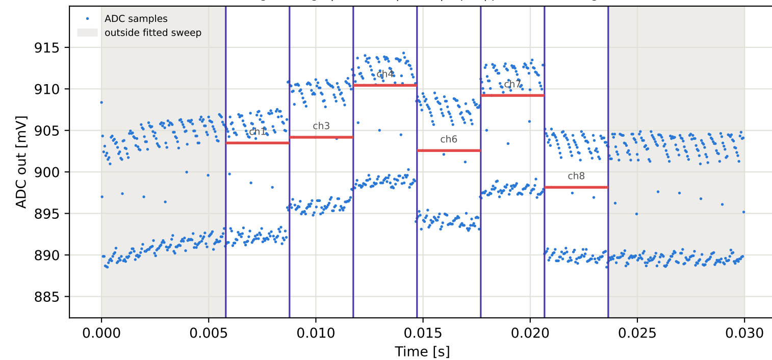
Tag5 &lt;- Tag8 | 905 MHz | run 0 | rep 1 | phase 55.65 deg
