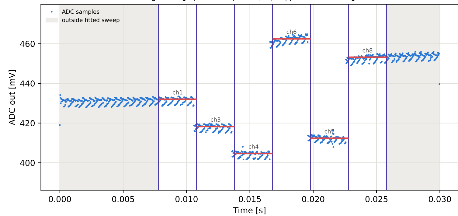
Tag7 &lt;- Tag4 | 965 MHz | run 0 | rep 1 | phase 80.62 deg
