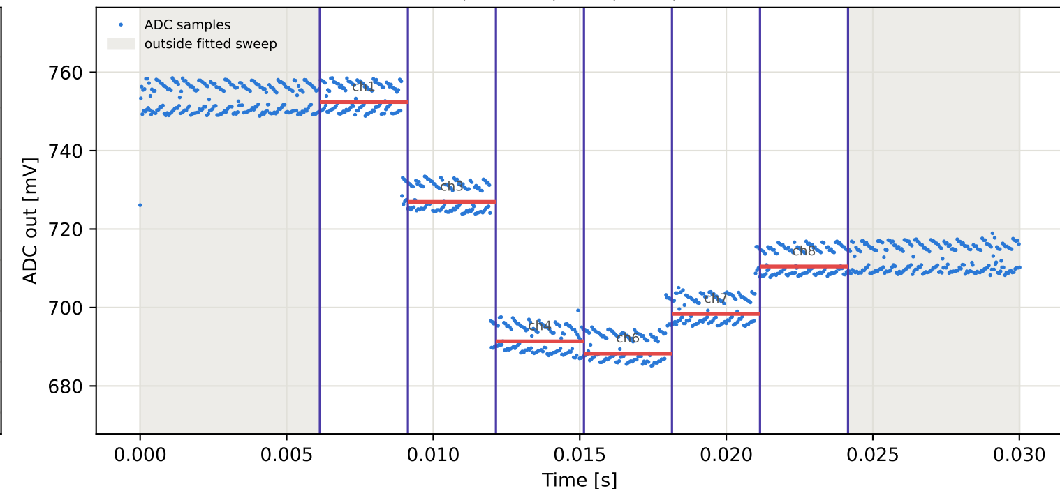
Tag2 &lt;- Tag16 | 855 MHz | run 0 | rep 1 | phase 58.65 deg
