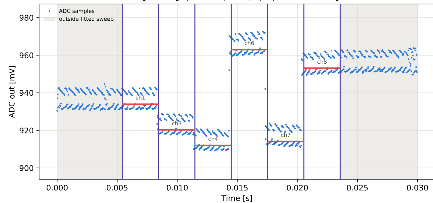
Tag16 &lt;- Tag4 | 865 MHz | run 0 | rep 1 | phase -42.72 deg
