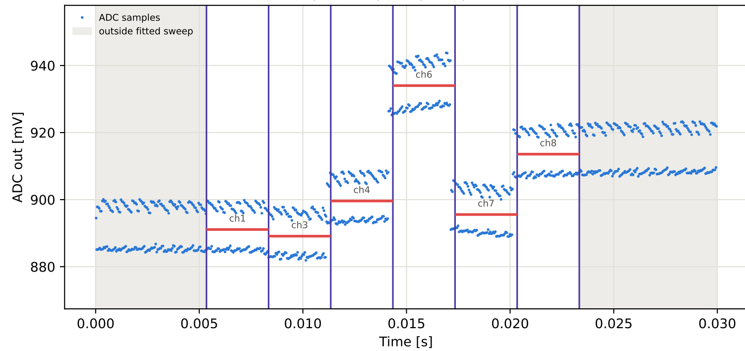
Tag5 &lt;- Tag4 | 905 MHz | run 0 | rep 1 | phase -165.87 deg
