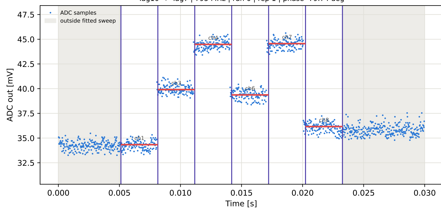
Tag10 &lt;- Tag9 | 795 MHz | run 0 | rep 1 | phase -170.10 deg
