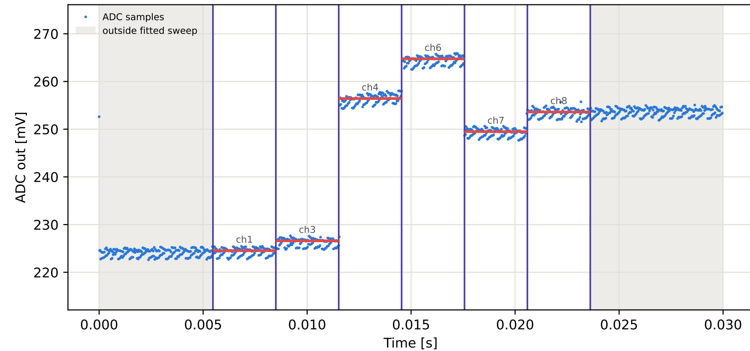
Tag9 &lt;- Tag16 | 835 MHz | run 0 | rep 1 | phase 163.40 deg
