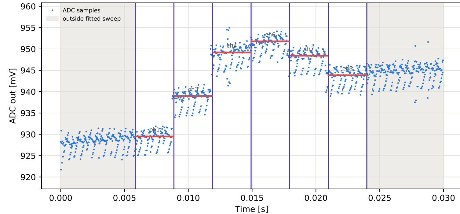
Tag8 &lt;- Tag15 | 875 MHz | run 0 | rep 1 | phase -139.37 deg
