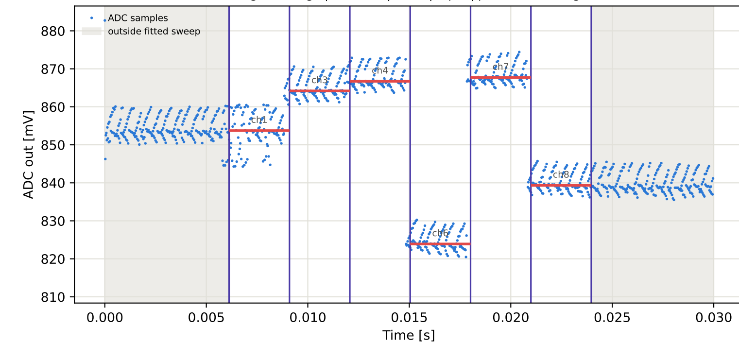
Tag15 &lt;- Tag5 | 985 MHz | run 0 | rep 1 | phase 117.80 deg
