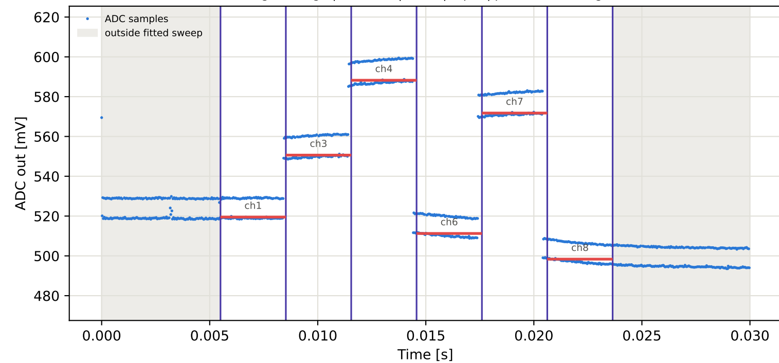
Tag8 &lt;- Tag5 | 945 MHz | run 0 | rep 1 | phase 106.40 deg
