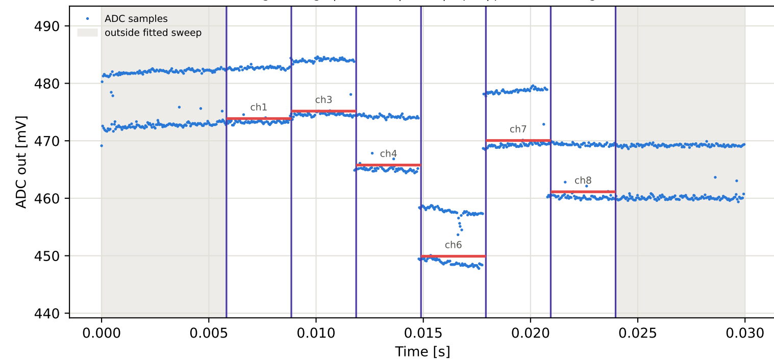
Tag6 &lt;- Tag9 | 905 MHz | run 0 | rep 1 | phase 60.95 deg
