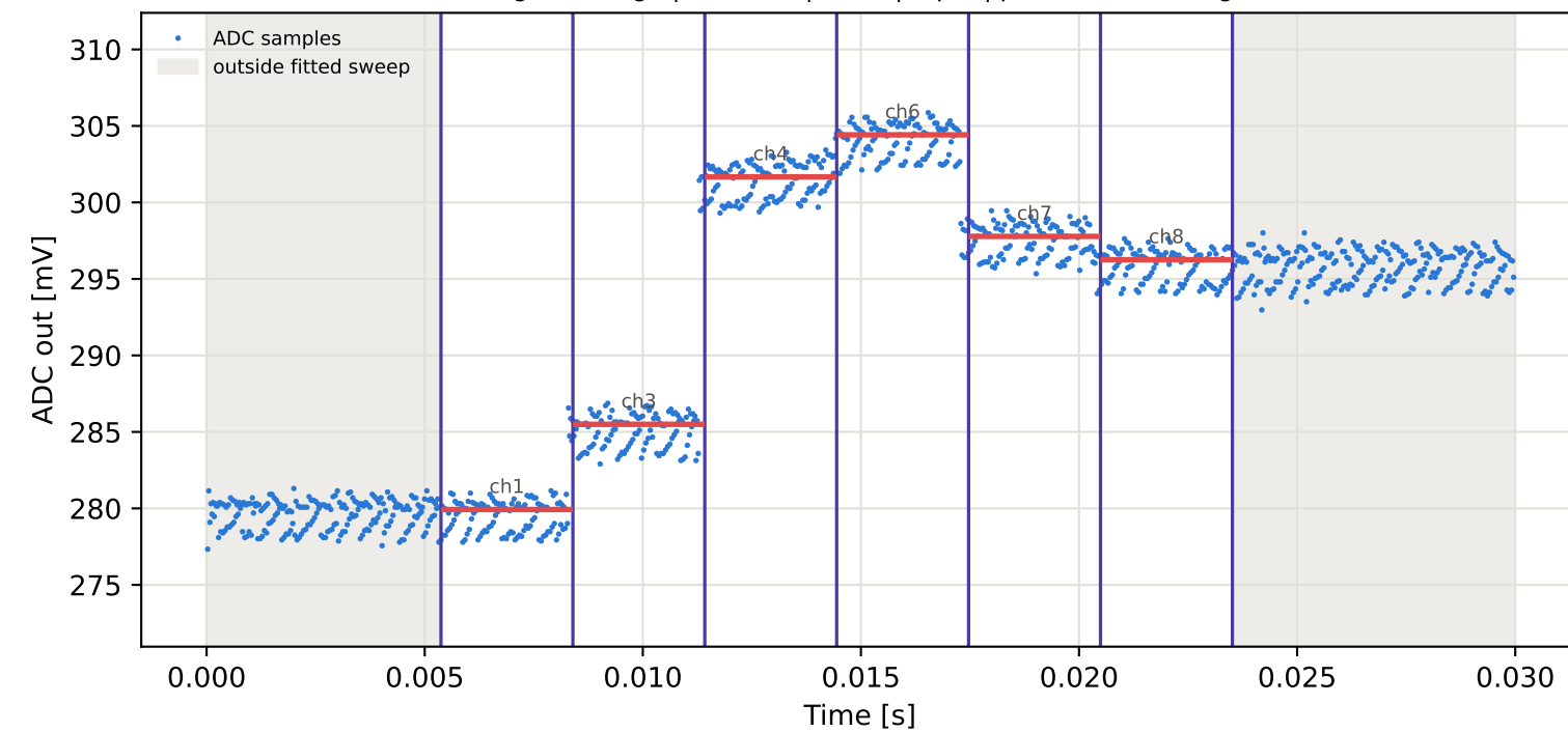
Tag15 &lt;- Tag1 | 855 MHz | run 0 | rep 1 | phase 10.68 deg
