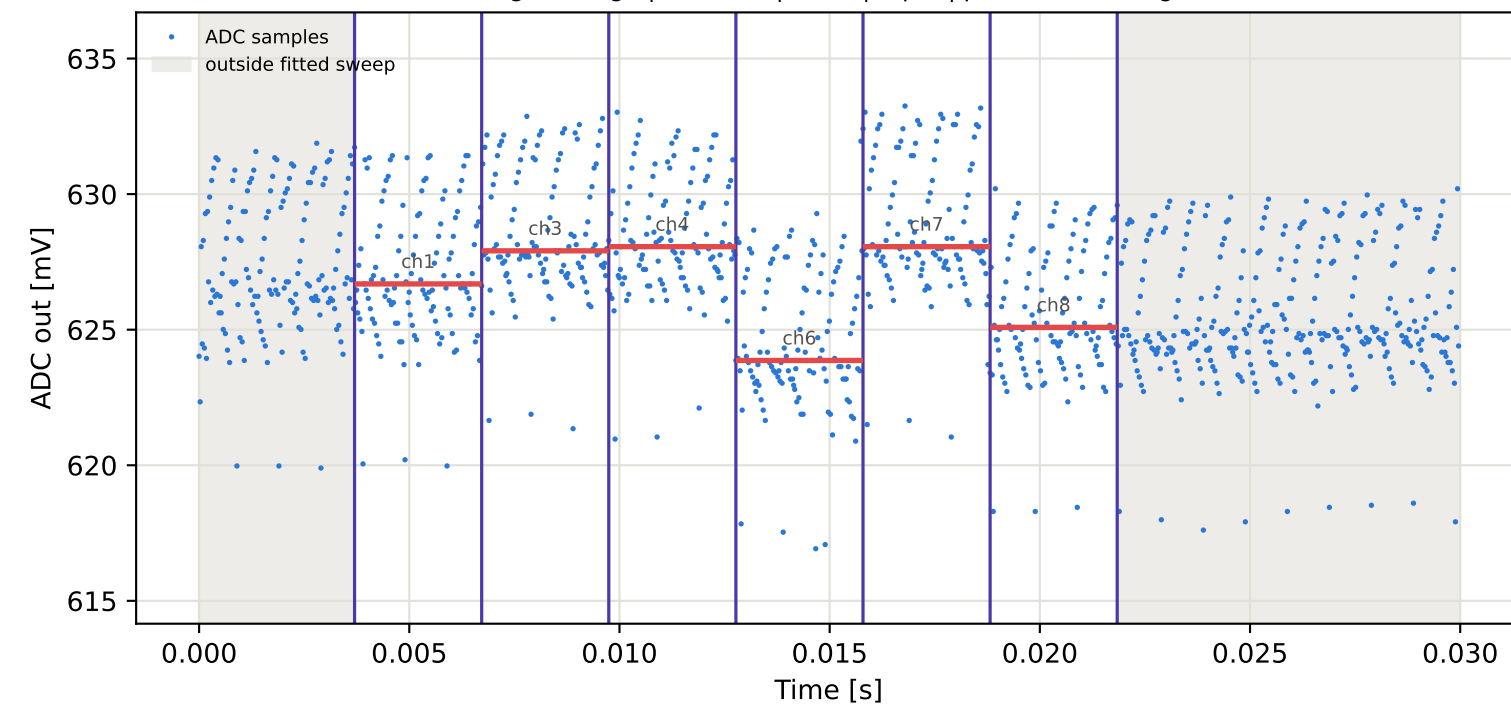
Tag2 &lt;- Tag15 | 965 MHz | run 0 | rep 1 | phase 114.56 deg
