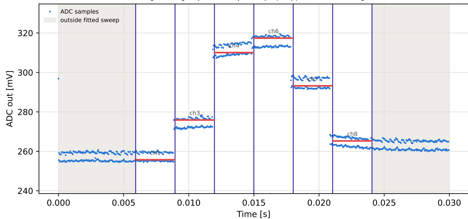
Tag6 &lt;- Tag10 | 925 MHz | run 0 | rep 1 | phase -125.34 deg
