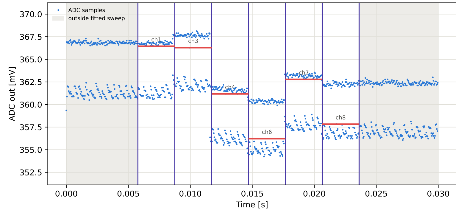
Tag2 &lt;- Tag16 | 825 MHz | run 0 | rep 1 | phase 90.36 deg
