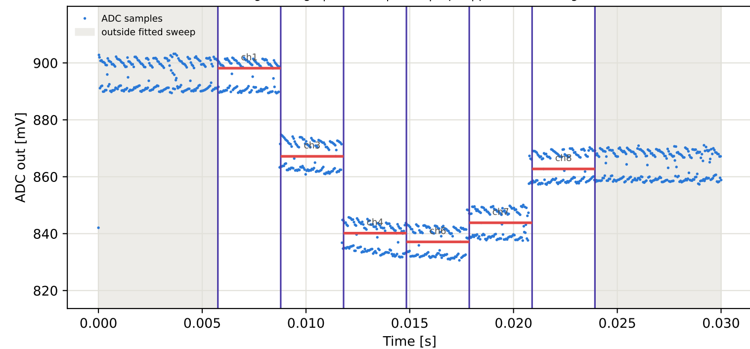
Tag6 &lt;- Tag1 | 875 MHz | run 0 | rep 1 | phase 61.20 deg
