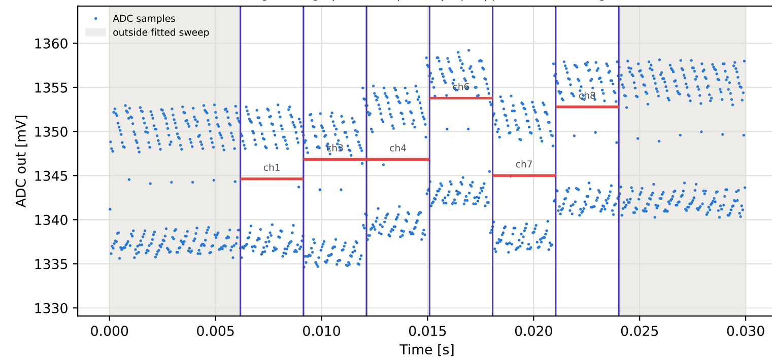
Tag3 &lt;- Tag10 | 875 MHz | run 0 | rep 1 | phase -142.51 deg
