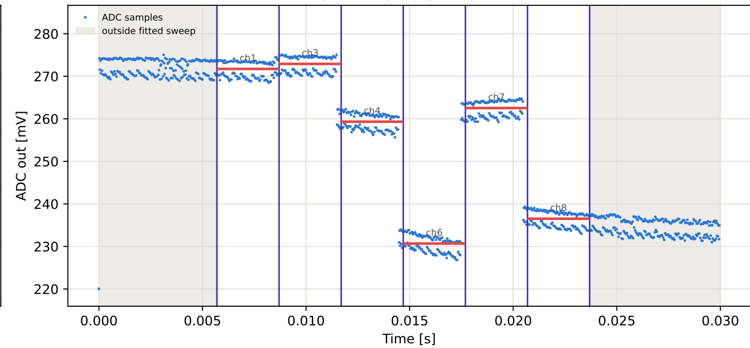
Tag4 &lt;- Tag3 | 875 MHz | run 0 | rep 1 | phase 15.13 deg
