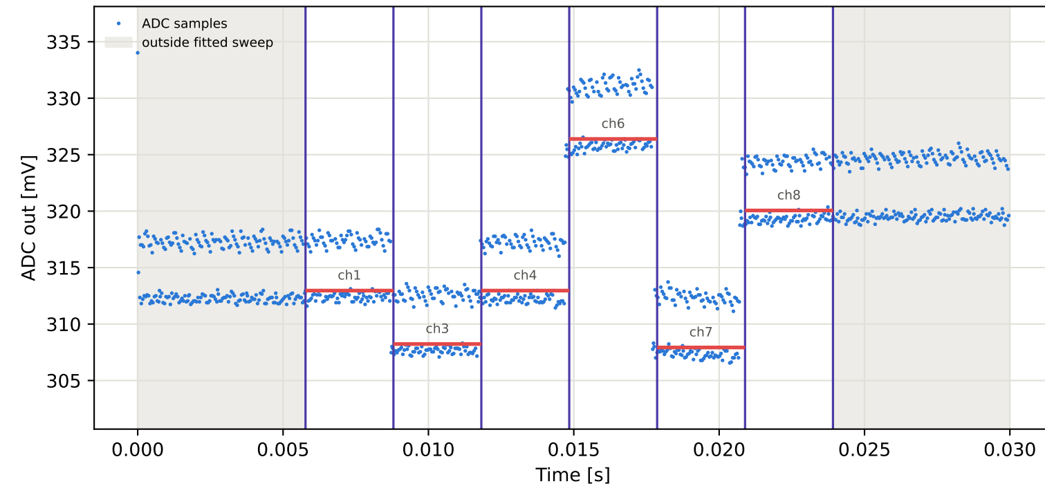
Tag3 &lt;- Tag8 | 995 MHz | run 0 | rep 1 | phase -51.18 deg
