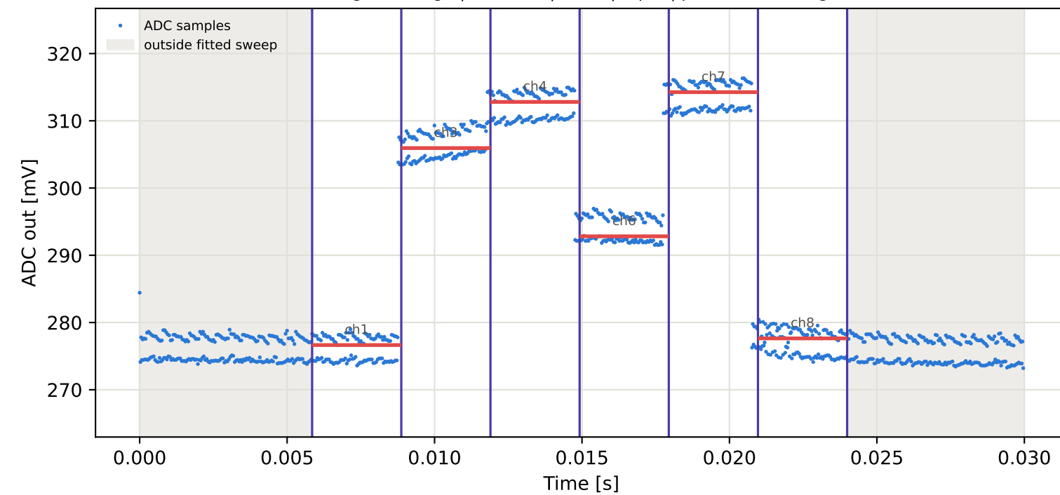
Tag10 &lt;- Tag8 | 855 MHz | run 0 | rep 1 | phase -128.32 deg
