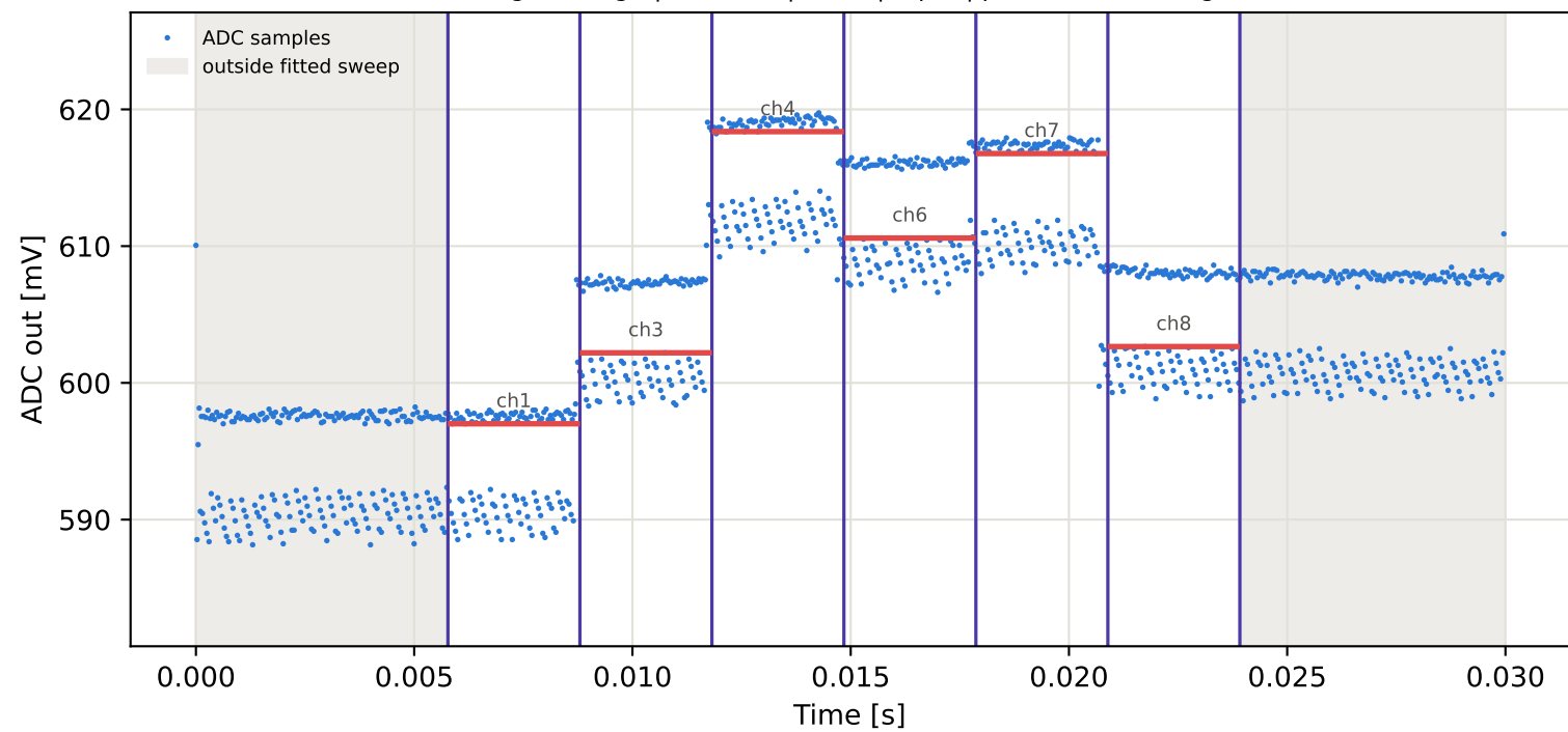
Tag3 &lt;- Tag7 | 845 MHz | run 0 | rep 1 | phase -114.12 deg
