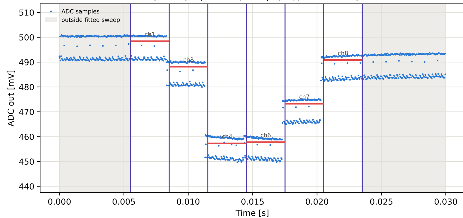
Tag3 &lt;- Tag2 | 945 MHz | run 0 | rep 1 | phase -161.65 deg
