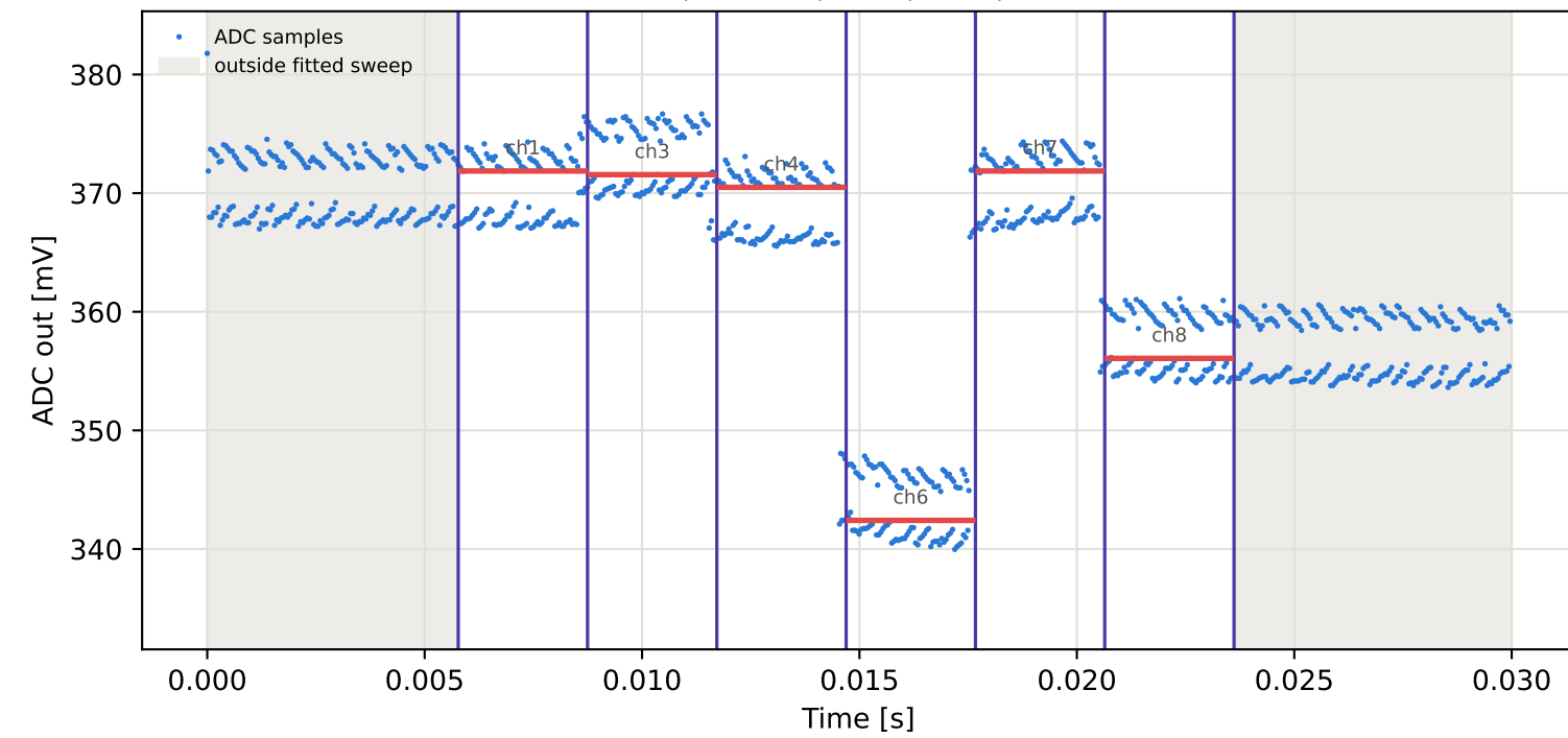
Tag7 &lt;- Tag5 | 915 MHz | run 0 | rep 1 | phase 2.13 deg
