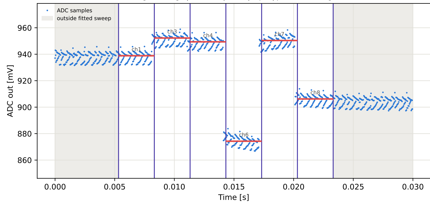
Tag15 &lt;- Tag4 | 925 MHz | run 0 | rep 1 | phase -61.02 deg
