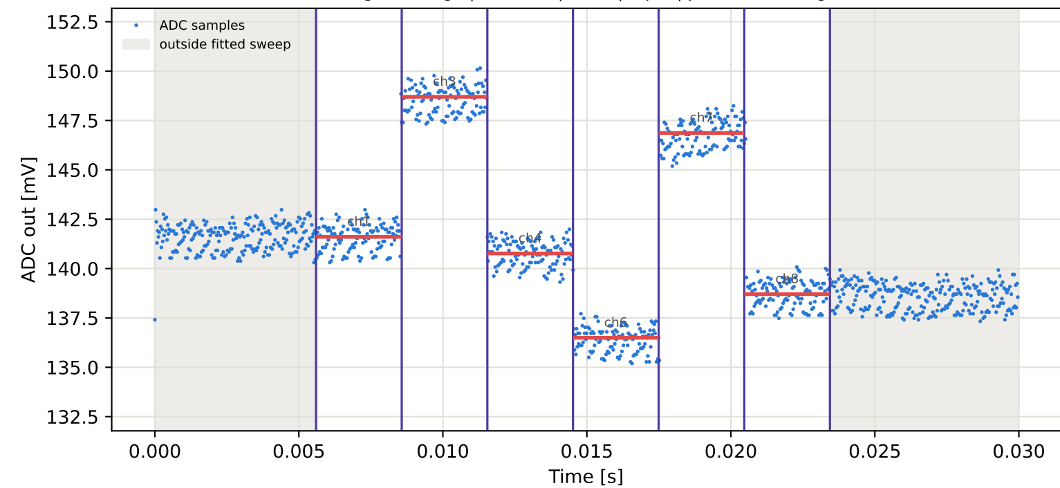
Tag2 &lt;- Tag1 | 775 MHz | run 0 | rep 1 | phase -23.60 deg
