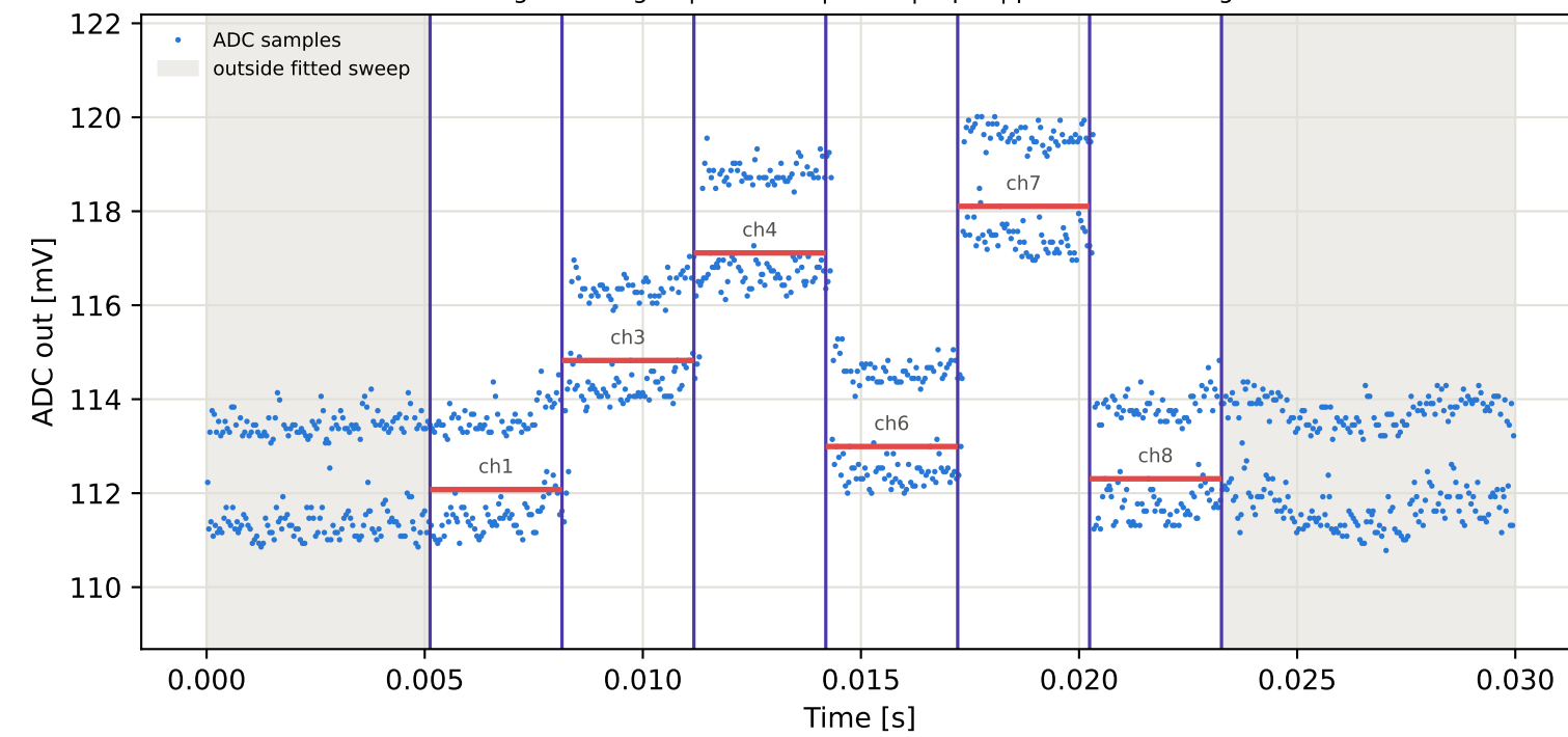
Tag10 &lt;- Tag2 | 785 MHz | run 0 | rep 1 | phase 151.02 deg
