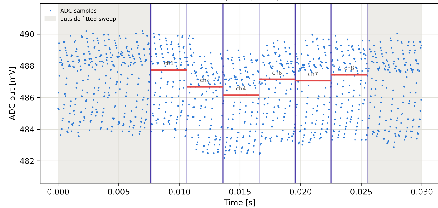
Tag2 &lt;- Tag6 | 975 MHz | run 0 | rep 1 | phase 97.76 deg
