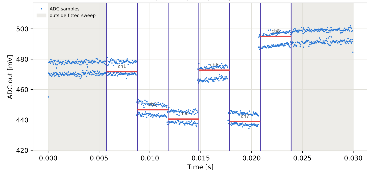
Tag4 &lt;- Tag15 | 885 MHz | run 0 | rep 1 | phase -128.34 deg
