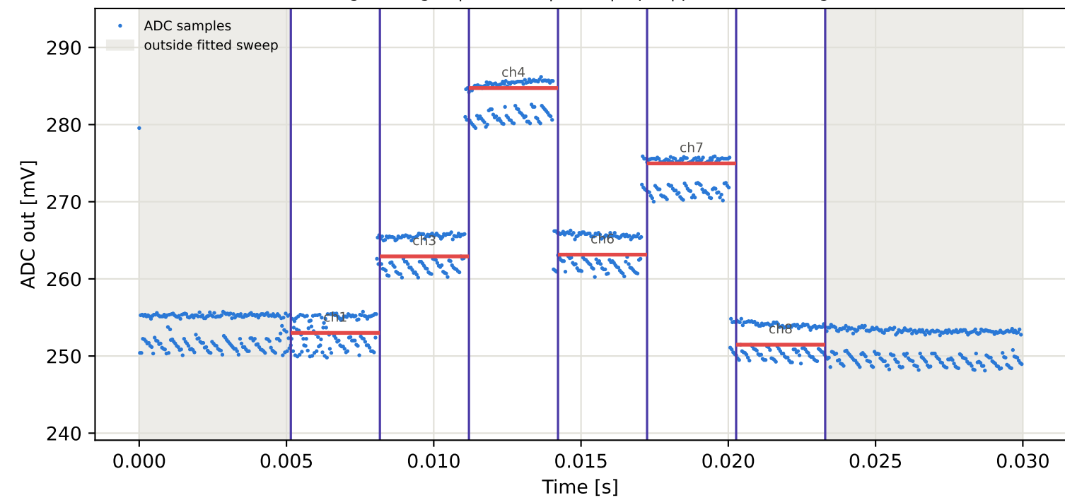
Tag5 &lt;- Tag2 | 965 MHz | run 0 | rep 1 | phase 164.10 deg
