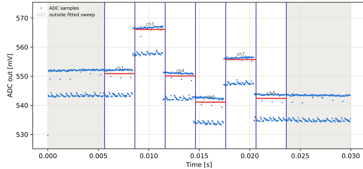
Tag15 &lt;- Tag5 | 825 MHz | run 0 | rep 1 | phase -108.39 deg
