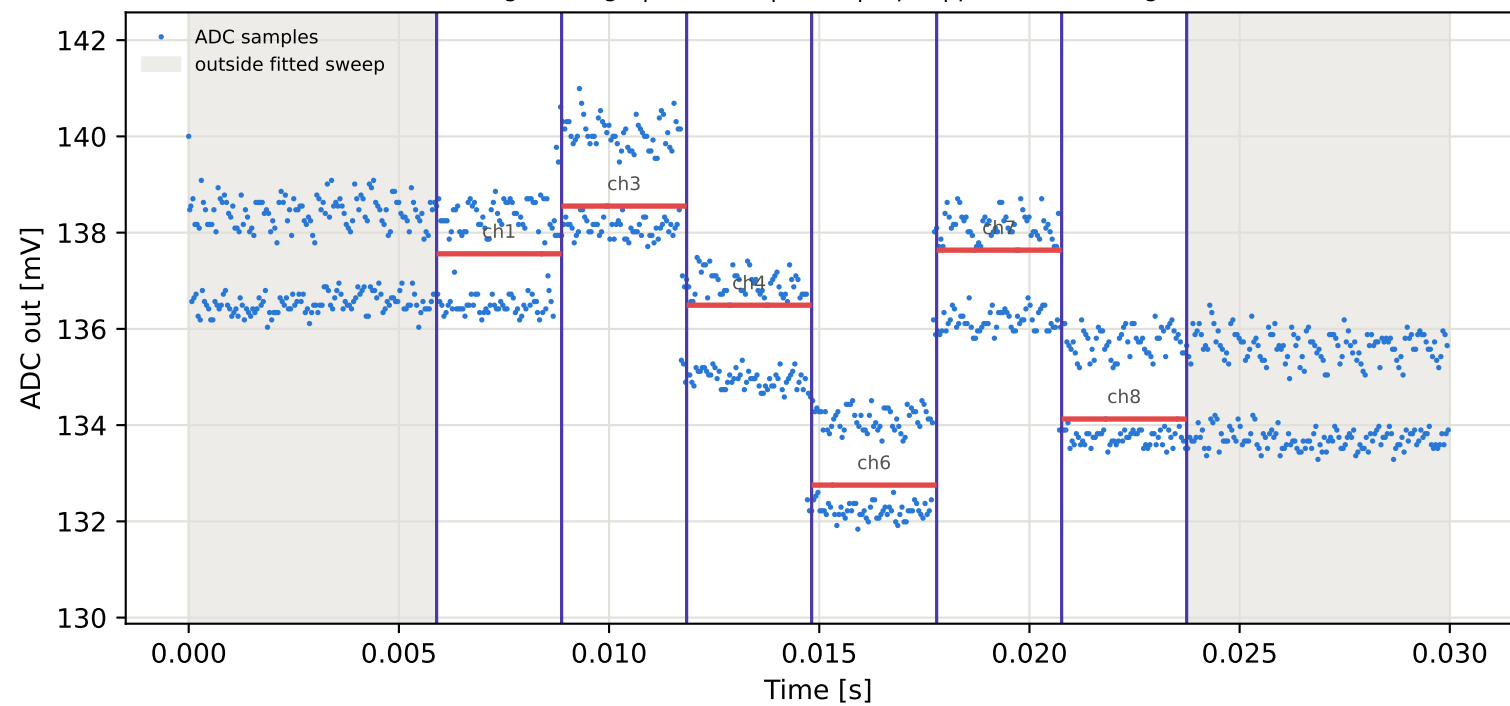
Tag5 &lt;- Tag4 | 775 MHz | run 0 | rep 1 | phase 9.13 deg
