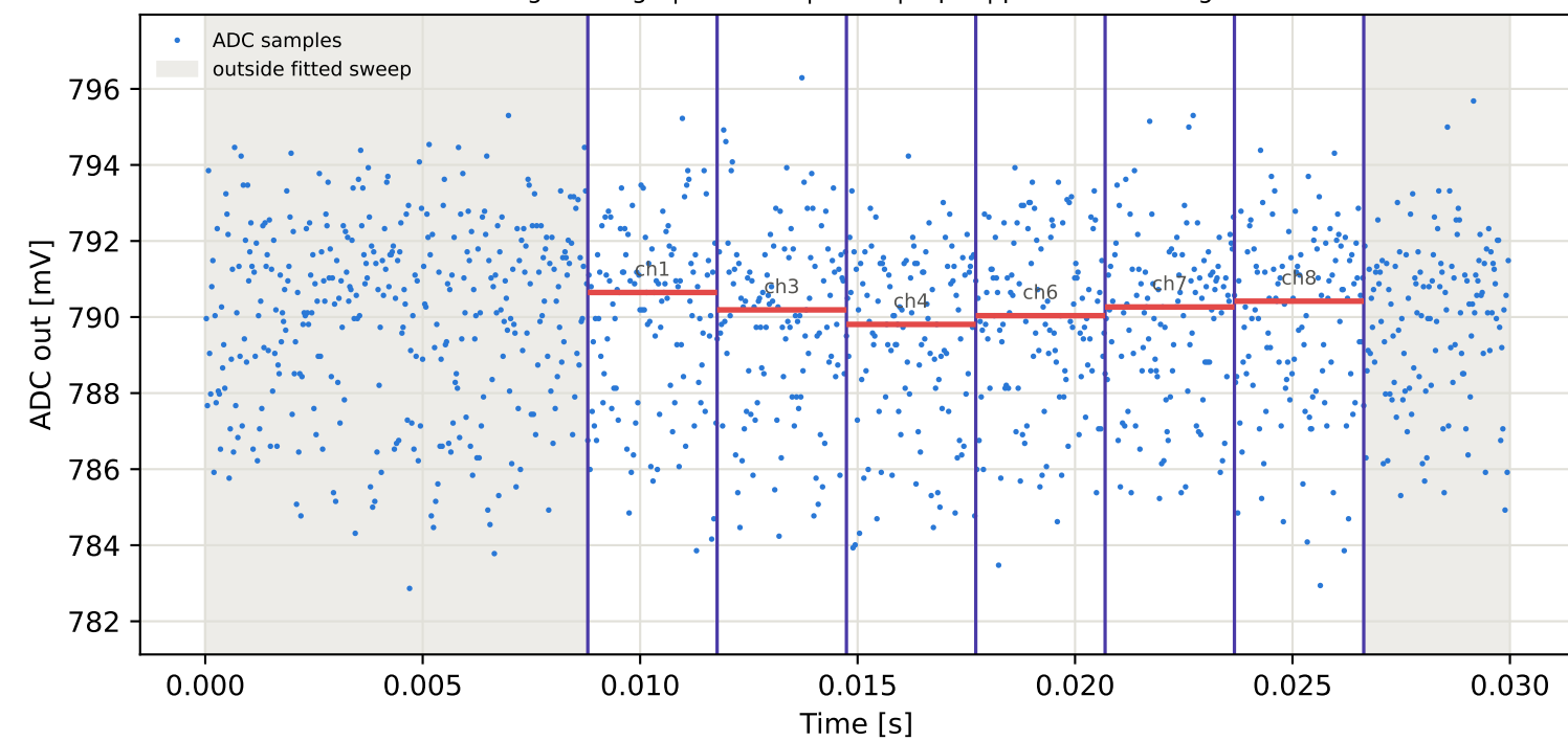
Tag8 &lt;- Tag10 | 885 MHz | run 0 | rep 1 | phase -134.63 deg
