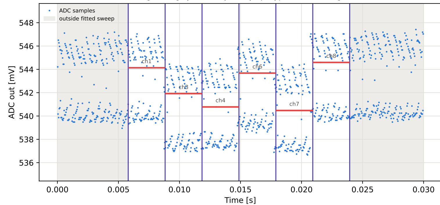
Tag2 &lt;- Tag6 | 845 MHz | run 0 | rep 1 | phase 140.15 deg
