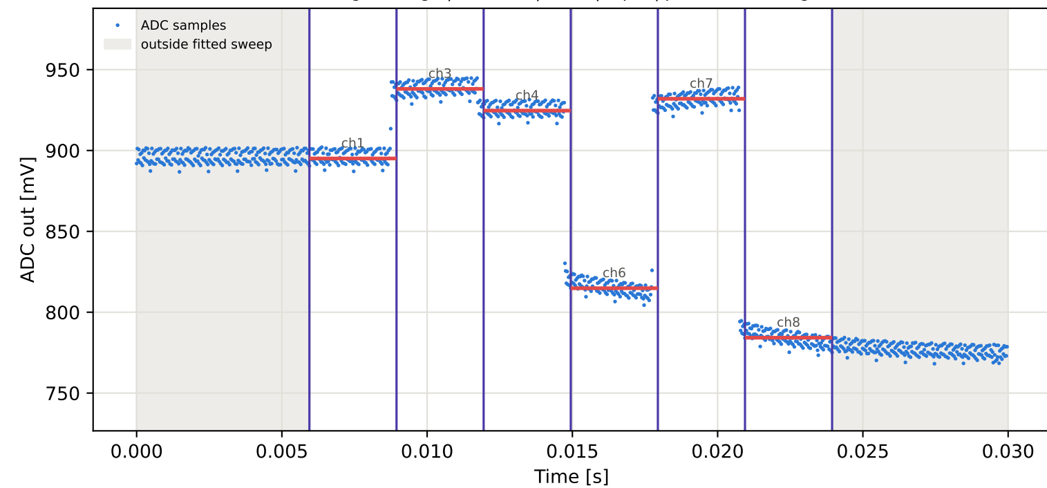
Tag3 &lt;- Tag7 | 885 MHz | run 0 | rep 1 | phase -69.12 deg
