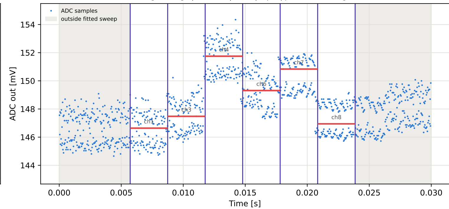
Tag7 &lt;- Tag1 | 805 MHz | run 0 | rep 1 | phase 41.61 deg
