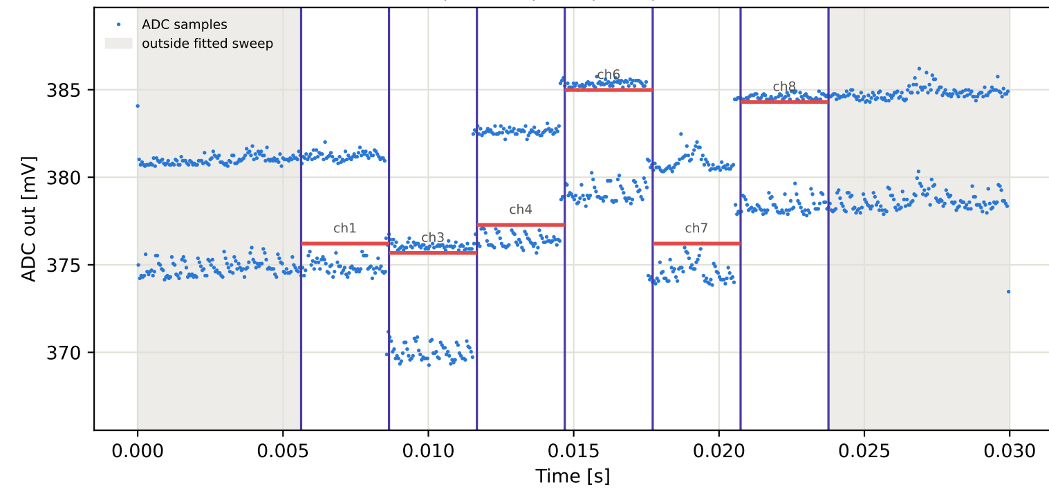
Tag6 &lt;- Tag4 | 825 MHz | run 0 | rep 1 | phase -172.82 deg
