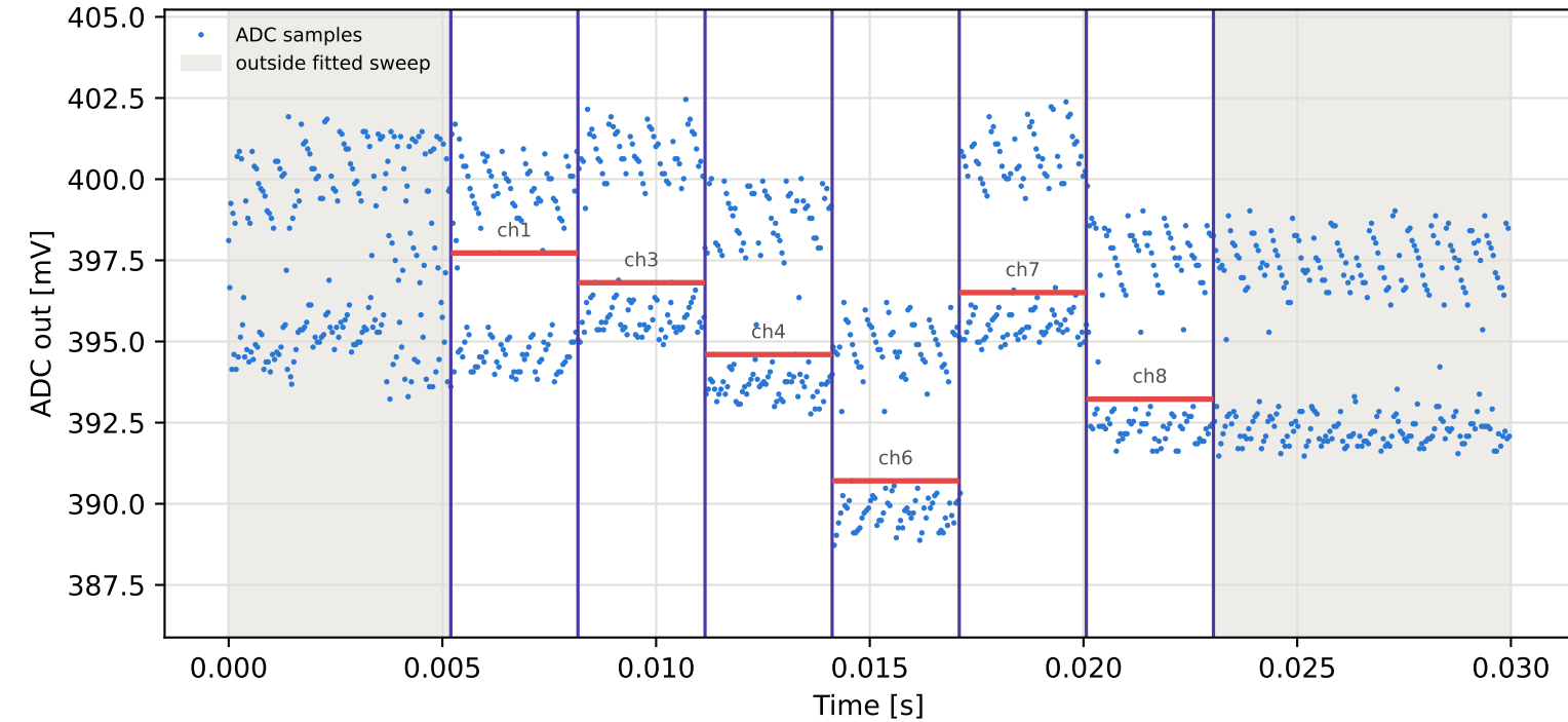
Tag2 &lt;- Tag16 | 985 MHz | run 0 | rep 1 | phase 110.70 deg
