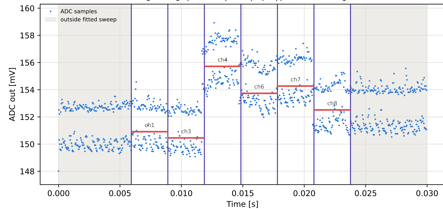
Tag6 &lt;- Tag9 | 775 MHz | run 0 | rep 1 | phase -26.69 deg
