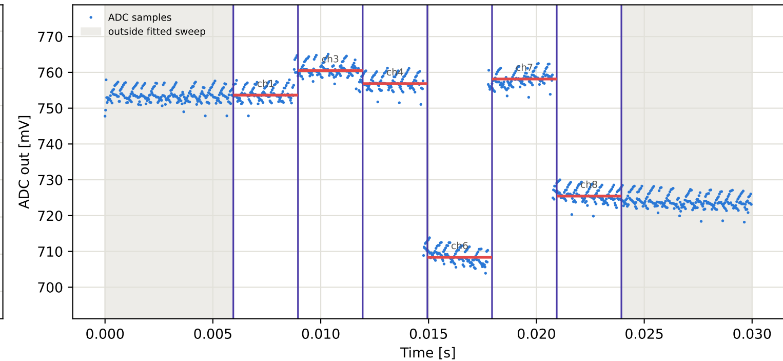
Tag5 &lt;- Tag1 | 915 MHz | run 0 | rep 1 | phase -35.28 deg
