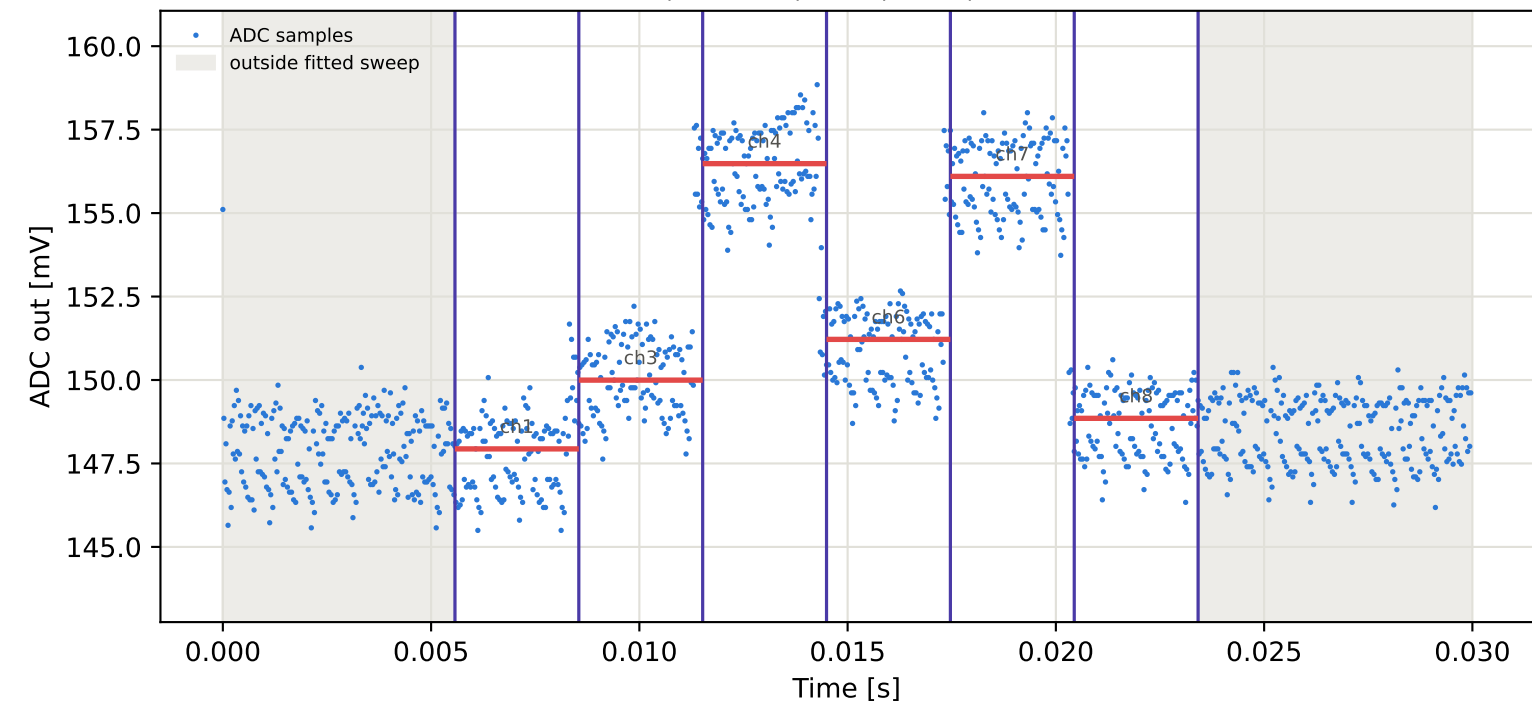
Tag6 &lt;- Tag5 | 775 MHz | run 0 | rep 1 | phase -81.37 deg
