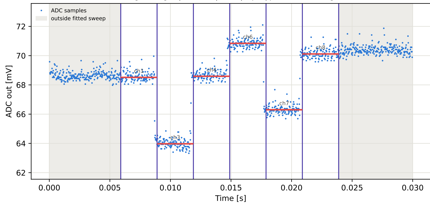
Tag1 &lt;- Tag16 | 795 MHz | run 0 | rep 1 | phase 69.02 deg
