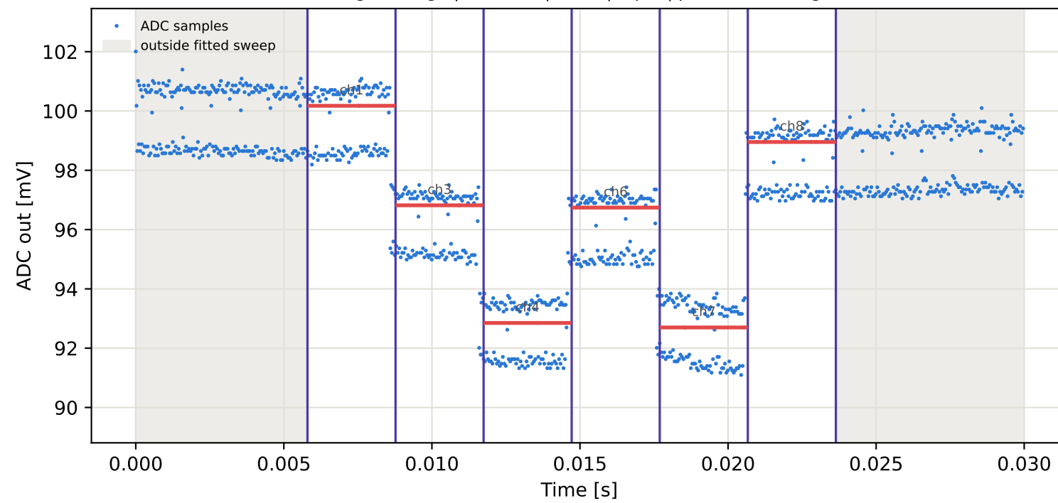
Tag1 &lt;- Tag7 | 825 MHz | run 0 | rep 1 | phase 26.37 deg
