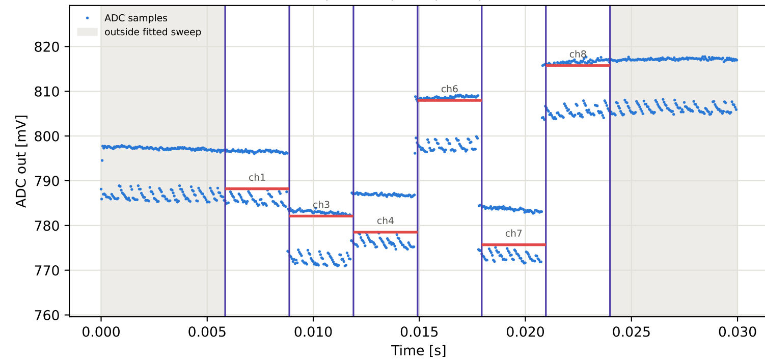
Tag7 &lt;- Tag5 | 875 MHz | run 0 | rep 1 | phase 152.91 deg
