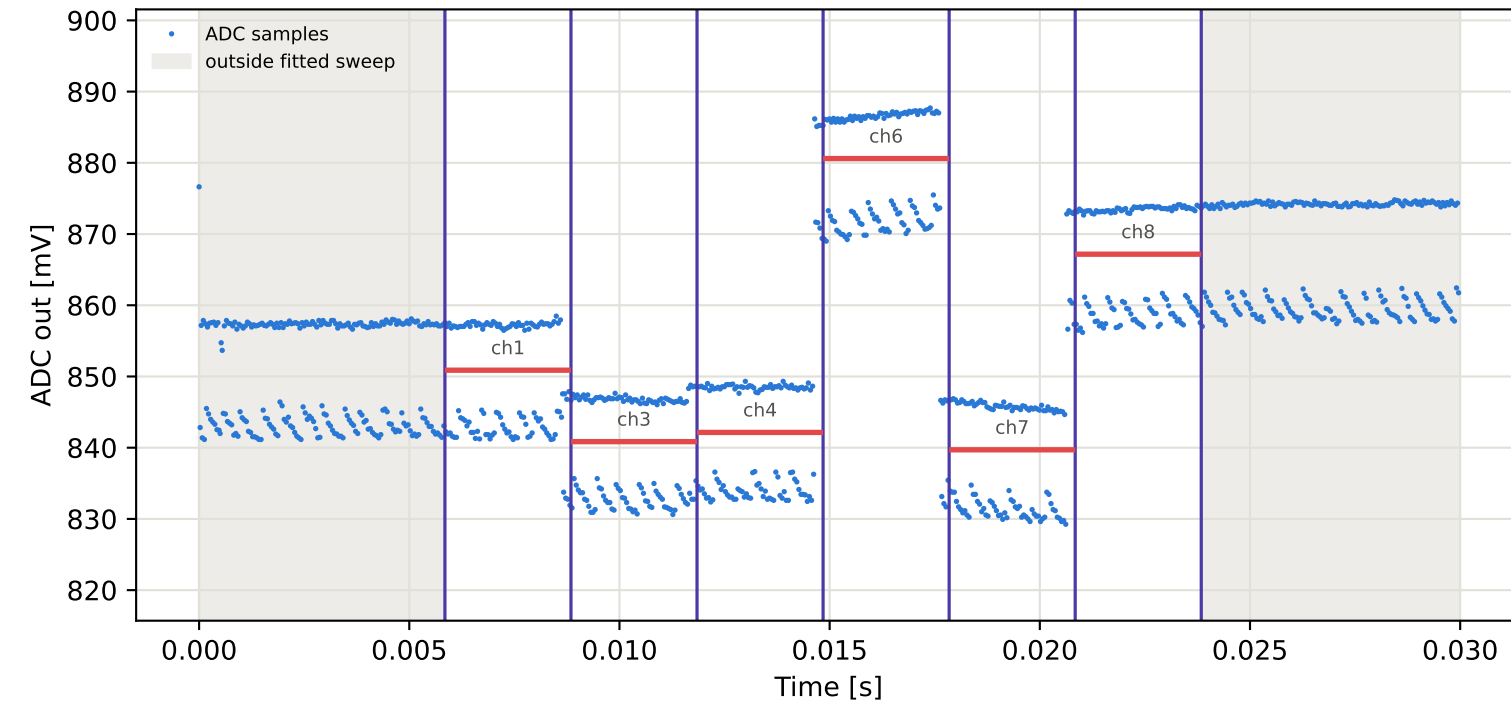
Tag16 &lt;- Tag10 | 955 MHz | run 0 | rep 1 | phase -113.03 deg
