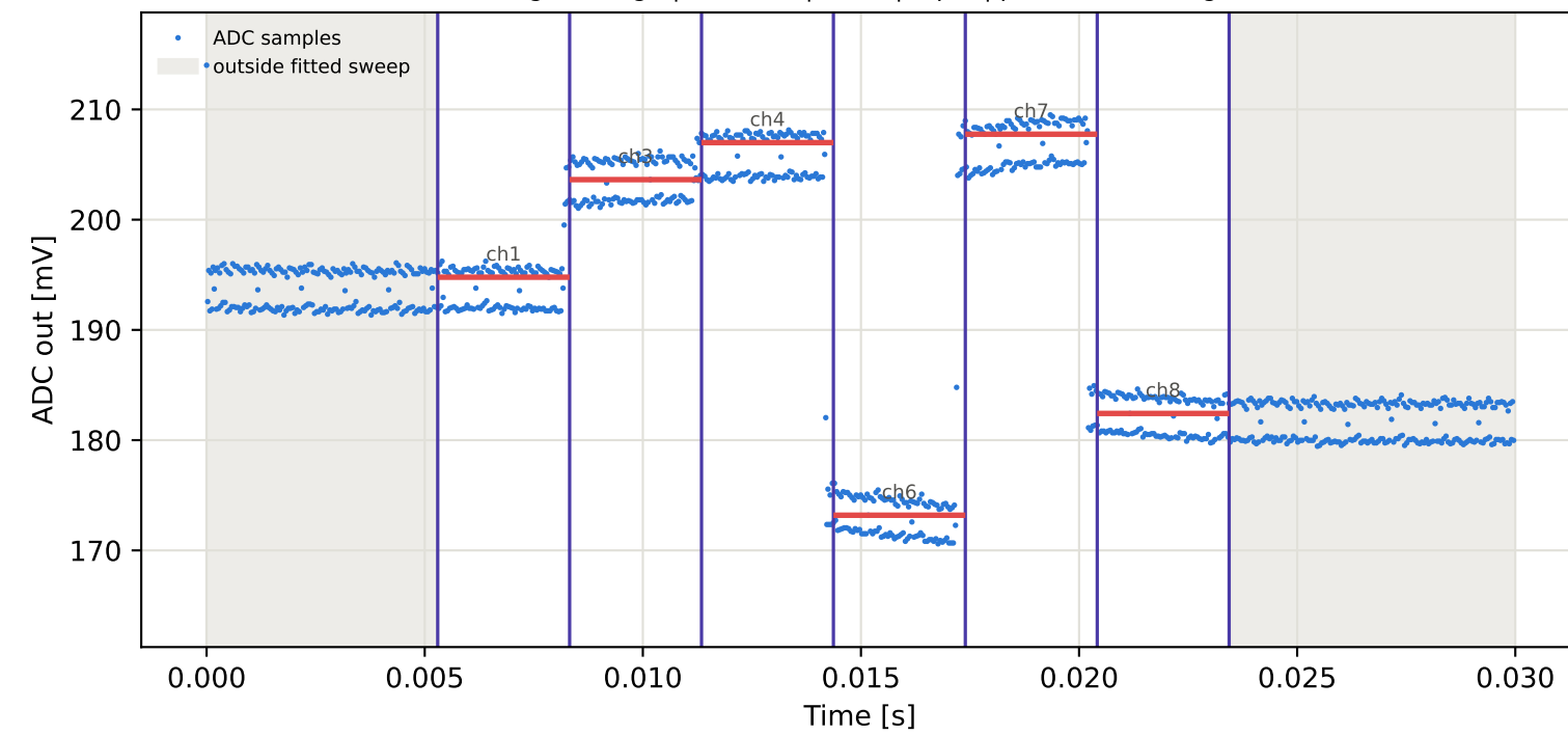
Tag1 &lt;- Tag7 | 985 MHz | run 0 | rep 1 | phase 174.53 deg
