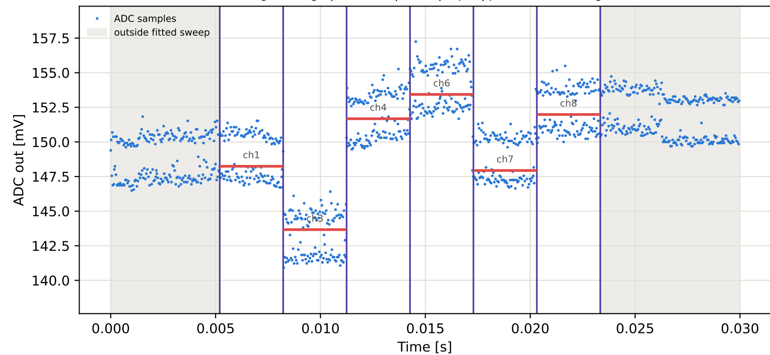
Tag6 &lt;- Tag5 | 805 MHz | run 0 | rep 1 | phase -3.07 deg
