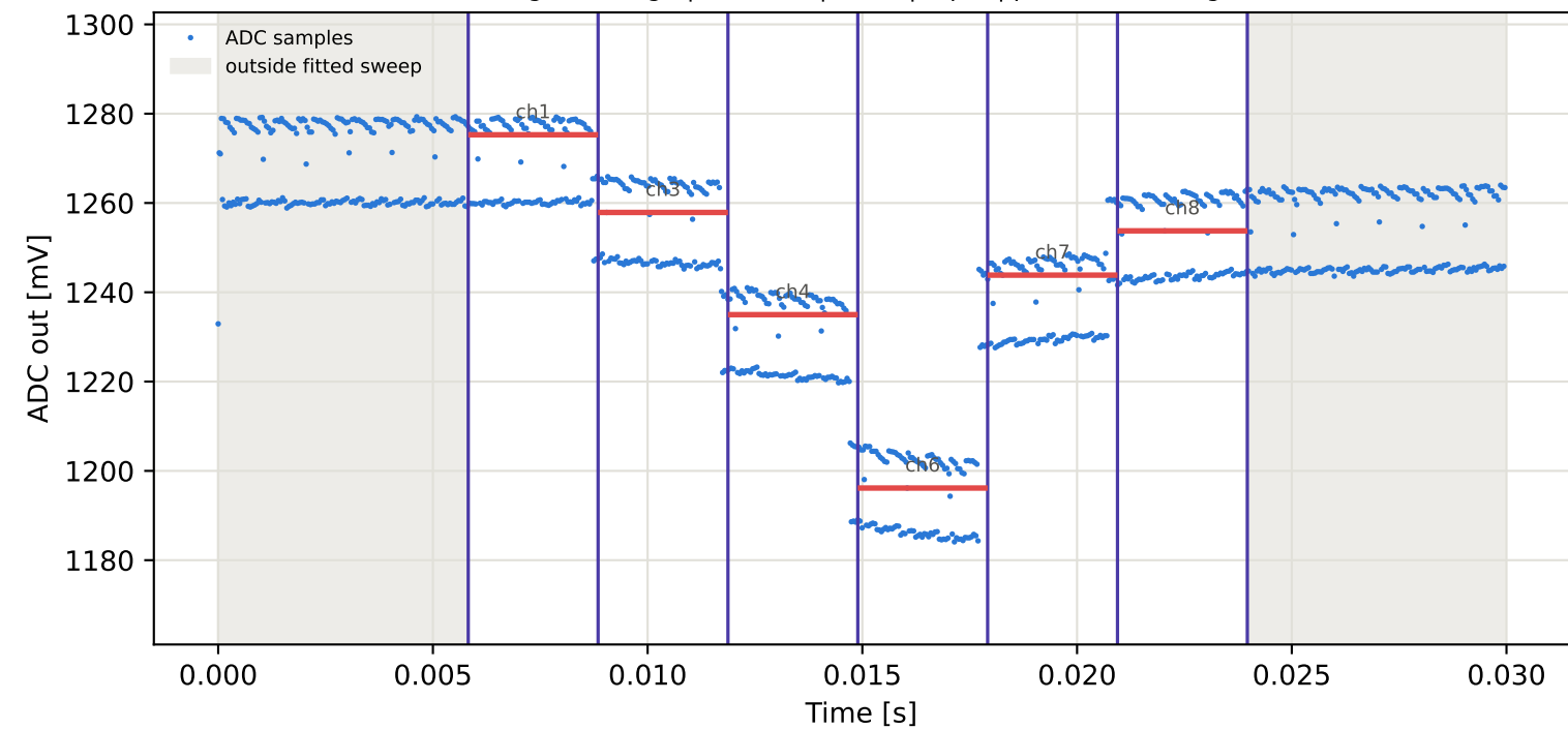
Tag16 &lt;- Tag1 | 915 MHz | run 0 | rep 1 | phase 119.31 deg
