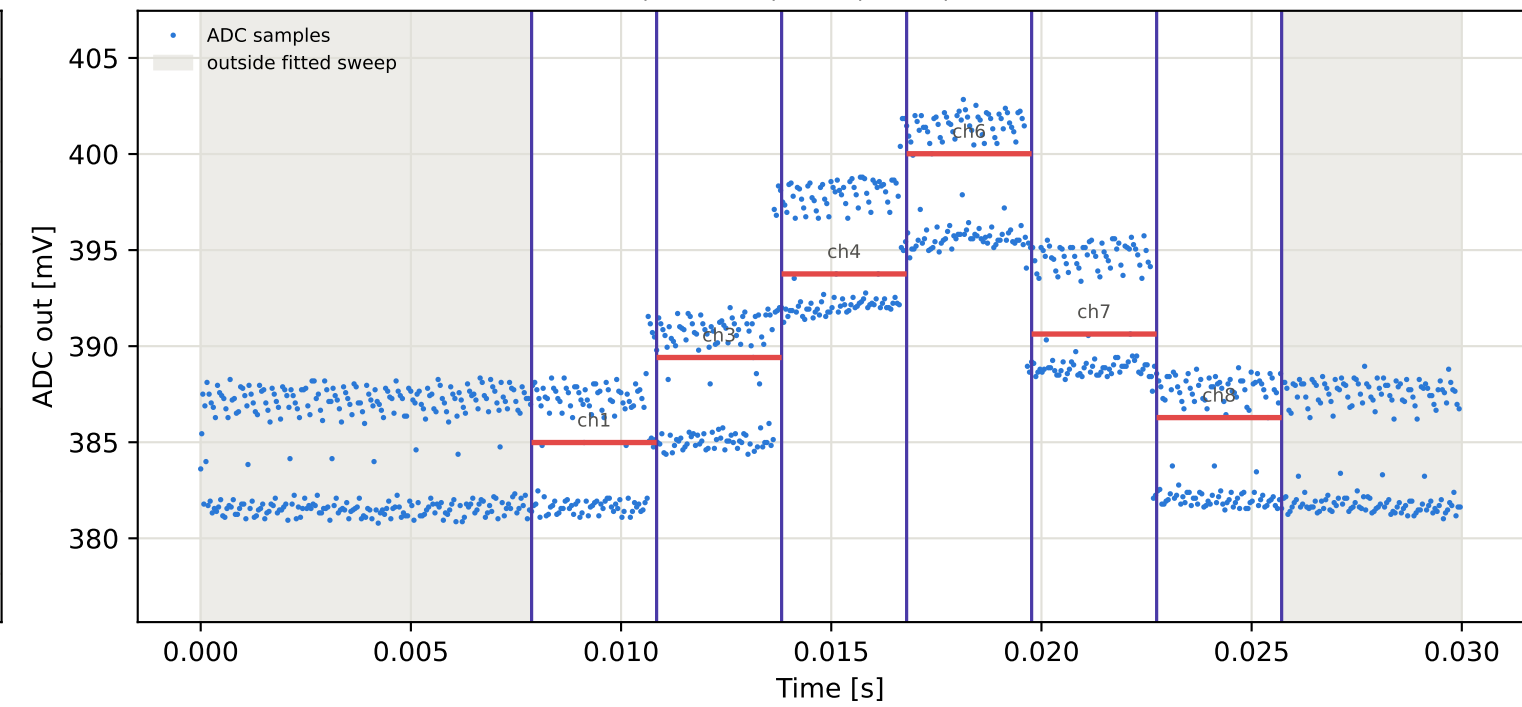
Tag3 &lt;- Tag2 | 965 MHz | run 0 | rep 1 | phase -141.91 deg
