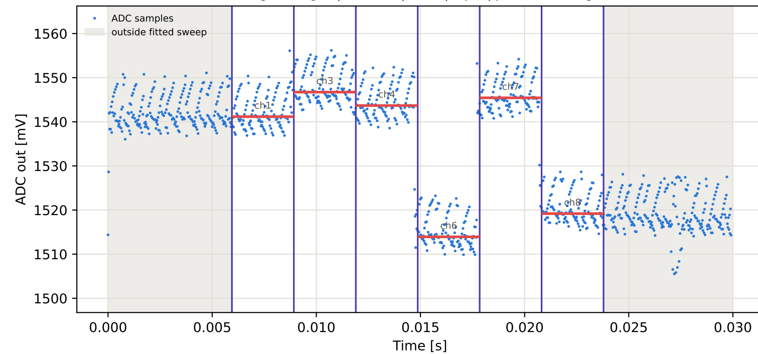
Tag5 &lt;- Tag16 | 895 MHz | run 0 | rep 1 | phase 31.26 deg
