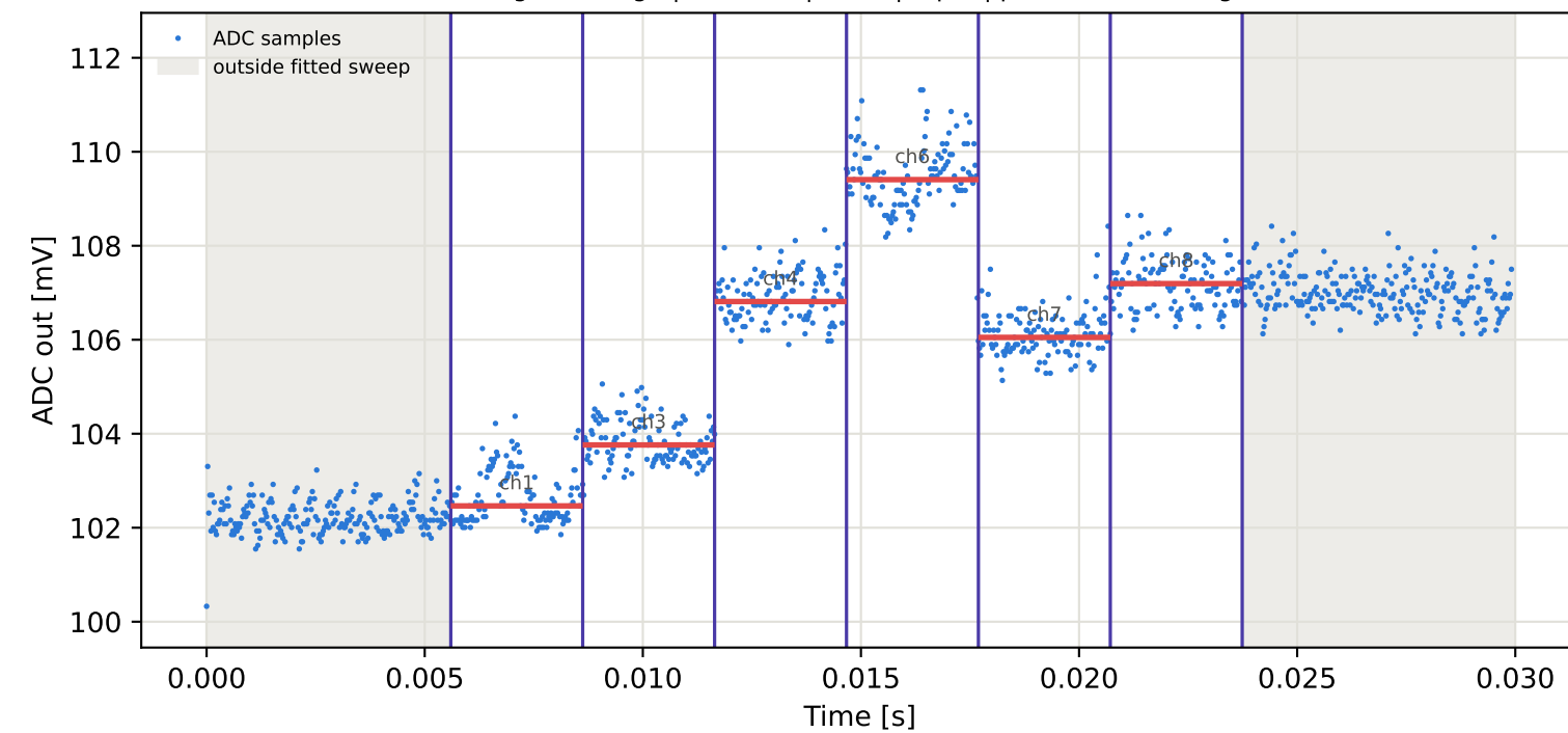
Tag10 &lt;- Tag4 | 805 MHz | run 0 | rep 1 | phase -164.77 deg
