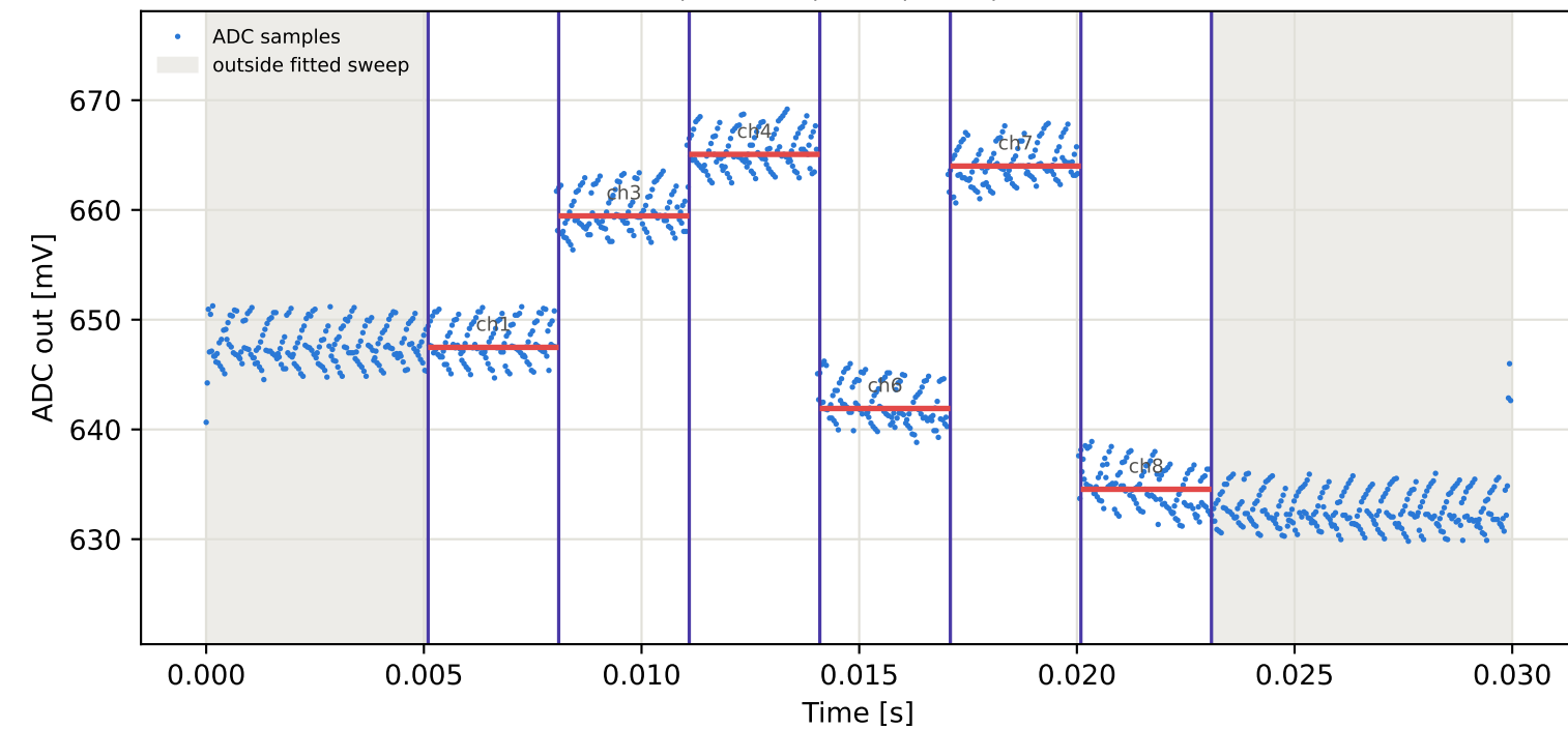
Tag10 &lt;- Tag4 | 905 MHz | run 0 | rep 1 | phase -48.76 deg
