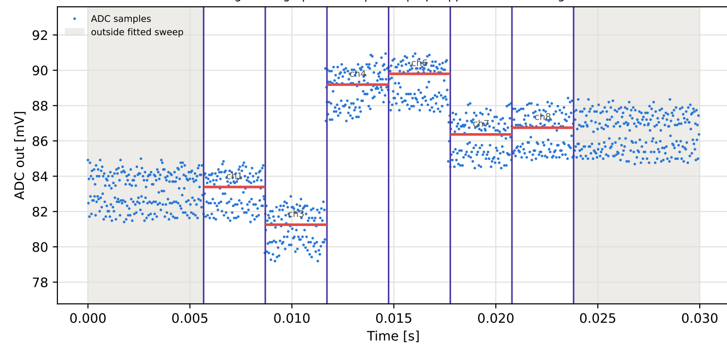
Tag3 &lt;- Tag7 | 795 MHz | run 0 | rep 1 | phase -144.25 deg
