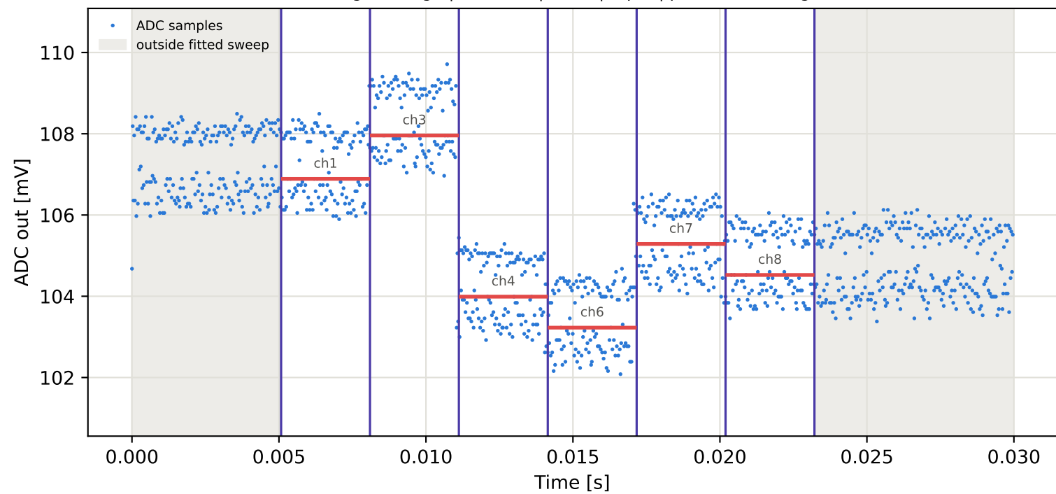
Tag5 &lt;- Tag9 | 795 MHz | run 0 | rep 1 | phase -175.50 deg
