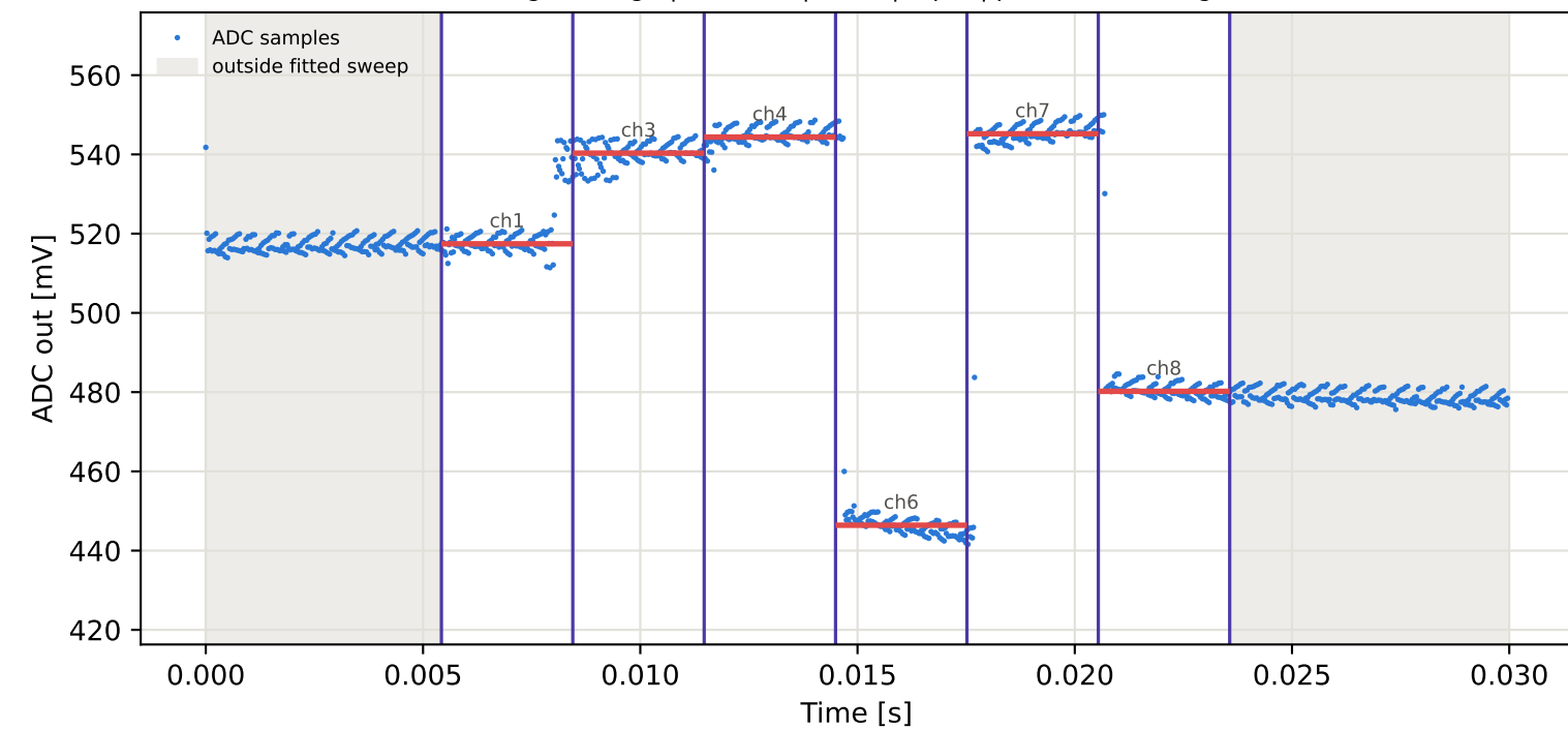
Tag4 &lt;- Tag7 | 945 MHz | run 0 | rep 1 | phase -97.19 deg
