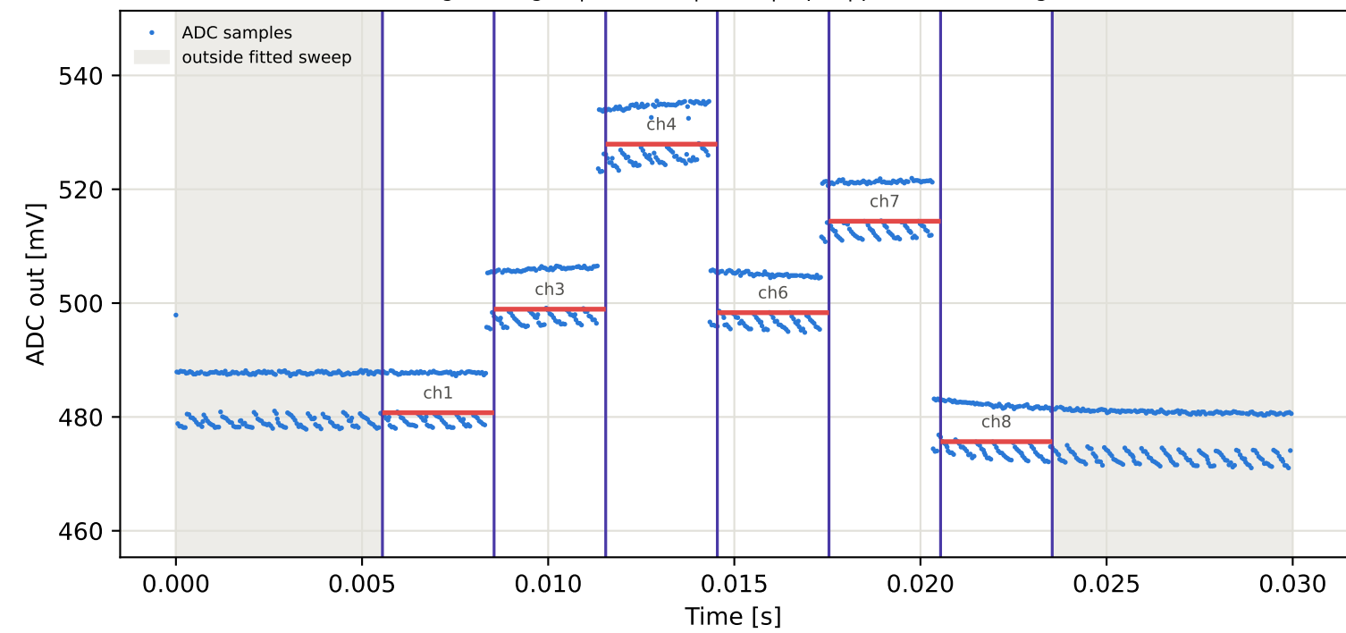
Tag5 &lt;- Tag2 | 945 MHz | run 0 | rep 1 | phase 159.51 deg
