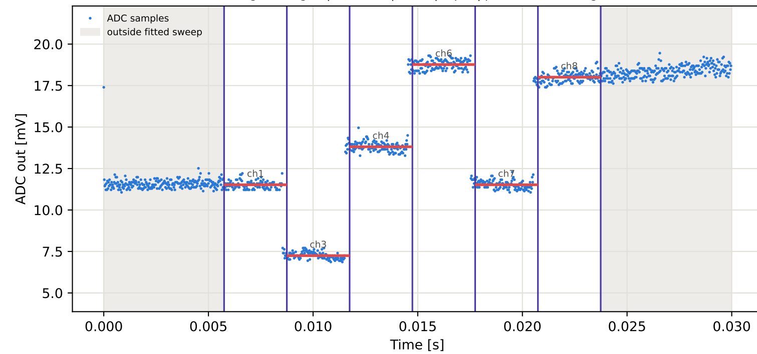
Tag1 &lt;- Tag16 | 835 MHz | run 0 | rep 1 | phase 140.31 deg
