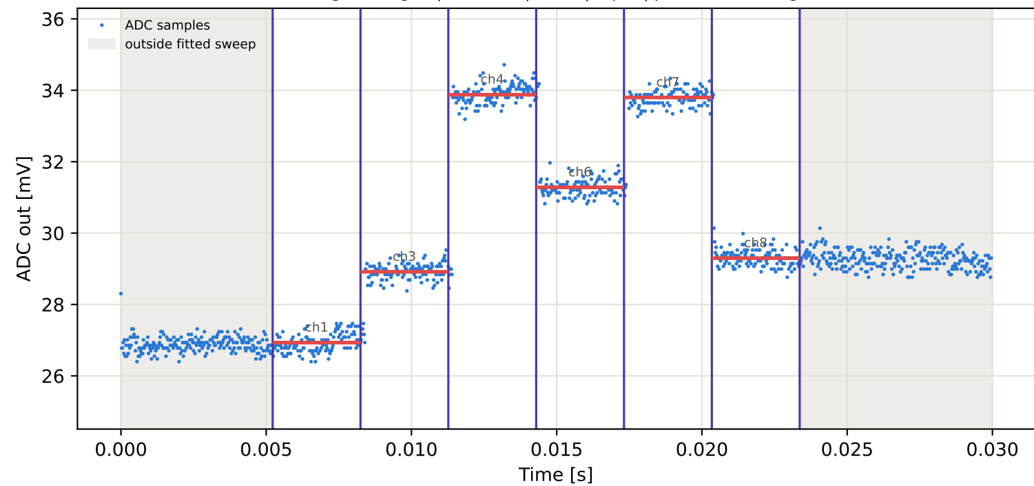
Tag4 &lt;- Tag16 | 805 MHz | run 0 | rep 1 | phase 167.74 deg
