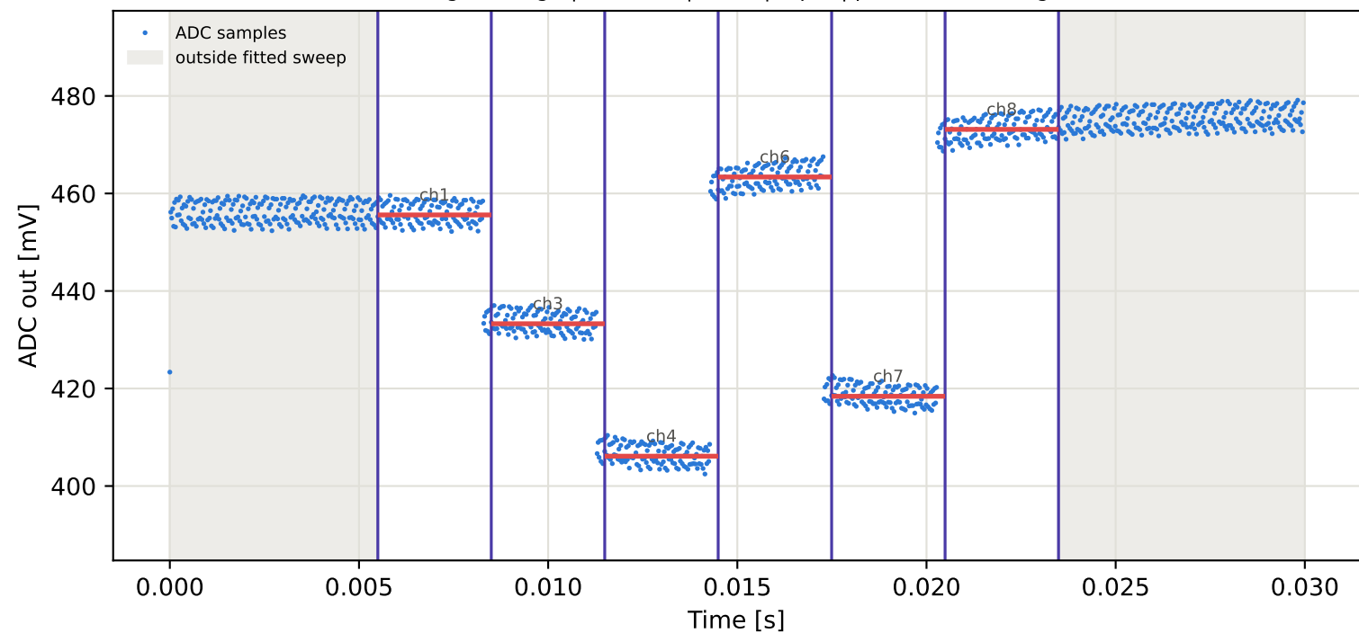
Tag3 &lt;- Tag7 | 935 MHz | run 0 | rep 1 | phase 34.85 deg
