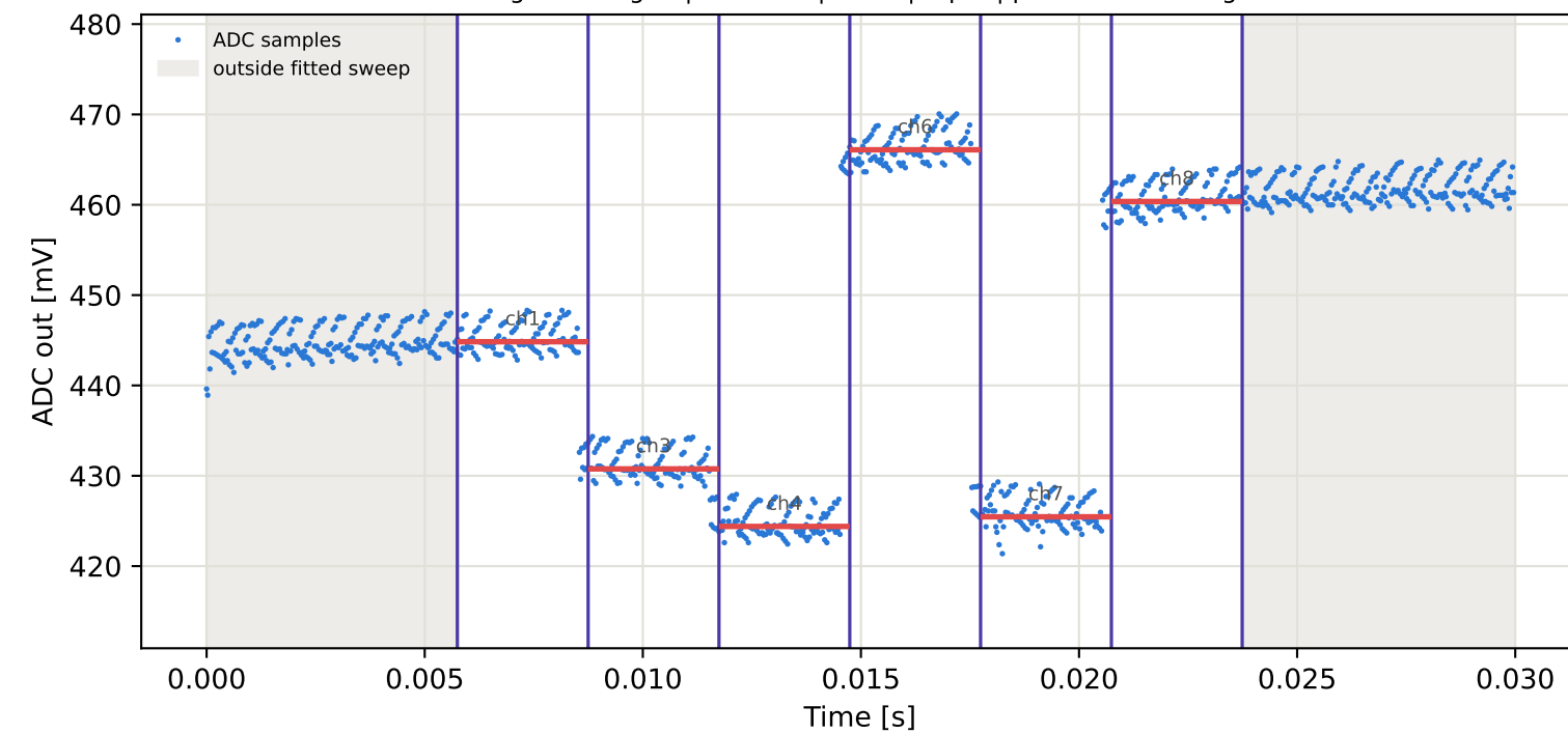
Tag10 &lt;- Tag2 | 975 MHz | run 0 | rep 1 | phase -22.34 deg
