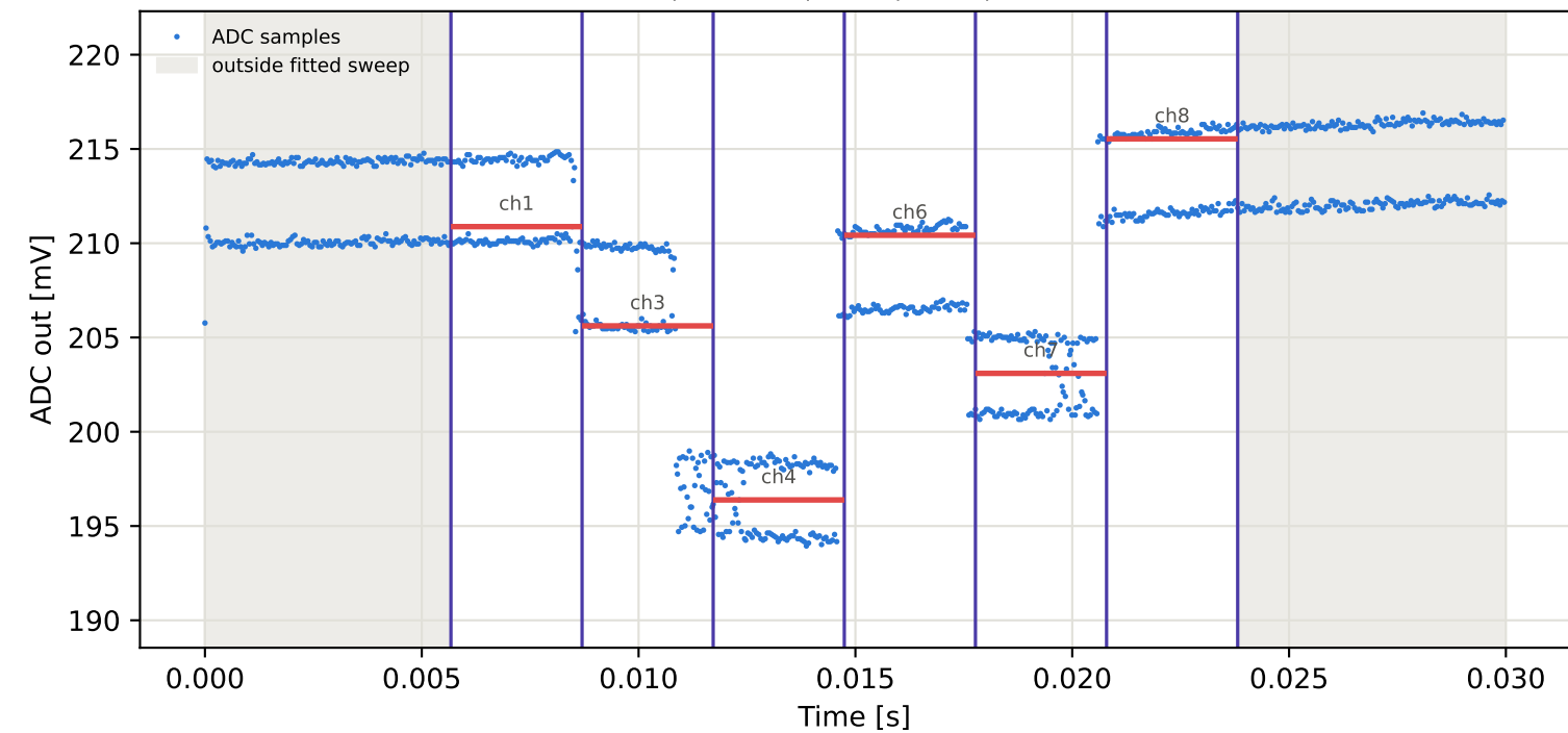
Tag4 &lt;- Tag3 | 975 MHz | run 0 | rep 1 | phase 94.60 deg
