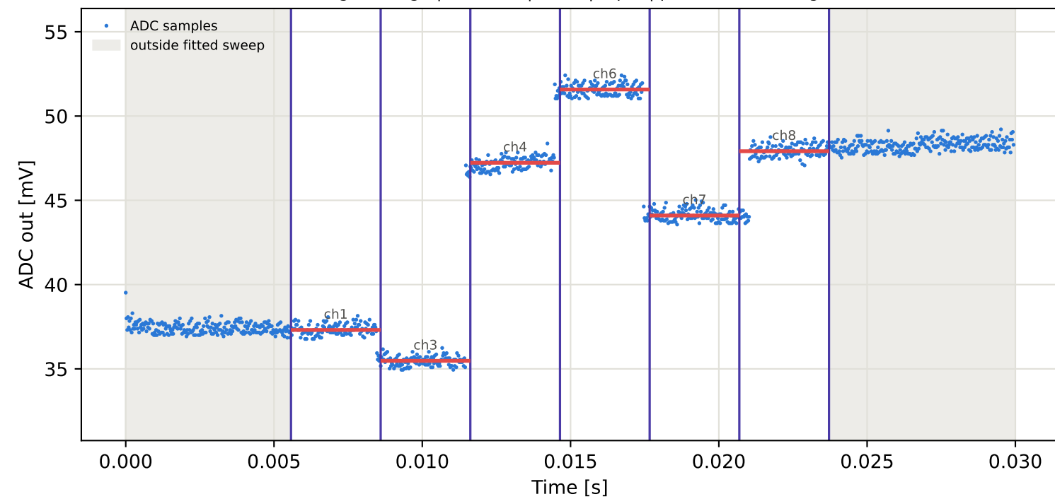
Tag1 &lt;- Tag8 | 845 MHz | run 0 | rep 1 | phase -3.34 deg
