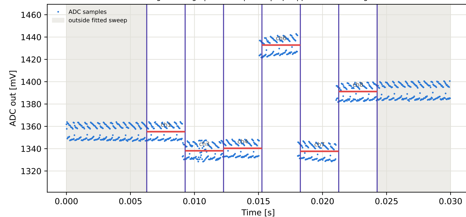
Tag16 &lt;- Tag4 | 875 MHz | run 0 | rep 1 | phase -58.15 deg
