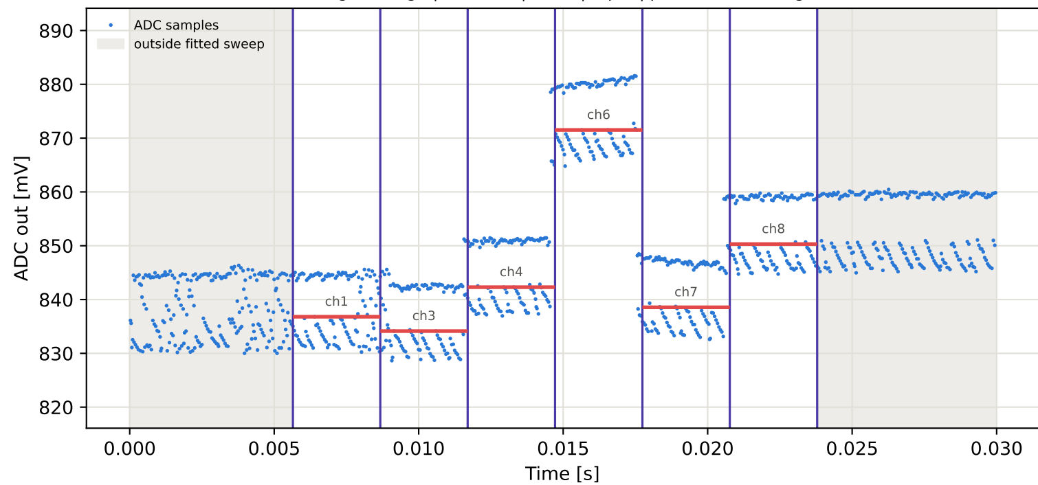
Tag4 &lt;- Tag8 | 925 MHz | run 0 | rep 1 | phase -61.73 deg
