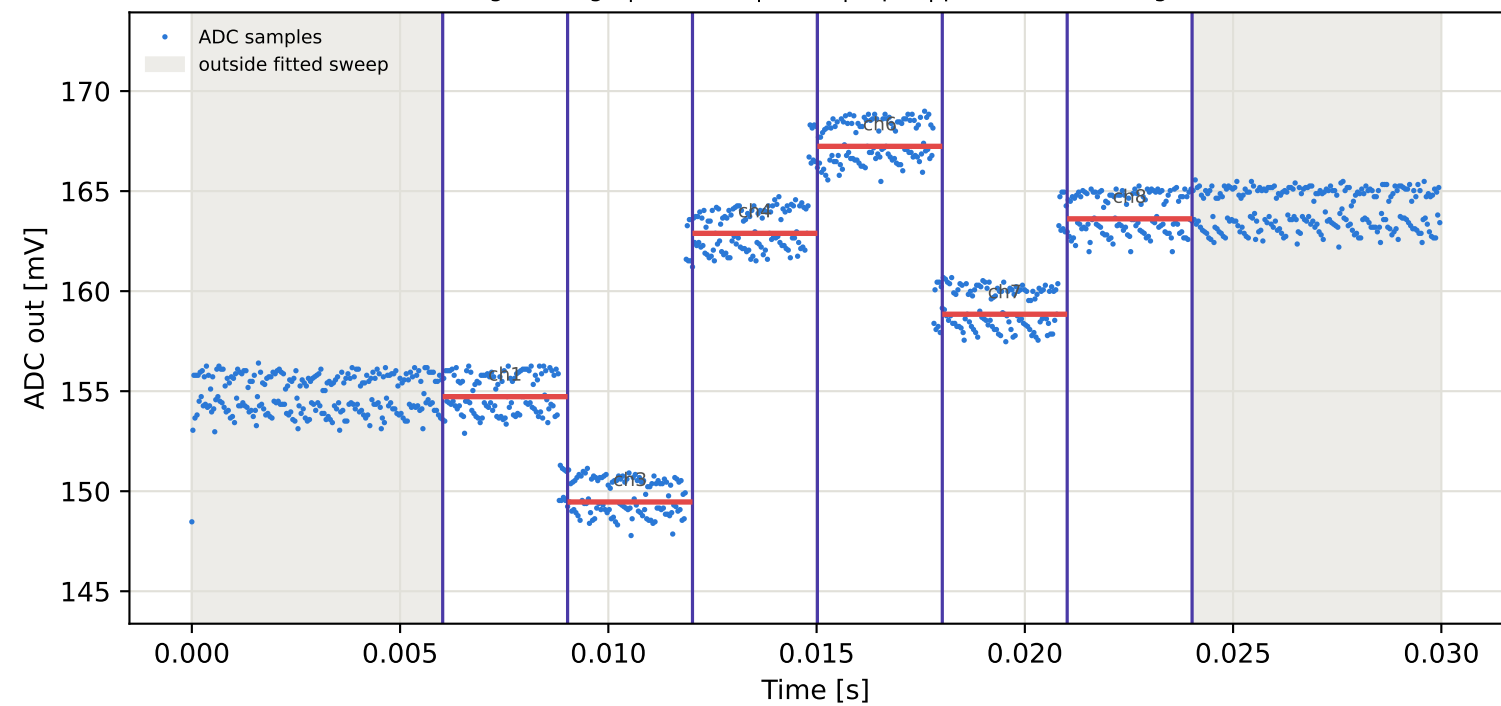
Tag5 &lt;- Tag1 | 825 MHz | run 0 | rep 1 | phase -62.12 deg
