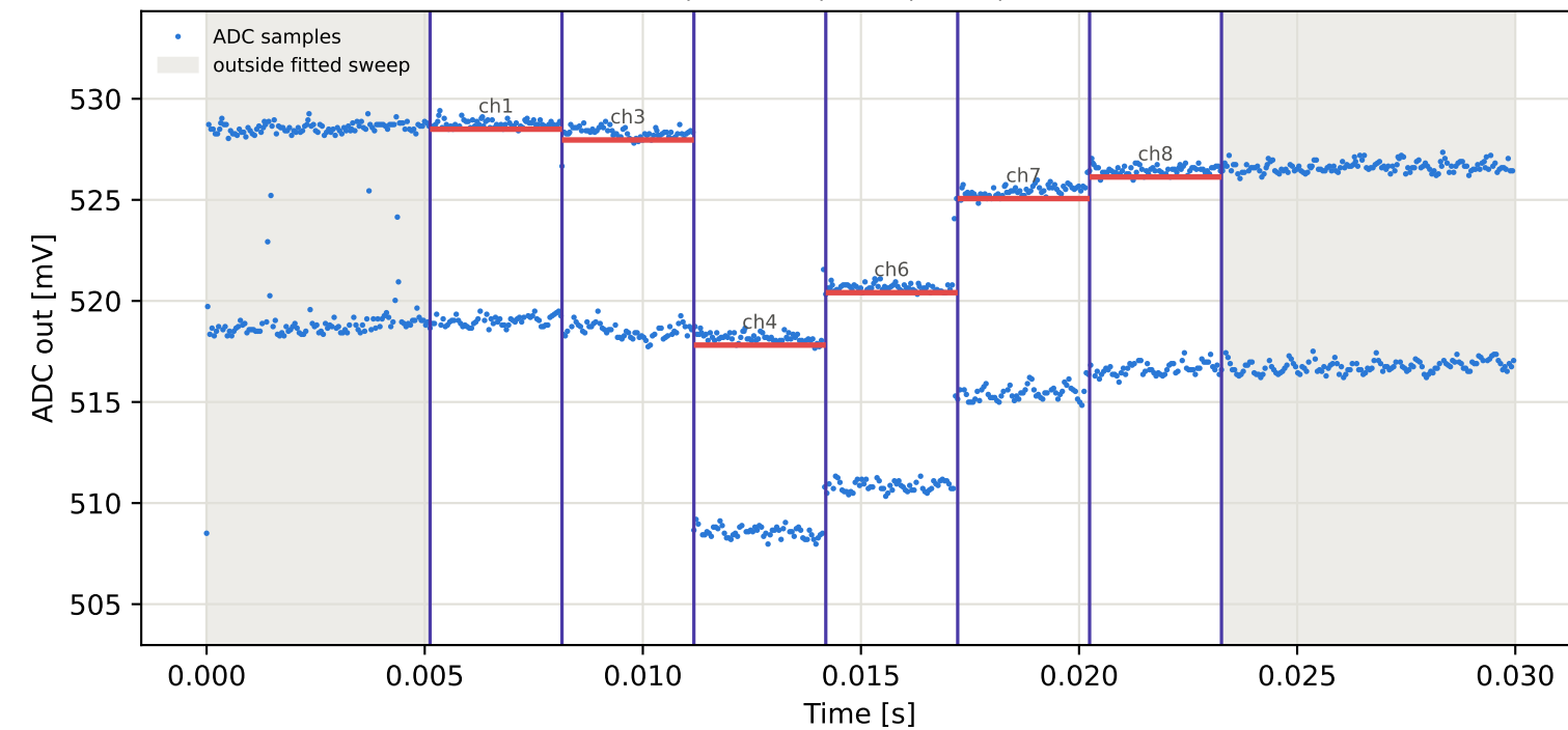
Tag7 &lt;- Tag10 | 985 MHz | run 0 | rep 1 | phase 47.13 deg
