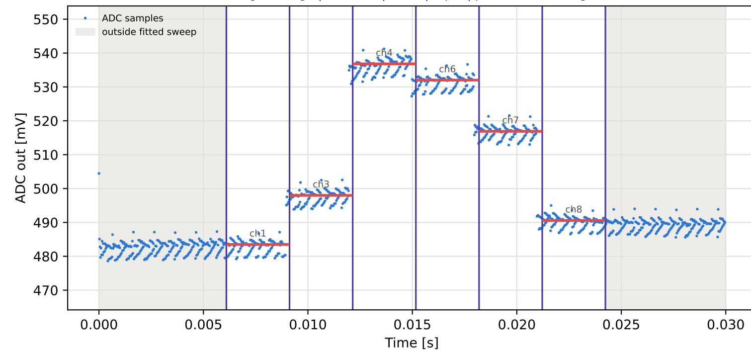
Tag8 &lt;- Tag1 | 945 MHz | run 0 | rep 1 | phase 139.07 deg
