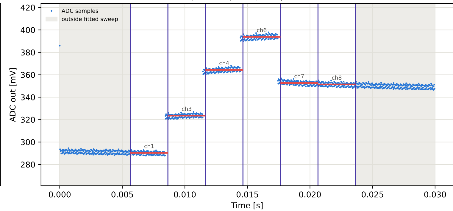
Tag1 &lt;- Tag8 | 875 MHz | run 0 | rep 1 | phase -97.50 deg
