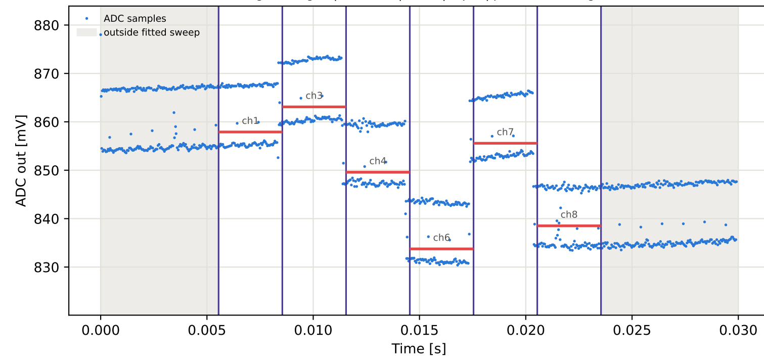
Tag6 &lt;- Tag2 | 875 MHz | run 0 | rep 1 | phase 88.57 deg
