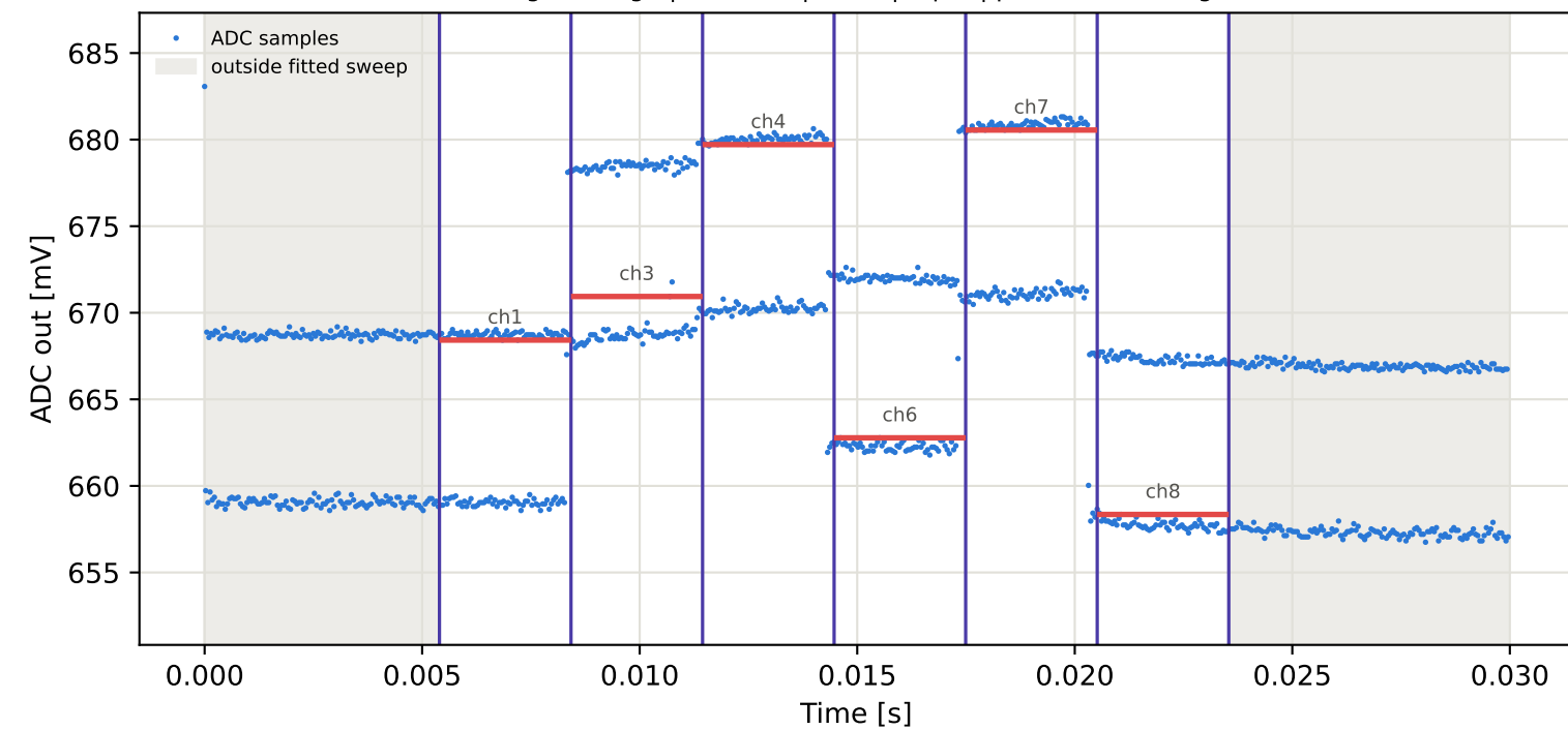
Tag6 &lt;- Tag10 | 865 MHz | run 0 | rep 1 | phase -172.06 deg
