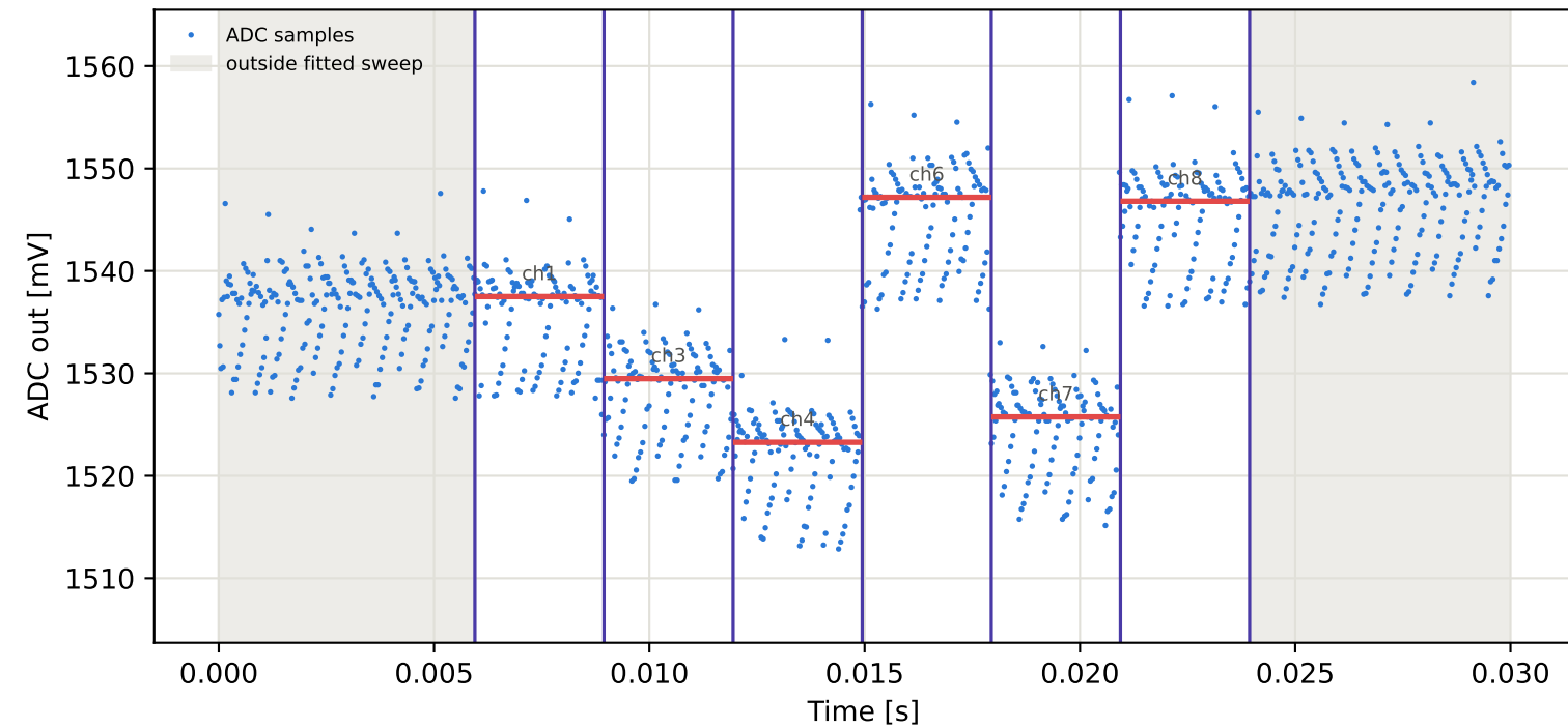
Tag2 &lt;- Tag16 | 925 MHz | run 0 | rep 1 | phase 36.52 deg
