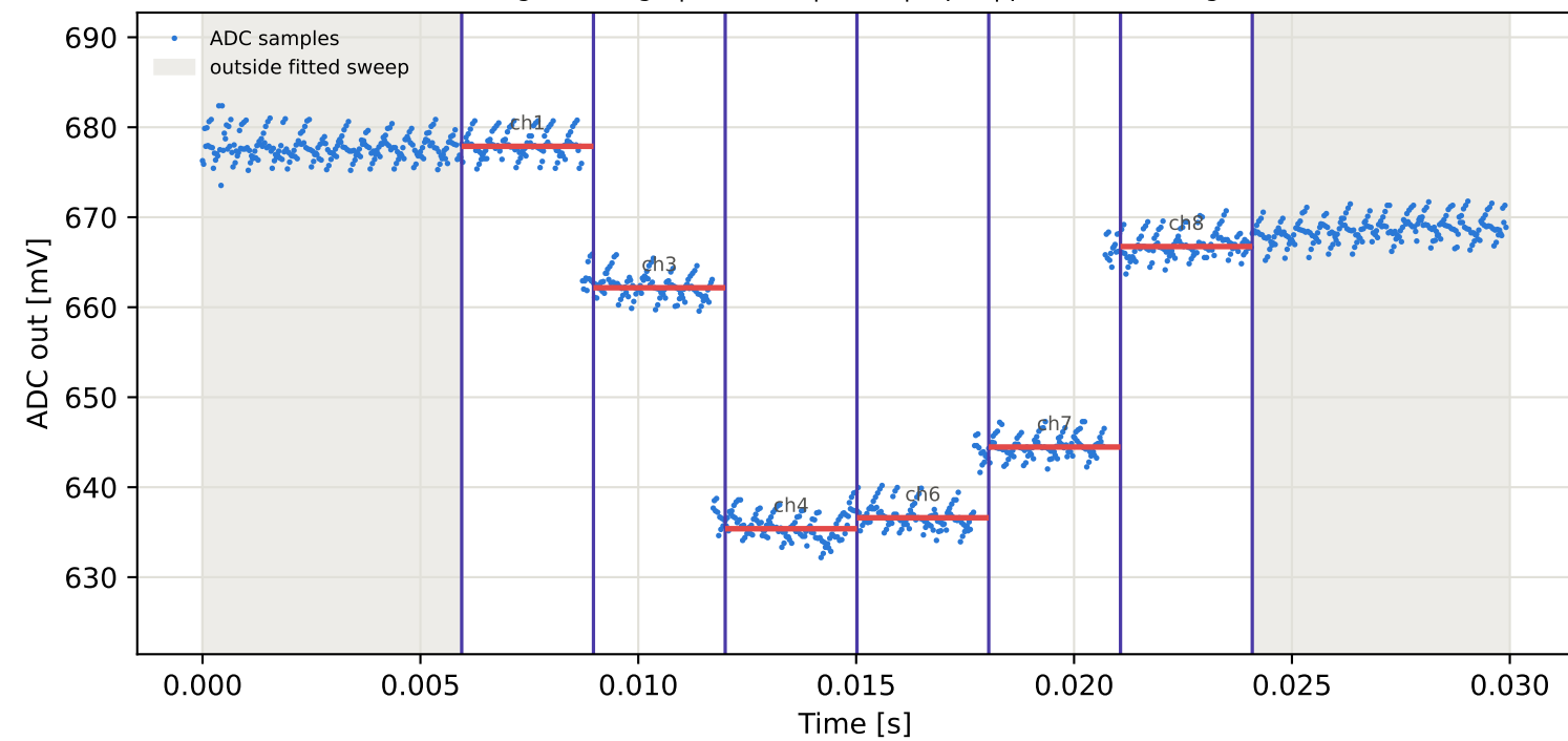
Tag10 &lt;- Tag9 | 905 MHz | run 0 | rep 1 | phase -43.44 deg
