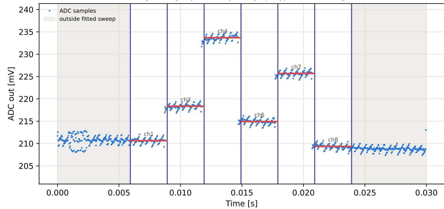
Tag5 &lt;- Tag2 | 995 MHz | run 0 | rep 1 | phase 172.67 deg
