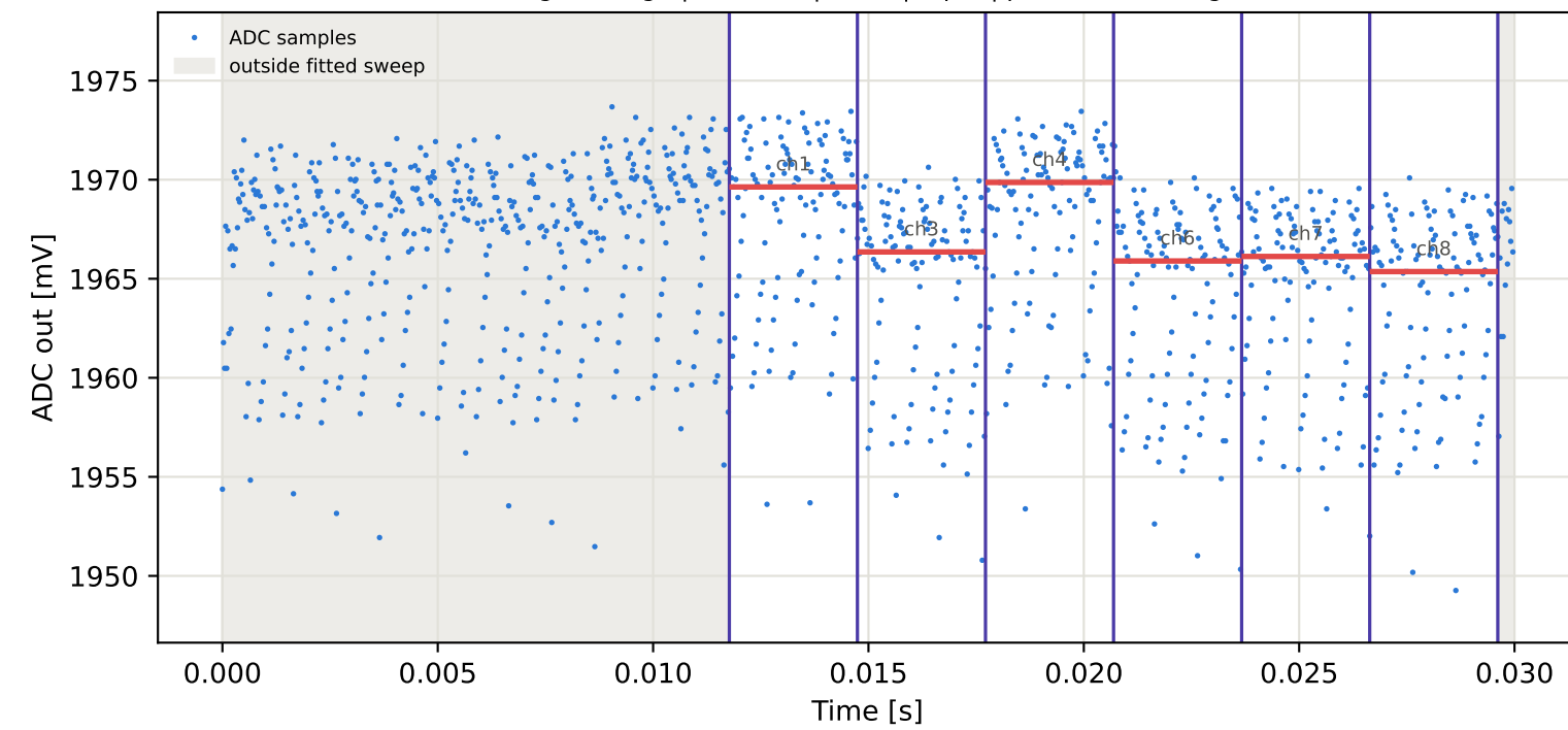
Tag3 &lt;- Tag10 | 915 MHz | run 0 | rep 1 | phase -62.97 deg
