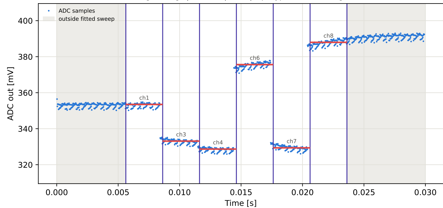
Tag4 &lt;- Tag8 | 895 MHz | run 0 | rep 1 | phase -116.60 deg
