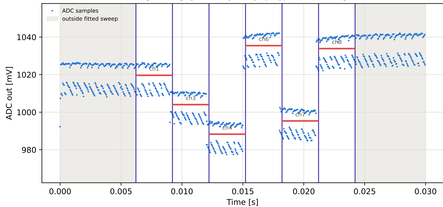
Tag16 &lt;- Tag1 | 945 MHz | run 0 | rep 1 | phase -97.93 deg
