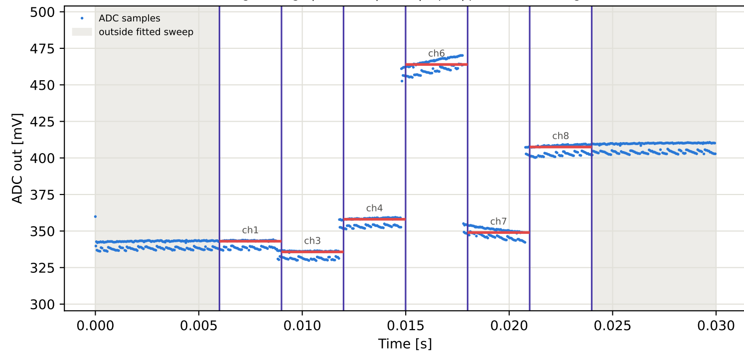
Tag8 &lt;- Tag1 | 915 MHz | run 0 | rep 1 | phase 19.69 deg
