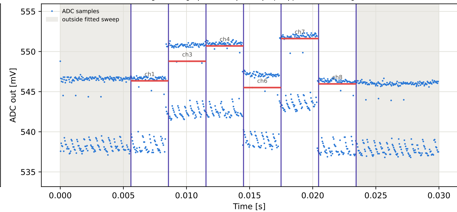
Tag15 &lt;- Tag6 | 825 MHz | run 0 | rep 1 | phase -47.37 deg
