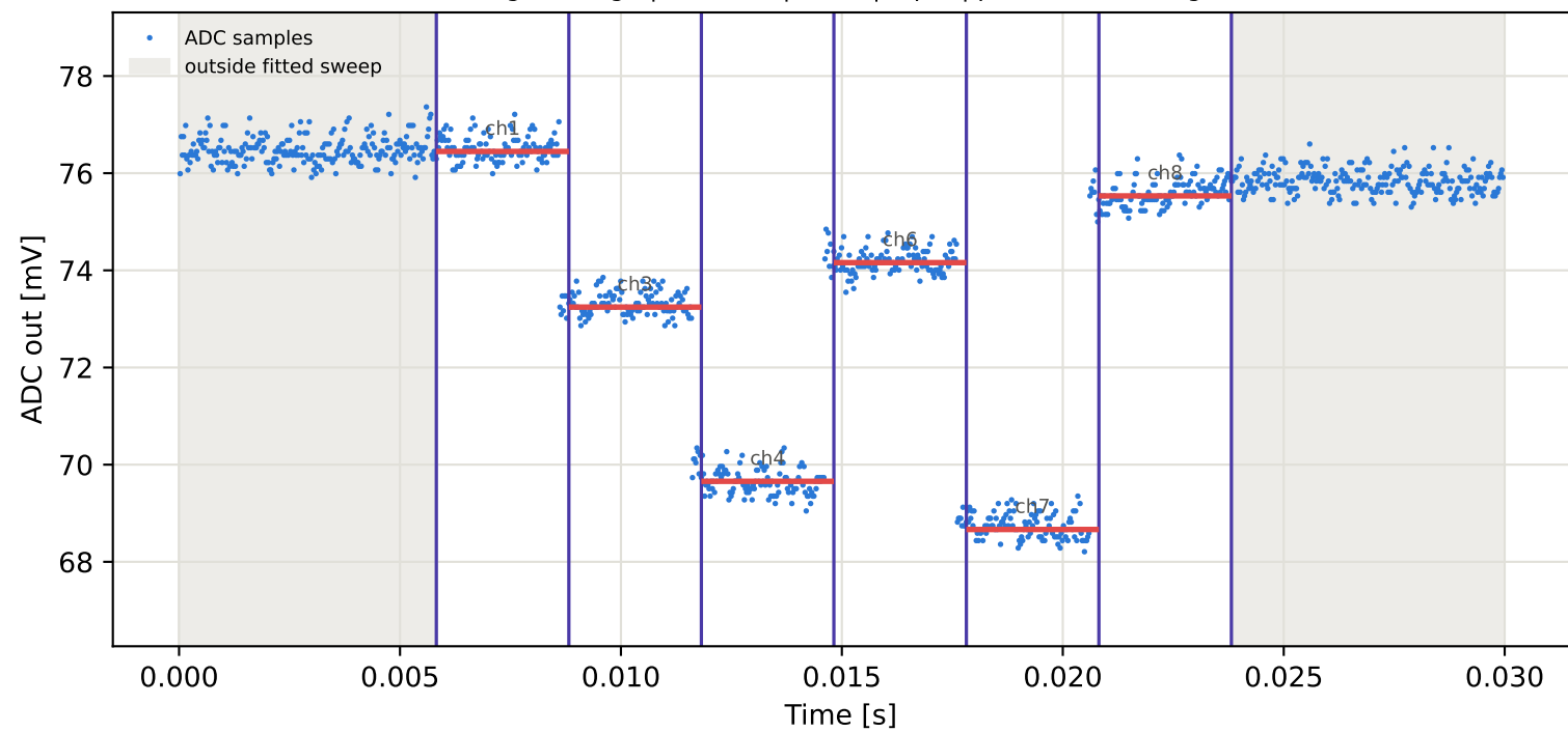
Tag9 &lt;- Tag6 | 795 MHz | run 0 | rep 1 | phase -8.09 deg
