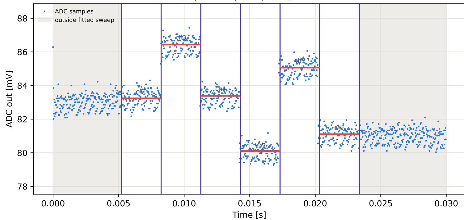
Tag5 &lt;- Tag8 | 805 MHz | run 0 | rep 1 | phase -67.69 deg
