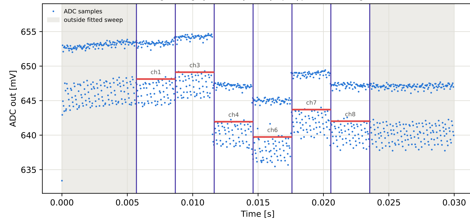
Tag3 &lt;- Tag6 | 835 MHz | run 0 | rep 1 | phase 170.46 deg
