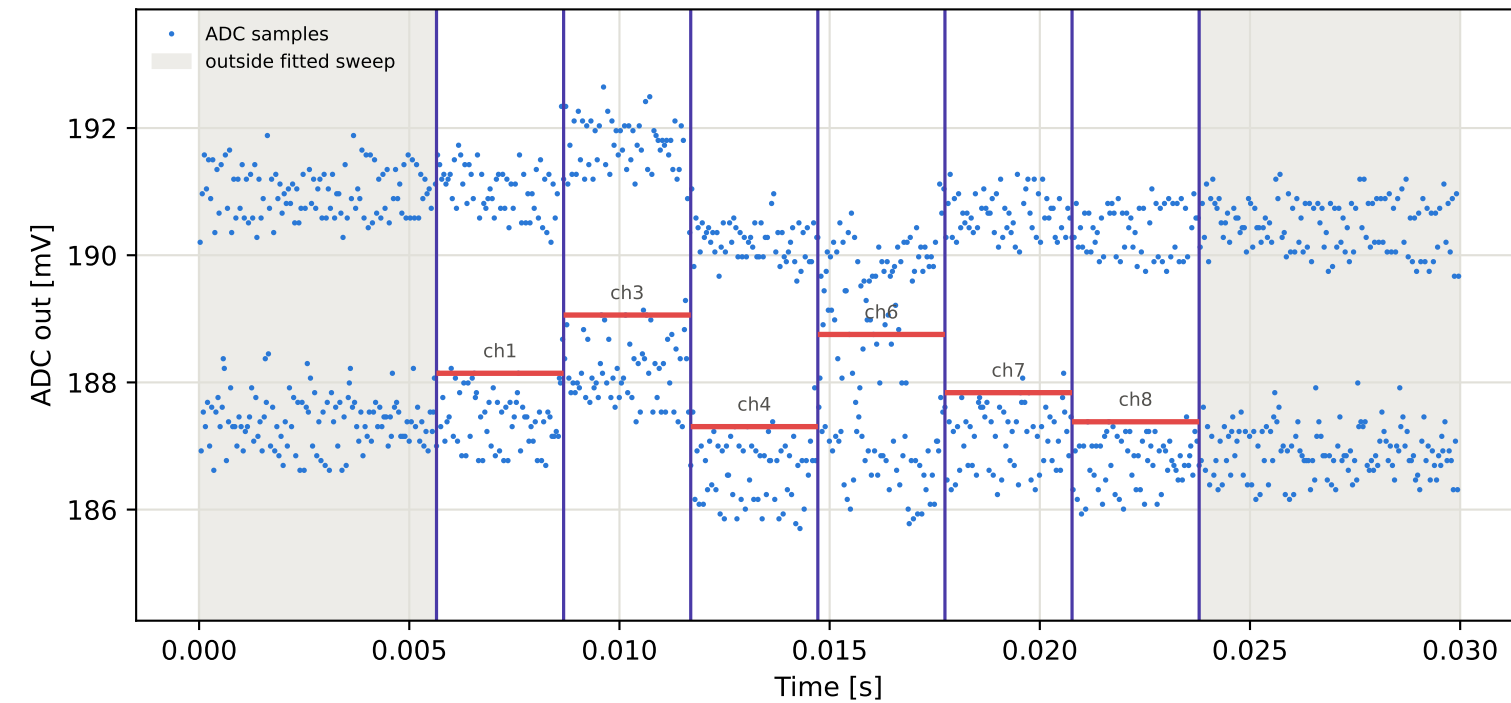
Tag16 &lt;- Tag6 | 795 MHz | run 0 | rep 1 | phase -85.69 deg
