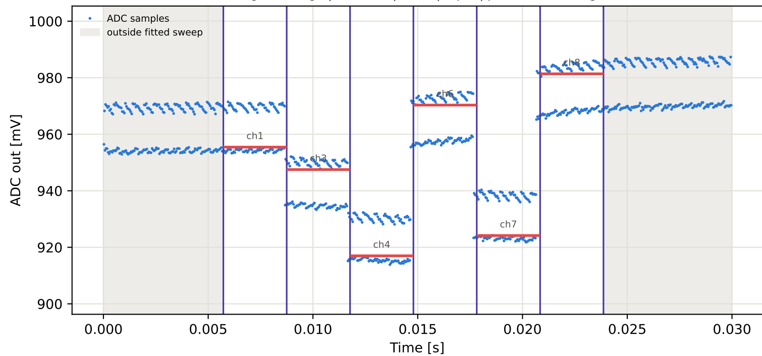
Tag2 &lt;- Tag10 | 935 MHz | run 0 | rep 1 | phase 173.56 deg
