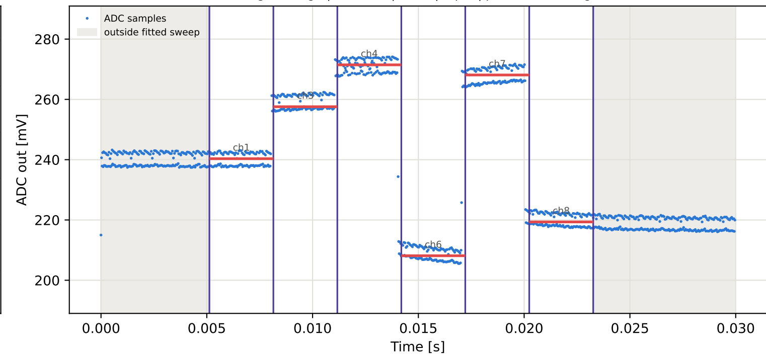
Tag1 &lt;- Tag8 | 965 MHz | run 0 | rep 1 | phase 71.17 deg
