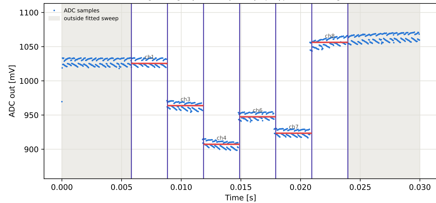
Tag7 &lt;- Tag3 | 905 MHz | run 0 | rep 1 | phase 162.57 deg
