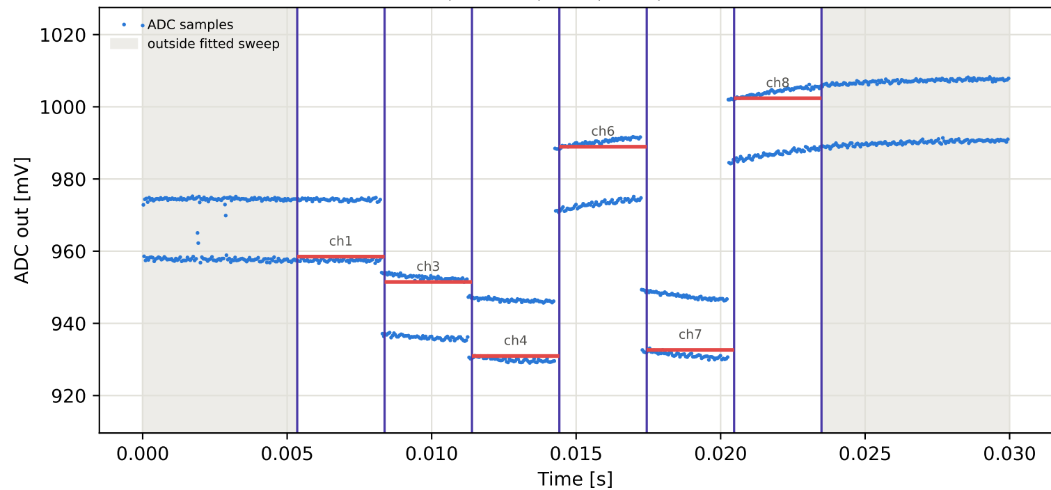
Tag3 &lt;- Tag9 | 905 MHz | run 0 | rep 1 | phase 138.08 deg
