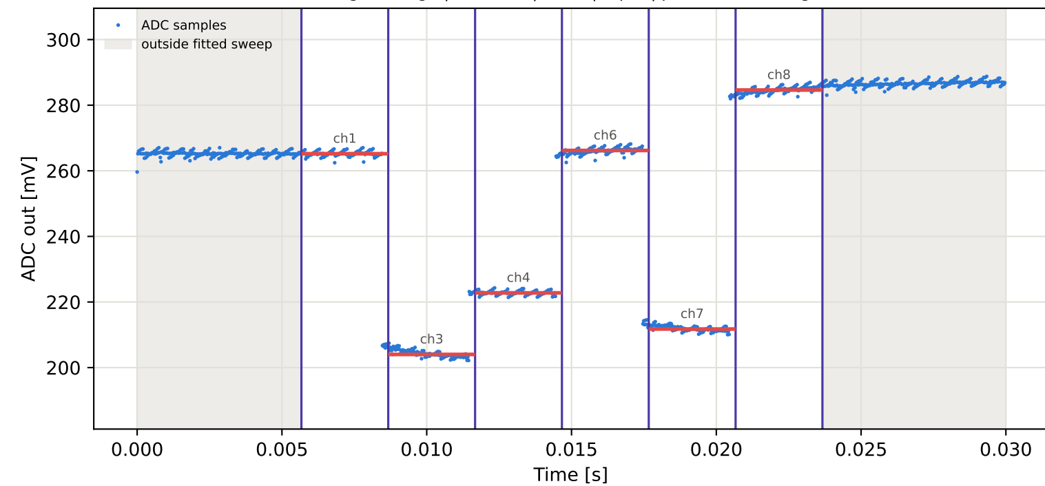
Tag9 &lt;- Tag5 | 845 MHz | run 0 | rep 1 | phase -173.51 deg
