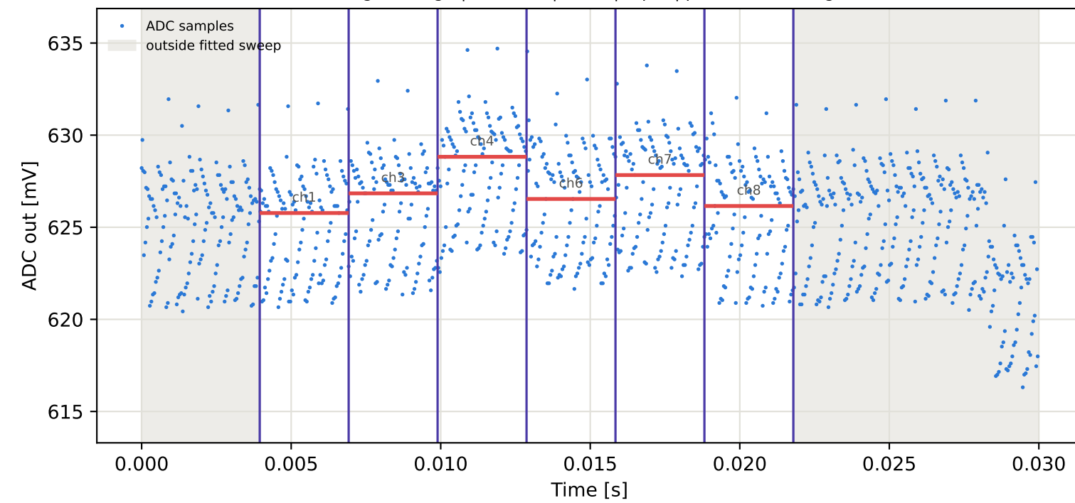
Tag3 &lt;- Tag10 | 965 MHz | run 0 | rep 1 | phase 11.80 deg
