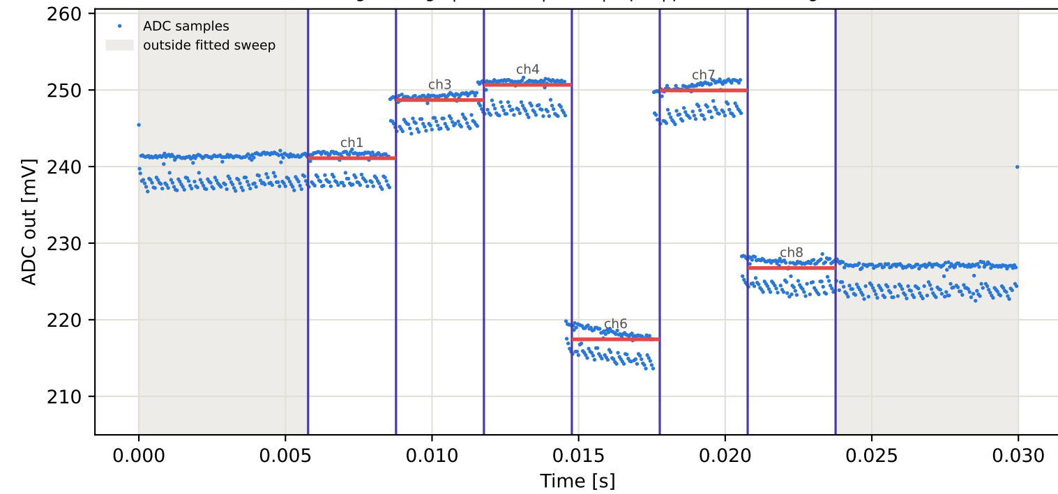
Tag1 &lt;- Tag3 | 925 MHz | run 0 | rep 1 | phase -17.62 deg
