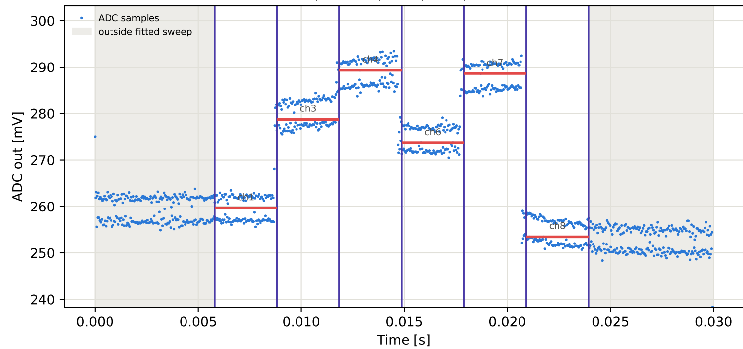
Tag9 &lt;- Tag15 | 885 MHz | run 0 | rep 1 | phase -123.62 deg
