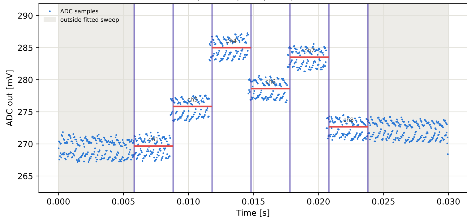
Tag8 &lt;- Tag10 | 835 MHz | run 0 | rep 1 | phase 125.69 deg
