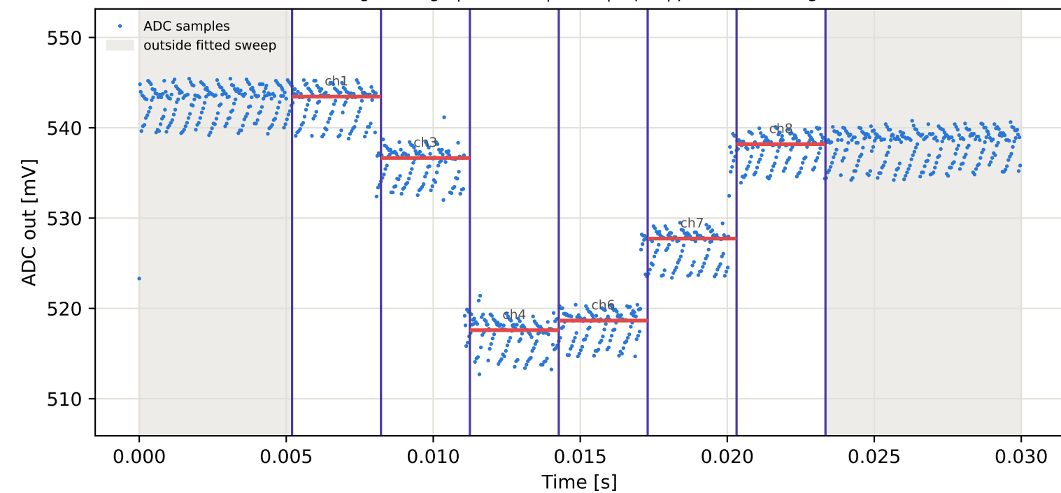
Tag4 &lt;- Tag9 | 945 MHz | run 0 | rep 1 | phase 53.41 deg
