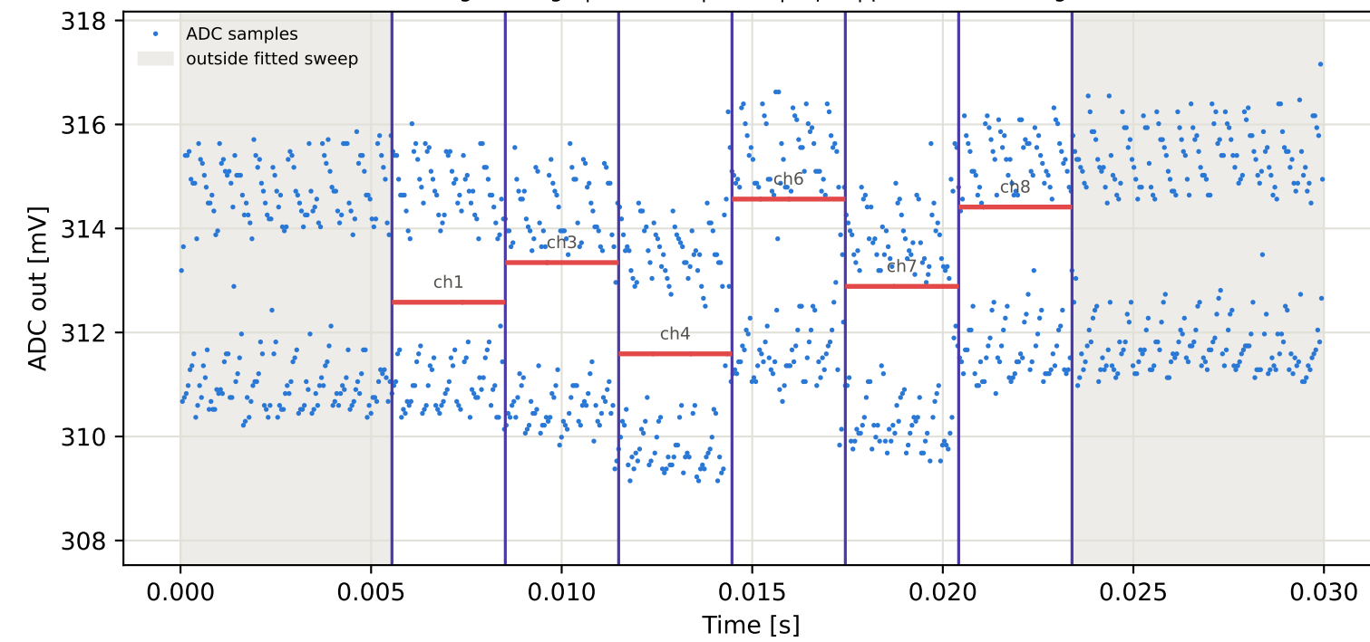
Tag4 &lt;- Tag2 | 995 MHz | run 0 | rep 1 | phase 122.58 deg
