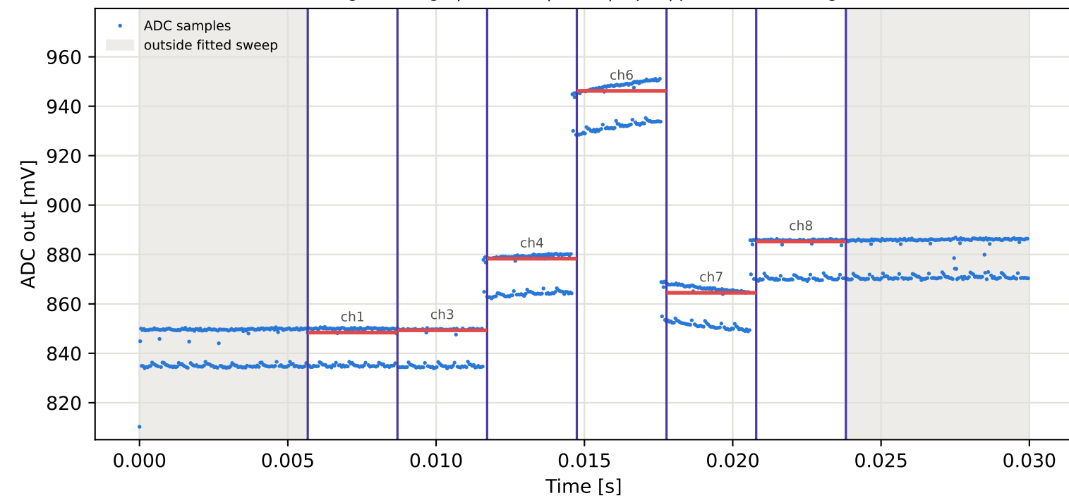
Tag16 &lt;- Tag5 | 925 MHz | run 0 | rep 1 | phase -163.32 deg
