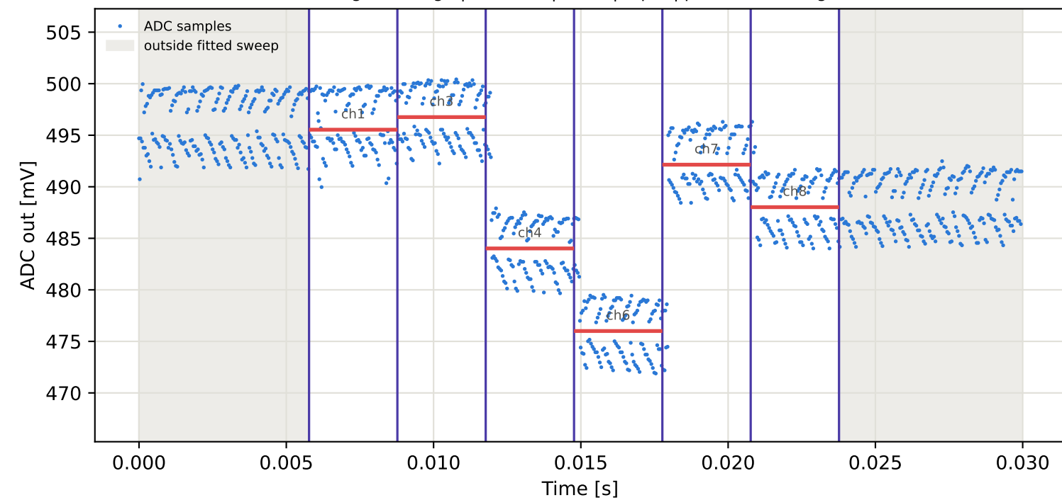
Tag16 &lt;- Tag15 | 975 MHz | run 0 | rep 1 | phase 165.46 deg
