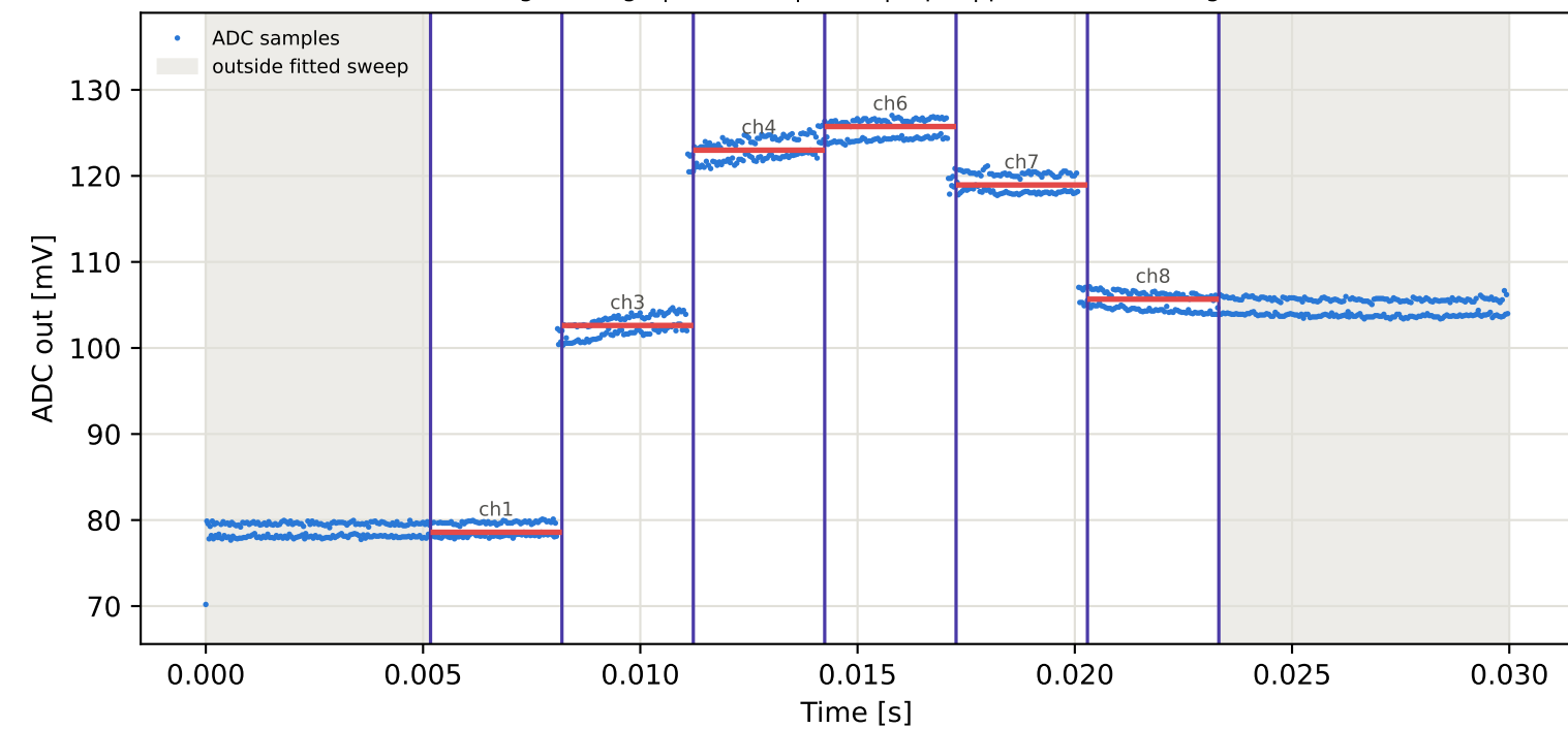
Tag9 &lt;- Tag7 | 865 MHz | run 0 | rep 1 | phase -14.28 deg
