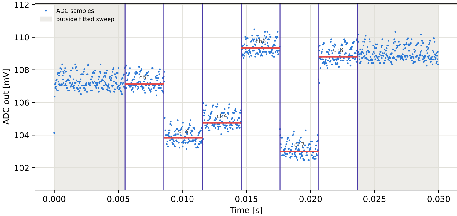
Tag5 &lt;- Tag1 | 795 MHz | run 0 | rep 1 | phase 165.03 deg
