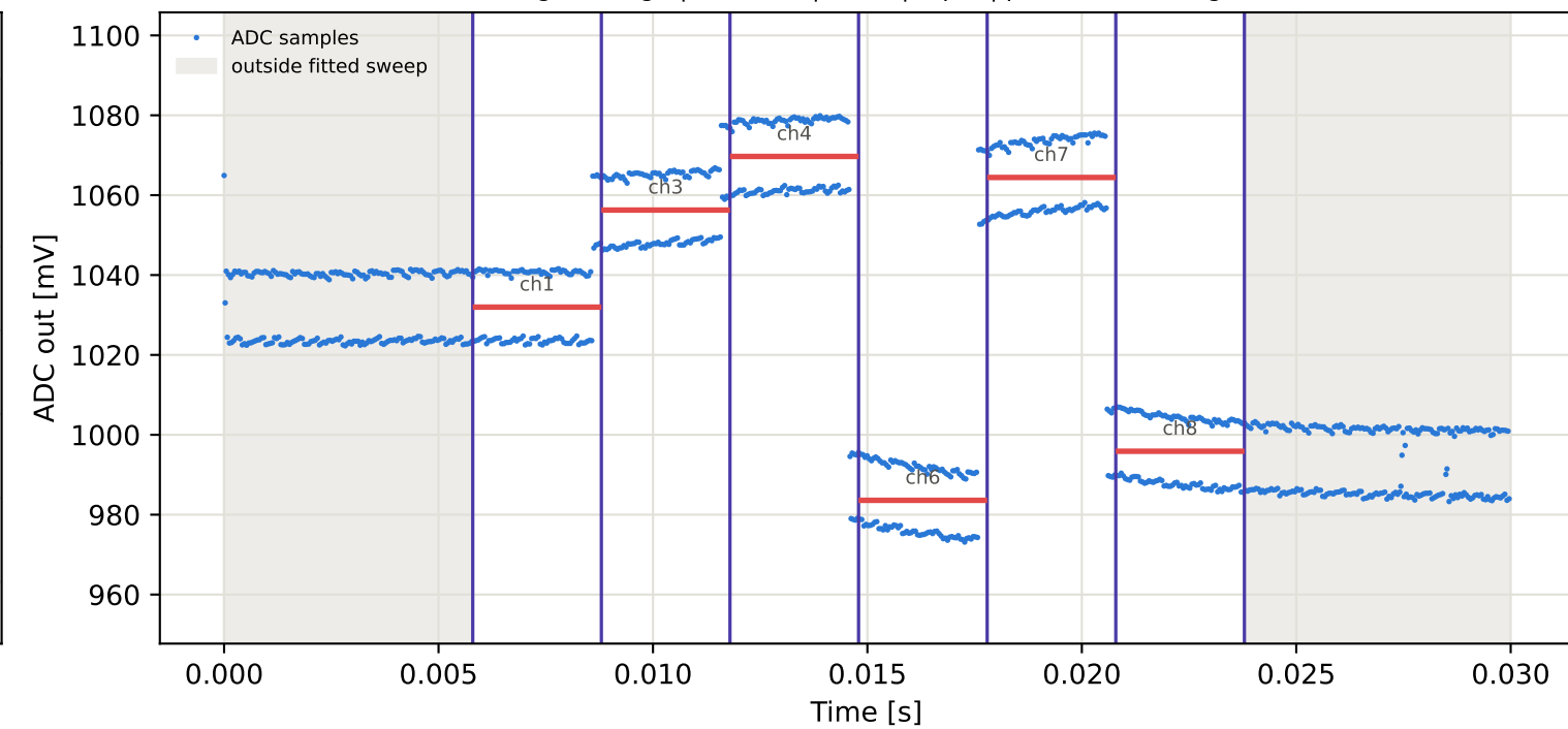
Tag8 &lt;- Tag5 | 925 MHz | run 0 | rep 1 | phase 56.51 deg
