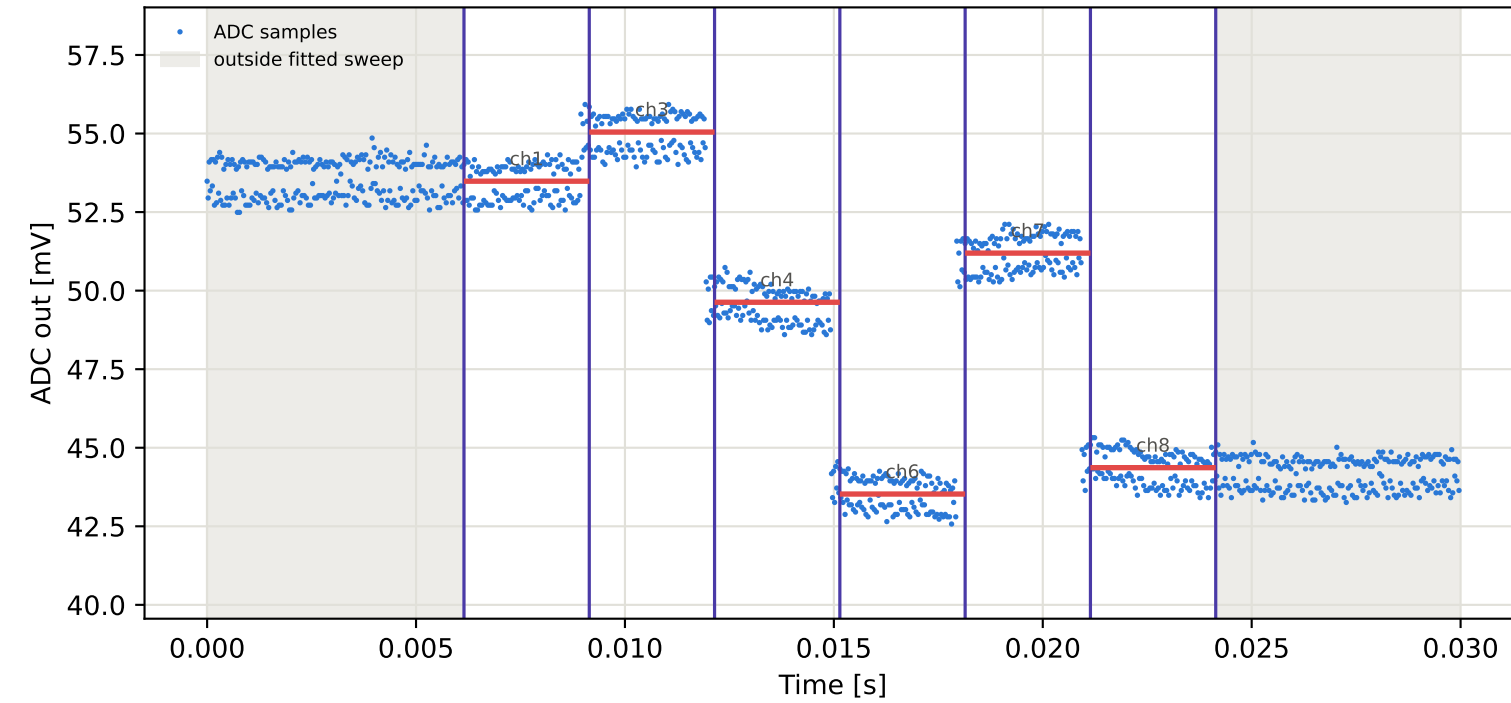
Tag1 &lt;- Tag3 | 865 MHz | run 0 | rep 1 | phase -40.96 deg
