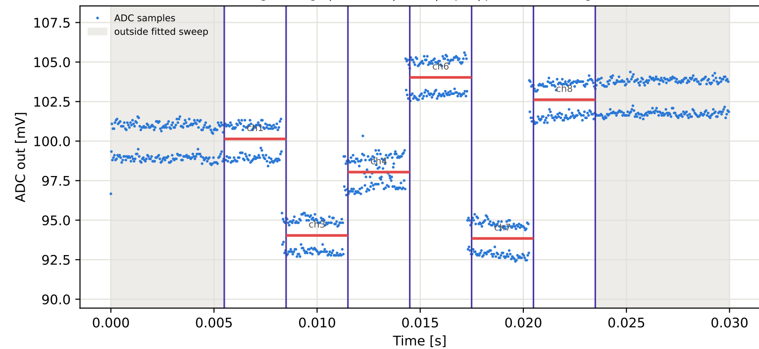
Tag4 &lt;- Tag7 | 775 MHz | run 0 | rep 1 | phase -94.25 deg
