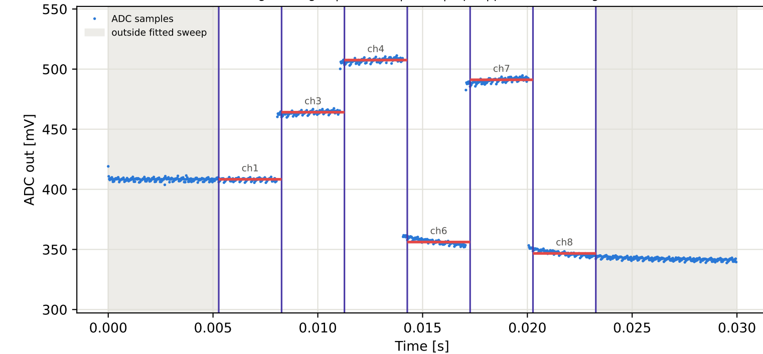
Tag3 &lt;- Tag16 | 935 MHz | run 0 | rep 1 | phase -47.98 deg
