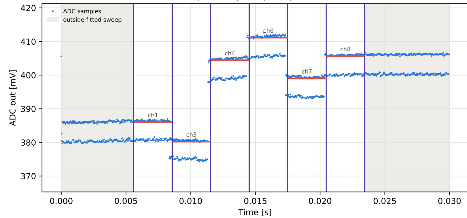
Tag2 &lt;- Tag5 | 835 MHz | run 0 | rep 1 | phase -138.58 deg
