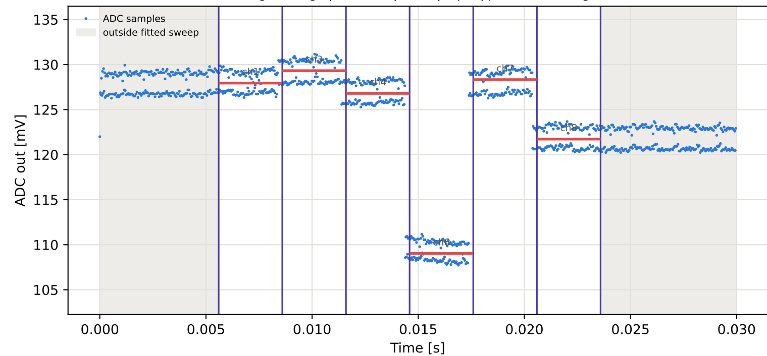
Tag1 &lt;- Tag4 | 855 MHz | run 0 | rep 1 | phase -131.25 deg
