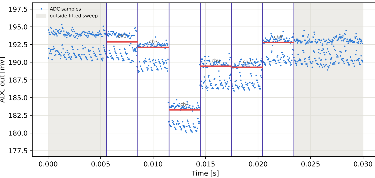
Tag6 &lt;- Tag4 | 985 MHz | run 0 | rep 1 | phase 62.91 deg
