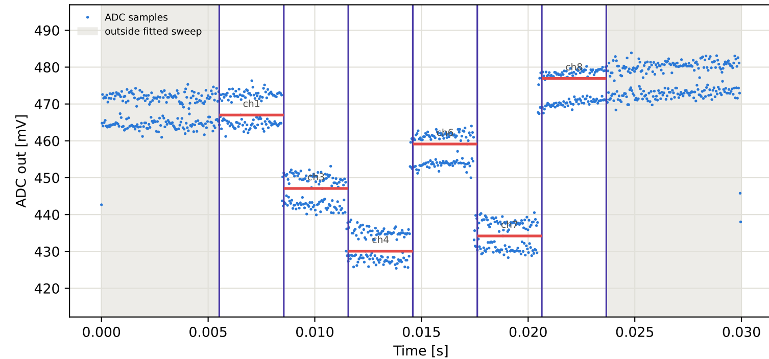
Tag1 &lt;- Tag9 | 885 MHz | run 0 | rep 1 | phase -139.84 deg
