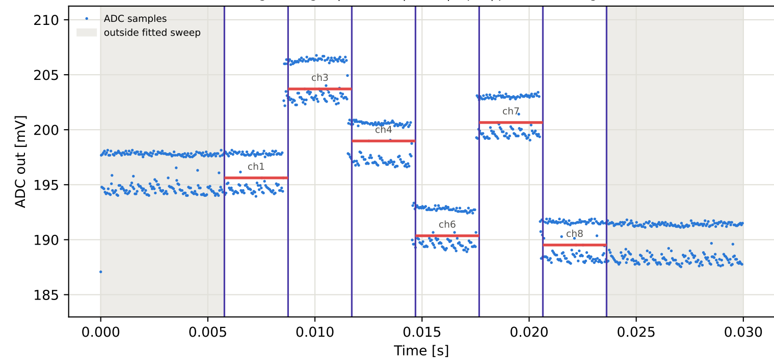
Tag4 &lt;- Tag16 | 835 MHz | run 0 | rep 1 | phase -117.26 deg
