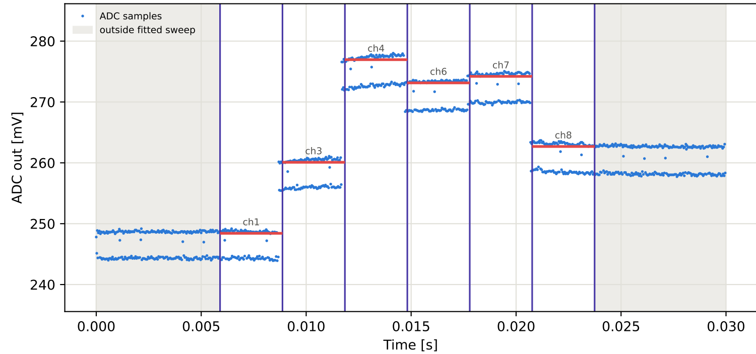
Tag4 &lt;- Tag2 | 855 MHz | run 0 | rep 1 | phase 142.01 deg
