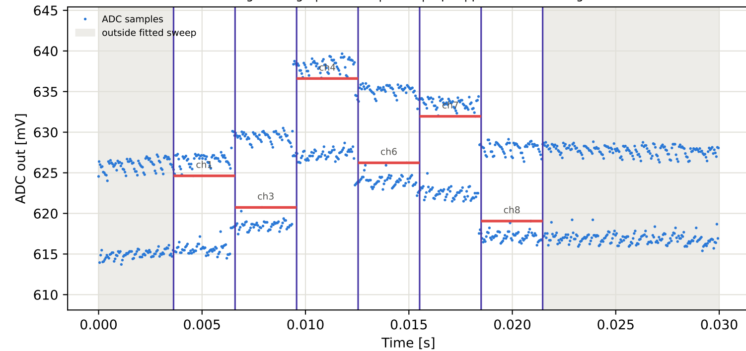
Tag2 &lt;- Tag5 | 965 MHz | run 0 | rep 1 | phase 84.34 deg
