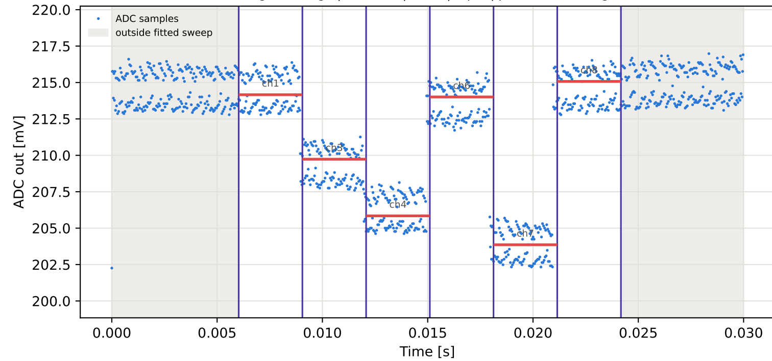
Tag16 &lt;- Tag1 | 785 MHz | run 0 | rep 1 | phase 146.98 deg
