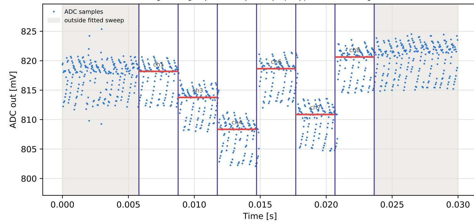
Tag2 &lt;- Tag15 | 955 MHz | run 0 | rep 1 | phase 109.00 deg
