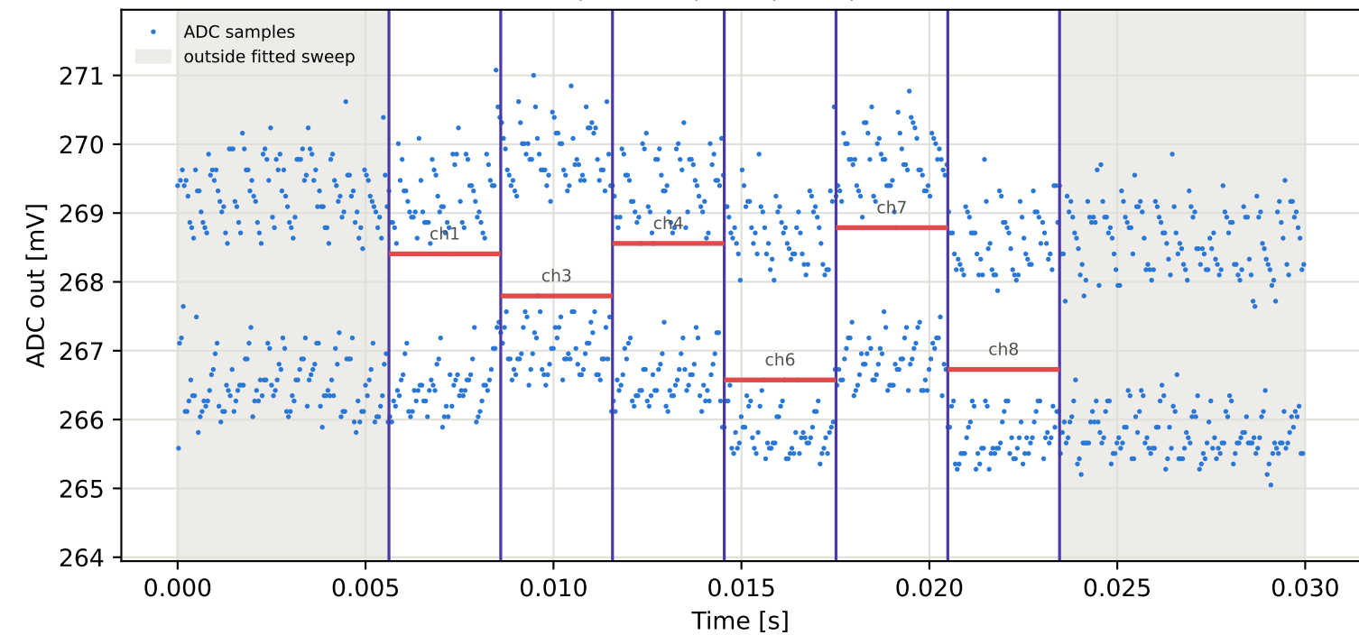
Tag5 &lt;- Tag1 | 835 MHz | run 0 | rep 1 | phase -17.42 deg
