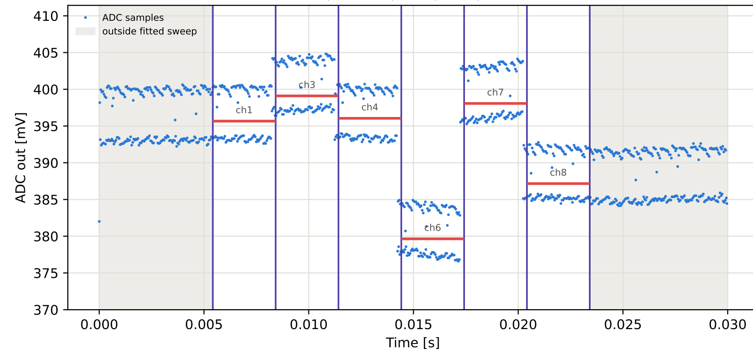
Tag9 &lt;- Tag7 | 955 MHz | run 0 | rep 1 | phase -2.16 deg
