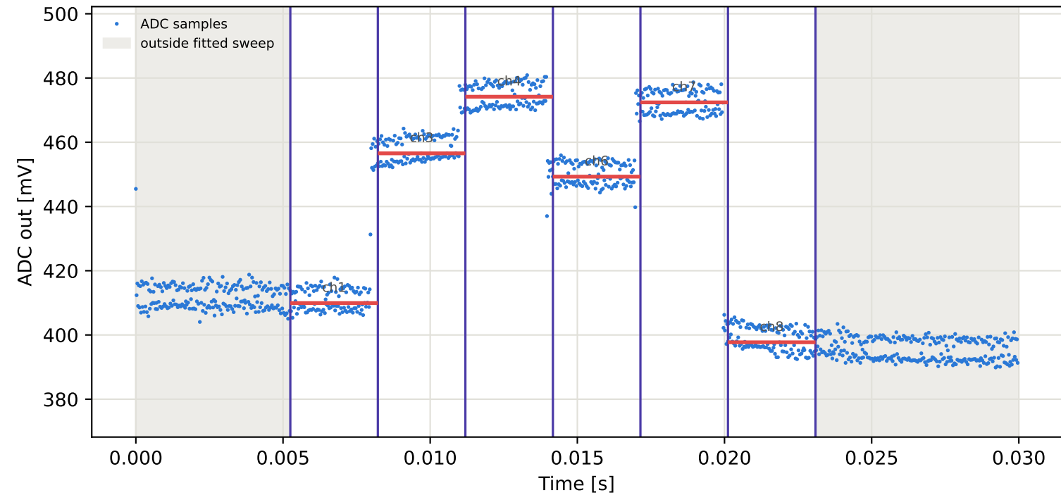
Tag10 &lt;- Tag1 | 885 MHz | run 0 | rep 1 | phase 5.44 deg
