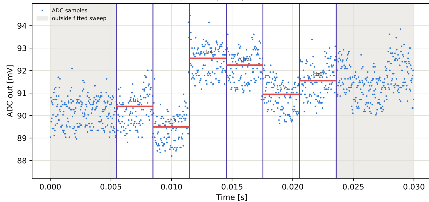
Tag6 &lt;- Tag2 | 785 MHz | run 0 | rep 1 | phase -170.19 deg
