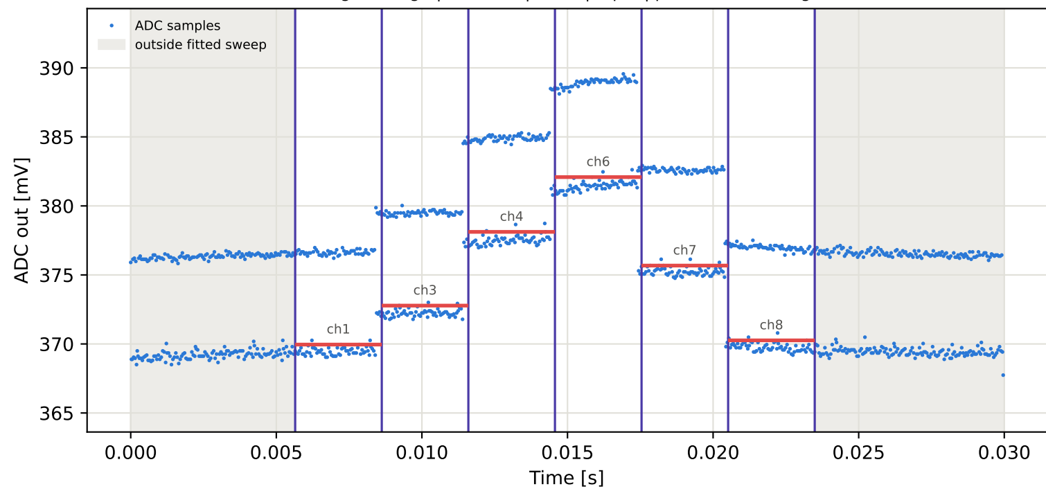
Tag1 &lt;- Tag4 | 955 MHz | run 0 | rep 1 | phase 70.40 deg
