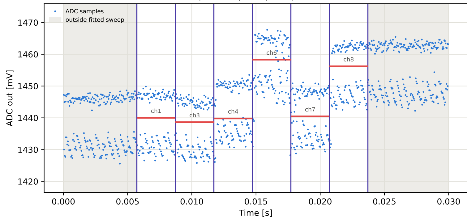
Tag2 &lt;- Tag6 | 885 MHz | run 0 | rep 1 | phase -114.61 deg
