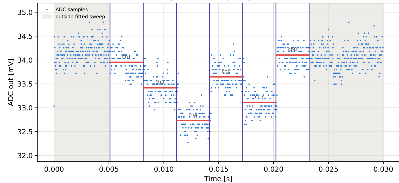
Tag4 &lt;- Tag15 | 805 MHz | run 0 | rep 1 | phase 95.18 deg
