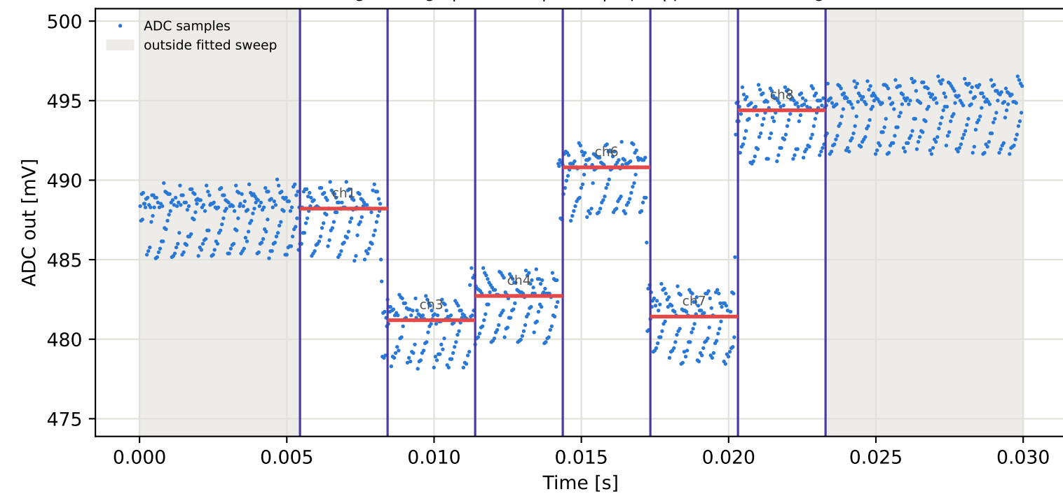
Tag8 &lt;- Tag6 | 865 MHz | run 0 | rep 1 | phase -92.68 deg
