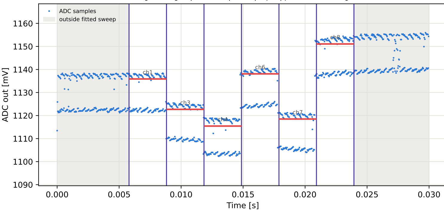
Tag7 &lt;- Tag10 | 895 MHz | run 0 | rep 1 | phase 124.36 deg
