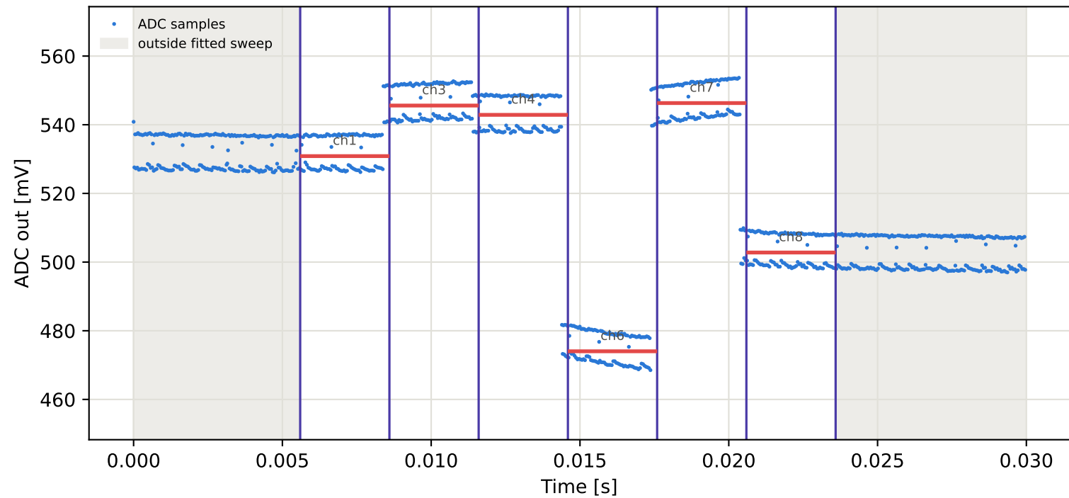
Tag10 &lt;- Tag5 | 945 MHz | run 0 | rep 1 | phase 19.86 deg
