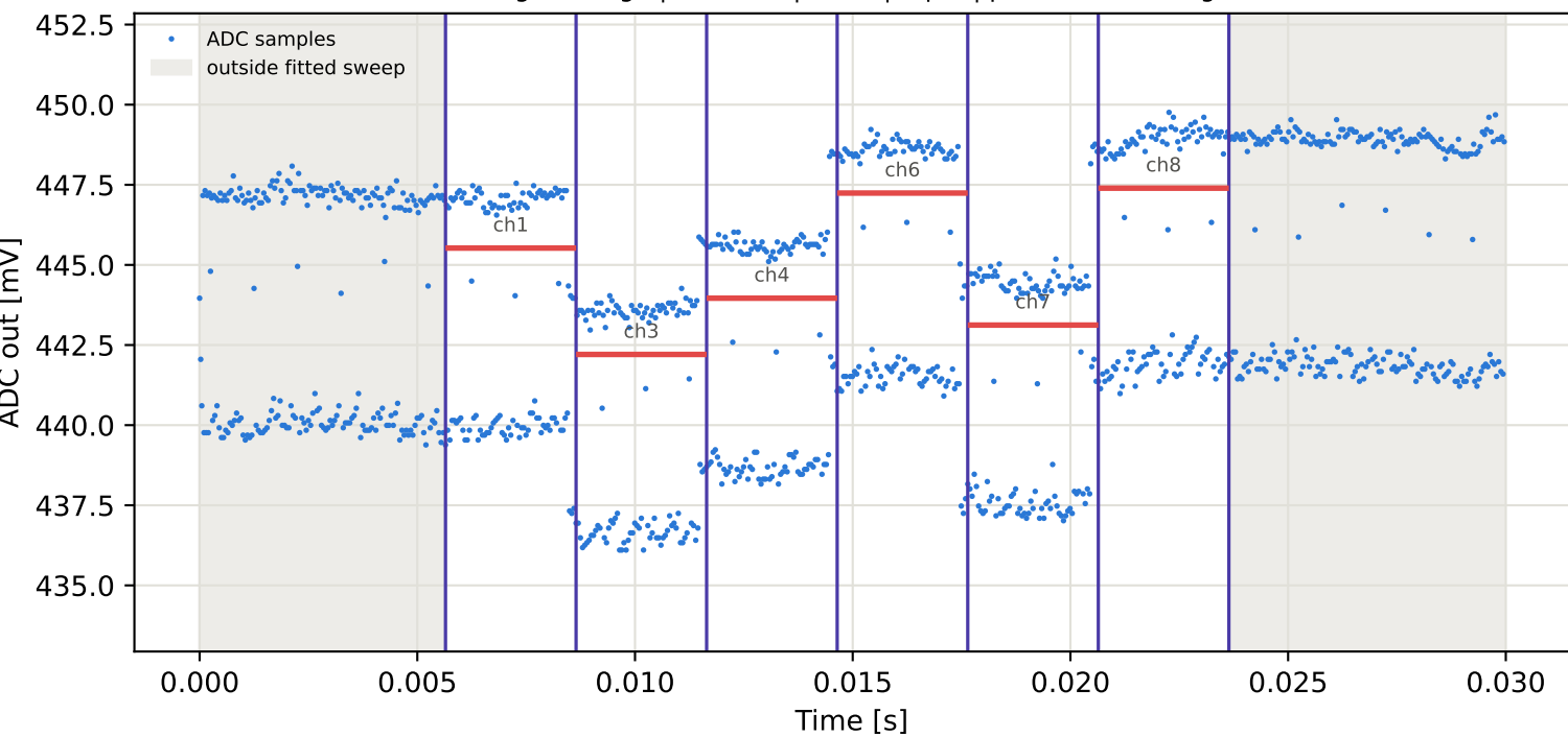
Tag6 &lt;- Tag1 | 835 MHz | run 0 | rep 1 | phase 169.37 deg
