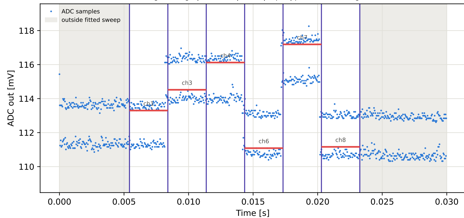
Tag2 &lt;- Tag8 | 775 MHz | run 0 | rep 1 | phase 53.27 deg
