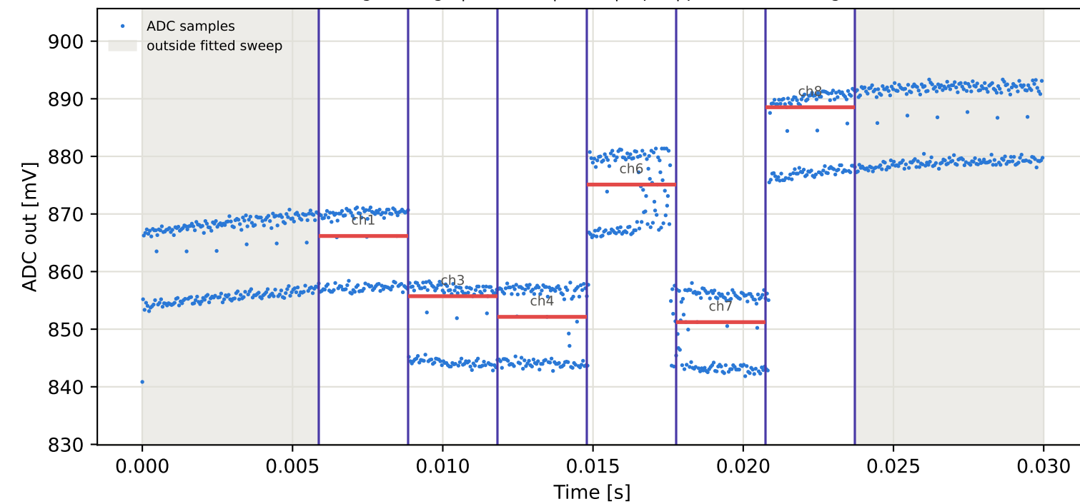
Tag3 &lt;- Tag6 | 885 MHz | run 0 | rep 1 | phase -66.40 deg
