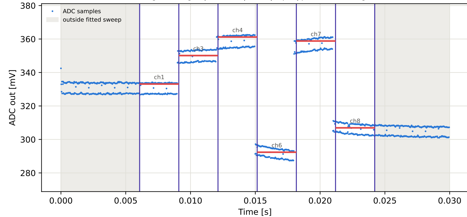
Tag10 &lt;- Tag3 | 955 MHz | run 0 | rep 1 | phase 40.17 deg
