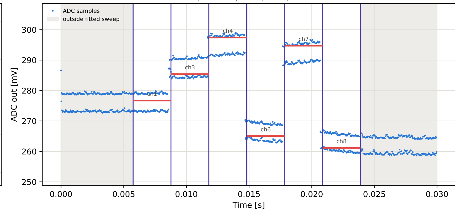
Tag6 &lt;- Tag3 | 925 MHz | run 0 | rep 1 | phase -16.55 deg
