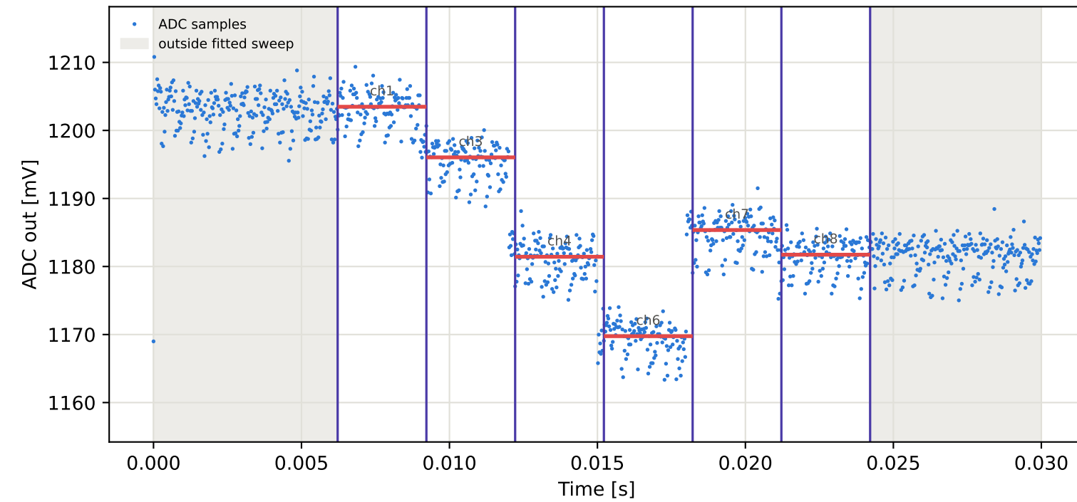
Tag7 &lt;- Tag10 | 885 MHz | run 0 | rep 1 | phase 105.88 deg
