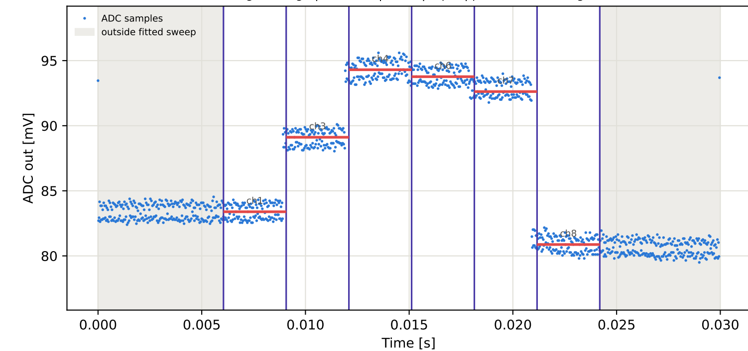
Tag1 &lt;- Tag4 | 825 MHz | run 0 | rep 1 | phase -162.84 deg
