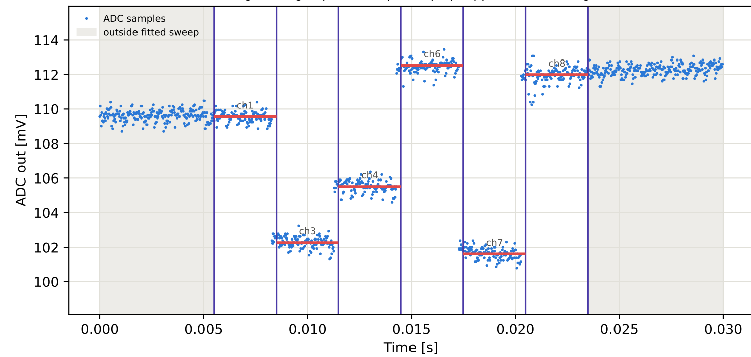
Tag5 &lt;- Tag2 | 795 MHz | run 0 | rep 1 | phase -37.72 deg
