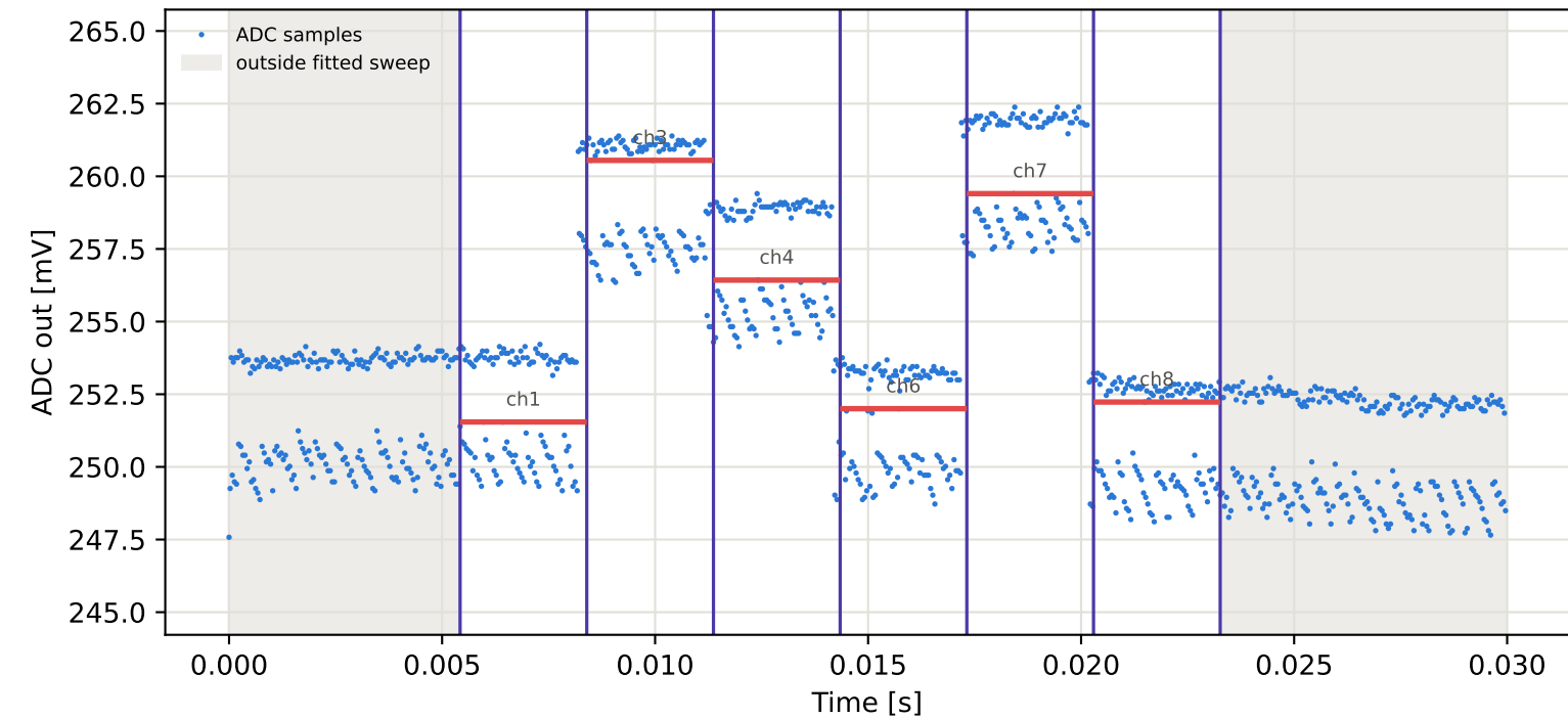
Tag15 &lt;- Tag5 | 805 MHz | run 0 | rep 1 | phase -166.95 deg
