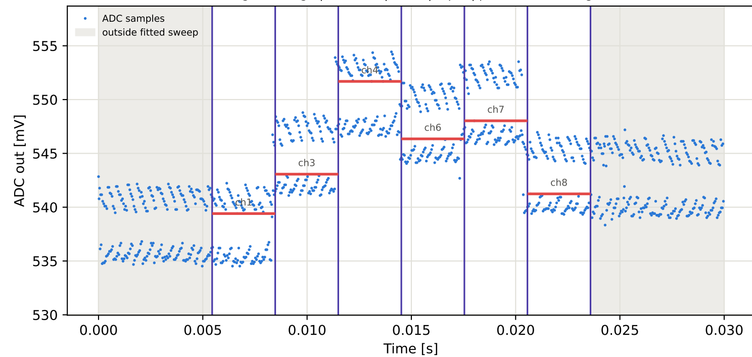
Tag16 &lt;- Tag1 | 855 MHz | run 0 | rep 1 | phase 92.20 deg
