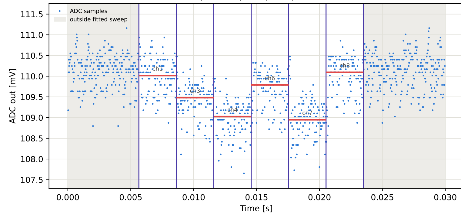
Tag3 &lt;- Tag10 | 795 MHz | run 0 | rep 1 | phase 113.46 deg
