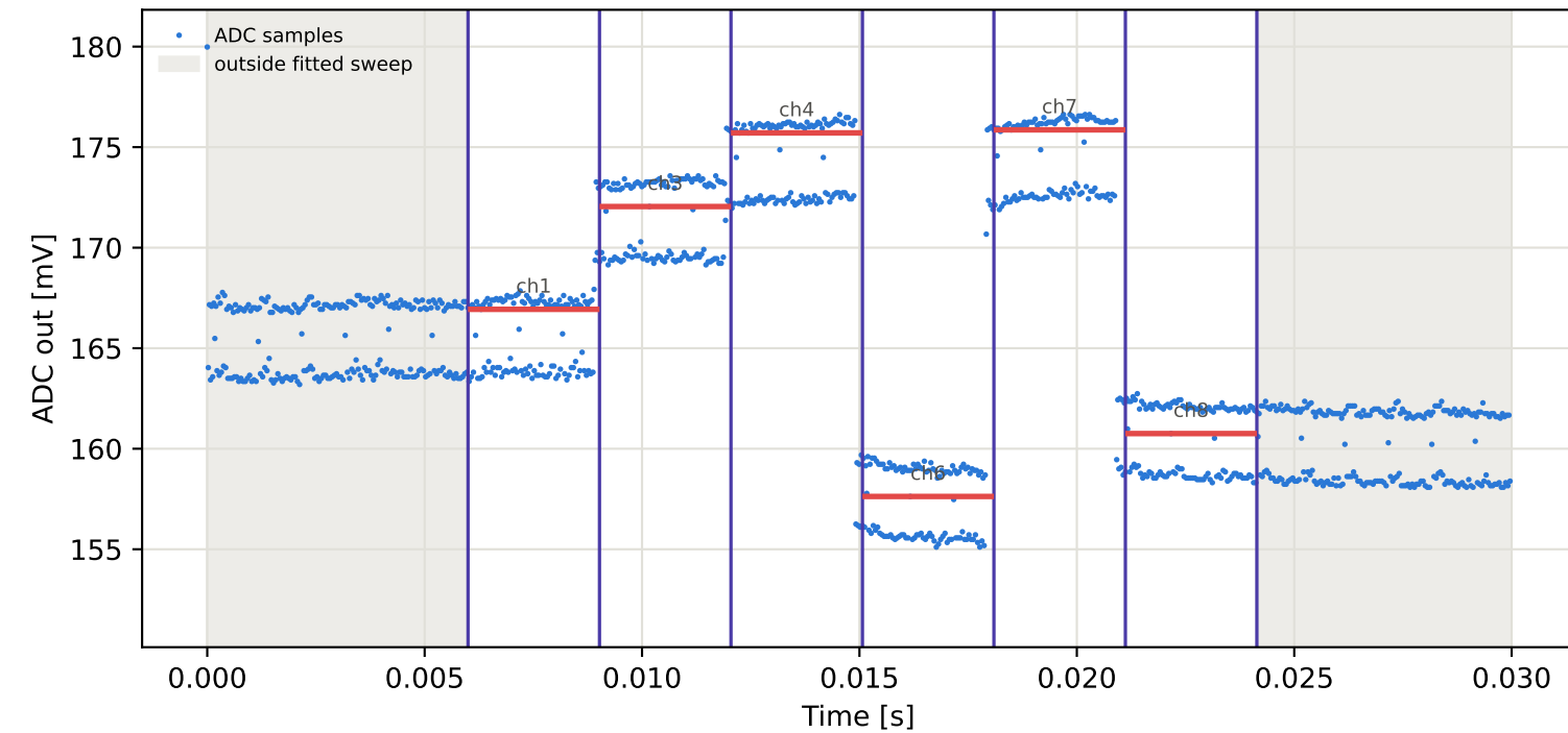
Tag1 &lt;- Tag3 | 995 MHz | run 0 | rep 1 | phase -52.48 deg
