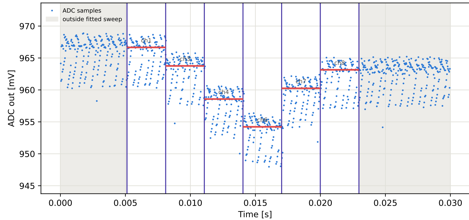
Tag7 &lt;- Tag6 | 905 MHz | run 0 | rep 1 | phase -84.55 deg
