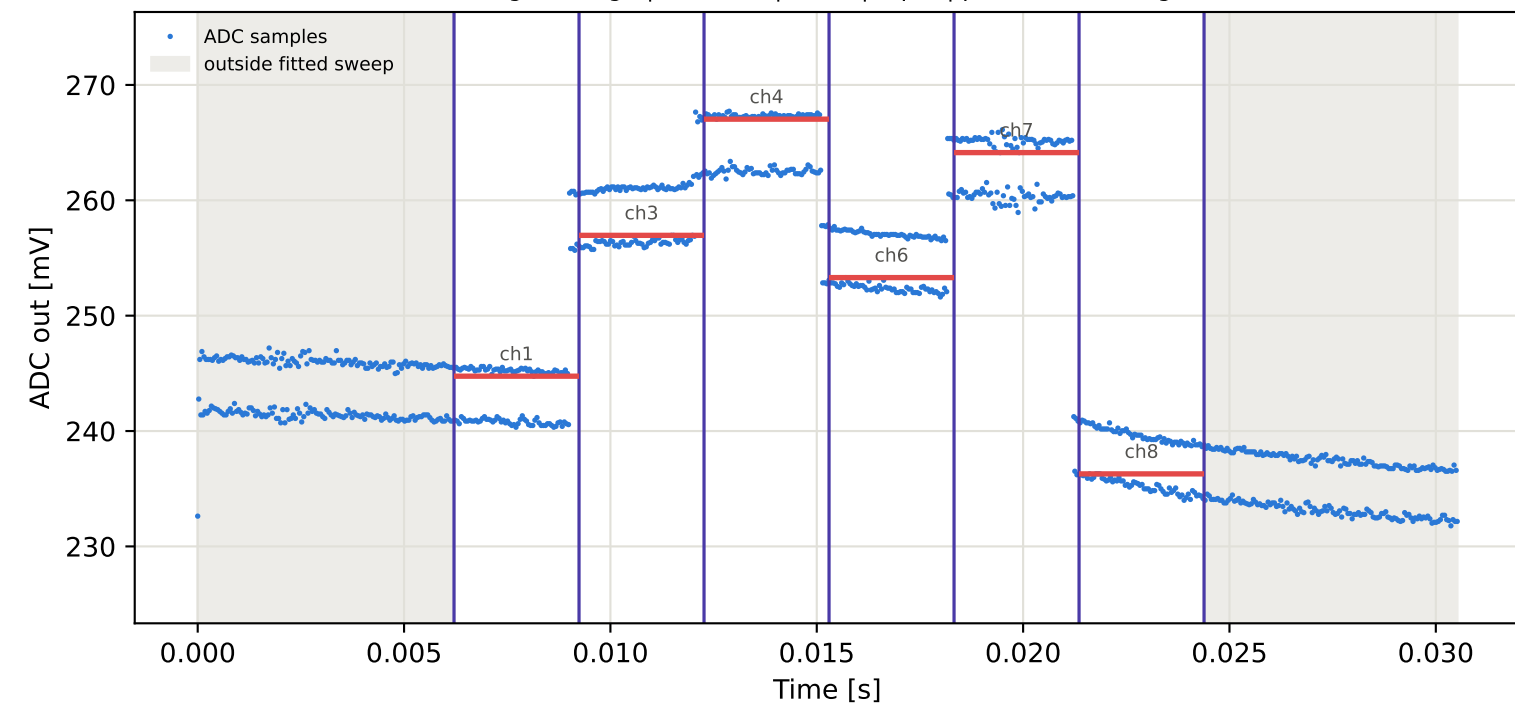
Tag9 &lt;- Tag6 | 875 MHz | run 0 | rep 1 | phase -174.09 deg
