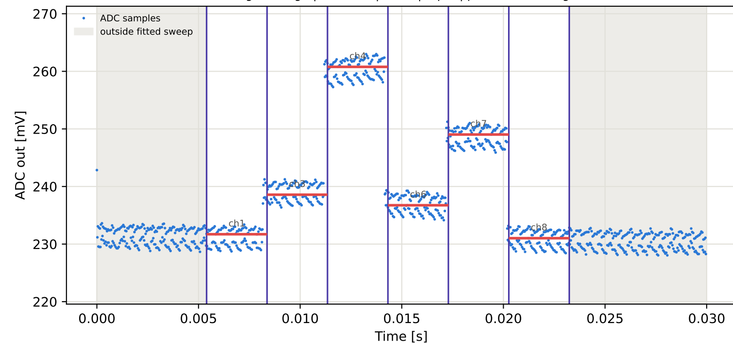
Tag6 &lt;- Tag1 | 995 MHz | run 0 | rep 1 | phase -99.26 deg
