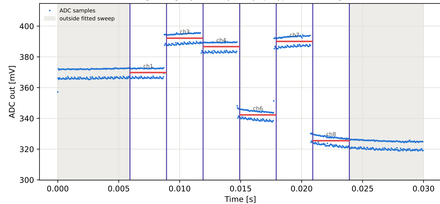
Tag1 &lt;- Tag16 | 875 MHz | run 0 | rep 1 | phase -131.34 deg
