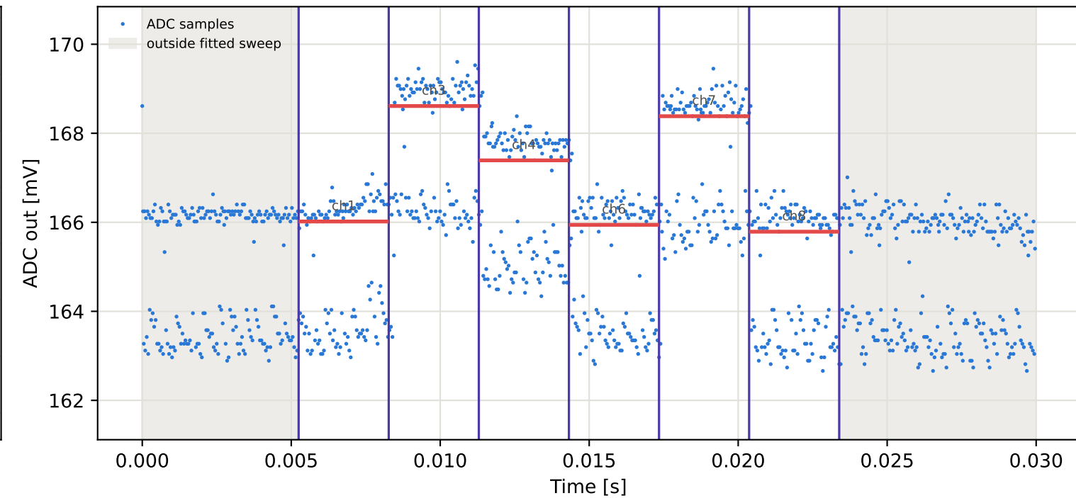
Tag2 &lt;- Tag16 | 805 MHz | run 0 | rep 1 | phase 106.08 deg
