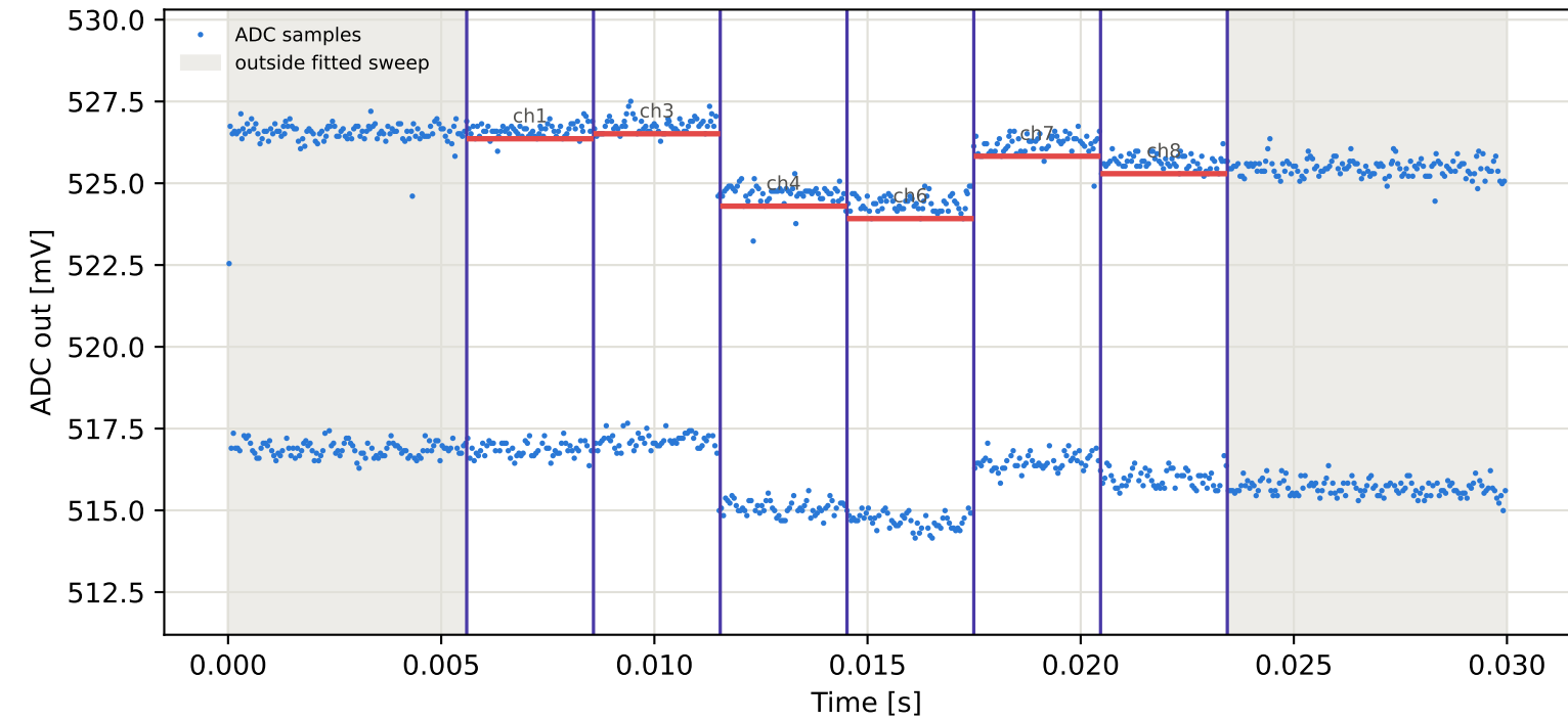
Tag7 &lt;- Tag6 | 985 MHz | run 0 | rep 1 | phase 147.13 deg
