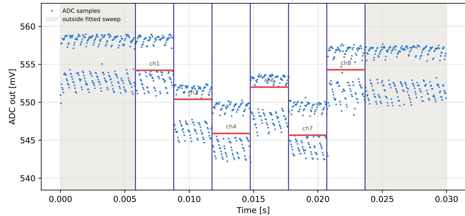
Tag15 &lt;- Tag6 | 855 MHz | run 0 | rep 1 | phase 104.10 deg
