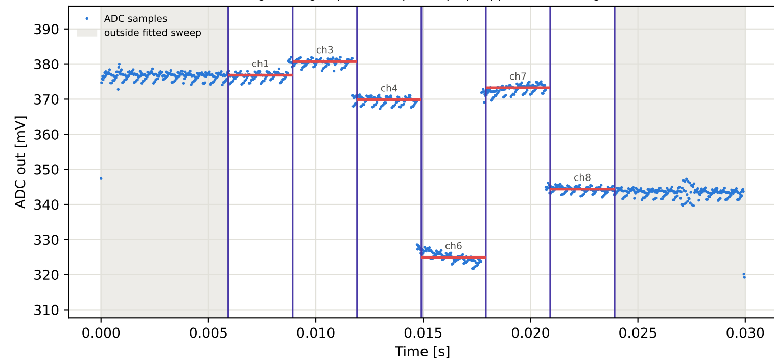
Tag4 &lt;- Tag16 | 895 MHz | run 0 | rep 1 | phase -90.63 deg
