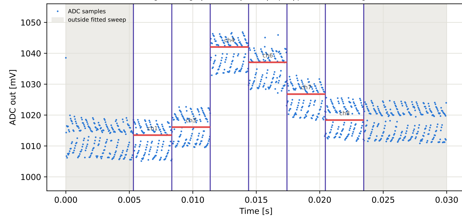
Tag16 &lt;- Tag10 | 975 MHz | run 0 | rep 1 | phase -67.13 deg
