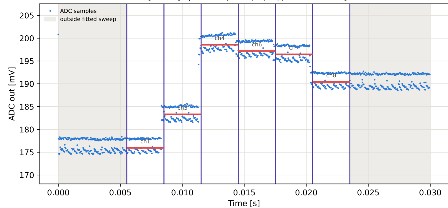
Tag4 &lt;- Tag3 | 835 MHz | run 0 | rep 1 | phase -117.37 deg
