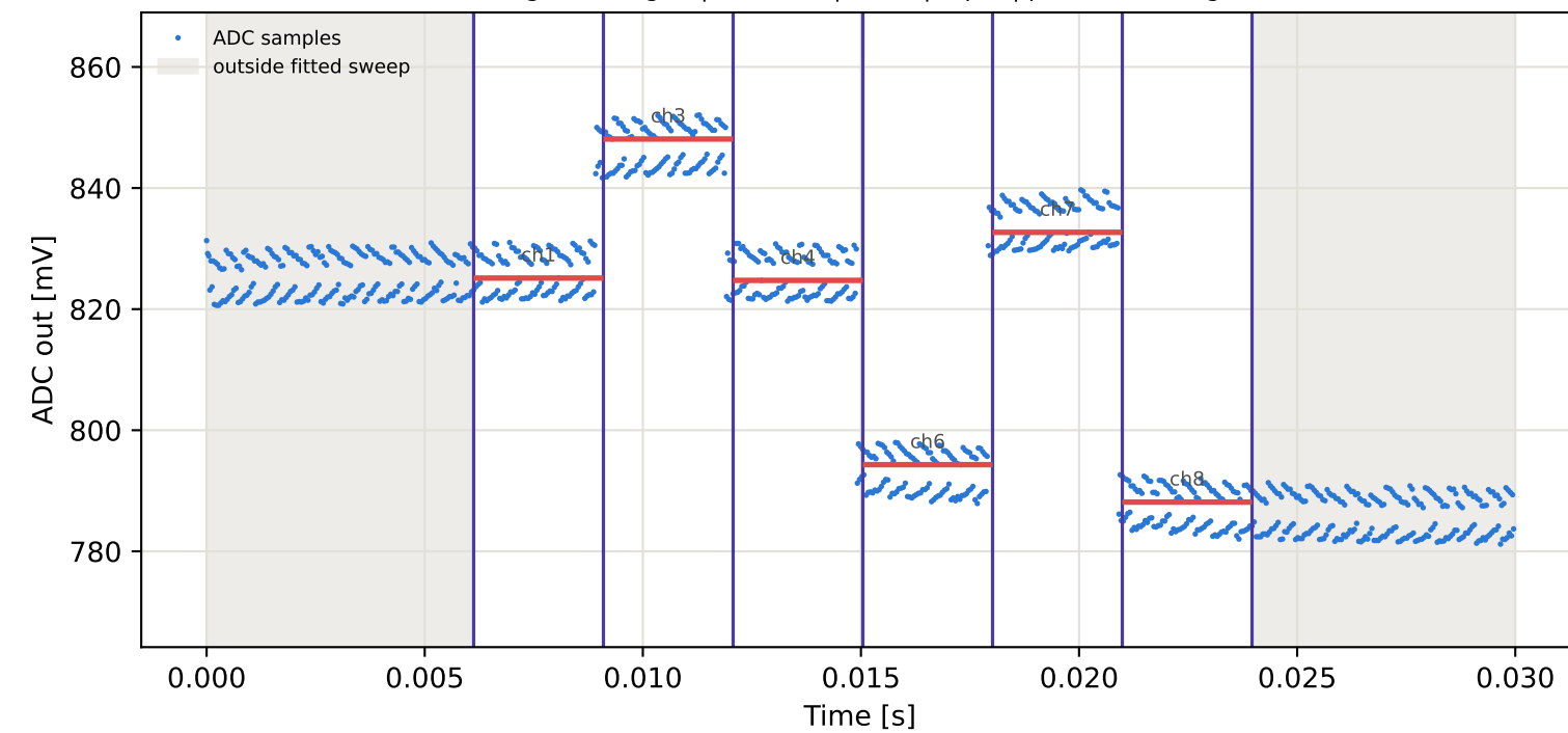
Tag15 &lt;- Tag3 | 865 MHz | run 0 | rep 1 | phase 100.52 deg
