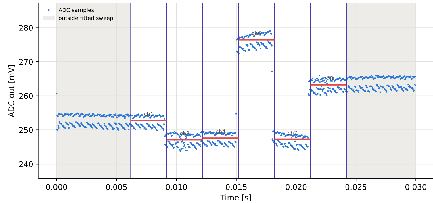
Tag9 &lt;- Tag2 | 875 MHz | run 0 | rep 1 | phase 176.81 deg
