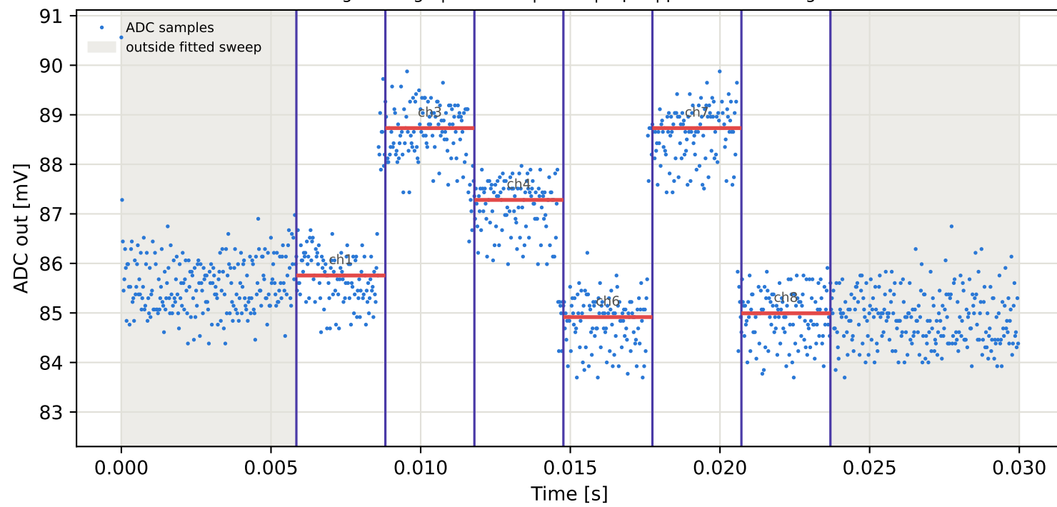
Tag3 &lt;- Tag6 | 795 MHz | run 0 | rep 1 | phase 120.36 deg
