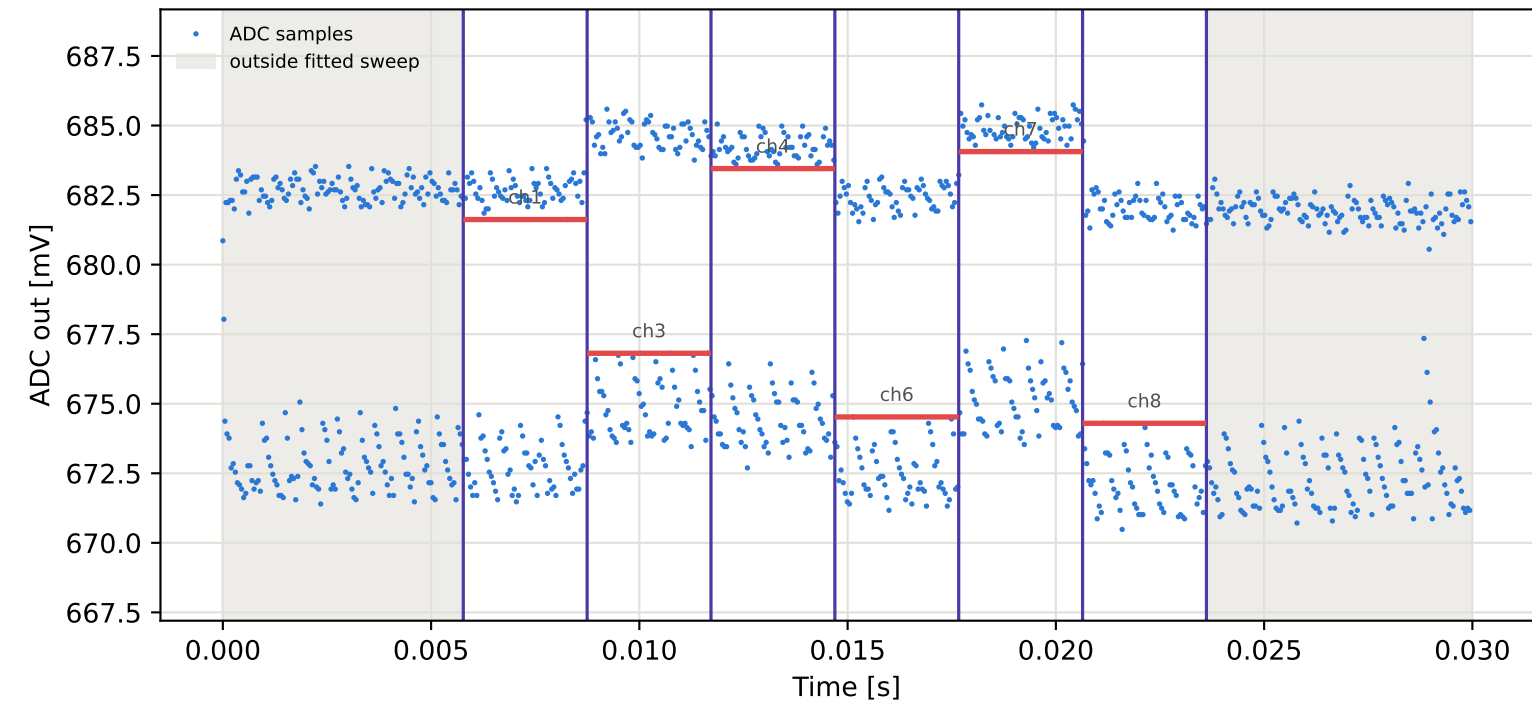
Tag16 &lt;- Tag15 | 845 MHz | run 0 | rep 1 | phase 59.49 deg
