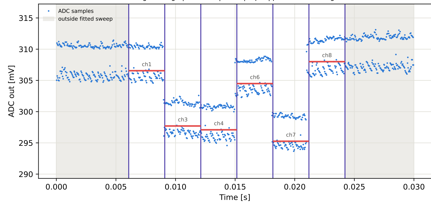
Tag7 &lt;- Tag1 | 845 MHz | run 0 | rep 1 | phase 75.69 deg
