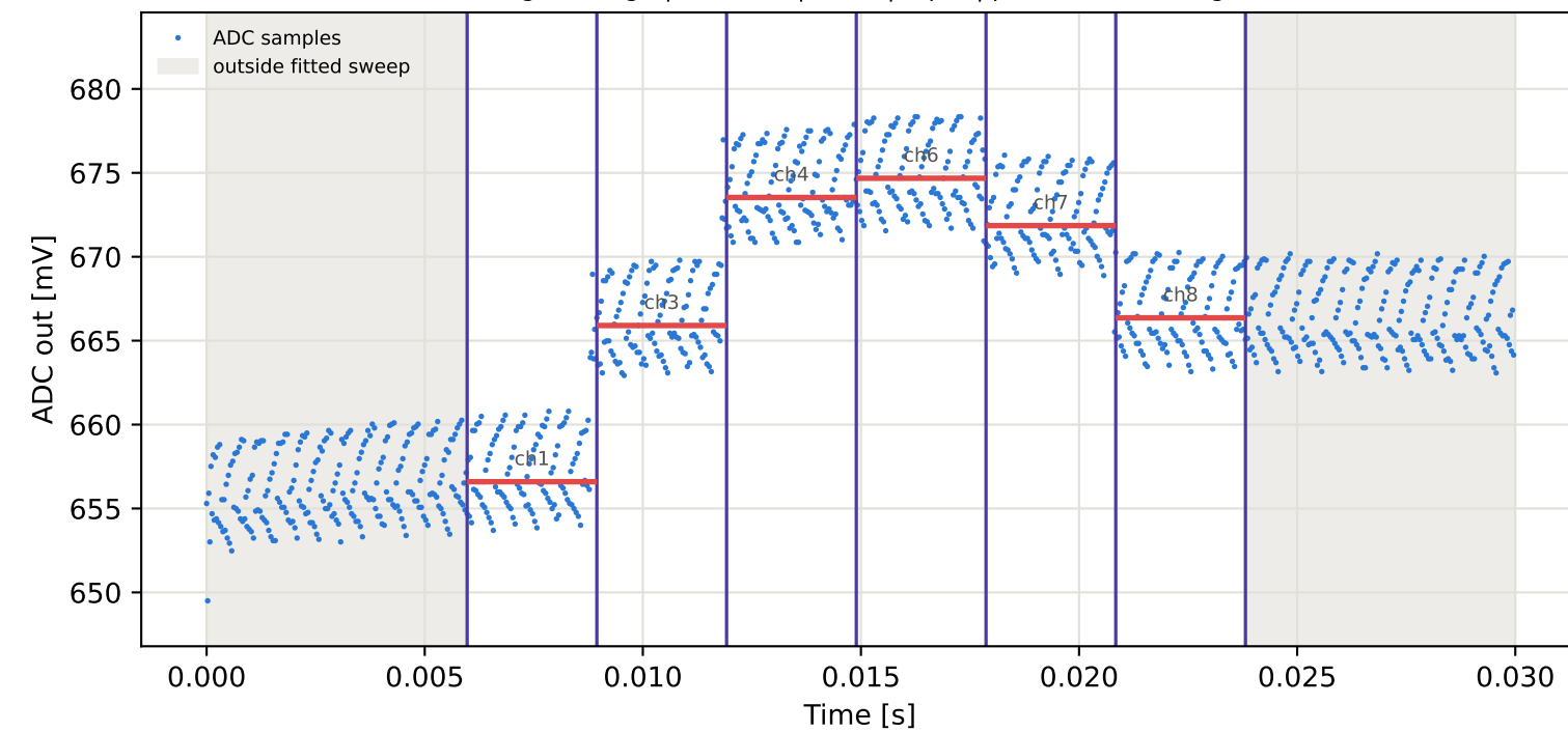
Tag5 &lt;- Tag8 | 865 MHz | run 0 | rep 1 | phase 82.08 deg
