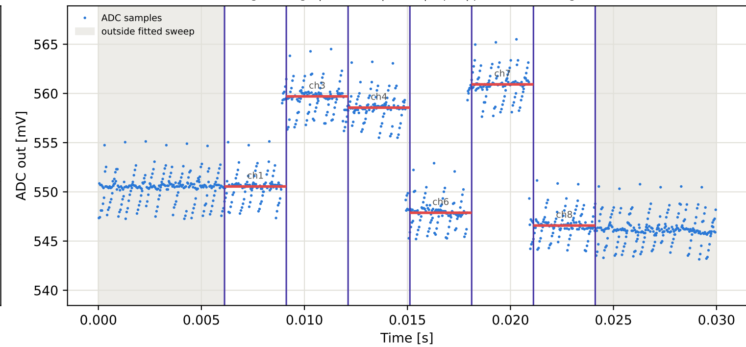
Tag8 &lt;- Tag10 | 845 MHz | run 0 | rep 1 | phase 167.00 deg
