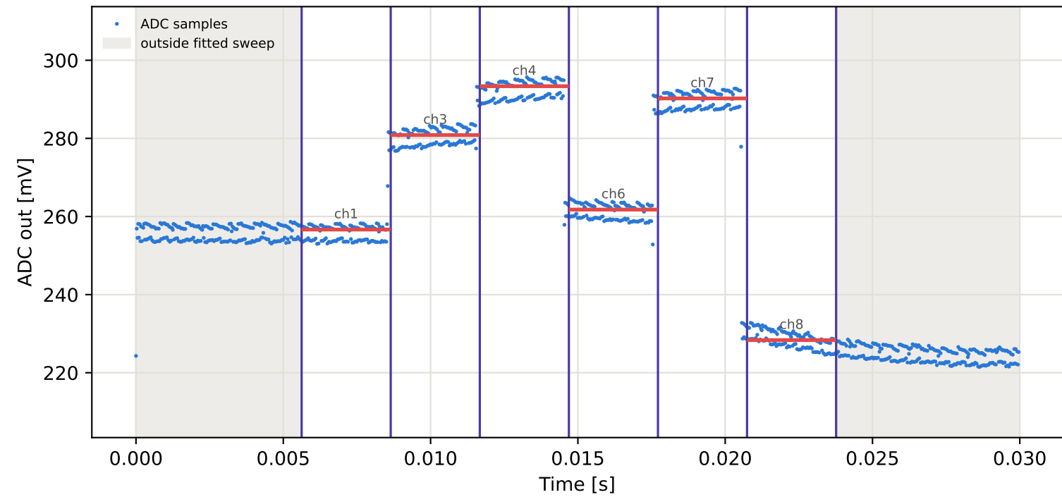
Tag9 &lt;- Tag2 | 905 MHz | run 0 | rep 1 | phase -19.68 deg
