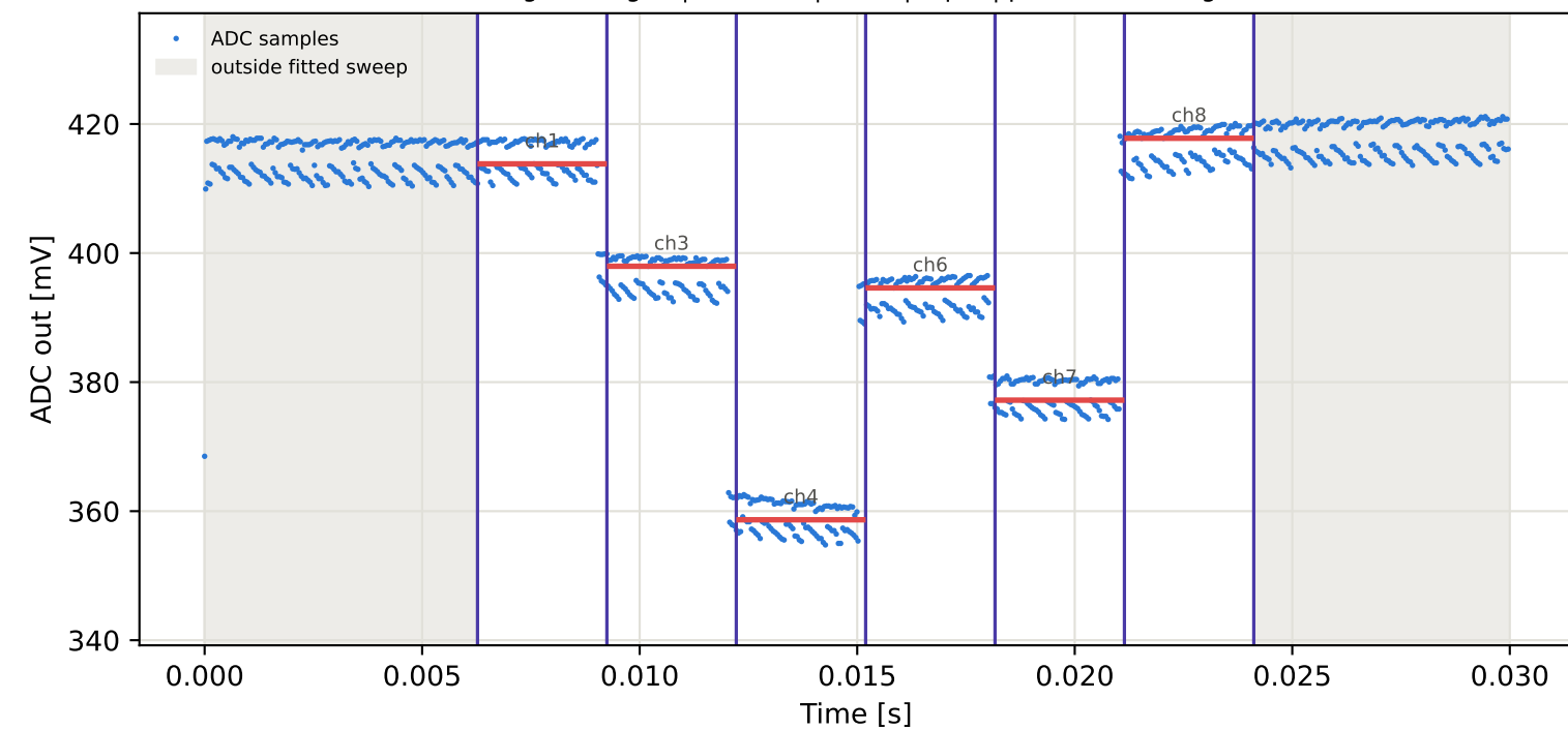
Tag8 &lt;- Tag16 | 955 MHz | run 0 | rep 1 | phase 79.90 deg
