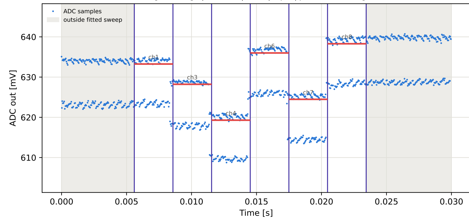
Tag16 &lt;- Tag4 | 985 MHz | run 0 | rep 1 | phase -78.58 deg
