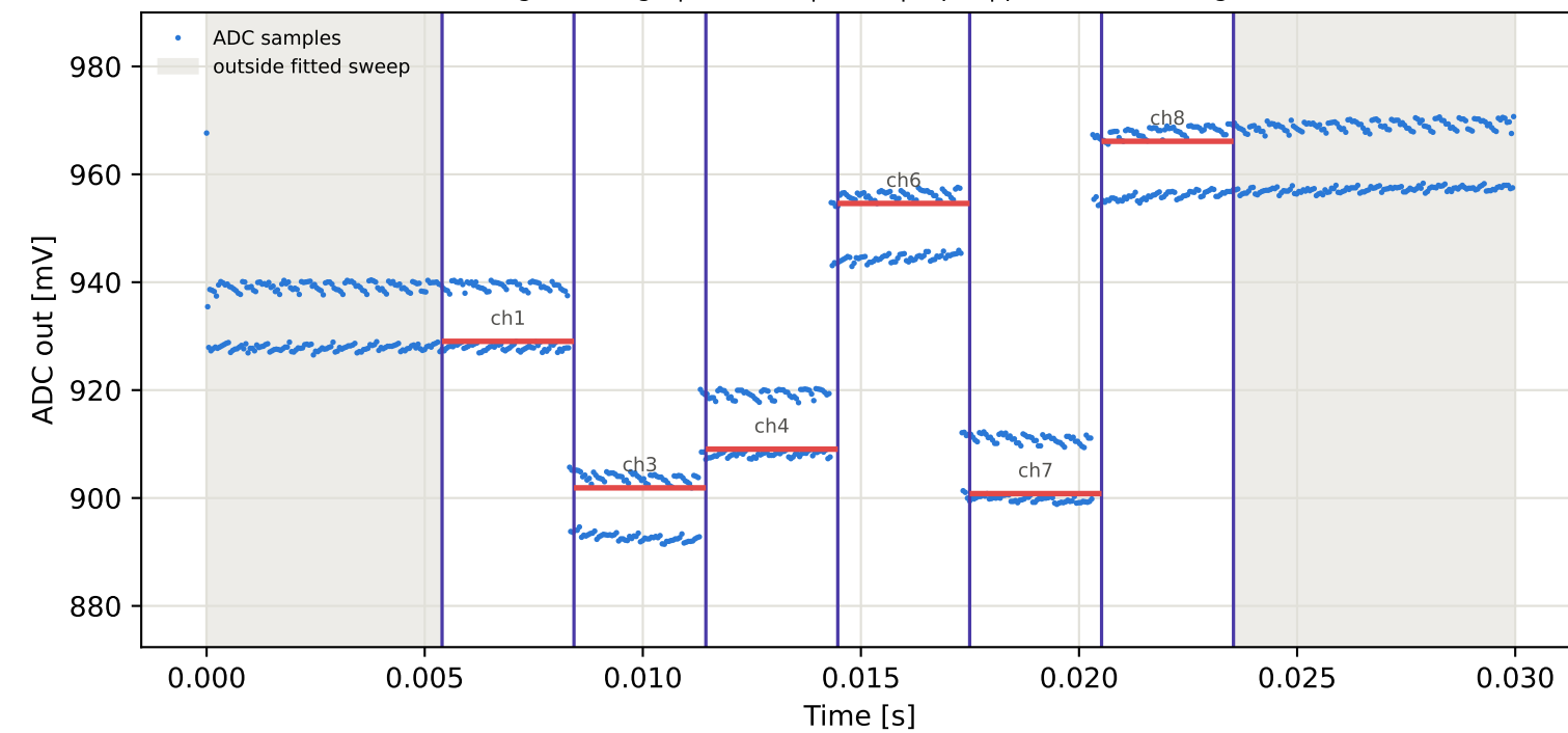
Tag2 &lt;- Tag1 | 865 MHz | run 0 | rep 1 | phase -19.16 deg
