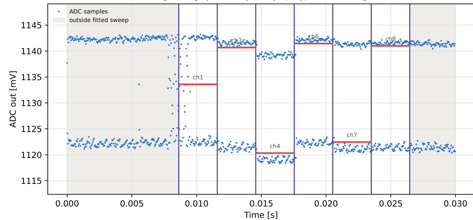
Tag2 &lt;- Tag7 | 945 MHz | run 0 | rep 1 | phase -177.47 deg
