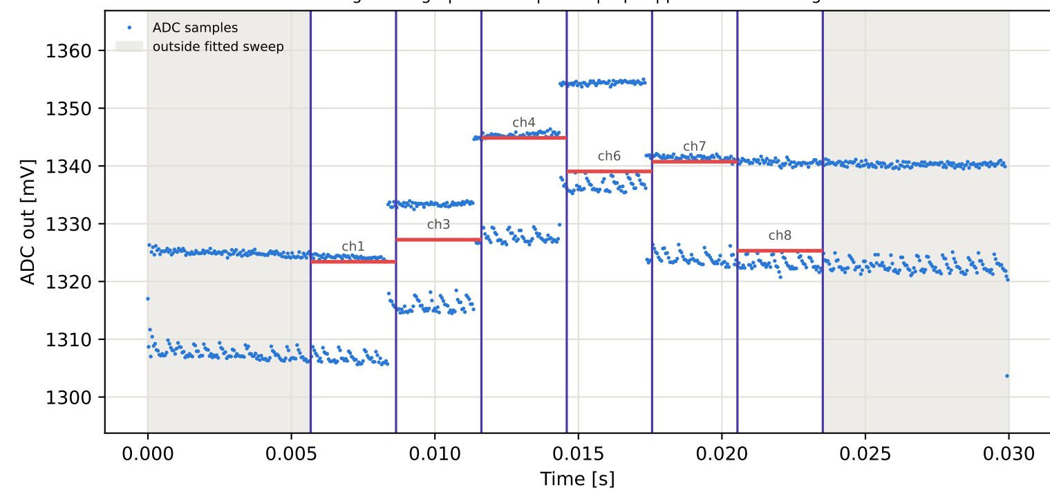
Tag2 &lt;- Tag8 | 875 MHz | run 0 | rep 1 | phase 173.43 deg
