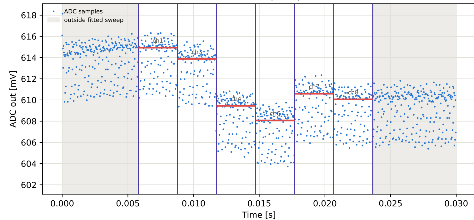
Tag3 &lt;- Tag6 | 845 MHz | run 0 | rep 1 | phase 161.62 deg
