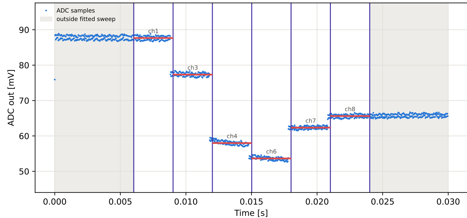
Tag9 &lt;- Tag8 | 855 MHz | run 0 | rep 1 | phase -0.47 deg
