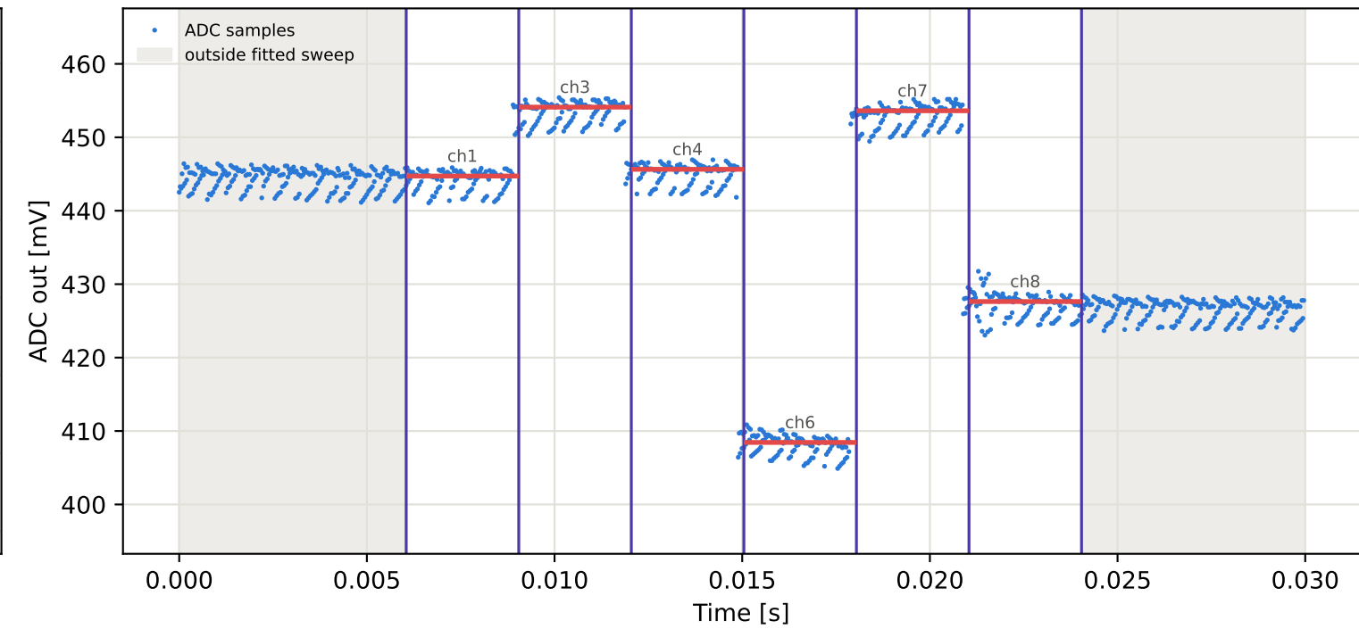
Tag8 &lt;- Tag16 | 975 MHz | run 0 | rep 1 | phase 72.57 deg
