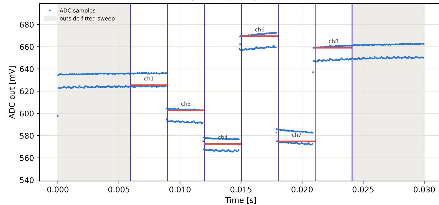
Tag15 &lt;- Tag3 | 995 MHz | run 0 | rep 1 | phase -4.26 deg
