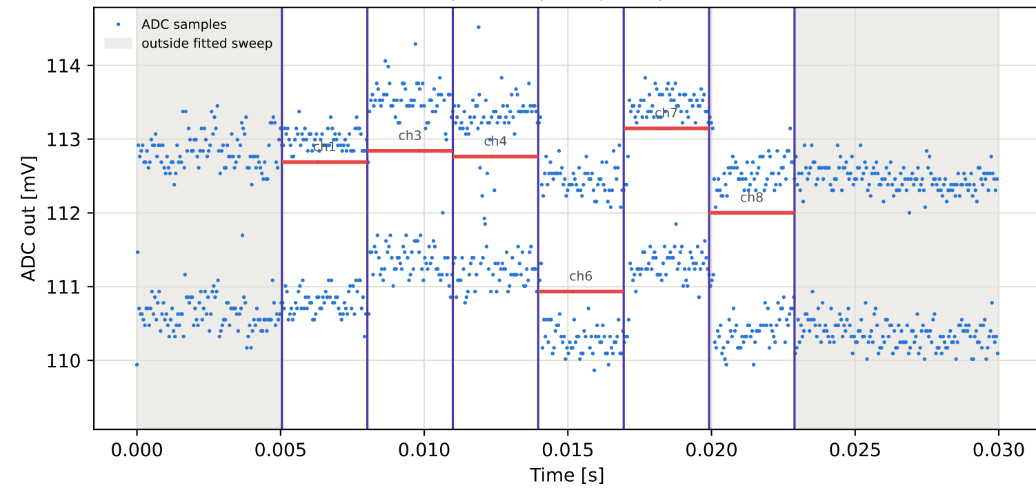
Tag4 &lt;- Tag2 | 785 MHz | run 0 | rep 1 | phase 9.15 deg
