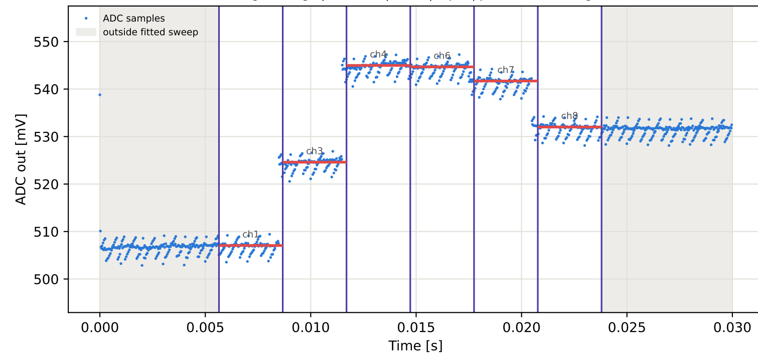
Tag2 &lt;- Tag5 | 845 MHz | run 0 | rep 1 | phase -94.95 deg
