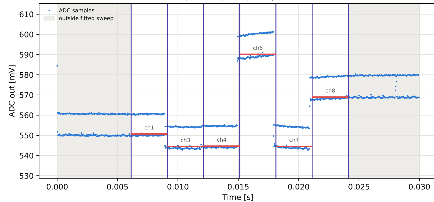
Tag8 &lt;- Tag4 | 945 MHz | run 0 | rep 1 | phase -108.16 deg
