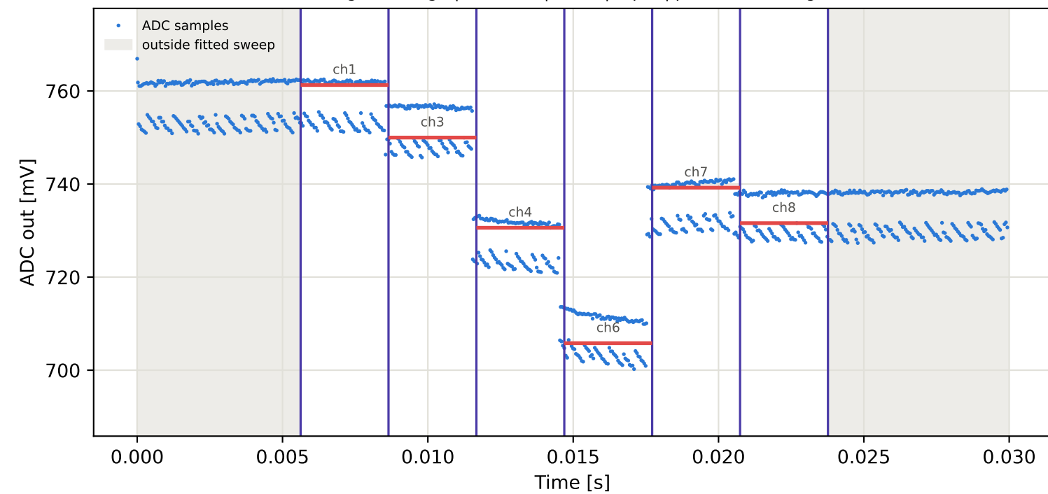
Tag10 &lt;- Tag9 | 895 MHz | run 0 | rep 1 | phase -28.39 deg
