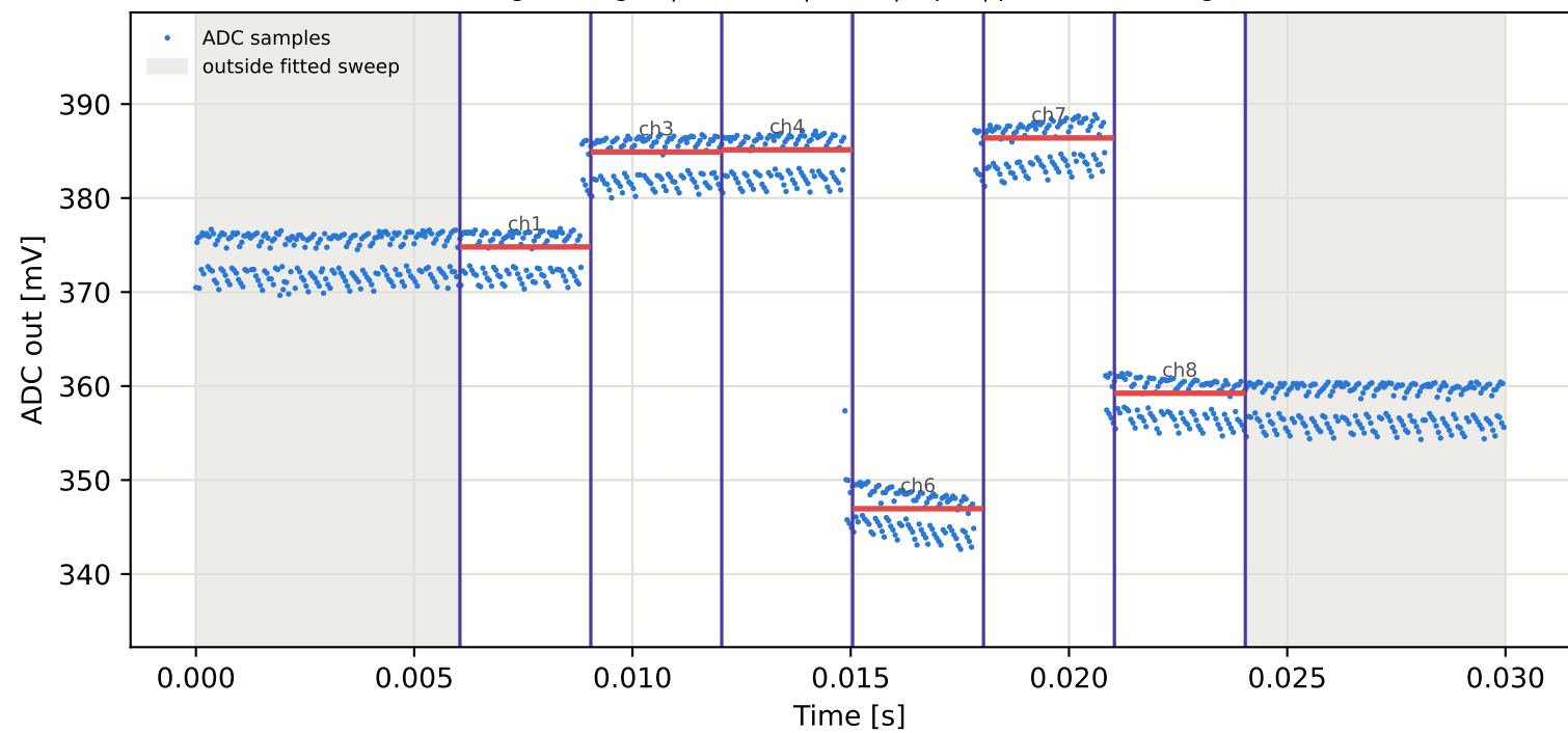
Tag1 &lt;- Tag2 | 955 MHz | run 0 | rep 1 | phase -136.14 deg
