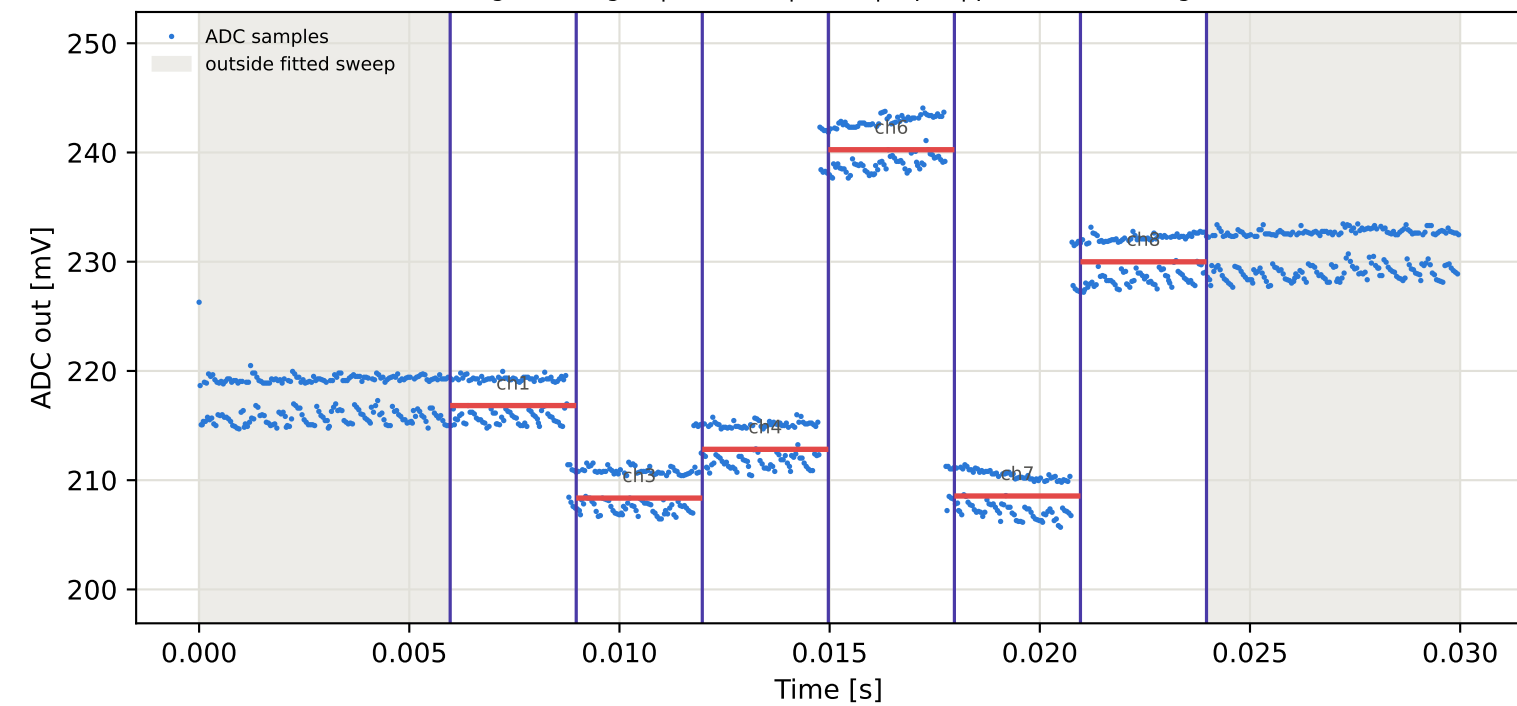
Tag10 &lt;- Tag2 | 995 MHz | run 0 | rep 1 | phase 11.93 deg
