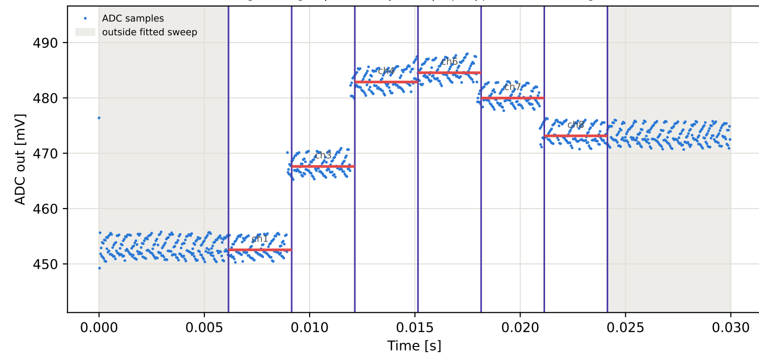
Tag6 &lt;- Tag3 | 865 MHz | run 0 | rep 1 | phase -121.44 deg
