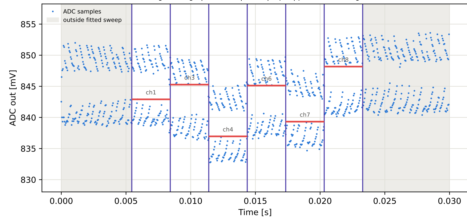
Tag7 &lt;- Tag5 | 935 MHz | run 0 | rep 1 | phase 94.75 deg
