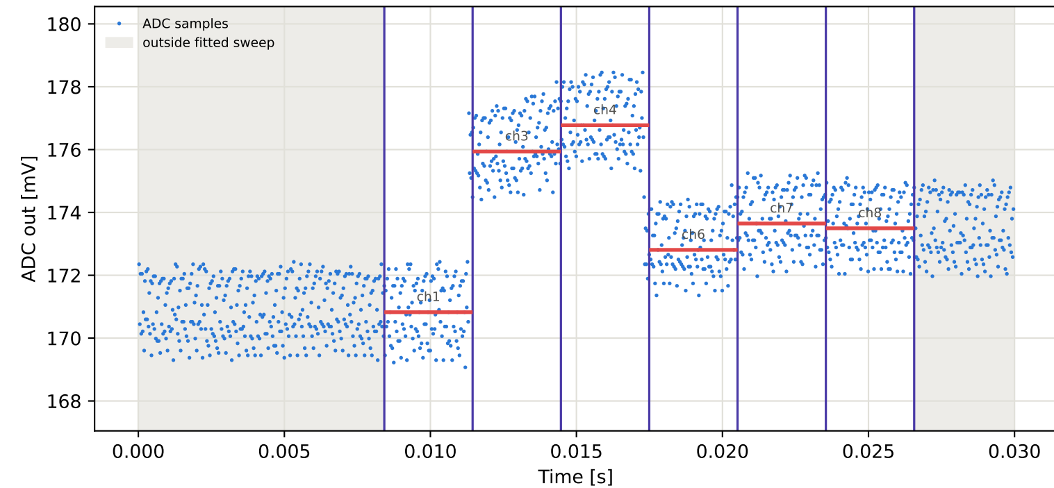
Tag1 &lt;- Tag9 | 995 MHz | run 0 | rep 1 | phase 24.16 deg
