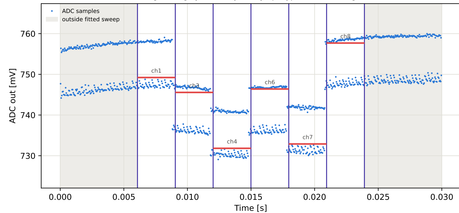
Tag3 &lt;- Tag6 | 875 MHz | run 0 | rep 1 | phase -142.36 deg
