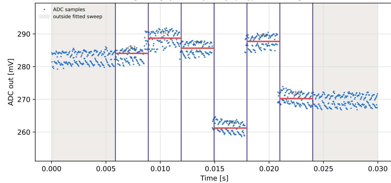
Tag6 &lt;- Tag9 | 925 MHz | run 0 | rep 1 | phase 66.22 deg
