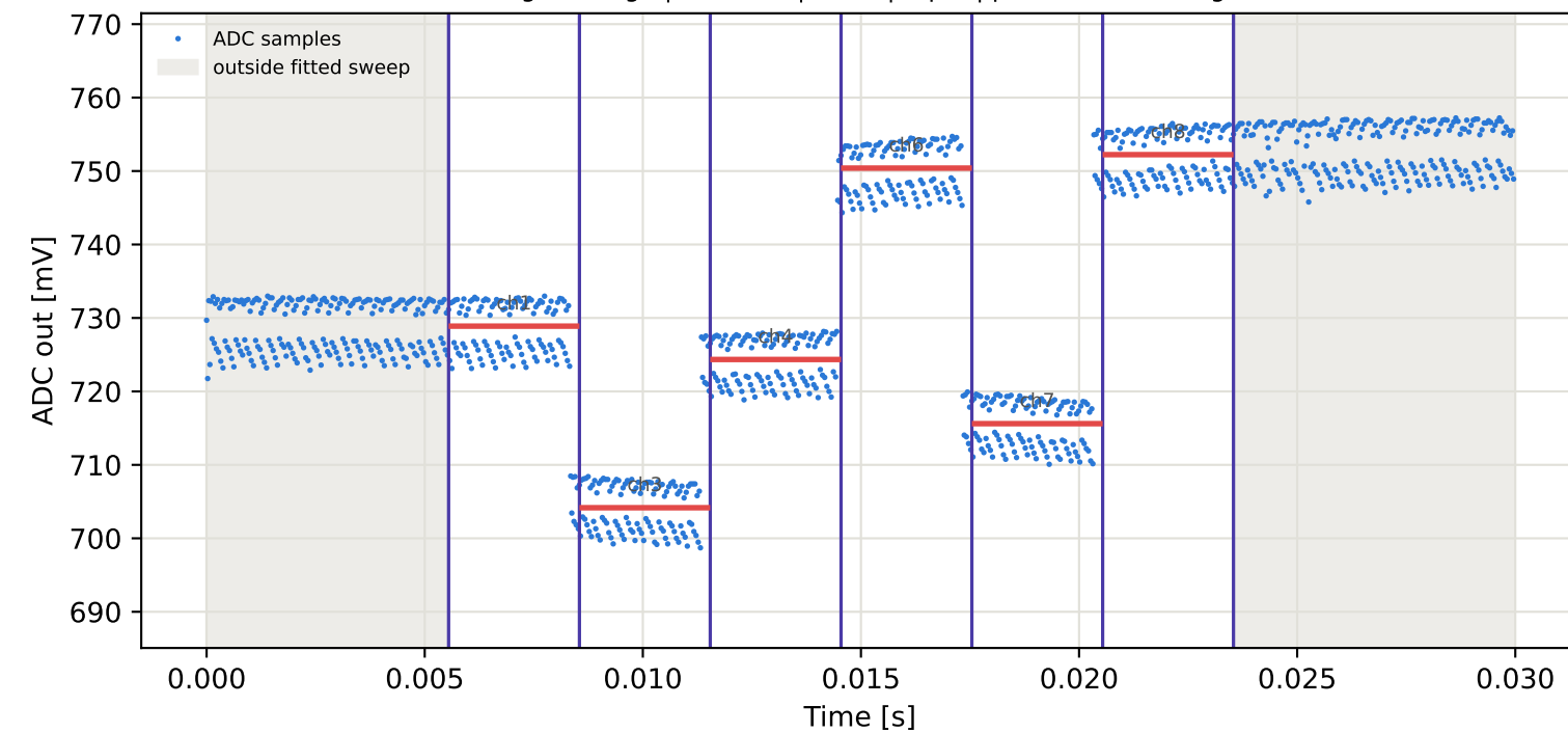
Tag3 &lt;- Tag8 | 855 MHz | run 0 | rep 1 | phase -178.35 deg
