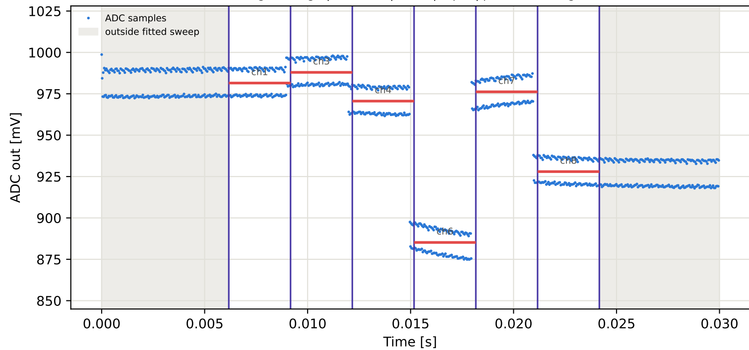
Tag3 &lt;- Tag7 | 905 MHz | run 0 | rep 1 | phase -41.00 deg
