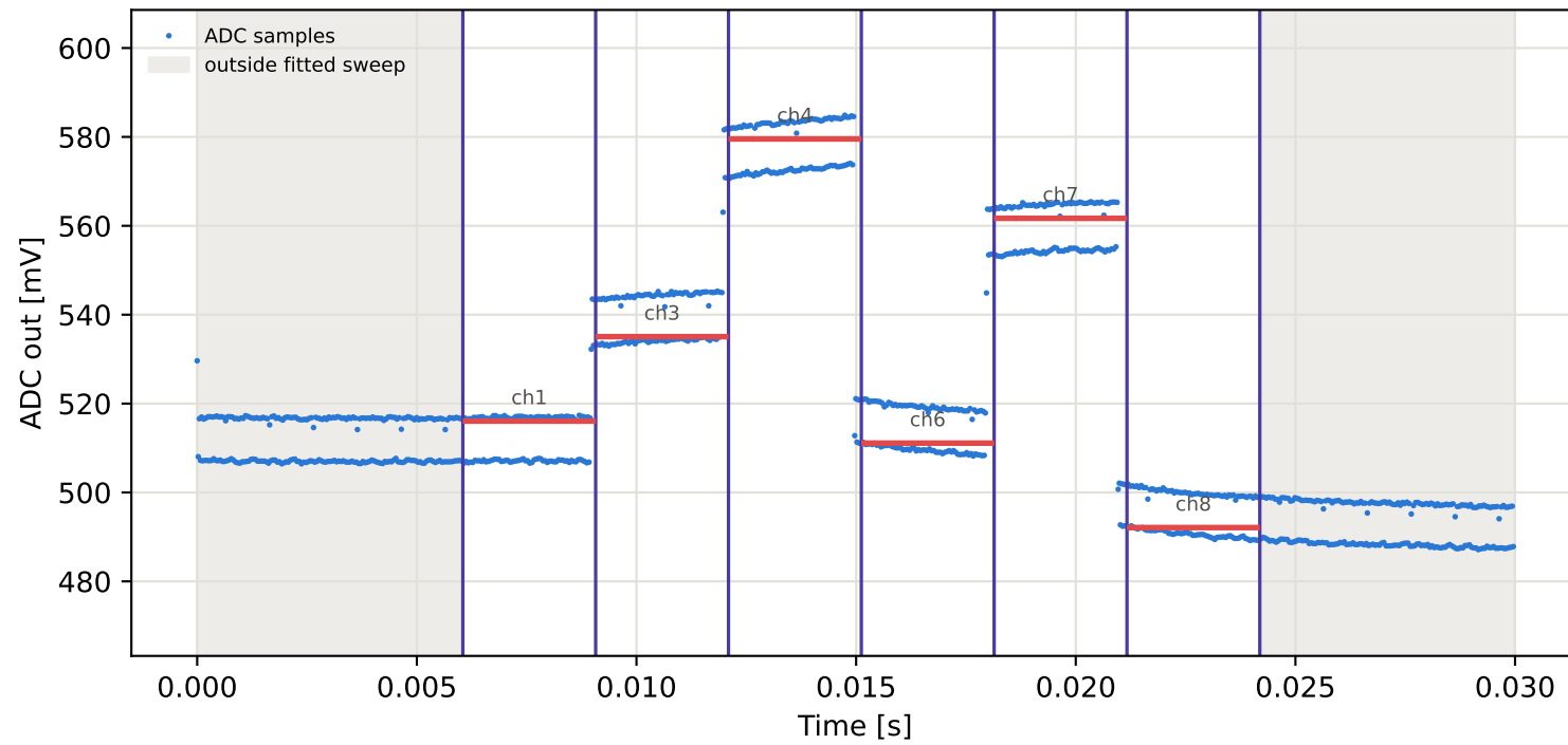
Tag15 &lt;- Tag1 | 945 MHz | run 0 | rep 1 | phase -67.15 deg
