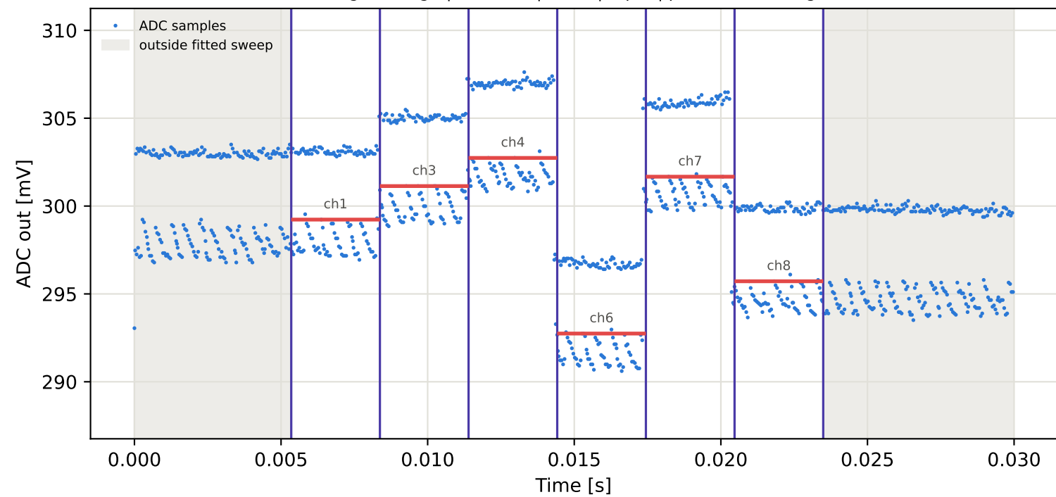
Tag8 &lt;- Tag4 | 985 MHz | run 0 | rep 1 | phase 29.01 deg
