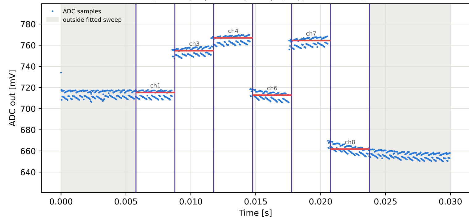
Tag10 &lt;- Tag3 | 895 MHz | run 0 | rep 1 | phase 16.45 deg
