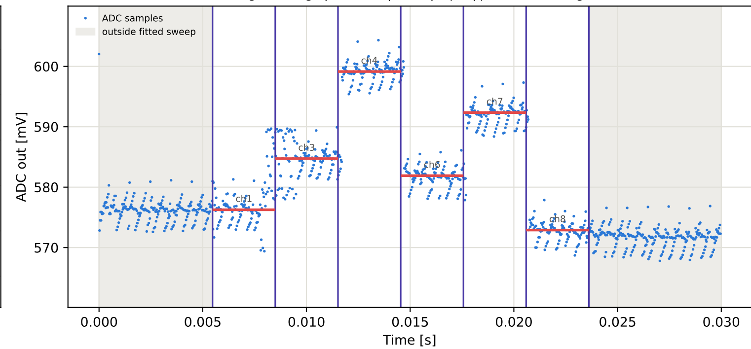
Tag16 &lt;- Tag7 | 945 MHz | run 0 | rep 1 | phase -143.02 deg
