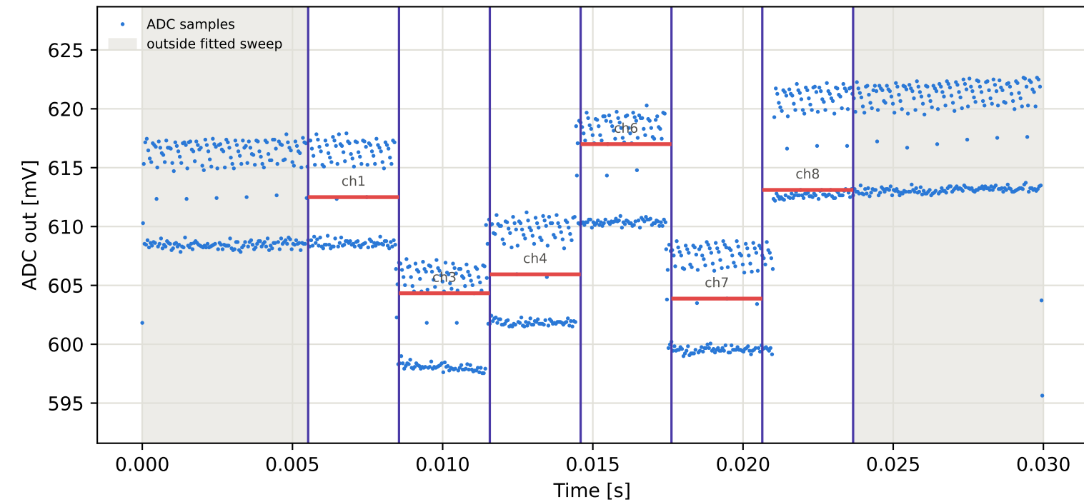
Tag3 &lt;- Tag8 | 845 MHz | run 0 | rep 1 | phase 151.97 deg
