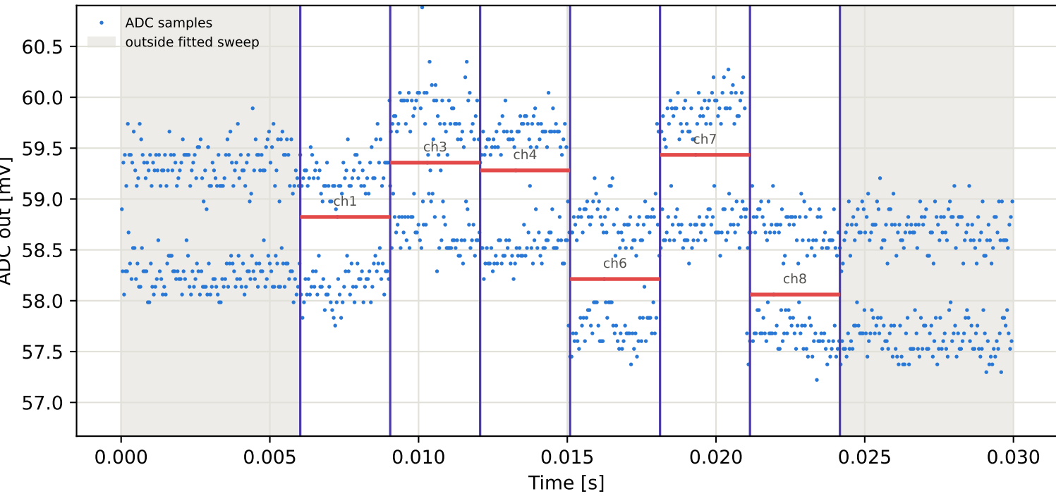
Tag4 &lt;- Tag2 | 795 MHz | run 0 | rep 1 | phase -17.36 deg
