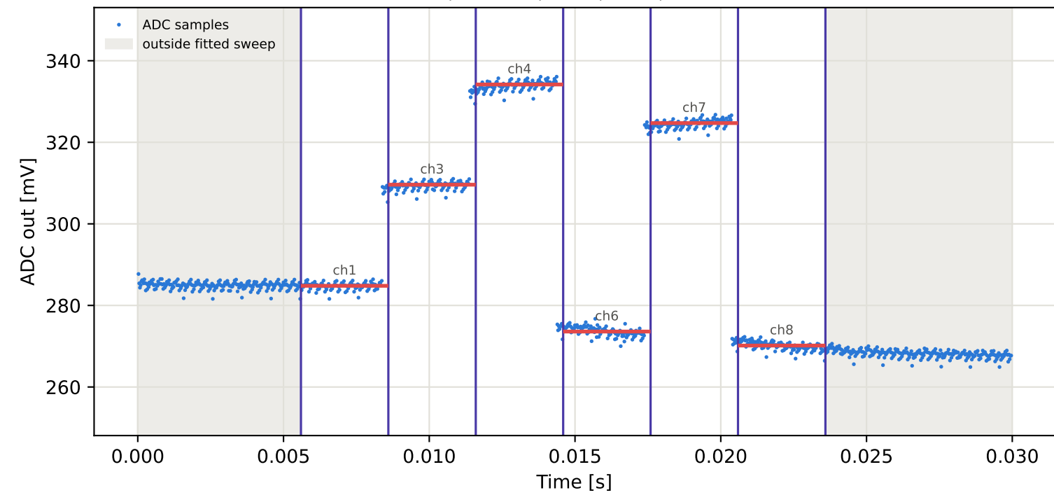
Tag3 &lt;- Tag9 | 975 MHz | run 0 | rep 1 | phase -63.09 deg
