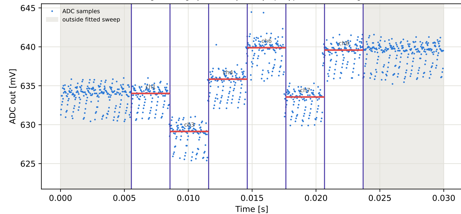
Tag16 &lt;- Tag6 | 835 MHz | run 0 | rep 1 | phase 11.47 deg
