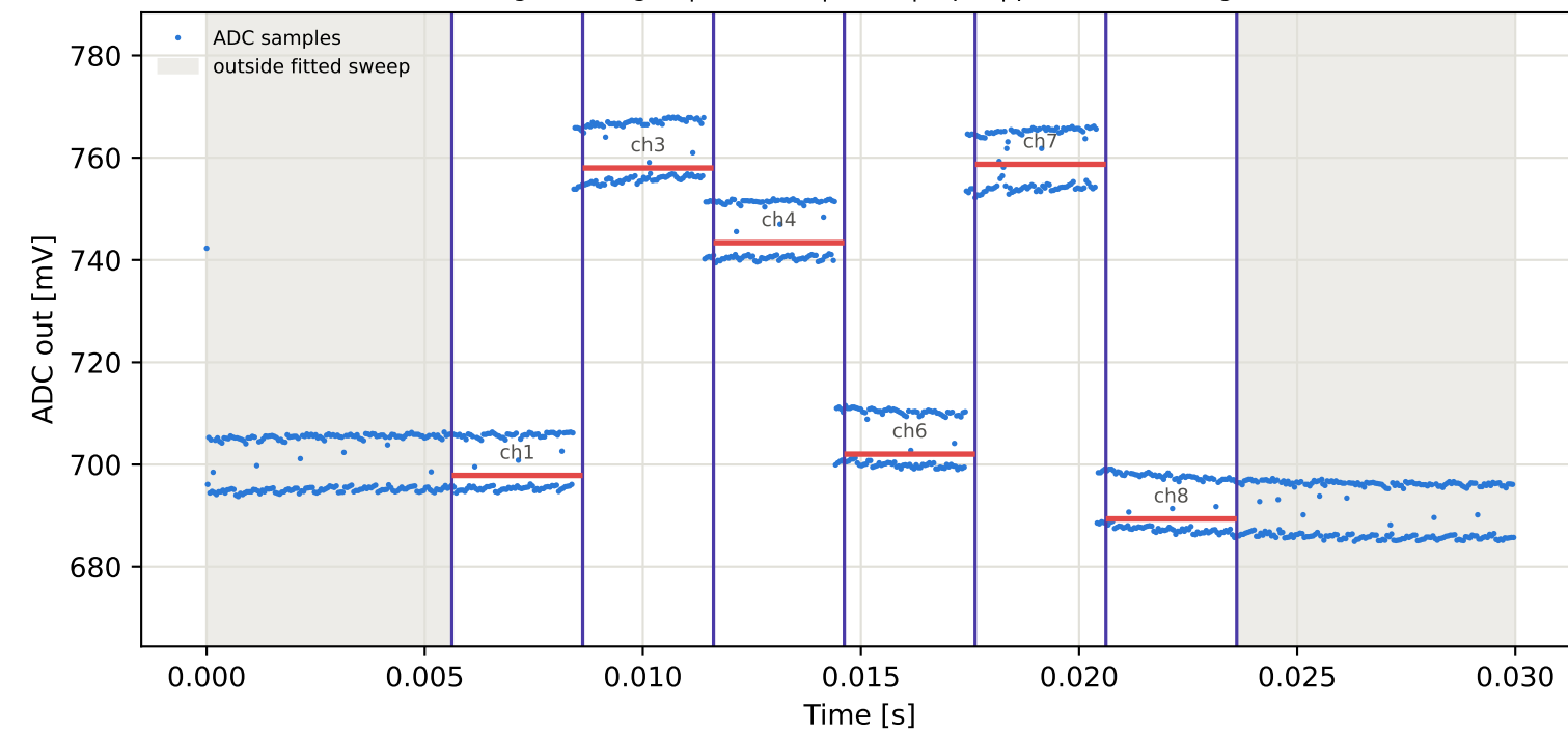
Tag15 &lt;- Tag3 | 835 MHz | run 0 | rep 1 | phase 31.19 deg
