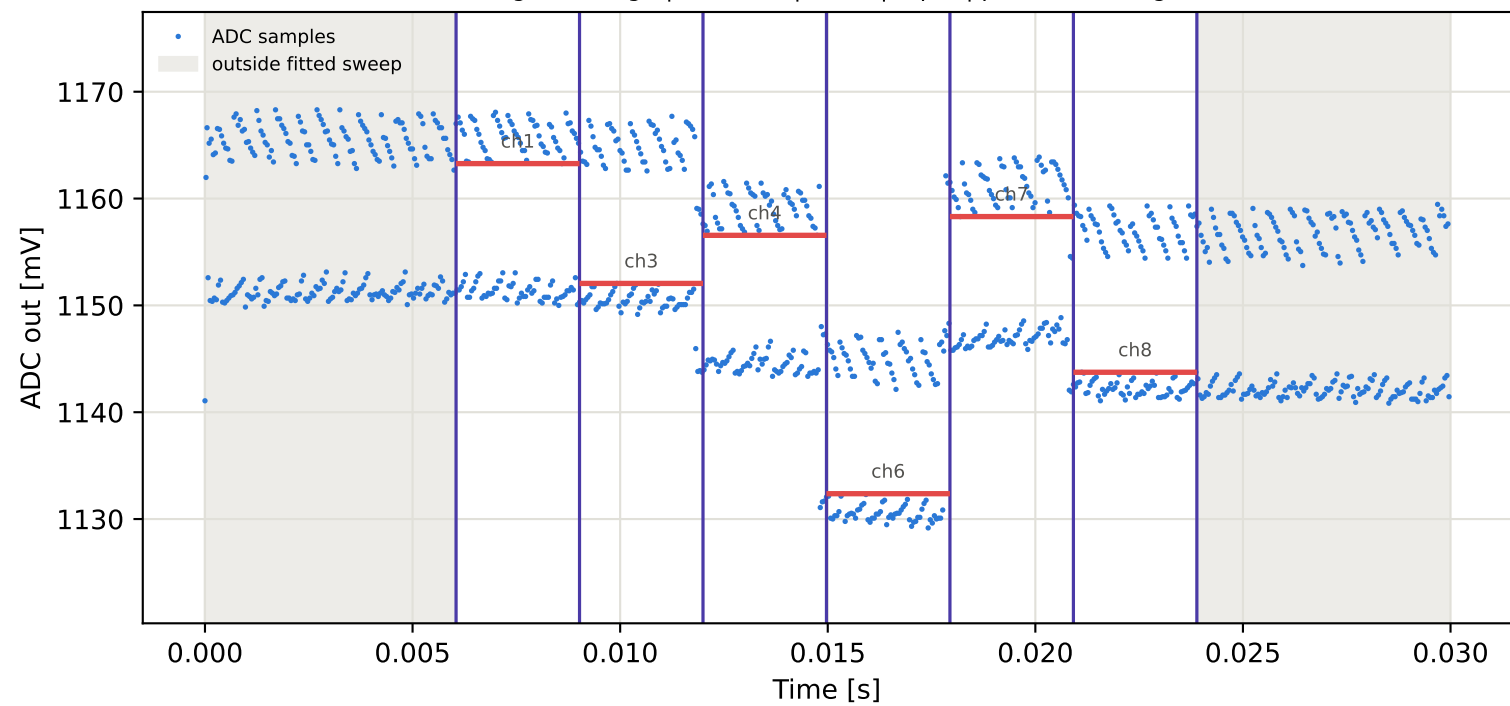
Tag2 &lt;- Tag10 | 915 MHz | run 0 | rep 1 | phase 139.59 deg
