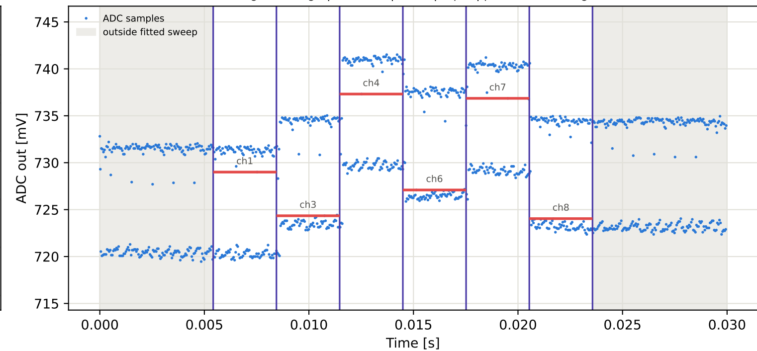
Tag16 &lt;- Tag7 | 825 MHz | run 0 | rep 1 | phase 42.40 deg
