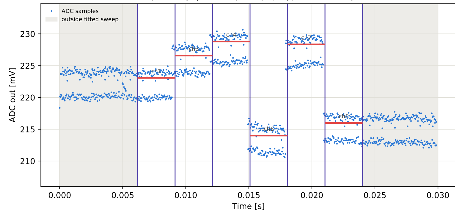
Tag10 &lt;- Tag4 | 845 MHz | run 0 | rep 1 | phase -67.00 deg
