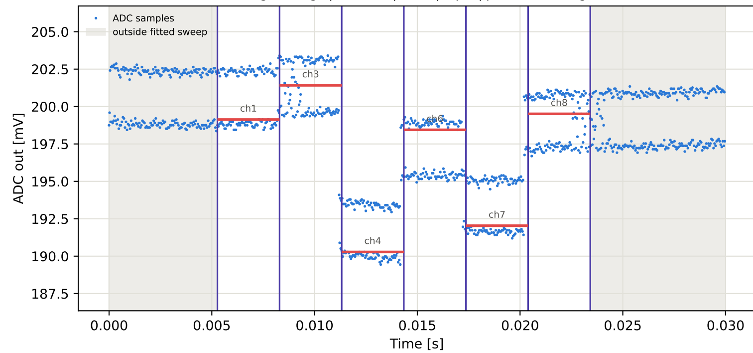
Tag8 &lt;- Tag5 | 775 MHz | run 0 | rep 1 | phase 122.52 deg
