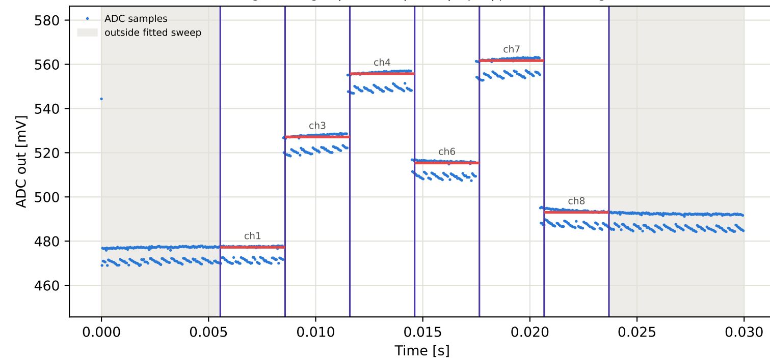
Tag15 &lt;- Tag3 | 825 MHz | run 0 | rep 1 | phase 15.88 deg
