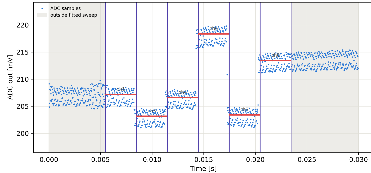
Tag1 &lt;- Tag9 | 985 MHz | run 0 | rep 1 | phase -10.49 deg
