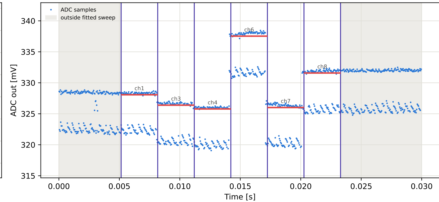
Tag5 &lt;- Tag4 | 975 MHz | run 0 | rep 1 | phase -23.09 deg
