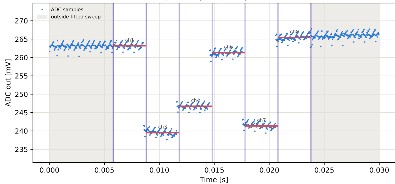
Tag9 &lt;- Tag6 | 825 MHz | run 0 | rep 1 | phase -5.29 deg
