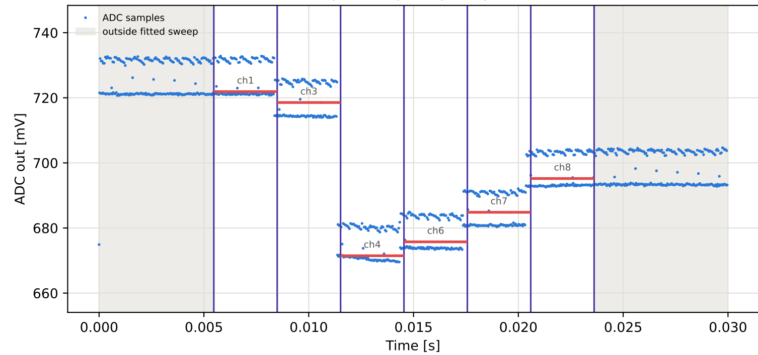
Tag16 &lt;- Tag15 | 845 MHz | run 0 | rep 1 | phase 59.49 deg
