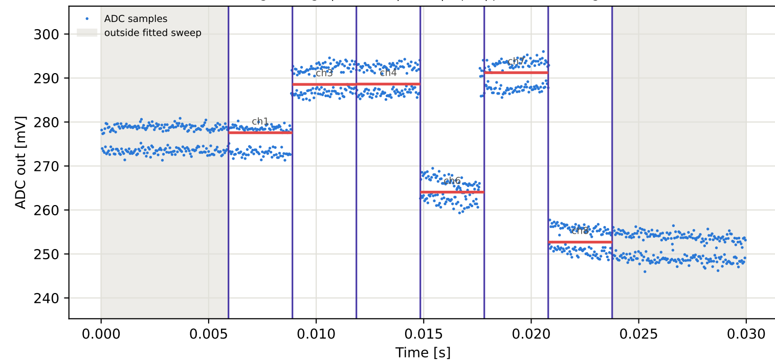
Tag9 &lt;- Tag6 | 885 MHz | run 0 | rep 1 | phase -140.43 deg
