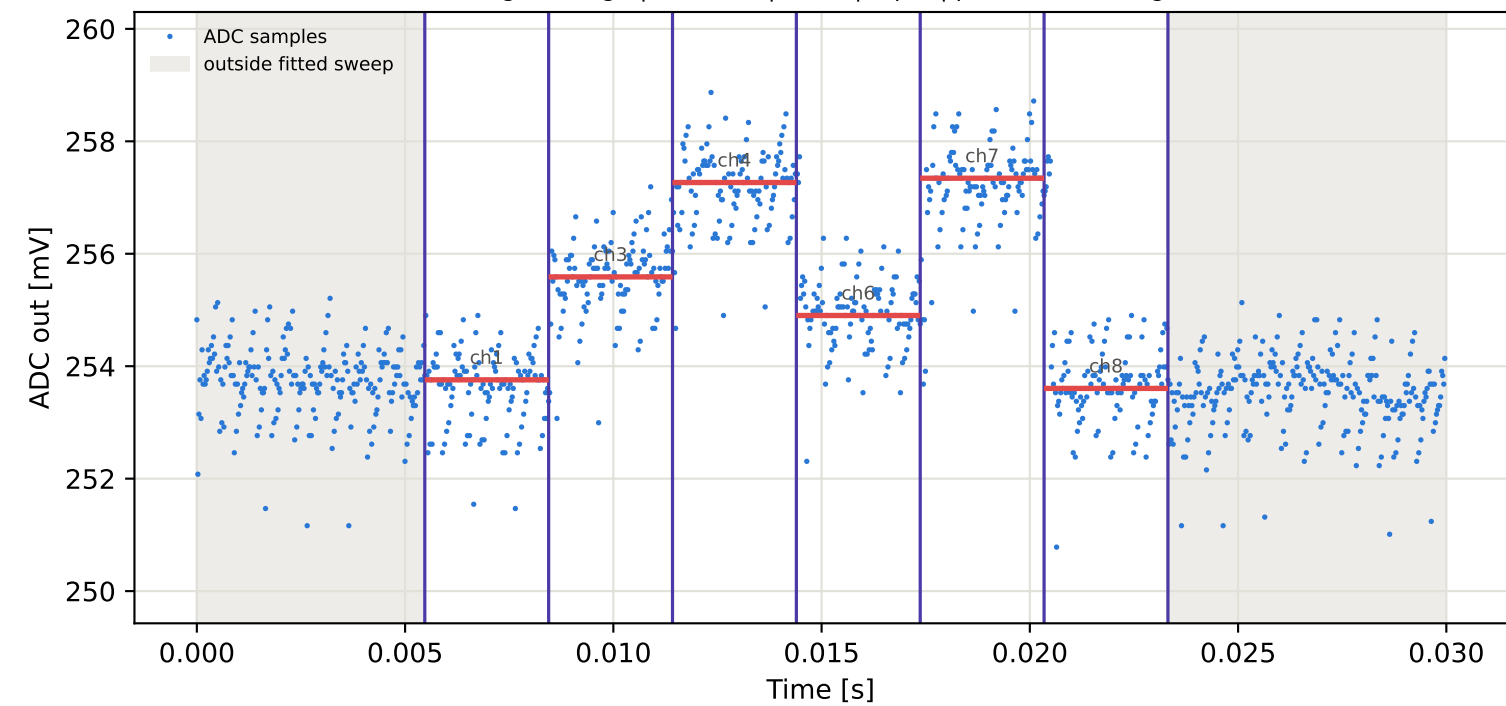
Tag9 &lt;- Tag15 | 835 MHz | run 0 | rep 1 | phase -127.51 deg
