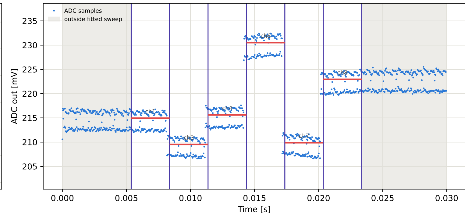
Tag10 &lt;- Tag1 | 995 MHz | run 0 | rep 1 | phase 176.96 deg
