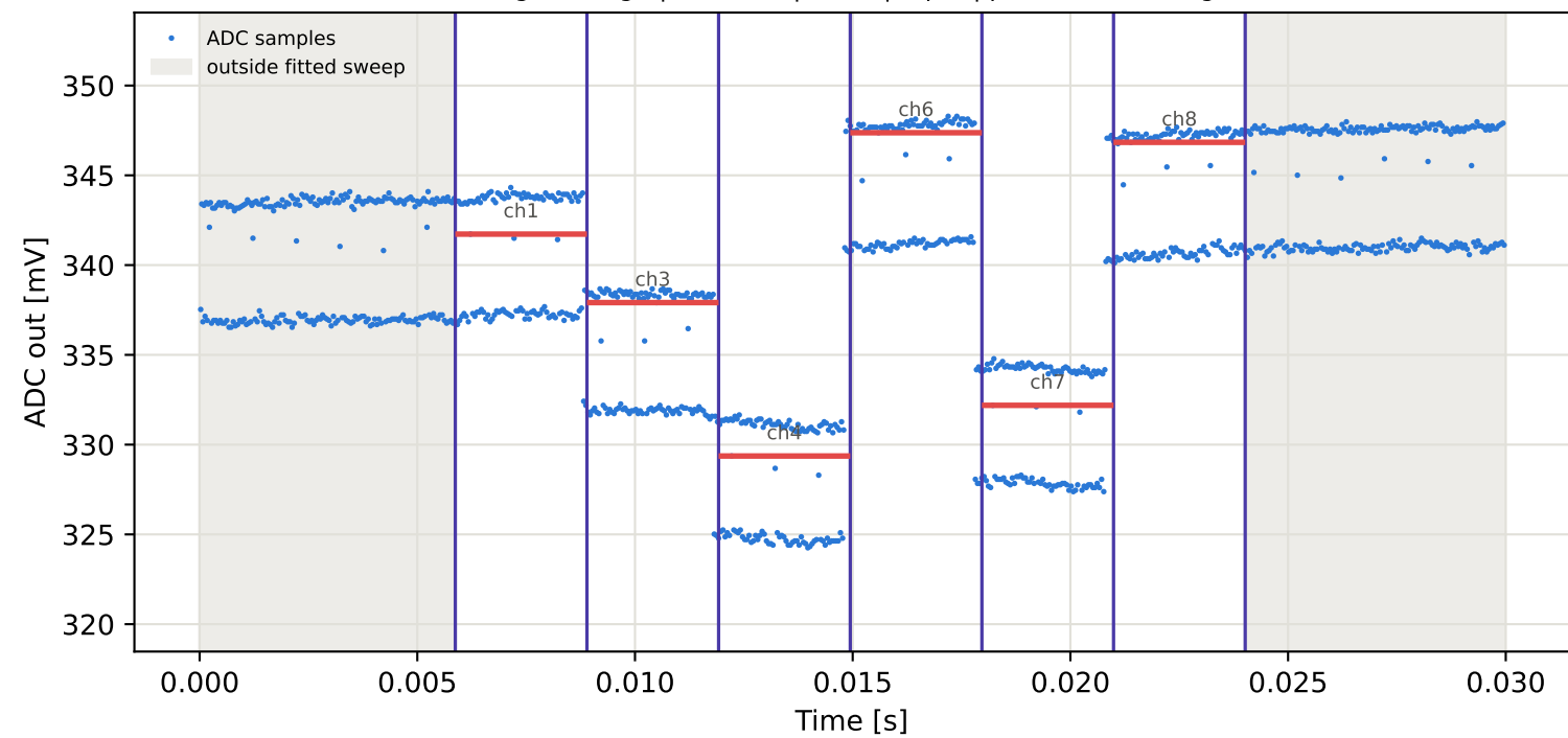
Tag5 &lt;- Tag8 | 985 MHz | run 0 | rep 1 | phase -124.81 deg
