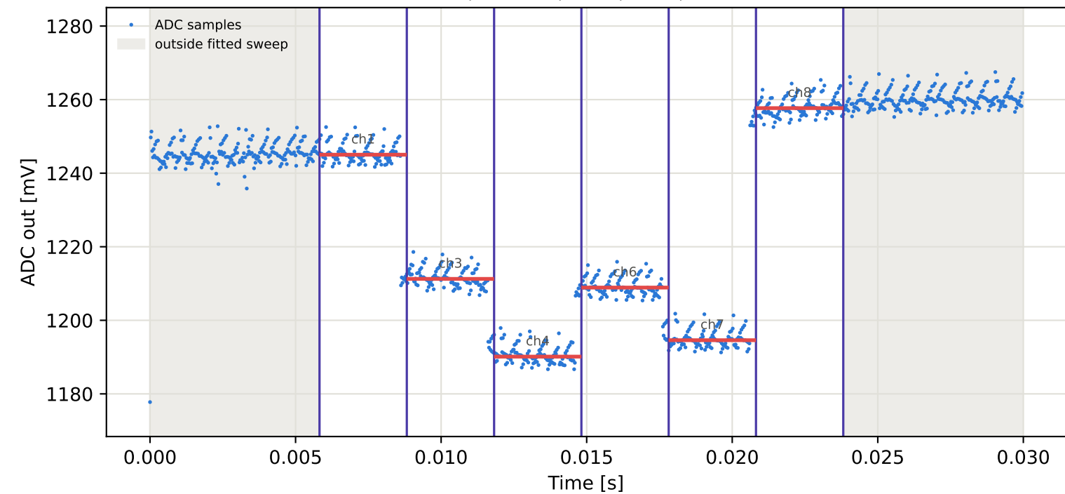
Tag8 &lt;- Tag16 | 895 MHz | run 0 | rep 1 | phase 88.68 deg
