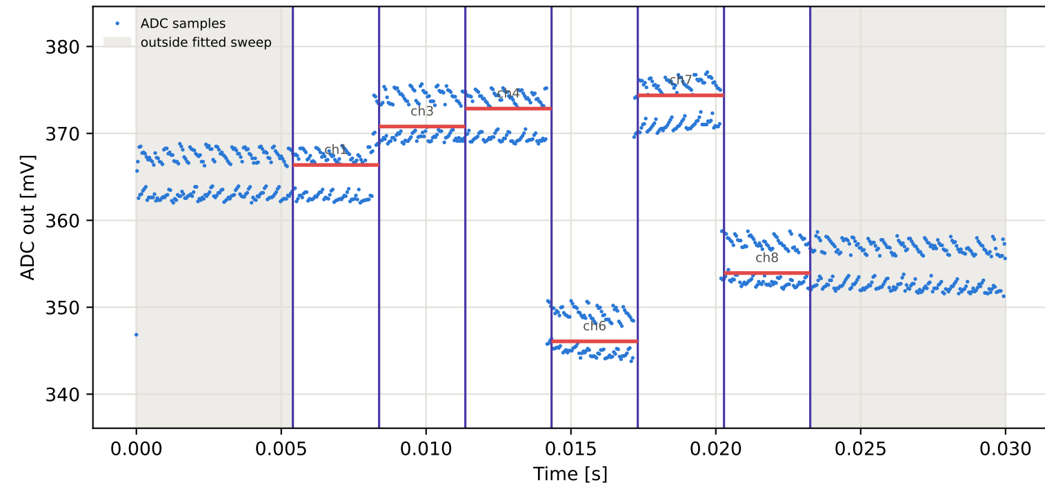
Tag4 &lt;- Tag3 | 965 MHz | run 0 | rep 1 | phase 28.87 deg
