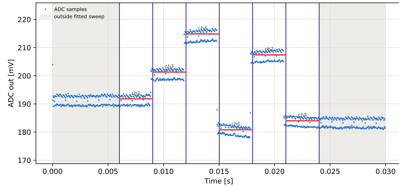
Tag1 &lt;- Tag3 | 985 MHz | run 0 | rep 1 | phase -59.44 deg
