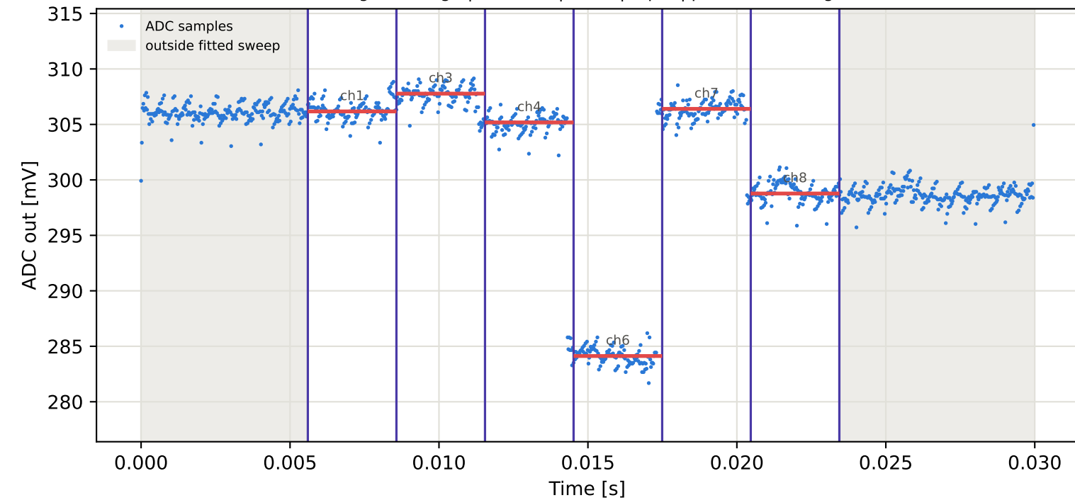
Tag10 &lt;- Tag4 | 855 MHz | run 0 | rep 1 | phase -124.84 deg
