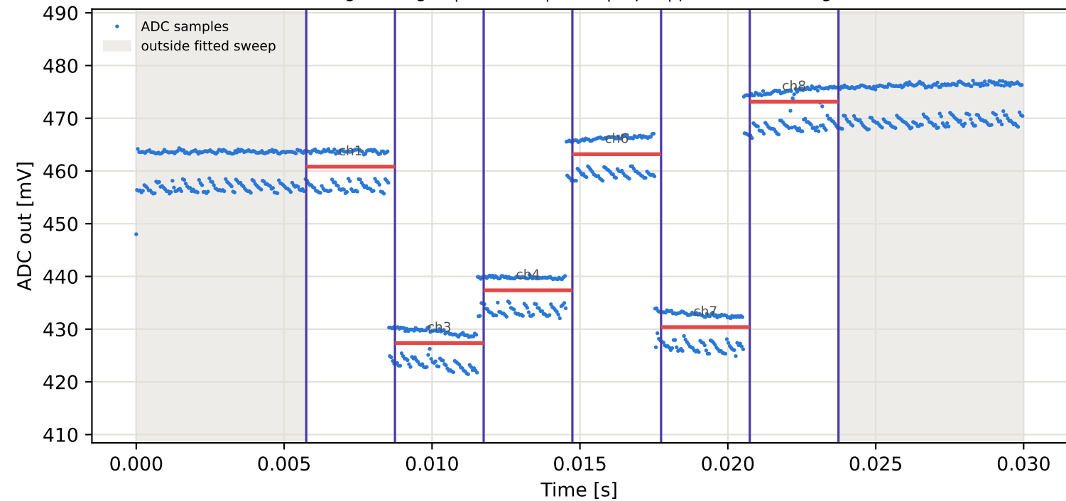
Tag6 &lt;- Tag10 | 835 MHz | run 0 | rep 1 | phase 152.14 deg
