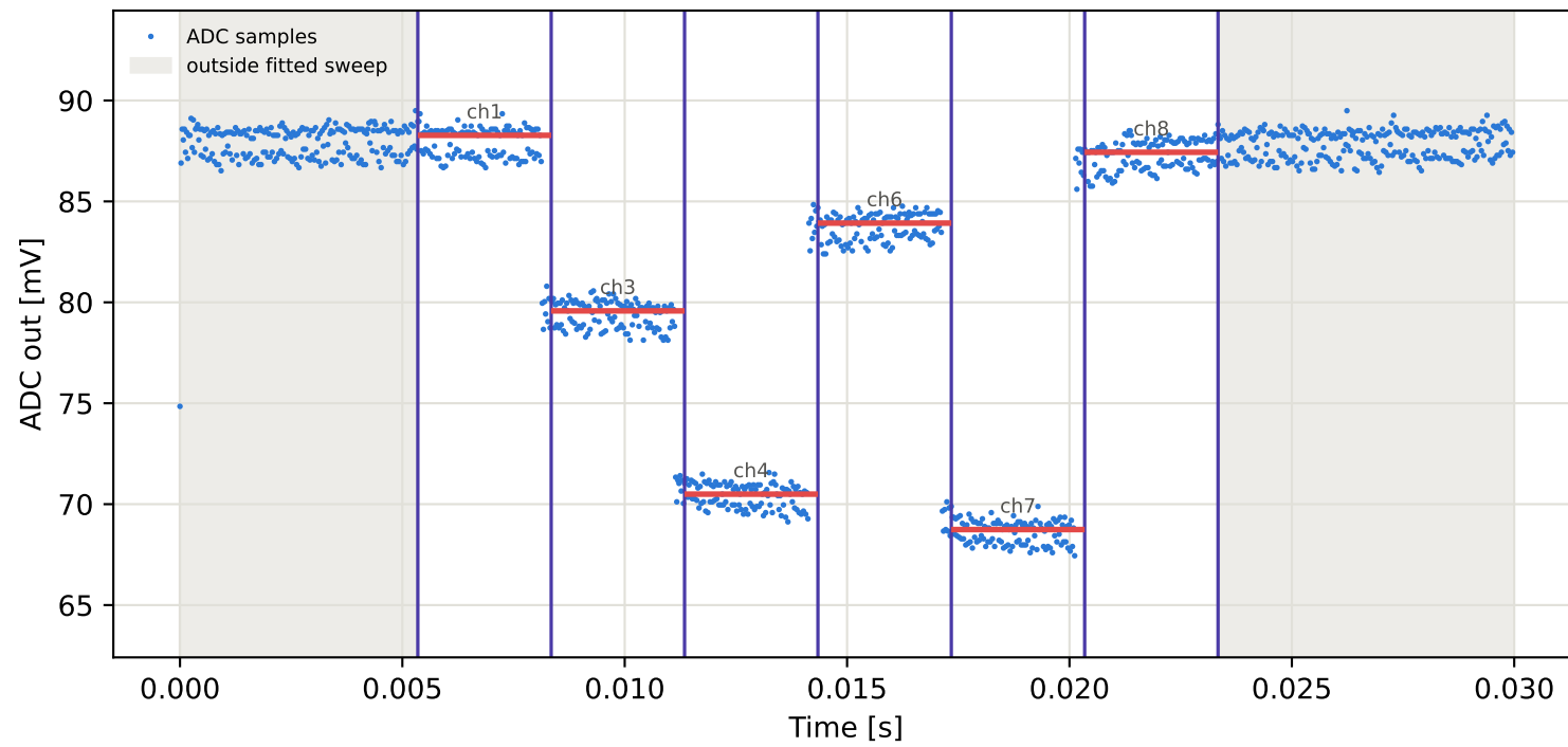
Tag10 &lt;- Tag8 | 775 MHz | run 0 | rep 1 | phase 129.87 deg
