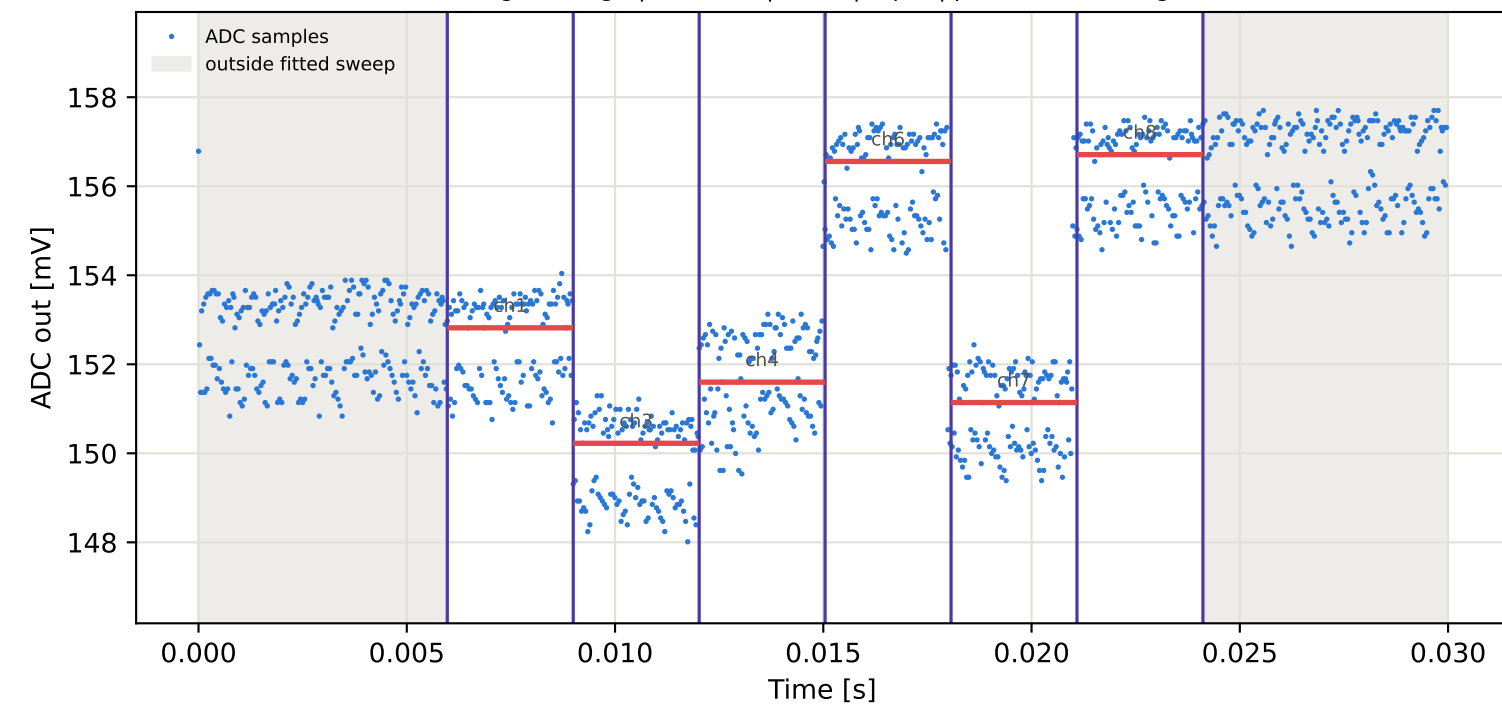
Tag8 &lt;- Tag4 | 795 MHz | run 0 | rep 1 | phase -113.97 deg
