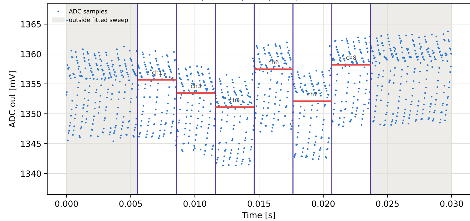
Tag2 &lt;- Tag6 | 935 MHz | run 0 | rep 1 | phase -122.74 deg
