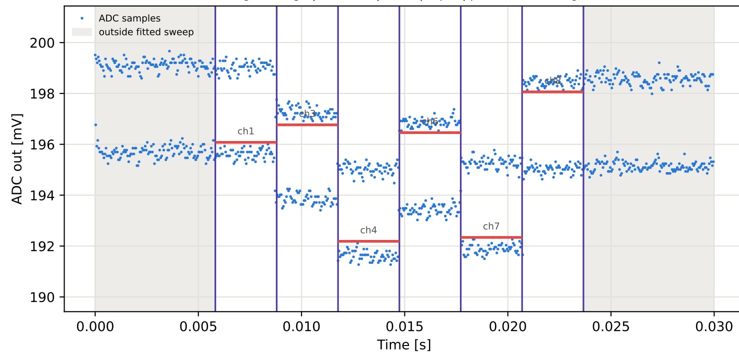
Tag8 &lt;- Tag4 | 775 MHz | run 0 | rep 1 | phase 134.45 deg
