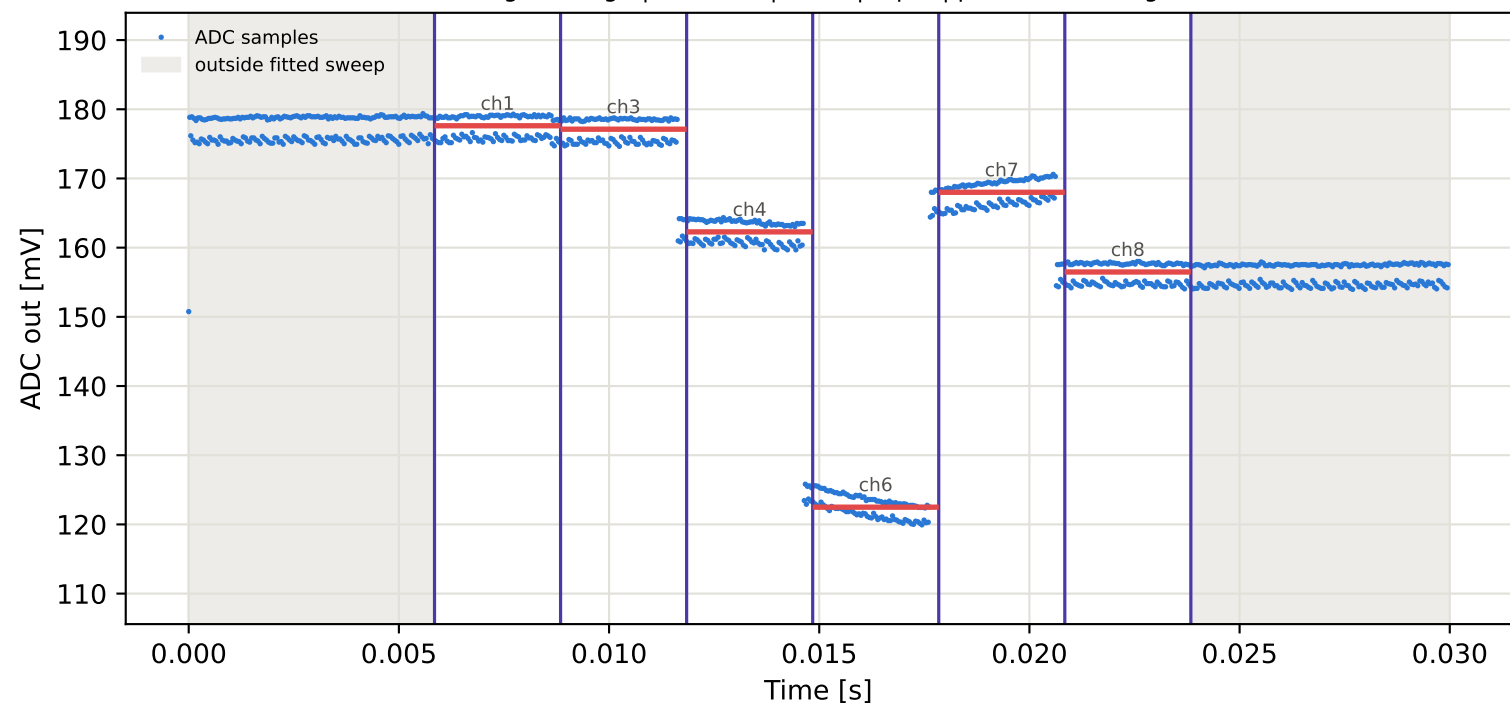
Tag1 &lt;- Tag4 | 915 MHz | run 0 | rep 1 | phase 20.35 deg
