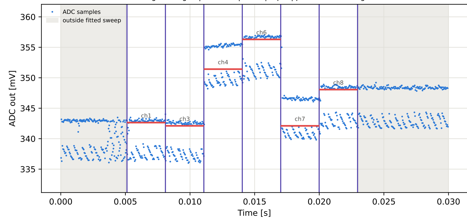
Tag4 &lt;- Tag16 | 985 MHz | run 0 | rep 1 | phase -5.19 deg
