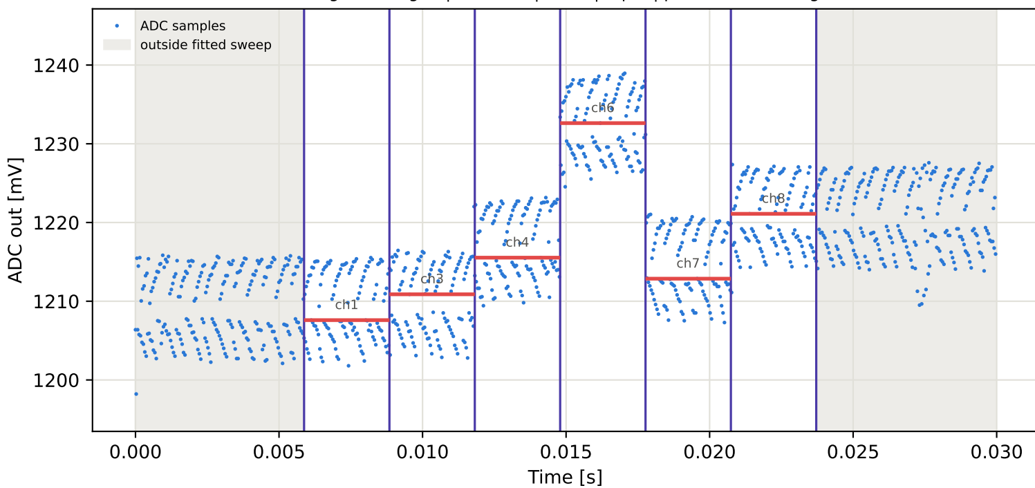
Tag15 &lt;- Tag10 | 895 MHz | run 0 | rep 1 | phase -158.78 deg
