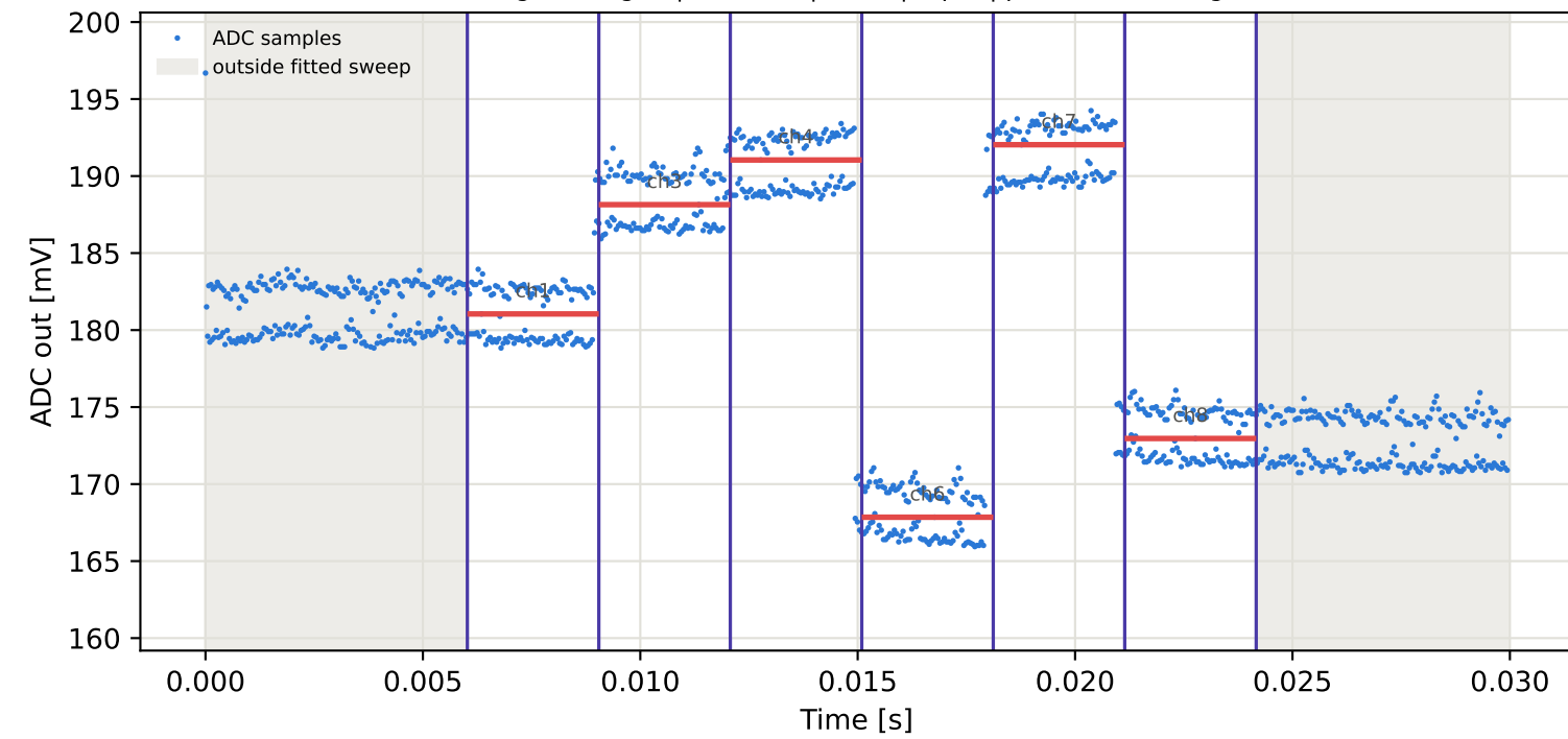
Tag6 &lt;- Tag3 | 985 MHz | run 0 | rep 1 | phase -32.36 deg
