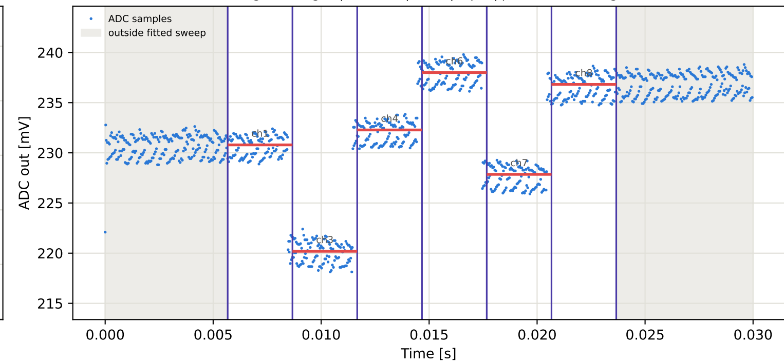
Tag10 &lt;- Tag3 | 825 MHz | run 0 | rep 1 | phase -116.63 deg
