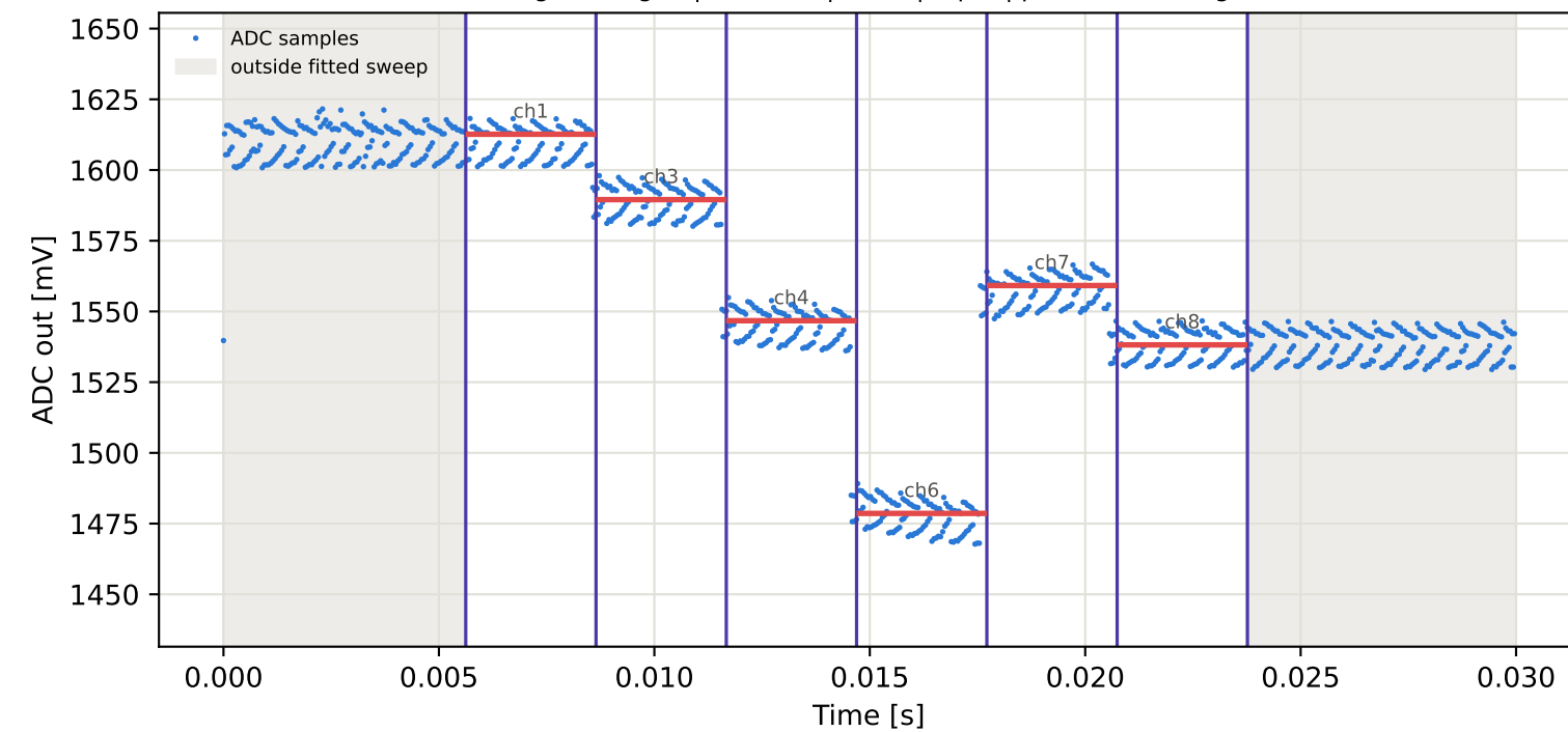
Tag5 &lt;- Tag3 | 895 MHz | run 0 | rep 1 | phase 157.84 deg
