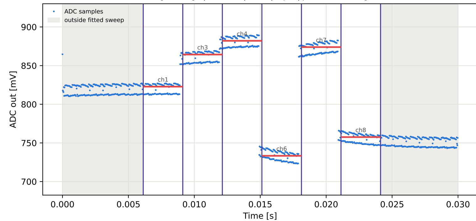
Tag4 &lt;- Tag7 | 925 MHz | run 0 | rep 1 | phase 110.44 deg
