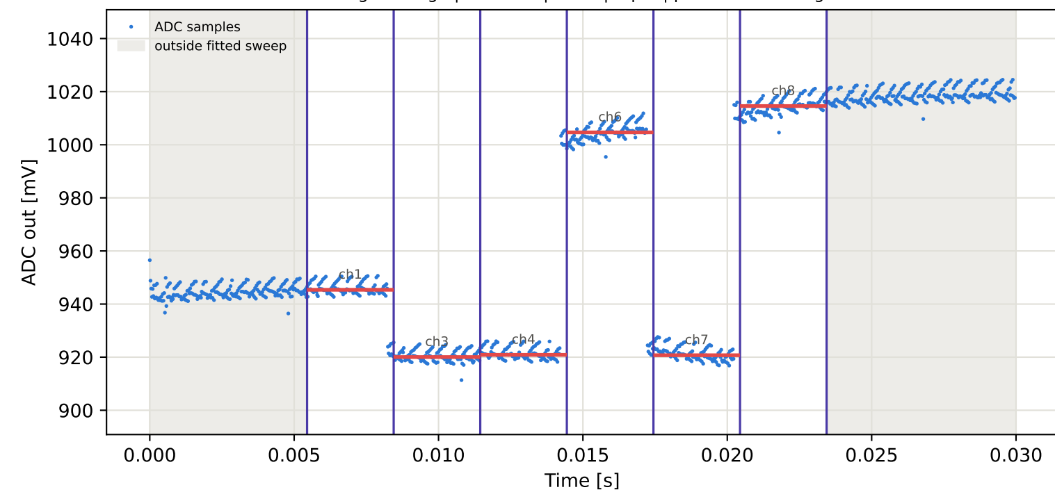
Tag8 &lt;- Tag1 | 905 MHz | run 0 | rep 1 | phase 12.43 deg
