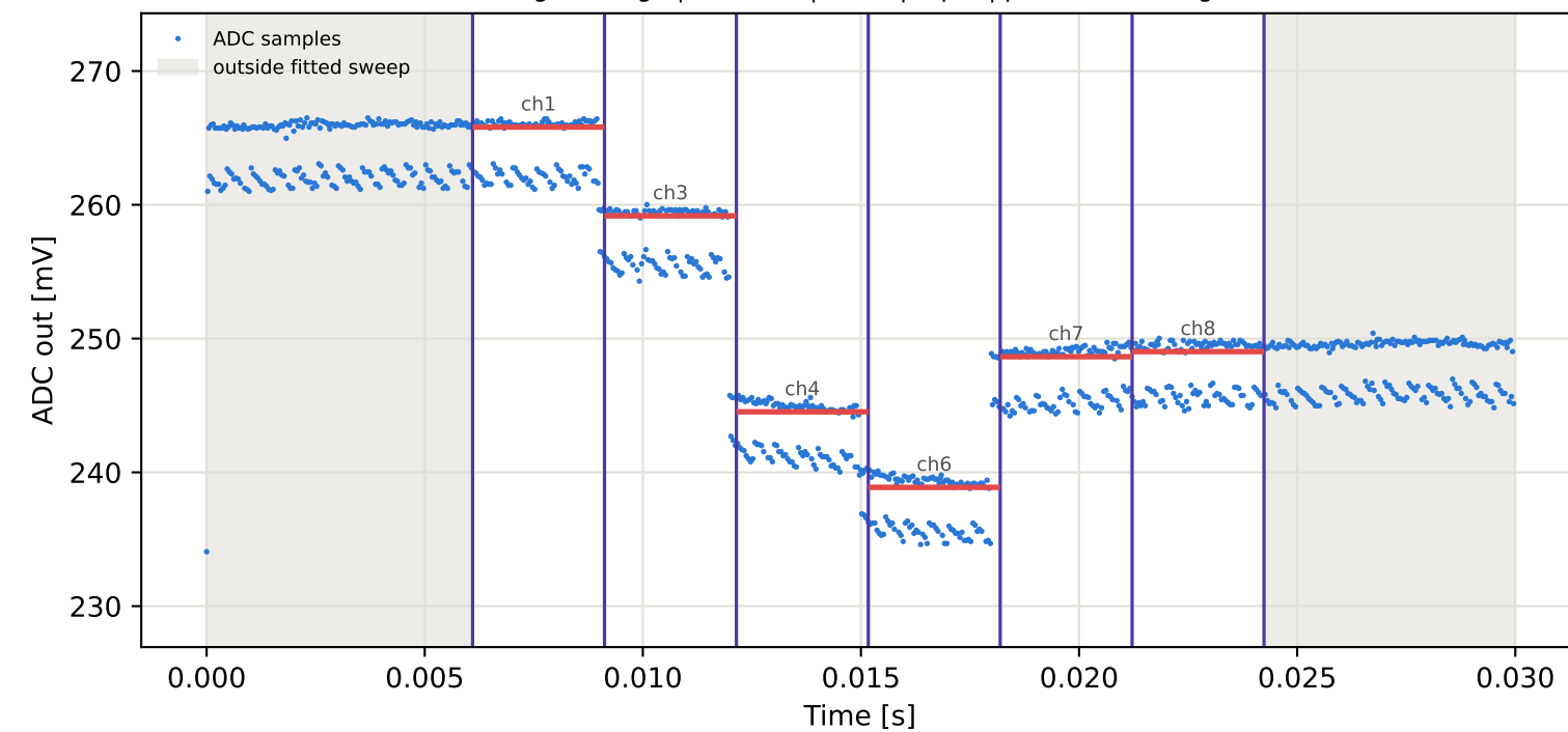
Tag4 &lt;- Tag9 | 875 MHz | run 0 | rep 1 | phase 47.54 deg
