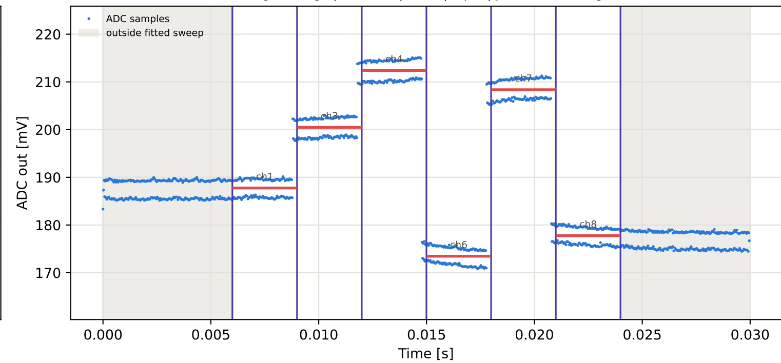
Tag1 &lt;- Tag8 | 985 MHz | run 0 | rep 1 | phase 73.21 deg
