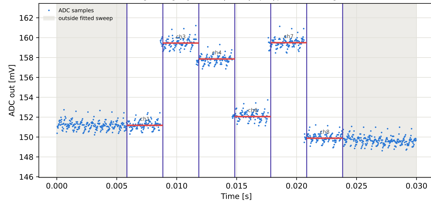
Tag5 &lt;- Tag16 | 825 MHz | run 0 | rep 1 | phase -63.14 deg
