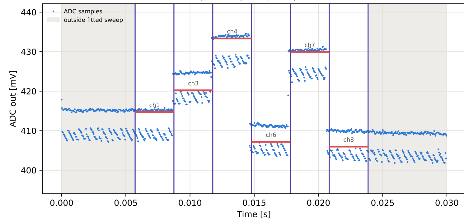
Tag2 &lt;- Tag10 | 995 MHz | run 0 | rep 1 | phase 91.39 deg
