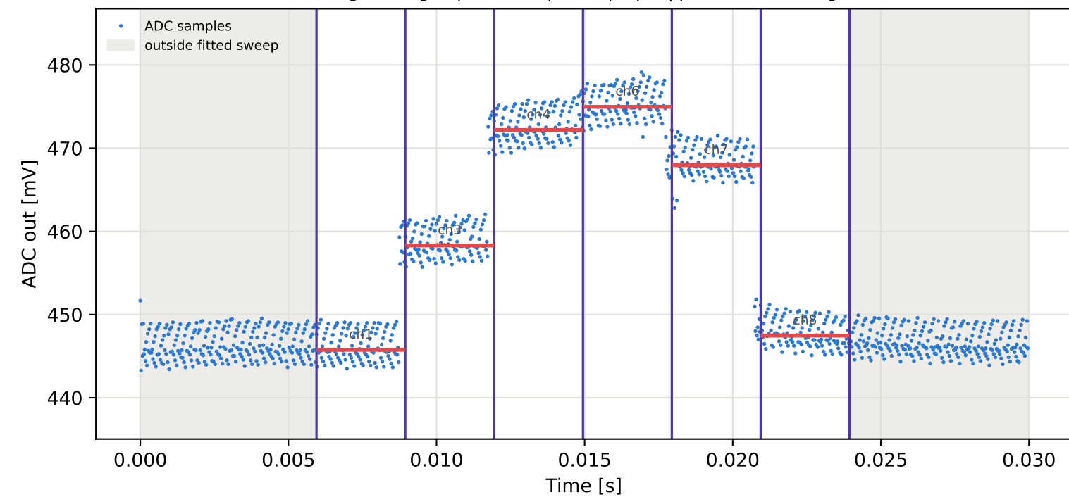
Tag1 &lt;- Tag3 | 905 MHz | run 0 | rep 1 | phase -96.04 deg
