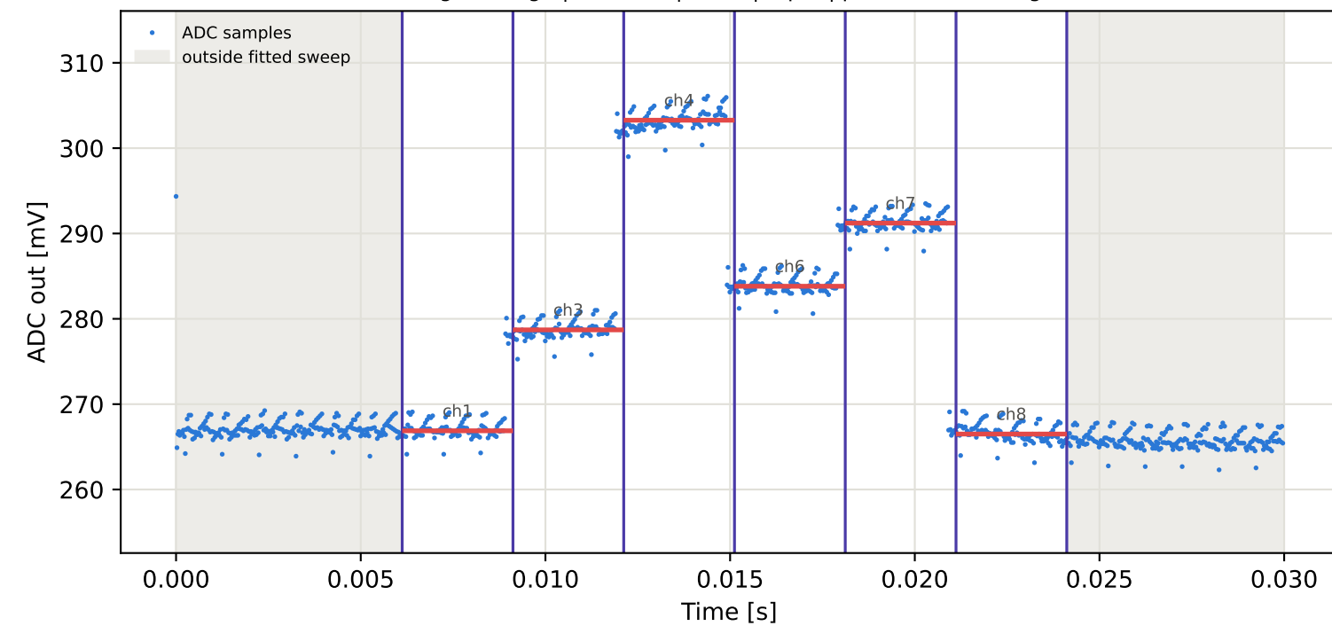
Tag7 &lt;- Tag5 | 955 MHz | run 0 | rep 1 | phase 71.65 deg
