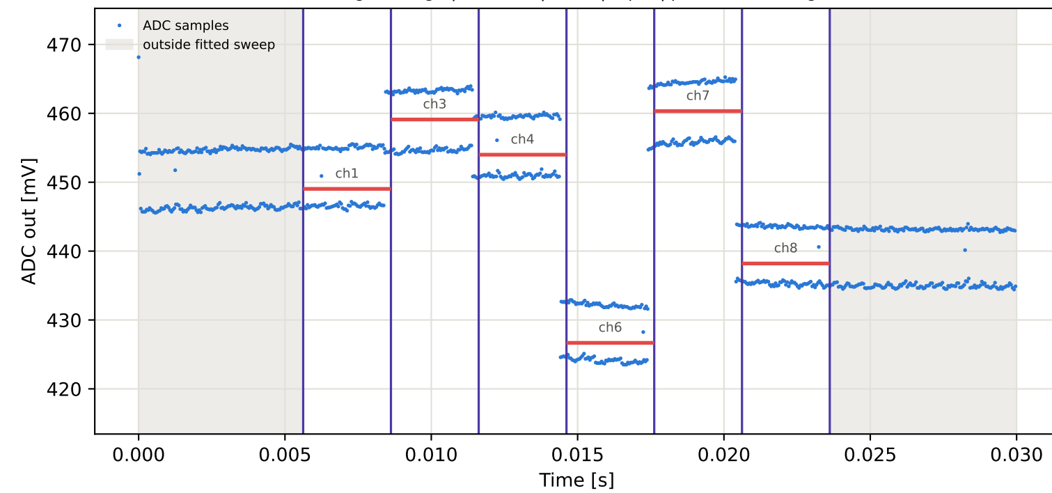
Tag8 &lt;- Tag1 | 995 MHz | run 0 | rep 1 | phase -87.29 deg
