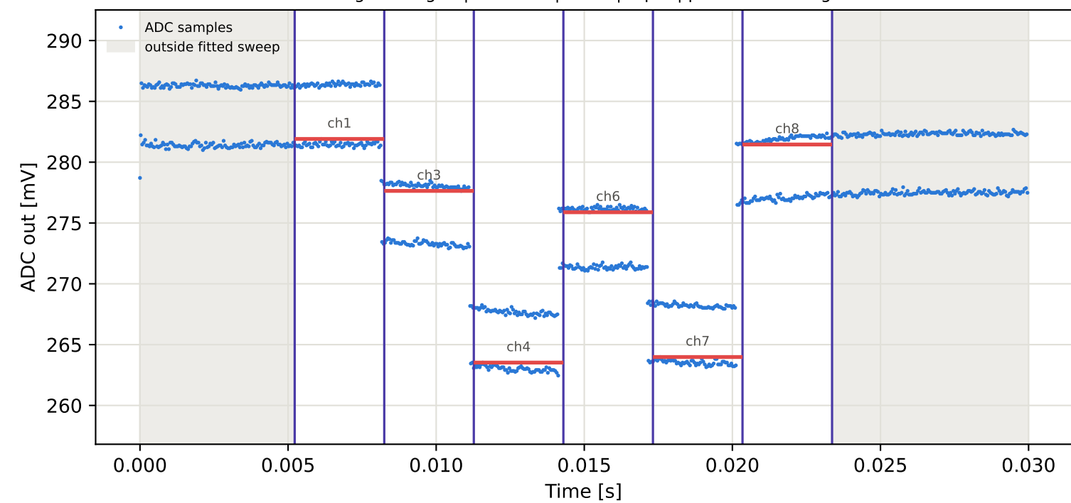
Tag5 &lt;- Tag2 | 835 MHz | run 0 | rep 1 | phase -173.49 deg
