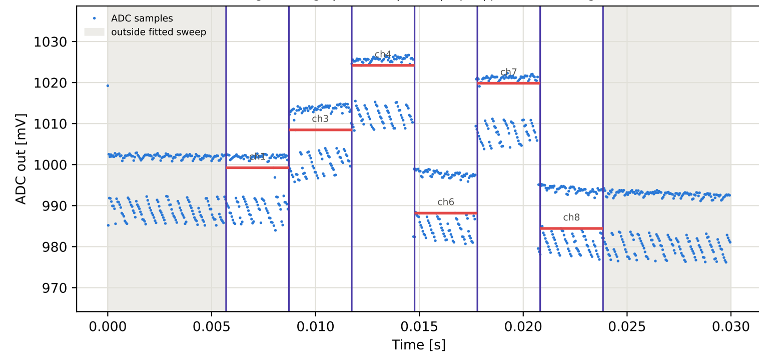
Tag15 &lt;- Tag9 | 945 MHz | run 0 | rep 1 | phase 128.71 deg
