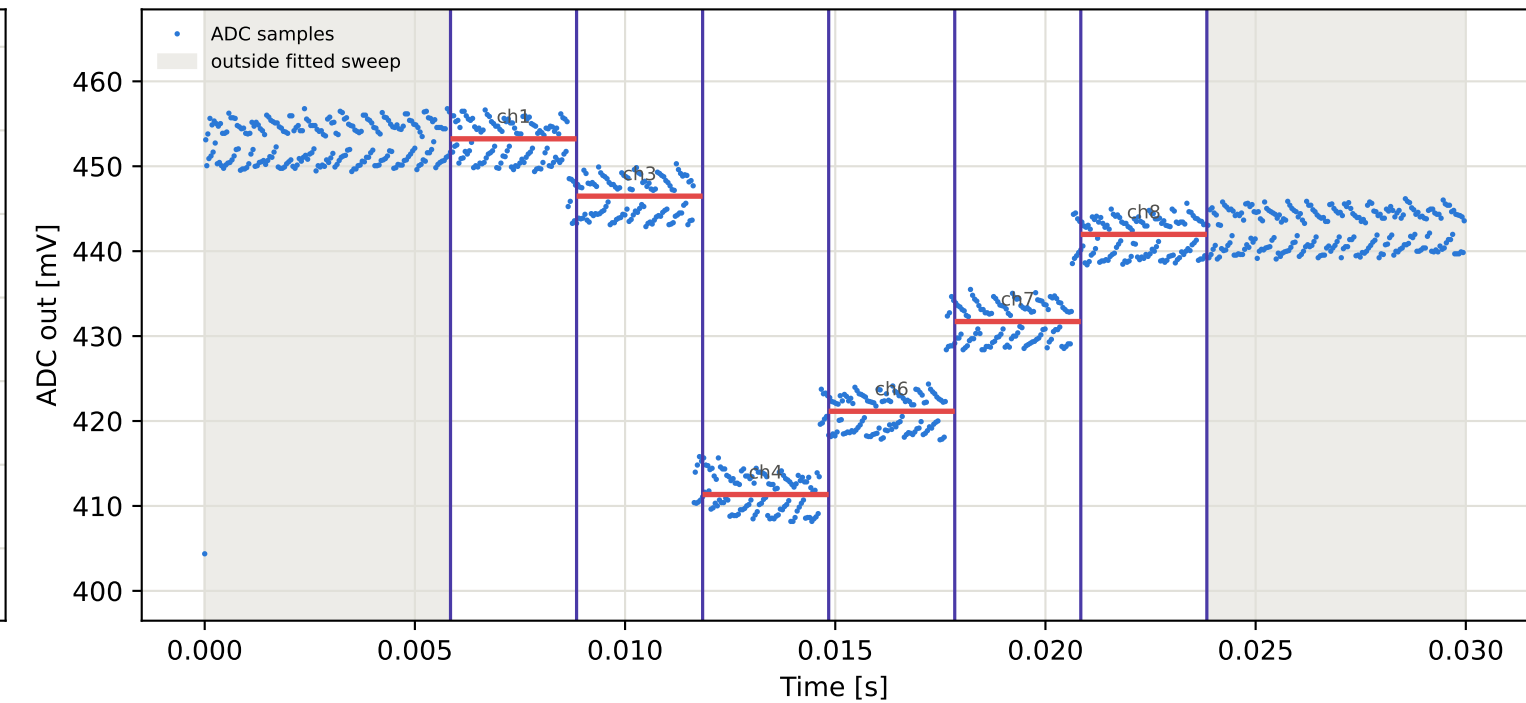
Tag15 &lt;- Tag10 | 985 MHz | run 0 | rep 1 | phase 97.17 deg
