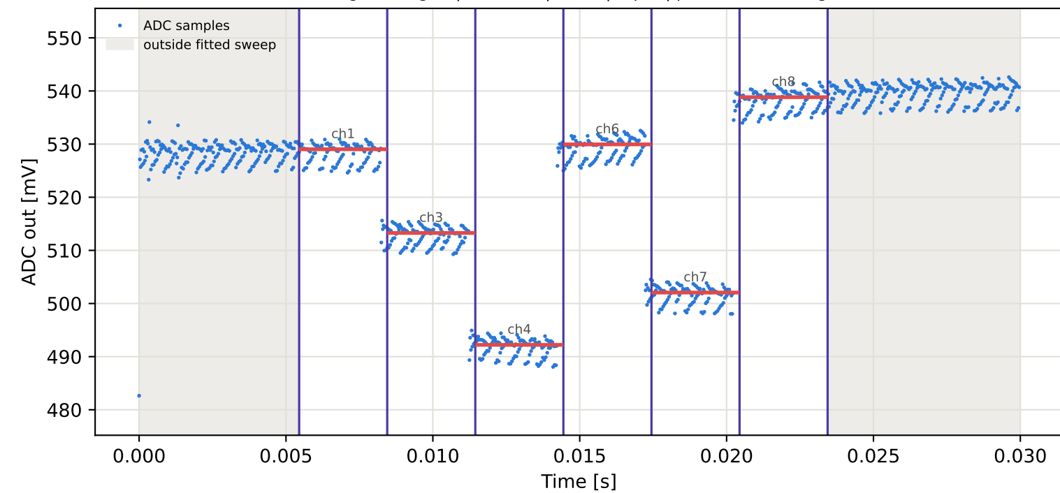
Tag5 &lt;- Tag16 | 935 MHz | run 0 | rep 1 | phase 56.11 deg
