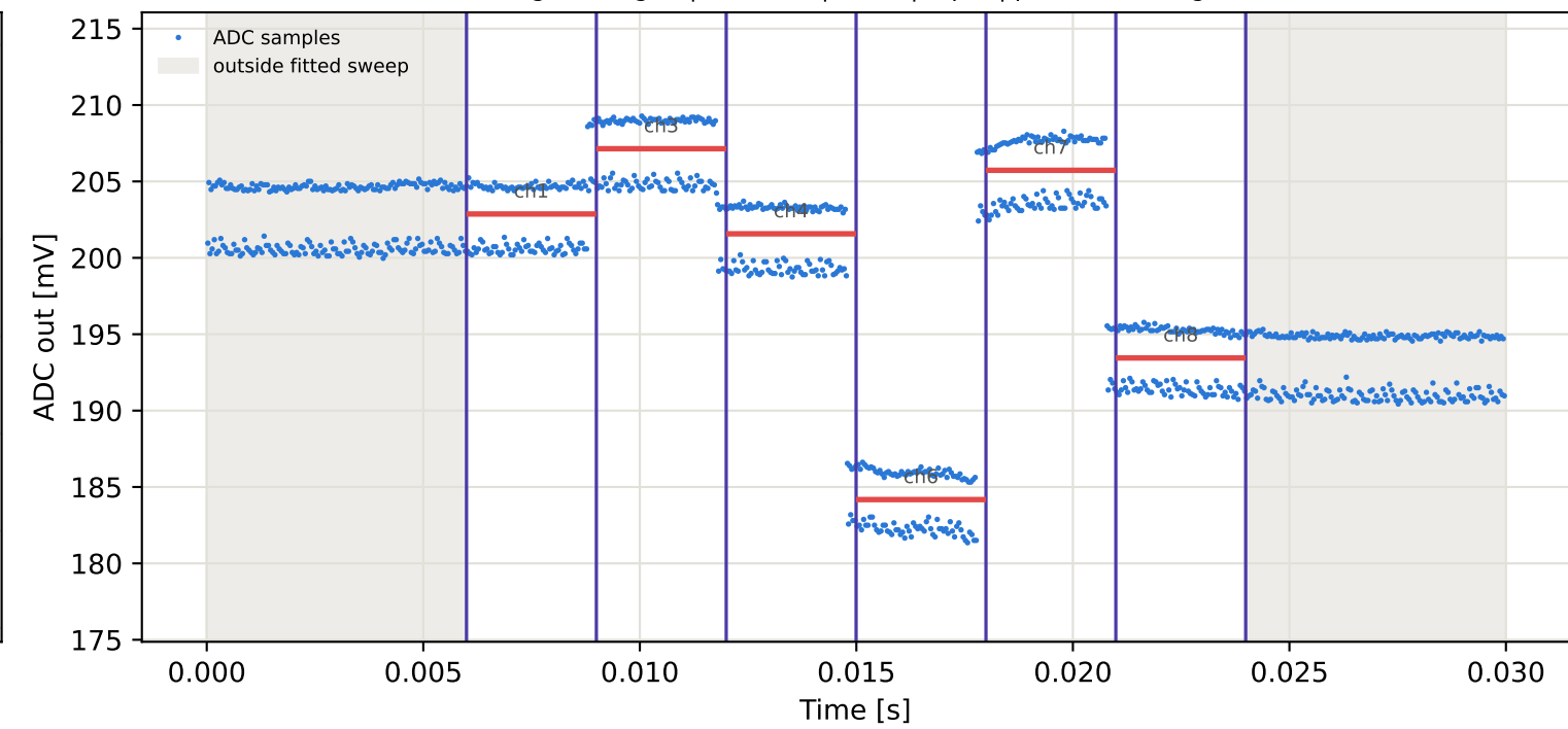
Tag1 &lt;- Tag2 | 985 MHz | run 0 | rep 1 | phase -84.34 deg
