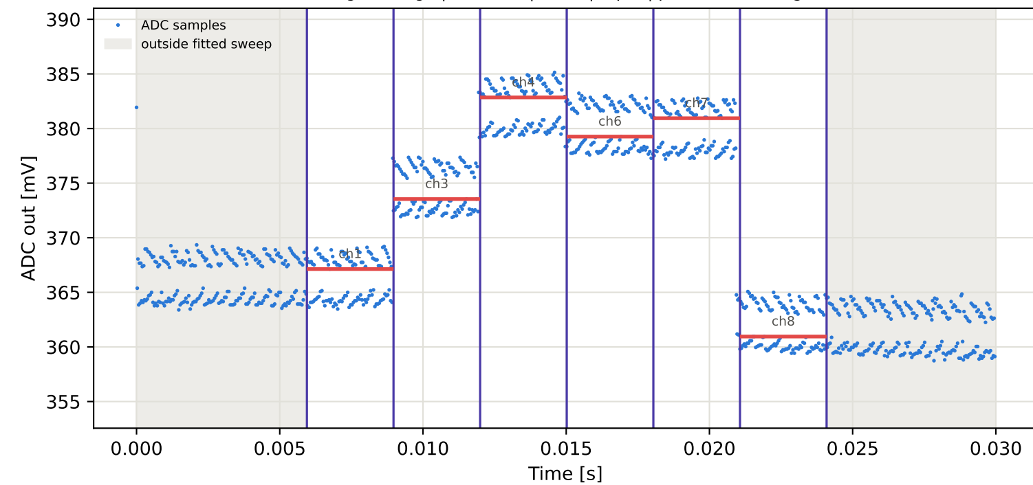
Tag8 &lt;- Tag4 | 825 MHz | run 0 | rep 1 | phase -42.98 deg
