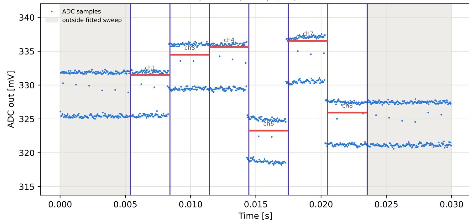
Tag5 &lt;- Tag9 | 985 MHz | run 0 | rep 1 | phase 38.61 deg
