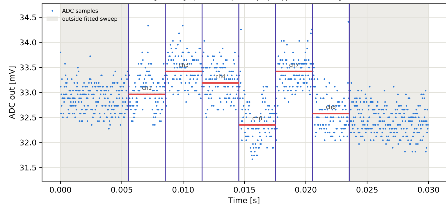
Tag4 &lt;- Tag2 | 805 MHz | run 0 | rep 1 | phase -2.42 deg
