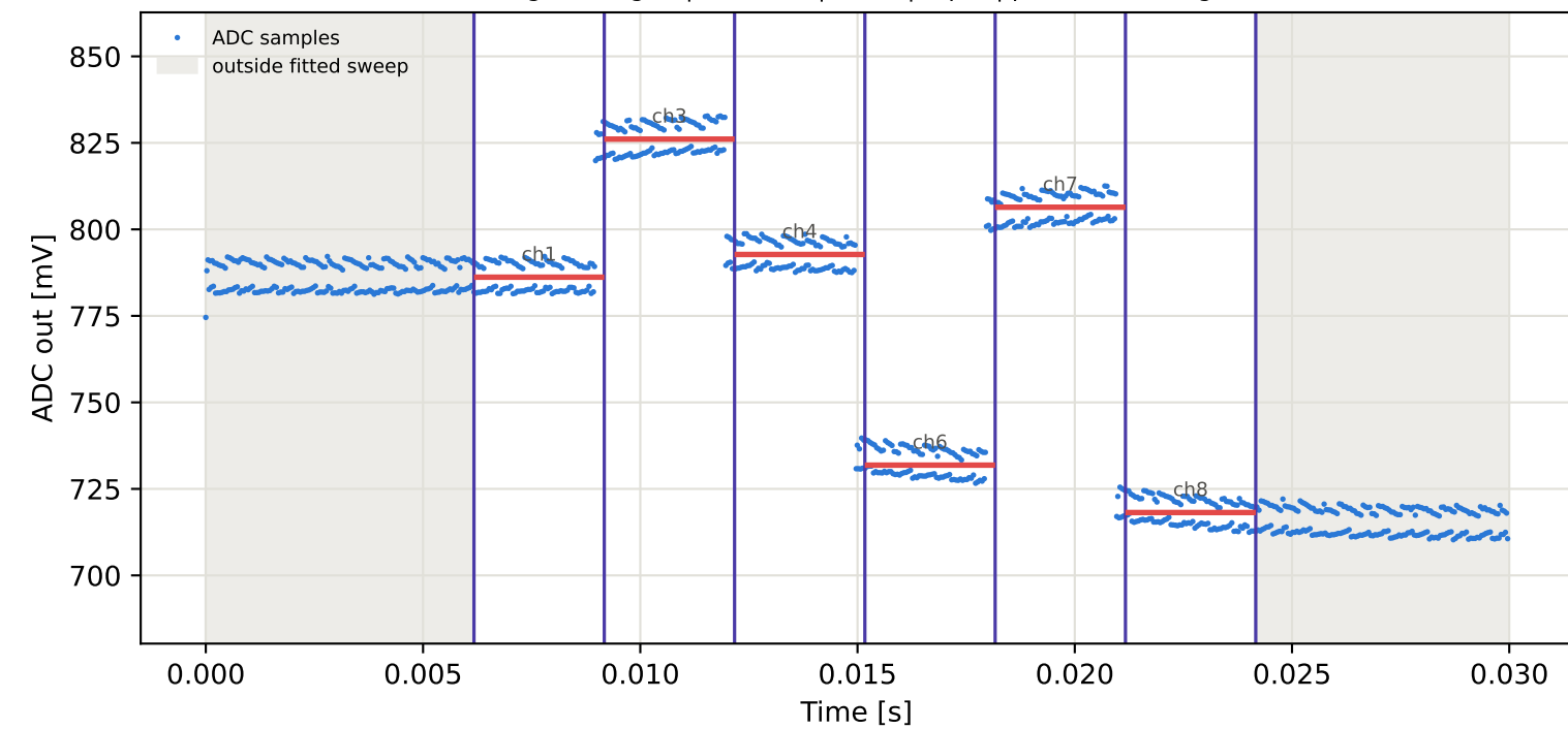
Tag7 &lt;- Tag3 | 865 MHz | run 0 | rep 1 | phase 33.47 deg
