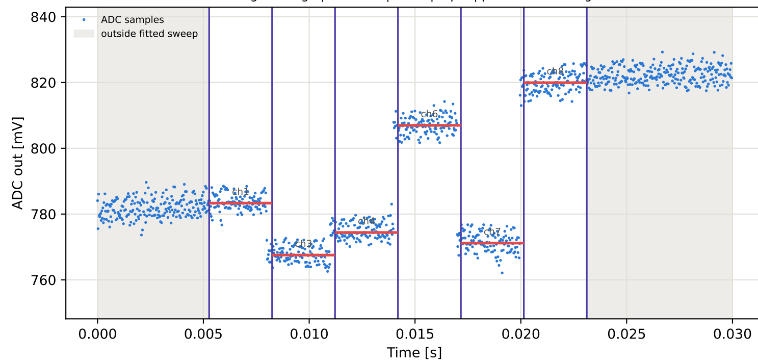
Tag8 &lt;- Tag1 | 885 MHz | run 0 | rep 1 | phase -58.32 deg
