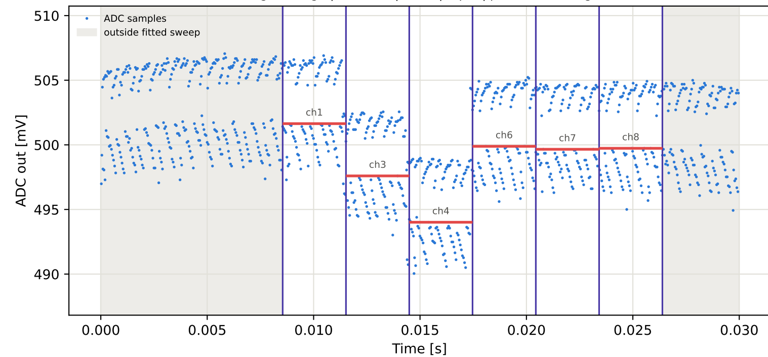
Tag5 &lt;- Tag8 | 945 MHz | run 0 | rep 1 | phase 177.49 deg
