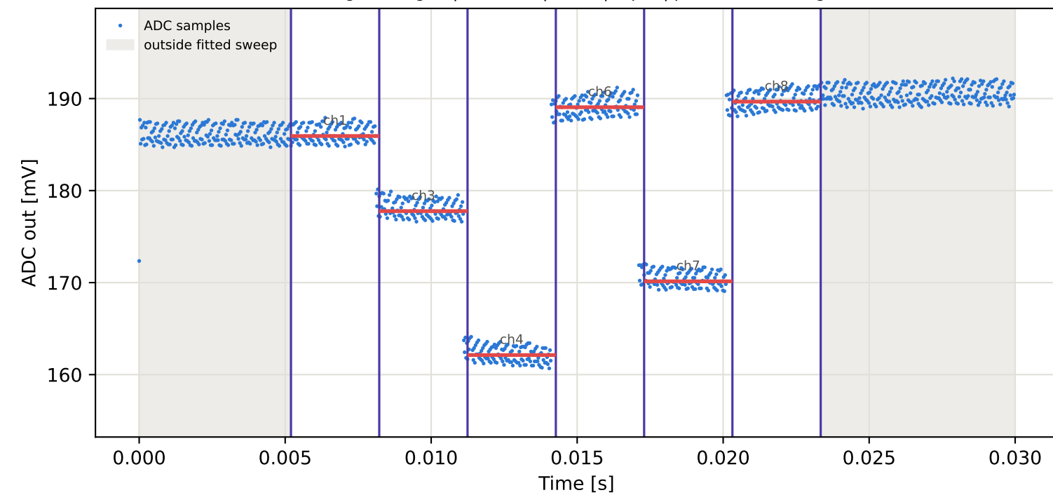
Tag1 &lt;- Tag16 | 995 MHz | run 0 | rep 1 | phase -40.38 deg
