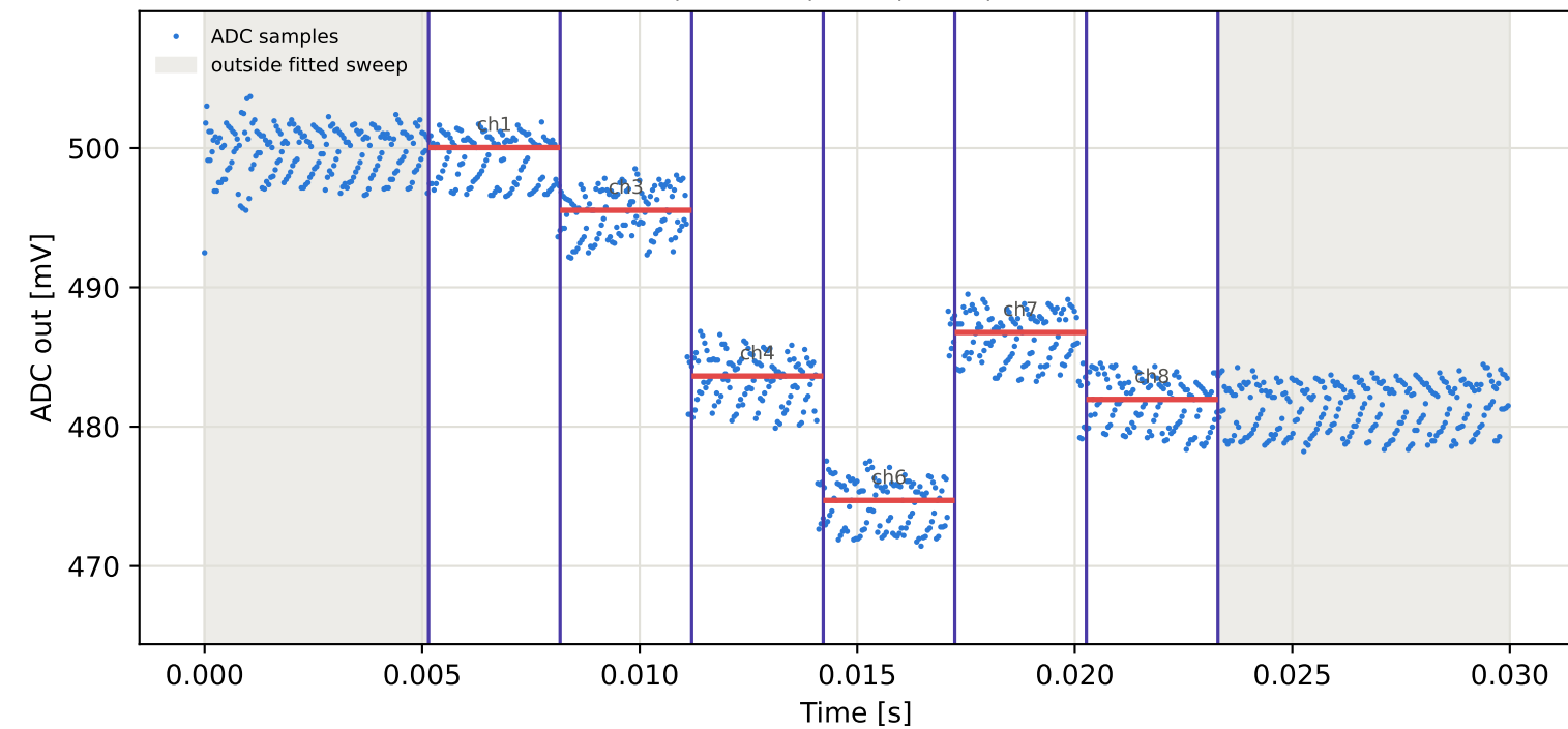
Tag6 &lt;- Tag5 | 865 MHz | run 0 | rep 1 | phase 38.11 deg
