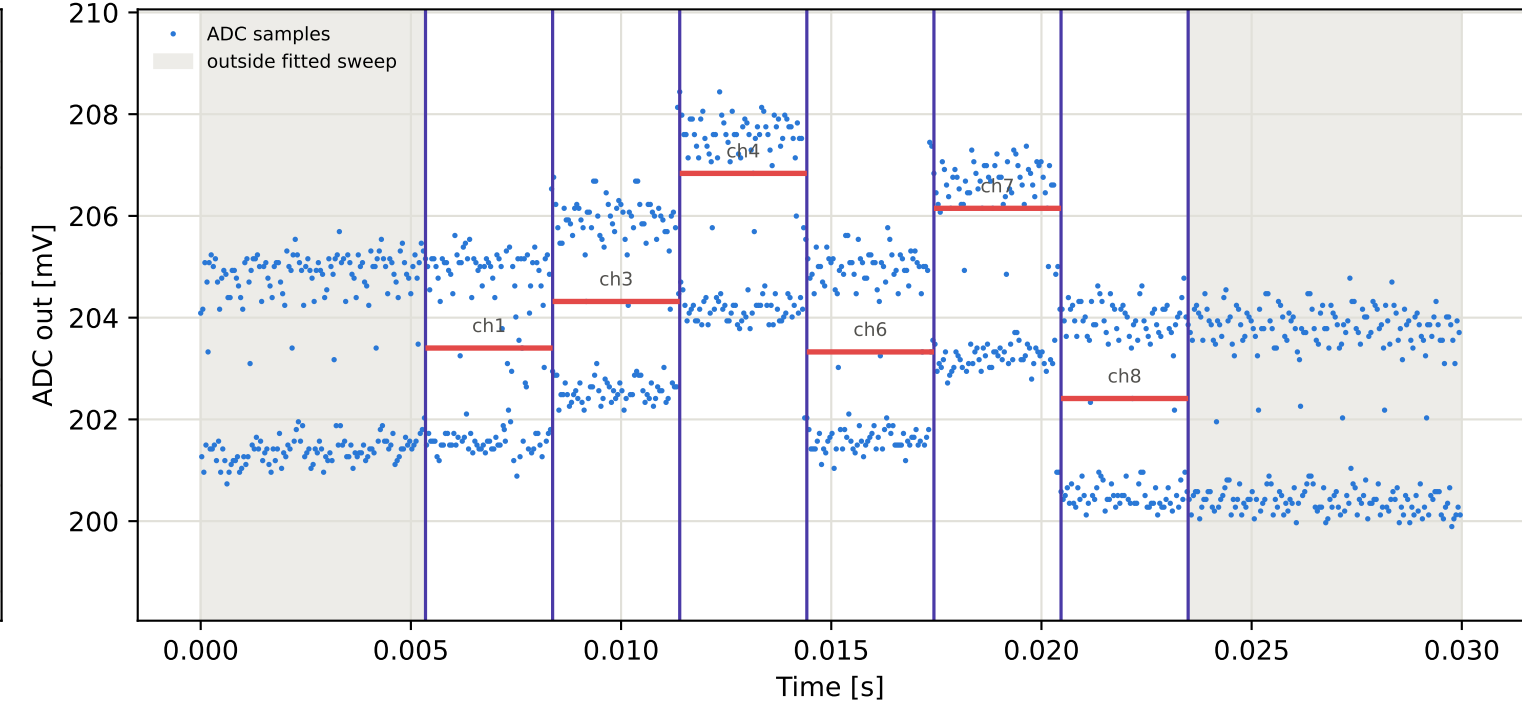
Tag1 &lt;- Tag4 | 985 MHz | run 0 | rep 1 | phase 96.80 deg
