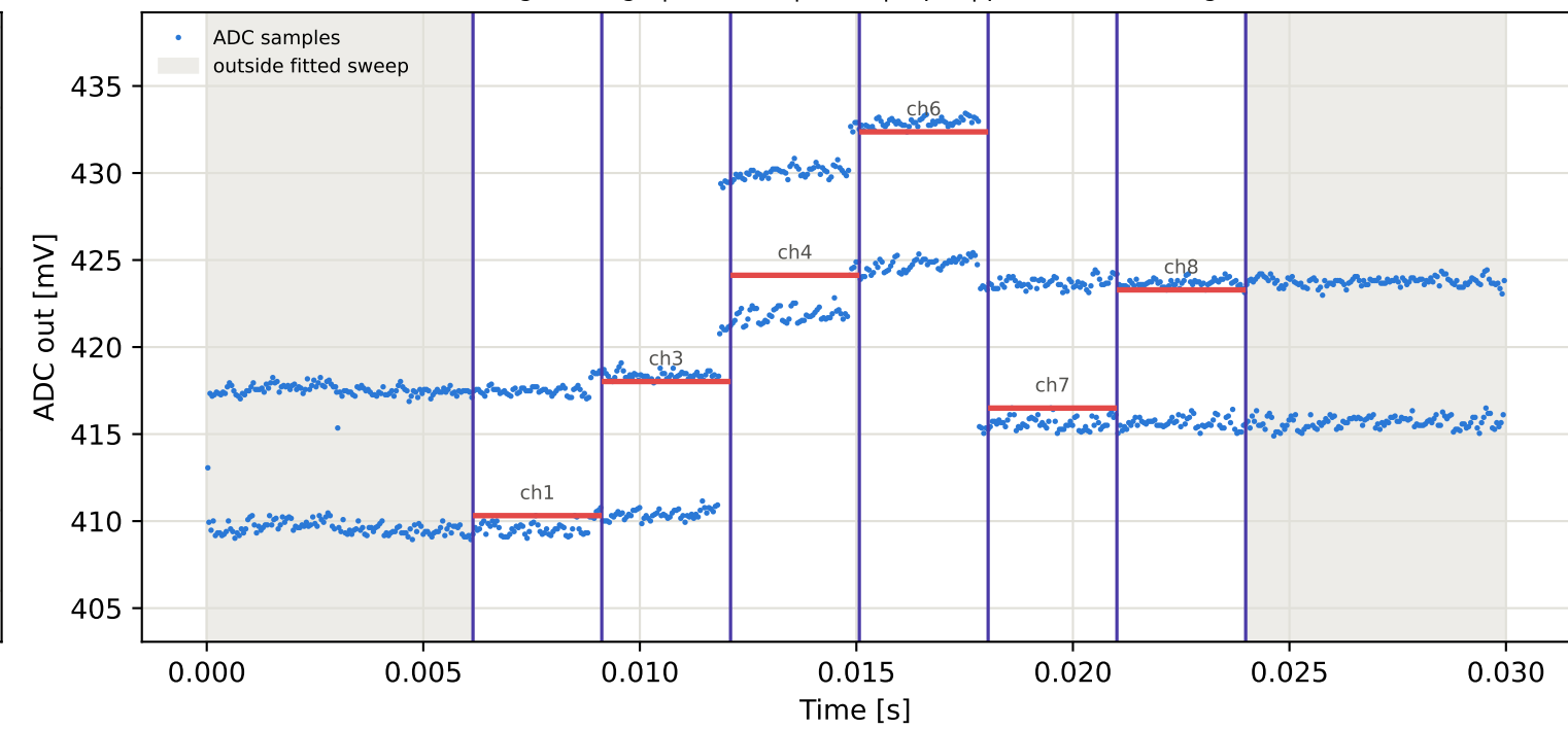
Tag8 &lt;- Tag10 | 965 MHz | run 0 | rep 1 | phase -20.12 deg
