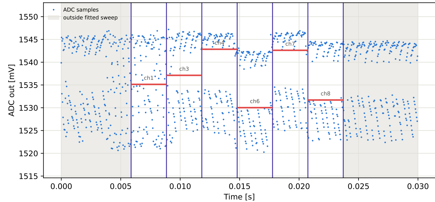
Tag2 &lt;- Tag8 | 925 MHz | run 0 | rep 1 | phase 21.04 deg
