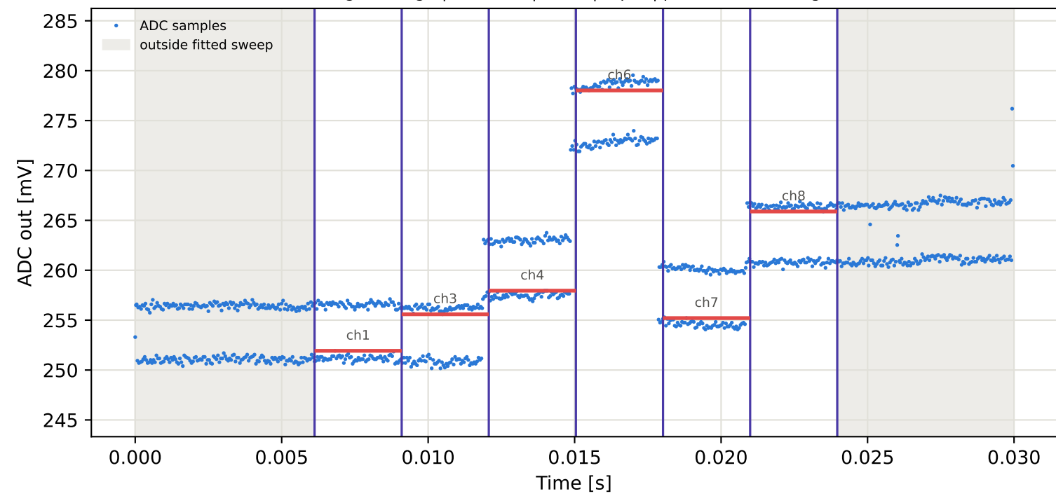
Tag3 &lt;- Tag15 | 925 MHz | run 0 | rep 1 | phase 3.84 deg
