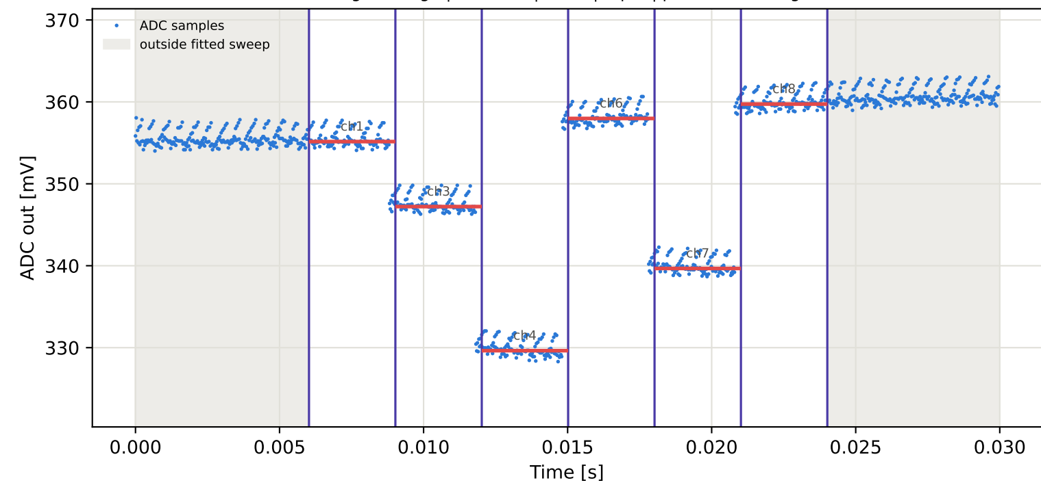
Tag4 &lt;- Tag3 | 985 MHz | run 0 | rep 1 | phase 98.41 deg
