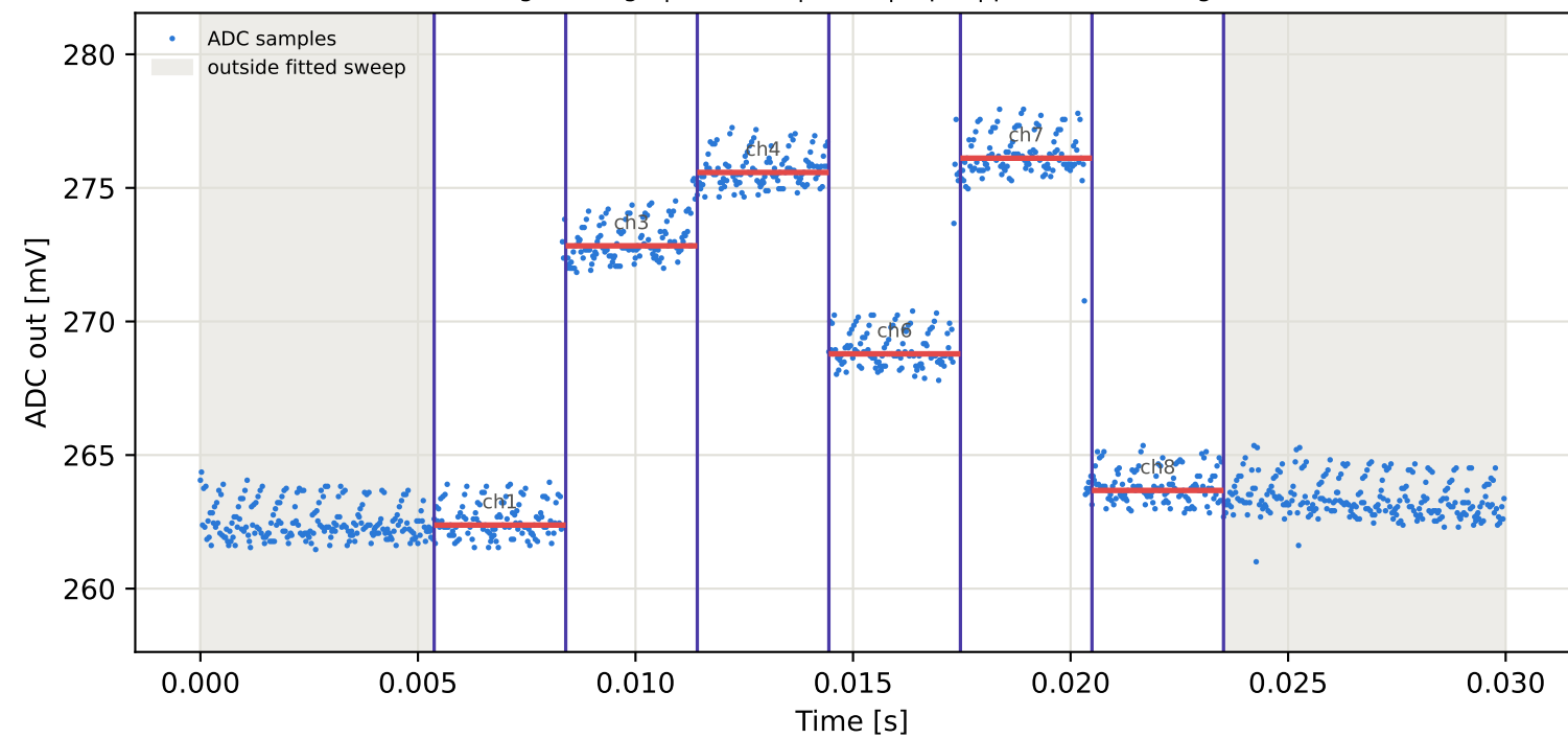
Tag5 &lt;- Tag1 | 855 MHz | run 0 | rep 1 | phase -88.70 deg
