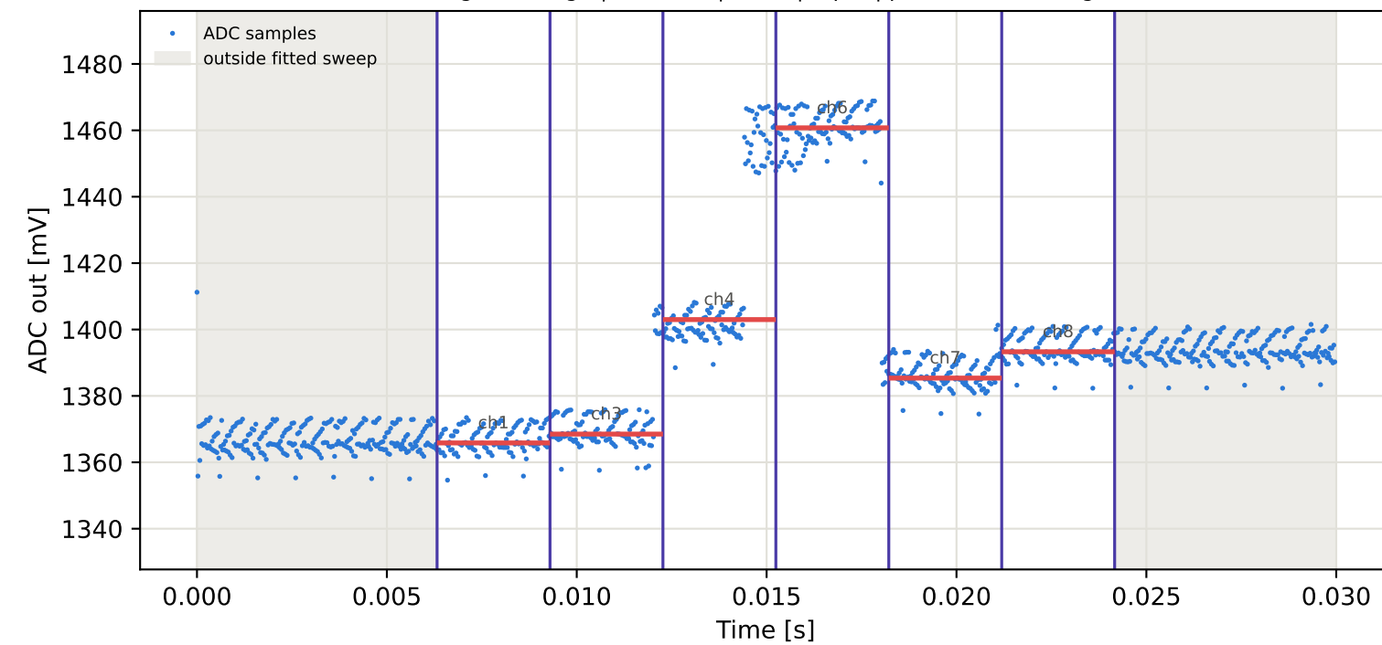
Tag16 &lt;- Tag4 | 885 MHz | run 0 | rep 1 | phase -15.34 deg
