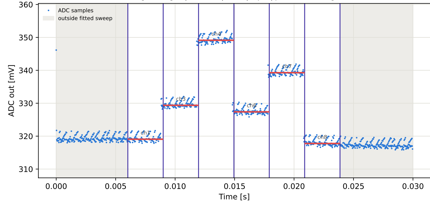
Tag5 &lt;- Tag2 | 985 MHz | run 0 | rep 1 | phase -178.37 deg
