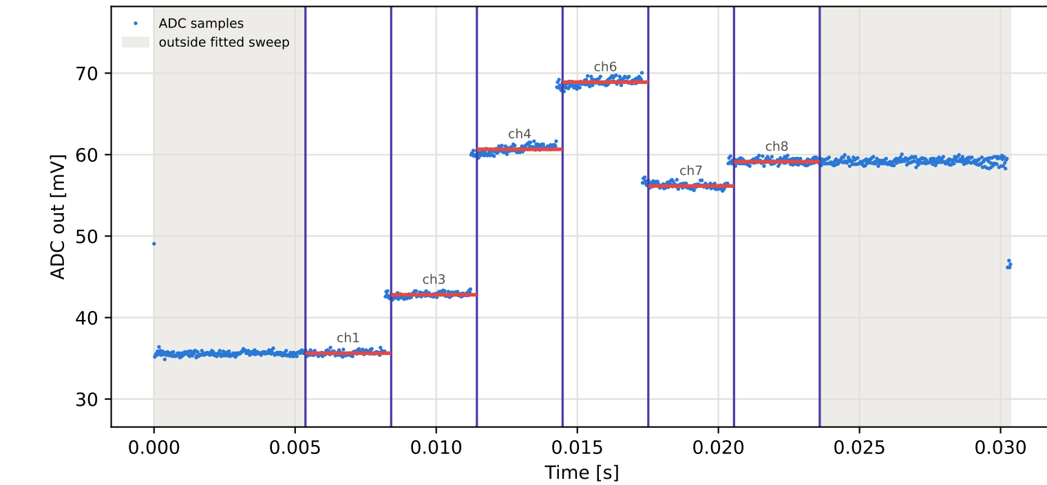
Tag9 &lt;- Tag16 | 855 MHz | run 0 | rep 1 | phase 109.75 deg
