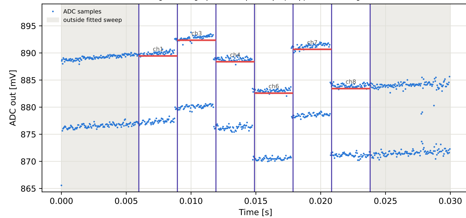
Tag15 &lt;- Tag1 | 875 MHz | run 0 | rep 1 | phase 6.94 deg
