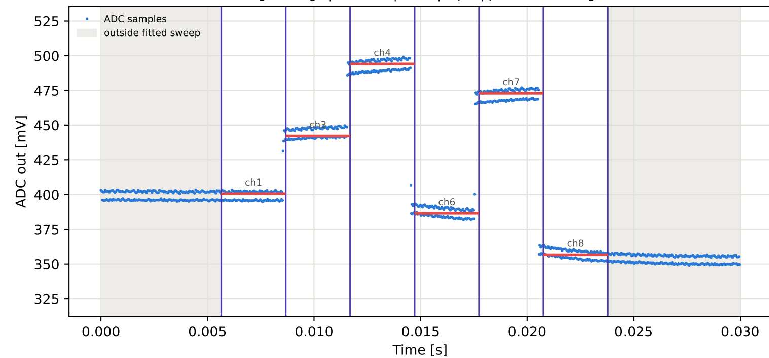
Tag3 &lt;- Tag8 | 935 MHz | run 0 | rep 1 | phase -65.86 deg
