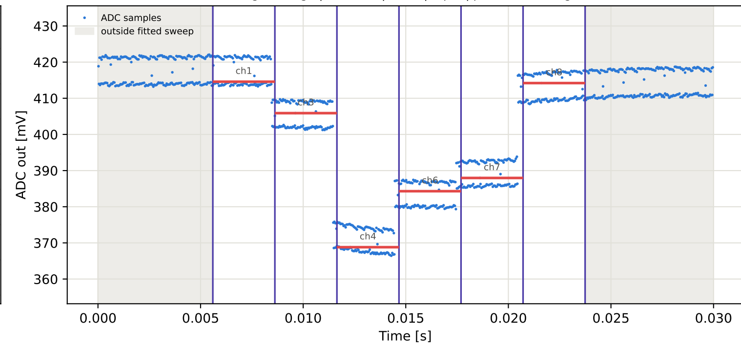
Tag9 &lt;- Tag6 | 955 MHz | run 0 | rep 1 | phase -7.41 deg
