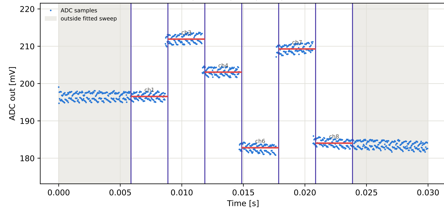
Tag4 &lt;- Tag9 | 835 MHz | run 0 | rep 1 | phase -5.98 deg
