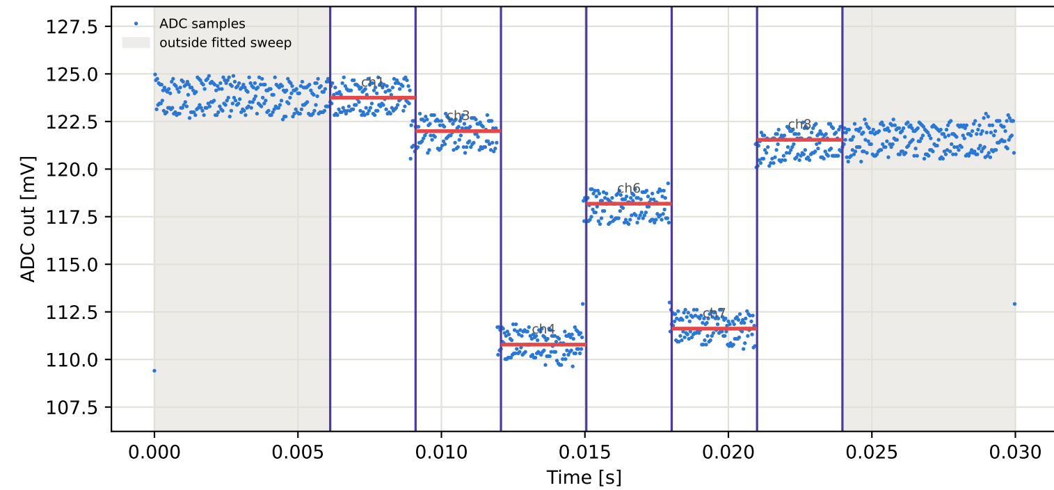
Tag5 &lt;- Tag1 | 785 MHz | run 0 | rep 1 | phase 110.25 deg
