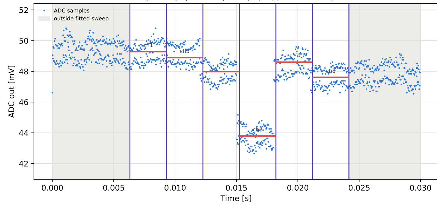
Tag1 &lt;- Tag4 | 845 MHz | run 0 | rep 1 | phase -67.70 deg
