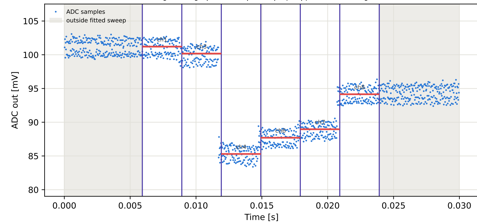
Tag3 &lt;- Tag9 | 795 MHz | run 0 | rep 1 | phase 67.49 deg
