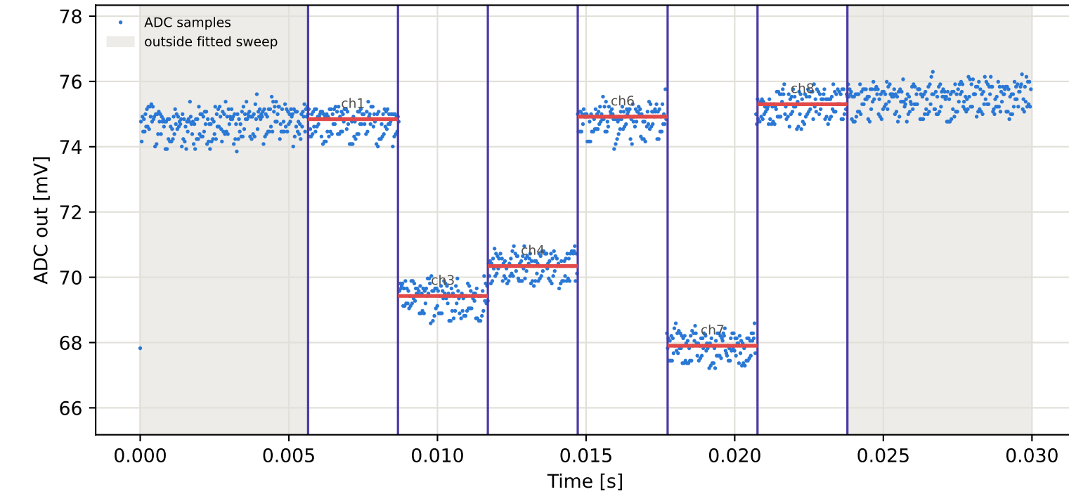
Tag9 &lt;- Tag16 | 795 MHz | run 0 | rep 1 | phase 96.55 deg
