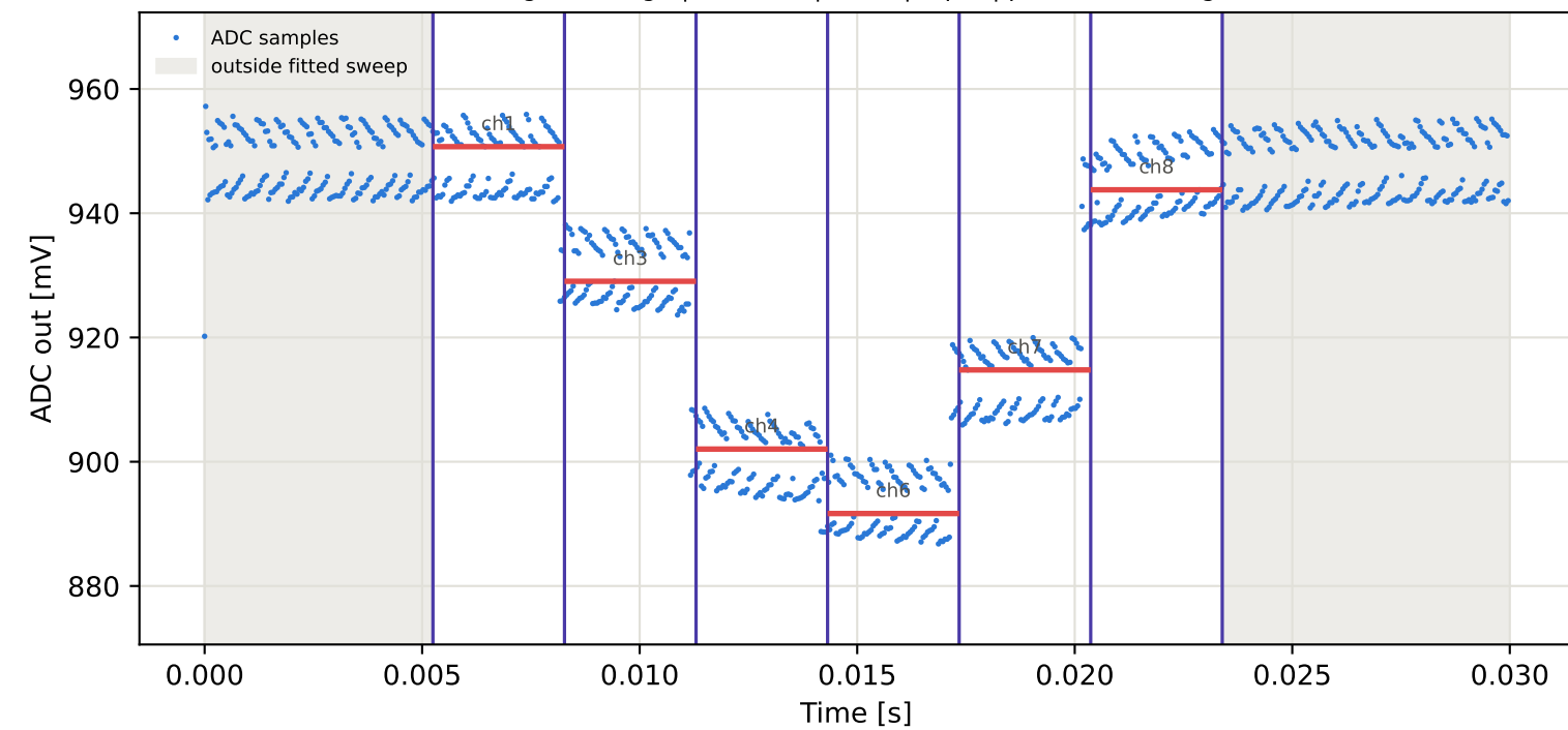
Tag16 &lt;- Tag1 | 925 MHz | run 0 | rep 1 | phase 138.04 deg
