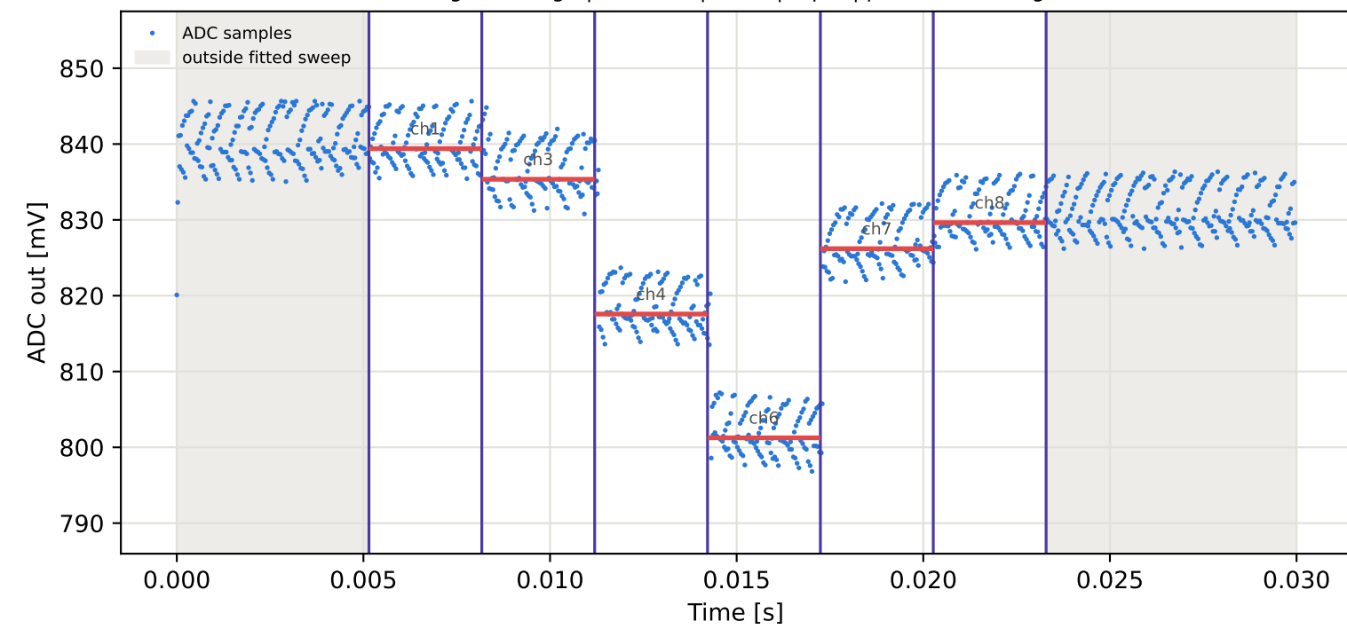
Tag15 &lt;- Tag5 | 935 MHz | run 0 | rep 1 | phase 34.90 deg
