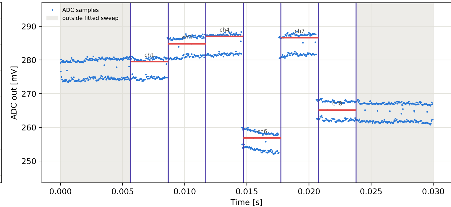
Tag6 &lt;- Tag5 | 925 MHz | run 0 | rep 1 | phase 135.29 deg
