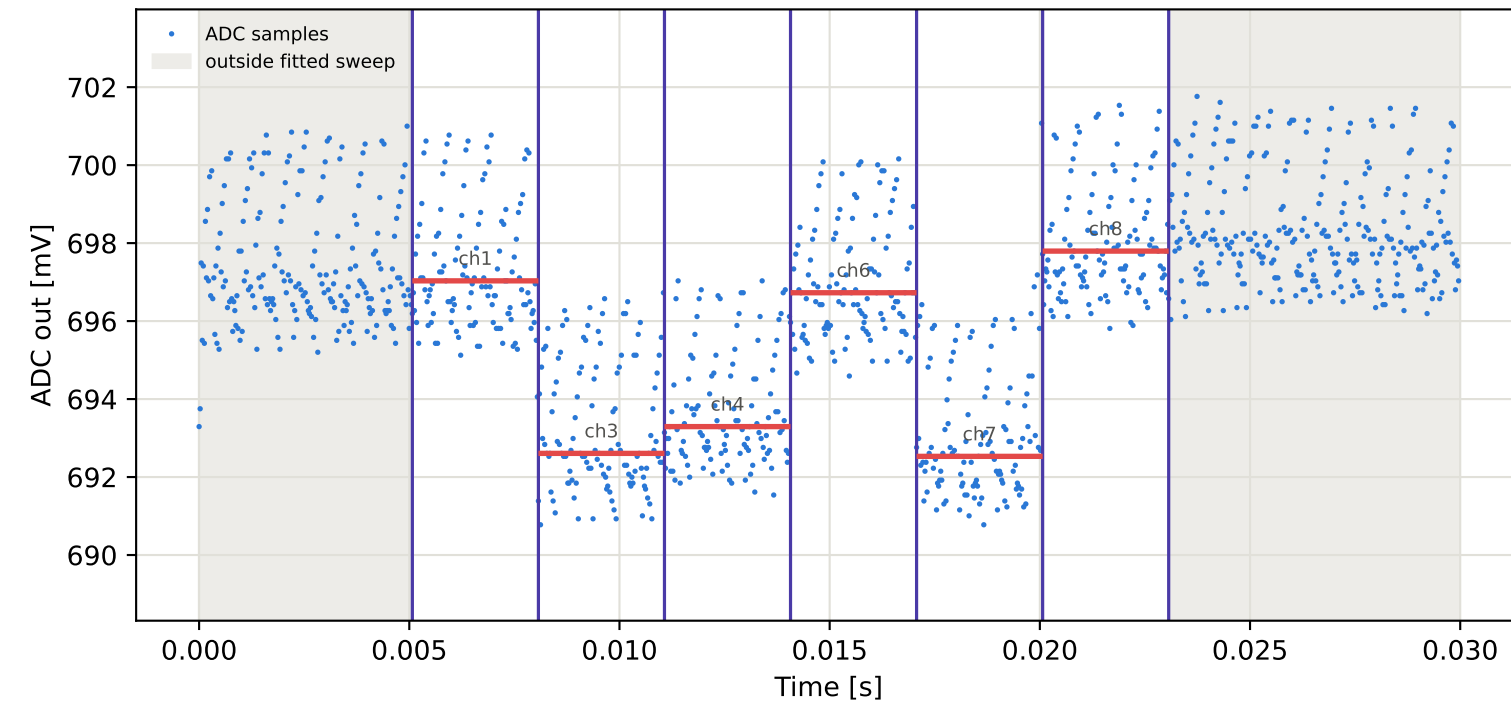
Tag2 &lt;- Tag15 | 855 MHz | run 0 | rep 1 | phase 98.90 deg
