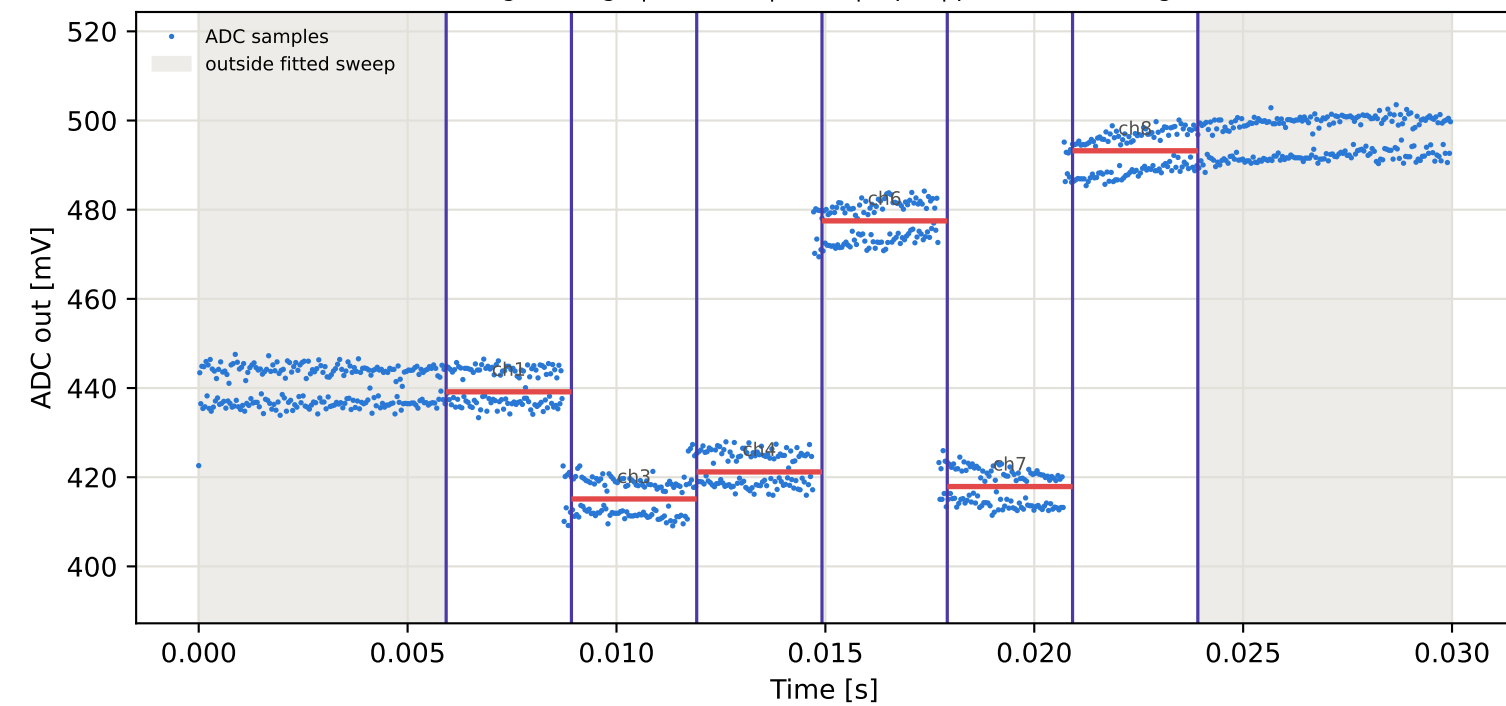
Tag1 &lt;- Tag7 | 885 MHz | run 0 | rep 1 | phase 104.75 deg
