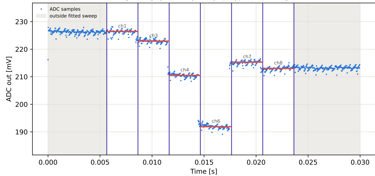
Tag9 &lt;- Tag15 | 915 MHz | run 0 | rep 1 | phase 9.18 deg
