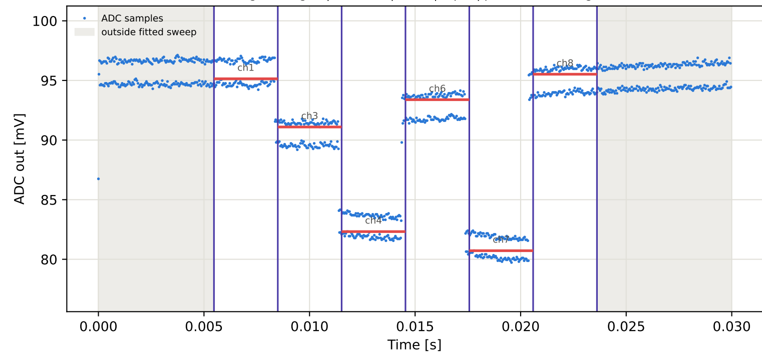
Tag5 &lt;- Tag2 | 785 MHz | run 0 | rep 1 | phase 85.25 deg
