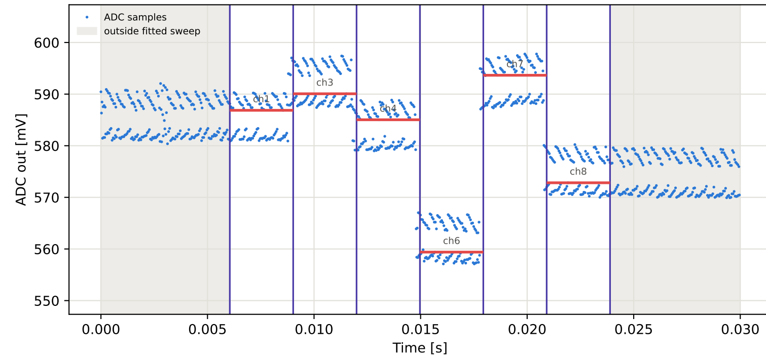
Tag15 &lt;- Tag5 | 995 MHz | run 0 | rep 1 | phase 161.88 deg
