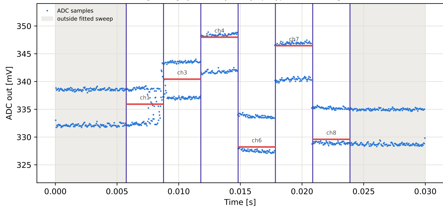
Tag4 &lt;- Tag8 | 985 MHz | run 0 | rep 1 | phase 74.63 deg
