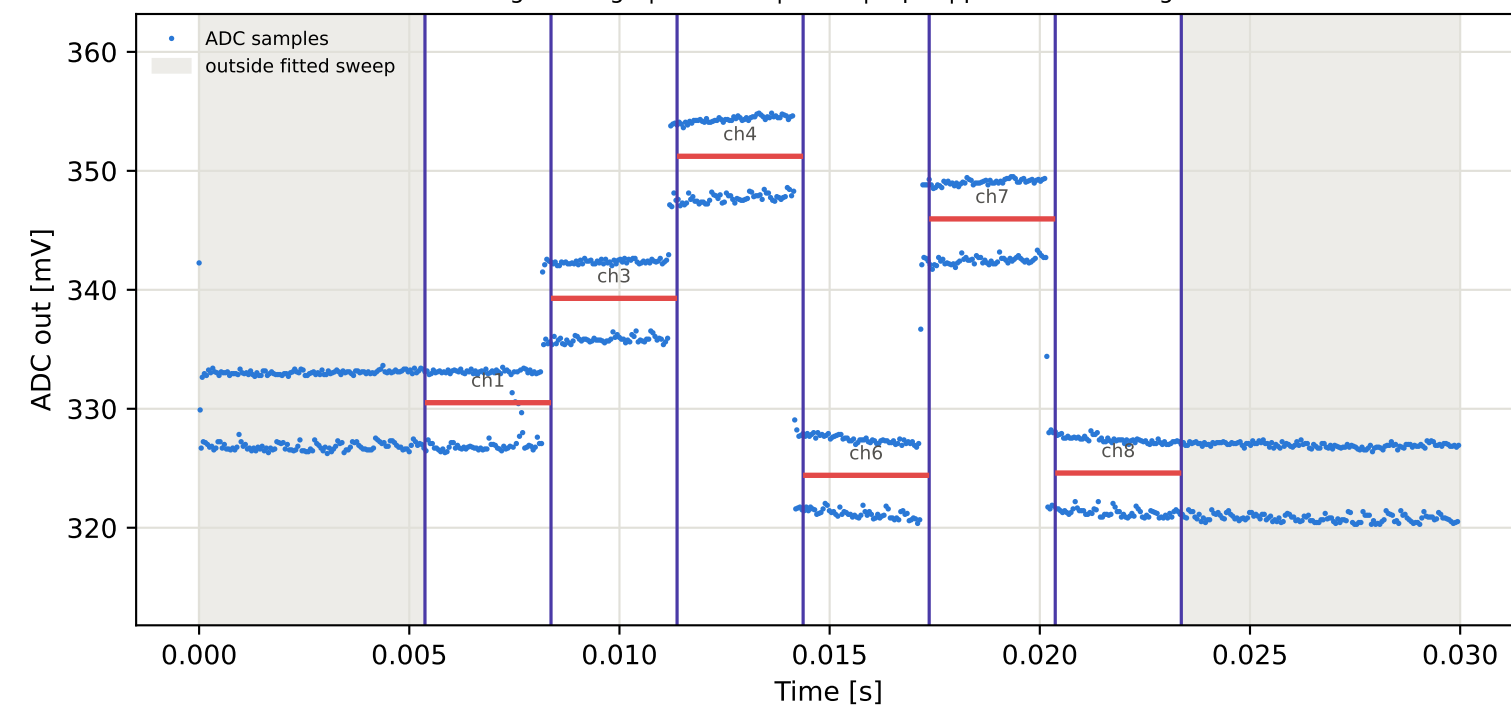
Tag4 &lt;- Tag15 | 985 MHz | run 0 | rep 1 | phase -47.60 deg
