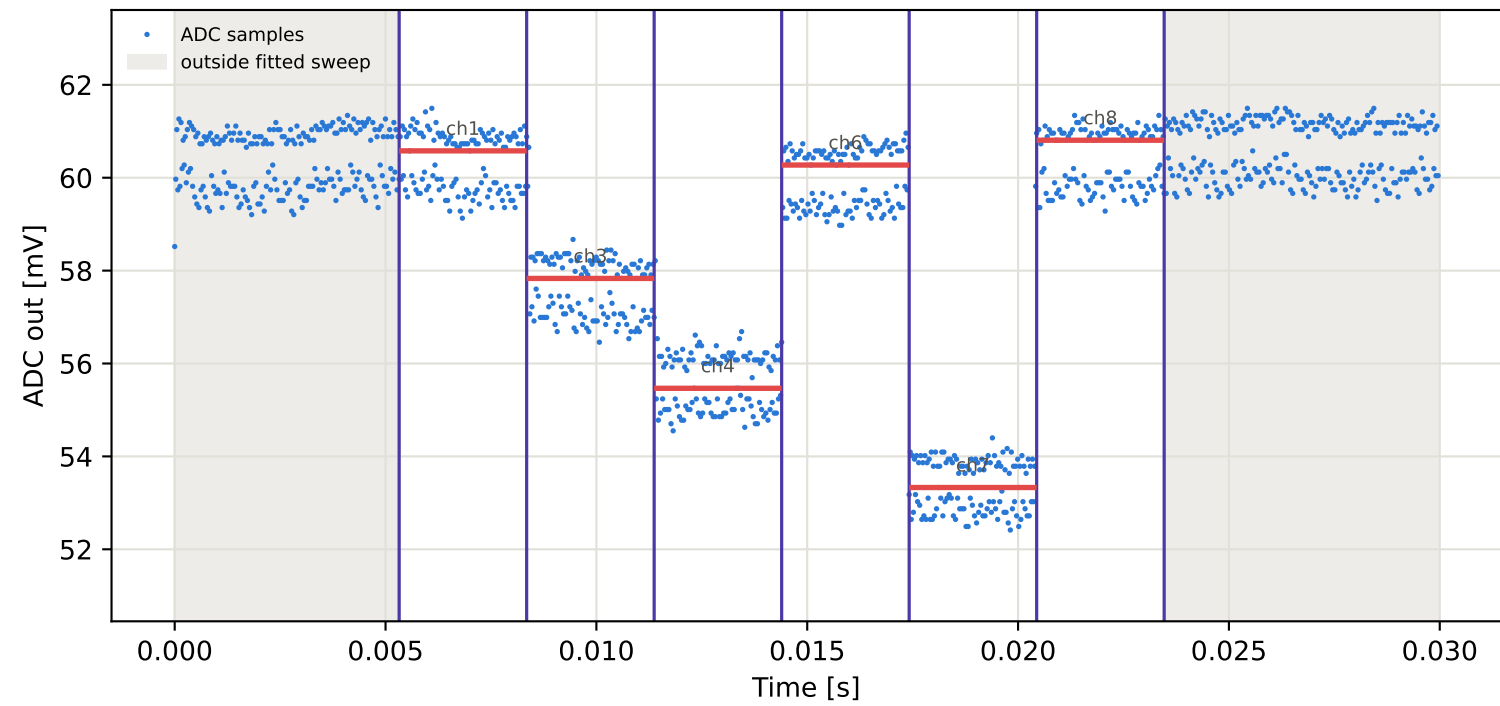
Tag1 &lt;- Tag16 | 775 MHz | run 0 | rep 1 | phase 71.71 deg
