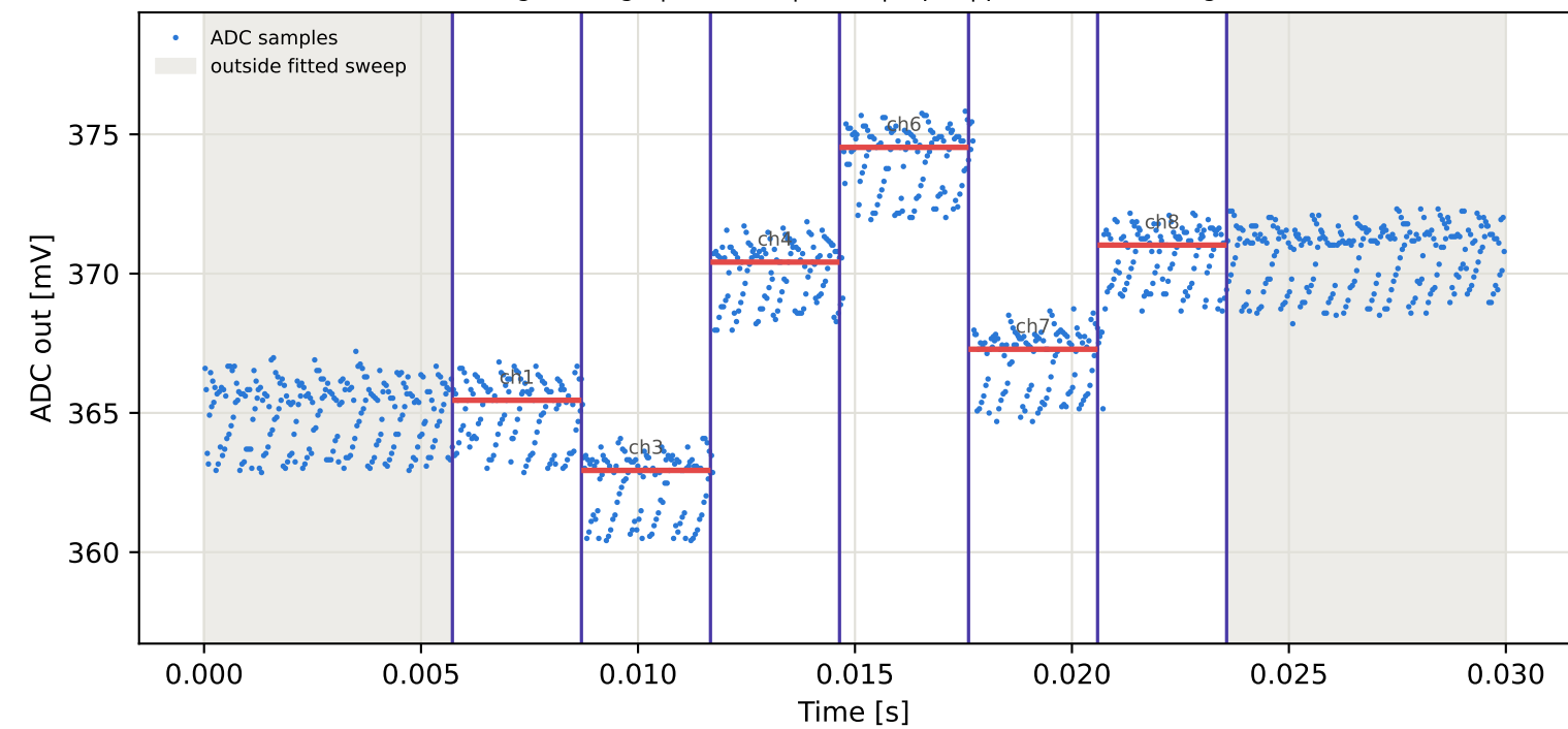
Tag8 &lt;- Tag10 | 825 MHz | run 0 | rep 1 | phase 108.71 deg
