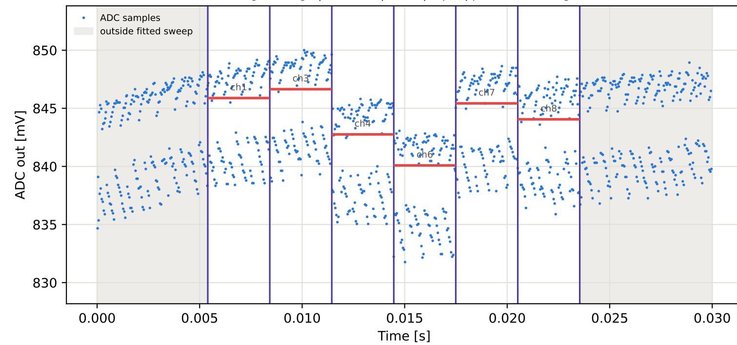
Tag6 &lt;- Tag9 | 875 MHz | run 0 | rep 1 | phase 50.56 deg
