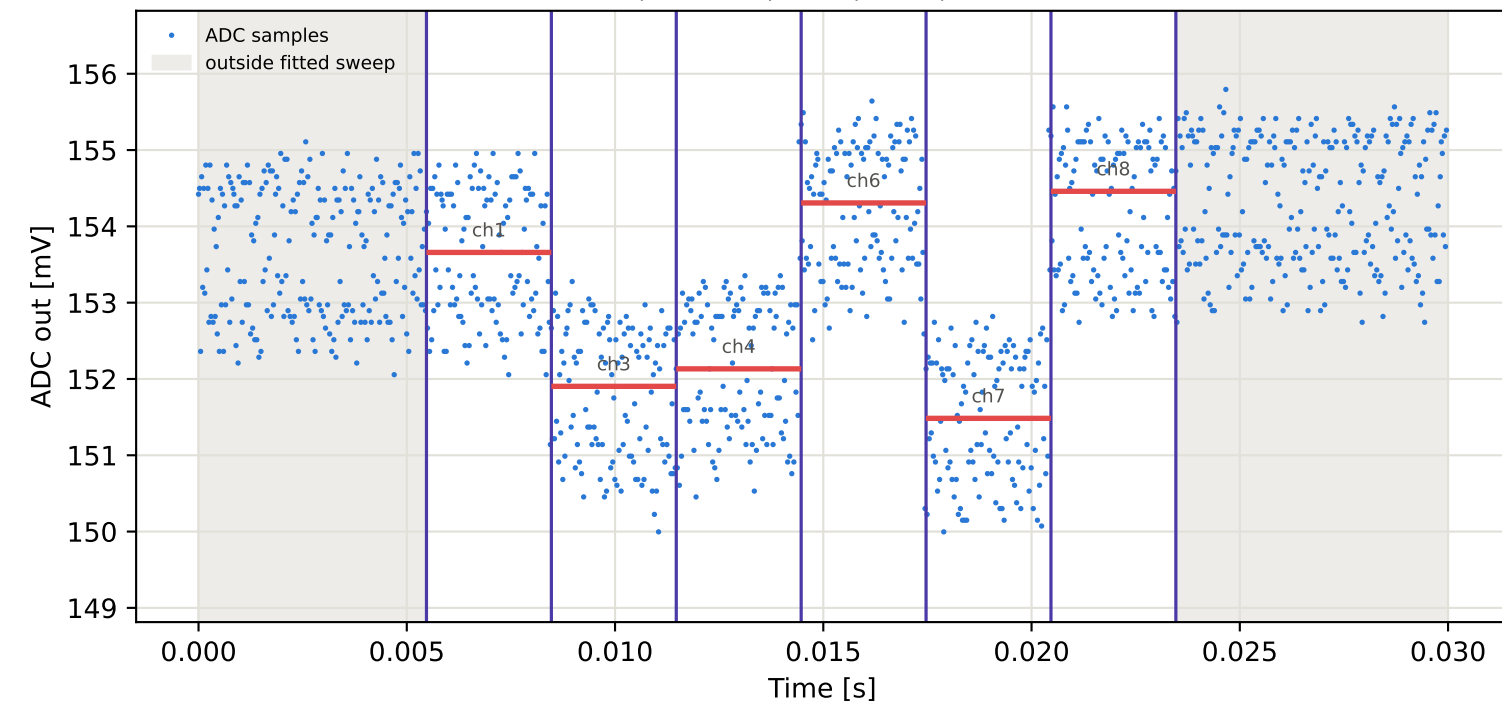
Tag8 &lt;- Tag6 | 795 MHz | run 0 | rep 1 | phase 155.01 deg
