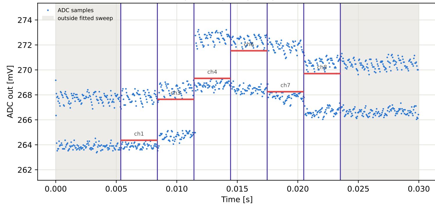
Tag10 &lt;- Tag5 | 835 MHz | run 0 | rep 1 | phase -136.64 deg
