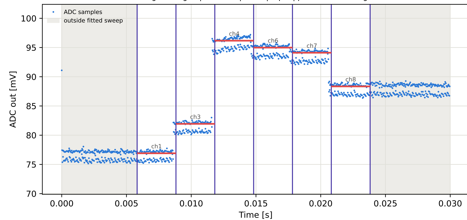
Tag1 &lt;- Tag16 | 825 MHz | run 0 | rep 1 | phase 131.56 deg
