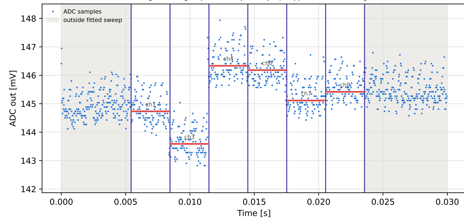
Tag16 &lt;- Tag10 | 775 MHz | run 0 | rep 1 | phase -126.47 deg
