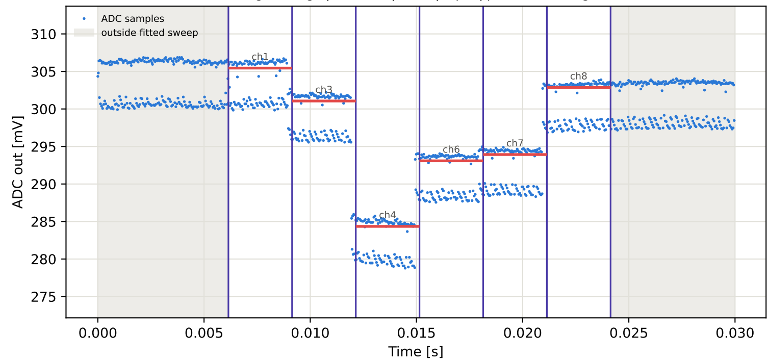
Tag3 &lt;- Tag15 | 975 MHz | run 0 | rep 1 | phase 73.53 deg
