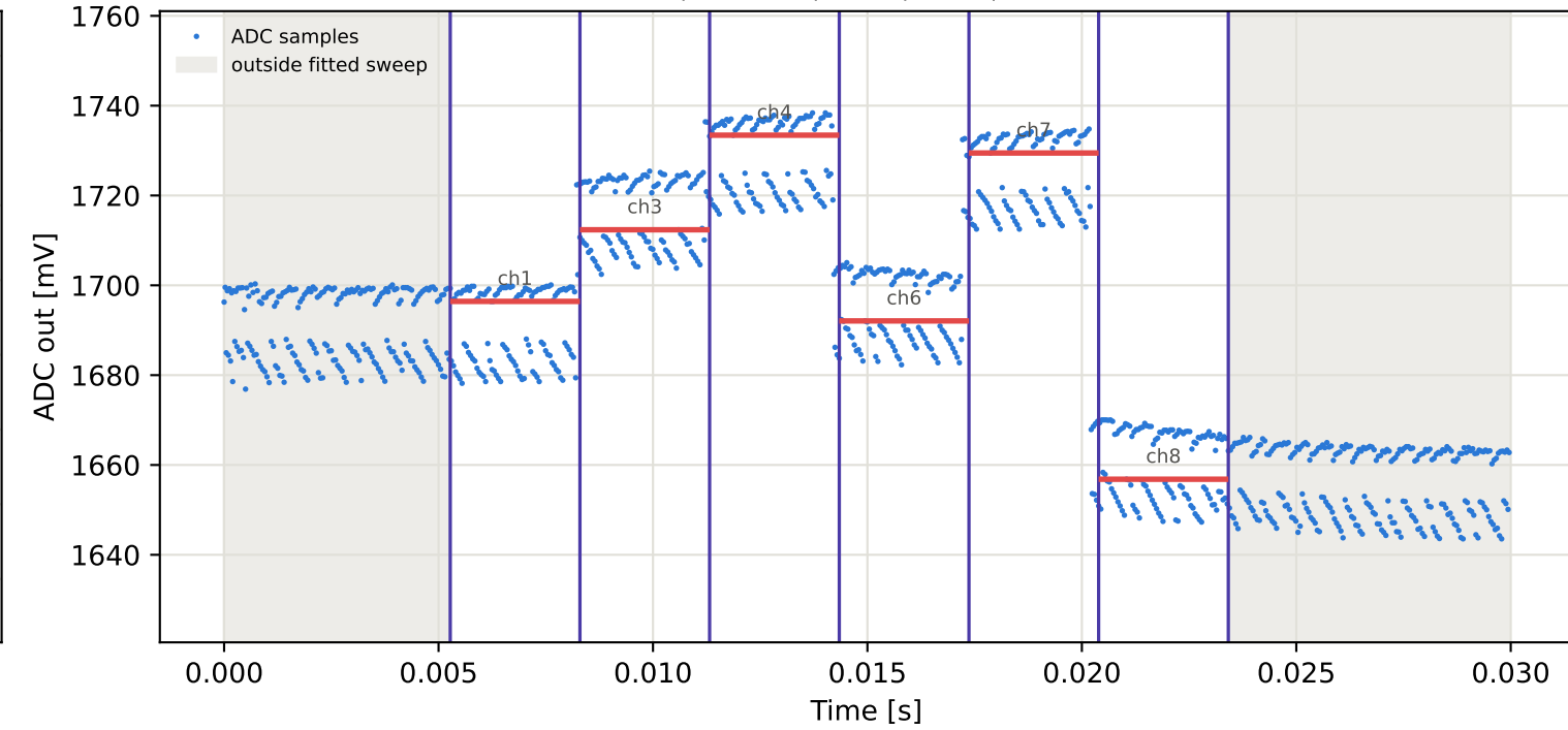
Tag2 &lt;- Tag8 | 905 MHz | run 0 | rep 1 | phase -64.21 deg
