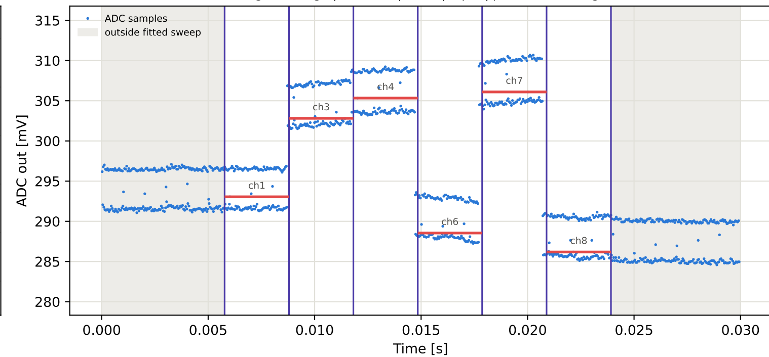
Tag10 &lt;- Tag9 | 855 MHz | run 0 | rep 1 | phase 13.70 deg
