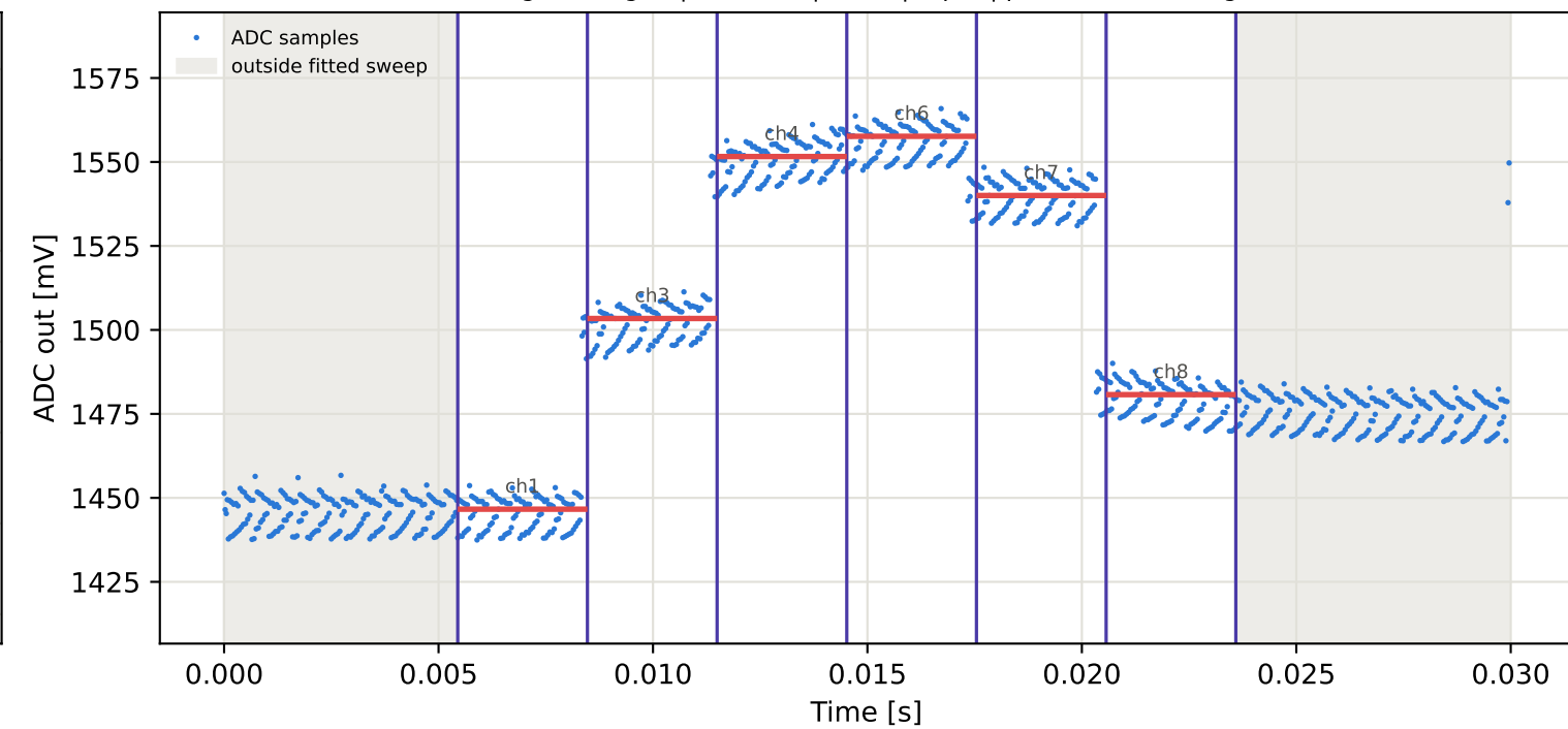
Tag5 &lt;- Tag2 | 895 MHz | run 0 | rep 1 | phase 44.93 deg
