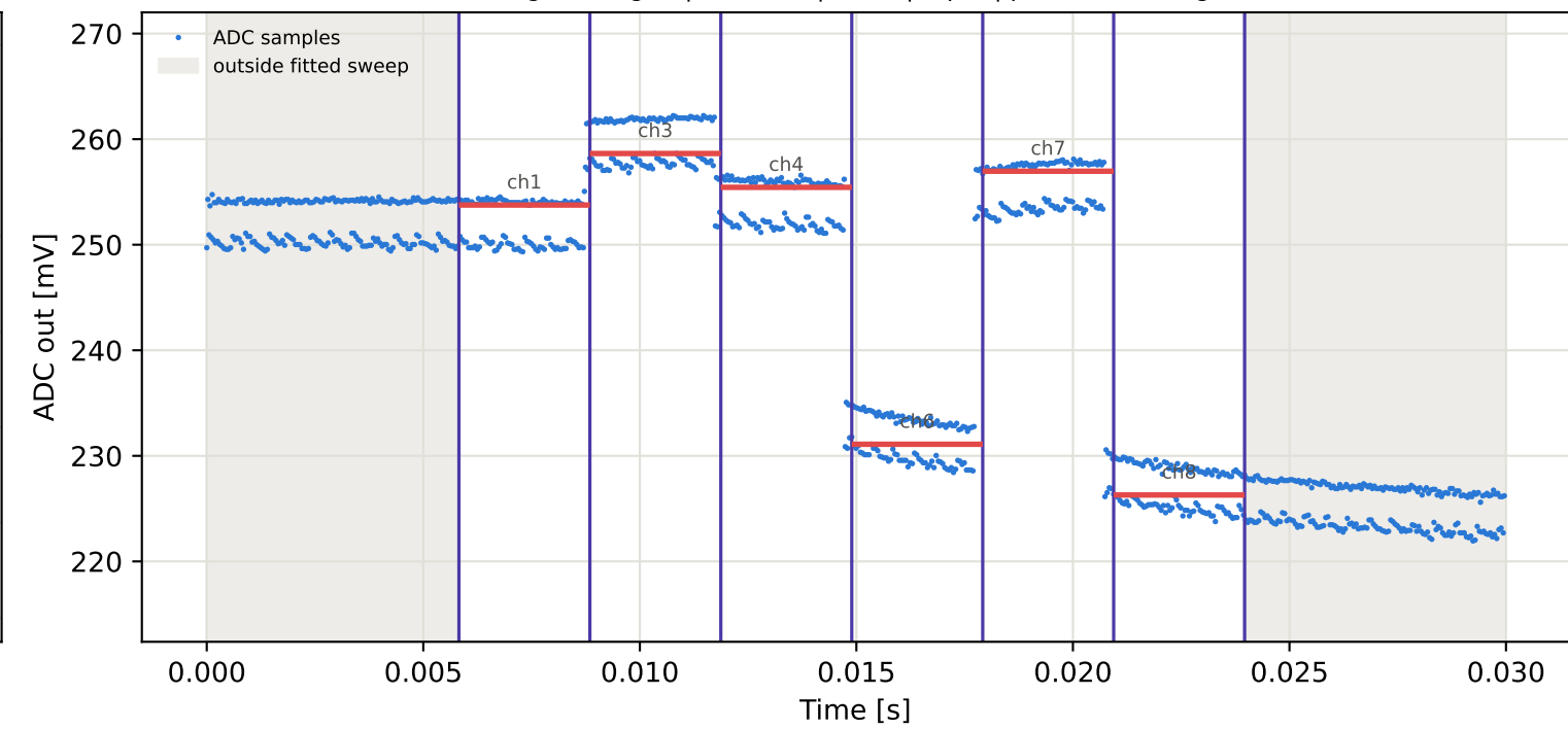
Tag4 &lt;- Tag16 | 875 MHz | run 0 | rep 1 | phase -65.72 deg
