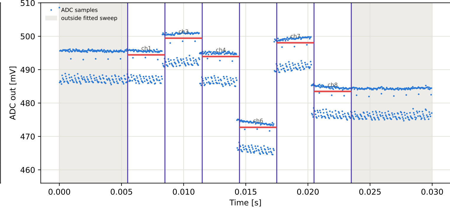
Tag3 &lt;- Tag9 | 955 MHz | run 0 | rep 1 | phase -129.12 deg
