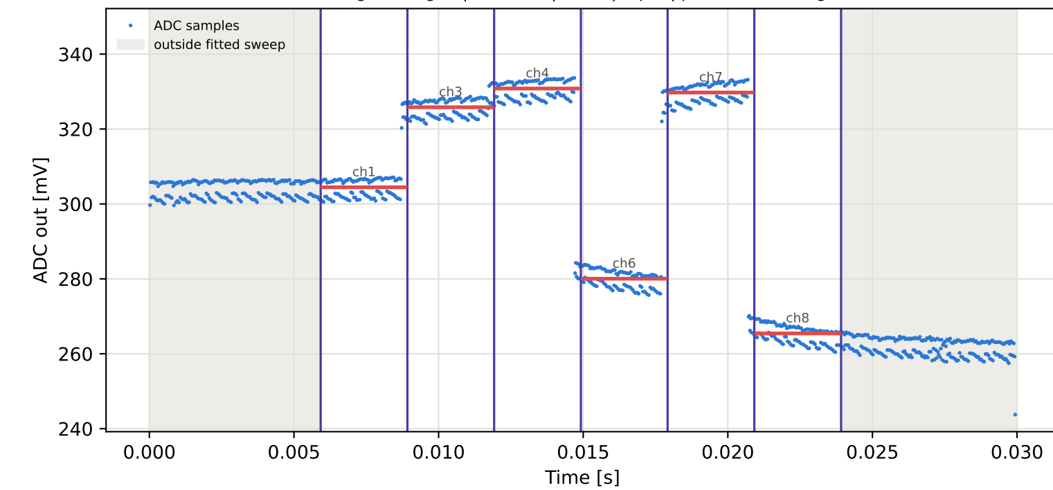
Tag9 &lt;- Tag16 | 895 MHz | run 0 | rep 1 | phase -86.14 deg
