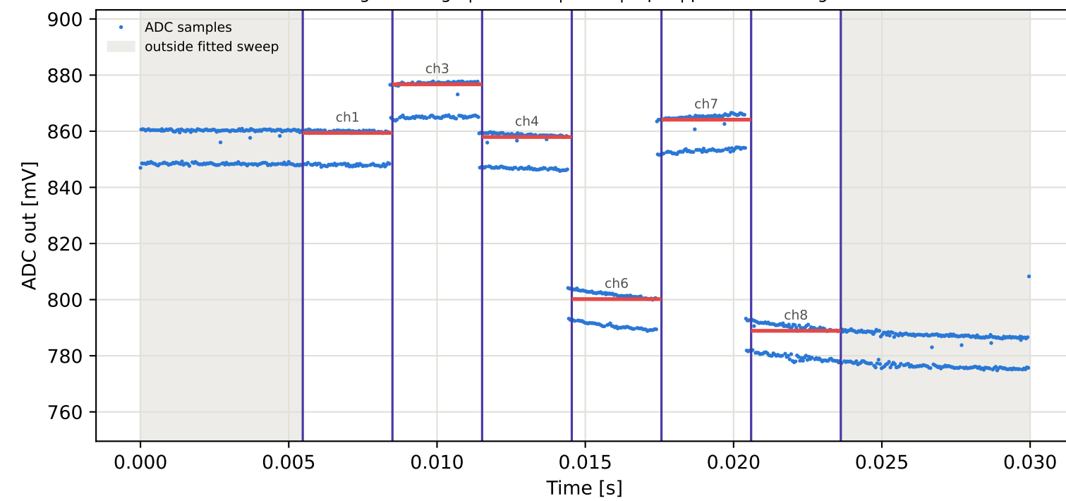
Tag10 &lt;- Tag8 | 875 MHz | run 0 | rep 1 | phase -147.46 deg
