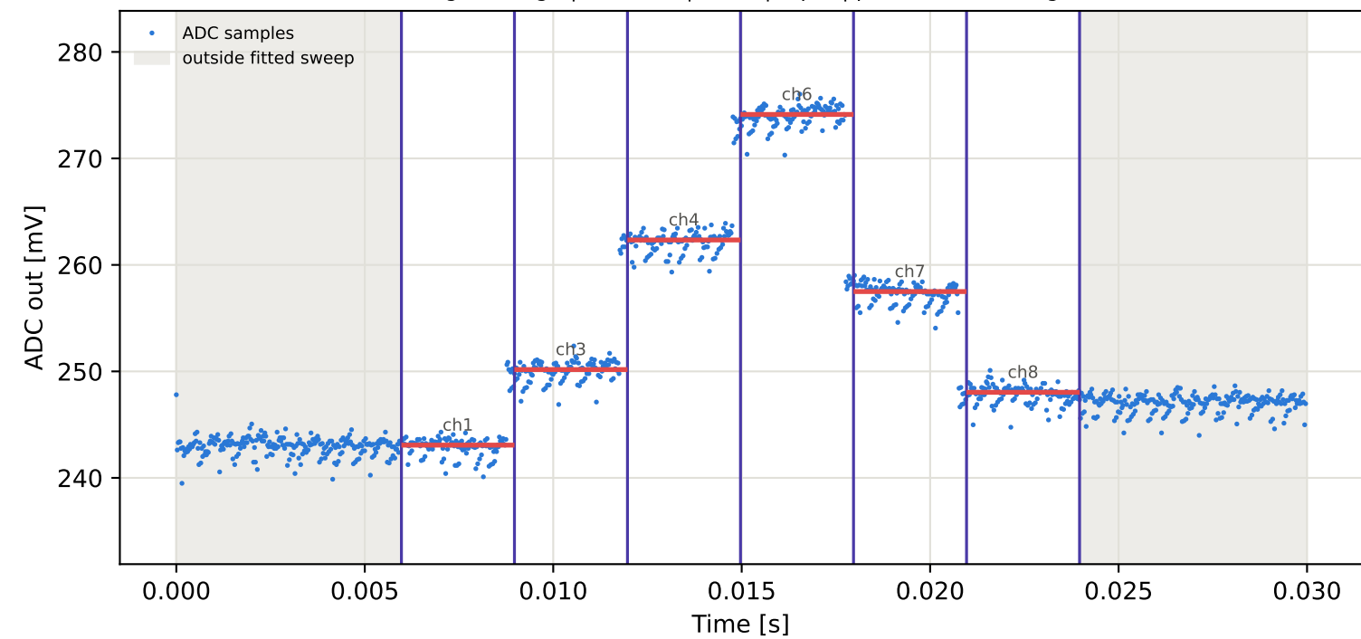
Tag7 &lt;- Tag1 | 915 MHz | run 0 | rep 1 | phase -16.76 deg
