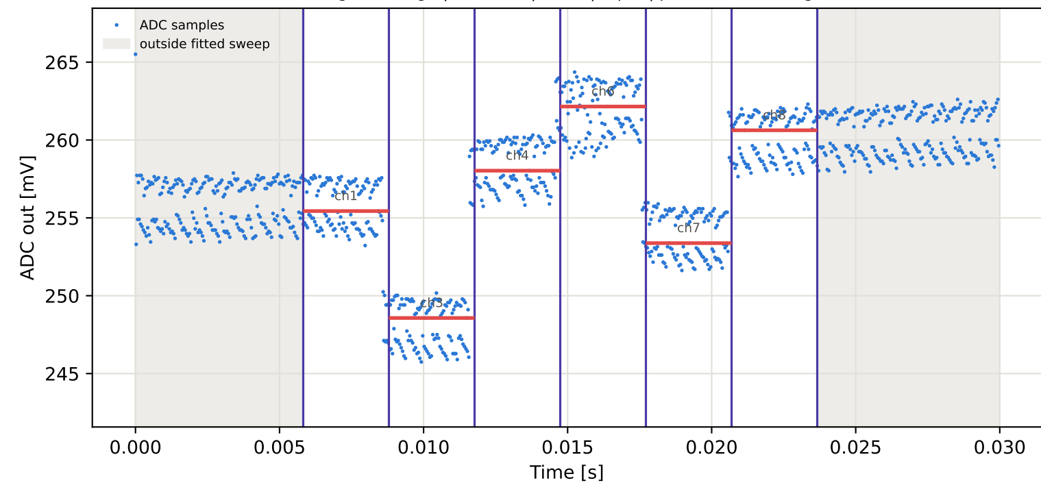
Tag16 &lt;- Tag1 | 805 MHz | run 0 | rep 1 | phase -93.26 deg
