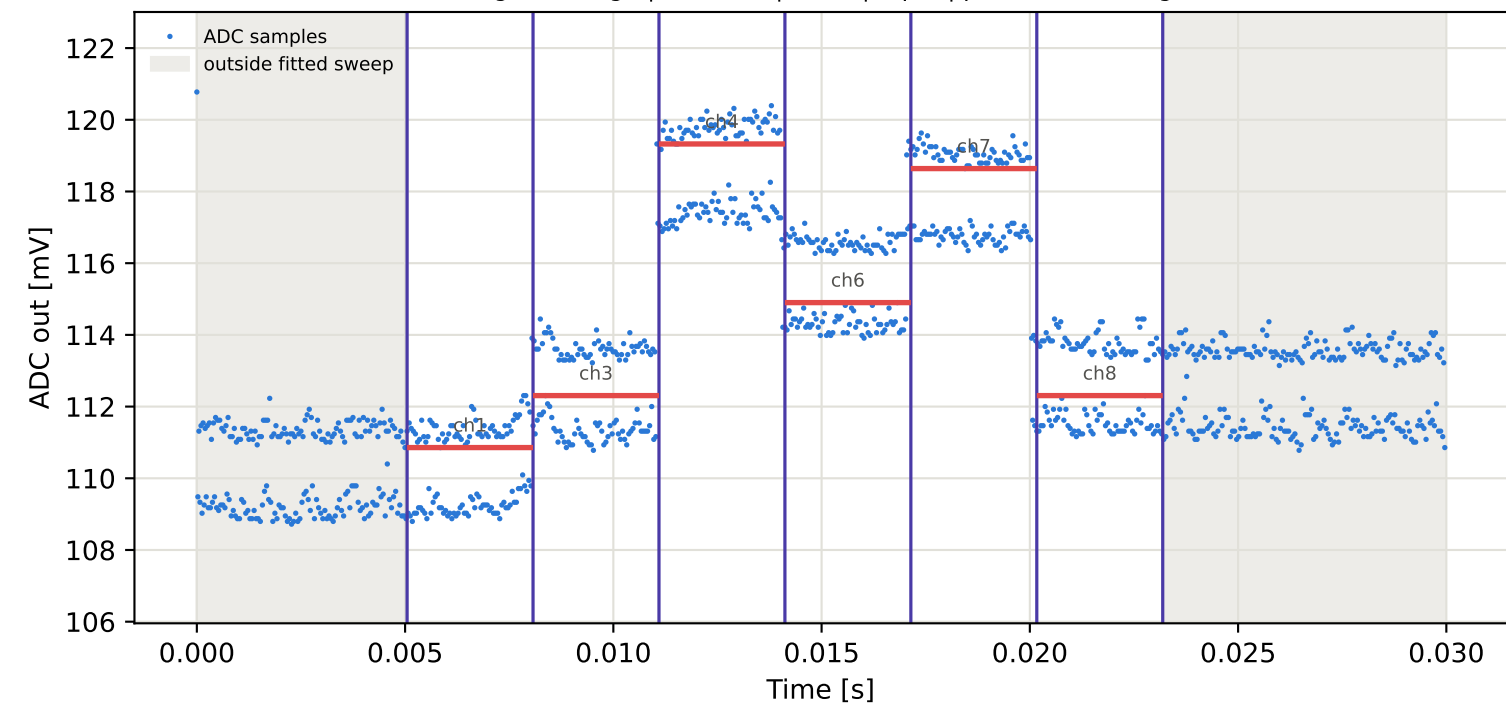
Tag10 &lt;- Tag9 | 785 MHz | run 0 | rep 1 | phase 166.09 deg
