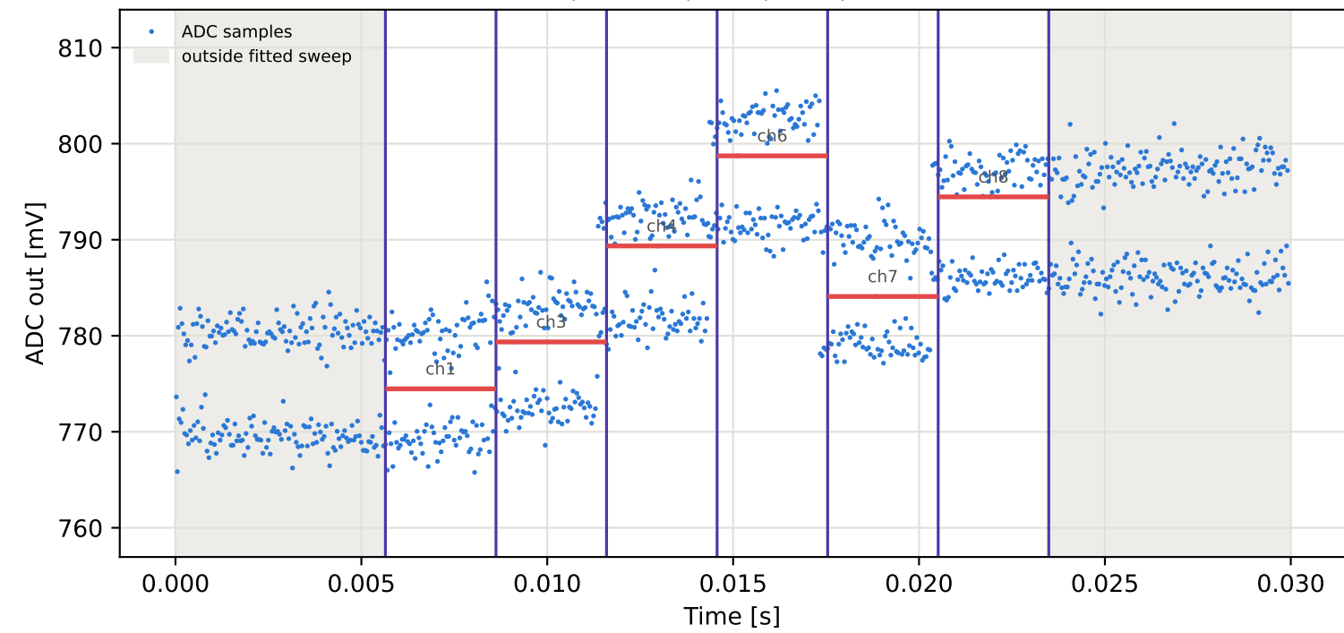
Tag7 &lt;- Tag15 | 885 MHz | run 0 | rep 1 | phase -147.73 deg
