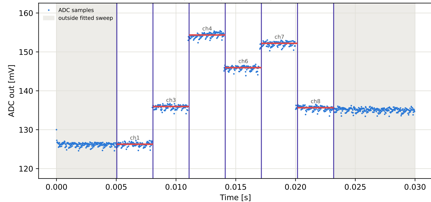
Tag8 &lt;- Tag7 | 795 MHz | run 0 | rep 1 | phase -98.75 deg
