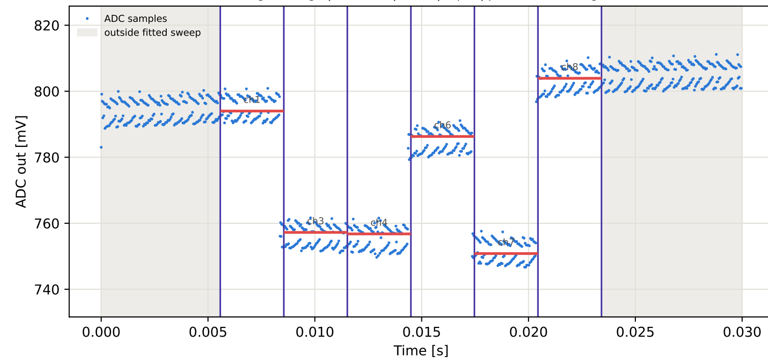
Tag8 &lt;- Tag1 | 865 MHz | run 0 | rep 1 | phase 128.20 deg
