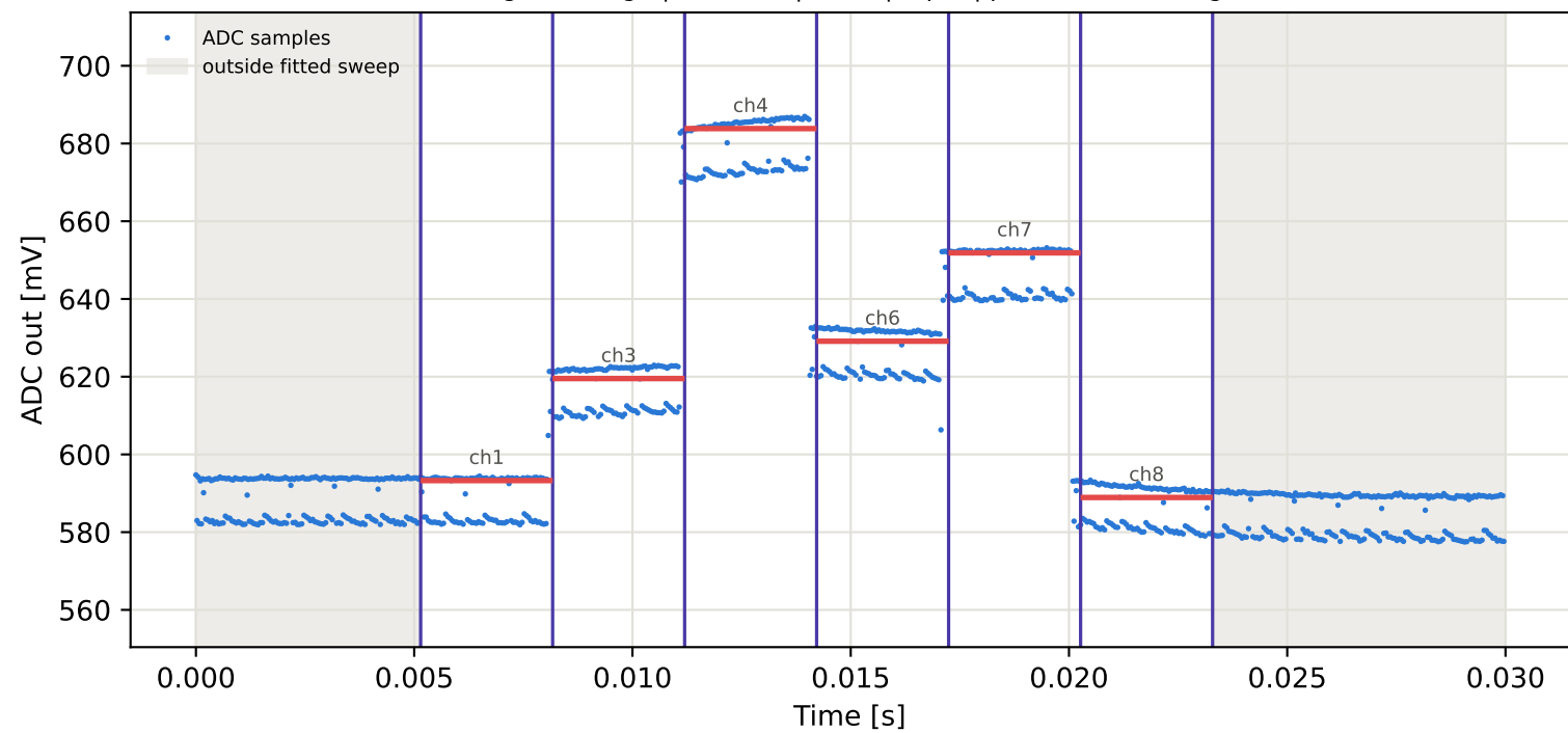
Tag16 &lt;- Tag5 | 965 MHz | run 0 | rep 1 | phase -43.72 deg
