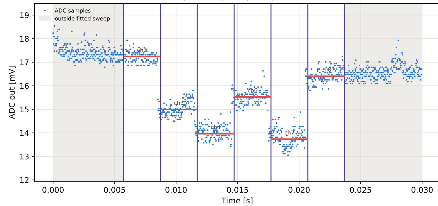
Tag1 &lt;- Tag7 | 835 MHz | run 0 | rep 1 | phase -59.73 deg
