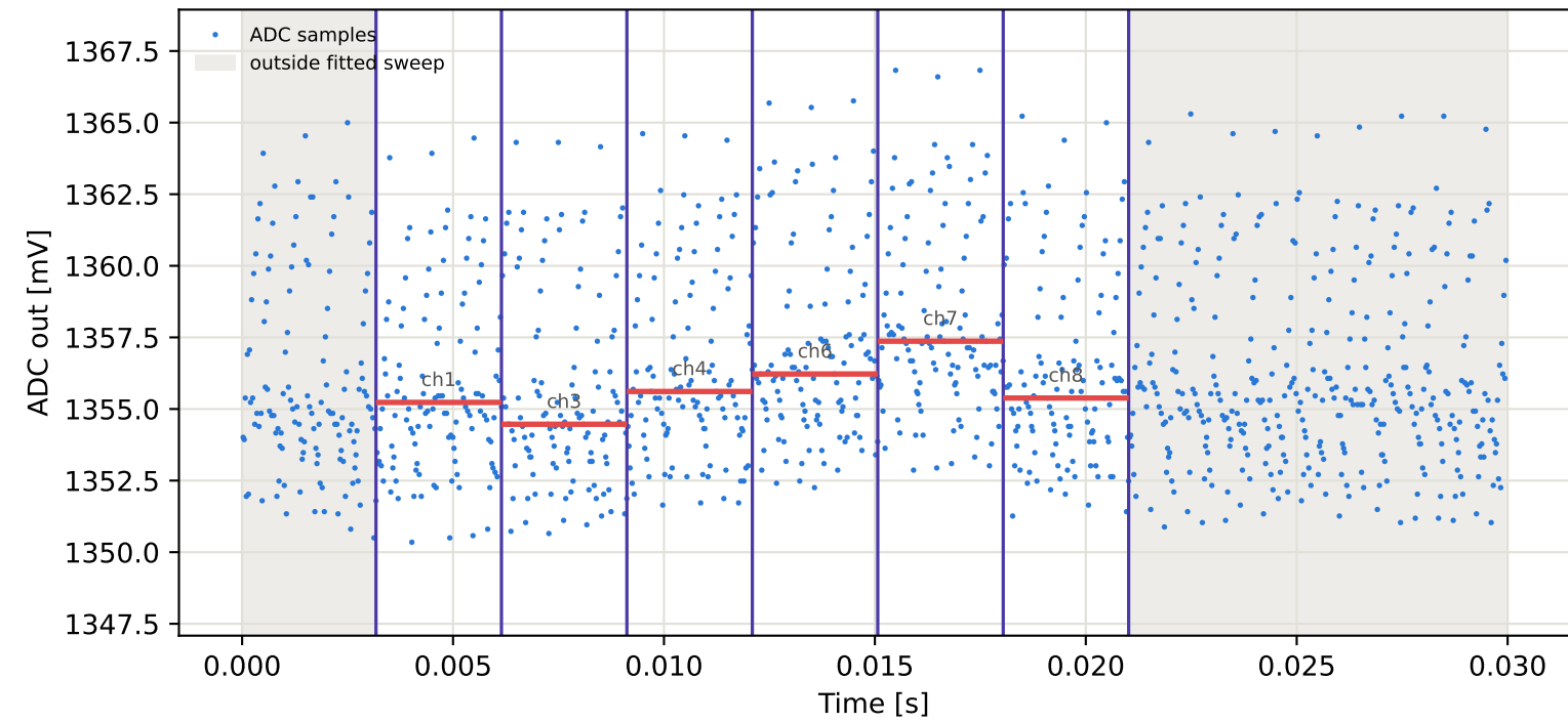
Tag2 &lt;- Tag8 | 935 MHz | run 0 | rep 1 | phase 106.98 deg
