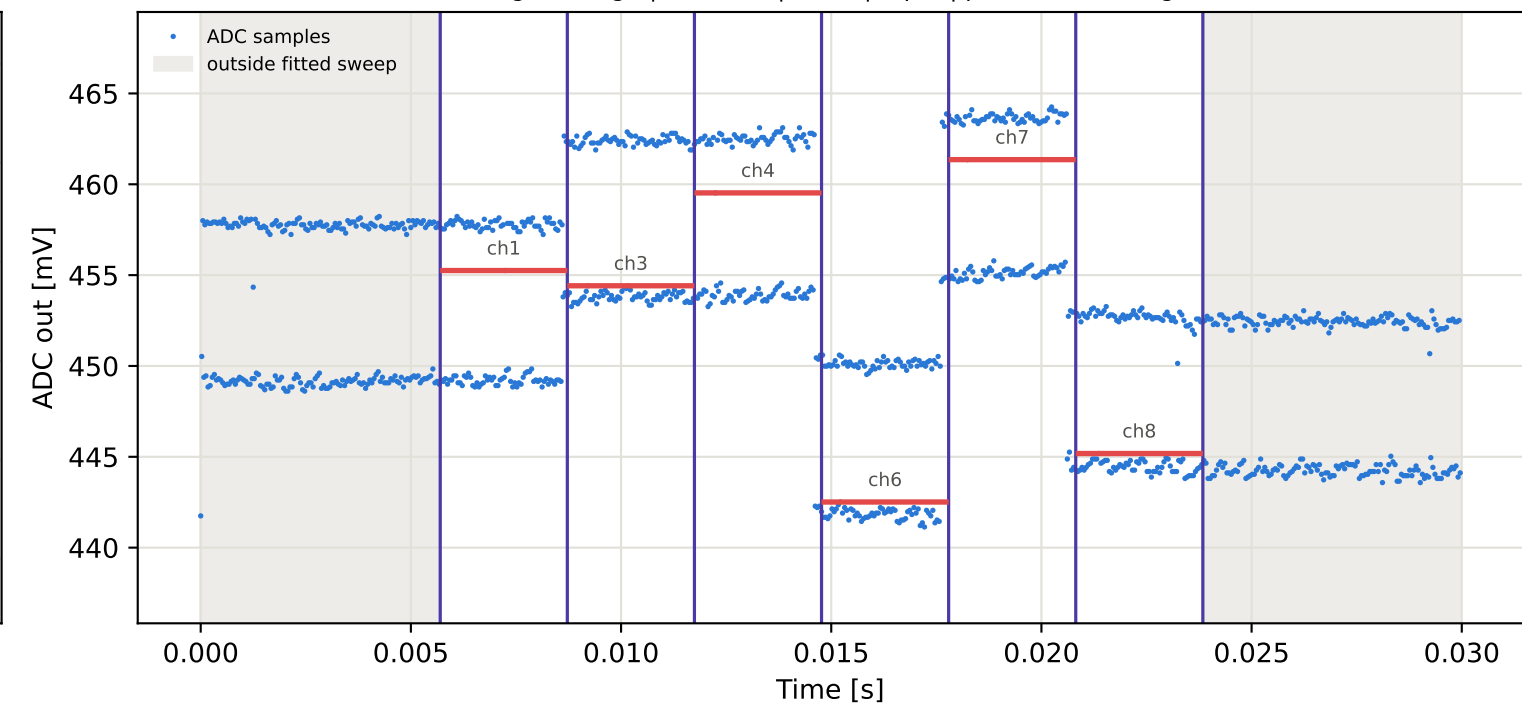
Tag8 &lt;- Tag10 | 995 MHz | run 0 | rep 1 | phase 55.07 deg
