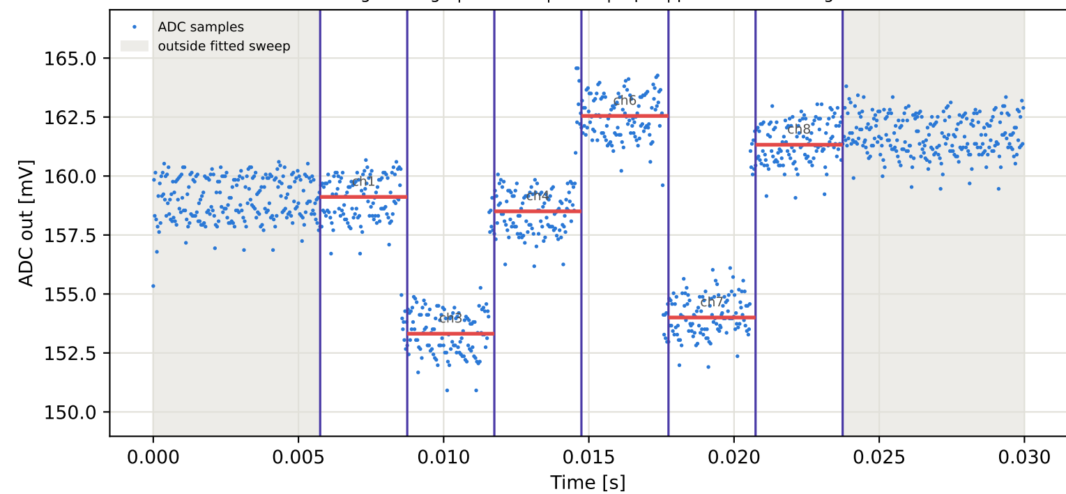
Tag7 &lt;- Tag1 | 775 MHz | run 0 | rep 1 | phase -75.16 deg
