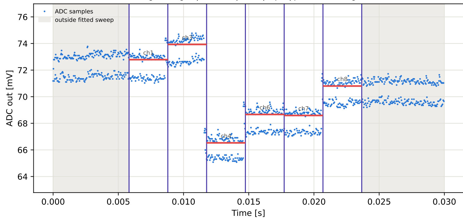
Tag1 &lt;- Tag3 | 795 MHz | run 0 | rep 1 | phase 48.43 deg
