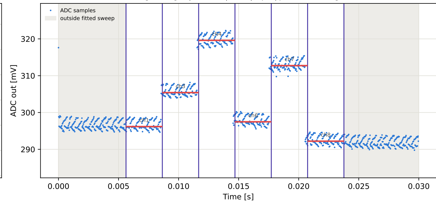
Tag5 &lt;- Tag2 | 975 MHz | run 0 | rep 1 | phase 167.09 deg
