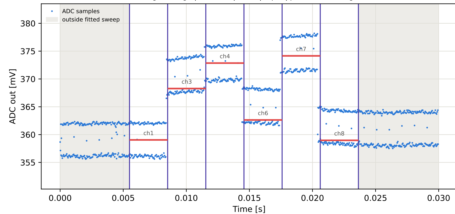
Tag7 &lt;- Tag5 | 825 MHz | run 0 | rep 1 | phase 23.76 deg
