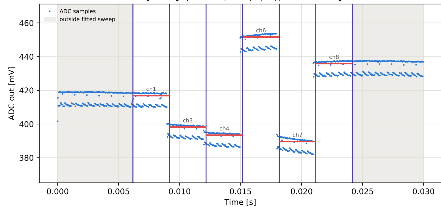
Tag9 &lt;- Tag15 | 975 MHz | run 0 | rep 1 | phase -13.16 deg
