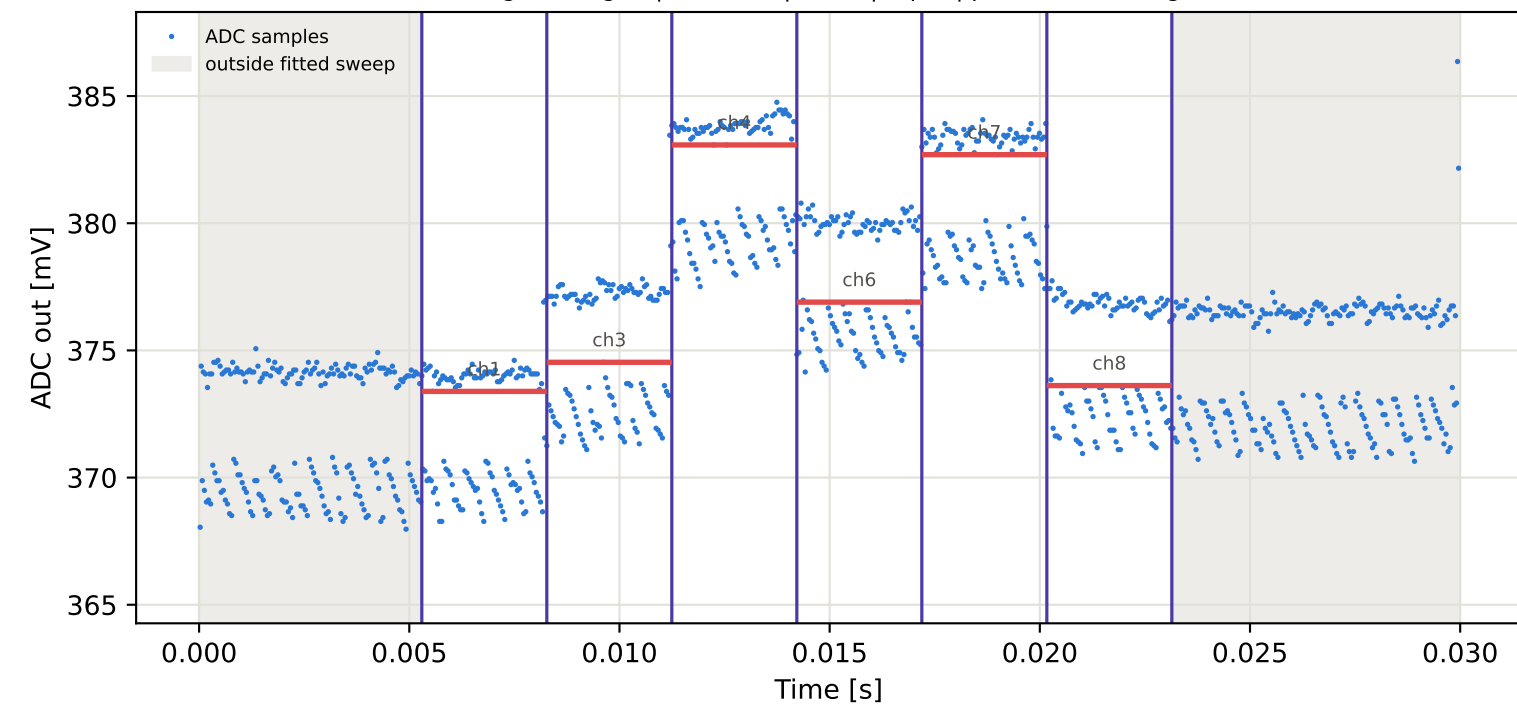
Tag6 &lt;- Tag2 | 825 MHz | run 0 | rep 1 | phase -140.33 deg
