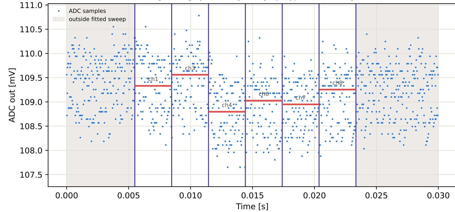
Tag2 &lt;- Tag6 | 795 MHz | run 0 | rep 1 | phase 103.38 deg
