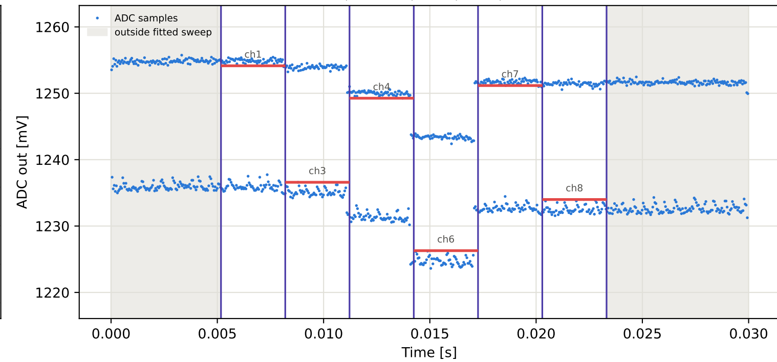
Tag15 &lt;- Tag6 | 915 MHz | run 0 | rep 1 | phase -9.59 deg
