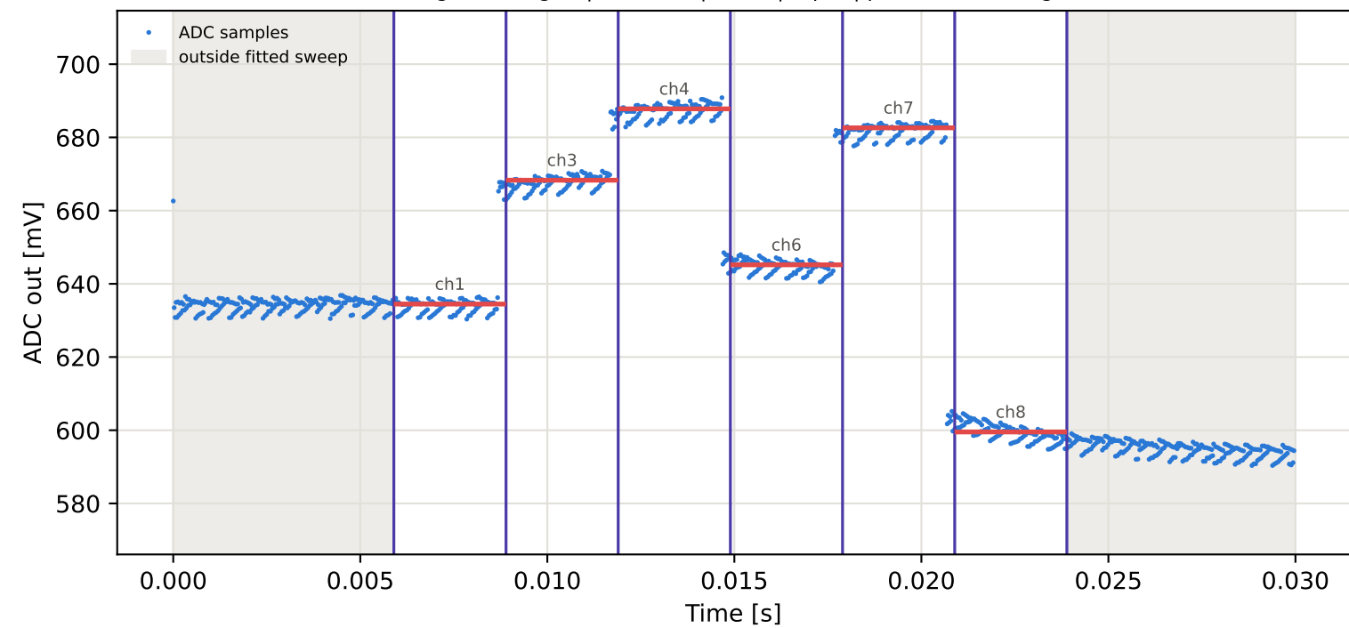
Tag10 &lt;- Tag3 | 905 MHz | run 0 | rep 1 | phase 24.05 deg
