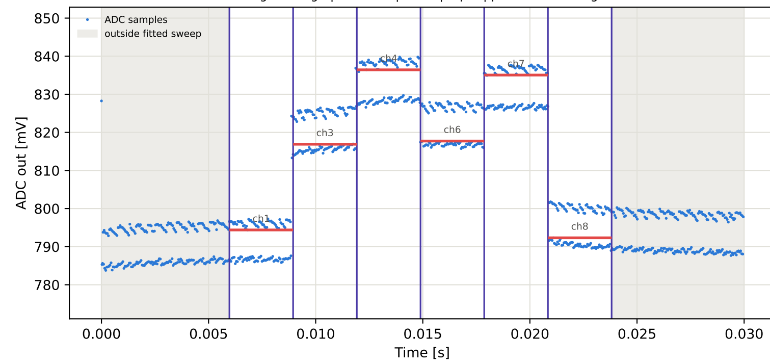
Tag2 &lt;- Tag5 | 865 MHz | run 0 | rep 1 | phase -139.09 deg
