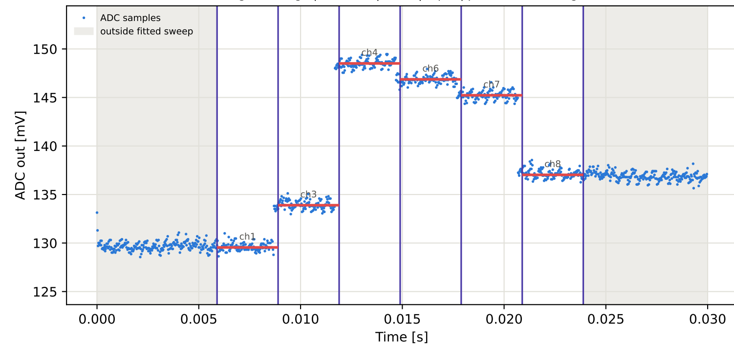
Tag16 &lt;- Tag4 | 775 MHz | run 0 | rep 1 | phase 3.83 deg
