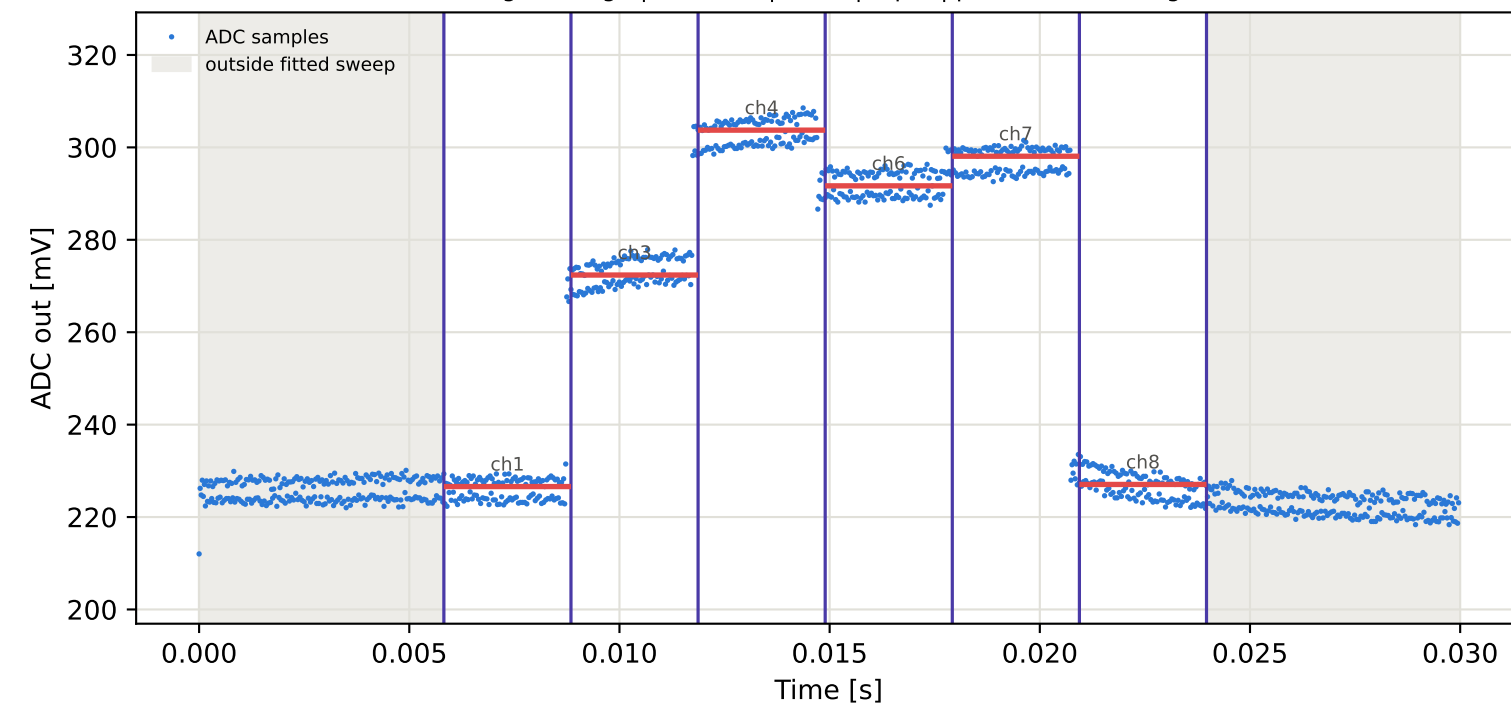
Tag9 &lt;- Tag7 | 885 MHz | run 0 | rep 1 | phase -65.82 deg
