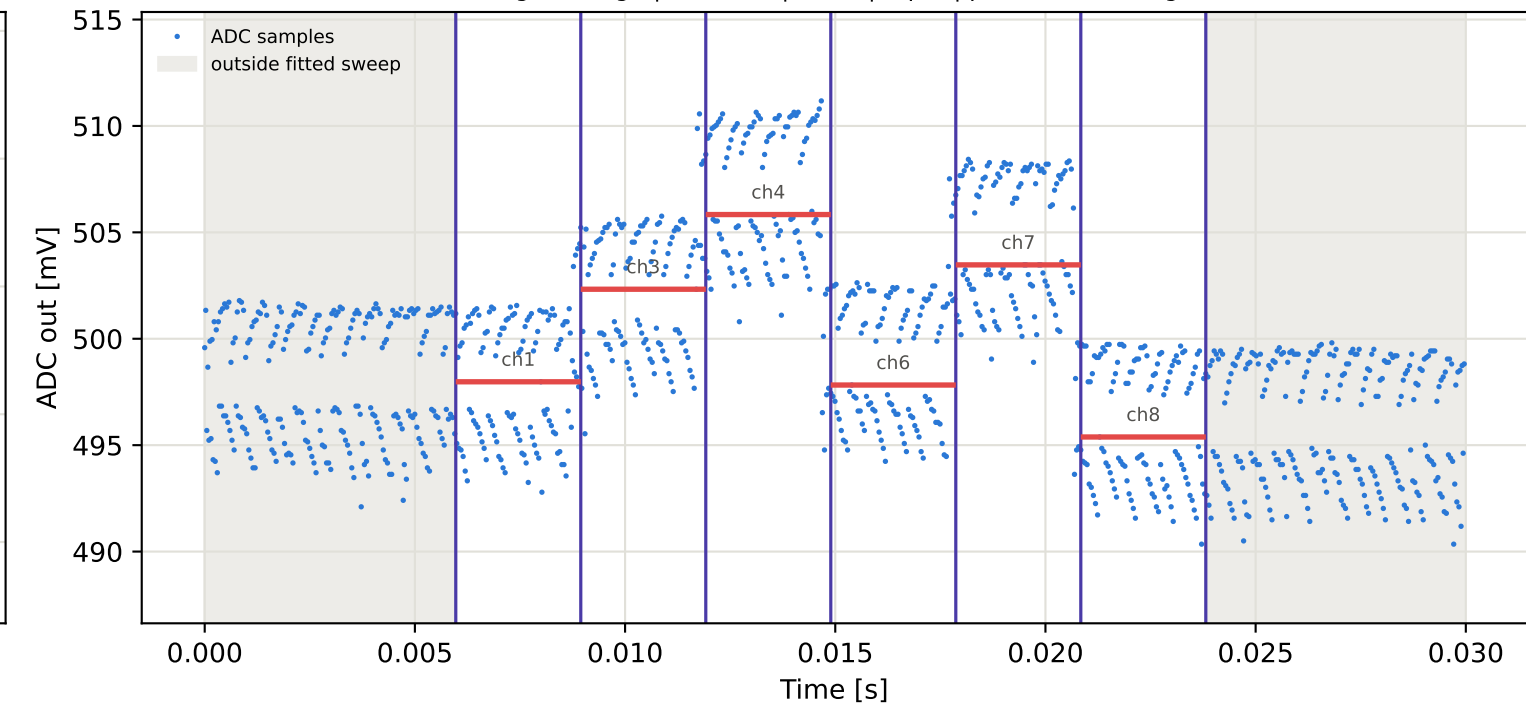
Tag5 &lt;- Tag9 | 945 MHz | run 0 | rep 1 | phase -24.49 deg
