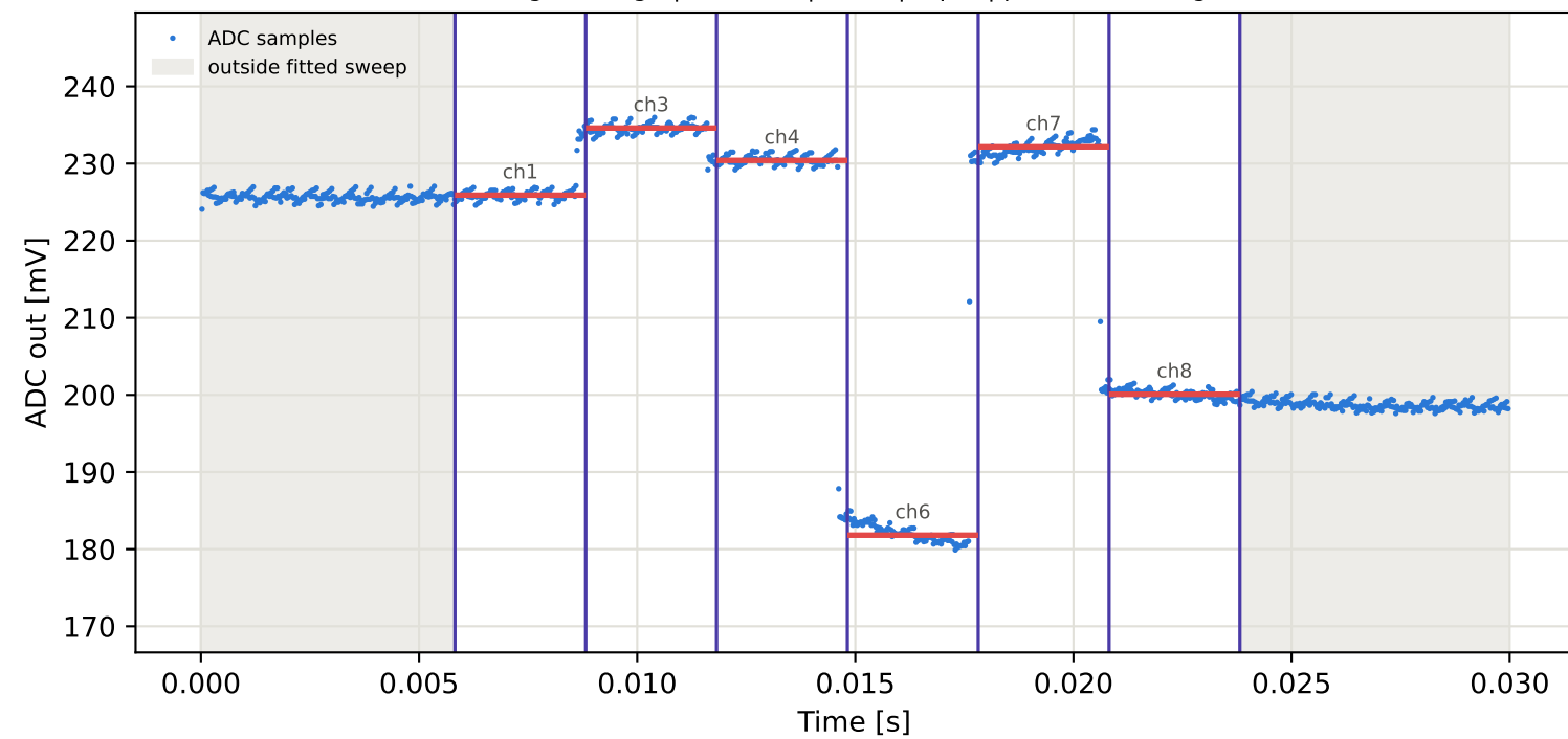
Tag9 &lt;- Tag6 | 915 MHz | run 0 | rep 1 | phase -11.83 deg
