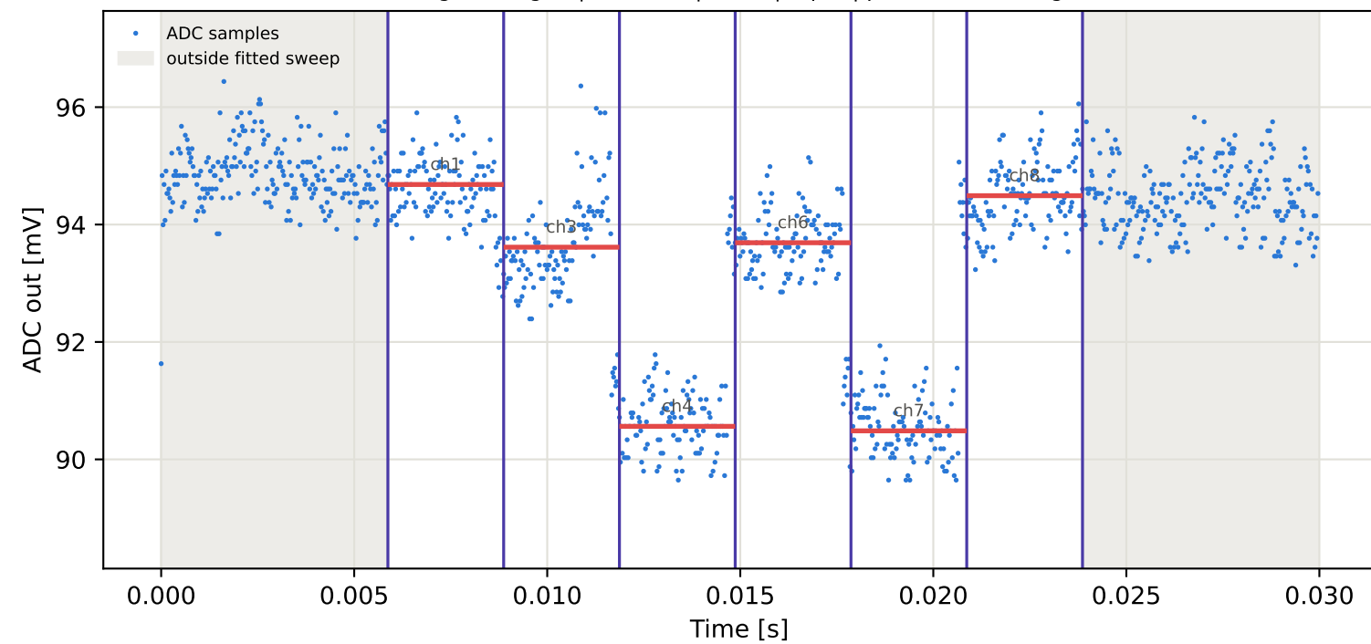
Tag6 &lt;- Tag3 | 785 MHz | run 0 | rep 1 | phase 138.74 deg
