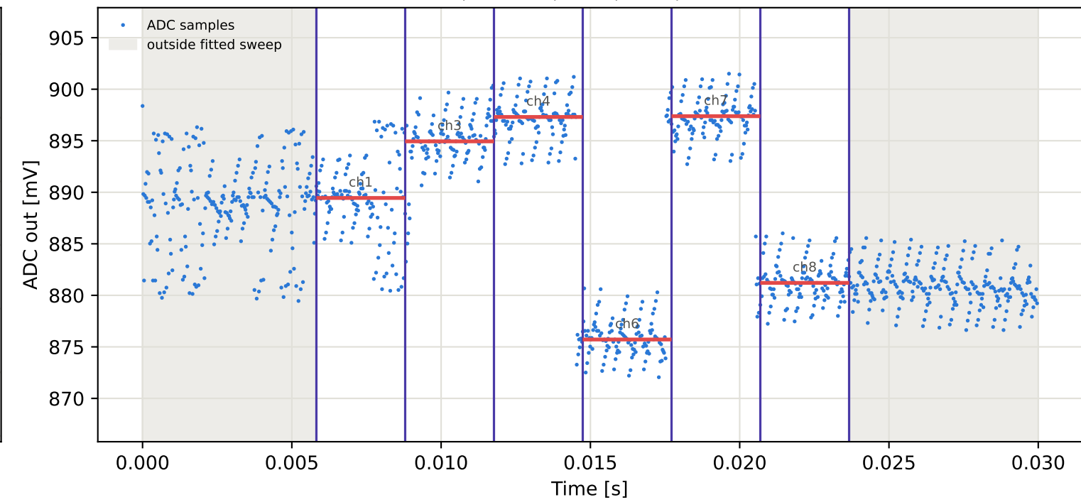
Tag7 &lt;- Tag6 | 925 MHz | run 0 | rep 1 | phase -23.95 deg
