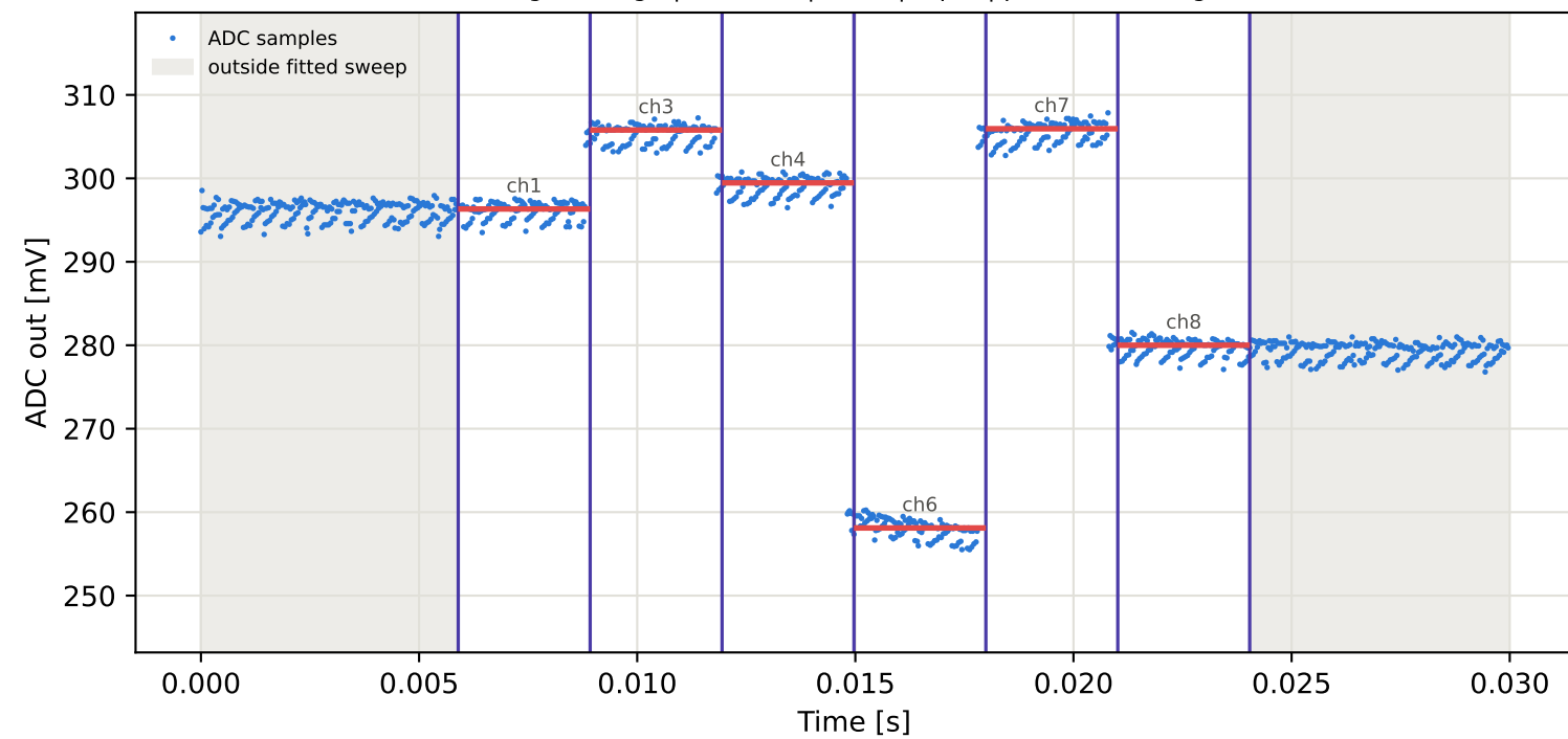
Tag8 &lt;- Tag5 | 985 MHz | run 0 | rep 1 | phase -170.33 deg
