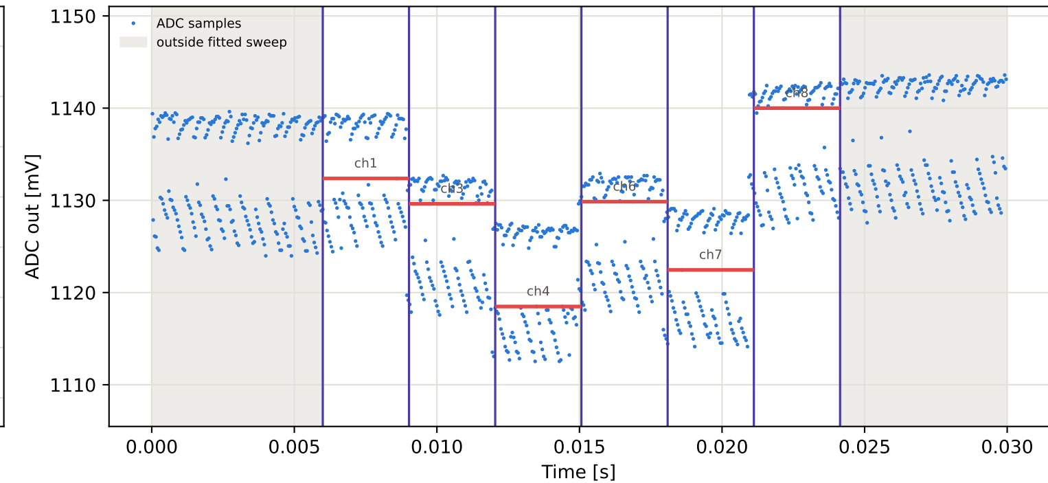
Tag7 &lt;- Tag6 | 895 MHz | run 0 | rep 1 | phase -150.16 deg
