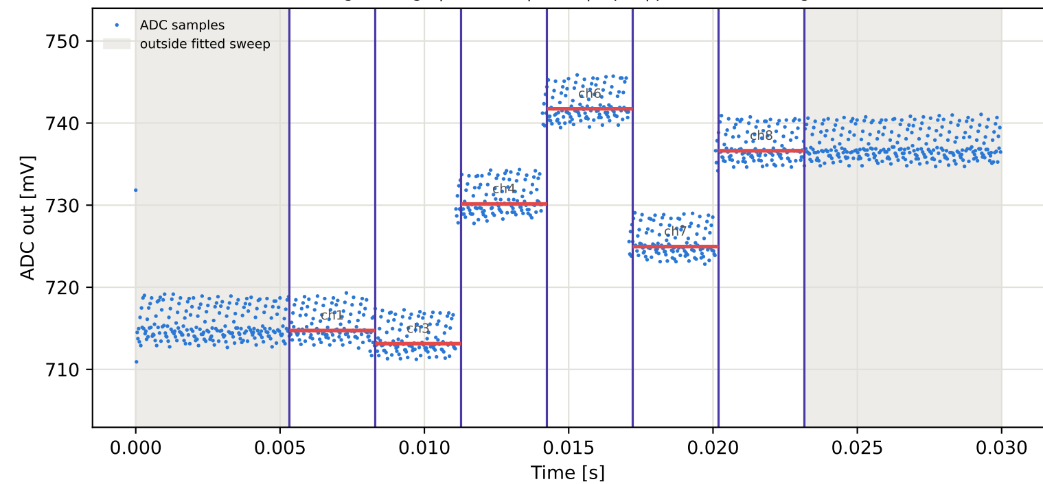
Tag3 &lt;- Tag7 | 855 MHz | run 0 | rep 1 | phase -125.64 deg
