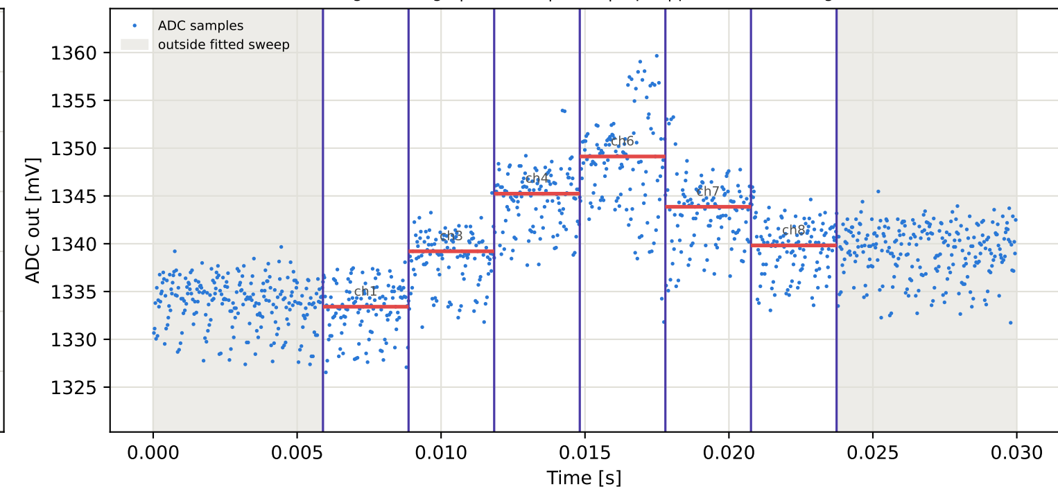
Tag15 &lt;- Tag6 | 885 MHz | run 0 | rep 1 | phase -122.80 deg
