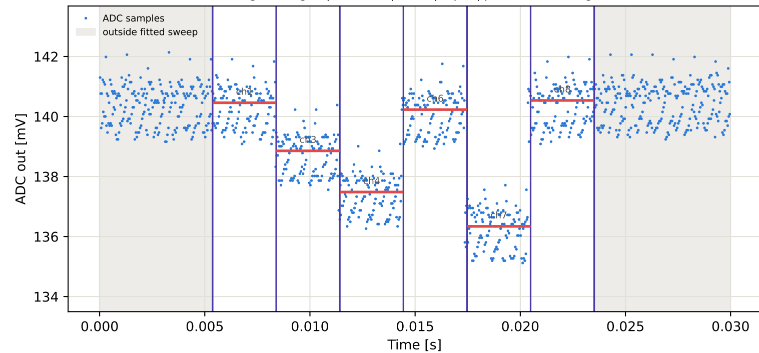
Tag5 &lt;- Tag16 | 775 MHz | run 0 | rep 1 | phase -94.20 deg
