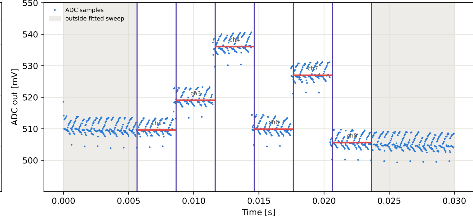
Tag9 &lt;- Tag8 | 985 MHz | run 0 | rep 1 | phase -84.87 deg
