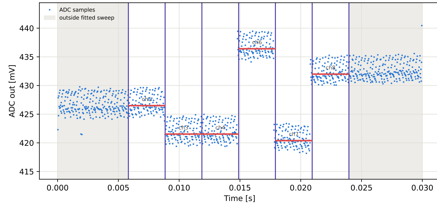
Tag3 &lt;- Tag8 | 985 MHz | run 0 | rep 1 | phase -34.68 deg
