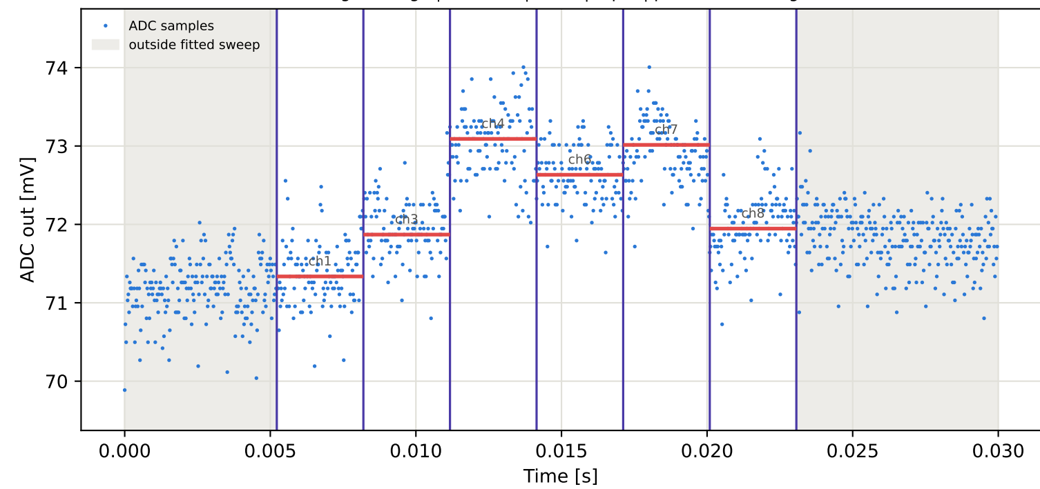
Tag3 &lt;- Tag2 | 785 MHz | run 0 | rep 1 | phase -99.16 deg
