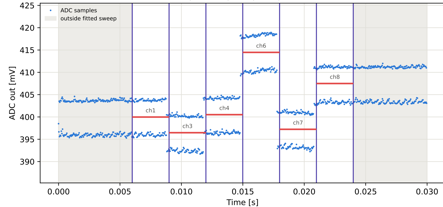
Tag2 &lt;- Tag15 | 985 MHz | run 0 | rep 1 | phase -179.54 deg
