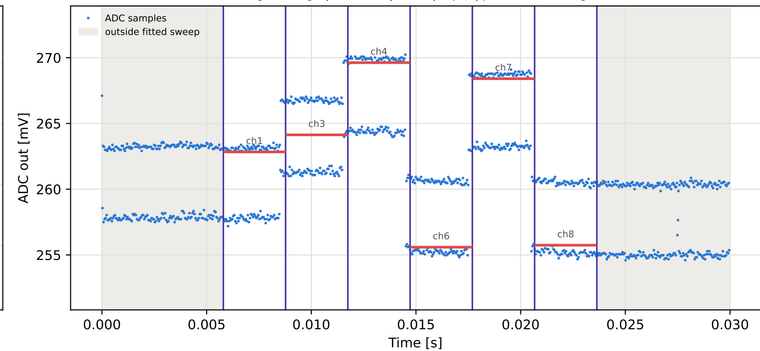
Tag5 &lt;- Tag9 | 965 MHz | run 0 | rep 1 | phase -13.78 deg
