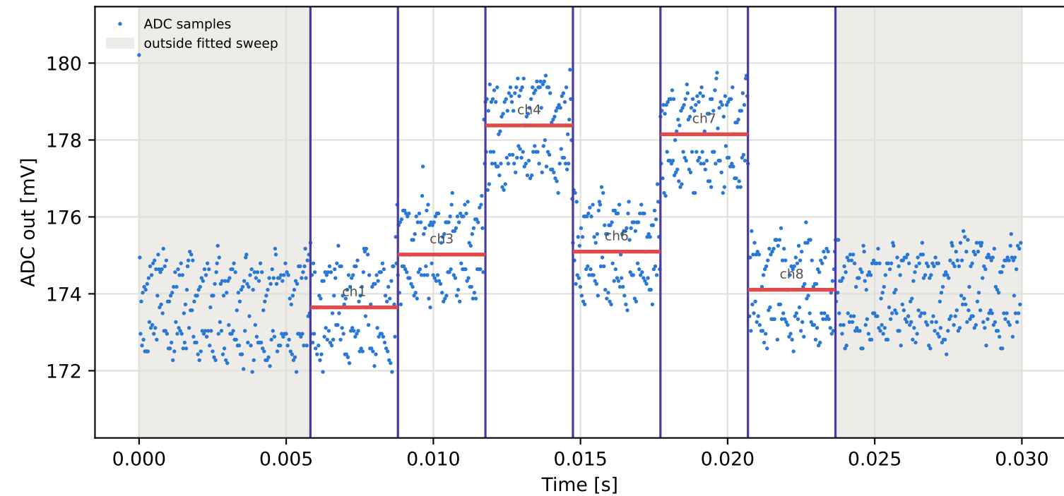
Tag16 &lt;- Tag7 | 785 MHz | run 0 | rep 1 | phase -8.85 deg
