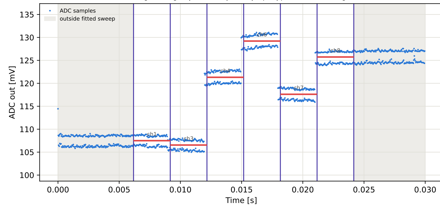
Tag1 &lt;- Tag3 | 855 MHz | run 0 | rep 1 | phase 140.23 deg
