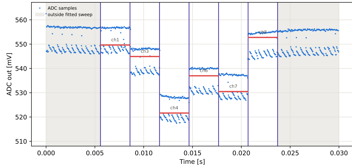
Tag10 &lt;- Tag9 | 945 MHz | run 0 | rep 1 | phase -32.23 deg
