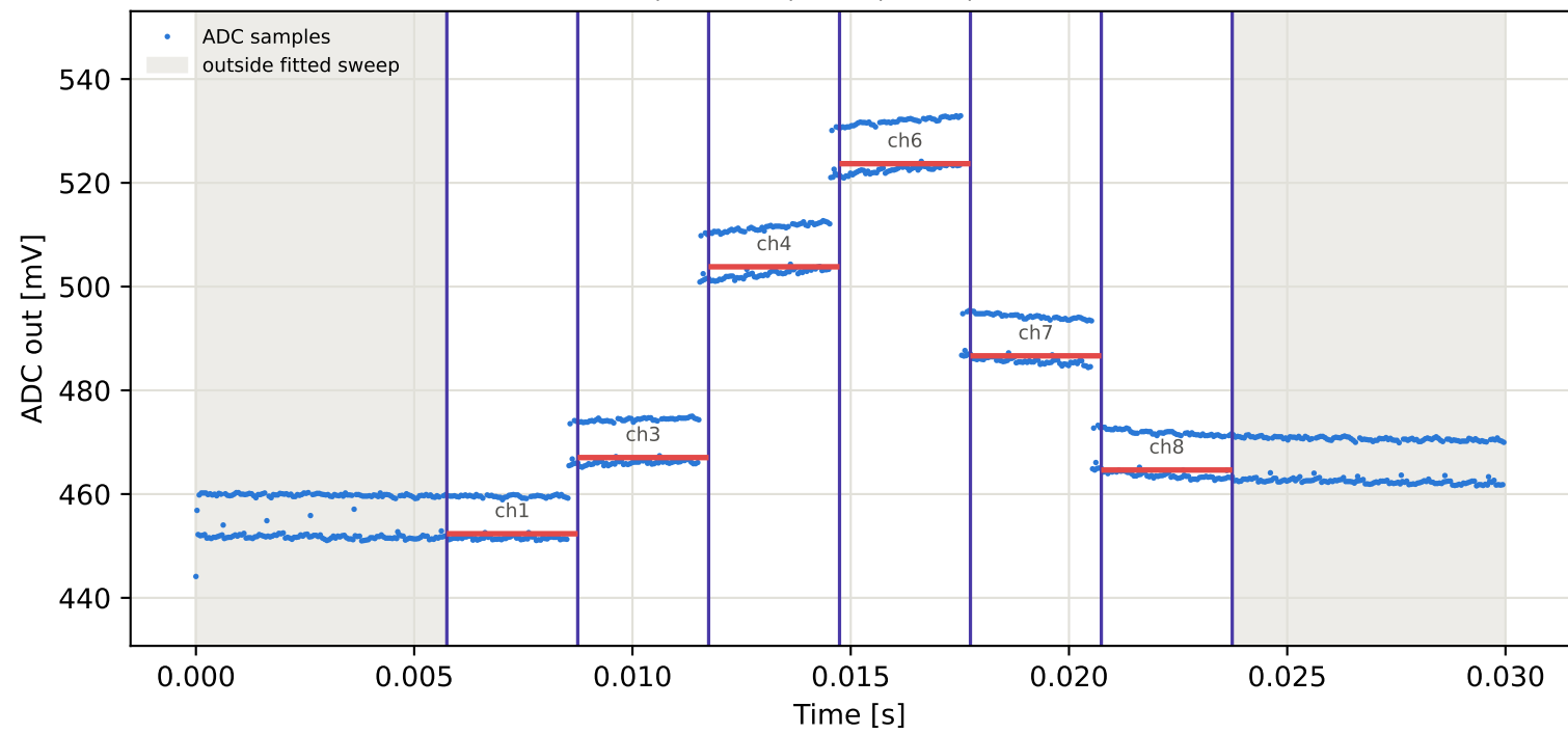
Tag9 &lt;- Tag8 | 935 MHz | run 0 | rep 1 | phase -135.91 deg
