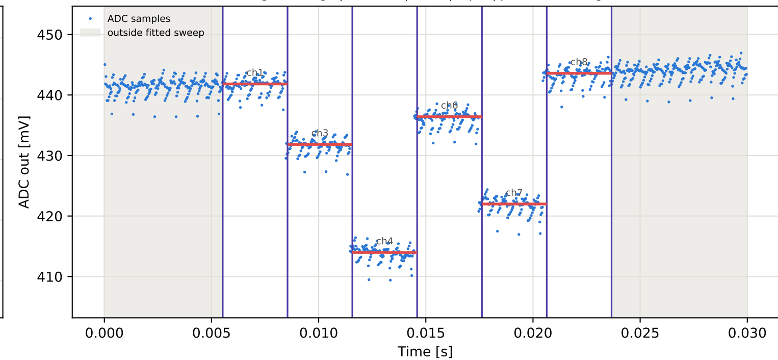
Tag10 &lt;- Tag9 | 965 MHz | run 0 | rep 1 | phase 21.24 deg
