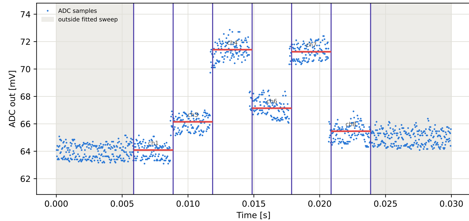
Tag10 &lt;- Tag9 | 775 MHz | run 0 | rep 1 | phase 141.67 deg
