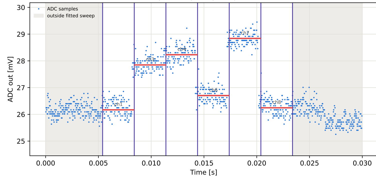
Tag1 &lt;- Tag3 | 805 MHz | run 0 | rep 1 | phase -55.11 deg
