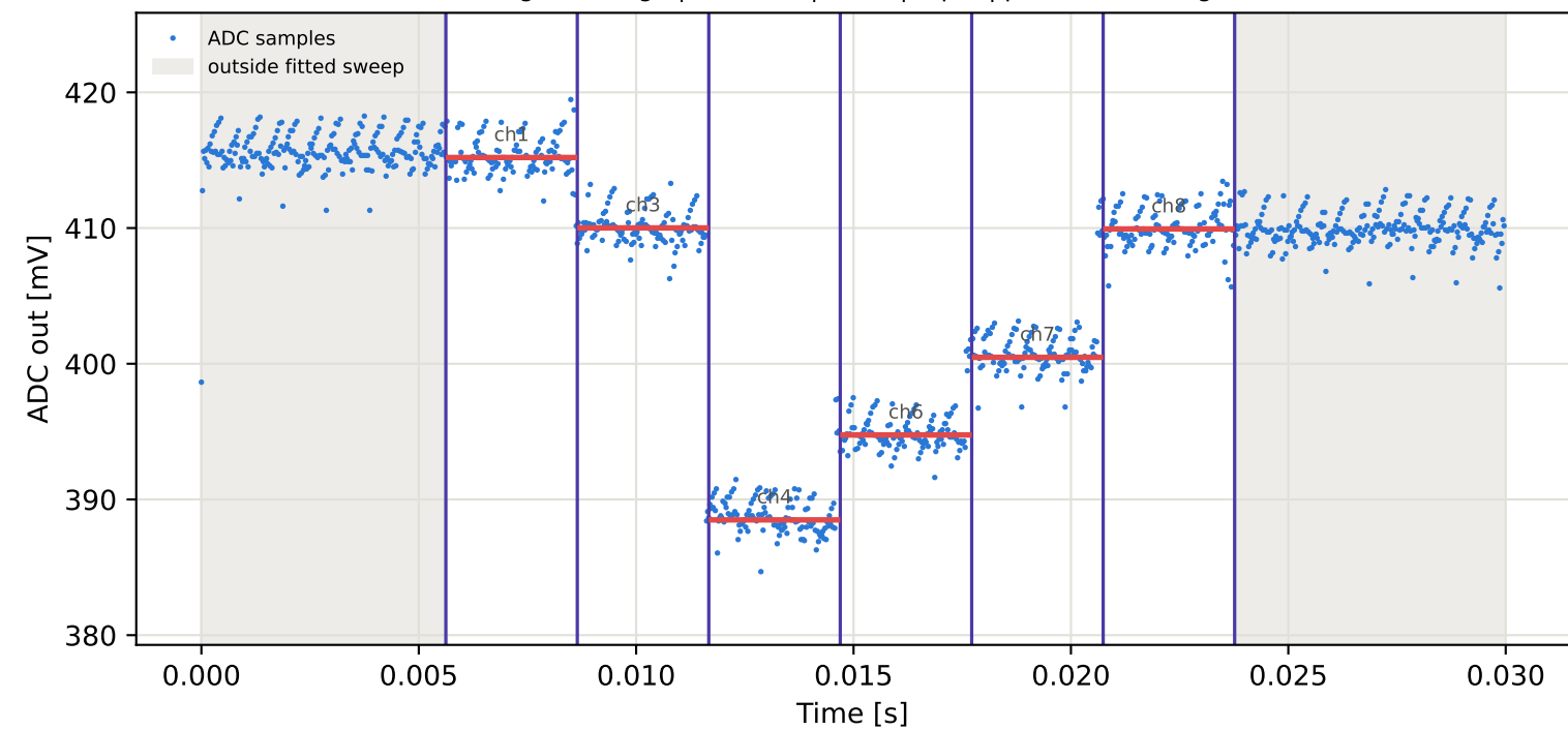
Tag10 &lt;- Tag5 | 975 MHz | run 0 | rep 1 | phase 88.18 deg
