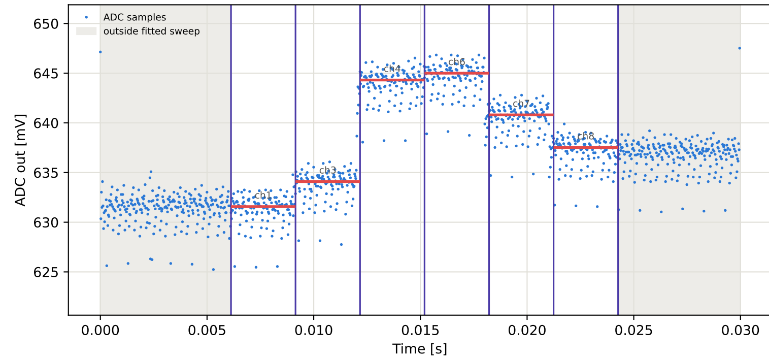
Tag3 &lt;- Tag9 | 835 MHz | run 0 | rep 1 | phase 112.51 deg
