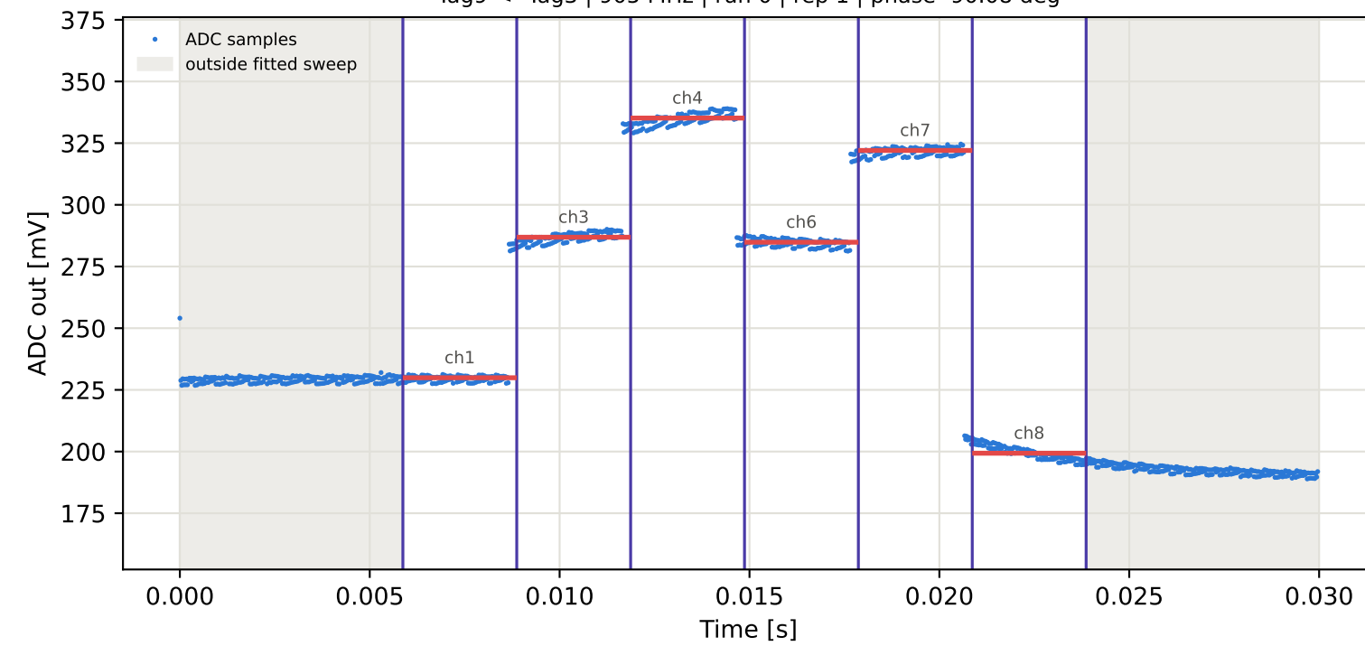
Tag9 &lt;- Tag5 | 905 MHz | run 0 | rep 1 | phase -93.83 deg
