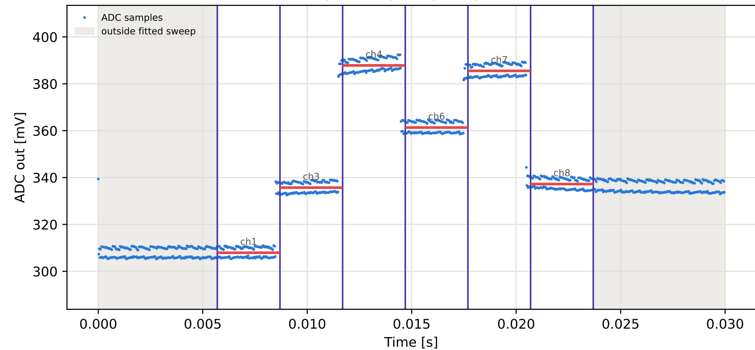
Tag8 &lt;- Tag16 | 825 MHz | run 0 | rep 1 | phase -98.61 deg
