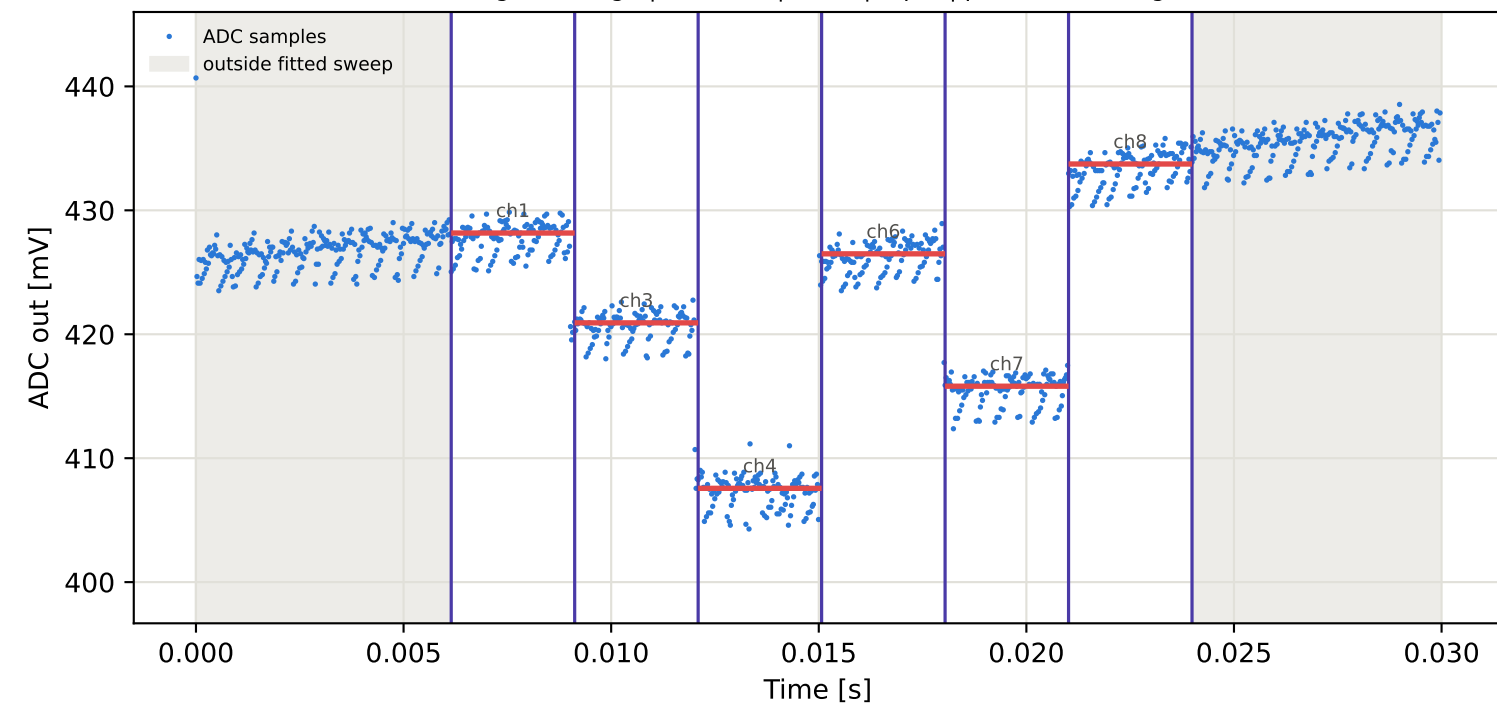
Tag10 &lt;- Tag9 | 975 MHz | run 0 | rep 1 | phase 57.64 deg
