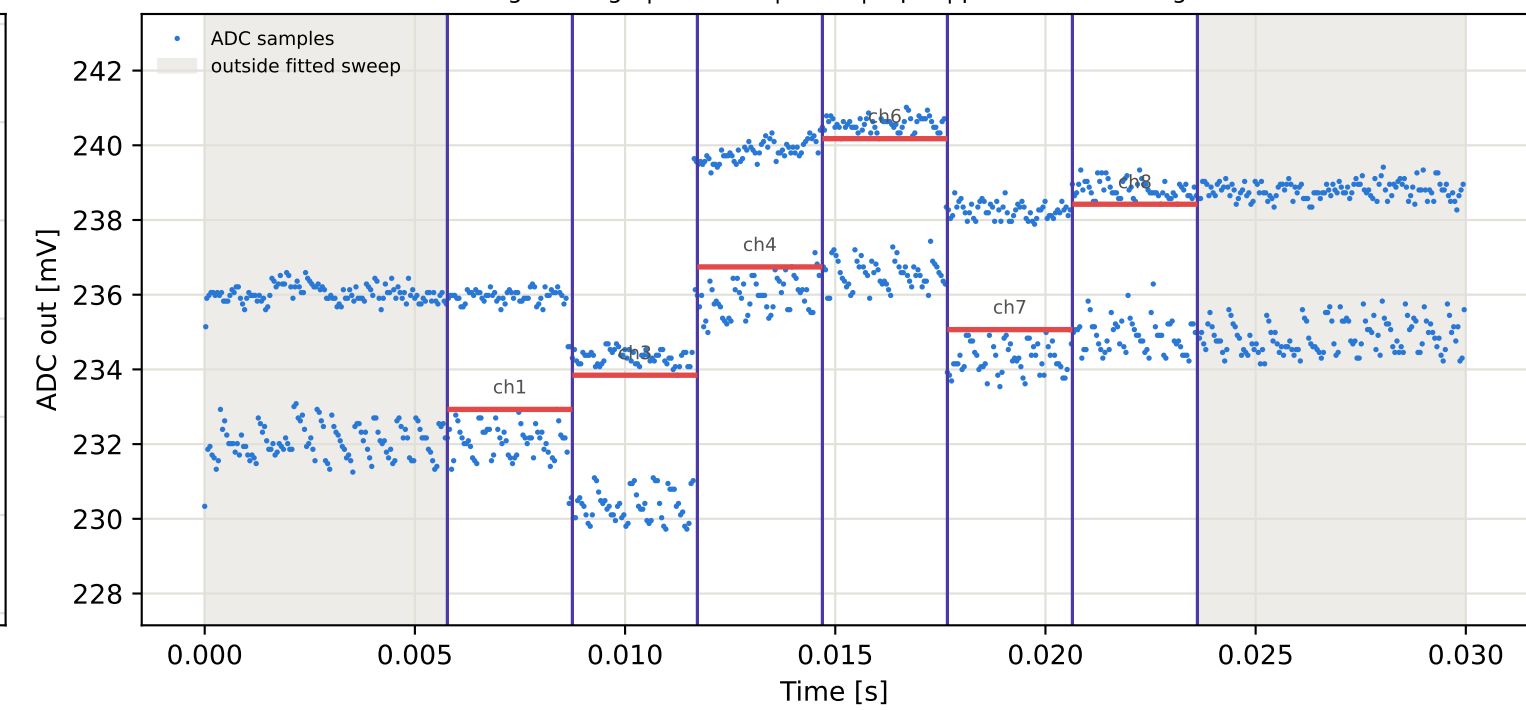
Tag9 &lt;- Tag15 | 845 MHz | run 0 | rep 1 | phase -130.66 deg
