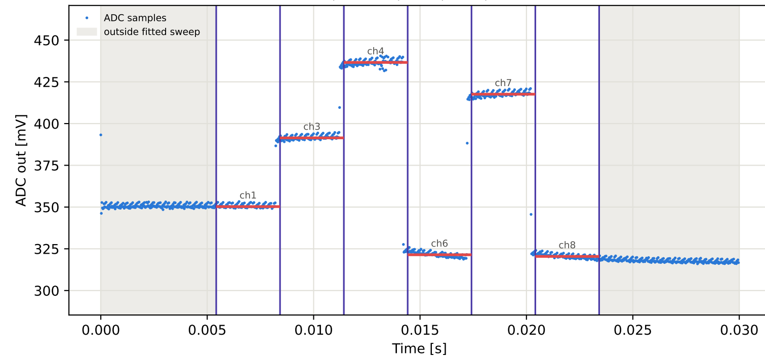
Tag3 &lt;- Tag16 | 965 MHz | run 0 | rep 1 | phase -59.60 deg
