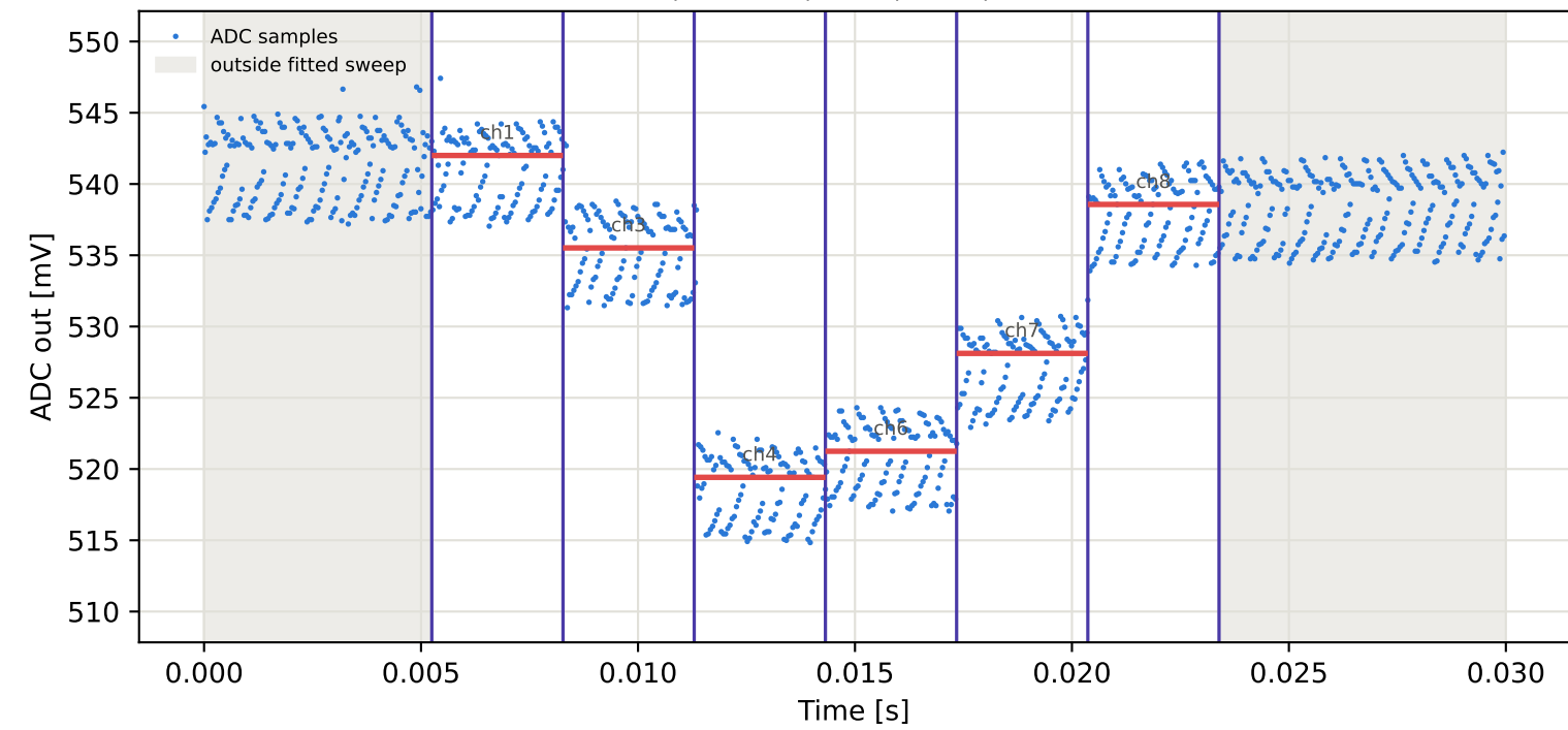
Tag4 &lt;- Tag3 | 945 MHz | run 0 | rep 1 | phase 53.88 deg
