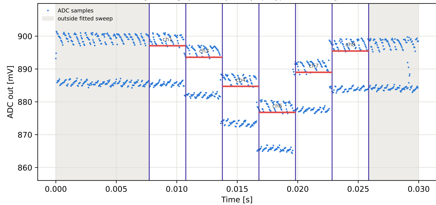
Tag15 &lt;- Tag4 | 965 MHz | run 0 | rep 1 | phase 167.64 deg
