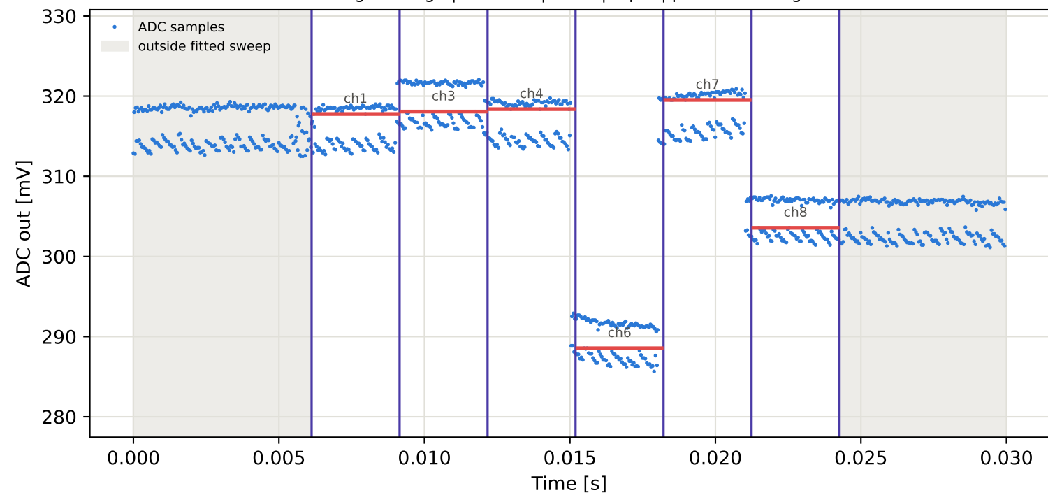
Tag8 &lt;- Tag4 | 845 MHz | run 0 | rep 1 | phase 57.73 deg
