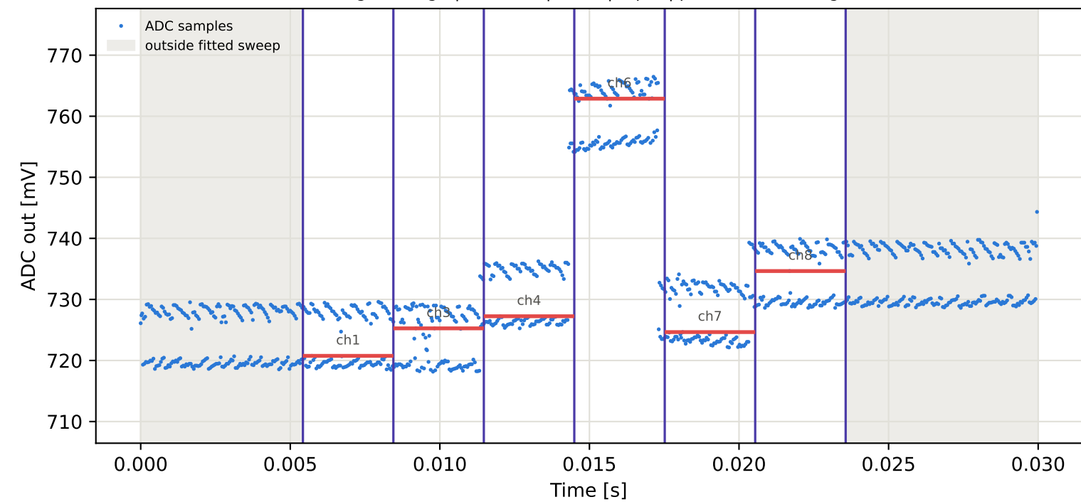
Tag7 &lt;- Tag4 | 855 MHz | run 0 | rep 1 | phase -89.30 deg
