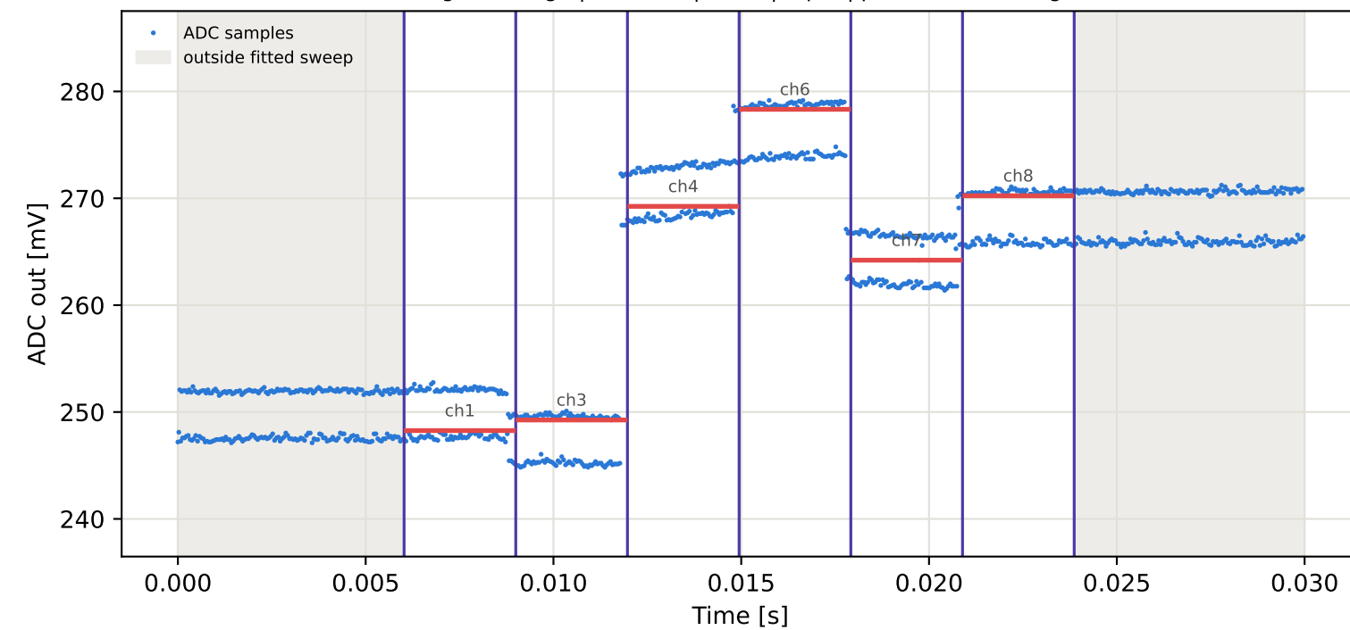
Tag15 &lt;- Tag1 | 835 MHz | run 0 | rep 1 | phase 23.50 deg
