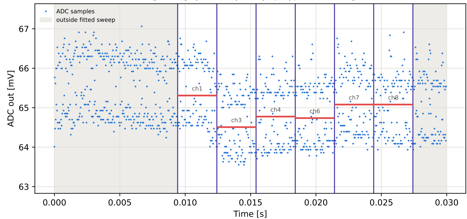
Tag2 &lt;- Tag6 | 785 MHz | run 0 | rep 1 | phase 94.72 deg
