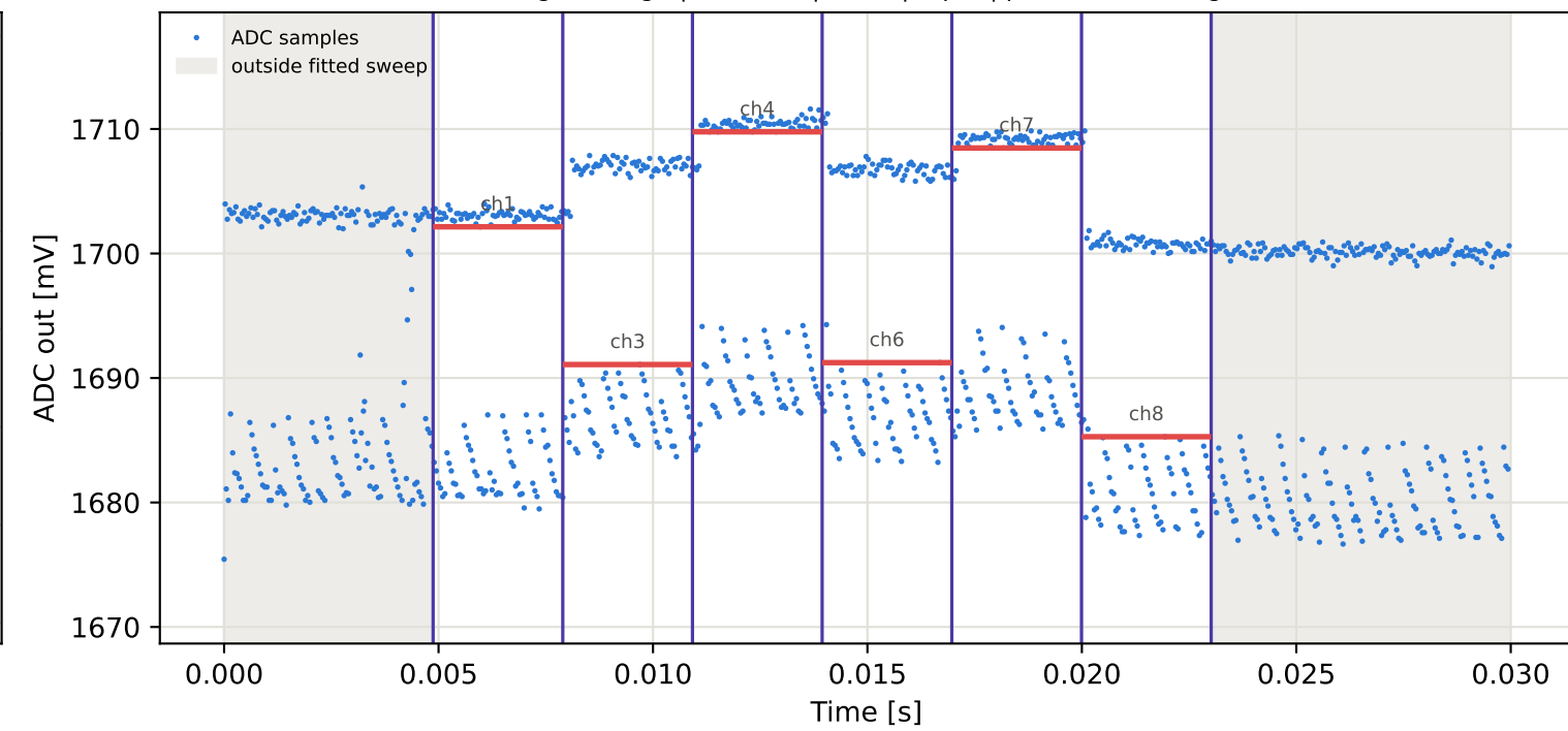
Tag2 &lt;- Tag6 | 905 MHz | run 0 | rep 1 | phase 119.23 deg
