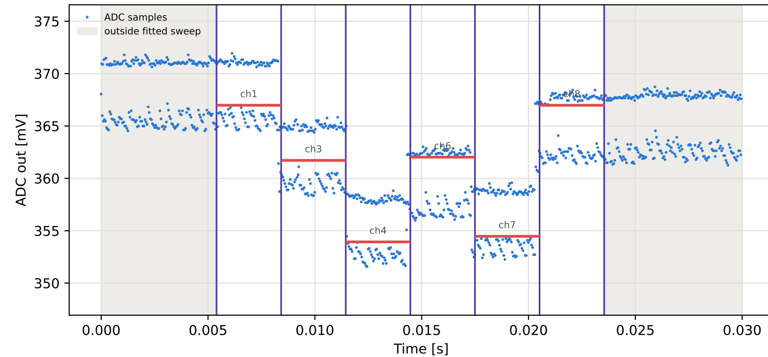
Tag7 &lt;- Tag10 | 855 MHz | run 0 | rep 1 | phase -9.99 deg
