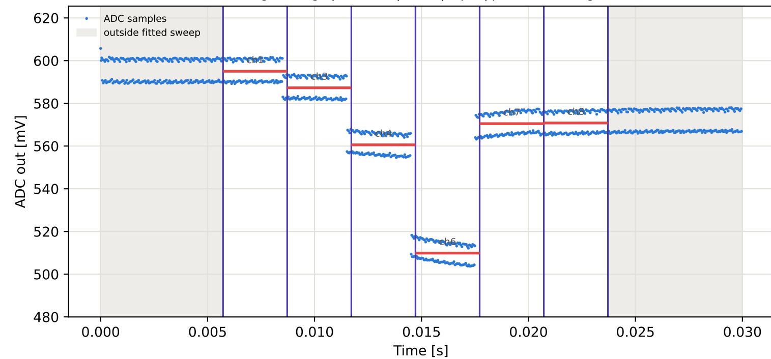
Tag3 &lt;- Tag7 | 915 MHz | run 0 | rep 1 | phase -24.29 deg
