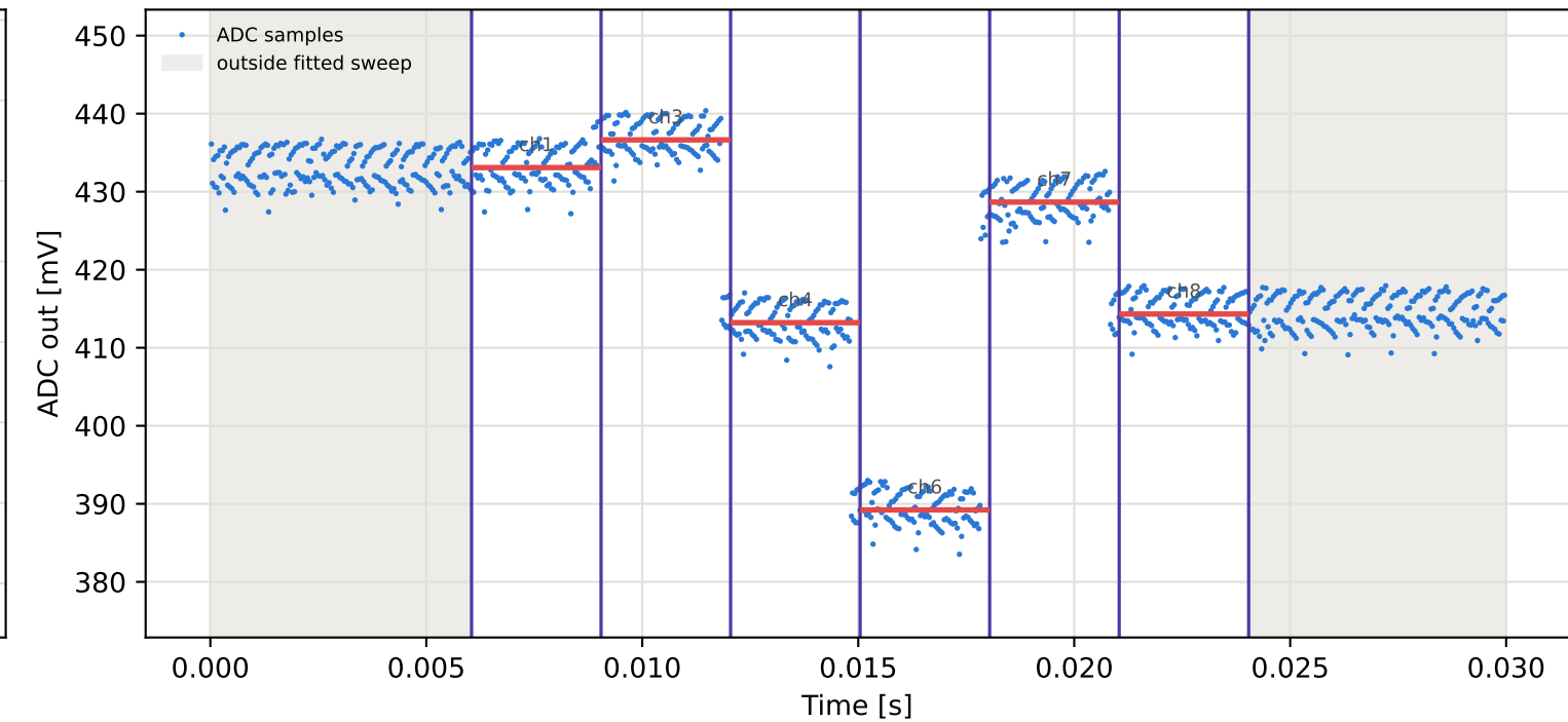
Tag15 &lt;- Tag10 | 965 MHz | run 0 | rep 1 | phase 27.08 deg
