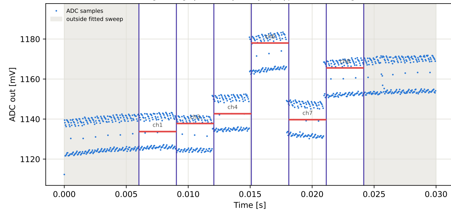
Tag3 &lt;- Tag6 | 895 MHz | run 0 | rep 1 | phase -18.53 deg
