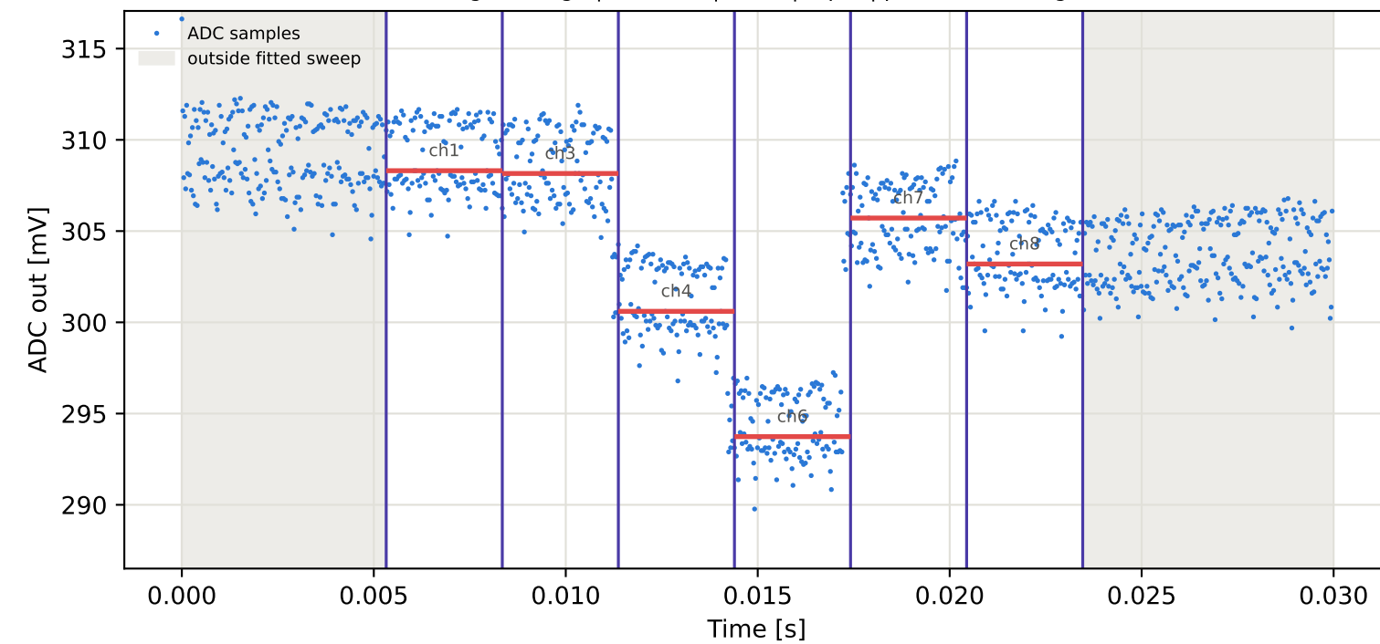
Tag6 &lt;- Tag9 | 935 MHz | run 0 | rep 1 | phase 109.68 deg
