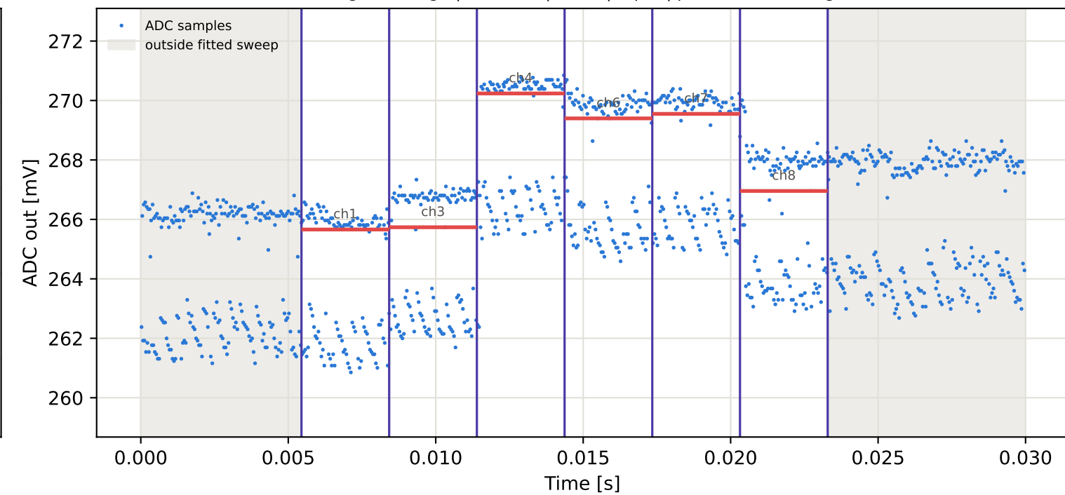
Tag2 &lt;- Tag10 | 805 MHz | run 0 | rep 1 | phase -15.94 deg
