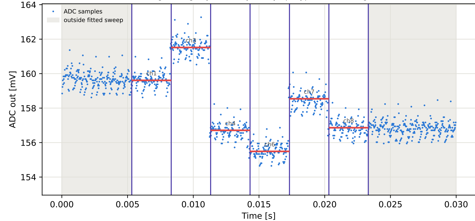
Tag5 &lt;- Tag2 | 825 MHz | run 0 | rep 1 | phase 147.63 deg
