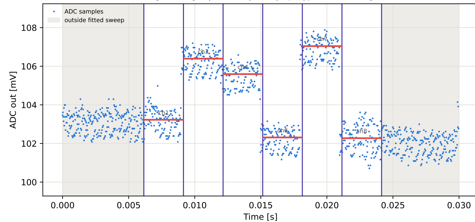
Tag10 &lt;- Tag2 | 805 MHz | run 0 | rep 1 | phase -136.06 deg
