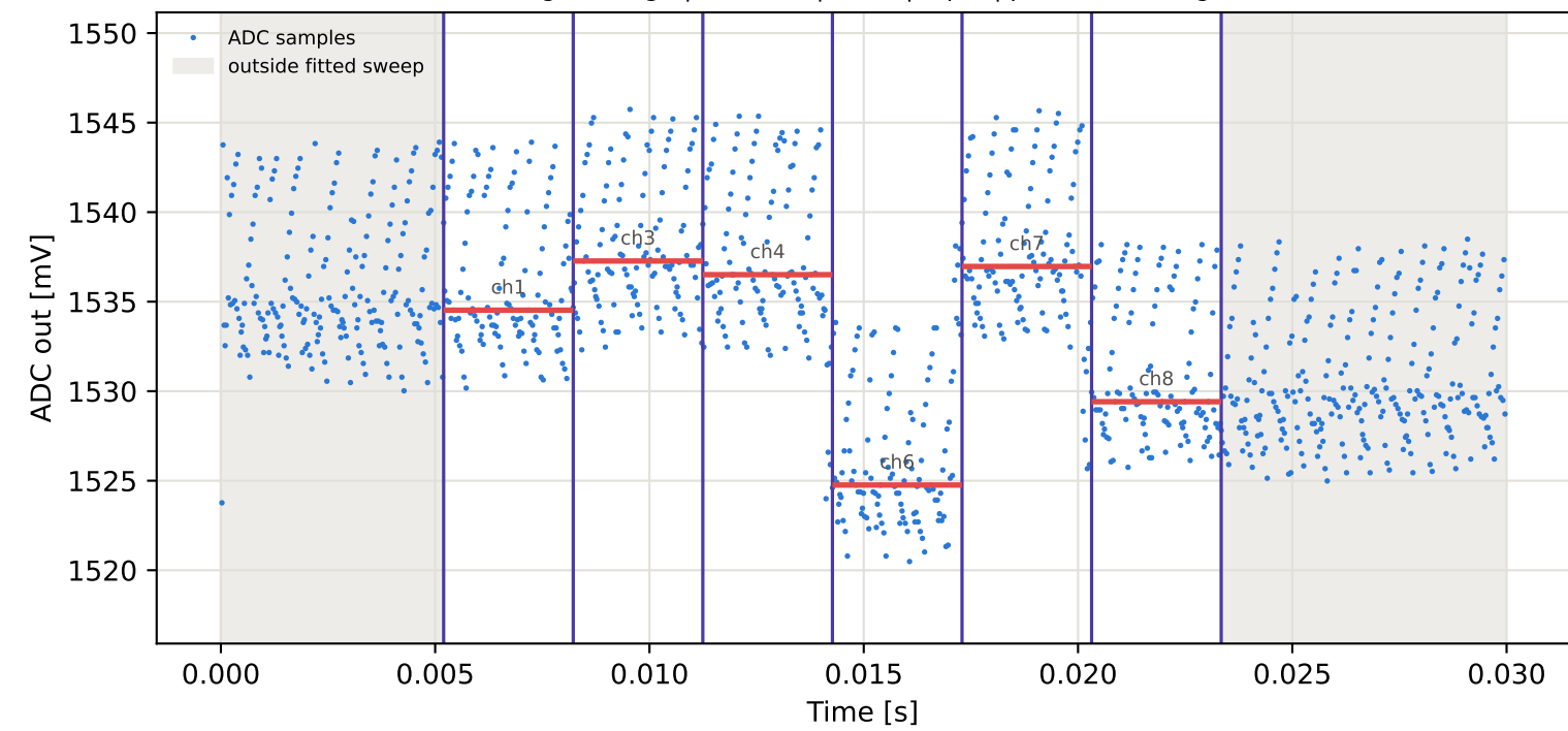
Tag2 &lt;- Tag6 | 925 MHz | run 0 | rep 1 | phase -51.88 deg
