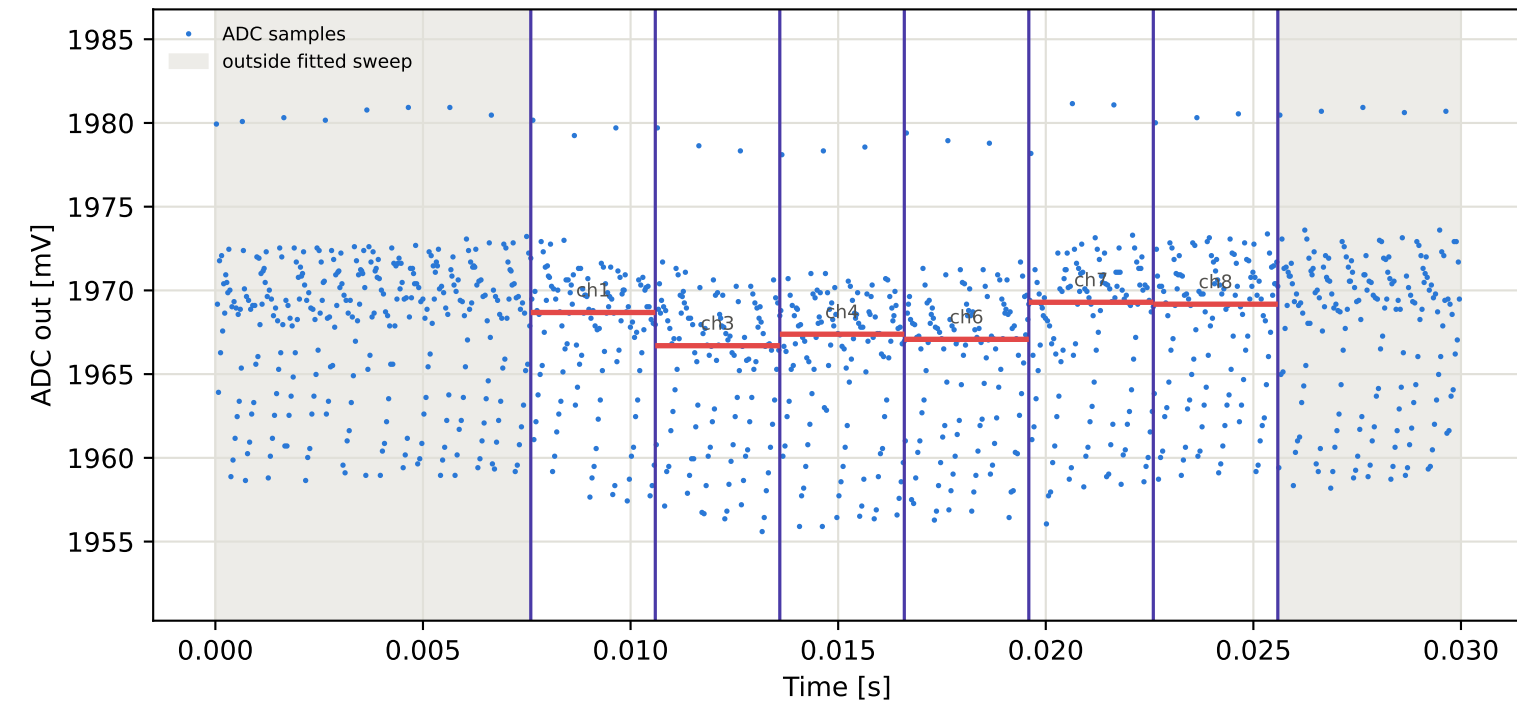
Tag2 &lt;- Tag15 | 915 MHz | run 0 | rep 1 | phase 131.04 deg
