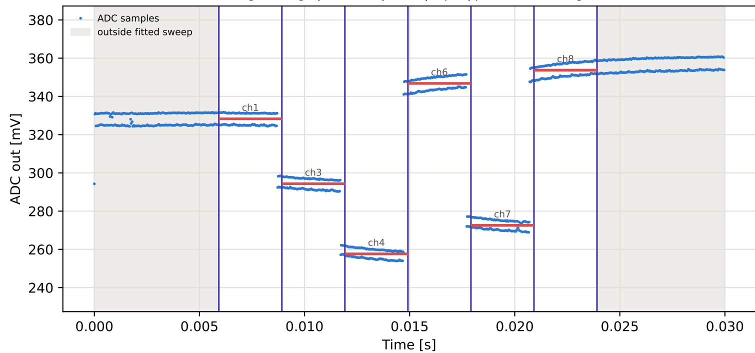
Tag9 &lt;- Tag15 | 945 MHz | run 0 | rep 1 | phase -11.73 deg
