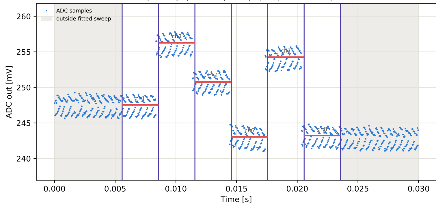
Tag9 &lt;- Tag8 | 825 MHz | run 0 | rep 1 | phase 38.41 deg
