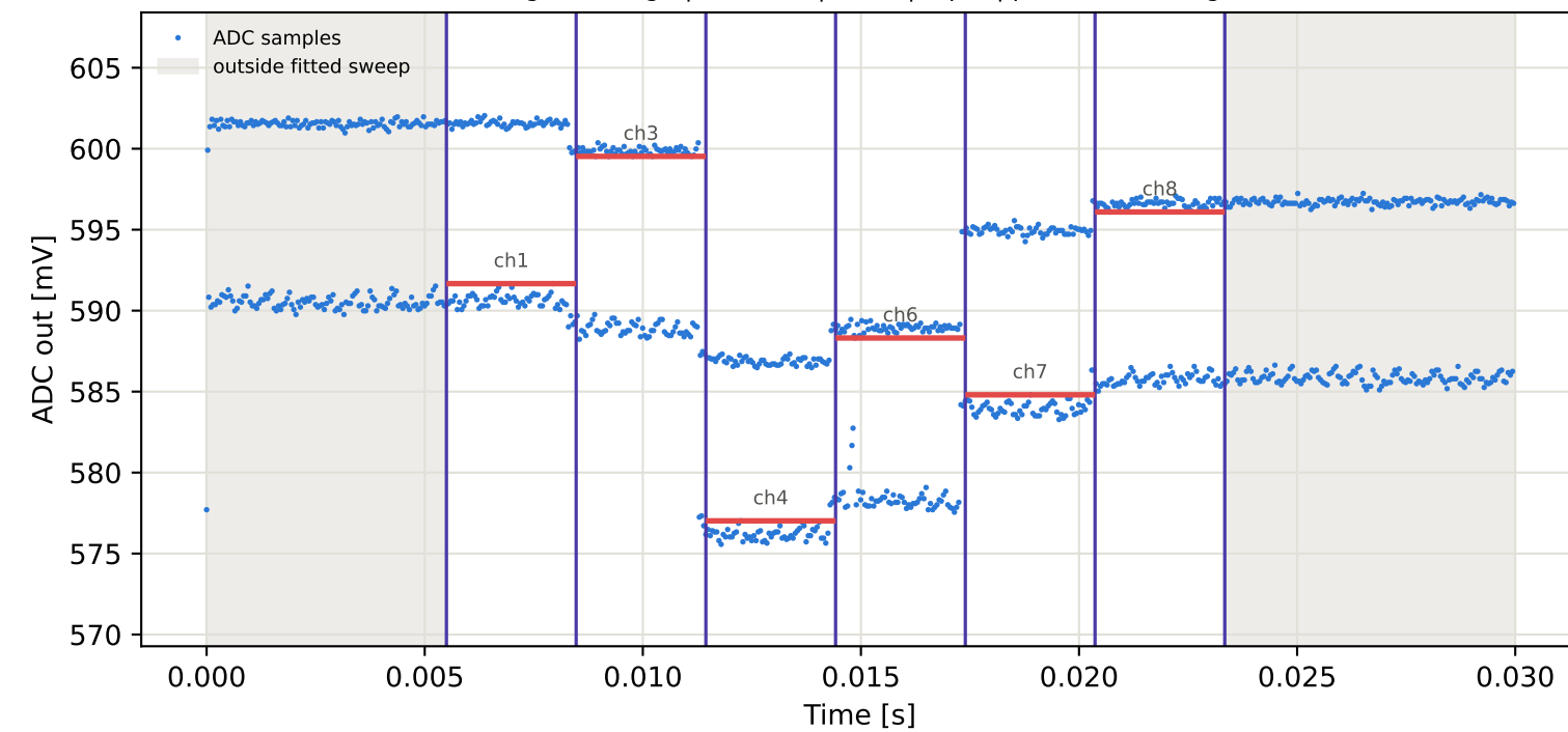
Tag15 &lt;- Tag9 | 995 MHz | run 0 | rep 1 | phase -53.81 deg
