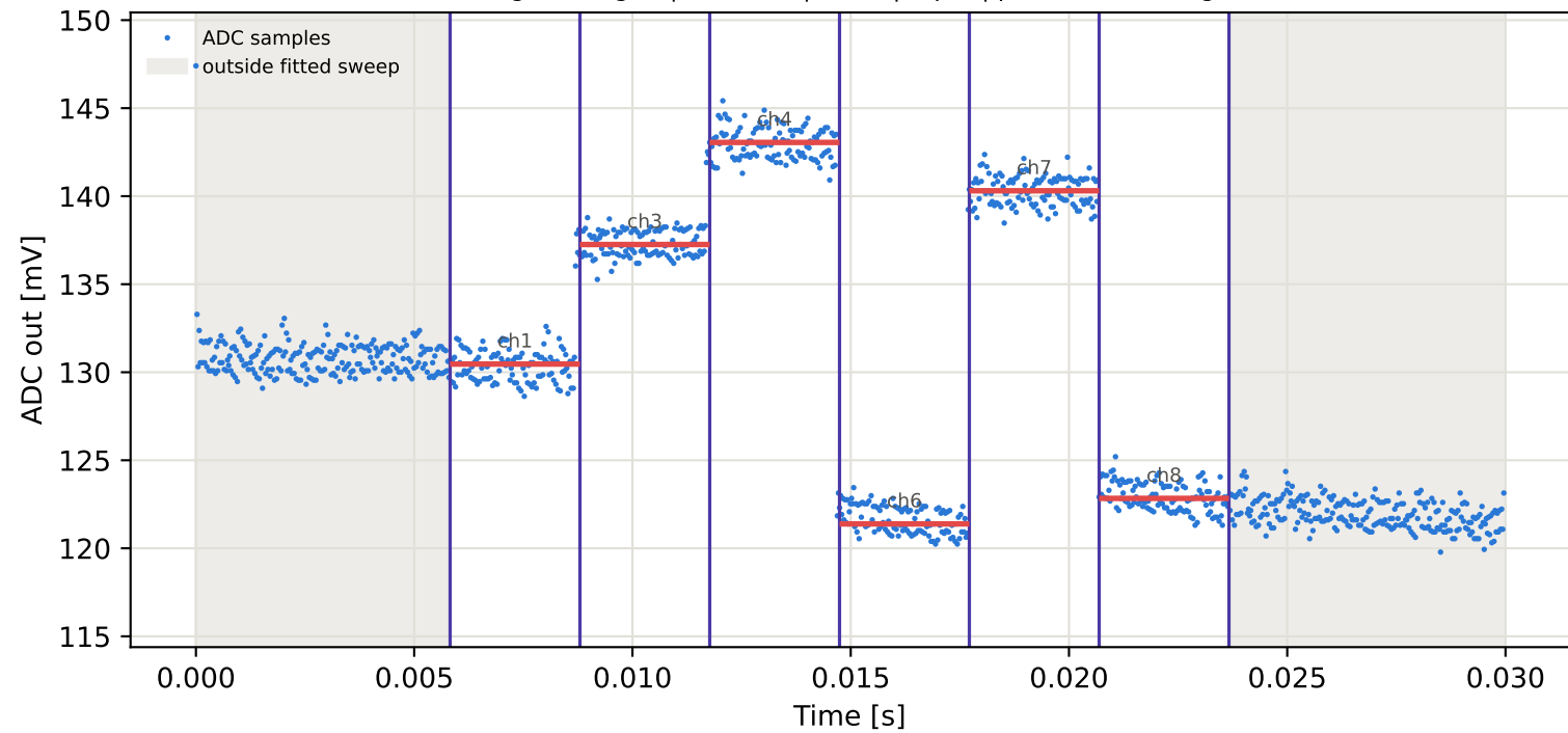
Tag6 &lt;- Tag3 | 975 MHz | run 0 | rep 1 | phase -53.55 deg
