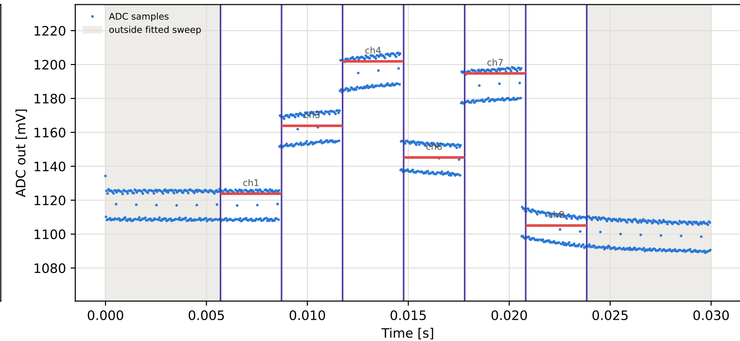
Tag3 &lt;- Tag9 | 895 MHz | run 0 | rep 1 | phase 154.30 deg
