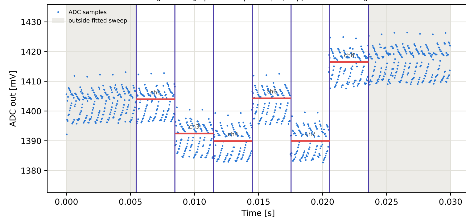
Tag16 &lt;- Tag6 | 875 MHz | run 0 | rep 1 | phase 126.78 deg
