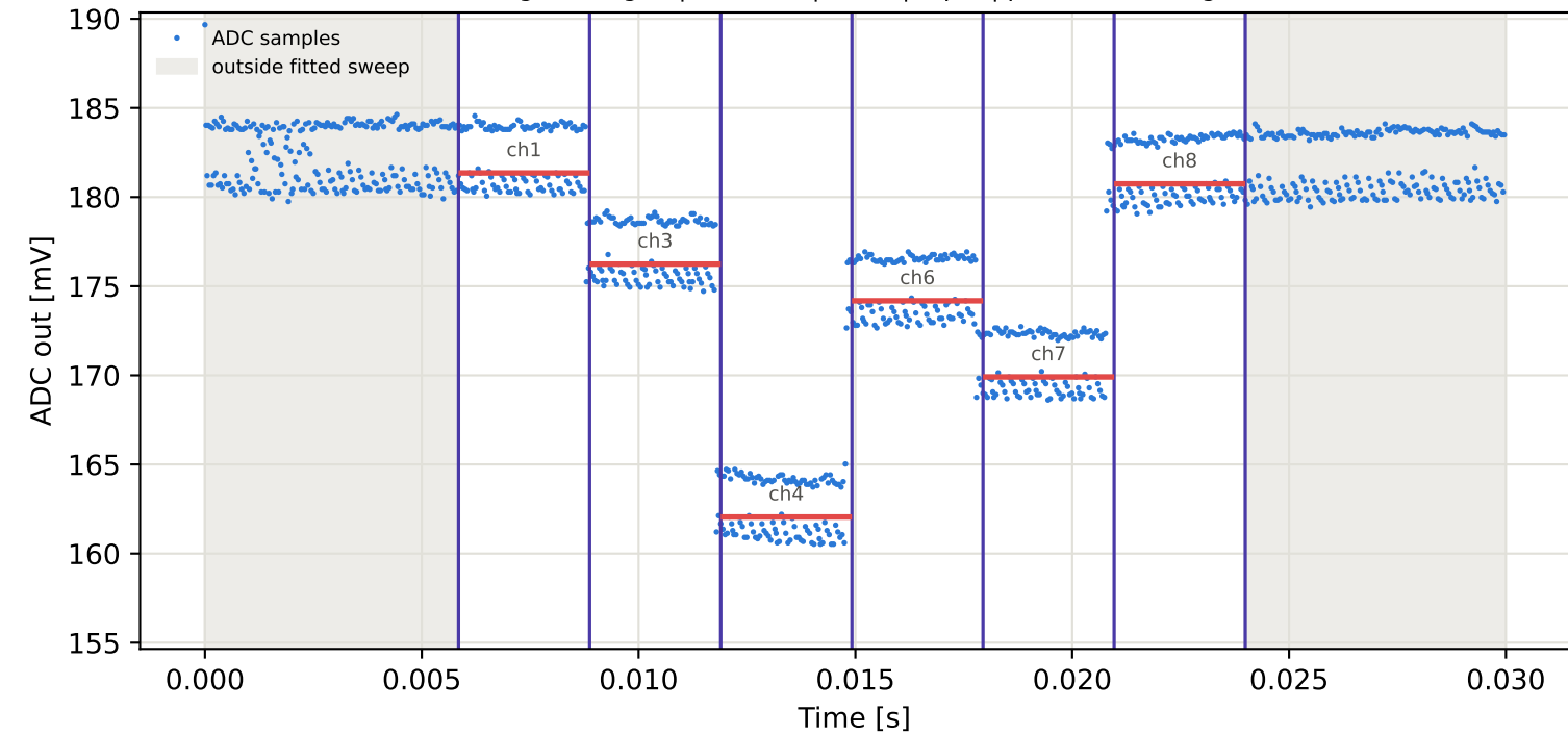
Tag1 &lt;- Tag2 | 995 MHz | run 0 | rep 1 | phase -35.14 deg
