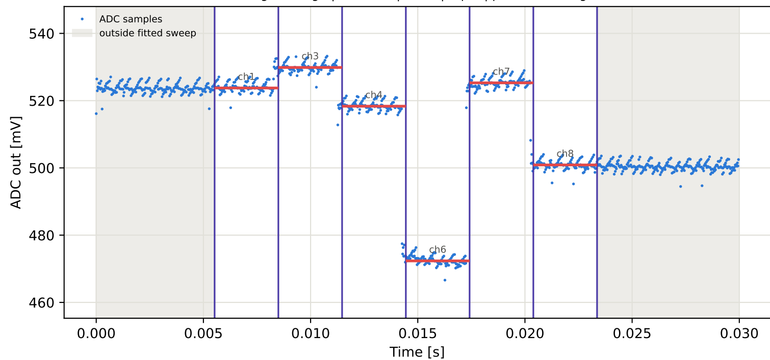
Tag5 &lt;- Tag1 | 935 MHz | run 0 | rep 1 | phase 6.72 deg
