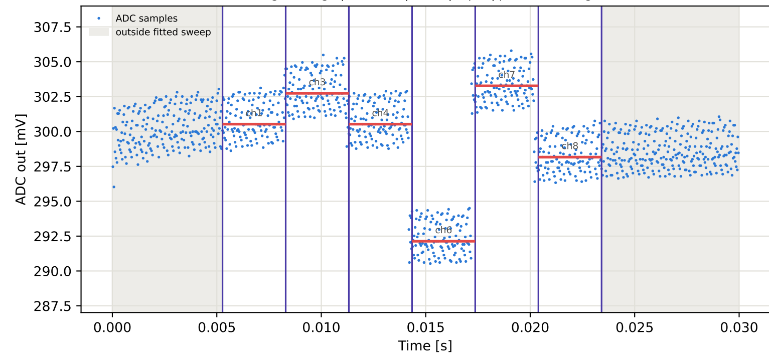
Tag3 &lt;- Tag6 | 975 MHz | run 0 | rep 1 | phase 160.43 deg
