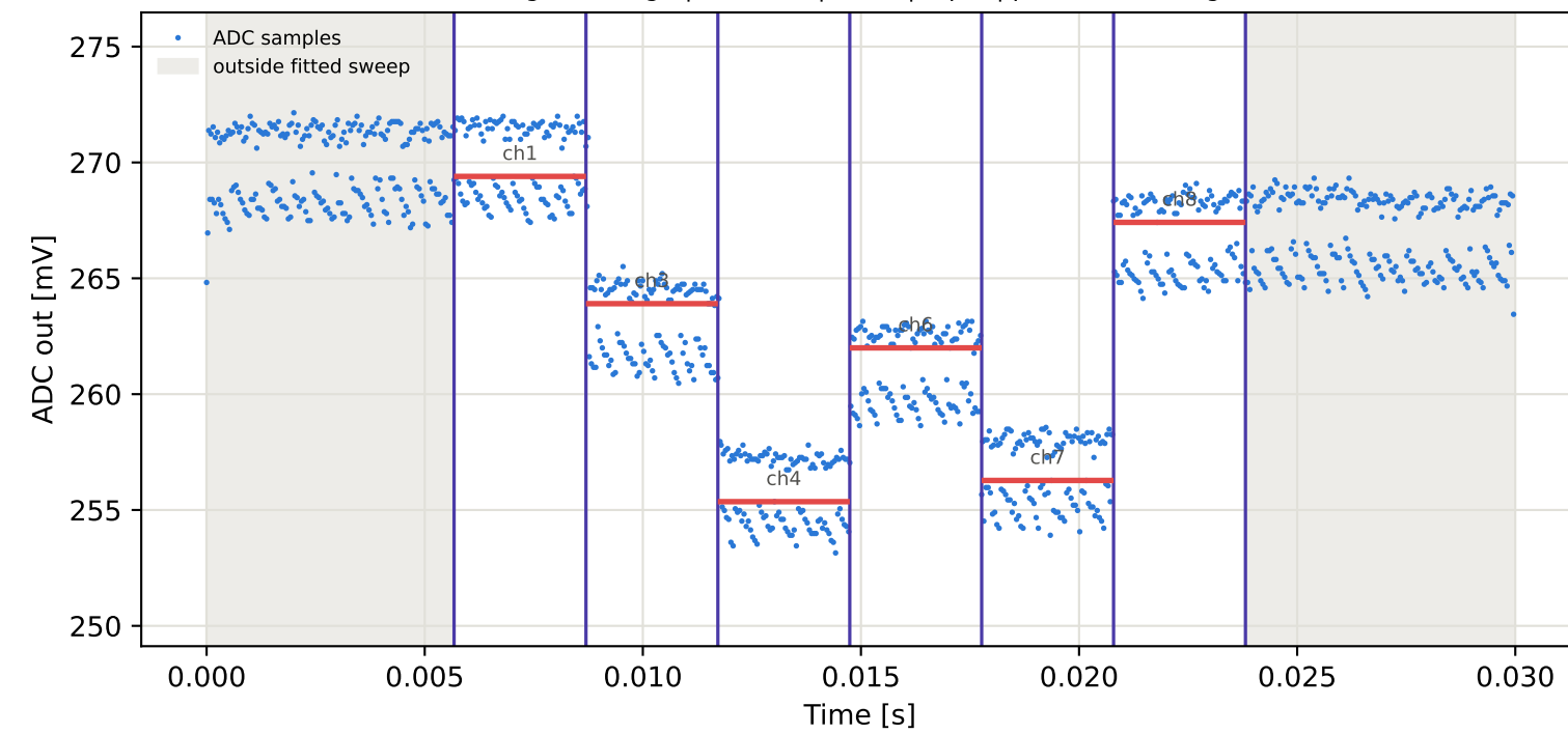
Tag15 &lt;- Tag9 | 805 MHz | run 0 | rep 1 | phase -135.16 deg
