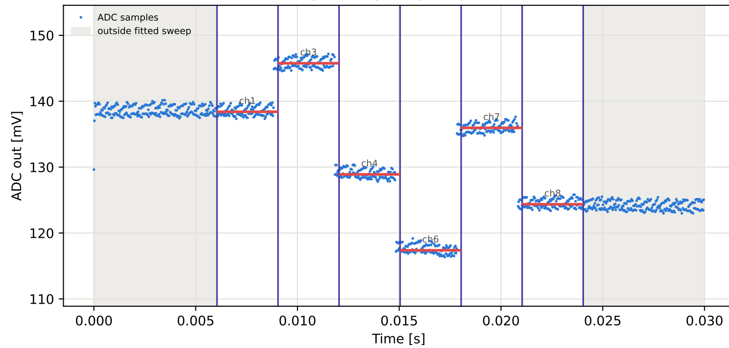
Tag4 &lt;- Tag9 | 845 MHz | run 0 | rep 1 | phase 27.44 deg
