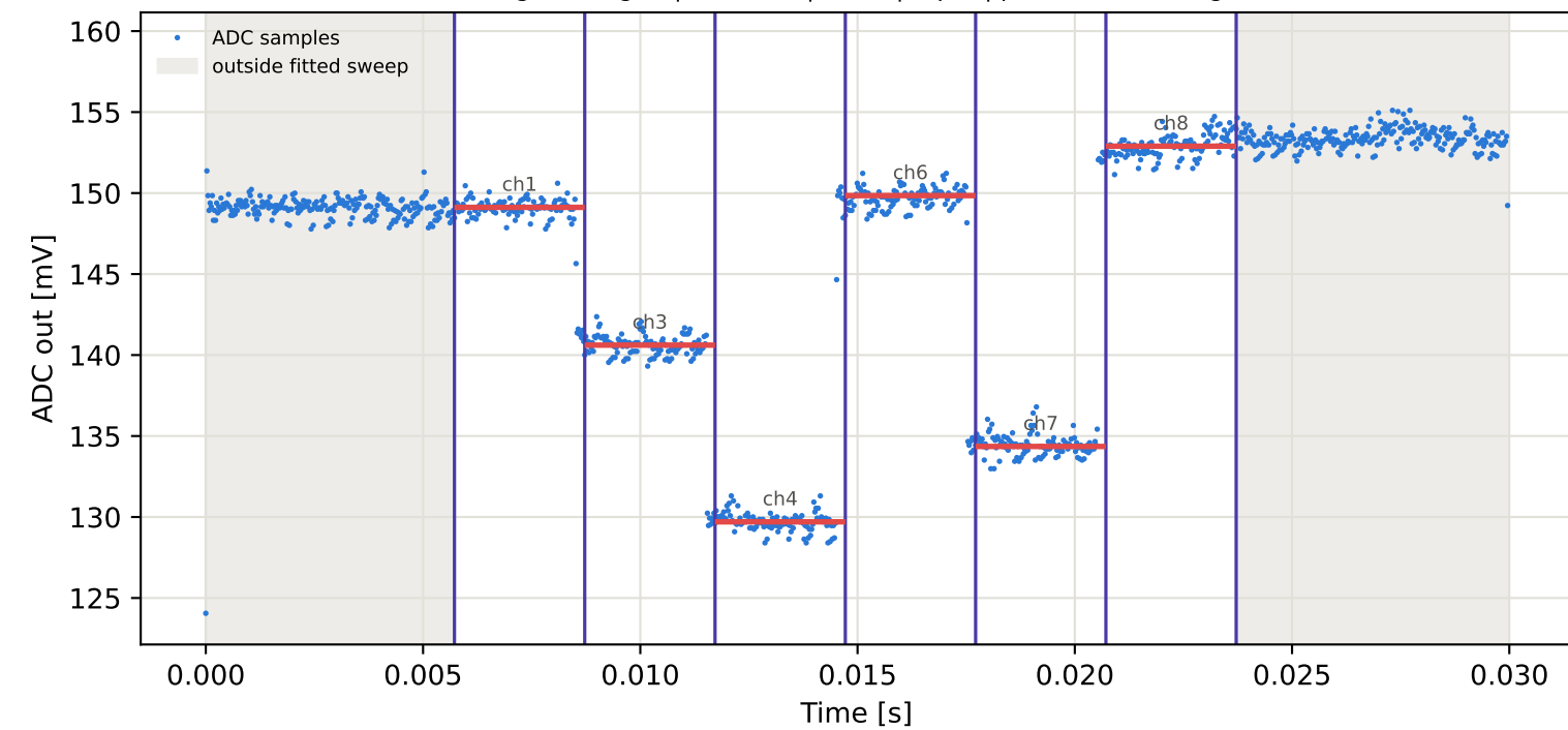
Tag6 &lt;- Tag2 | 975 MHz | run 0 | rep 1 | phase -86.19 deg
