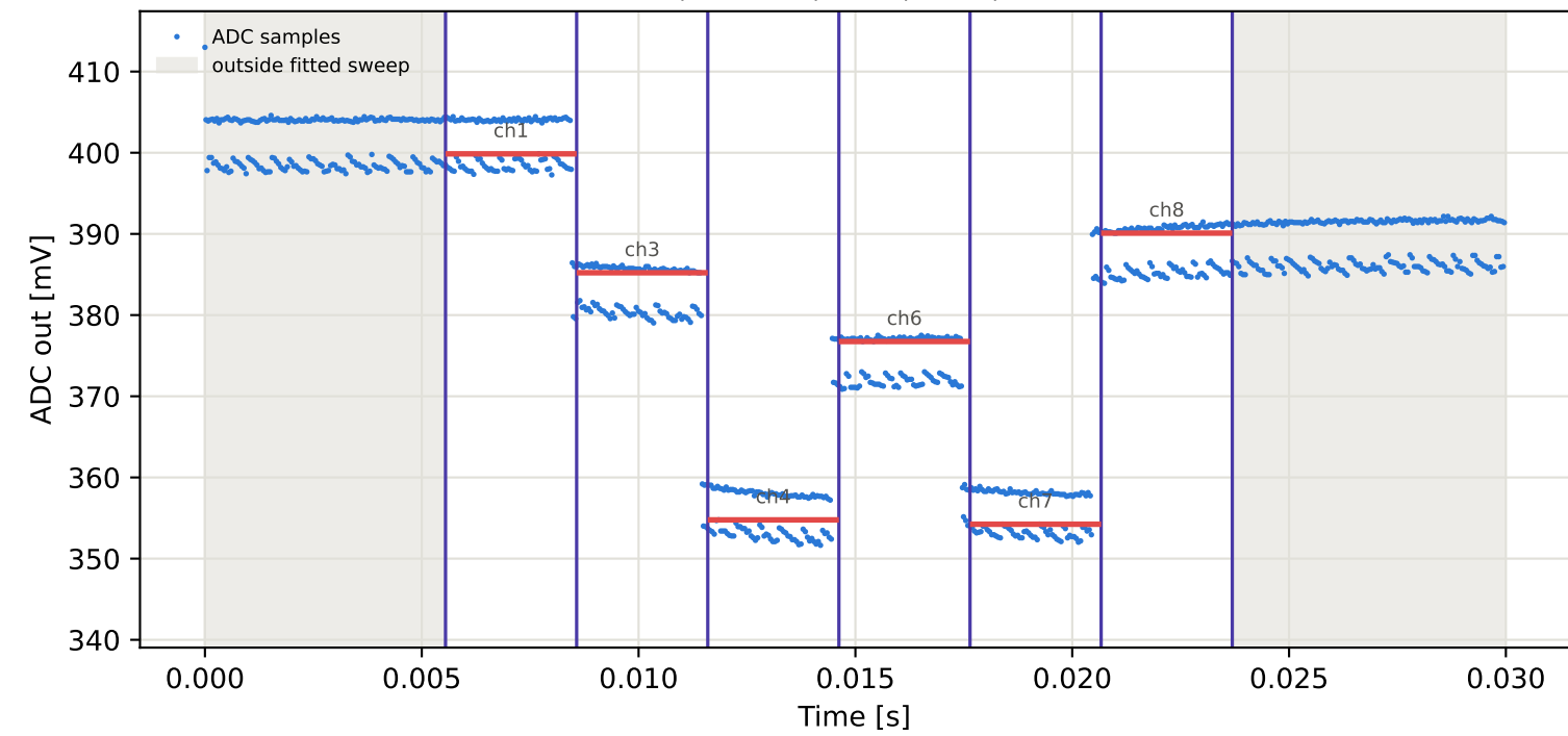
Tag2 &lt;- Tag16 | 825 MHz | run 0 | rep 1 | phase 90.36 deg
