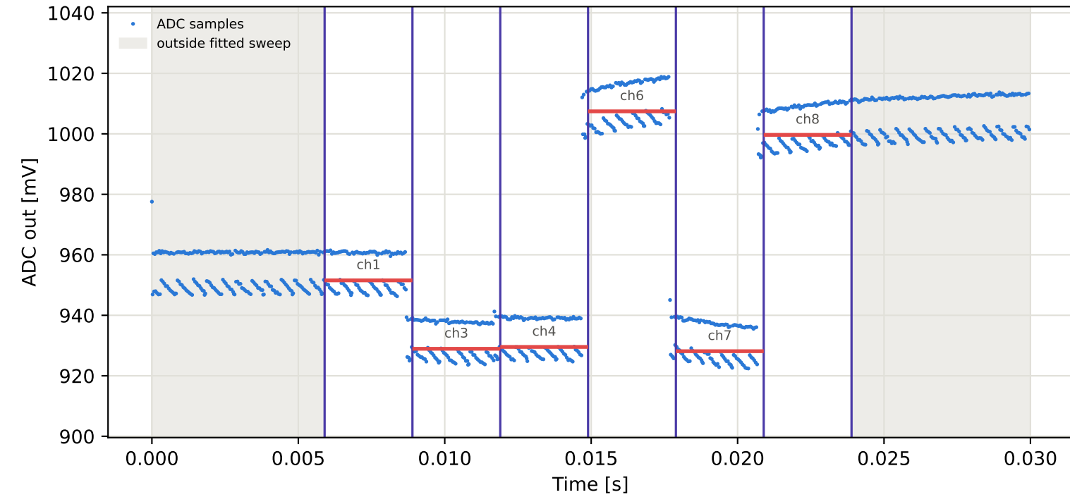
Tag7 &lt;- Tag5 | 905 MHz | run 0 | rep 1 | phase -61.31 deg
