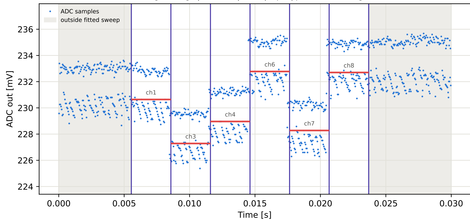
Tag8 &lt;- Tag10 | 805 MHz | run 0 | rep 1 | phase 36.69 deg
