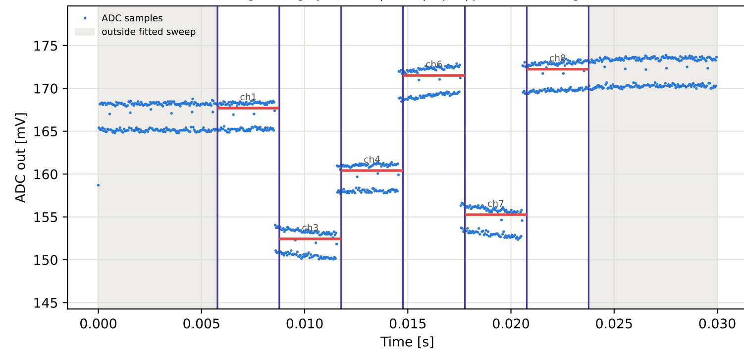
Tag4 &lt;- Tag7 | 825 MHz | run 0 | rep 1 | phase -20.89 deg
