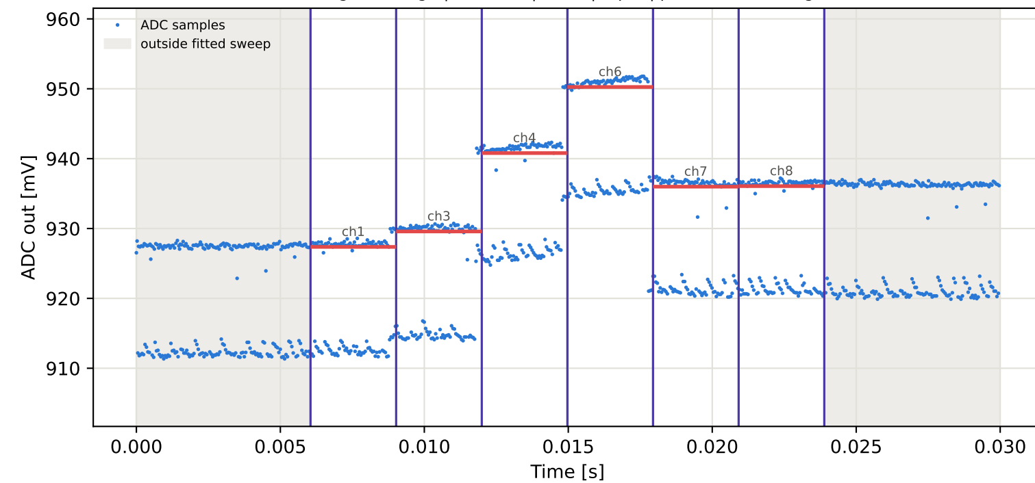
Tag15 &lt;- Tag9 | 925 MHz | run 0 | rep 1 | phase 34.12 deg
