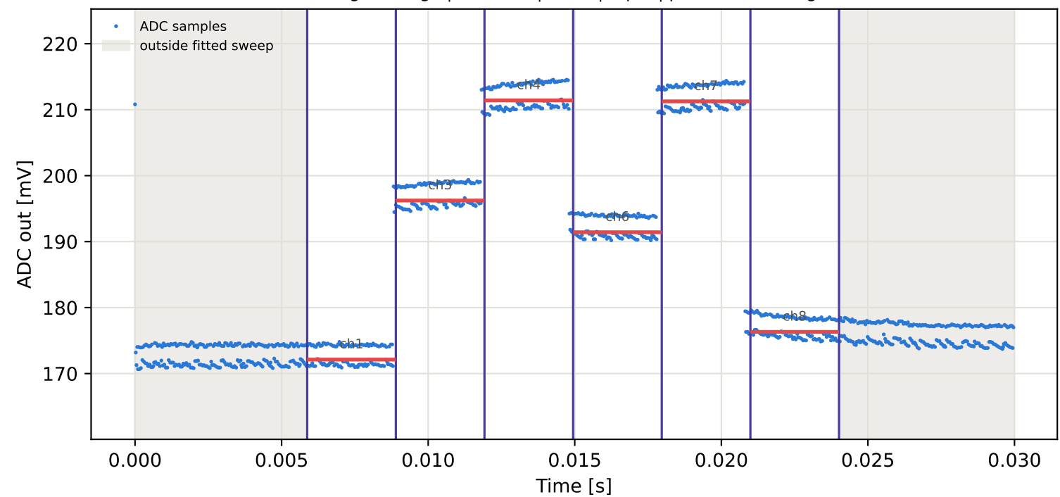
Tag8 &lt;- Tag7 | 805 MHz | run 0 | rep 1 | phase -77.96 deg
