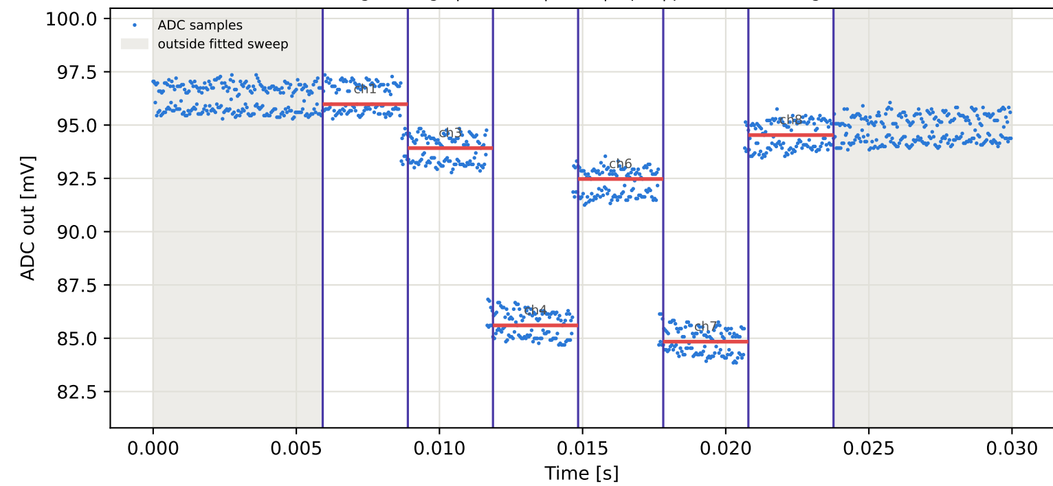
Tag9 &lt;- Tag6 | 785 MHz | run 0 | rep 1 | phase 22.83 deg
