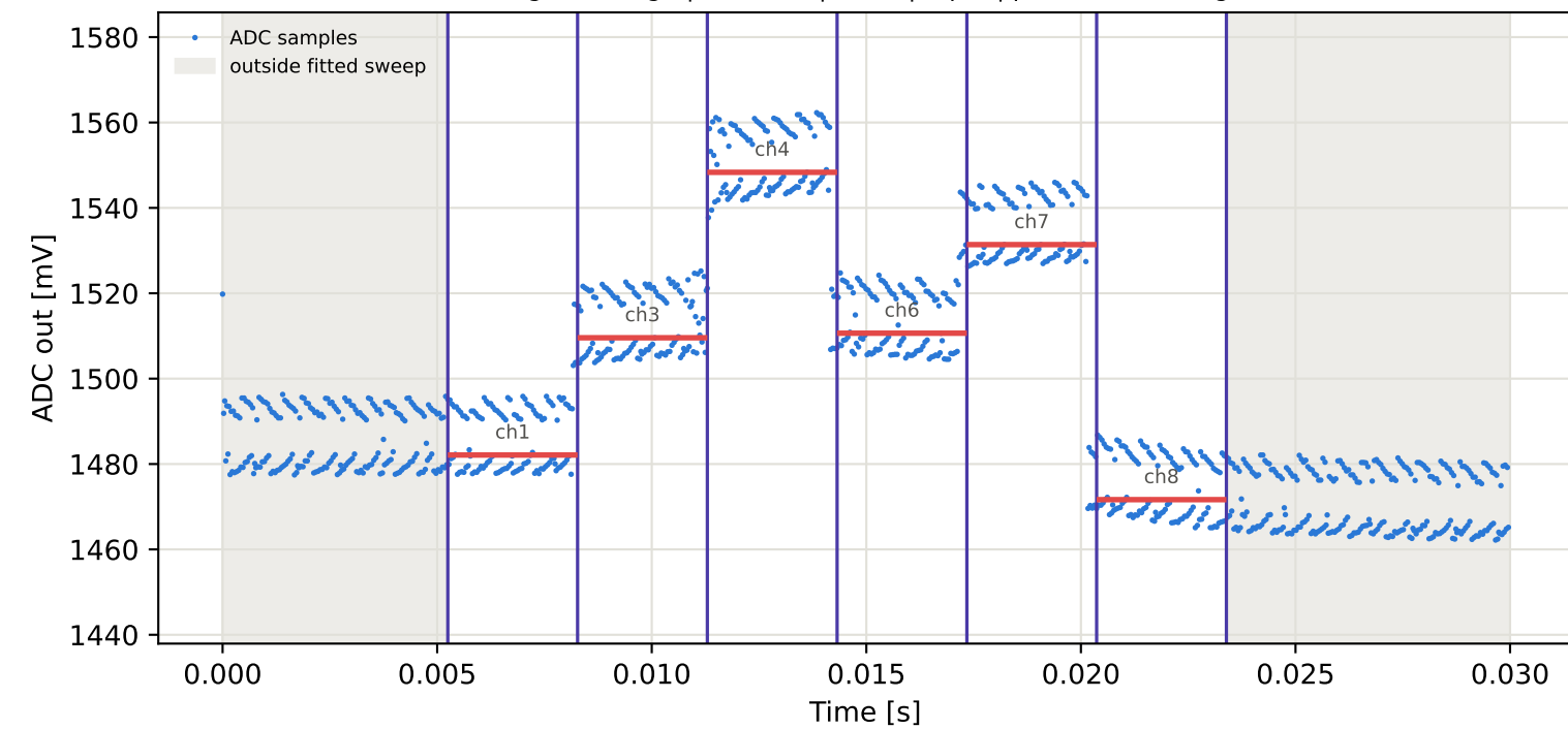
Tag16 &lt;- Tag4 | 905 MHz | run 0 | rep 1 | phase 4.17 deg
