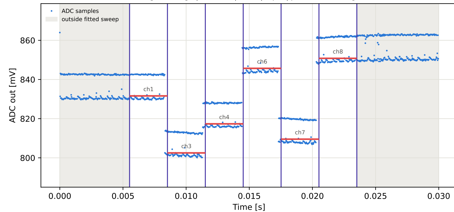
Tag2 &lt;- Tag1 | 855 MHz | run 0 | rep 1 | phase 139.01 deg
