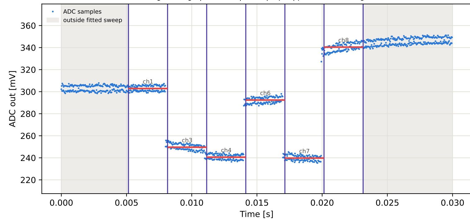
Tag9 &lt;- Tag8 | 885 MHz | run 0 | rep 1 | phase 120.94 deg
