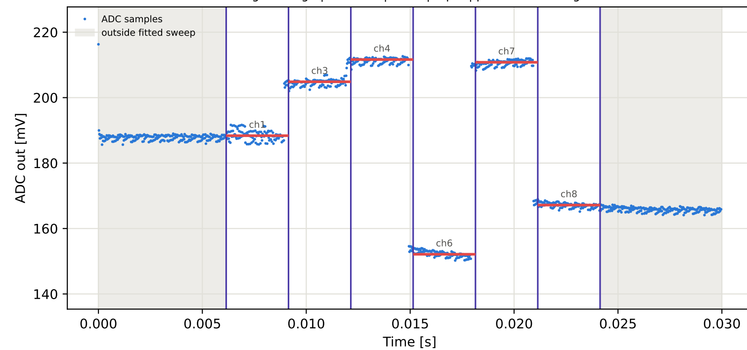
Tag4 &lt;- Tag7 | 975 MHz | run 0 | rep 1 | phase -177.37 deg
