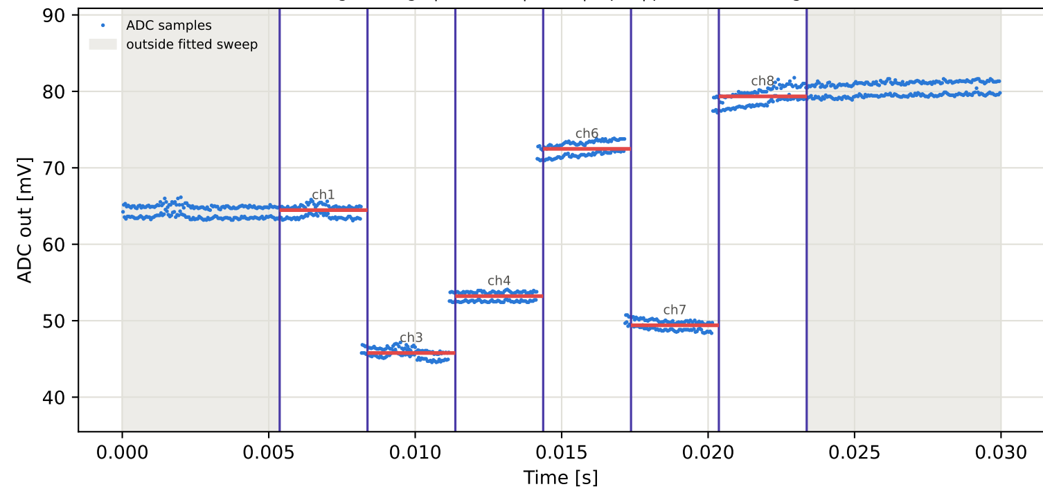
Tag9 &lt;- Tag6 | 855 MHz | run 0 | rep 1 | phase 52.63 deg
