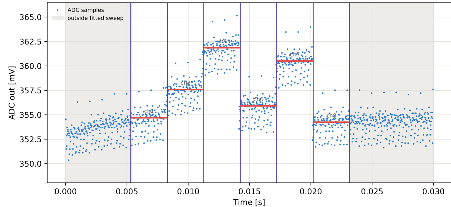
Tag1 &lt;- Tag4 | 975 MHz | run 0 | rep 1 | phase 79.58 deg
