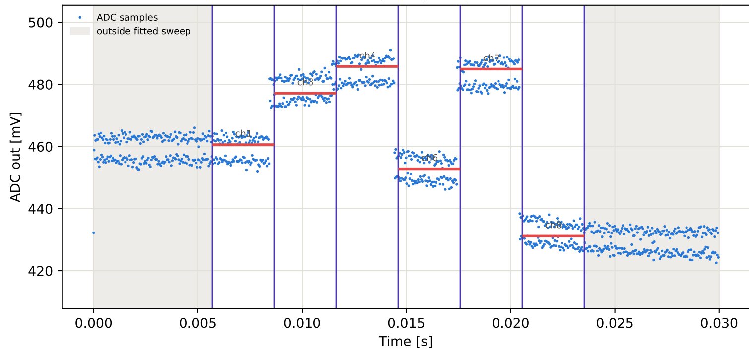
Tag4 &lt;- Tag3 | 885 MHz | run 0 | rep 1 | phase -50.21 deg
