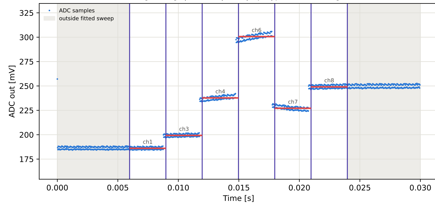
Tag1 &lt;- Tag7 | 895 MHz | run 0 | rep 1 | phase -177.36 deg
