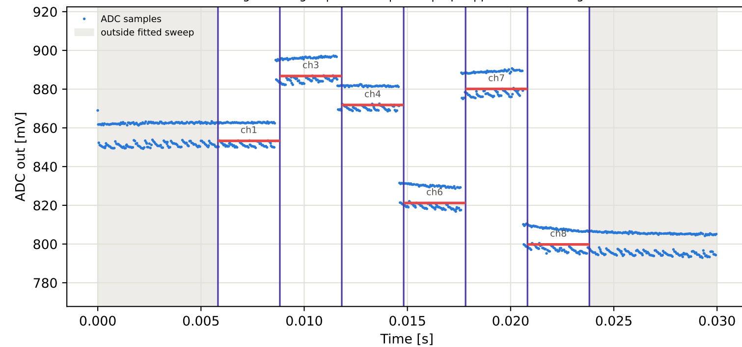
Tag15 &lt;- Tag3 | 875 MHz | run 0 | rep 1 | phase 139.56 deg
