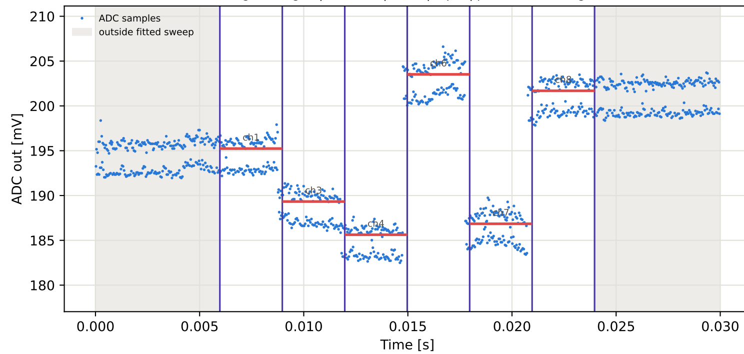
Tag6 &lt;- Tag2 | 985 MHz | run 0 | rep 1 | phase -51.18 deg
