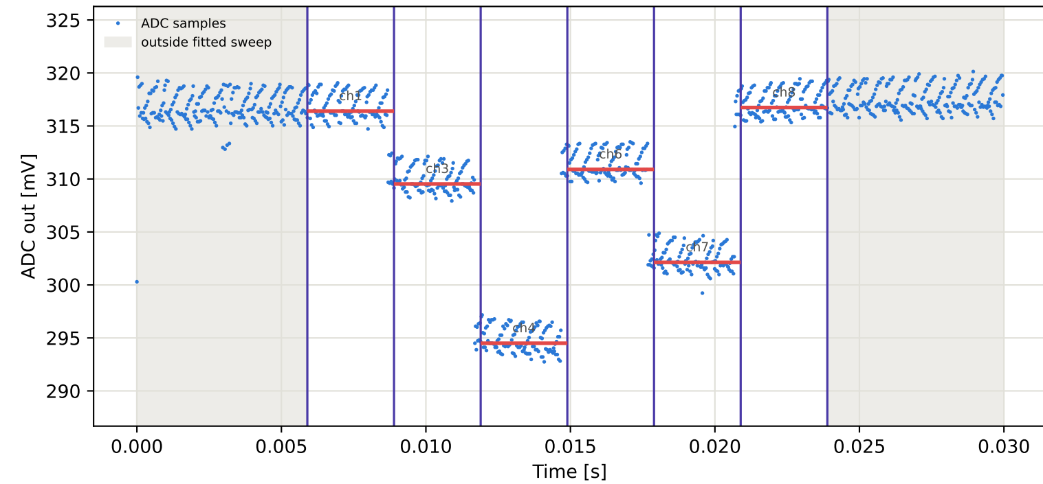
Tag5 &lt;- Tag3 | 975 MHz | run 0 | rep 1 | phase -152.58 deg
