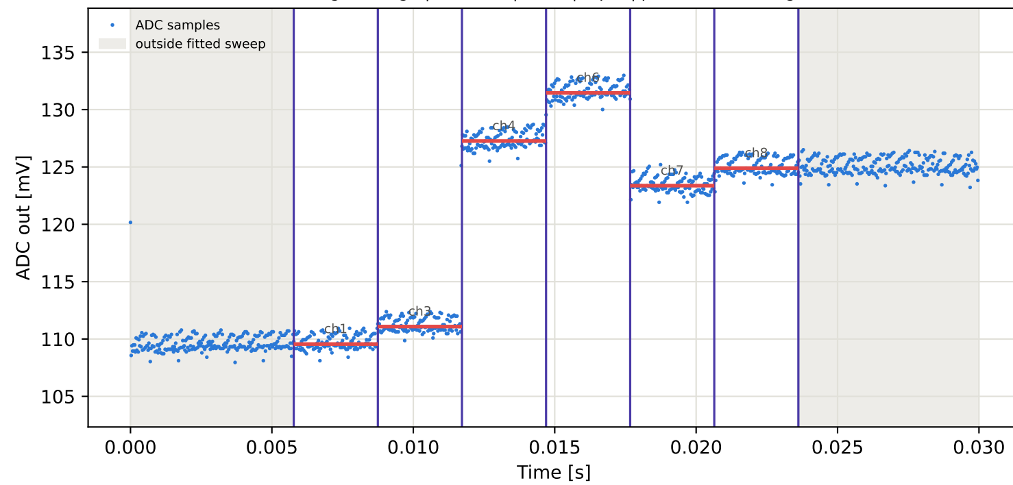
Tag4 &lt;- Tag7 | 845 MHz | run 0 | rep 1 | phase -39.47 deg
