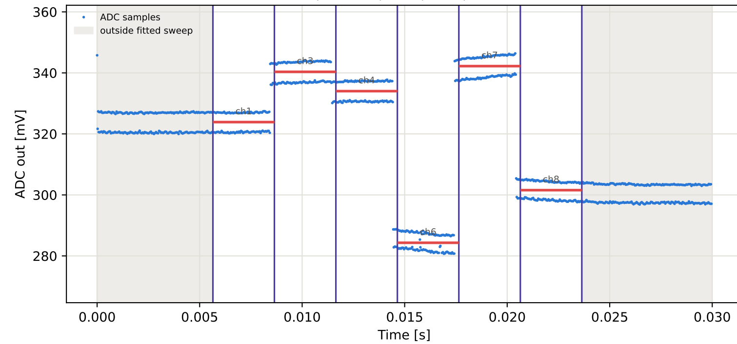
Tag1 &lt;- Tag9 | 975 MHz | run 0 | rep 1 | phase -13.24 deg
