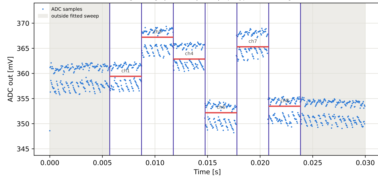
Tag6 &lt;- Tag9 | 855 MHz | run 0 | rep 1 | phase 97.20 deg
