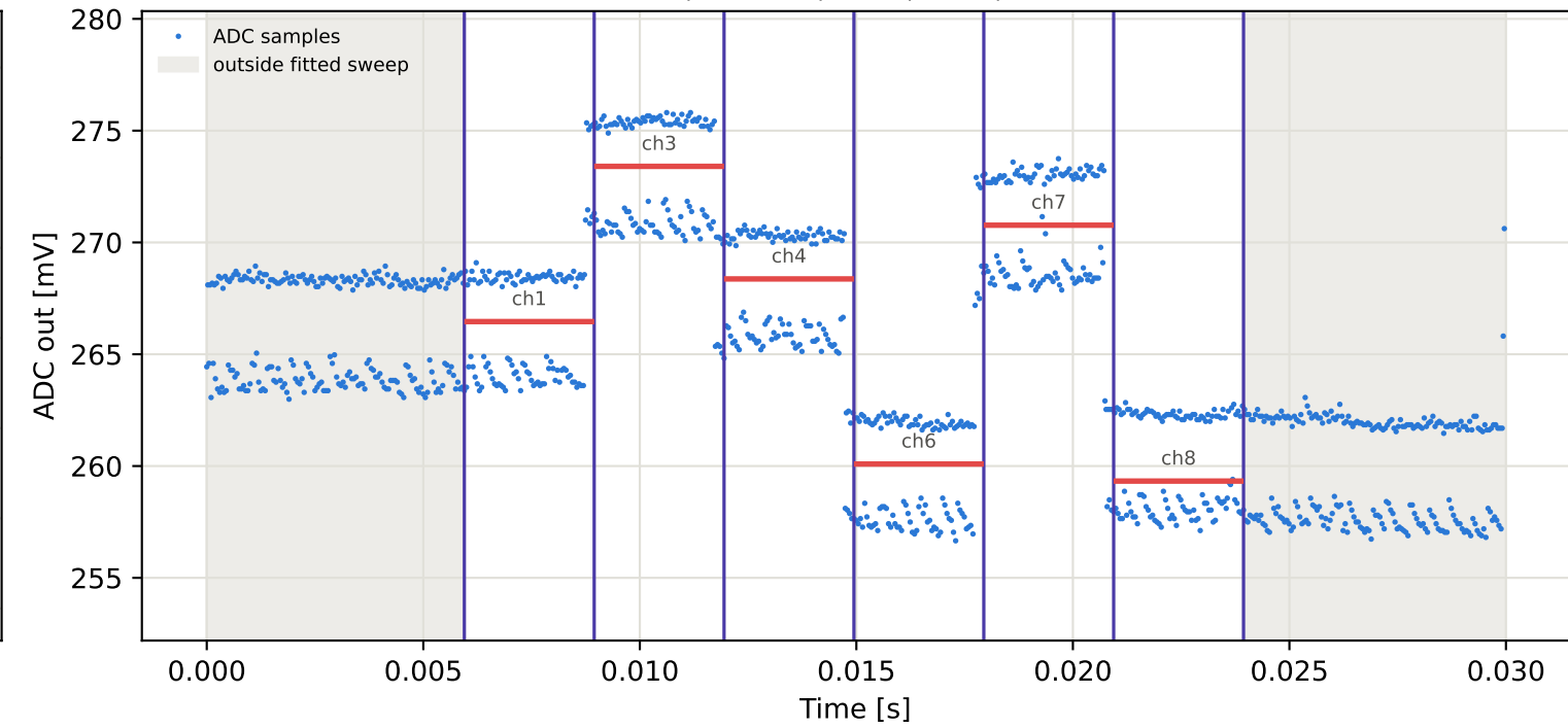
Tag16 &lt;- Tag7 | 805 MHz | run 0 | rep 1 | phase -0.04 deg
