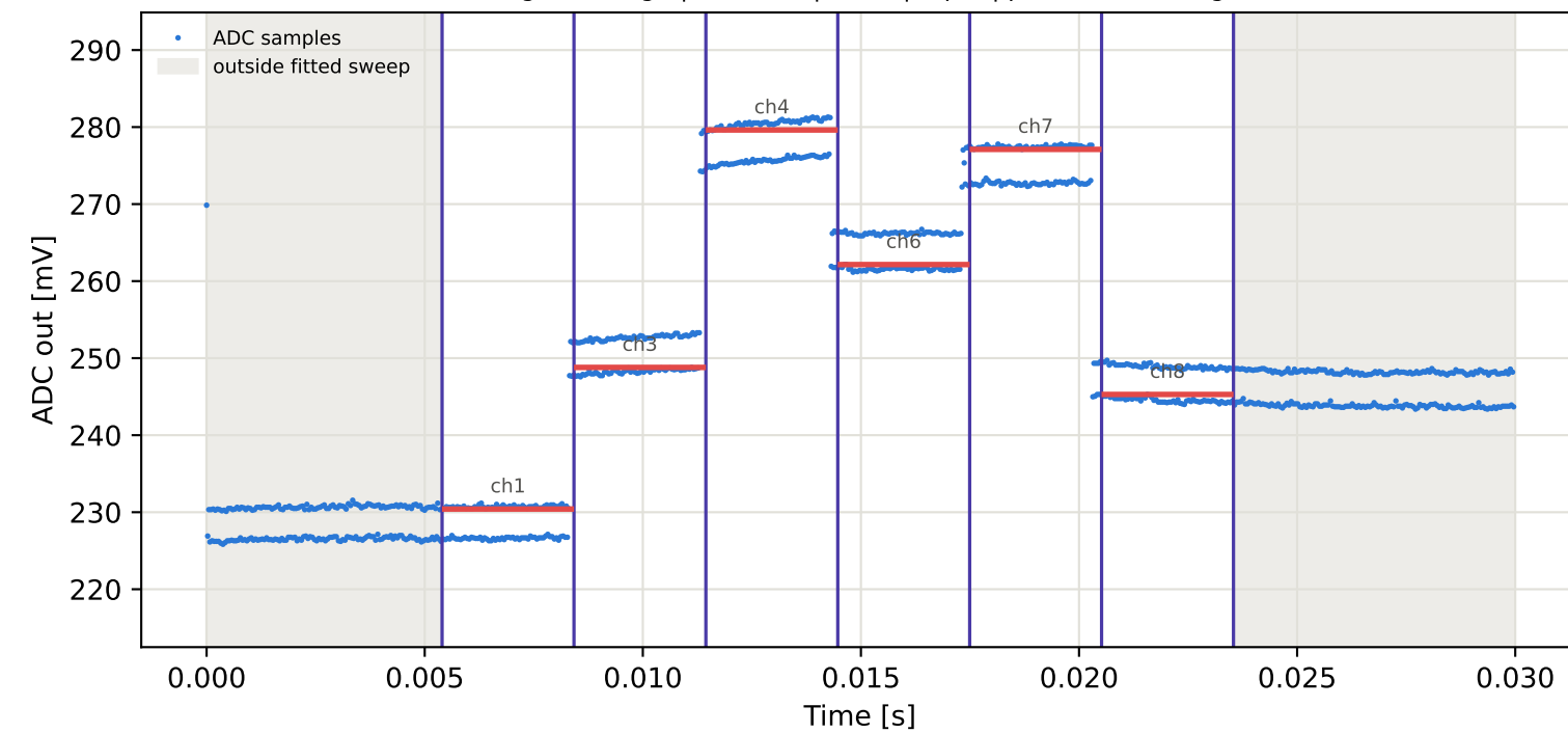
Tag10 &lt;- Tag8 | 835 MHz | run 0 | rep 1 | phase -137.66 deg
