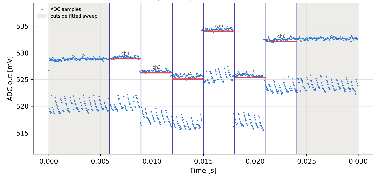
Tag7 &lt;- Tag6 | 985 MHz | run 0 | rep 1 | phase 147.13 deg
