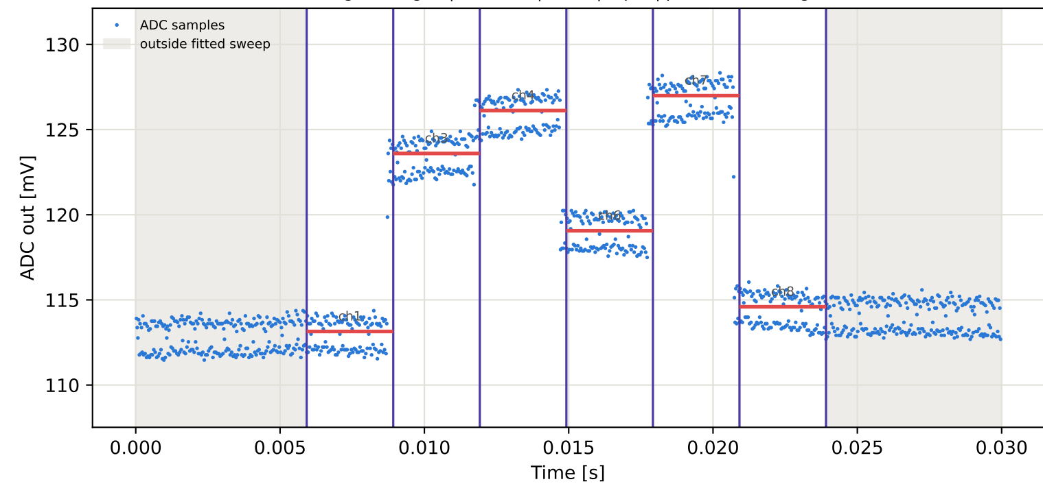
Tag1 &lt;- Tag2 | 855 MHz | run 0 | rep 1 | phase 13.99 deg
