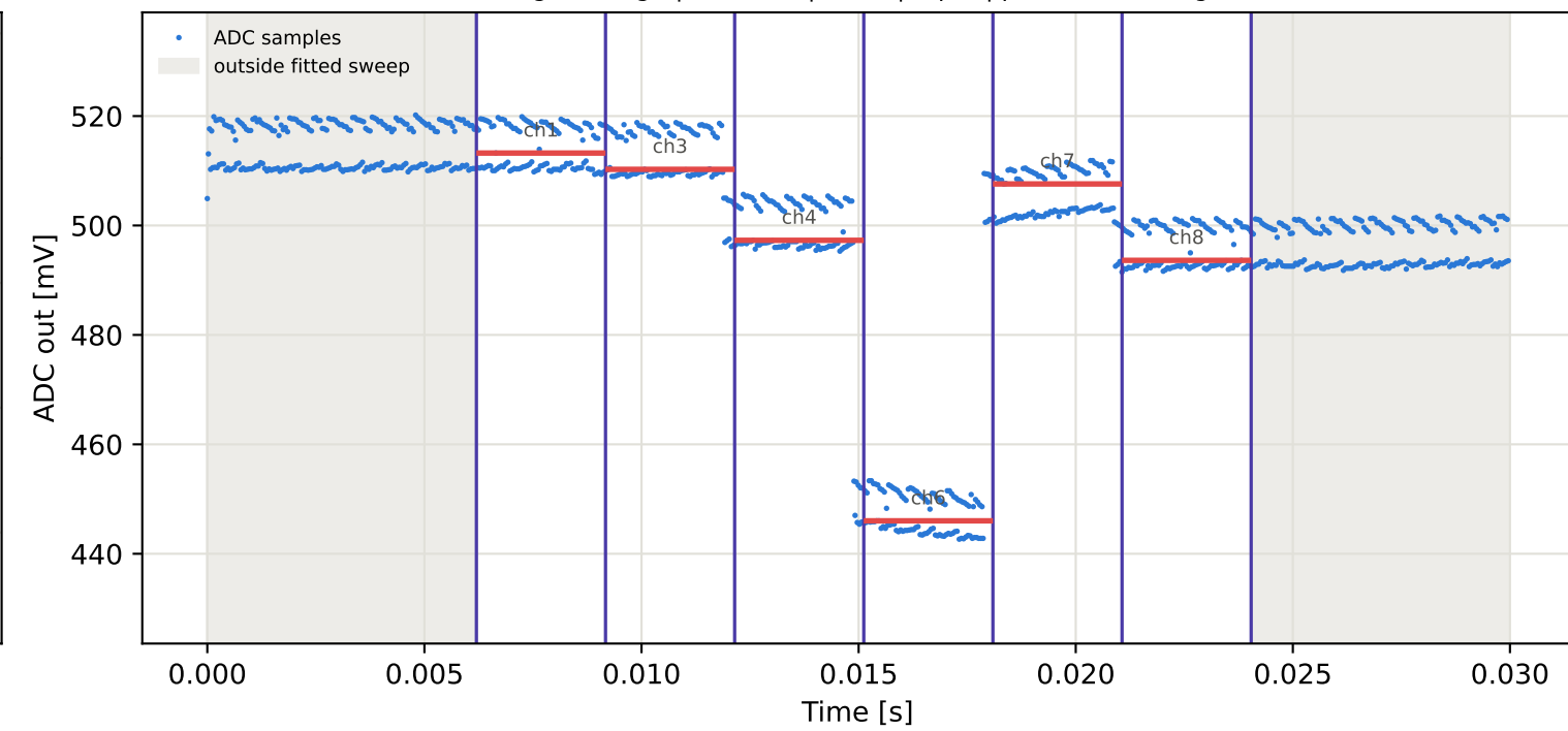
Tag7 &lt;- Tag4 | 945 MHz | run 0 | rep 1 | phase -101.12 deg
