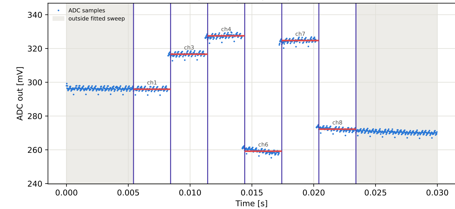
Tag3 &lt;- Tag8 | 975 MHz | run 0 | rep 1 | phase -33.87 deg
