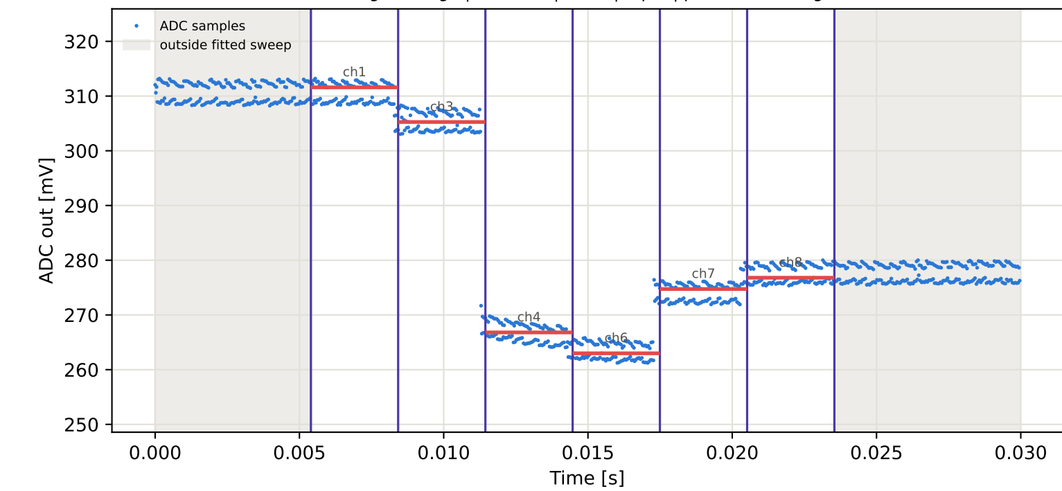
Tag5 &lt;- Tag3 | 835 MHz | run 0 | rep 1 | phase 52.65 deg
