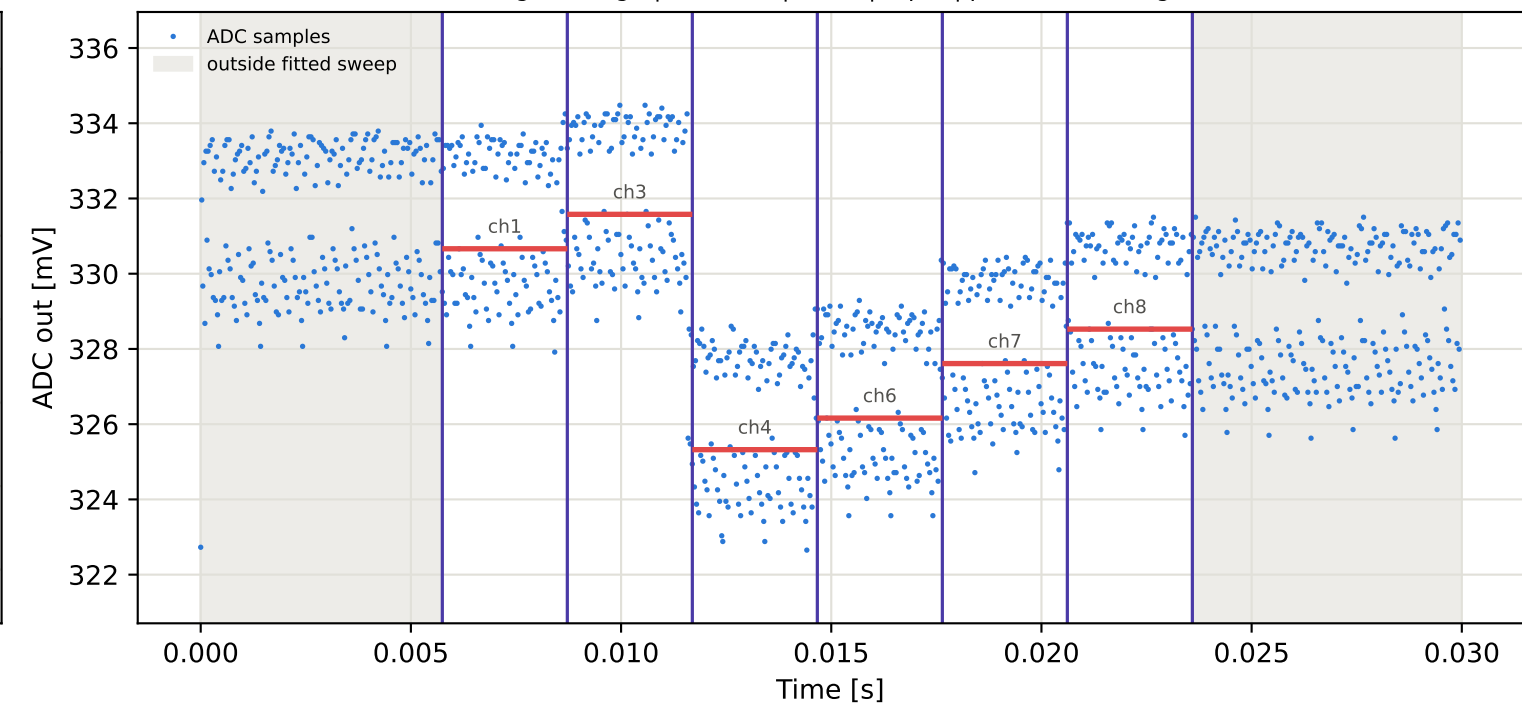
Tag3 &lt;- Tag15 | 825 MHz | run 0 | rep 1 | phase -89.19 deg
