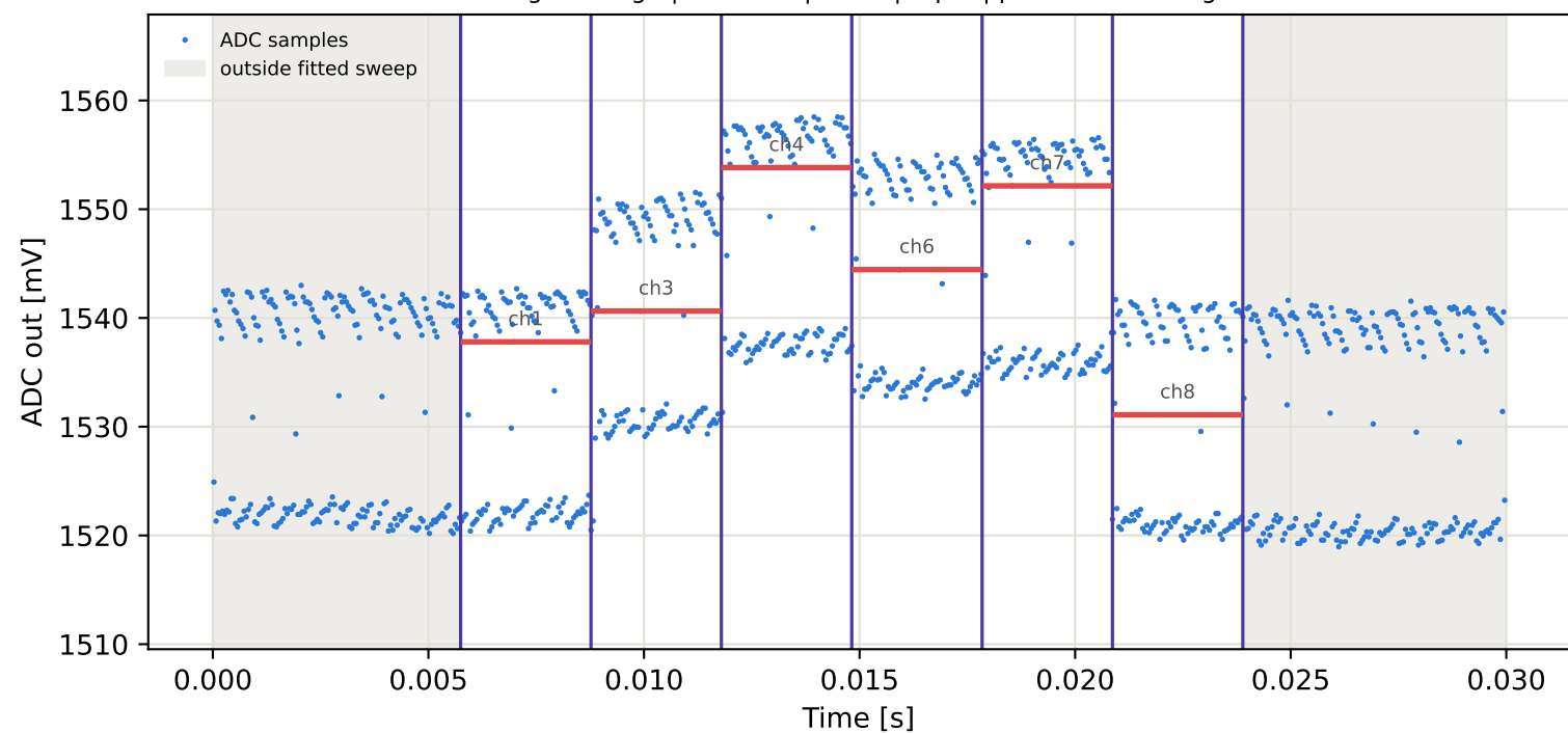
Tag2 &lt;- Tag6 | 895 MHz | run 0 | rep 1 | phase -27.12 deg
