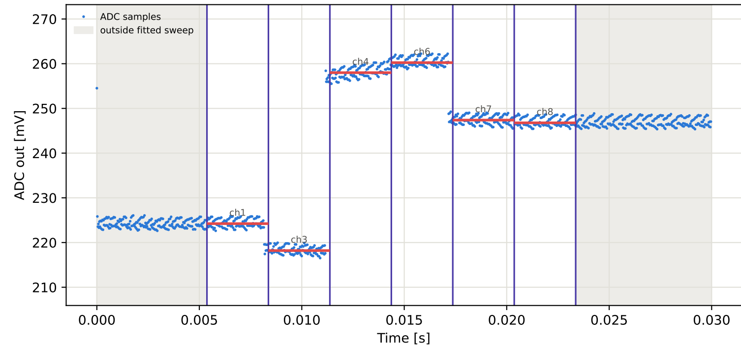
Tag9 &lt;- Tag2 | 835 MHz | run 0 | rep 1 | phase -11.69 deg
