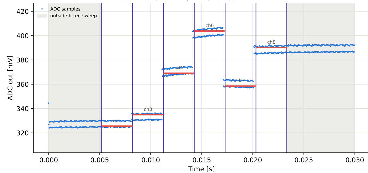
Tag4 &lt;- Tag7 | 865 MHz | run 0 | rep 1 | phase 3.56 deg
