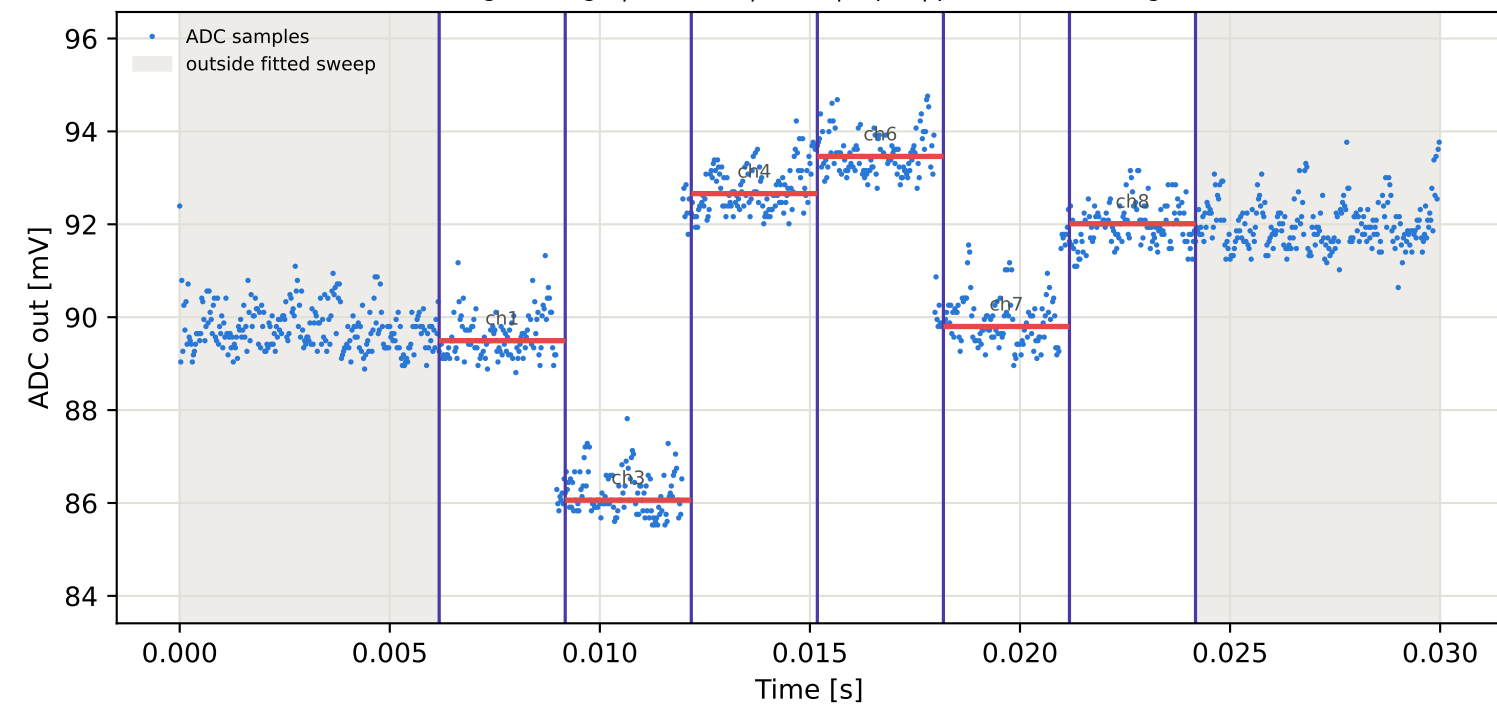
Tag7 &lt;- Tag1 | 785 MHz | run 0 | rep 1 | phase -45.21 deg
