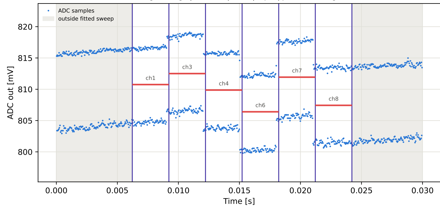
Tag8 &lt;- Tag10 | 875 MHz | run 0 | rep 1 | phase -166.83 deg
