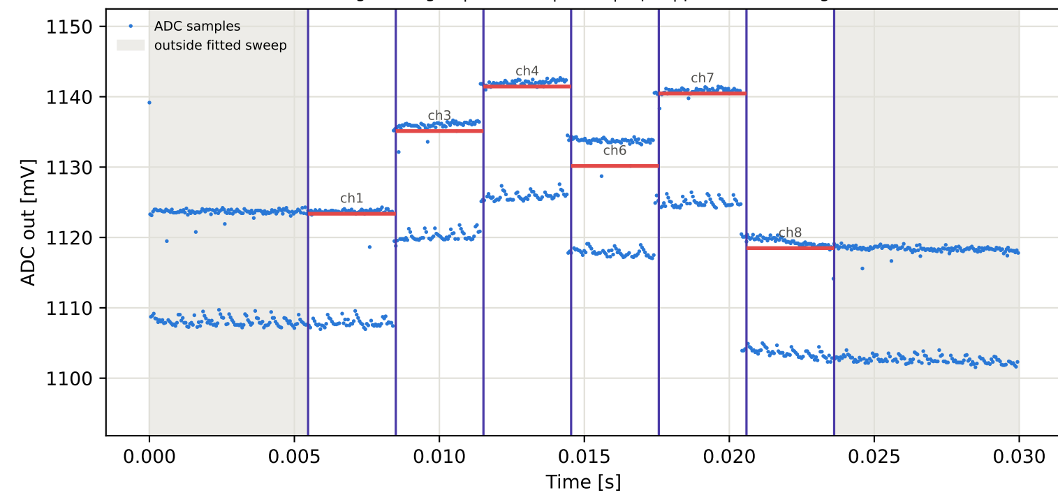
Tag7 &lt;- Tag15 | 895 MHz | run 0 | rep 1 | phase -75.55 deg
