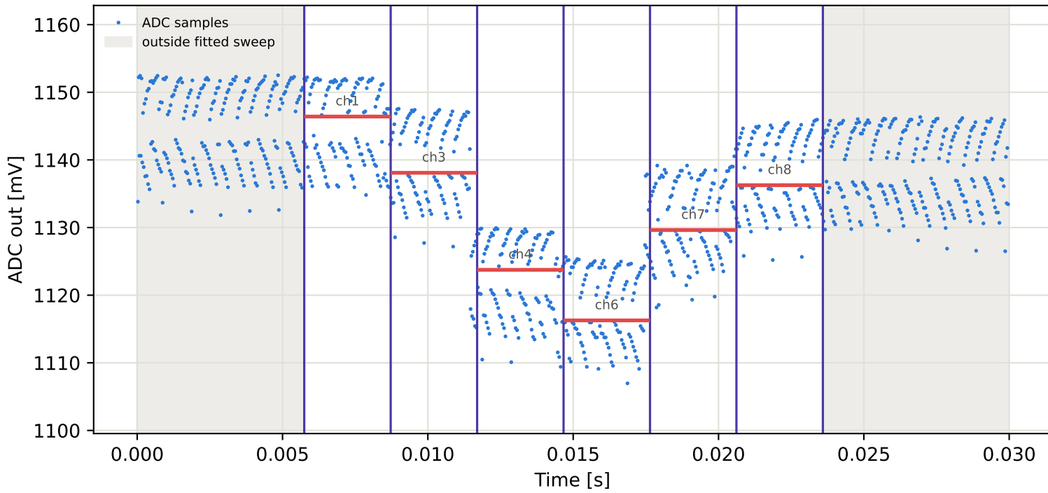
Tag2 &lt;- Tag16 | 945 MHz | run 0 | rep 1 | phase 44.15 deg
