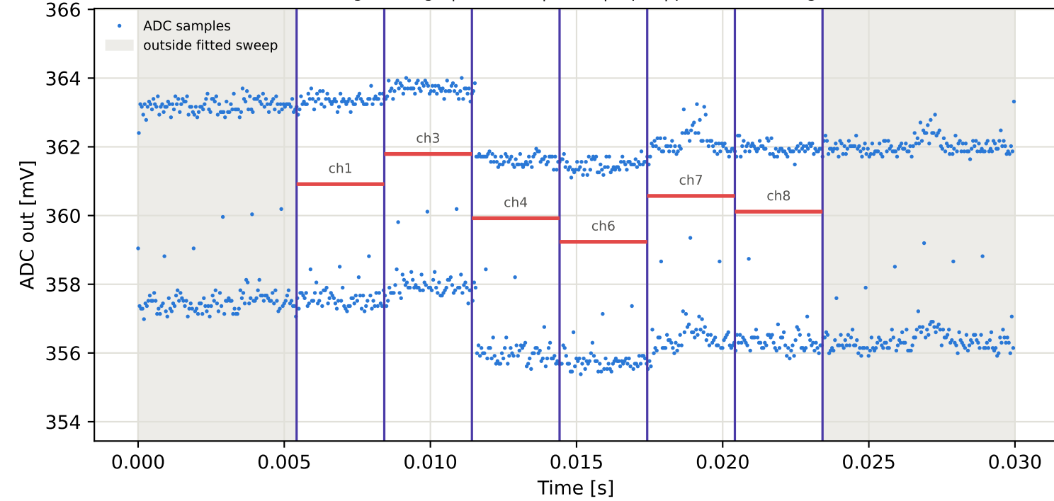
Tag2 &lt;- Tag6 | 825 MHz | run 0 | rep 1 | phase 84.95 deg
