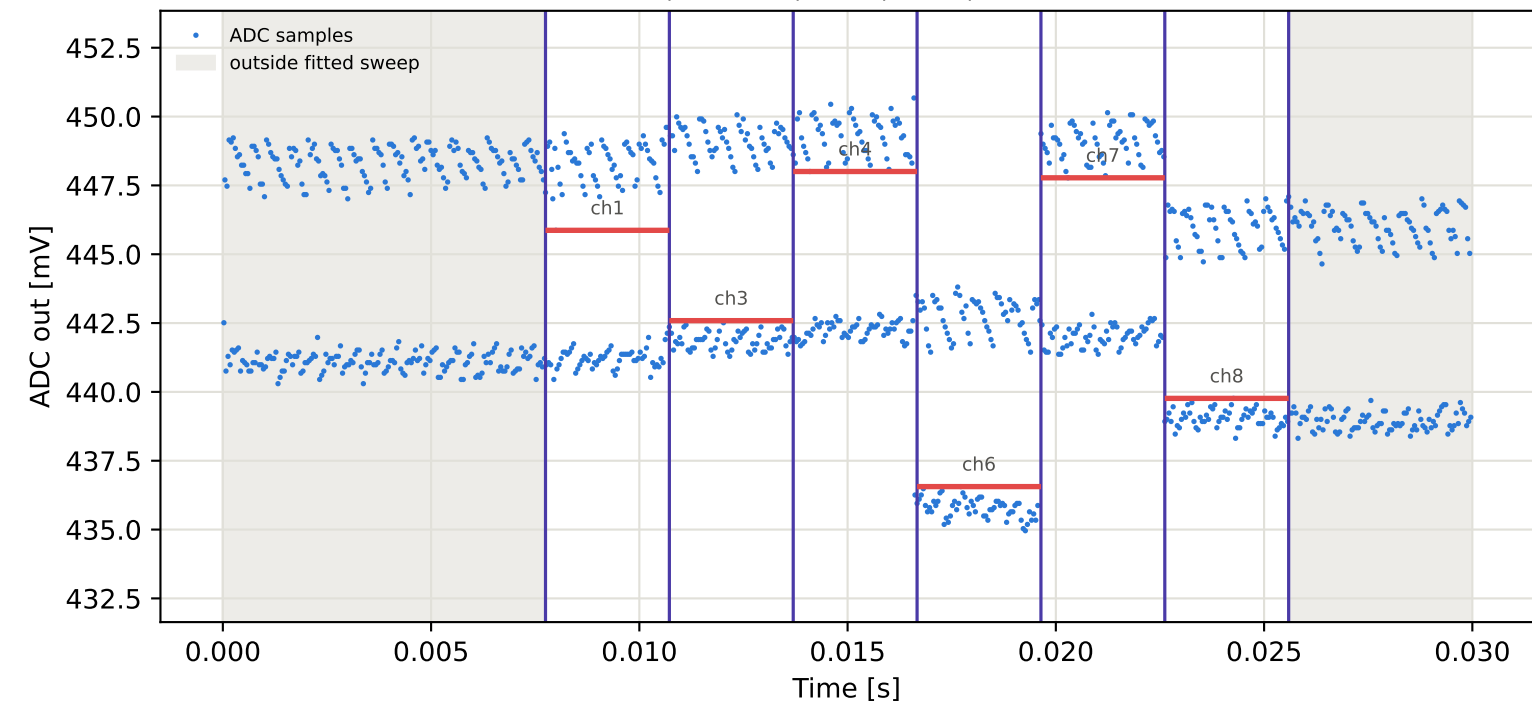
Tag9 &lt;- Tag2 | 965 MHz | run 0 | rep 1 | phase -32.89 deg
