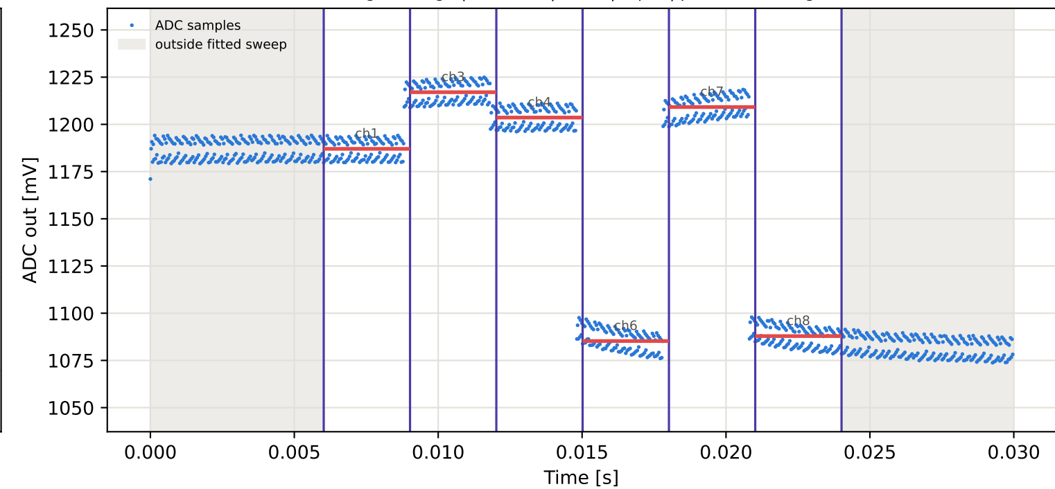
Tag3 &lt;- Tag7 | 895 MHz | run 0 | rep 1 | phase -79.61 deg
