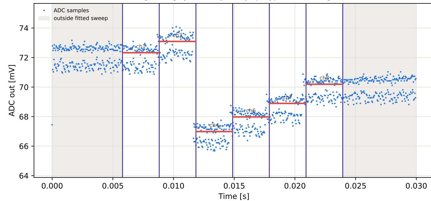
Tag1 &lt;- Tag7 | 795 MHz | run 0 | rep 1 | phase -65.90 deg
