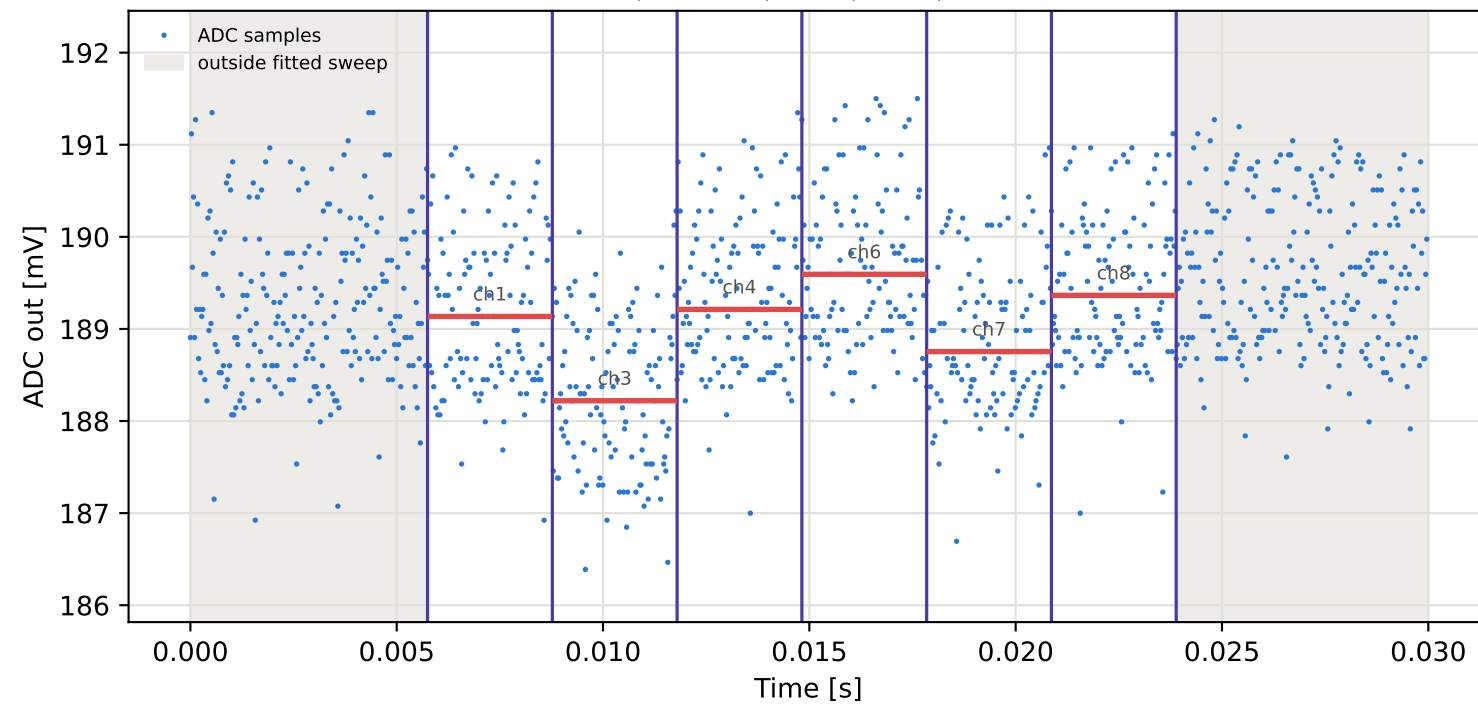
Tag16 &lt;- Tag10 | 795 MHz | run 0 | rep 1 | phase -155.63 deg
