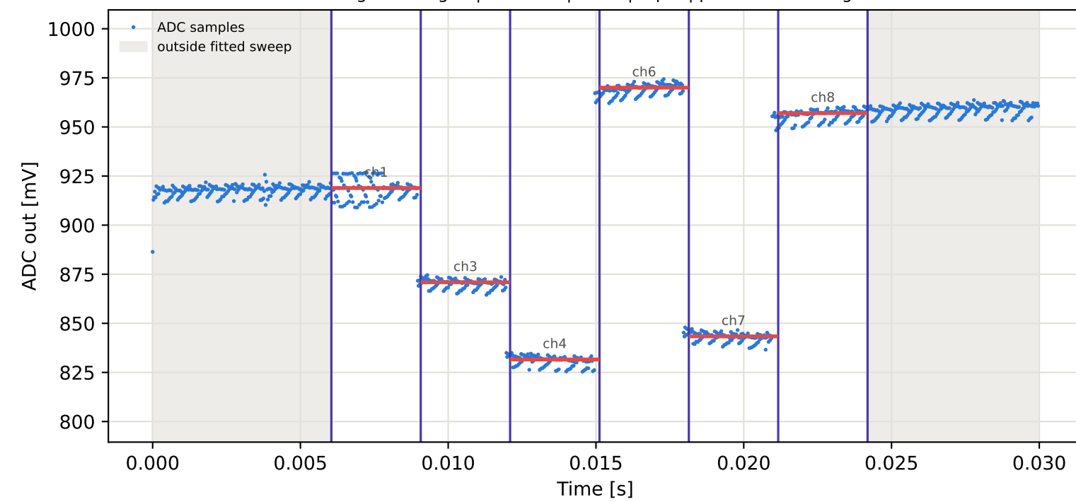
Tag15 &lt;- Tag3 | 985 MHz | run 0 | rep 1 | phase -22.84 deg
