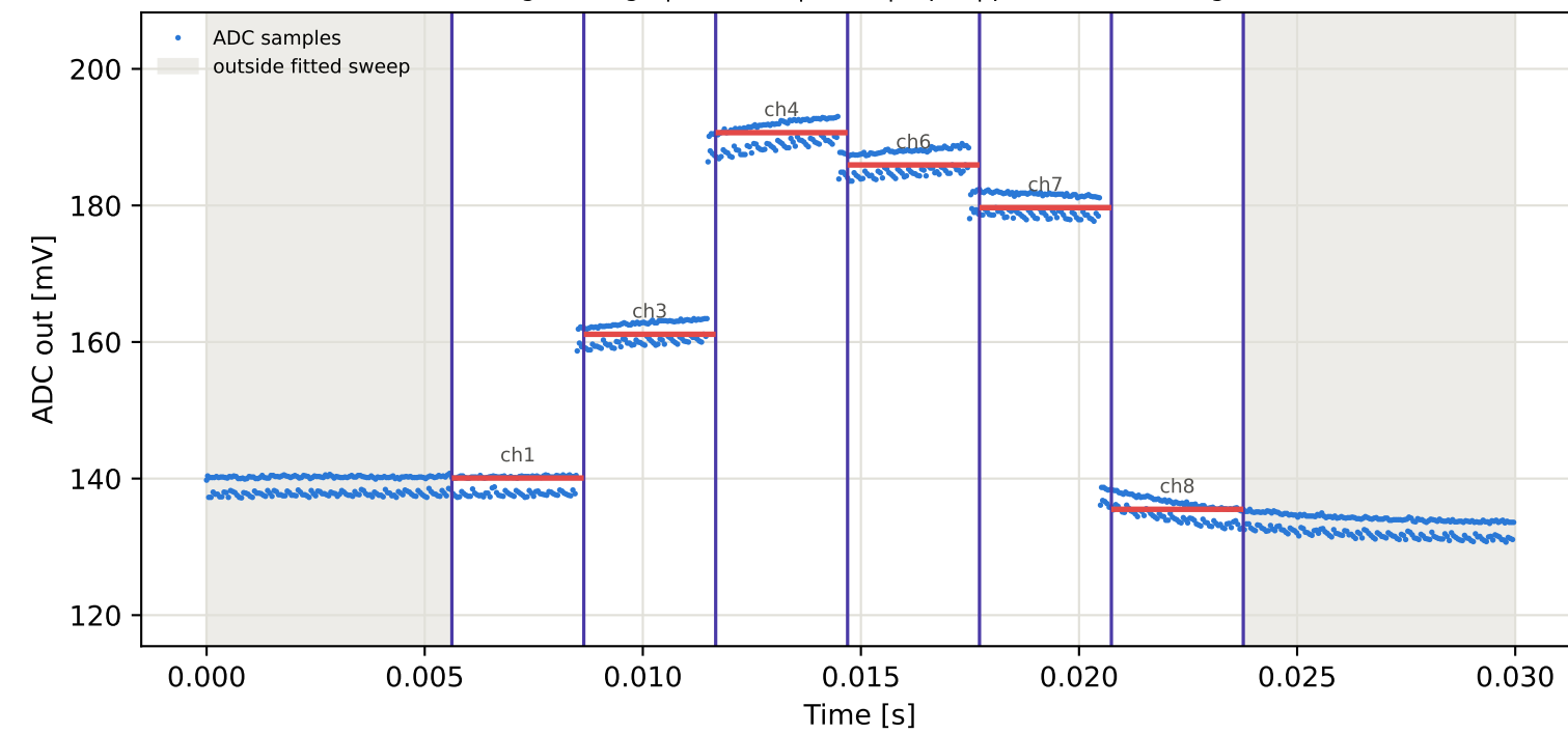
Tag1 &lt;- Tag7 | 915 MHz | run 0 | rep 1 | phase -163.62 deg
