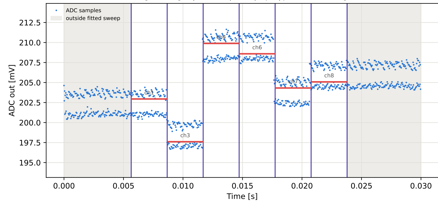
Tag15 &lt;- Tag3 | 785 MHz | run 0 | rep 1 | phase -66.36 deg
