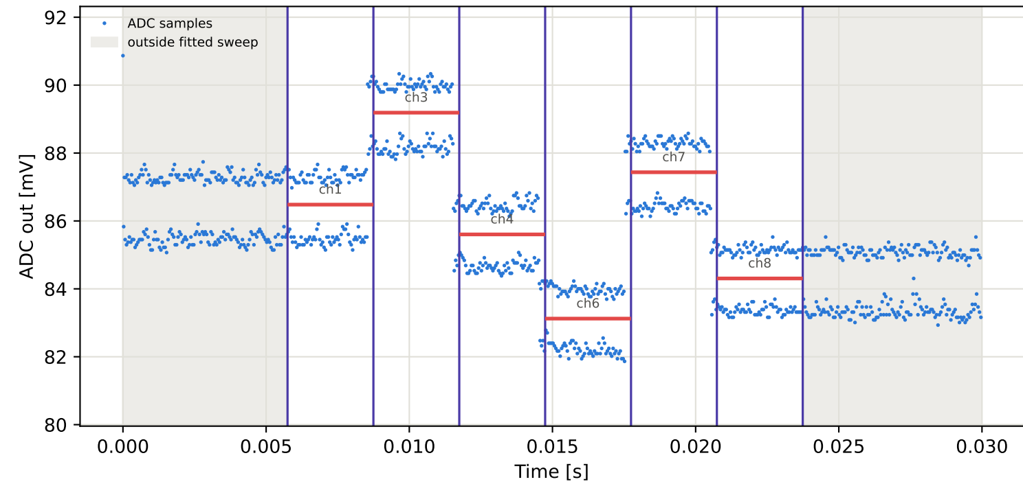
Tag9 &lt;- Tag8 | 785 MHz | run 0 | rep 1 | phase 18.73 deg
