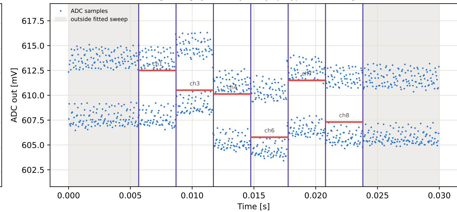
Tag3 &lt;- Tag15 | 845 MHz | run 0 | rep 1 | phase -93.14 deg
