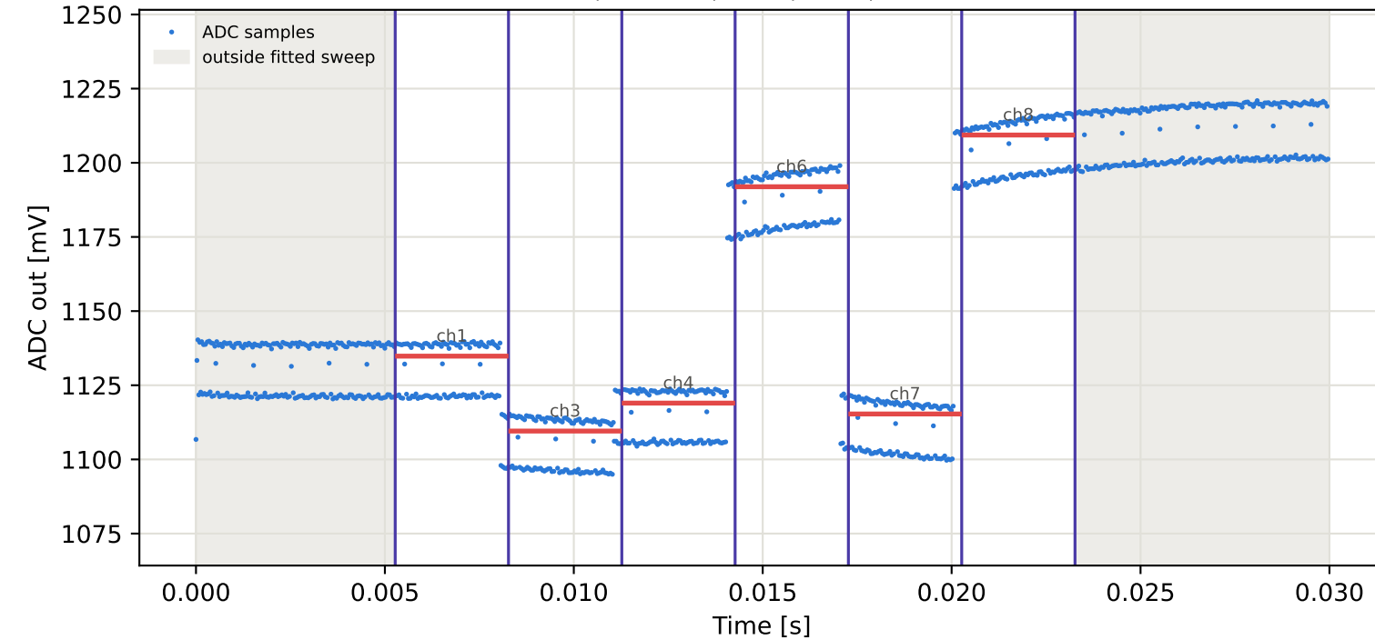
Tag3 &lt;- Tag8 | 895 MHz | run 0 | rep 1 | phase 165.18 deg
