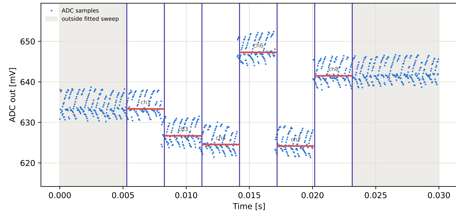
Tag8 &lt;- Tag6 | 965 MHz | run 0 | rep 1 | phase 152.32 deg
