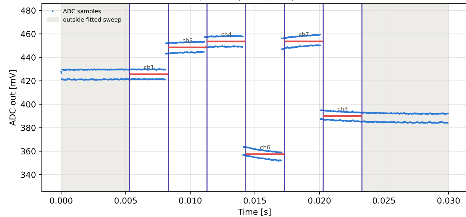
Tag9 &lt;- Tag5 | 965 MHz | run 0 | rep 1 | phase 16.66 deg
