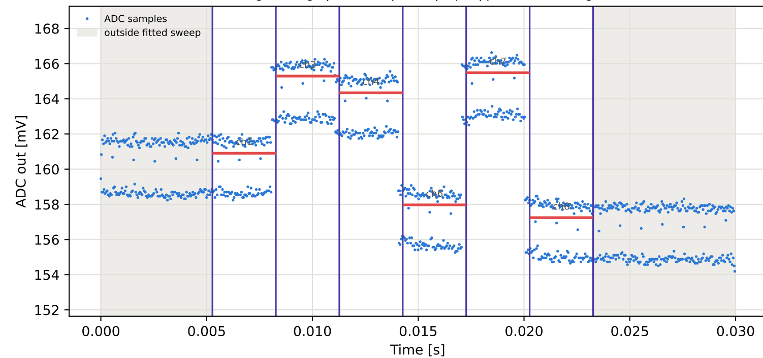
Tag4 &lt;- Tag9 | 825 MHz | run 0 | rep 1 | phase -24.20 deg
