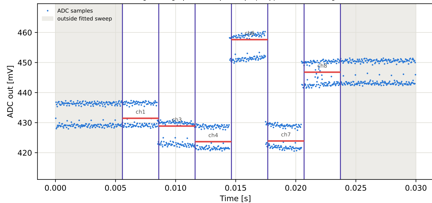
Tag3 &lt;- Tag2 | 935 MHz | run 0 | rep 1 | phase 161.57 deg
