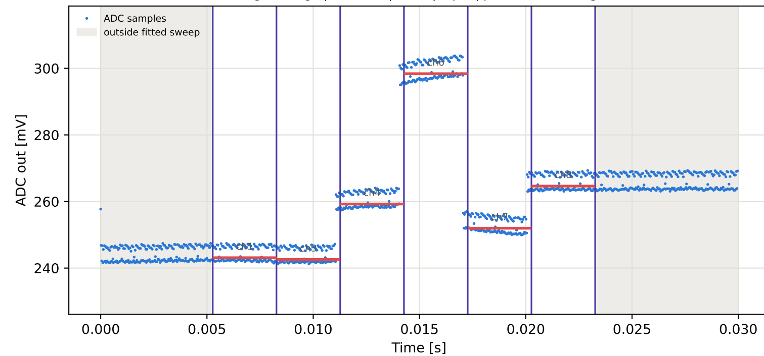
Tag3 &lt;- Tag6 | 925 MHz | run 0 | rep 1 | phase -1.69 deg
