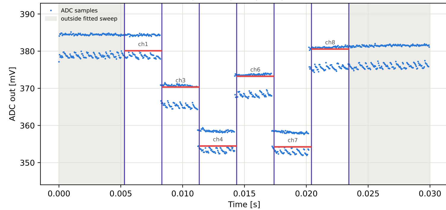
Tag2 &lt;- Tag15 | 825 MHz | run 0 | rep 1 | phase 106.31 deg
