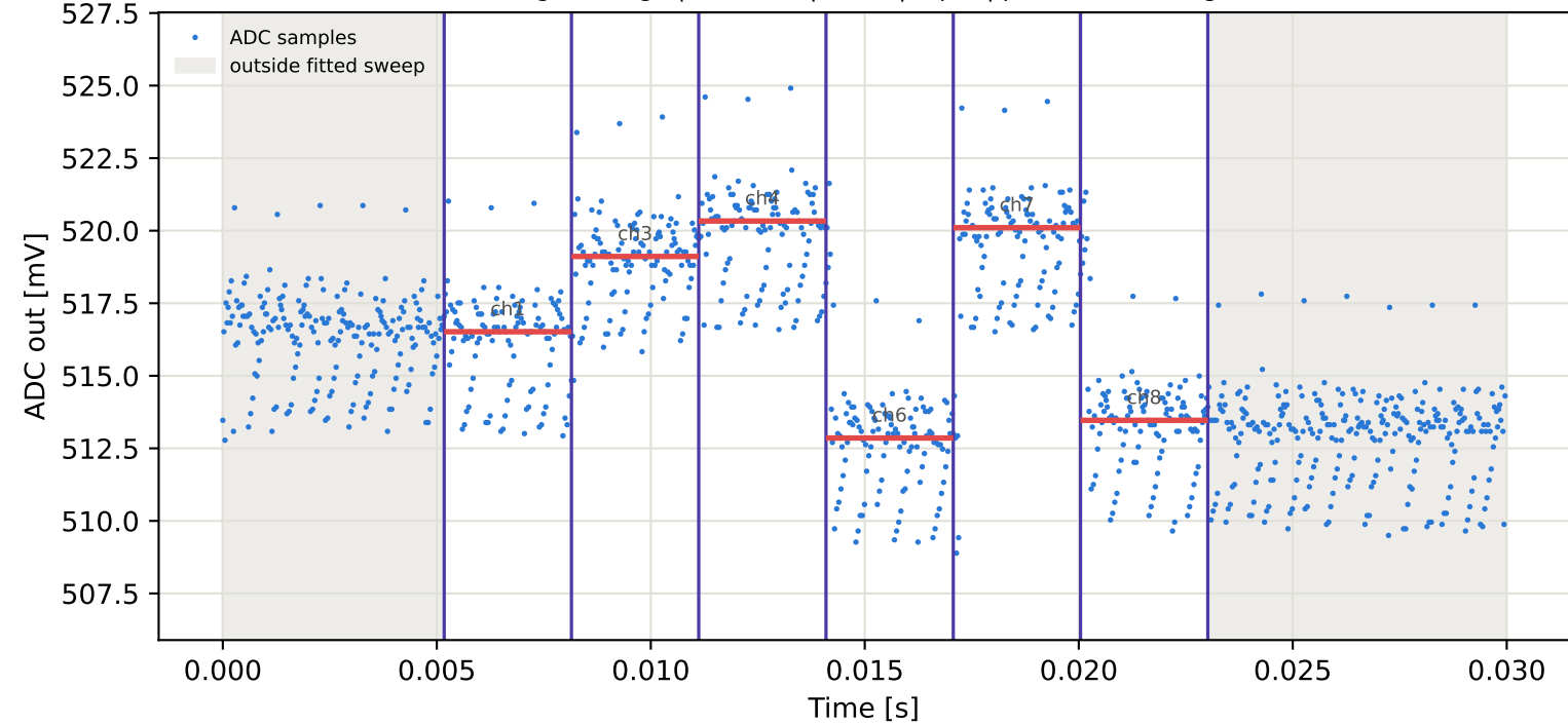
Tag5 &lt;- Tag9 | 935 MHz | run 0 | rep 1 | phase -24.87 deg
