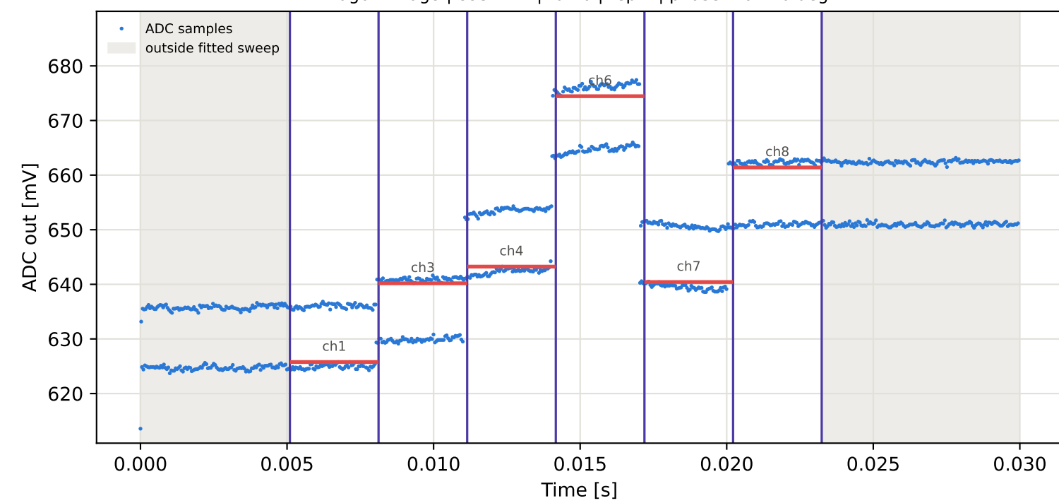
Tag7 &lt;- Tag1 | 895 MHz | run 0 | rep 1 | phase -86.21 deg
