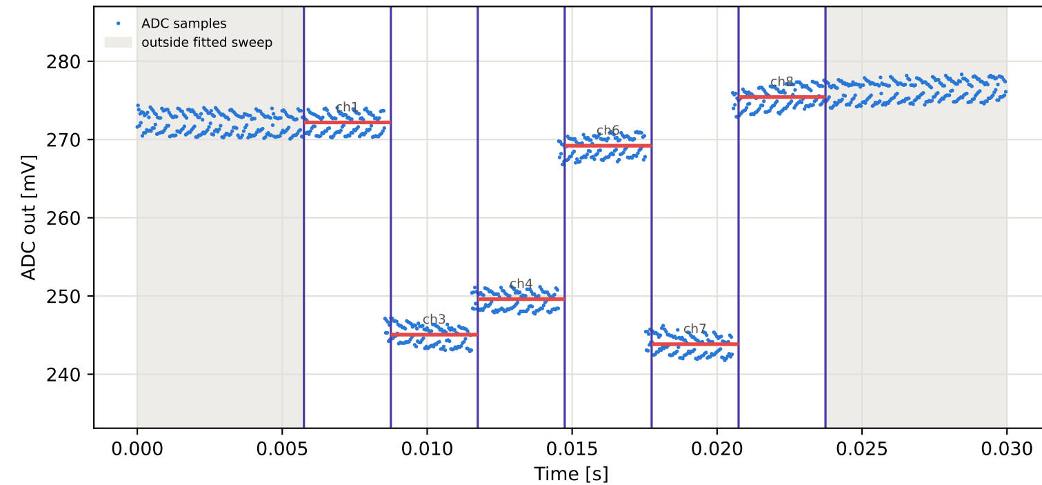
Tag9 &lt;- Tag7 | 835 MHz | run 0 | rep 1 | phase -177.16 deg
