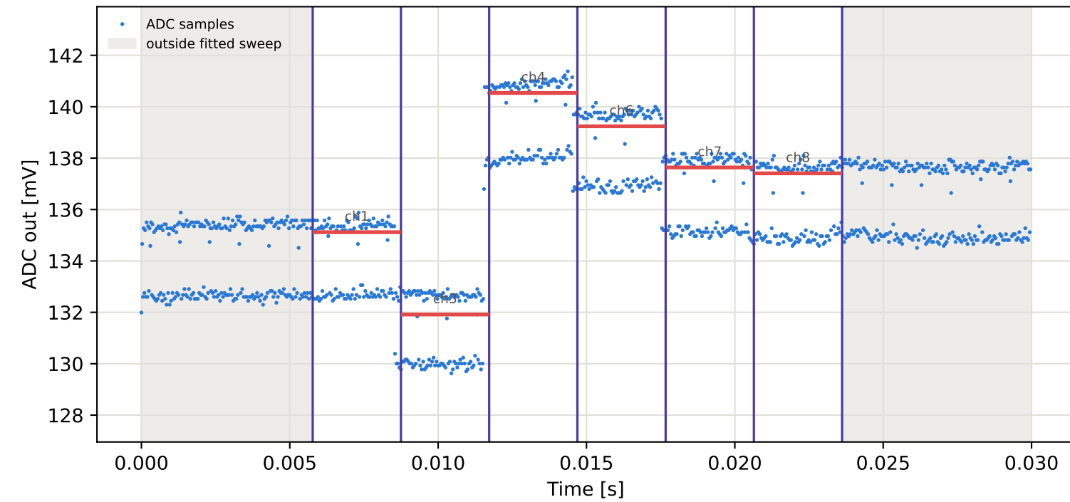
Tag6 &lt;- Tag1 | 775 MHz | run 0 | rep 1 | phase 71.55 deg
