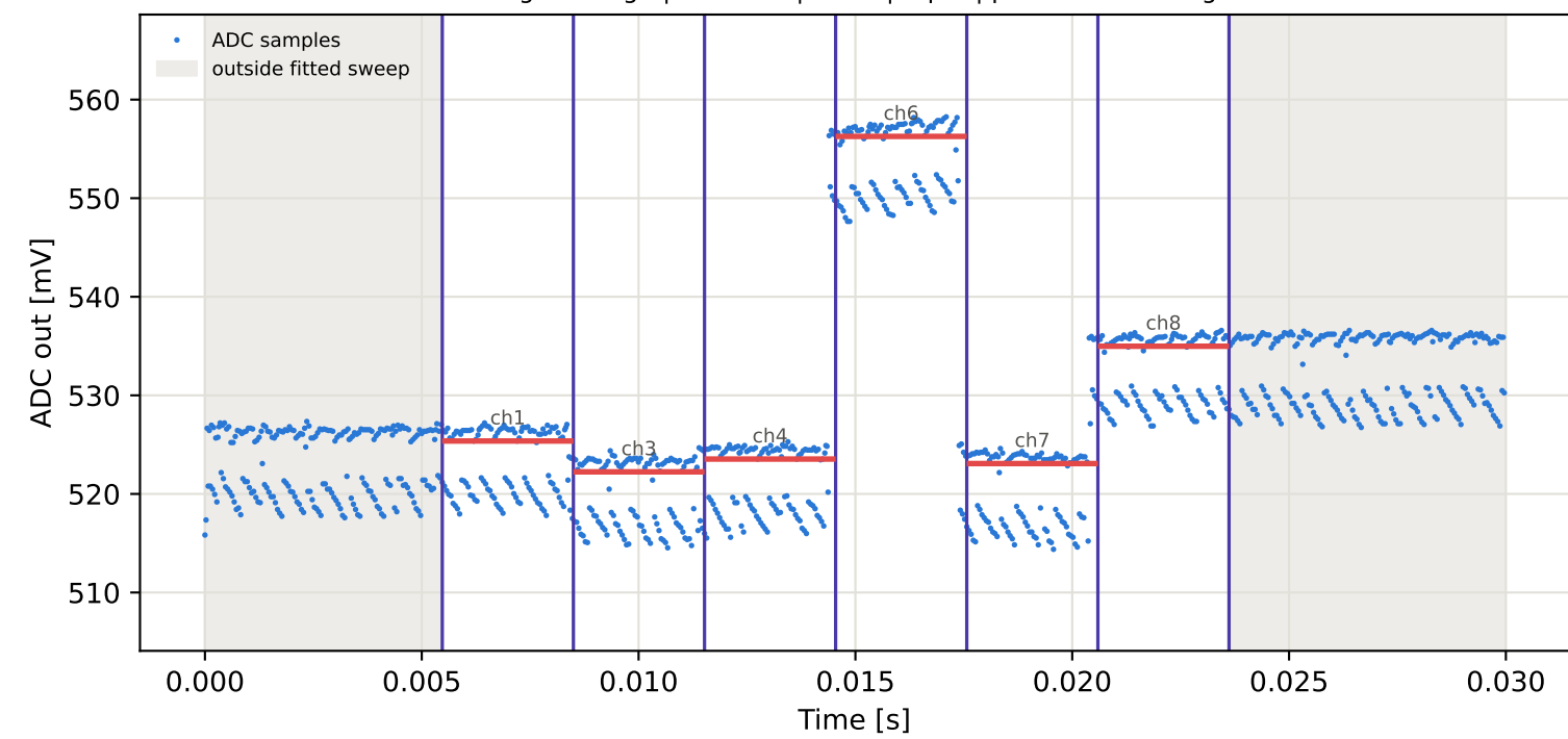
Tag7 &lt;- Tag4 | 985 MHz | run 0 | rep 1 | phase 32.21 deg
