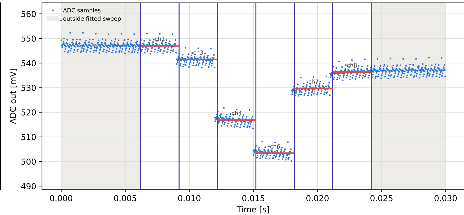
Tag10 &lt;- Tag1 | 945 MHz | run 0 | rep 1 | phase 103.20 deg
