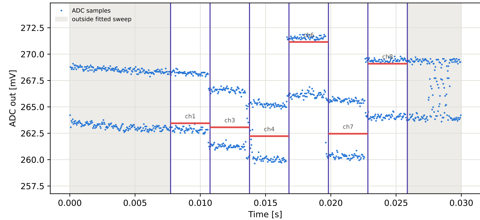
Tag5 &lt;- Tag4 | 965 MHz | run 0 | rep 1 | phase -5.43 deg
