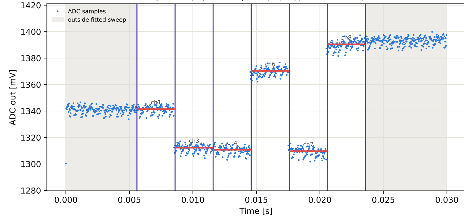
Tag15 &lt;- Tag5 | 885 MHz | run 0 | rep 1 | phase -140.76 deg
