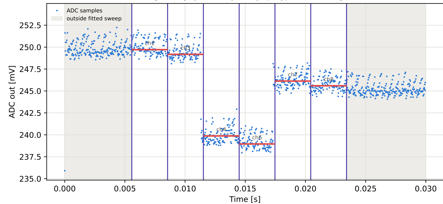
Tag6 &lt;- Tag9 | 995 MHz | run 0 | rep 1 | phase 175.69 deg
