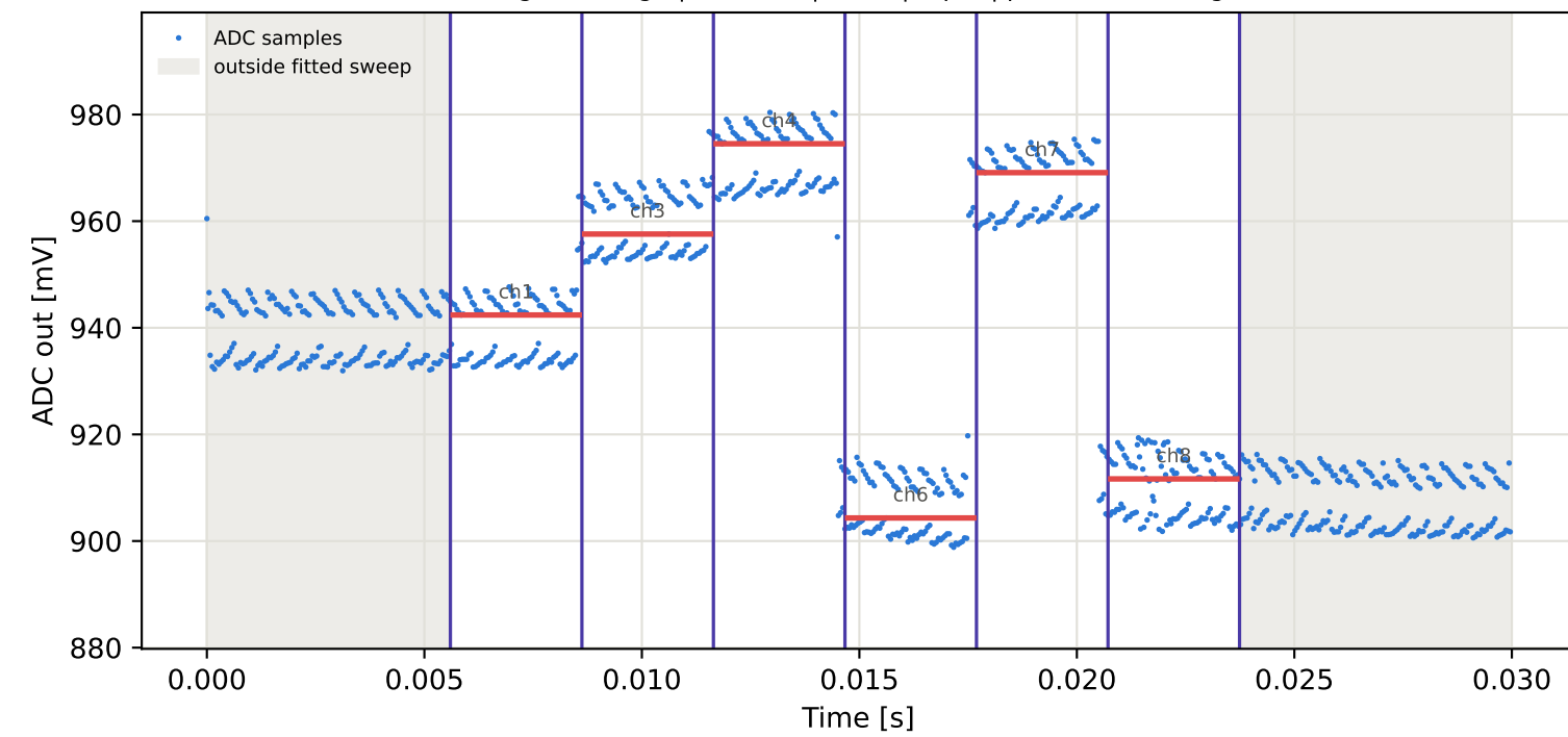
Tag16 &lt;- Tag4 | 935 MHz | run 0 | rep 1 | phase 131.19 deg
