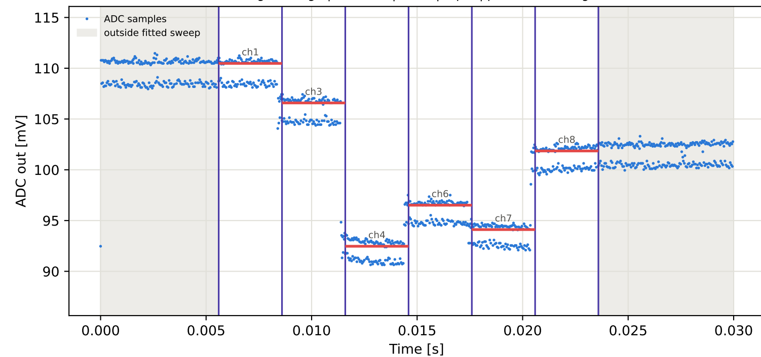
Tag1 &lt;- Tag3 | 825 MHz | run 0 | rep 1 | phase 69.89 deg
