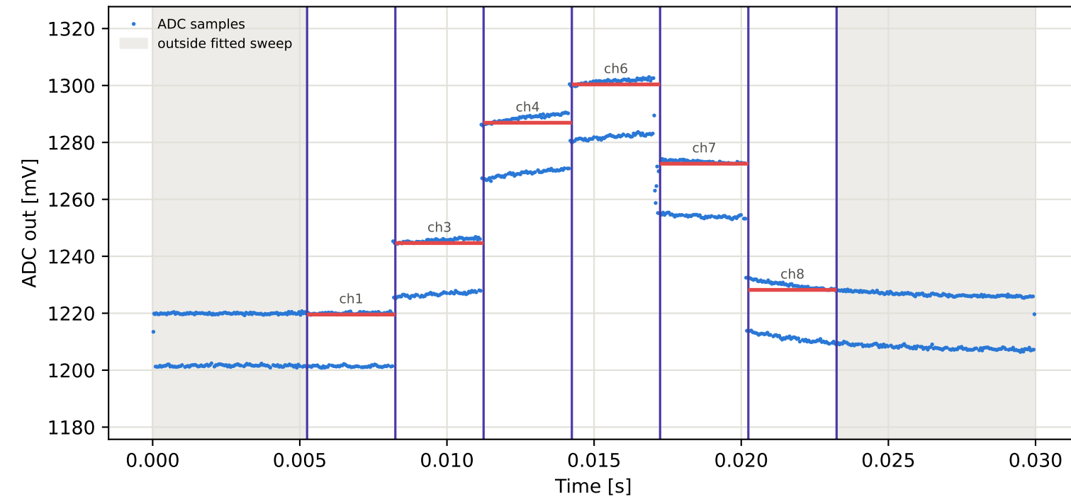
Tag15 &lt;- Tag5 | 915 MHz | run 0 | rep 1 | phase -1.84 deg
