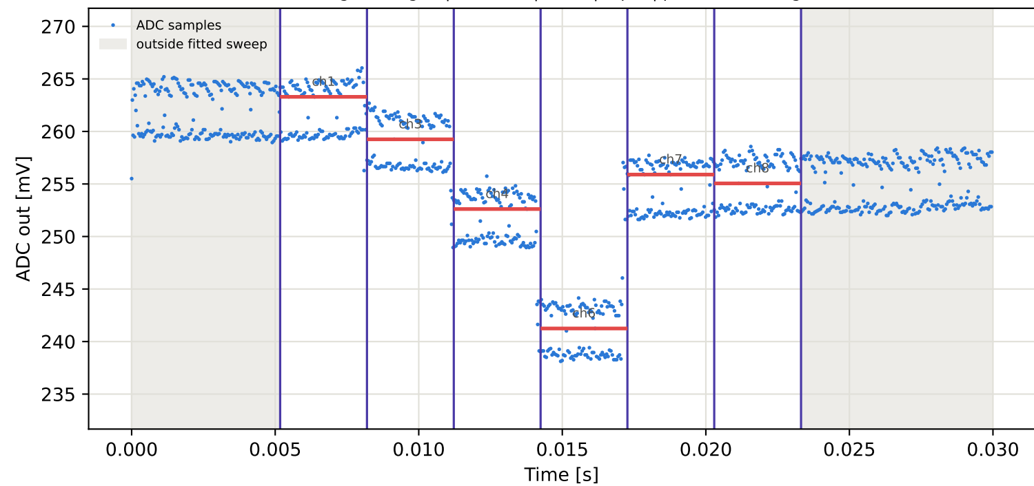
Tag6 &lt;- Tag2 | 915 MHz | run 0 | rep 1 | phase -154.39 deg
