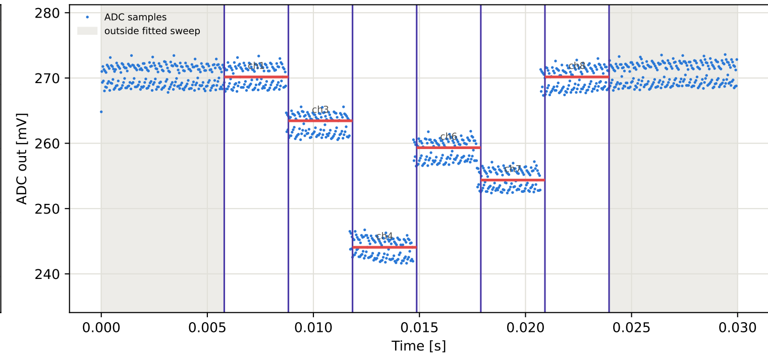
Tag10 &lt;- Tag1 | 965 MHz | run 0 | rep 1 | phase 155.66 deg
