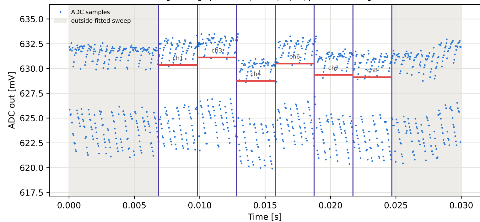
Tag2 &lt;- Tag6 | 965 MHz | run 0 | rep 1 | phase 19.55 deg
