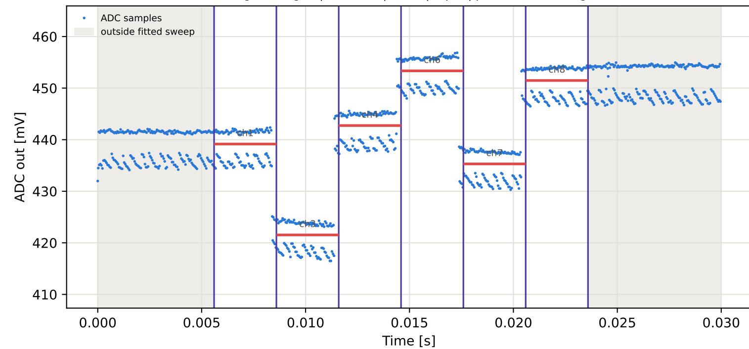
Tag6 &lt;- Tag3 | 835 MHz | run 0 | rep 1 | phase 145.52 deg
