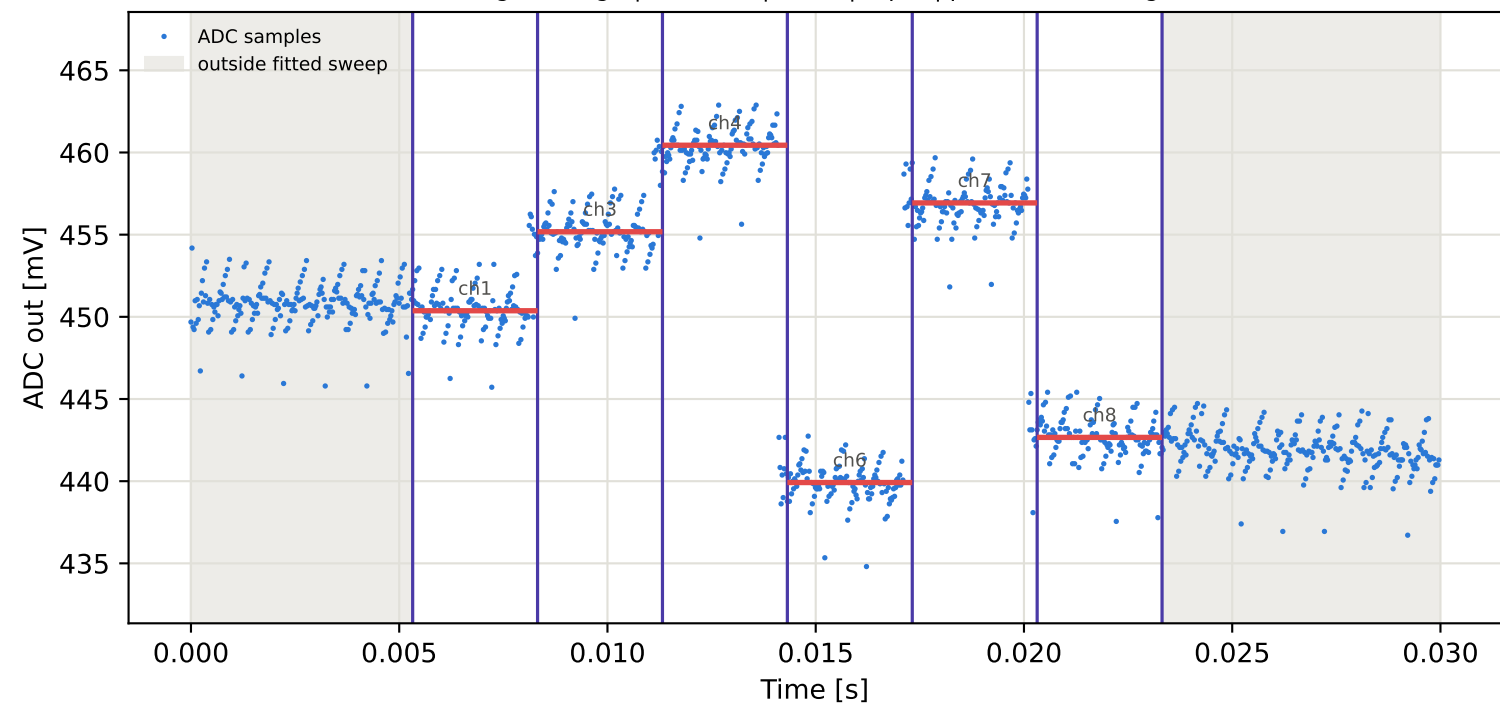
Tag8 &lt;- Tag4 | 975 MHz | run 0 | rep 1 | phase 0.39 deg
