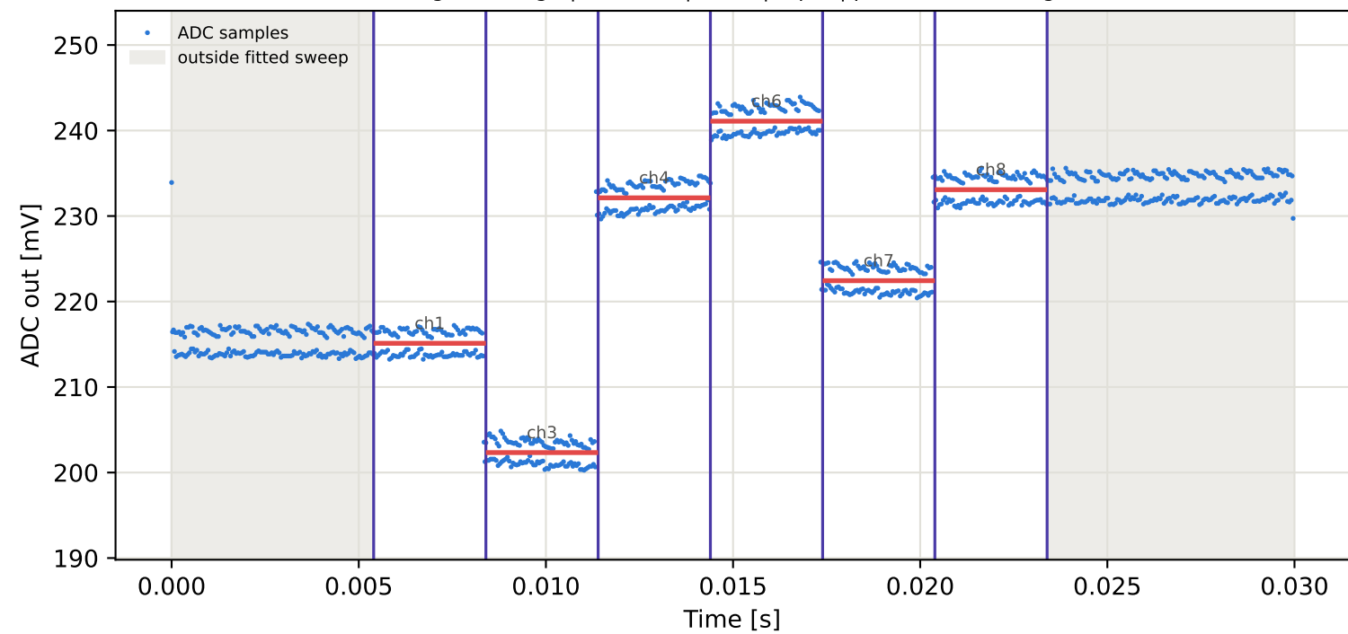
Tag10 &lt;- Tag8 | 825 MHz | run 0 | rep 1 | phase -149.36 deg
