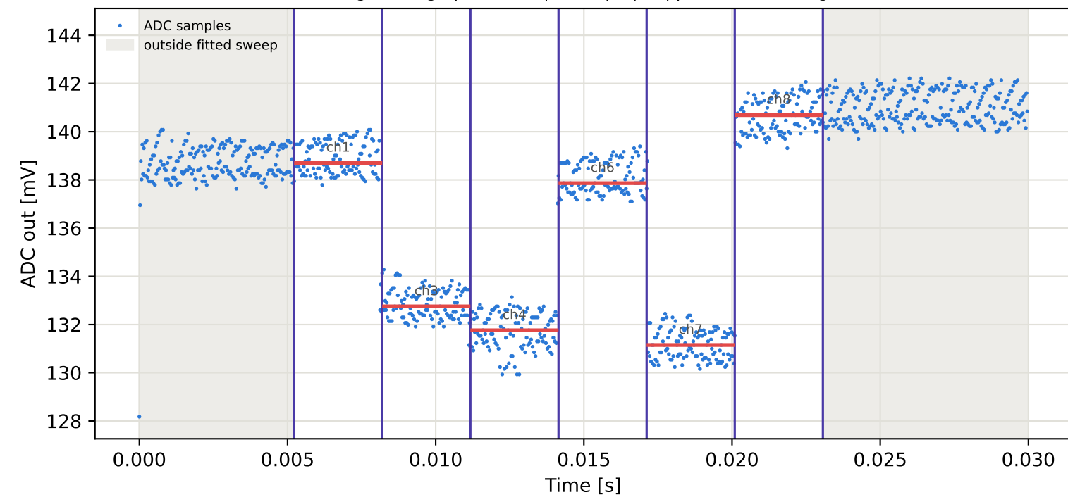
Tag7 &lt;- Tag4 | 785 MHz | run 0 | rep 1 | phase 92.66 deg
