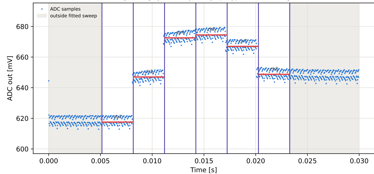
Tag3 &lt;- Tag7 | 865 MHz | run 0 | rep 1 | phase -136.42 deg
