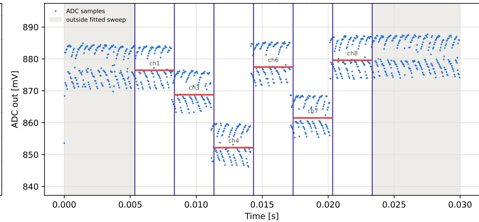
Tag15 &lt;- Tag10 | 985 MHz | run 0 | rep 1 | phase 97.17 deg
