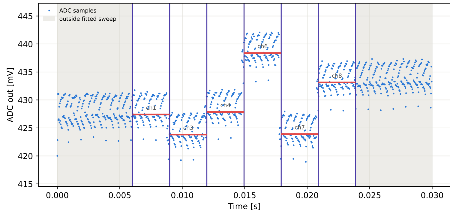
Tag16 &lt;- Tag6 | 995 MHz | run 0 | rep 1 | phase 177.08 deg
