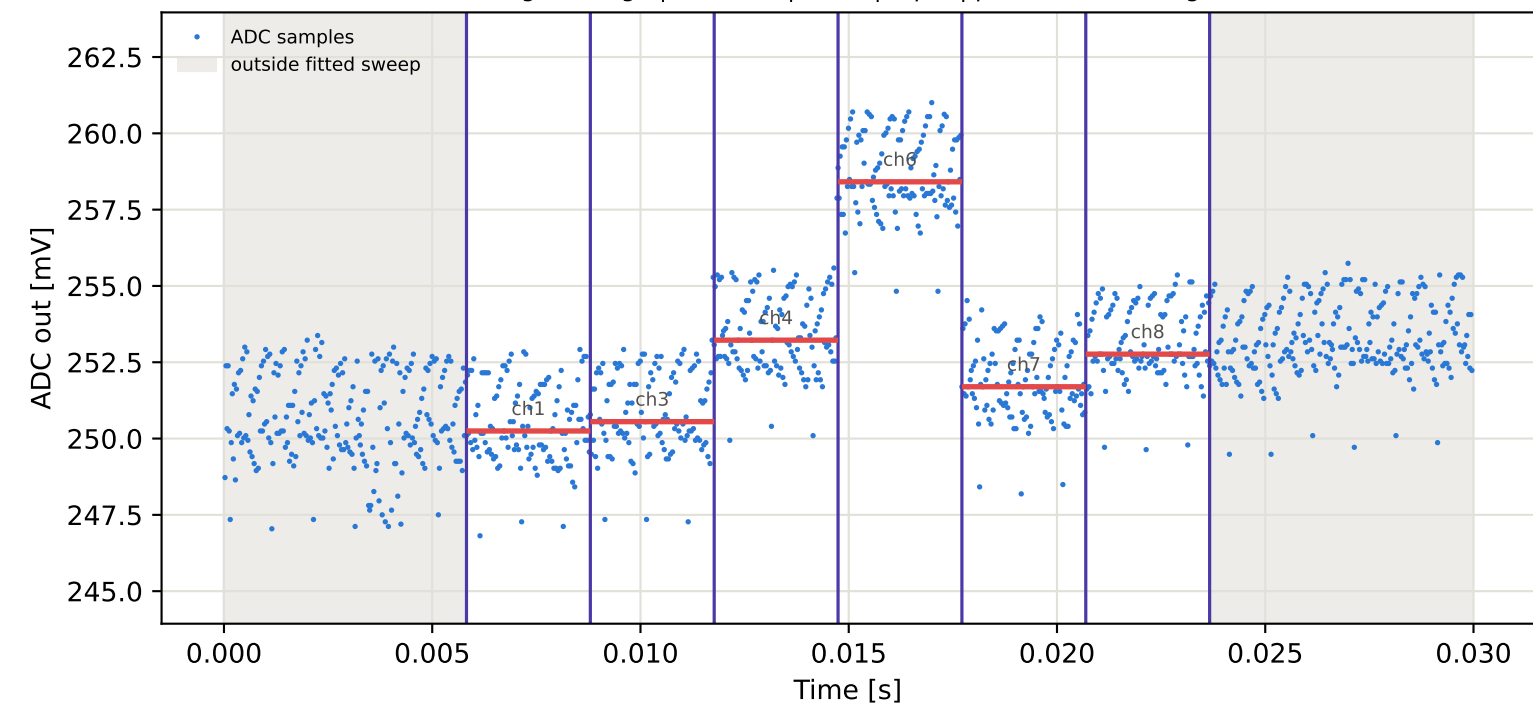
Tag6 &lt;- Tag4 | 915 MHz | run 0 | rep 1 | phase -119.32 deg
