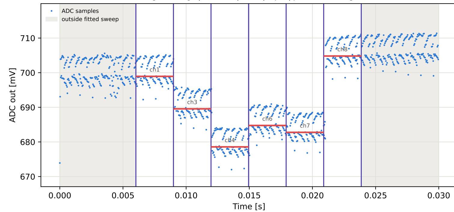
Tag16 &lt;- Tag4 | 845 MHz | run 0 | rep 1 | phase -75.30 deg
