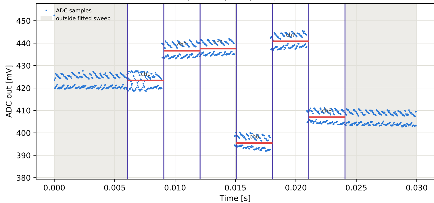
Tag10 &lt;- Tag3 | 985 MHz | run 0 | rep 1 | phase 68.45 deg
