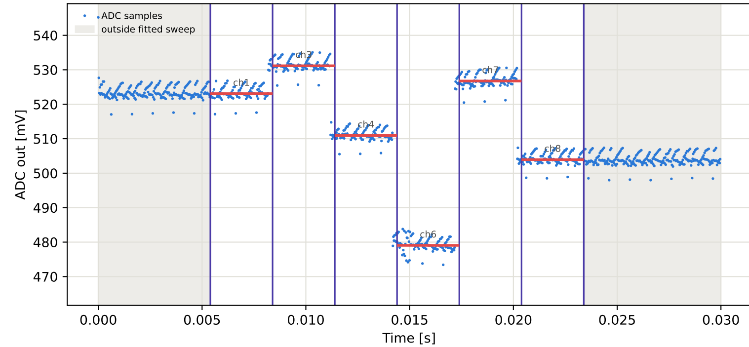
Tag9 &lt;- Tag7 | 985 MHz | run 0 | rep 1 | phase 24.75 deg
