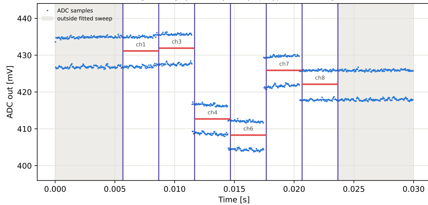
Tag2 &lt;- Tag1 | 995 MHz | run 0 | rep 1 | phase 103.79 deg
