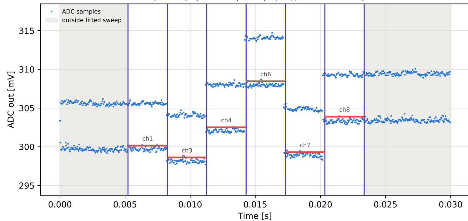
Tag8 &lt;- Tag7 | 985 MHz | run 0 | rep 1 | phase 94.77 deg
