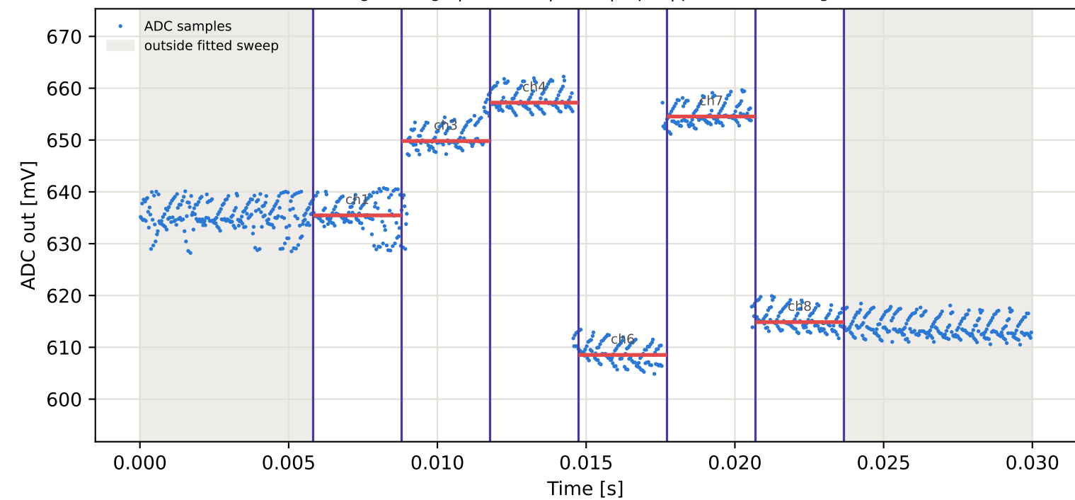
Tag9 &lt;- Tag8 | 925 MHz | run 0 | rep 1 | phase -148.34 deg
