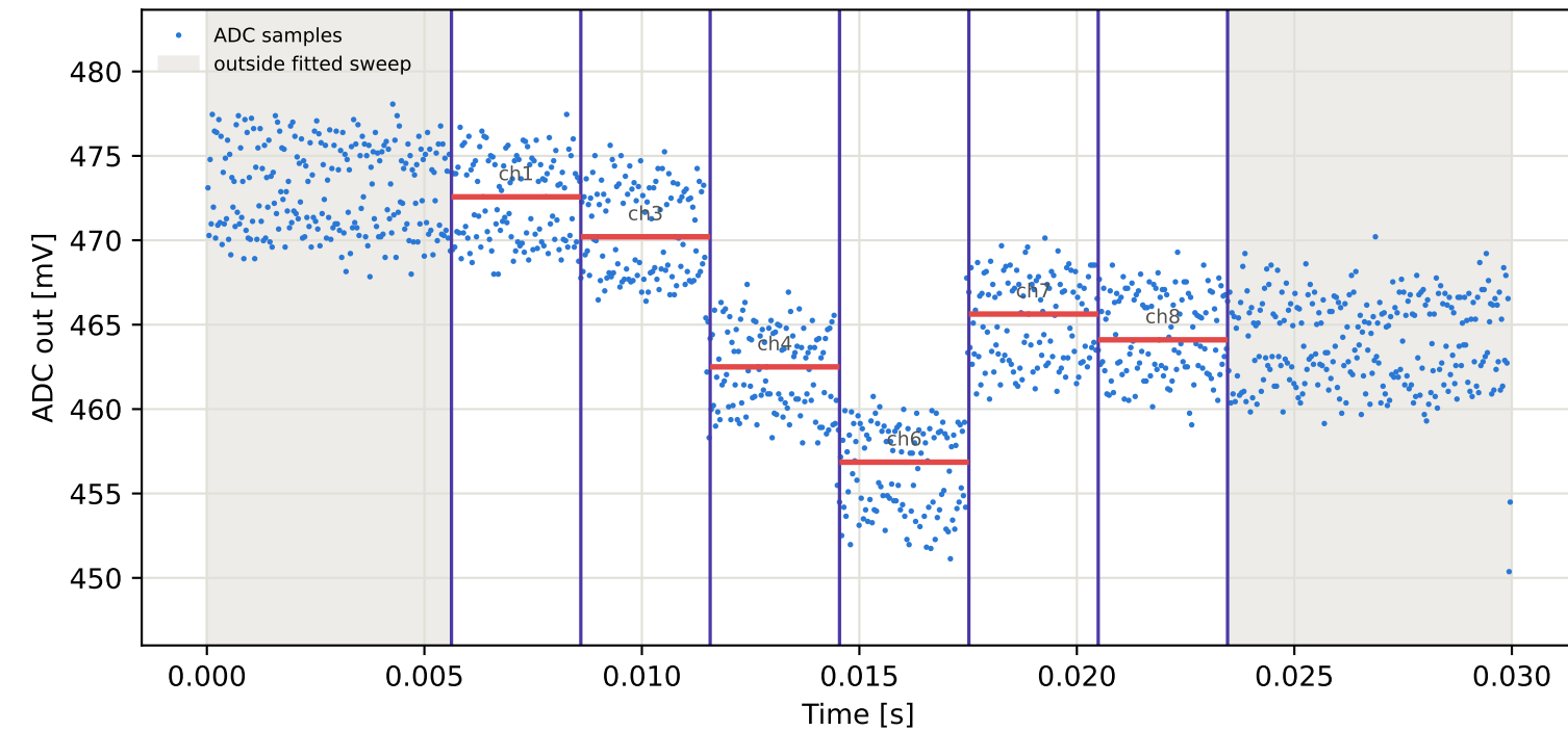
Tag4 &lt;- Tag9 | 885 MHz | run 0 | rep 1 | phase 27.79 deg
