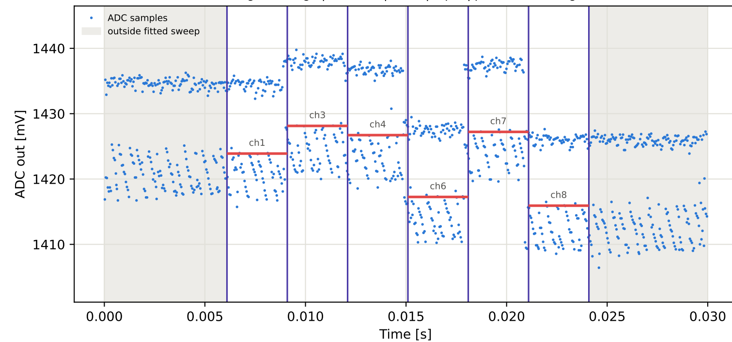
Tag16 &lt;- Tag6 | 885 MHz | run 0 | rep 1 | phase 165.95 deg
