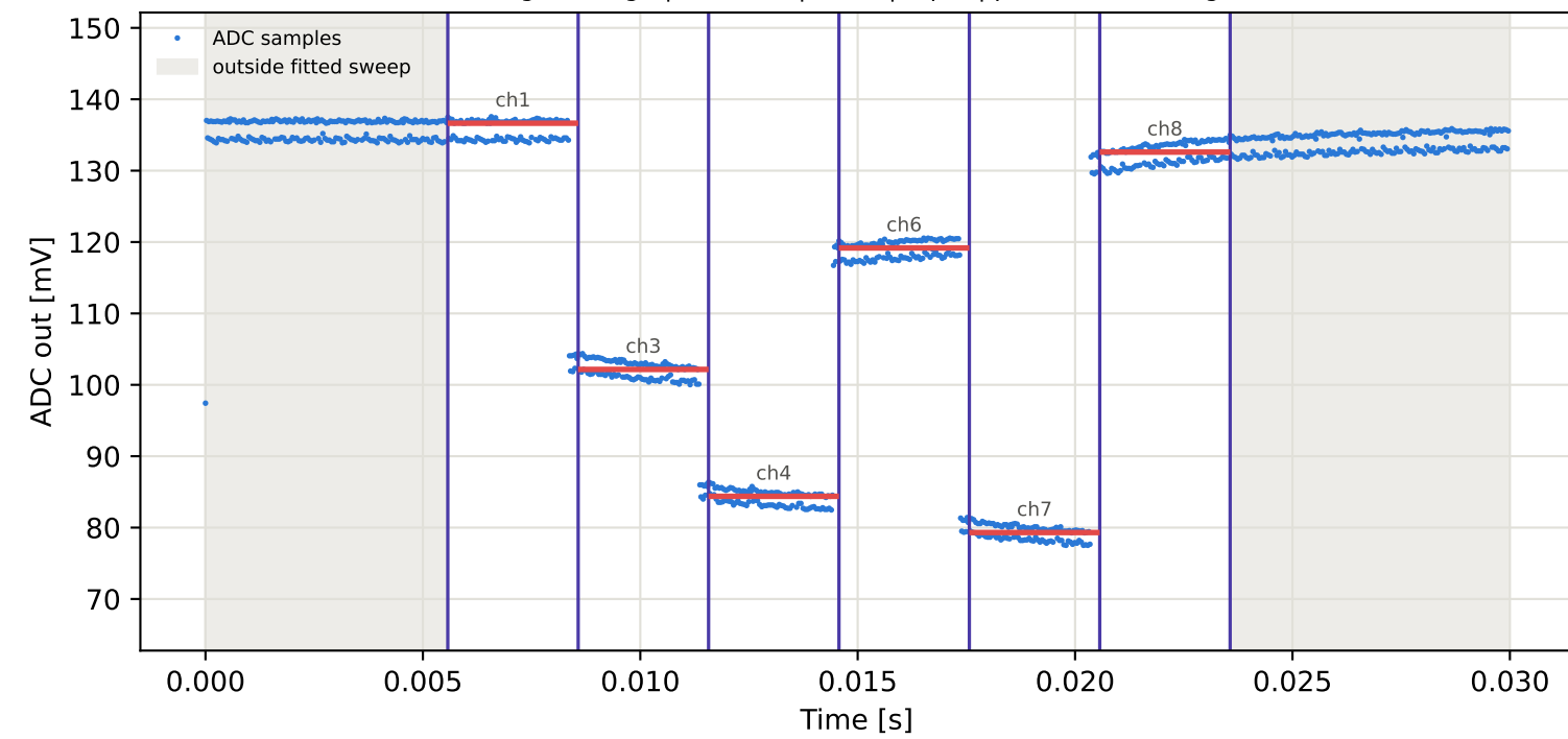
Tag1 &lt;- Tag8 | 825 MHz | run 0 | rep 1 | phase -98.48 deg
