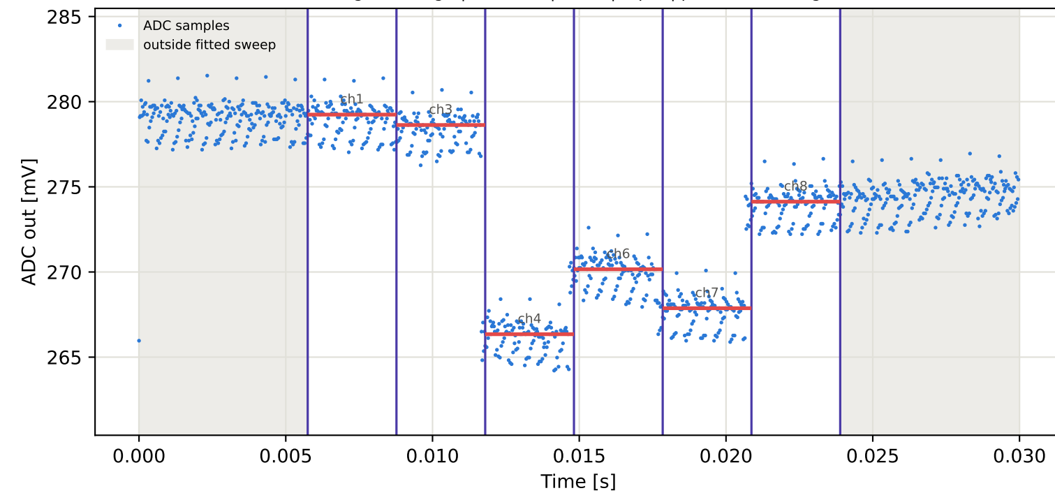
Tag2 &lt;- Tag1 | 805 MHz | run 0 | rep 1 | phase -132.30 deg
