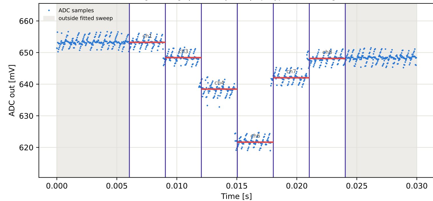
Tag16 &lt;- Tag4 | 835 MHz | run 0 | rep 1 | phase -159.57 deg
