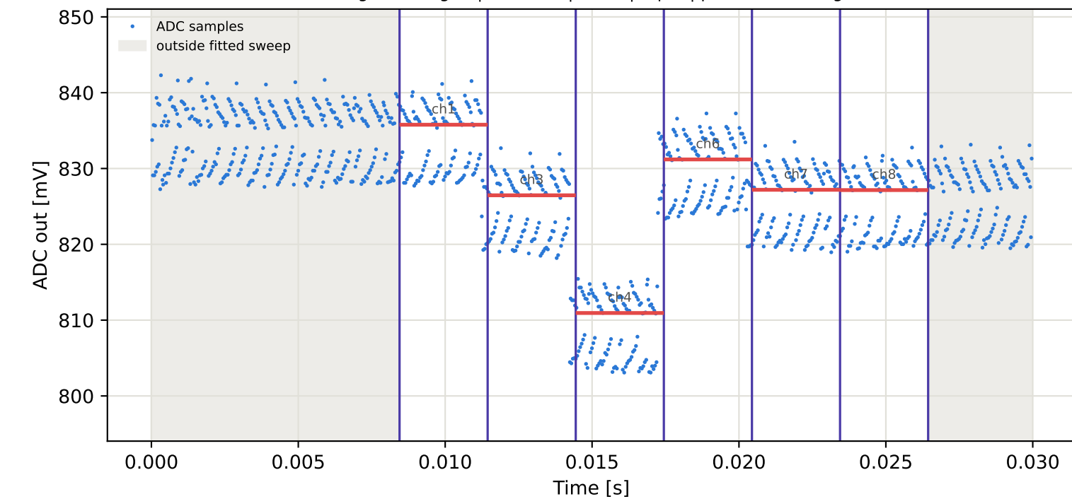
Tag15 &lt;- Tag10 | 935 MHz | run 0 | rep 1 | phase 80.70 deg
