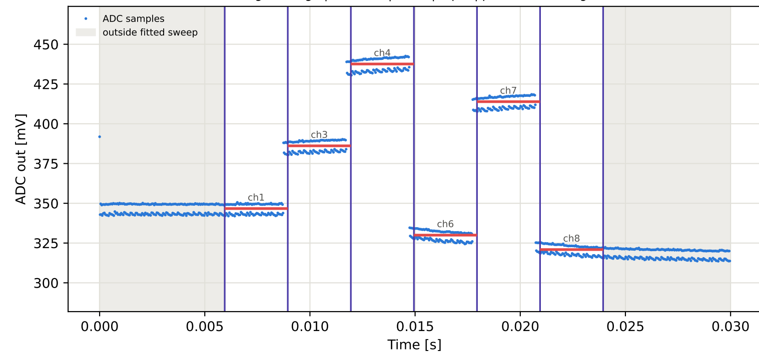
Tag3 &lt;- Tag8 | 965 MHz | run 0 | rep 1 | phase -68.01 deg
