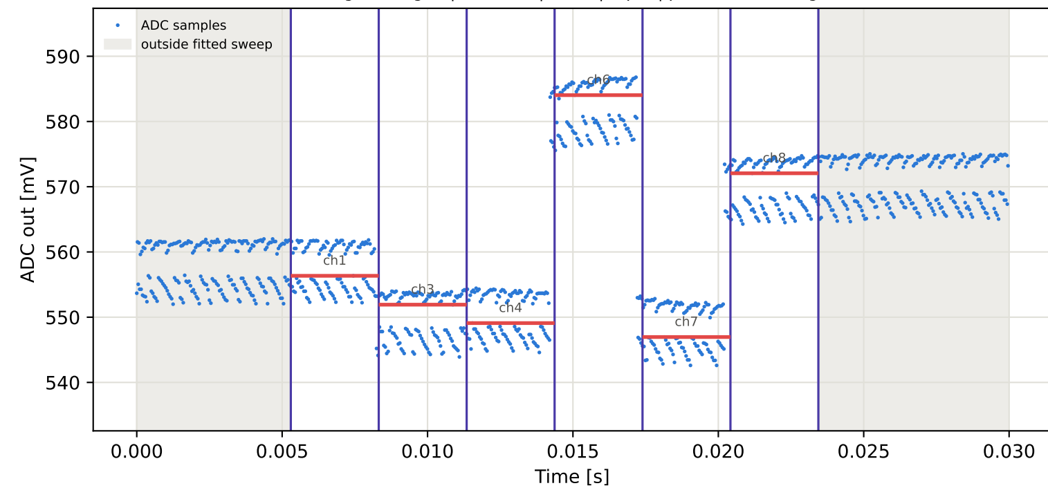
Tag4 &lt;- Tag16 | 955 MHz | run 0 | rep 1 | phase 4.81 deg
