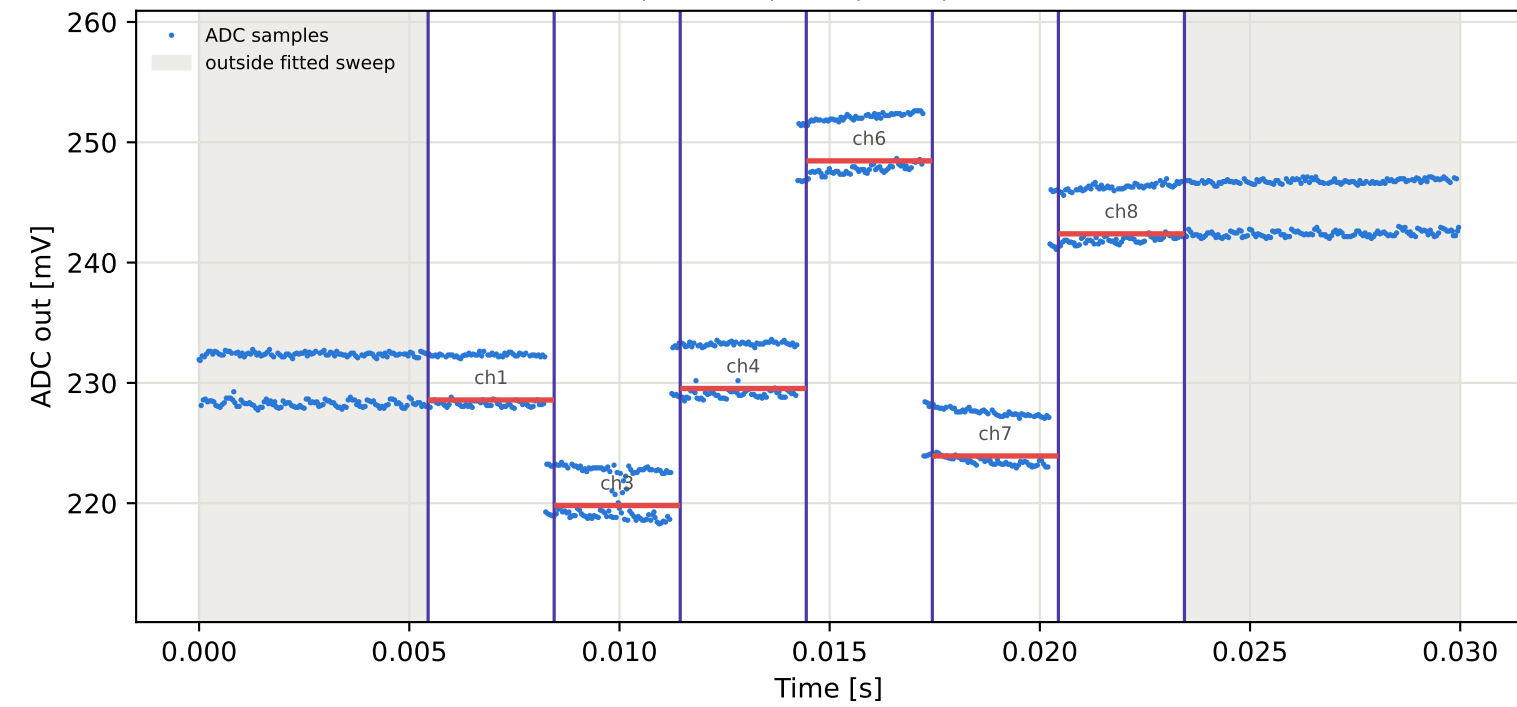
Tag9 &lt;- Tag7 | 845 MHz | run 0 | rep 1 | phase -171.14 deg
