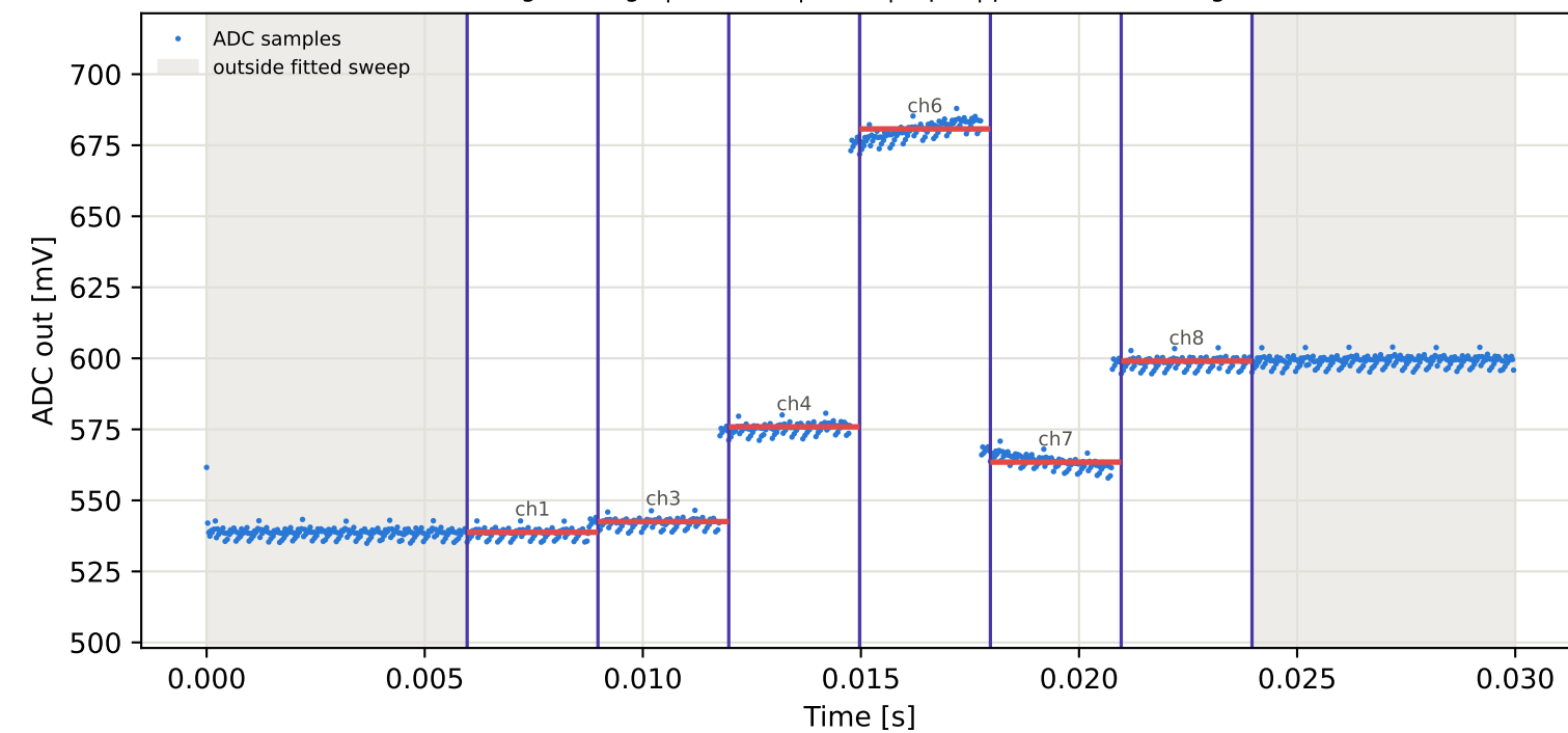
Tag3 &lt;- Tag8 | 915 MHz | run 0 | rep 1 | phase -161.41 deg
