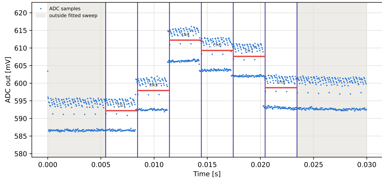
Tag3 &lt;- Tag9 | 845 MHz | run 0 | rep 1 | phase 125.14 deg
