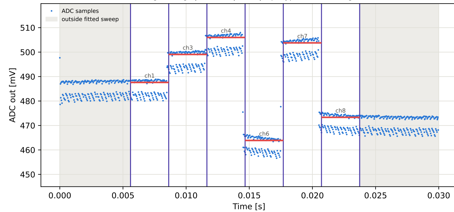
Tag3 &lt;- Tag6 | 955 MHz | run 0 | rep 1 | phase 96.33 deg
