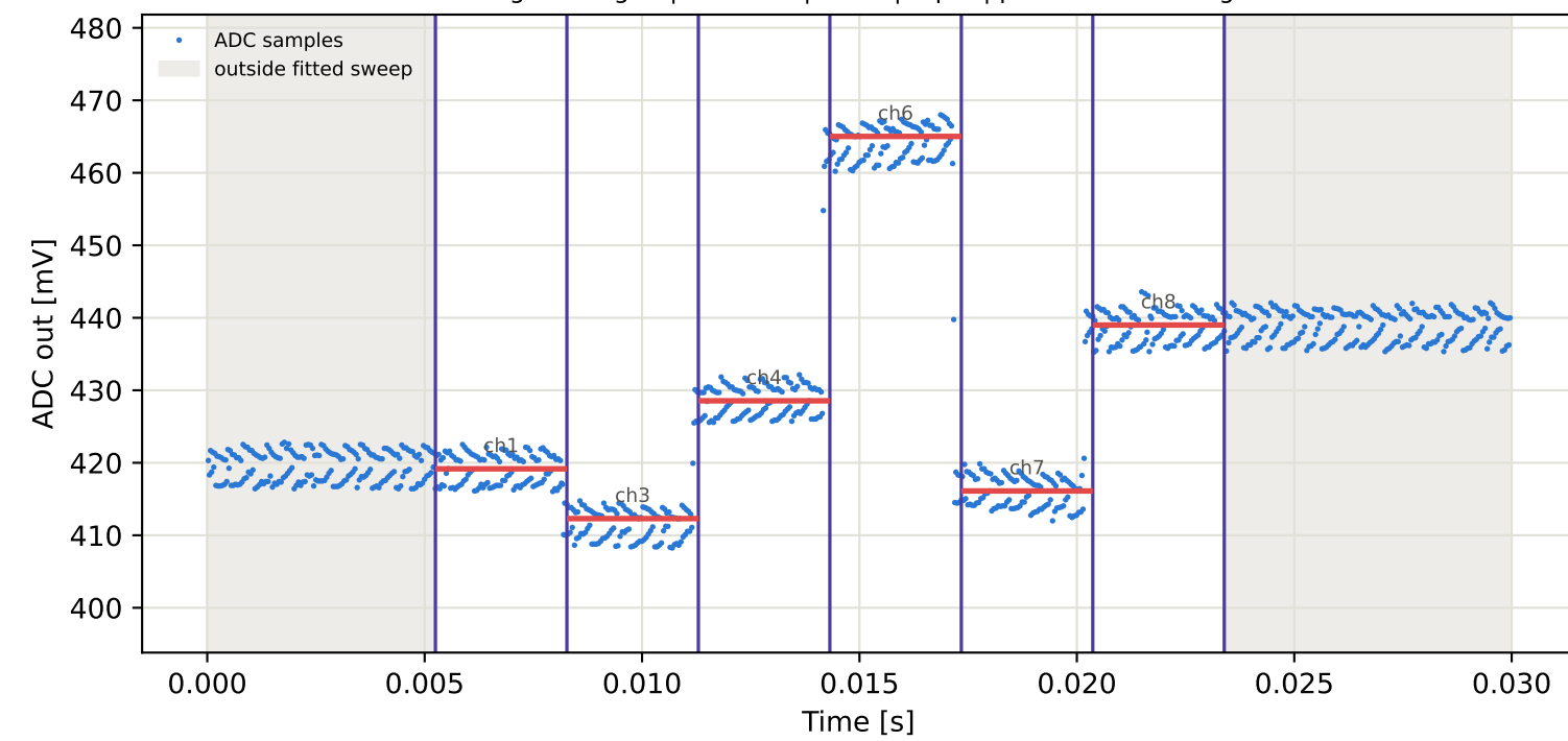
Tag7 &lt;- Tag3 | 965 MHz | run 0 | rep 1 | phase -50.99 deg
