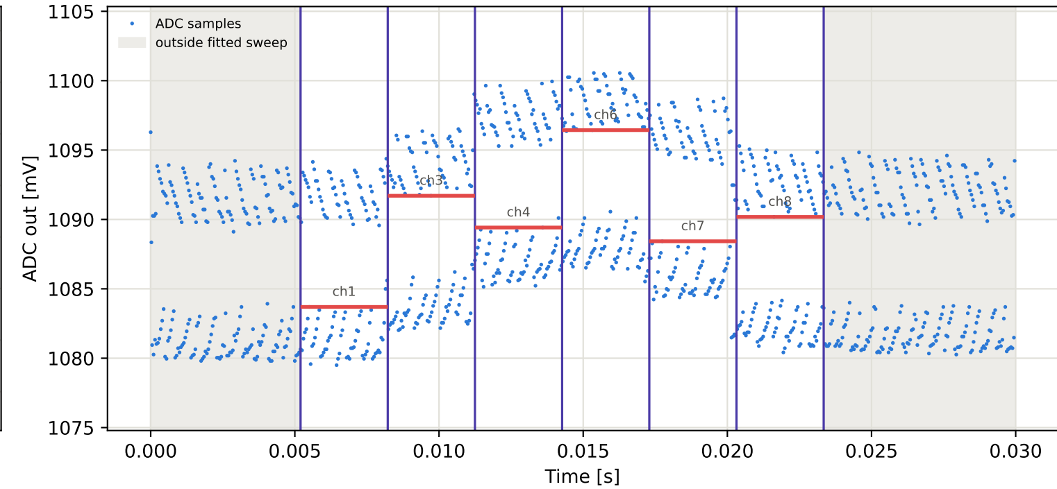
Tag15 &lt;- Tag6 | 905 MHz | run 0 | rep 1 | phase -1.90 deg
