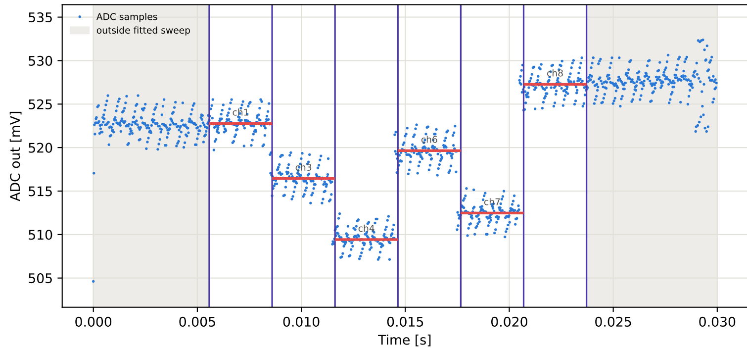
Tag5 &lt;- Tag4 | 935 MHz | run 0 | rep 1 | phase -66.89 deg
