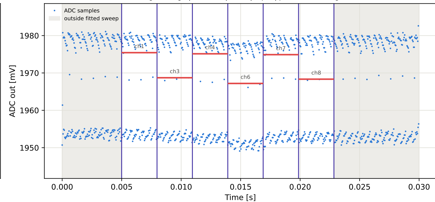
Tag2 &lt;- Tag8 | 915 MHz | run 0 | rep 1 | phase -5.59 deg
