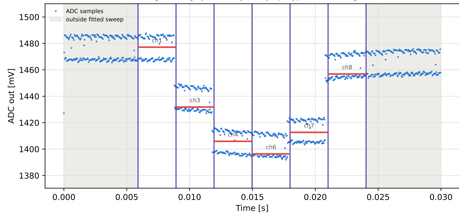
Tag16 &lt;- Tag7 | 885 MHz | run 0 | rep 1 | phase 97.41 deg
