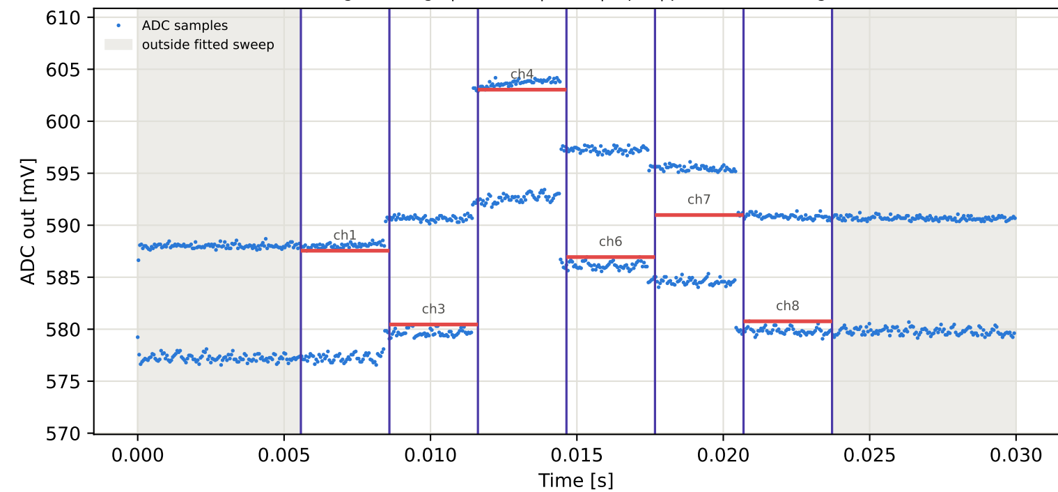
Tag16 &lt;- Tag1 | 995 MHz | run 0 | rep 1 | phase 96.36 deg
