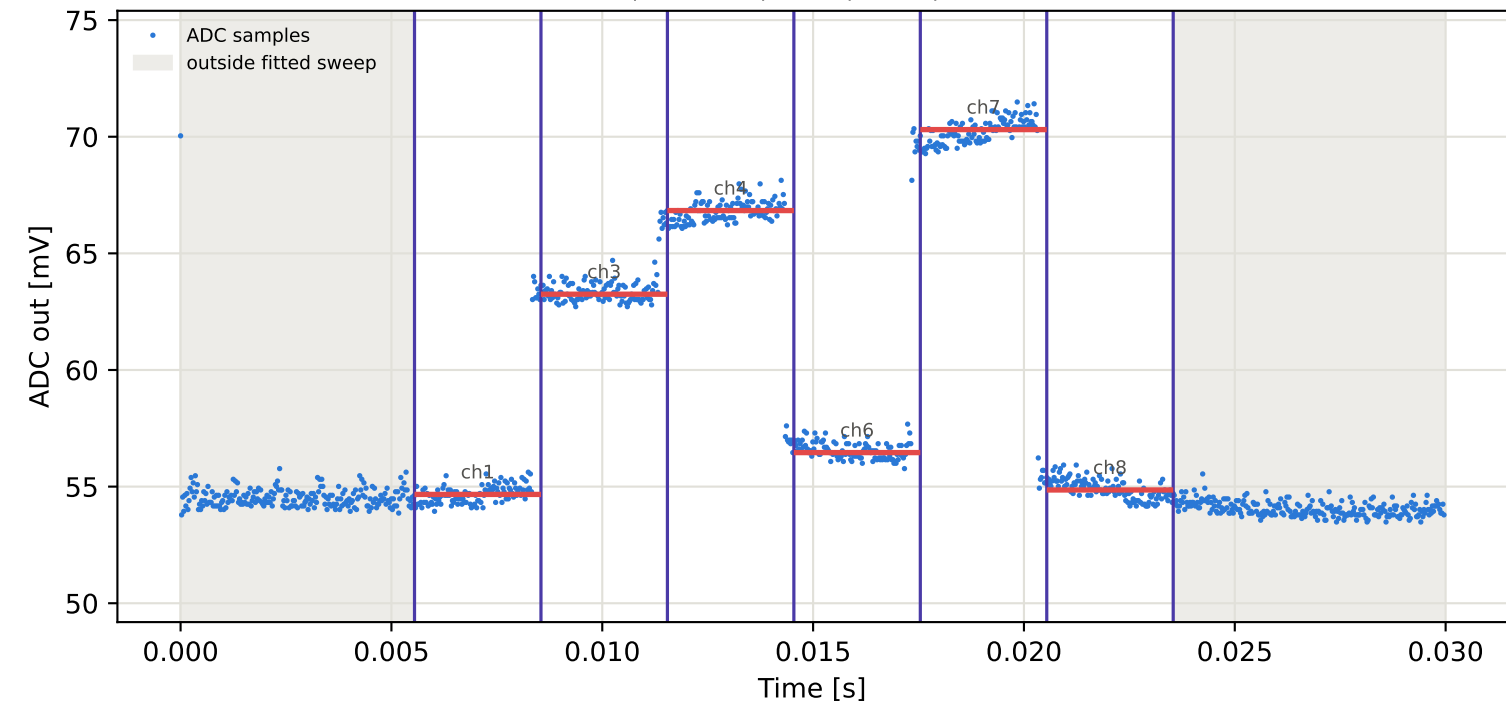
Tag3 &lt;- Tag9 | 775 MHz | run 0 | rep 1 | phase -48.97 deg
