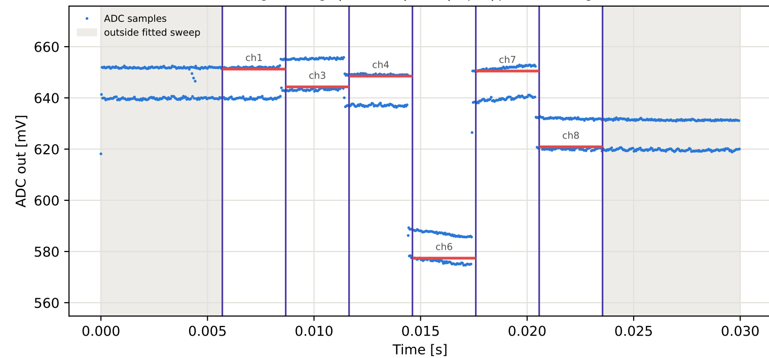
Tag16 &lt;- Tag4 | 955 MHz | run 0 | rep 1 | phase -153.03 deg
