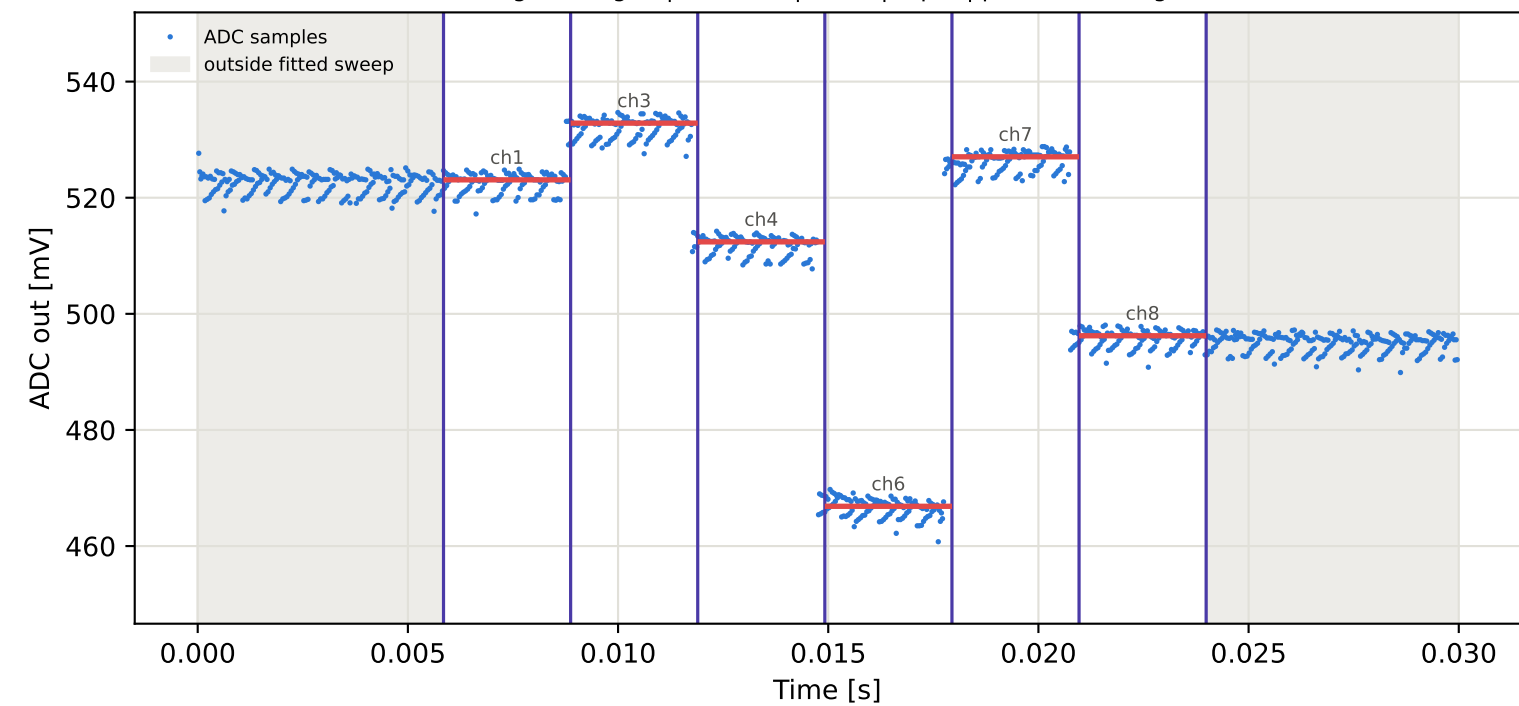
Tag9 &lt;- Tag2 | 985 MHz | run 0 | rep 1 | phase -0.39 deg
