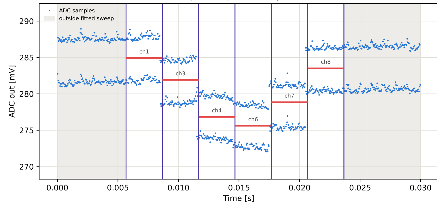
Tag6 &lt;- Tag2 | 925 MHz | run 0 | rep 1 | phase -117.37 deg
