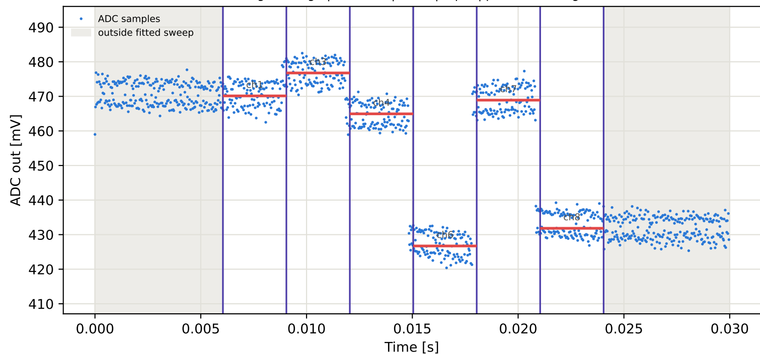
Tag1 &lt;- Tag4 | 885 MHz | run 0 | rep 1 | phase 5.40 deg
