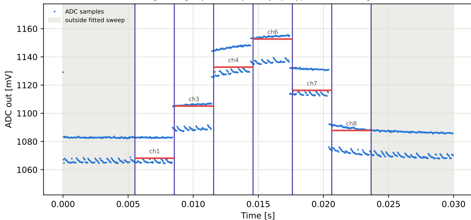
Tag8 &lt;- Tag16 | 915 MHz | run 0 | rep 1 | phase 47.58 deg
