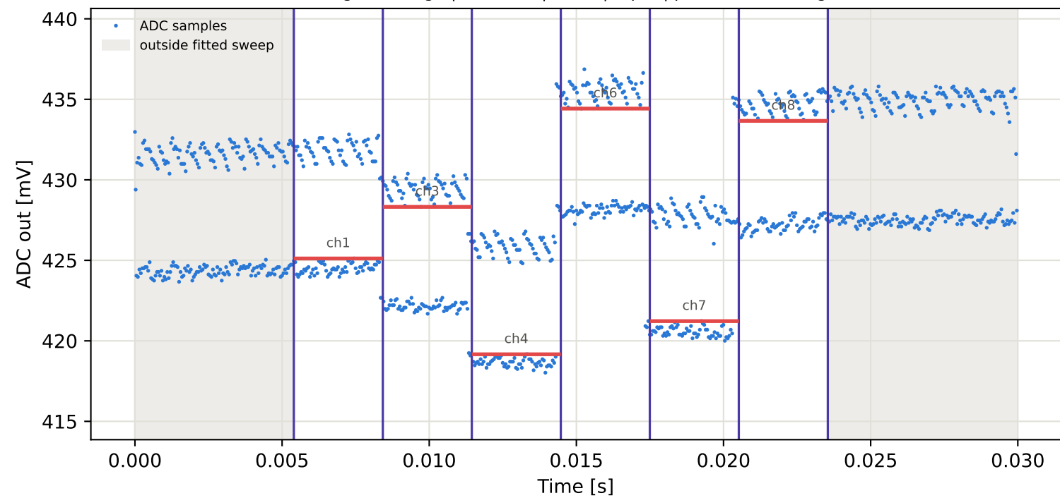
Tag16 &lt;- Tag4 | 995 MHz | run 0 | rep 1 | phase -55.09 deg
