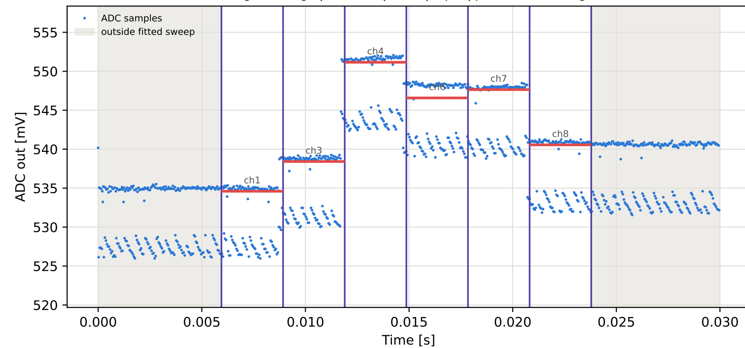
Tag16 &lt;- Tag10 | 825 MHz | run 0 | rep 1 | phase -60.25 deg
