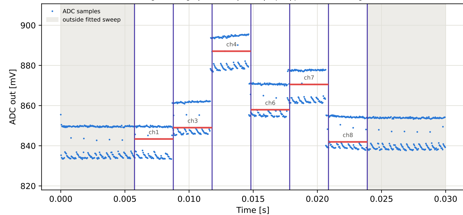
Tag16 &lt;- Tag10 | 985 MHz | run 0 | rep 1 | phase -37.27 deg
