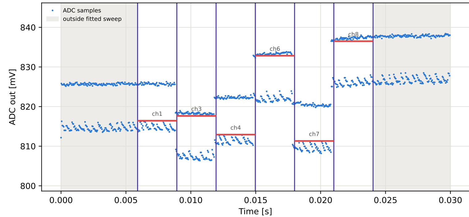
Tag2 &lt;- Tag8 | 865 MHz | run 0 | rep 1 | phase 132.38 deg
