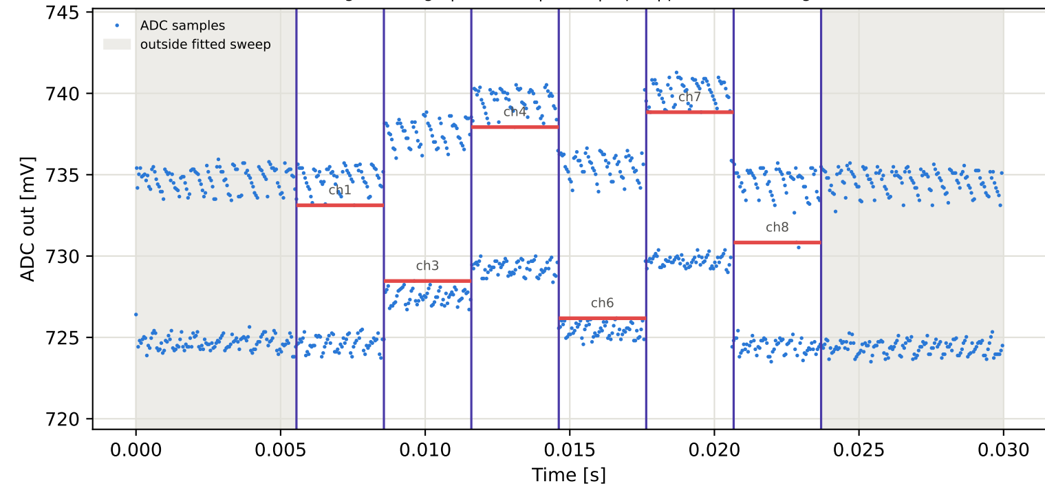
Tag16 &lt;- Tag15 | 825 MHz | run 0 | rep 1 | phase 20.28 deg
