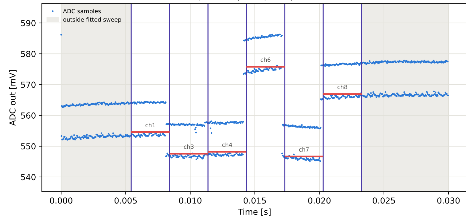
Tag9 &lt;- Tag10 | 945 MHz | run 0 | rep 1 | phase 104.97 deg
