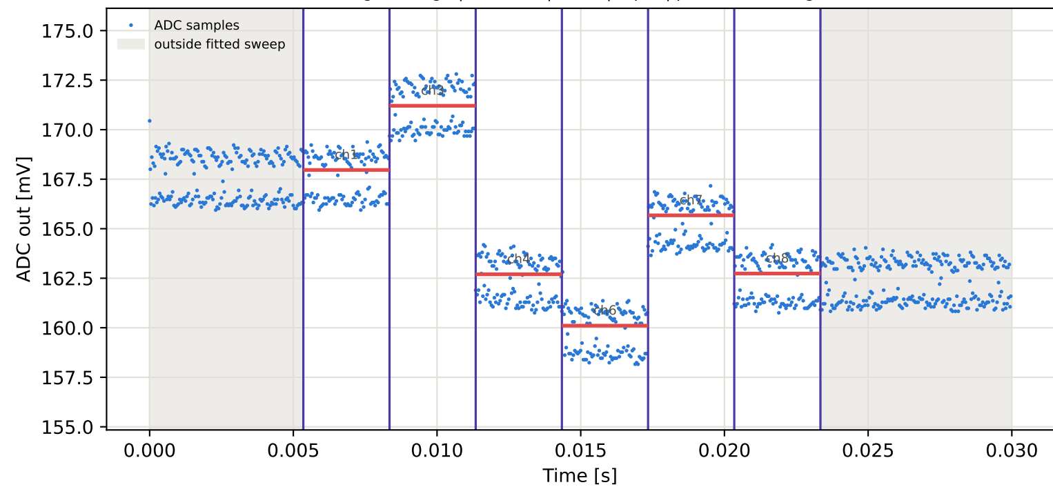
Tag4 &lt;- Tag8 | 825 MHz | run 0 | rep 1 | phase -141.76 deg
