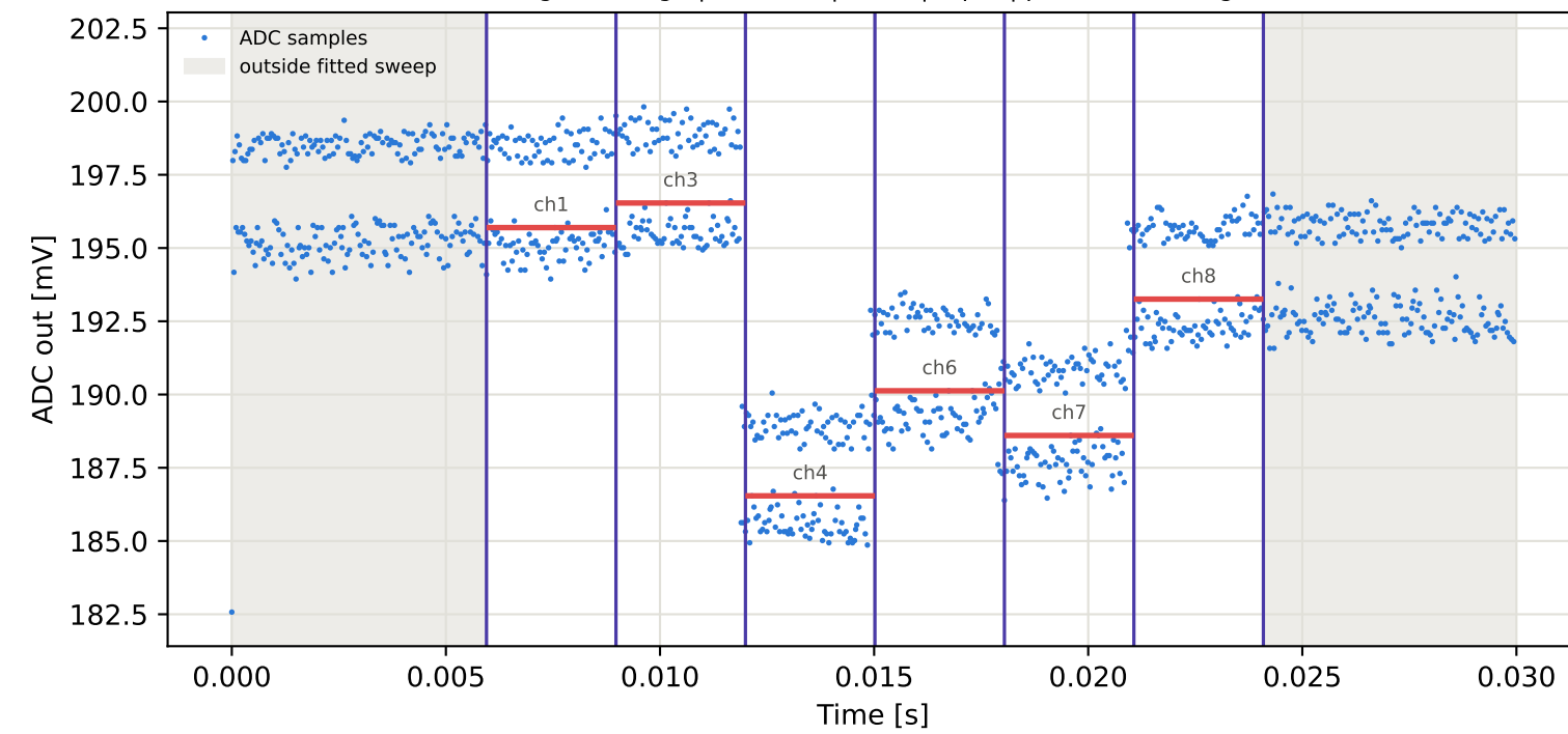
Tag2 &lt;- Tag1 | 795 MHz | run 0 | rep 1 | phase 4.94 deg
