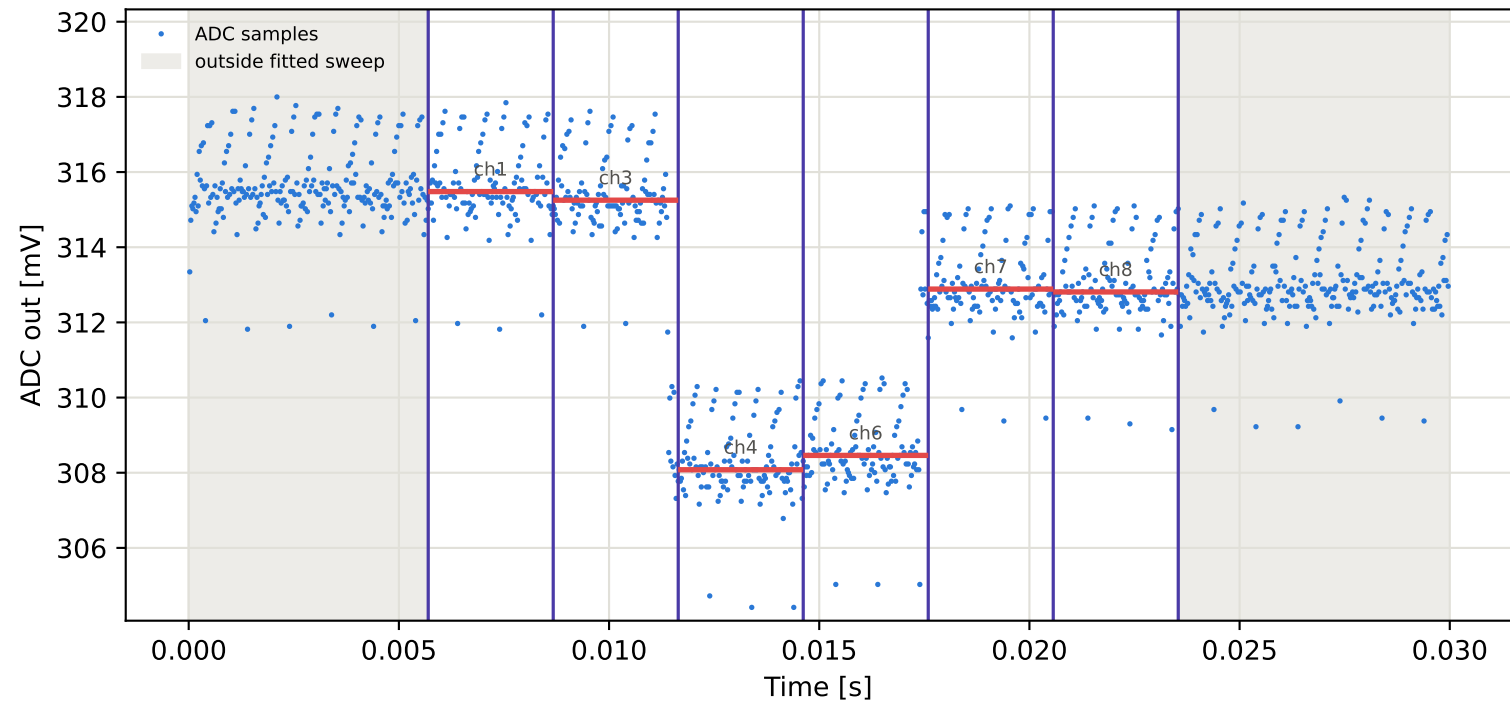
Tag5 &lt;- Tag1 | 995 MHz | run 0 | rep 1 | phase 175.42 deg
