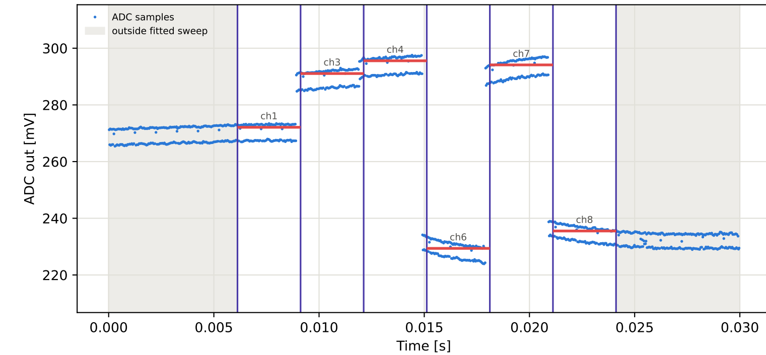
Tag9 &lt;- Tag16 | 905 MHz | run 0 | rep 1 | phase -72.45 deg
