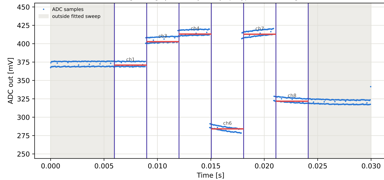
Tag9 &lt;- Tag5 | 955 MHz | run 0 | rep 1 | phase -10.61 deg
