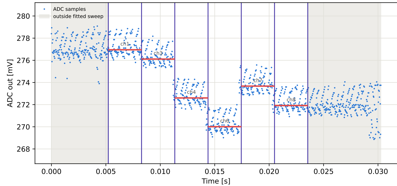
Tag4 &lt;- Tag16 | 855 MHz | run 0 | rep 1 | phase -94.35 deg
