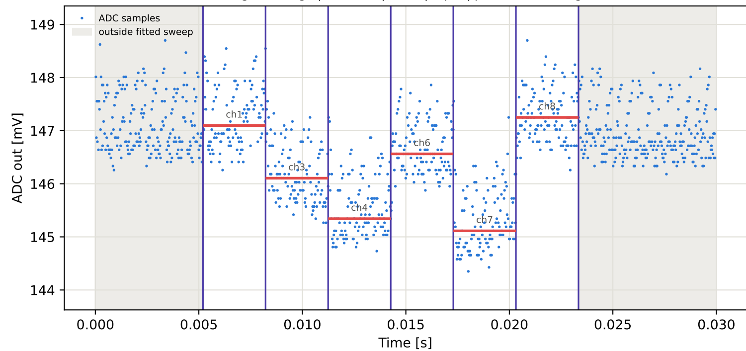
Tag2 &lt;- Tag10 | 775 MHz | run 0 | rep 1 | phase -5.04 deg
