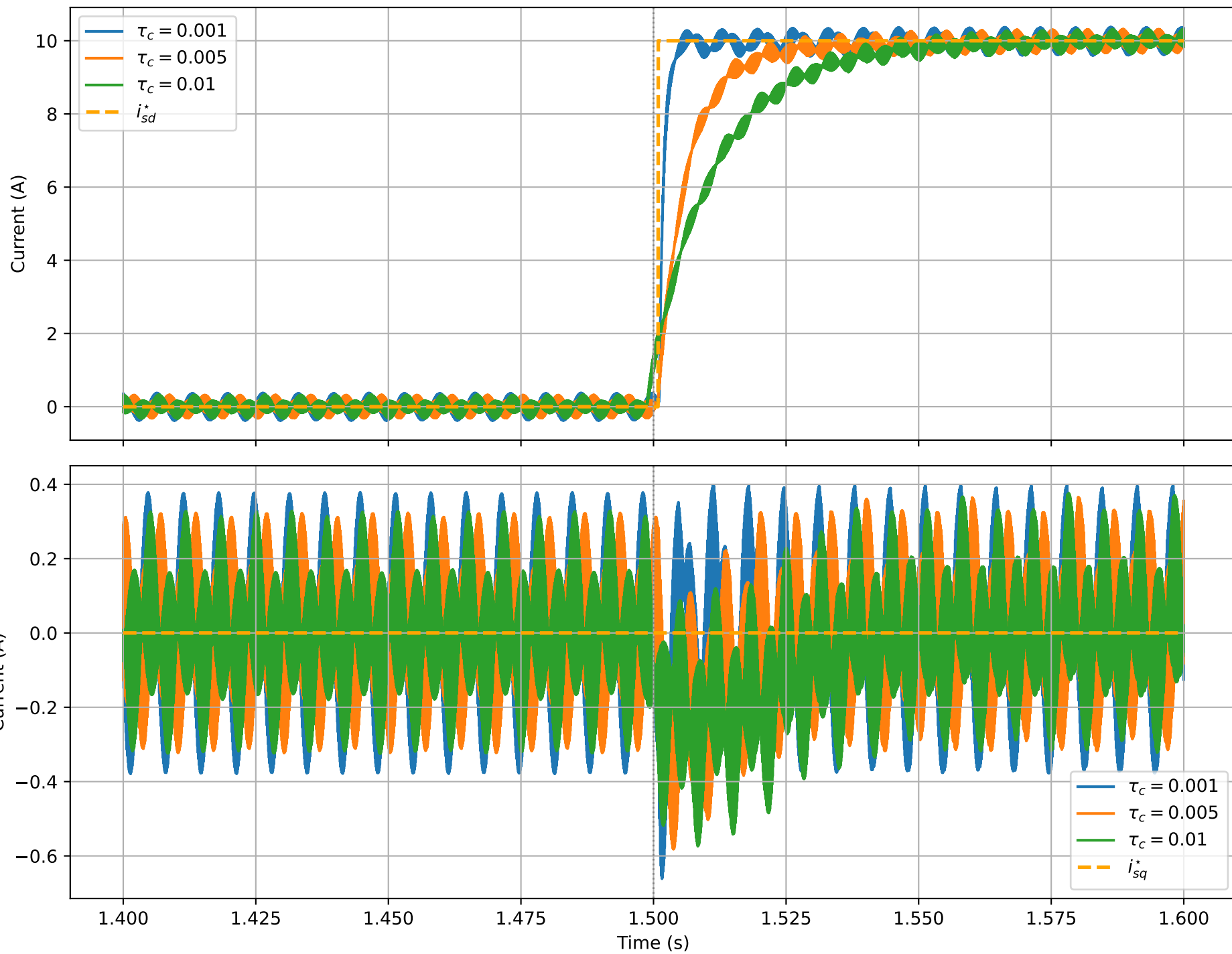
Parametric sweep — \tau_c — zoom at t = 1.5 s
